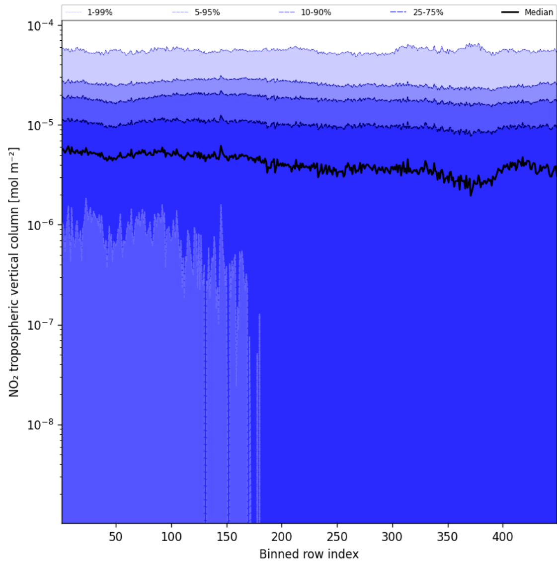
Figure 44: Along track statistics of “NO 2 tropospheric vertical column” for 2025-04-08 to 2025-04-09
