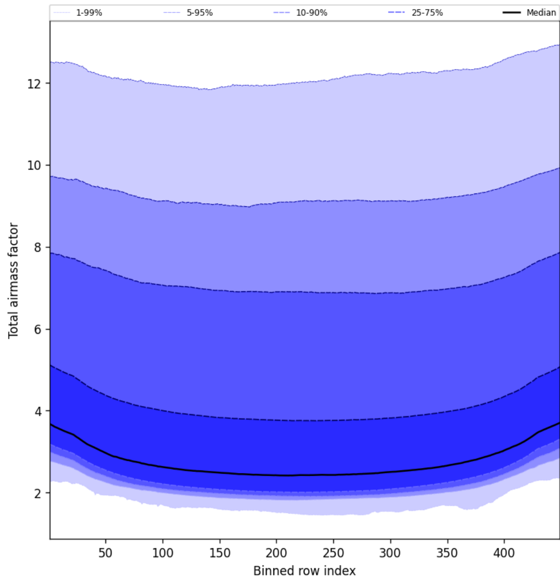
Figure 47: Along track statistics of “Total airmass factor” for 2025-04-08 to 2025-04-09
