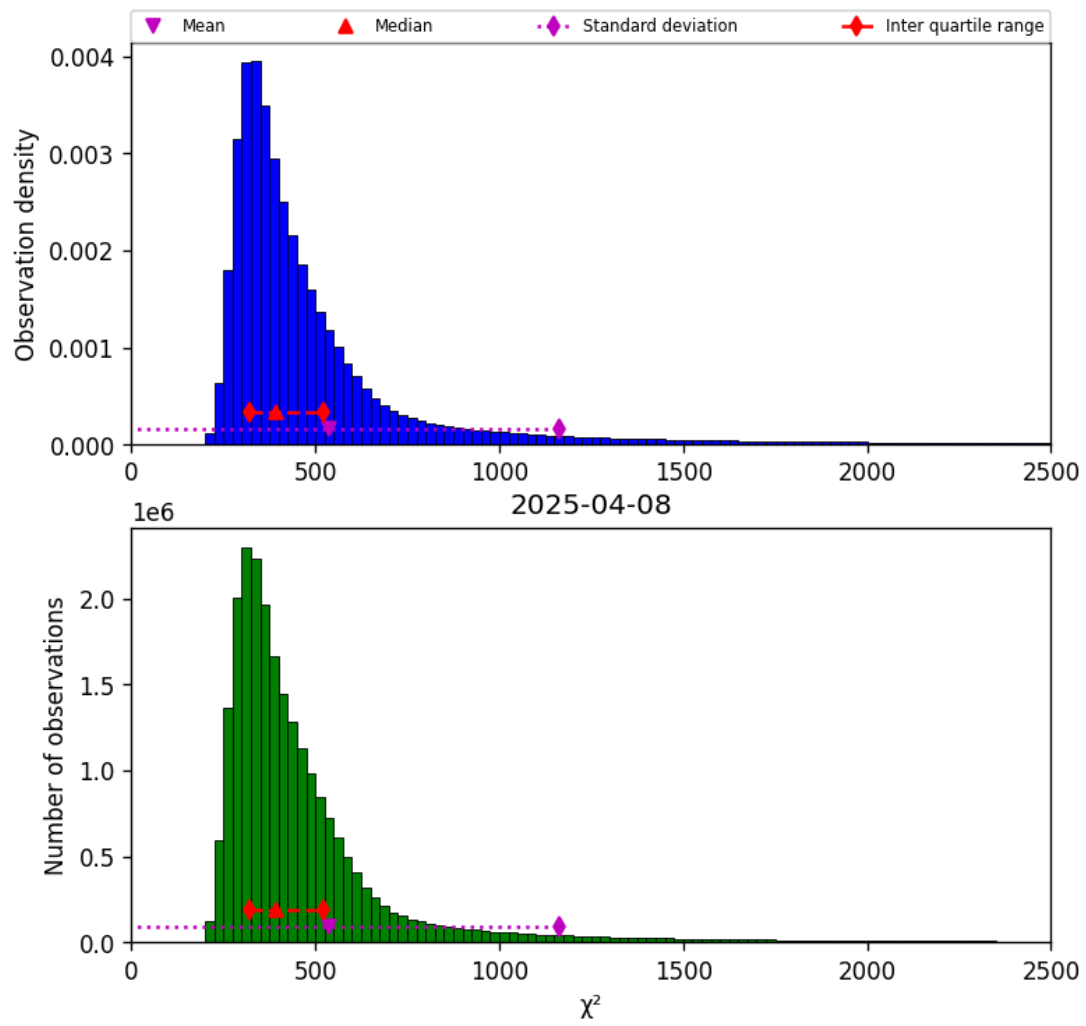
Figure 40: Histogram of “ \chi^2 ” for 2025-04-08 to 2025-04-09
