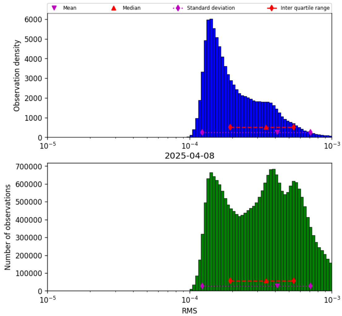
Figure 41: Histogram of “RMS” for 2025-04-08 to 2025-04-09
