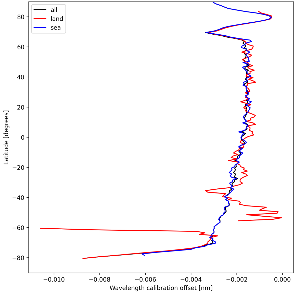
Figure 16: Zonal average of “Wavelength calibration offset” for 2025-04-08 to 2025-04-09.
