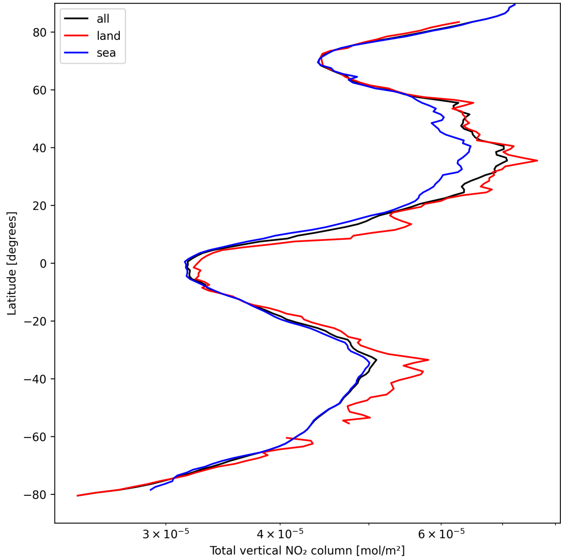
Figure 19: Zonal average of “Total vertical NO 2 column” for 2025-04-08 to 2025-04-09.
