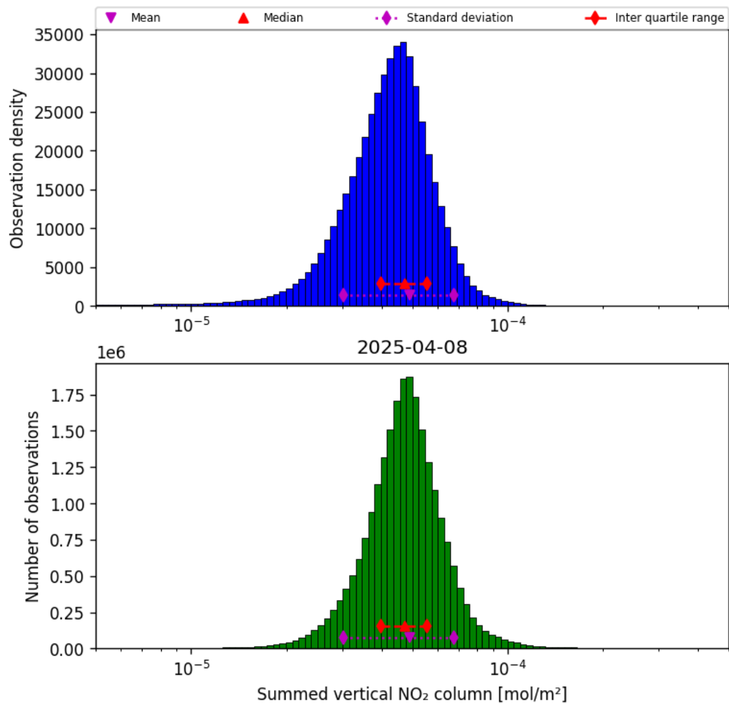
Figure 38: Histogram of "Summed vertical NO 2 column" for 2025-04-08 to 2025-04-09
