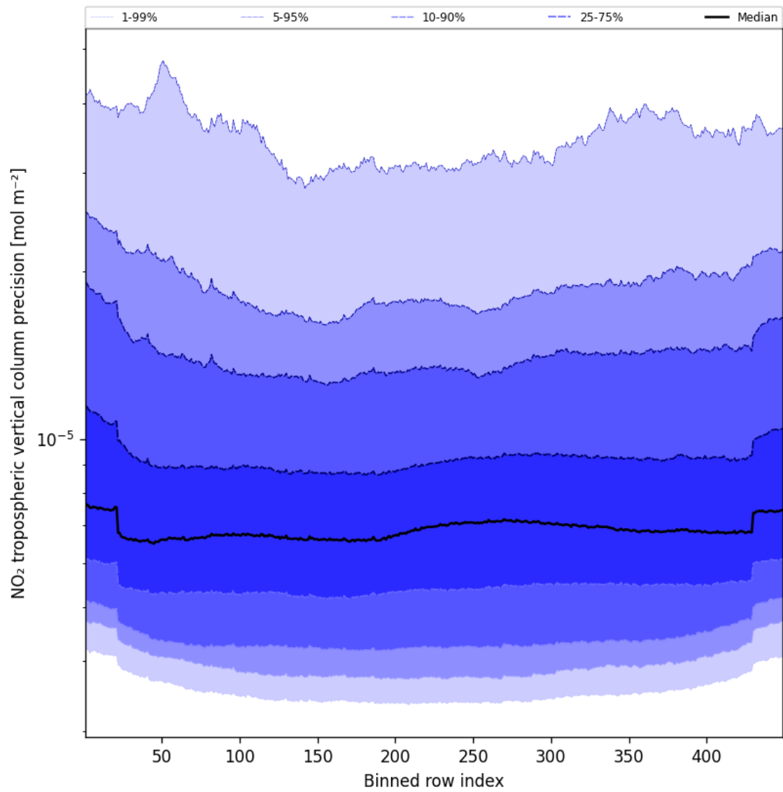
Figure 45: Along track statistics of “NO 2 tropospheric vertical column precision” for 2025-04-08 to 2025-04-09
