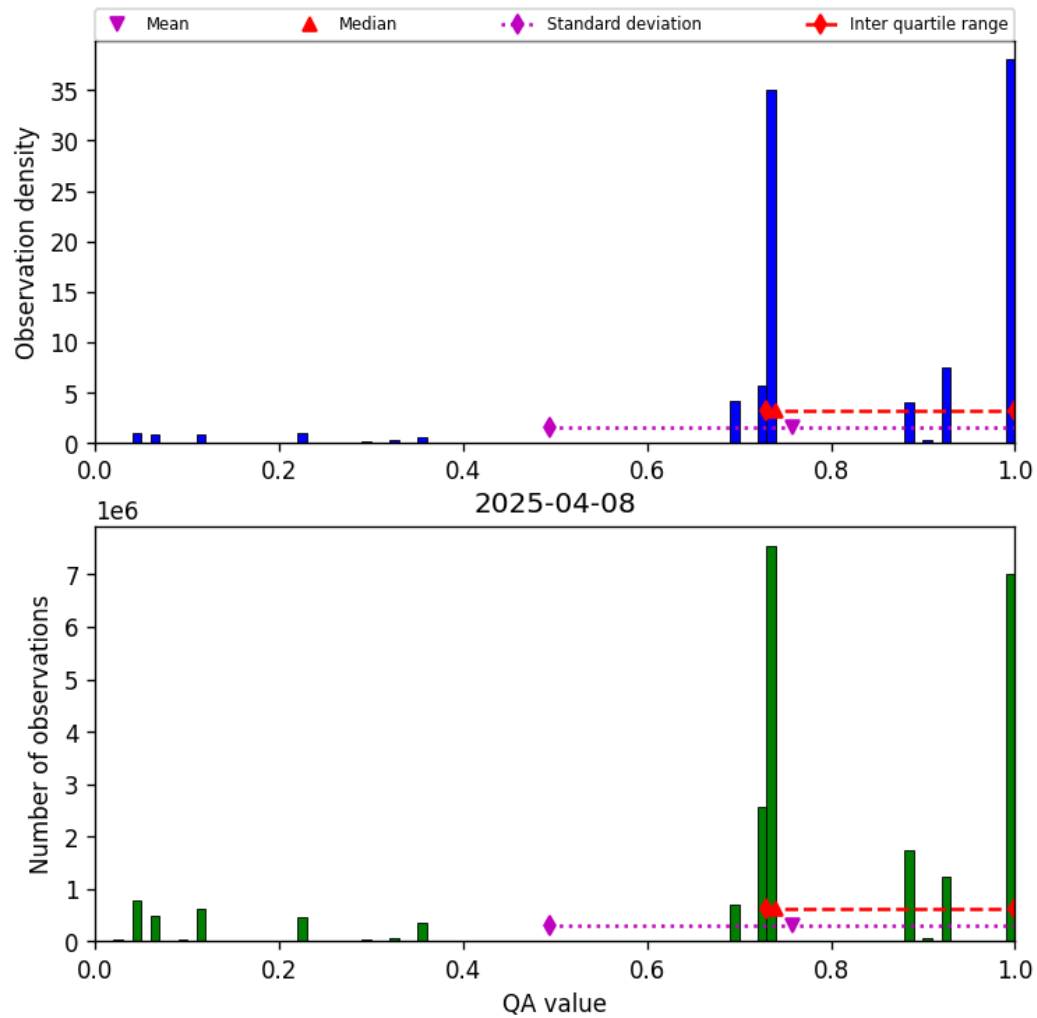
Figure 26: Histogram of “QA value” for 2025-04-08 to 2025-04-09
