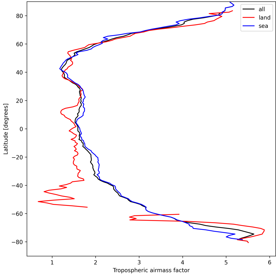
Figure 12: Zonal average of “Tropospheric air mass factor” for 2025-04-08 to 2025-04-09.
