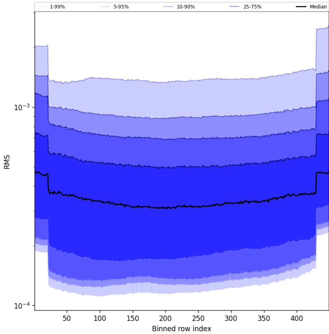
Figure 58: Along track statistics of “RMS” for 2025-04-08 to 2025-04-09
