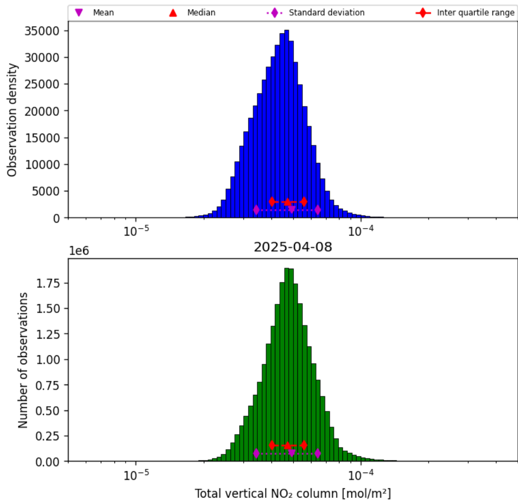
Figure 36: Histogram of "Total vertical NO 2 column" for 2025-04-08 to 2025-04-09
