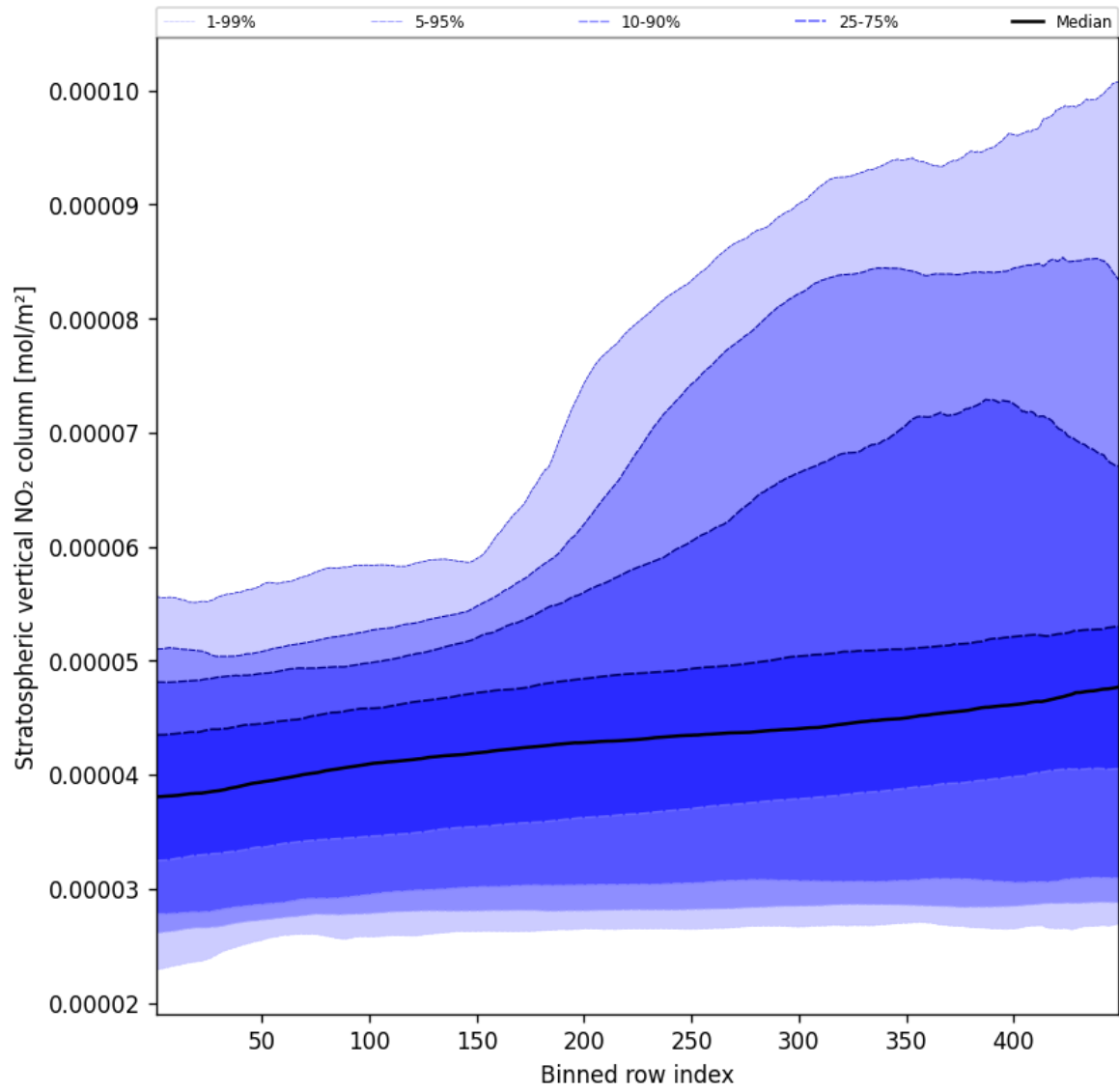
Figure 51: Along track statistics of “Stratospheric vertical NO 2 column” for 2025-04-08 to 2025-04-09
