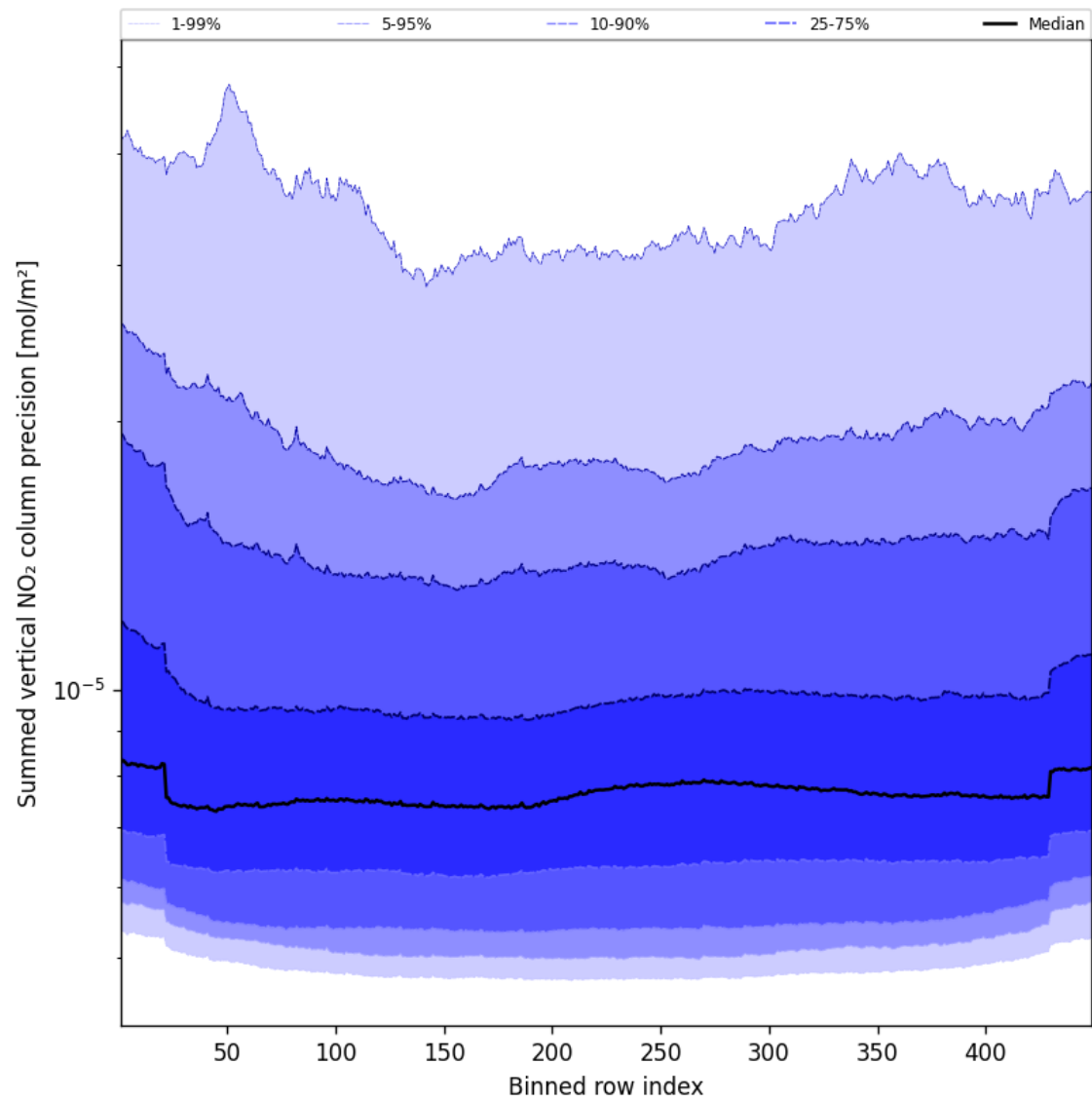
Figure 56: Along track statistics of “Summed vertical NO 2 column precision” for 2025-04-08 to 2025-04-09
