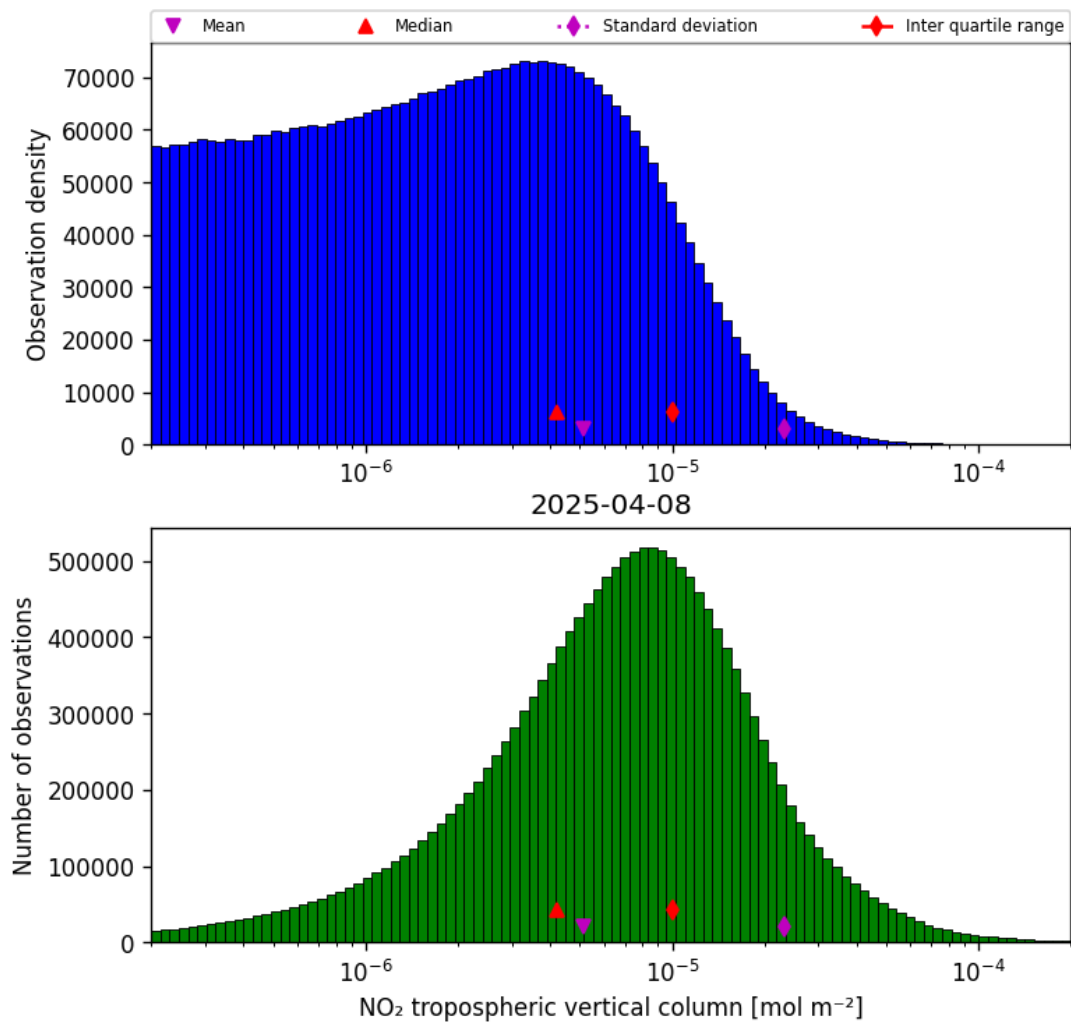
Figure 27: Histogram of “NO 2 tropospheric vertical column” for 2025-04-08 to 2025-04-09
