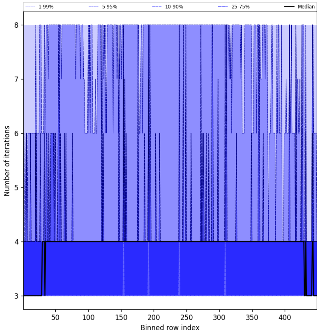
Figure 49: Along track statistics of “Number of iterations” for 2025-04-08 to 2025-04-09
