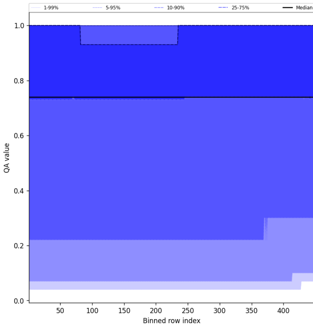
Figure 43: Along track statistics of “QA value” for 2025-04-08 to 2025-04-09
