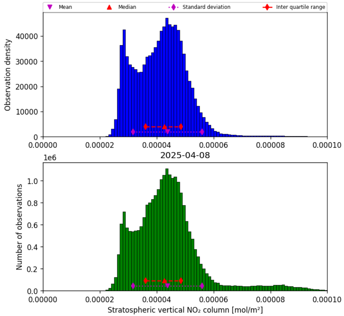
Figure 34: Histogram of “Stratospheric vertical NO 2 column” for 2025-04-08 to 2025-04-09
