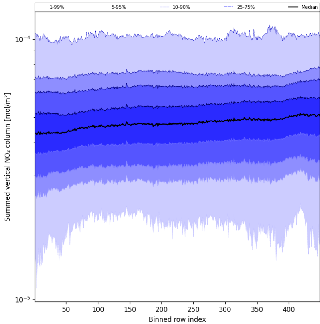
Figure 55: Along track statistics of “Summed vertical NO 2 column” for 2025-04-08 to 2025-04-09
