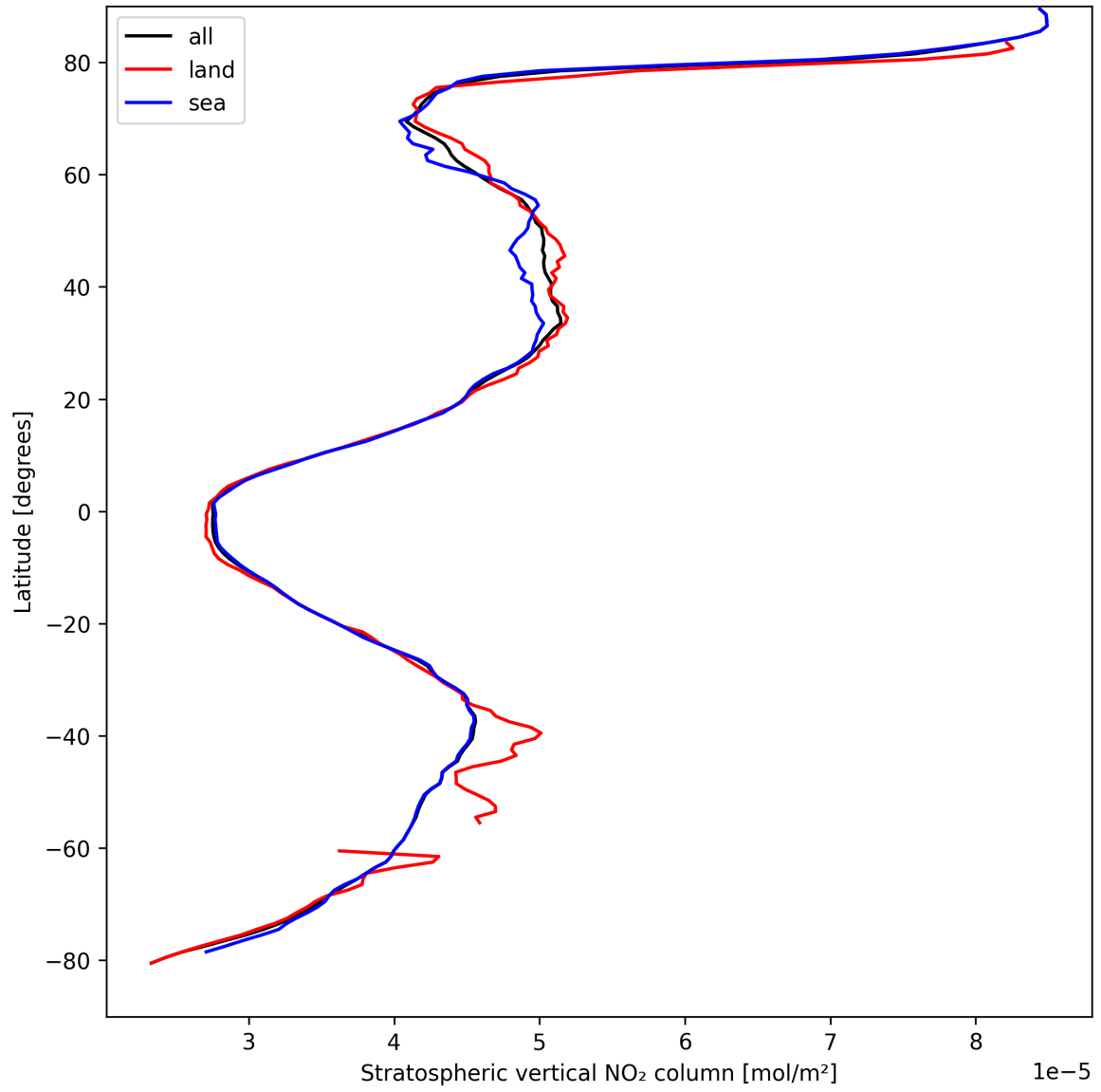
Figure 17: Zonal average of “Stratospheric vertical NO 2 column” for 2025-04-08 to 2025-04-09.
