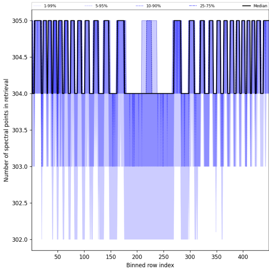
Figure 48: Along track statistics of “Number of spectral points in retrieval” for 2025-04-08 to 2025-04-09
