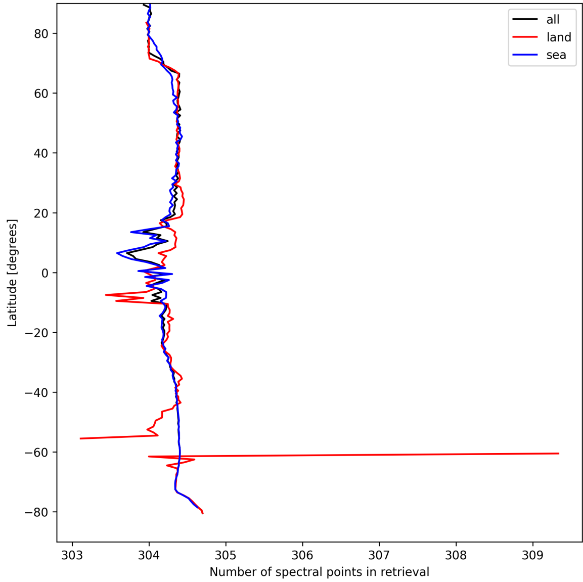
Figure 14: Zonal average of “Number of spectral points in retrieval” for 2025-04-08 to 2025-04-09.
