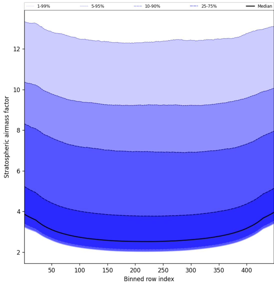
Figure 59: Along track statistics of “Stratospheric airmass factor” for 2025-04-08 to 2025-04-09
