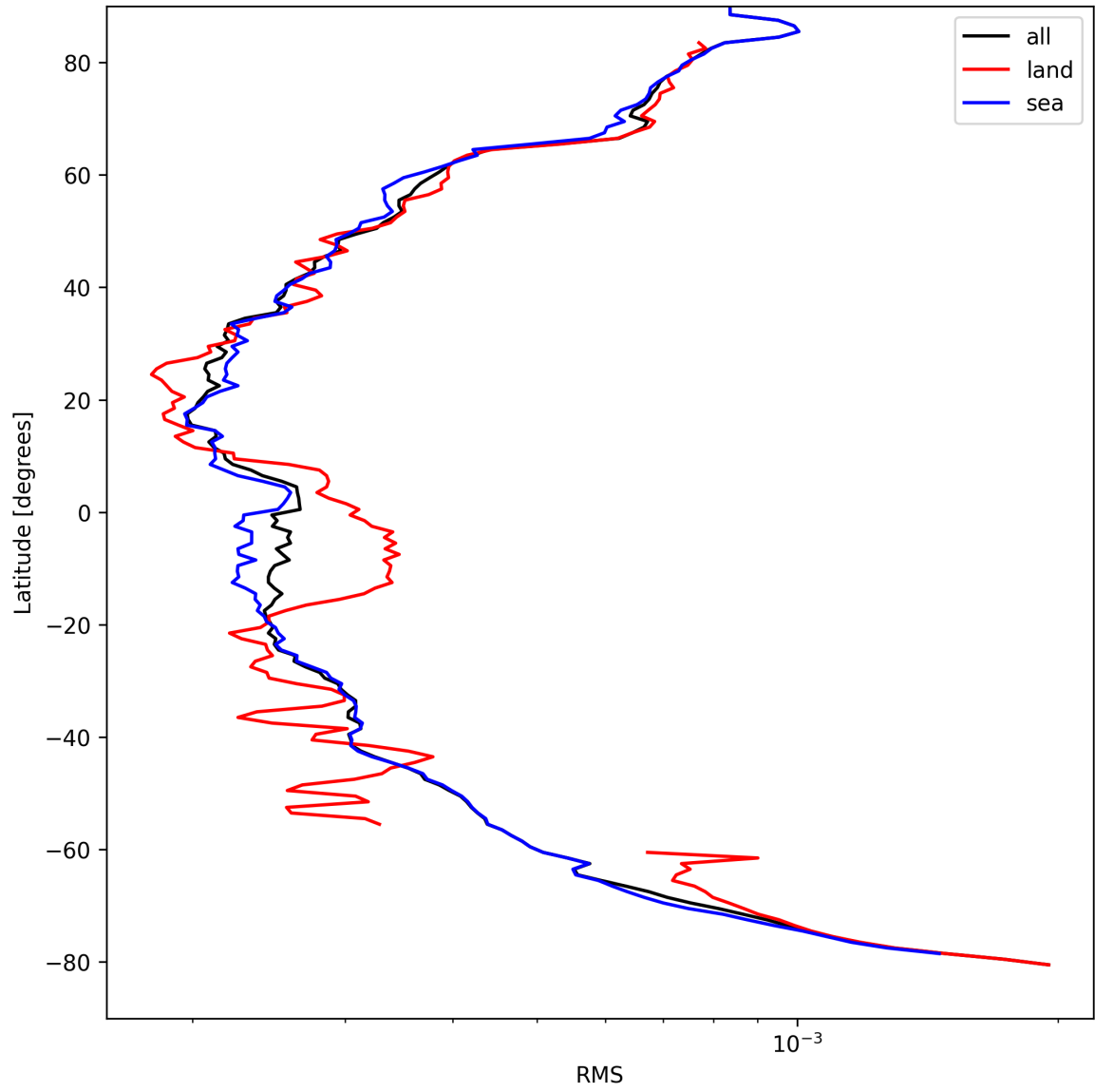
Figure 24: Zonal average of “RMS” for 2025-04-08 to 2025-04-09.
