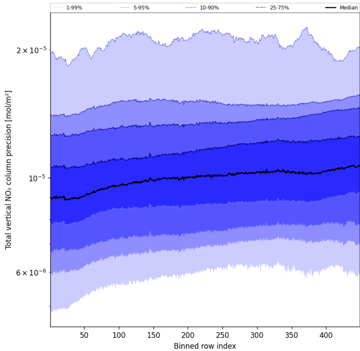
Figure 54: Along track statistics of “Total vertical NO 2 column precision” for 2025-04-08 to 2025-04-09
