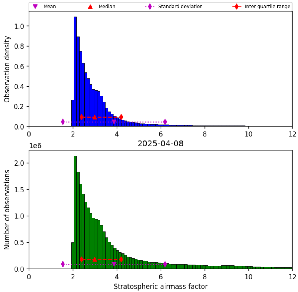
Figure 42: Histogram of “Stratospheric airmass factor” for 2025-04-08 to 2025-04-09
