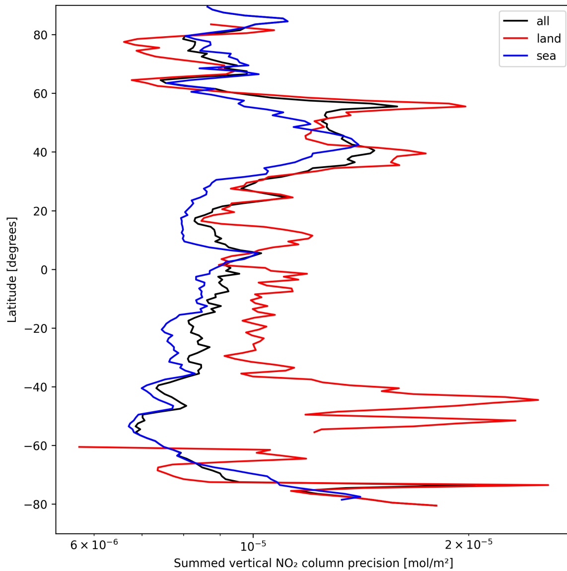
Figure 22: Zonal average of “Summed vertical NO 2 column precision” for 2025-04-08 to 2025-04-09.
