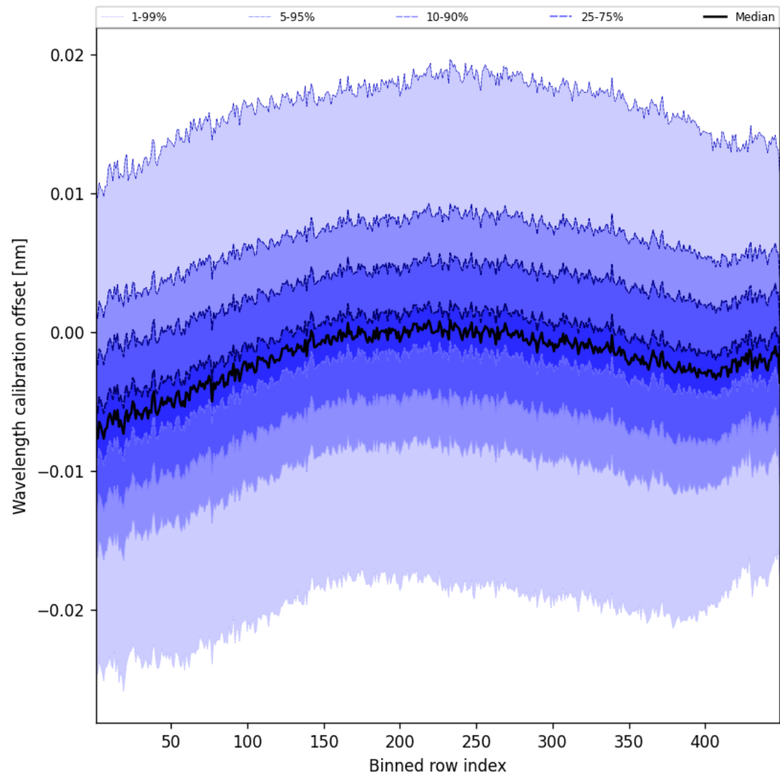
Figure 50: Along track statistics of “Wavelength calibration offset” for 2025-04-08 to 2025-04-09
