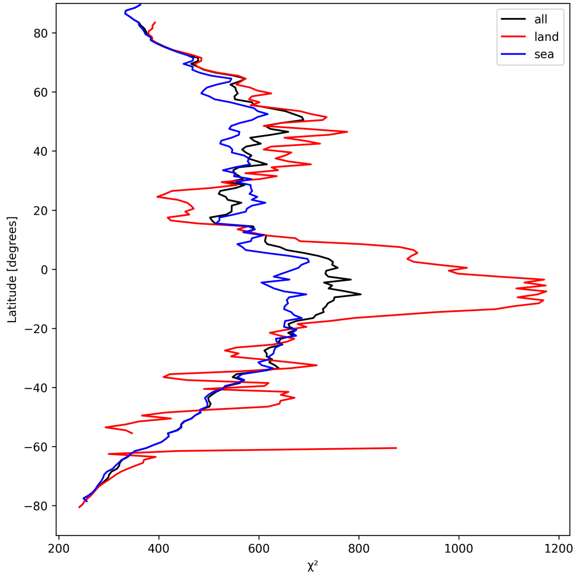
Figure 23: Zonal average of “ \chi^2 ” for 2025-04-08 to 2025-04-09.
