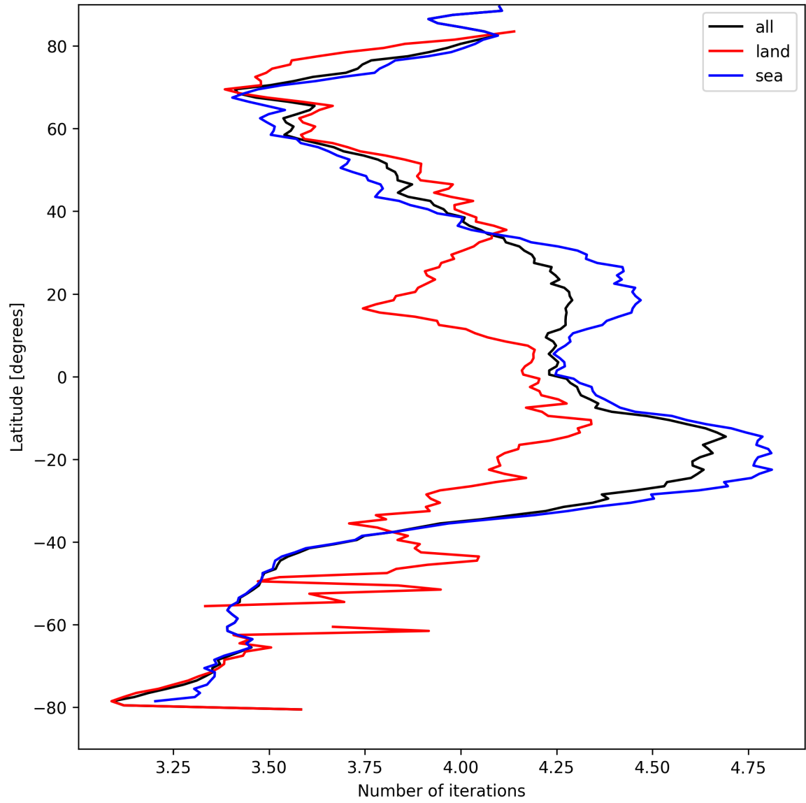
Figure 15: Zonal average of “Number of iterations” for 2025-04-08 to 2025-04-09.
