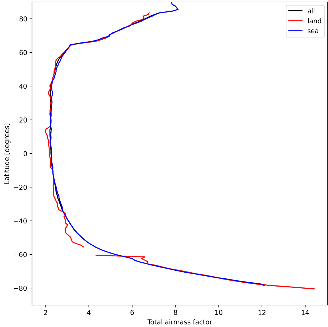
Figure 13: Zonal average of “Total airmass factor” for 2025-04-08 to 2025-04-09.
