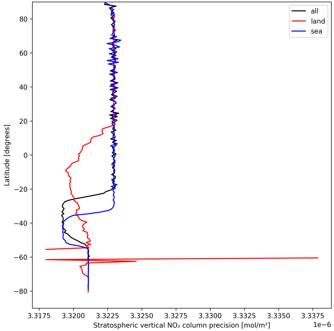
Figure 18: Zonal average of “Stratospheric vertical NO 2 column precision” for 2025-04-08 to 2025-04-09.
