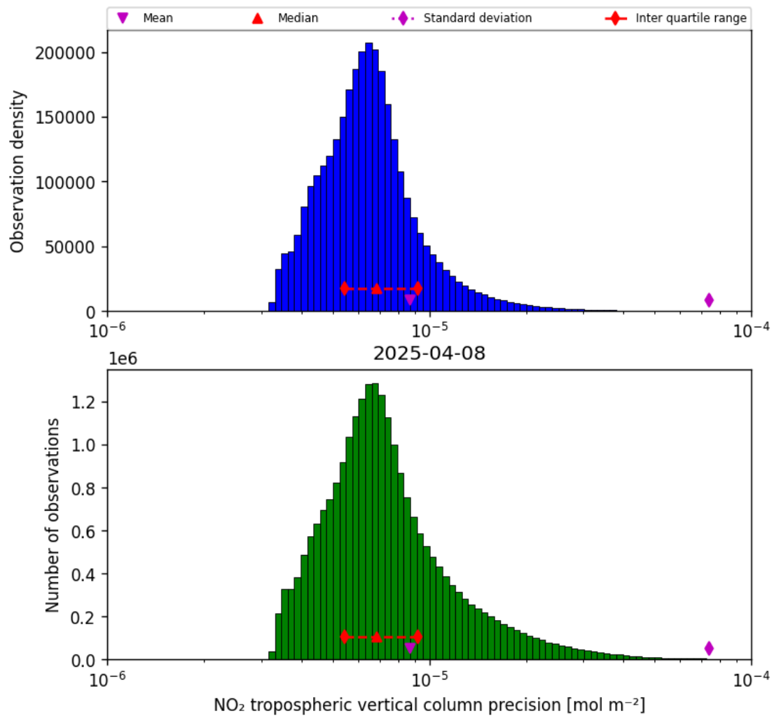
Figure 28: Histogram of “NO 2 tropospheric vertical column precision” for 2025-04-08 to 2025-04-09
