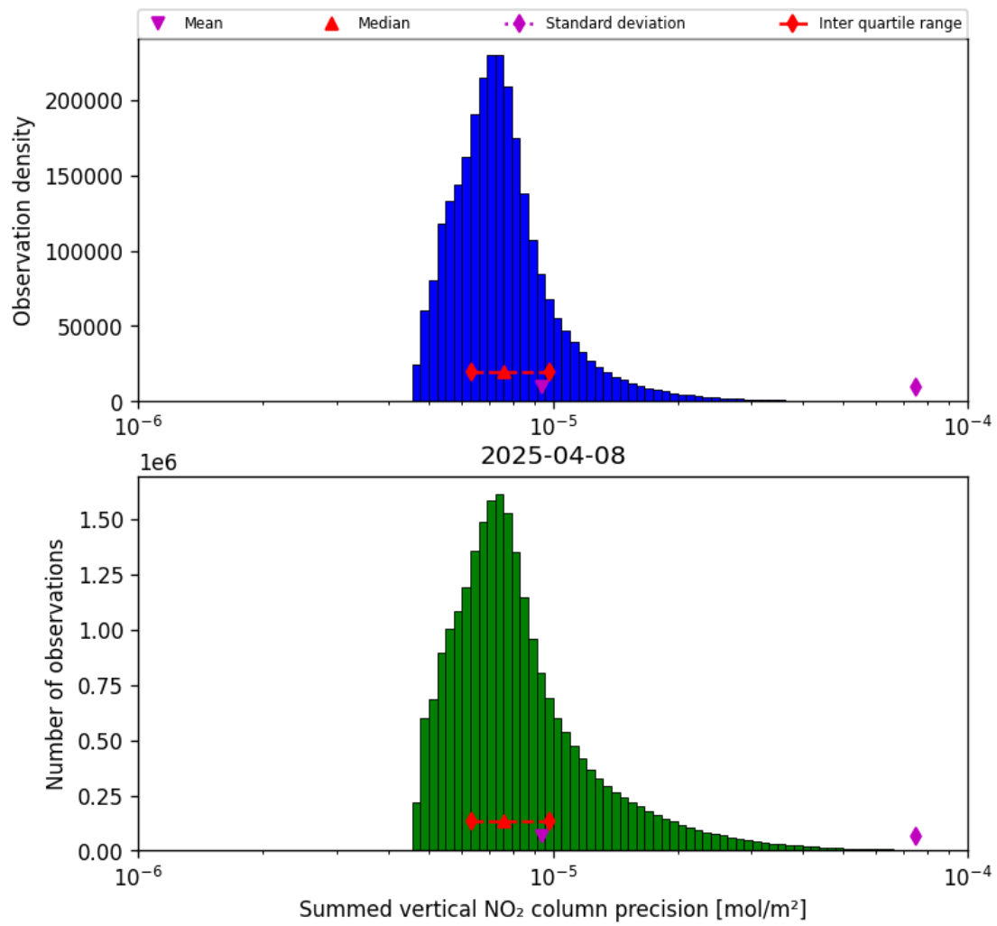
Figure 39: Histogram of “Summed vertical NO 2 column precision” for 2025-04-08 to 2025-04-09
