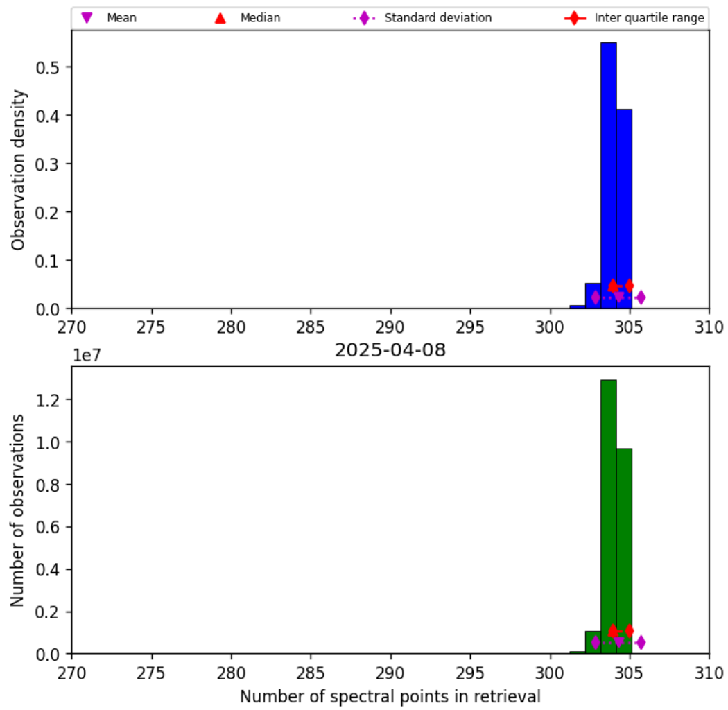
Figure 31: Histogram of “Number of spectral points in retrieval” for 2025-04-08 to 2025-04-09
