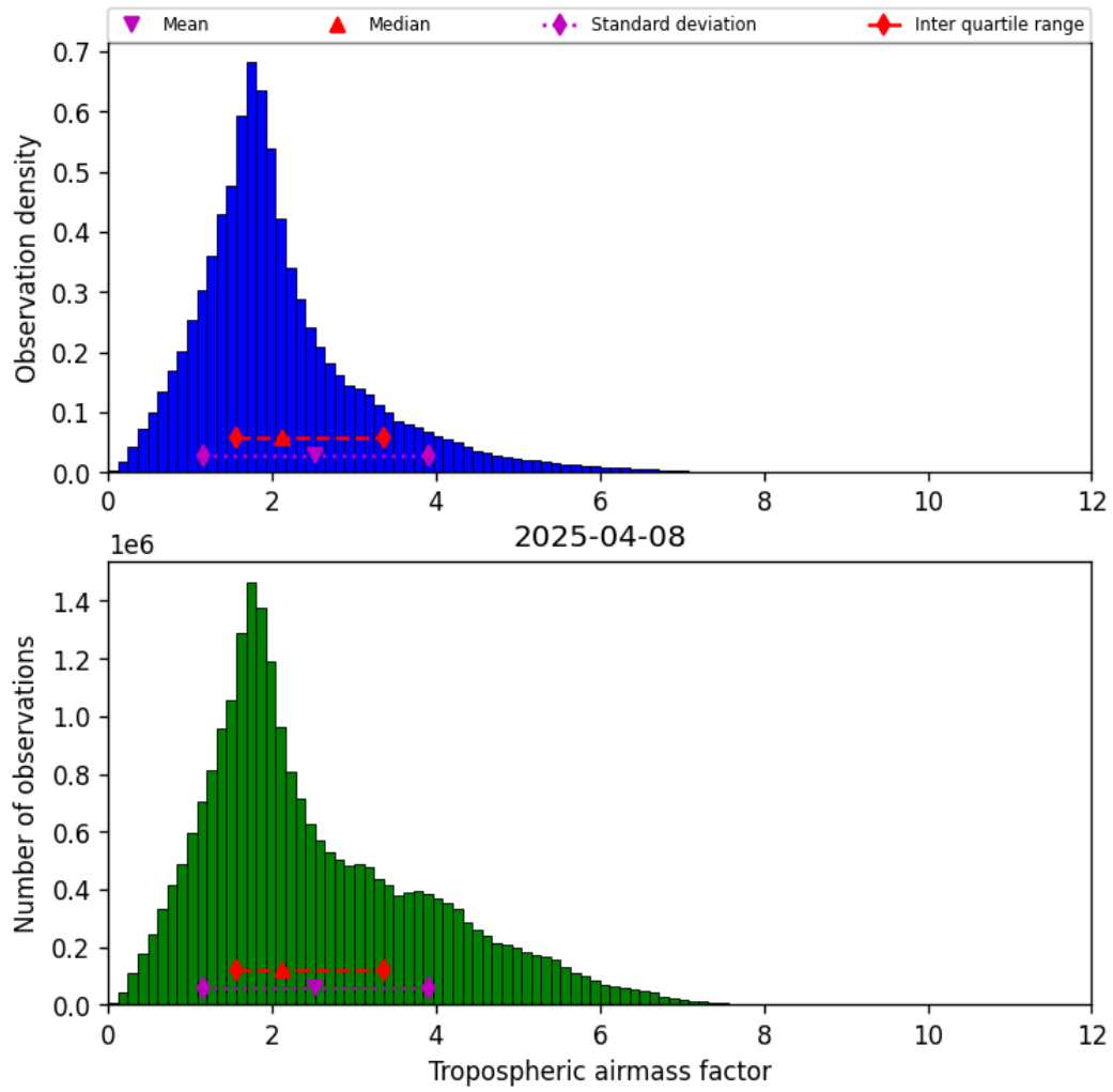
Figure 29: Histogram of “Tropospheric airmass factor” for 2025-04-08 to 2025-04-09
