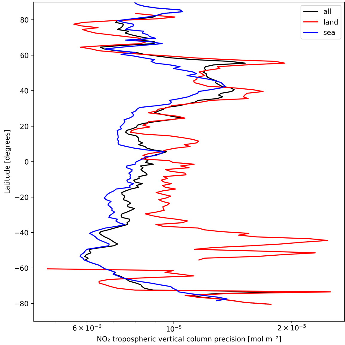
Figure 11: Zonal average of “NO 2 tropospheric vertical column precision” for 2025-04-08 to 2025-04-09.
