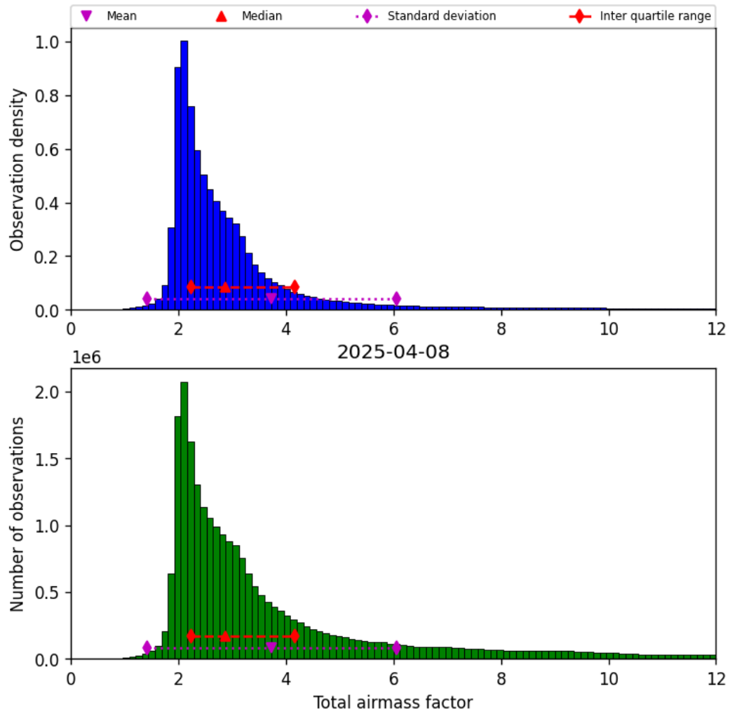
Figure 30: Histogram of “Total airmass factor” for 2025-04-08 to 2025-04-09
