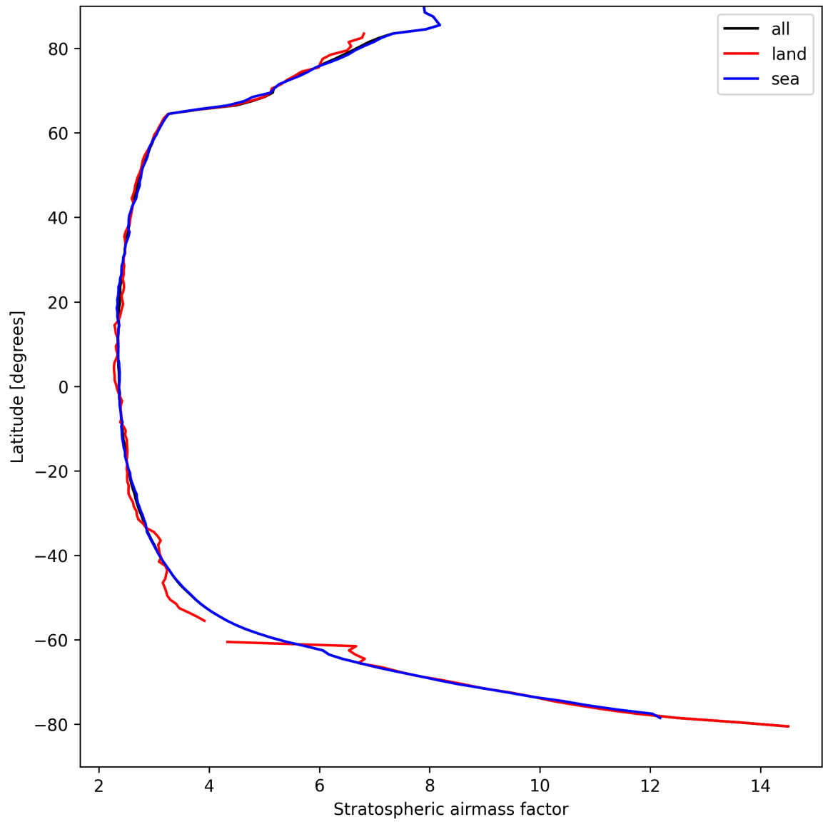
Figure 25: Zonal average of “Stratospheric air mass factor” for 2025-04-08 to 2025-04-09.
