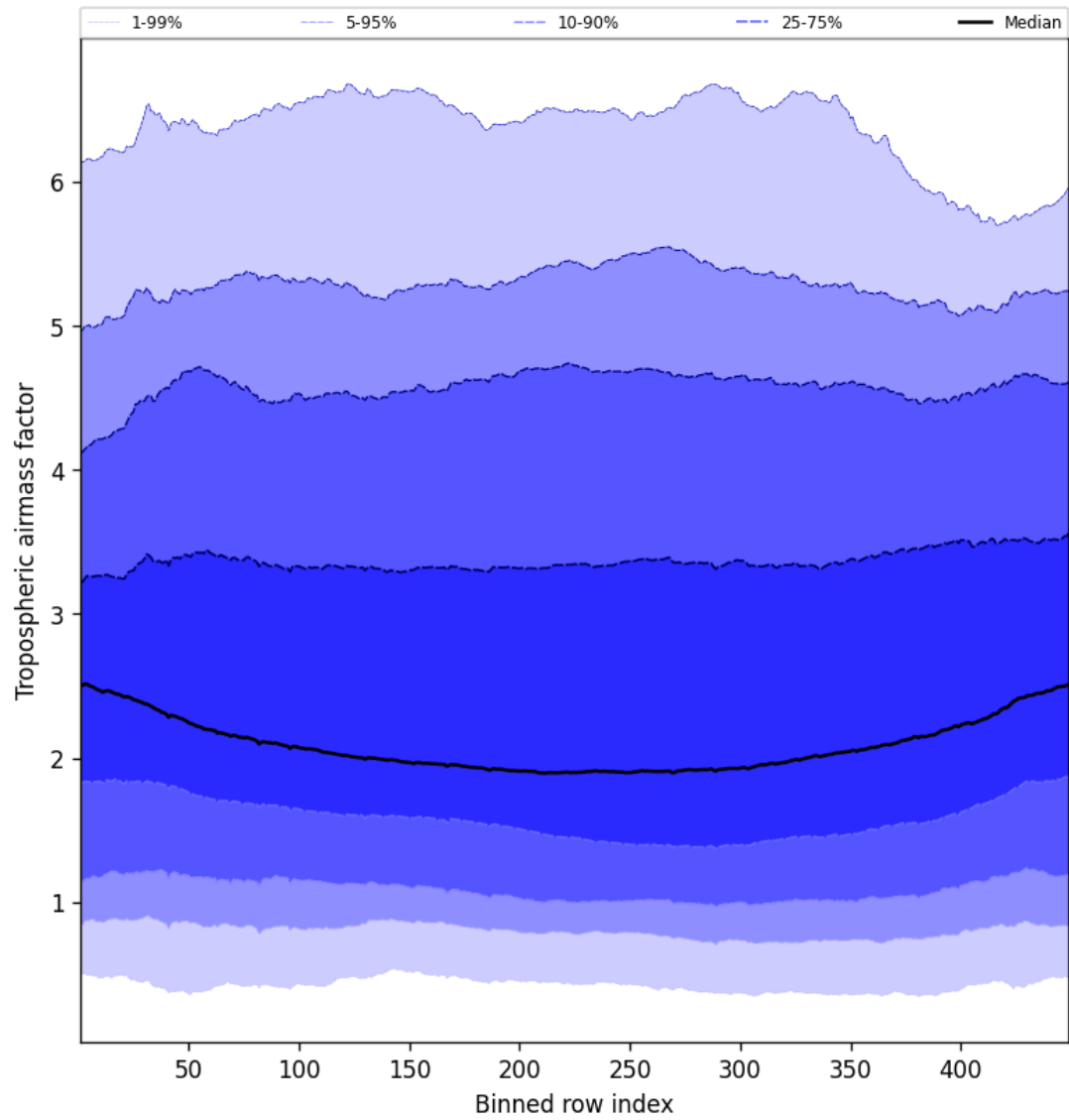
Figure 46: Along track statistics of “Tropospheric airmass factor” for 2025-04-08 to 2025-04-09
