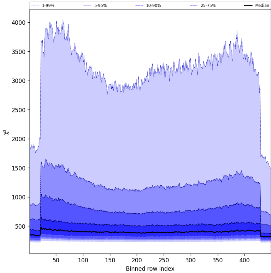
Figure 57: Along track statistics of “ \chi^2 ” for 2025-04-08 to 2025-04-09
