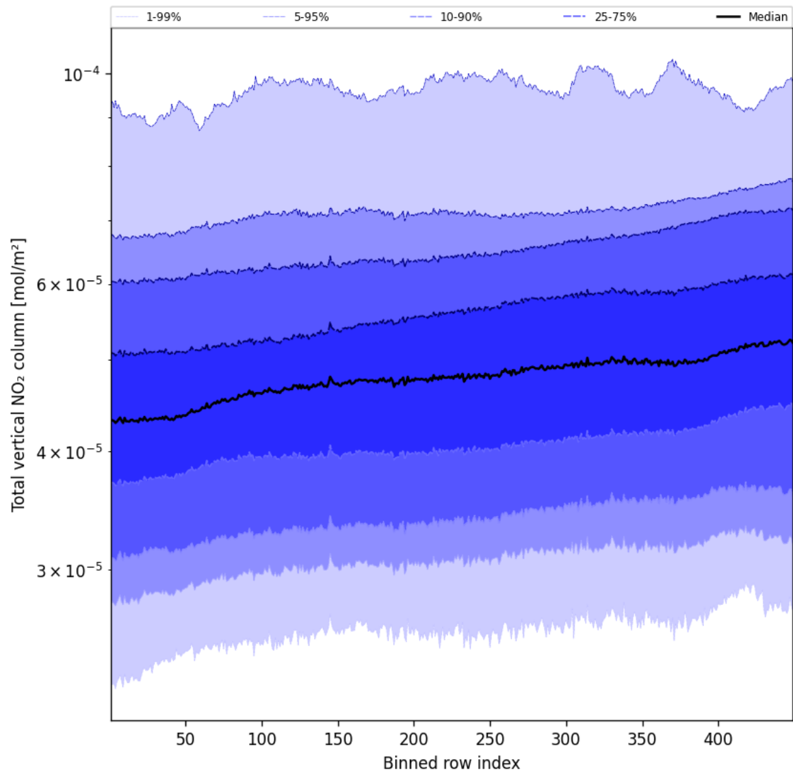
Figure 53: Along track statistics of “Total vertical NO 2 column” for 2025-04-08 to 2025-04-09
