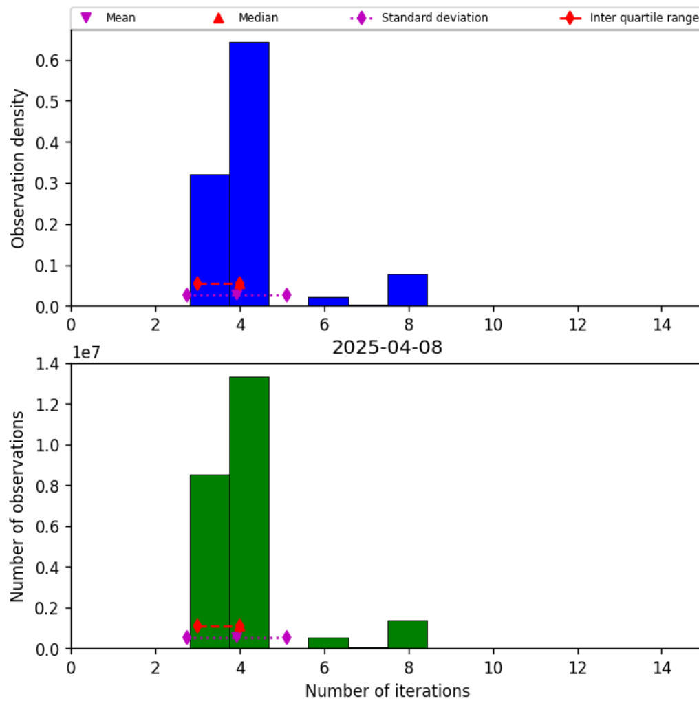
Figure 32: Histogram of “Number of iterations” for 2025-04-08 to 2025-04-09
