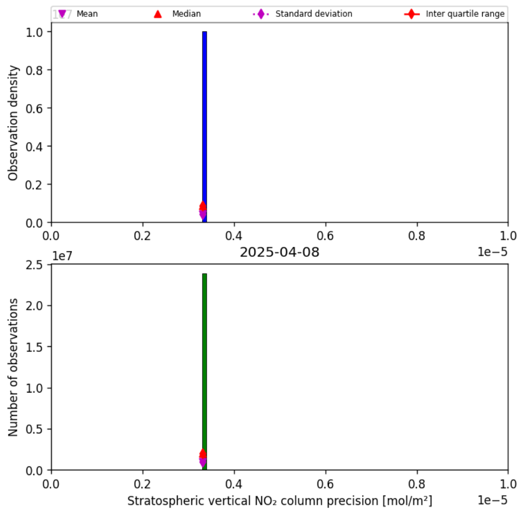
Figure 35: Histogram of “Stratospheric vertical NO 2 column precision” for 2025-04-08 to 2025-04-09
