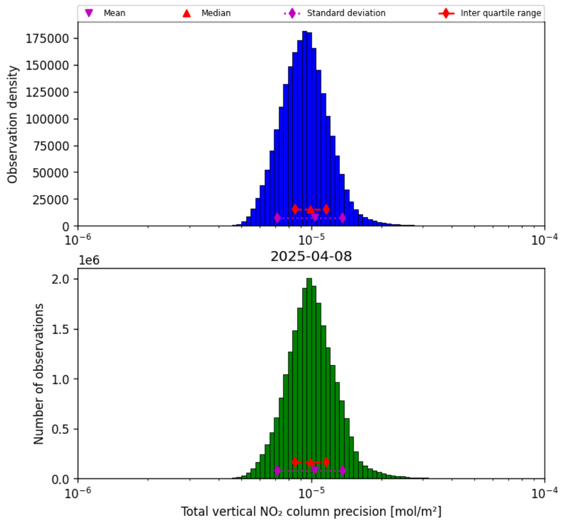
Figure 37: Histogram of “Total vertical NO 2 column precision” for 2025-04-08 to 2025-04-09
