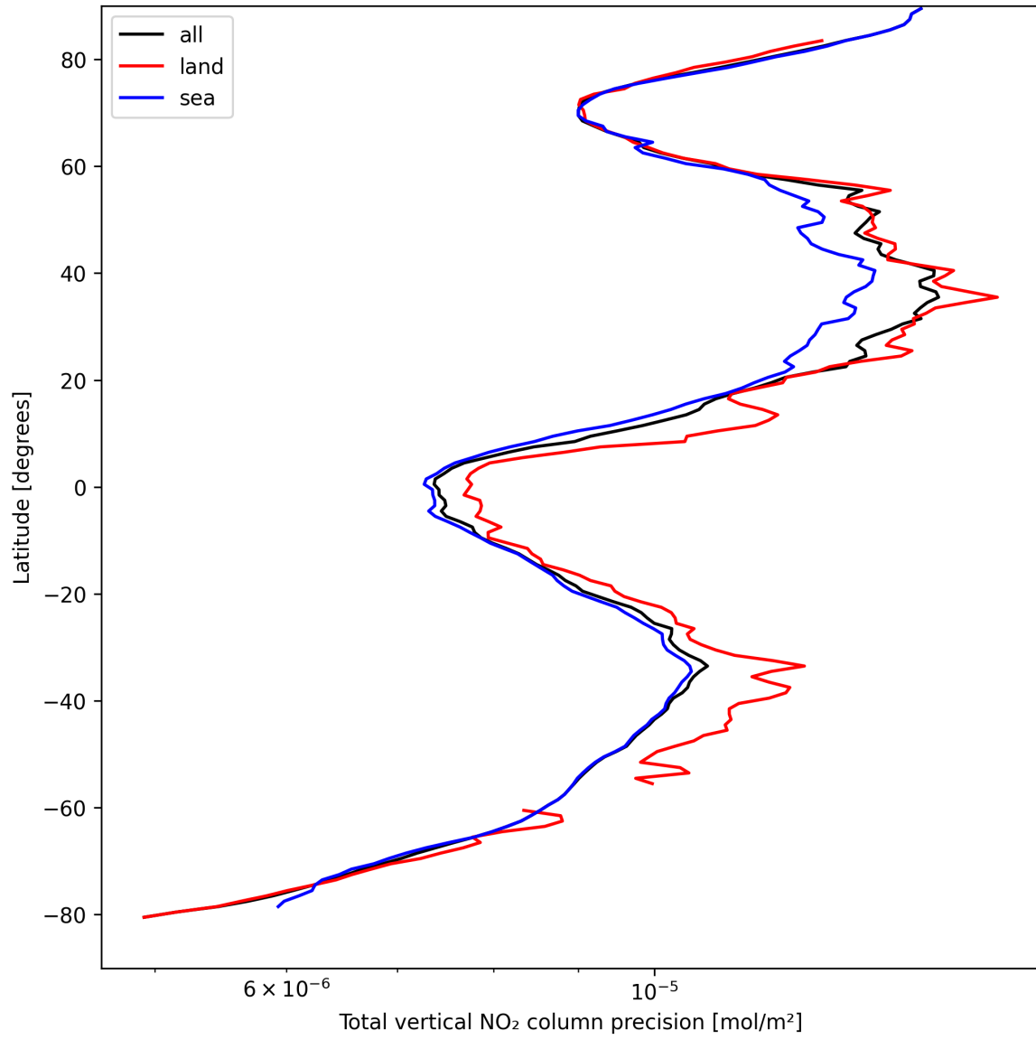
Figure 20: Zonal average of “Total vertical NO 2 column precision” for 2025-04-08 to 2025-04-09.
