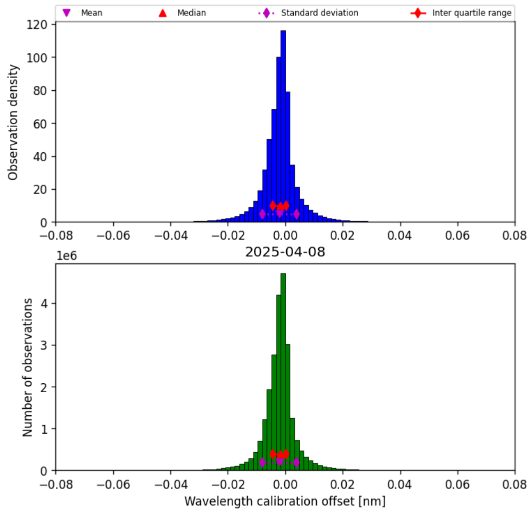
Figure 33: Histogram of “Wavelength calibration offset” for 2025-04-08 to 2025-04-09
