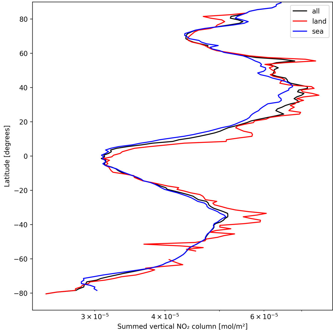
Figure 21: Zonal average of “Summed vertical NO 2 column” for 2025-04-08 to 2025-04-09.
