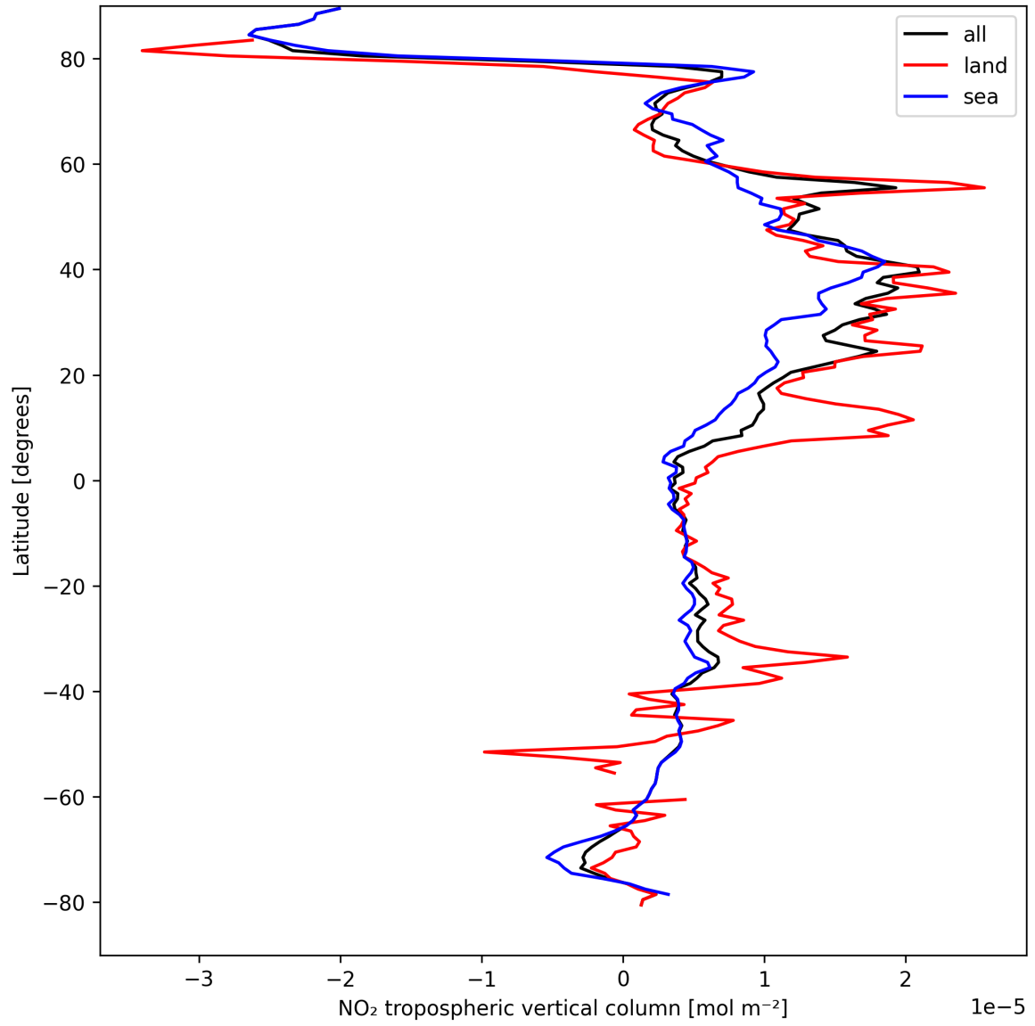
Figure 10: Zonal average of “NO 2 tropospheric vertical column” for 2025-04-08 to 2025-04-09.
