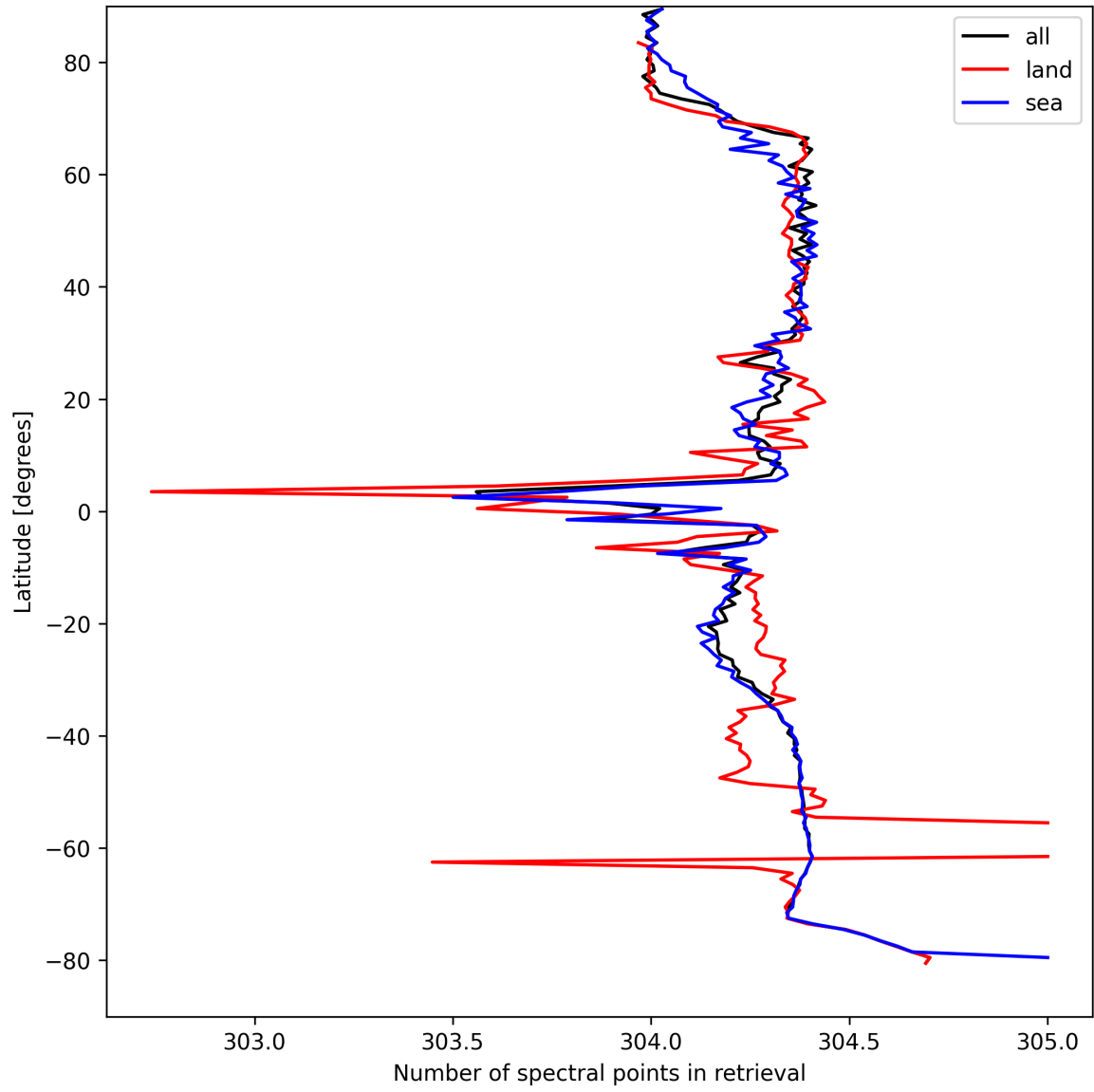
Figure 14: Zonal average of “Number of spectral points in retrieval” for 2025-04-09 to 2025-04-10.
