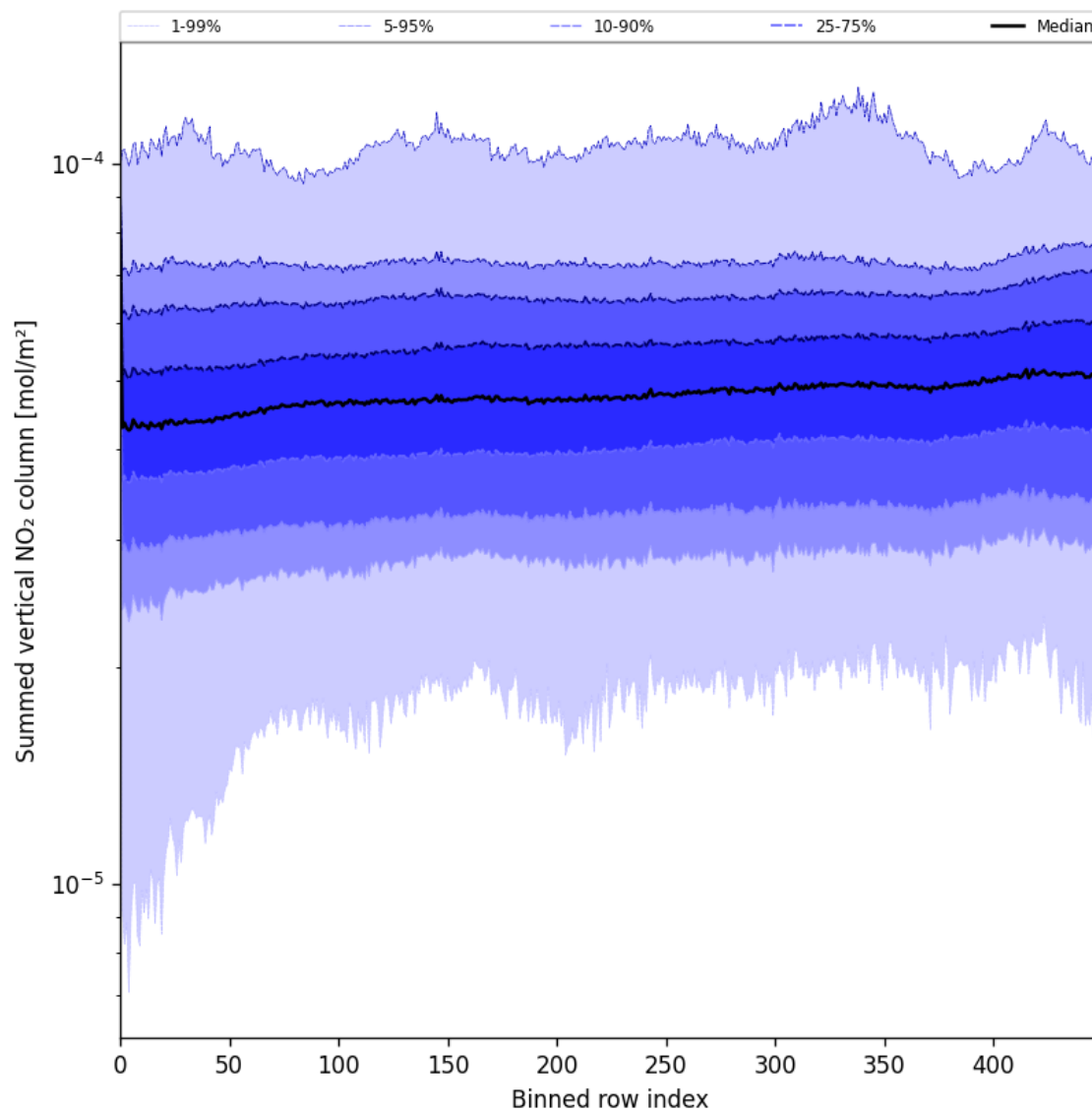
Figure 55: Along track statistics of “Summed vertical NO 2 column” for 2025-04-09 to 2025-04-10
