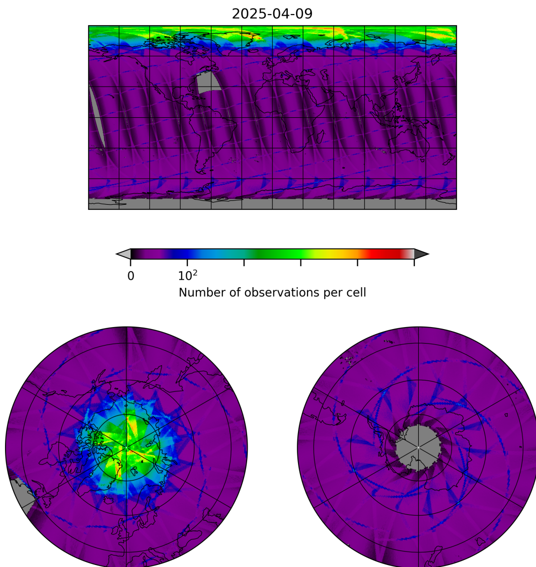
Figure 8: Map of the number of observations for 2025-04-09 to 2025-04-10
