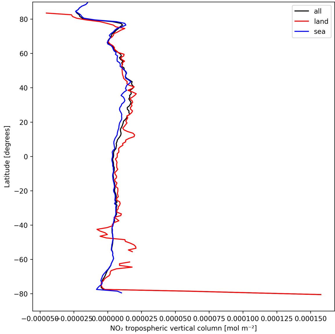
Figure 10: Zonal average of “NO 2 tropospheric vertical column” for 2025-04-09 to 2025-04-10.
