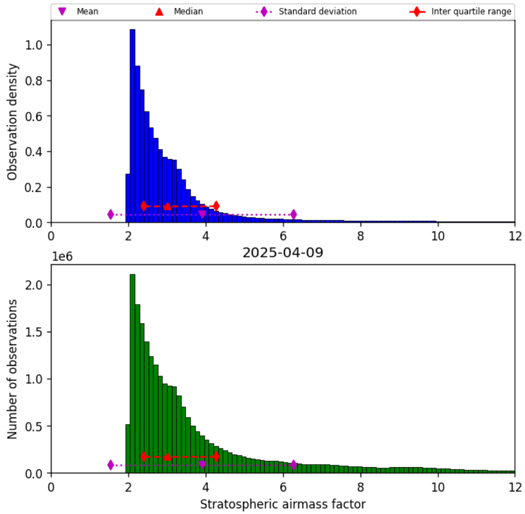
Figure 42: Histogram of “Stratospheric airmass factor” for 2025-04-09 to 2025-04-10
