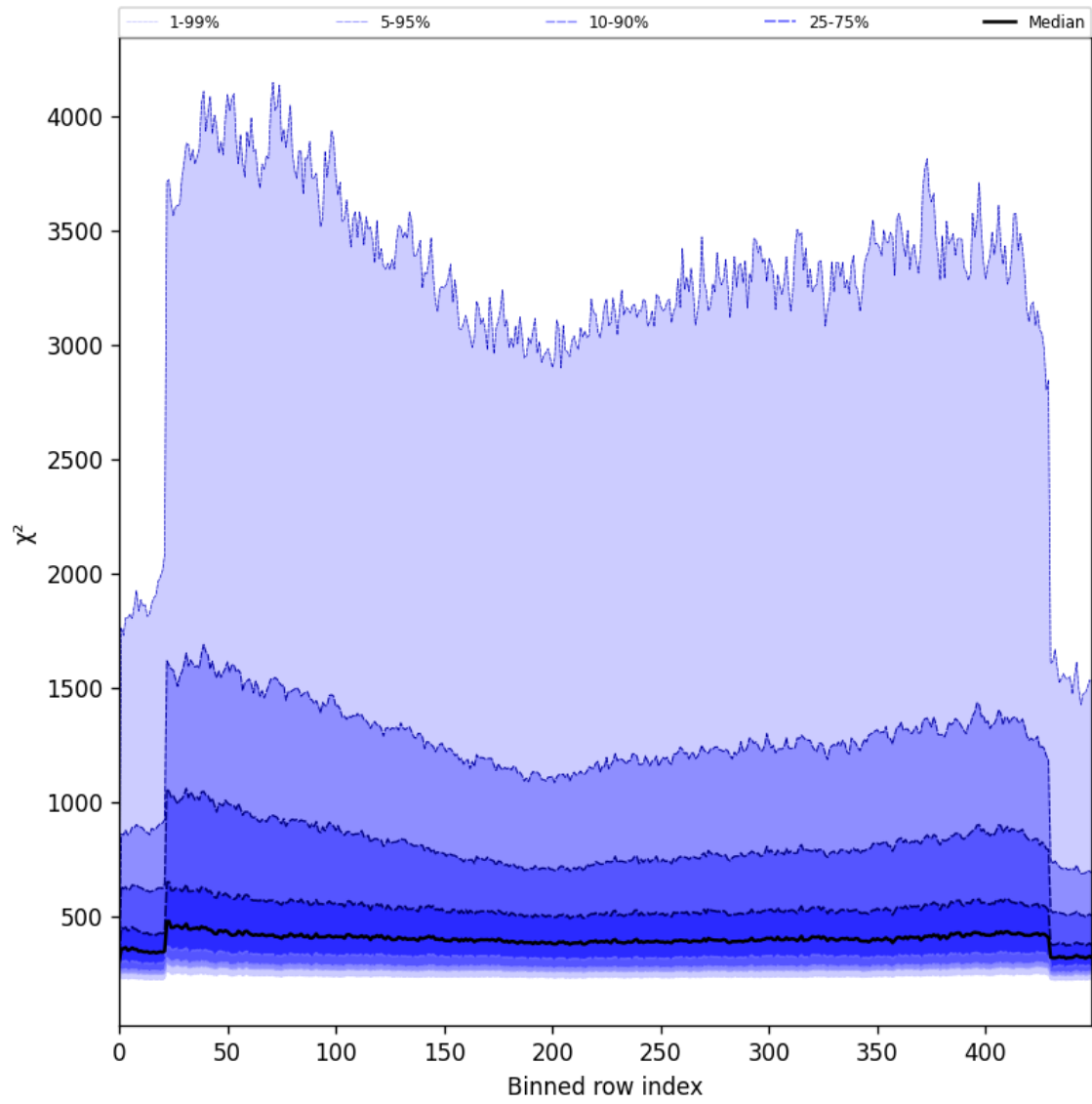
Figure 57: Along track statistics of “ \chi^2 ” for 2025-04-09 to 2025-04-10
