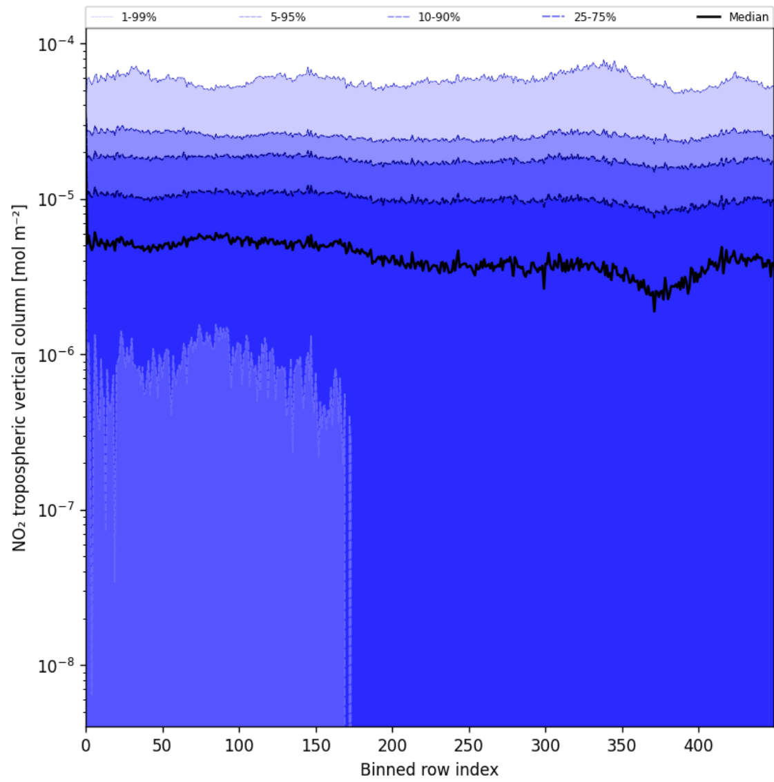
Figure 44: Along track statistics of “NO 2 tropospheric vertical column” for 2025-04-09 to 2025-04-10
