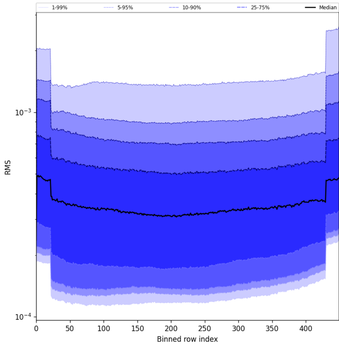
Figure 58: Along track statistics of “RMS” for 2025-04-09 to 2025-04-10
