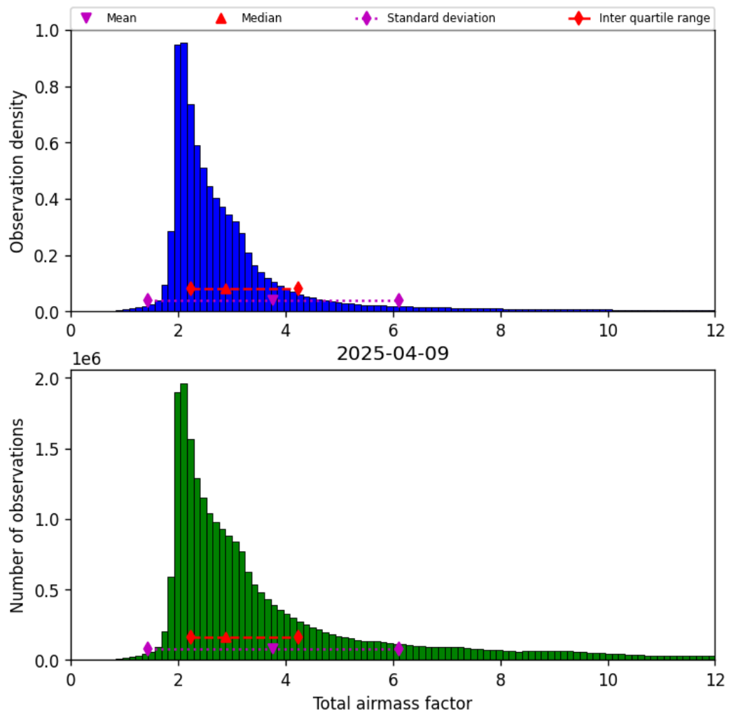
Figure 30: Histogram of “Total airmass factor” for 2025-04-09 to 2025-04-10
