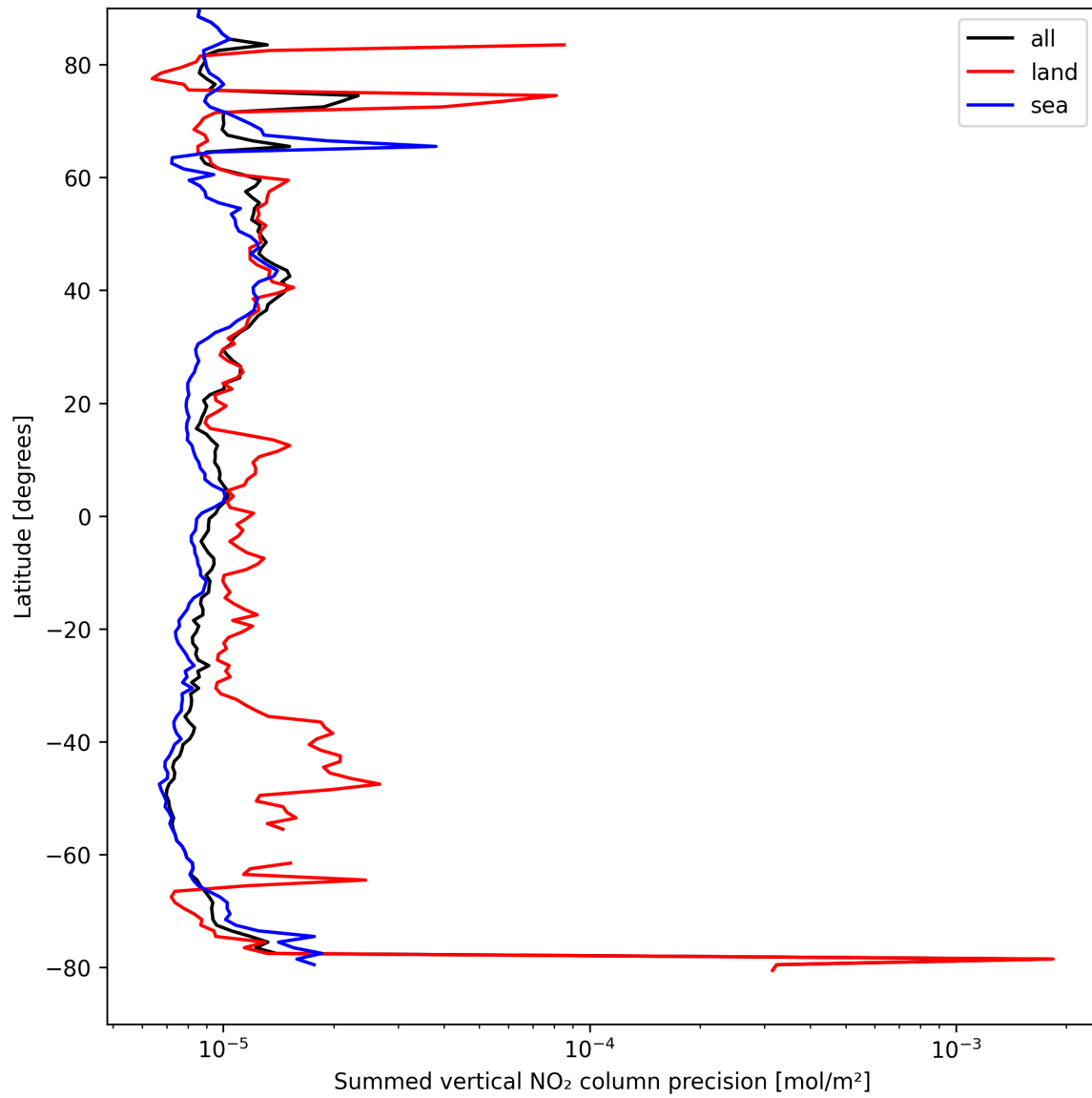
Figure 22: Zonal average of “Summed vertical NO 2 column precision” for 2025-04-09 to 2025-04-10.
