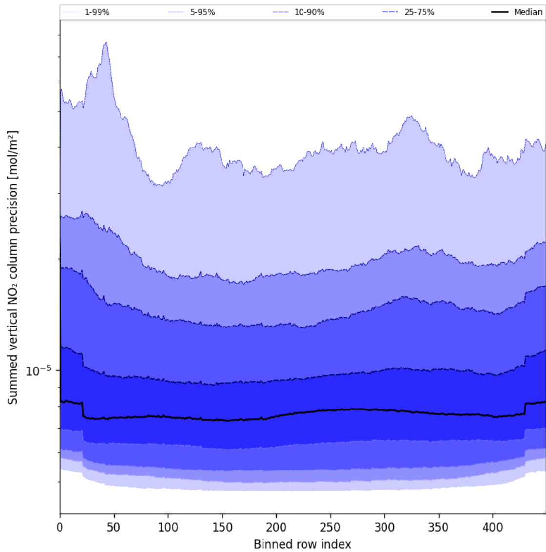
Figure 56: Along track statistics of “Summed vertical NO 2 column precision” for 2025-04-09 to 2025-04-10
