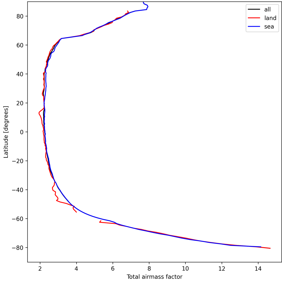
Figure 13: Zonal average of “Total airmass factor” for 2025-04-09 to 2025-04-10.
