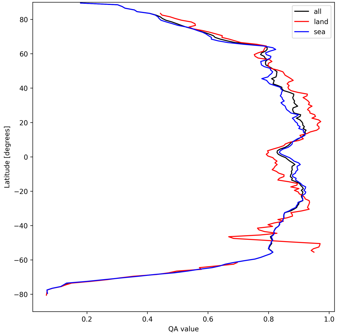
Figure 9: Zonal average of “QA value” for 2025-04-09 to 2025-04-10.
