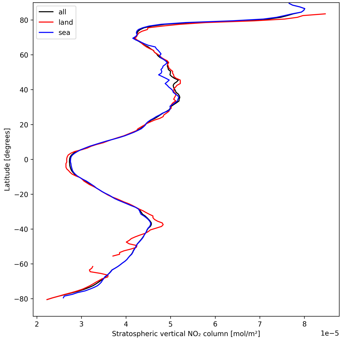
Figure 17: Zonal average of “Stratospheric vertical NO 2 column” for 2025-04-09 to 2025-04-10.
