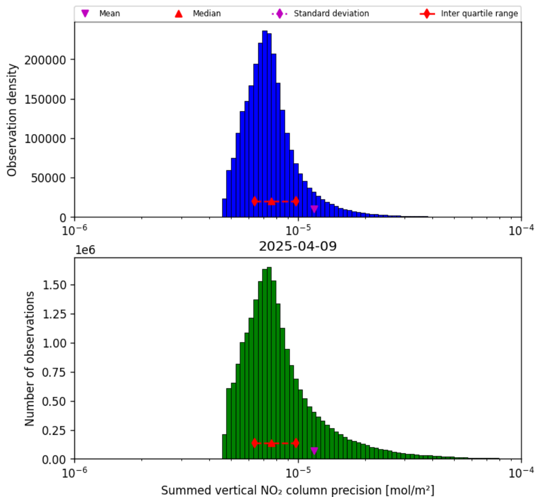
Figure 39: Histogram of “Summed vertical NO 2 column precision” for 2025-04-09 to 2025-04-10
