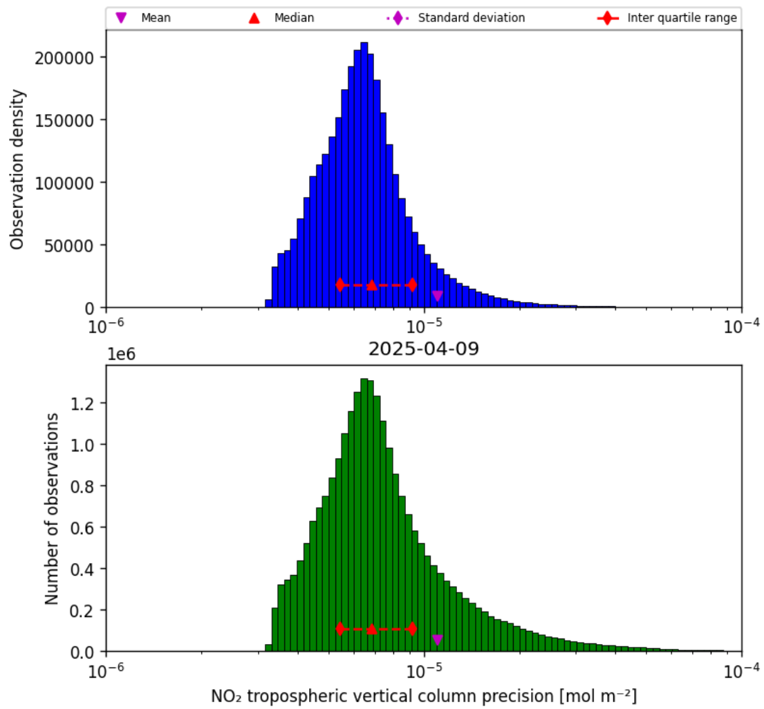
Figure 28: Histogram of “NO 2 tropospheric vertical column precision” for 2025-04-09 to 2025-04-10
