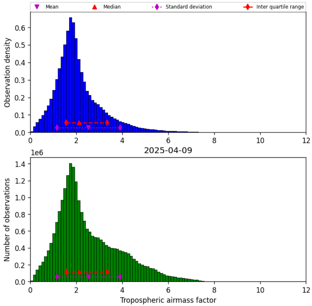
Figure 29: Histogram of “Tropospheric airmass factor” for 2025-04-09 to 2025-04-10
