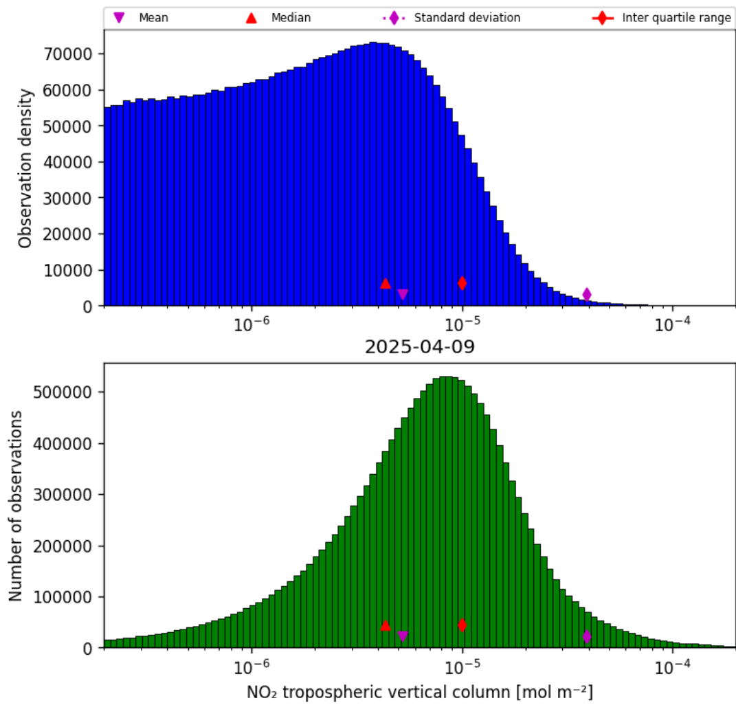
Figure 27: Histogram of “NO 2 tropospheric vertical column” for 2025-04-09 to 2025-04-10
