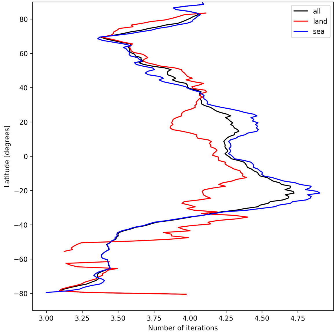
Figure 15: Zonal average of “Number of iterations” for 2025-04-09 to 2025-04-10.
