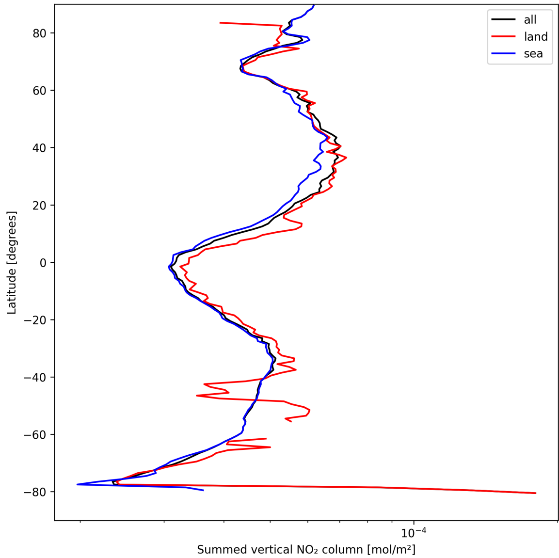
Figure 21: Zonal average of “Summed vertical NO 2 column” for 2025-04-09 to 2025-04-10.
