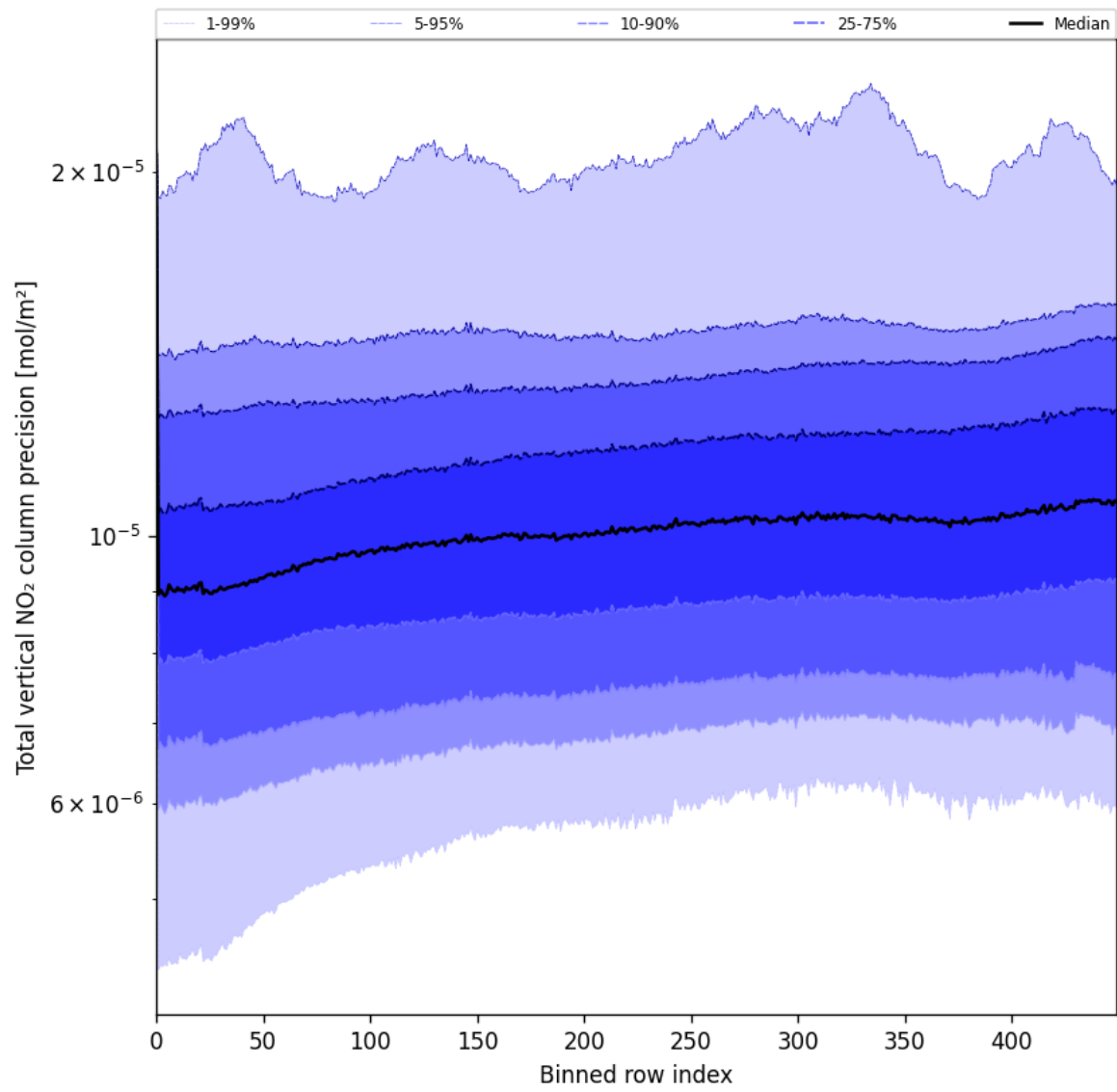
Figure 54: Along track statistics of “Total vertical NO 2 column precision” for 2025-04-09 to 2025-04-10
