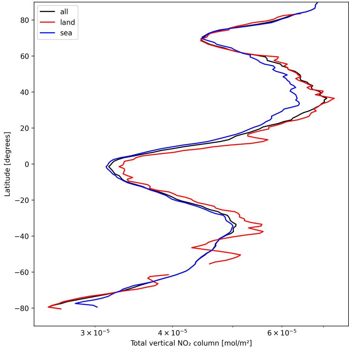
Figure 19: Zonal average of “Total vertical NO 2 column” for 2025-04-09 to 2025-04-10.
