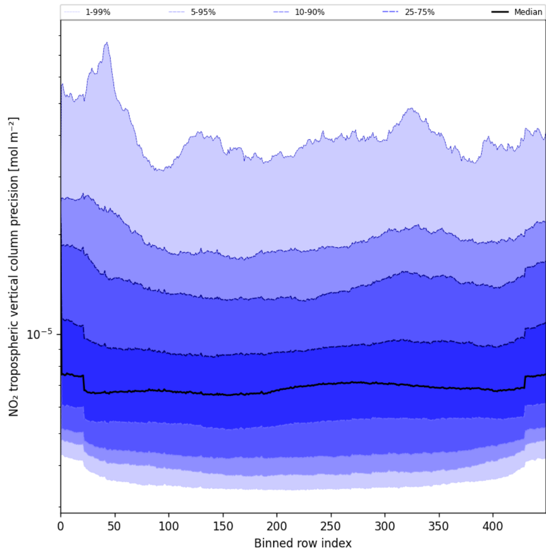
Figure 45: Along track statistics of “NO 2 tropospheric vertical column precision” for 2025-04-09 to 2025-04-10
