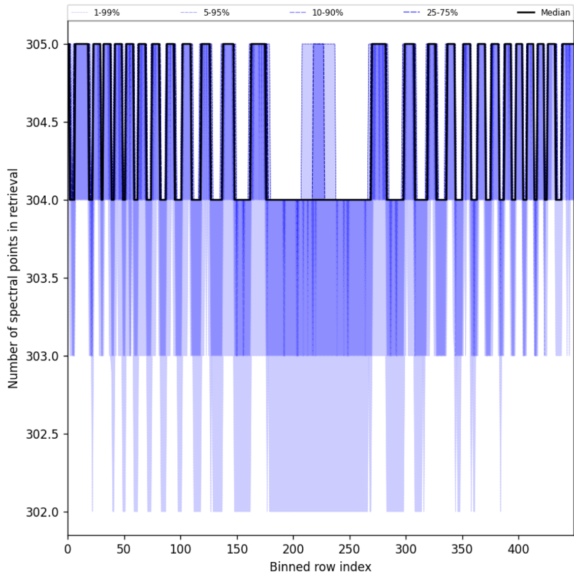
Figure 48: Along track statistics of “Number of spectral points in retrieval” for 2025-04-09 to 2025-04-10
