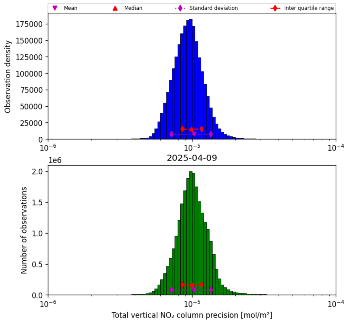
Figure 37: Histogram of "Total vertical NO 2 column precision" for 2025-04-09 to 2025-04-10
