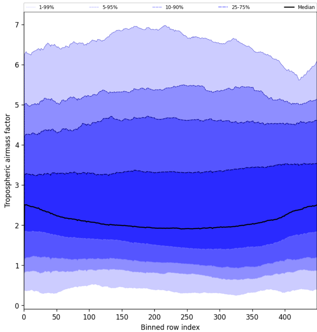
Figure 46: Along track statistics of “Tropospheric airmass factor” for 2025-04-09 to 2025-04-10
