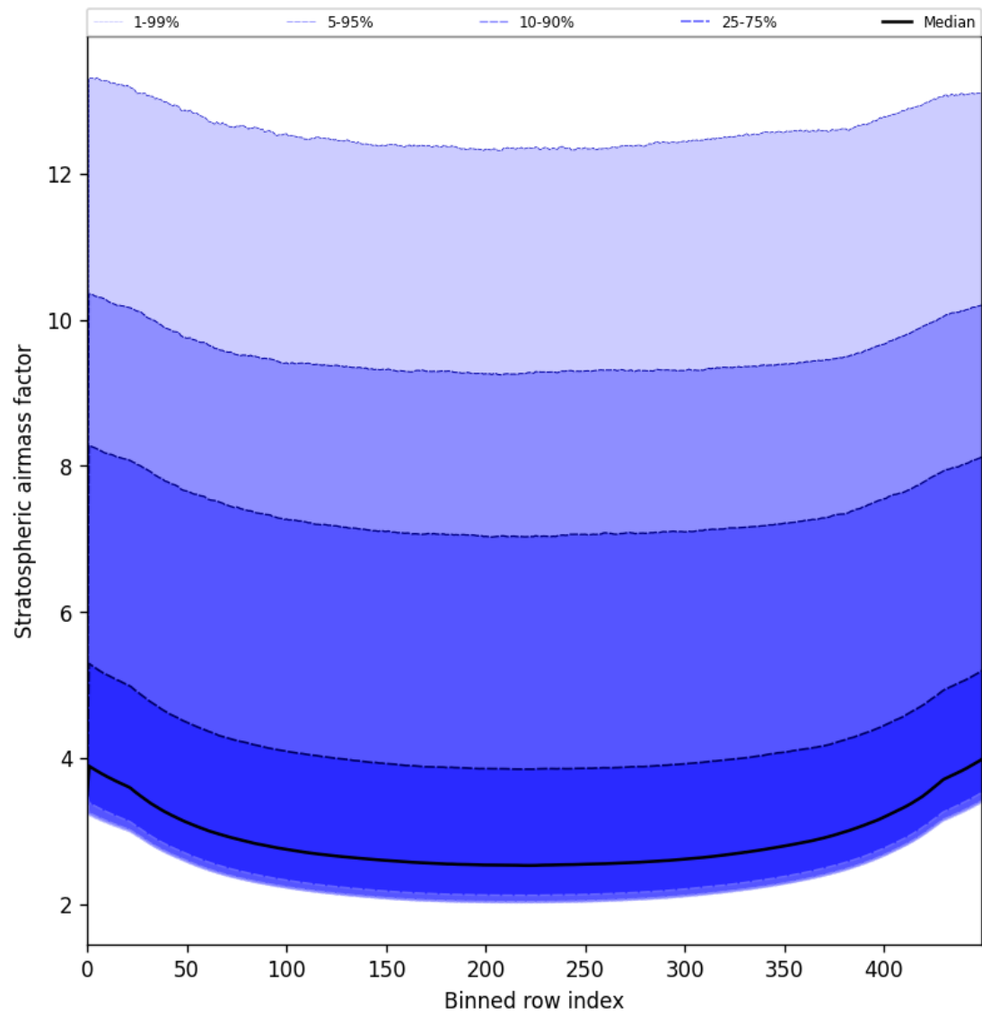
Figure 59: Along track statistics of “Stratospheric airmass factor” for 2025-04-09 to 2025-04-10
