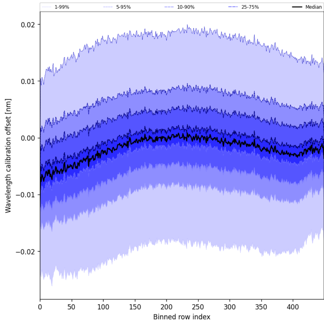
Figure 50: Along track statistics of “Wavelength calibration offset” for 2025-04-09 to 2025-04-10
