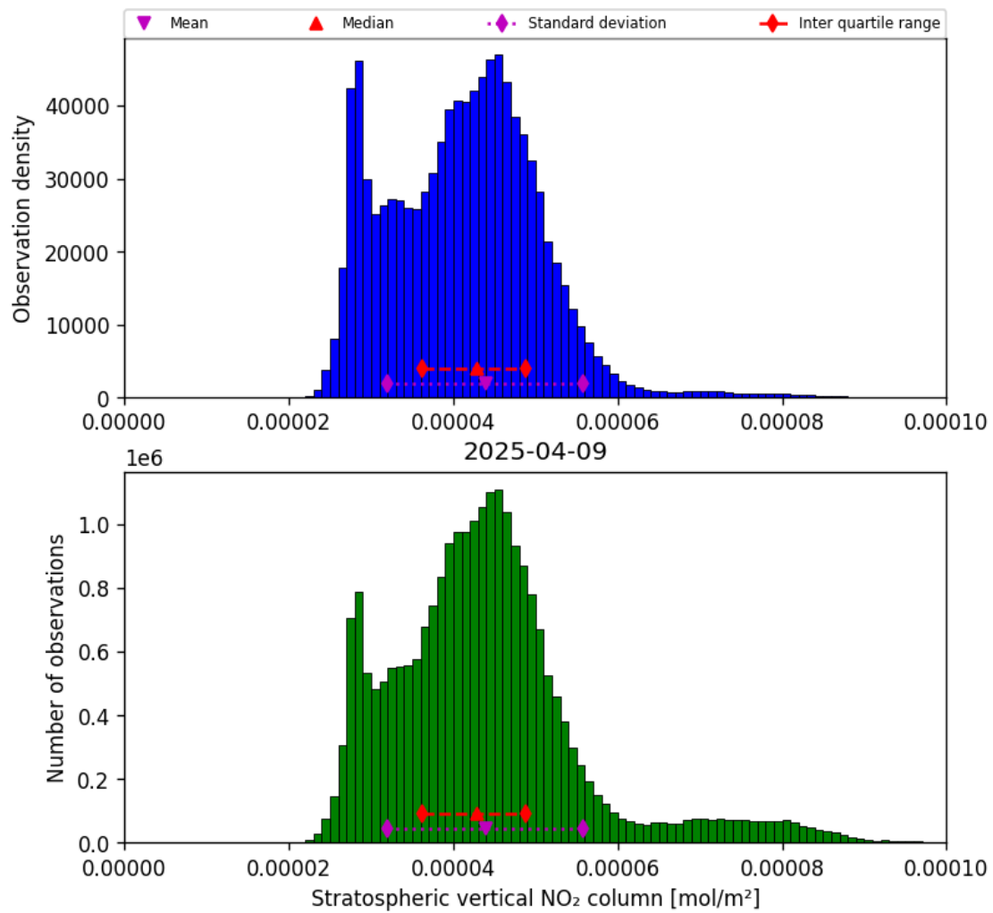
Figure 34: Histogram of “Stratospheric vertical NO 2 column” for 2025-04-09 to 2025-04-10
