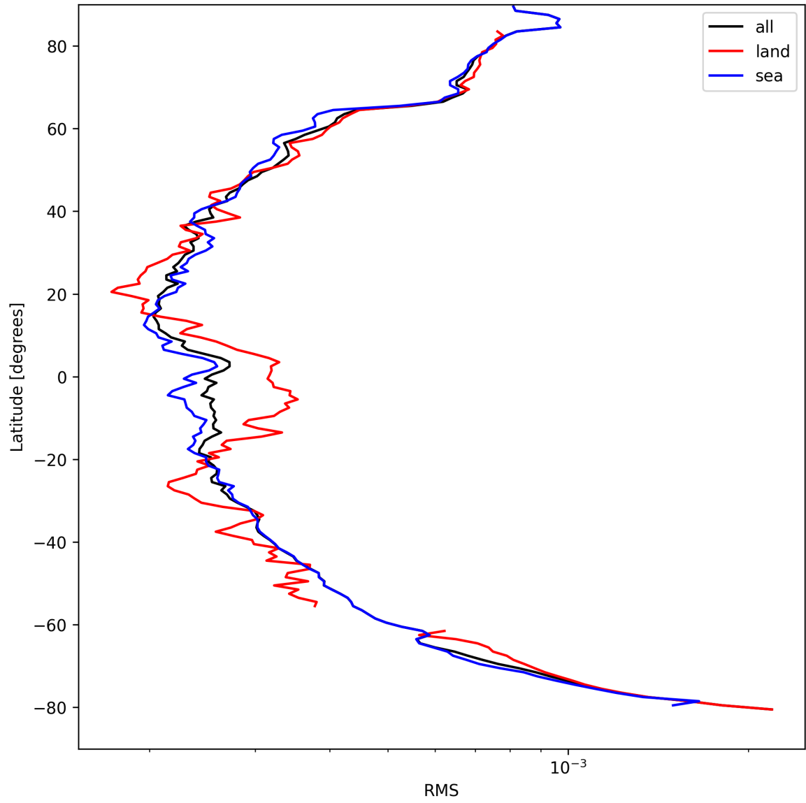
Figure 24: Zonal average of “RMS” for 2025-04-09 to 2025-04-10.
