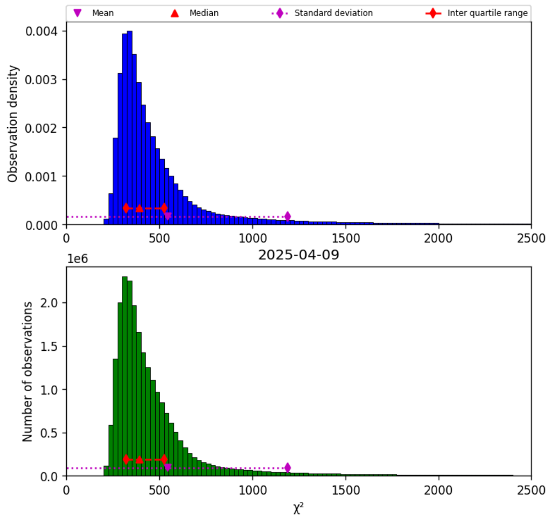
Figure 40: Histogram of “ \chi^2 ” for 2025-04-09 to 2025-04-10
