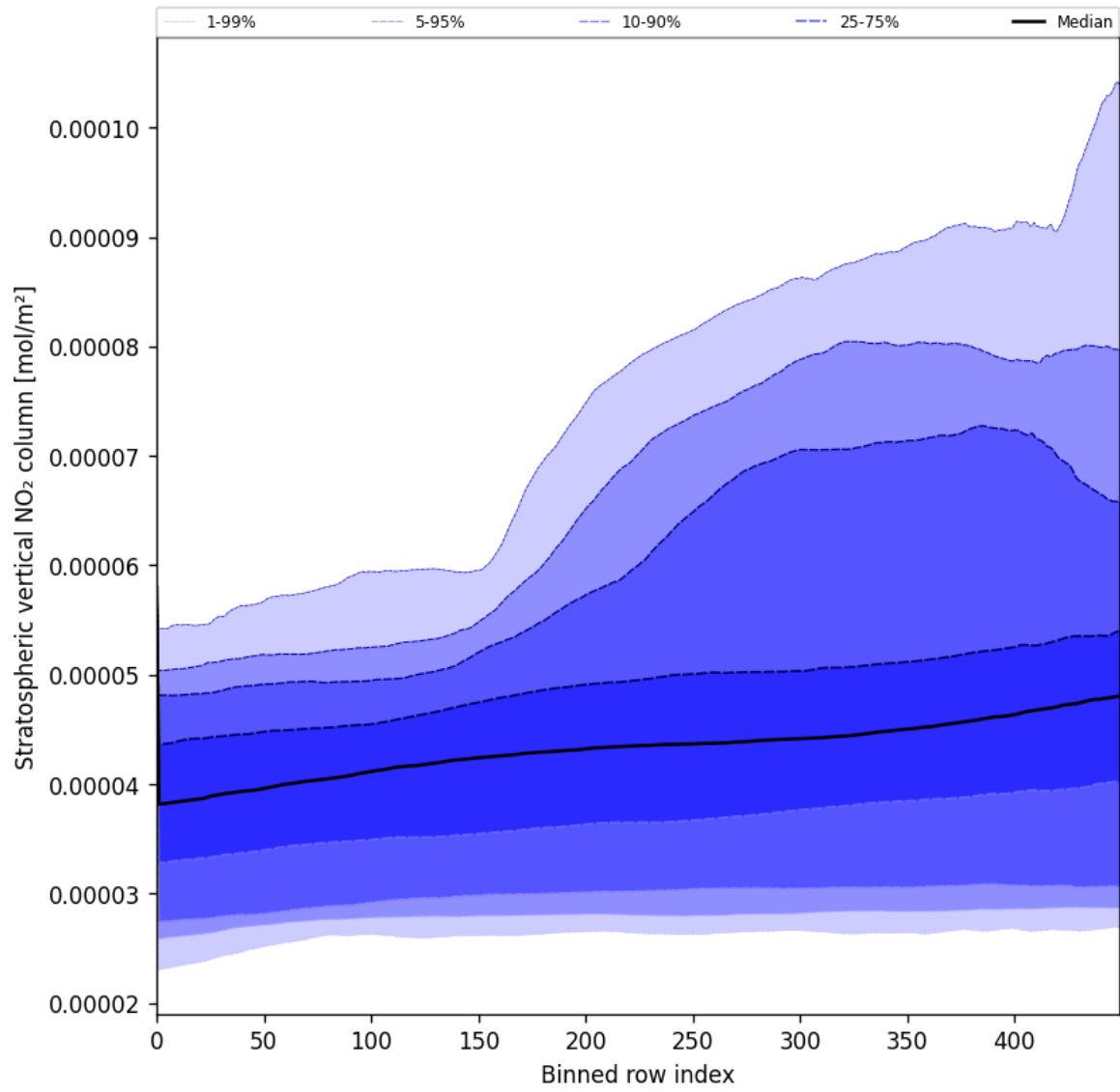
Figure 51: Along track statistics of “Stratospheric vertical NO 2 column” for 2025-04-09 to 2025-04-10
