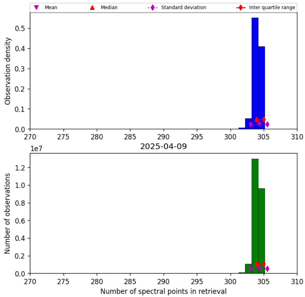
Figure 31: Histogram of “Number of spectral points in retrieval” for 2025-04-09 to 2025-04-10
