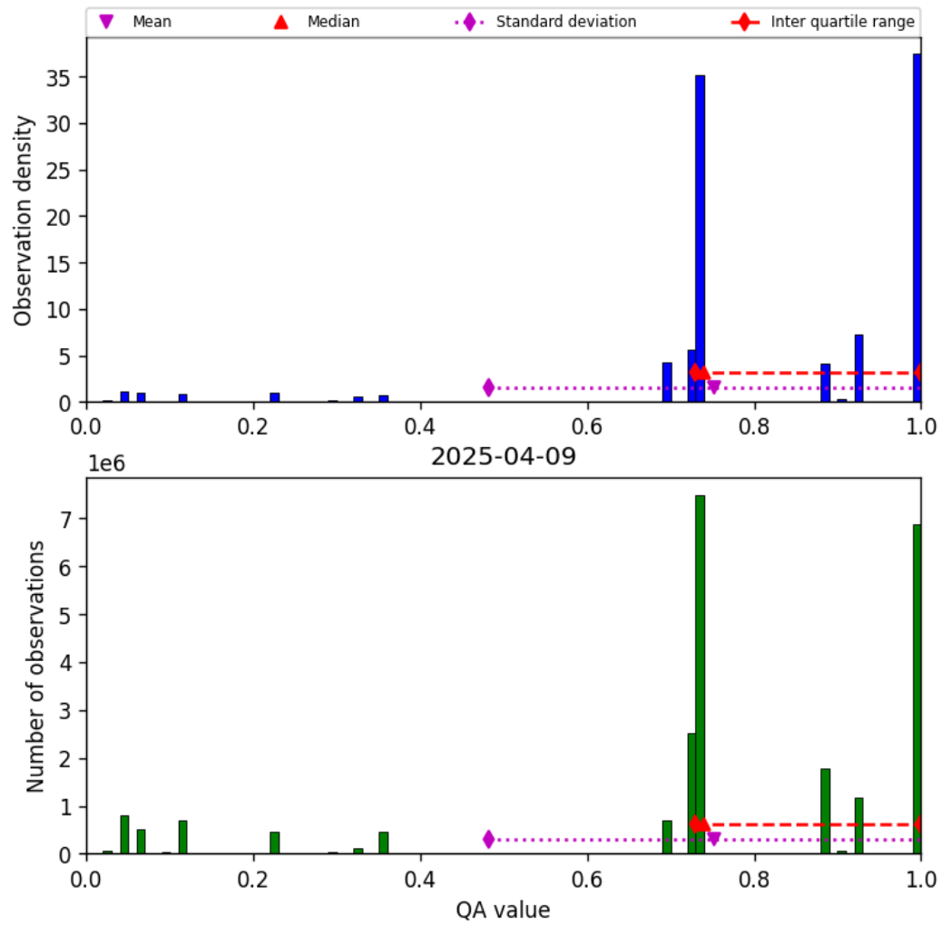
Figure 26: Histogram of “QA value” for 2025-04-09 to 2025-04-10
