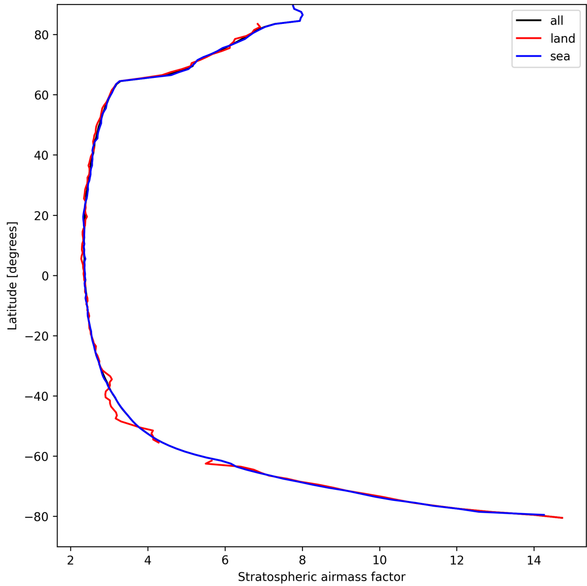
Figure 25: Zonal average of “Stratospheric air mass factor” for 2025-04-09 to 2025-04-10.
