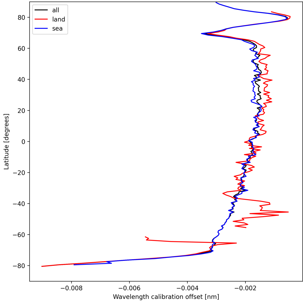
Figure 16: Zonal average of “Wavelength calibration offset” for 2025-04-09 to 2025-04-10.
