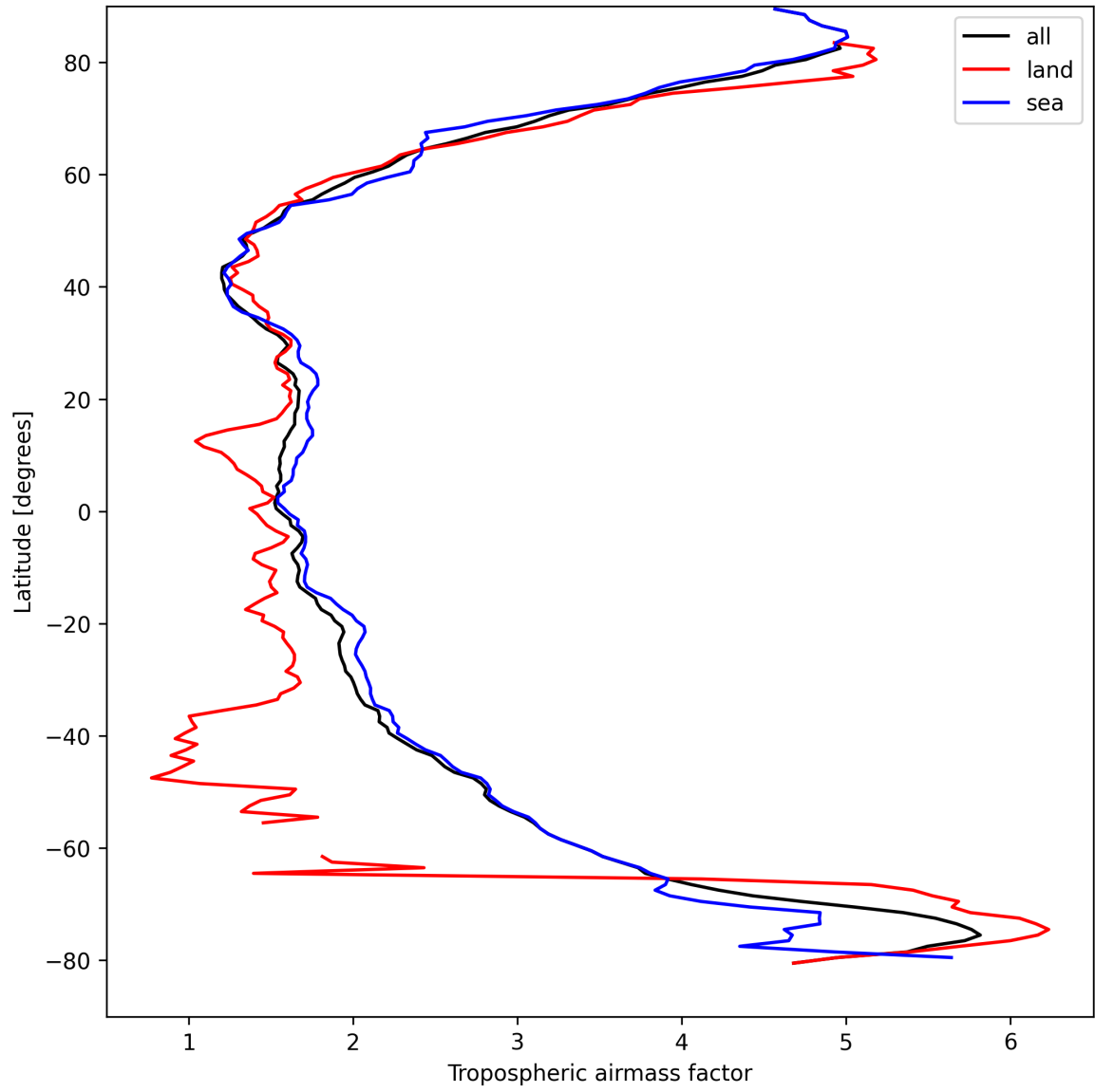
Figure 12: Zonal average of “Tropospheric airmass factor” for 2025-04-09 to 2025-04-10.
