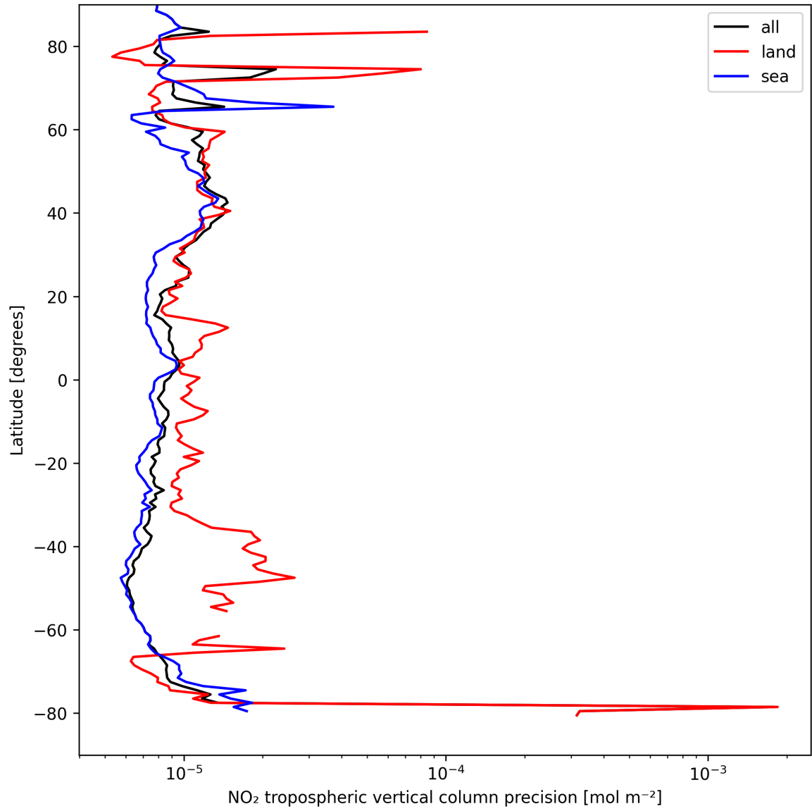
Figure 11: Zonal average of “NO 2 tropospheric vertical column precision” for 2025-04-09 to 2025-04-10.
