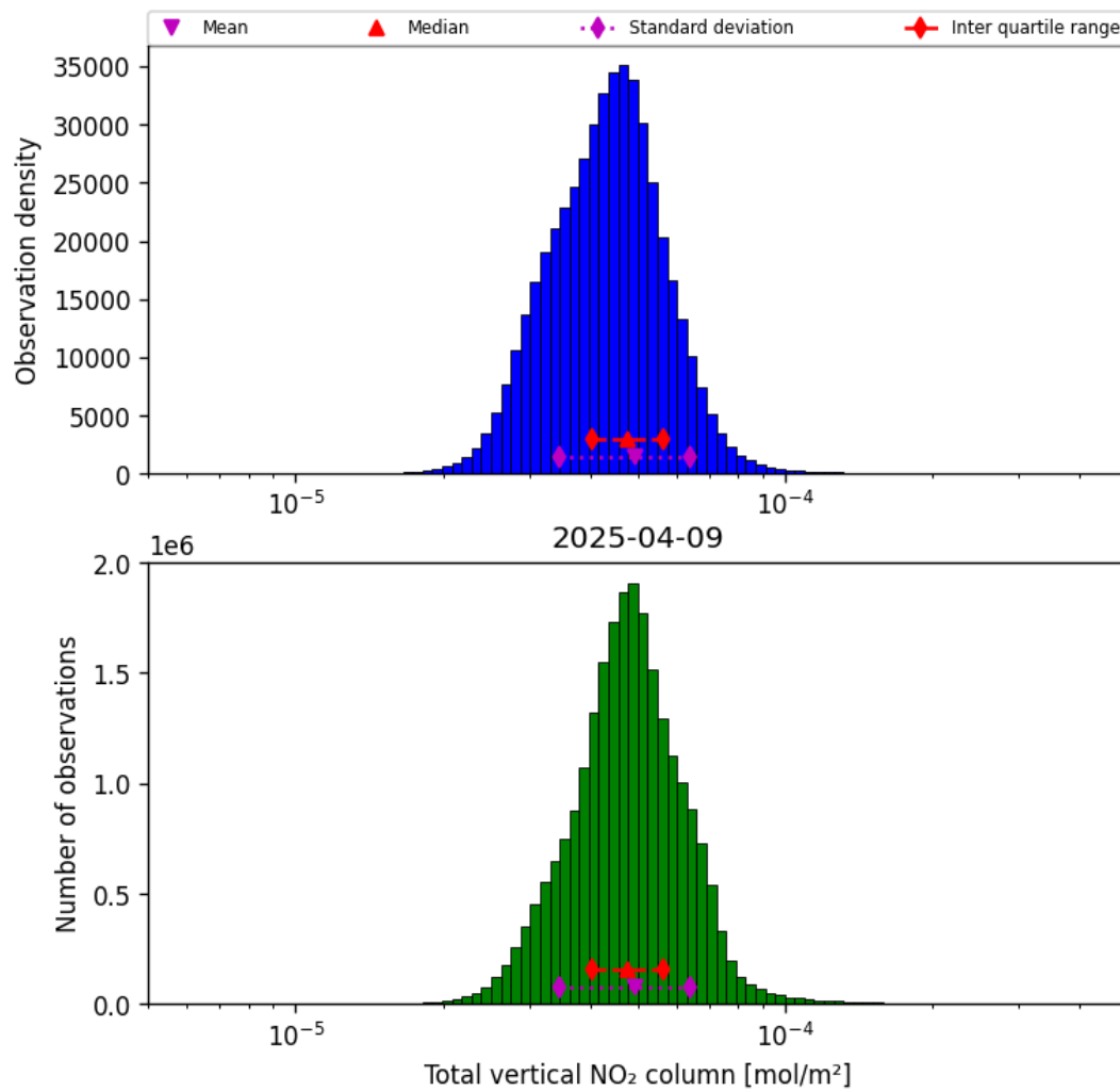
Figure 36: Histogram of “Total vertical NO 2 column” for 2025-04-09 to 2025-04-10
