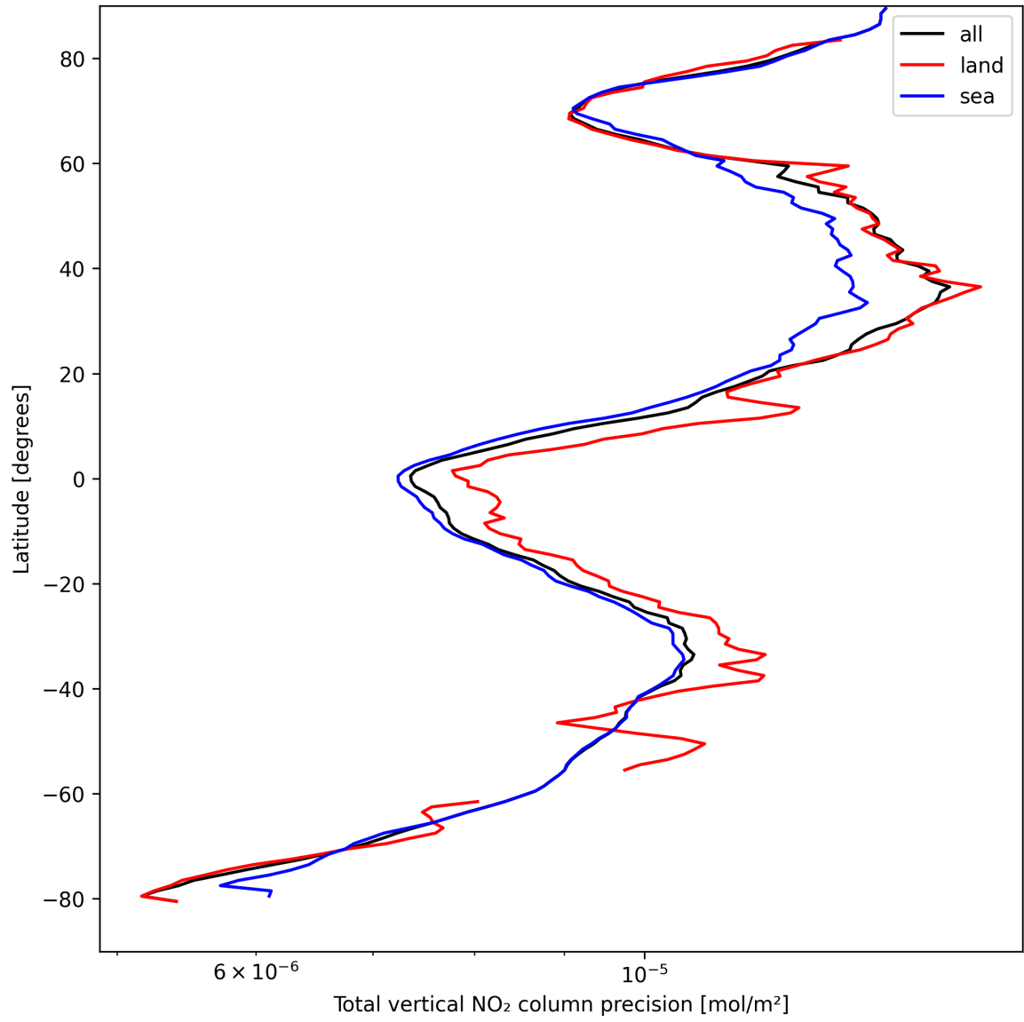
Figure 20: Zonal average of “Total vertical NO 2 column precision” for 2025-04-09 to 2025-04-10.
