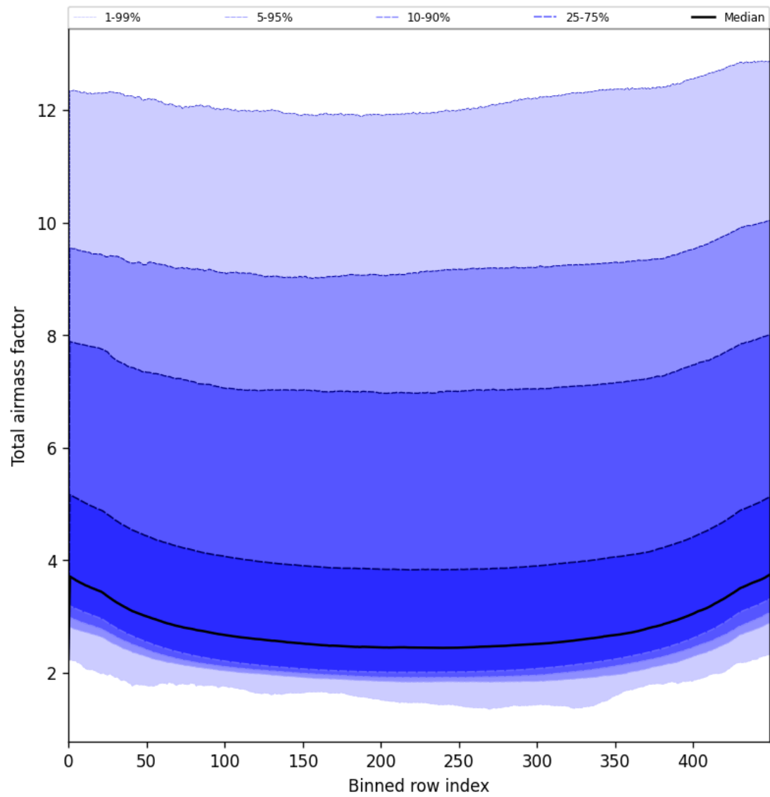
Figure 47: Along track statistics of “Total airmass factor” for 2025-04-09 to 2025-04-10
