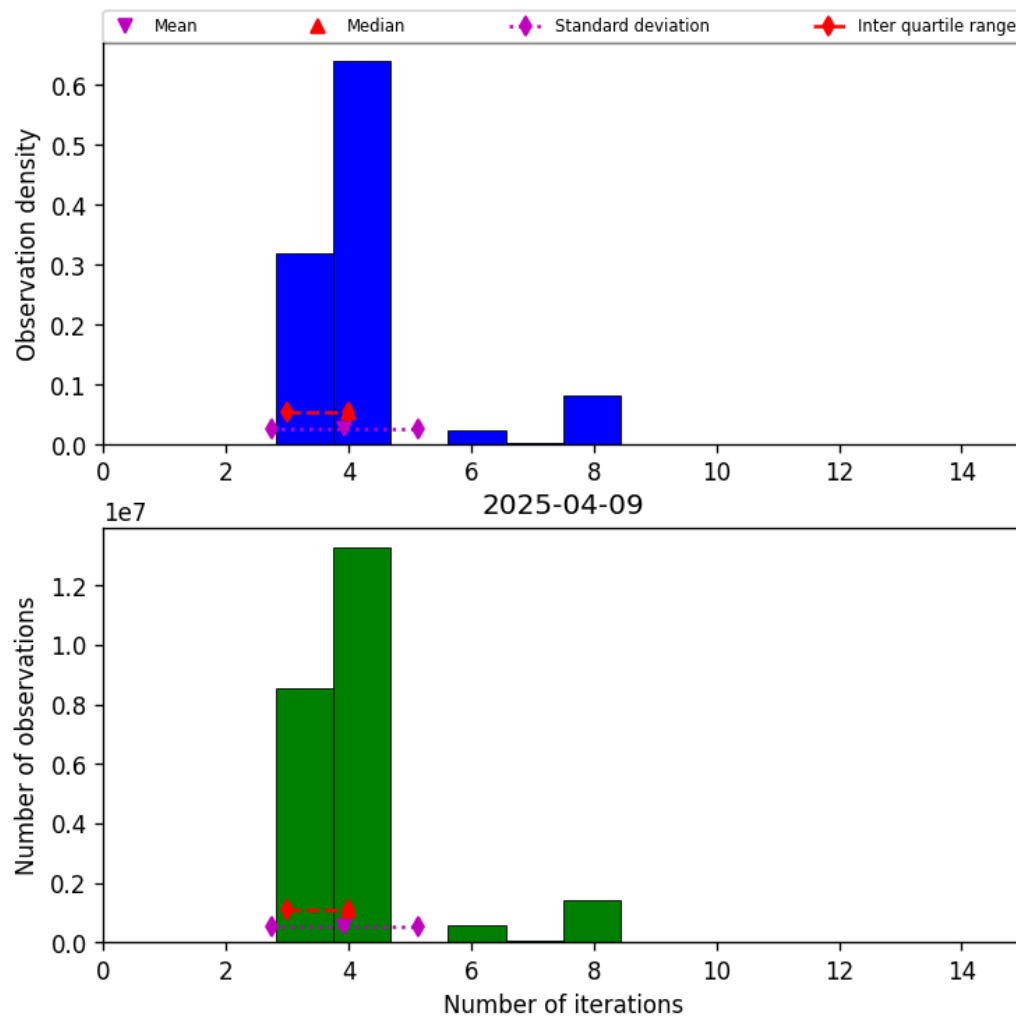
Figure 32: Histogram of “Number of iterations” for 2025-04-09 to 2025-04-10
