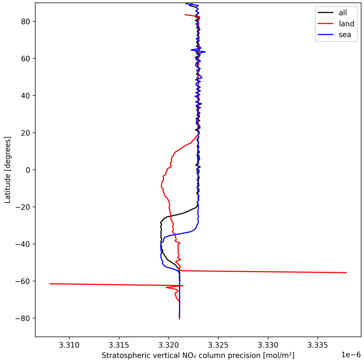
Figure 18: Zonal average of “Stratospheric vertical NO 2 column precision” for 2025-04-09 to 2025-04-10.
