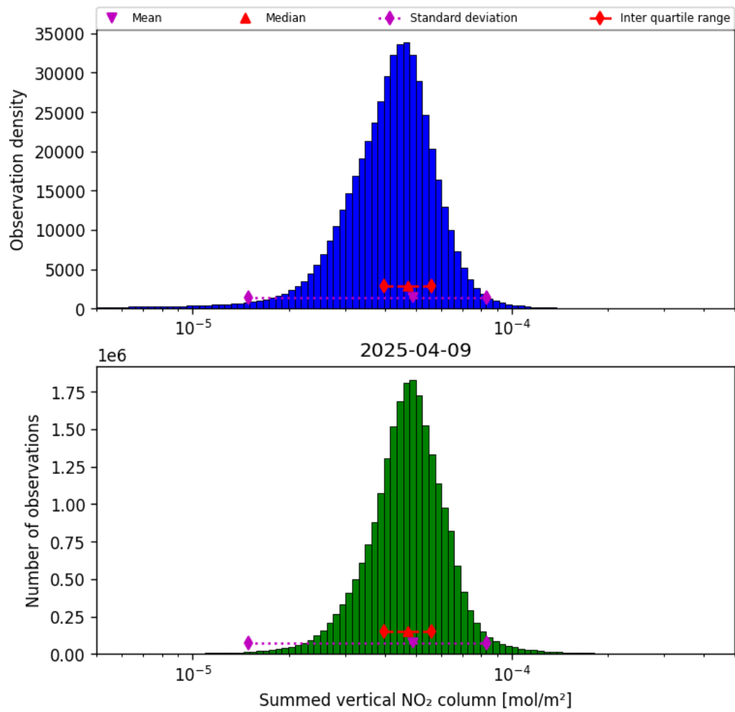
Figure 38: Histogram of “Summed vertical NO 2 column” for 2025-04-09 to 2025-04-10
