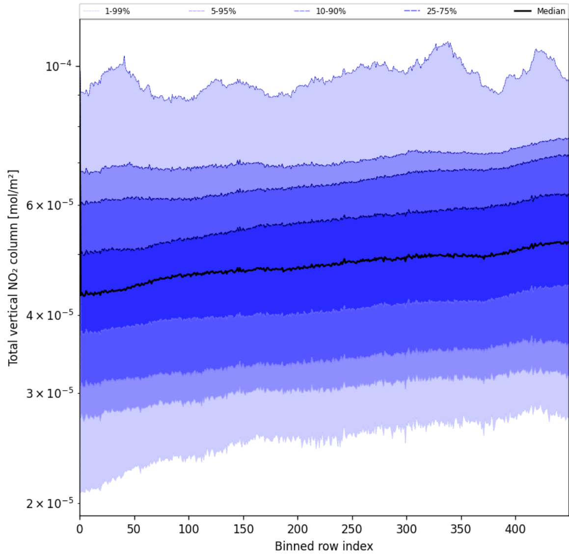
Figure 53: Along track statistics of “Total vertical NO 2 column” for 2025-04-09 to 2025-04-10
