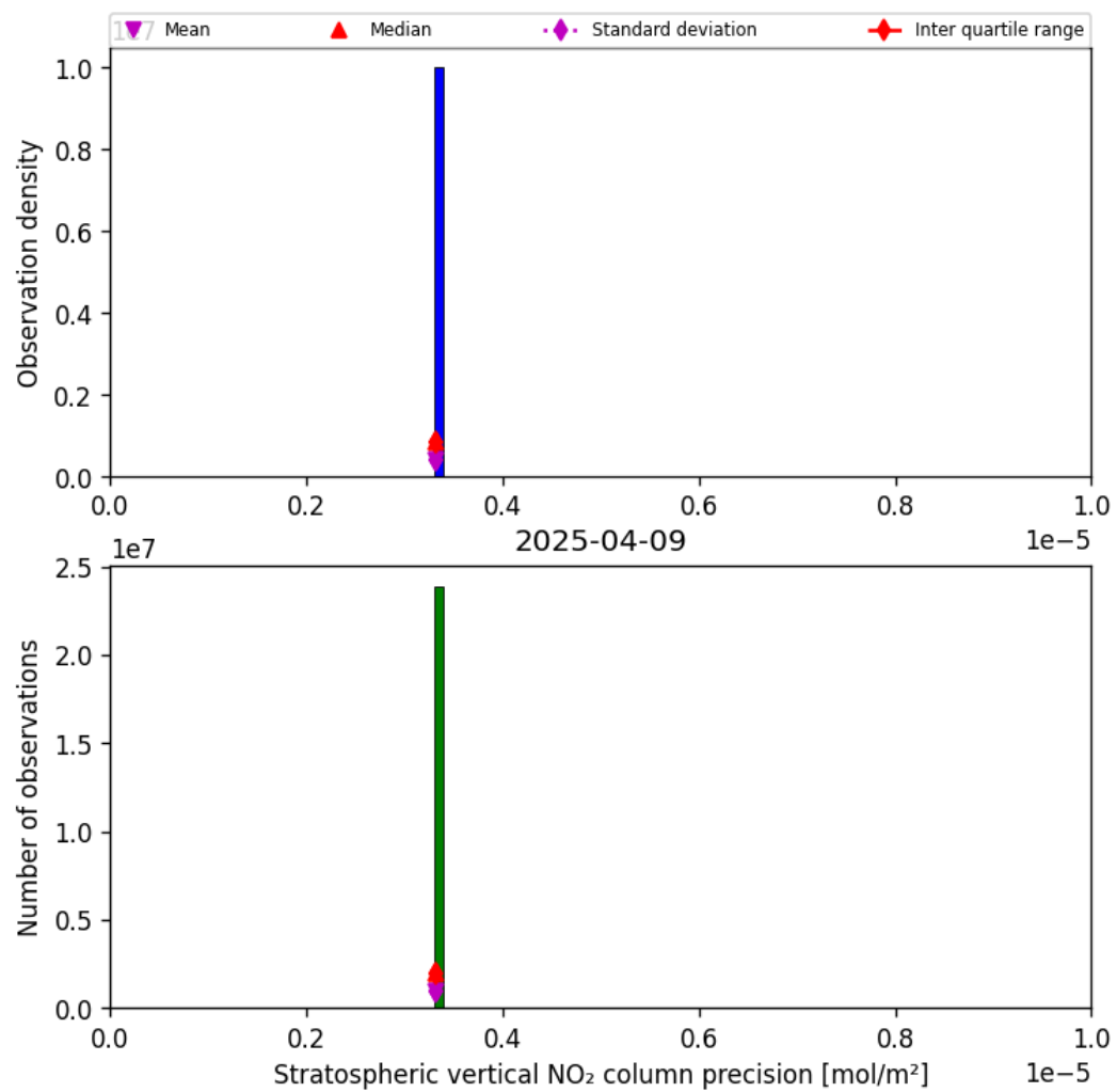
Figure 35: Histogram of “Stratospheric vertical NO 2 column precision” for 2025-04-09 to 2025-04-10
