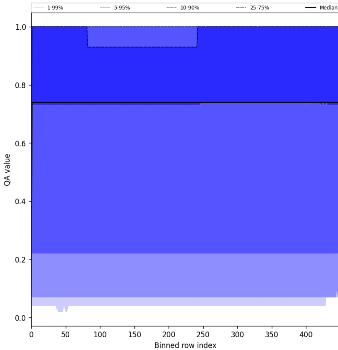
Figure 43: Along track statistics of “QA value” for 2025-04-09 to 2025-04-10
