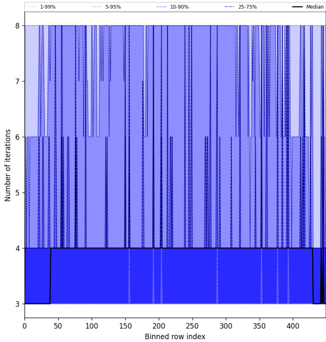
Figure 49: Along track statistics of “Number of iterations” for 2025-04-09 to 2025-04-10
