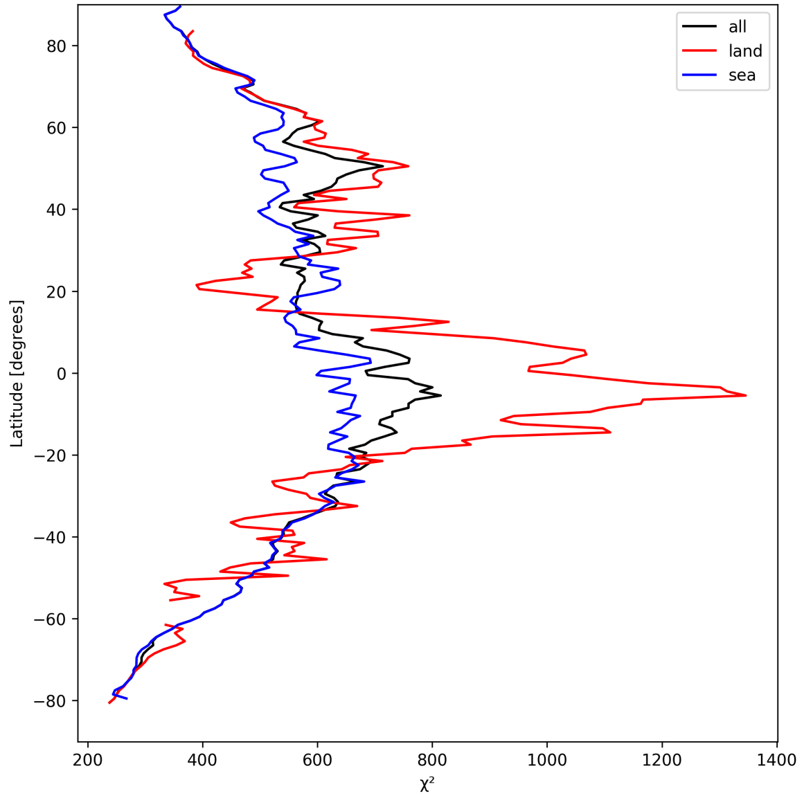
Figure 23: Zonal average of “ \chi^2 ” for 2025-04-09 to 2025-04-10.
