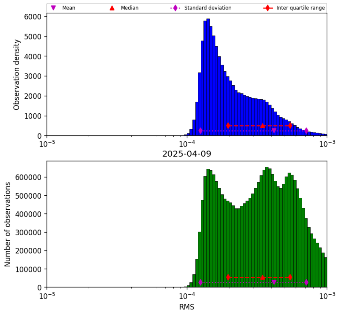
Figure 41: Histogram of “RMS” for 2025-04-09 to 2025-04-10
