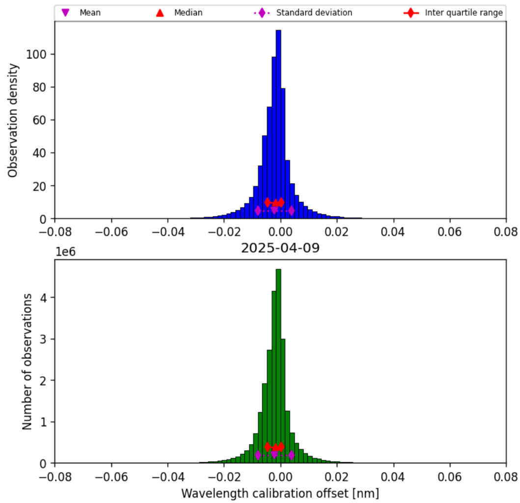
Figure 33: Histogram of “Wavelength calibration offset” for 2025-04-09 to 2025-04-10
