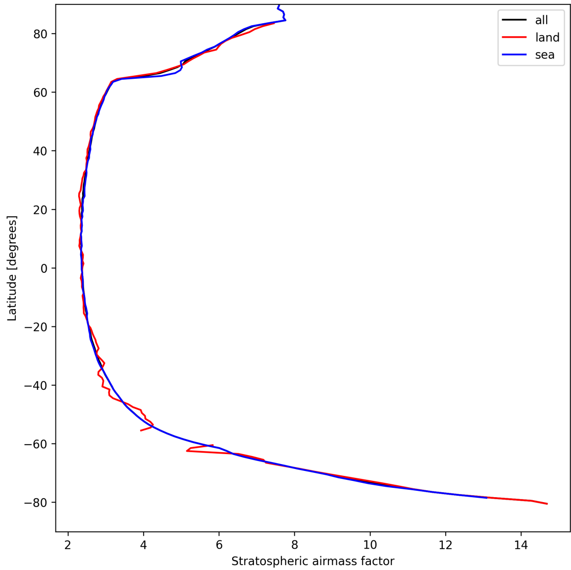
Figure 25: Zonal average of “Stratospheric air mass factor” for 2025-04-10 to 2025-04-11.
