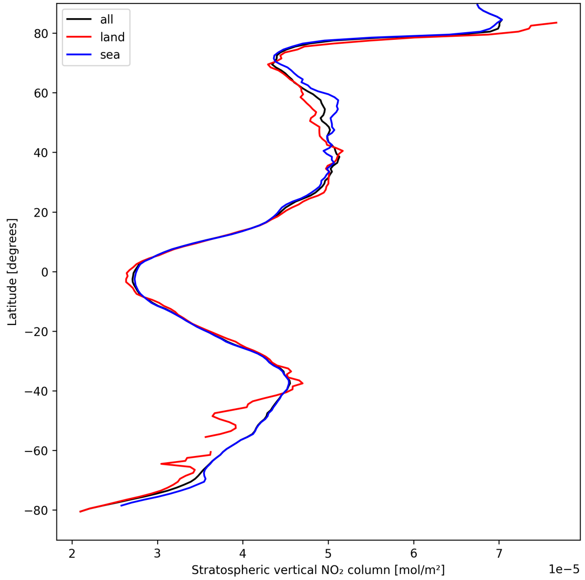
Figure 17: Zonal average of “Stratospheric vertical NO 2 column” for 2025-04-10 to 2025-04-11.
