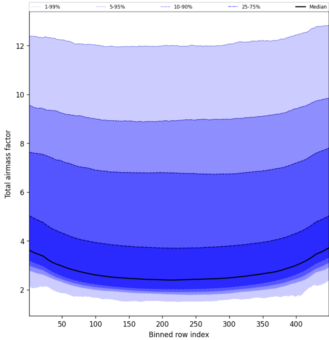
Figure 47: Along track statistics of “Total airmass factor” for 2025-04-10 to 2025-04-11
