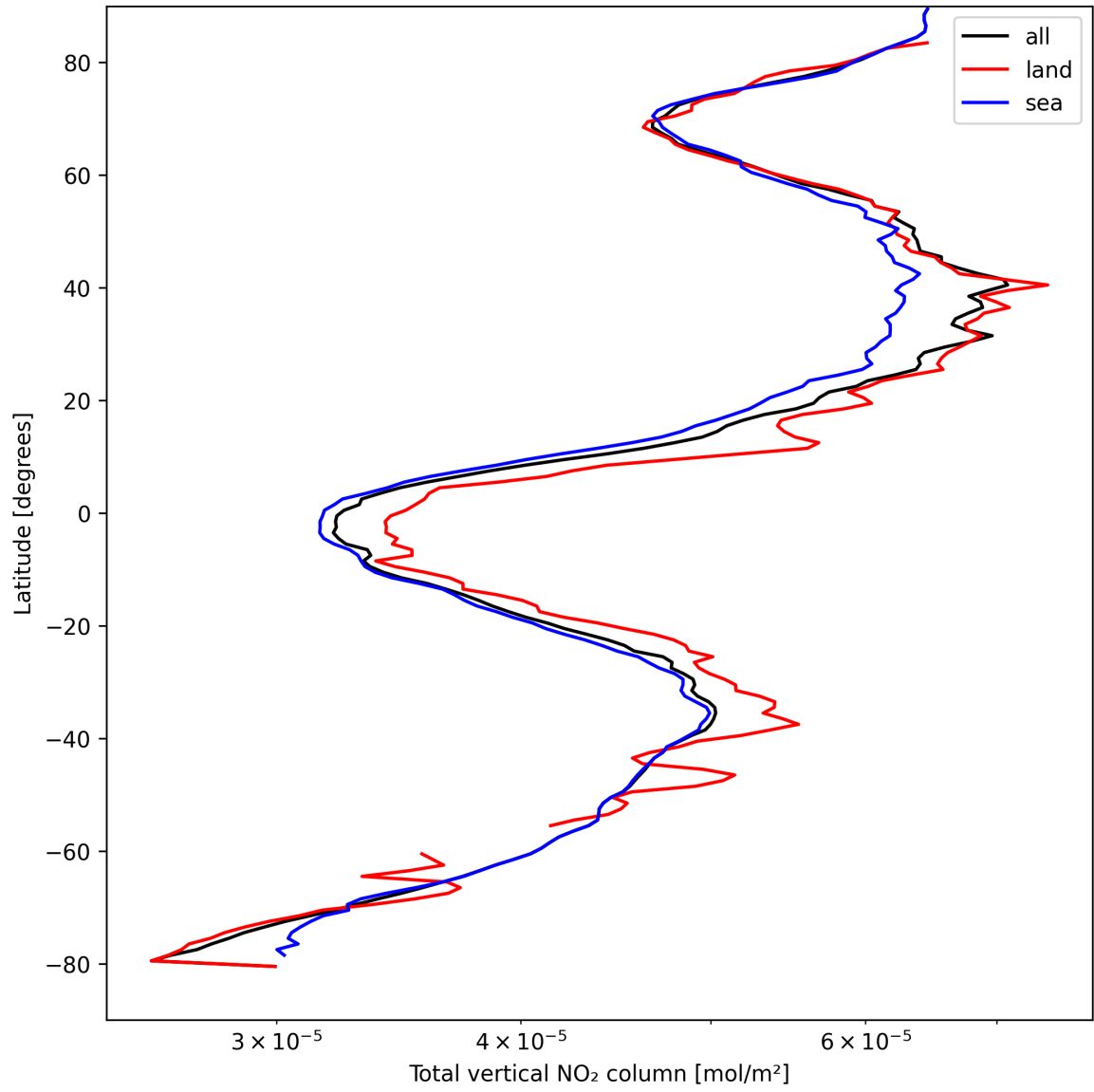
Figure 19: Zonal average of “Total vertical NO 2 column” for 2025-04-10 to 2025-04-11.
