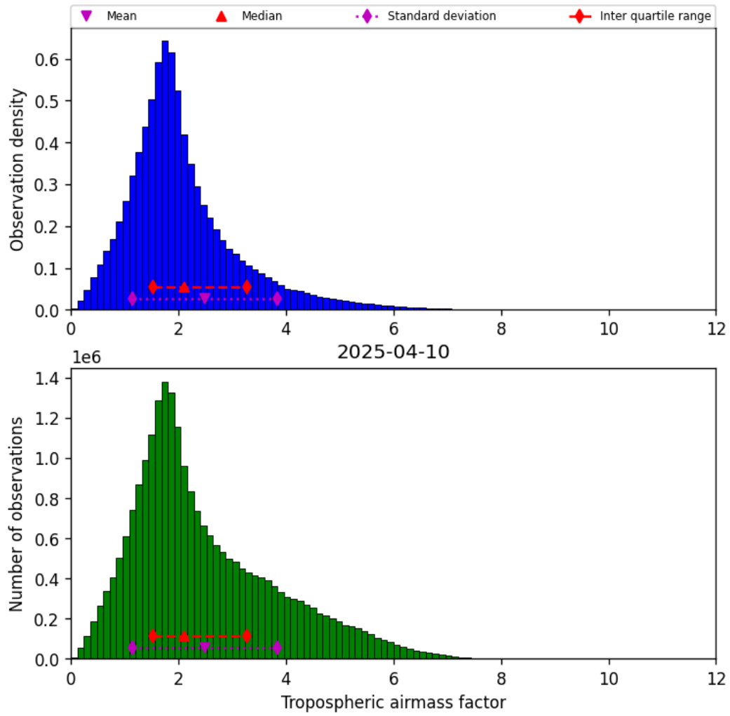
Figure 29: Histogram of “Tropospheric airmass factor” for 2025-04-10 to 2025-04-11
