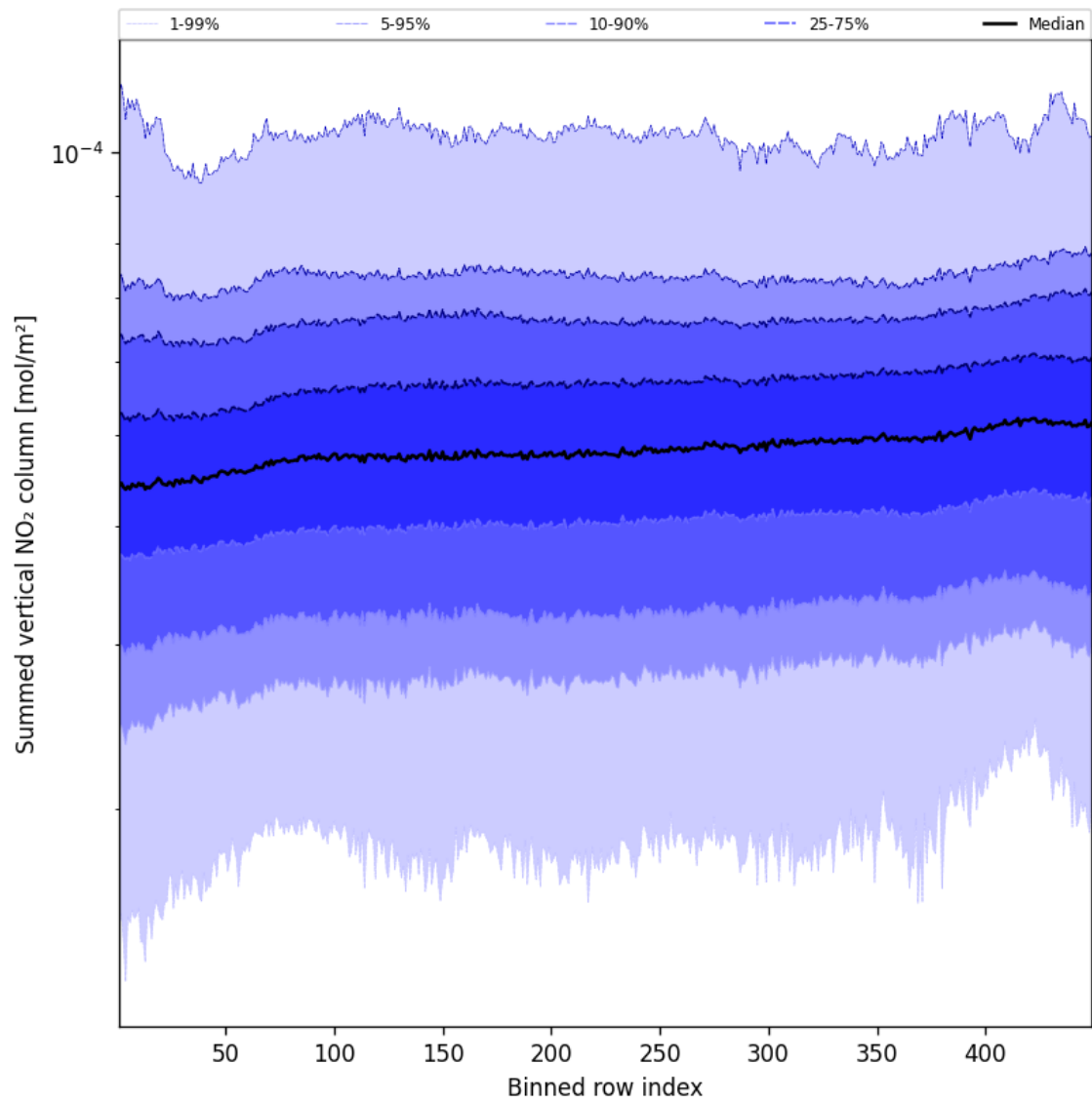
Figure 55: Along track statistics of “Summed vertical NO 2 column” for 2025-04-10 to 2025-04-11
