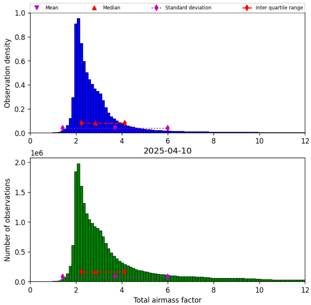
Figure 30: Histogram of “Total airmass factor” for 2025-04-10 to 2025-04-11
