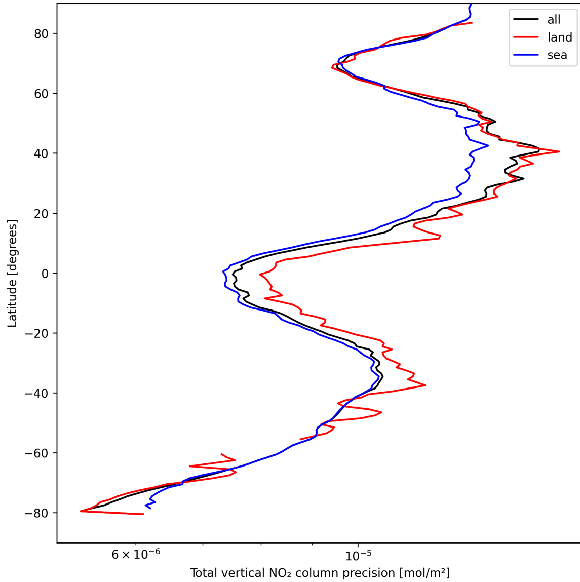
Figure 20: Zonal average of “Total vertical NO 2 column precision” for 2025-04-10 to 2025-04-11.
