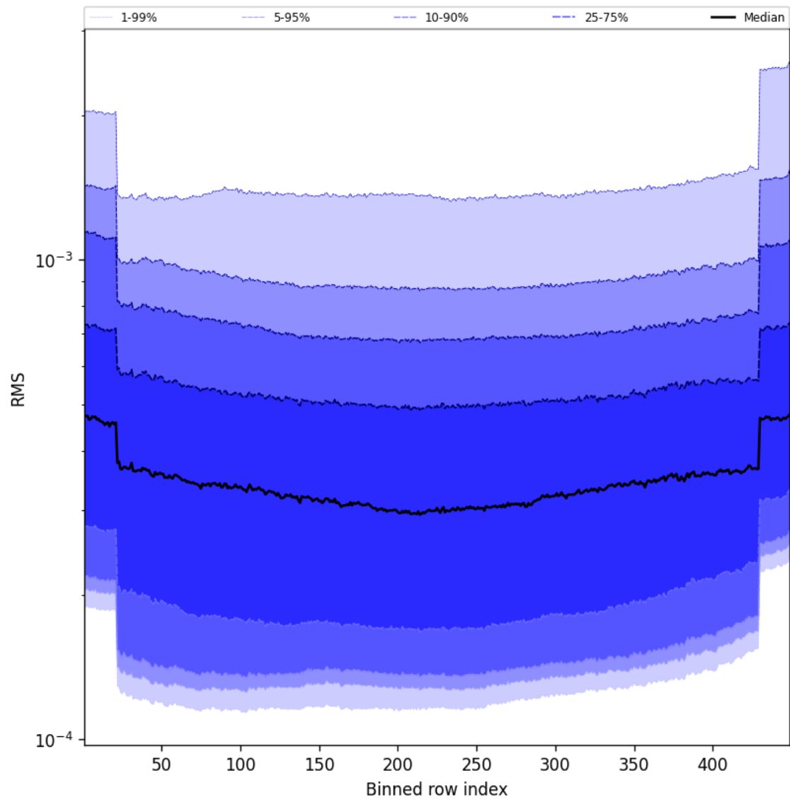
Figure 58: Along track statistics of “RMS” for 2025-04-10 to 2025-04-11
