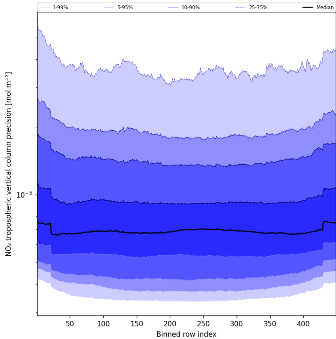
Figure 45: Along track statistics of “NO 2 tropospheric vertical column precision” for 2025-04-10 to 2025-04-11
