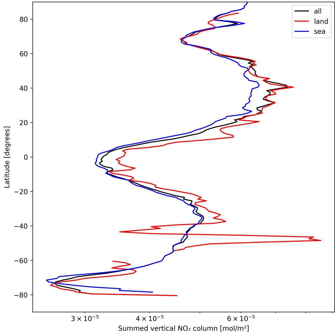
Figure 21: Zonal average of “Summed vertical NO 2 column” for 2025-04-10 to 2025-04-11.
