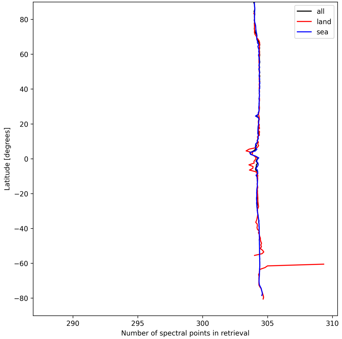
Figure 14: Zonal average of “Number of spectral points in retrieval” for 2025-04-10 to 2025-04-11.
