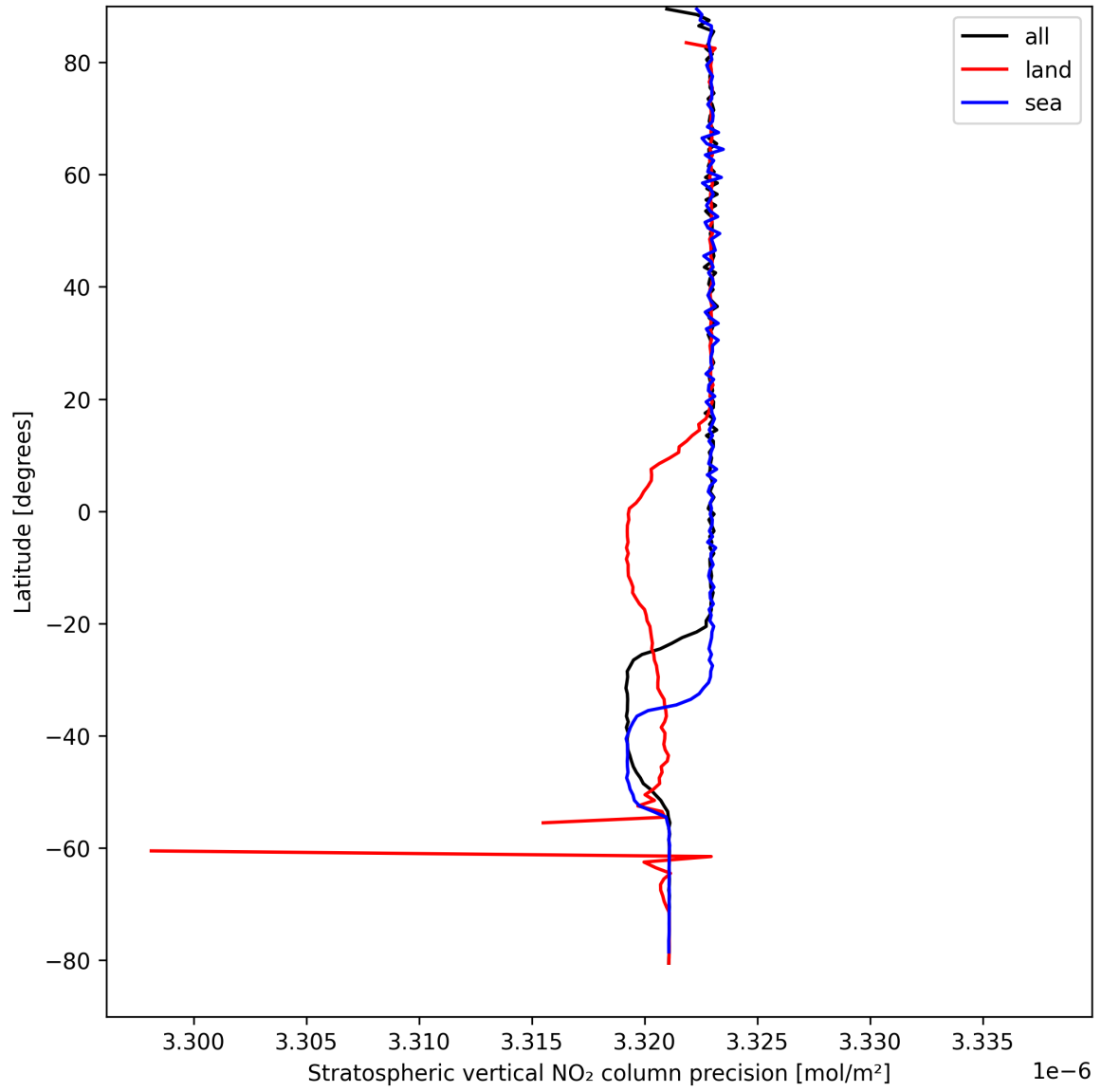
Figure 18: Zonal average of “Stratospheric vertical NO 2 column precision” for 2025-04-10 to 2025-04-11.
