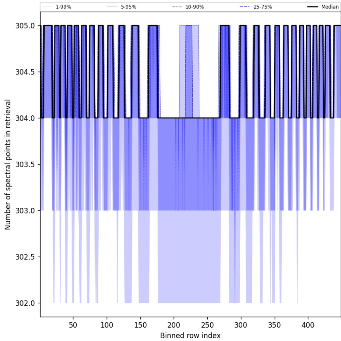
Figure 48: Along track statistics of “Number of spectral points in retrieval” for 2025-04-10 to 2025-04-11
