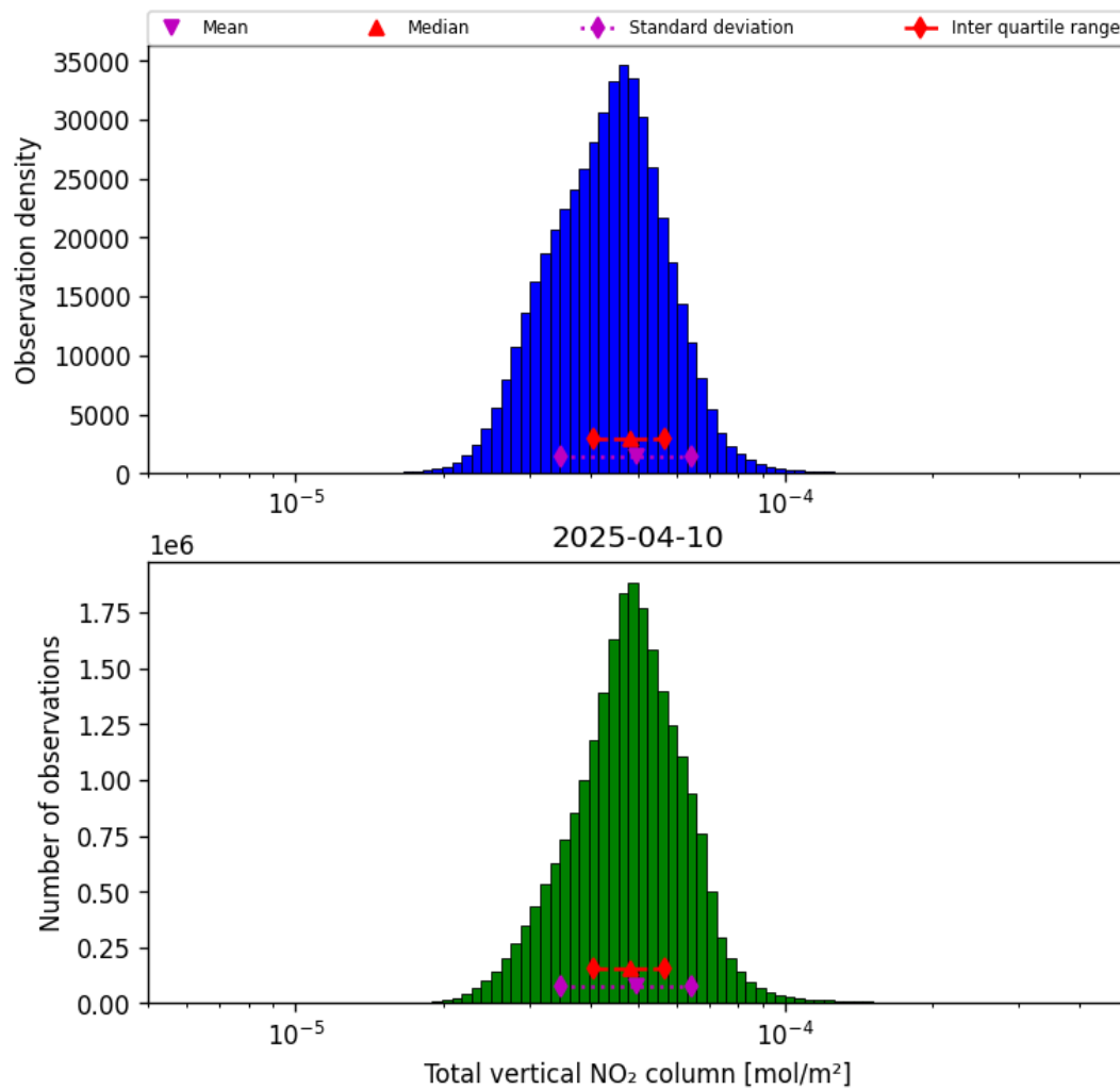
Figure 36: Histogram of "Total vertical NO 2 column" for 2025-04-10 to 2025-04-11
