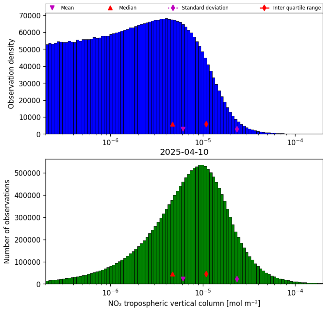
Figure 27: Histogram of “NO 2 tropospheric vertical column” for 2025-04-10 to 2025-04-11
