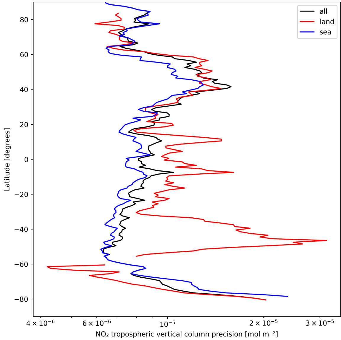
Figure 11: Zonal average of “NO 2 tropospheric vertical column precision” for 2025-04-10 to 2025-04-11.
