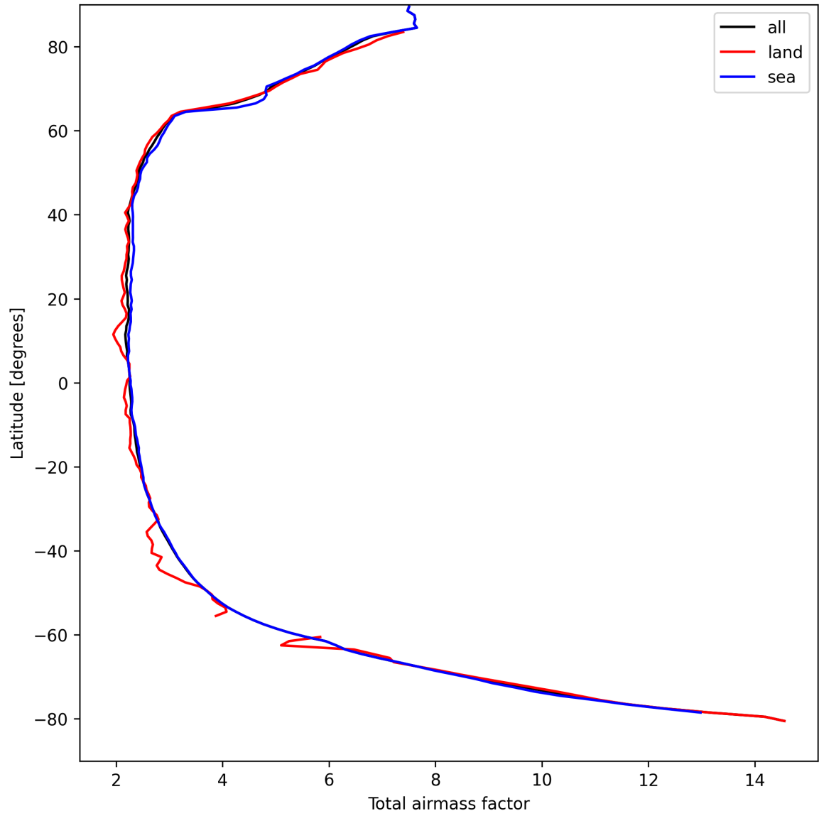
Figure 13: Zonal average of “Total airmass factor” for 2025-04-10 to 2025-04-11.
