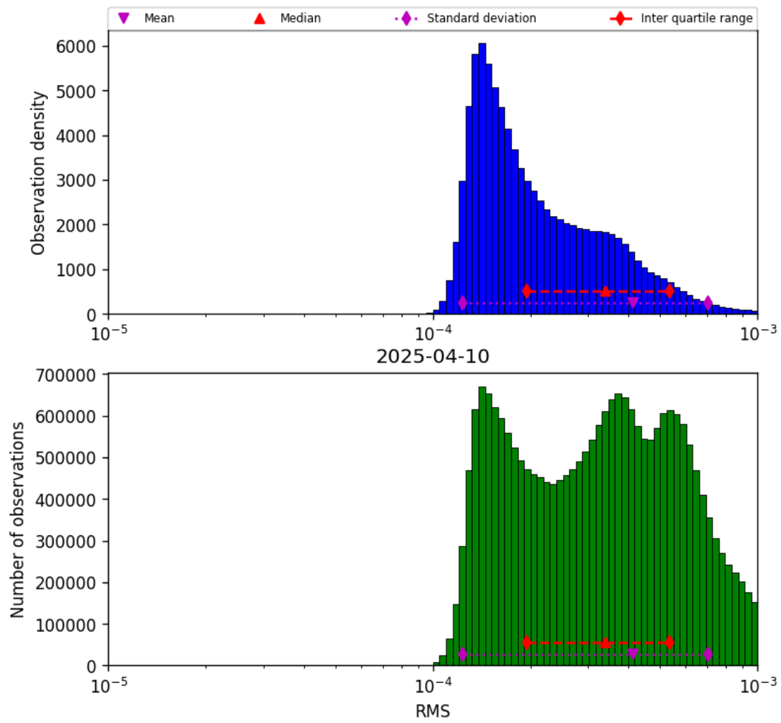
Figure 41: Histogram of “RMS” for 2025-04-10 to 2025-04-11
