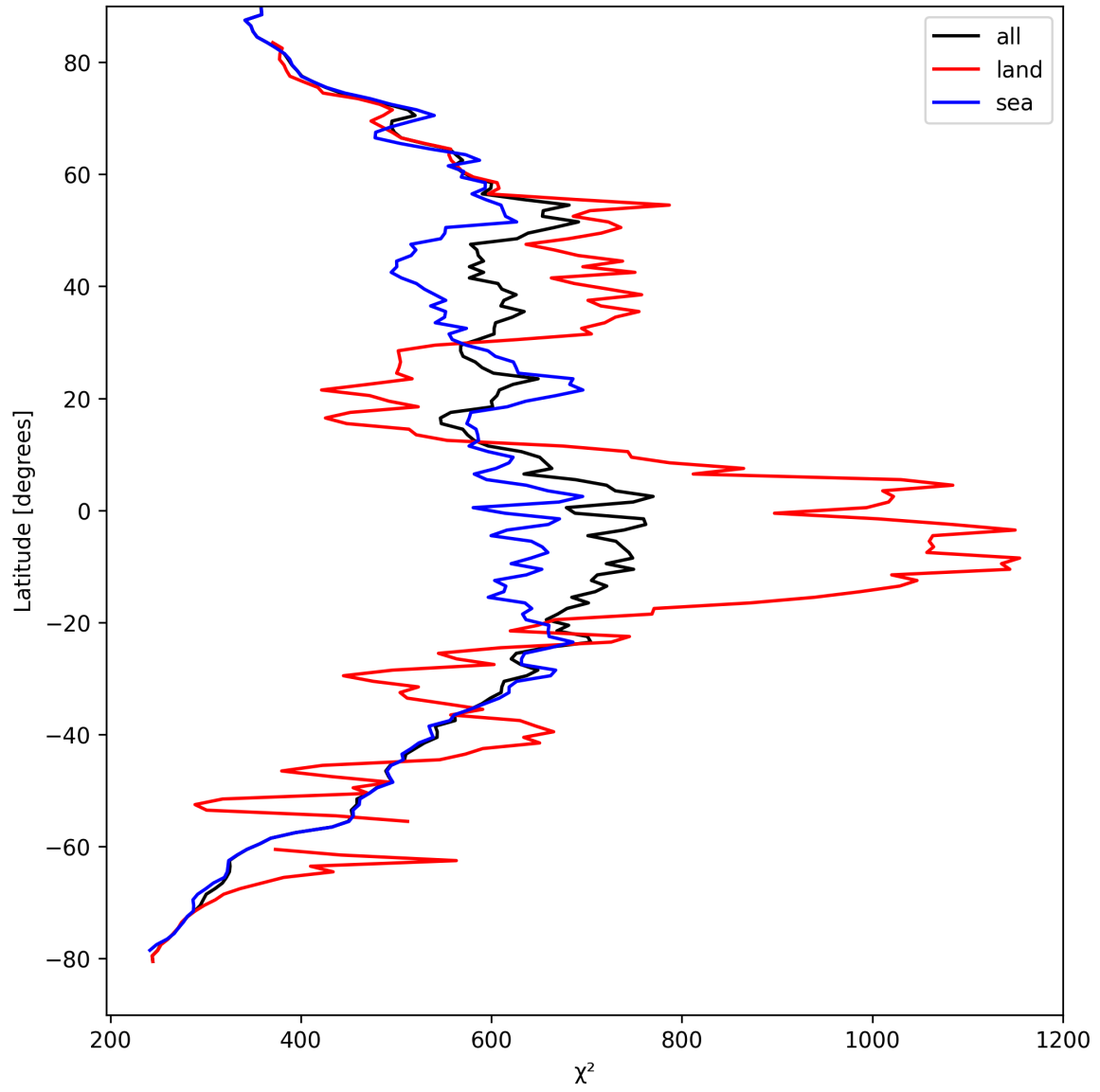
Figure 23: Zonal average of “ \chi^2 ” for 2025-04-10 to 2025-04-11.
