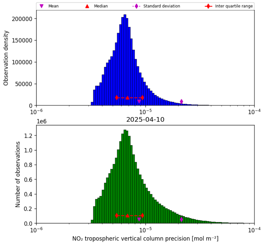
Figure 28: Histogram of “NO 2 tropospheric vertical column precision” for 2025-04-10 to 2025-04-11
