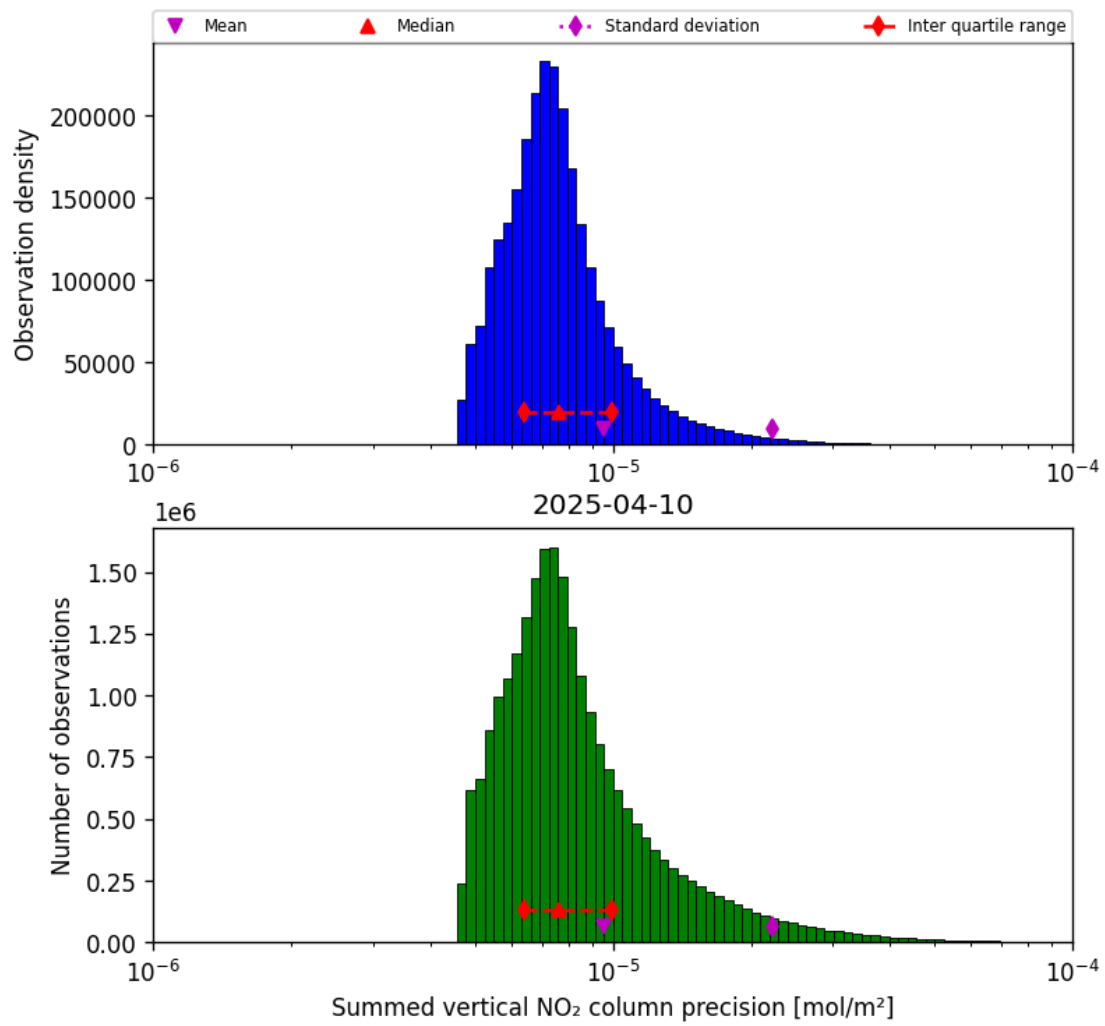
Figure 39: Histogram of “Summed vertical NO 2 column precision” for 2025-04-10 to 2025-04-11
