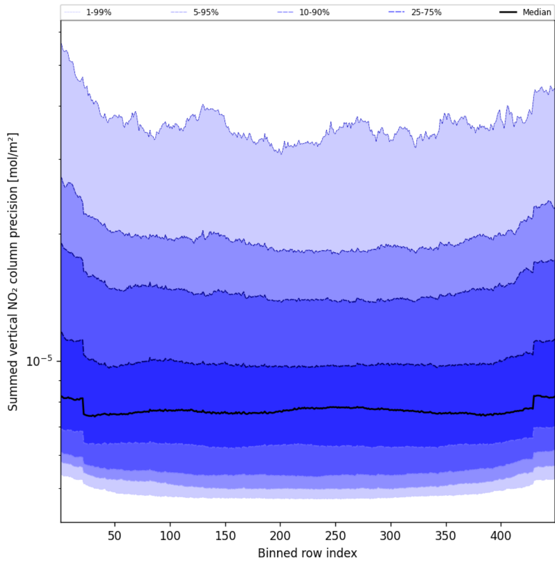
Figure 56: Along track statistics of “Summed vertical NO 2 column precision” for 2025-04-10 to 2025-04-11
