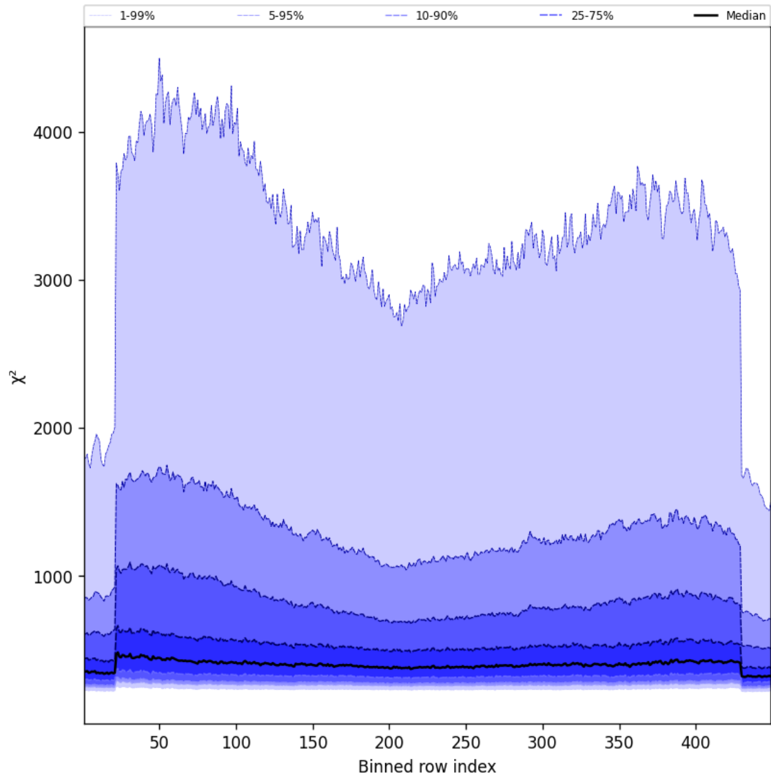
Figure 57: Along track statistics of “ \chi^2 ” for 2025-04-10 to 2025-04-11
