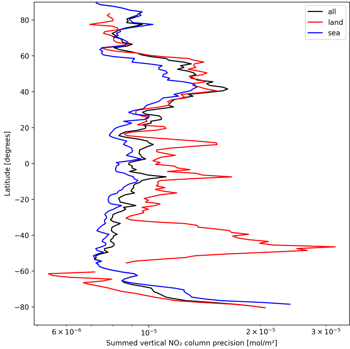
Figure 22: Zonal average of “Summed vertical NO 2 column precision” for 2025-04-10 to 2025-04-11.
