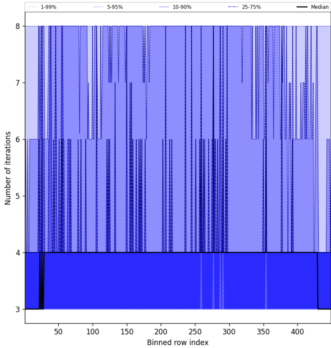
Figure 49: Along track statistics of “Number of iterations” for 2025-04-10 to 2025-04-11
