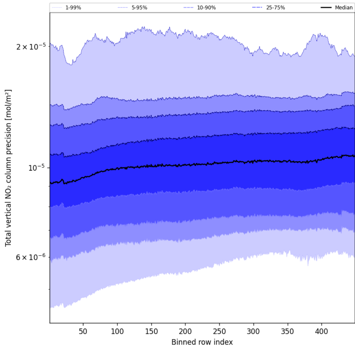
Figure 54: Along track statistics of “Total vertical NO 2 column precision” for 2025-04-10 to 2025-04-11
