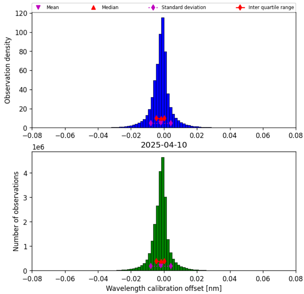
Figure 33: Histogram of “Wavelength calibration offset” for 2025-04-10 to 2025-04-11
