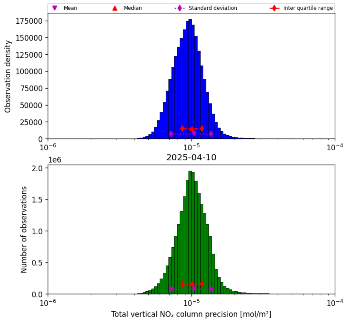
Figure 37: Histogram of “Total vertical NO 2 column precision” for 2025-04-10 to 2025-04-11
