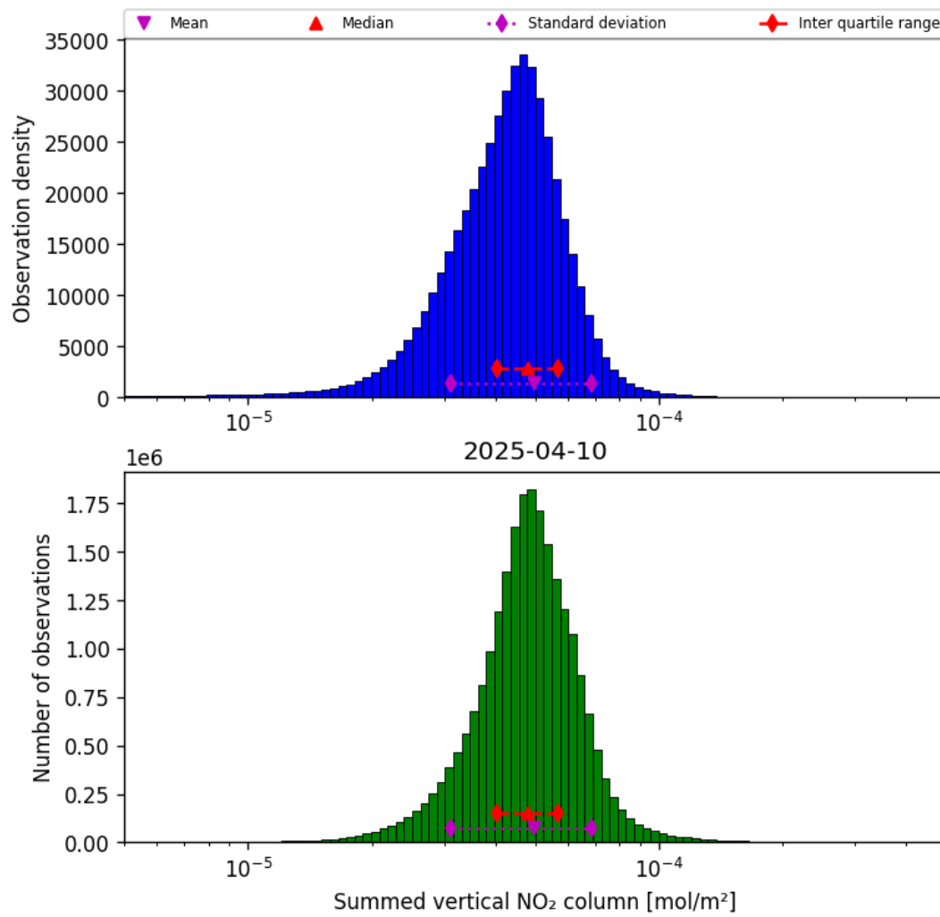
Figure 38: Histogram of “Summed vertical NO 2 column” for 2025-04-10 to 2025-04-11
