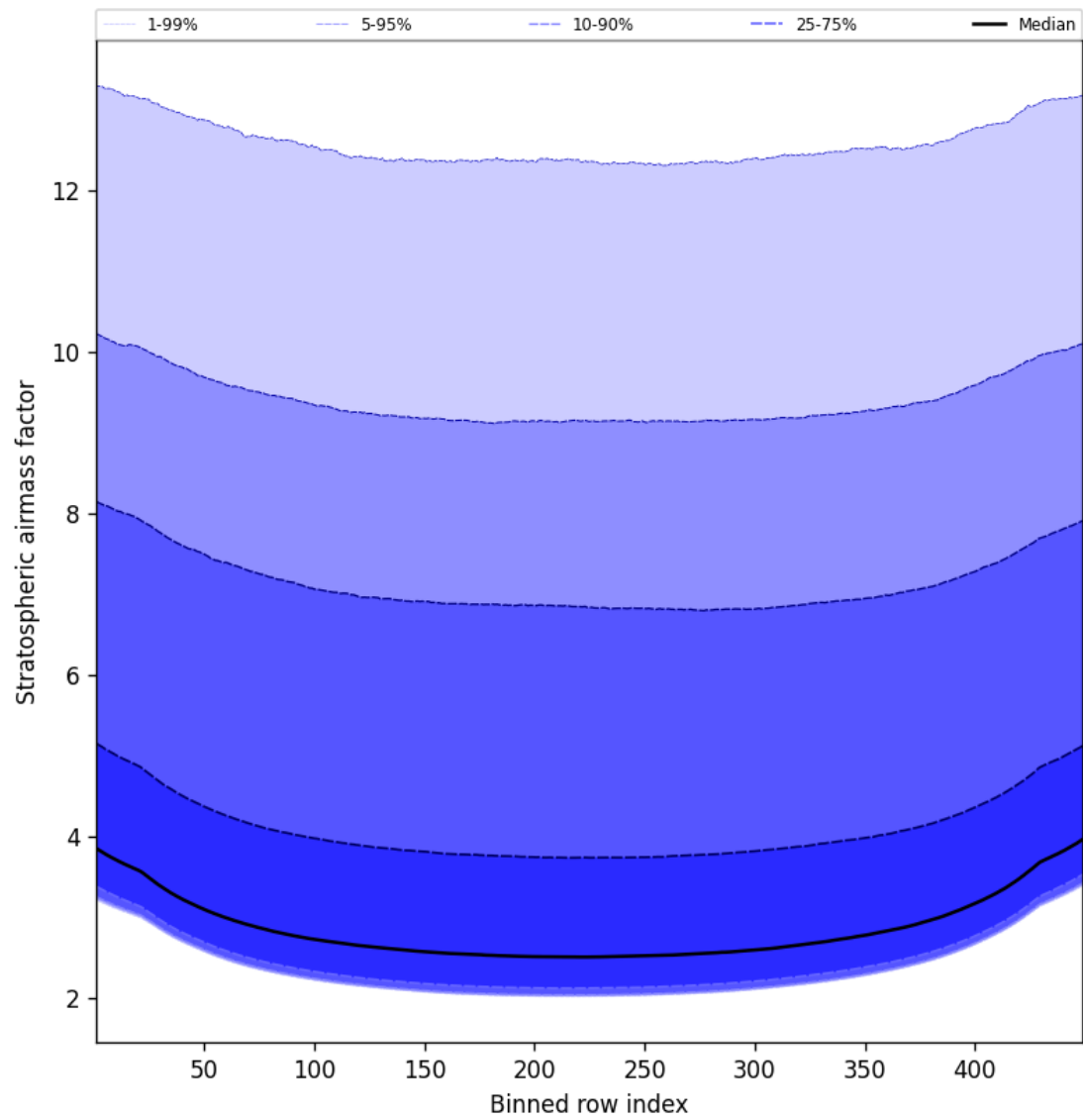
Figure 59: Along track statistics of “Stratospheric airmass factor” for 2025-04-10 to 2025-04-11
