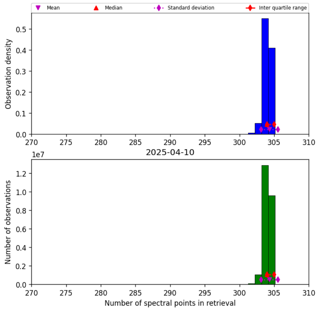
Figure 31: Histogram of “Number of spectral points in retrieval” for 2025-04-10 to 2025-04-11
