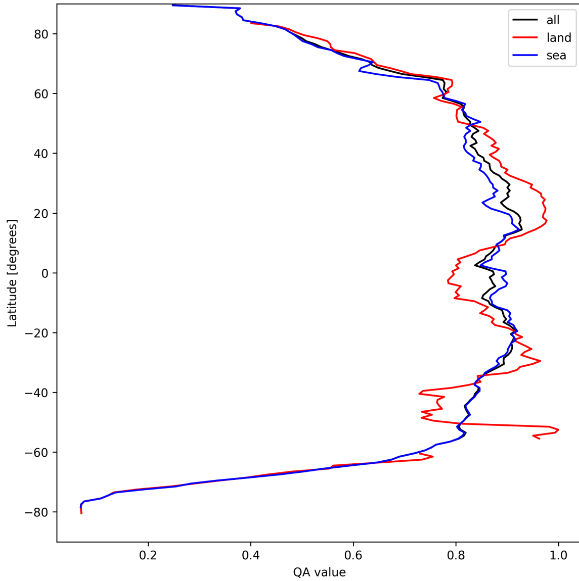
Figure 9: Zonal average of “QA value” for 2025-04-10 to 2025-04-11.
