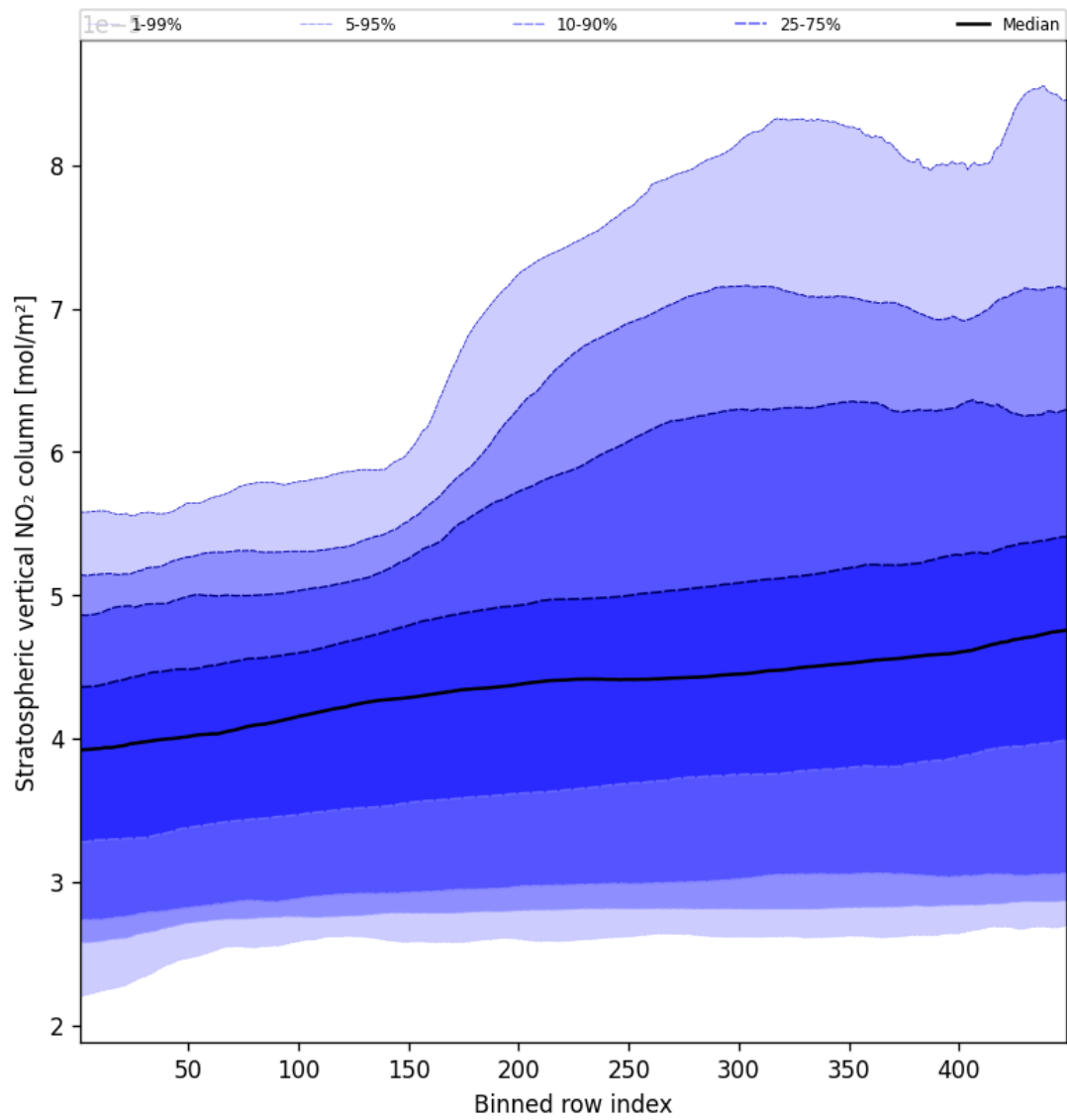
Figure 51: Along track statistics of “Stratospheric vertical NO 2 column” for 2025-04-10 to 2025-04-11
