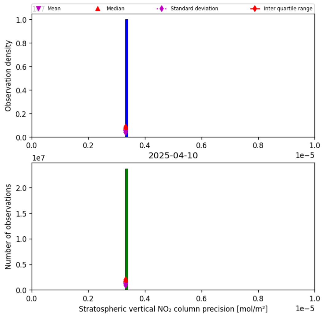
Figure 35: Histogram of “Stratospheric vertical NO 2 column precision” for 2025-04-10 to 2025-04-11
