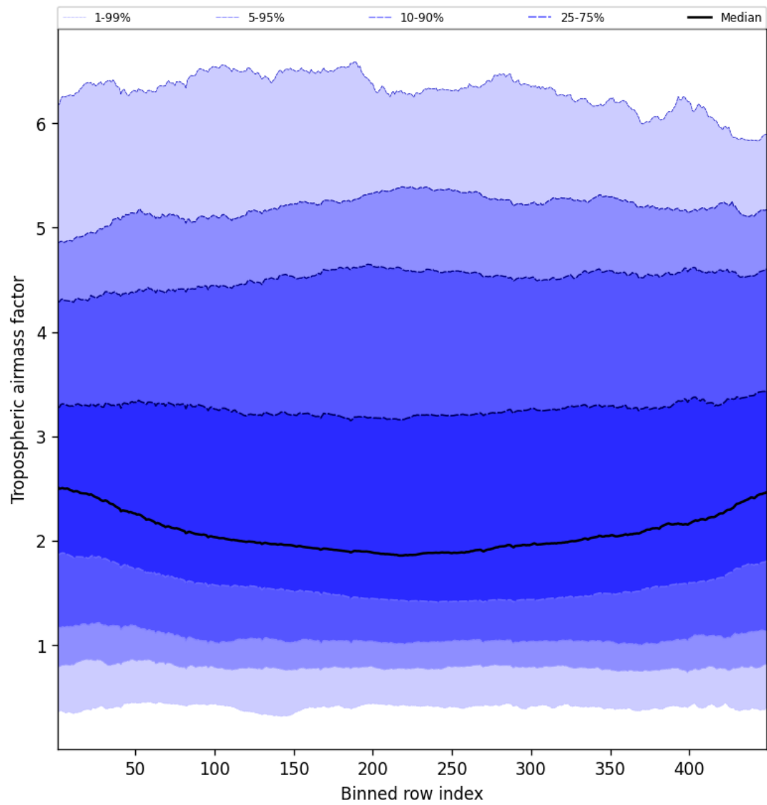
Figure 46: Along track statistics of “Tropospheric airmass factor” for 2025-04-10 to 2025-04-11
