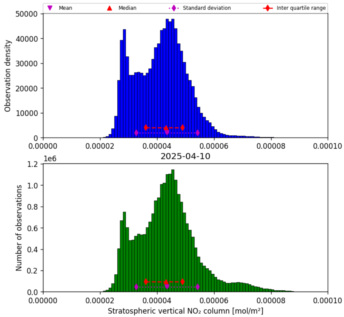
Figure 34: Histogram of “Stratospheric vertical NO 2 column” for 2025-04-10 to 2025-04-11
