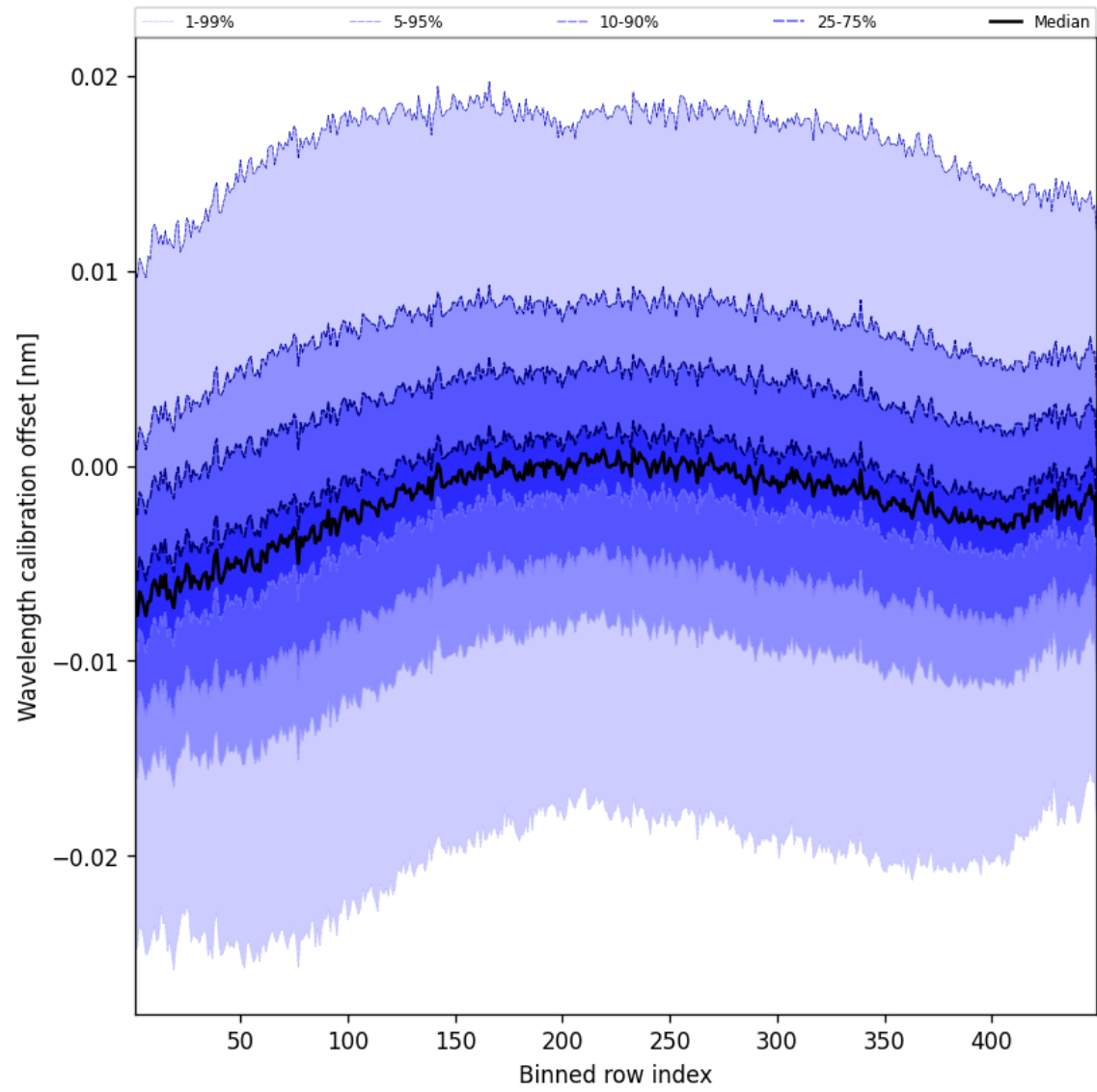
Figure 50: Along track statistics of “Wavelength calibration offset” for 2025-04-10 to 2025-04-11
