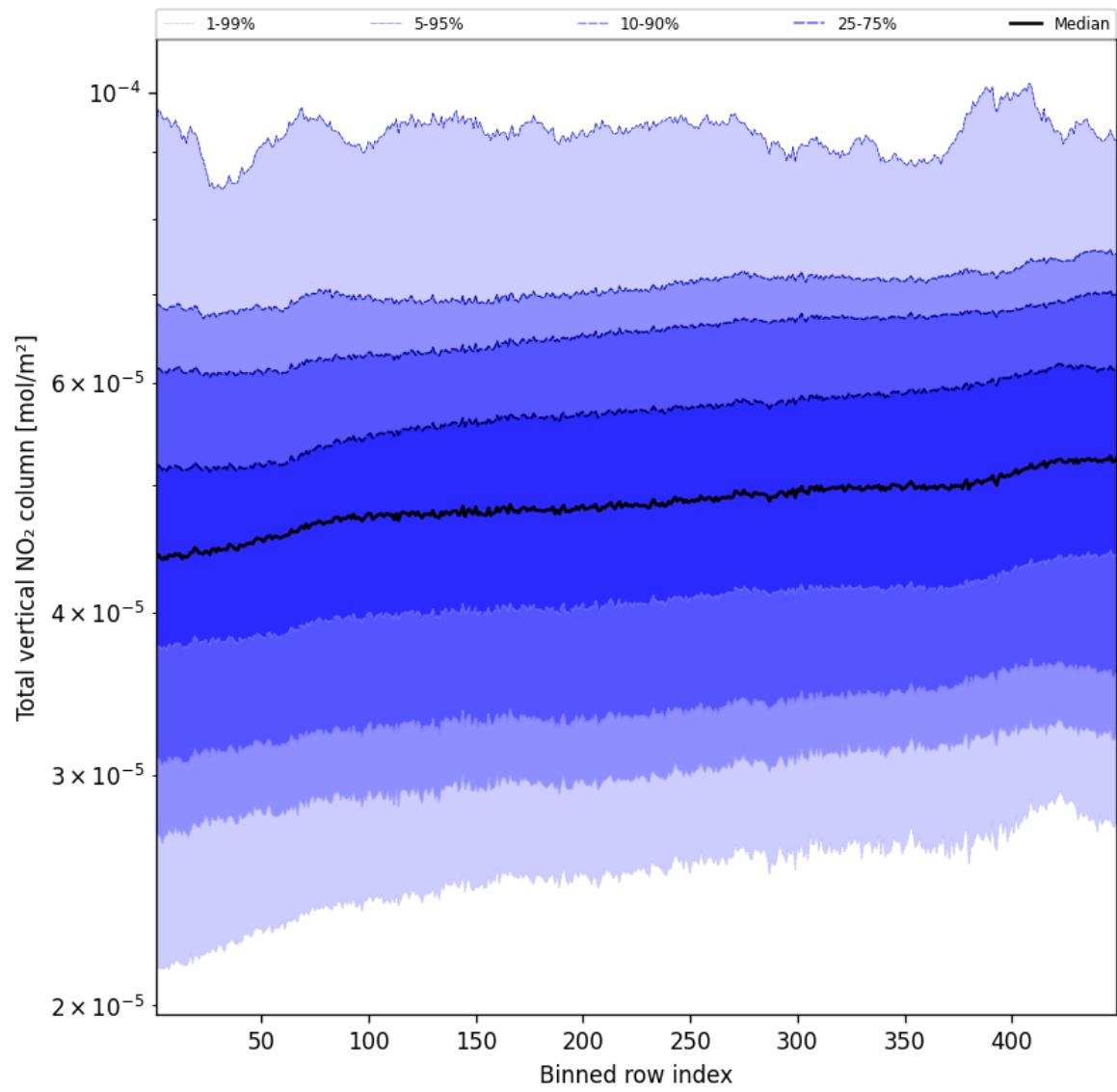
Figure 53: Along track statistics of “Total vertical NO 2 column” for 2025-04-10 to 2025-04-11
