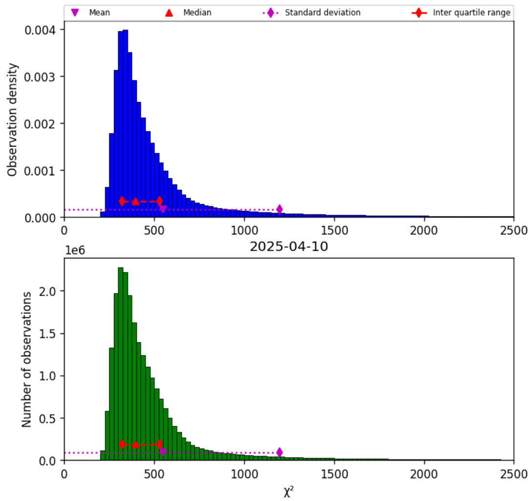
Figure 40: Histogram of “ \chi^2 ” for 2025-04-10 to 2025-04-11
