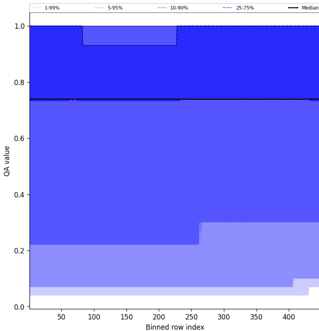
Figure 43: Along track statistics of “QA value” for 2025-04-10 to 2025-04-11
