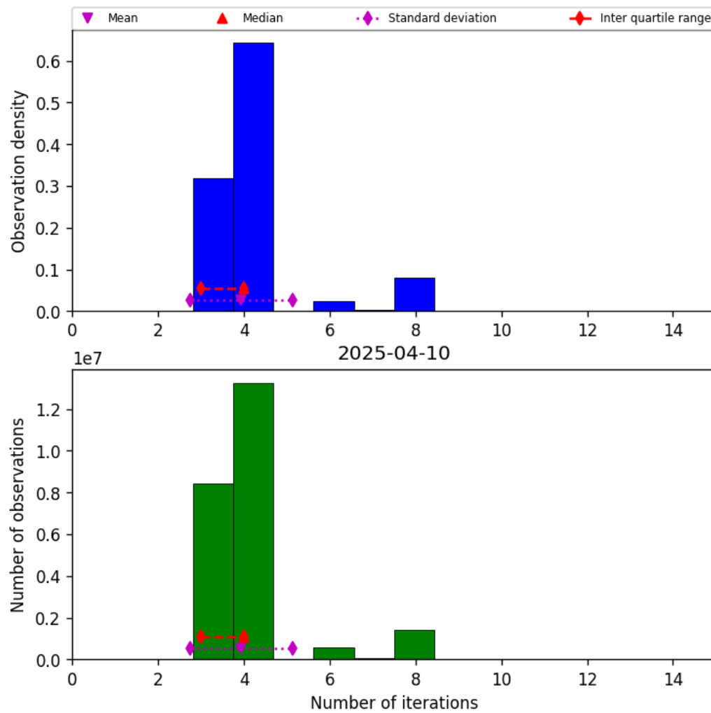
Figure 32: Histogram of “Number of iterations” for 2025-04-10 to 2025-04-11
