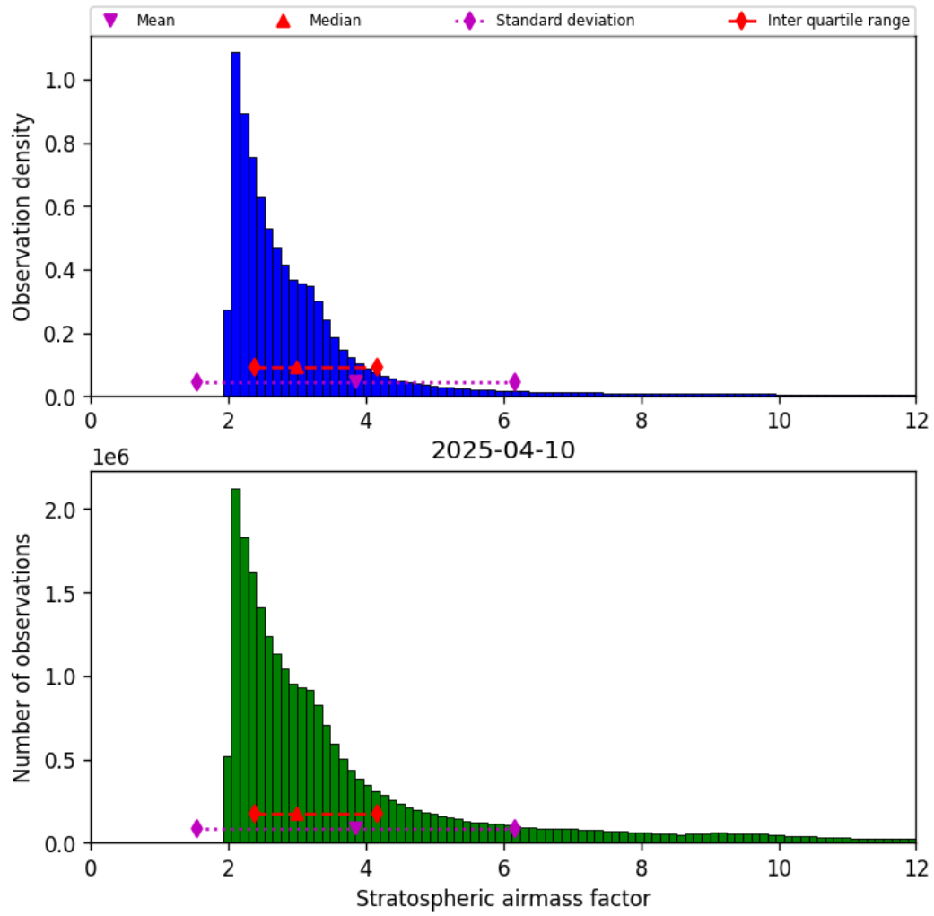
Figure 42: Histogram of “Stratospheric airmass factor” for 2025-04-10 to 2025-04-11
