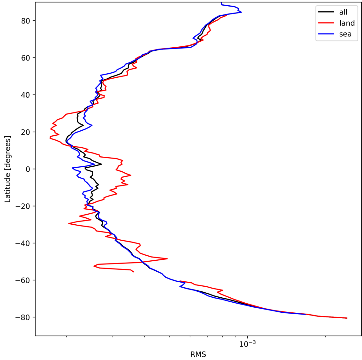
Figure 24: Zonal average of “RMS” for 2025-04-10 to 2025-04-11.
