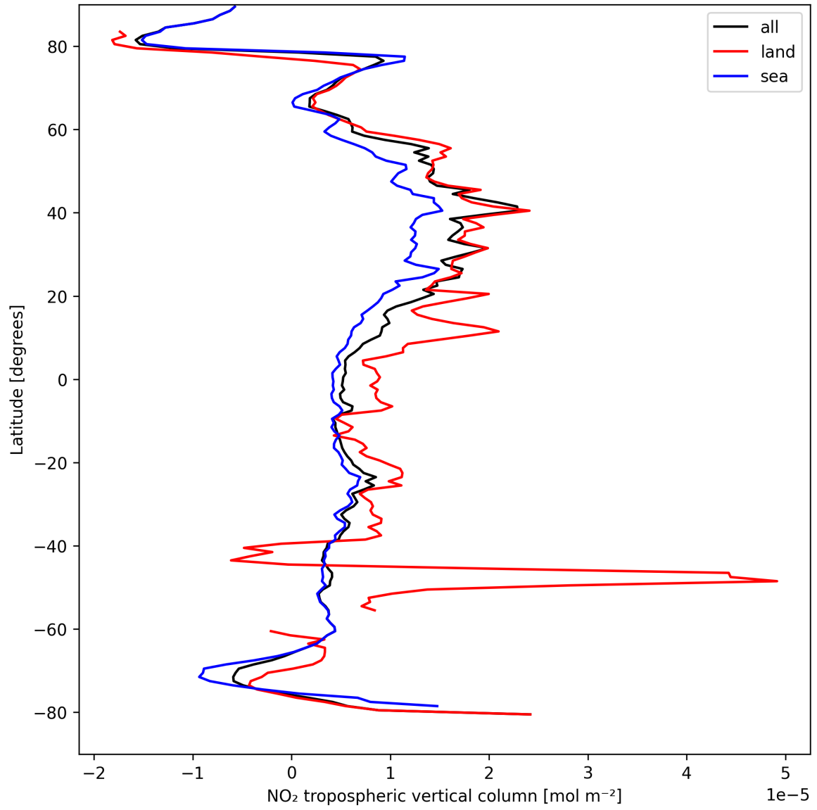
Figure 10: Zonal average of “NO 2 tropospheric vertical column” for 2025-04-10 to 2025-04-11.
