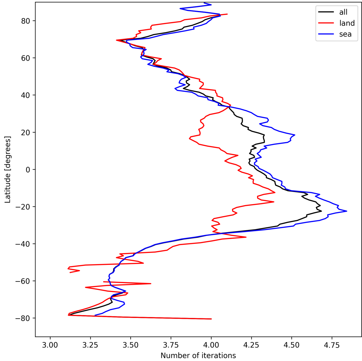
Figure 15: Zonal average of “Number of iterations” for 2025-04-10 to 2025-04-11.
