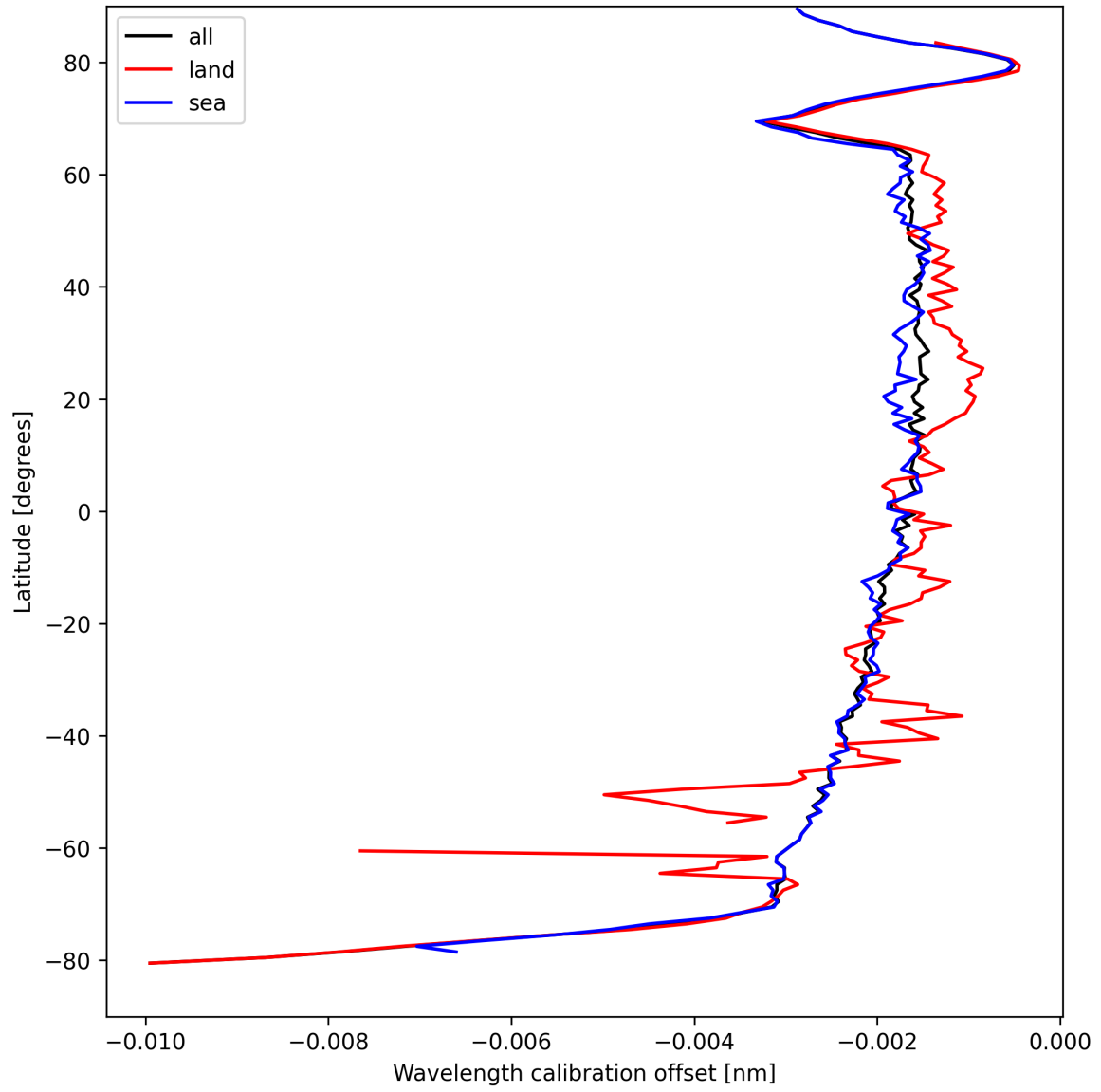
Figure 16: Zonal average of “Wavelength calibration offset” for 2025-04-10 to 2025-04-11.
