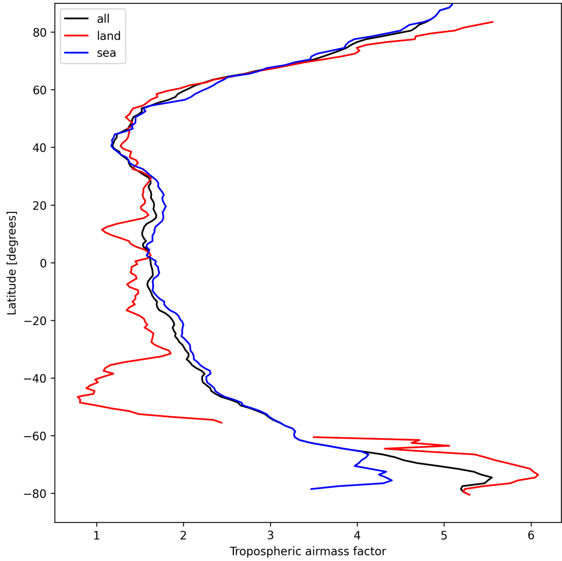
Figure 12: Zonal average of “Tropospheric air mass factor” for 2025-04-10 to 2025-04-11.
