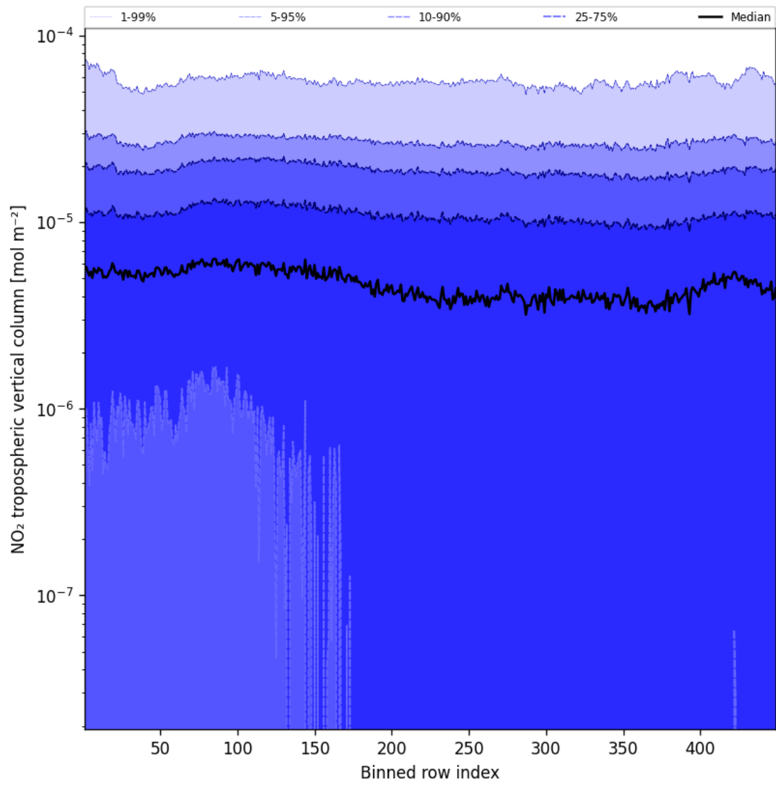
Figure 44: Along track statistics of “NO 2 tropospheric vertical column” for 2025-04-10 to 2025-04-11
