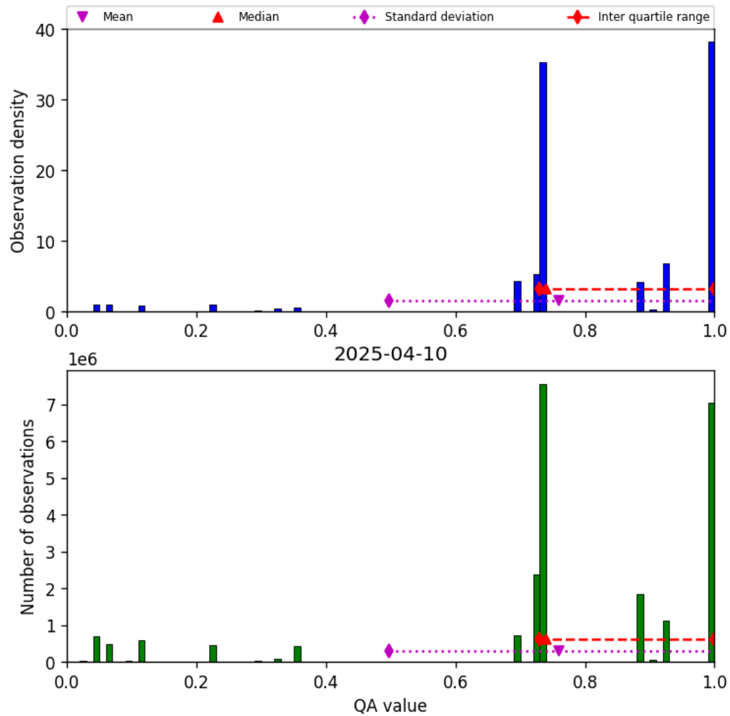
Figure 26: Histogram of “QA value” for 2025-04-10 to 2025-04-11
