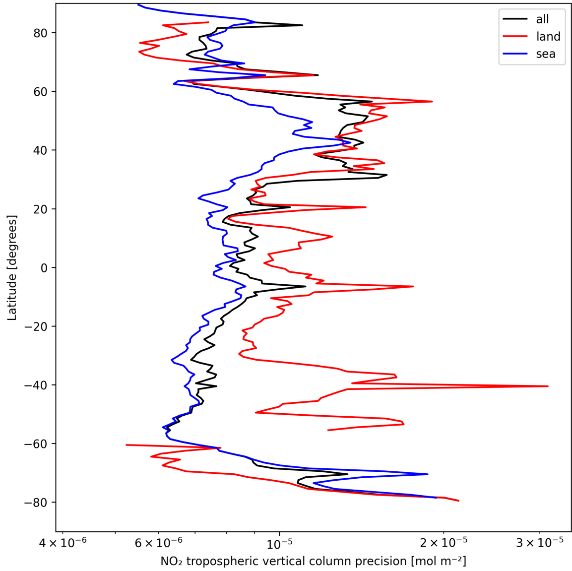
Figure 11: Zonal average of “NO 2 tropospheric vertical column precision” for 2025-04-11 to 2025-04-11.
