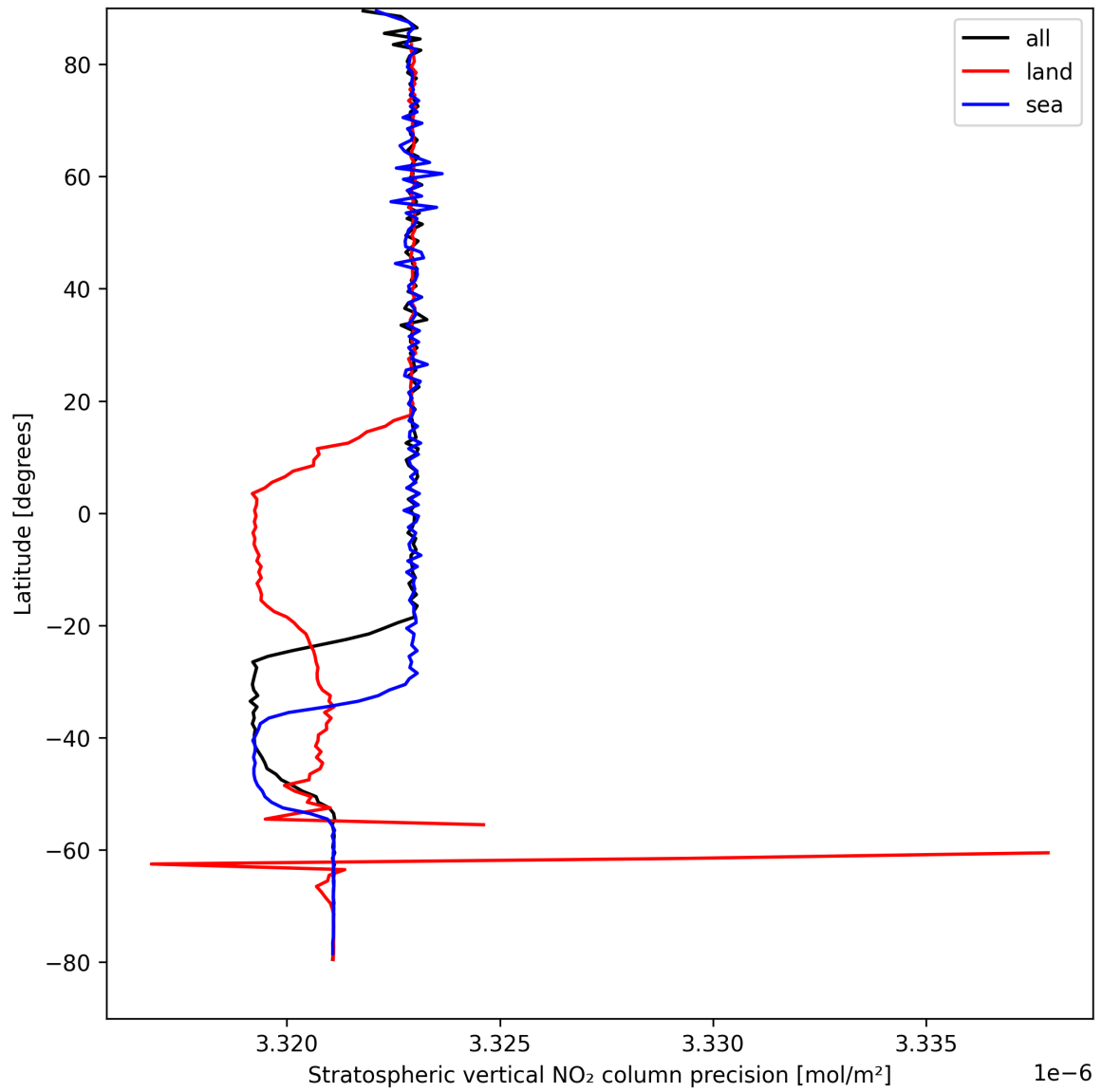
Figure 18: Zonal average of “Stratospheric vertical NO 2 column precision” for 2025-04-11 to 2025-04-11.
