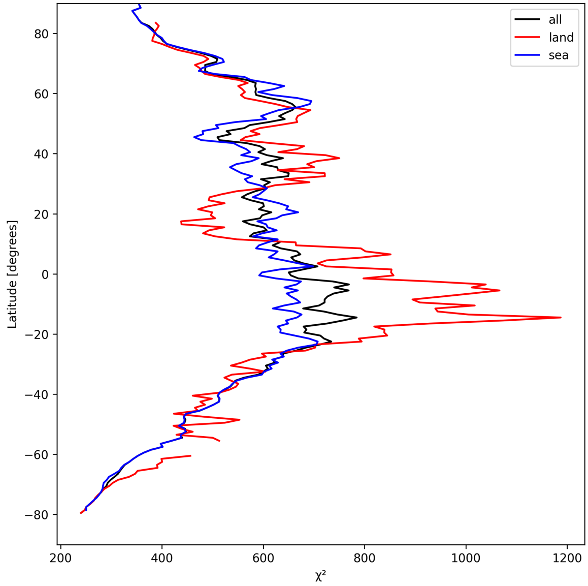
Figure 23: Zonal average of “ \chi^2 ” for 2025-04-11 to 2025-04-11.
