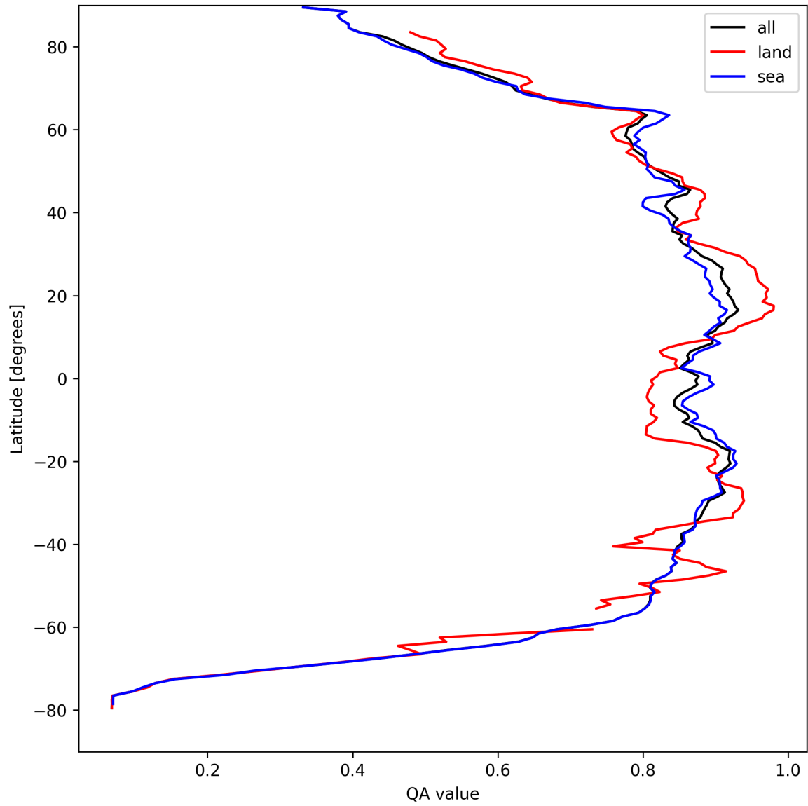
Figure 9: Zonal average of “QA value” for 2025-04-11 to 2025-04-11.
