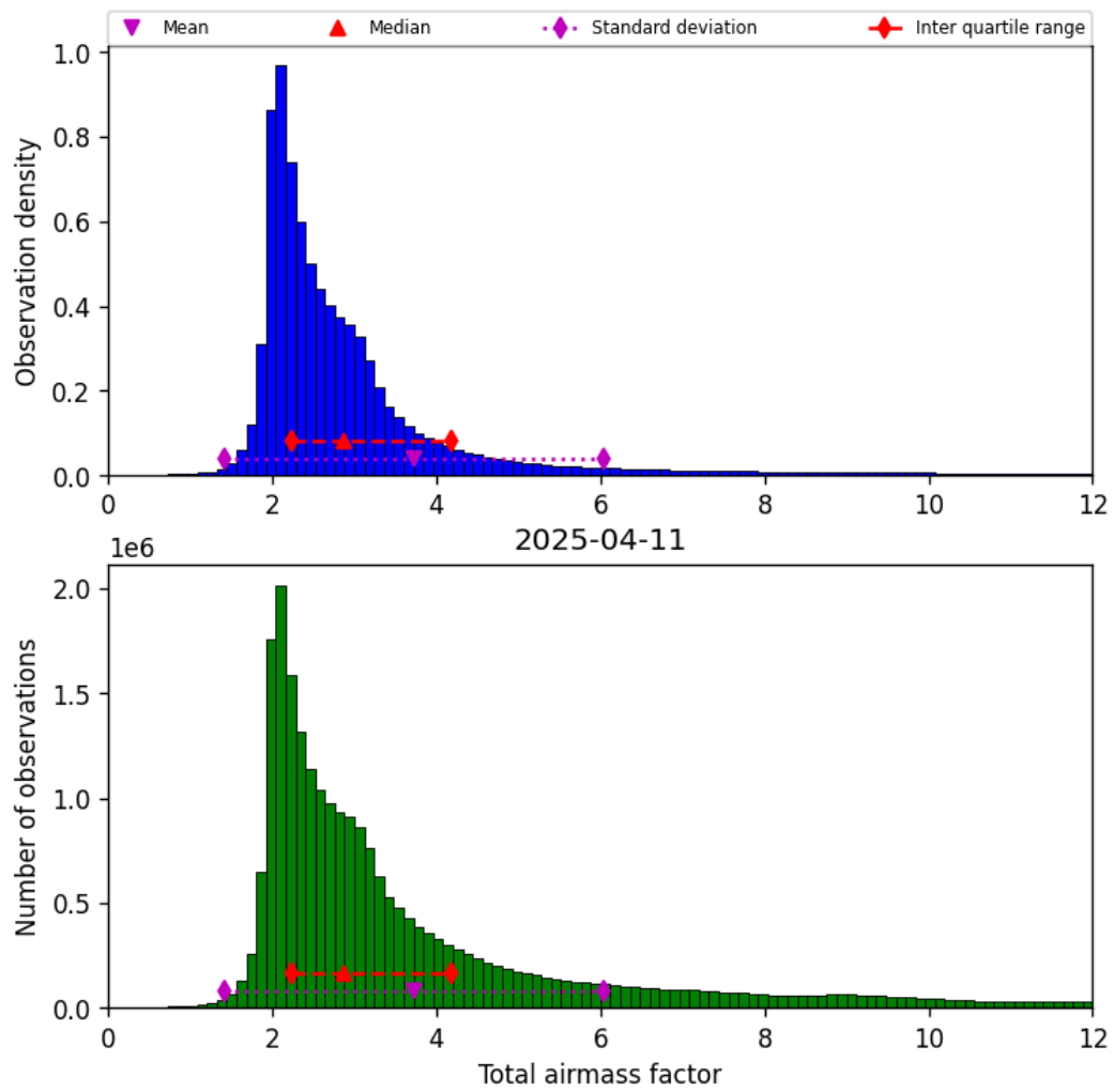
Figure 30: Histogram of “Total airmass factor” for 2025-04-11 to 2025-04-11
