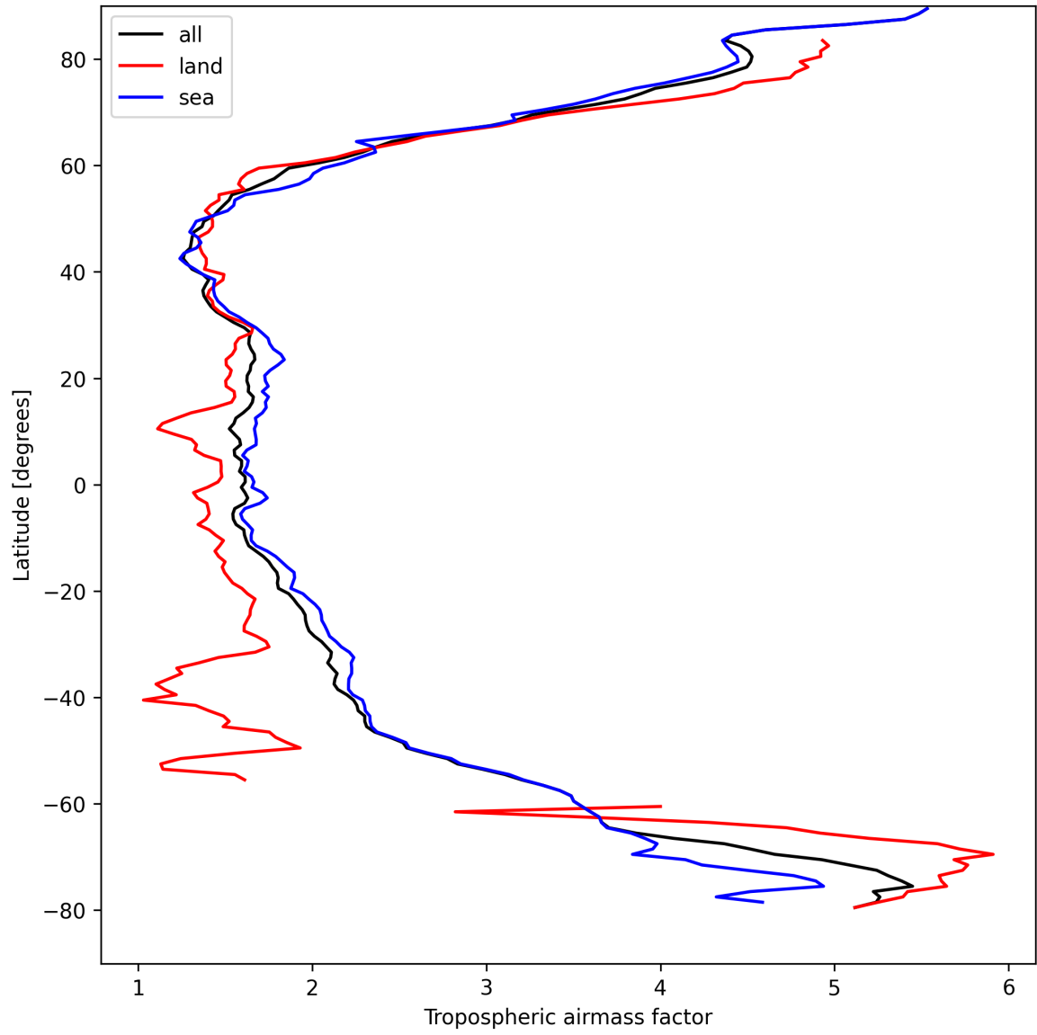
Figure 12: Zonal average of “Tropospheric airmass factor” for 2025-04-11 to 2025-04-11.
