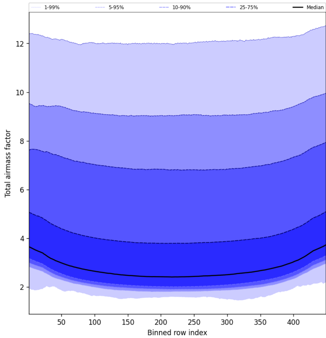
Figure 47: Along track statistics of “Total airmass factor” for 2025-04-11 to 2025-04-11
