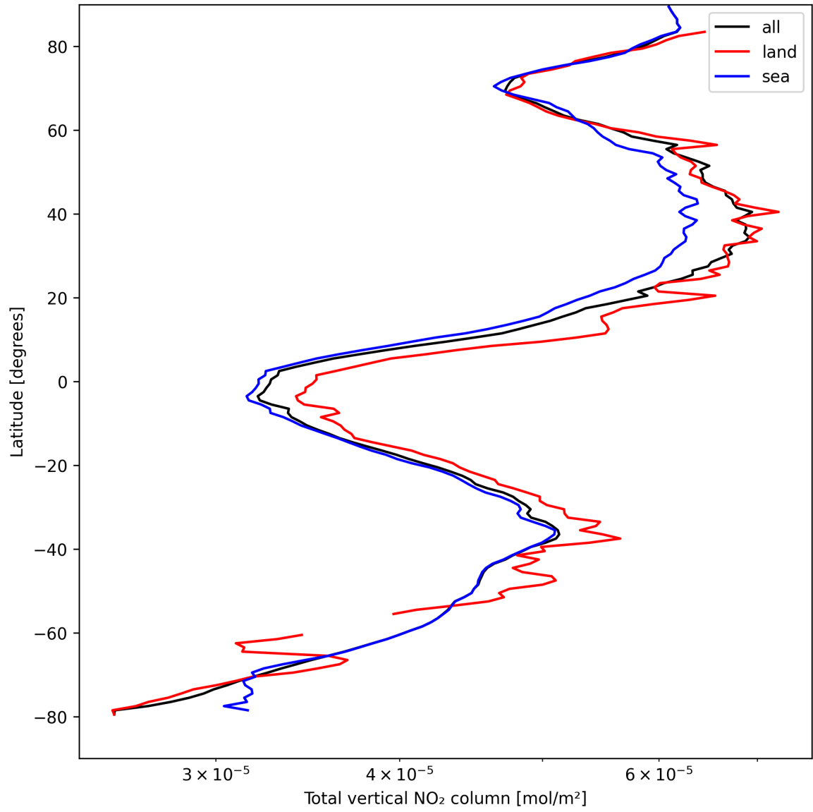
Figure 19: Zonal average of “Total vertical NO 2 column” for 2025-04-11 to 2025-04-11.
