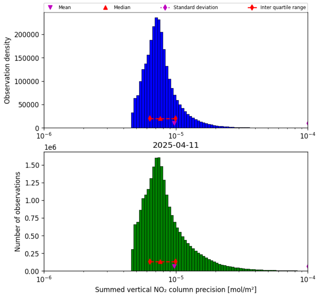
Figure 39: Histogram of “Summed vertical NO 2 column precision” for 2025-04-11 to 2025-04-11
