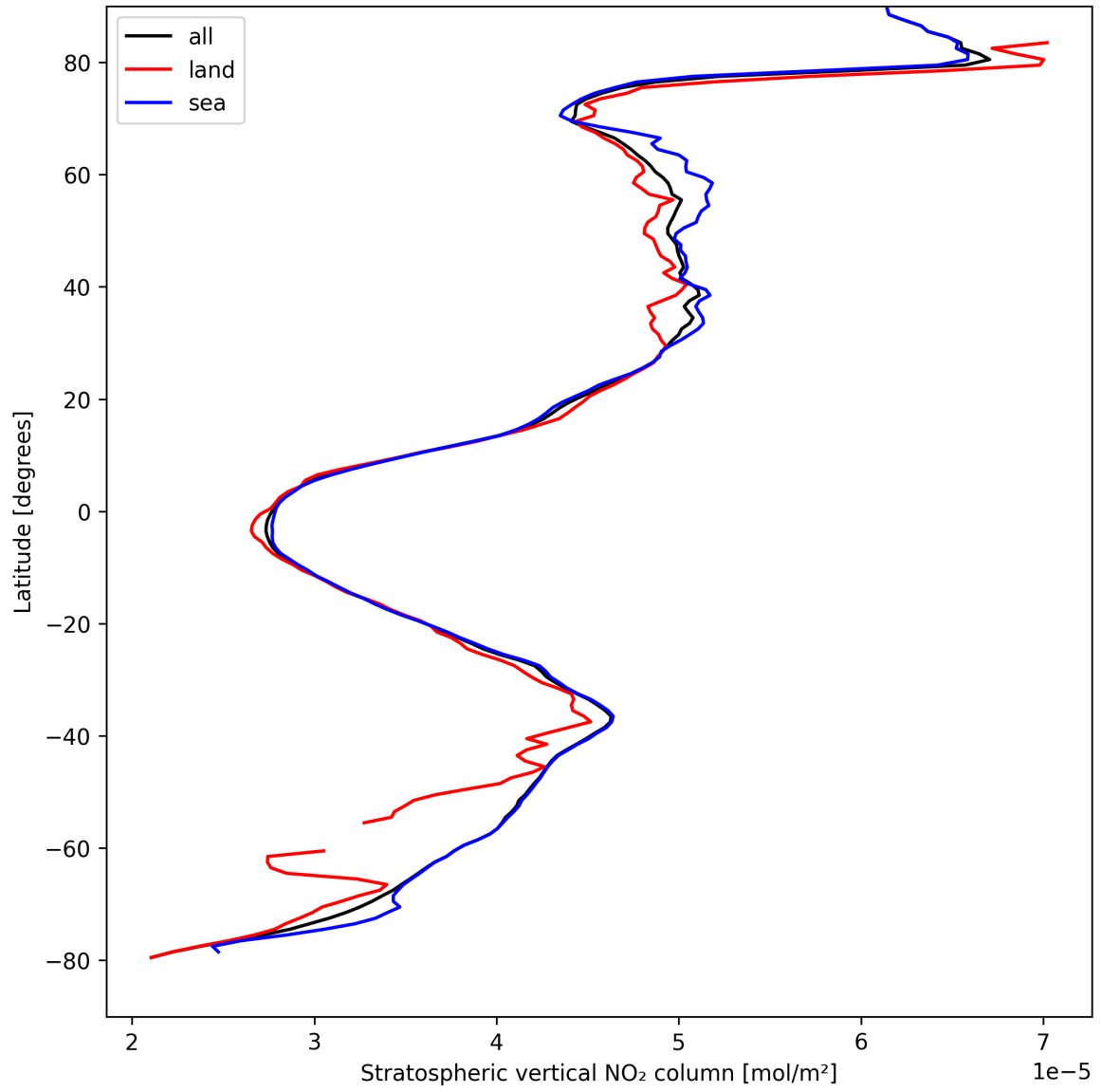
Figure 17: Zonal average of “Stratospheric vertical NO 2 column” for 2025-04-11 to 2025-04-11.
