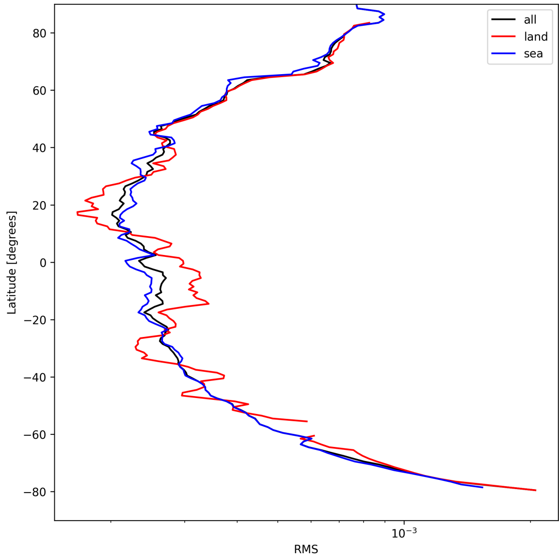
Figure 24: Zonal average of “RMS” for 2025-04-11 to 2025-04-11.
