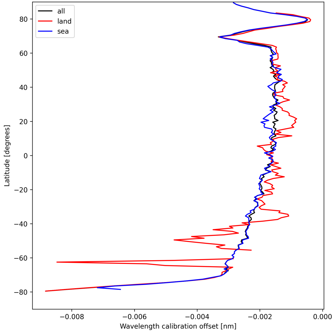
Figure 16: Zonal average of “Wavelength calibration offset” for 2025-04-11 to 2025-04-11.
