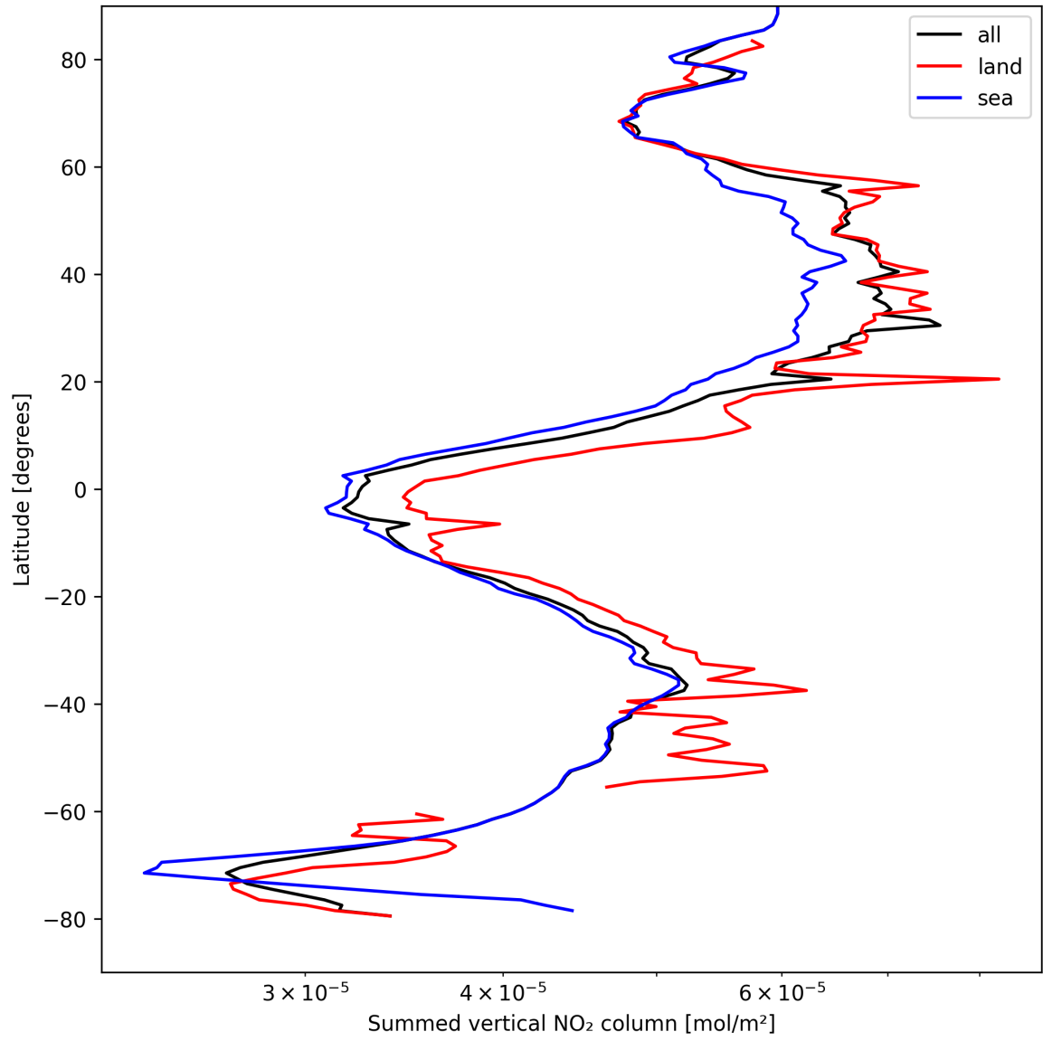
Figure 21: Zonal average of “Summed vertical NO 2 column” for 2025-04-11 to 2025-04-11.
