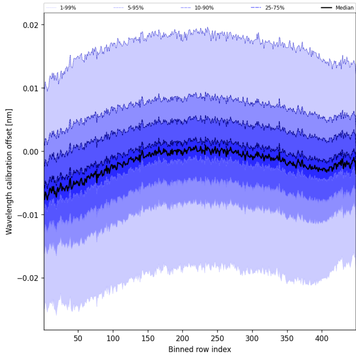
Figure 50: Along track statistics of “Wavelength calibration offset” for 2025-04-11 to 2025-04-11
