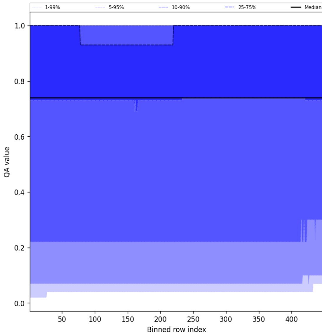
Figure 43: Along track statistics of "QA value" for 2025-04-11 to 2025-04-11
