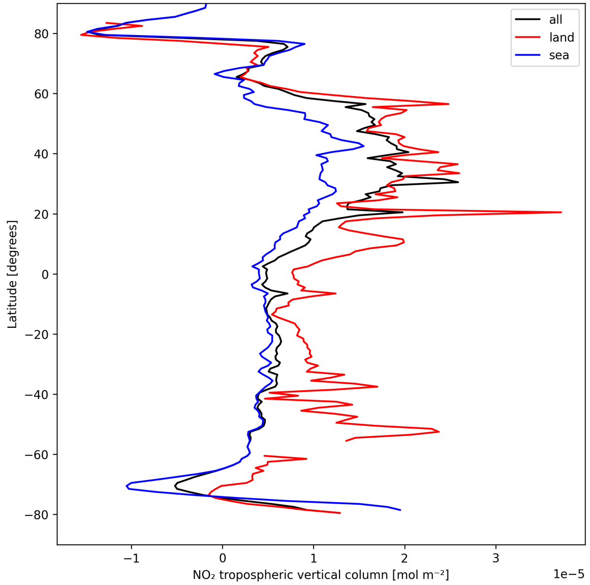
Figure 10: Zonal average of “NO 2 tropospheric vertical column” for 2025-04-11 to 2025-04-11.
