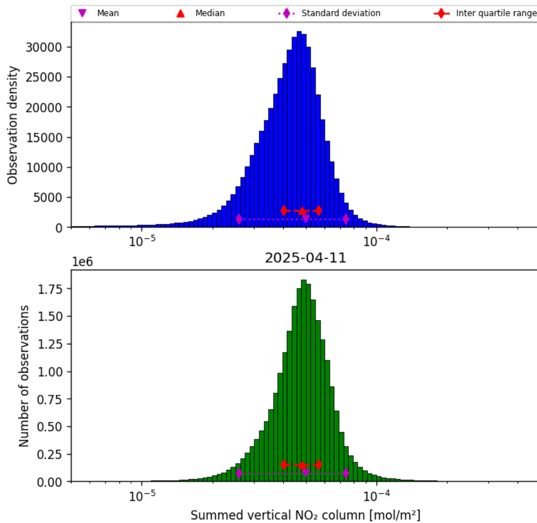
Figure 38: Histogram of "Summed vertical NO 2 column" for 2025-04-11 to 2025-04-11
