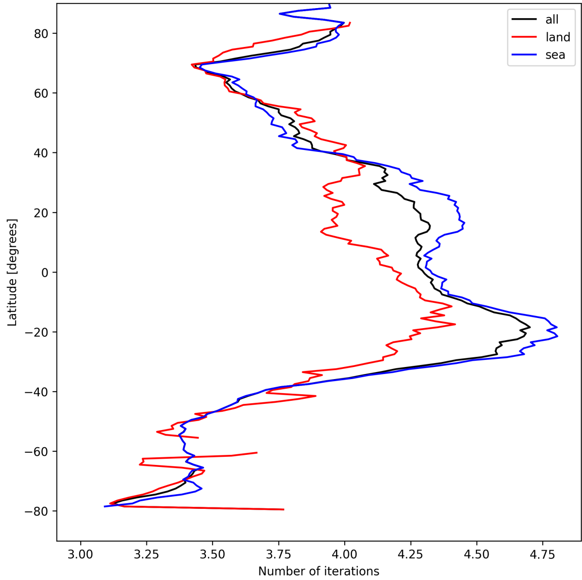
Figure 15: Zonal average of “Number of iterations” for 2025-04-11 to 2025-04-11.
