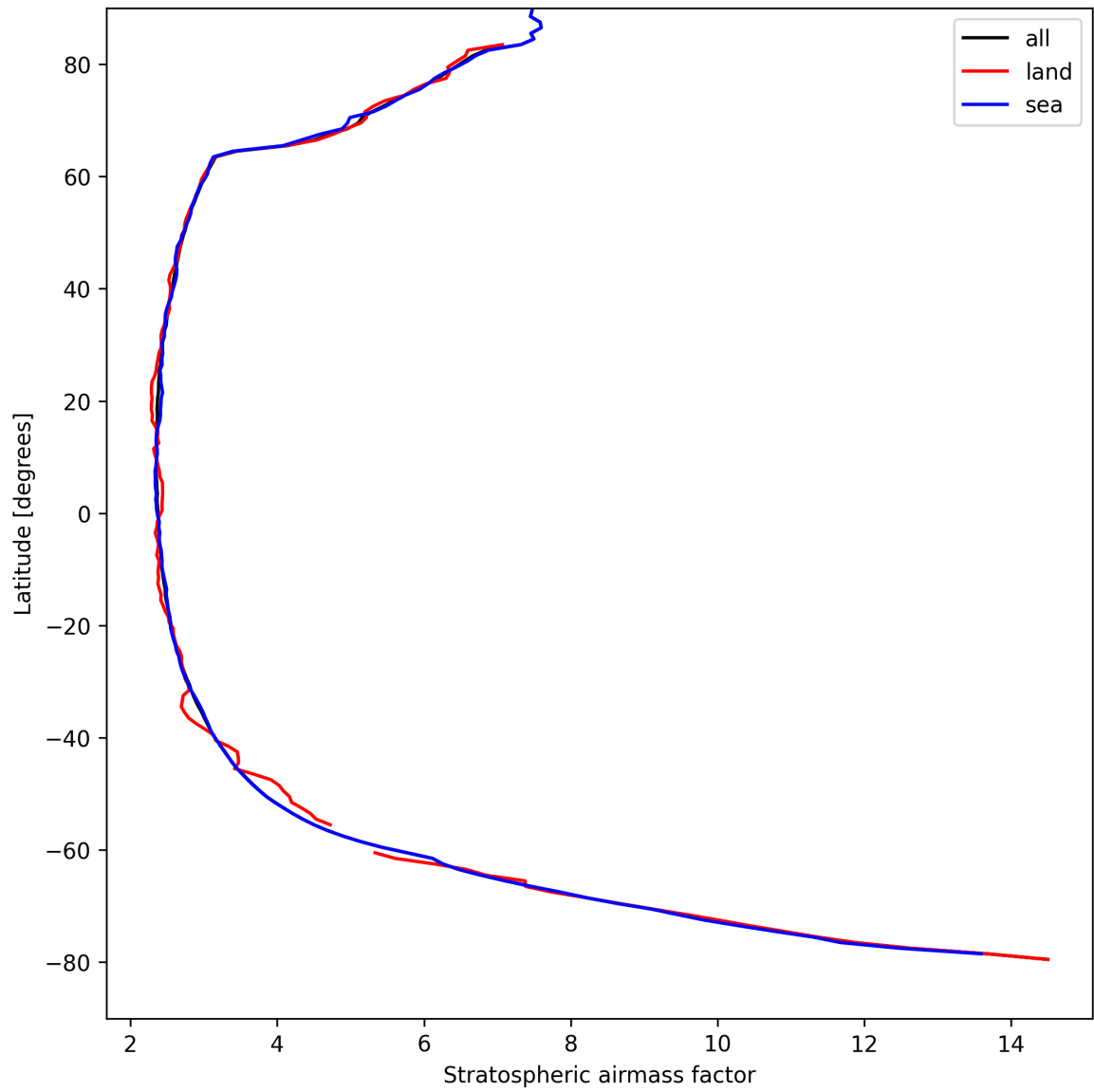
Figure 25: Zonal average of “Stratospheric airmass factor” for 2025-04-11 to 2025-04-11.
