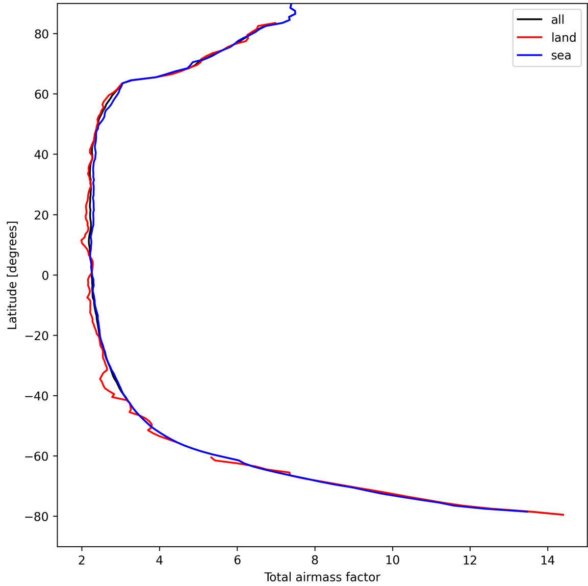
Figure 13: Zonal average of “Total airmass factor” for 2025-04-11 to 2025-04-11.
