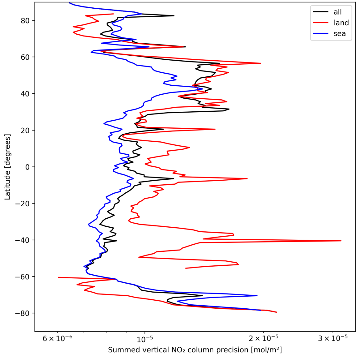
Figure 22: Zonal average of “Summed vertical NO 2 column precision” for 2025-04-11 to 2025-04-11.
