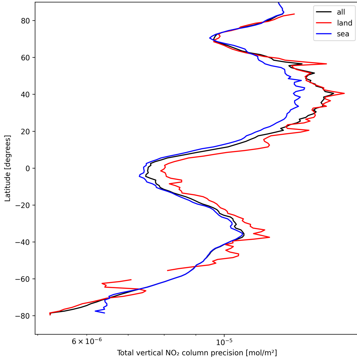
Figure 20: Zonal average of “Total vertical NO 2 column precision” for 2025-04-11 to 2025-04-11.
