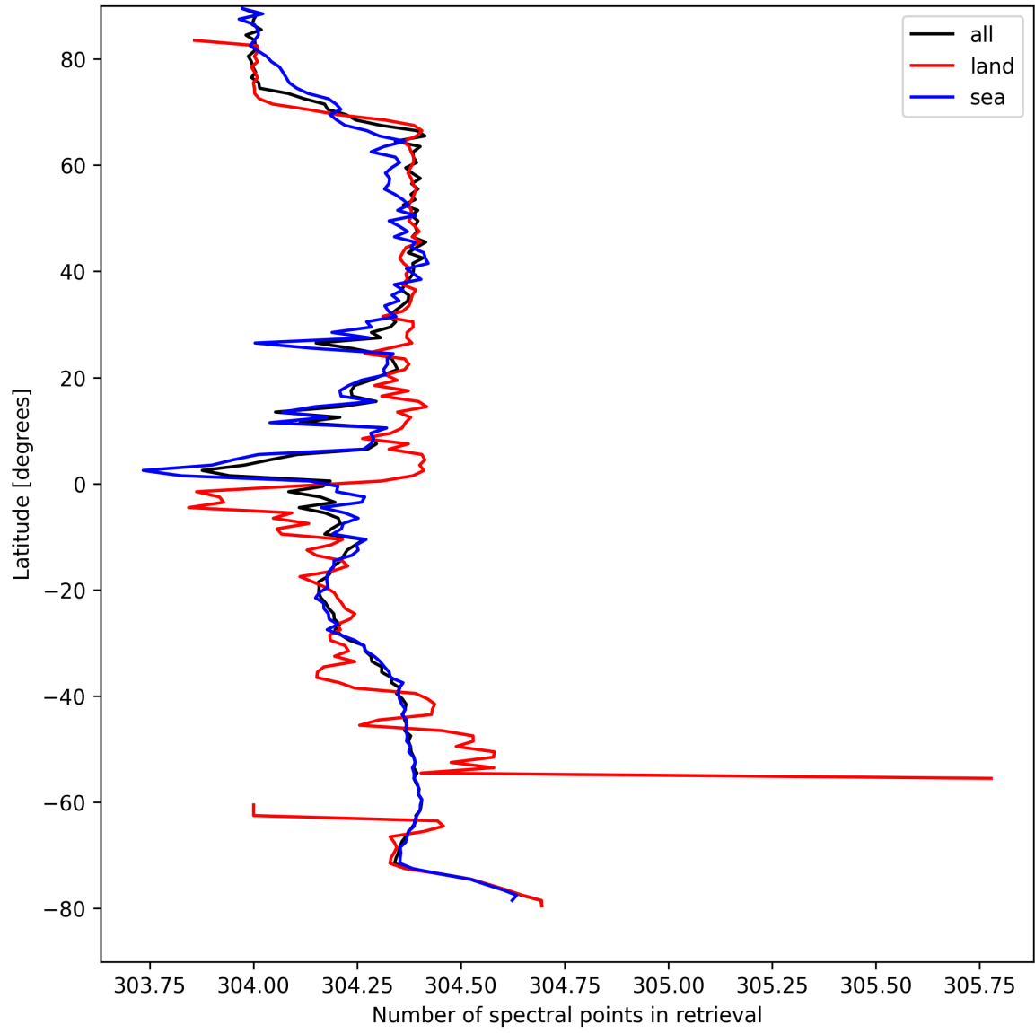
Figure 14: Zonal average of “Number of spectral points in retrieval” for 2025-04-11 to 2025-04-11.
