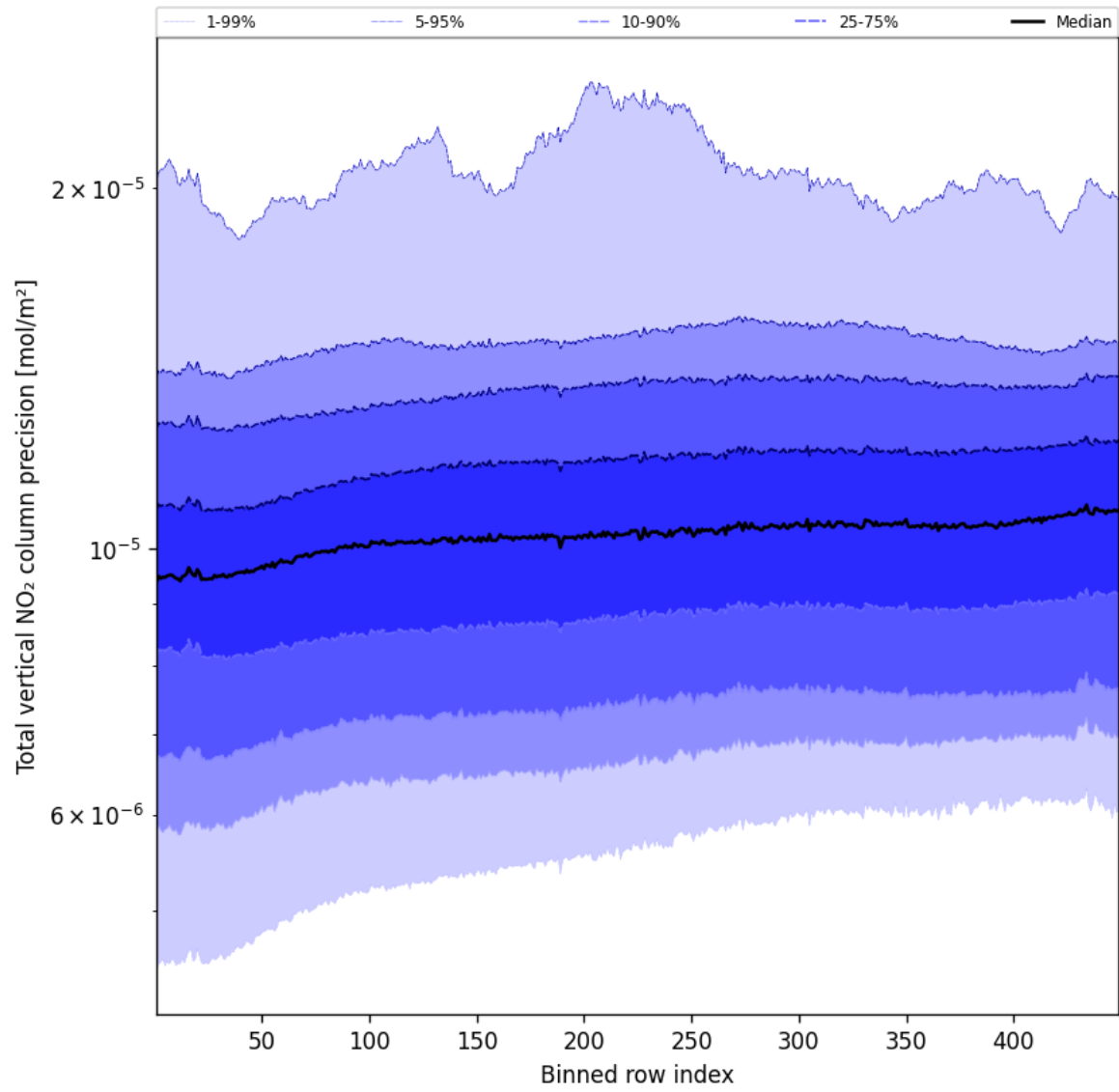
Figure 54: Along track statistics of “Total vertical NO 2 column precision” for 2025-04-12 to 2025-04-13
