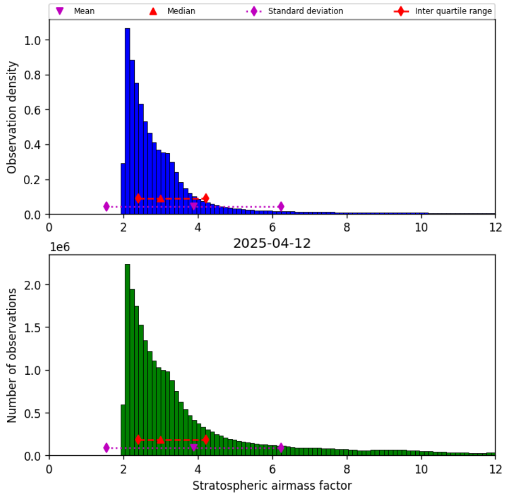
Figure 42: Histogram of “Stratospheric airmass factor” for 2025-04-12 to 2025-04-13
