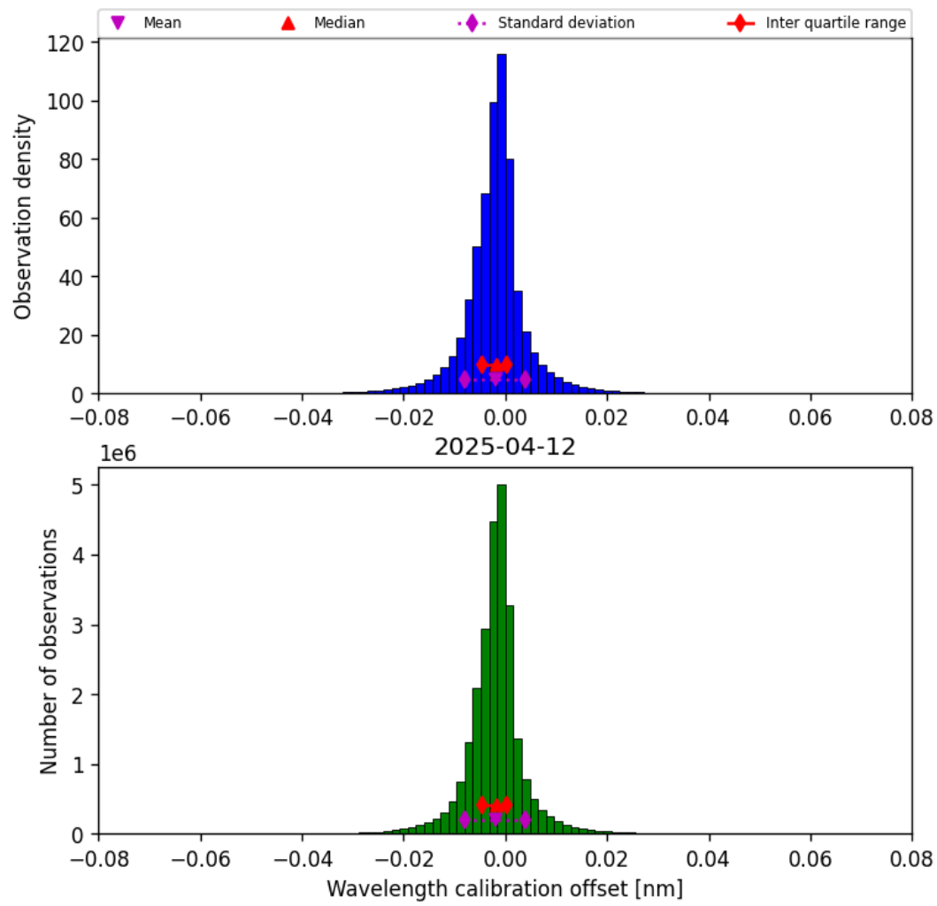
Figure 33: Histogram of “Wavelength calibration offset” for 2025-04-12 to 2025-04-13
