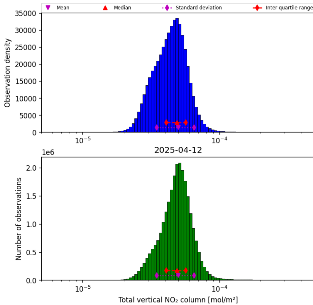
Figure 36: Histogram of "Total vertical NO 2 column" for 2025-04-12 to 2025-04-13
