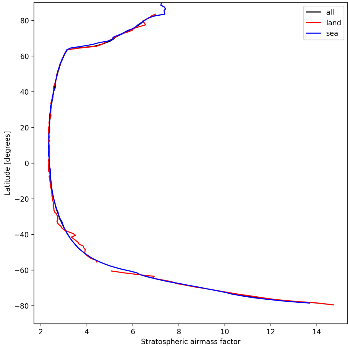
Figure 25: Zonal average of “Stratospheric airmass factor” for 2025-04-12 to 2025-04-13.
