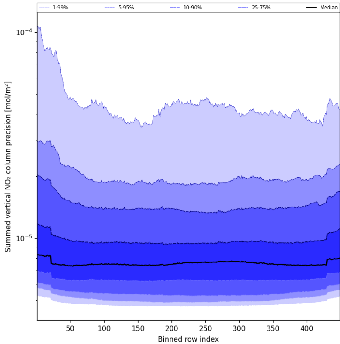
Figure 56: Along track statistics of “Summed vertical NO 2 column precision” for 2025-04-12 to 2025-04-13
