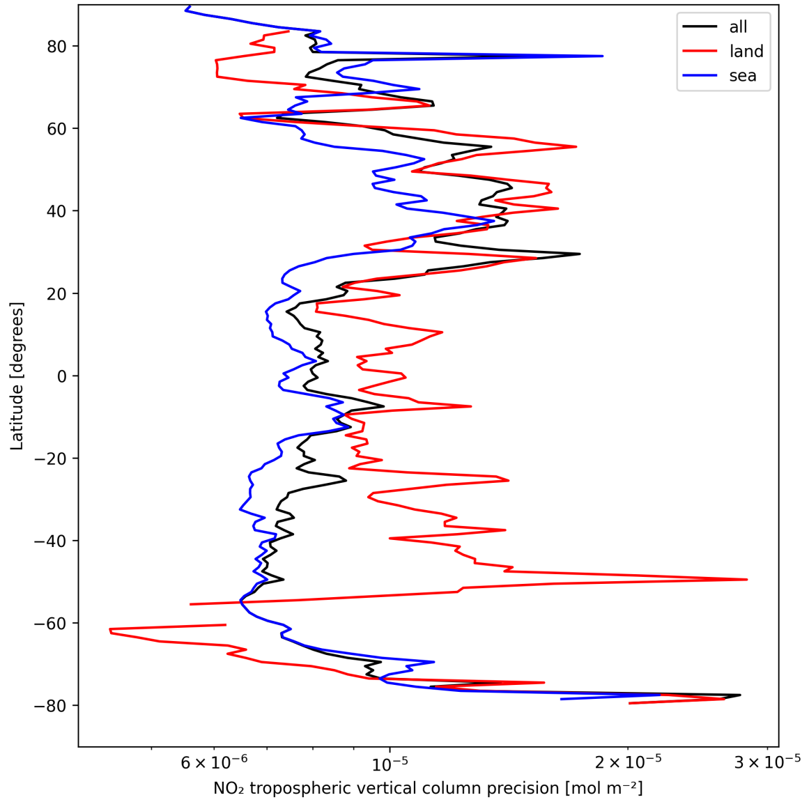
Figure 11: Zonal average of “NO 2 tropospheric vertical column precision” for 2025-04-12 to 2025-04-13.
