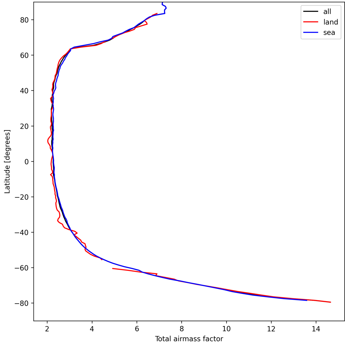
Figure 13: Zonal average of “Total airmass factor” for 2025-04-12 to 2025-04-13.
