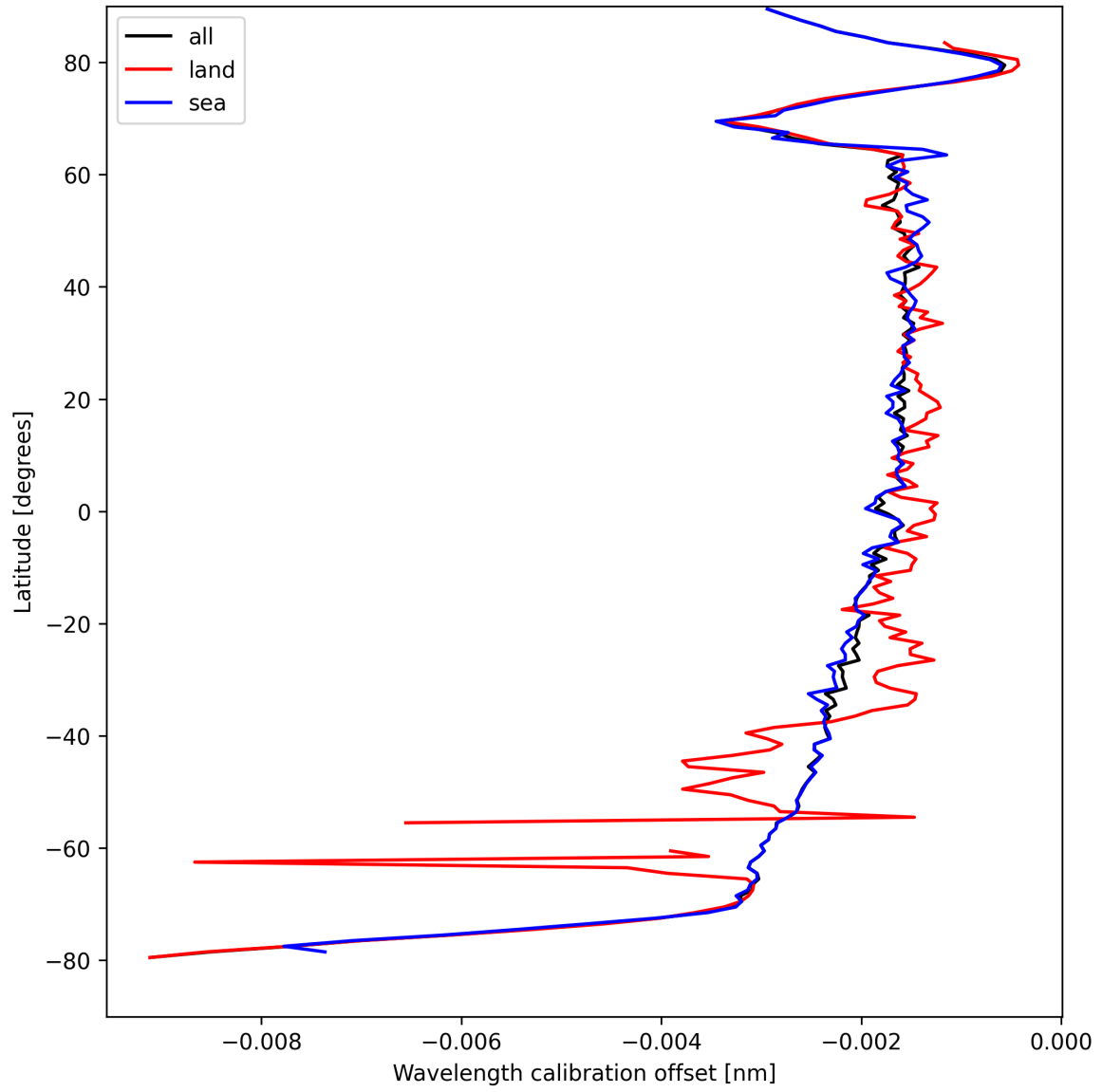
Figure 16: Zonal average of “Wavelength calibration offset” for 2025-04-12 to 2025-04-13.
