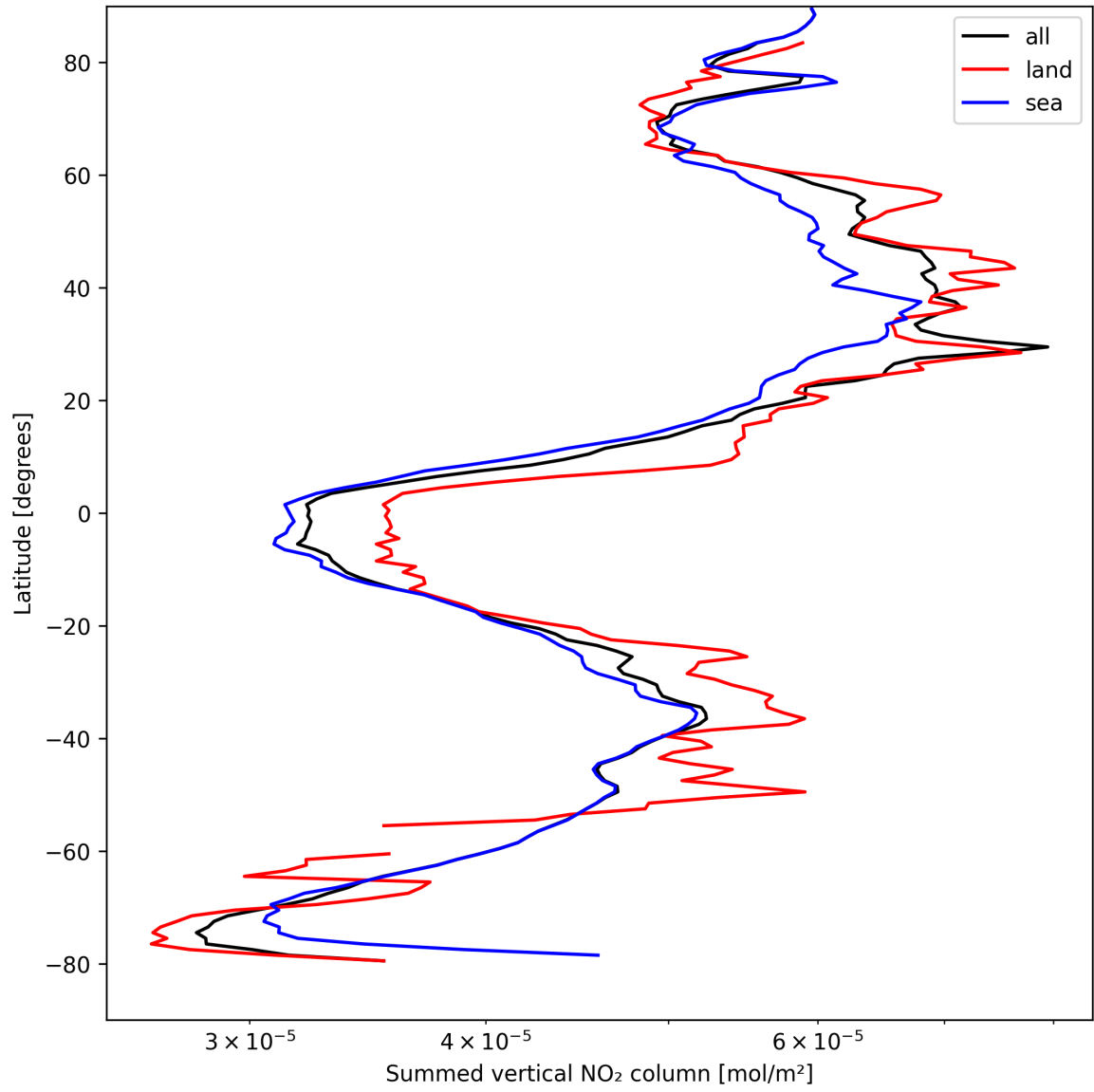
Figure 21: Zonal average of “Summed vertical NO 2 column” for 2025-04-12 to 2025-04-13.
