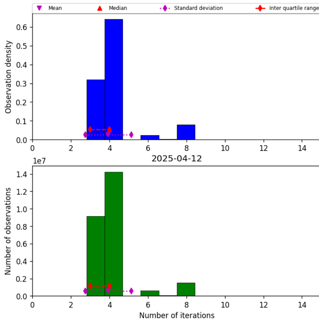
Figure 32: Histogram of “Number of iterations” for 2025-04-12 to 2025-04-13
