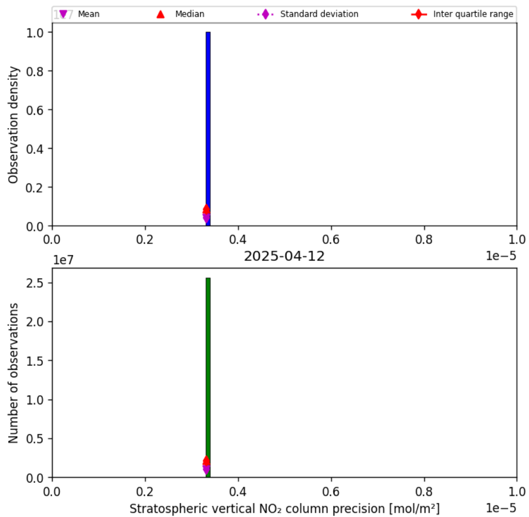
Figure 35: Histogram of “Stratospheric vertical NO 2 column precision” for 2025-04-12 to 2025-04-13
