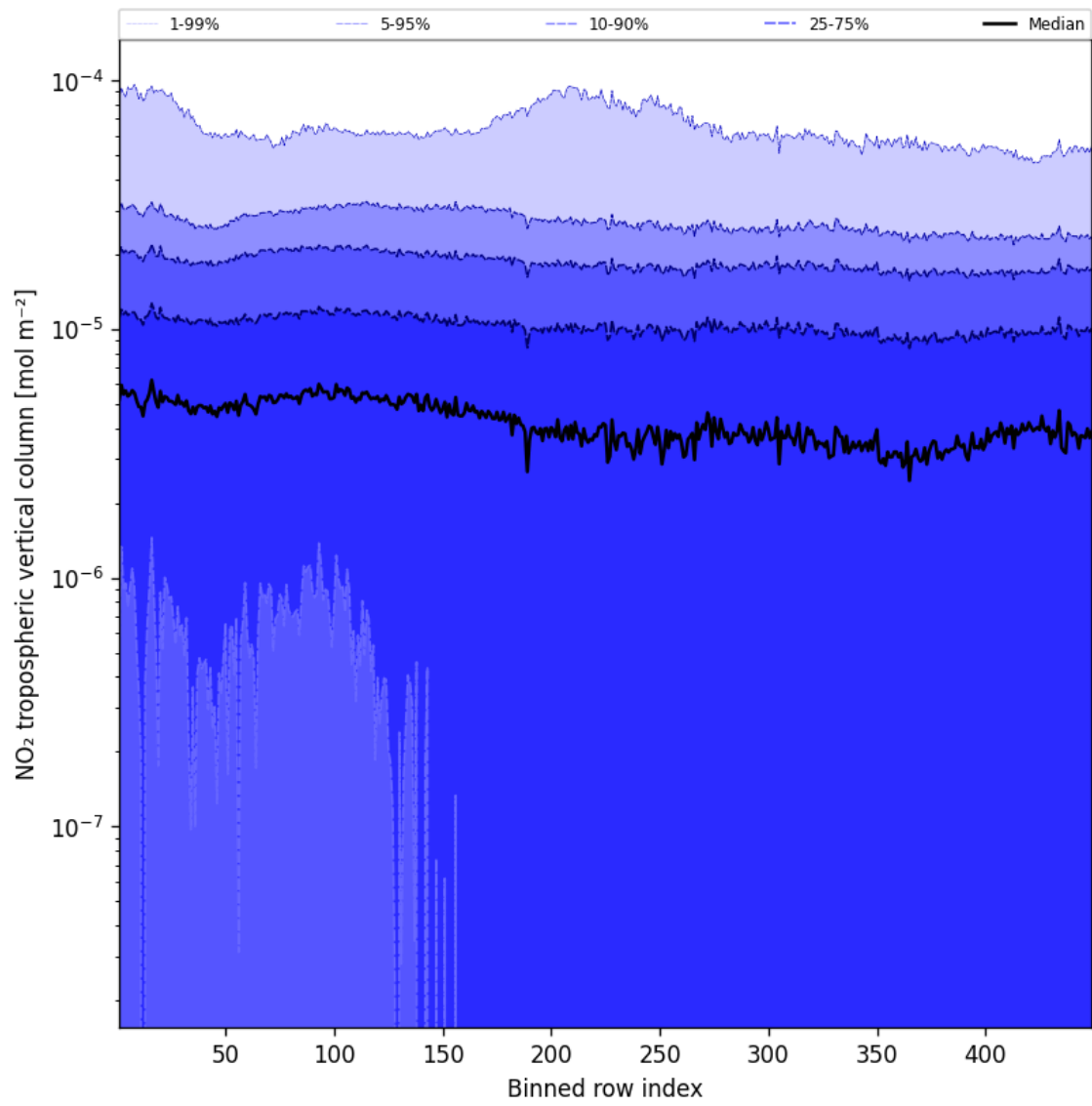
Figure 44: Along track statistics of “NO 2 tropospheric vertical column” for 2025-04-12 to 2025-04-13
