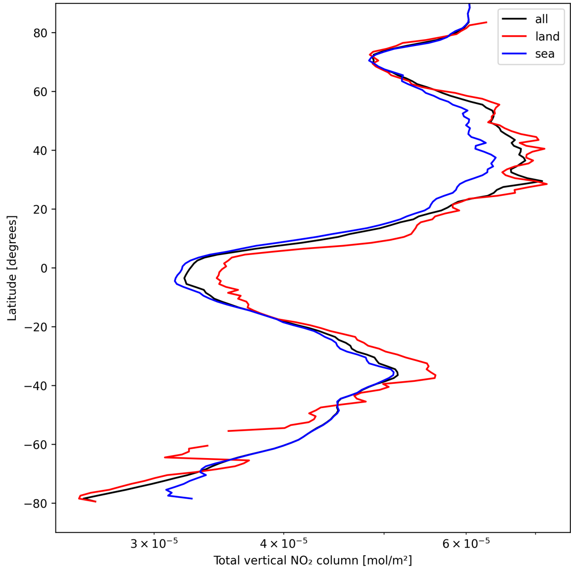
Figure 19: Zonal average of “Total vertical NO 2 column” for 2025-04-12 to 2025-04-13.
