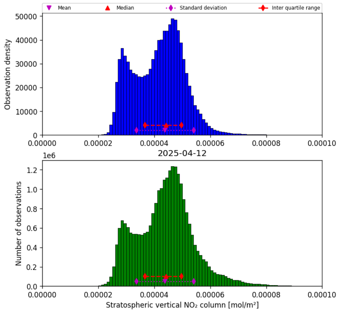
Figure 34: Histogram of “Stratospheric vertical NO 2 column” for 2025-04-12 to 2025-04-13
