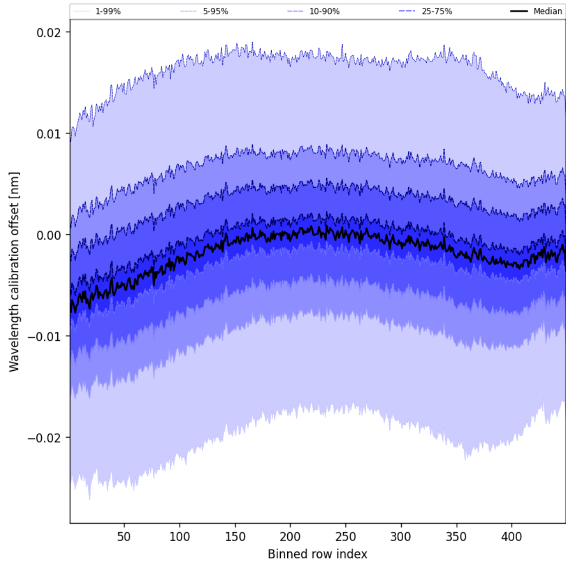
Figure 50: Along track statistics of “Wavelength calibration offset” for 2025-04-12 to 2025-04-13
