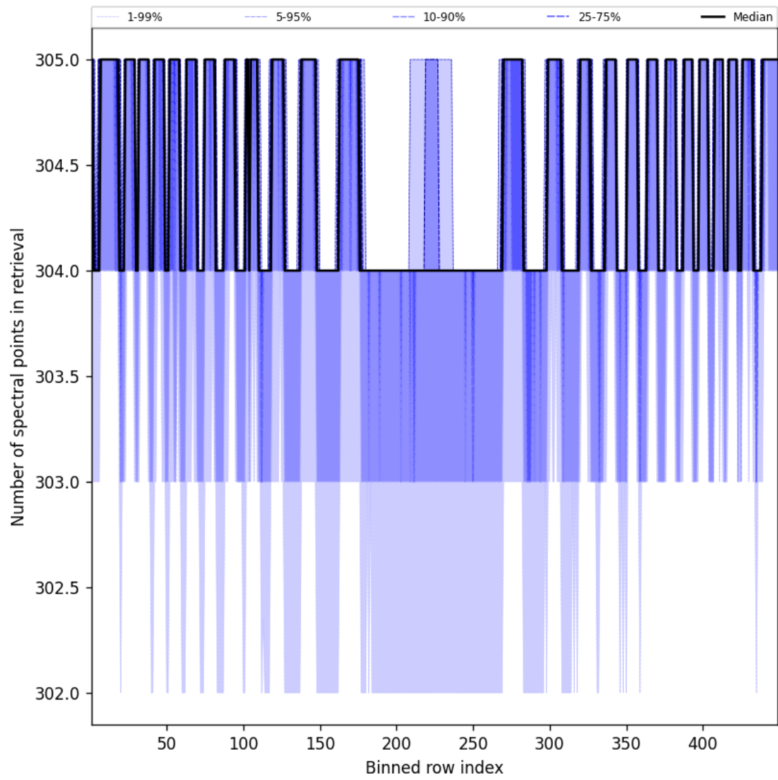
Figure 48: Along track statistics of “Number of spectral points in retrieval” for 2025-04-12 to 2025-04-13
