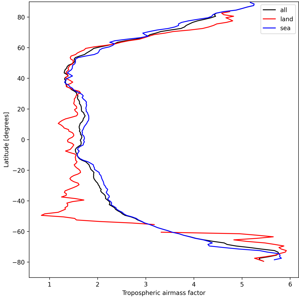
Figure 12: Zonal average of “Tropospheric air mass factor” for 2025-04-12 to 2025-04-13.
