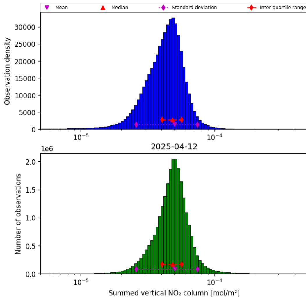
Figure 38: Histogram of “Summed vertical NO 2 column” for 2025-04-12 to 2025-04-13
