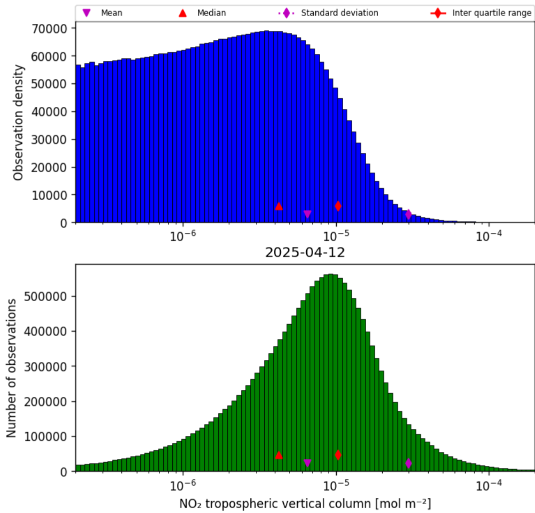
Figure 27: Histogram of “NO 2 tropospheric vertical column” for 2025-04-12 to 2025-04-13
