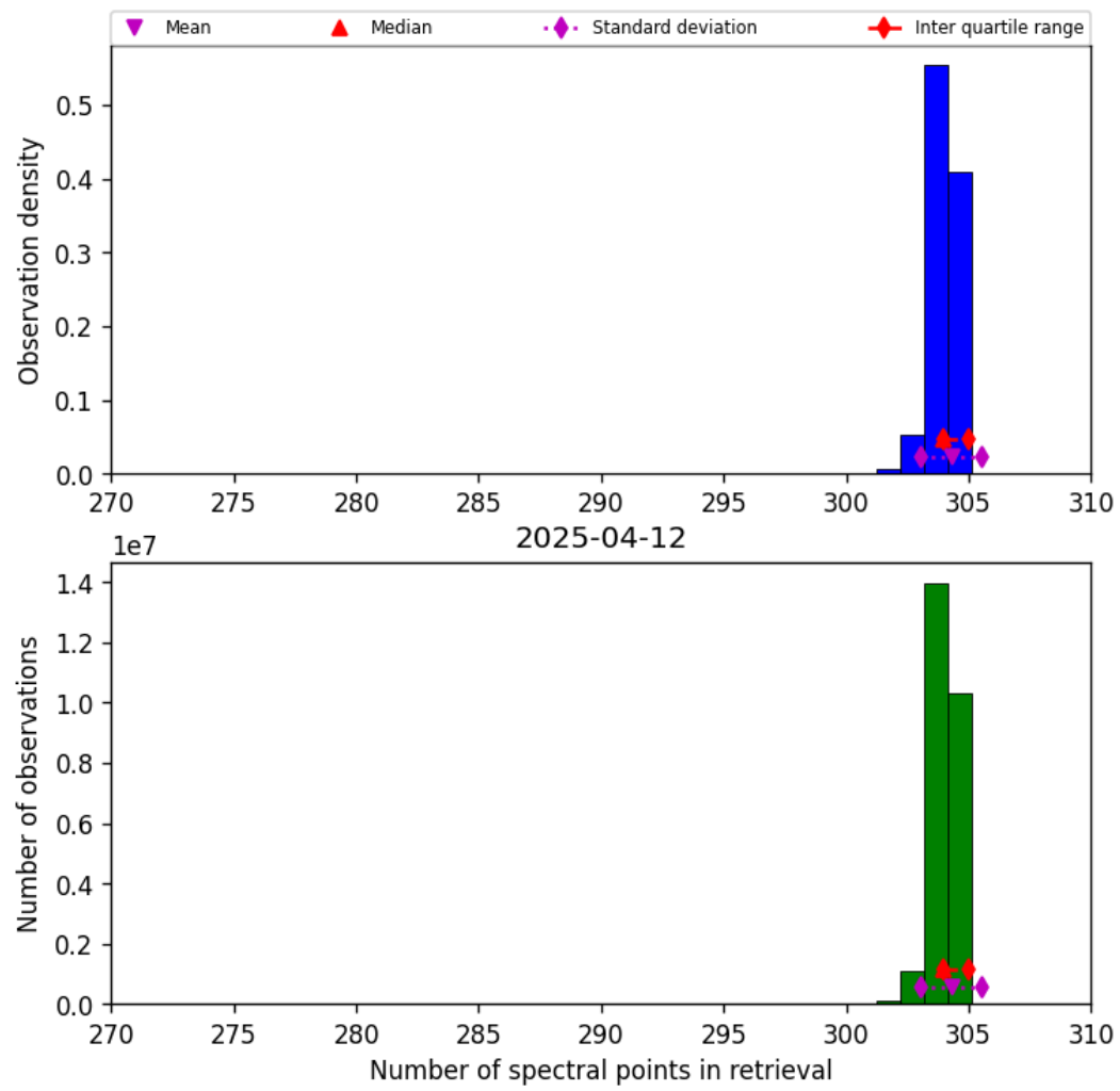
Figure 31: Histogram of “Number of spectral points in retrieval” for 2025-04-12 to 2025-04-13
