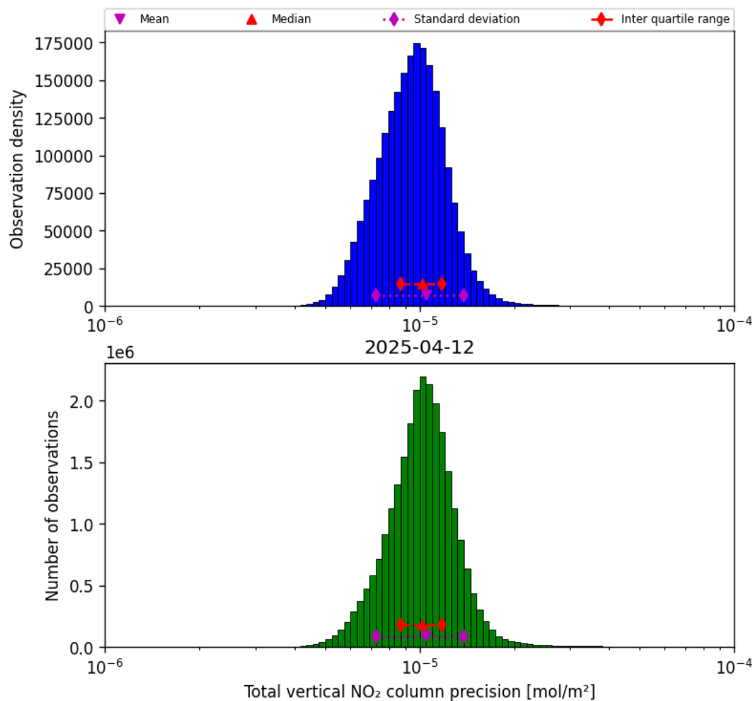
Figure 37: Histogram of “Total vertical NO 2 column precision” for 2025-04-12 to 2025-04-13
