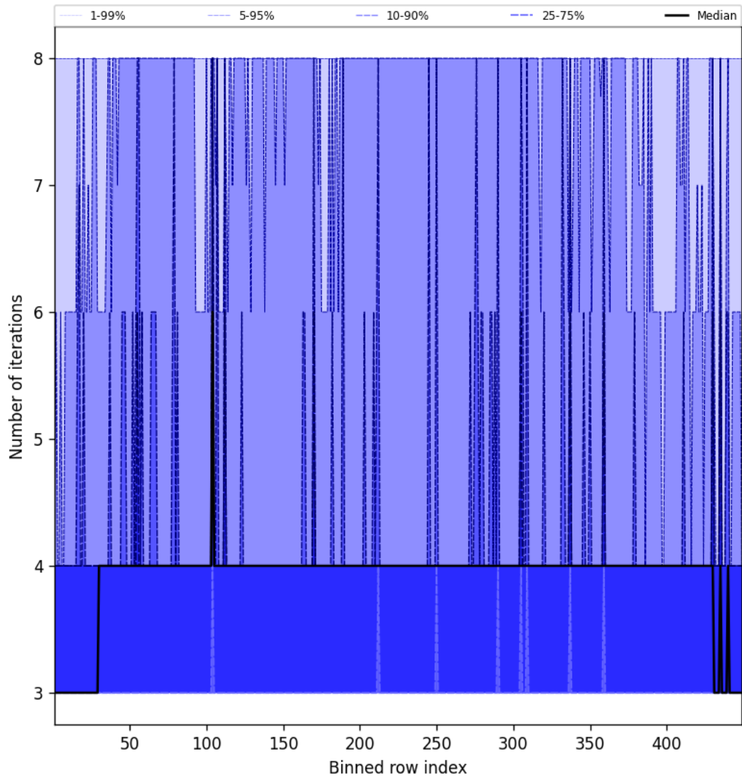
Figure 49: Along track statistics of “Number of iterations” for 2025-04-12 to 2025-04-13
