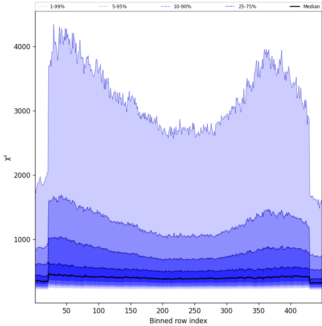
Figure 57: Along track statistics of “ \chi^2 ” for 2025-04-12 to 2025-04-13
