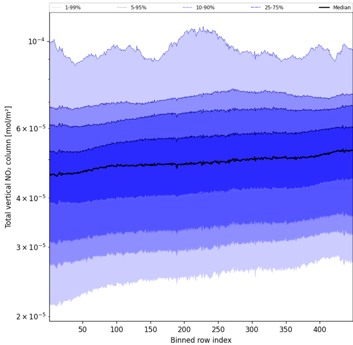
Figure 53: Along track statistics of “Total vertical NO 2 column” for 2025-04-12 to 2025-04-13
