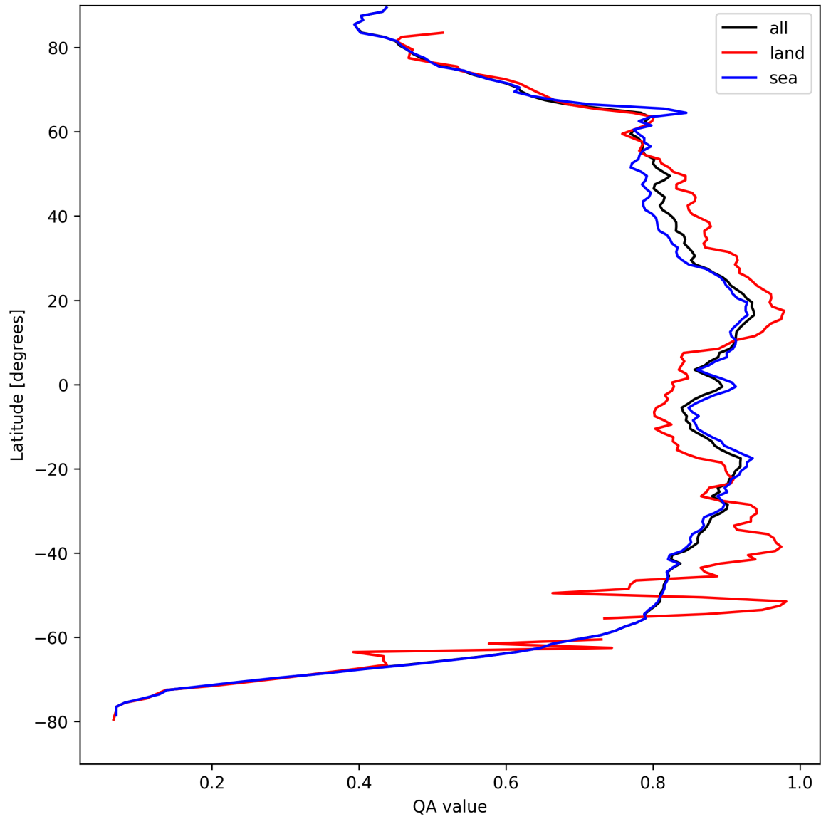
Figure 9: Zonal average of “QA value” for 2025-04-12 to 2025-04-13.
