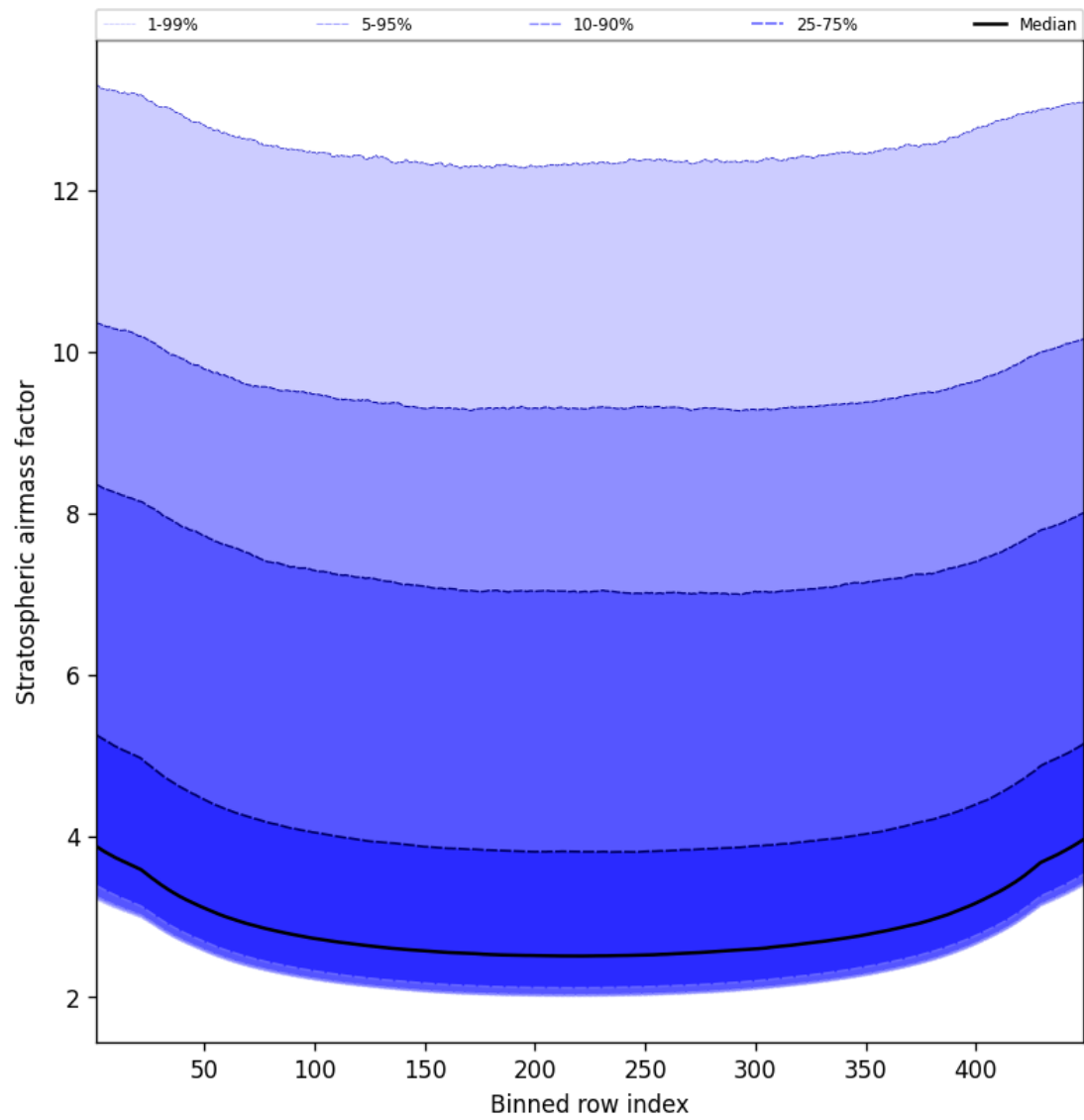
Figure 59: Along track statistics of “Stratospheric airmass factor” for 2025-04-12 to 2025-04-13
