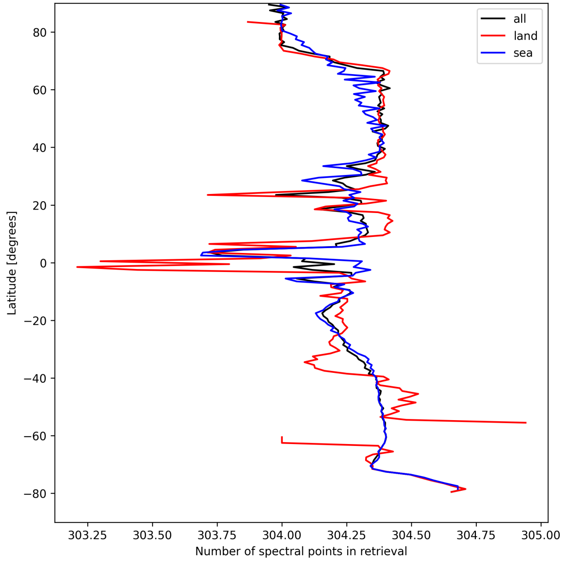
Figure 14: Zonal average of “Number of spectral points in retrieval” for 2025-04-12 to 2025-04-13.
