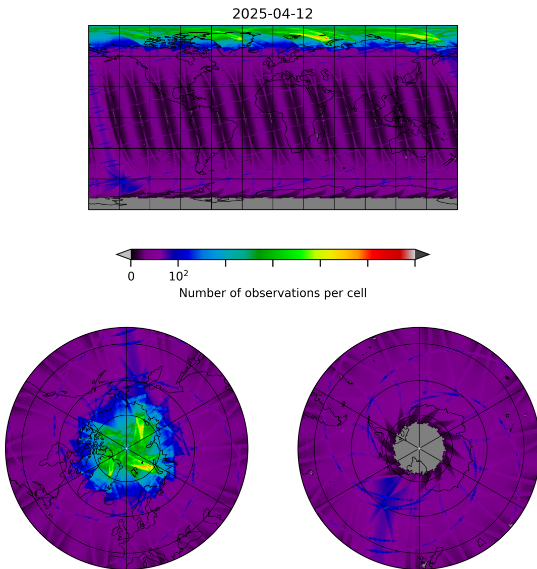
Figure 8: Map of the number of observations for 2025-04-12 to 2025-04-13
