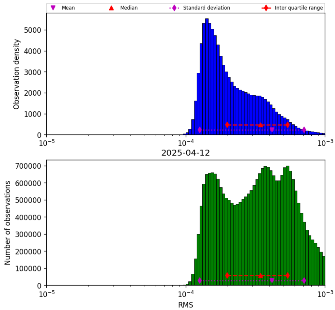
Figure 41: Histogram of “RMS” for 2025-04-12 to 2025-04-13
