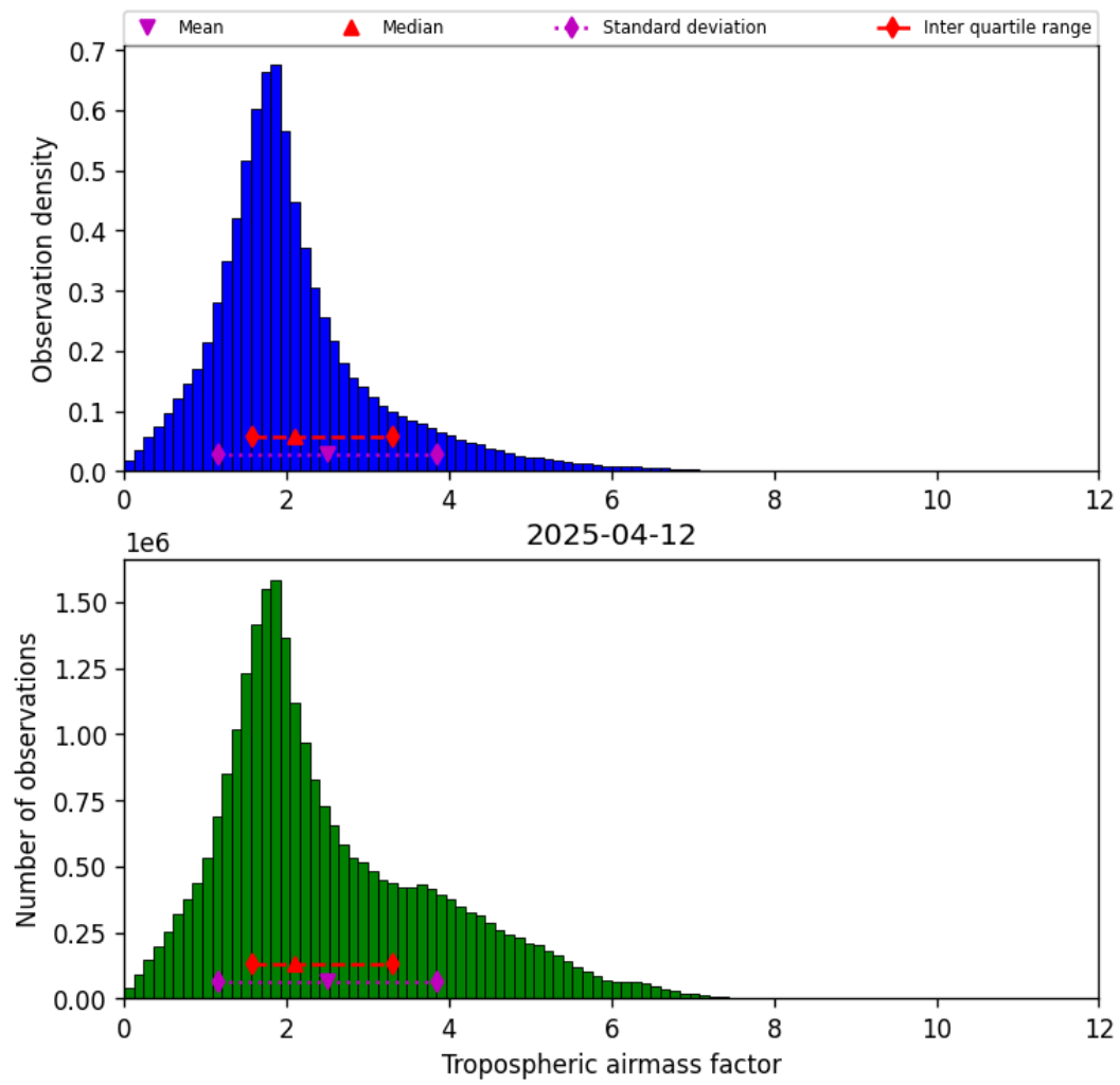
Figure 29: Histogram of “Tropospheric airmass factor” for 2025-04-12 to 2025-04-13
