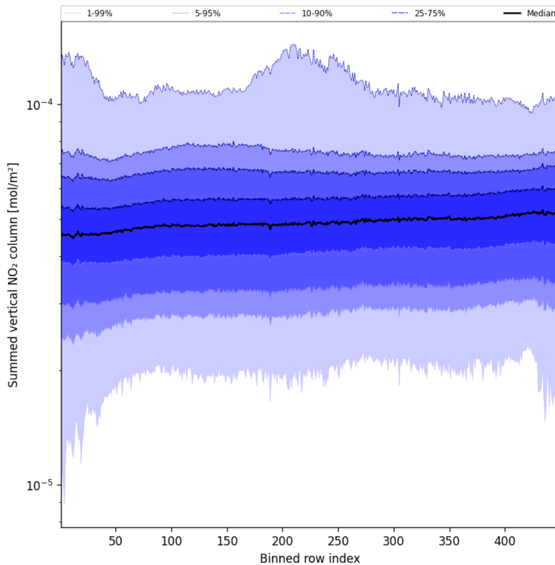
Figure 55: Along track statistics of “Summed vertical NO 2 column” for 2025-04-12 to 2025-04-13
