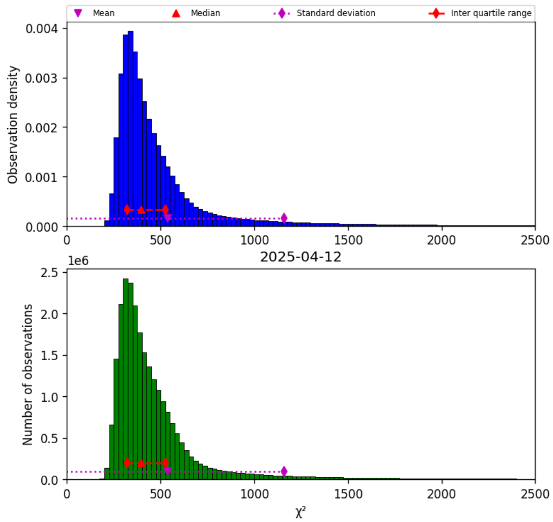
Figure 40: Histogram of “ \chi^2 ” for 2025-04-12 to 2025-04-13
