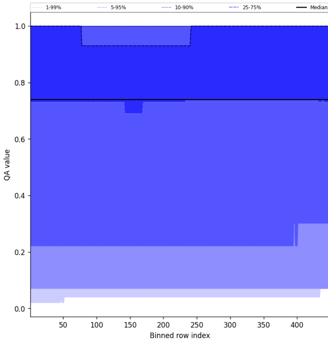
Figure 43: Along track statistics of "QA value" for 2025-04-12 to 2025-04-13
