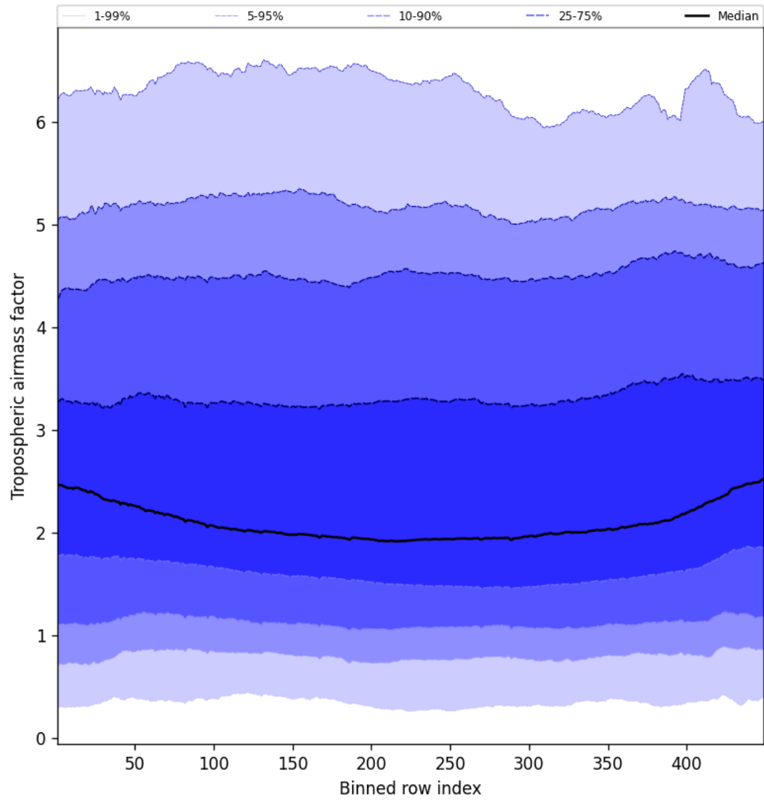
Figure 46: Along track statistics of “Tropospheric airmass factor” for 2025-04-12 to 2025-04-13
