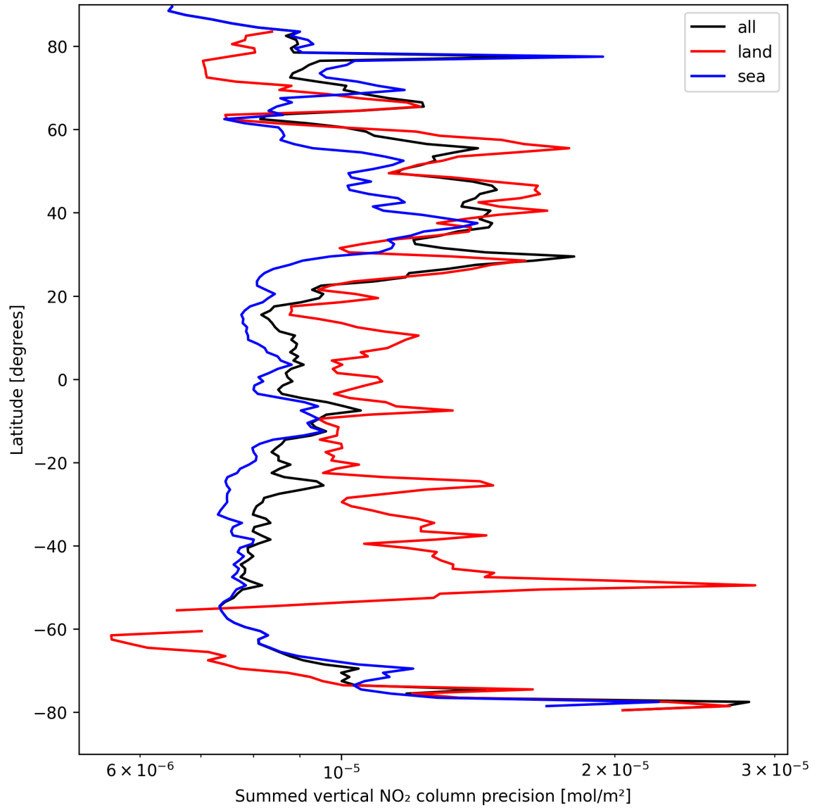
Figure 22: Zonal average of “Summed vertical NO 2 column precision” for 2025-04-12 to 2025-04-13.
