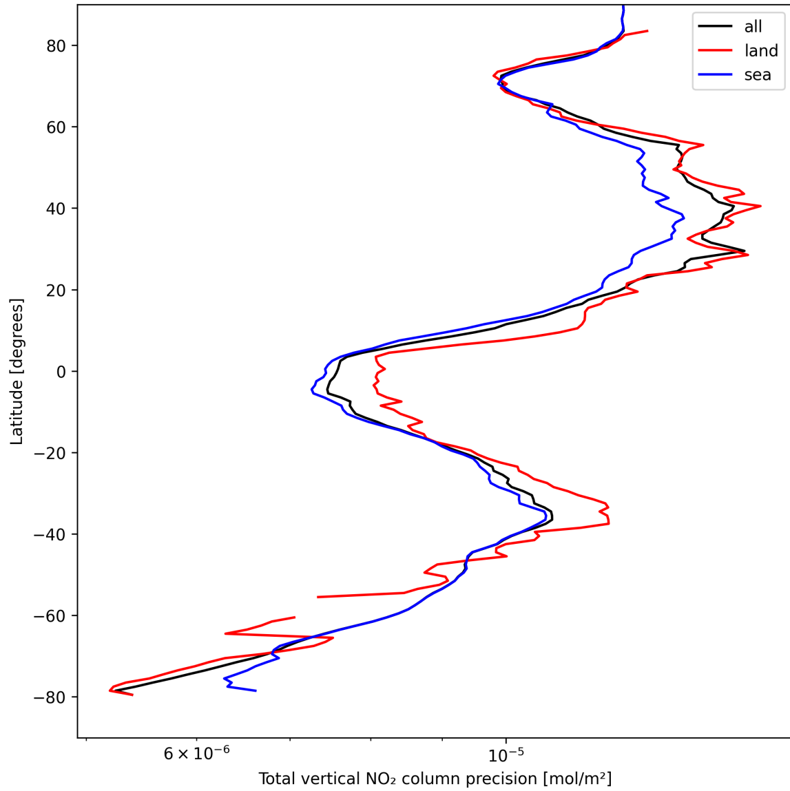
Figure 20: Zonal average of "Total vertical NO 2 column precision" for 2025-04-12 to 2025-04-13.
