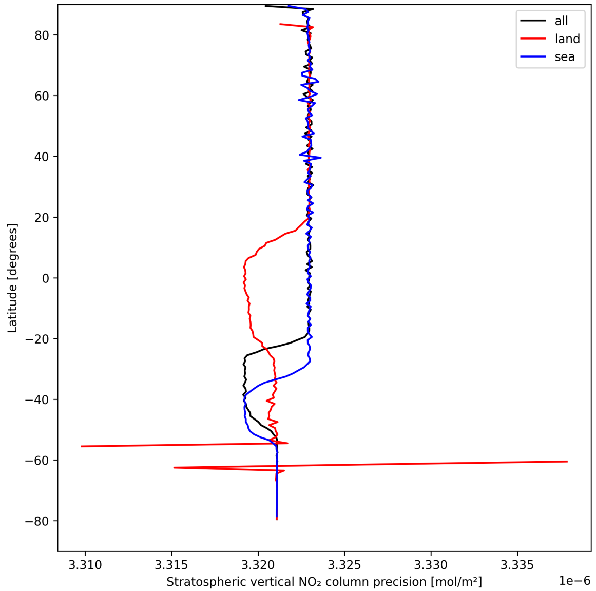
Figure 18: Zonal average of “Stratospheric vertical NO 2 column precision” for 2025-04-12 to 2025-04-13.
