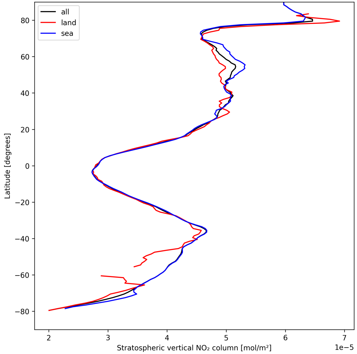
Figure 17: Zonal average of “Stratospheric vertical NO 2 column” for 2025-04-12 to 2025-04-13.
