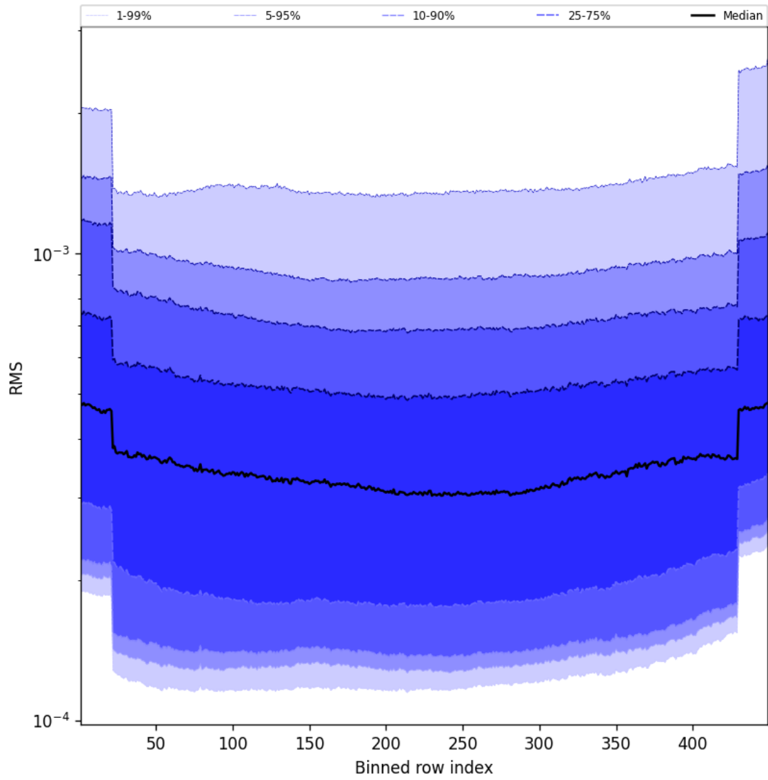
Figure 58: Along track statistics of “RMS” for 2025-04-12 to 2025-04-13
