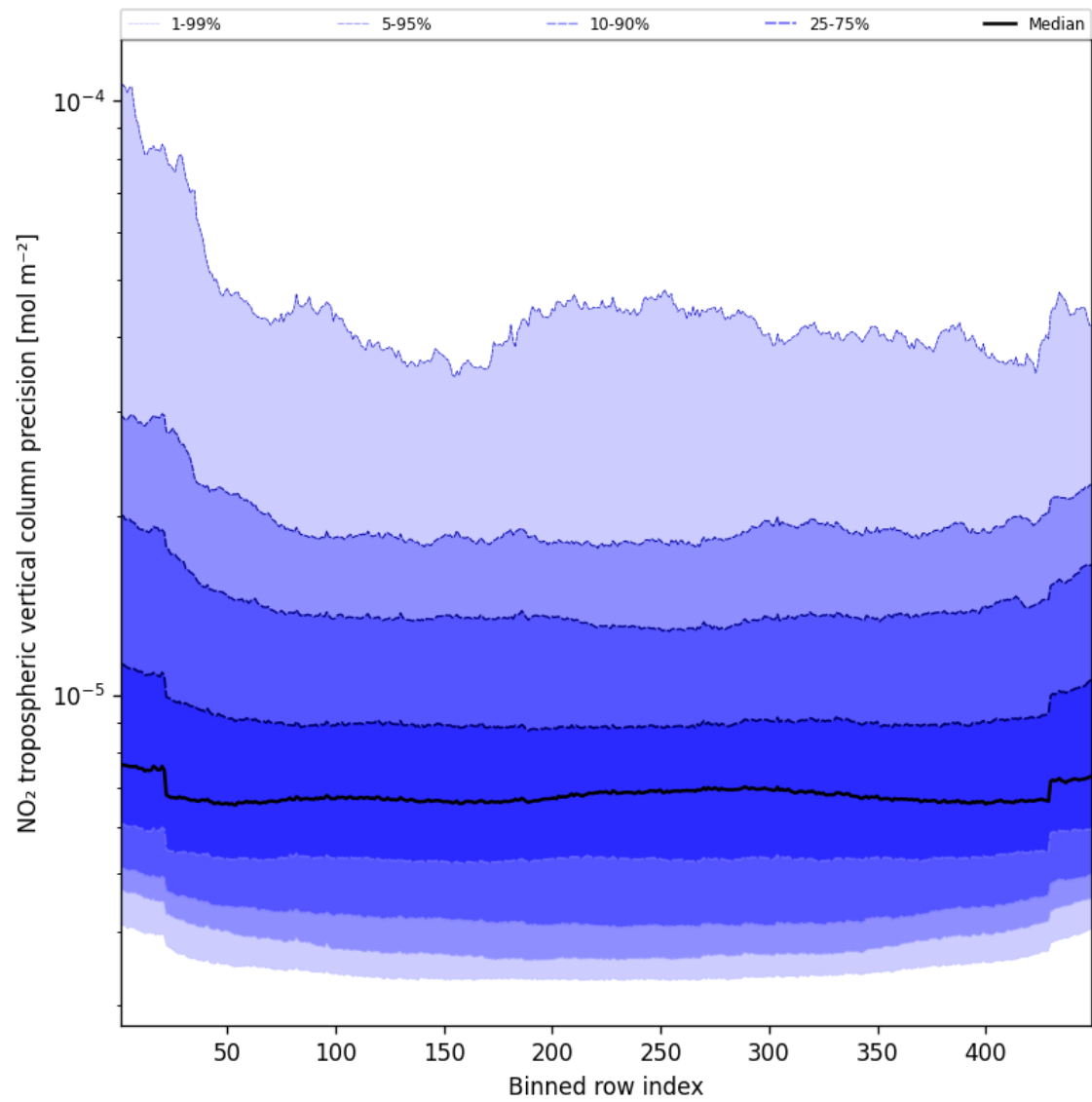
Figure 45: Along track statistics of “NO 2 tropospheric vertical column precision” for 2025-04-12 to 2025-04-13
