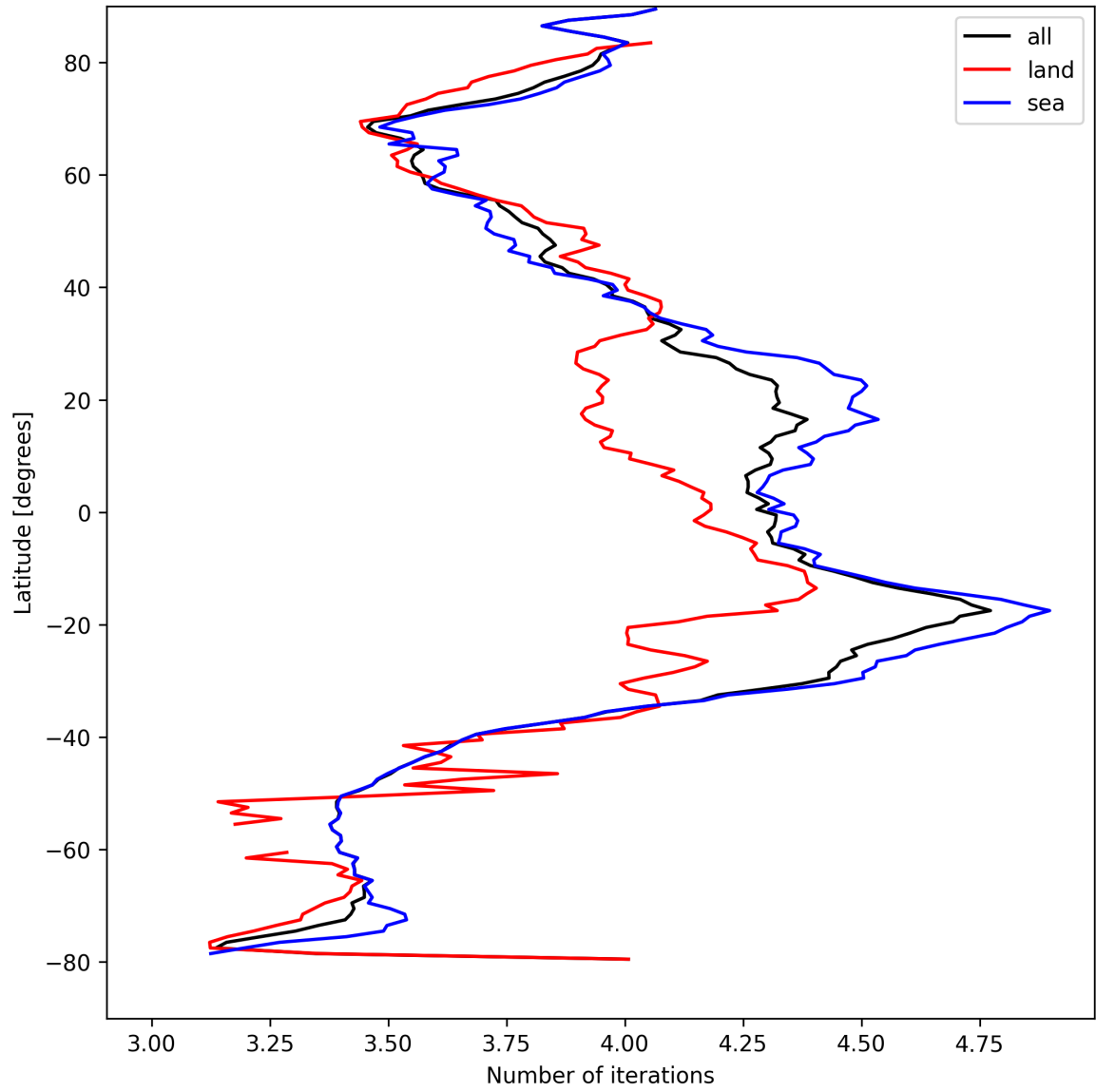
Figure 15: Zonal average of “Number of iterations” for 2025-04-12 to 2025-04-13.
