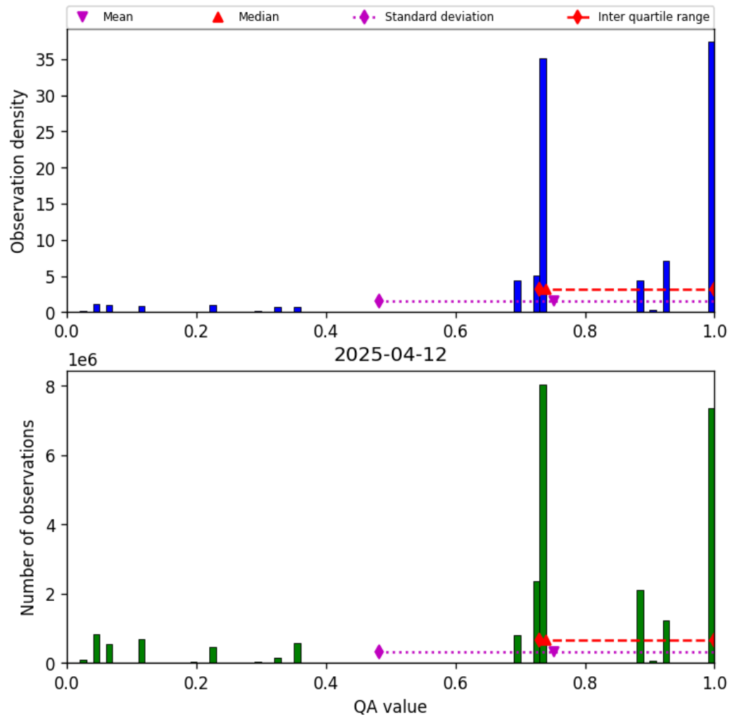
Figure 26: Histogram of “QA value” for 2025-04-12 to 2025-04-13
