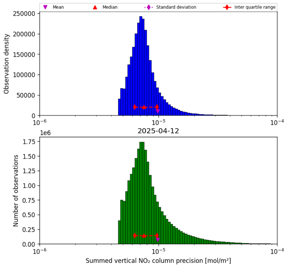
Figure 39: Histogram of "Summed vertical NO 2 column precision" for 2025-04-12 to 2025-04-13
