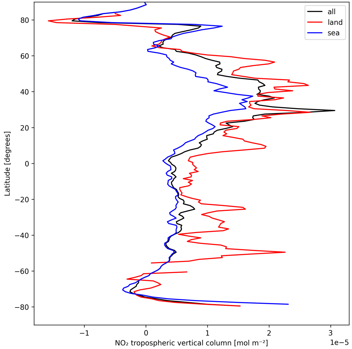
Figure 10: Zonal average of “NO 2 tropospheric vertical column” for 2025-04-12 to 2025-04-13.
