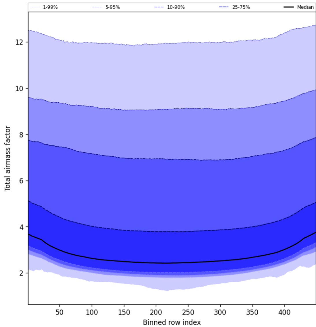
Figure 47: Along track statistics of “Total airmass factor” for 2025-04-12 to 2025-04-13
