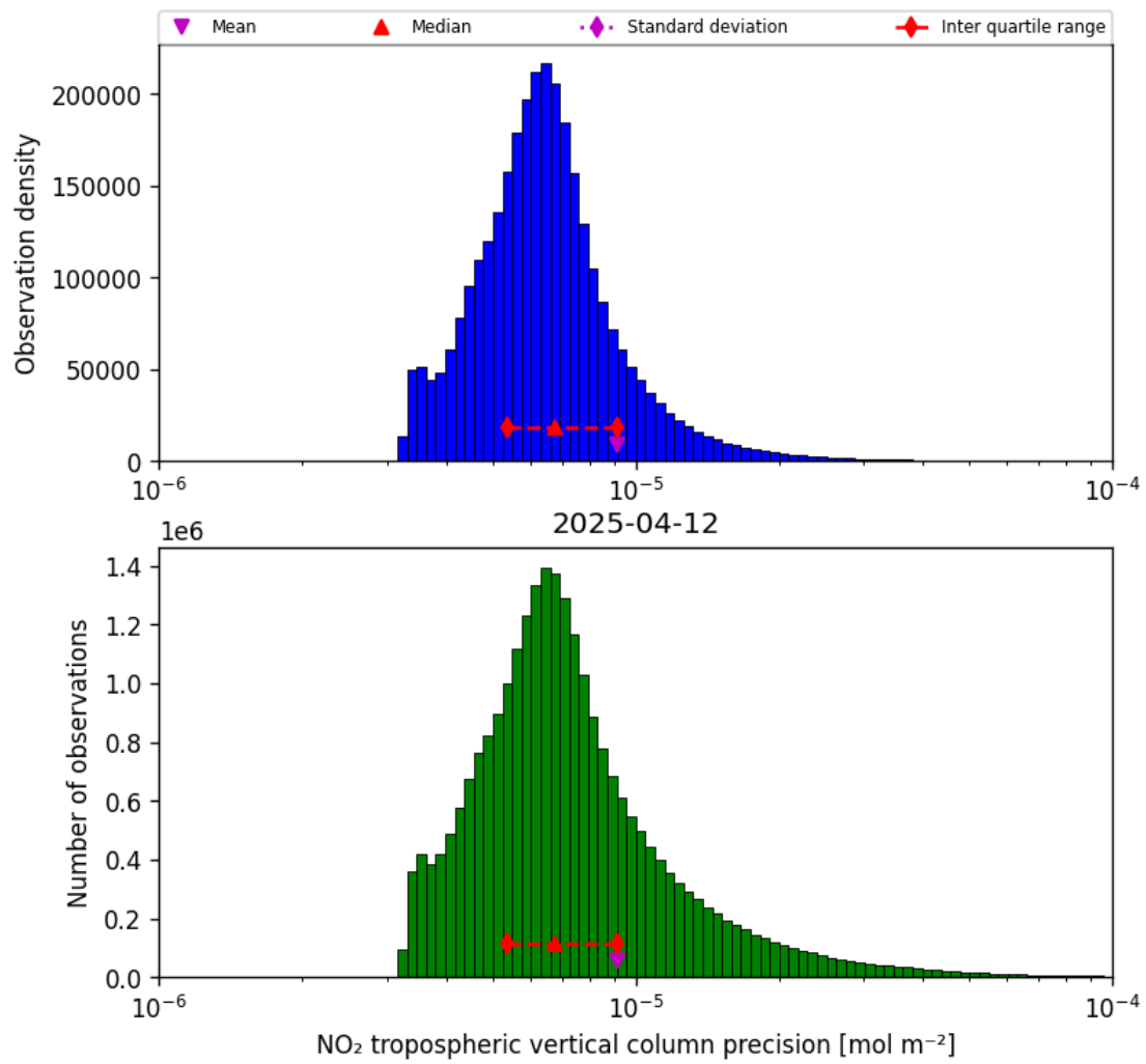
Figure 28: Histogram of “NO 2 tropospheric vertical column precision” for 2025-04-12 to 2025-04-13
