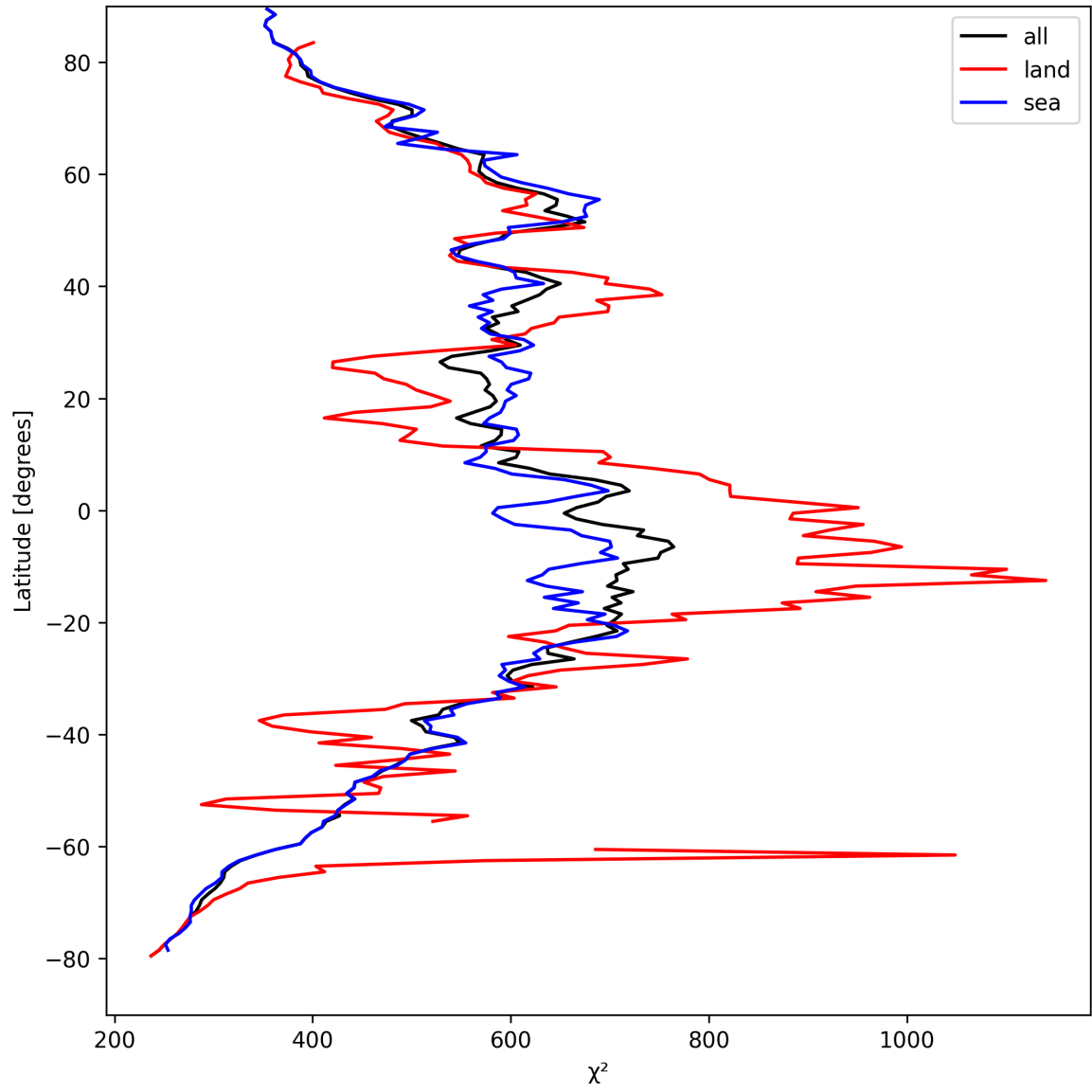
Figure 23: Zonal average of “ \chi^2 ” for 2025-04-12 to 2025-04-13.
