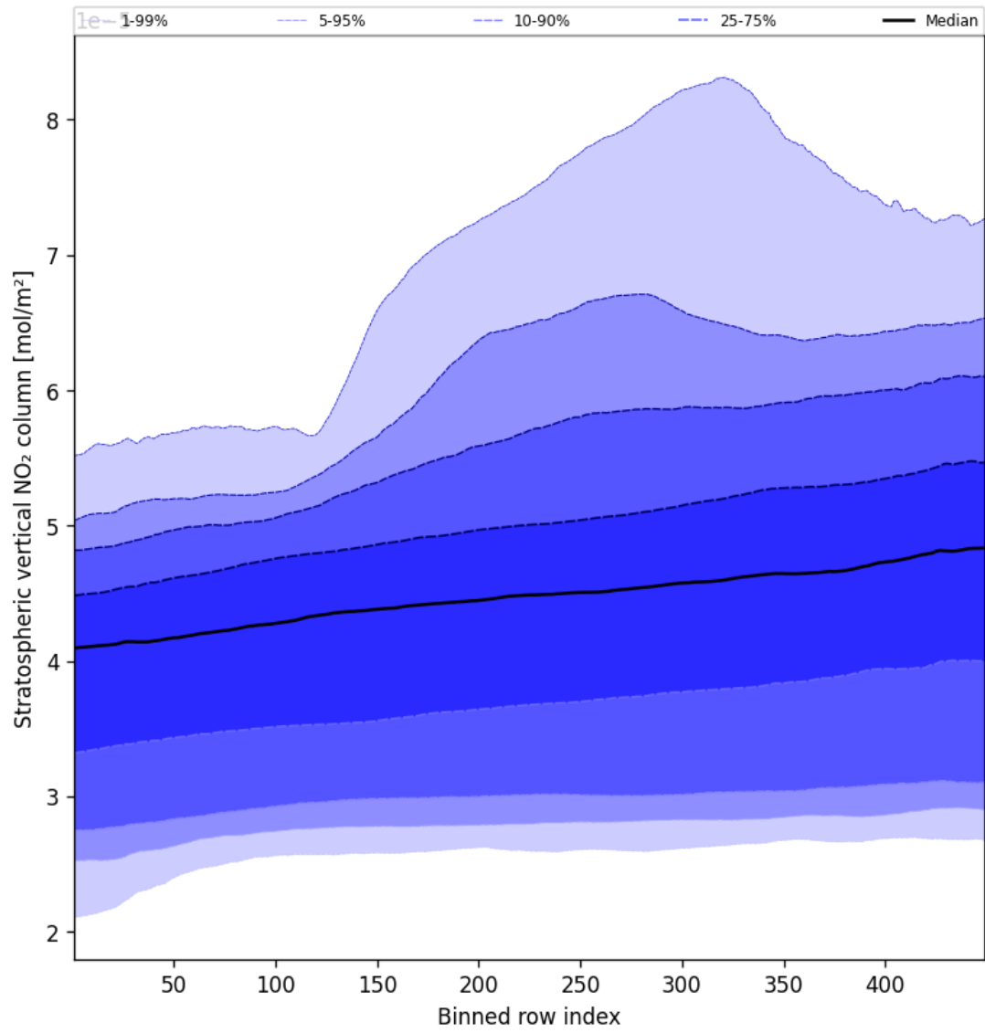
Figure 51: Along track statistics of “Stratospheric vertical NO 2 column” for 2025-04-12 to 2025-04-13
