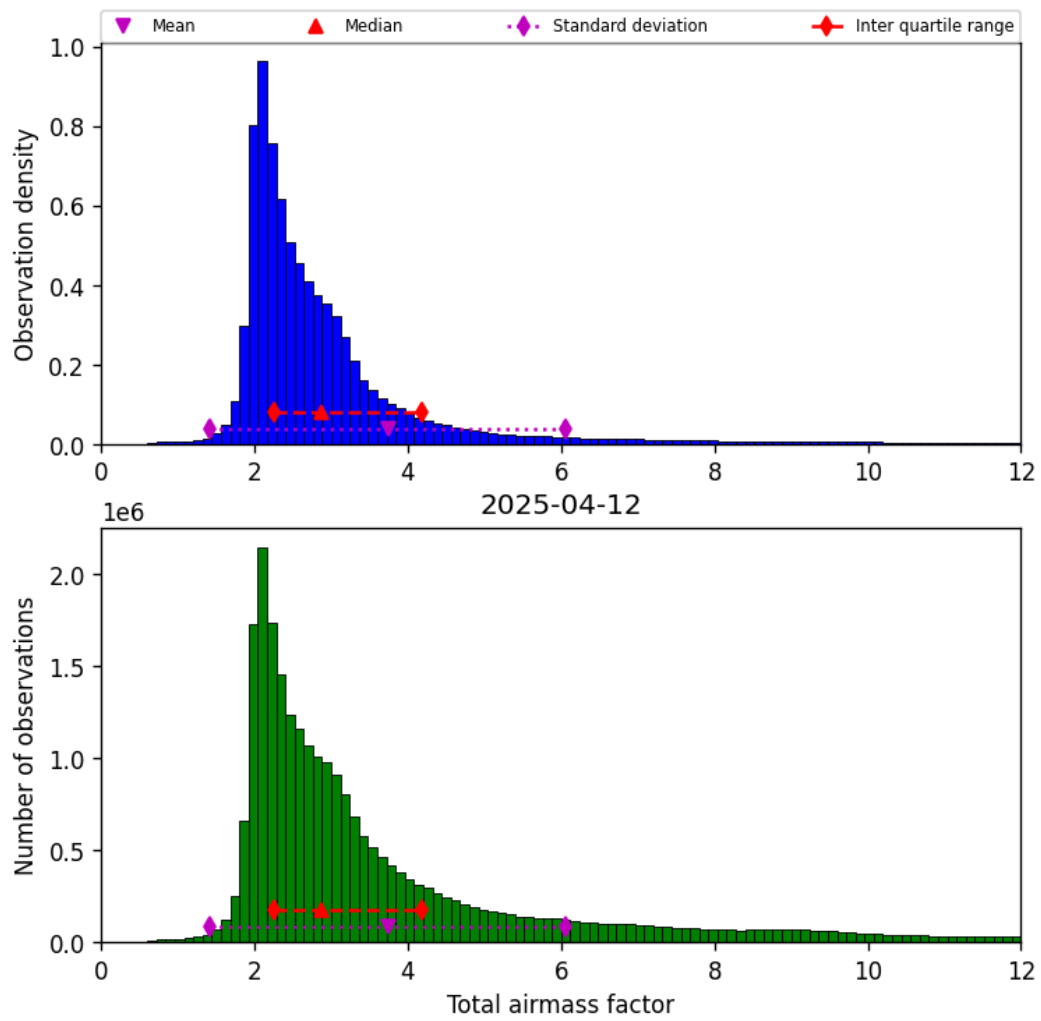
Figure 30: Histogram of “Total airmass factor” for 2025-04-12 to 2025-04-13
