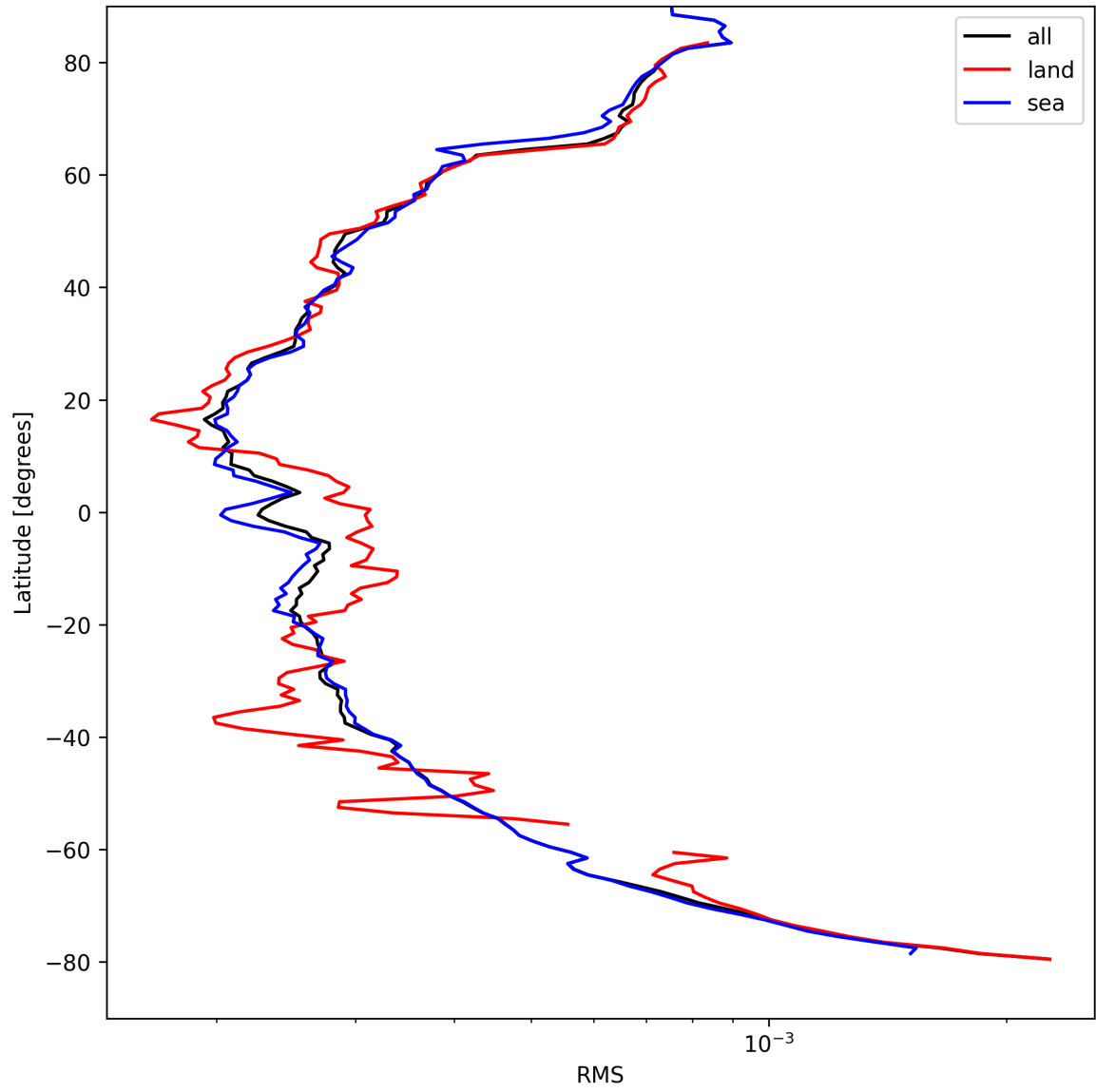
Figure 24: Zonal average of “RMS” for 2025-04-12 to 2025-04-13.
