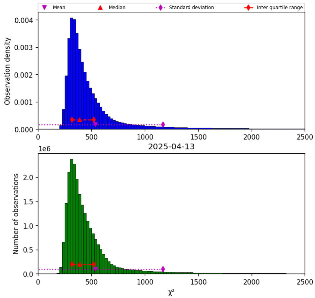
Figure 40: Histogram of “ \chi^2 ” for 2025-04-13 to 2025-04-14
