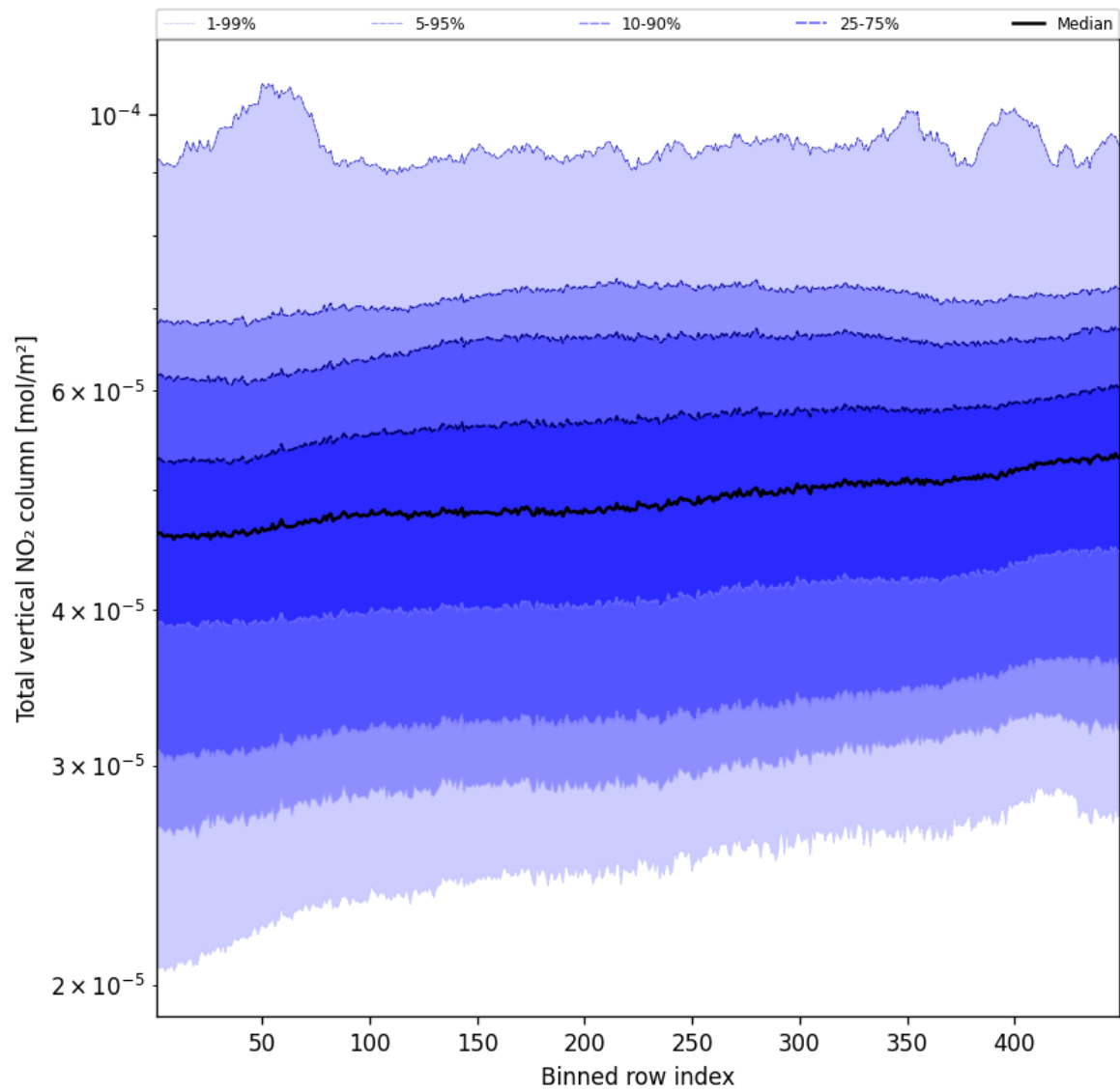
Figure 53: Along track statistics of “Total vertical NO 2 column” for 2025-04-13 to 2025-04-14
