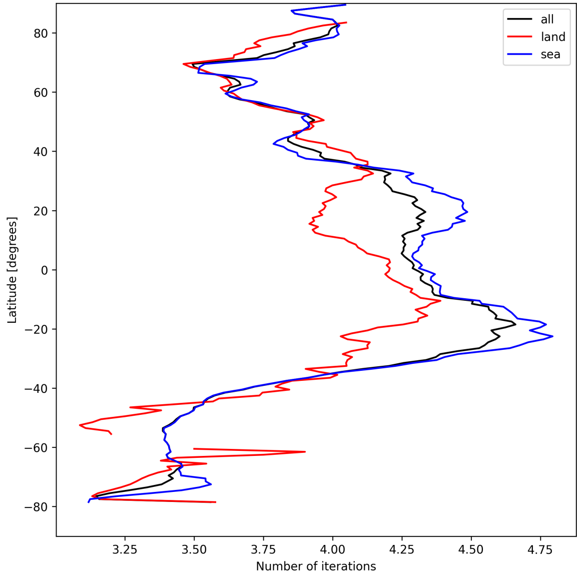
Figure 15: Zonal average of “Number of iterations” for 2025-04-13 to 2025-04-14.
