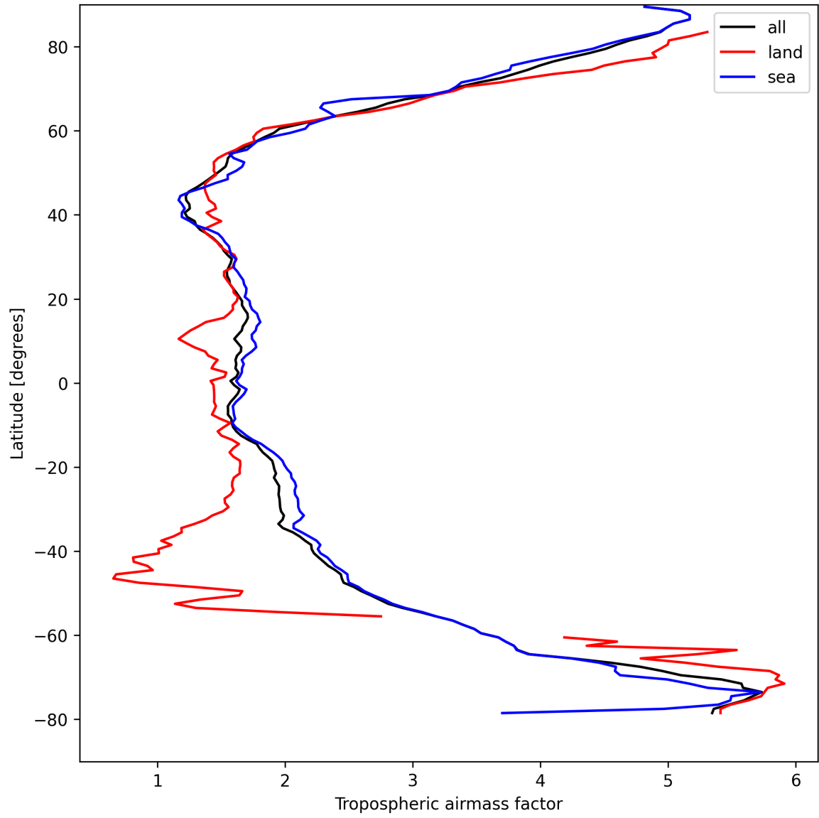
Figure 12: Zonal average of “Tropospheric airmass factor” for 2025-04-13 to 2025-04-14.
