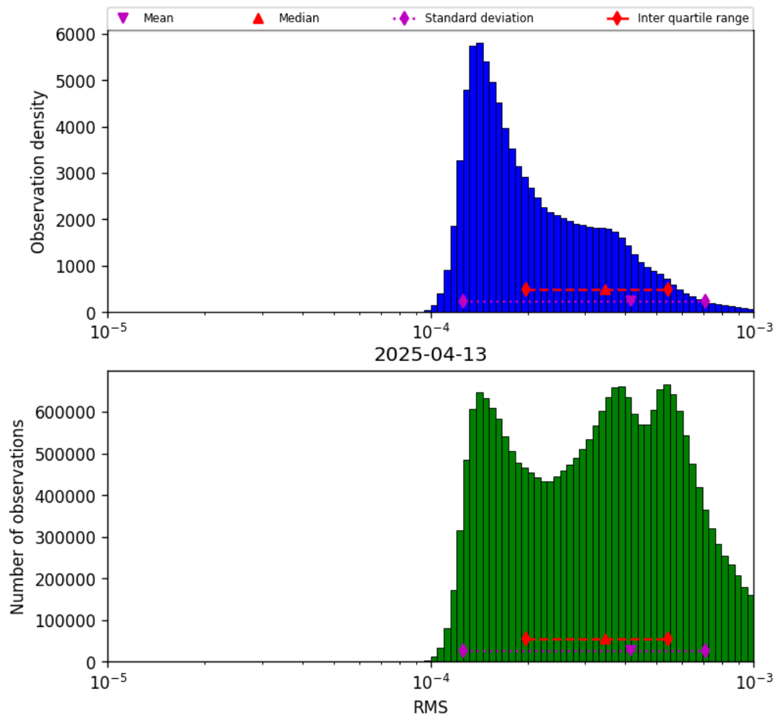
Figure 41: Histogram of “RMS” for 2025-04-13 to 2025-04-14
