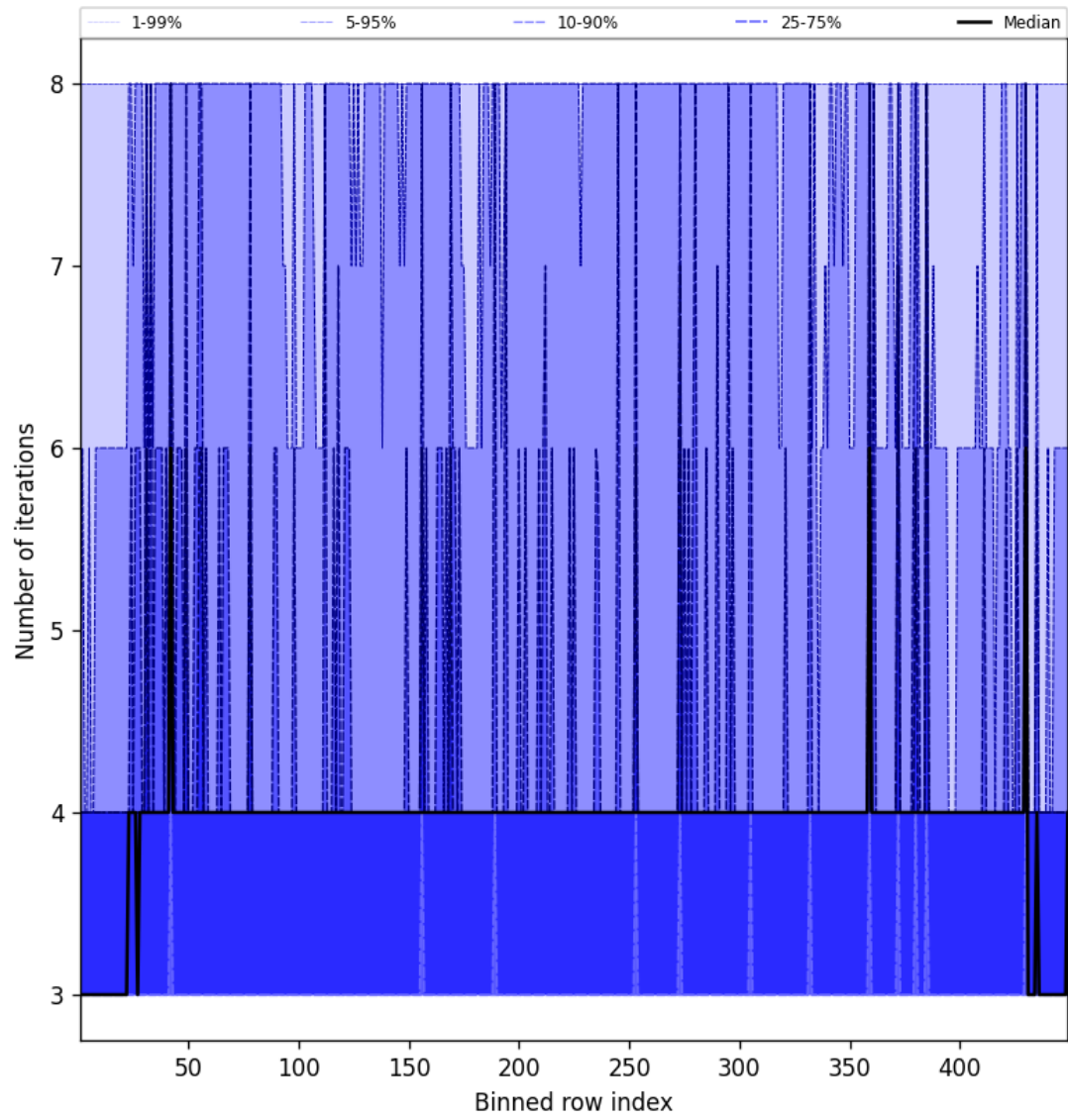
Figure 49: Along track statistics of “Number of iterations” for 2025-04-13 to 2025-04-14
