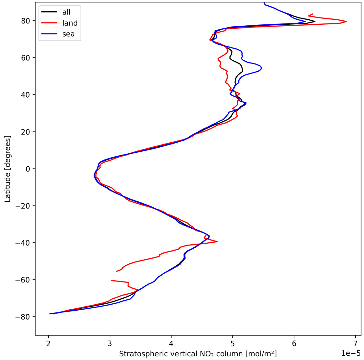
Figure 17: Zonal average of “Stratospheric vertical NO 2 column” for 2025-04-13 to 2025-04-14.
