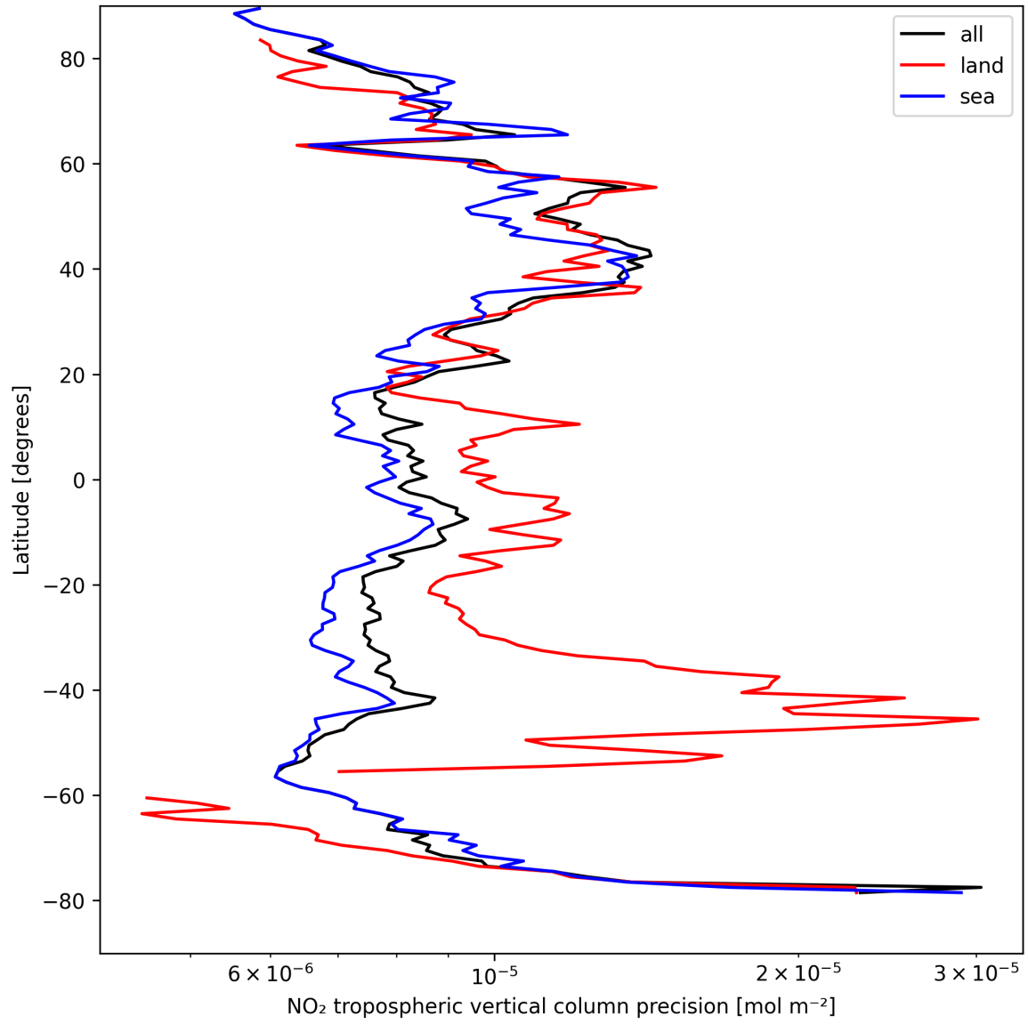
Figure 11: Zonal average of “NO 2 tropospheric vertical column precision” for 2025-04-13 to 2025-04-14.
