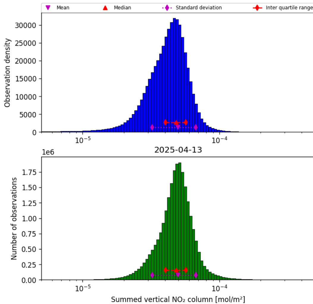
Figure 38: Histogram of "Summed vertical NO 2 column" for 2025-04-13 to 2025-04-14
