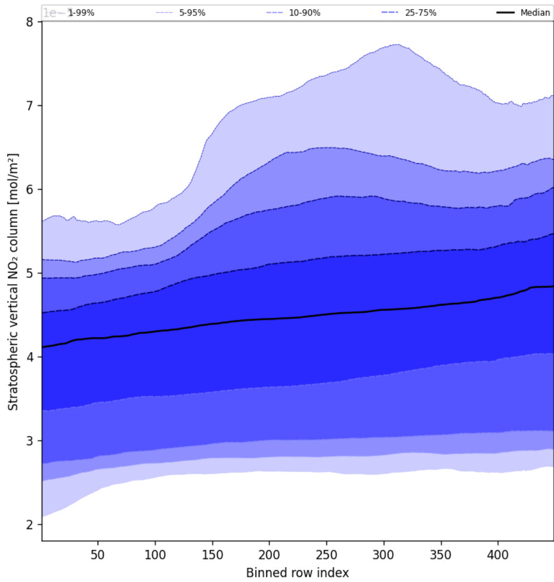
Figure 51: Along track statistics of “Stratospheric vertical NO 2 column” for 2025-04-13 to 2025-04-14
