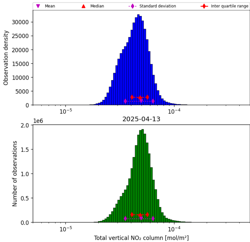
Figure 36: Histogram of “Total vertical NO 2 column” for 2025-04-13 to 2025-04-14
