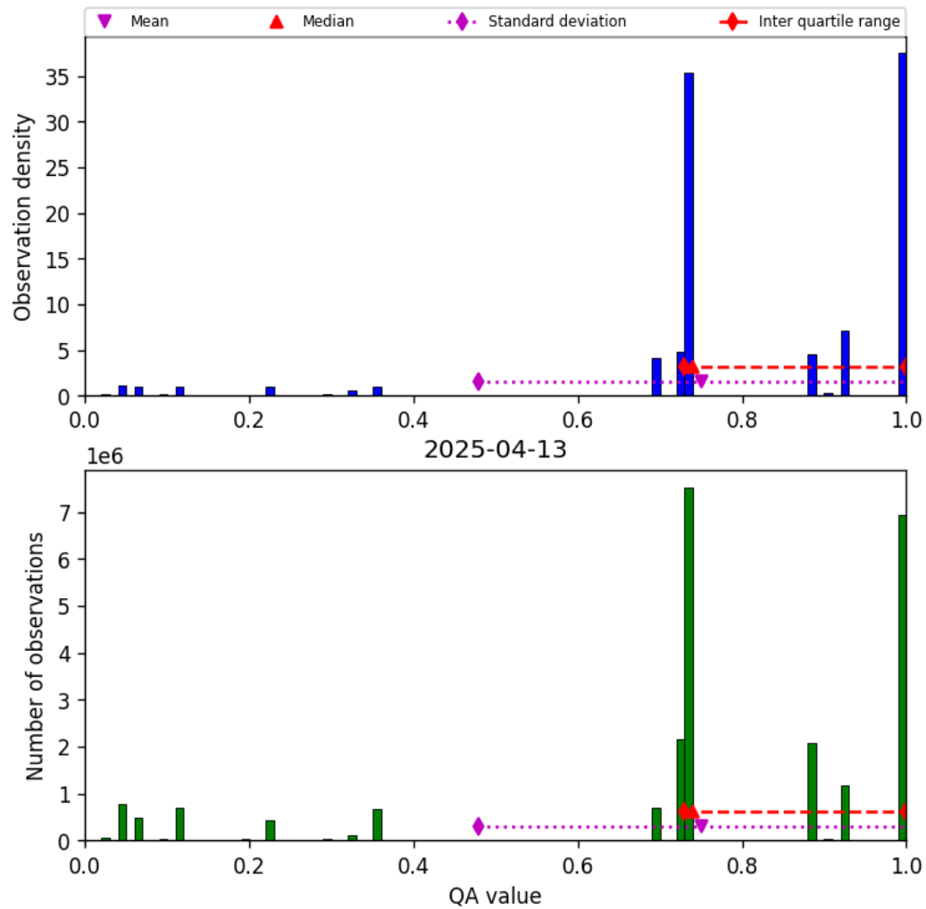
Figure 26: Histogram of “QA value” for 2025-04-13 to 2025-04-14
