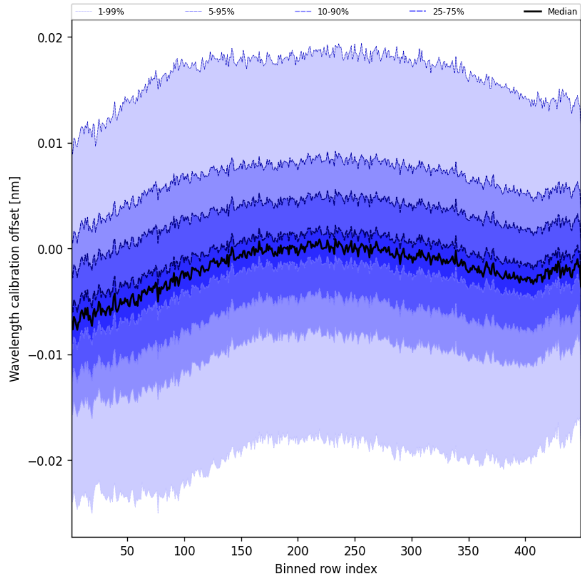
Figure 50: Along track statistics of “Wavelength calibration offset” for 2025-04-13 to 2025-04-14
