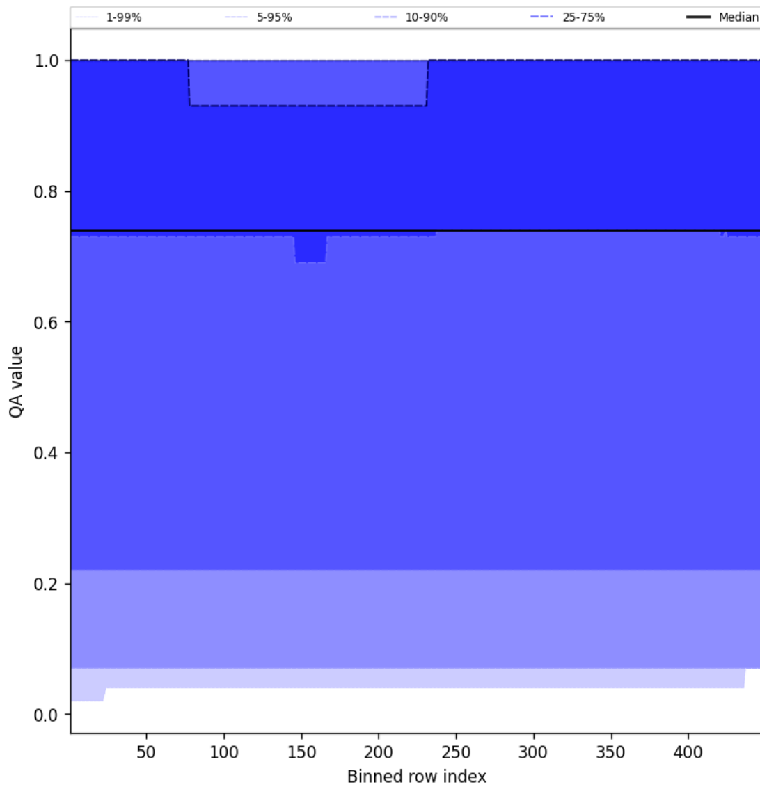
Figure 43: Along track statistics of “QA value” for 2025-04-13 to 2025-04-14
