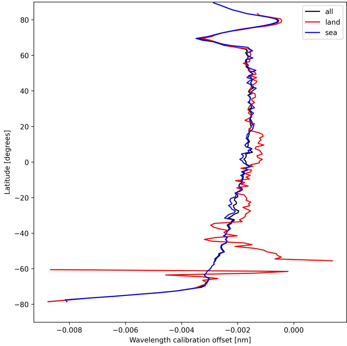
Figure 16: Zonal average of “Wavelength calibration offset” for 2025-04-13 to 2025-04-14.
