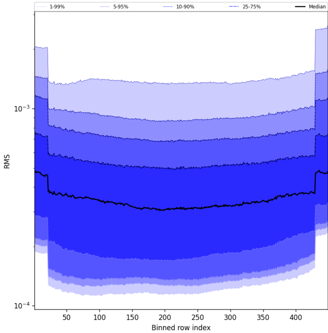
Figure 58: Along track statistics of “RMS” for 2025-04-13 to 2025-04-14
