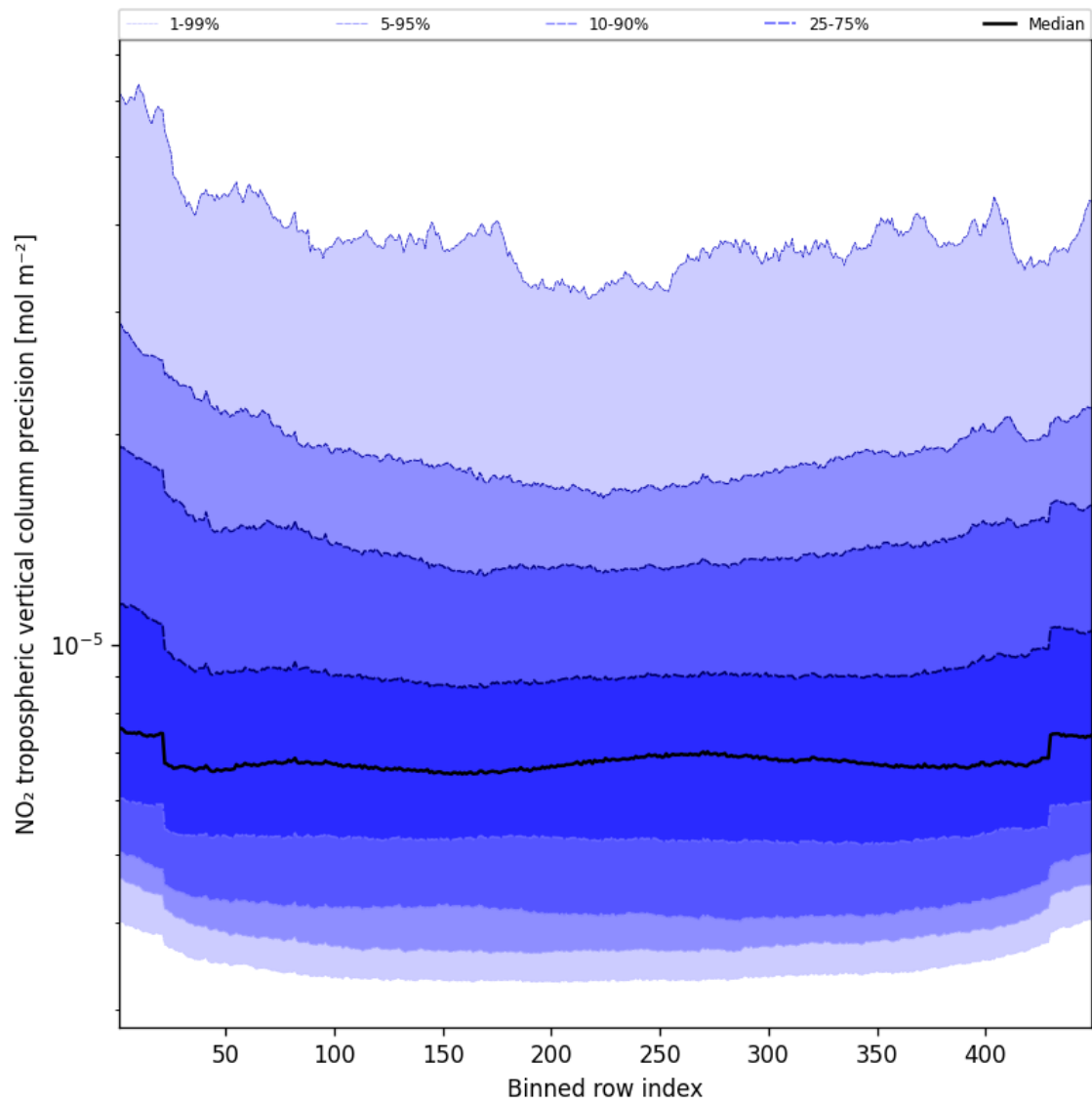
Figure 45: Along track statistics of “NO 2 tropospheric vertical column precision” for 2025-04-13 to 2025-04-14
