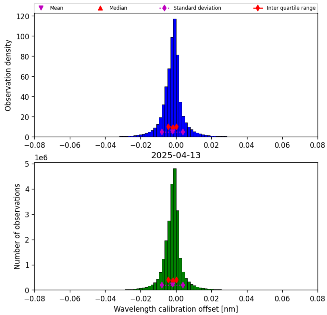
Figure 33: Histogram of “Wavelength calibration offset” for 2025-04-13 to 2025-04-14
