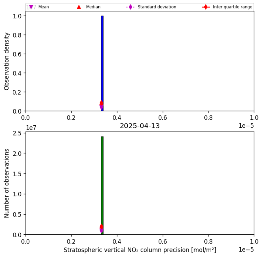
Figure 35: Histogram of “Stratospheric vertical NO 2 column precision” for 2025-04-13 to 2025-04-14
