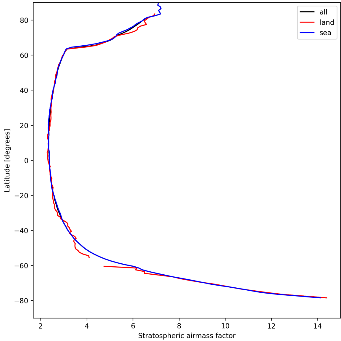
Figure 25: Zonal average of “Stratospheric air mass factor” for 2025-04-13 to 2025-04-14.
