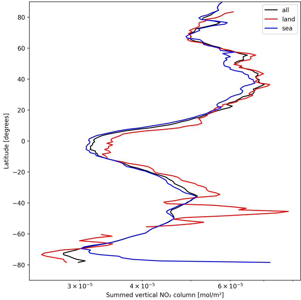
Figure 21: Zonal average of “Summed vertical NO 2 column” for 2025-04-13 to 2025-04-14.
