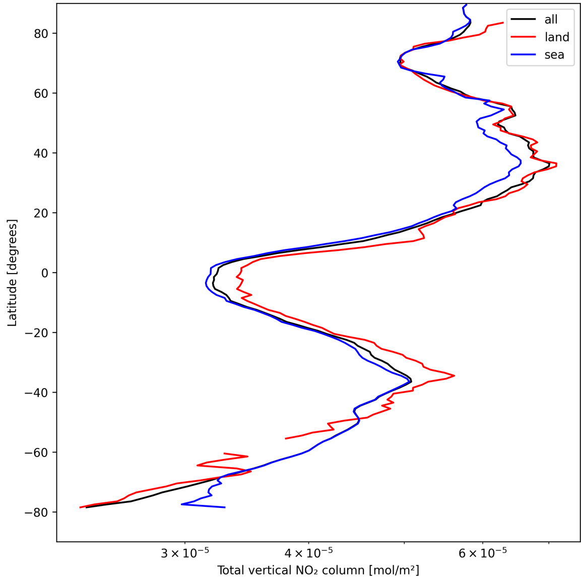
Figure 19: Zonal average of “Total vertical NO 2 column” for 2025-04-13 to 2025-04-14.
