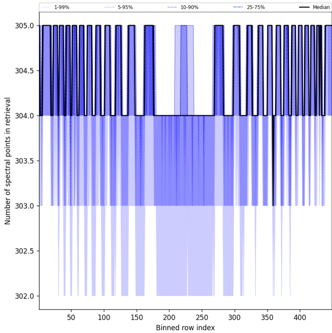
Figure 48: Along track statistics of “Number of spectral points in retrieval” for 2025-04-13 to 2025-04-14
