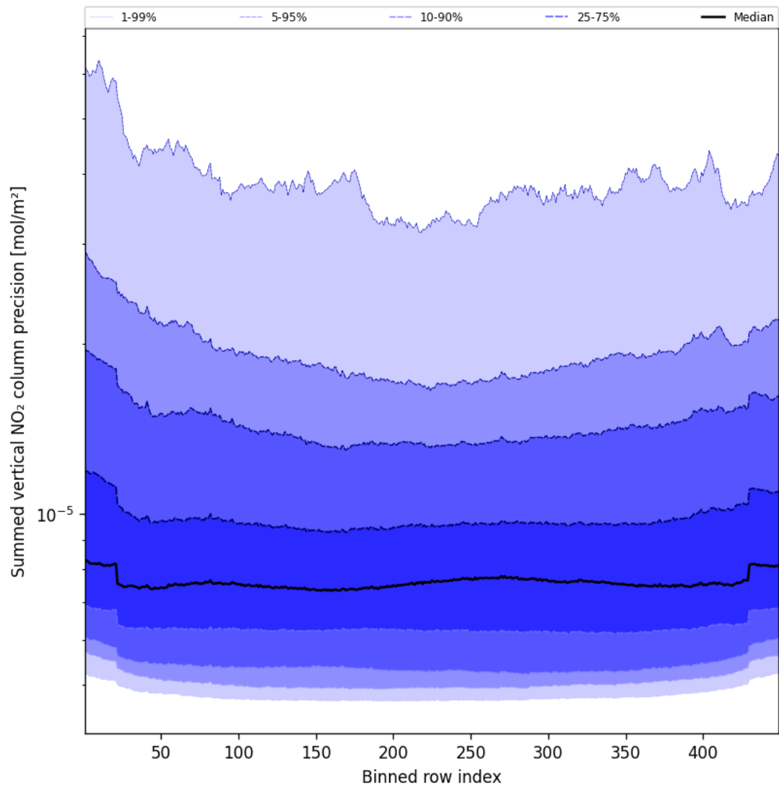
Figure 56: Along track statistics of “Summed vertical NO 2 column precision” for 2025-04-13 to 2025-04-14
