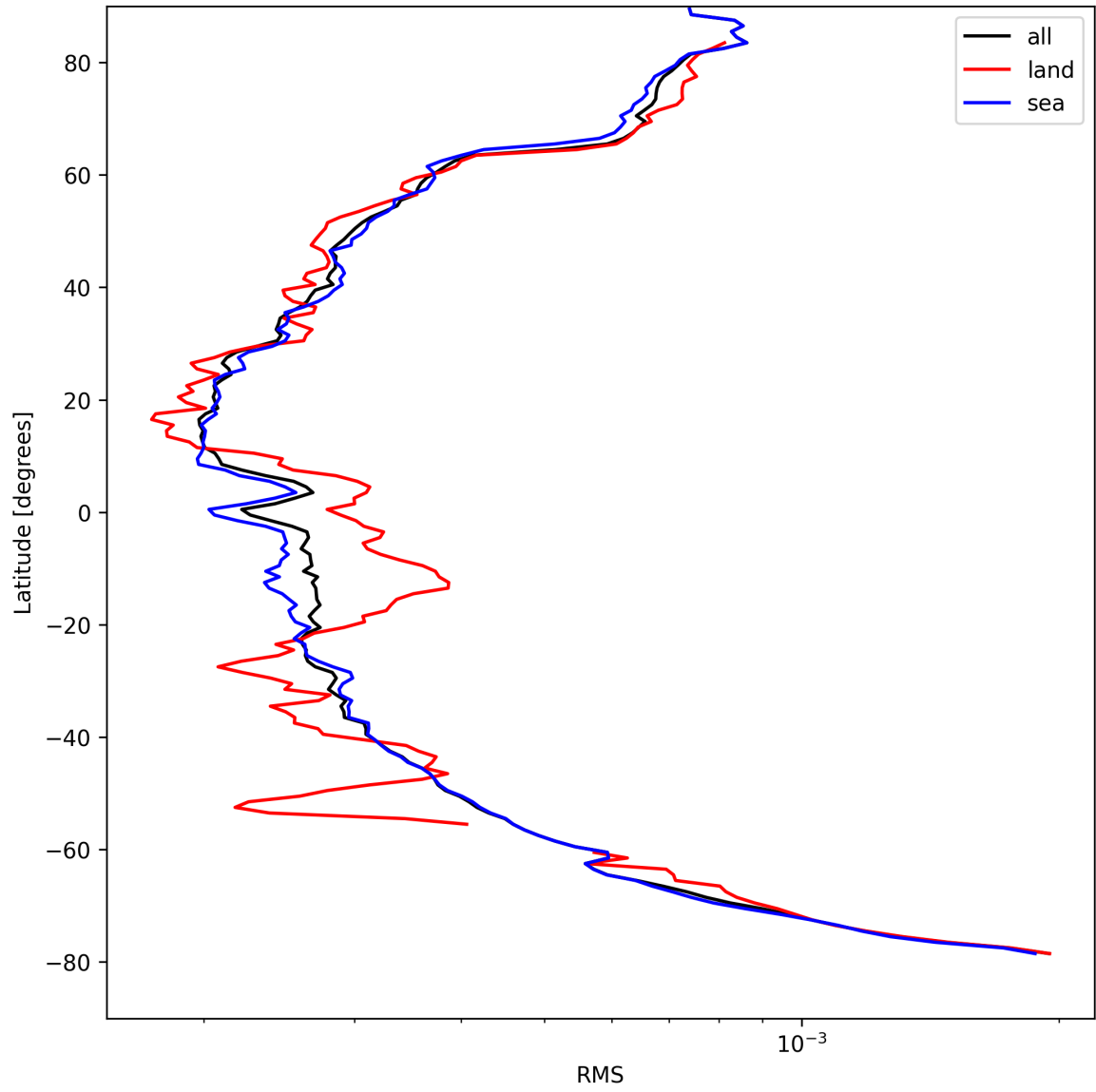
Figure 24: Zonal average of “RMS” for 2025-04-13 to 2025-04-14.
