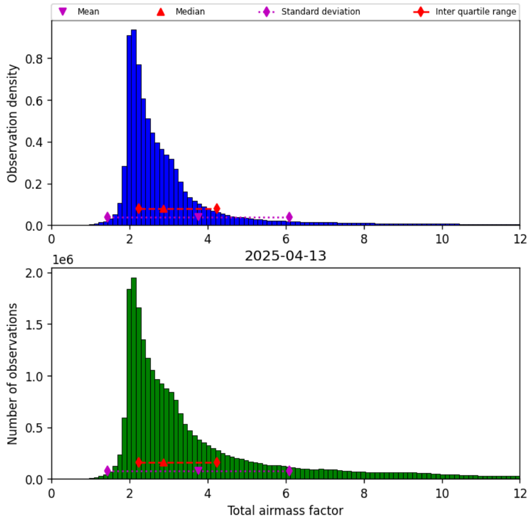
Figure 30: Histogram of “Total airmass factor” for 2025-04-13 to 2025-04-14
