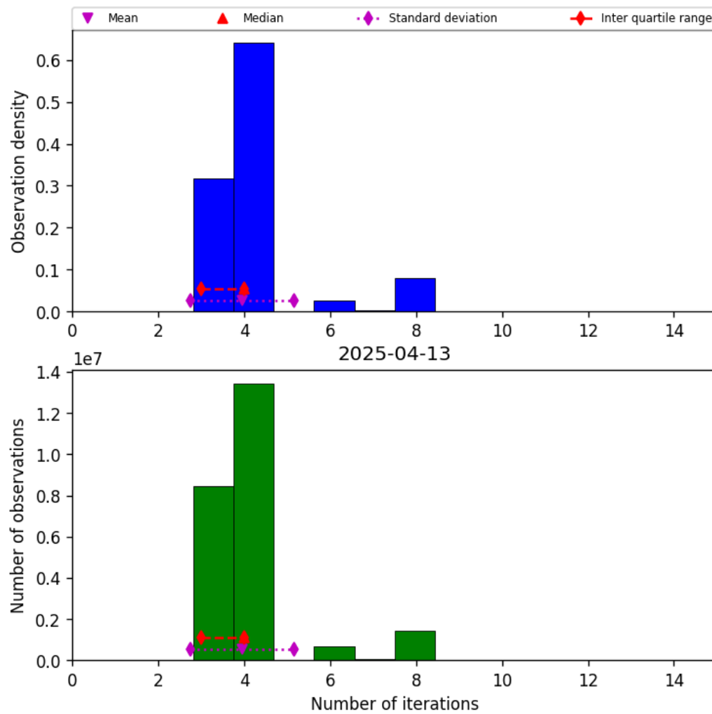
Figure 32: Histogram of “Number of iterations” for 2025-04-13 to 2025-04-14
