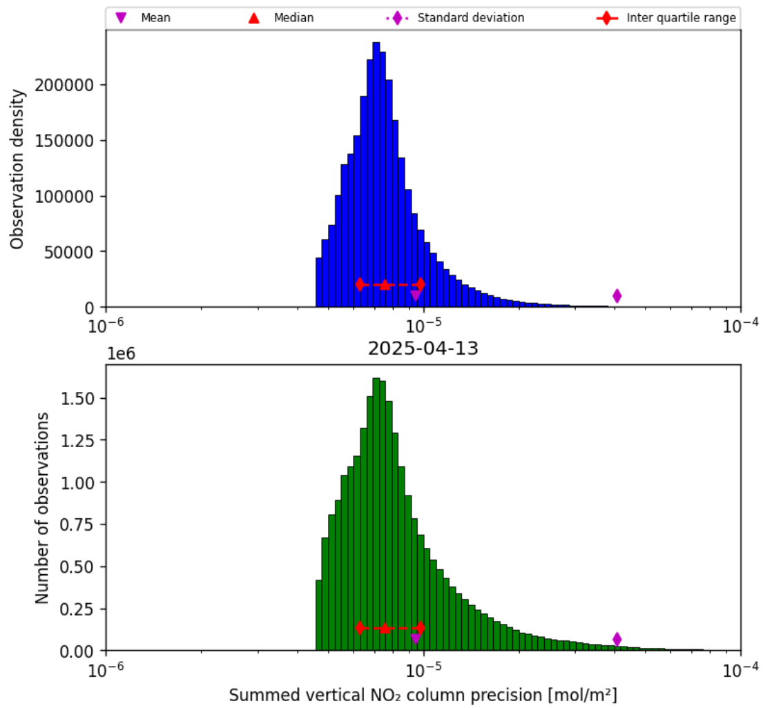
Figure 39: Histogram of “Summed vertical NO 2 column precision” for 2025-04-13 to 2025-04-14
