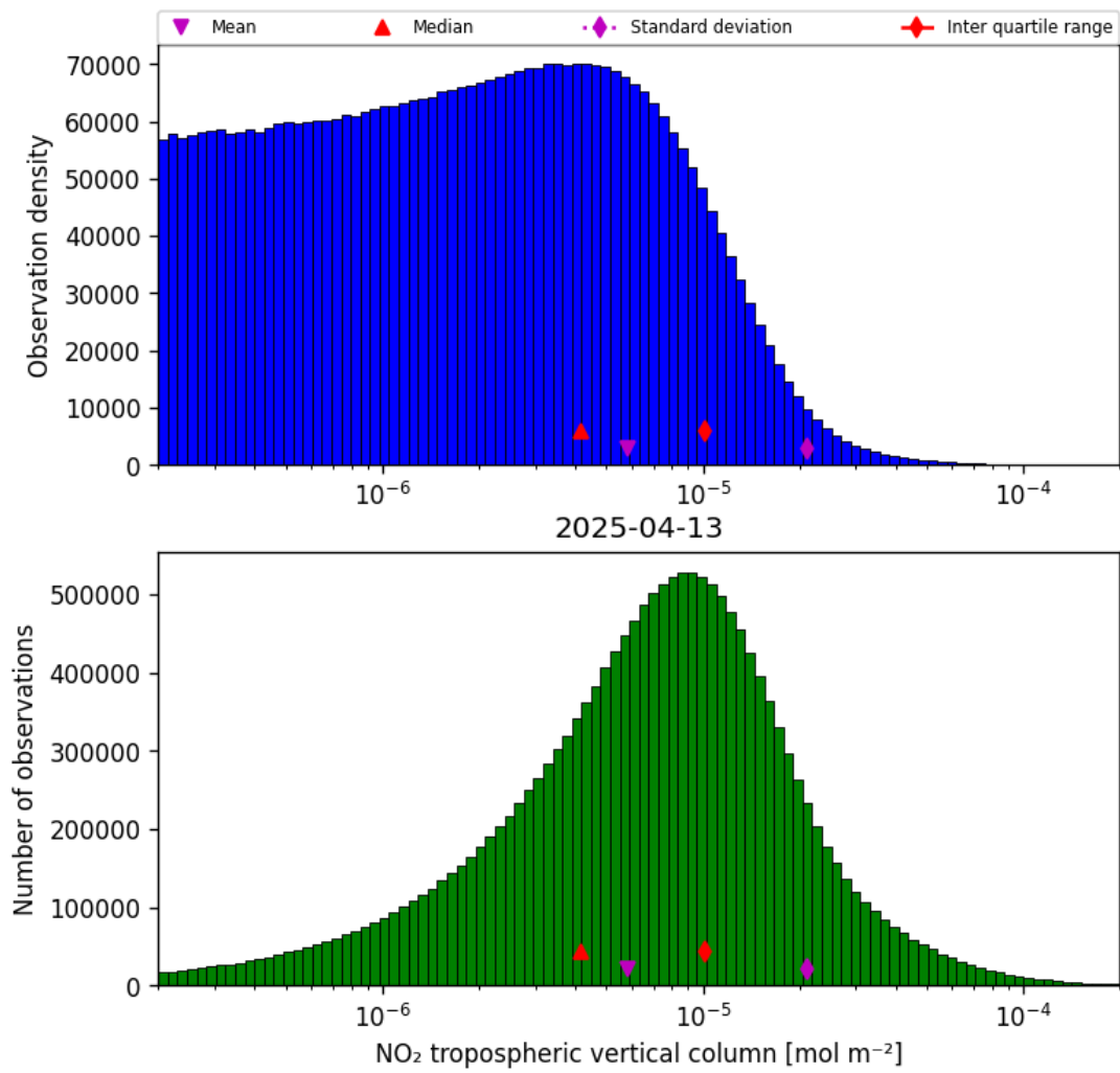
Figure 27: Histogram of “NO 2 tropospheric vertical column” for 2025-04-13 to 2025-04-14
