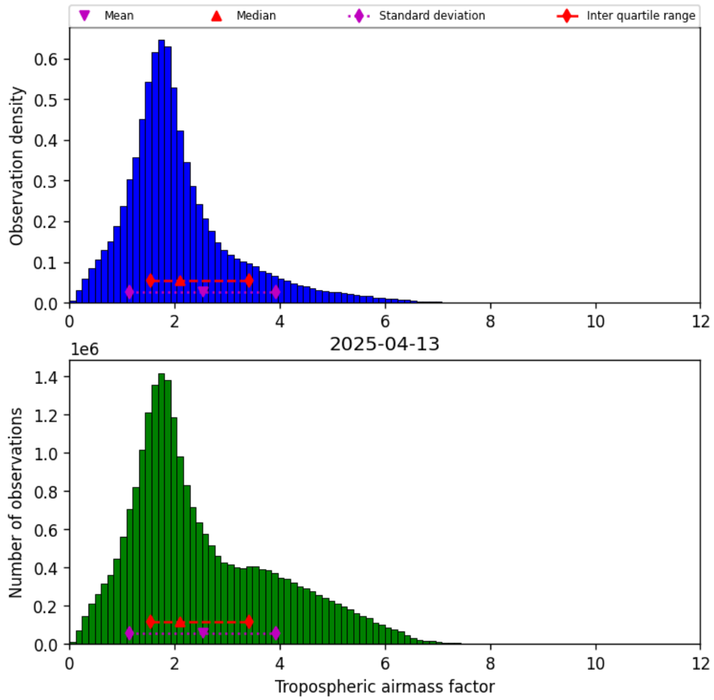
Figure 29: Histogram of “Tropospheric airmass factor” for 2025-04-13 to 2025-04-14
