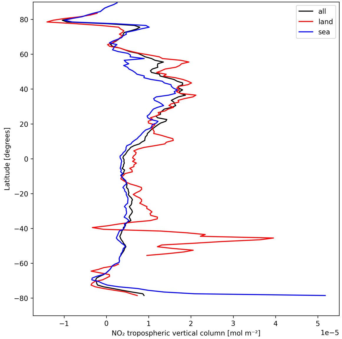
Figure 10: Zonal average of “NO 2 tropospheric vertical column” for 2025-04-13 to 2025-04-14.
