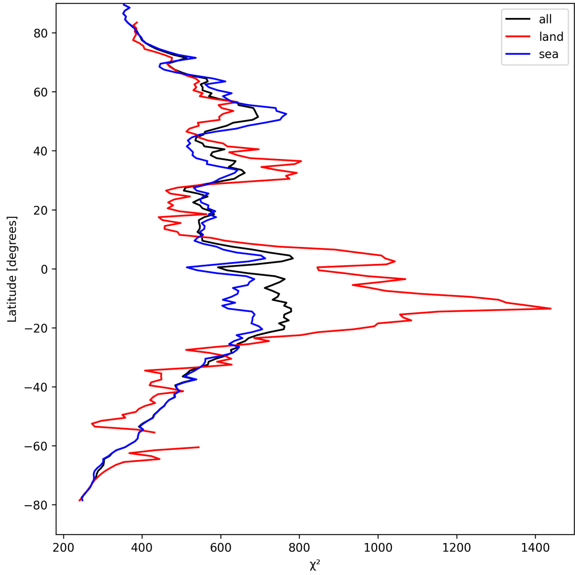
Figure 23: Zonal average of “ \chi^2 ” for 2025-04-13 to 2025-04-14.
