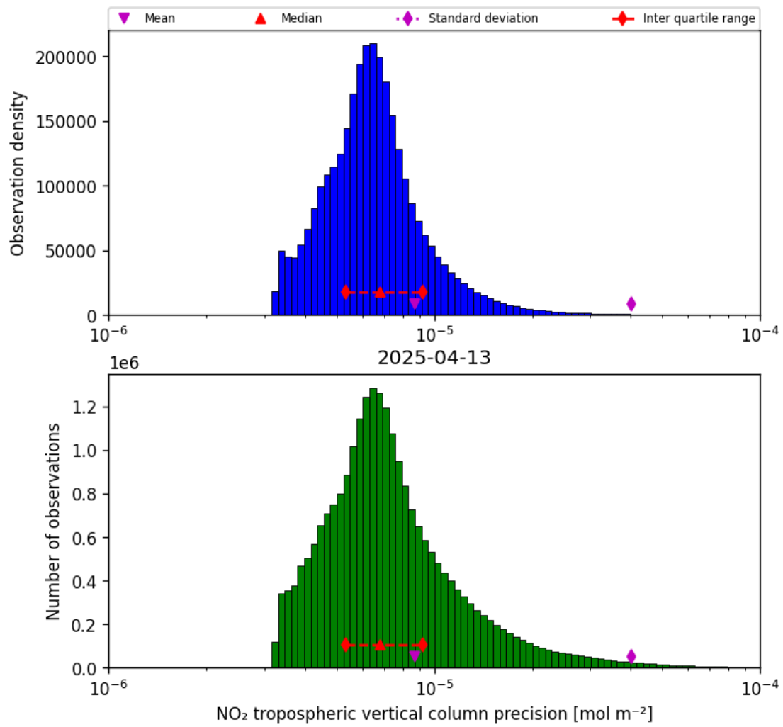
Figure 28: Histogram of “NO 2 tropospheric vertical column precision” for 2025-04-13 to 2025-04-14
