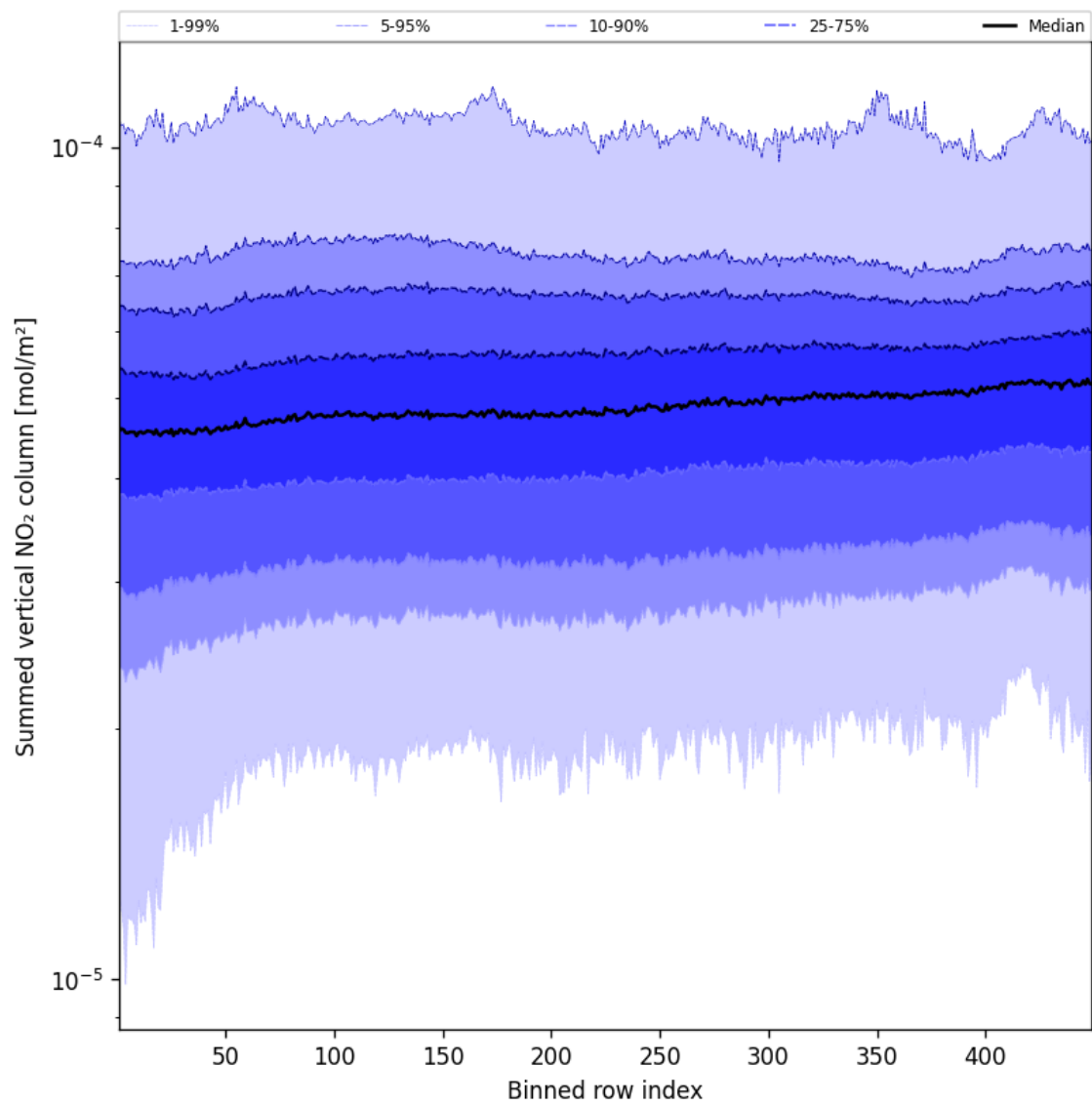
Figure 55: Along track statistics of “Summed vertical NO 2 column” for 2025-04-13 to 2025-04-14
