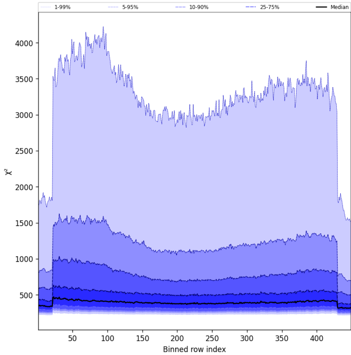
Figure 57: Along track statistics of “ \chi^2 ” for 2025-04-13 to 2025-04-14
