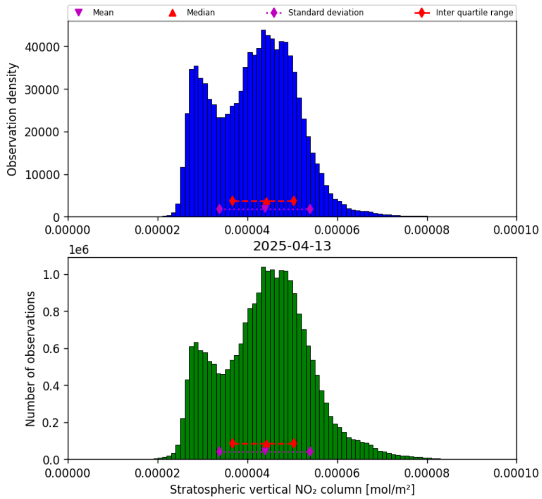
Figure 34: Histogram of “Stratospheric vertical NO 2 column” for 2025-04-13 to 2025-04-14
