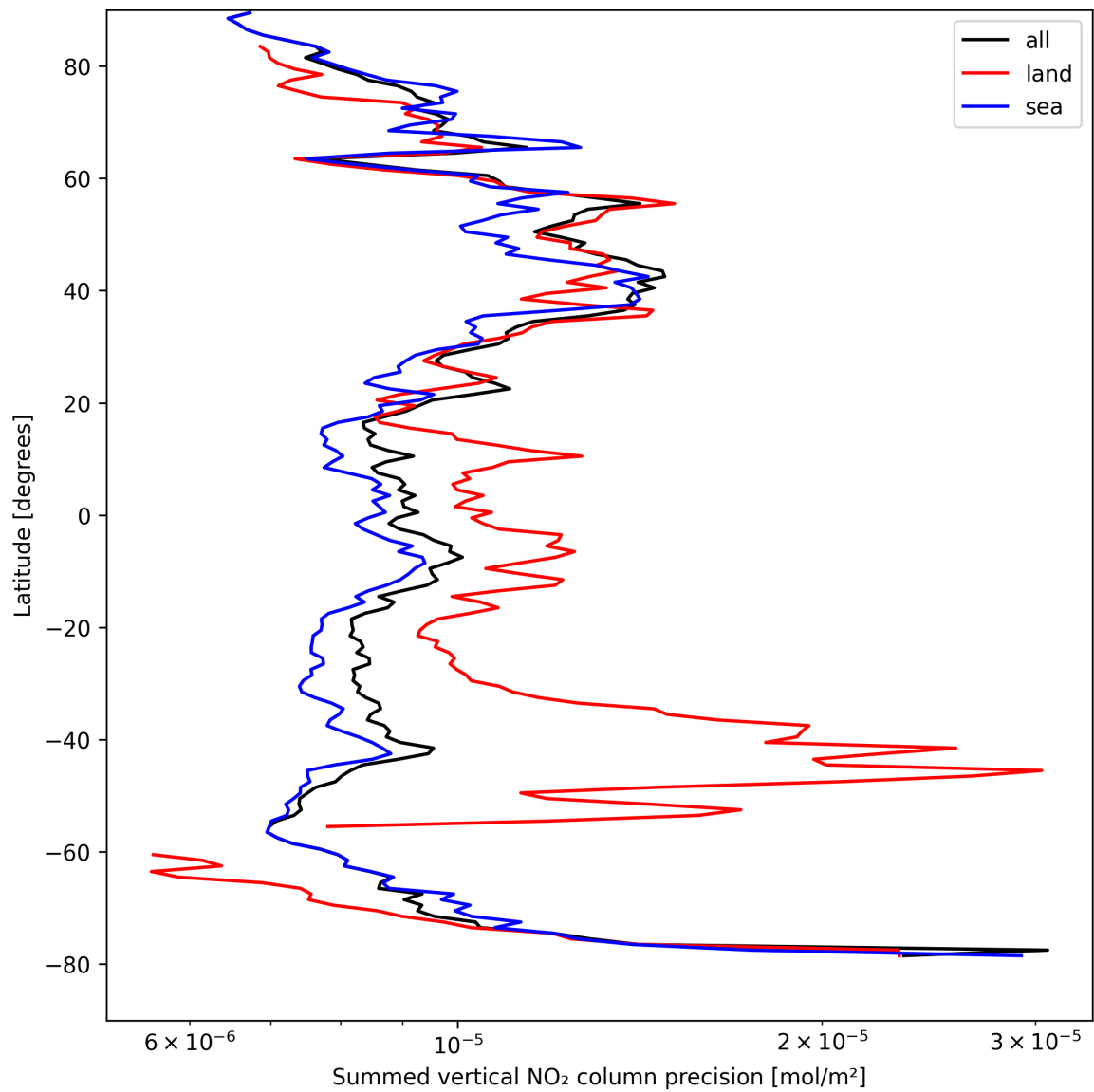
Figure 22: Zonal average of “Summed vertical NO 2 column precision” for 2025-04-13 to 2025-04-14.
