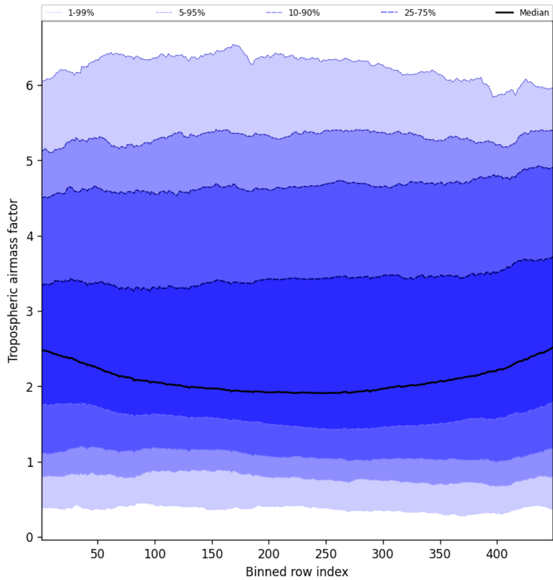
Figure 46: Along track statistics of “Tropospheric air mass factor” for 2025-04-13 to 2025-04-14
