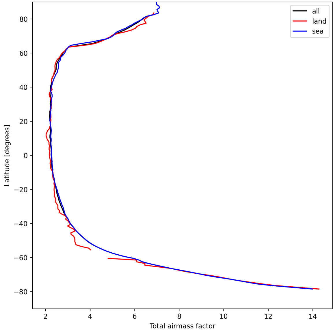
Figure 13: Zonal average of “Total airmass factor” for 2025-04-13 to 2025-04-14.
