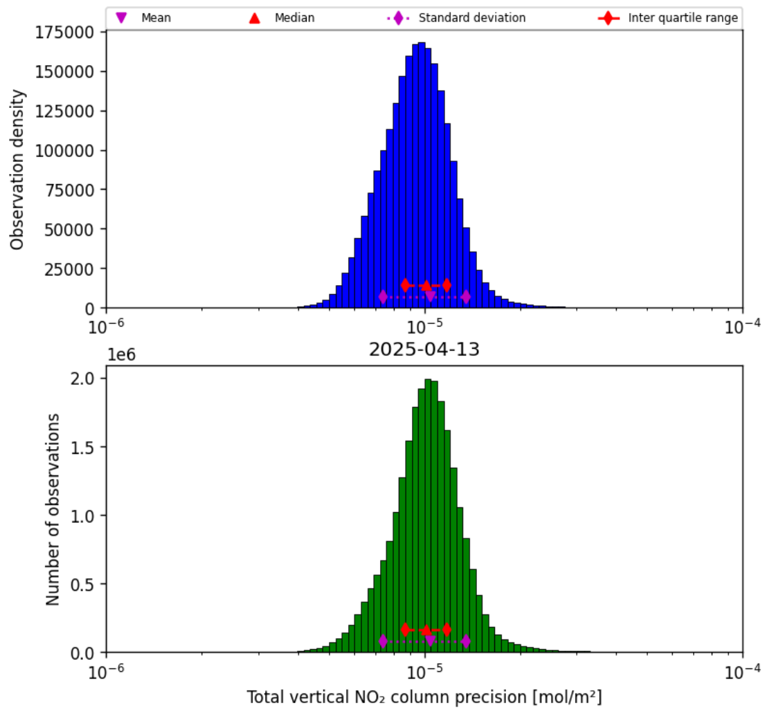
Figure 37: Histogram of “Total vertical NO 2 column precision” for 2025-04-13 to 2025-04-14
