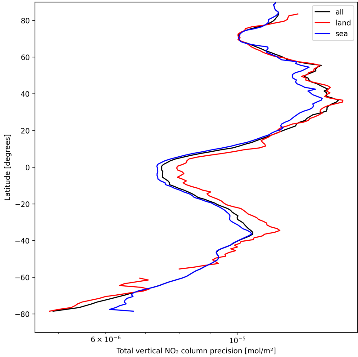
Figure 20: Zonal average of “Total vertical NO 2 column precision” for 2025-04-13 to 2025-04-14.
