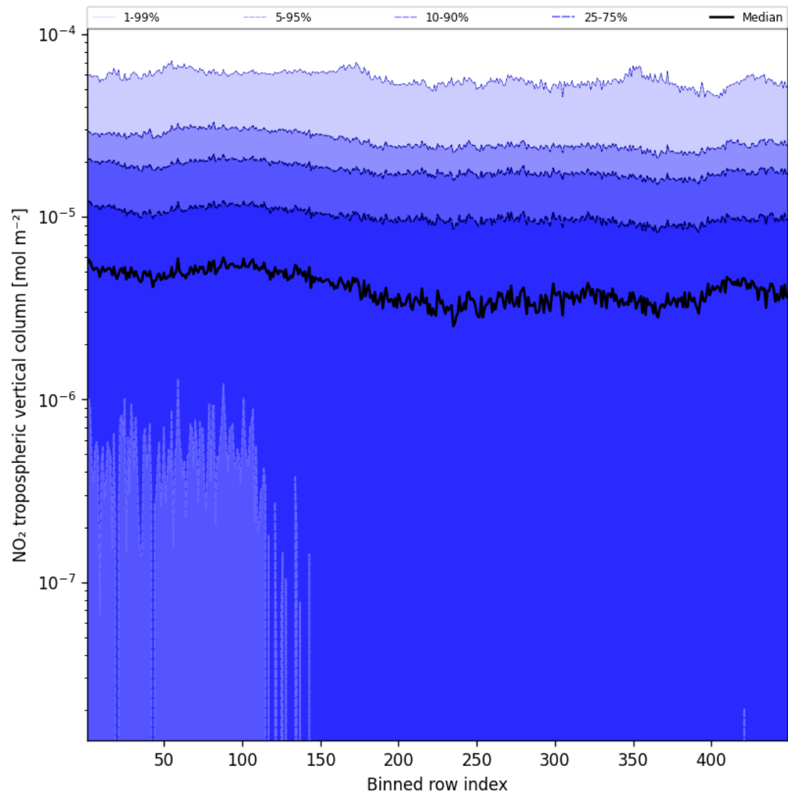
Figure 44: Along track statistics of “NO 2 tropospheric vertical column” for 2025-04-13 to 2025-04-14
