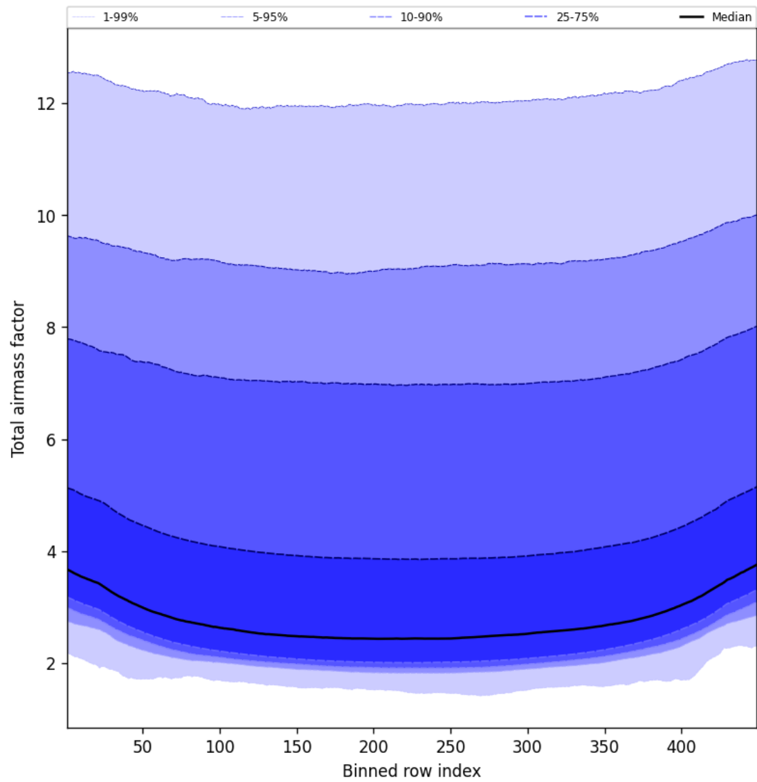
Figure 47: Along track statistics of “Total airmass factor” for 2025-04-13 to 2025-04-14
