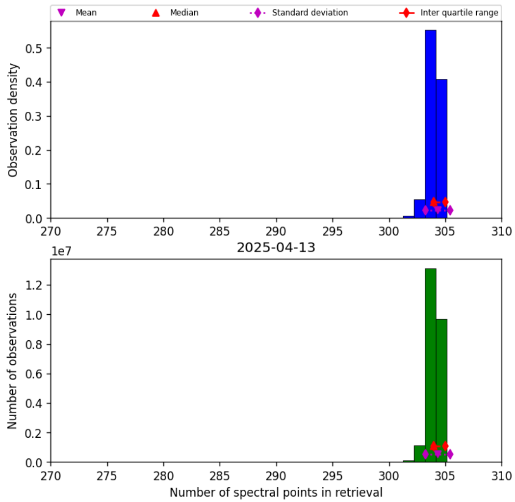
Figure 31: Histogram of “Number of spectral points in retrieval” for 2025-04-13 to 2025-04-14
