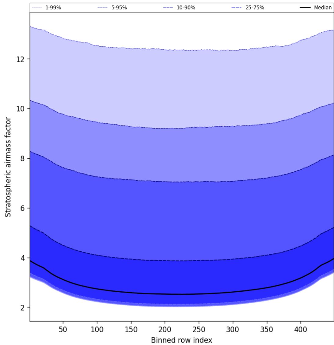
Figure 59: Along track statistics of “Stratospheric airmass factor” for 2025-04-13 to 2025-04-14
