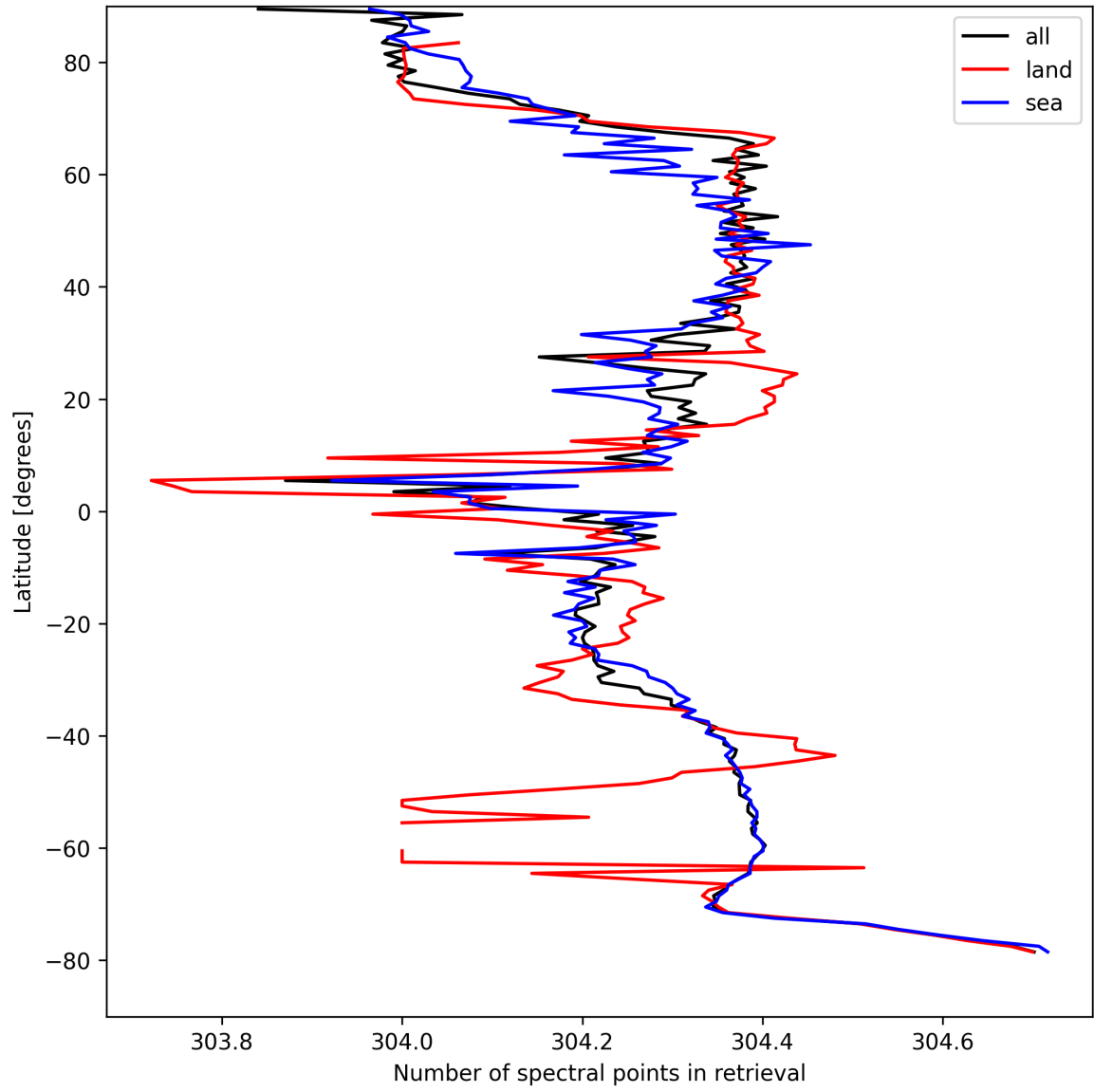
Figure 14: Zonal average of “Number of spectral points in retrieval” for 2025-04-13 to 2025-04-14.
