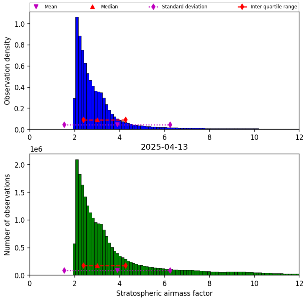
Figure 42: Histogram of “Stratospheric airmass factor” for 2025-04-13 to 2025-04-14
