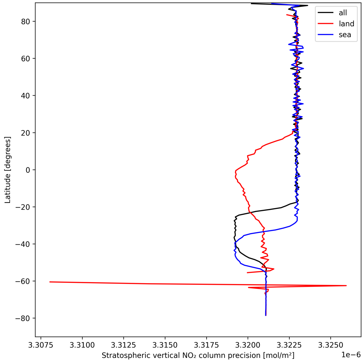
Figure 18: Zonal average of “Stratospheric vertical NO 2 column precision” for 2025-04-13 to 2025-04-14.
