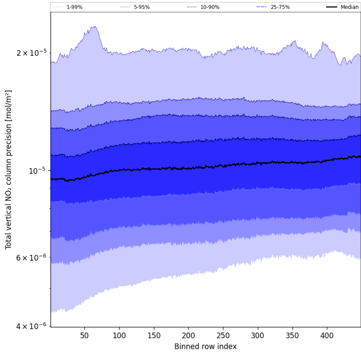
Figure 54: Along track statistics of “Total vertical NO 2 column precision” for 2025-04-13 to 2025-04-14
