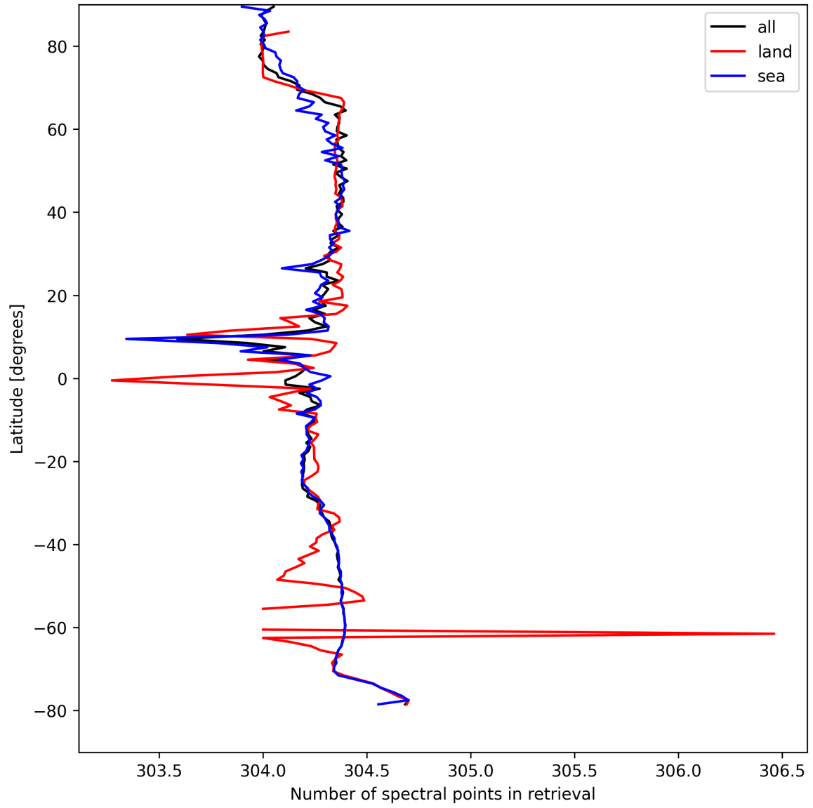
Figure 14: Zonal average of “Number of spectral points in retrieval” for 2025-04-14 to 2025-04-15.
