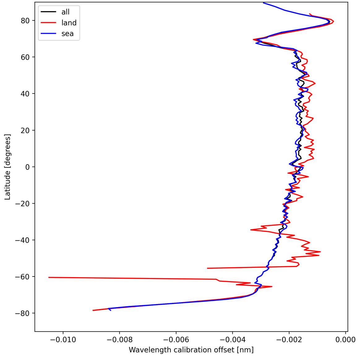
Figure 16: Zonal average of “Wavelength calibration offset” for 2025-04-14 to 2025-04-15.
