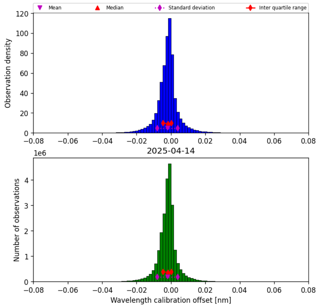
Figure 33: Histogram of “Wavelength calibration offset” for 2025-04-14 to 2025-04-15
