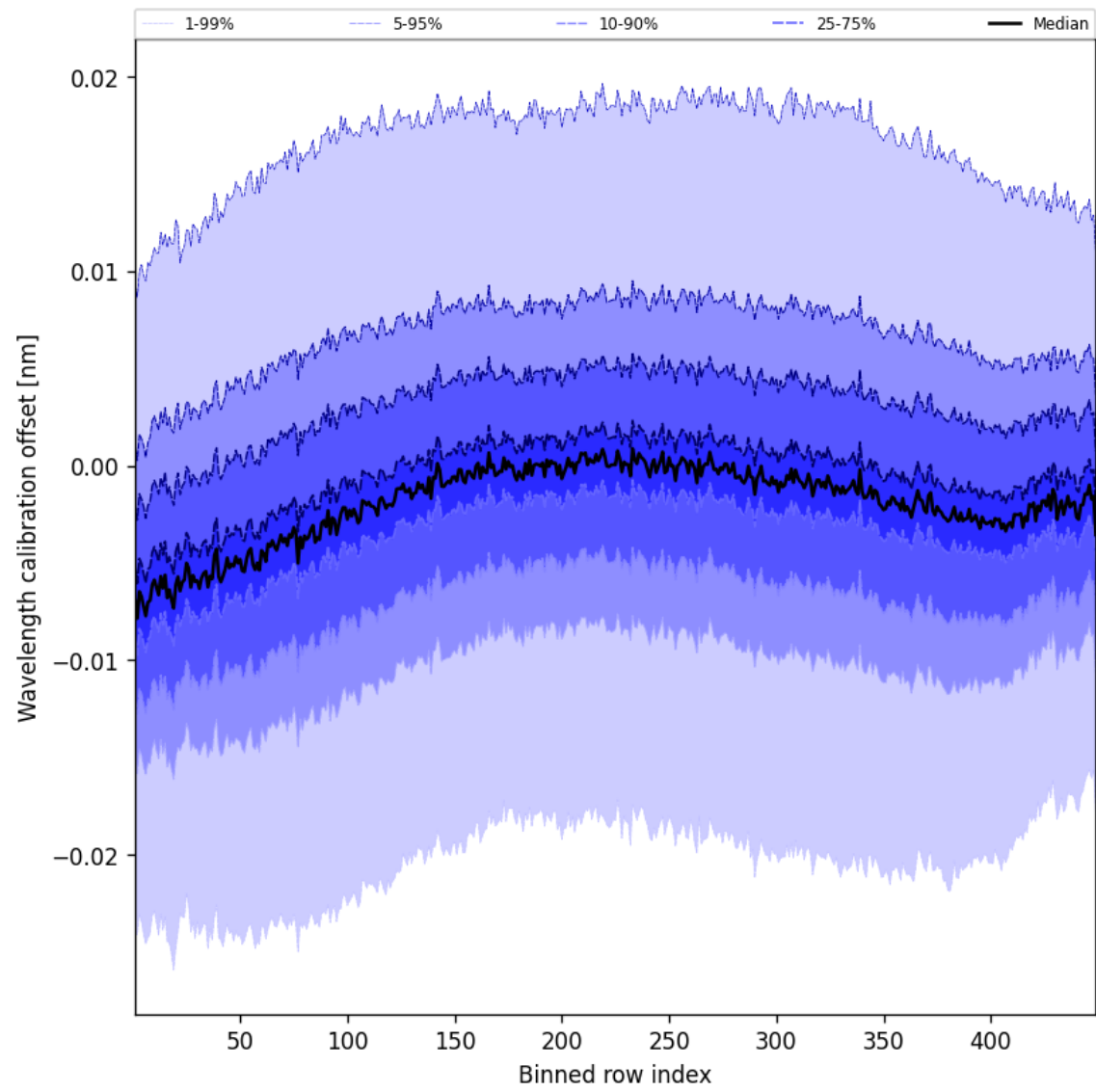
Figure 50: Along track statistics of “Wavelength calibration offset” for 2025-04-14 to 2025-04-15
