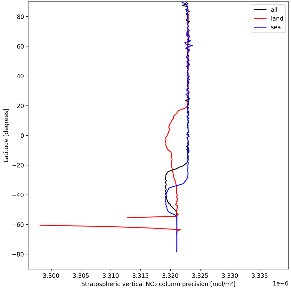
Figure 18: Zonal average of “Stratospheric vertical NO 2 column precision” for 2025-04-14 to 2025-04-15.
