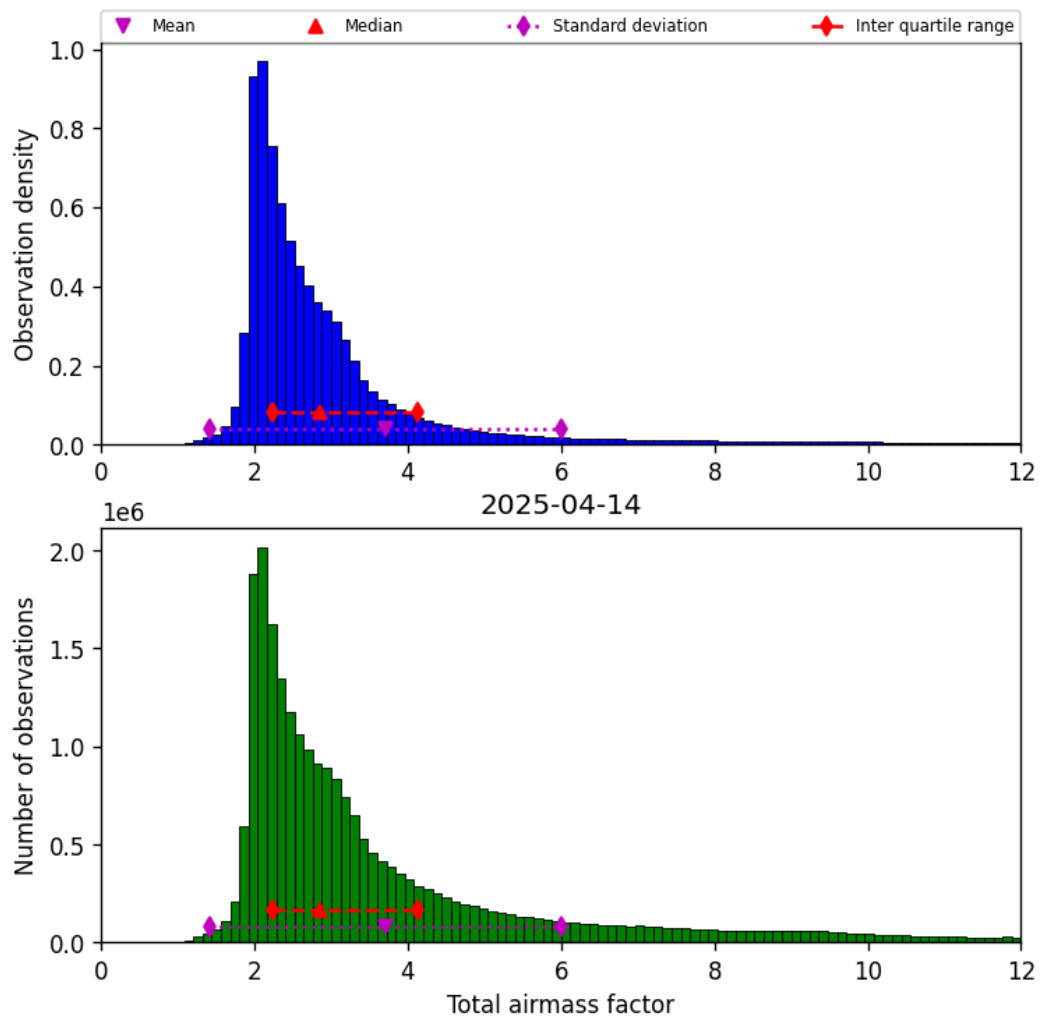
Figure 30: Histogram of “Total airmass factor” for 2025-04-14 to 2025-04-15
