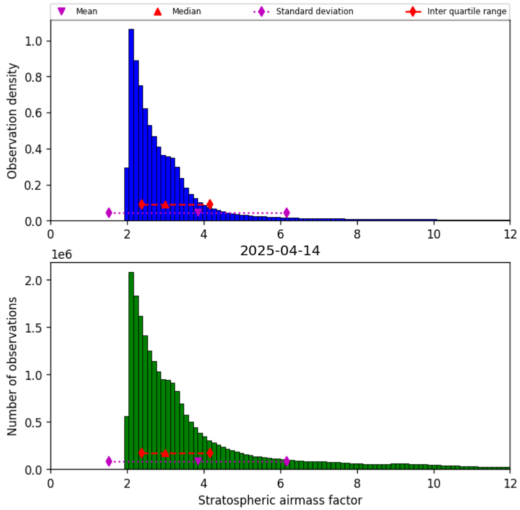
Figure 42: Histogram of “Stratospheric airmass factor” for 2025-04-14 to 2025-04-15
