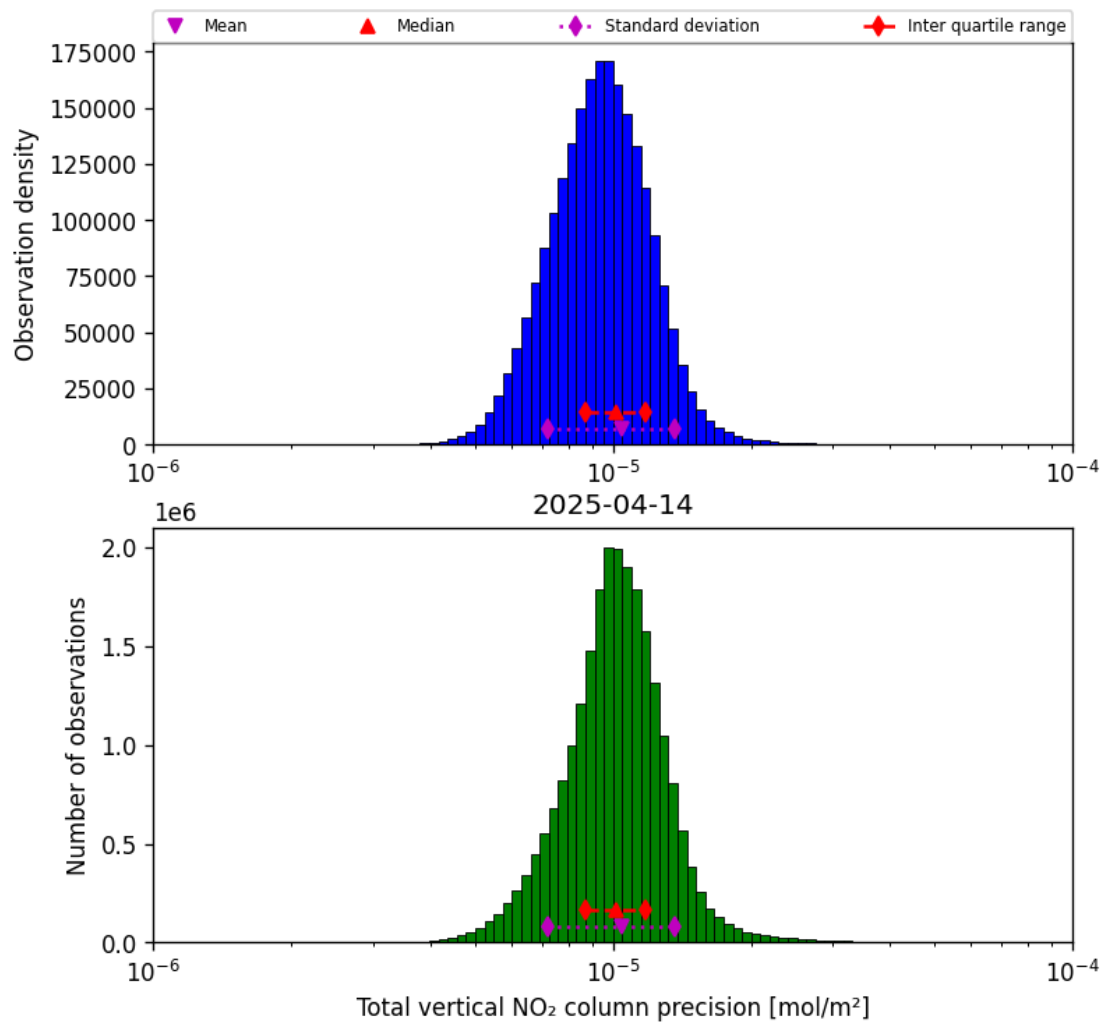
Figure 37: Histogram of “Total vertical NO 2 column precision” for 2025-04-14 to 2025-04-15
