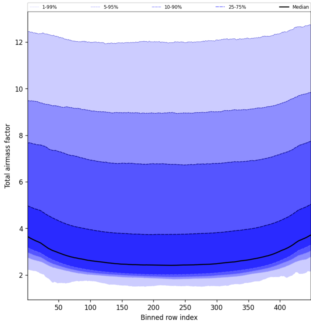
Figure 47: Along track statistics of “Total airmass factor” for 2025-04-14 to 2025-04-15
