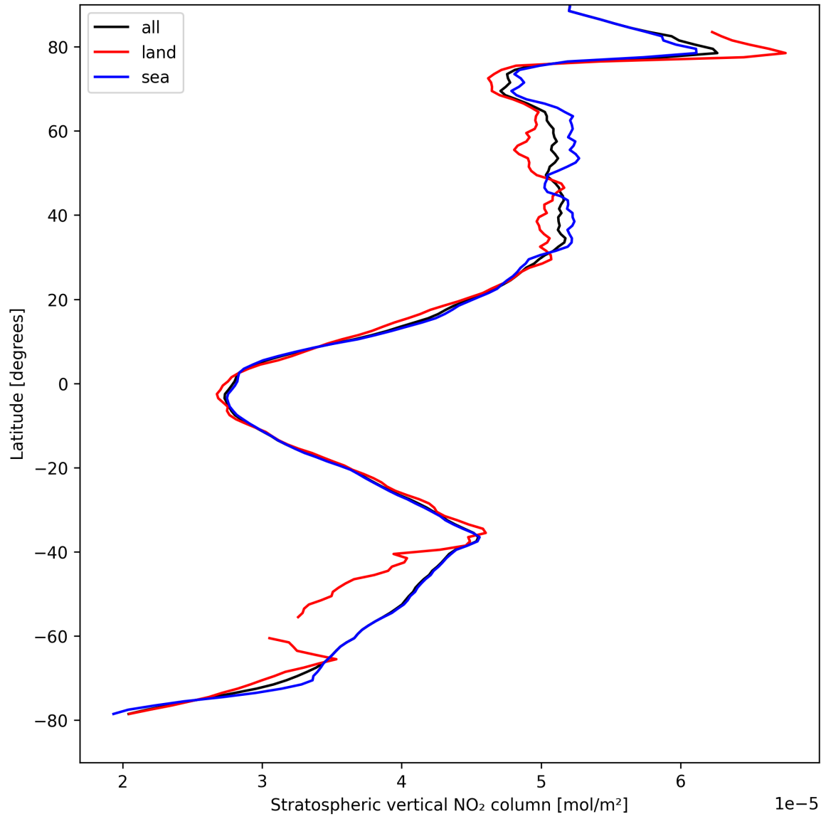
Figure 17: Zonal average of “Stratospheric vertical NO 2 column” for 2025-04-14 to 2025-04-15.
