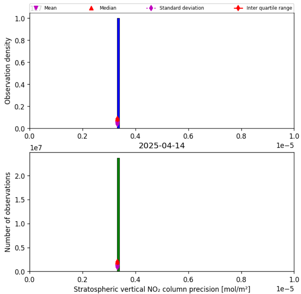
Figure 35: Histogram of “Stratospheric vertical NO 2 column precision” for 2025-04-14 to 2025-04-15
