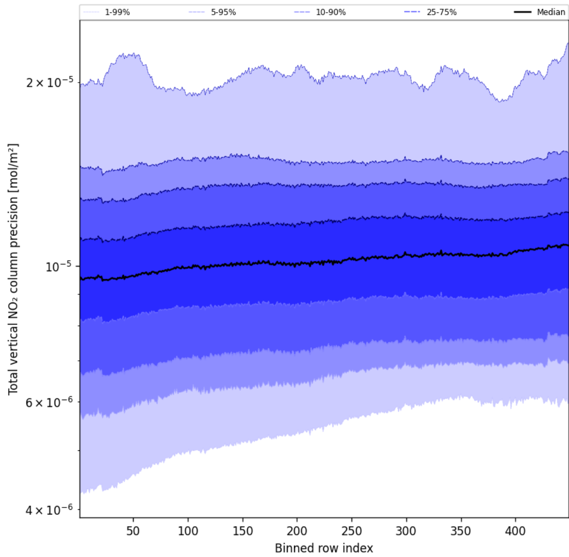
Figure 54: Along track statistics of "Total vertical NO 2 column precision" for 2025-04-14 to 2025-04-15
