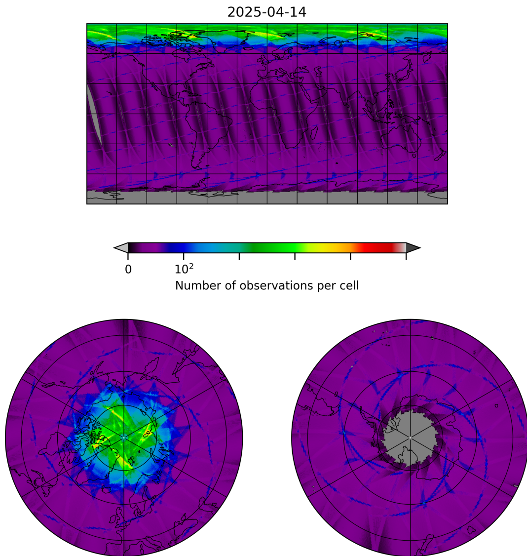
Figure 8: Map of the number of observations for 2025-04-14 to 2025-04-15
