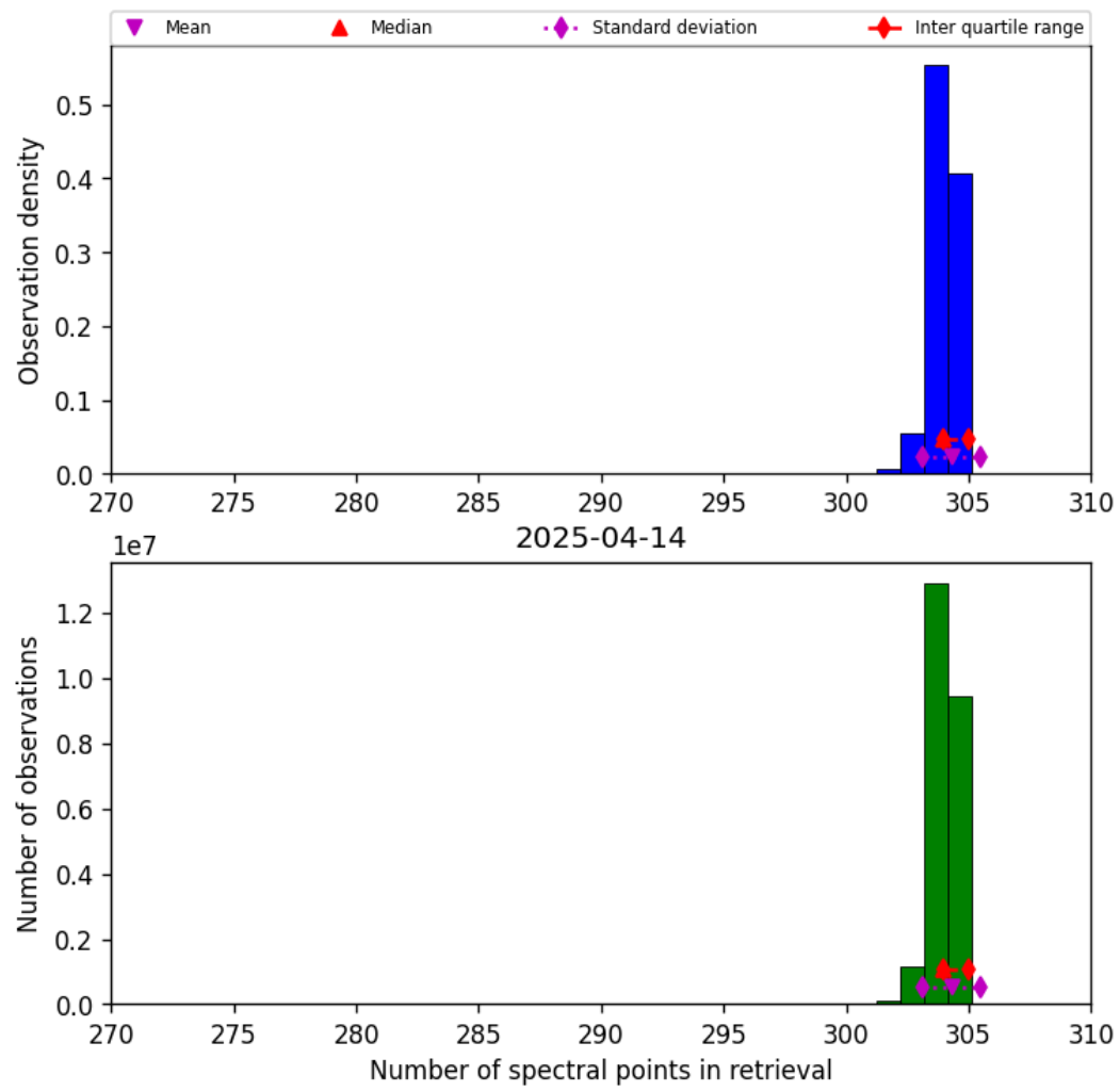
Figure 31: Histogram of “Number of spectral points in retrieval” for 2025-04-14 to 2025-04-15
