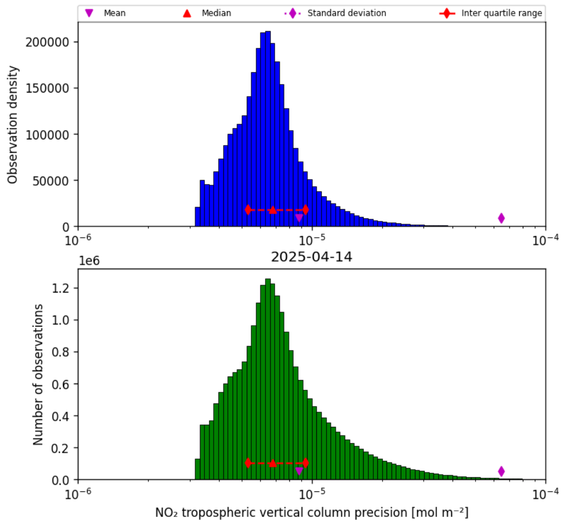
Figure 28: Histogram of “NO 2 tropospheric vertical column precision” for 2025-04-14 to 2025-04-15
