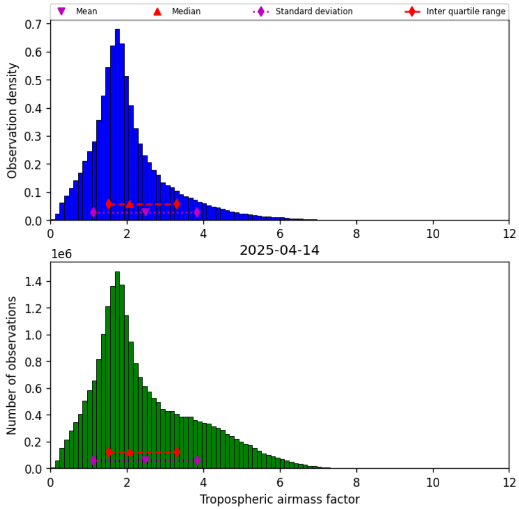
Figure 29: Histogram of “Tropospheric airmass factor” for 2025-04-14 to 2025-04-15
