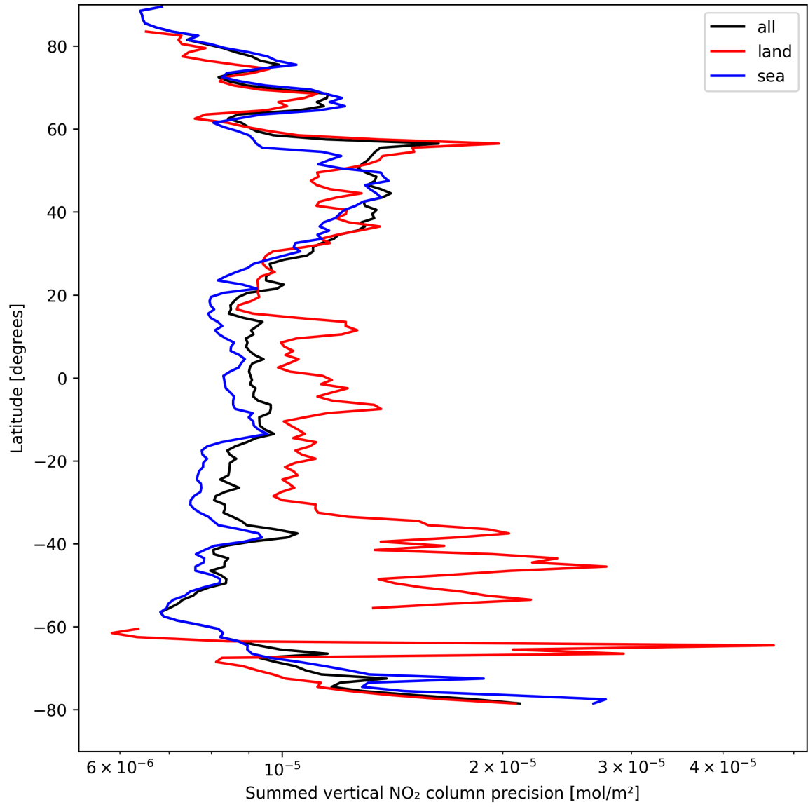
Figure 22: Zonal average of “Summed vertical NO 2 column precision” for 2025-04-14 to 2025-04-15.
