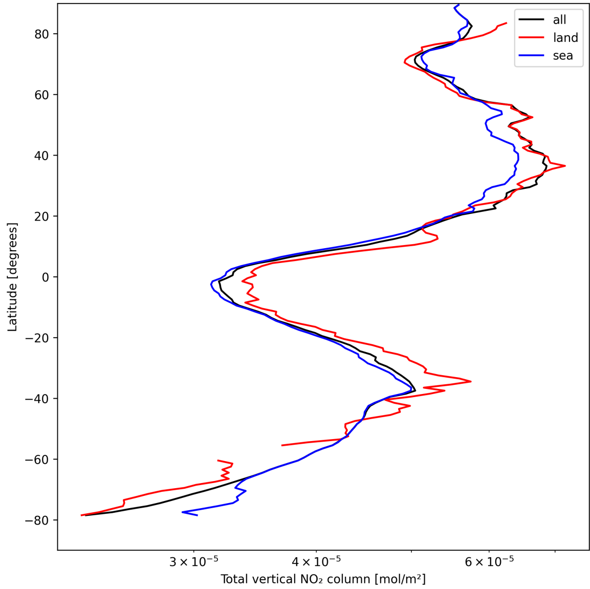
Figure 19: Zonal average of “Total vertical NO 2 column” for 2025-04-14 to 2025-04-15.
