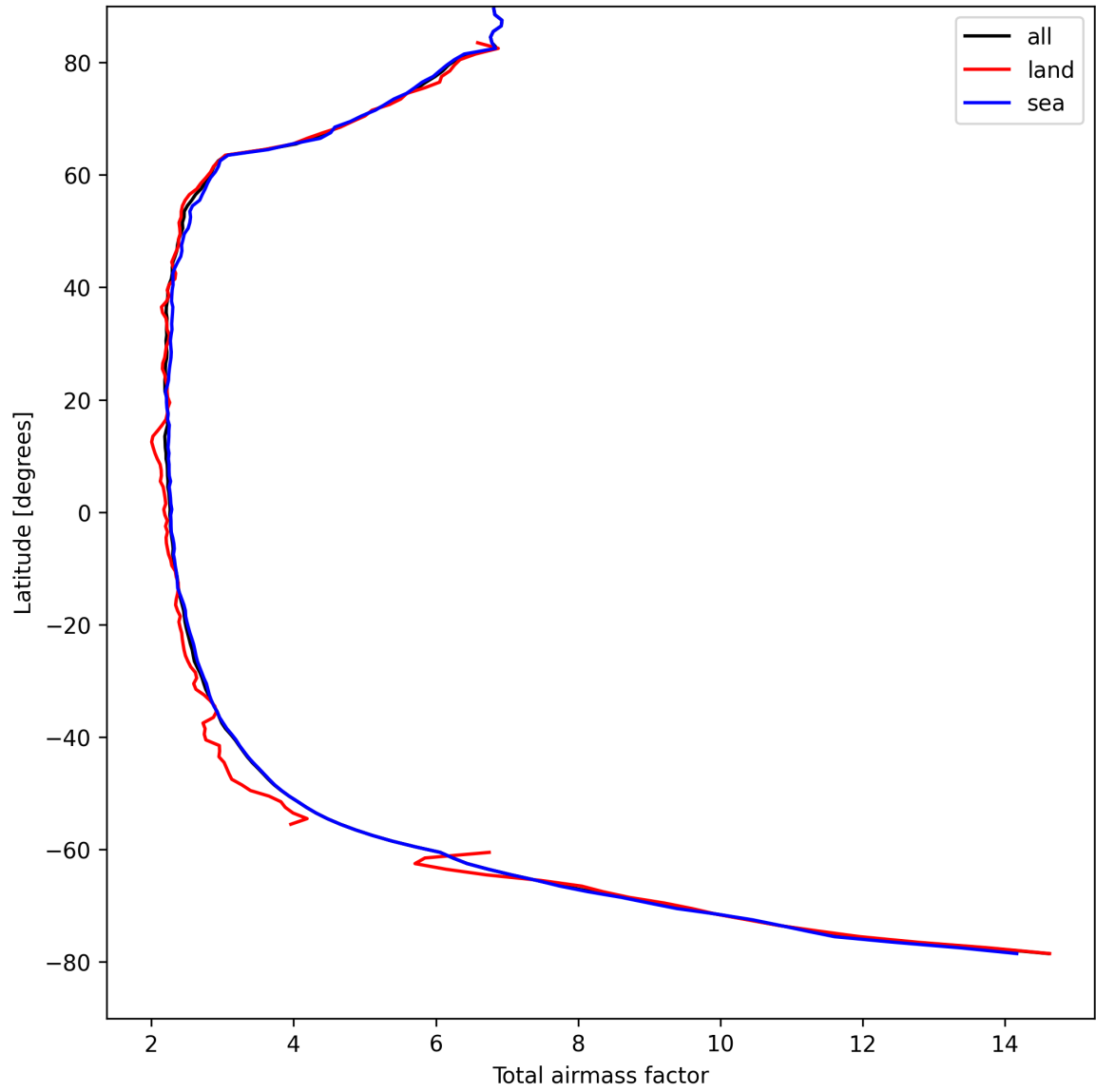
Figure 13: Zonal average of “Total airmass factor” for 2025-04-14 to 2025-04-15.
