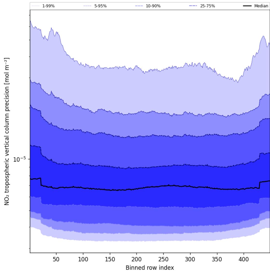
Figure 45: Along track statistics of “NO 2 tropospheric vertical column precision” for 2025-04-14 to 2025-04-15
