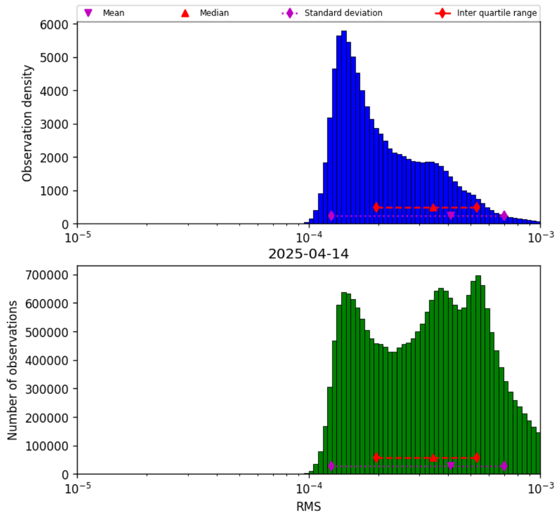
Figure 41: Histogram of “RMS” for 2025-04-14 to 2025-04-15
