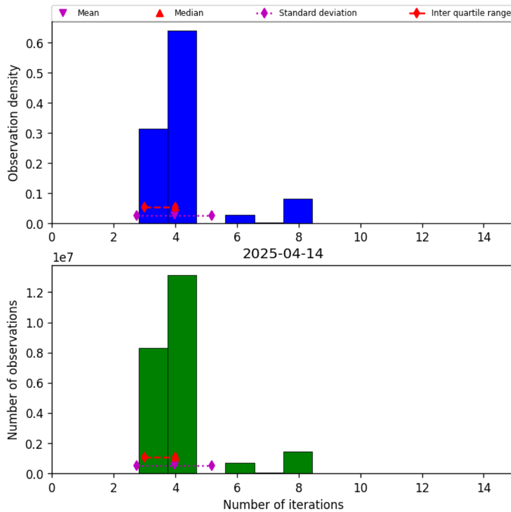
Figure 32: Histogram of “Number of iterations” for 2025-04-14 to 2025-04-15
