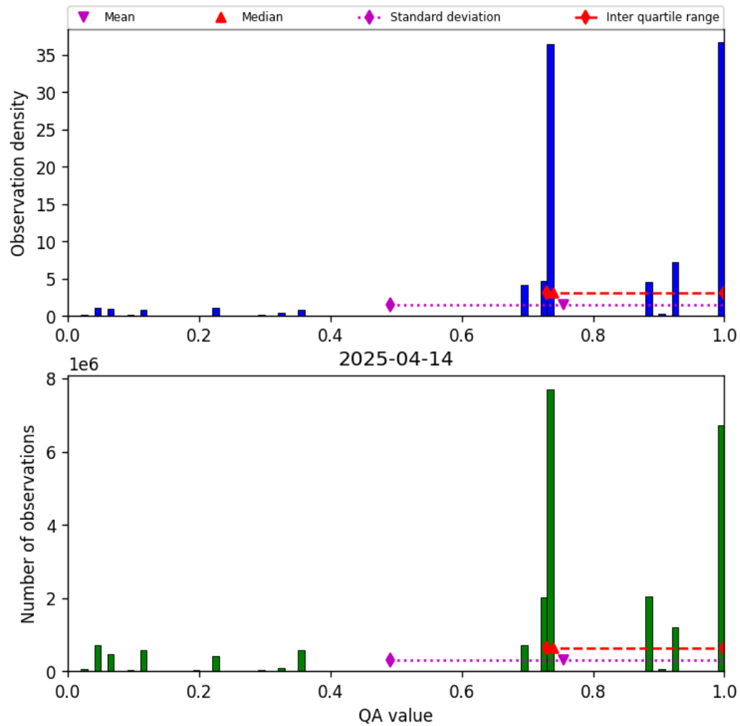
Figure 26: Histogram of “QA value” for 2025-04-14 to 2025-04-15
