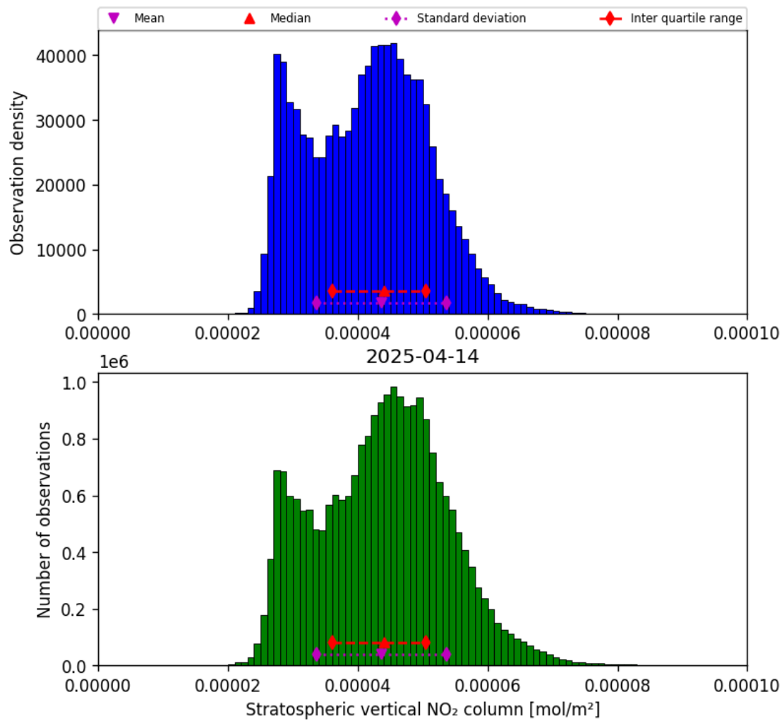
Figure 34: Histogram of “Stratospheric vertical NO 2 column” for 2025-04-14 to 2025-04-15
