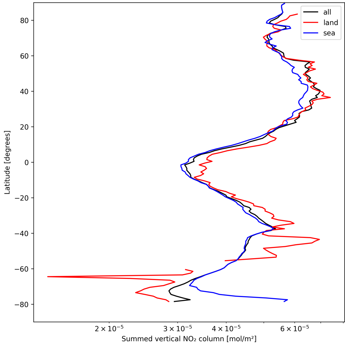
Figure 21: Zonal average of “Summed vertical NO 2 column” for 2025-04-14 to 2025-04-15.
