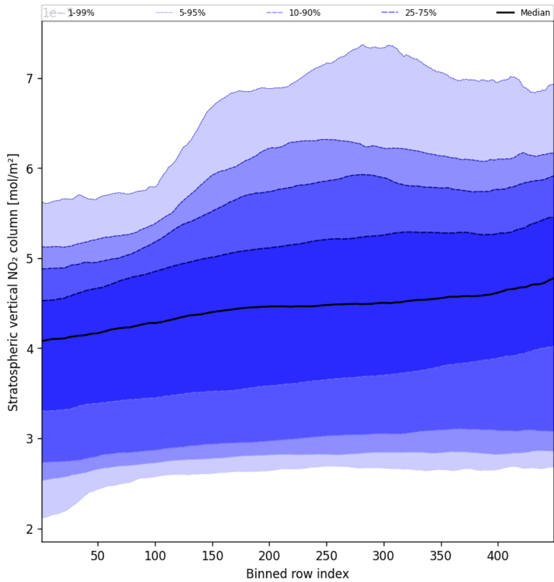
Figure 51: Along track statistics of “Stratospheric vertical NO 2 column” for 2025-04-14 to 2025-04-15
