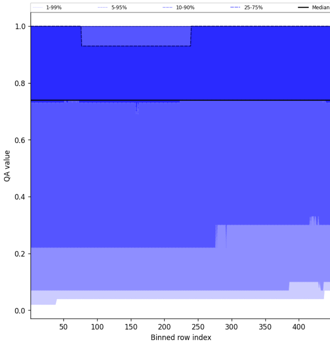
Figure 43: Along track statistics of “QA value” for 2025-04-14 to 2025-04-15
