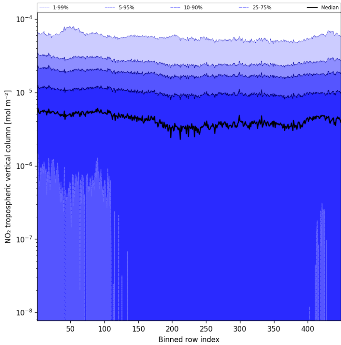
Figure 44: Along track statistics of “NO 2 tropospheric vertical column” for 2025-04-14 to 2025-04-15
