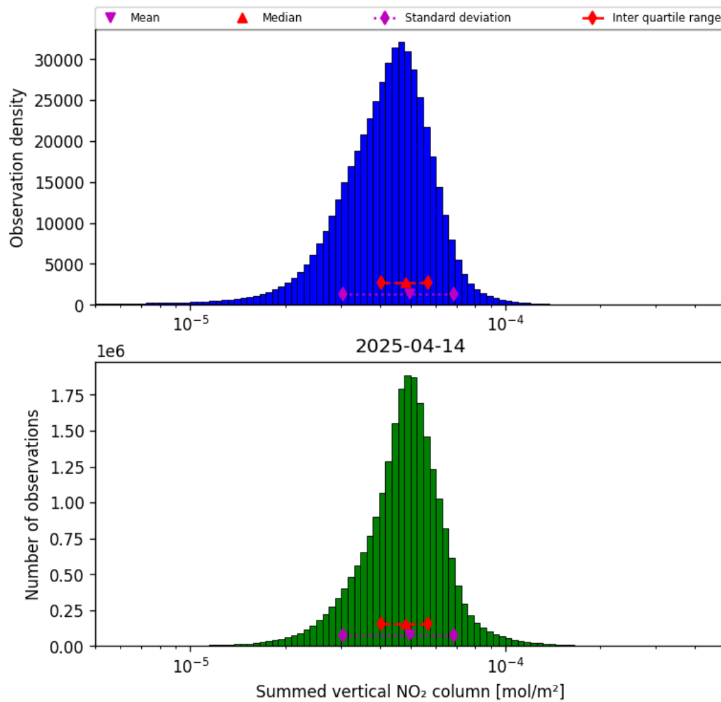
Figure 38: Histogram of “Summed vertical NO 2 column” for 2025-04-14 to 2025-04-15
