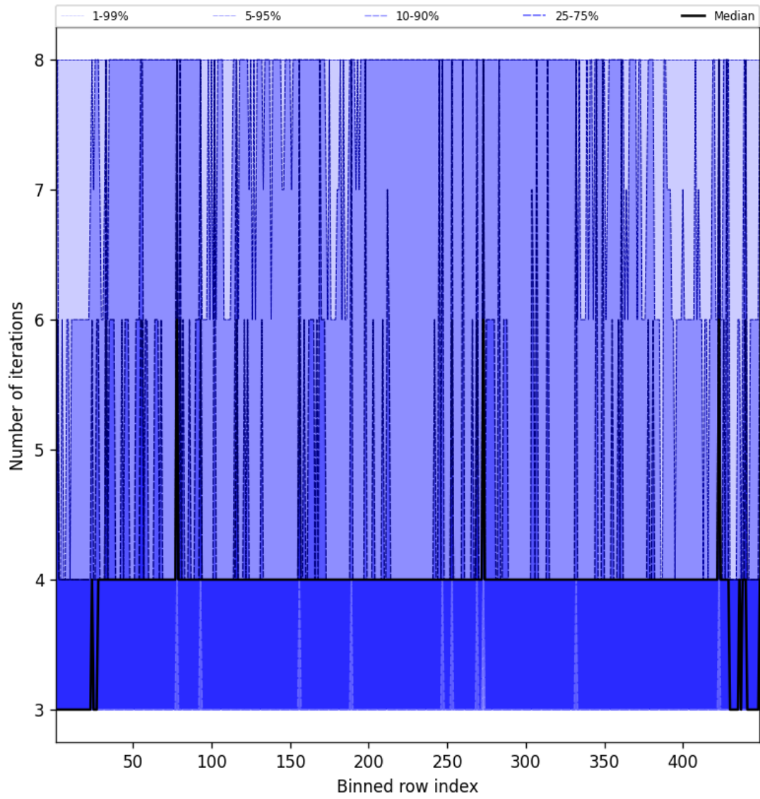
Figure 49: Along track statistics of “Number of iterations” for 2025-04-14 to 2025-04-15
