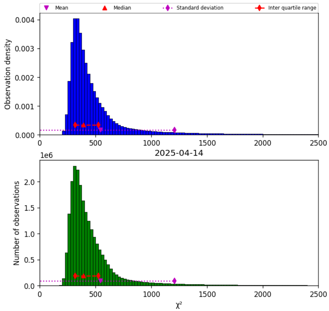
Figure 40: Histogram of “ \chi^2 ” for 2025-04-14 to 2025-04-15
