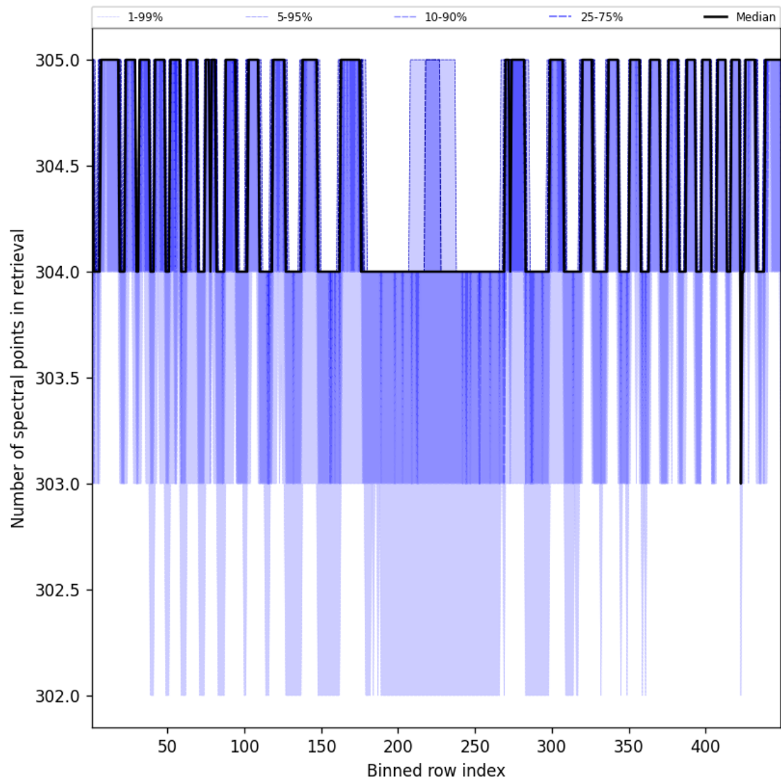
Figure 48: Along track statistics of “Number of spectral points in retrieval” for 2025-04-14 to 2025-04-15
