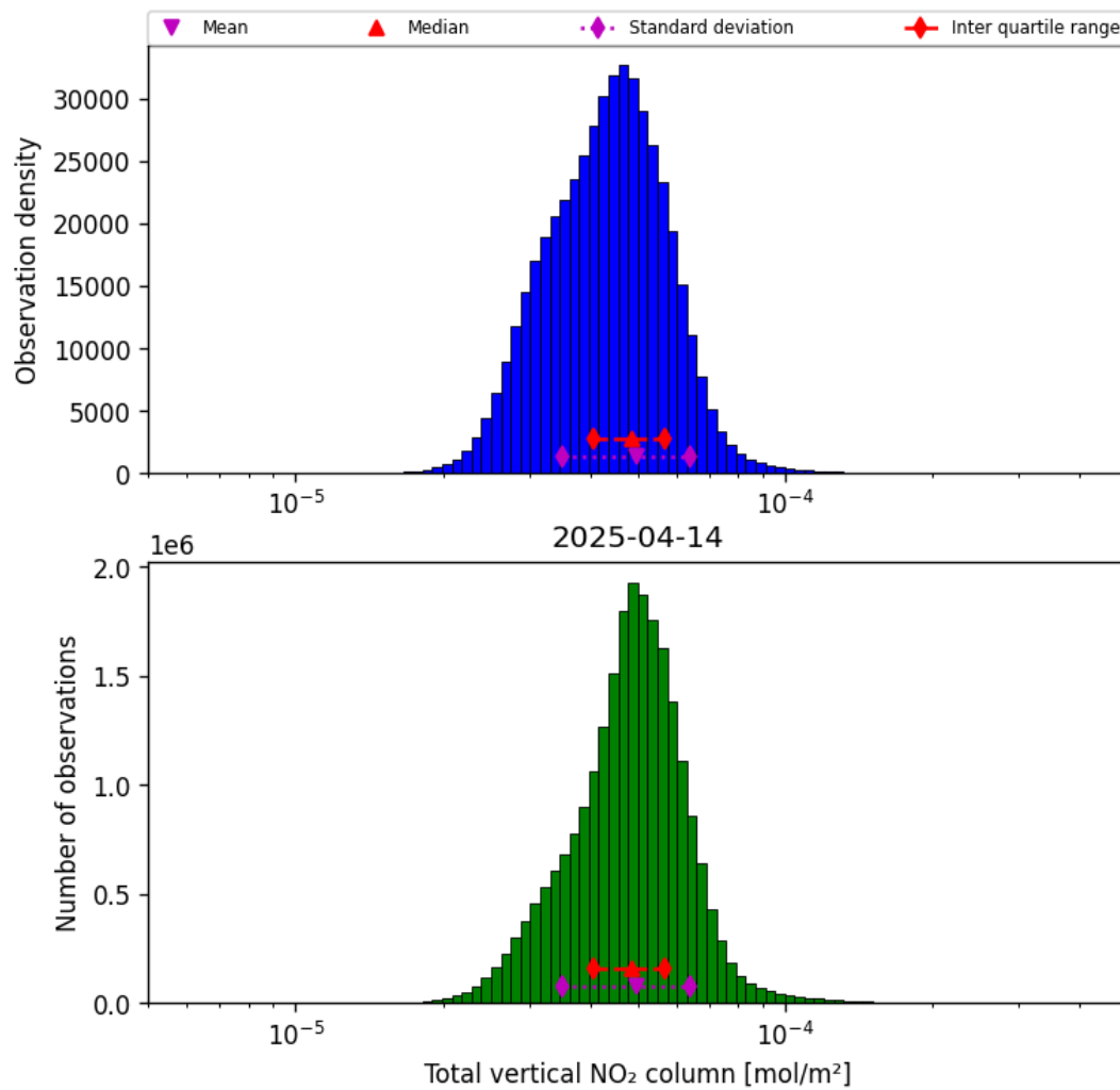
Figure 36: Histogram of “Total vertical NO 2 column” for 2025-04-14 to 2025-04-15
