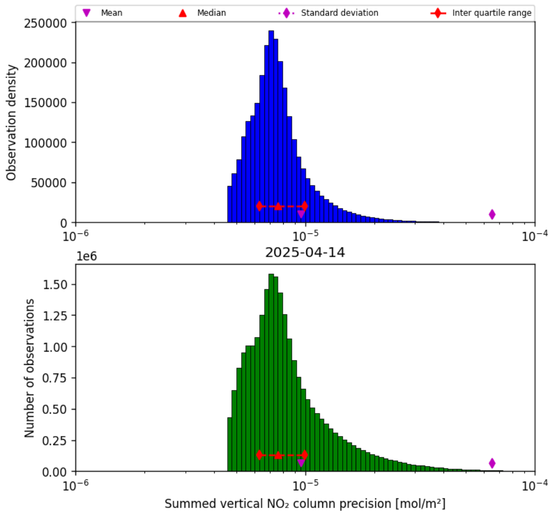
Figure 39: Histogram of "Summed vertical NO 2 column precision" for 2025-04-14 to 2025-04-15
