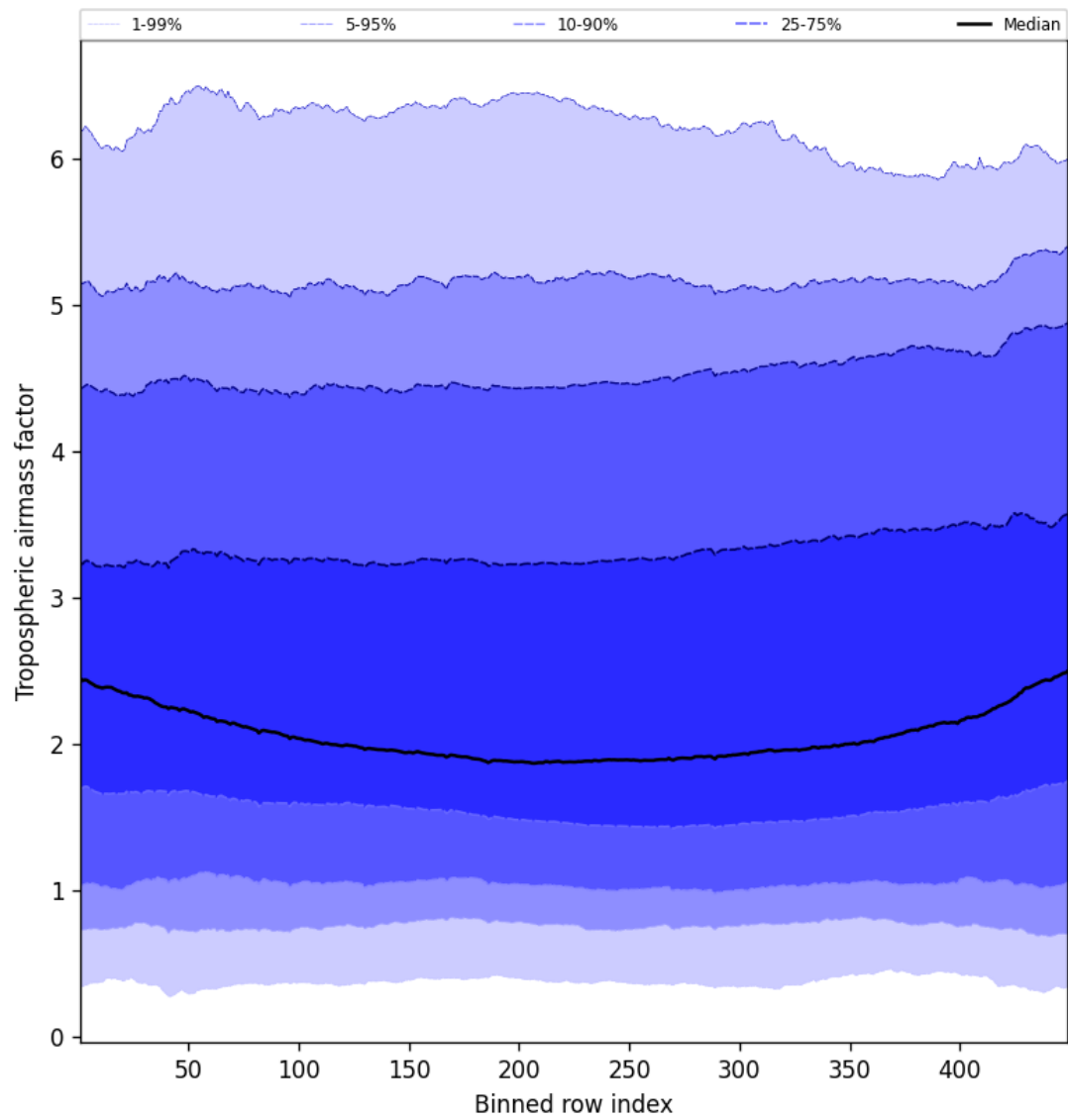
Figure 46: Along track statistics of “Tropospheric air mass factor” for 2025-04-14 to 2025-04-15
