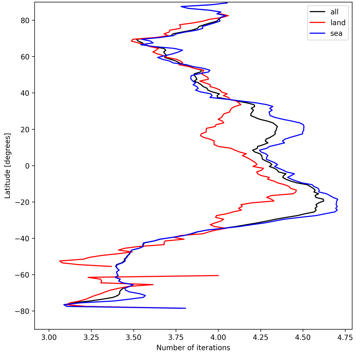
Figure 15: Zonal average of “Number of iterations” for 2025-04-14 to 2025-04-15.
