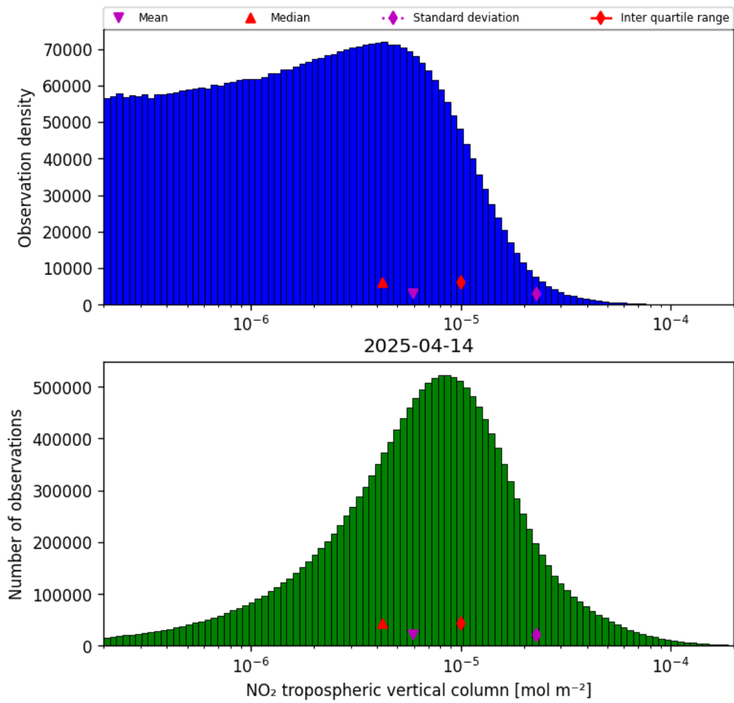
Figure 27: Histogram of “NO 2 tropospheric vertical column” for 2025-04-14 to 2025-04-15
