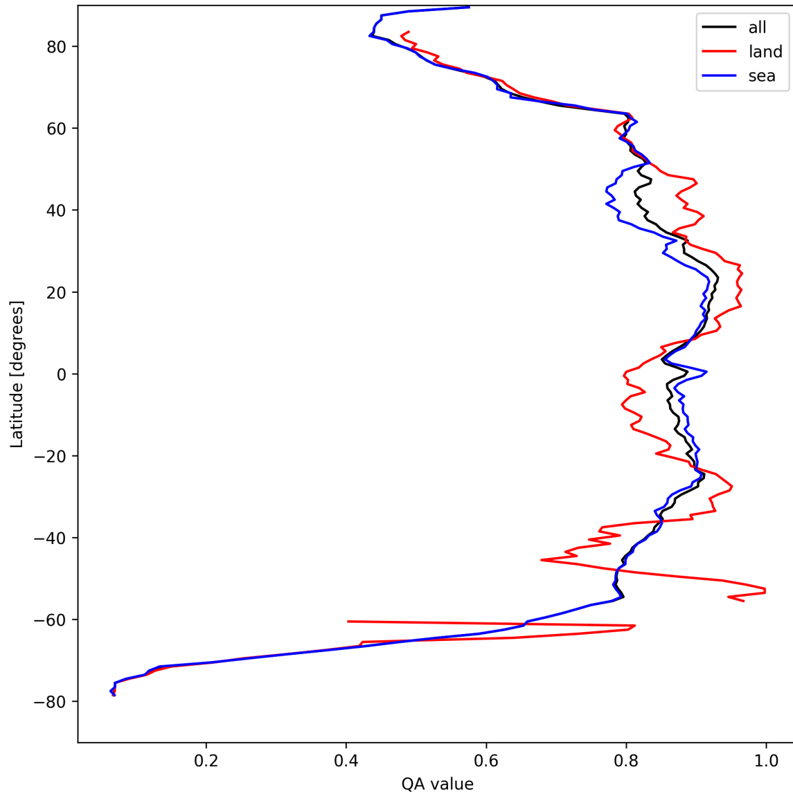
Figure 9: Zonal average of “QA value” for 2025-04-14 to 2025-04-15.
