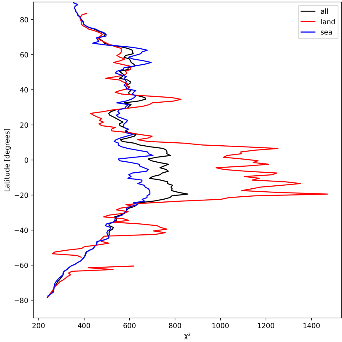
Figure 23: Zonal average of “ \chi^2 ” for 2025-04-14 to 2025-04-15.
