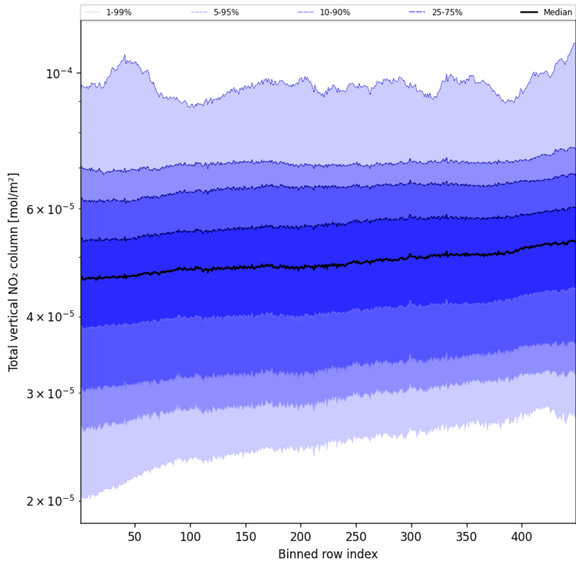
Figure 53: Along track statistics of “Total vertical NO 2 column” for 2025-04-14 to 2025-04-15
