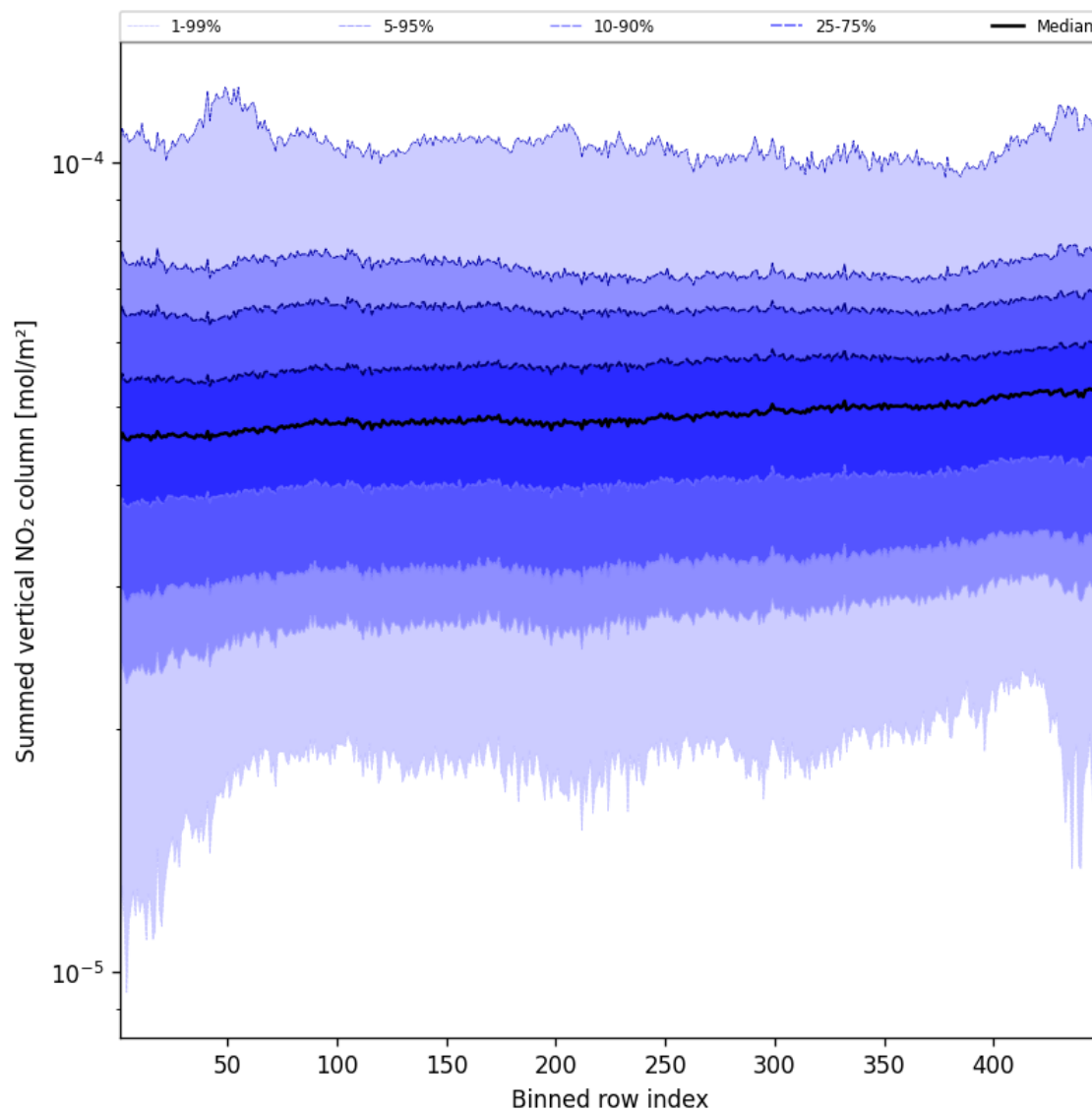
Figure 55: Along track statistics of “Summed vertical NO 2 column” for 2025-04-14 to 2025-04-15
