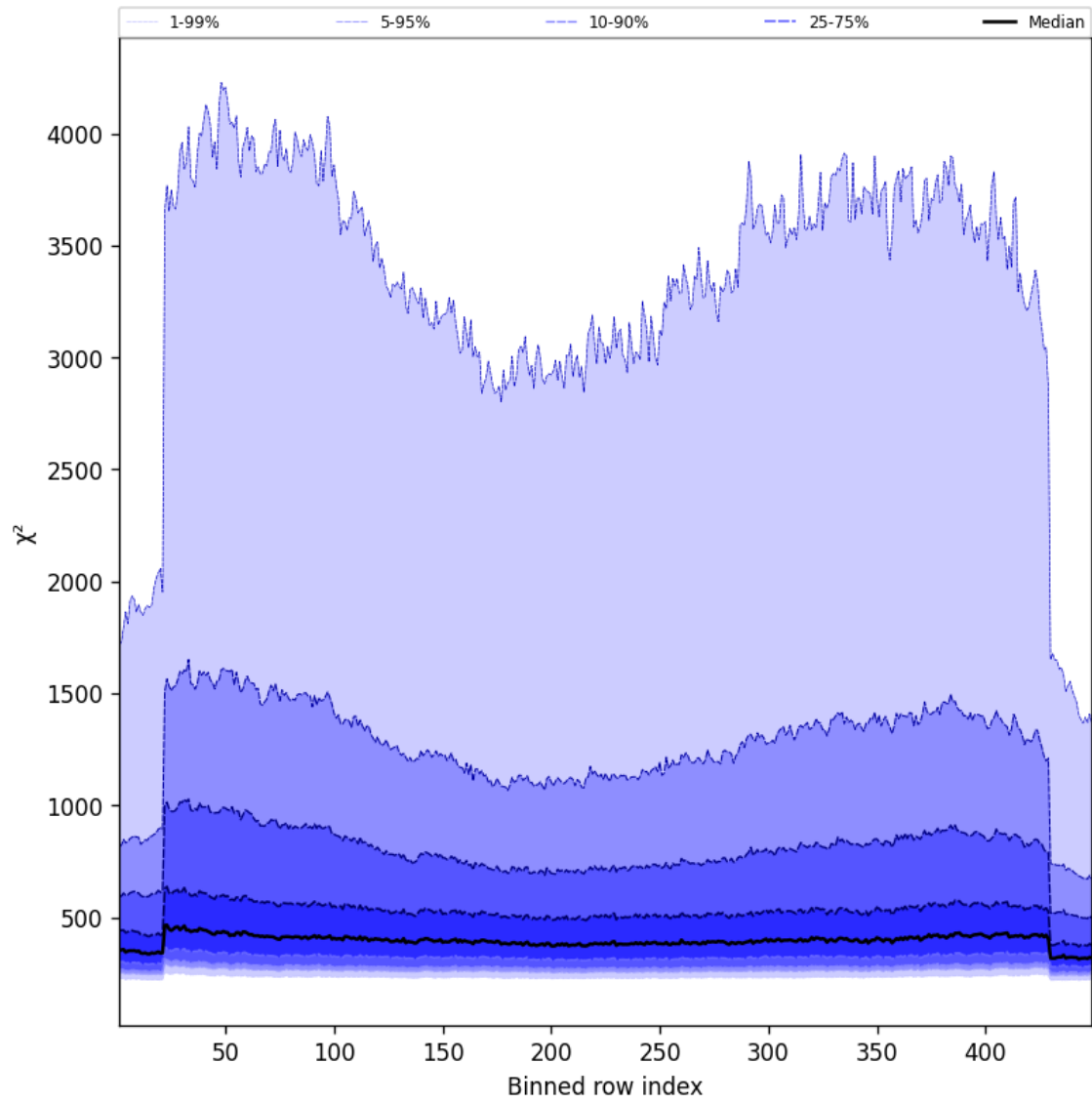
Figure 57: Along track statistics of “ \chi^2 ” for 2025-04-14 to 2025-04-15
