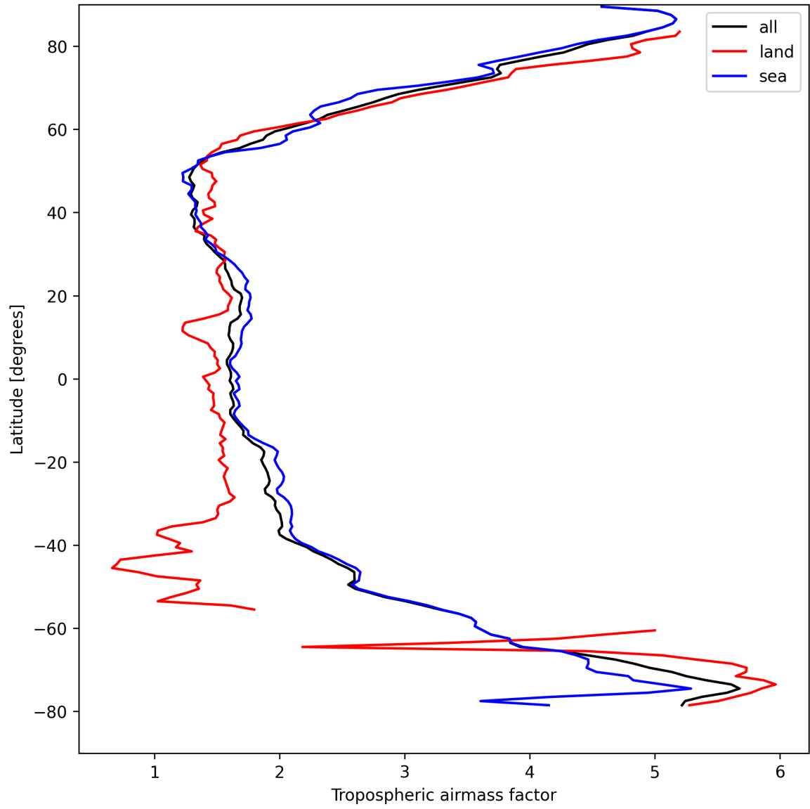
Figure 12: Zonal average of “Tropospheric air mass factor” for 2025-04-14 to 2025-04-15.
