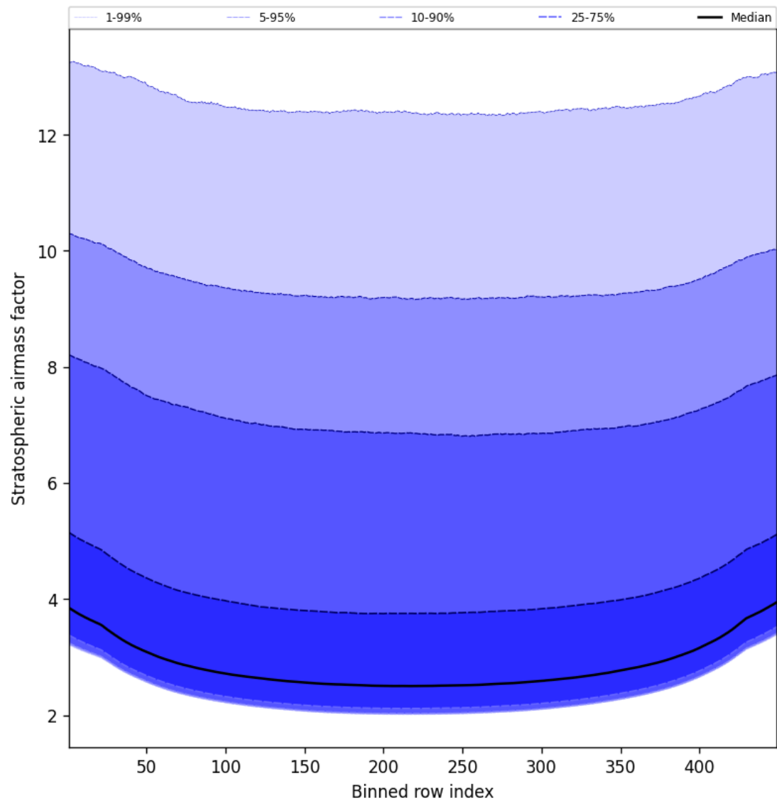
Figure 59: Along track statistics of “Stratospheric airmass factor” for 2025-04-14 to 2025-04-15
