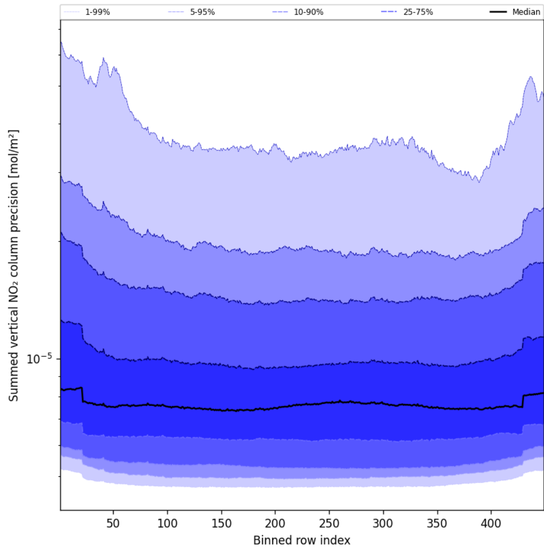
Figure 56: Along track statistics of “Summed vertical NO 2 column precision” for 2025-04-14 to 2025-04-15
