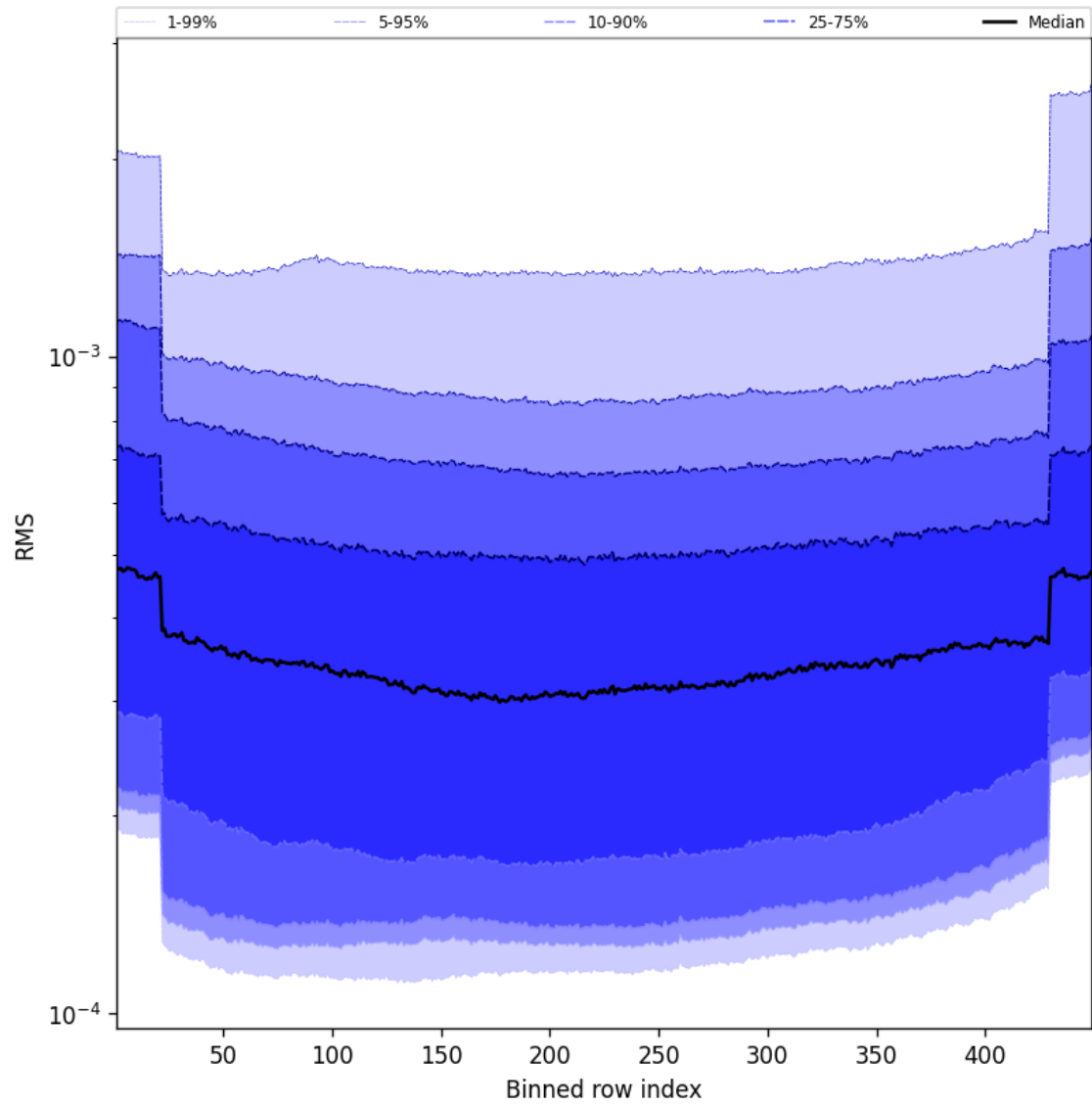
Figure 58: Along track statistics of “RMS” for 2025-04-14 to 2025-04-15
