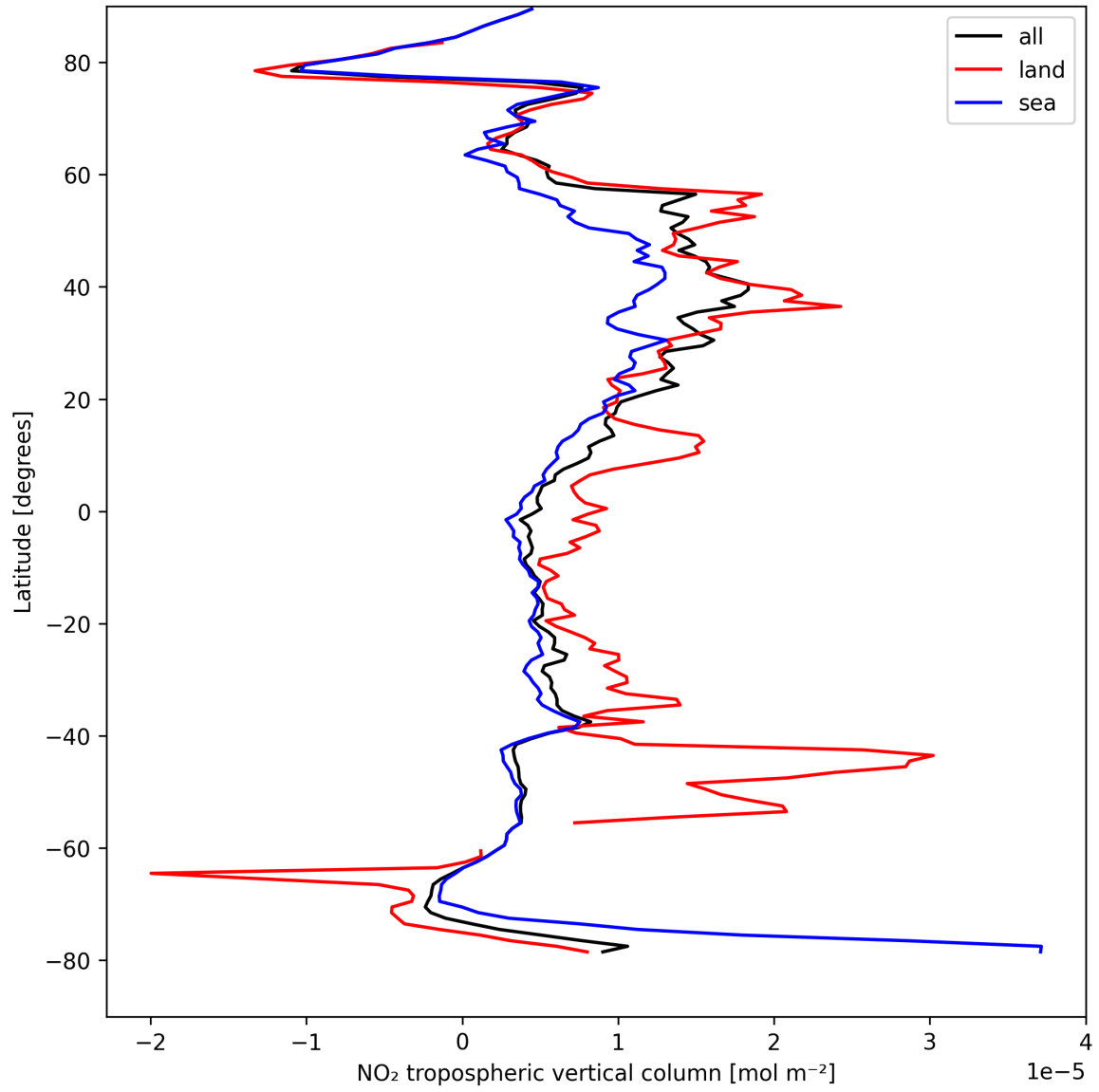
Figure 10: Zonal average of “NO 2 tropospheric vertical column” for 2025-04-14 to 2025-04-15.
