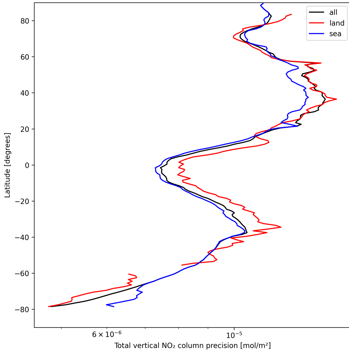
Figure 20: Zonal average of “Total vertical NO 2 column precision” for 2025-04-14 to 2025-04-15.
