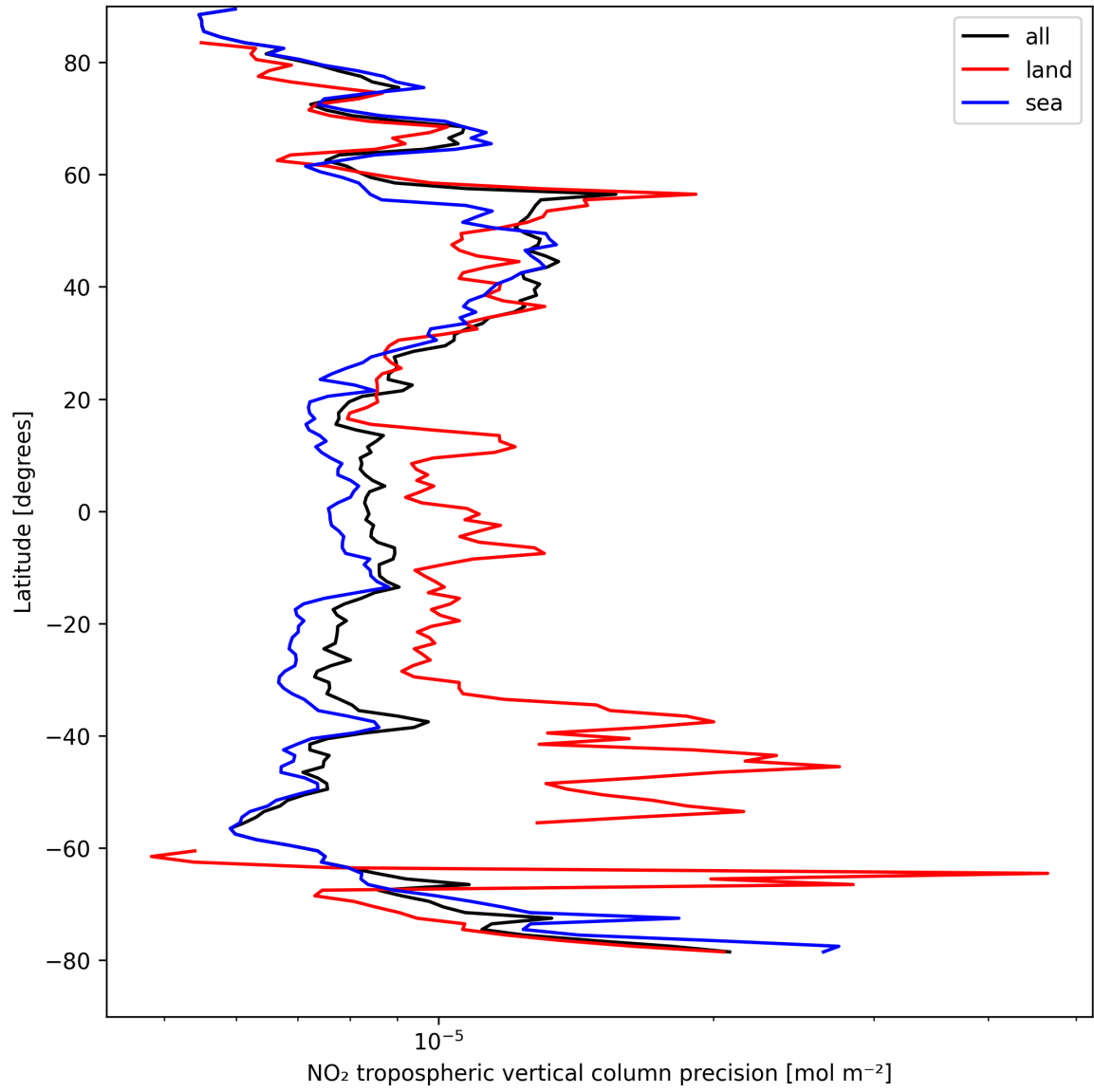
Figure 11: Zonal average of “NO 2 tropospheric vertical column precision” for 2025-04-14 to 2025-04-15.
