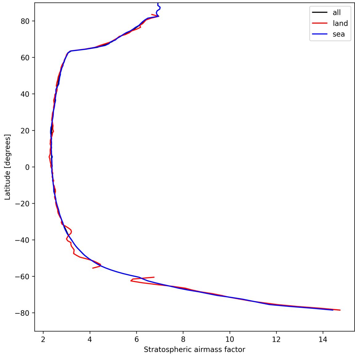
Figure 25: Zonal average of “Stratospheric airmass factor” for 2025-04-14 to 2025-04-15.
