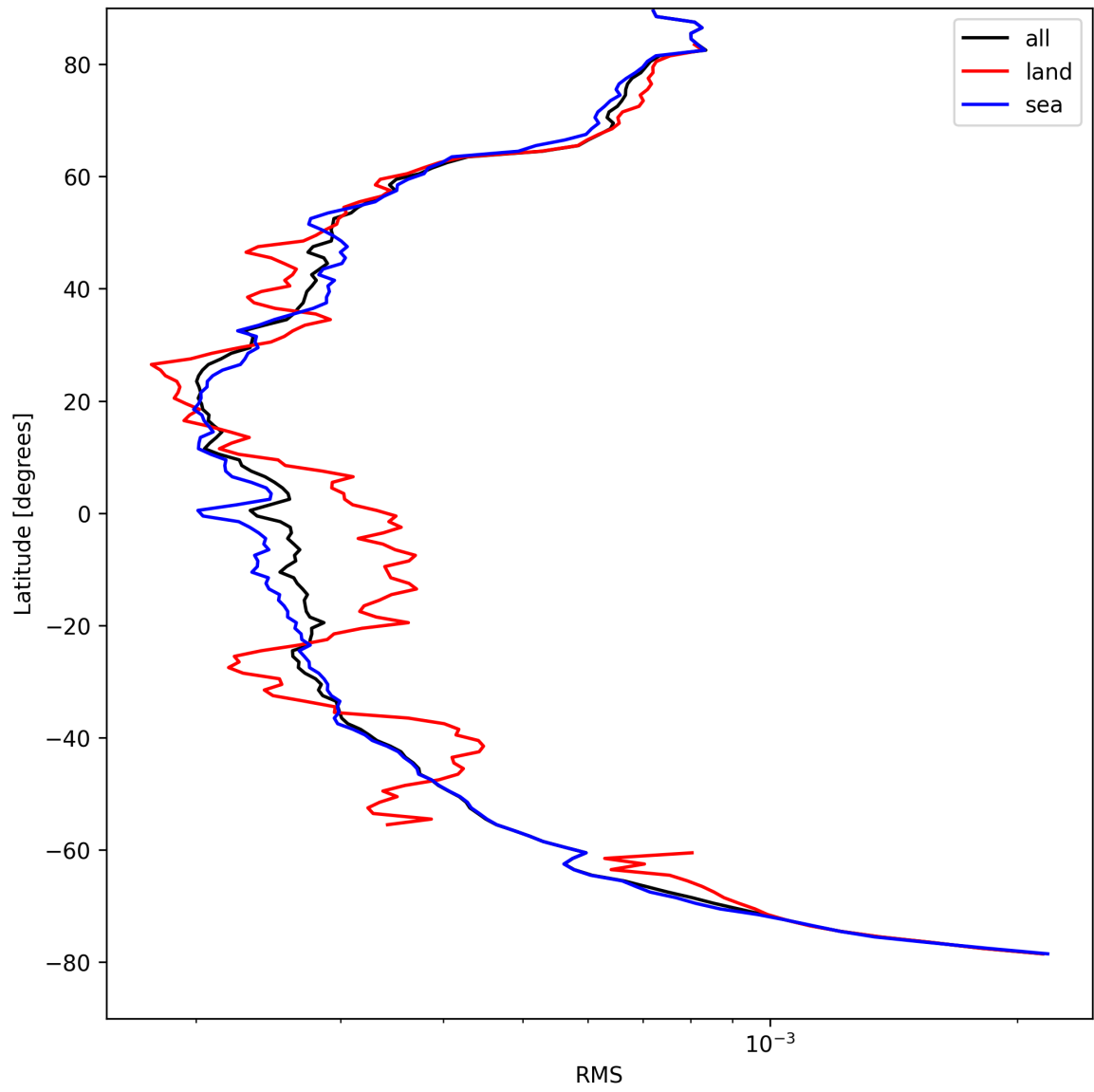
Figure 24: Zonal average of “RMS” for 2025-04-14 to 2025-04-15.
