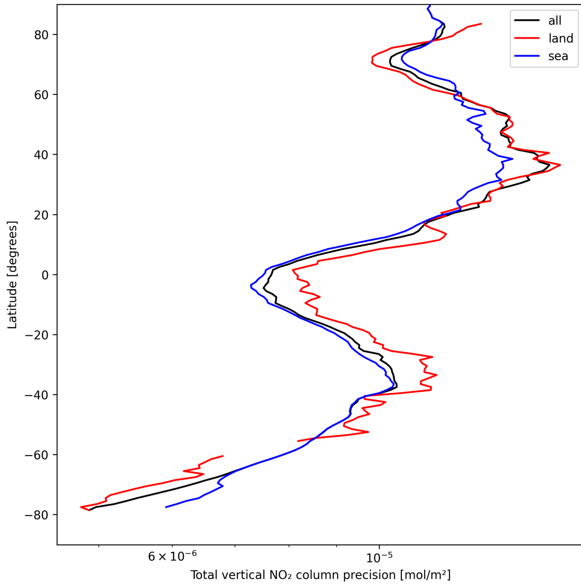
Figure 20: Zonal average of “Total vertical NO 2 column precision” for 2025-04-15 to 2025-04-16.
