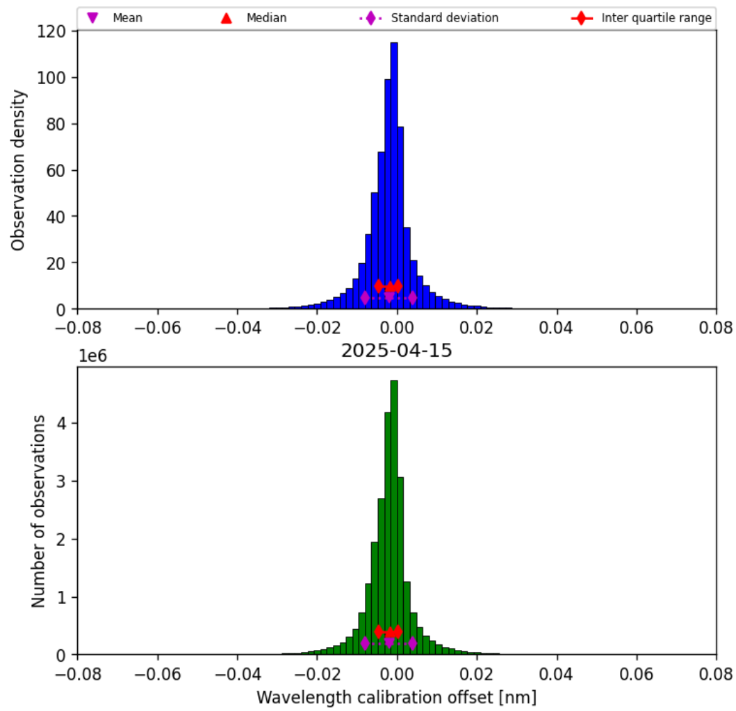
Figure 33: Histogram of “Wavelength calibration offset” for 2025-04-15 to 2025-04-16
