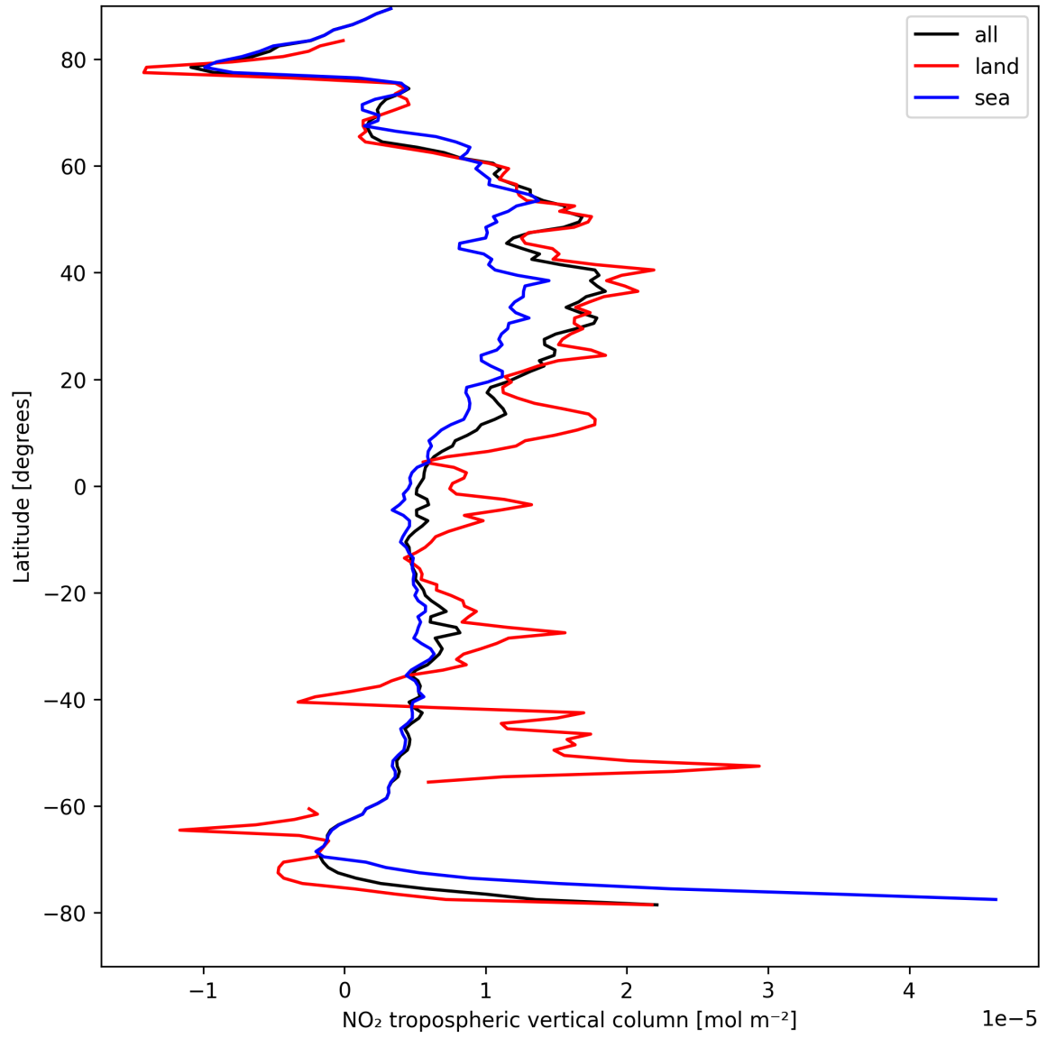
Figure 10: Zonal average of “NO 2 tropospheric vertical column” for 2025-04-15 to 2025-04-16.
