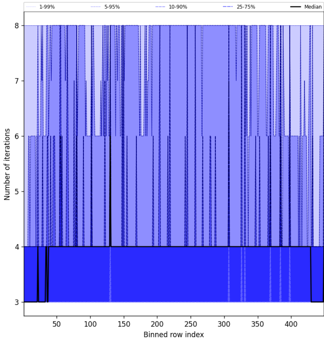
Figure 49: Along track statistics of “Number of iterations” for 2025-04-15 to 2025-04-16
