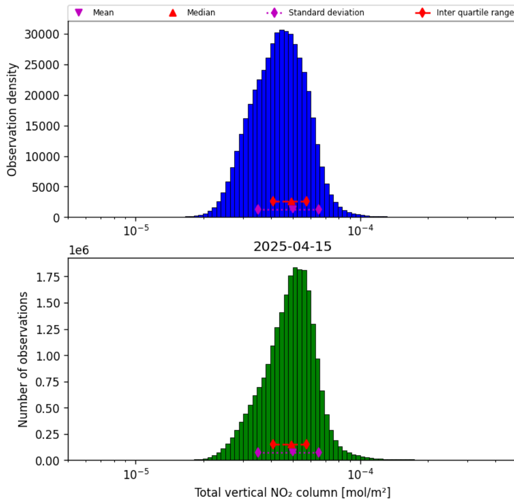
Figure 36: Histogram of "Total vertical NO 2 column" for 2025-04-15 to 2025-04-16
