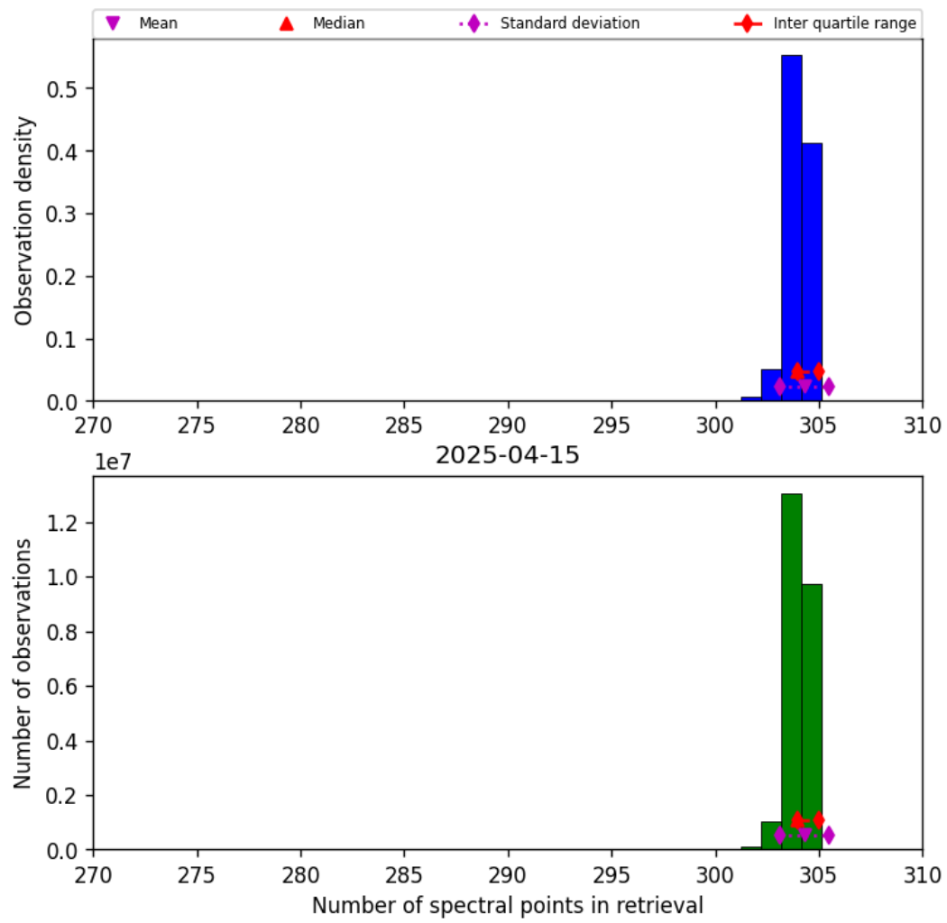
Figure 31: Histogram of “Number of spectral points in retrieval” for 2025-04-15 to 2025-04-16
