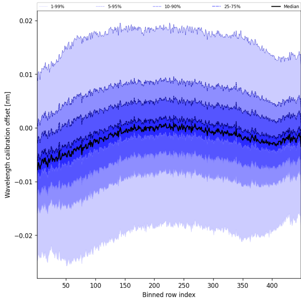
Figure 50: Along track statistics of “Wavelength calibration offset” for 2025-04-15 to 2025-04-16
