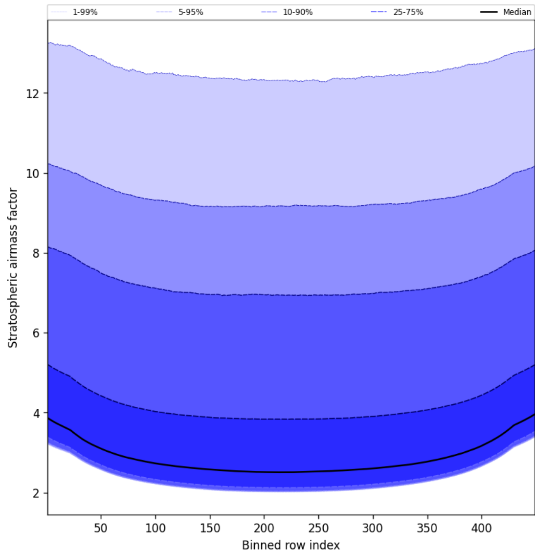
Figure 59: Along track statistics of “Stratospheric airmass factor” for 2025-04-15 to 2025-04-16
