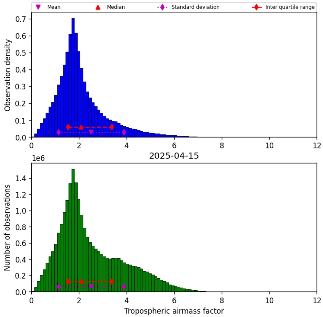
Figure 29: Histogram of “Tropospheric airmass factor” for 2025-04-15 to 2025-04-16
