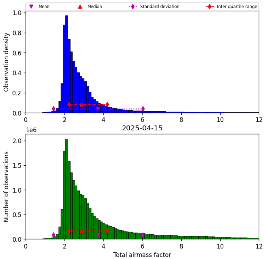
Figure 30: Histogram of “Total airmass factor” for 2025-04-15 to 2025-04-16
