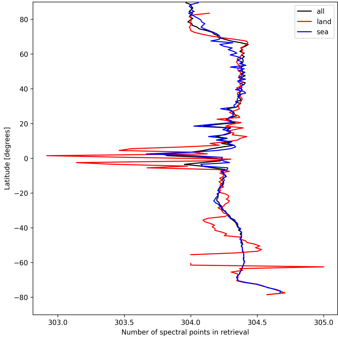
Figure 14: Zonal average of “Number of spectral points in retrieval” for 2025-04-15 to 2025-04-16.
