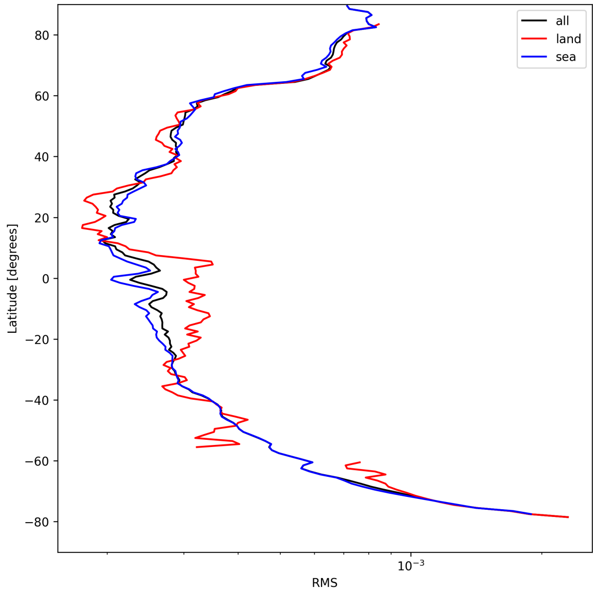
Figure 24: Zonal average of “RMS” for 2025-04-15 to 2025-04-16.
