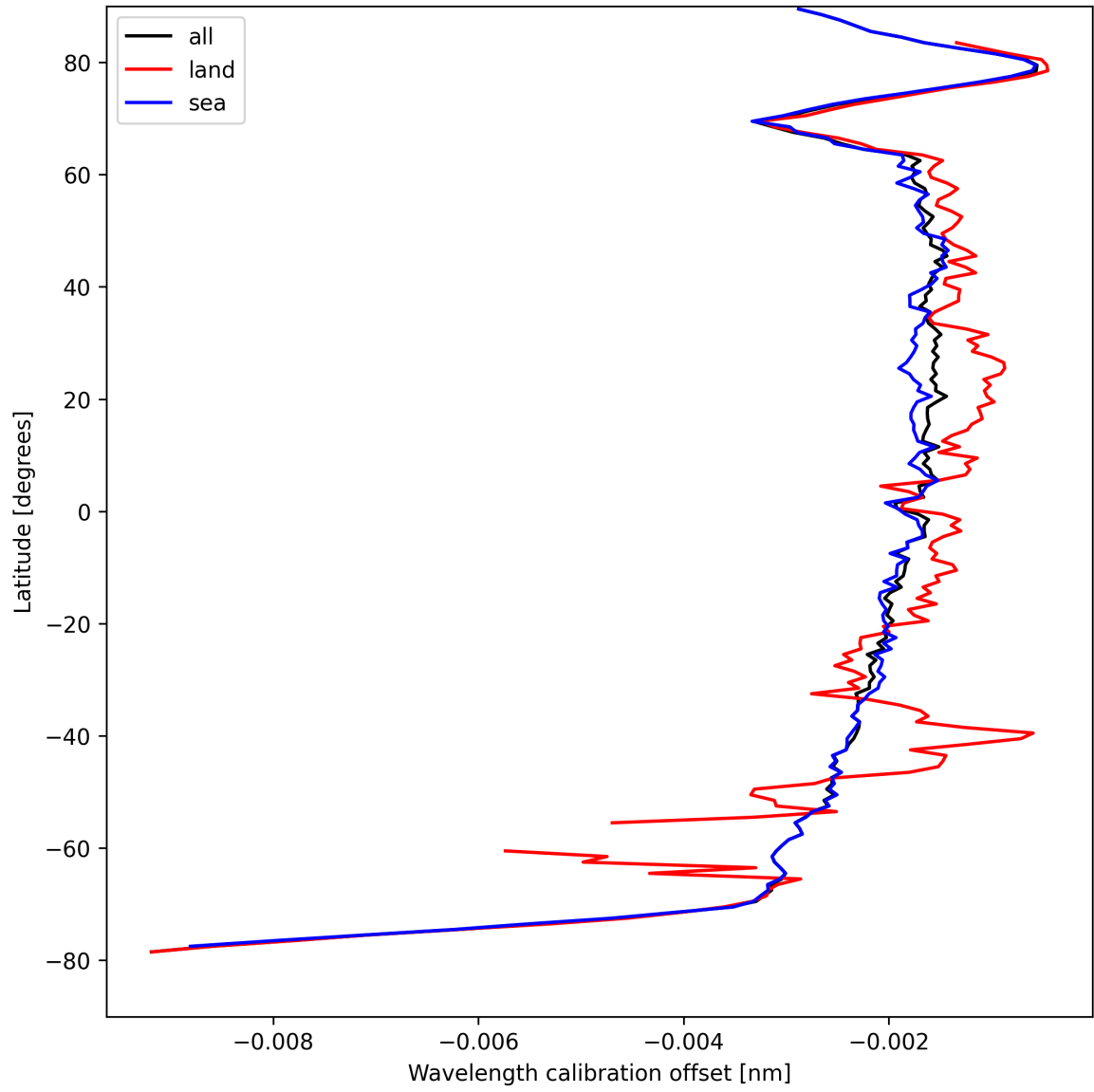
Figure 16: Zonal average of “Wavelength calibration offset” for 2025-04-15 to 2025-04-16.
