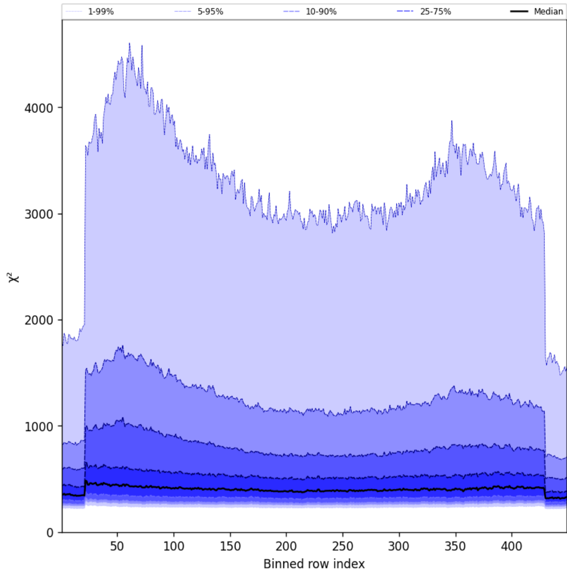
Figure 57: Along track statistics of “ \chi^2 ” for 2025-04-15 to 2025-04-16
