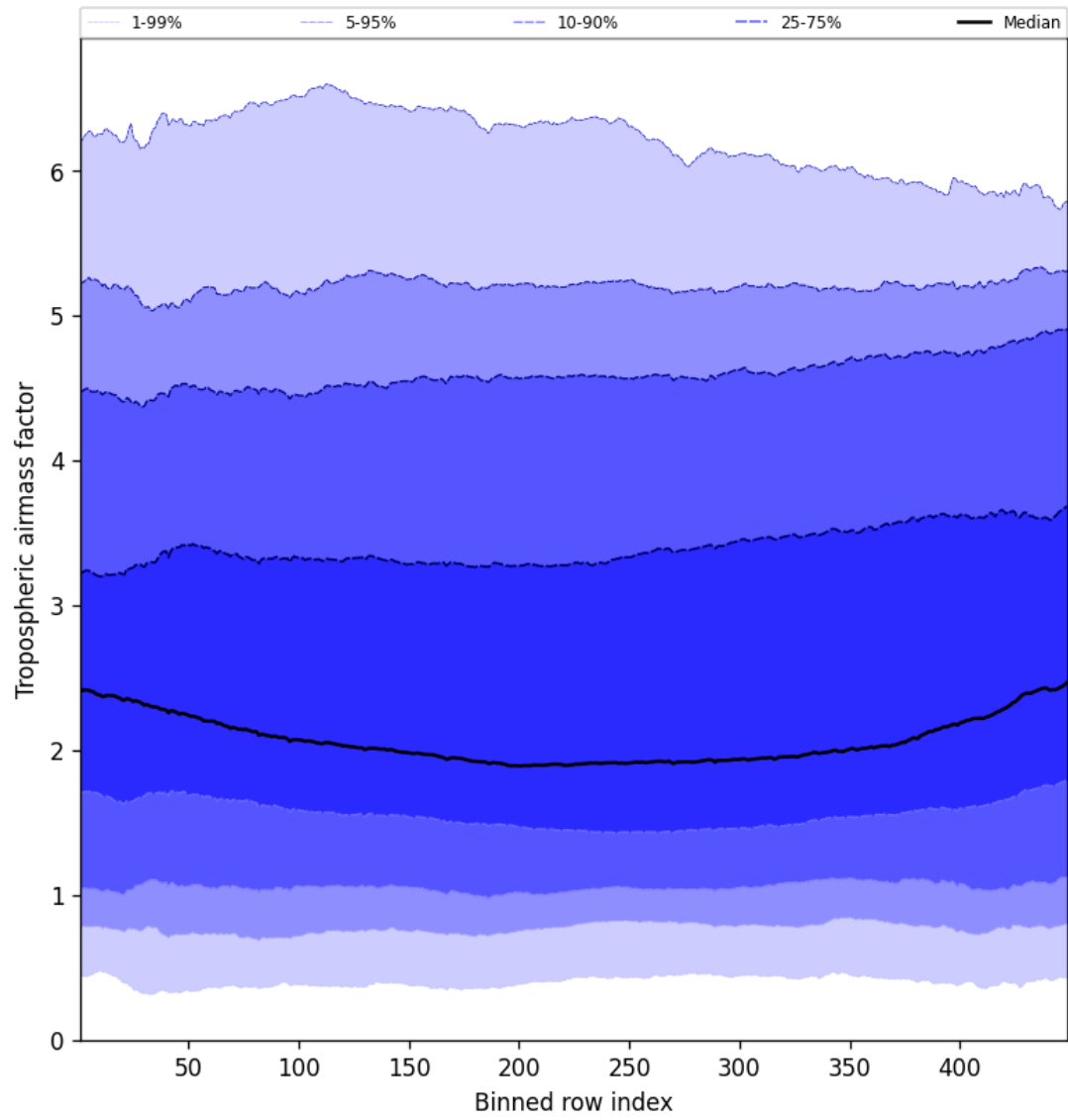
Figure 46: Along track statistics of “Tropospheric airmass factor” for 2025-04-15 to 2025-04-16
