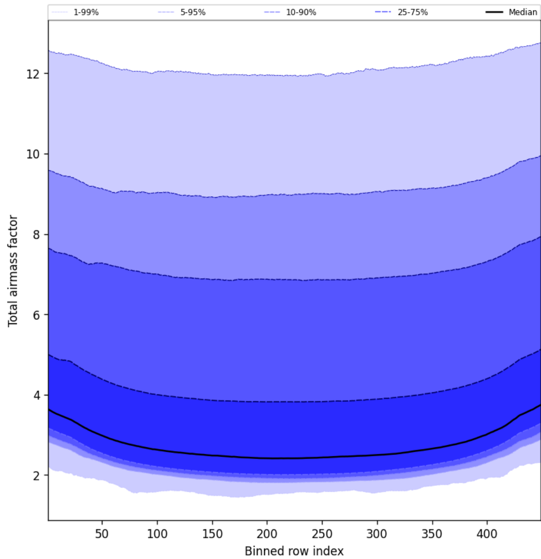
Figure 47: Along track statistics of “Total airmass factor” for 2025-04-15 to 2025-04-16
