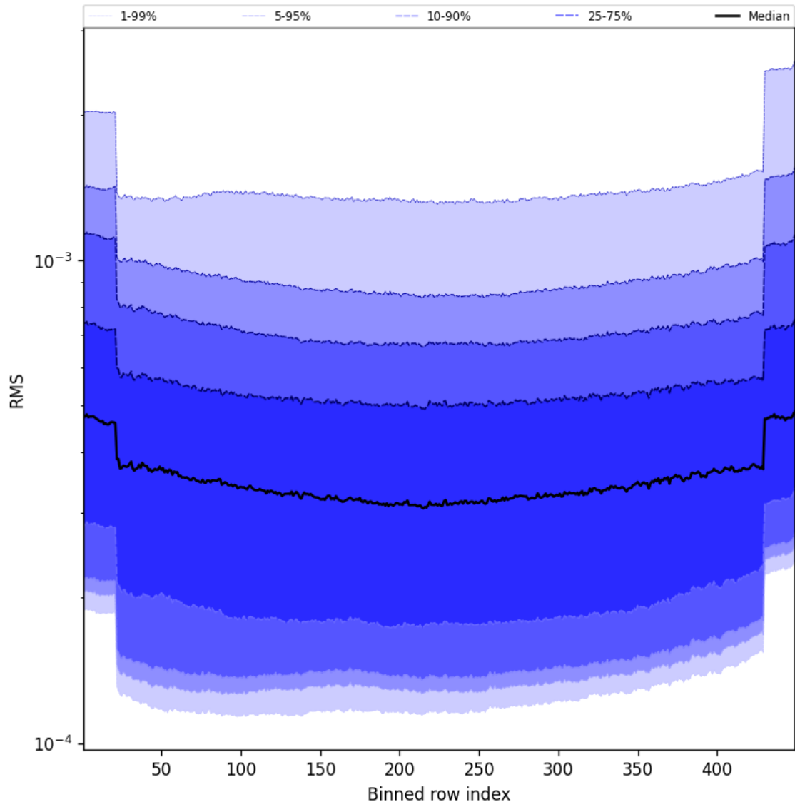
Figure 58: Along track statistics of “RMS” for 2025-04-15 to 2025-04-16
