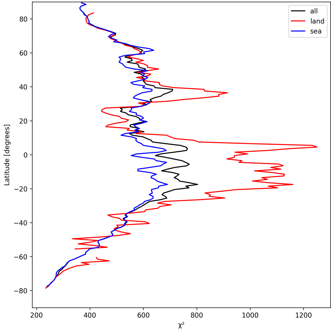
Figure 23: Zonal average of “ \chi^2 ” for 2025-04-15 to 2025-04-16.
