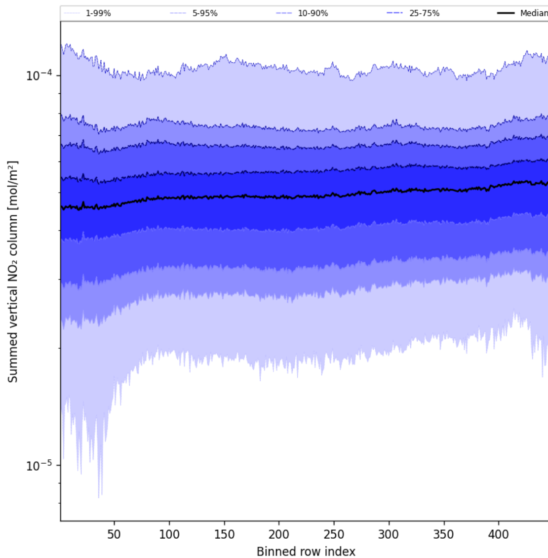
Figure 55: Along track statistics of “Summed vertical NO 2 column” for 2025-04-15 to 2025-04-16
