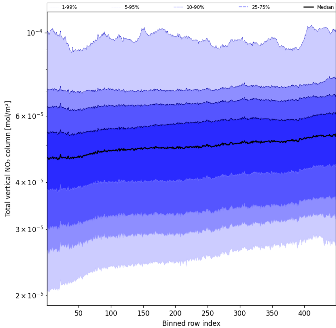
Figure 53: Along track statistics of “Total vertical NO 2 column” for 2025-04-15 to 2025-04-16
