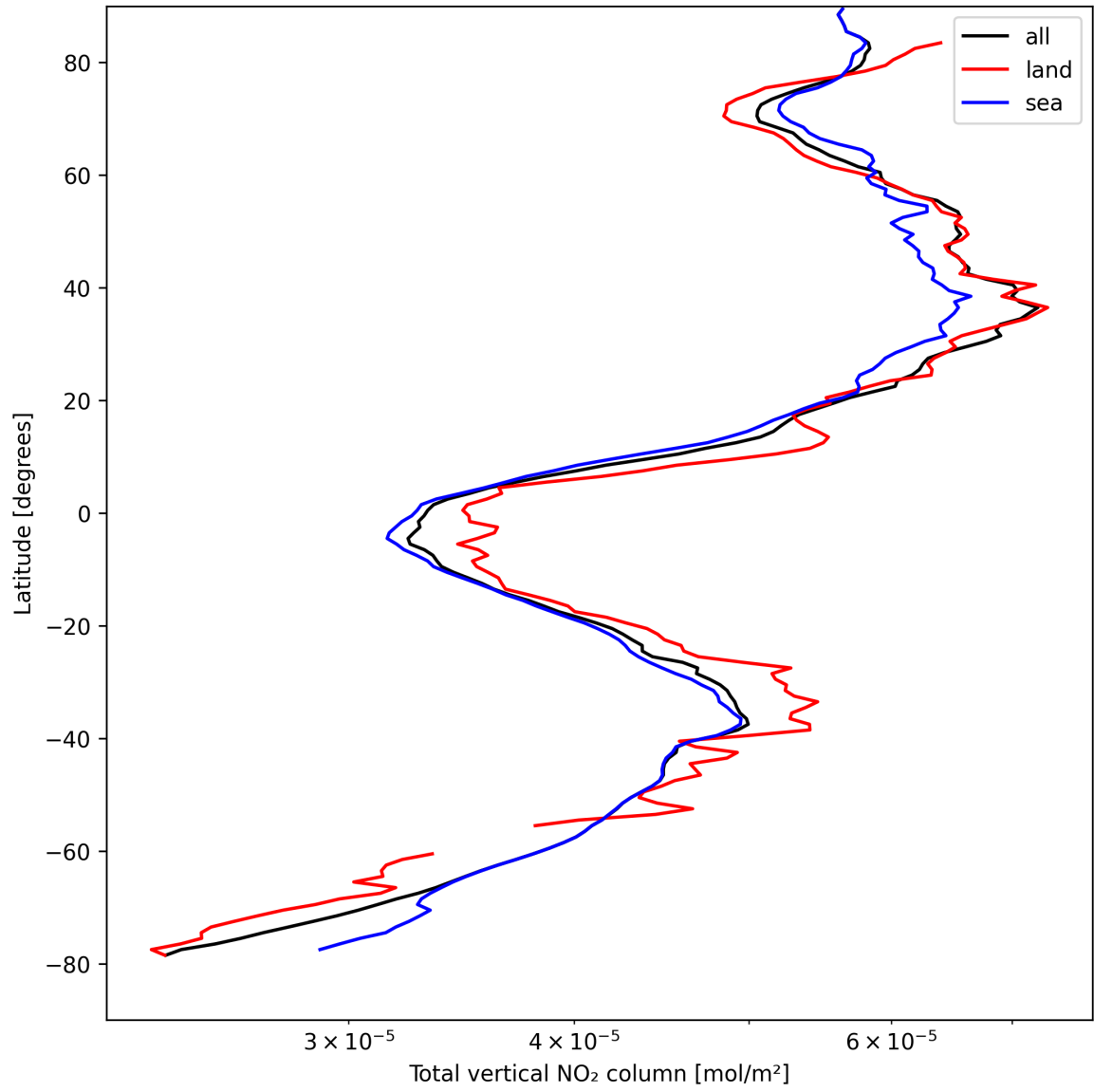
Figure 19: Zonal average of “Total vertical NO 2 column” for 2025-04-15 to 2025-04-16.
