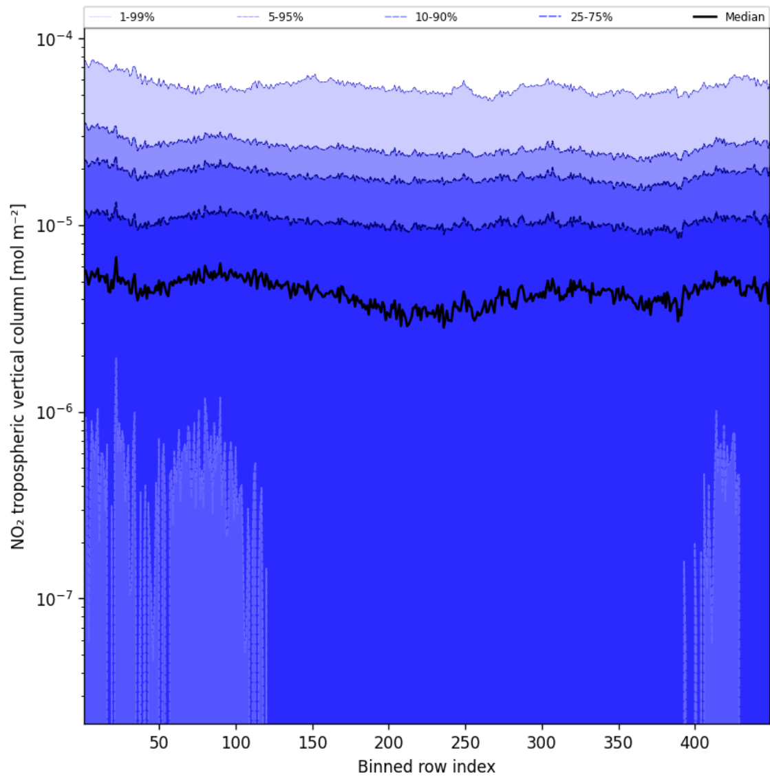
Figure 44: Along track statistics of “NO 2 tropospheric vertical column” for 2025-04-15 to 2025-04-16
