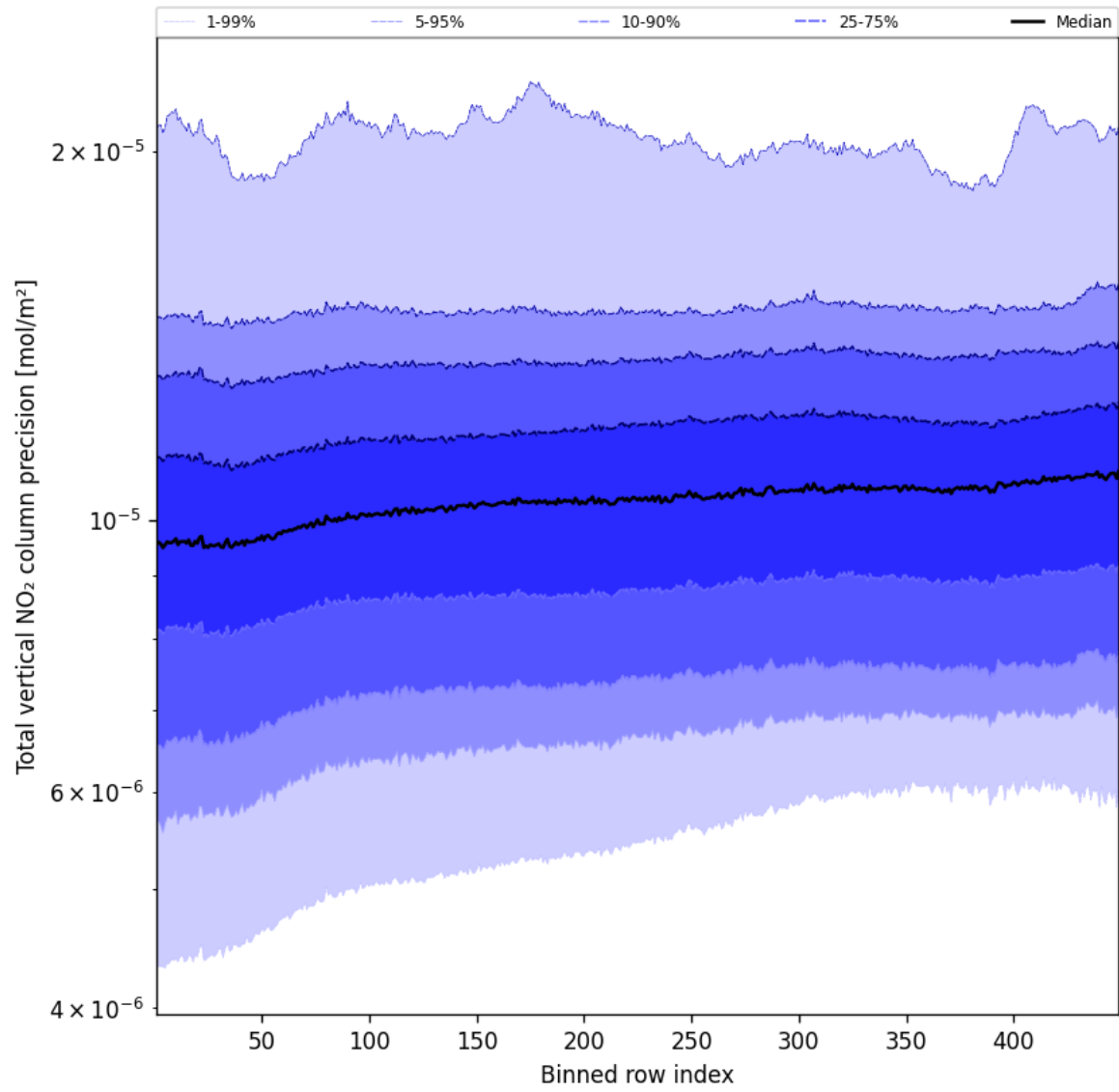
Figure 54: Along track statistics of “Total vertical NO 2 column precision” for 2025-04-15 to 2025-04-16
