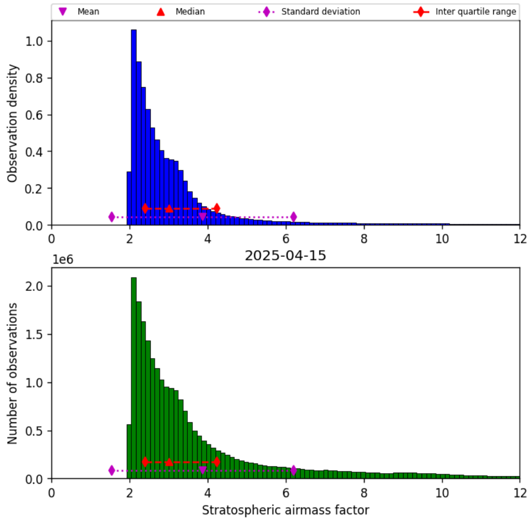
Figure 42: Histogram of “Stratospheric airmass factor” for 2025-04-15 to 2025-04-16
