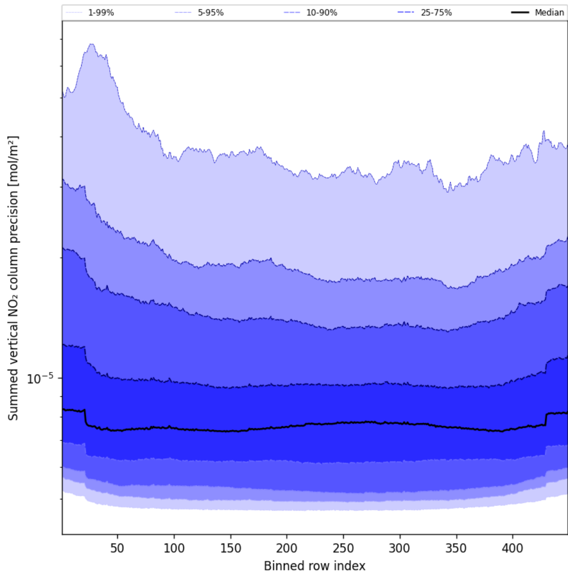
Figure 56: Along track statistics of “Summed vertical NO 2 column precision” for 2025-04-15 to 2025-04-16
