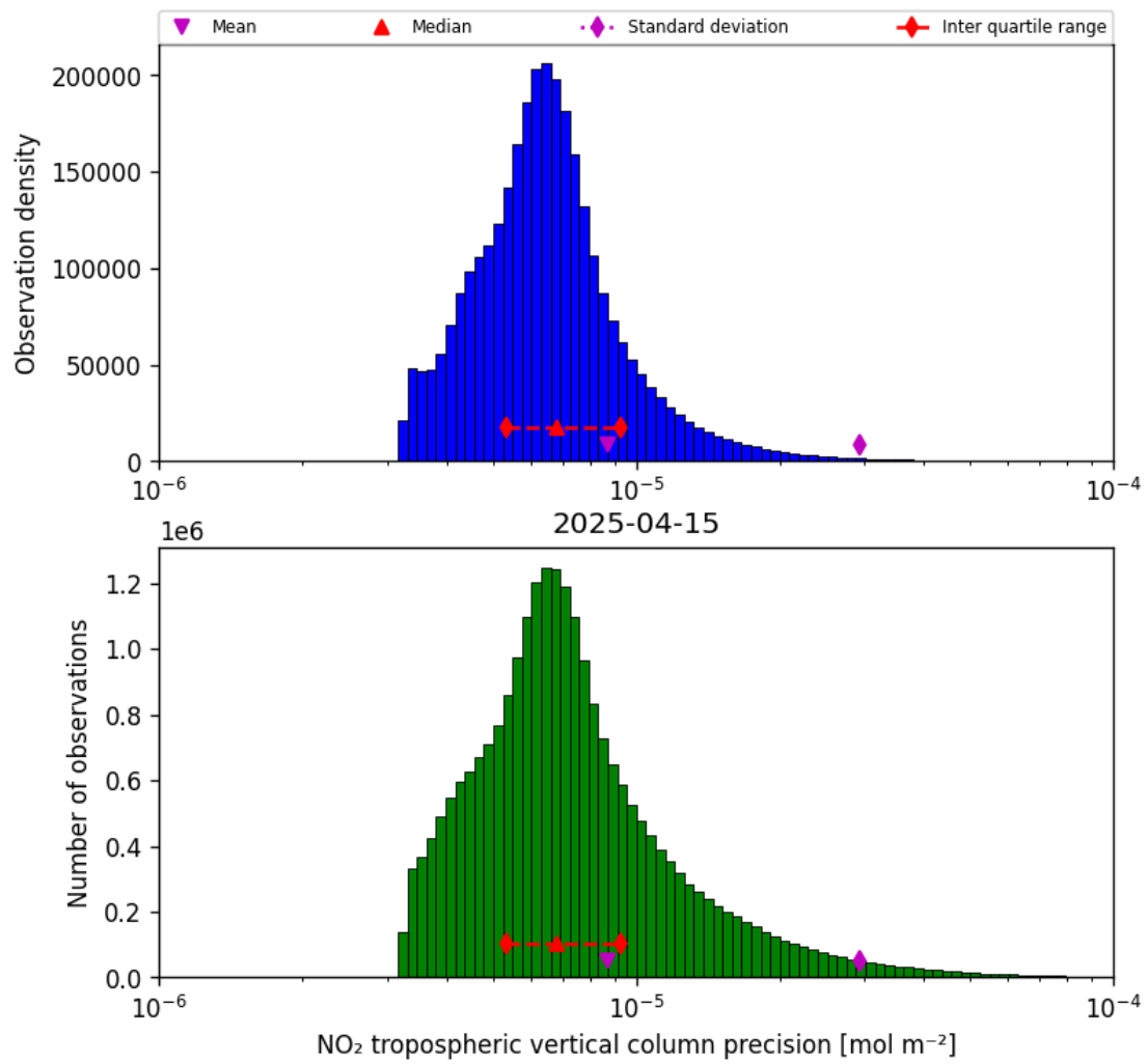
Figure 28: Histogram of “NO 2 tropospheric vertical column precision” for 2025-04-15 to 2025-04-16
