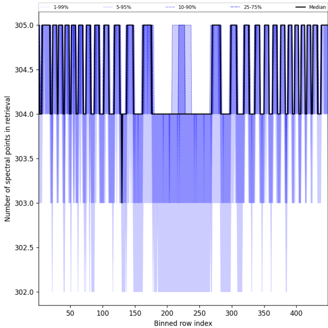
Figure 48: Along track statistics of “Number of spectral points in retrieval” for 2025-04-15 to 2025-04-16
