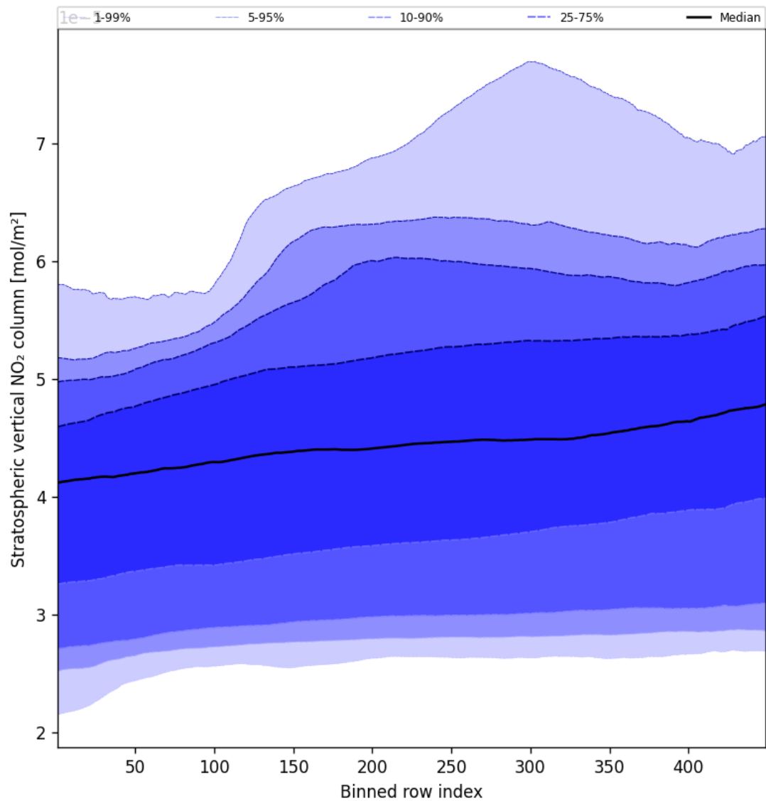
Figure 51: Along track statistics of “Stratospheric vertical NO 2 column” for 2025-04-15 to 2025-04-16
