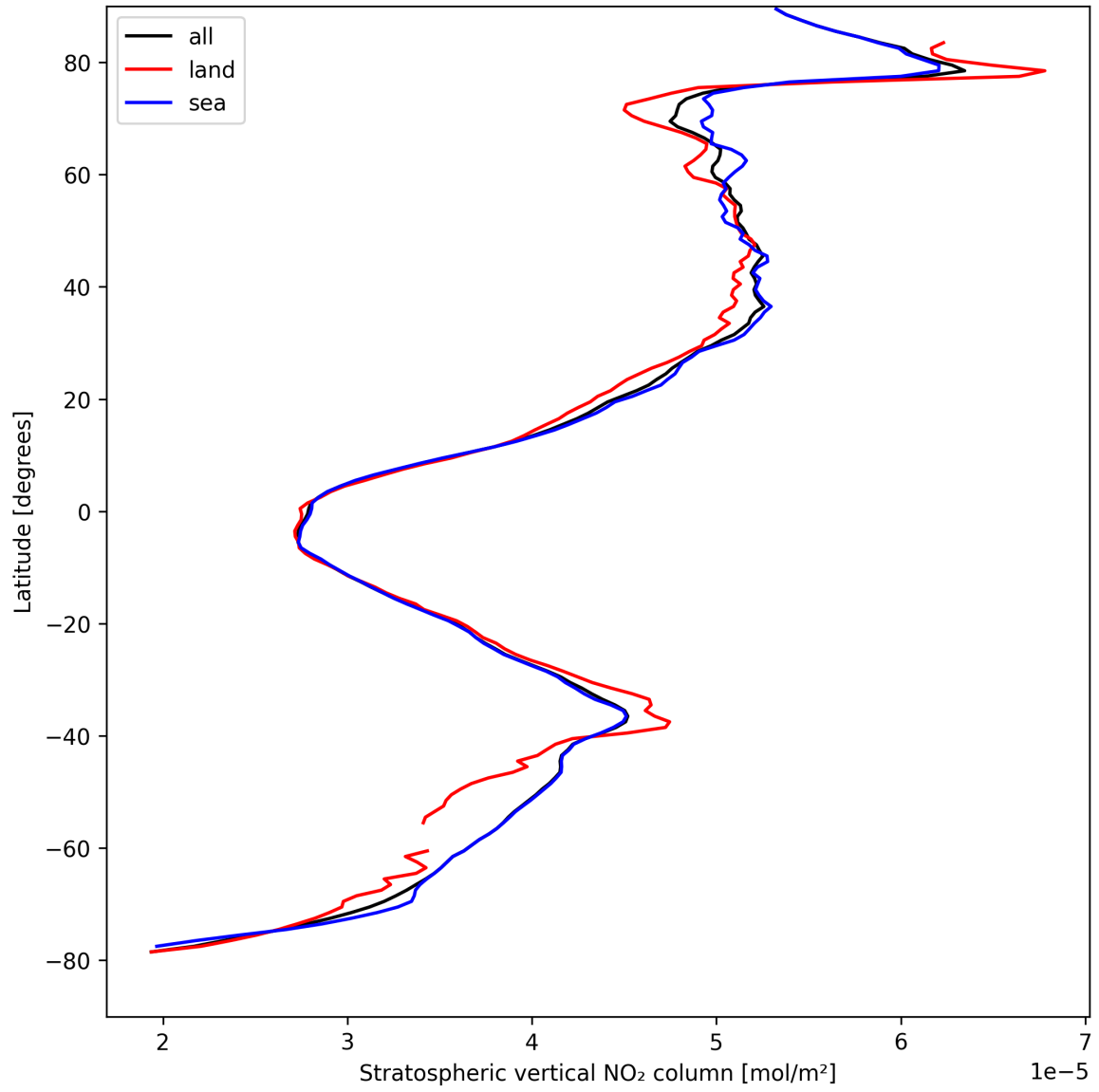
Figure 17: Zonal average of “Stratospheric vertical NO 2 column” for 2025-04-15 to 2025-04-16.
