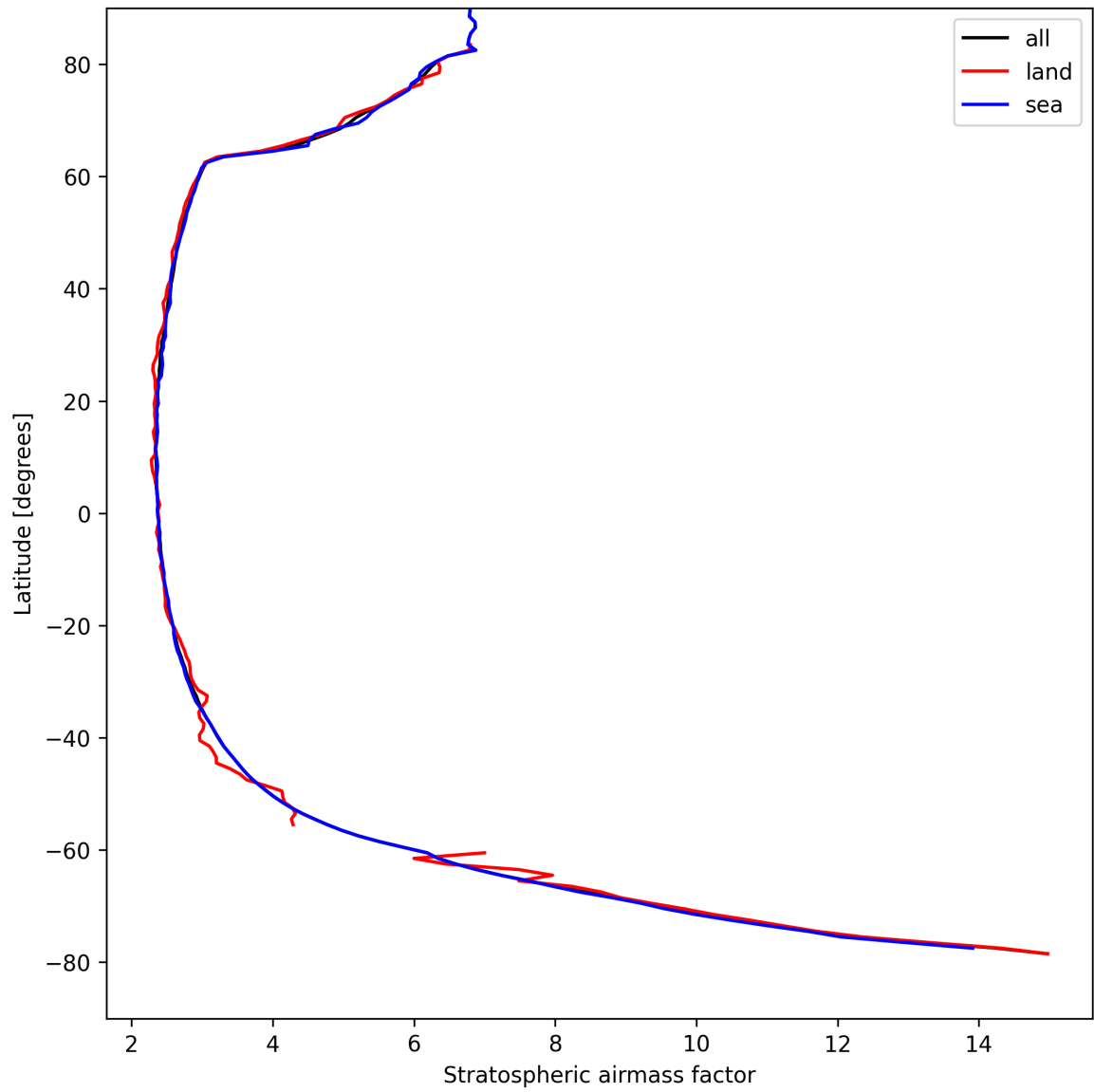
Figure 25: Zonal average of “Stratospheric airmass factor” for 2025-04-15 to 2025-04-16.
