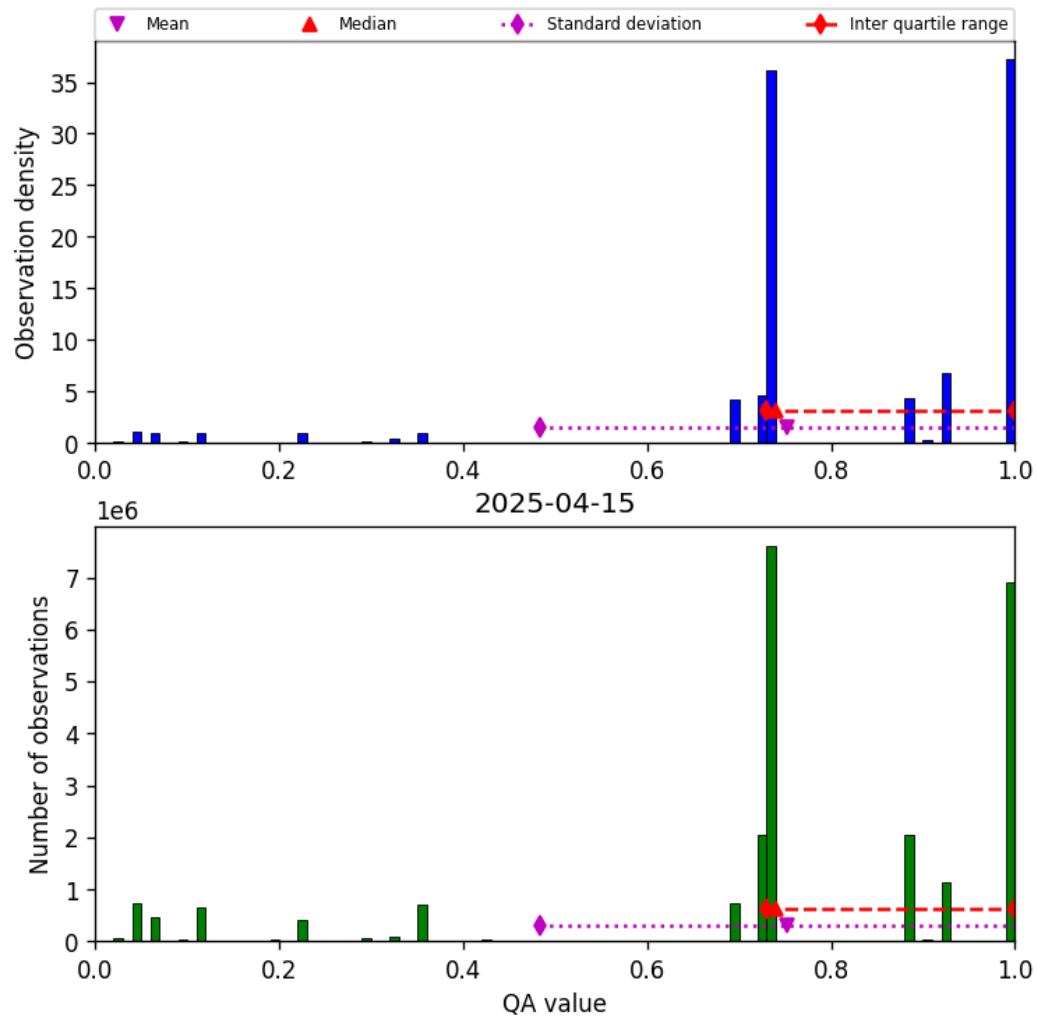
Figure 26: Histogram of “QA value” for 2025-04-15 to 2025-04-16
