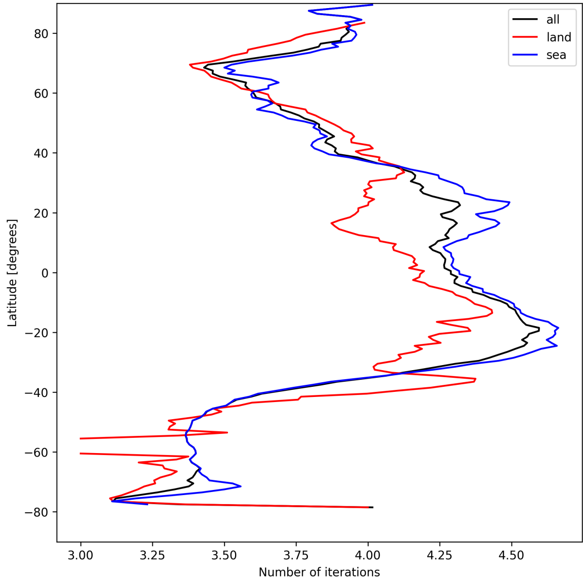
Figure 15: Zonal average of “Number of iterations” for 2025-04-15 to 2025-04-16.
