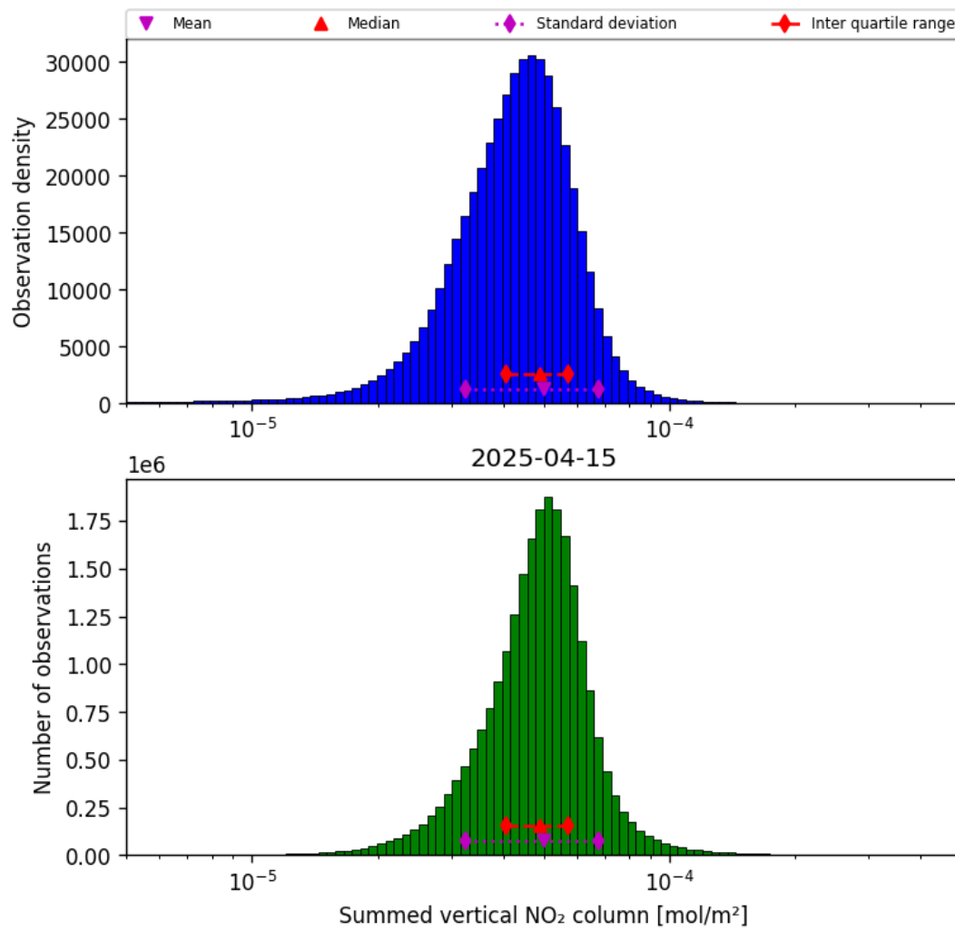
Figure 38: Histogram of "Summed vertical NO 2 column" for 2025-04-15 to 2025-04-16
