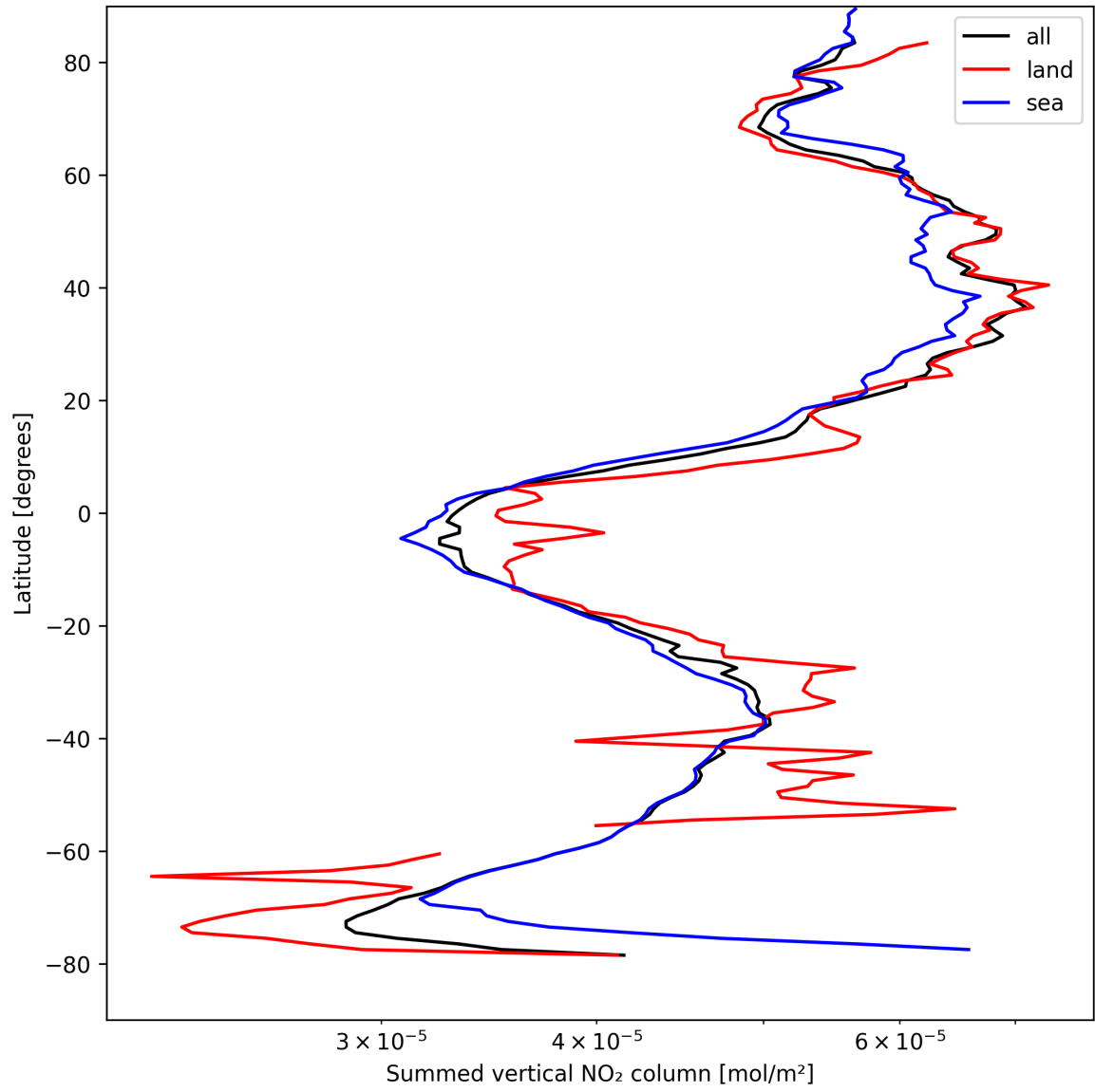
Figure 21: Zonal average of “Summed vertical NO 2 column” for 2025-04-15 to 2025-04-16.
