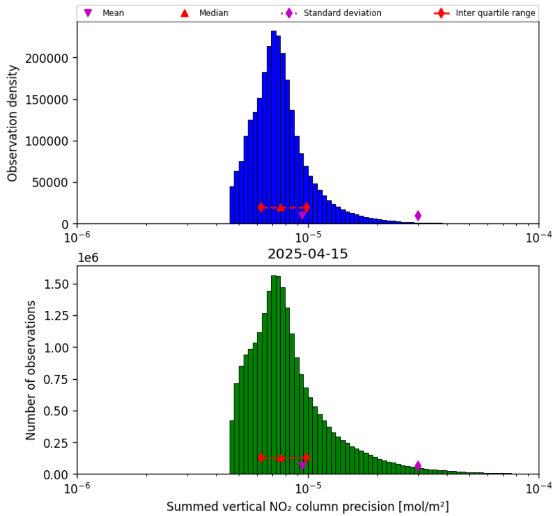
Figure 39: Histogram of "Summed vertical NO 2 column precision" for 2025-04-15 to 2025-04-16
