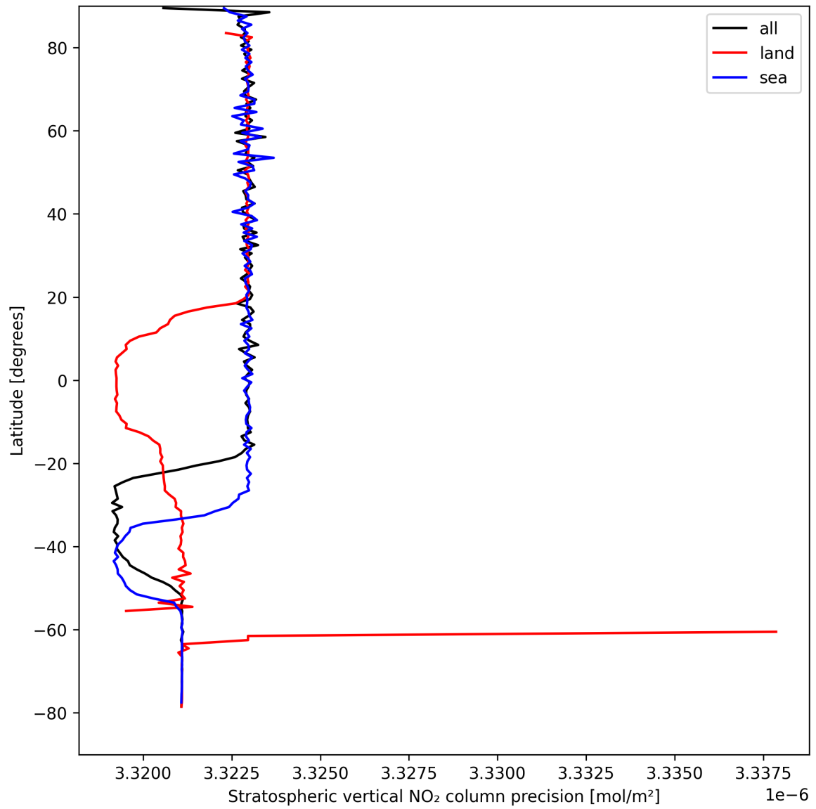
Figure 18: Zonal average of “Stratospheric vertical NO 2 column precision” for 2025-04-15 to 2025-04-16.
