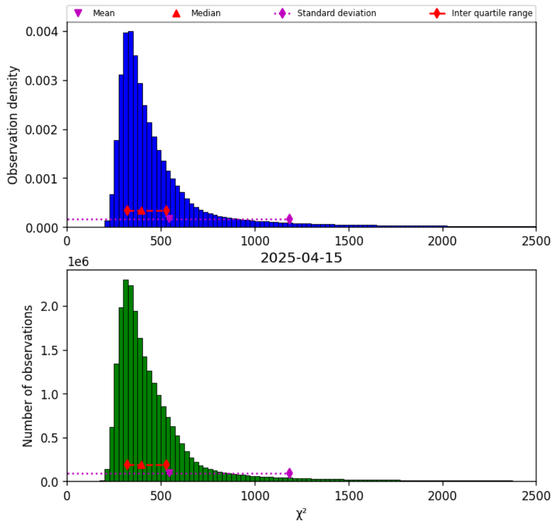
Figure 40: Histogram of “ \chi^2 ” for 2025-04-15 to 2025-04-16
