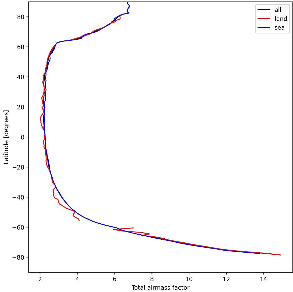
Figure 13: Zonal average of “Total airmass factor” for 2025-04-15 to 2025-04-16.
