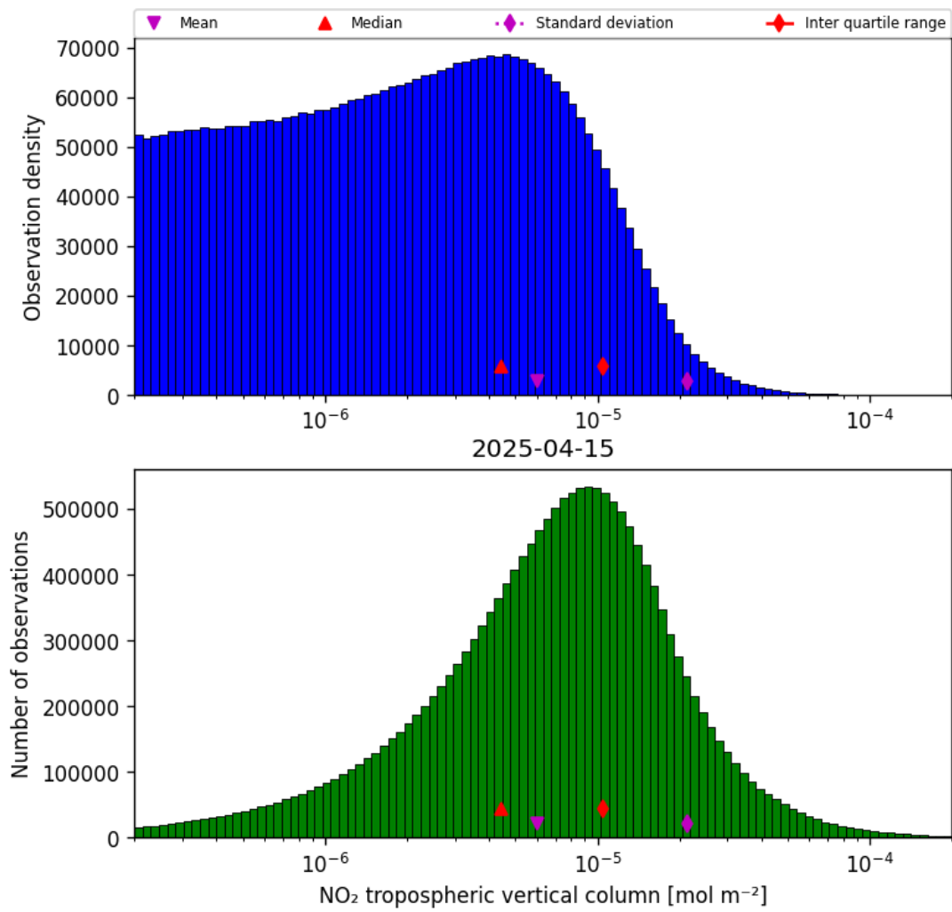
Figure 27: Histogram of “NO 2 tropospheric vertical column” for 2025-04-15 to 2025-04-16
