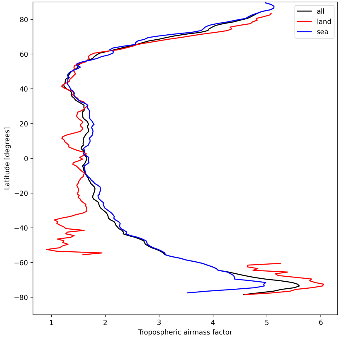
Figure 12: Zonal average of “Tropospheric airmass factor” for 2025-04-15 to 2025-04-16.
