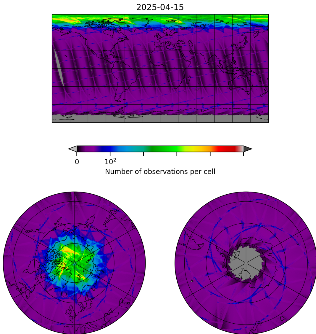
Figure 8: Map of the number of observations for 2025-04-15 to 2025-04-16
