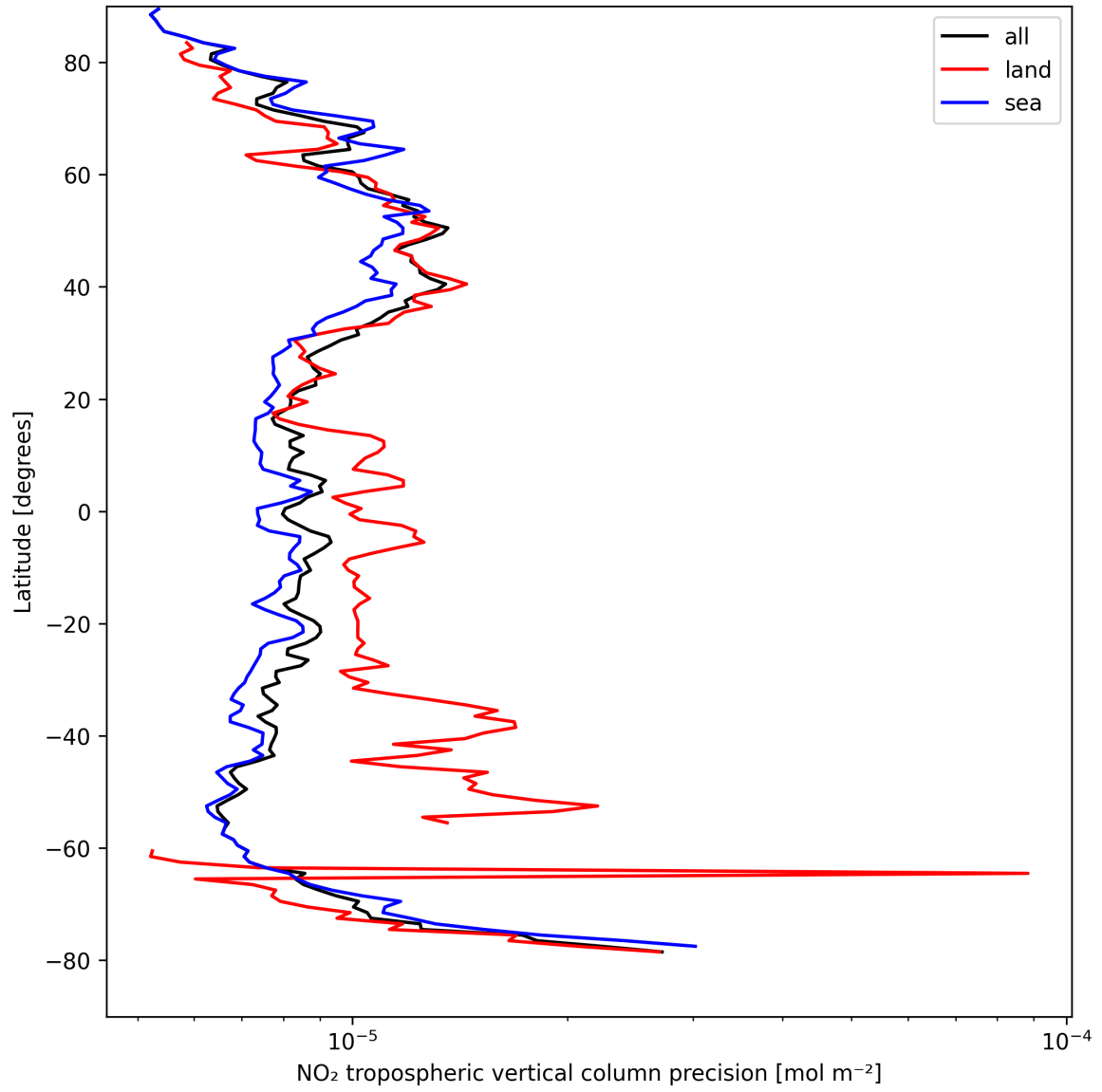
Figure 11: Zonal average of “NO 2 tropospheric vertical column precision” for 2025-04-15 to 2025-04-16.
