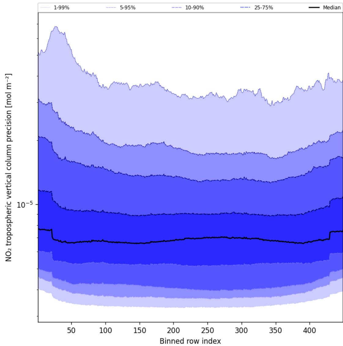
Figure 45: Along track statistics of “NO 2 tropospheric vertical column precision” for 2025-04-15 to 2025-04-16
