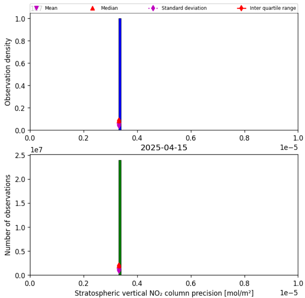
Figure 35: Histogram of “Stratospheric vertical NO 2 column precision” for 2025-04-15 to 2025-04-16
