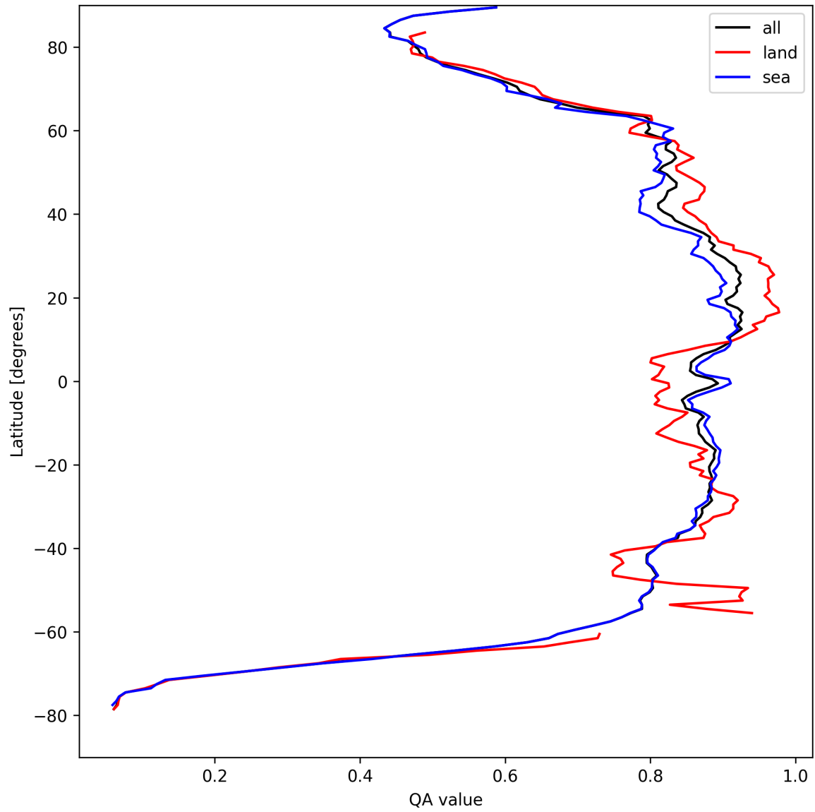
Figure 9: Zonal average of “QA value” for 2025-04-15 to 2025-04-16.
