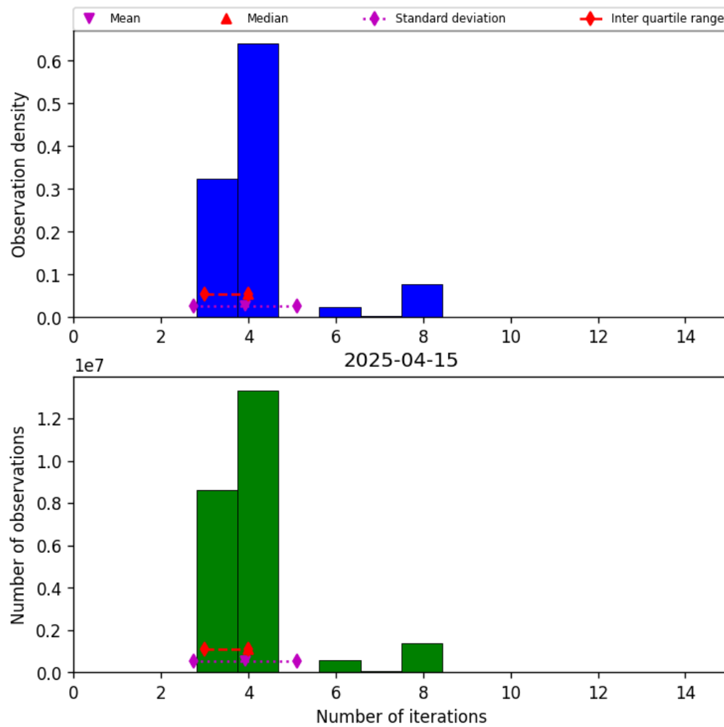
Figure 32: Histogram of “Number of iterations” for 2025-04-15 to 2025-04-16
