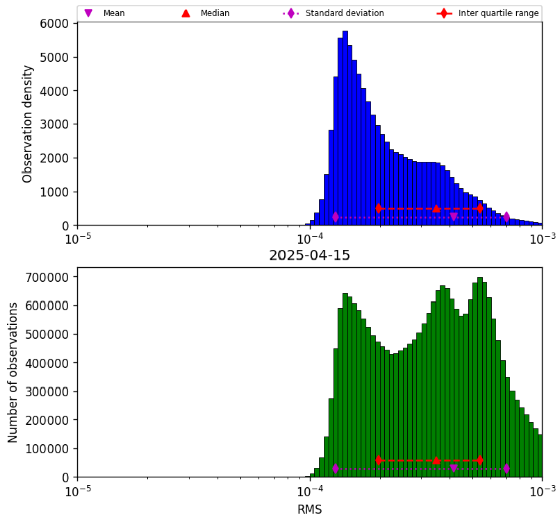
Figure 41: Histogram of “RMS” for 2025-04-15 to 2025-04-16
