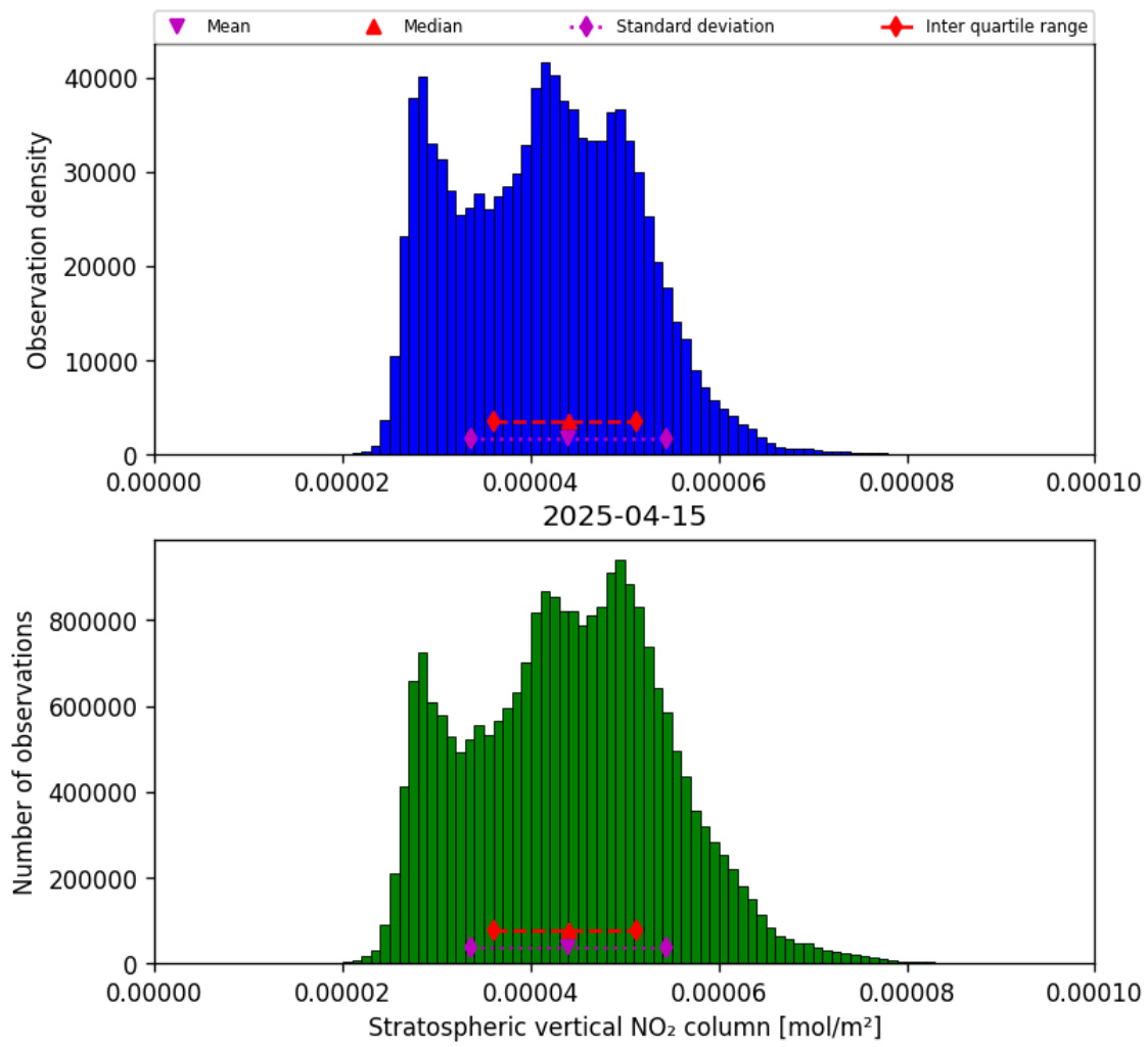
Figure 34: Histogram of “Stratospheric vertical NO 2 column” for 2025-04-15 to 2025-04-16
