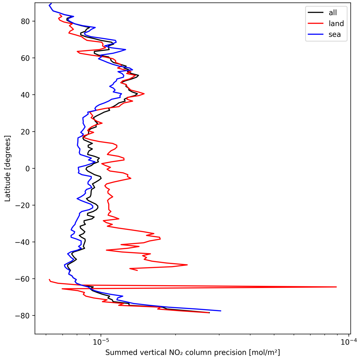
Figure 22: Zonal average of “Summed vertical NO 2 column precision” for 2025-04-15 to 2025-04-16.
