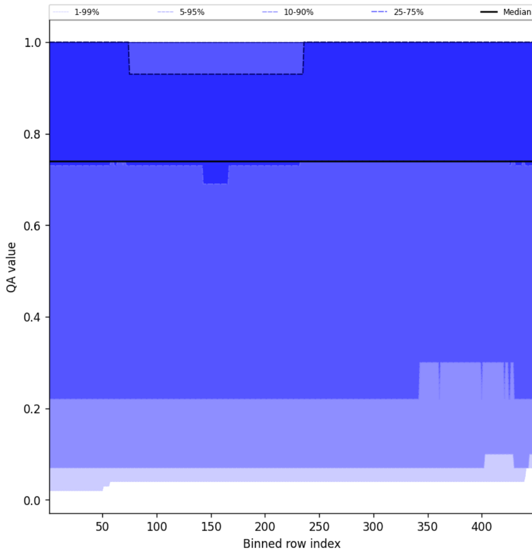
Figure 43: Along track statistics of "QA value" for 2025-04-15 to 2025-04-16
