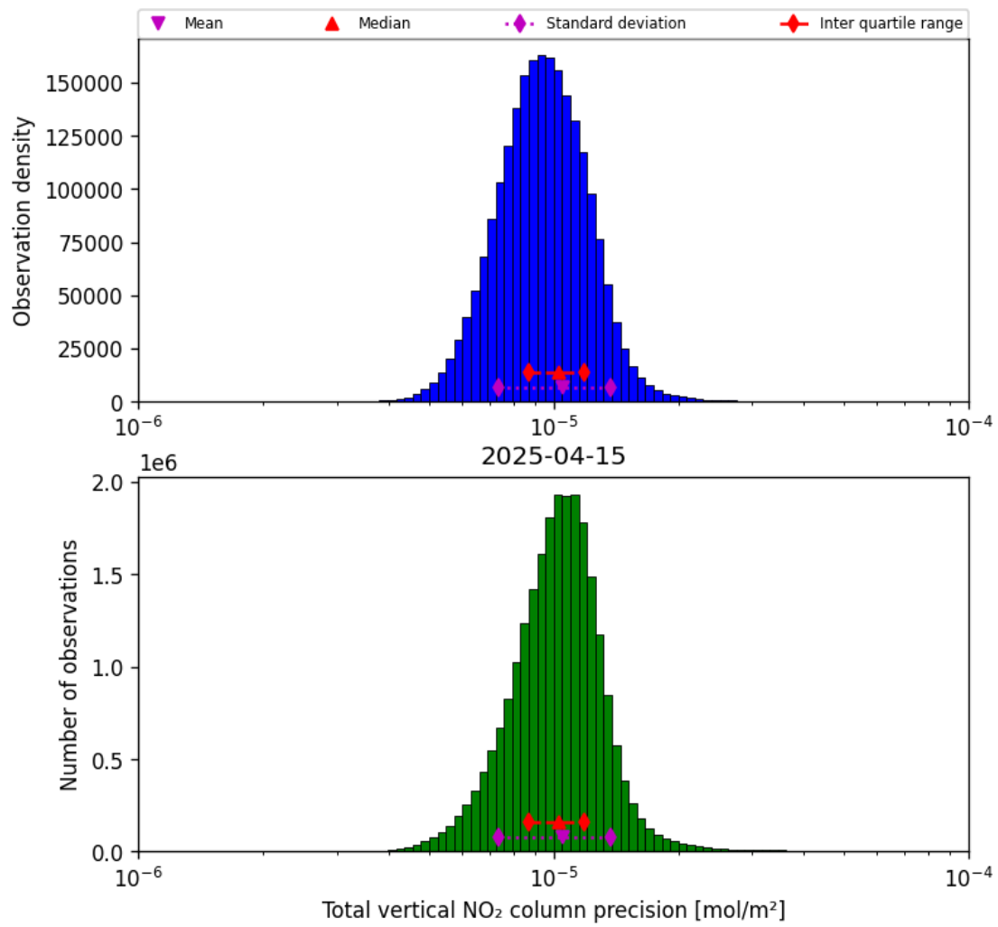
Figure 37: Histogram of "Total vertical NO 2 column precision" for 2025-04-15 to 2025-04-16
