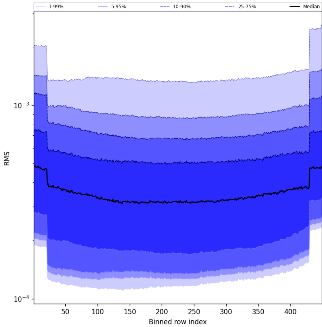
Figure 58: Along track statistics of “RMS” for 2025-04-16 to 2025-04-16
