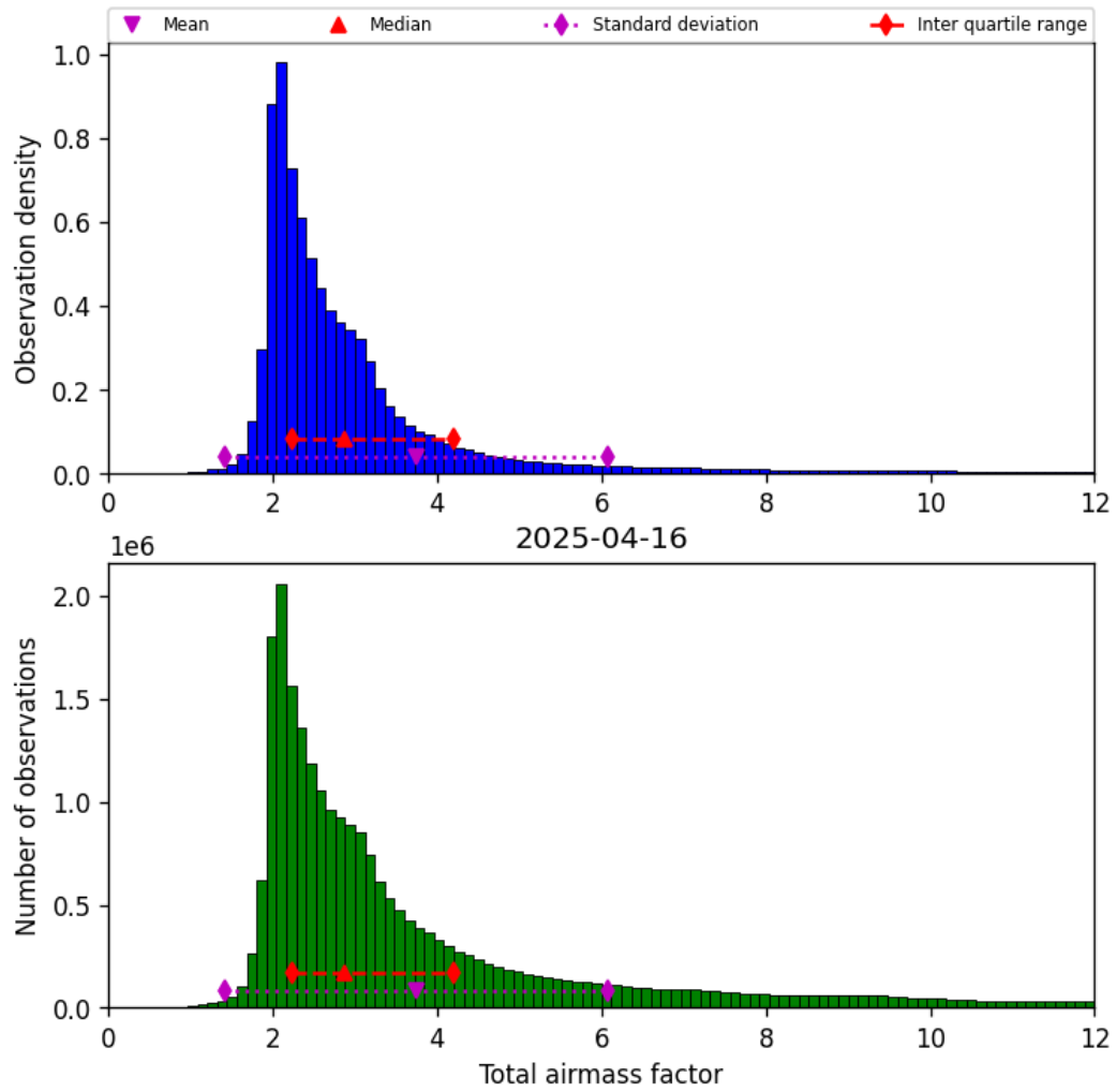
Figure 30: Histogram of “Total airmass factor” for 2025-04-16 to 2025-04-16
