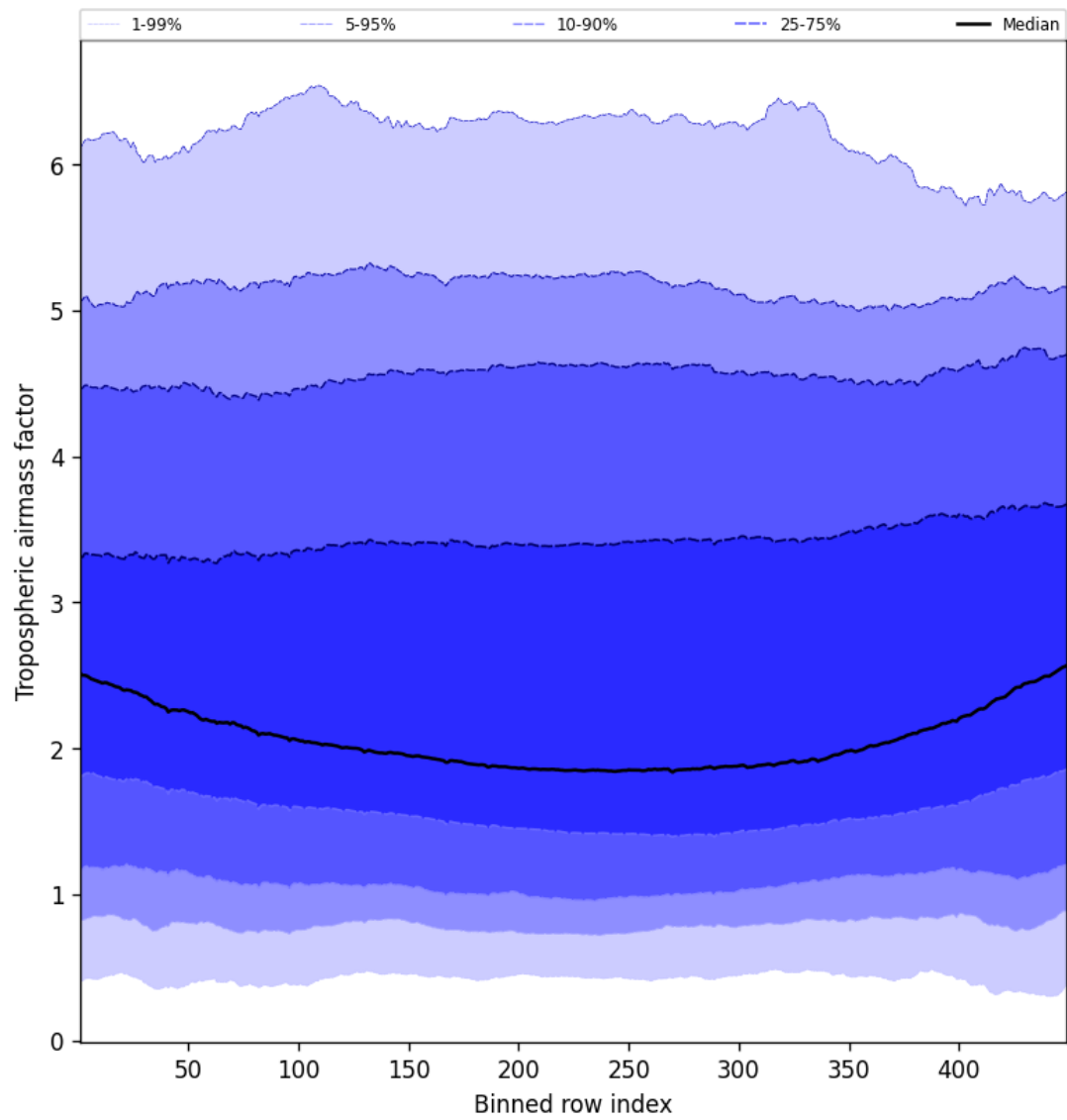
Figure 46: Along track statistics of “Tropospheric airmass factor” for 2025-04-16 to 2025-04-16
