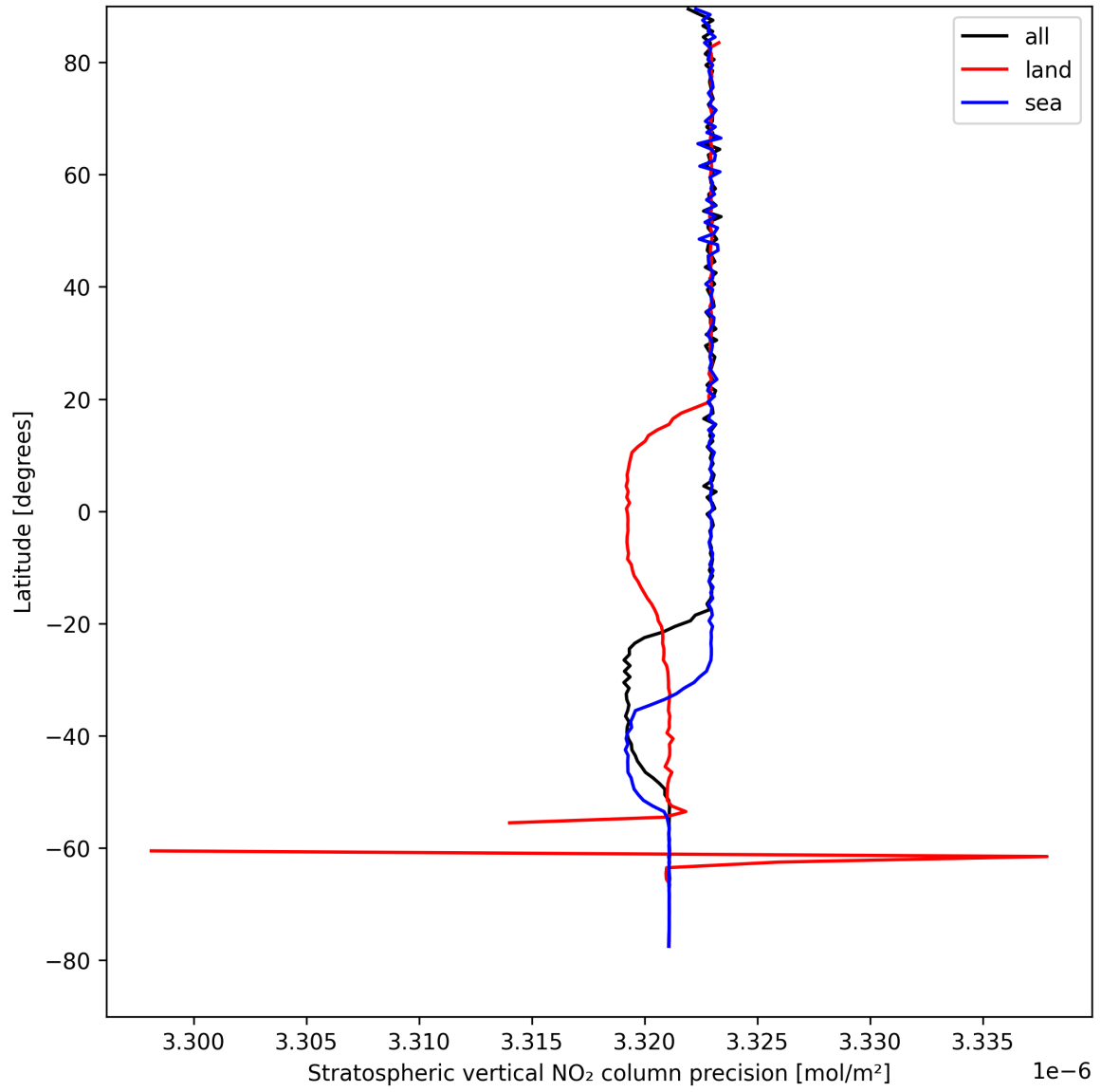
Figure 18: Zonal average of “Stratospheric vertical NO 2 column precision” for 2025-04-16 to 2025-04-16.
