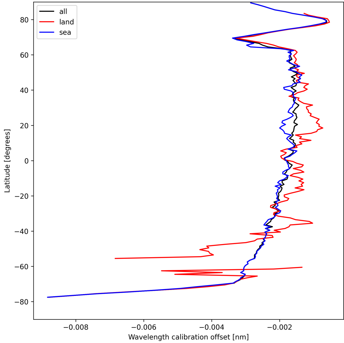
Figure 16: Zonal average of “Wavelength calibration offset” for 2025-04-16 to 2025-04-16.
