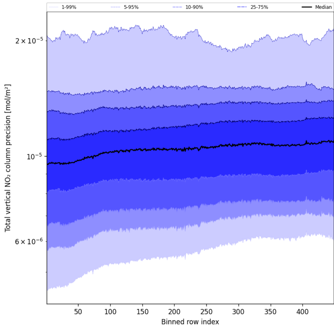
Figure 54: Along track statistics of “Total vertical NO 2 column precision” for 2025-04-16 to 2025-04-16
