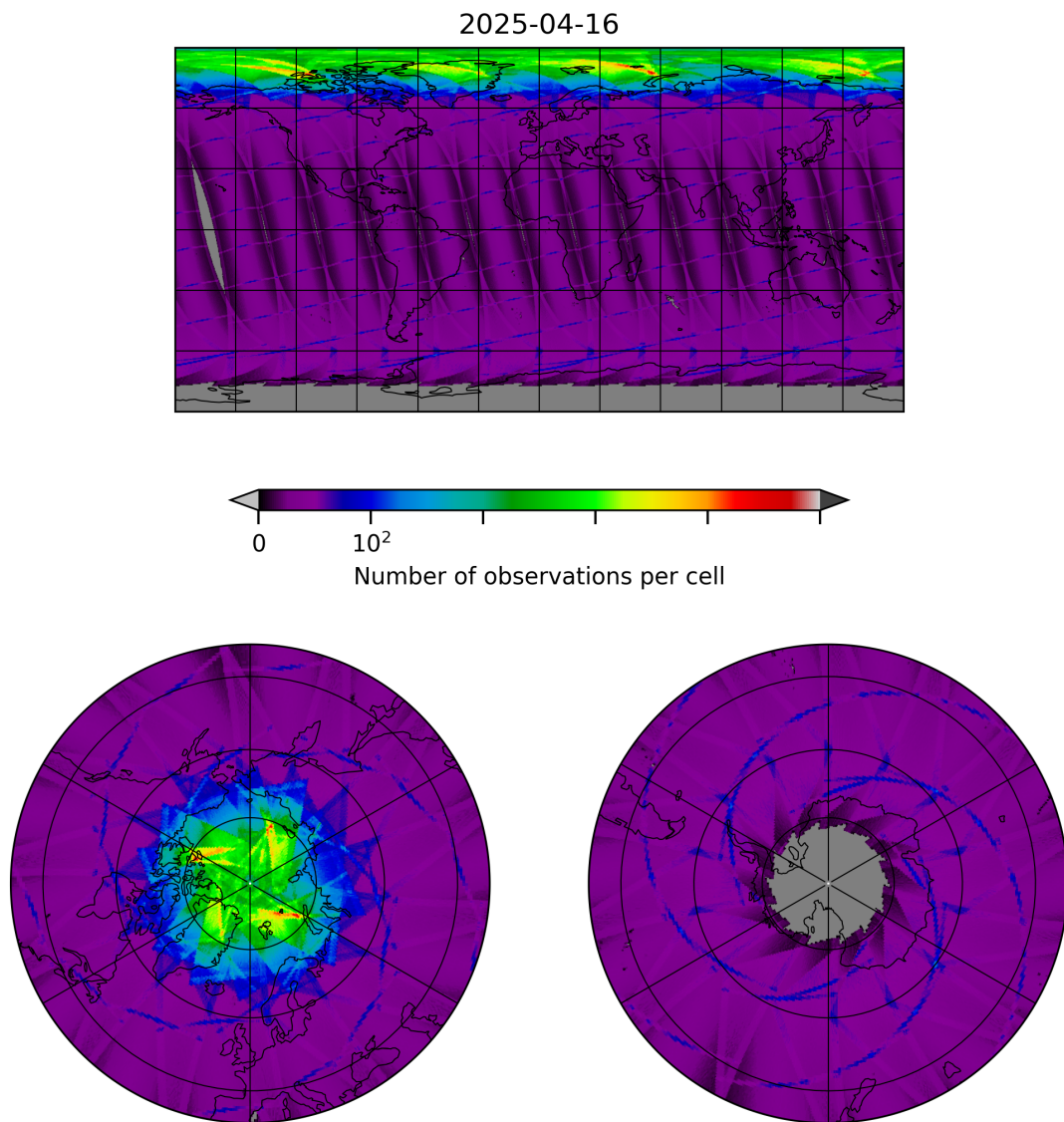
Figure 8: Map of the number of observations for 2025-04-16 to 2025-04-16
