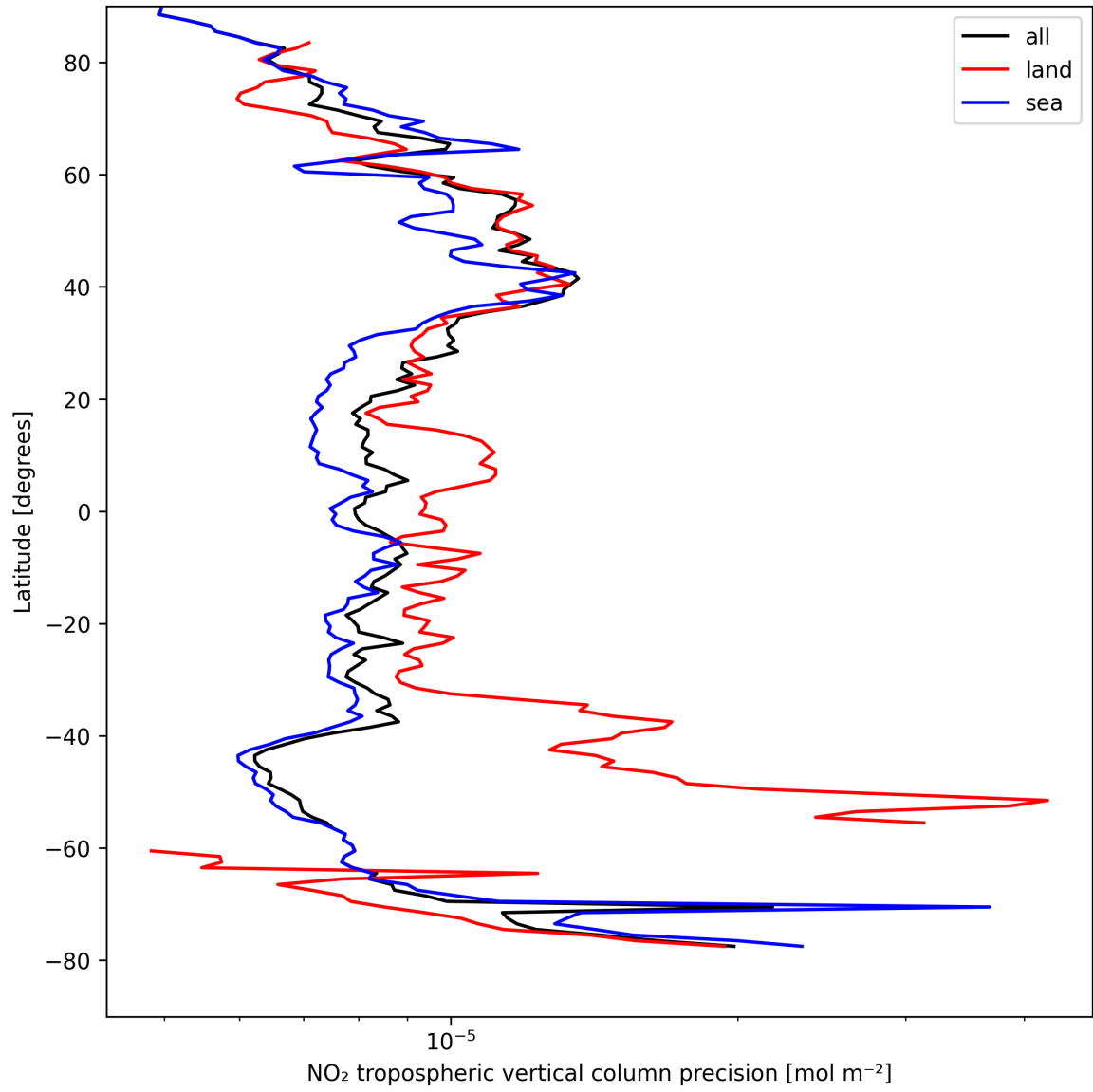
Figure 11: Zonal average of “NO 2 tropospheric vertical column precision” for 2025-04-16 to 2025-04-16.
