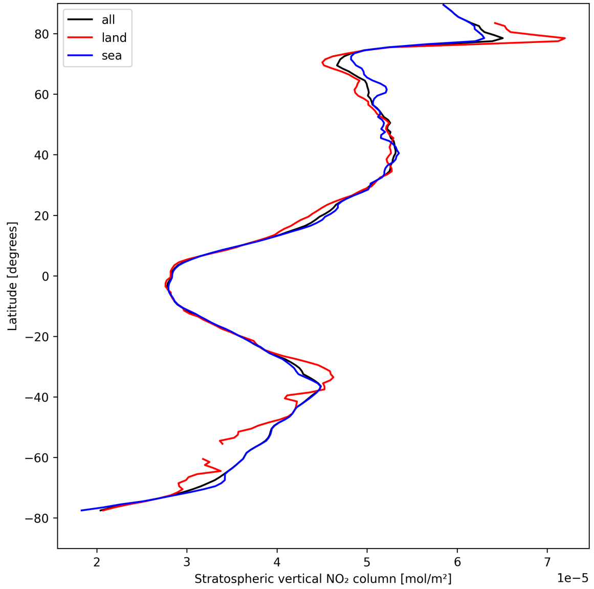
Figure 17: Zonal average of “Stratospheric vertical NO 2 column” for 2025-04-16 to 2025-04-16.
