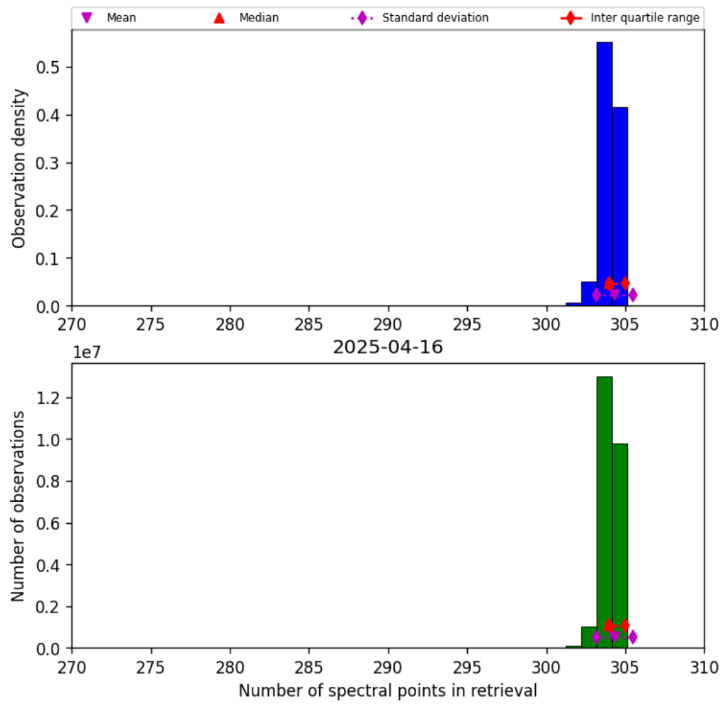
Figure 31: Histogram of “Number of spectral points in retrieval” for 2025-04-16 to 2025-04-16
