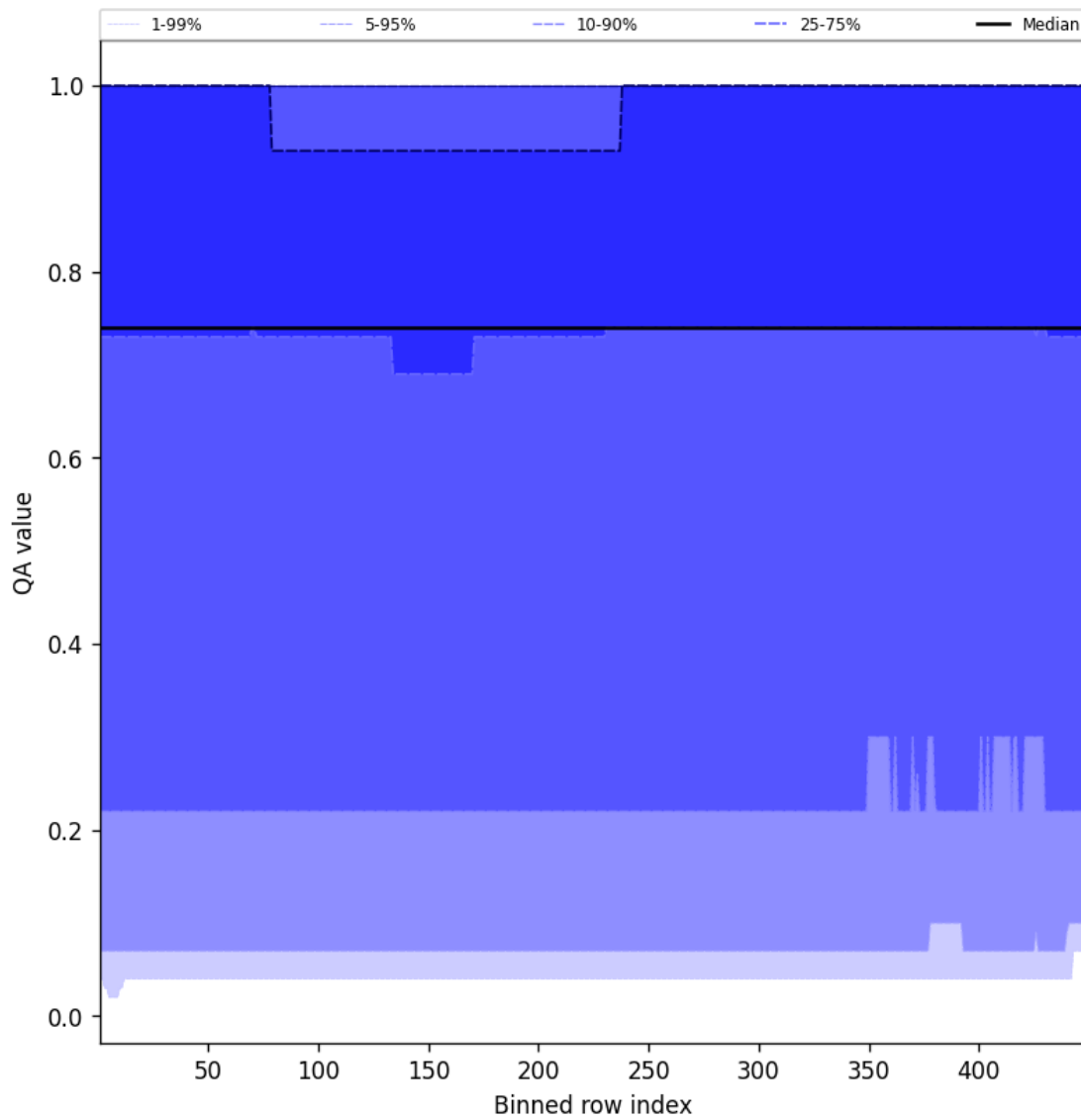
Figure 43: Along track statistics of "QA value" for 2025-04-16 to 2025-04-16
