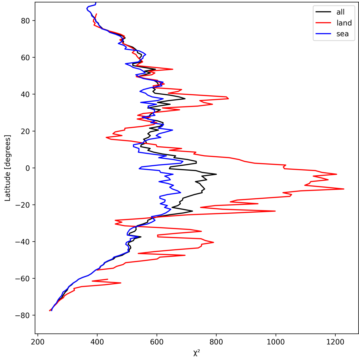
Figure 23: Zonal average of “ \chi^2 ” for 2025-04-16 to 2025-04-16.
