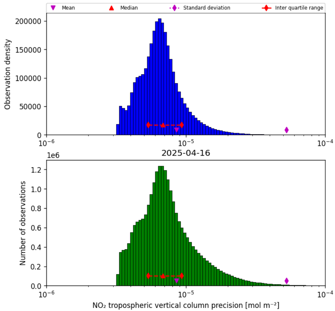
Figure 28: Histogram of “NO 2 tropospheric vertical column precision” for 2025-04-16 to 2025-04-16
