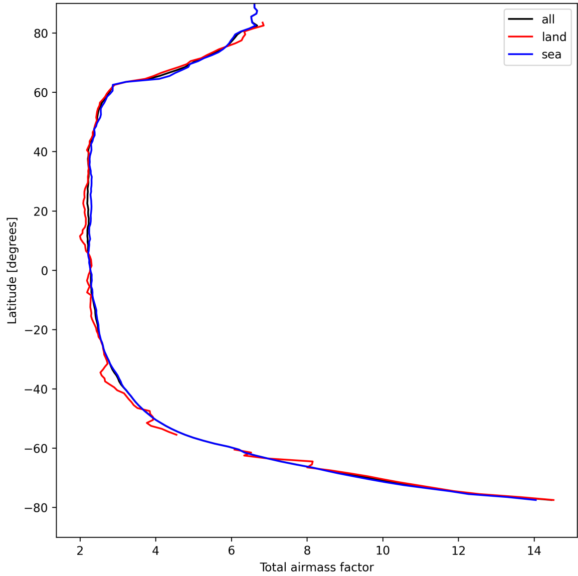
Figure 13: Zonal average of “Total airmass factor” for 2025-04-16 to 2025-04-16.
