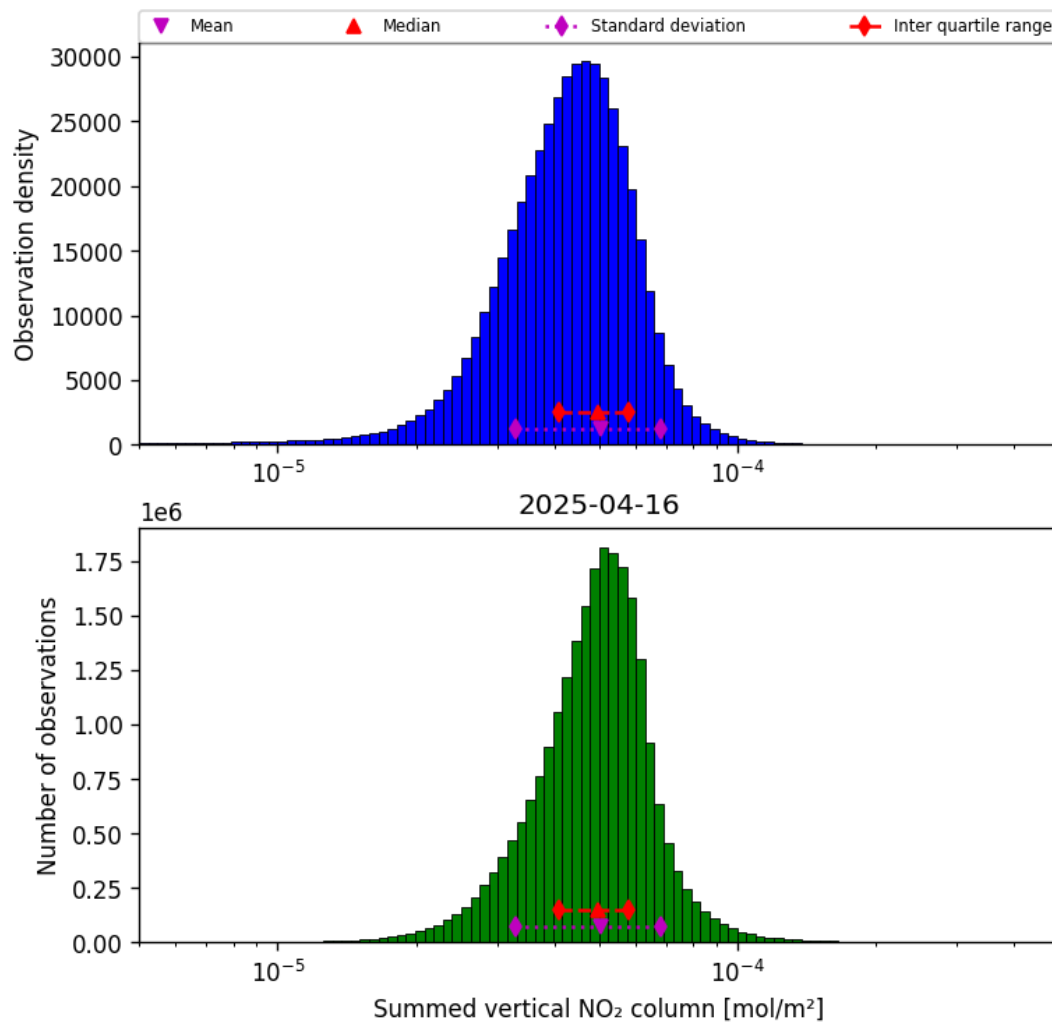
Figure 38: Histogram of “Summed vertical NO 2 column” for 2025-04-16 to 2025-04-16
