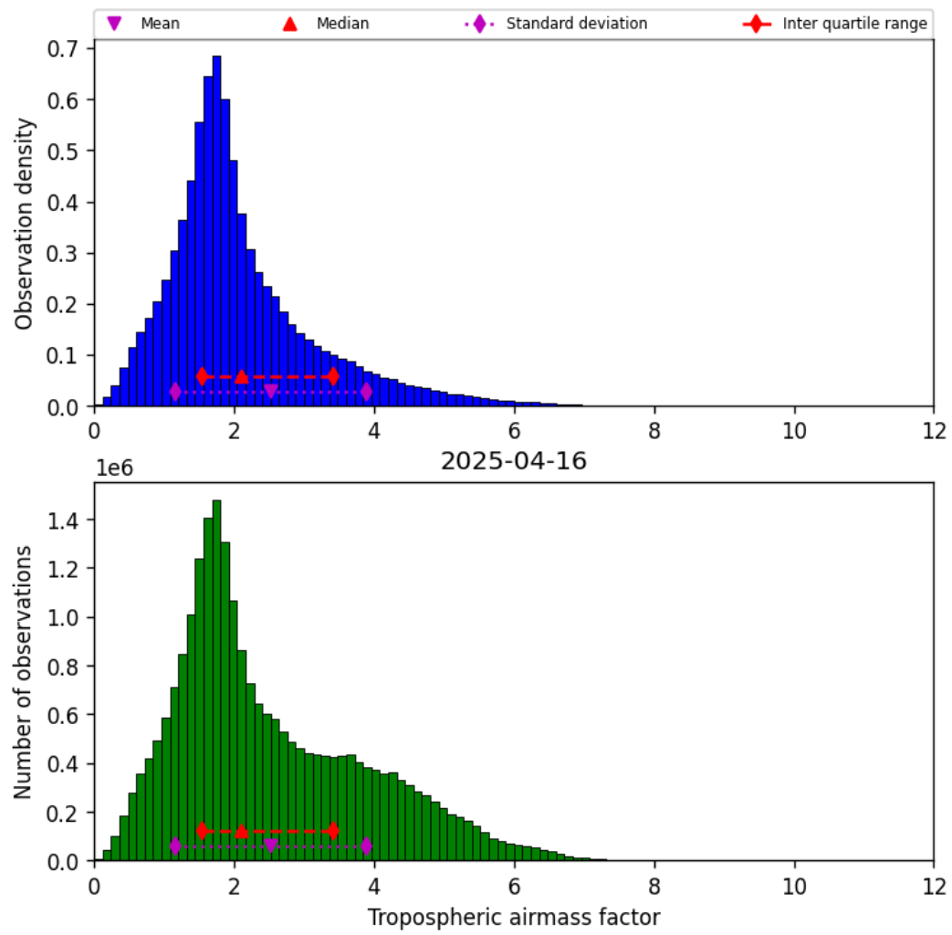
Figure 29: Histogram of “Tropospheric airmass factor” for 2025-04-16 to 2025-04-16
