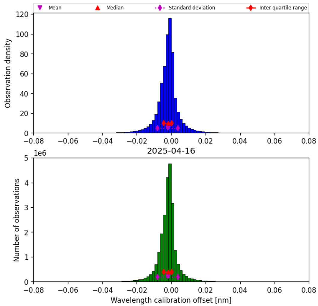
Figure 33: Histogram of “Wavelength calibration offset” for 2025-04-16 to 2025-04-16
