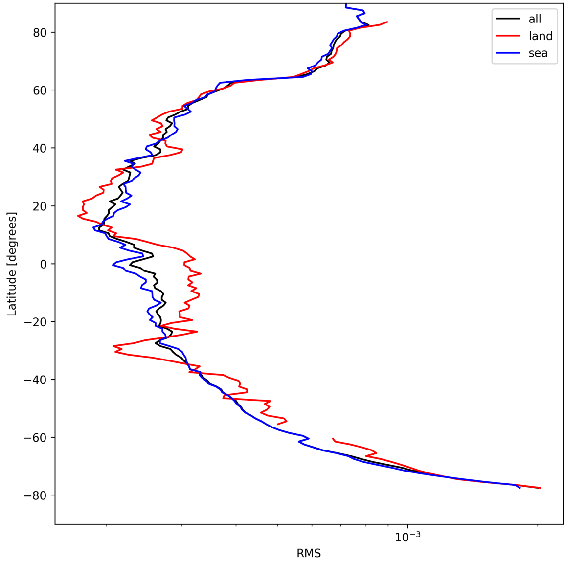
Figure 24: Zonal average of “RMS” for 2025-04-16 to 2025-04-16.
