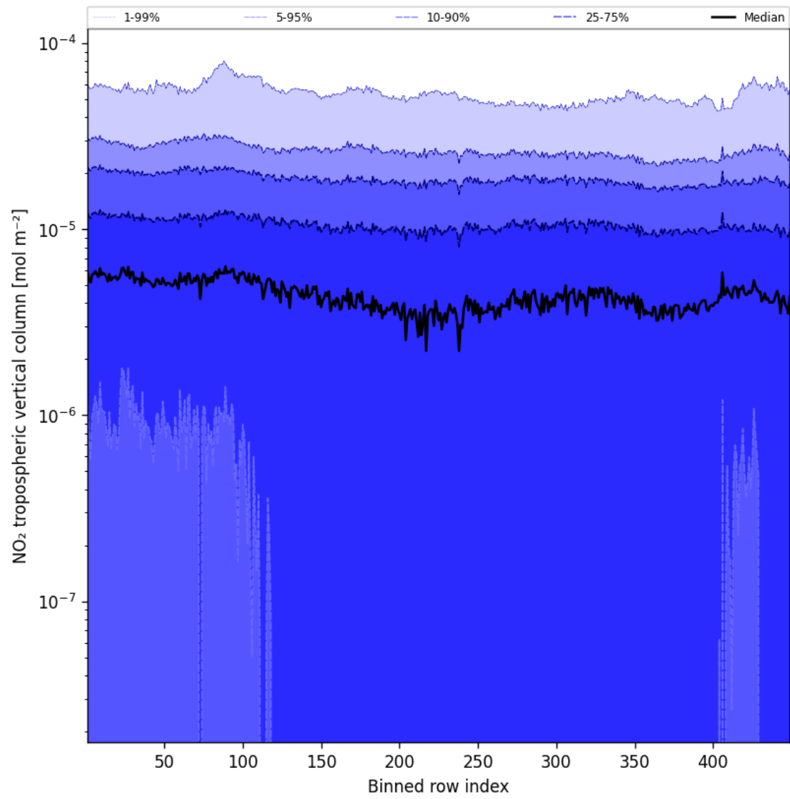
Figure 44: Along track statistics of "NO 2 tropospheric vertical column" for 2025-04-16 to 2025-04-16
