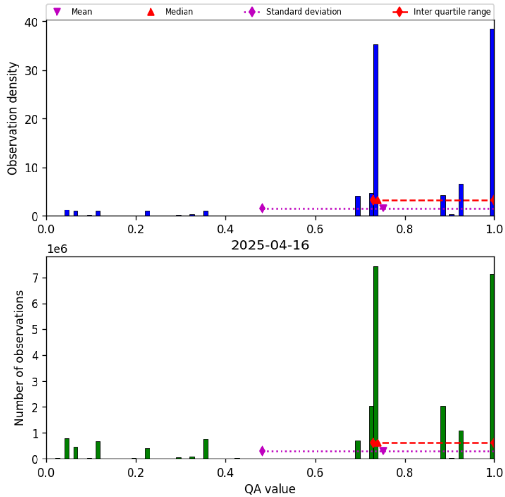
Figure 26: Histogram of “QA value” for 2025-04-16 to 2025-04-16
