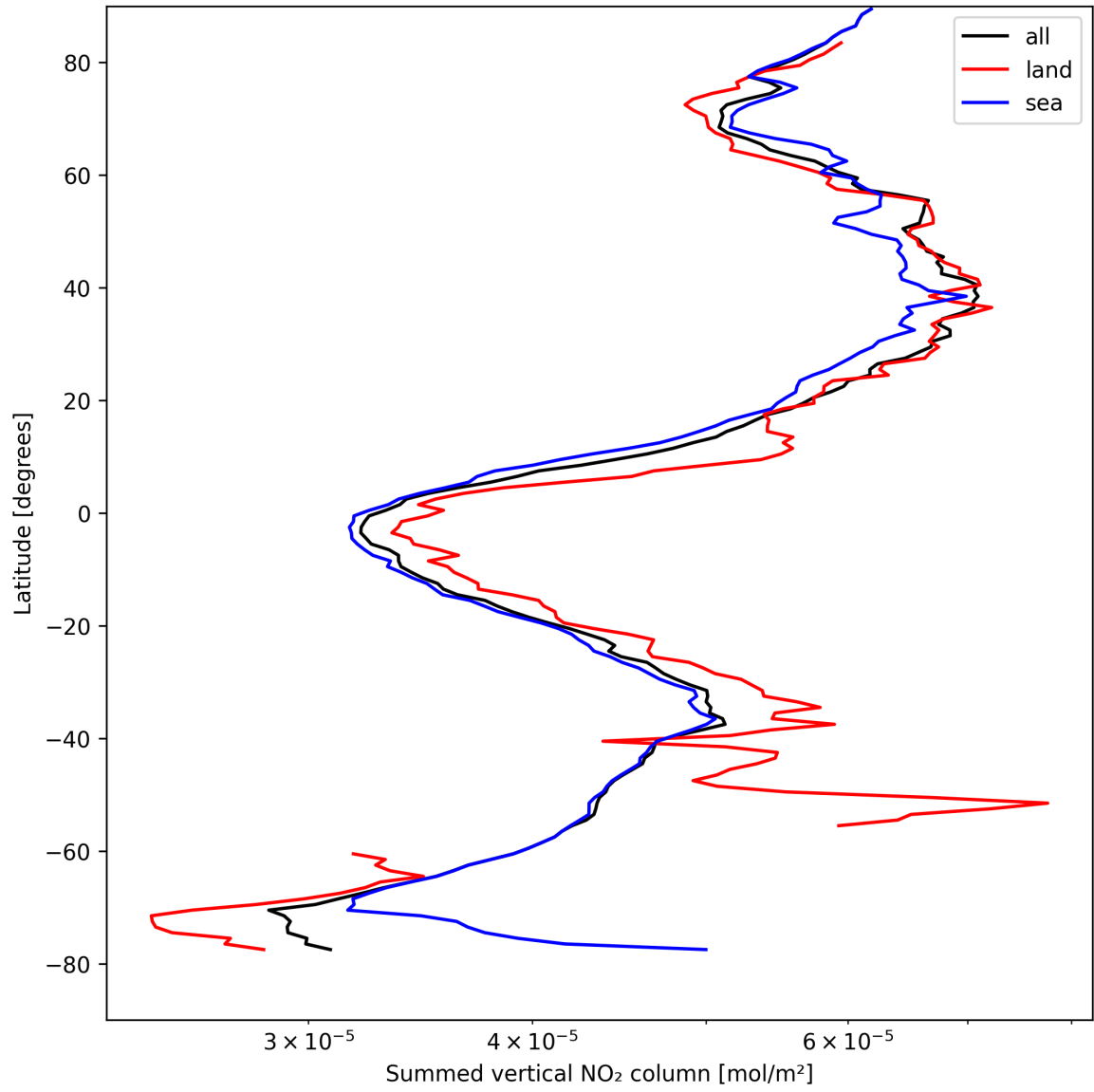
Figure 21: Zonal average of “Summed vertical NO 2 column” for 2025-04-16 to 2025-04-16.
