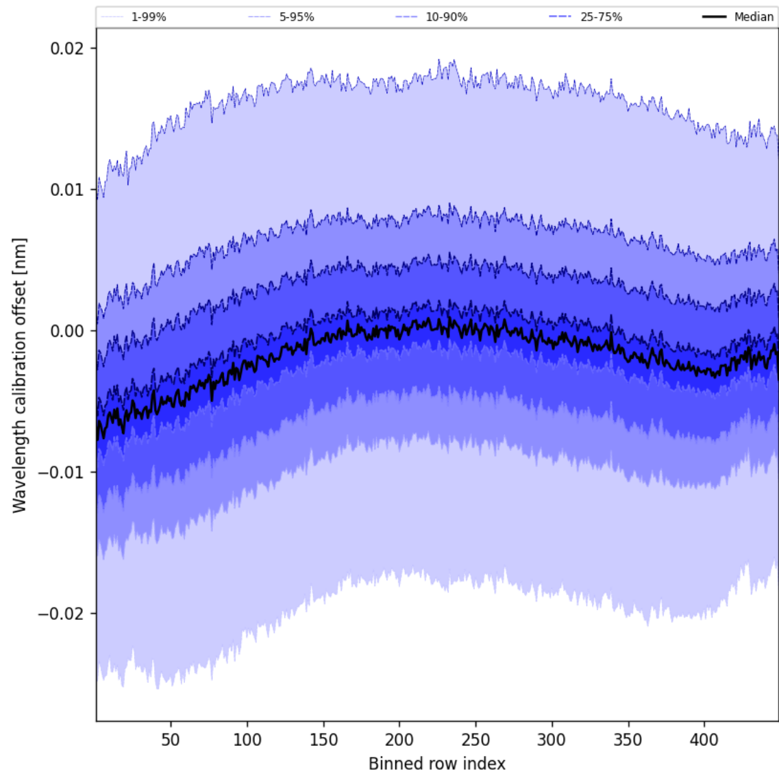
Figure 50: Along track statistics of “Wavelength calibration offset” for 2025-04-16 to 2025-04-16
