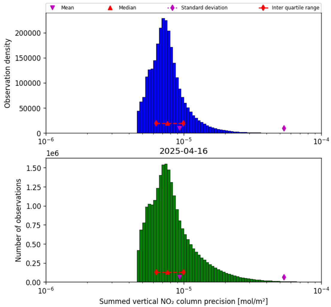
Figure 39: Histogram of "Summed vertical NO 2 column precision" for 2025-04-16 to 2025-04-16
