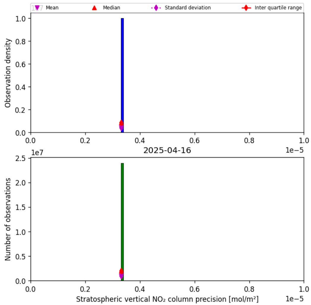
Figure 35: Histogram of “Stratospheric vertical NO 2 column precision” for 2025-04-16 to 2025-04-16
