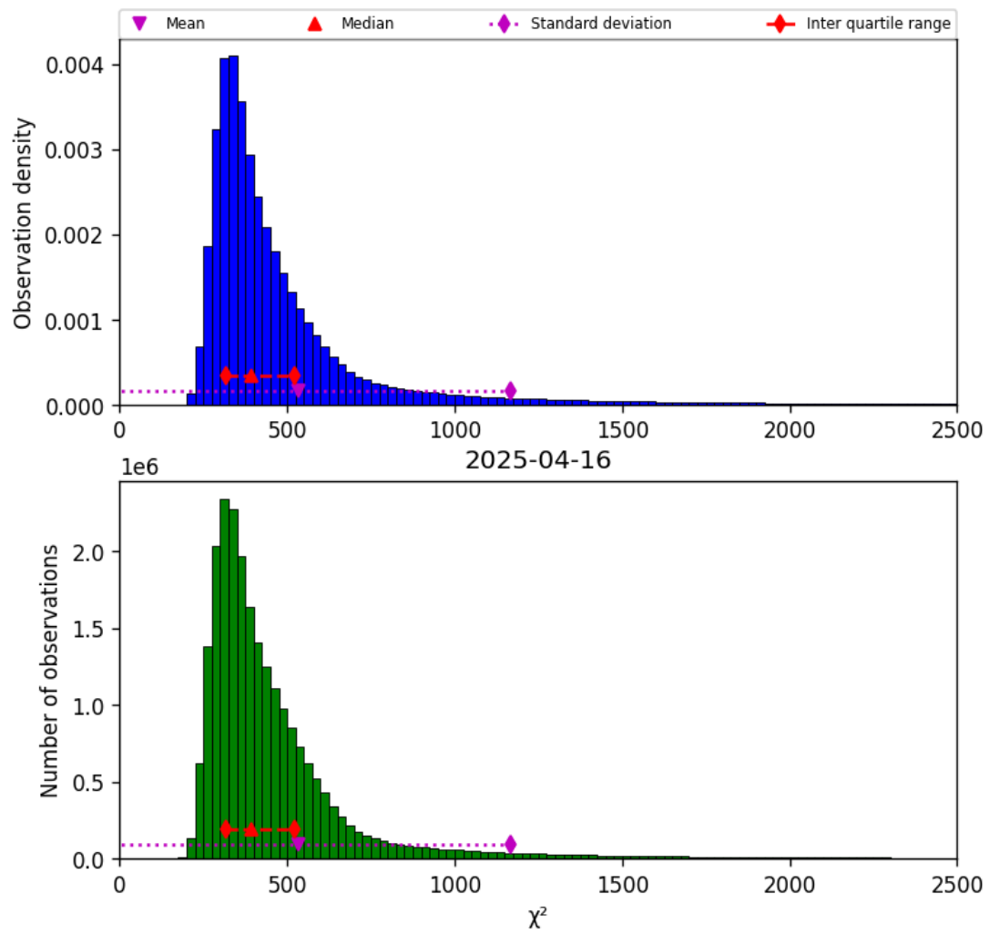
Figure 40: Histogram of “ \chi^2 ” for 2025-04-16 to 2025-04-16
