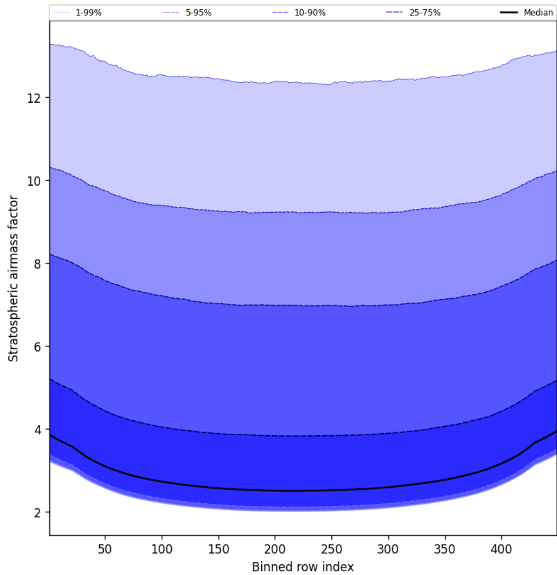
Figure 59: Along track statistics of “Stratospheric airmass factor” for 2025-04-16 to 2025-04-16
