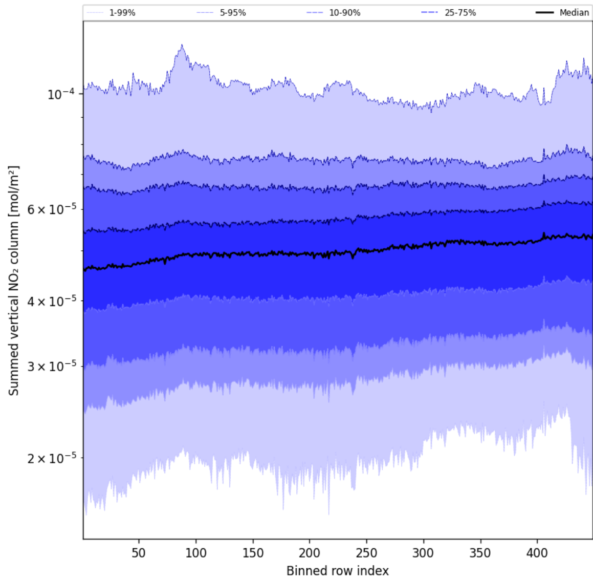
Figure 55: Along track statistics of “Summed vertical NO 2 column” for 2025-04-16 to 2025-04-16
