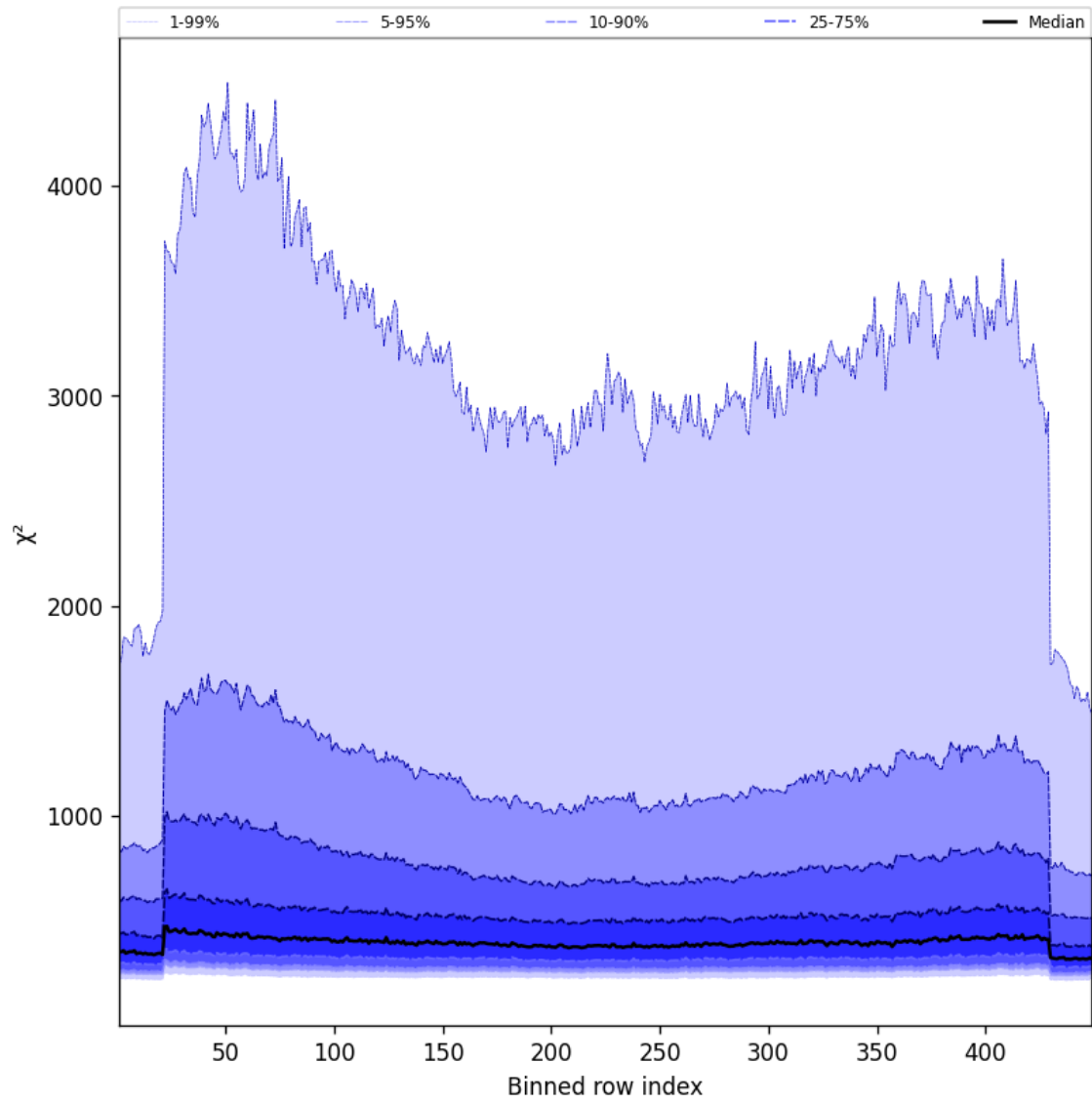
Figure 57: Along track statistics of “ \chi^2 ” for 2025-04-16 to 2025-04-16
