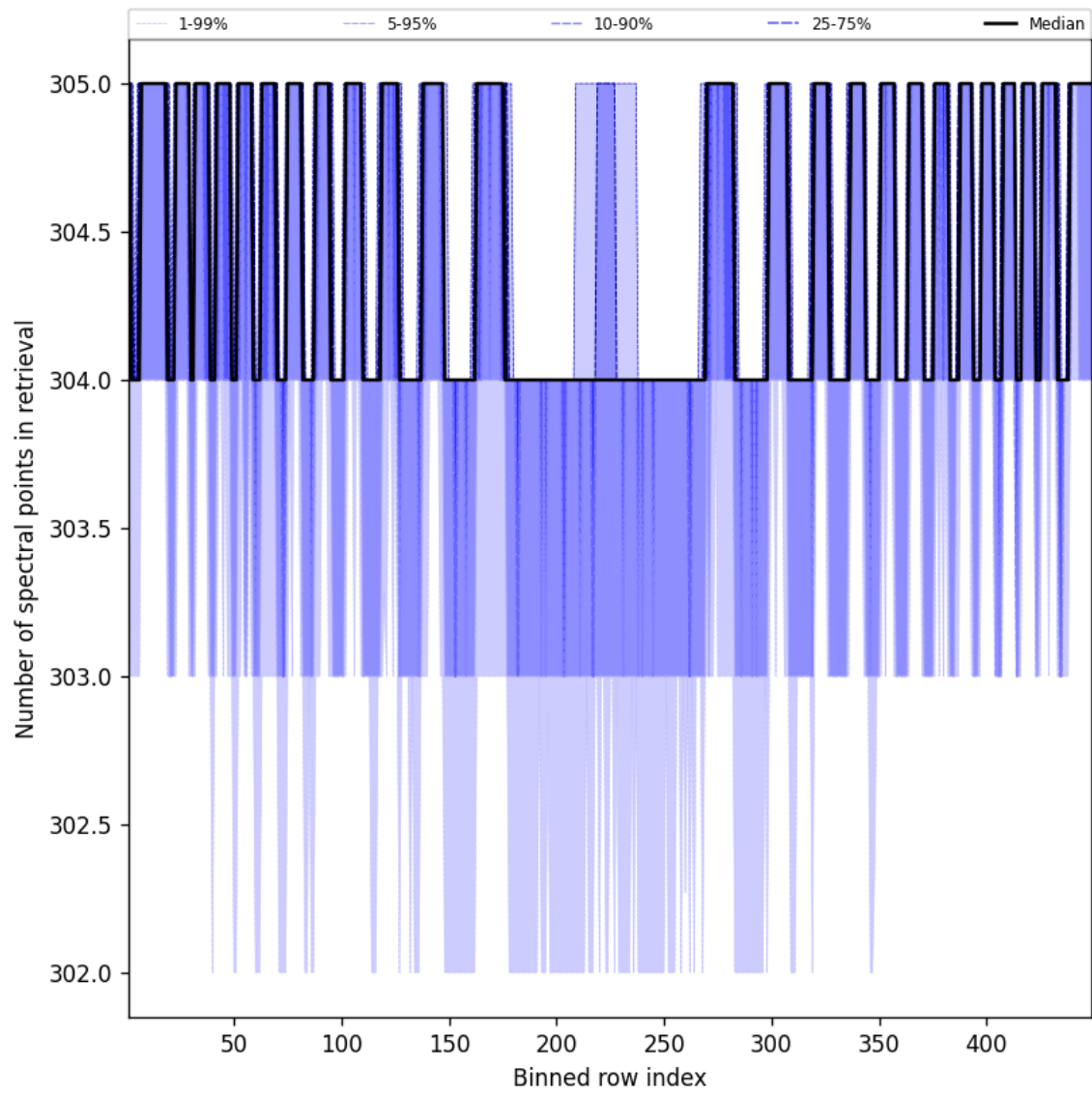
Figure 48: Along track statistics of “Number of spectral points in retrieval” for 2025-04-16 to 2025-04-16
