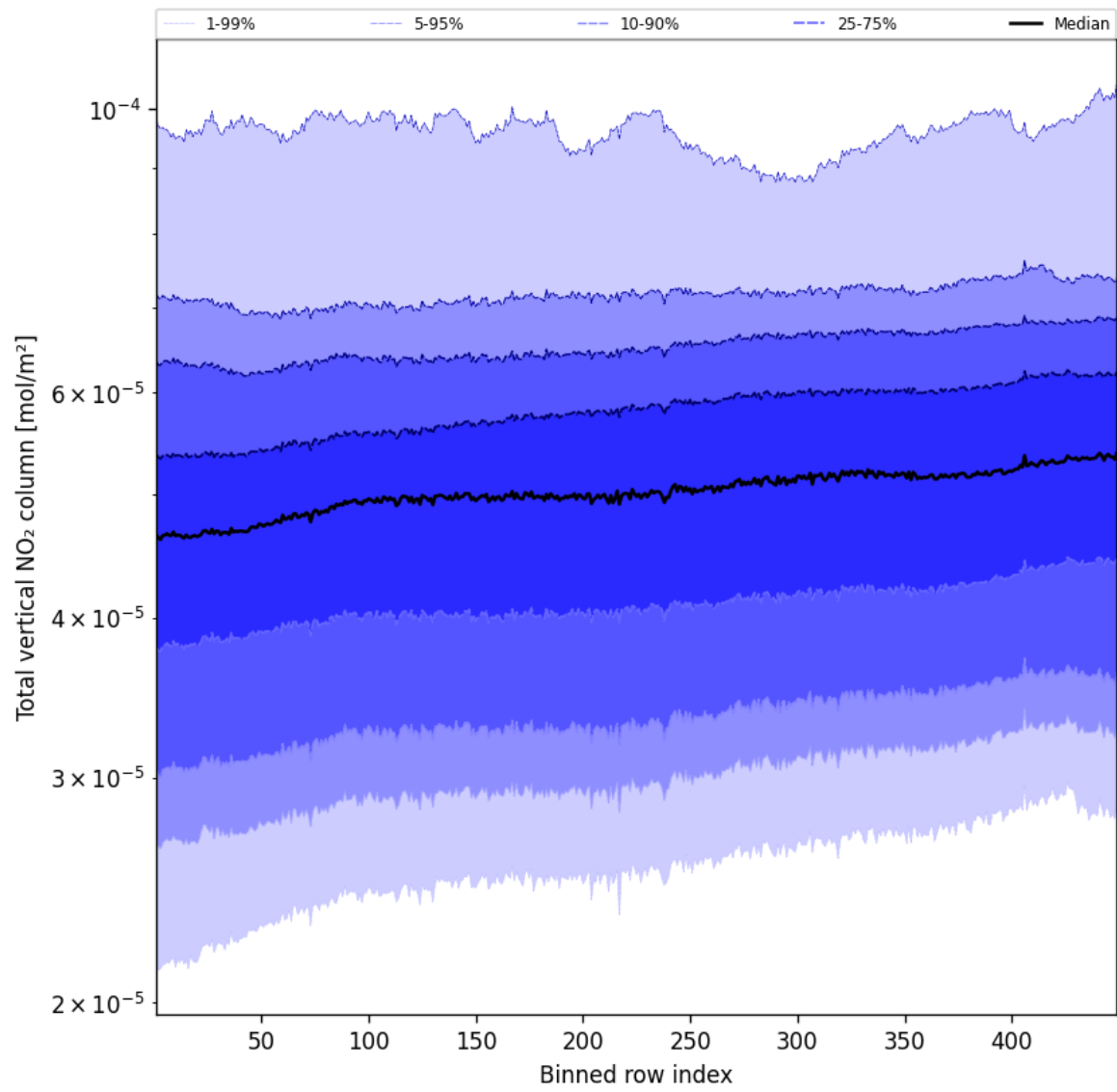
Figure 53: Along track statistics of “Total vertical NO 2 column” for 2025-04-16 to 2025-04-16
