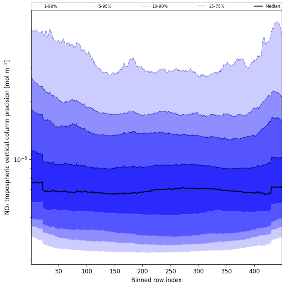
Figure 45: Along track statistics of “NO 2 tropospheric vertical column precision” for 2025-04-16 to 2025-04-16
