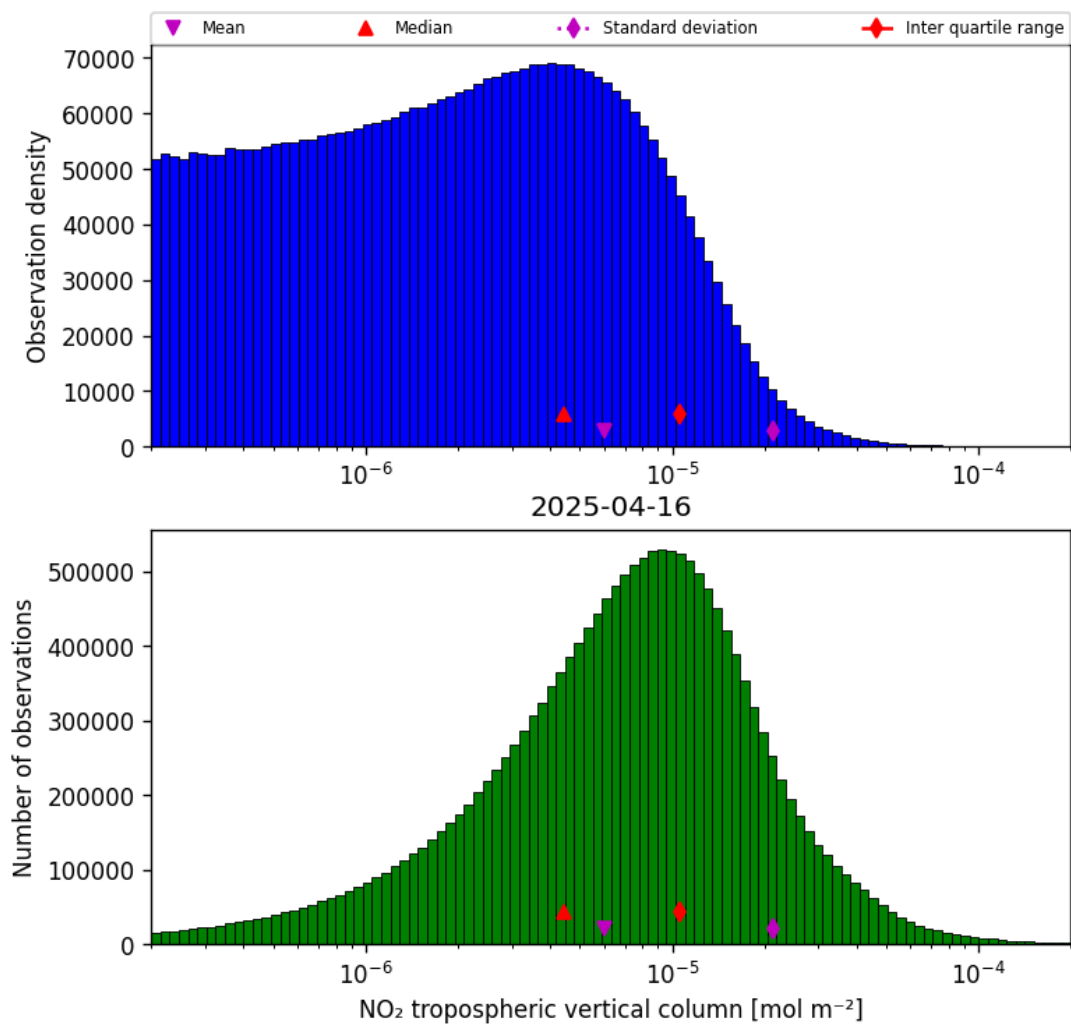
Figure 27: Histogram of “ \text{NO}_2 tropospheric vertical column” for 2025-04-16 to 2025-04-16
