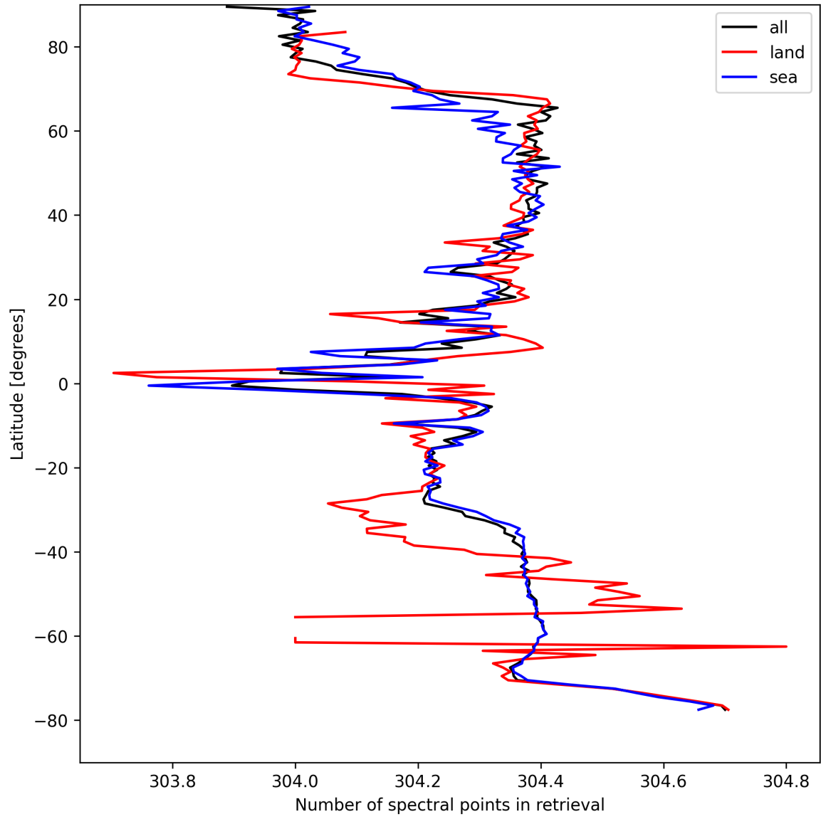
Figure 14: Zonal average of “Number of spectral points in retrieval” for 2025-04-16 to 2025-04-16.
