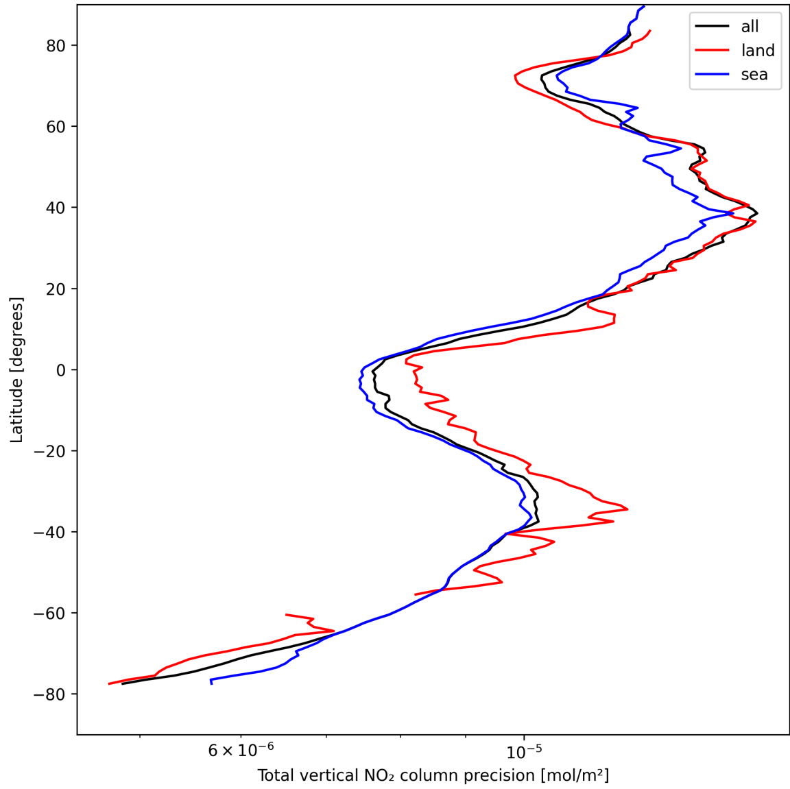
Figure 20: Zonal average of “Total vertical NO 2 column precision” for 2025-04-16 to 2025-04-16.
