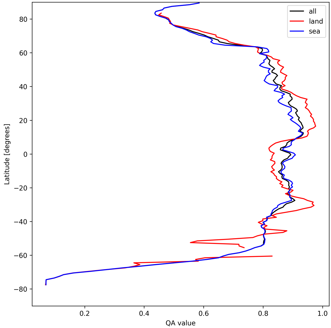
Figure 9: Zonal average of “QA value” for 2025-04-16 to 2025-04-16.
