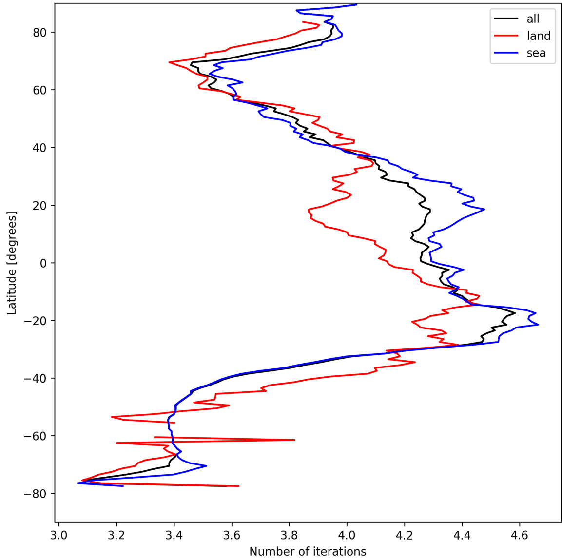
Figure 15: Zonal average of “Number of iterations” for 2025-04-16 to 2025-04-16.
