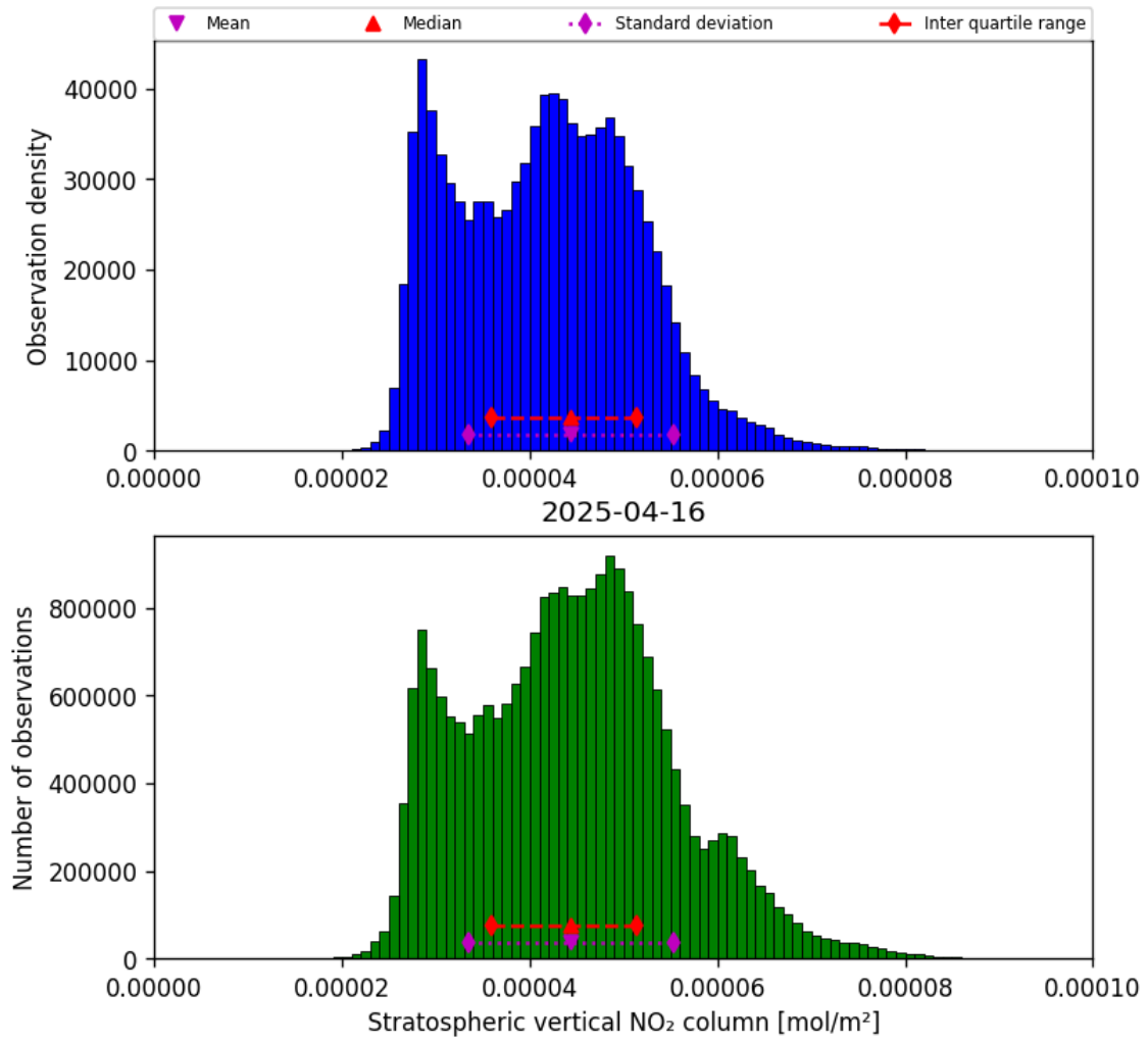
Figure 34: Histogram of “Stratospheric vertical NO 2 column” for 2025-04-16 to 2025-04-16
