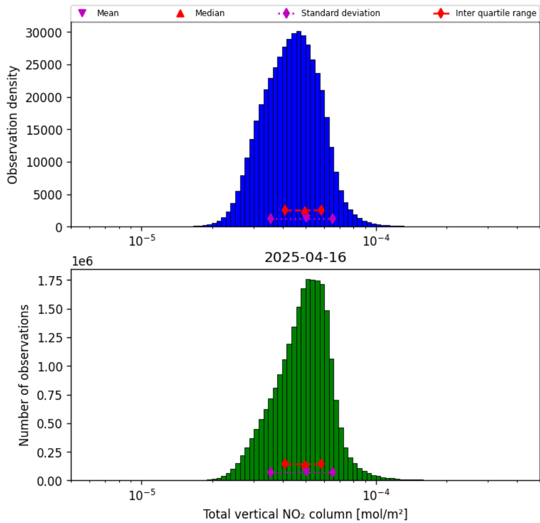
Figure 36: Histogram of "Total vertical NO 2 column" for 2025-04-16 to 2025-04-16
