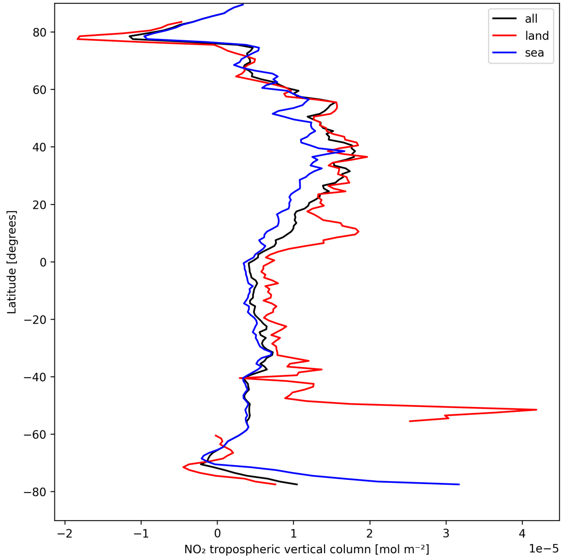
Figure 10: Zonal average of “NO 2 tropospheric vertical column” for 2025-04-16 to 2025-04-16.
