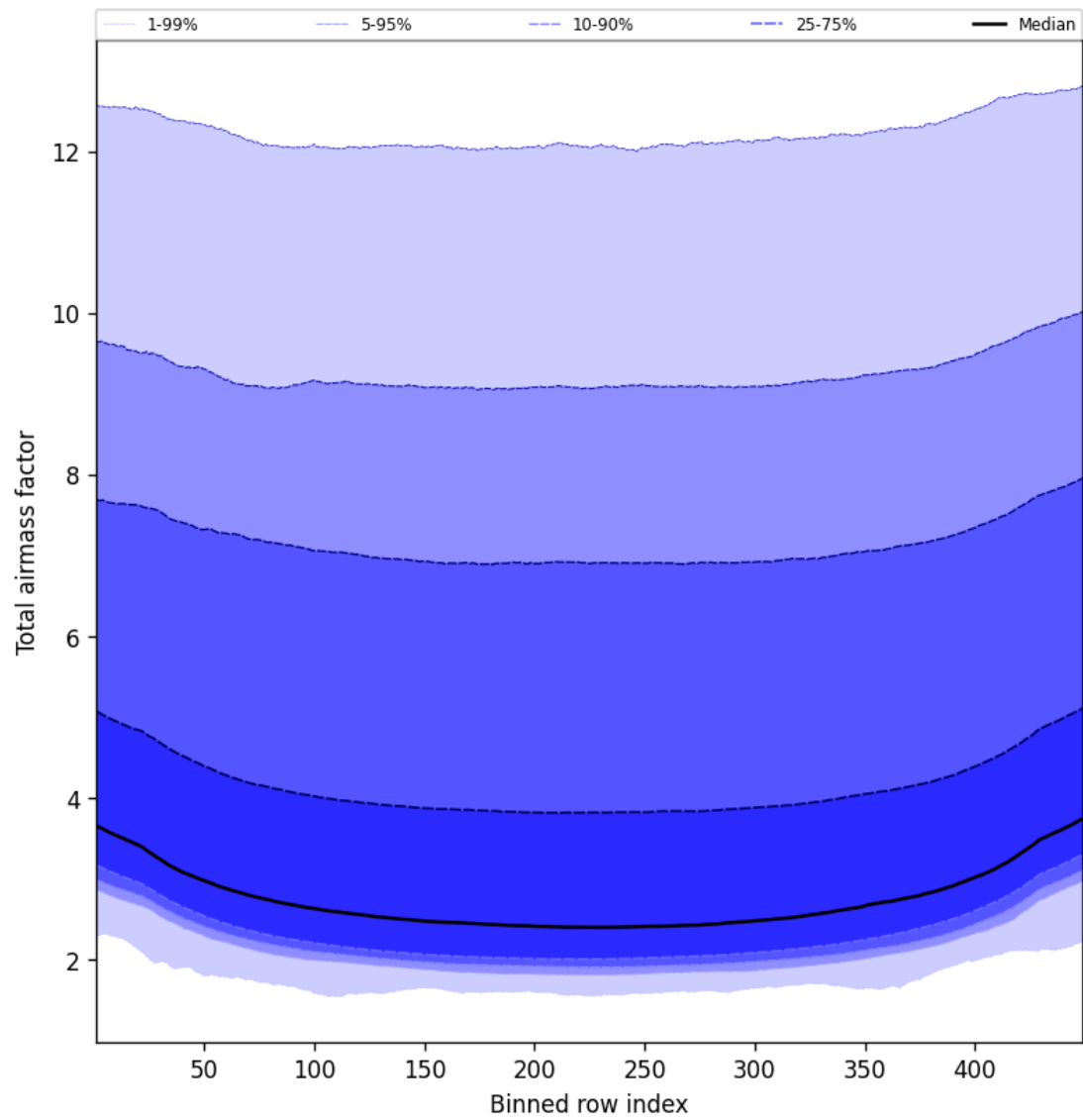
Figure 47: Along track statistics of “Total airmass factor” for 2025-04-16 to 2025-04-16
