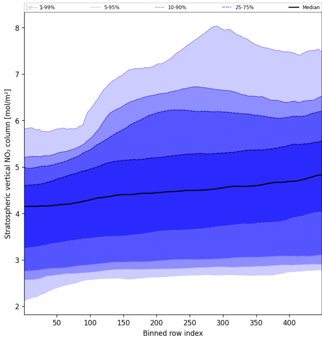
Figure 51: Along track statistics of "Stratospheric vertical NO 2 column" for 2025-04-16 to 2025-04-16
