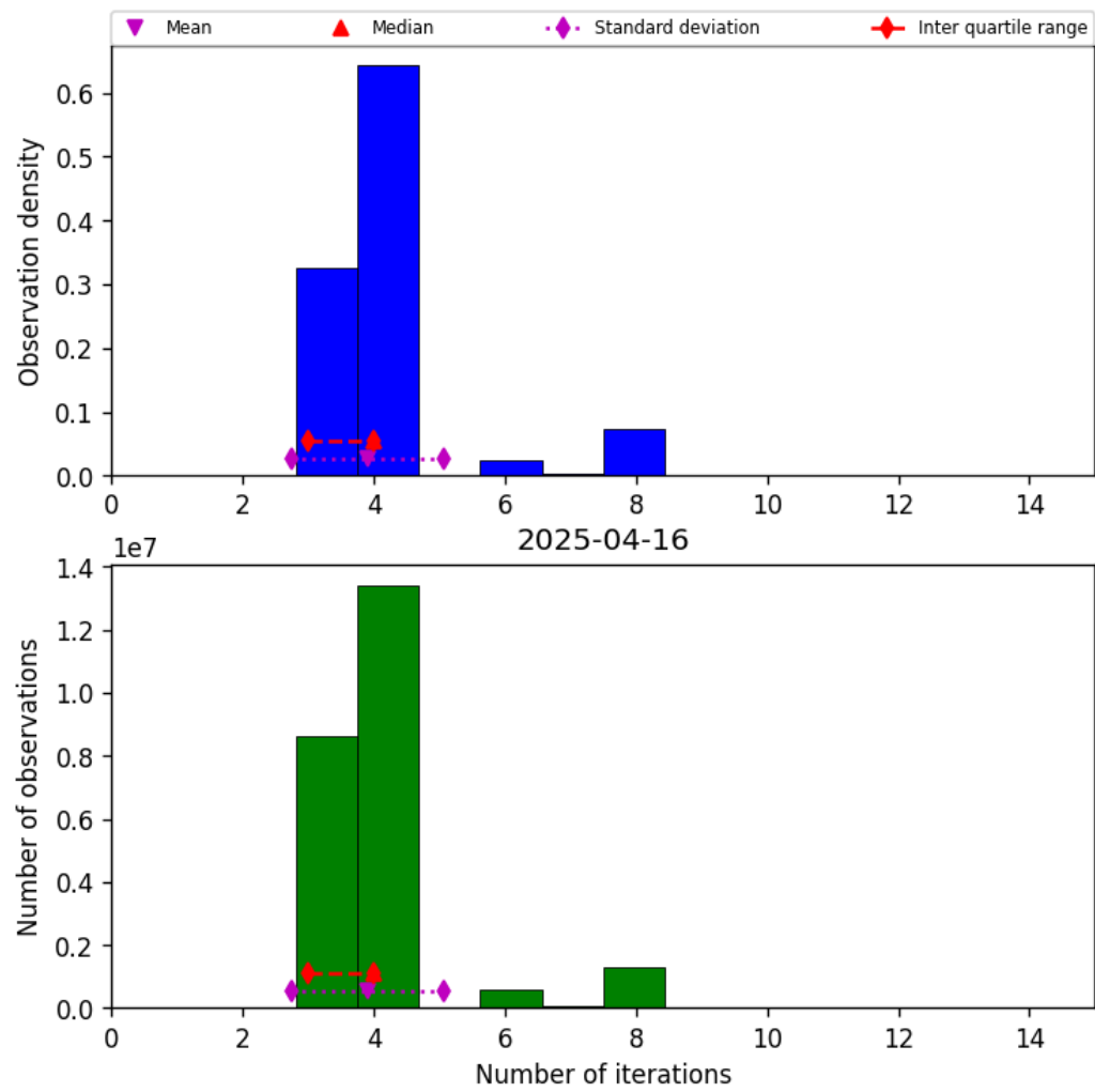
Figure 32: Histogram of “Number of iterations” for 2025-04-16 to 2025-04-16
