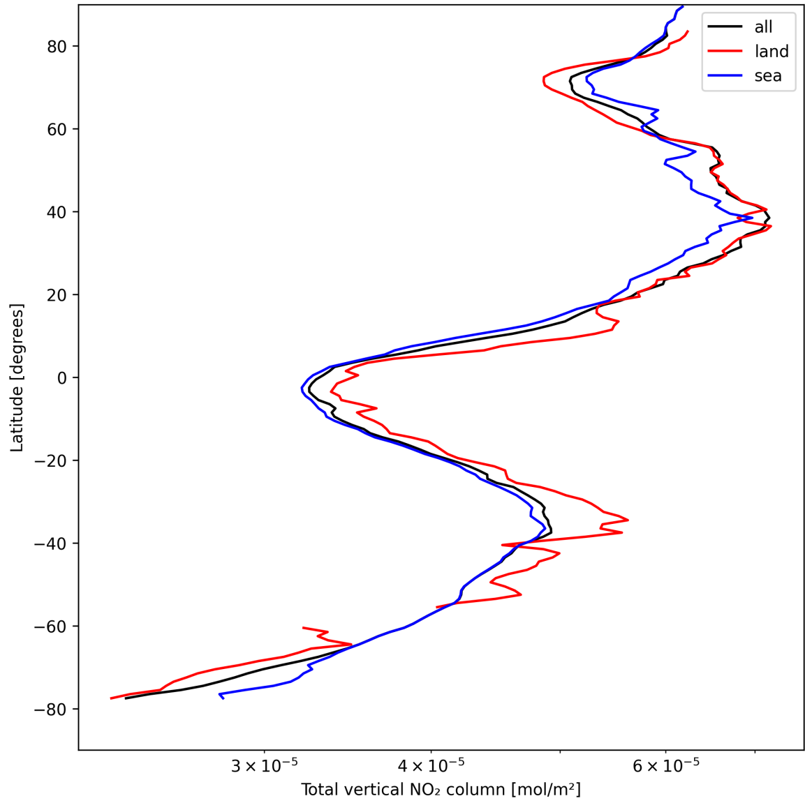
Figure 19: Zonal average of “Total vertical NO 2 column” for 2025-04-16 to 2025-04-16.
