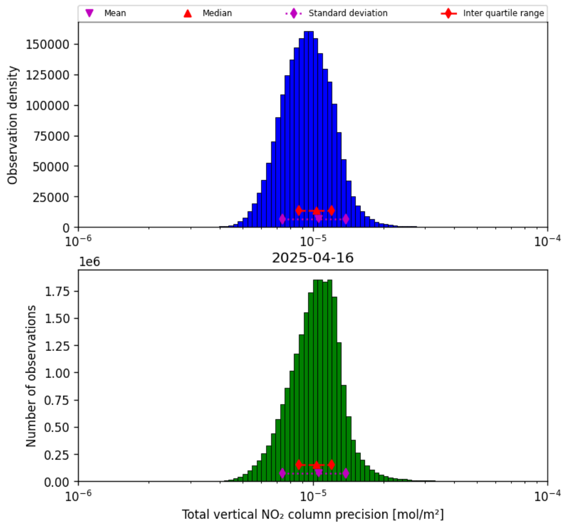
Figure 37: Histogram of “Total vertical NO 2 column precision” for 2025-04-16 to 2025-04-16
