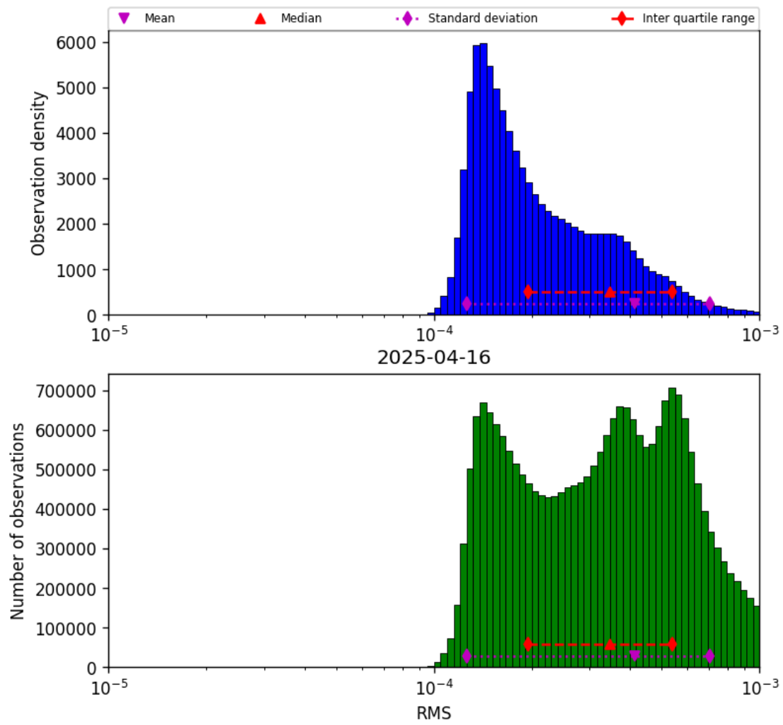
Figure 41: Histogram of “RMS” for 2025-04-16 to 2025-04-16
