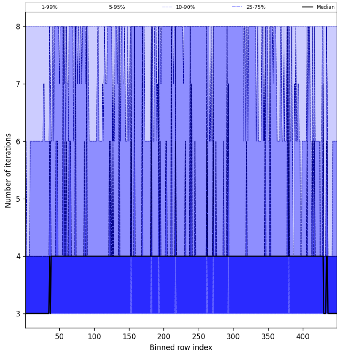
Figure 49: Along track statistics of “Number of iterations” for 2025-04-16 to 2025-04-16
