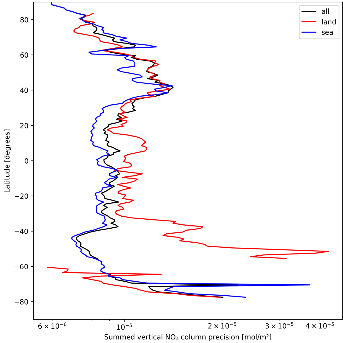
Figure 22: Zonal average of “Summed vertical NO 2 column precision” for 2025-04-16 to 2025-04-16.
