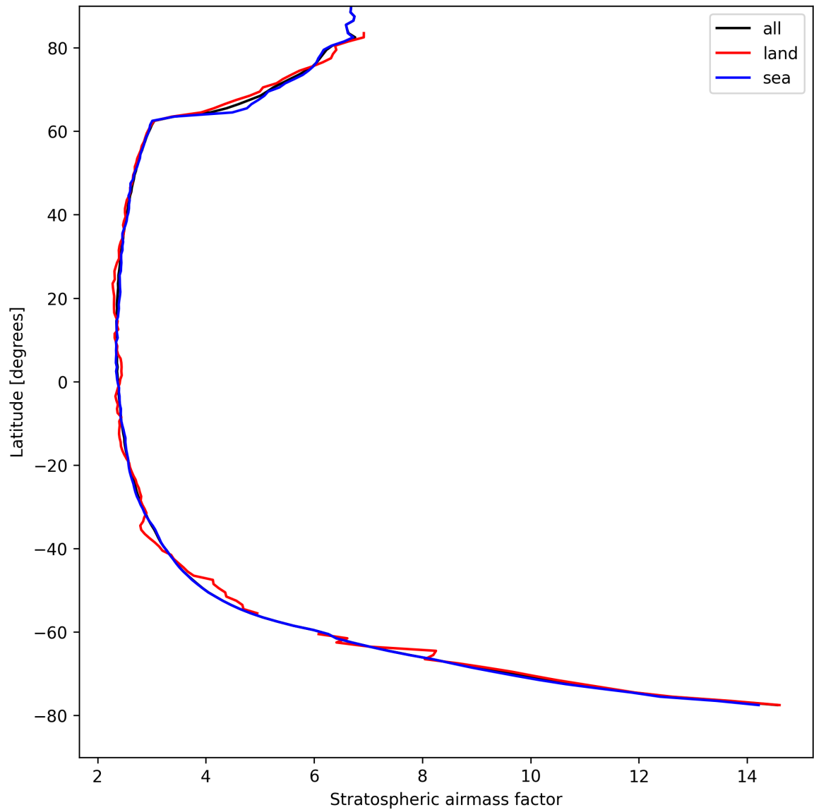
Figure 25: Zonal average of “Stratospheric air mass factor” for 2025-04-16 to 2025-04-16.
