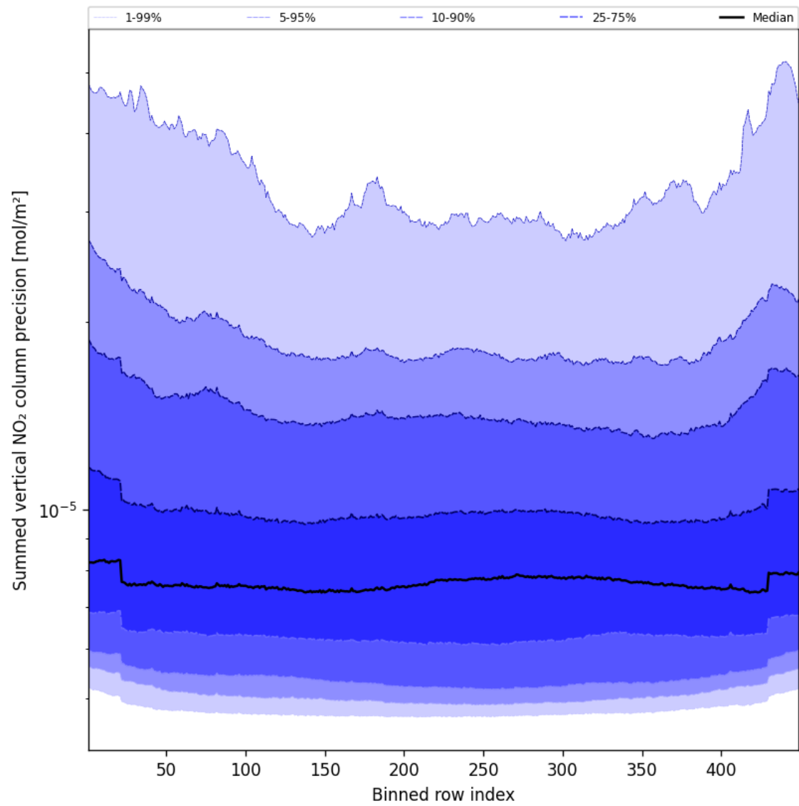
Figure 56: Along track statistics of “Summed vertical NO 2 column precision” for 2025-04-16 to 2025-04-16
