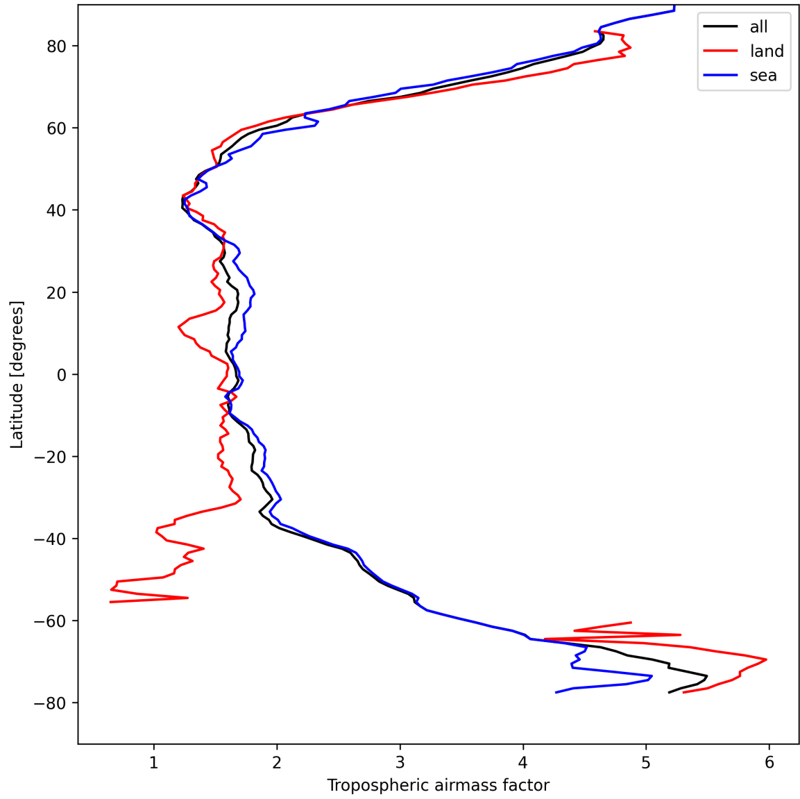
Figure 12: Zonal average of “Tropospheric air mass factor” for 2025-04-16 to 2025-04-16.
