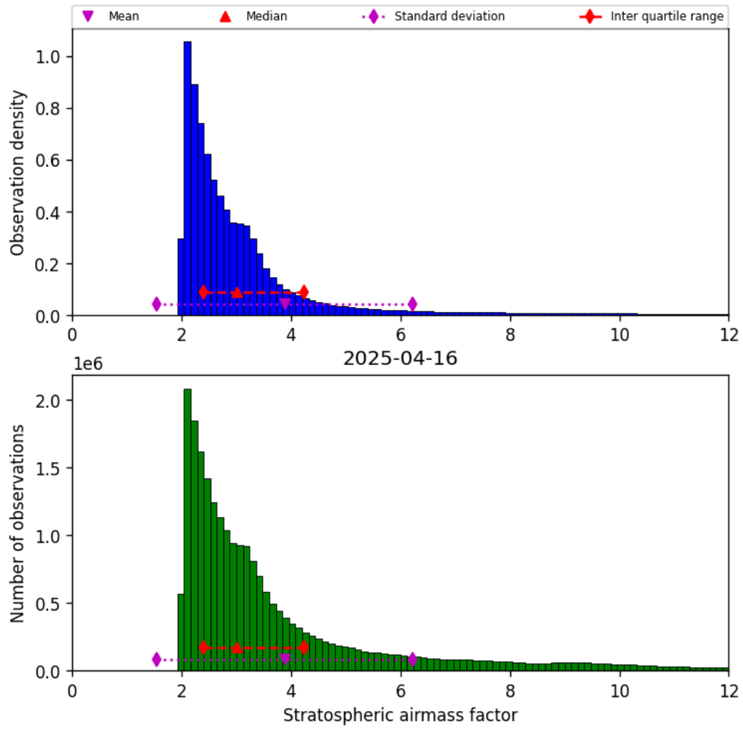
Figure 42: Histogram of “Stratospheric airmass factor” for 2025-04-16 to 2025-04-16
