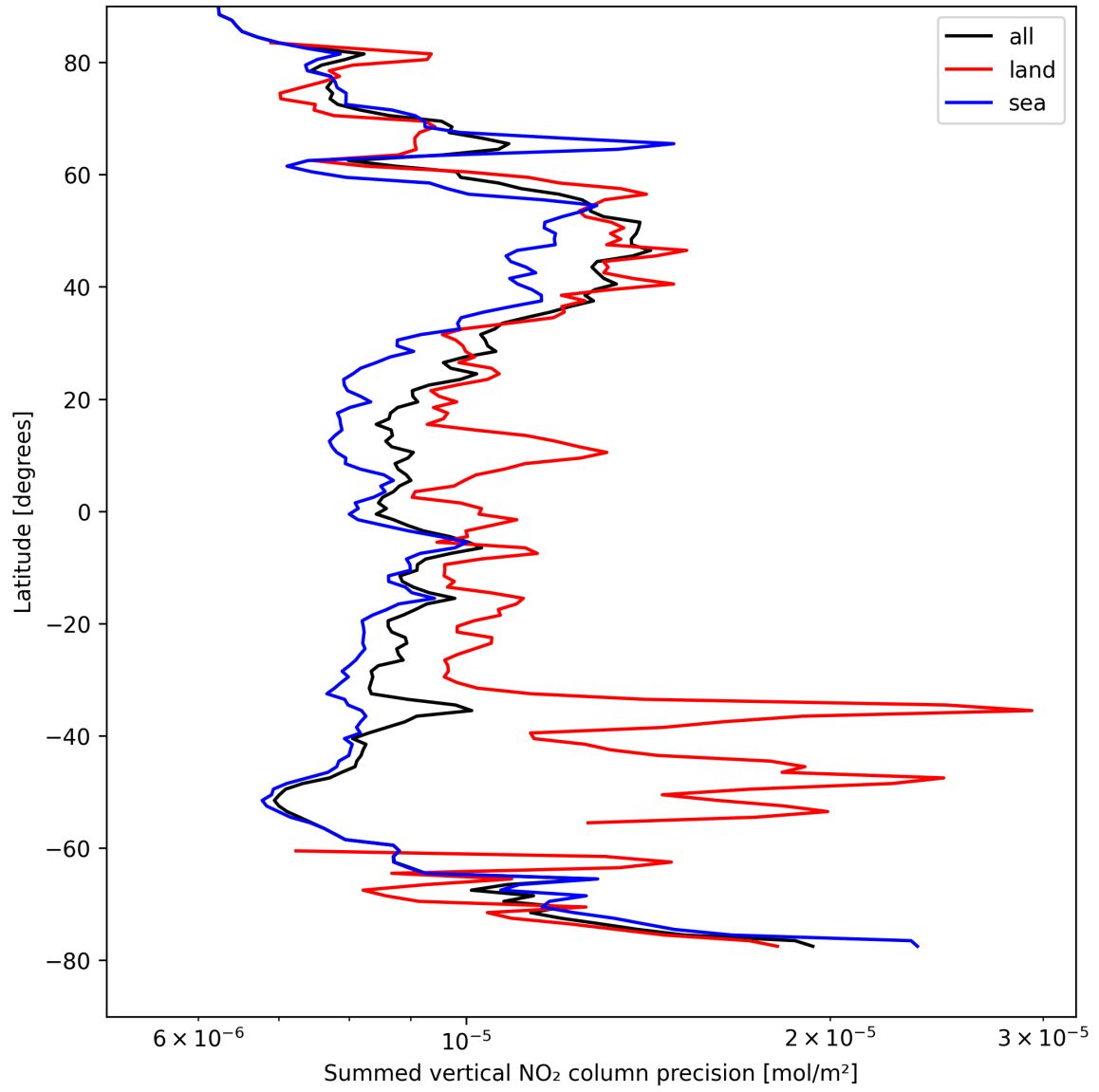
Figure 22: Zonal average of “Summed vertical NO 2 column precision” for 2025-04-17 to 2025-04-18.
