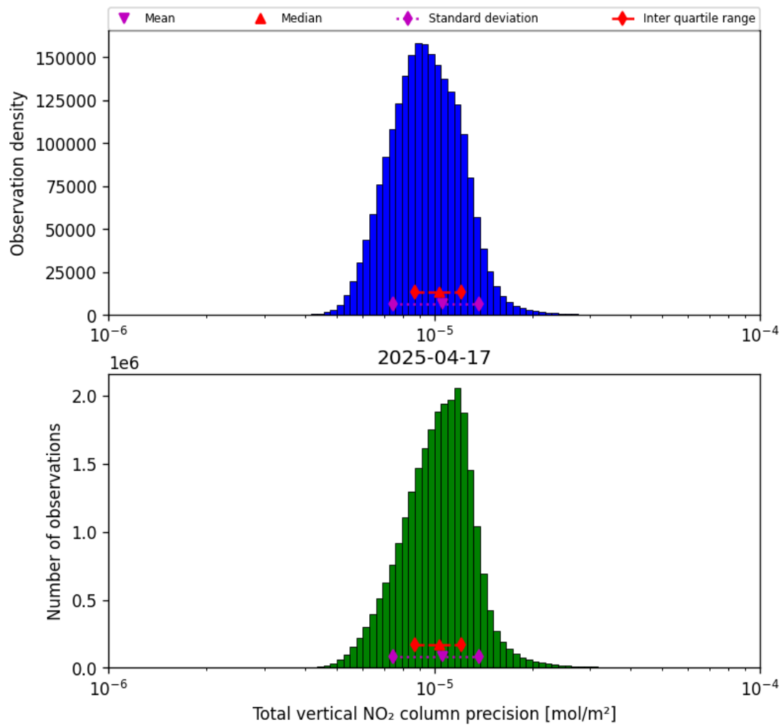
Figure 37: Histogram of “Total vertical NO 2 column precision” for 2025-04-17 to 2025-04-18
