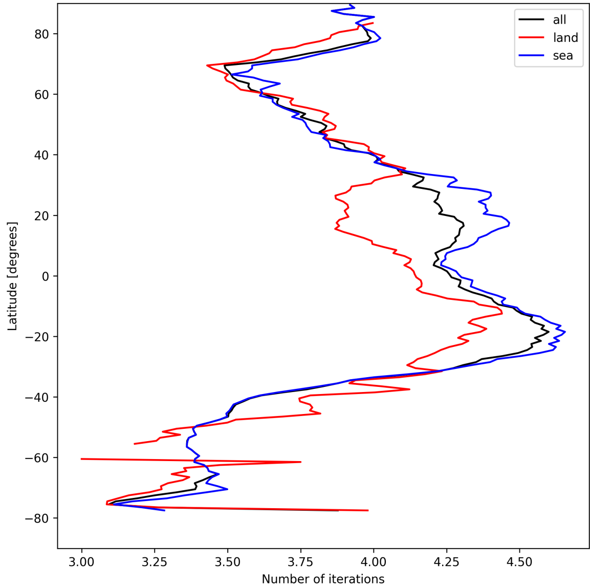
Figure 15: Zonal average of “Number of iterations” for 2025-04-17 to 2025-04-18.
