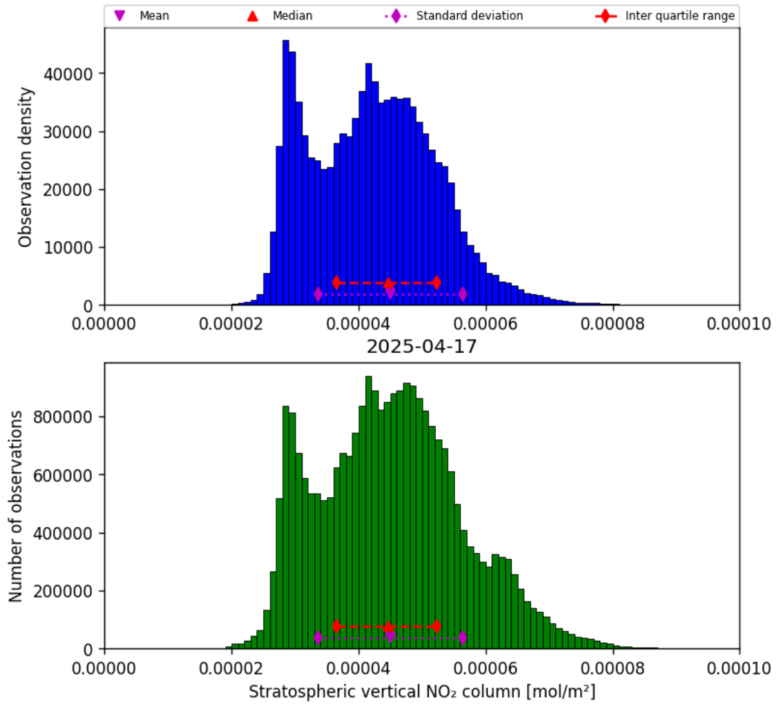
Figure 34: Histogram of “Stratospheric vertical NO 2 column” for 2025-04-17 to 2025-04-18
