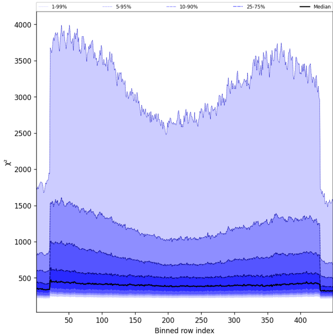
Figure 57: Along track statistics of “ \chi^2 ” for 2025-04-17 to 2025-04-18
