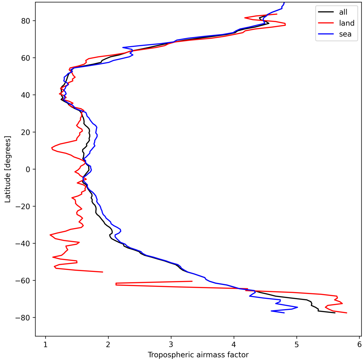
Figure 12: Zonal average of “Tropospheric airmass factor” for 2025-04-17 to 2025-04-18.
