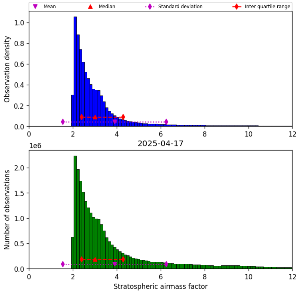
Figure 42: Histogram of “Stratospheric airmass factor” for 2025-04-17 to 2025-04-18
