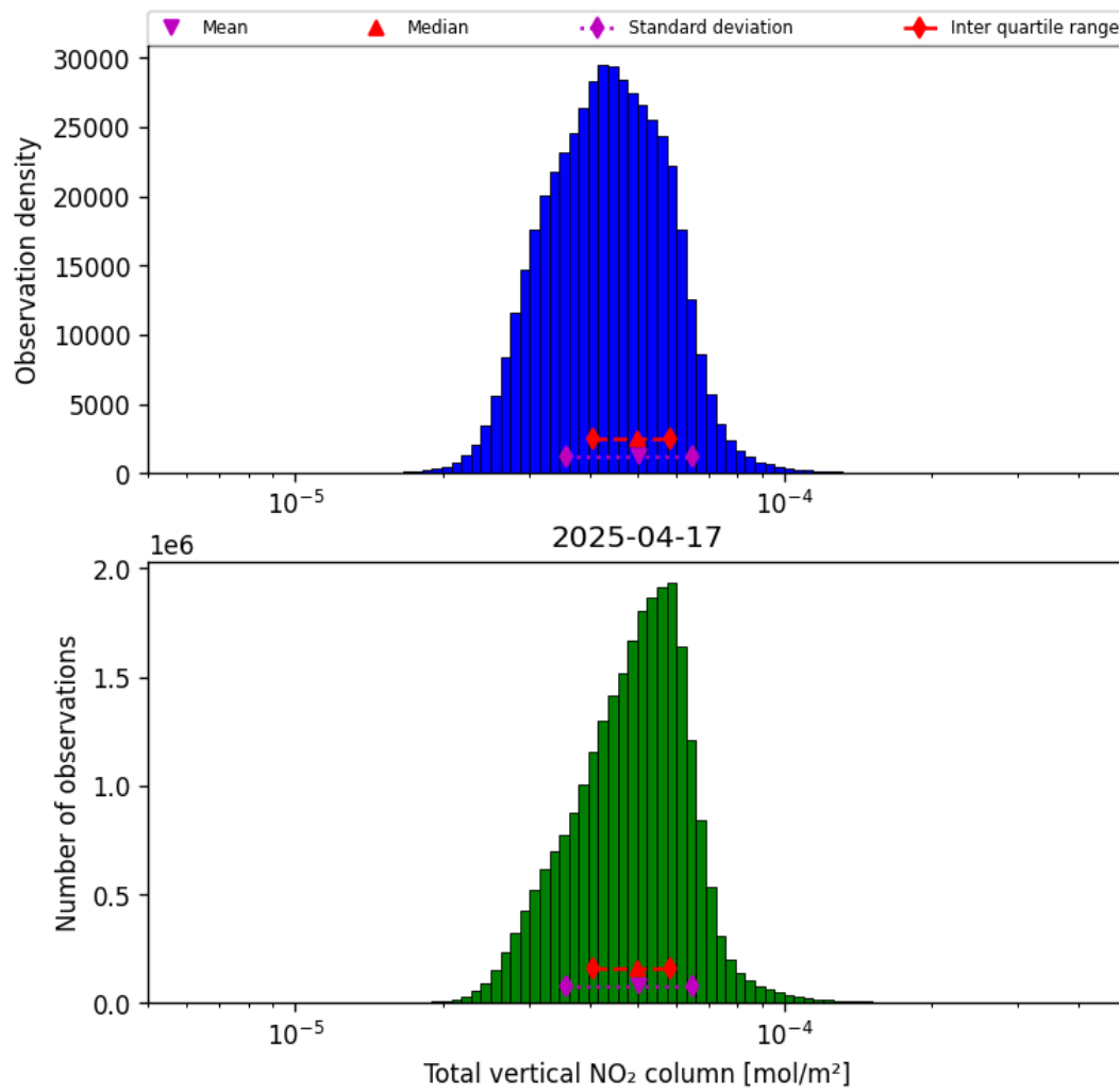
Figure 36: Histogram of "Total vertical NO 2 column" for 2025-04-17 to 2025-04-18
