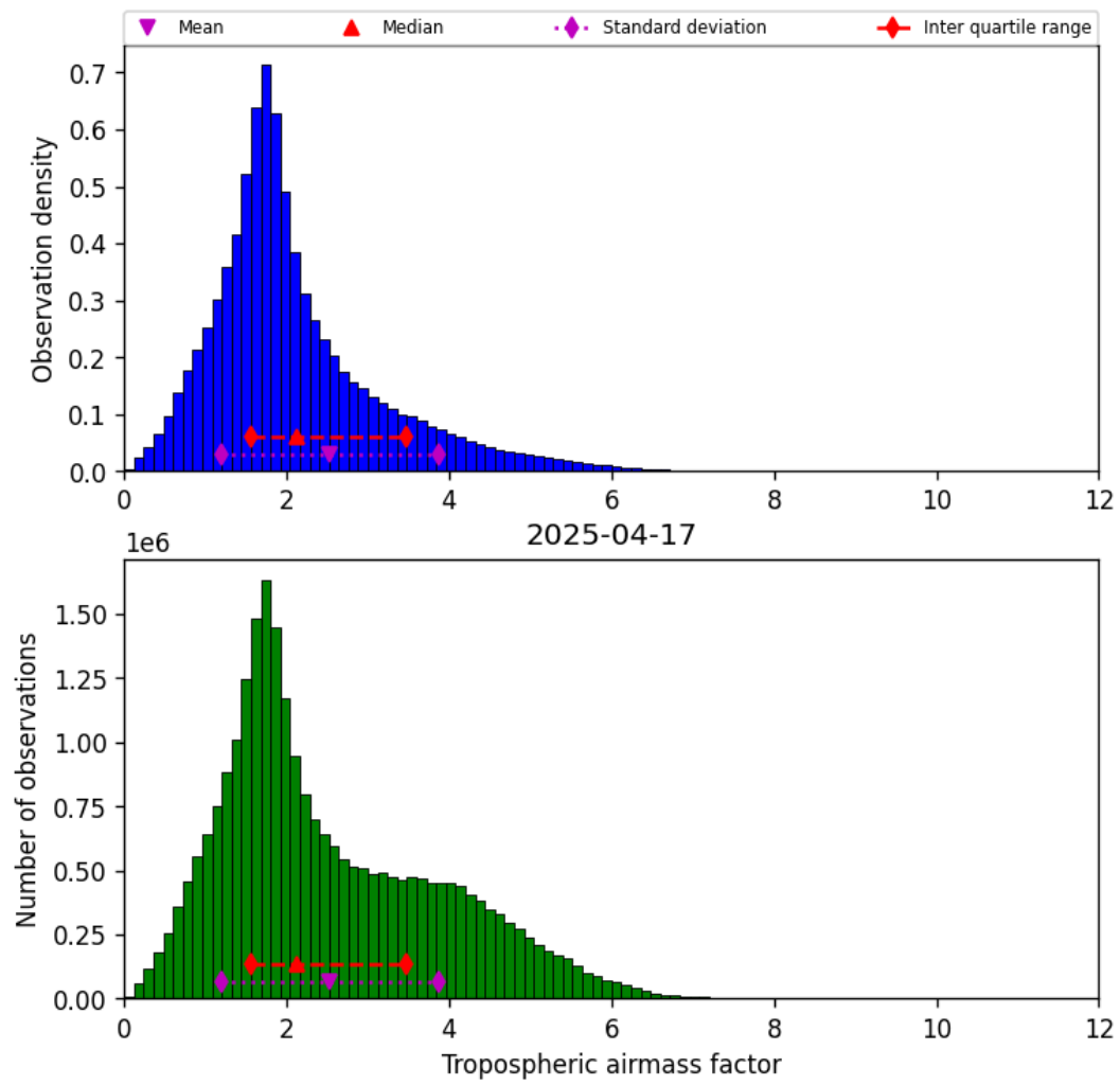
Figure 29: Histogram of “Tropospheric airmass factor” for 2025-04-17 to 2025-04-18
