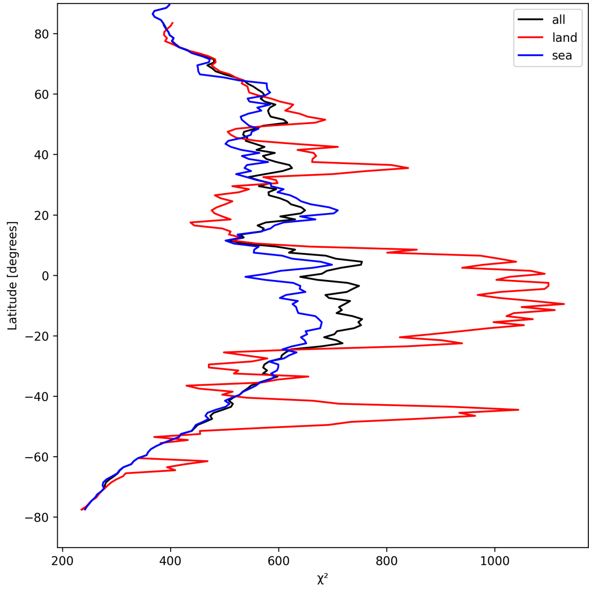
Figure 23: Zonal average of “ \chi^2 ” for 2025-04-17 to 2025-04-18.
