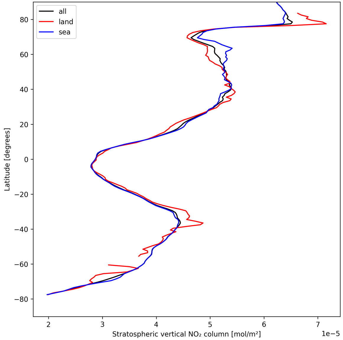
Figure 17: Zonal average of “Stratospheric vertical NO 2 column” for 2025-04-17 to 2025-04-18.
