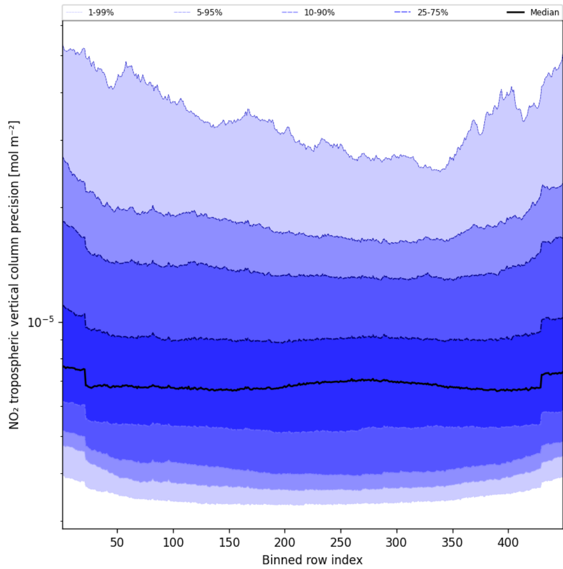
Figure 45: Along track statistics of “NO 2 tropospheric vertical column precision” for 2025-04-17 to 2025-04-18
