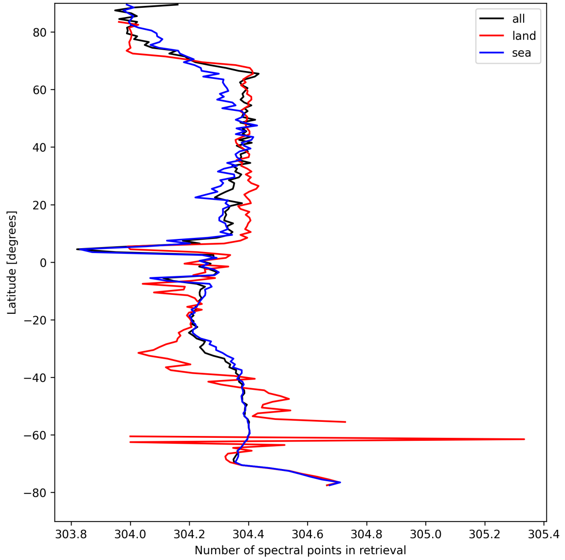
Figure 14: Zonal average of “Number of spectral points in retrieval” for 2025-04-17 to 2025-04-18.
