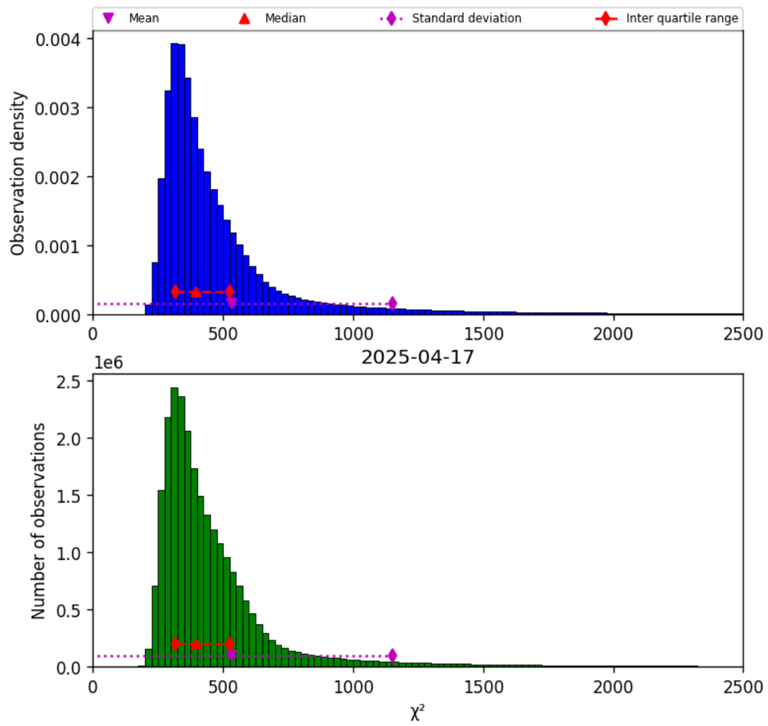
Figure 40: Histogram of “ \chi^2 ” for 2025-04-17 to 2025-04-18
