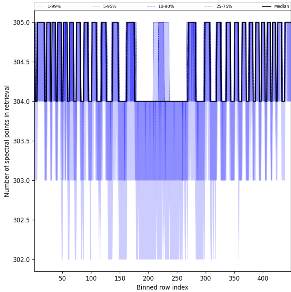
Figure 48: Along track statistics of “Number of spectral points in retrieval” for 2025-04-17 to 2025-04-18
