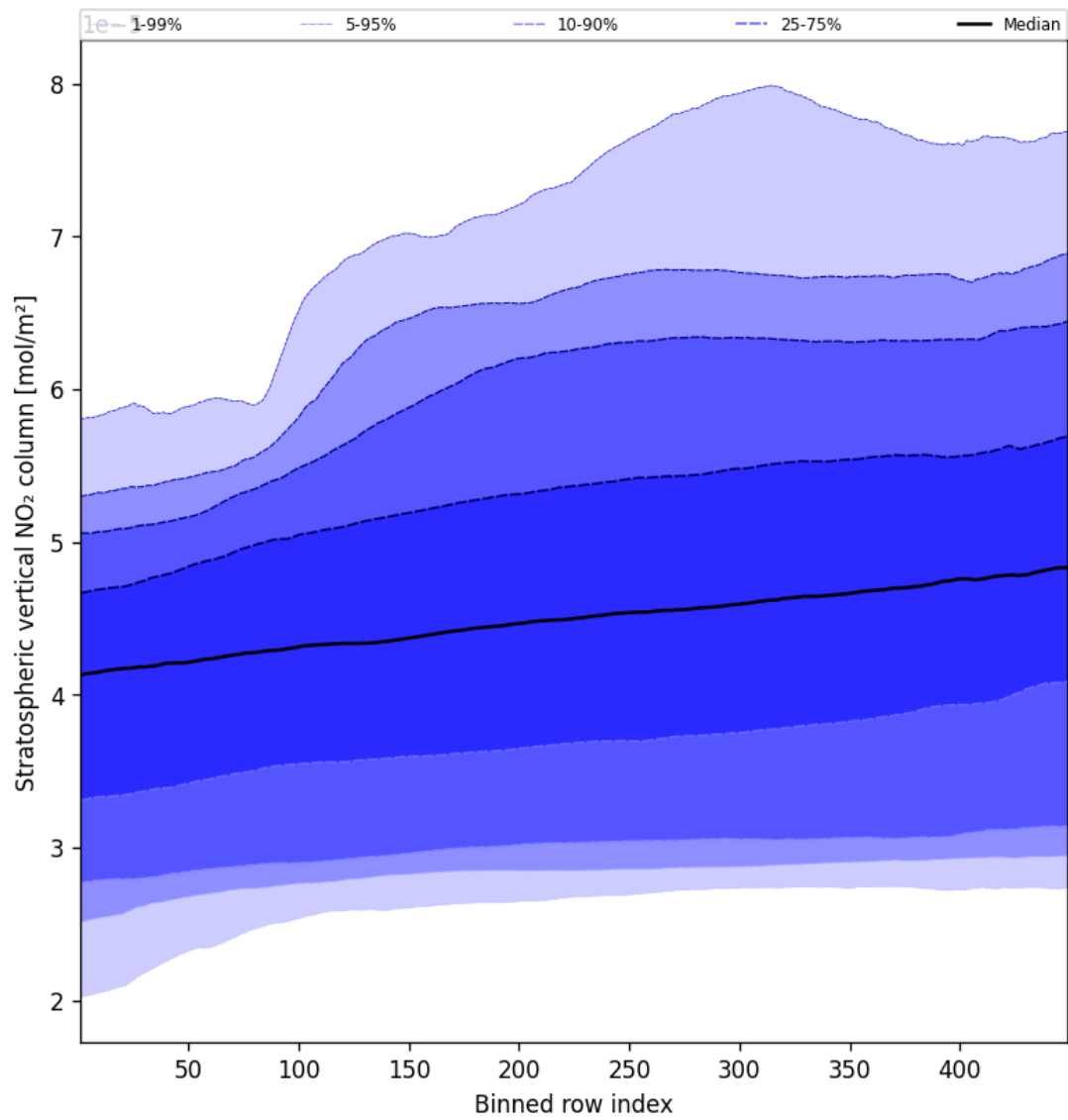
Figure 51: Along track statistics of “Stratospheric vertical NO 2 column” for 2025-04-17 to 2025-04-18
