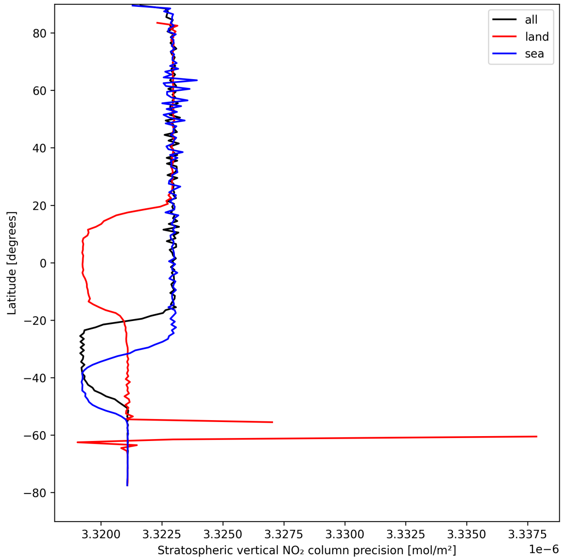
Figure 18: Zonal average of “Stratospheric vertical NO 2 column precision” for 2025-04-17 to 2025-04-18.
