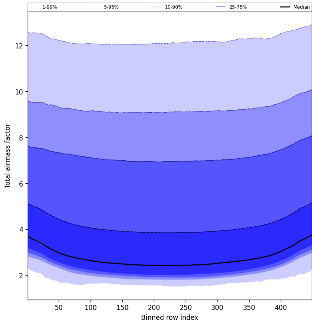
Figure 47: Along track statistics of “Total airmass factor” for 2025-04-17 to 2025-04-18
