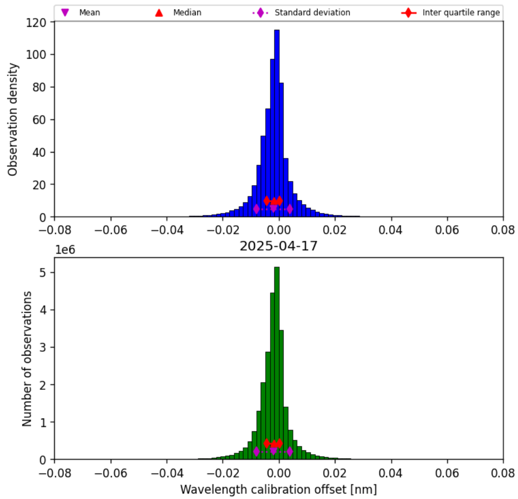
Figure 33: Histogram of “Wavelength calibration offset” for 2025-04-17 to 2025-04-18
