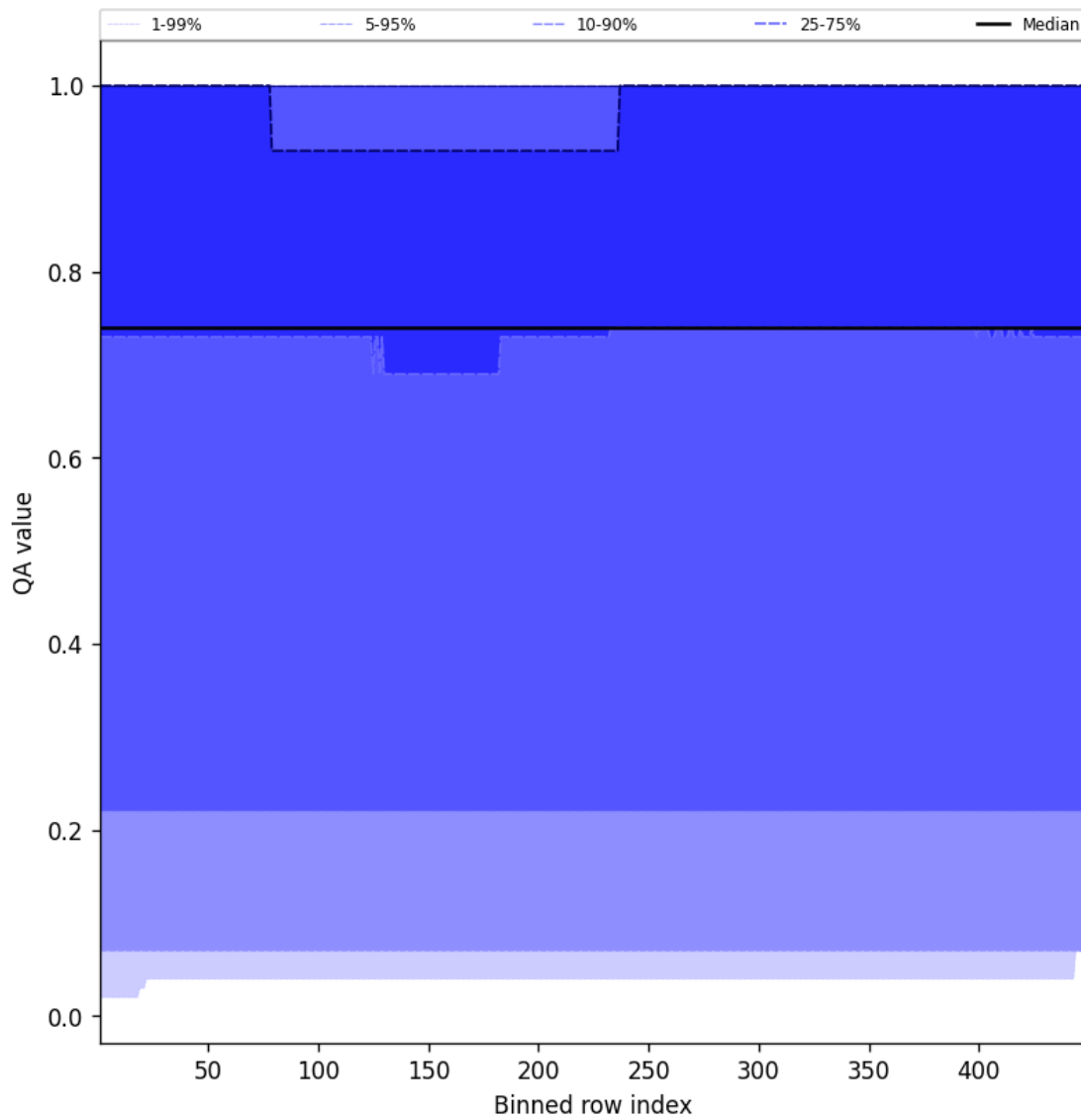
Figure 43: Along track statistics of “QA value” for 2025-04-17 to 2025-04-18
