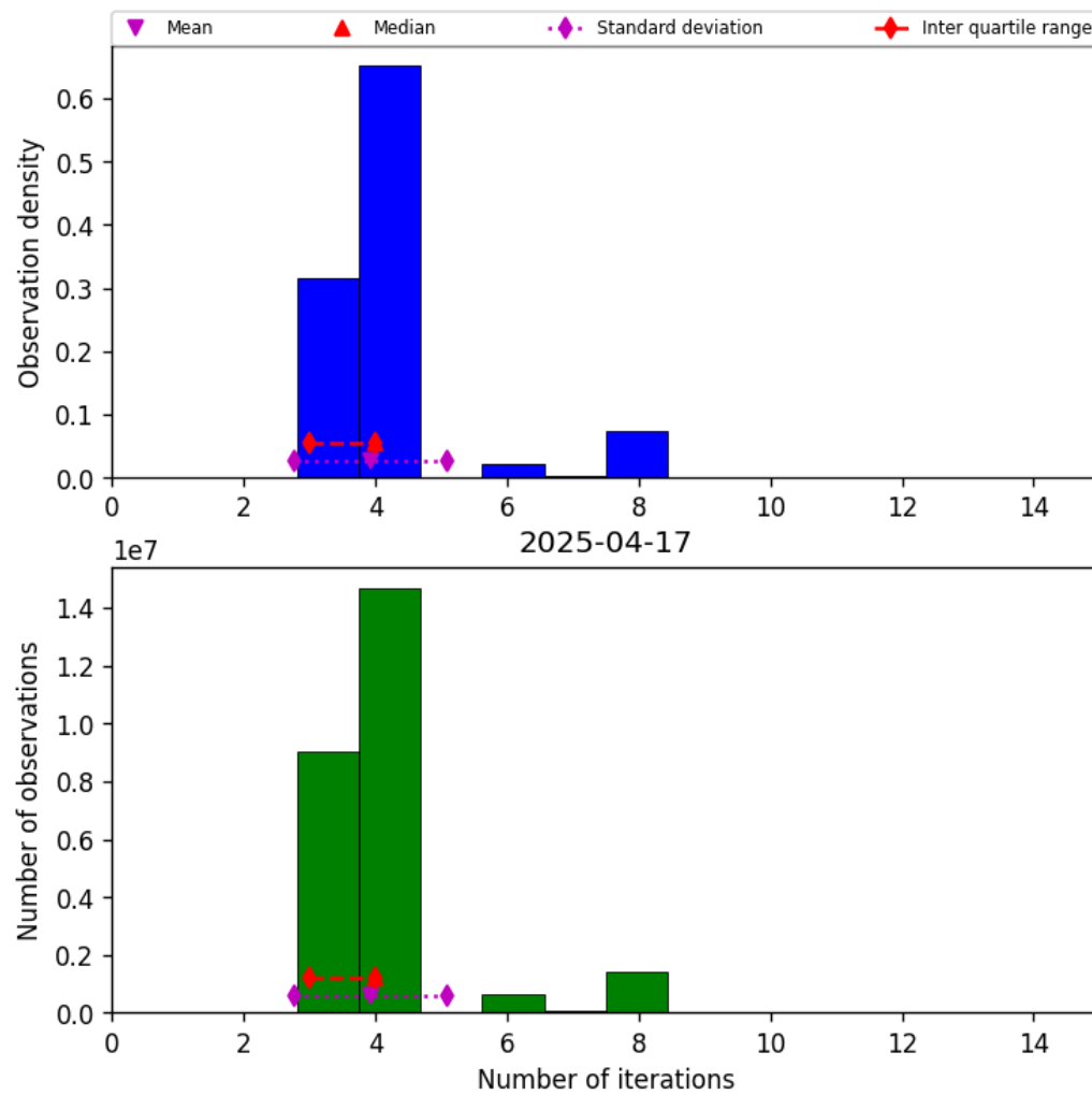
Figure 32: Histogram of “Number of iterations” for 2025-04-17 to 2025-04-18
