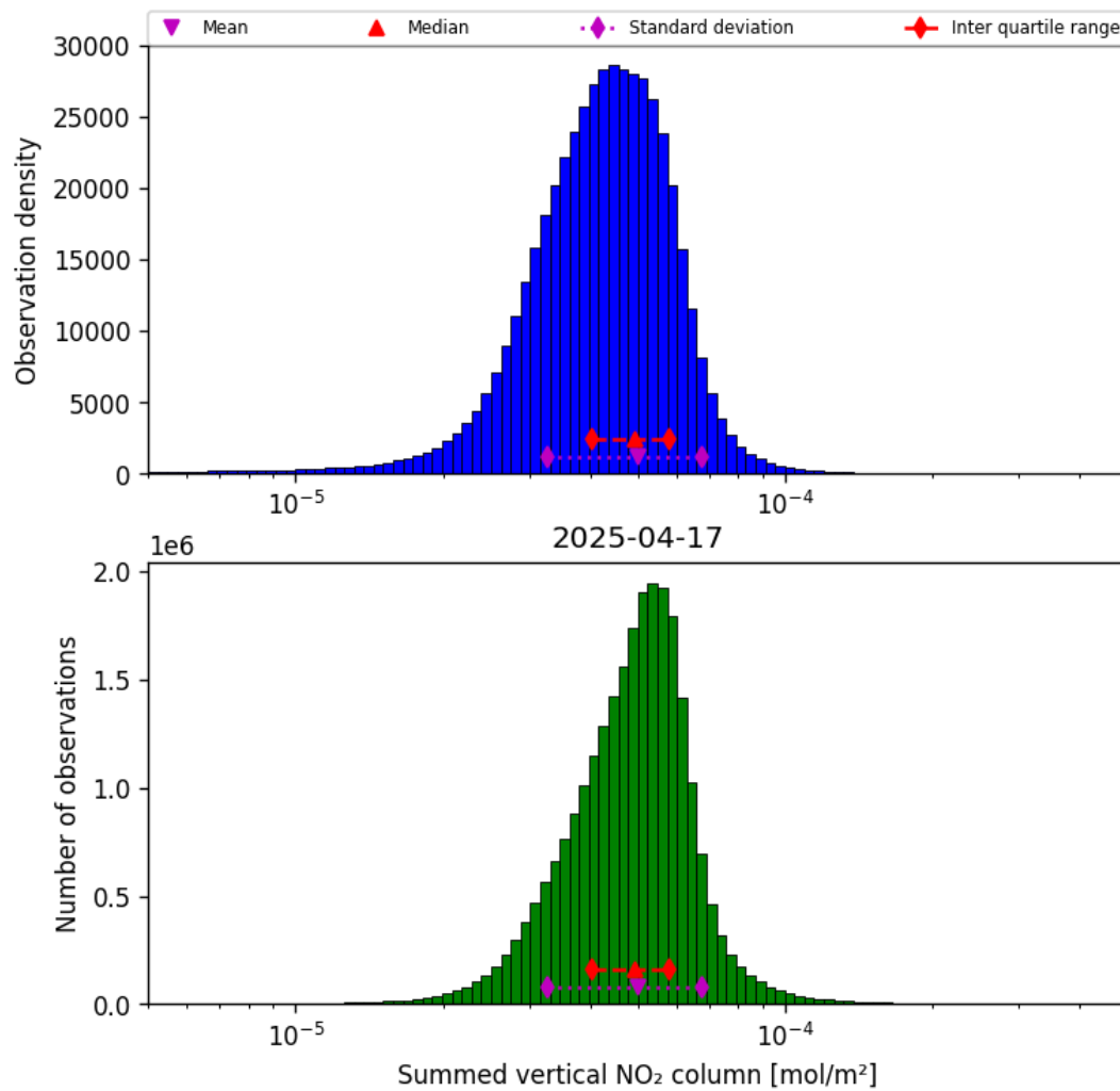
Figure 38: Histogram of “Summed vertical NO 2 column” for 2025-04-17 to 2025-04-18
