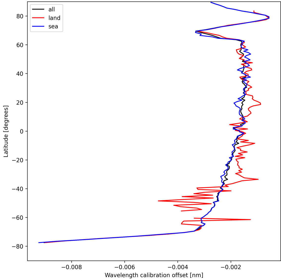
Figure 16: Zonal average of “Wavelength calibration offset” for 2025-04-17 to 2025-04-18.
