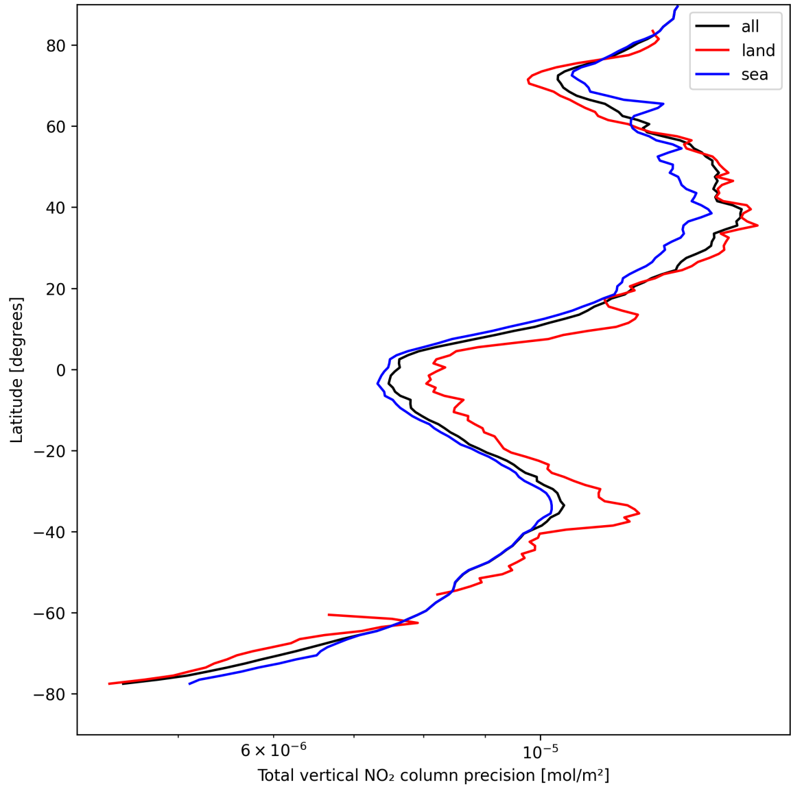
Figure 20: Zonal average of “Total vertical NO 2 column precision” for 2025-04-17 to 2025-04-18.
