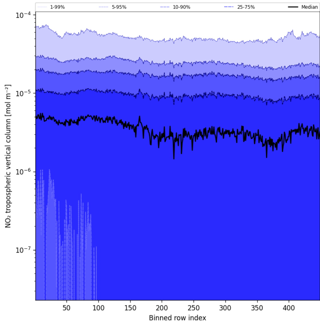
Figure 44: Along track statistics of “NO 2 tropospheric vertical column” for 2025-04-17 to 2025-04-18
