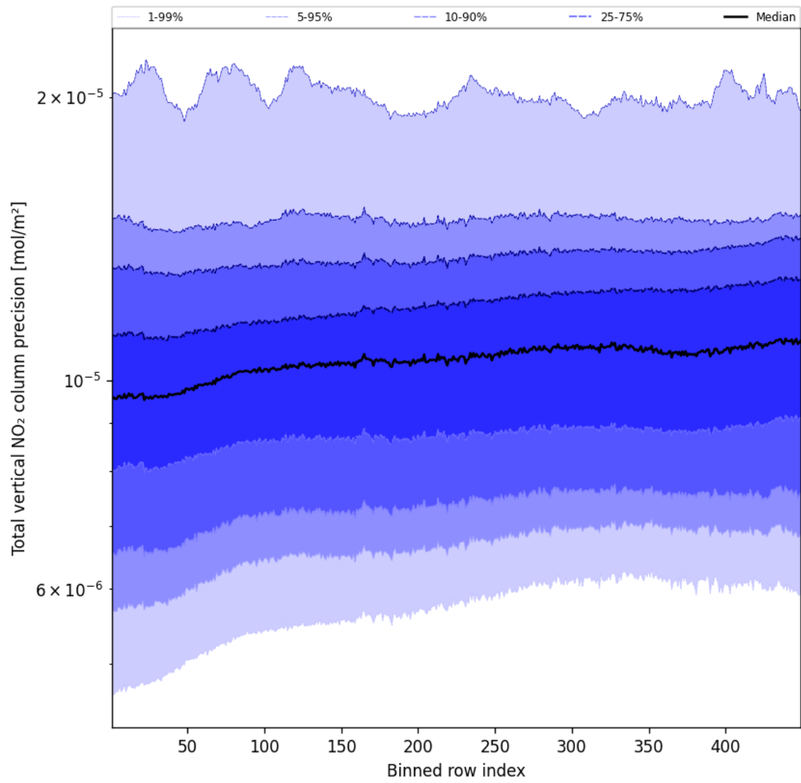
Figure 54: Along track statistics of "Total vertical NO 2 column precision" for 2025-04-17 to 2025-04-18
