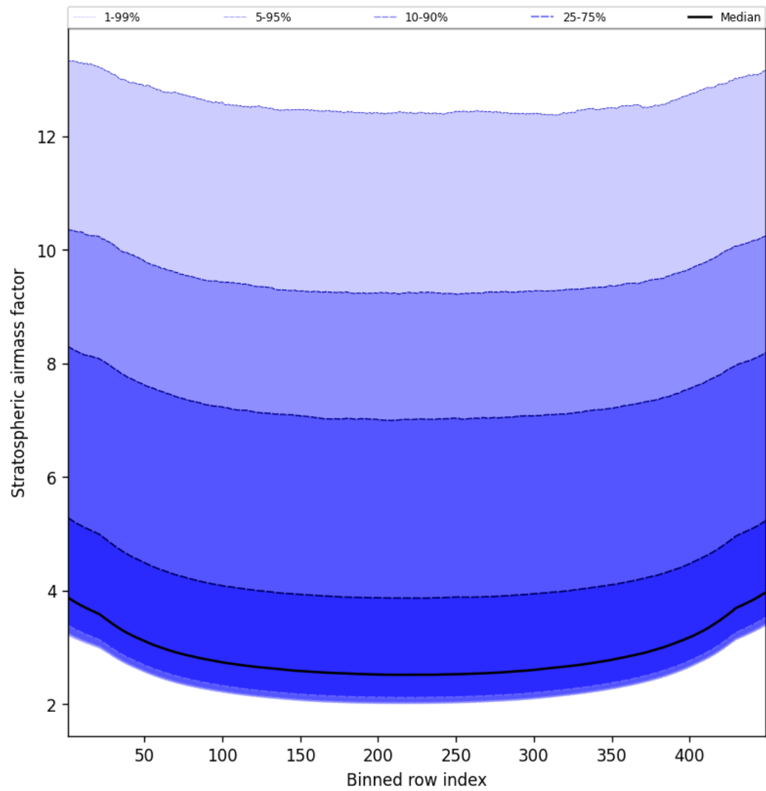
Figure 59: Along track statistics of “Stratospheric airmass factor” for 2025-04-17 to 2025-04-18
