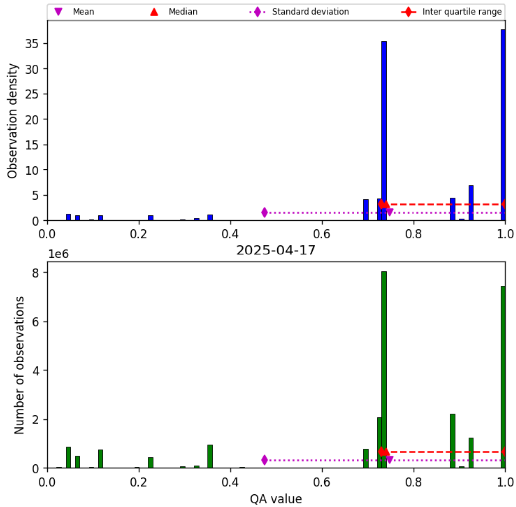
Figure 26: Histogram of “QA value” for 2025-04-17 to 2025-04-18
