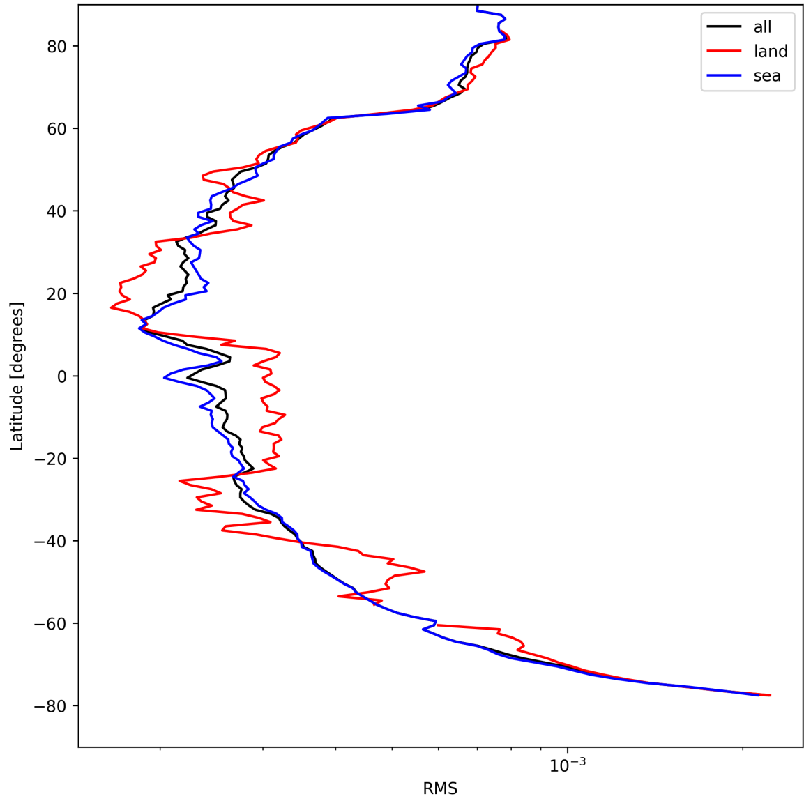
Figure 24: Zonal average of “RMS” for 2025-04-17 to 2025-04-18.
