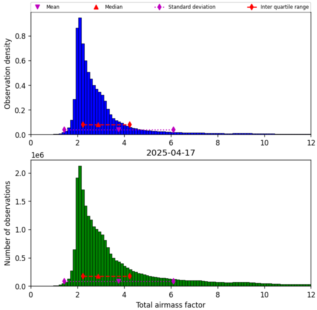
Figure 30: Histogram of “Total airmass factor” for 2025-04-17 to 2025-04-18
