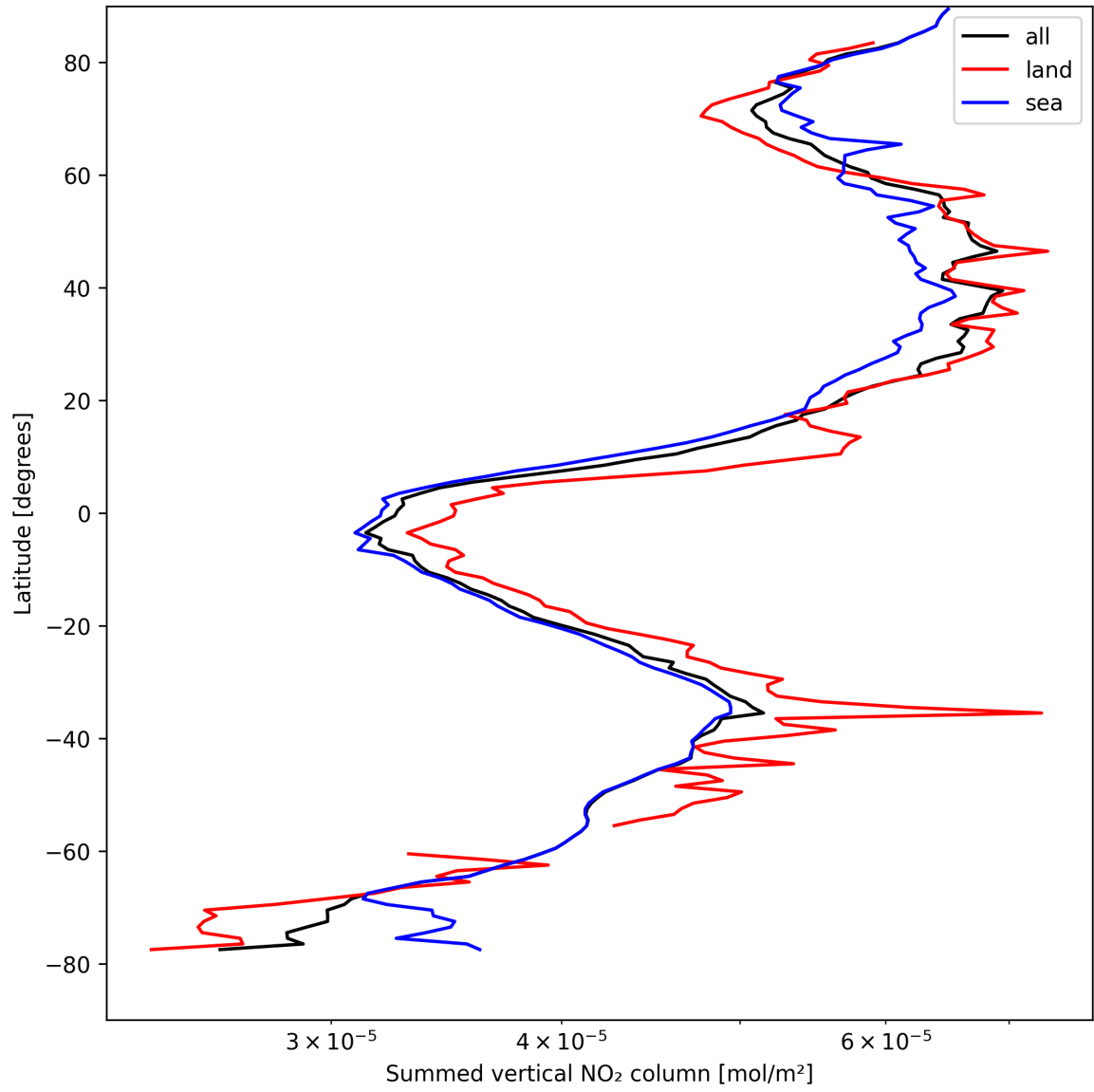
Figure 21: Zonal average of “Summed vertical NO 2 column” for 2025-04-17 to 2025-04-18.
