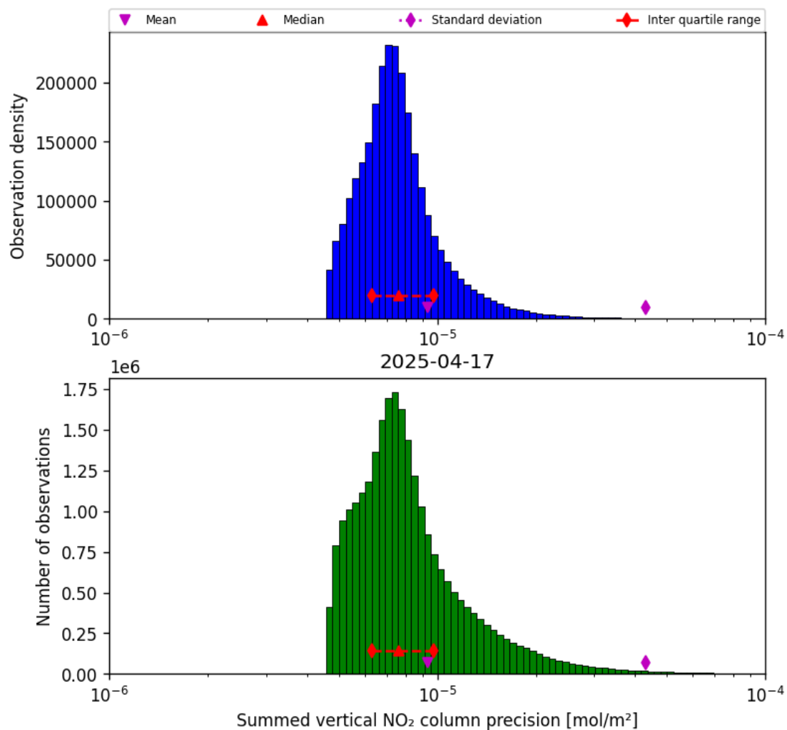
Figure 39: Histogram of “Summed vertical NO 2 column precision” for 2025-04-17 to 2025-04-18
