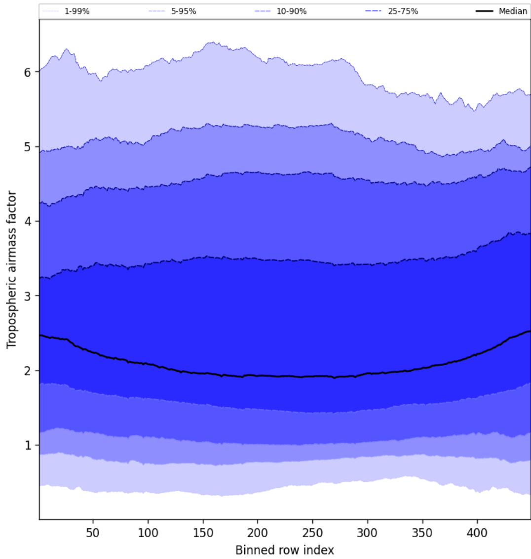
Figure 46: Along track statistics of “Tropospheric air mass factor” for 2025-04-17 to 2025-04-18
