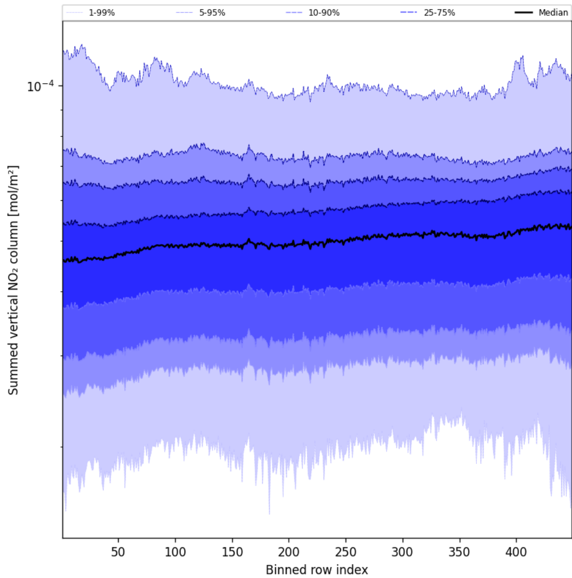
Figure 55: Along track statistics of “Summed vertical NO 2 column” for 2025-04-17 to 2025-04-18
