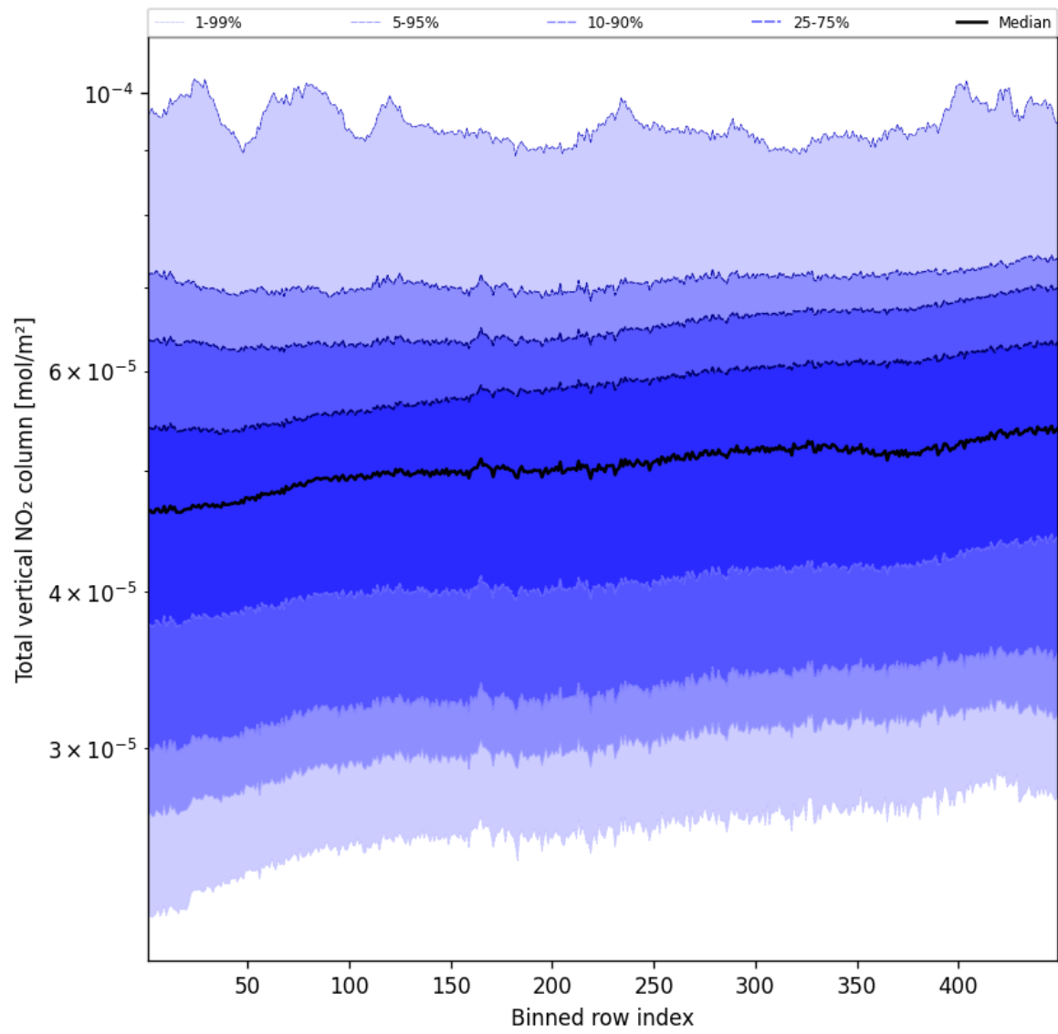
Figure 53: Along track statistics of “Total vertical NO 2 column” for 2025-04-17 to 2025-04-18
