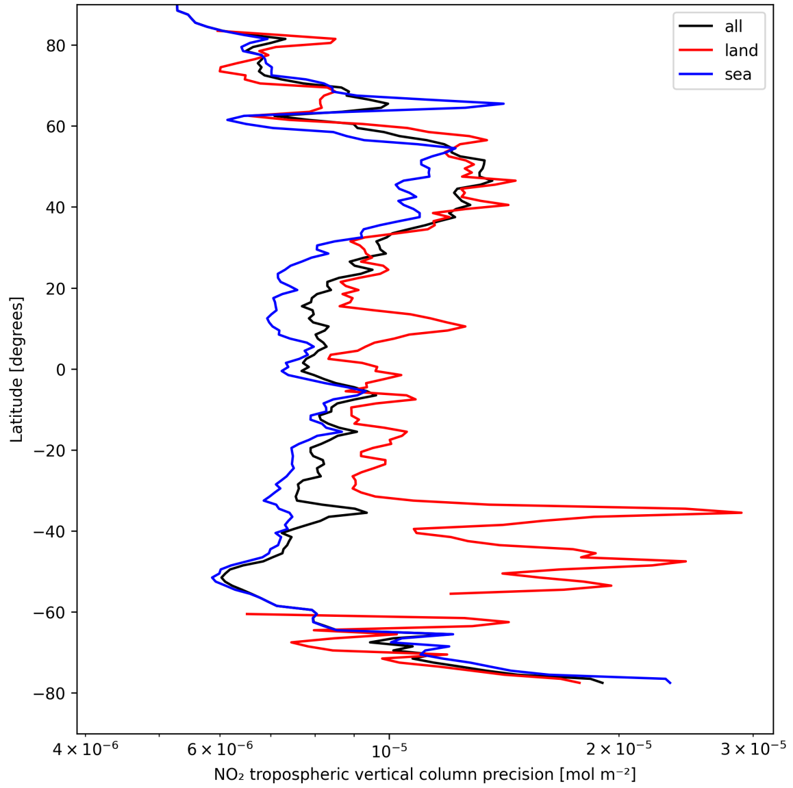
Figure 11: Zonal average of “NO 2 tropospheric vertical column precision” for 2025-04-17 to 2025-04-18.
