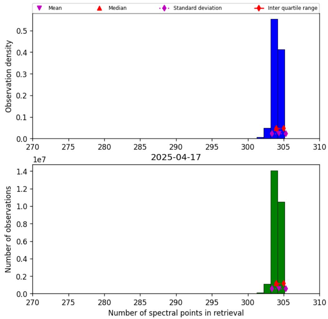
Figure 31: Histogram of “Number of spectral points in retrieval” for 2025-04-17 to 2025-04-18
