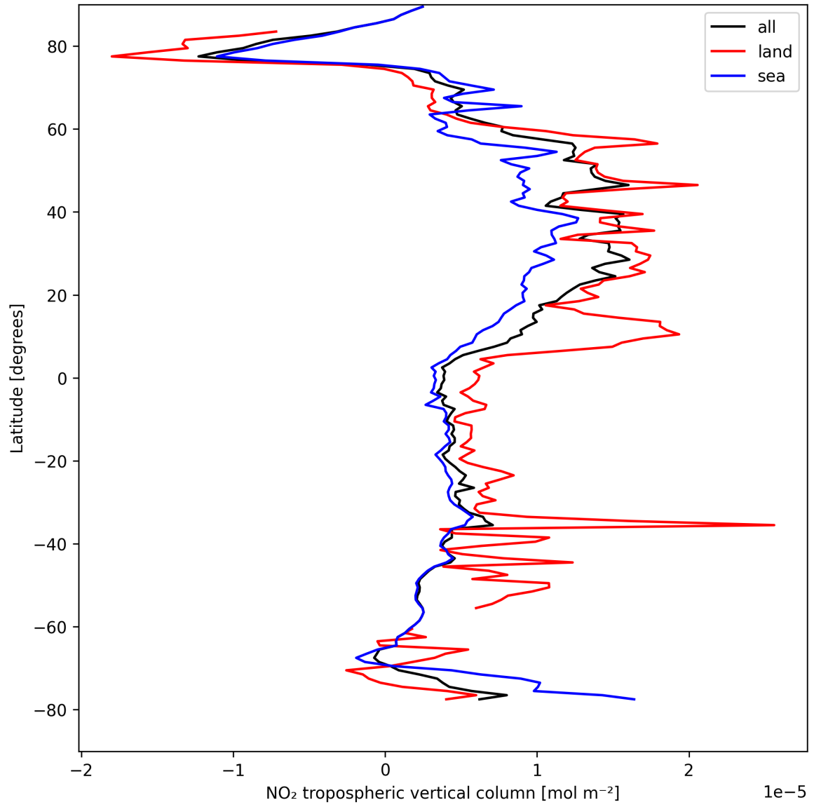
Figure 10: Zonal average of “NO 2 tropospheric vertical column” for 2025-04-17 to 2025-04-18.
