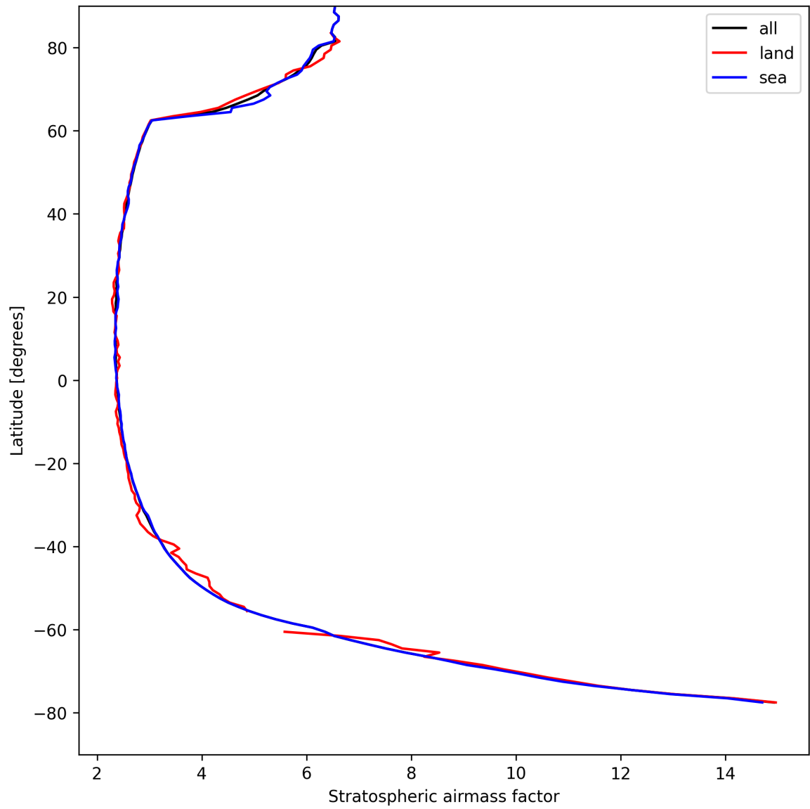
Figure 25: Zonal average of “Stratospheric air mass factor” for 2025-04-17 to 2025-04-18.
