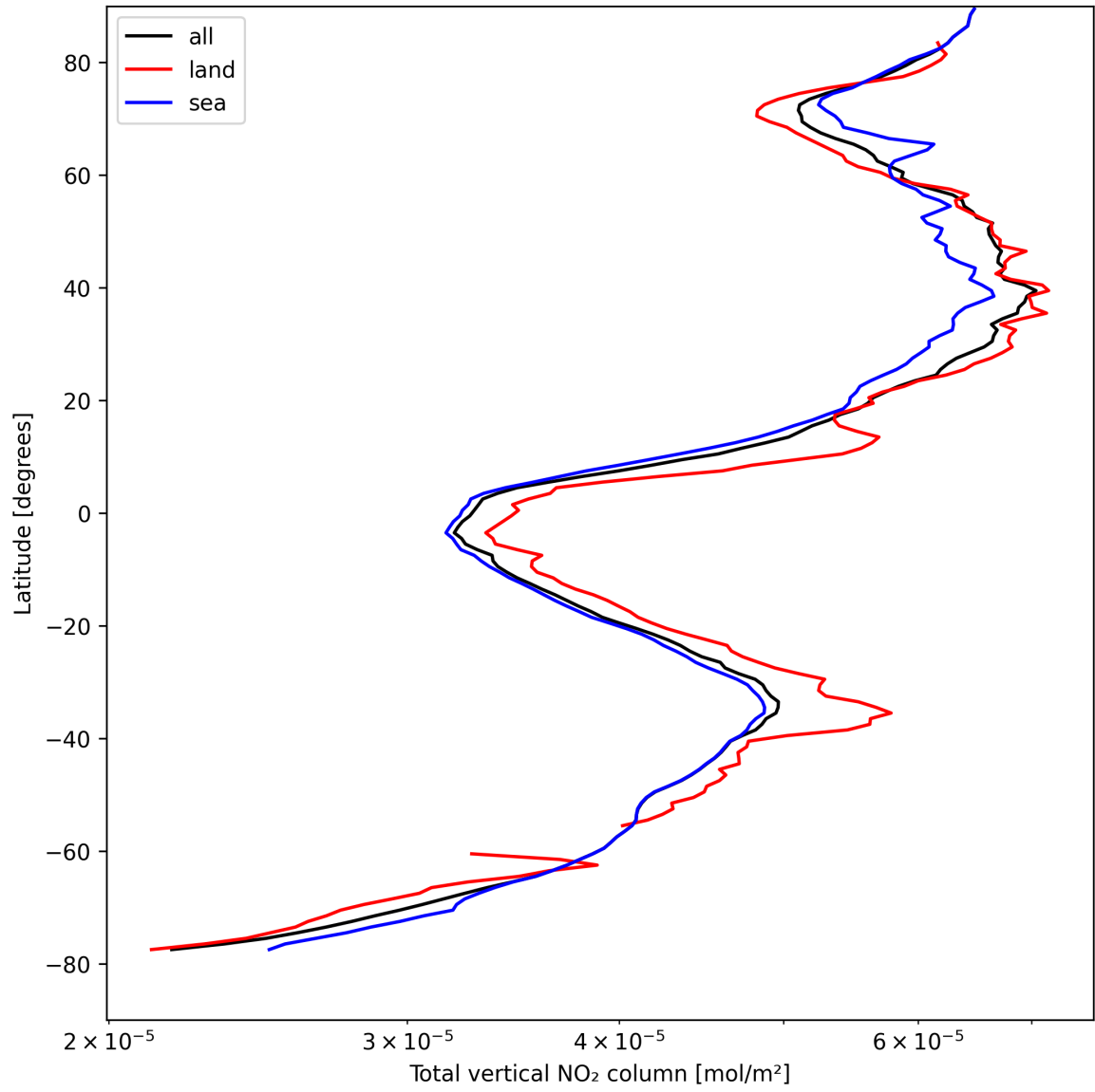
Figure 19: Zonal average of “Total vertical NO 2 column” for 2025-04-17 to 2025-04-18.
