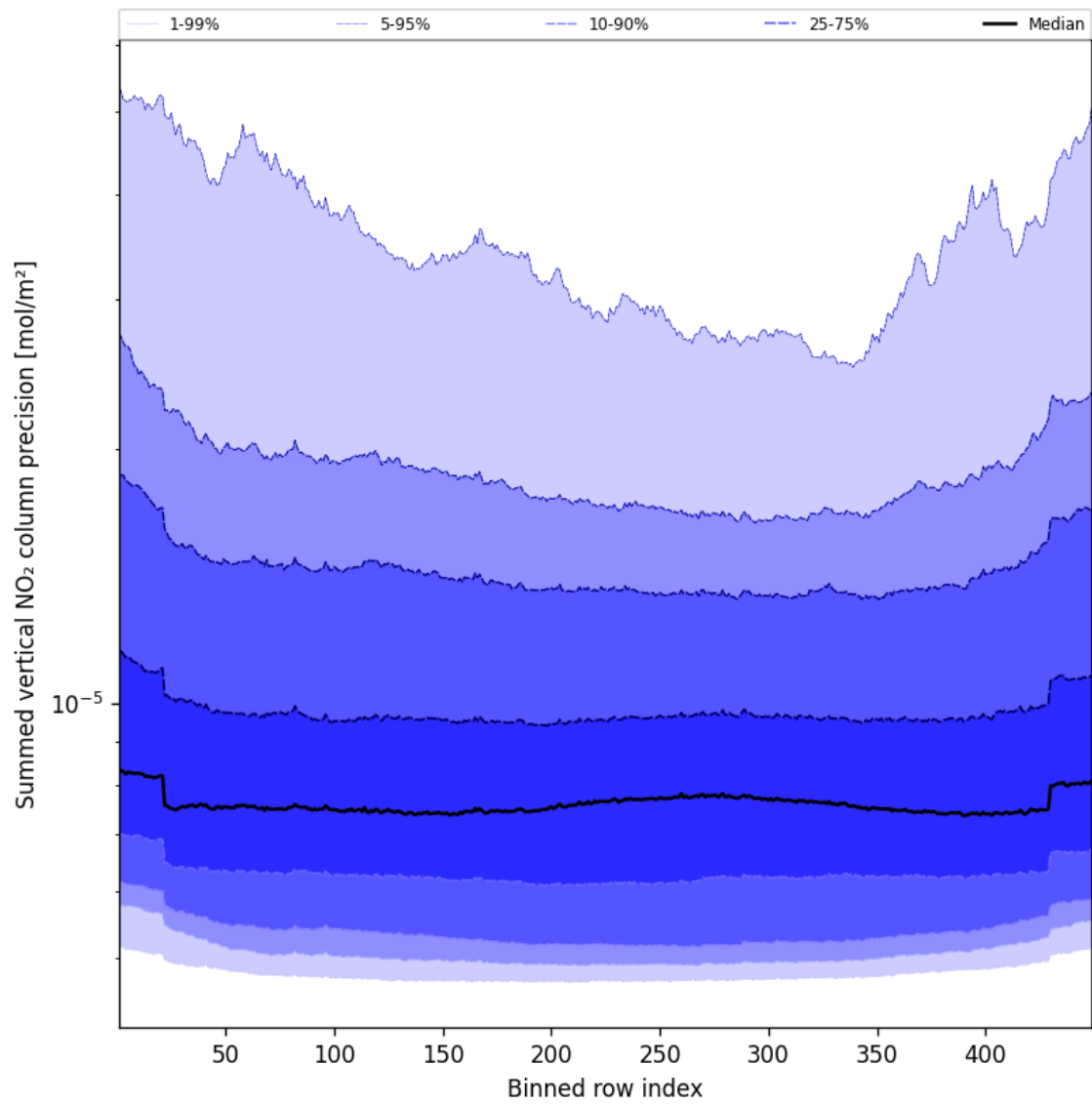
Figure 56: Along track statistics of “Summed vertical NO 2 column precision” for 2025-04-17 to 2025-04-18
