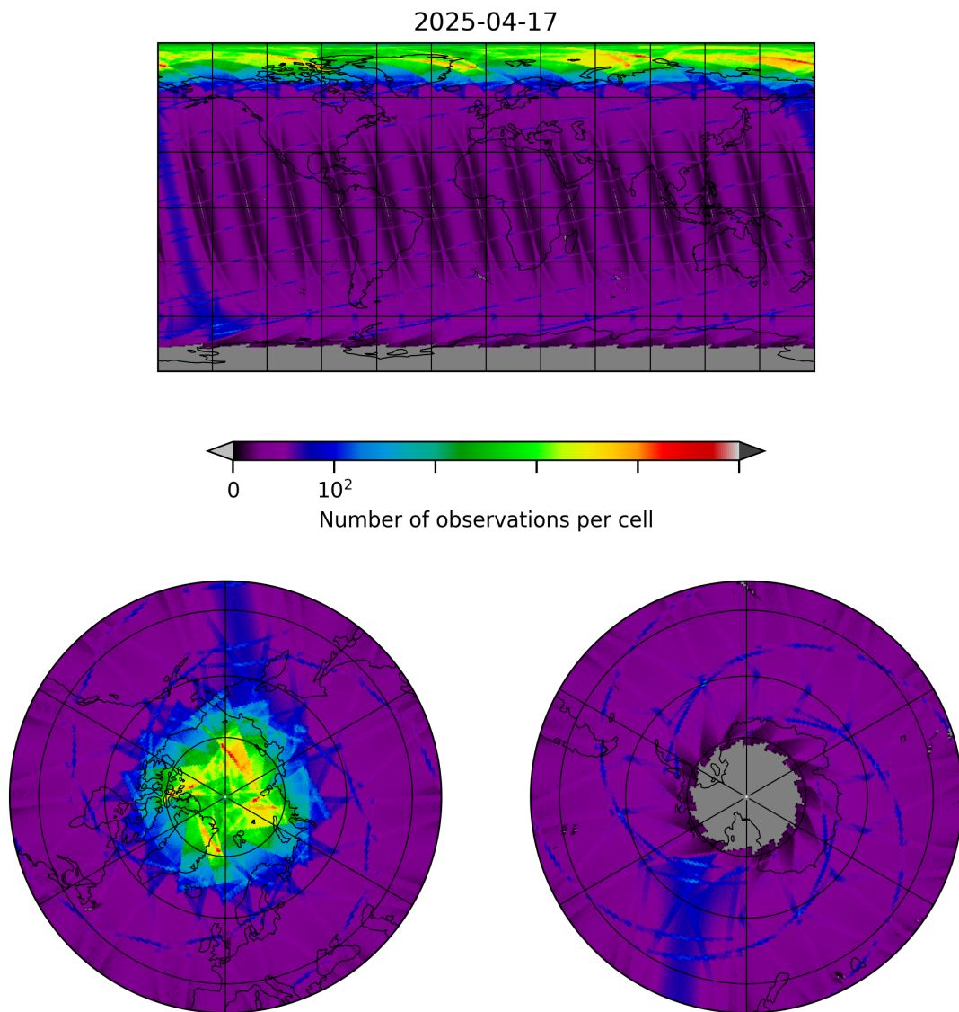
Figure 8: Map of the number of observations for 2025-04-17 to 2025-04-18
