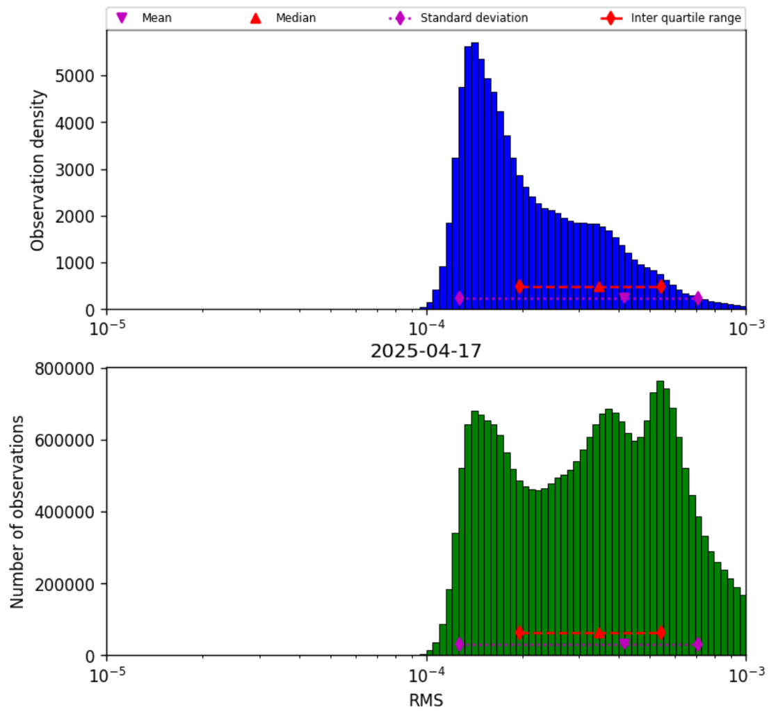
Figure 41: Histogram of “RMS” for 2025-04-17 to 2025-04-18
