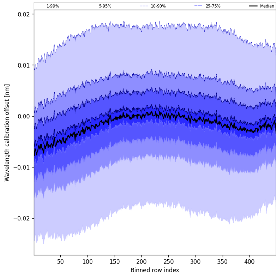
Figure 50: Along track statistics of “Wavelength calibration offset” for 2025-04-17 to 2025-04-18
