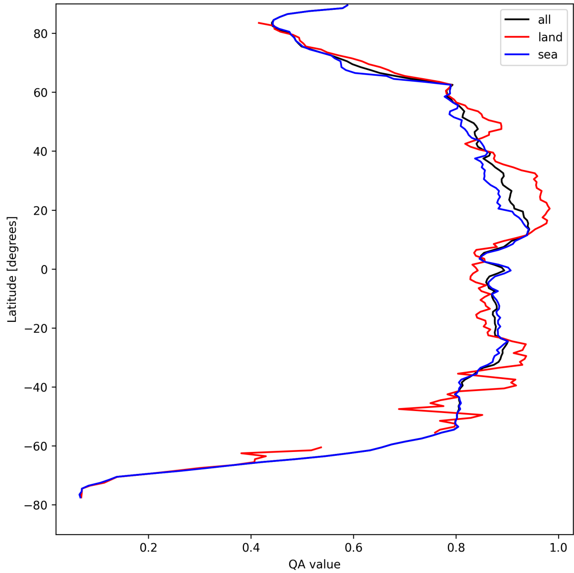
Figure 9: Zonal average of “QA value” for 2025-04-17 to 2025-04-18.
