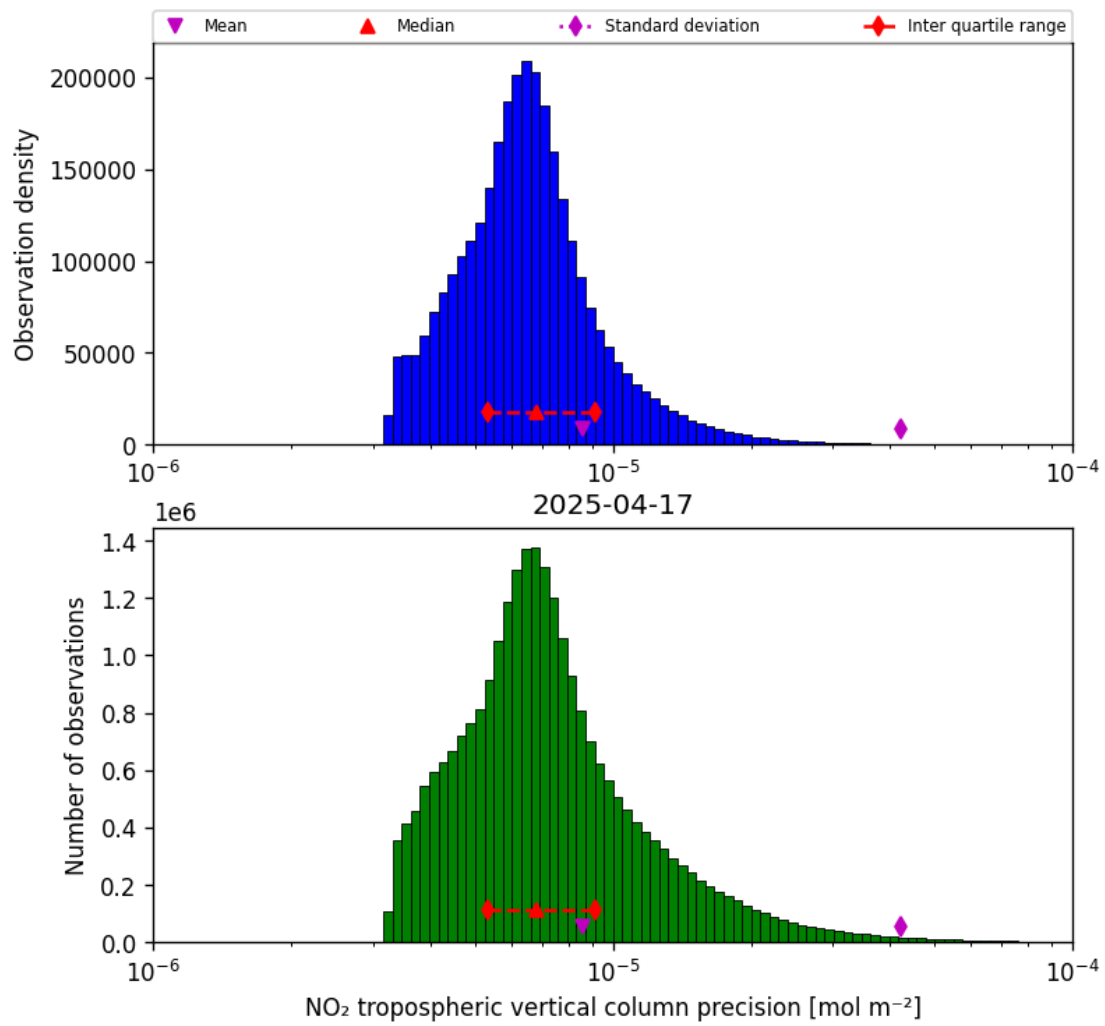
Figure 28: Histogram of “NO 2 tropospheric vertical column precision” for 2025-04-17 to 2025-04-18
