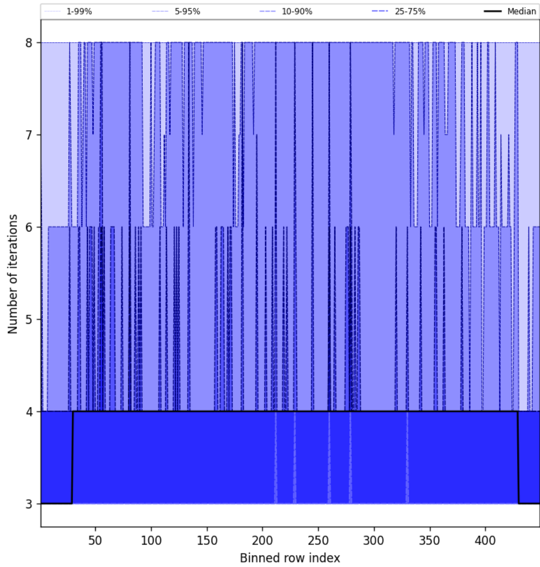
Figure 49: Along track statistics of “Number of iterations” for 2025-04-17 to 2025-04-18
