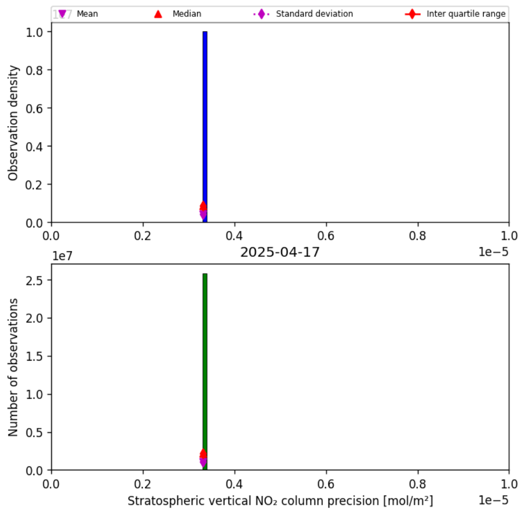
Figure 35: Histogram of “Stratospheric vertical NO 2 column precision” for 2025-04-17 to 2025-04-18
