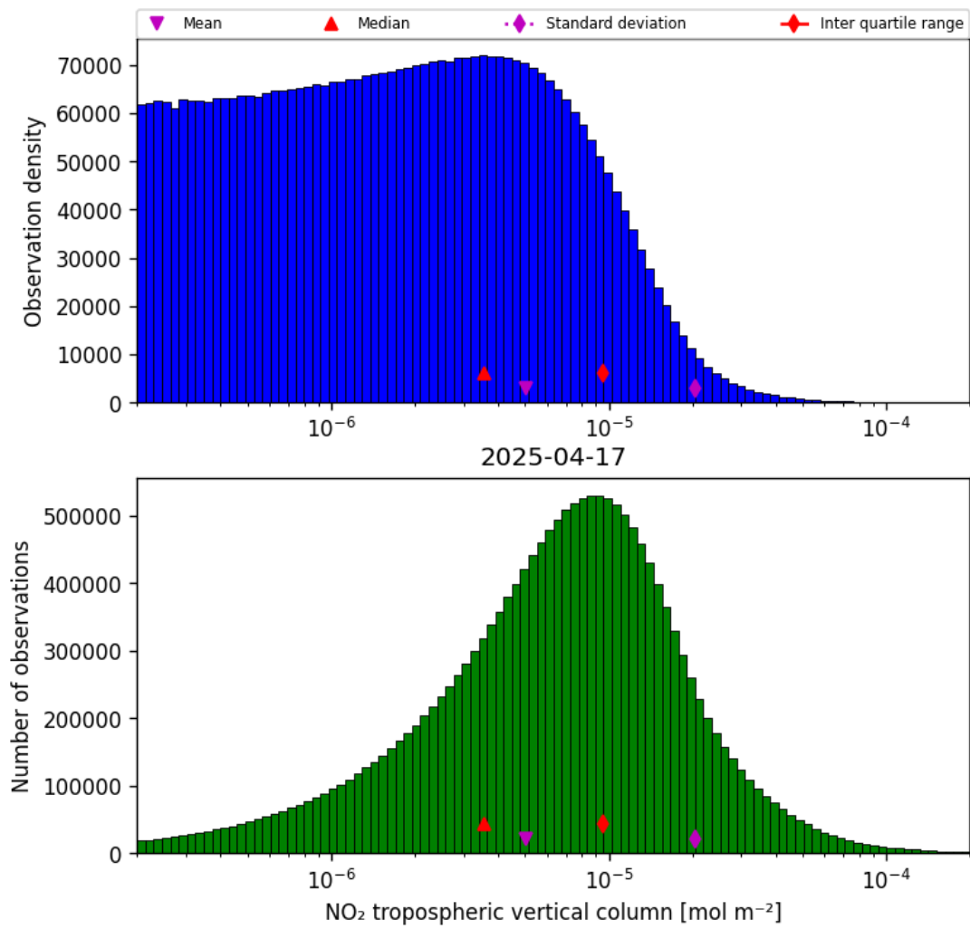
Figure 27: Histogram of “NO 2 tropospheric vertical column” for 2025-04-17 to 2025-04-18
