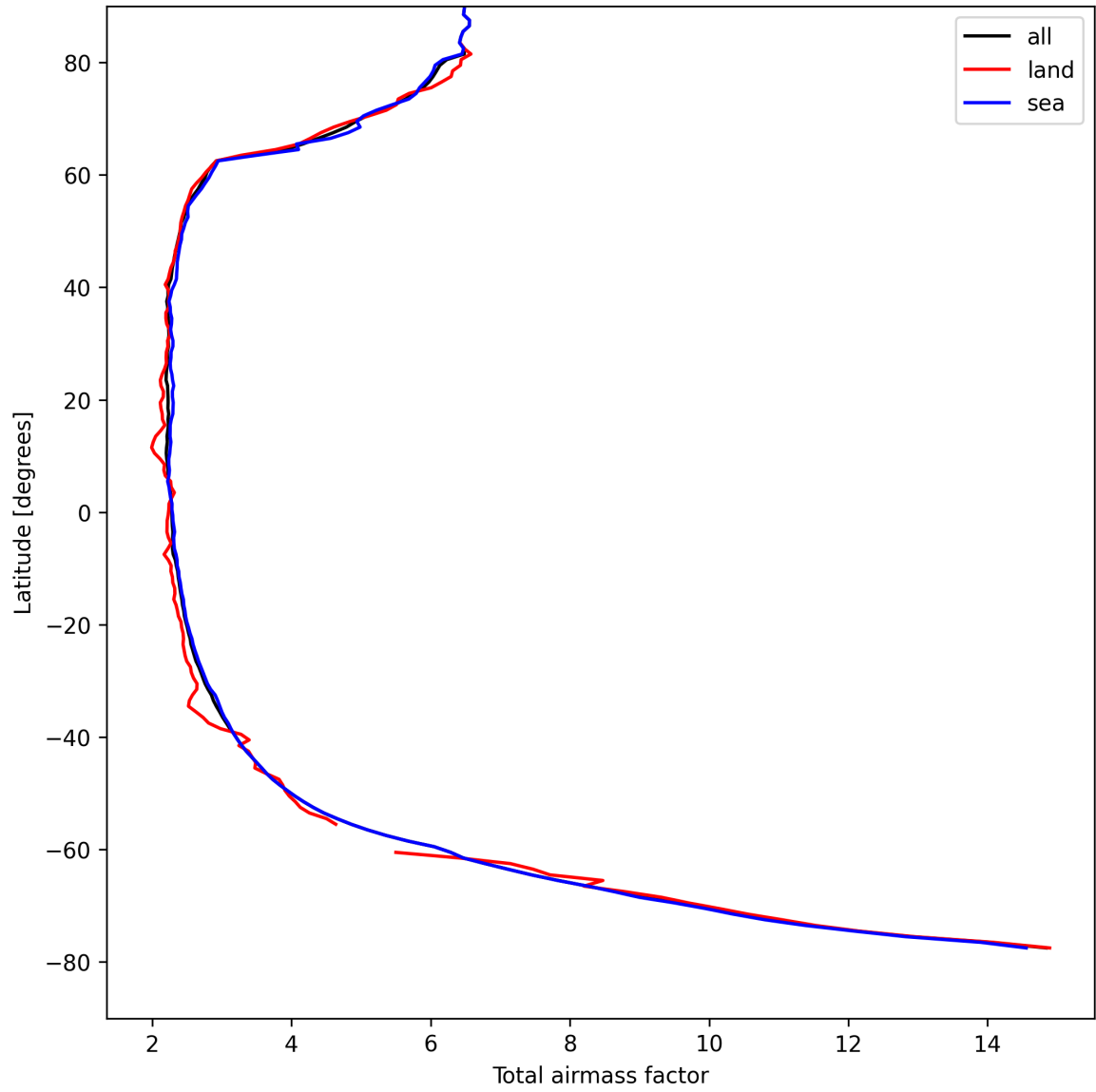
Figure 13: Zonal average of “Total airmass factor” for 2025-04-17 to 2025-04-18.
