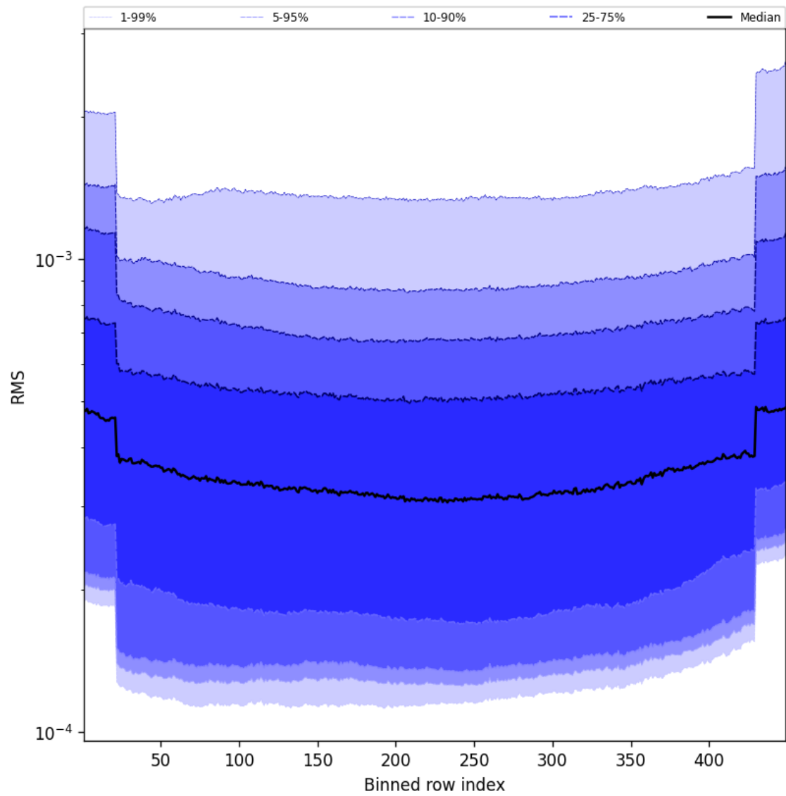
Figure 58: Along track statistics of “RMS” for 2025-04-17 to 2025-04-18
