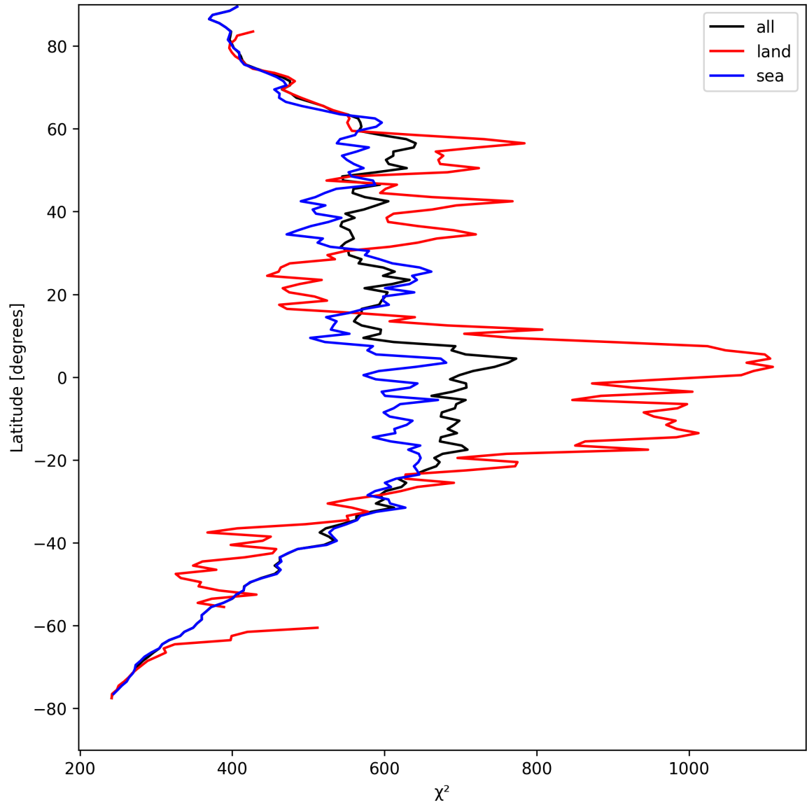
Figure 23: Zonal average of “ \chi^2 ” for 2025-04-18 to 2025-04-19.
