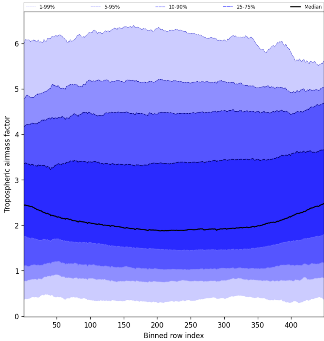
Figure 46: Along track statistics of “Tropospheric airmass factor” for 2025-04-18 to 2025-04-19
