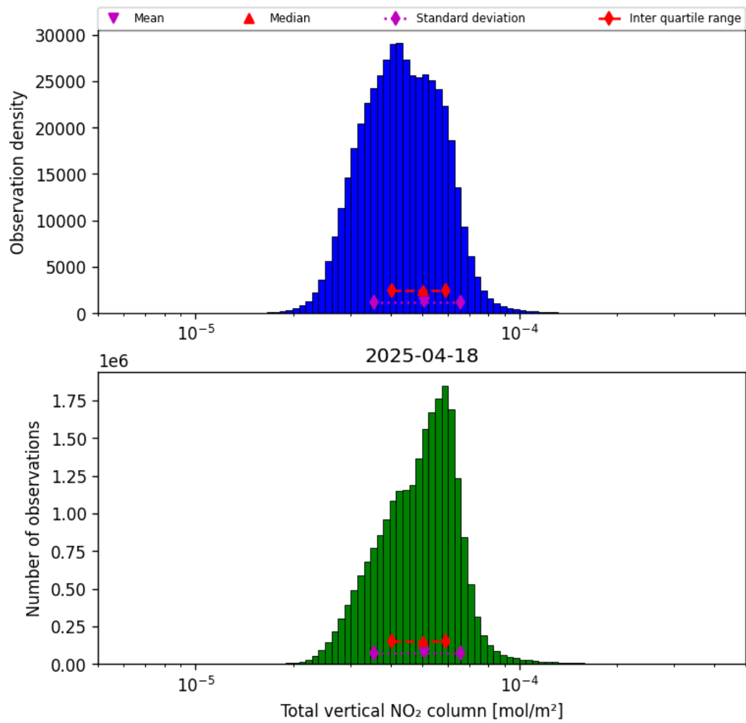
Figure 36: Histogram of “Total vertical NO 2 column” for 2025-04-18 to 2025-04-19
