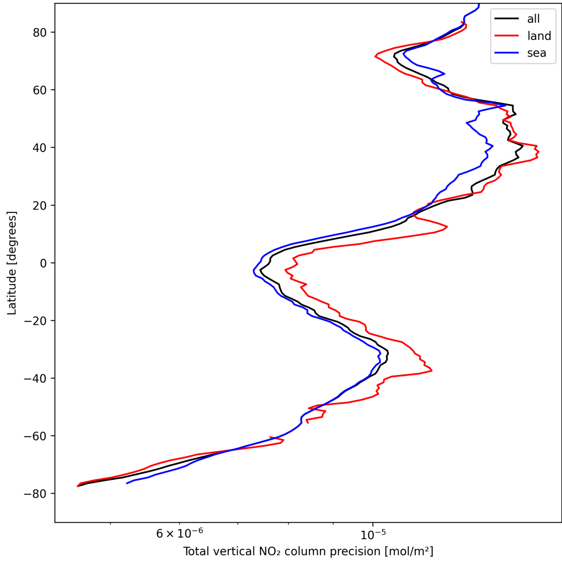
Figure 20: Zonal average of “Total vertical NO 2 column precision” for 2025-04-18 to 2025-04-19.
