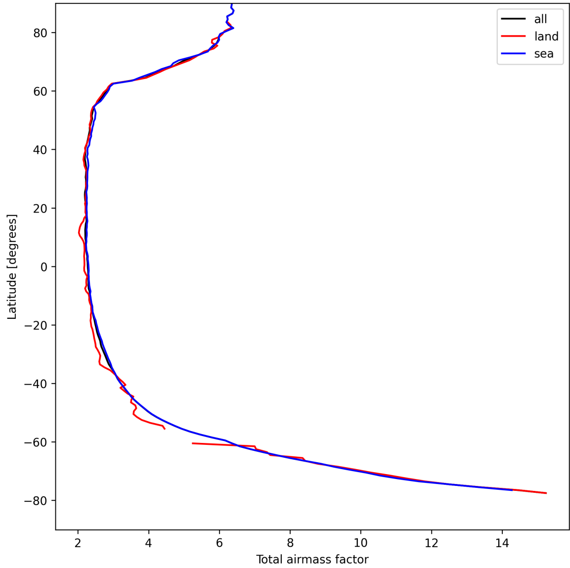
Figure 13: Zonal average of “Total airmass factor” for 2025-04-18 to 2025-04-19.
