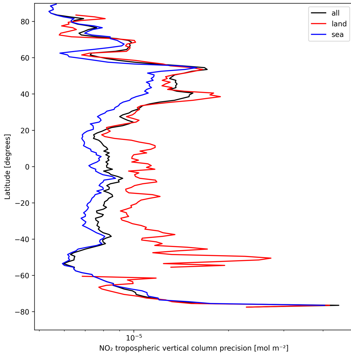
Figure 11: Zonal average of “NO 2 tropospheric vertical column precision” for 2025-04-18 to 2025-04-19.
