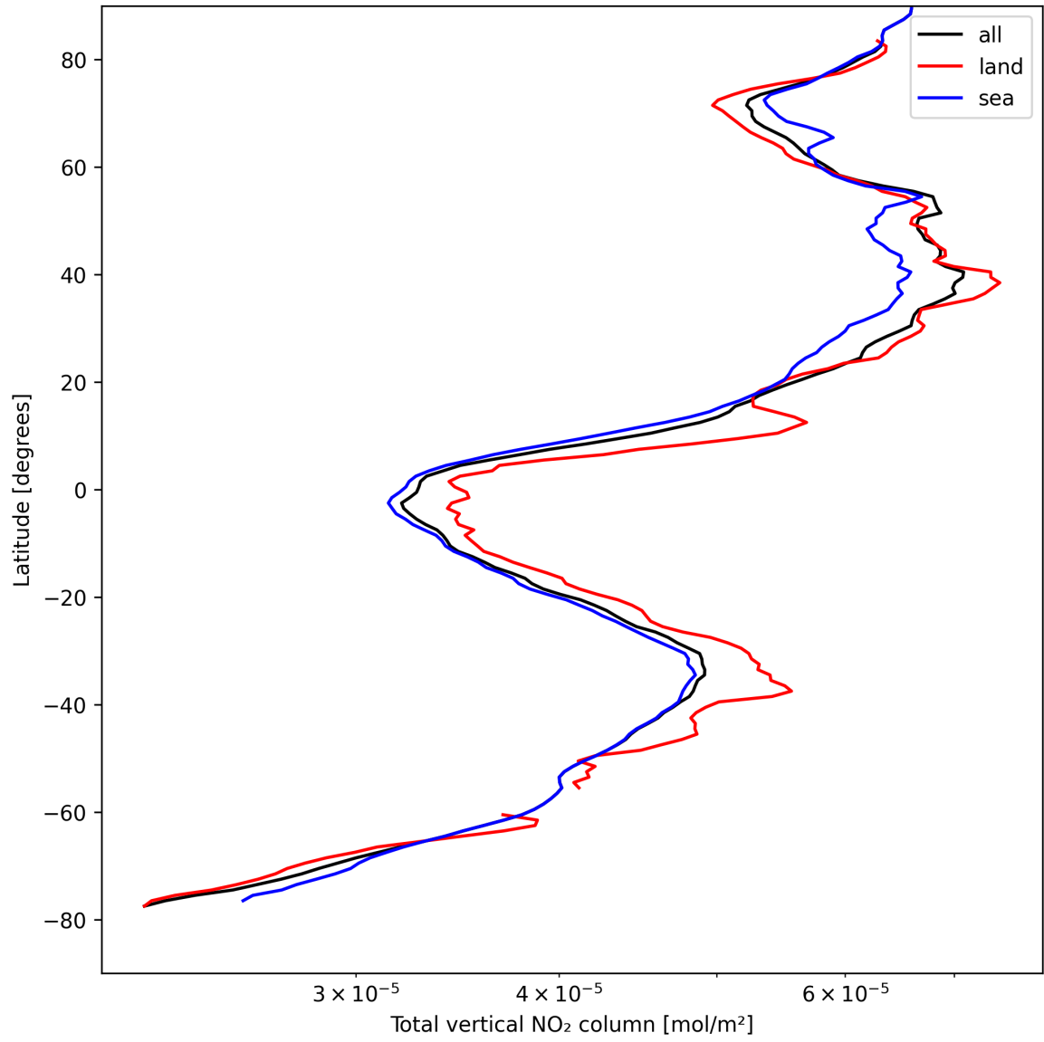
Figure 19: Zonal average of “Total vertical NO 2 column” for 2025-04-18 to 2025-04-19.
