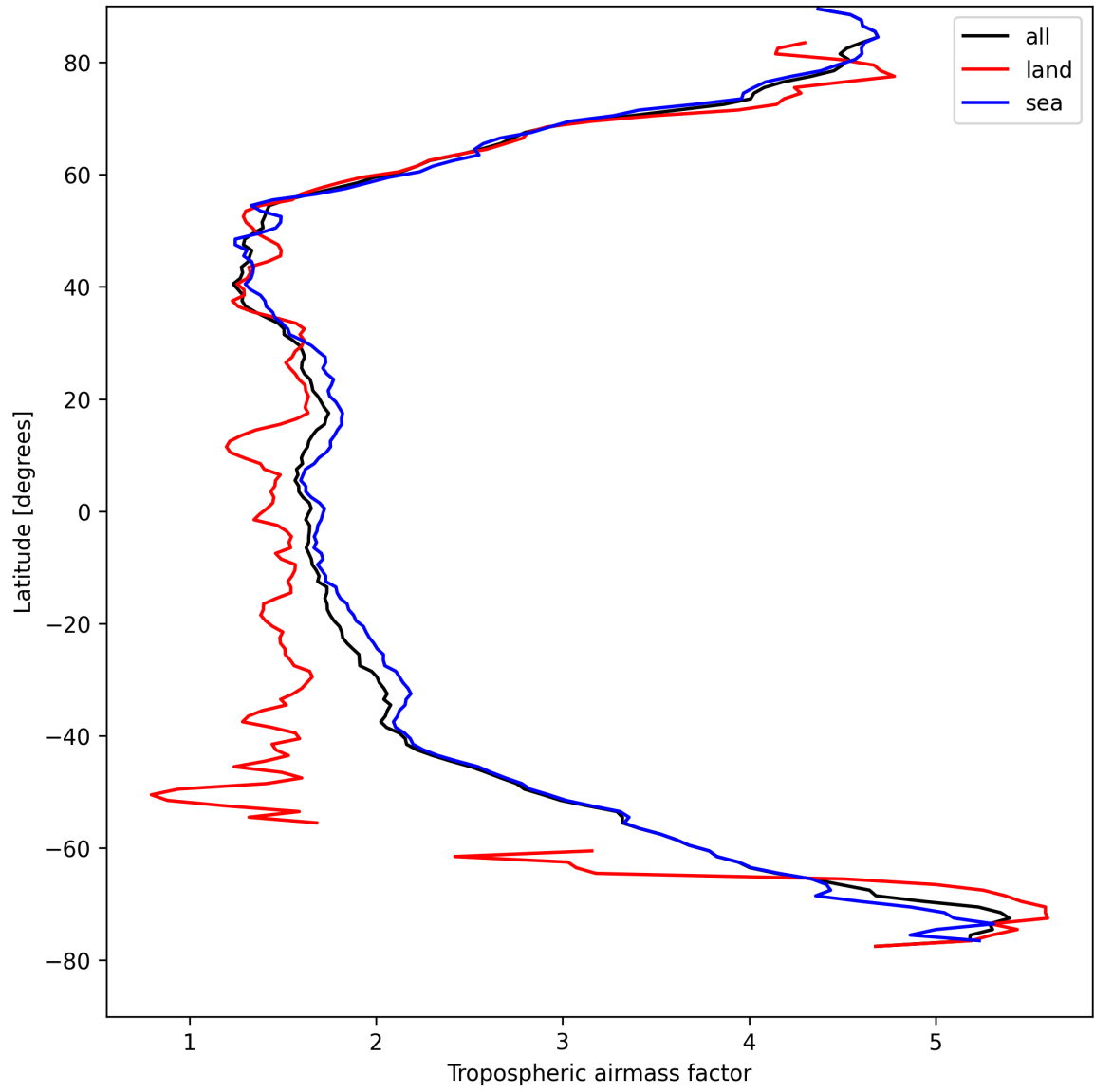
Figure 12: Zonal average of “Tropospheric airmass factor” for 2025-04-18 to 2025-04-19.
