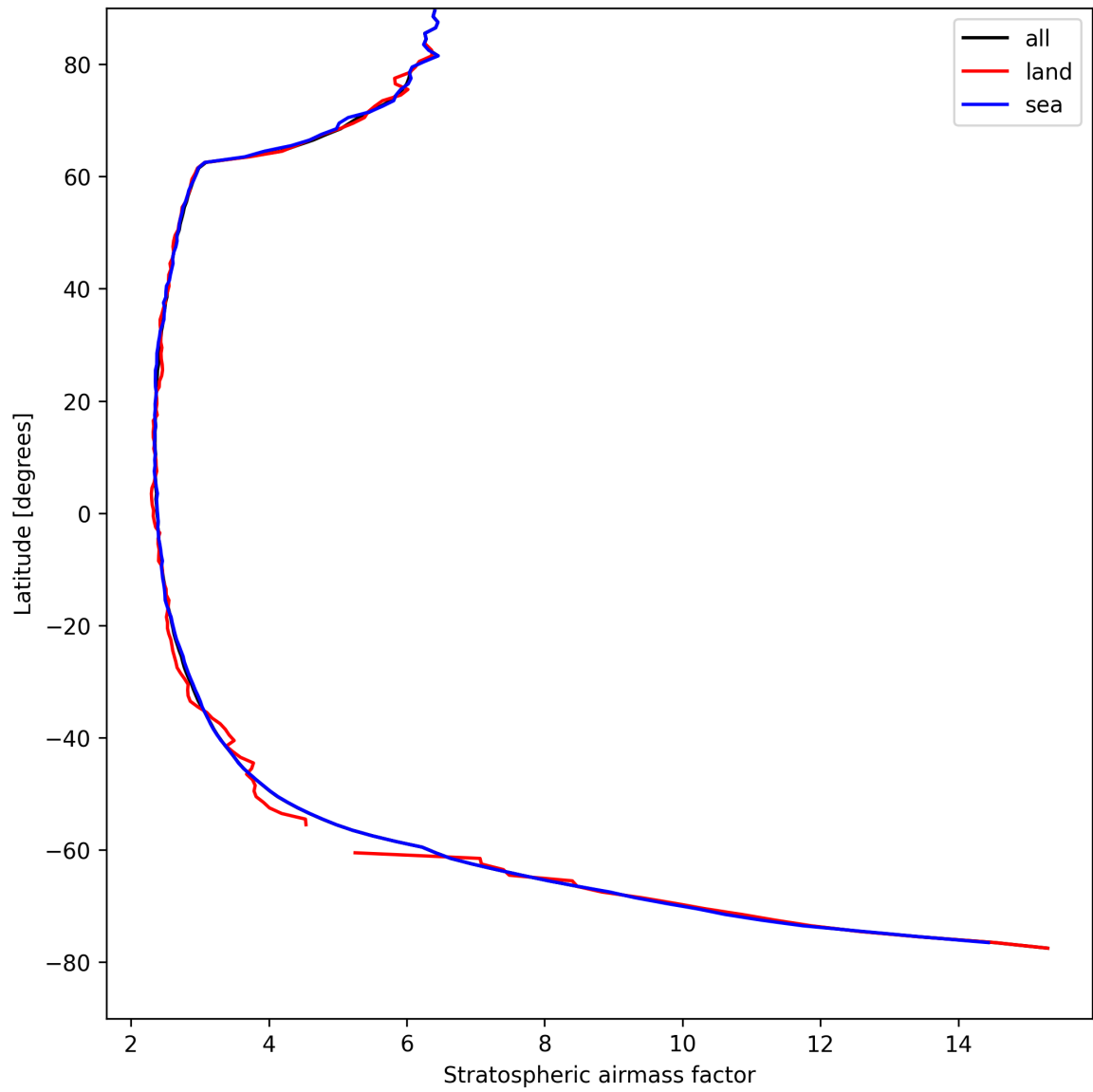
Figure 25: Zonal average of “Stratospheric airmass factor” for 2025-04-18 to 2025-04-19.
