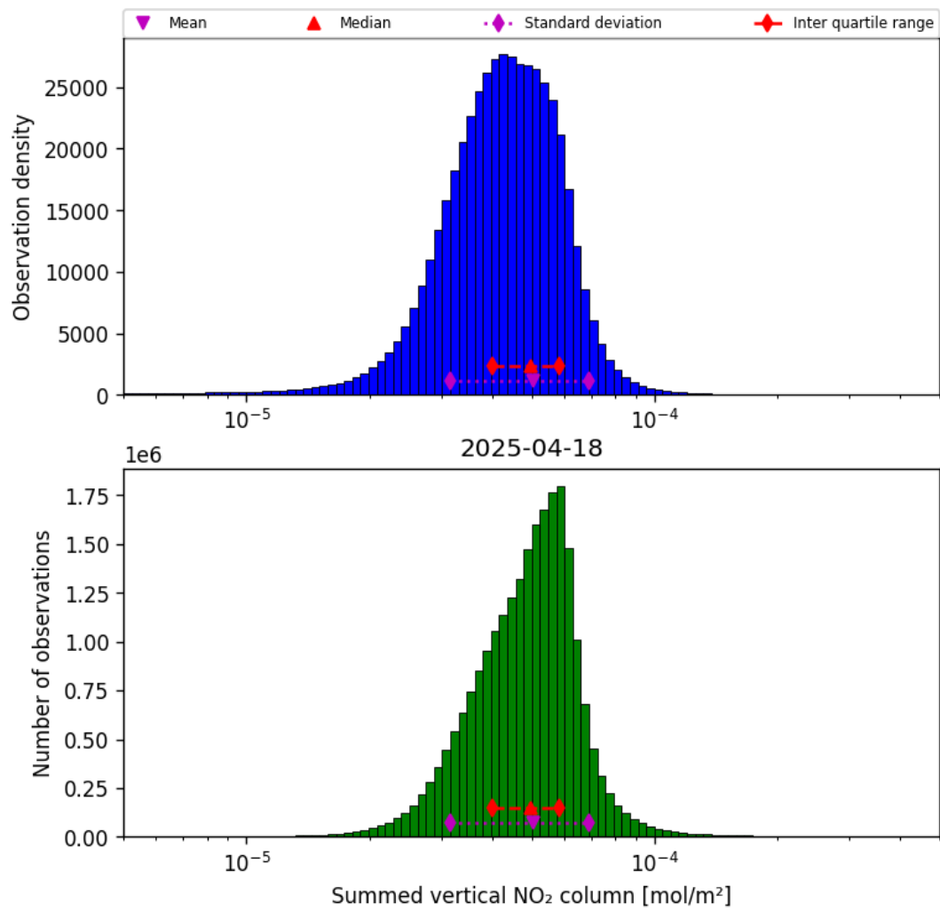
Figure 38: Histogram of “Summed vertical NO 2 column” for 2025-04-18 to 2025-04-19
