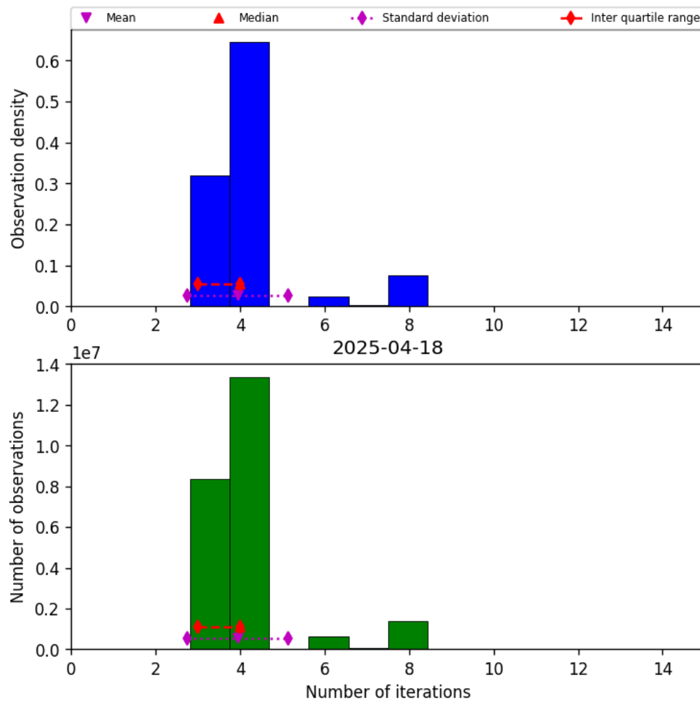
Figure 32: Histogram of “Number of iterations” for 2025-04-18 to 2025-04-19
