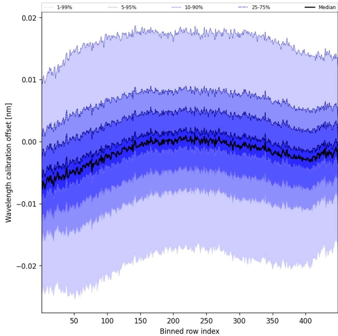
Figure 50: Along track statistics of “Wavelength calibration offset” for 2025-04-18 to 2025-04-19
