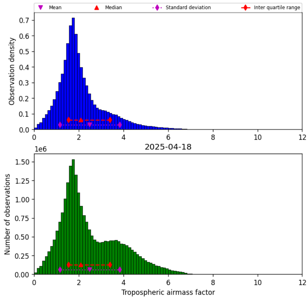
Figure 29: Histogram of “Tropospheric airmass factor” for 2025-04-18 to 2025-04-19
