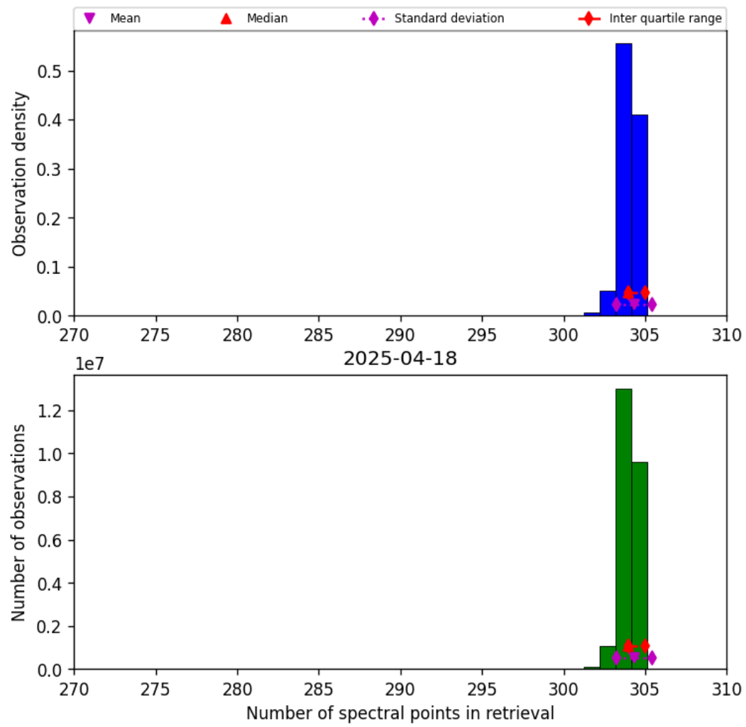
Figure 31: Histogram of “Number of spectral points in retrieval” for 2025-04-18 to 2025-04-19
