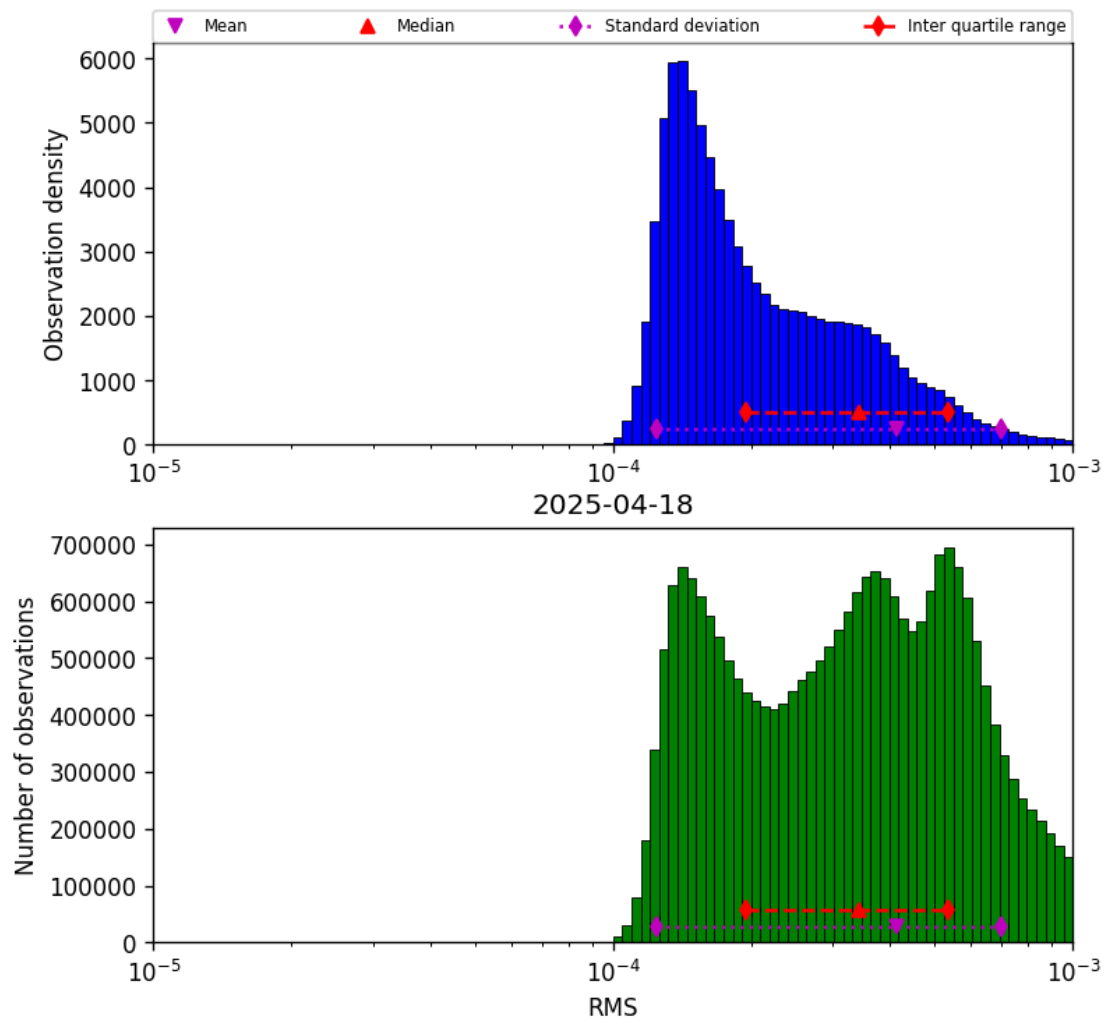
Figure 41: Histogram of “RMS” for 2025-04-18 to 2025-04-19
