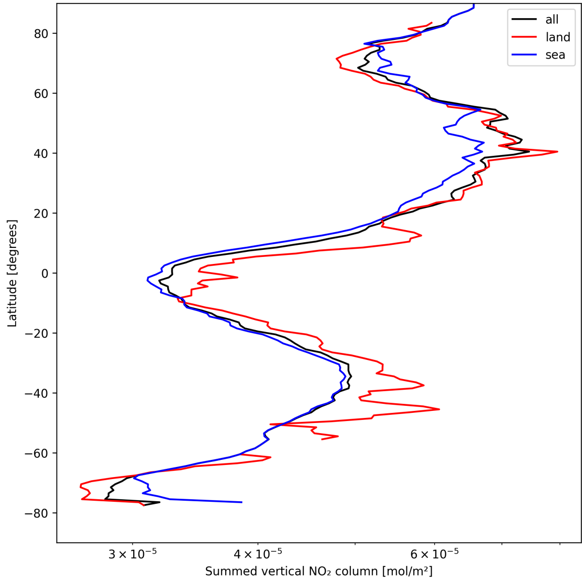
Figure 21: Zonal average of “Summed vertical NO 2 column” for 2025-04-18 to 2025-04-19.
