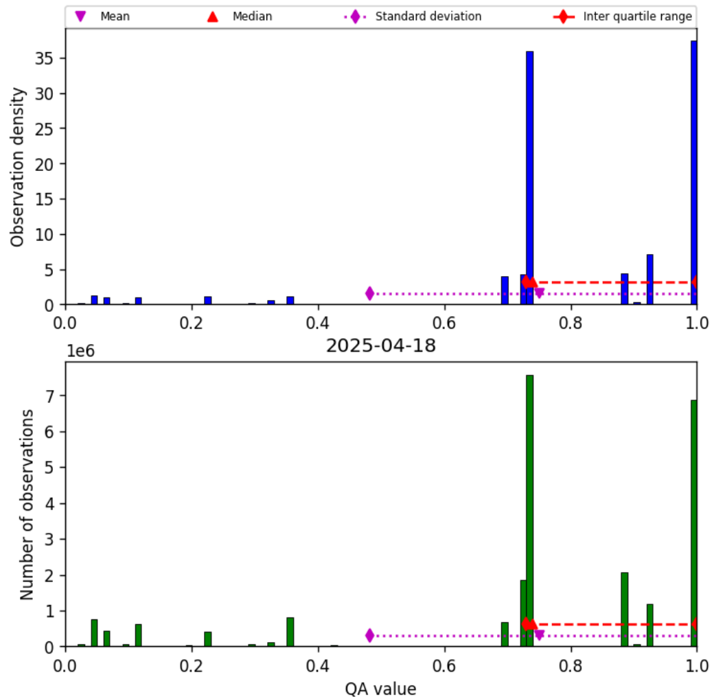
Figure 26: Histogram of “QA value” for 2025-04-18 to 2025-04-19
