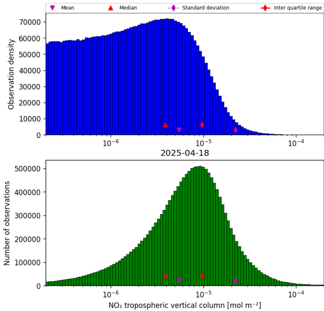
Figure 27: Histogram of “NO 2 tropospheric vertical column” for 2025-04-18 to 2025-04-19
