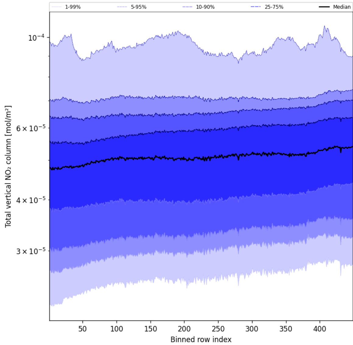
Figure 53: Along track statistics of “Total vertical NO 2 column” for 2025-04-18 to 2025-04-19
