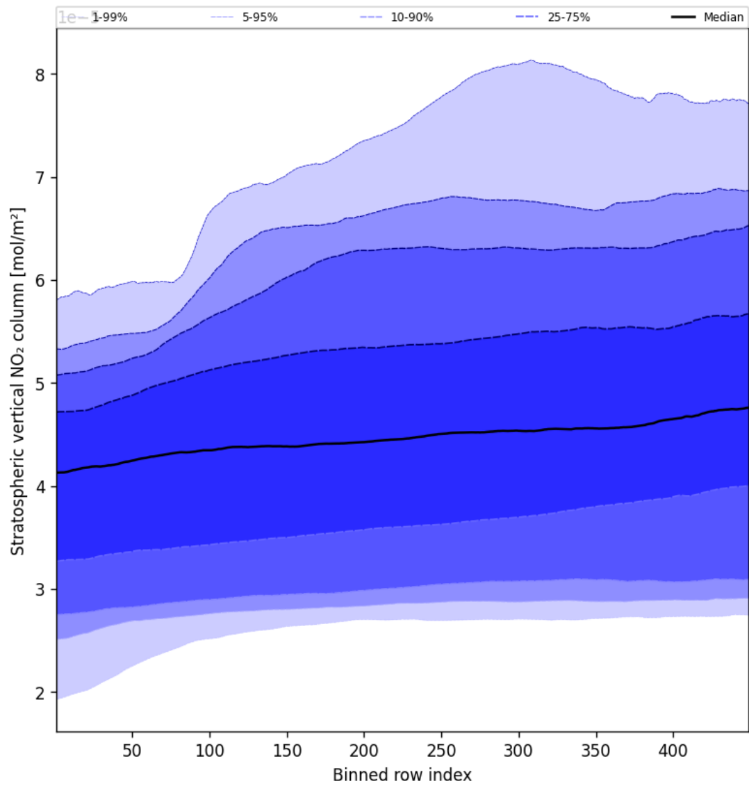
Figure 51: Along track statistics of “Stratospheric vertical NO 2 column” for 2025-04-18 to 2025-04-19
