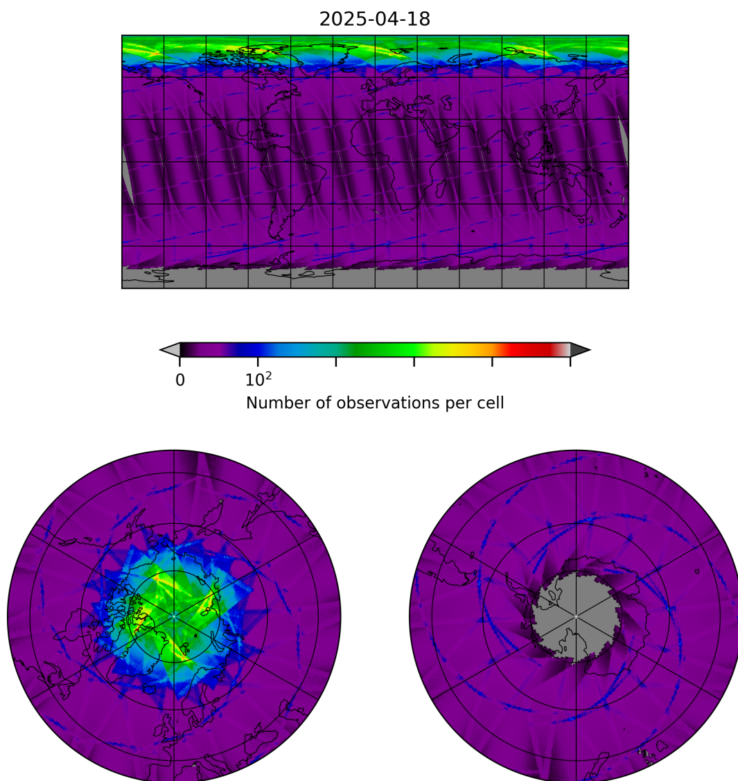
Figure 8: Map of the number of observations for 2025-04-18 to 2025-04-19
