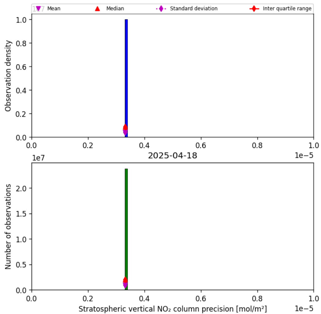
Figure 35: Histogram of “Stratospheric vertical NO 2 column precision” for 2025-04-18 to 2025-04-19
