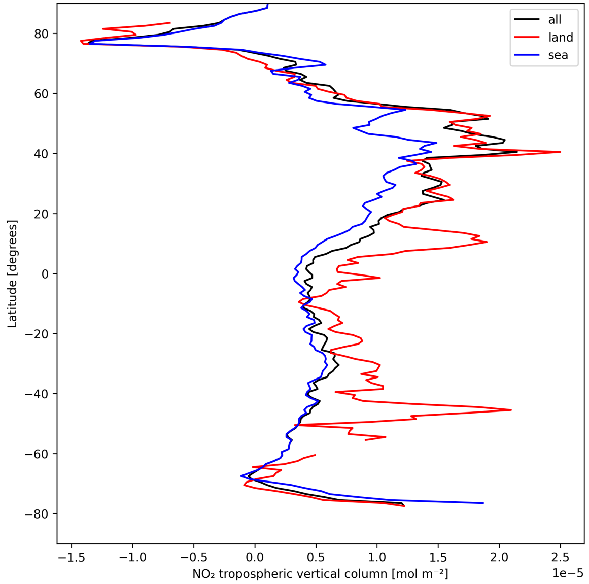
Figure 10: Zonal average of “NO 2 tropospheric vertical column” for 2025-04-18 to 2025-04-19.
