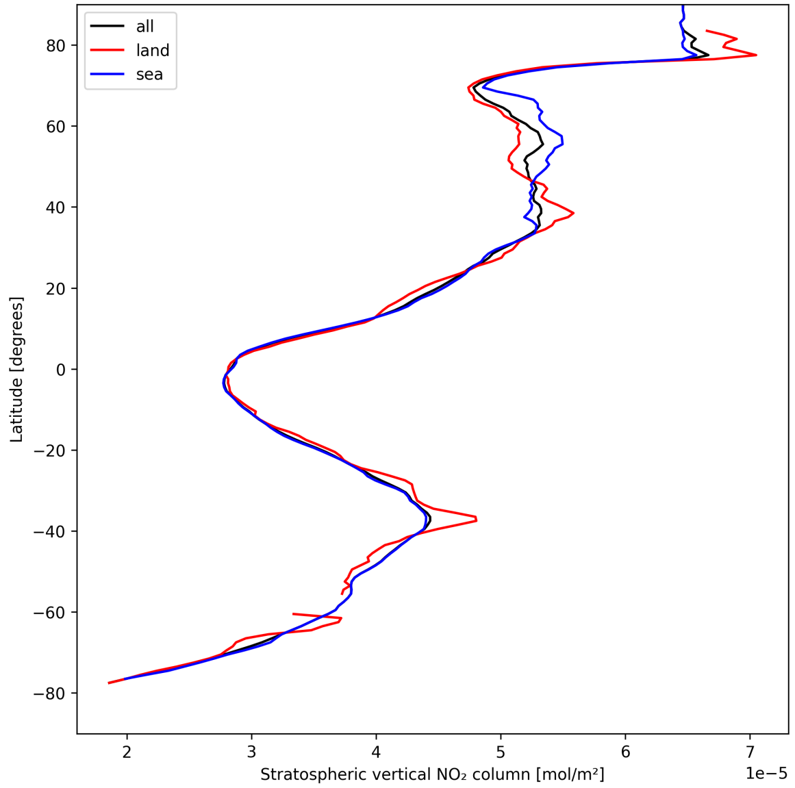
Figure 17: Zonal average of “Stratospheric vertical NO 2 column” for 2025-04-18 to 2025-04-19.
