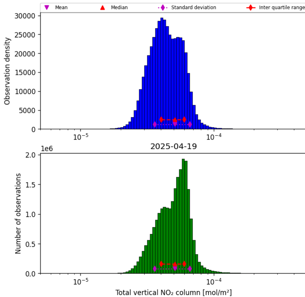
Figure 36: Histogram of “Total vertical NO 2 column” for 2025-04-19 to 2025-04-20
