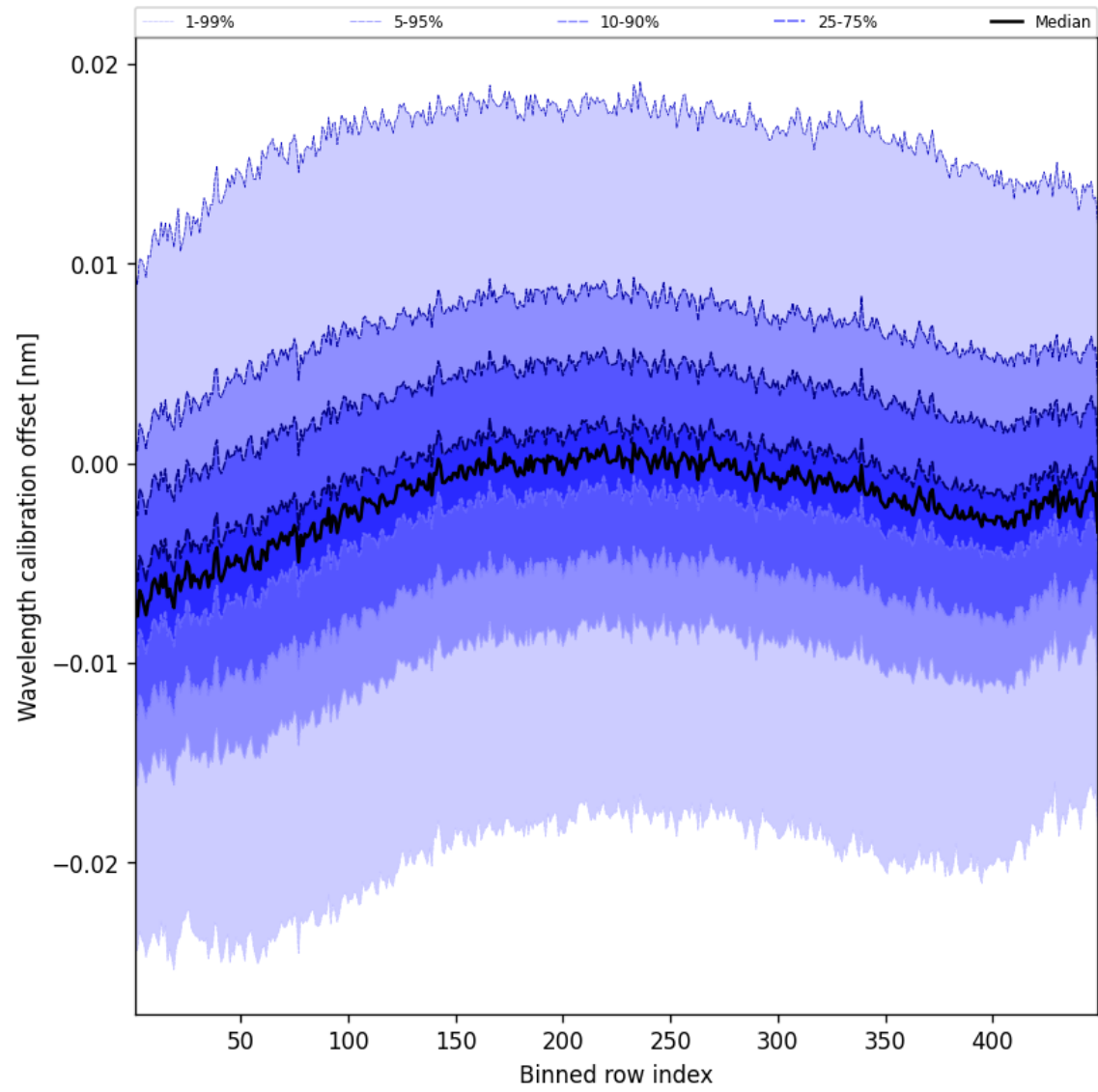
Figure 50: Along track statistics of “Wavelength calibration offset” for 2025-04-19 to 2025-04-20
