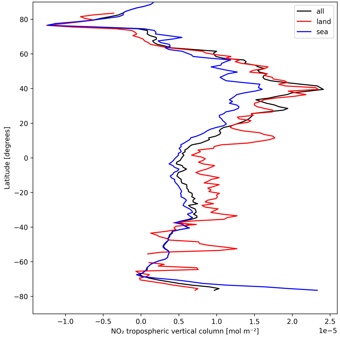
Figure 10: Zonal average of “NO 2 tropospheric vertical column” for 2025-04-19 to 2025-04-20.
