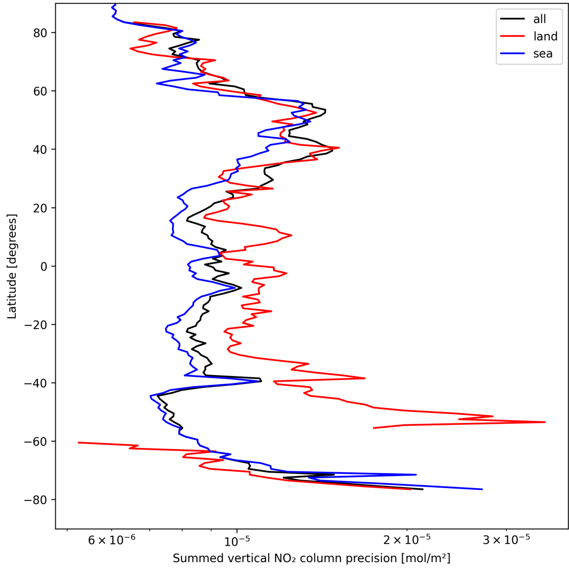
Figure 22: Zonal average of “Summed vertical NO 2 column precision” for 2025-04-19 to 2025-04-20.
