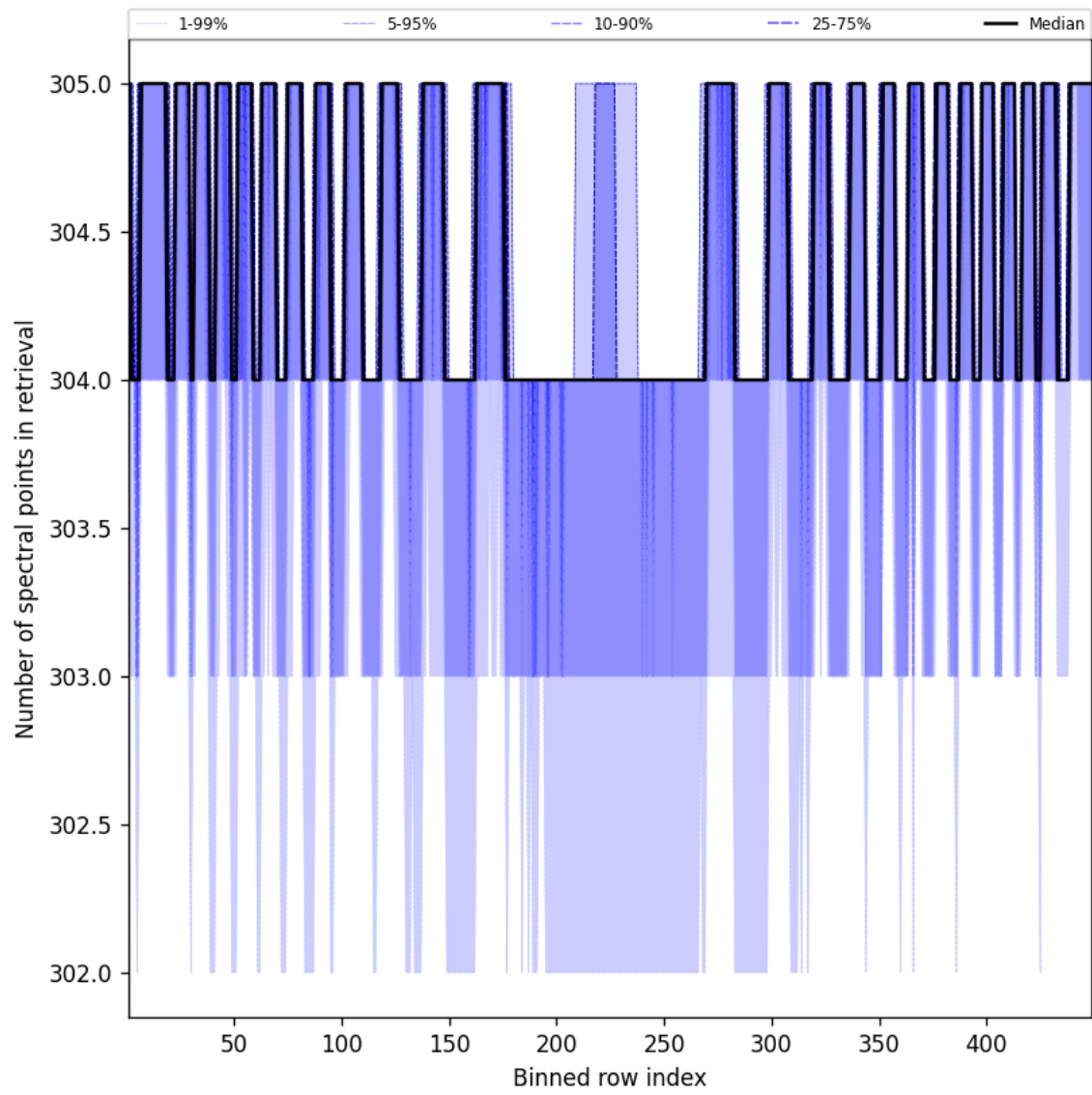
Figure 48: Along track statistics of “Number of spectral points in retrieval” for 2025-04-19 to 2025-04-20
