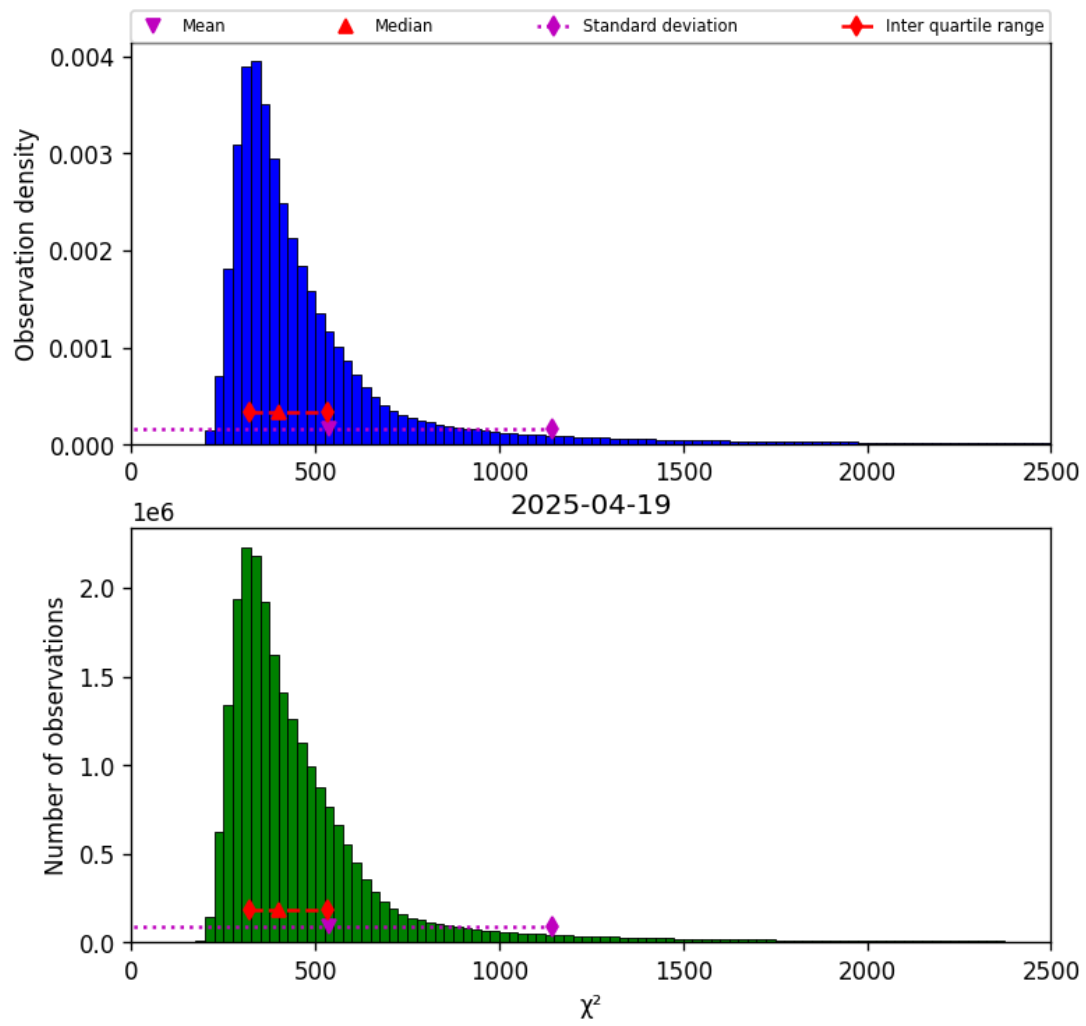
Figure 40: Histogram of “ \chi^2 ” for 2025-04-19 to 2025-04-20
