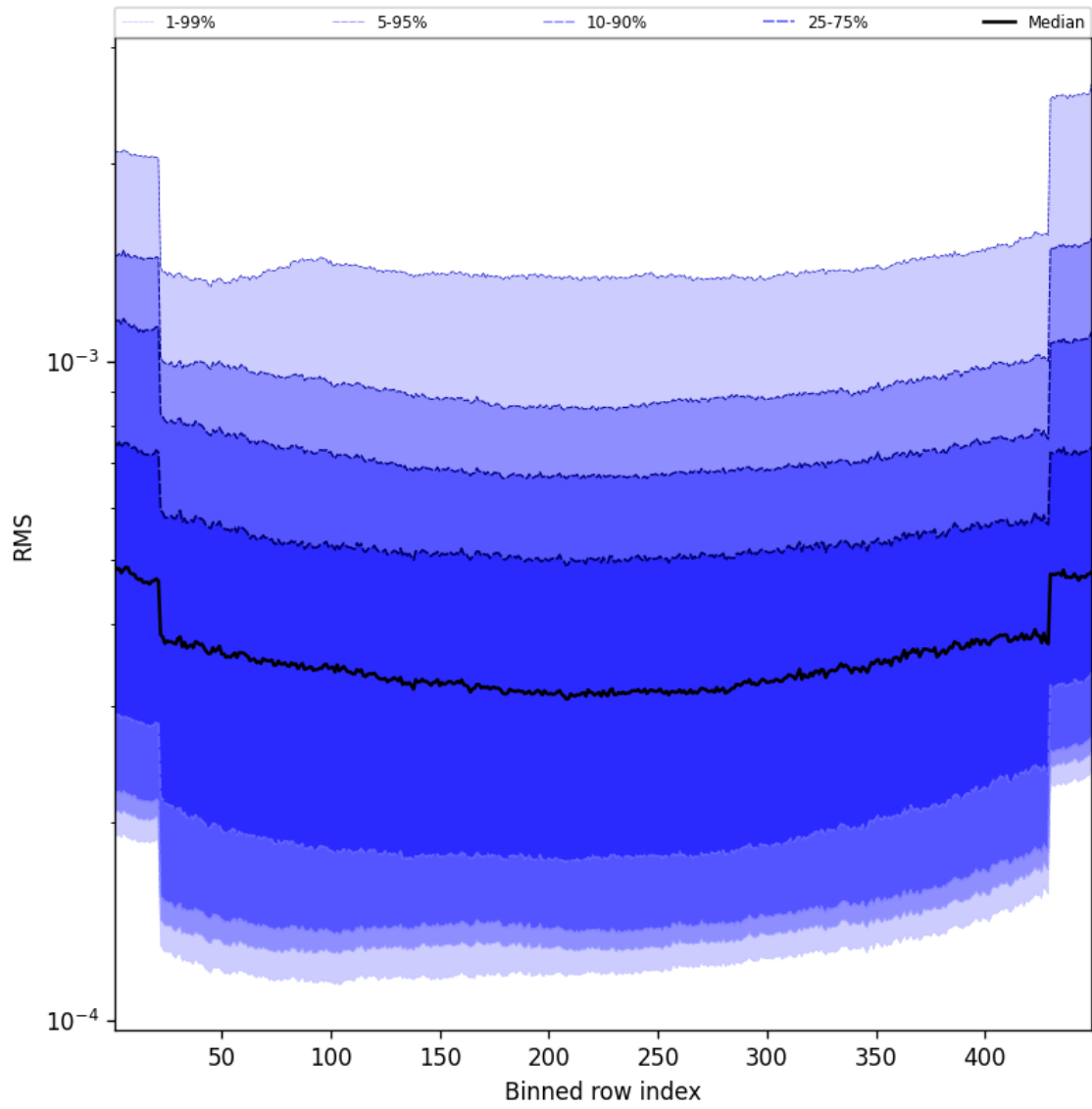
Figure 58: Along track statistics of “RMS” for 2025-04-19 to 2025-04-20
