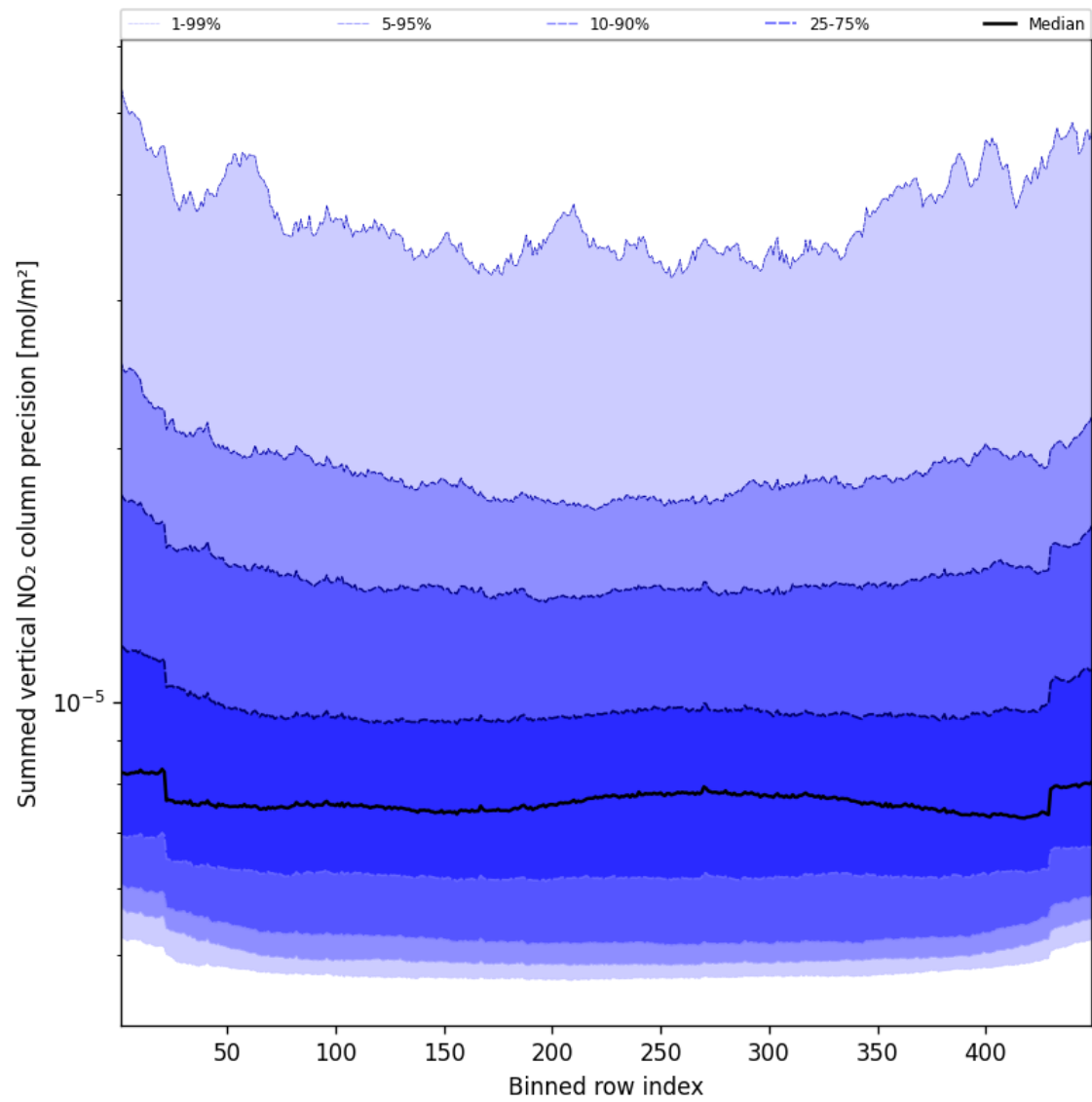
Figure 56: Along track statistics of “Summed vertical NO 2 column precision” for 2025-04-19 to 2025-04-20
