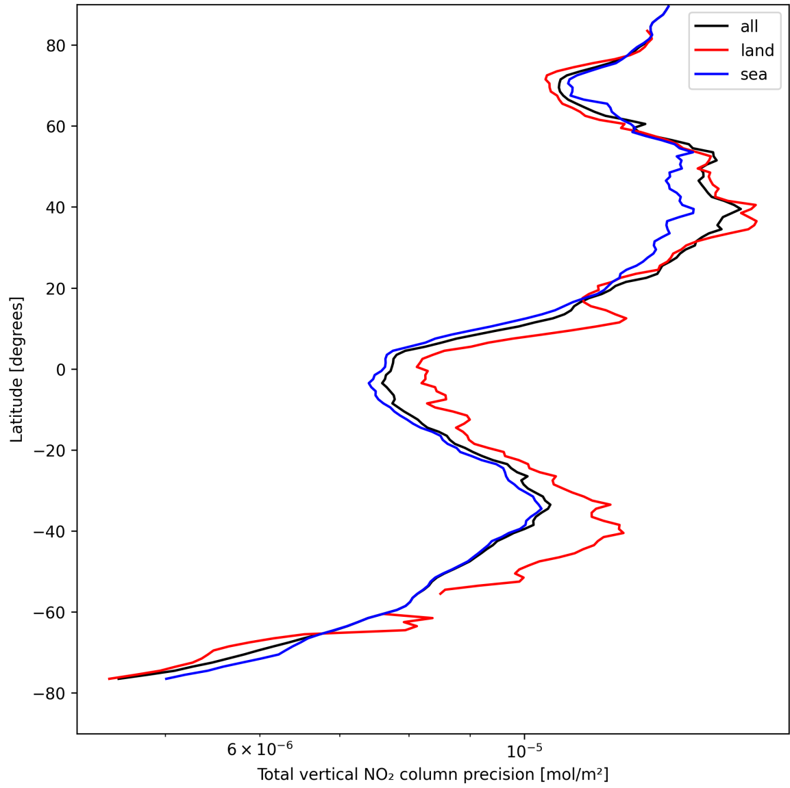
Figure 20: Zonal average of “Total vertical NO 2 column precision” for 2025-04-19 to 2025-04-20.
