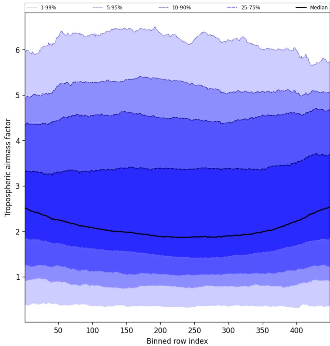
Figure 46: Along track statistics of “Tropospheric airmass factor” for 2025-04-19 to 2025-04-20
