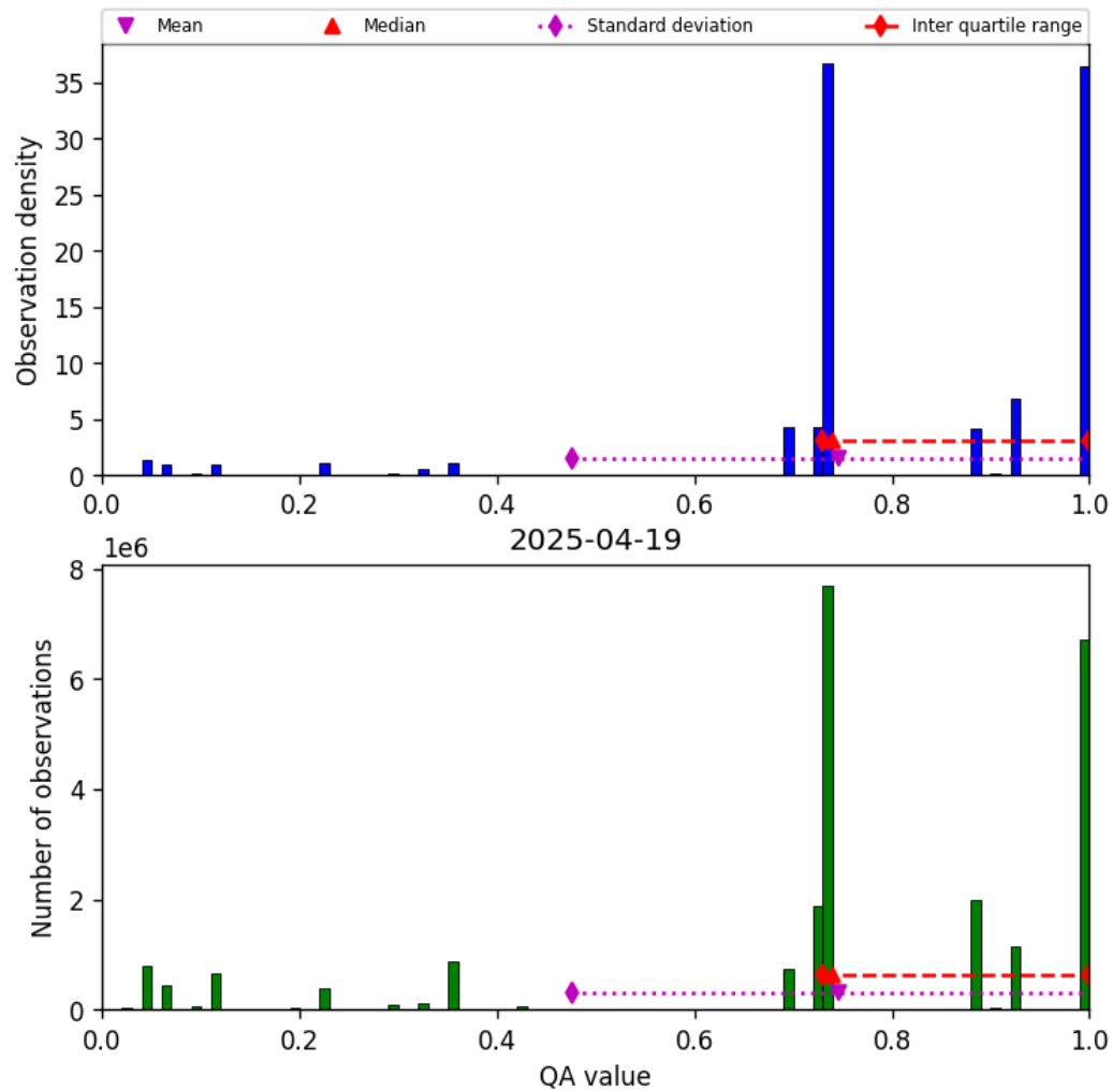
Figure 26: Histogram of “QA value” for 2025-04-19 to 2025-04-20
