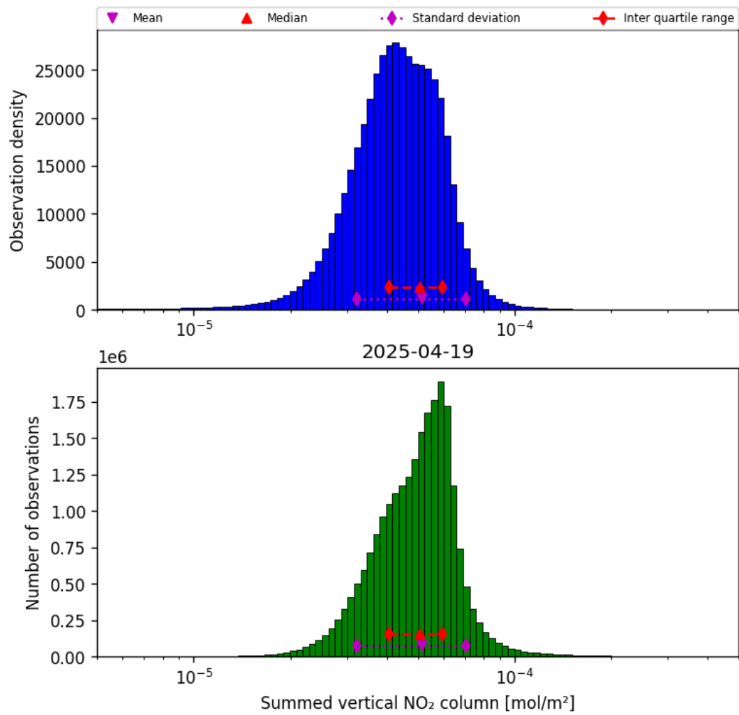
Figure 38: Histogram of "Summed vertical NO 2 column" for 2025-04-19 to 2025-04-20
