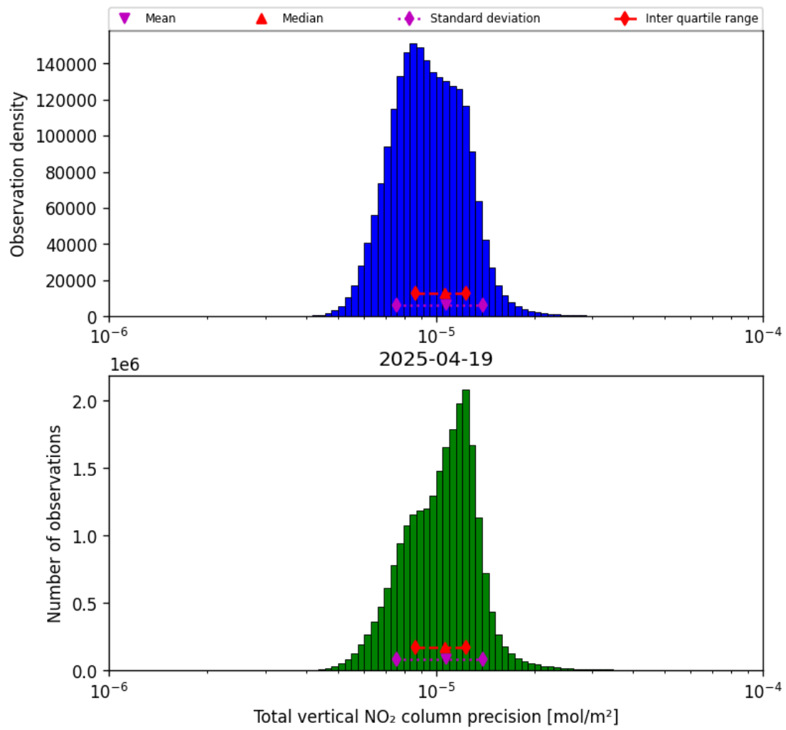
Figure 37: Histogram of "Total vertical NO 2 column precision" for 2025-04-19 to 2025-04-20
