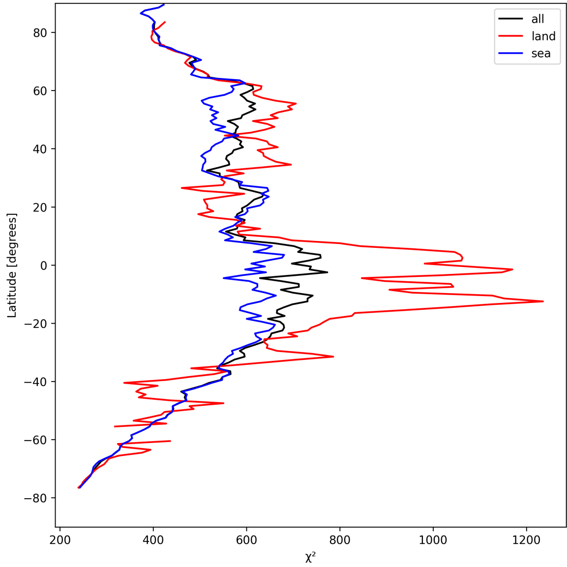
Figure 23: Zonal average of “ \chi^2 ” for 2025-04-19 to 2025-04-20.
