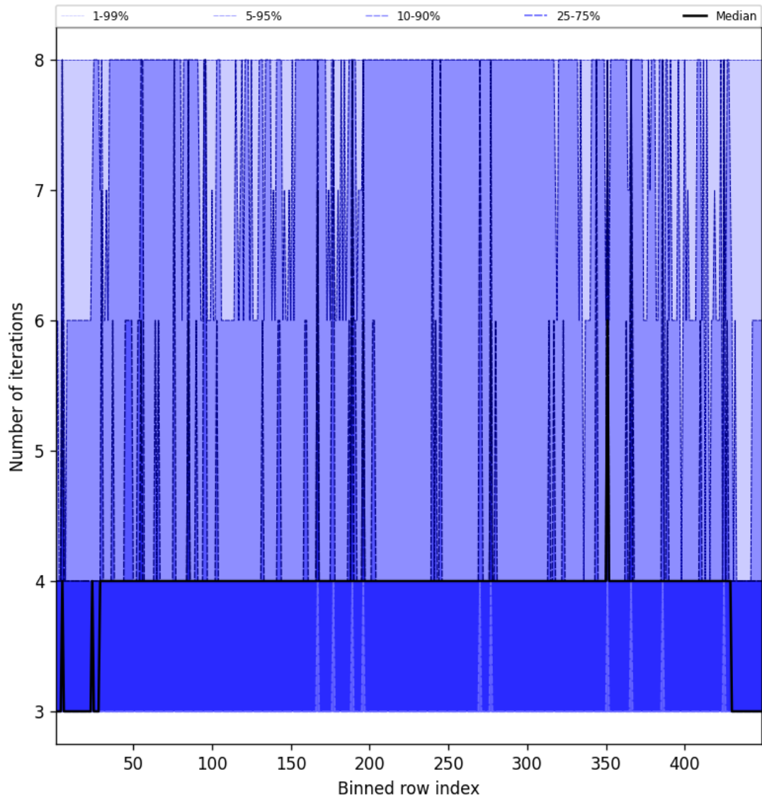
Figure 49: Along track statistics of “Number of iterations” for 2025-04-19 to 2025-04-20
