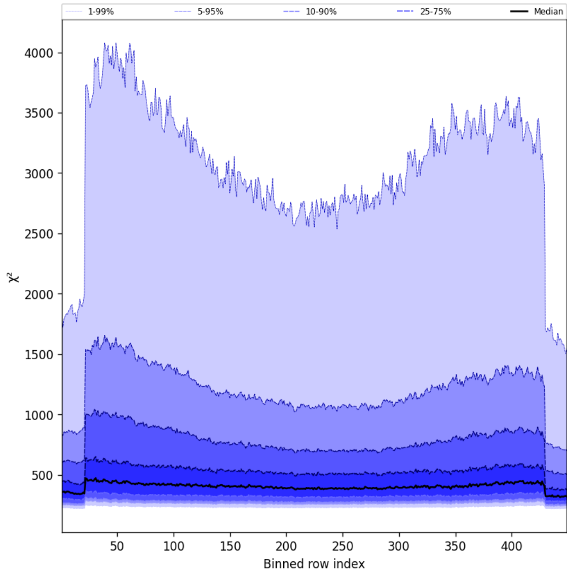
Figure 57: Along track statistics of “ \chi^2 ” for 2025-04-19 to 2025-04-20
