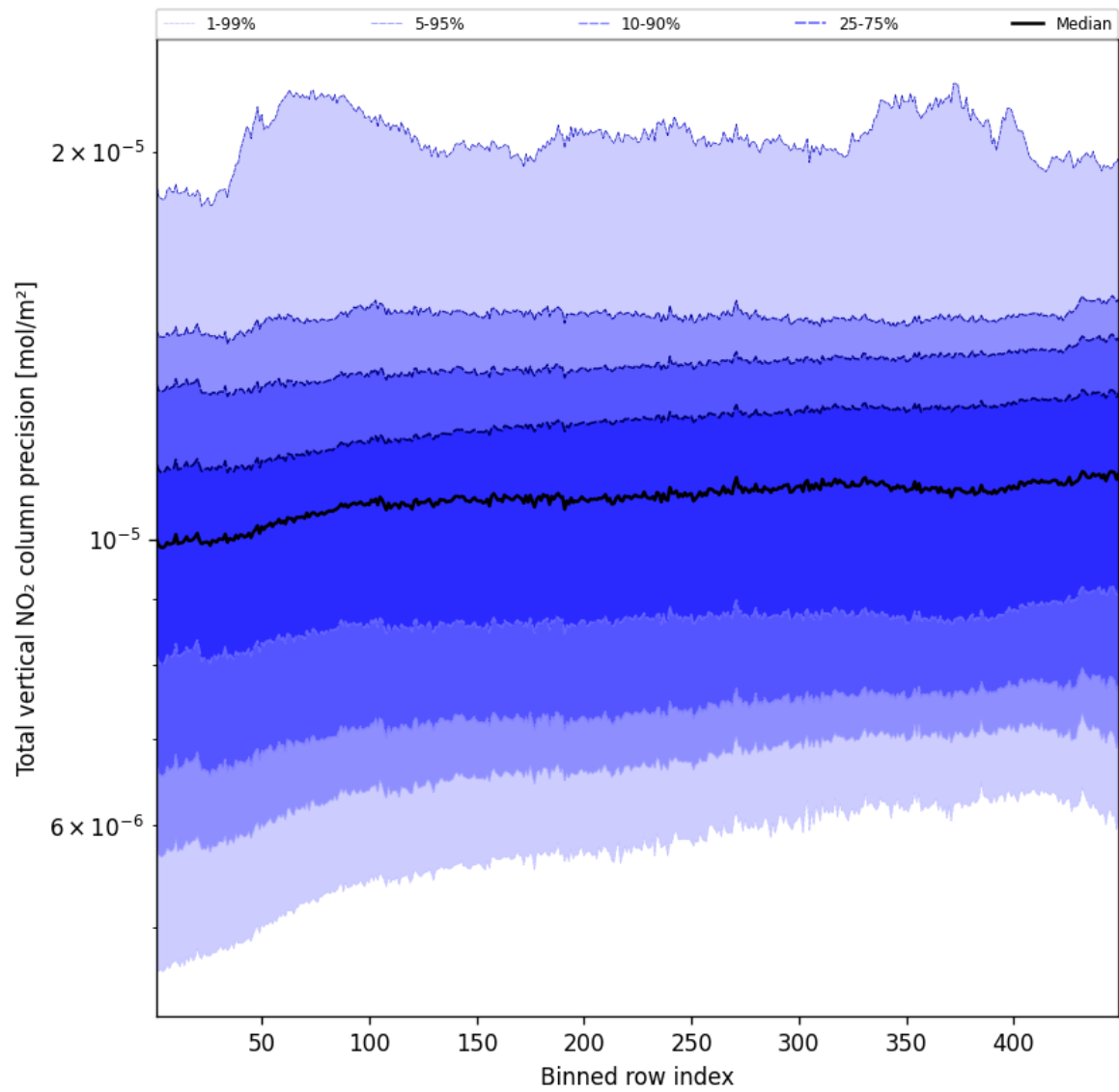
Figure 54: Along track statistics of “Total vertical NO 2 column precision” for 2025-04-19 to 2025-04-20
