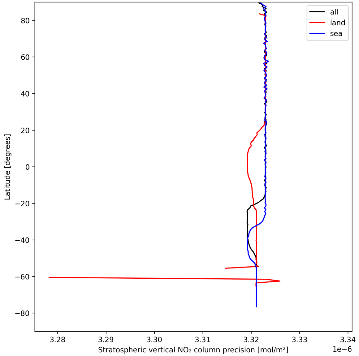
Figure 18: Zonal average of "Stratospheric vertical NO 2 column precision" for 2025-04-19 to 2025-04-20.
