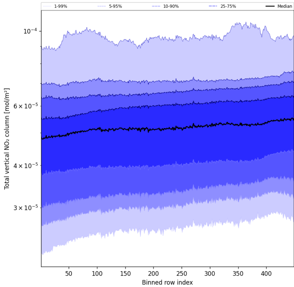
Figure 53: Along track statistics of “Total vertical NO 2 column” for 2025-04-19 to 2025-04-20
