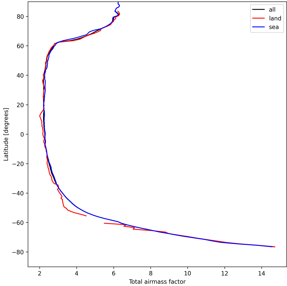
Figure 13: Zonal average of “Total airmass factor” for 2025-04-19 to 2025-04-20.
