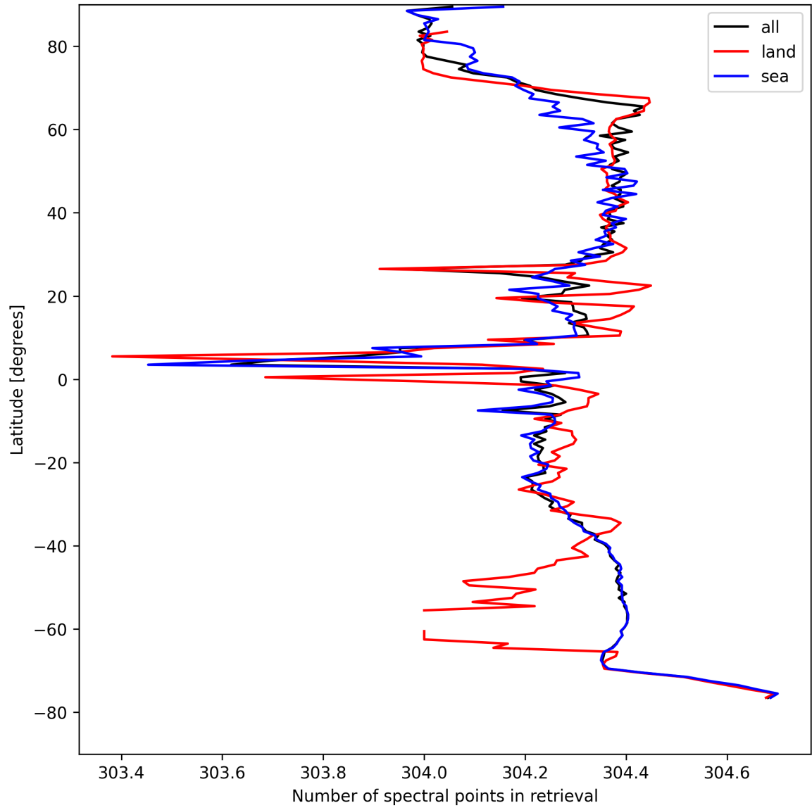
Figure 14: Zonal average of “Number of spectral points in retrieval” for 2025-04-19 to 2025-04-20.
