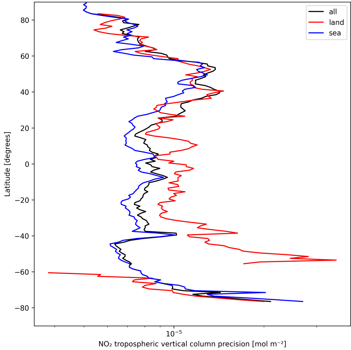
Figure 11: Zonal average of “NO 2 tropospheric vertical column precision” for 2025-04-19 to 2025-04-20.
