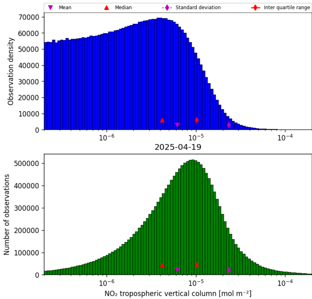
Figure 27: Histogram of “NO 2 tropospheric vertical column” for 2025-04-19 to 2025-04-20
