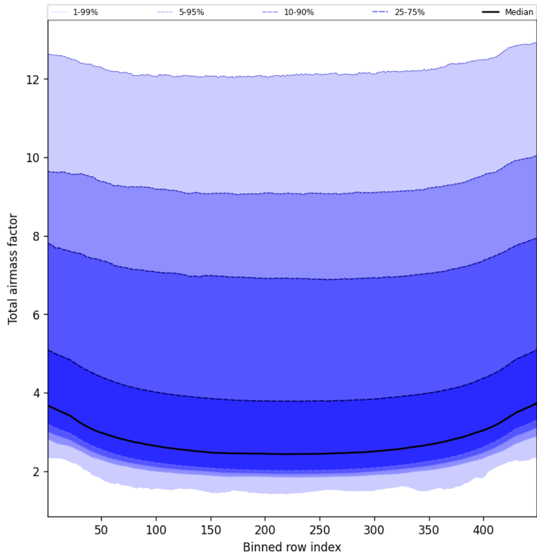
Figure 47: Along track statistics of “Total airmass factor” for 2025-04-19 to 2025-04-20
