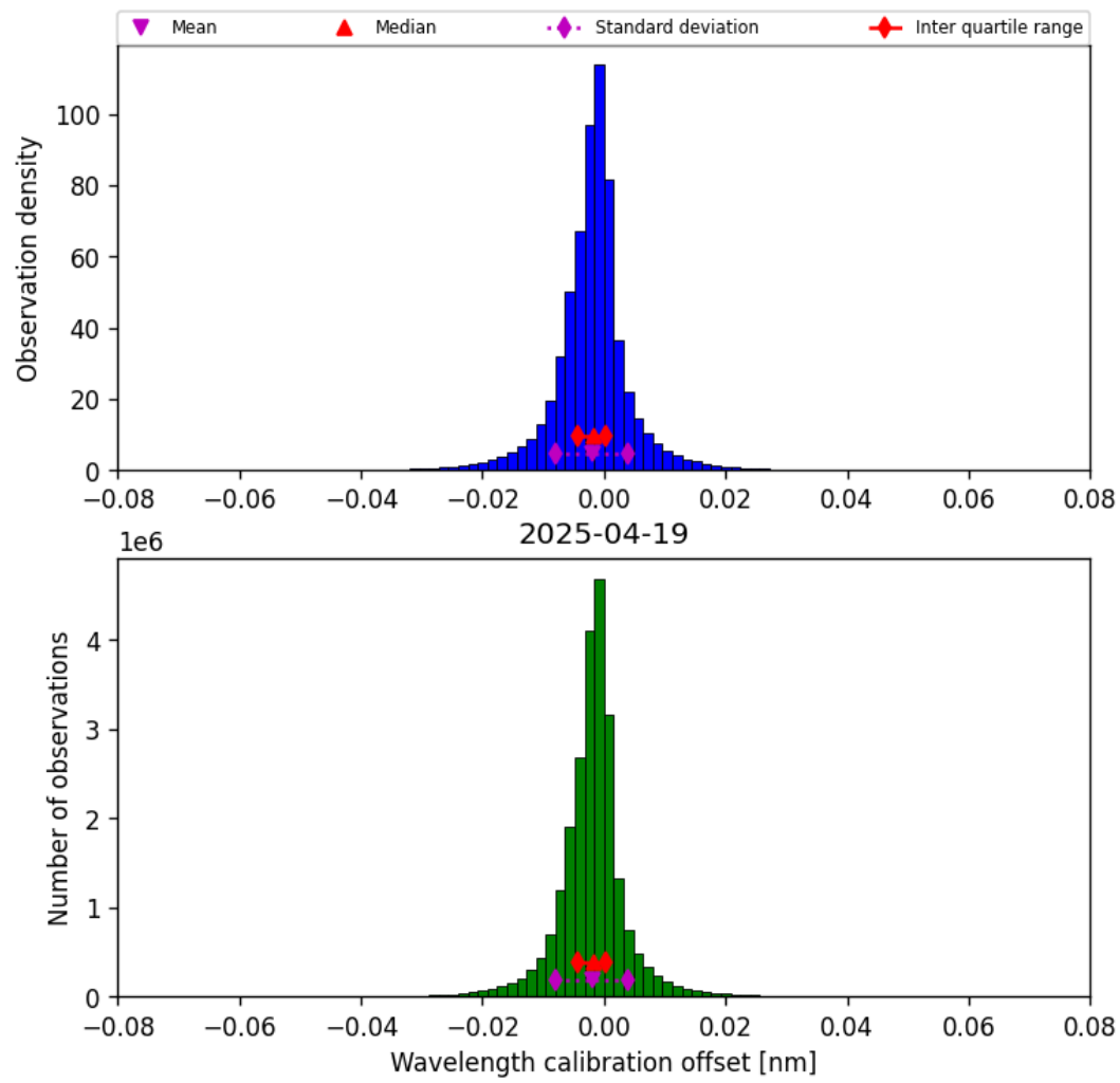
Figure 33: Histogram of “Wavelength calibration offset” for 2025-04-19 to 2025-04-20
