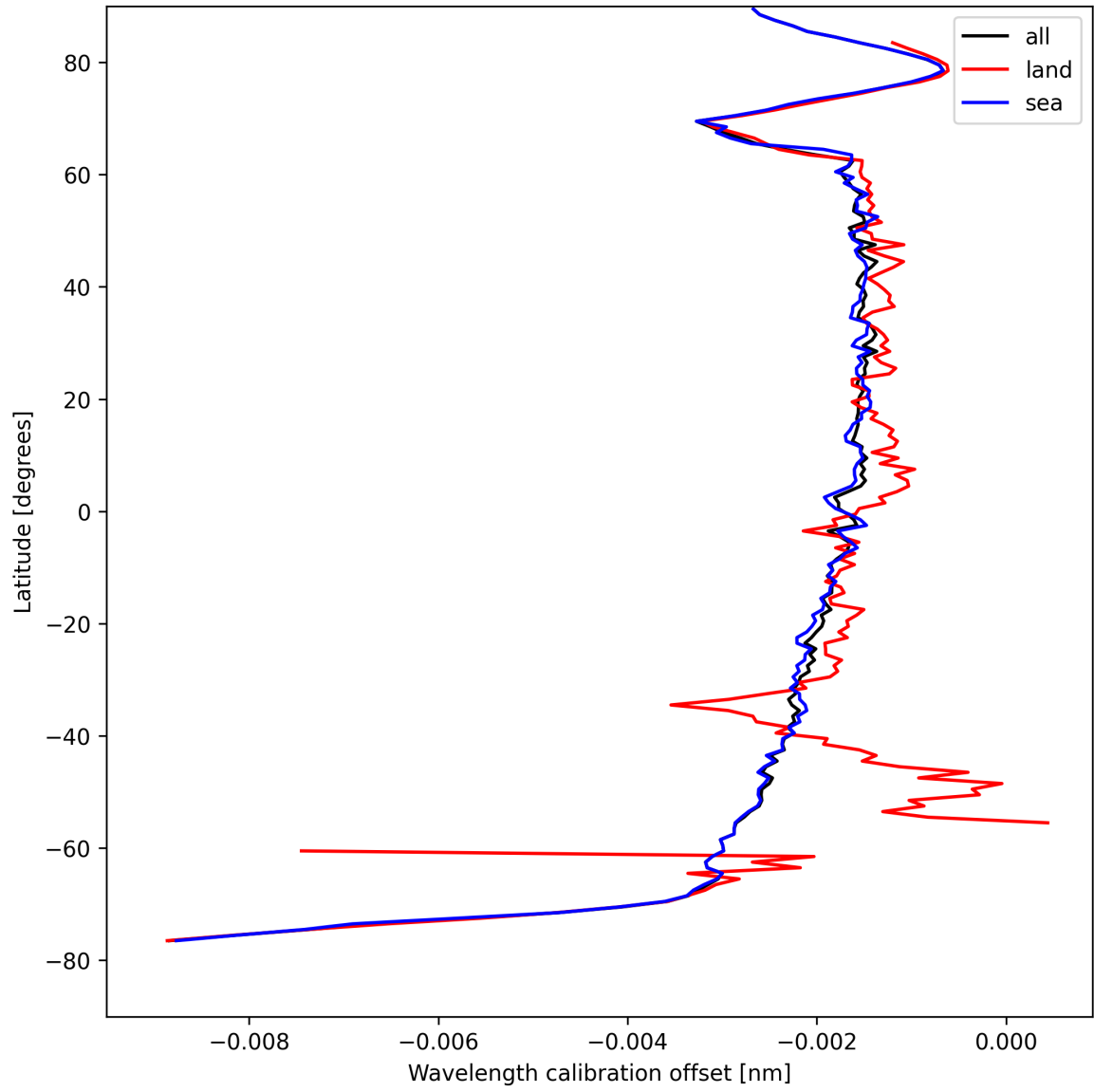
Figure 16: Zonal average of “Wavelength calibration offset” for 2025-04-19 to 2025-04-20.
