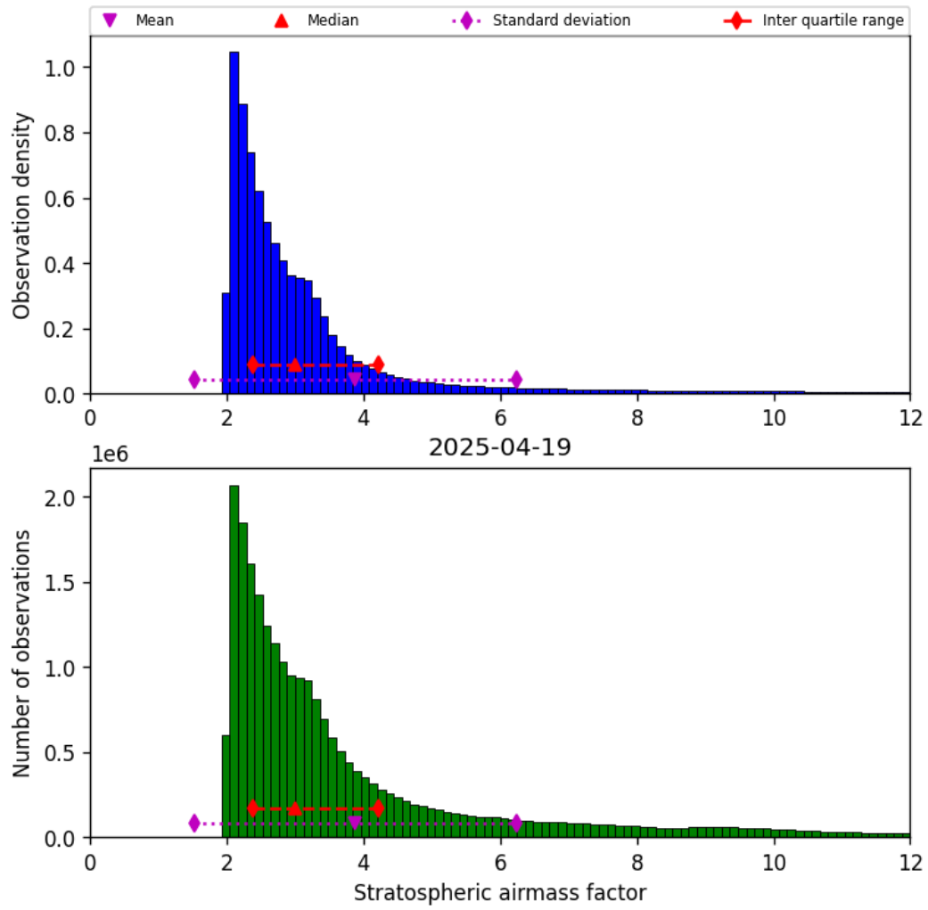
Figure 42: Histogram of “Stratospheric airmass factor” for 2025-04-19 to 2025-04-20
