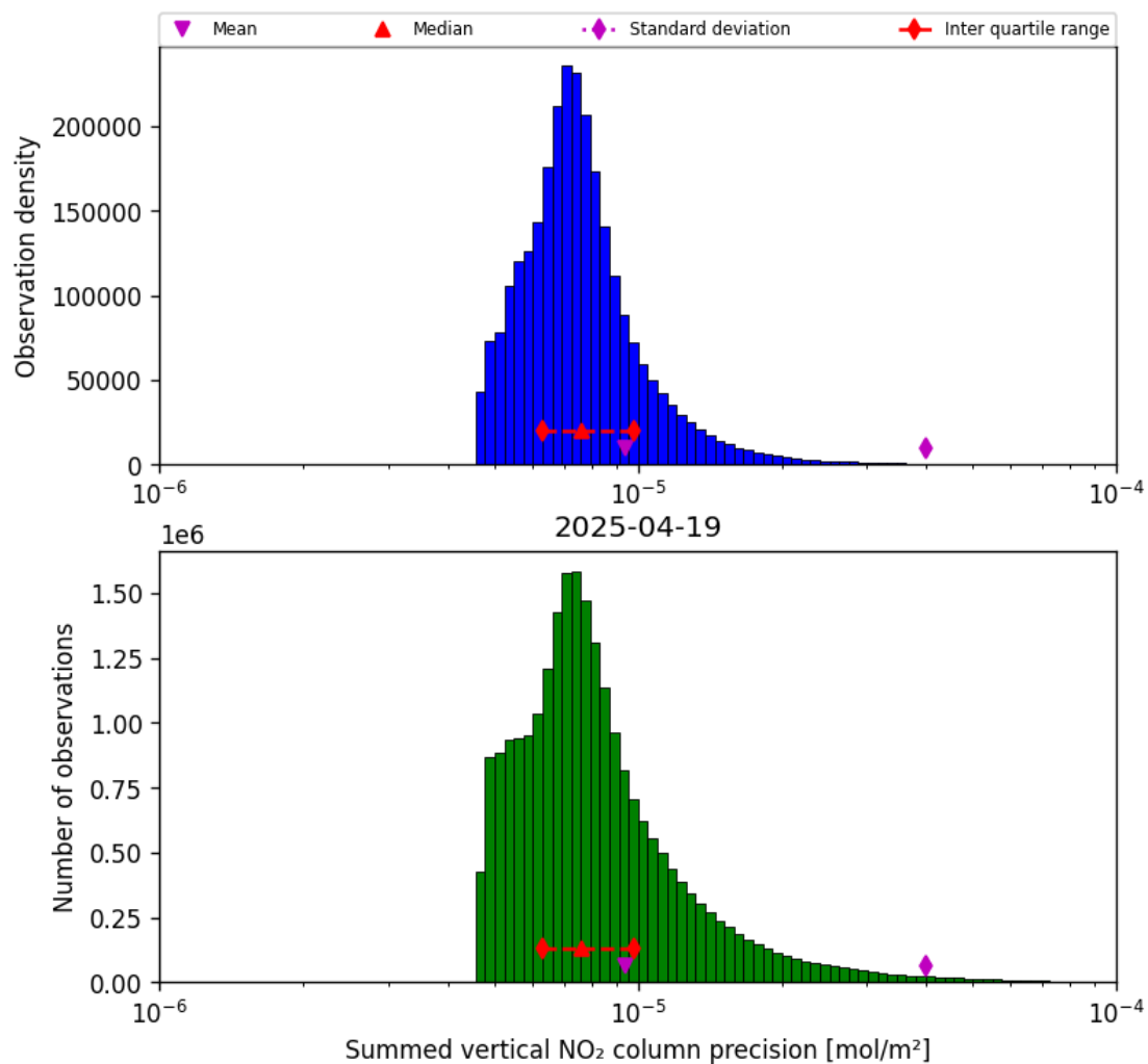
Figure 39: Histogram of “Summed vertical NO 2 column precision” for 2025-04-19 to 2025-04-20
