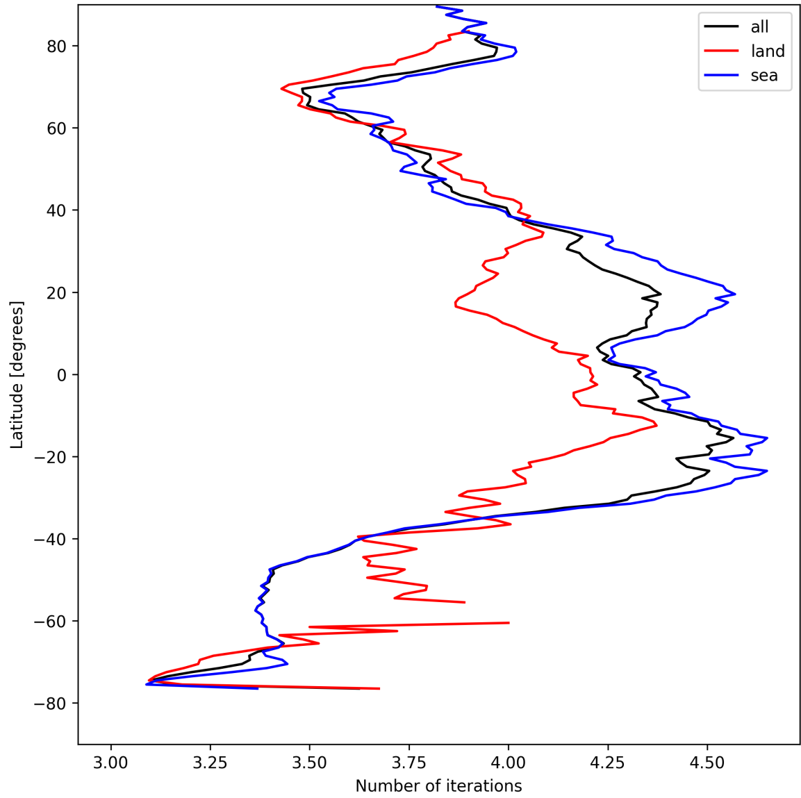
Figure 15: Zonal average of “Number of iterations” for 2025-04-19 to 2025-04-20.
