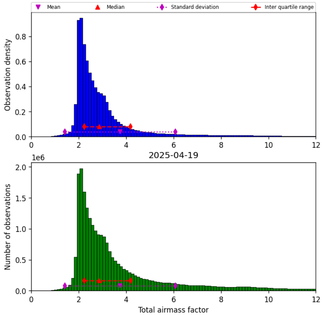
Figure 30: Histogram of “Total airmass factor” for 2025-04-19 to 2025-04-20
