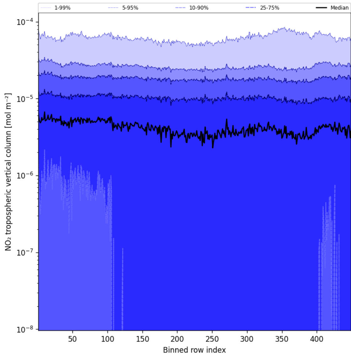
Figure 44: Along track statistics of “NO 2 tropospheric vertical column” for 2025-04-19 to 2025-04-20
