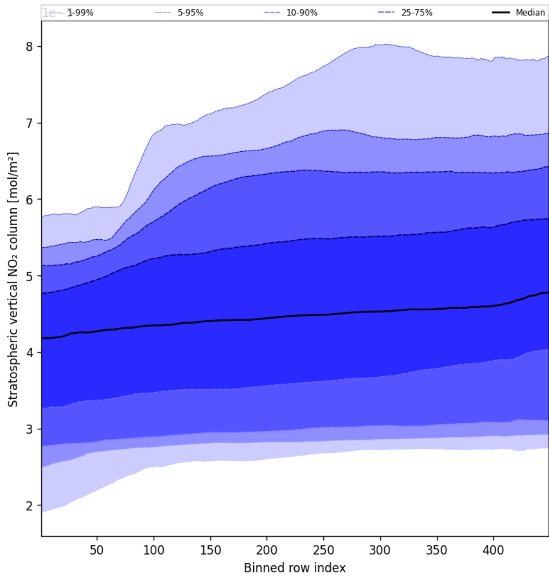
Figure 51: Along track statistics of “Stratospheric vertical NO 2 column” for 2025-04-19 to 2025-04-20
