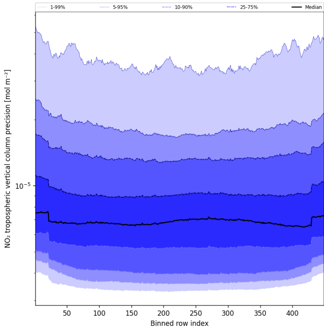
Figure 45: Along track statistics of “NO 2 tropospheric vertical column precision” for 2025-04-19 to 2025-04-20
