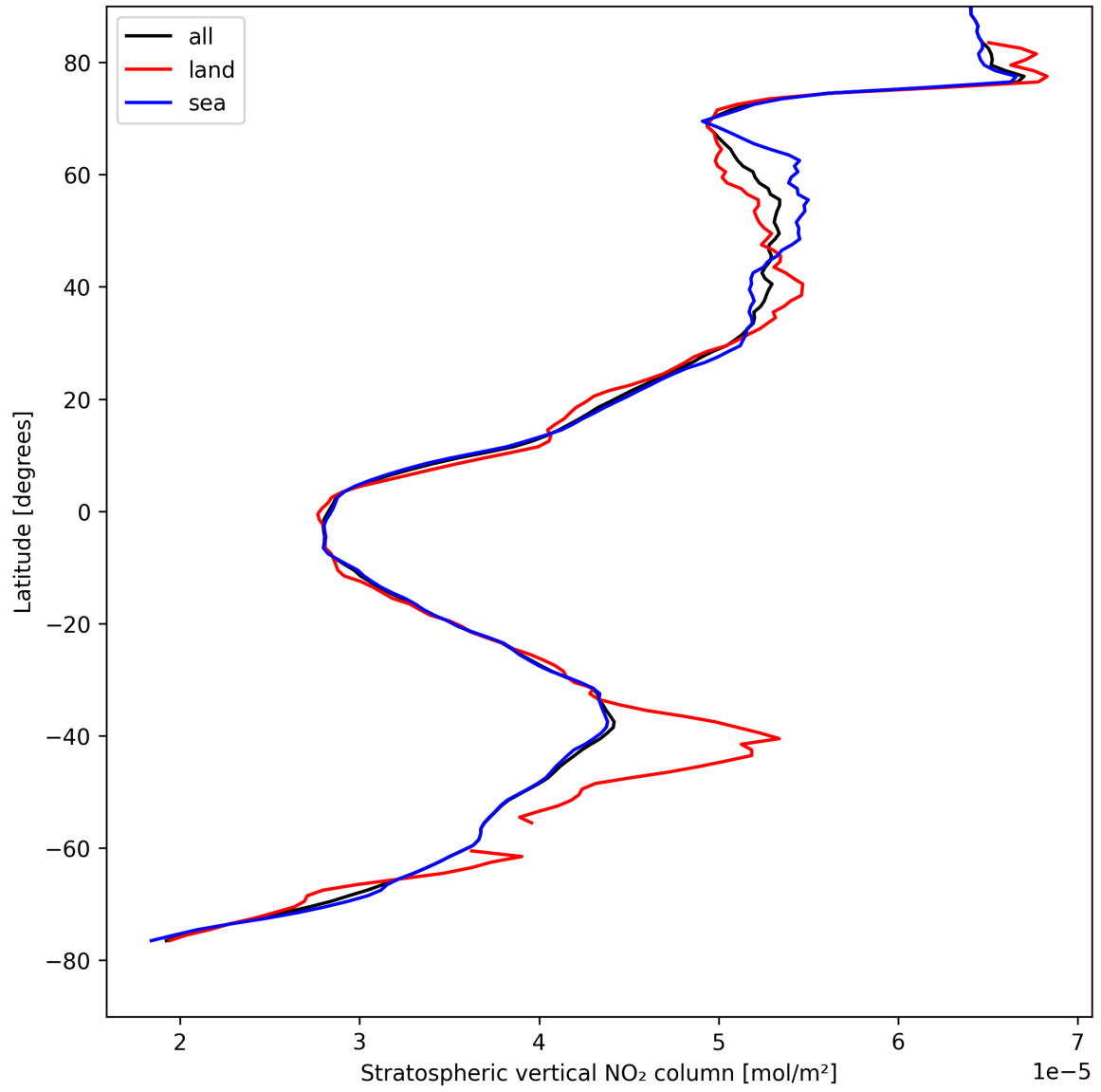
Figure 17: Zonal average of “Stratospheric vertical NO 2 column” for 2025-04-19 to 2025-04-20.
