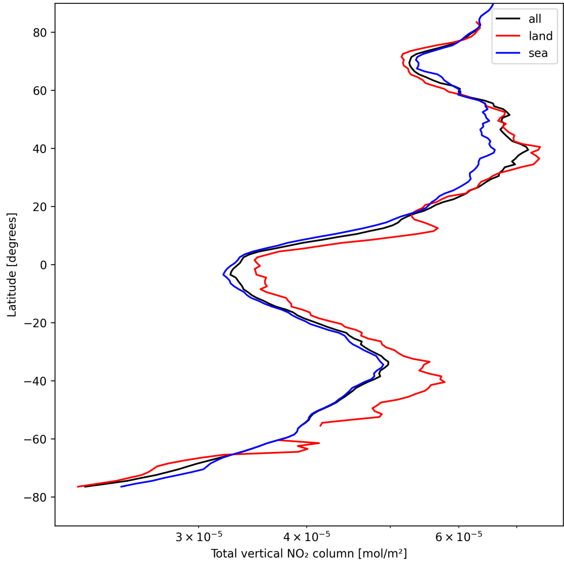
Figure 19: Zonal average of “Total vertical NO 2 column” for 2025-04-19 to 2025-04-20.
