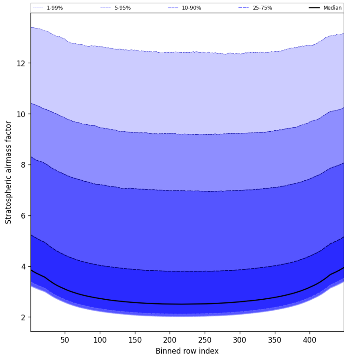
Figure 59: Along track statistics of “Stratospheric airmass factor” for 2025-04-19 to 2025-04-20
