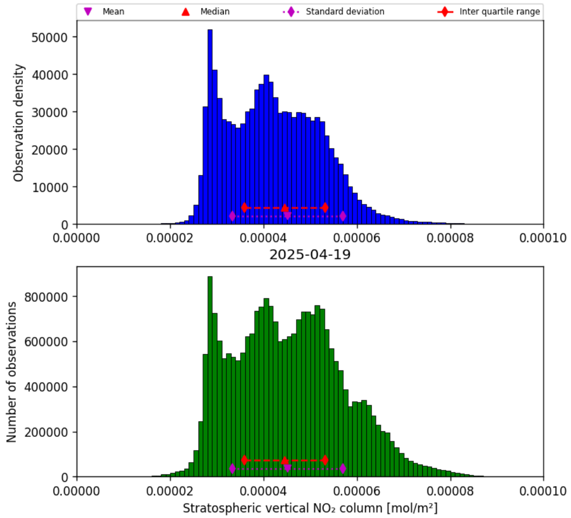
Figure 34: Histogram of “Stratospheric vertical NO 2 column” for 2025-04-19 to 2025-04-20
