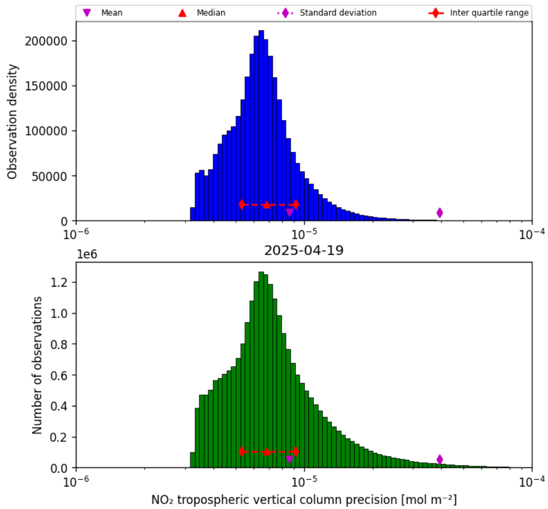
Figure 28: Histogram of “NO 2 tropospheric vertical column precision” for 2025-04-19 to 2025-04-20
