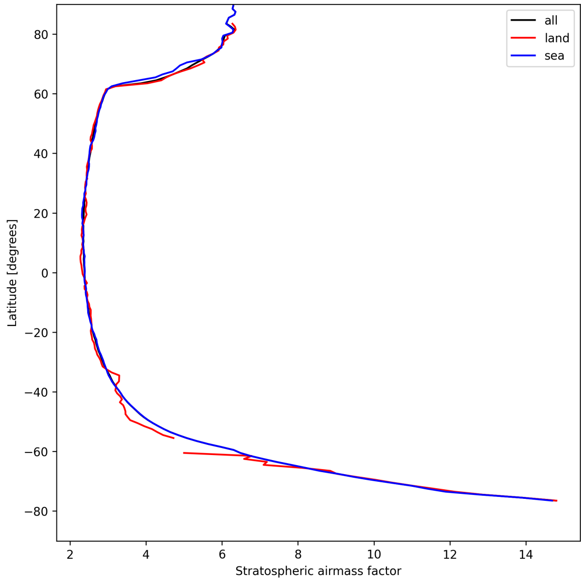
Figure 25: Zonal average of “Stratospheric airmass factor” for 2025-04-19 to 2025-04-20.
