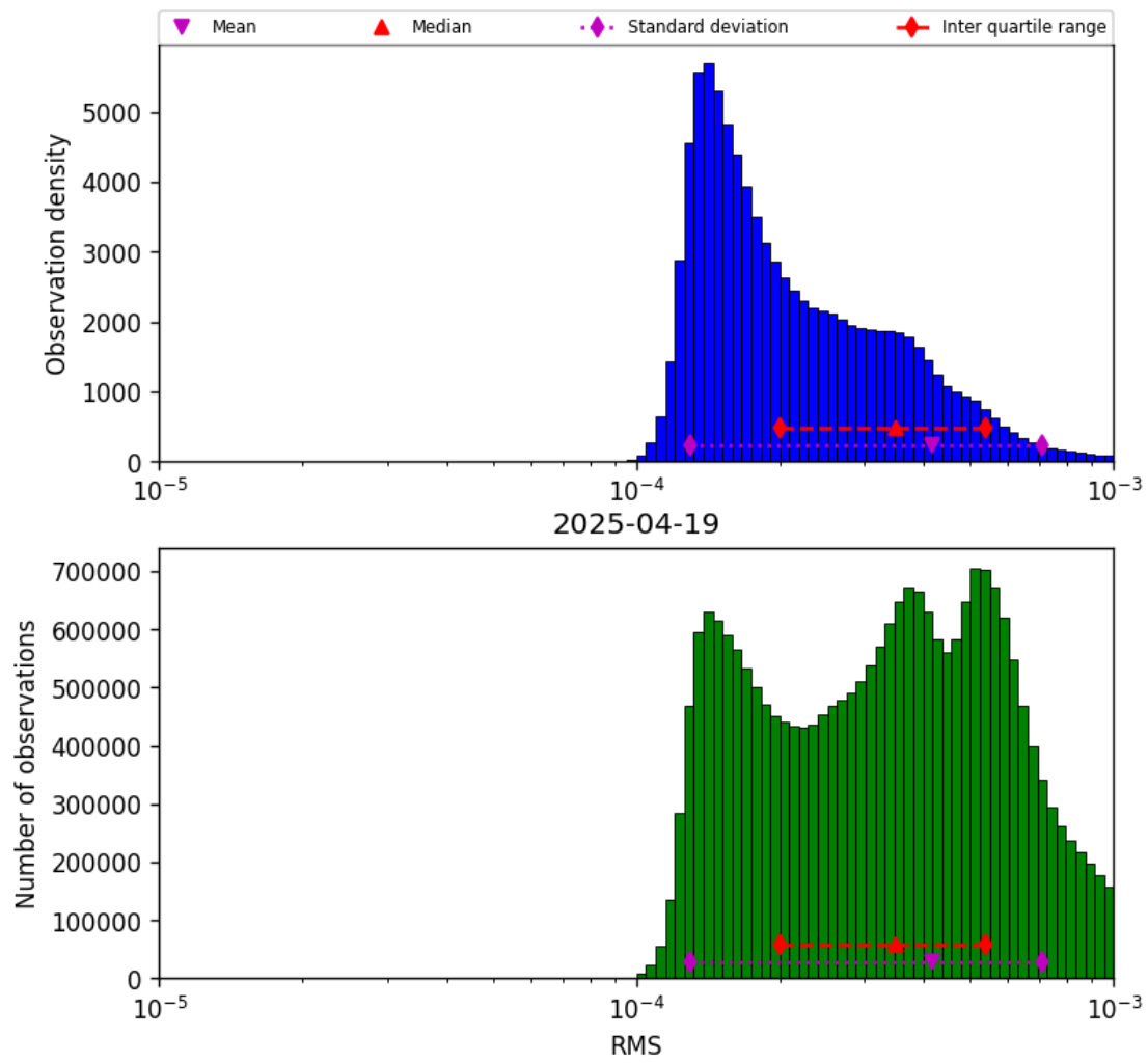
Figure 41: Histogram of “RMS” for 2025-04-19 to 2025-04-20
