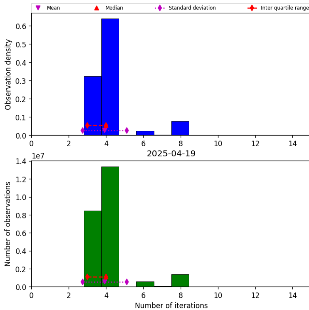
Figure 32: Histogram of “Number of iterations” for 2025-04-19 to 2025-04-20
