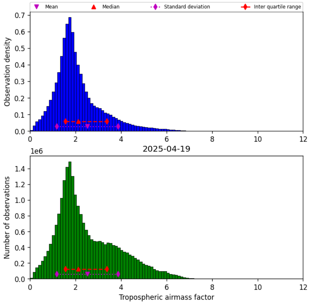
Figure 29: Histogram of “Tropospheric airmass factor” for 2025-04-19 to 2025-04-20
