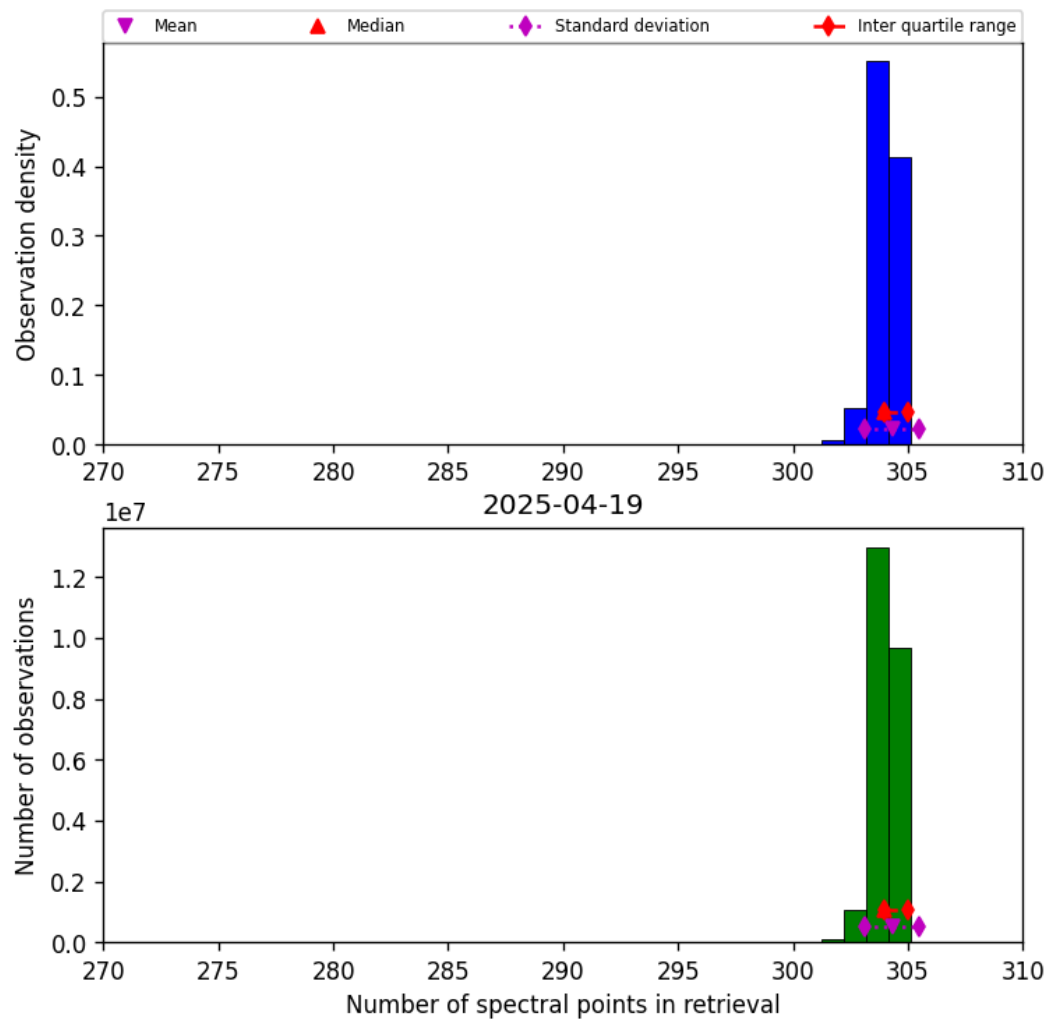
Figure 31: Histogram of “Number of spectral points in retrieval” for 2025-04-19 to 2025-04-20
