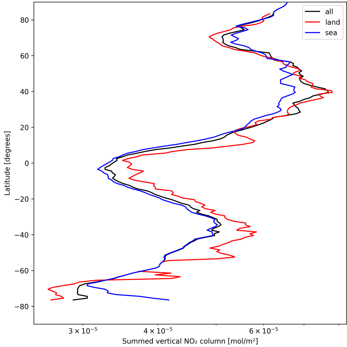
Figure 21: Zonal average of “Summed vertical NO 2 column” for 2025-04-19 to 2025-04-20.
