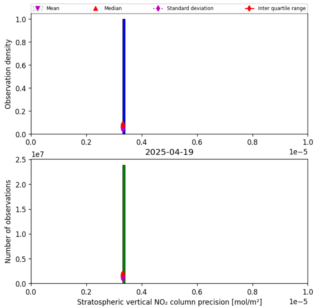
Figure 35: Histogram of “Stratospheric vertical NO 2 column precision” for 2025-04-19 to 2025-04-20
