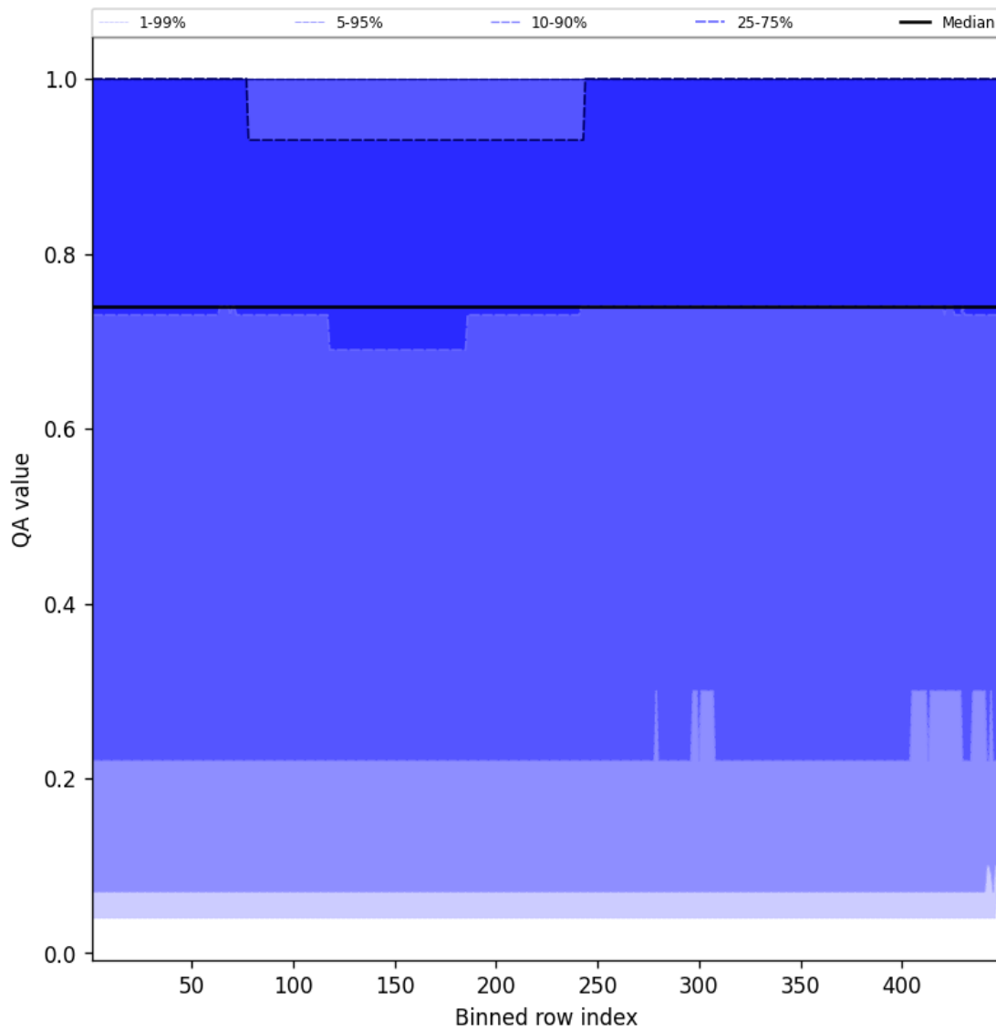
Figure 43: Along track statistics of "QA value" for 2025-04-19 to 2025-04-20
