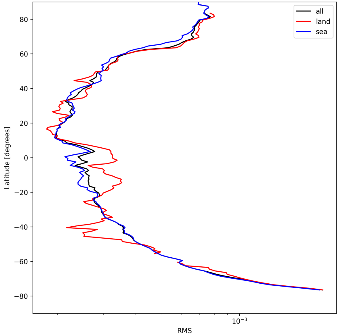
Figure 24: Zonal average of “RMS” for 2025-04-19 to 2025-04-20.
