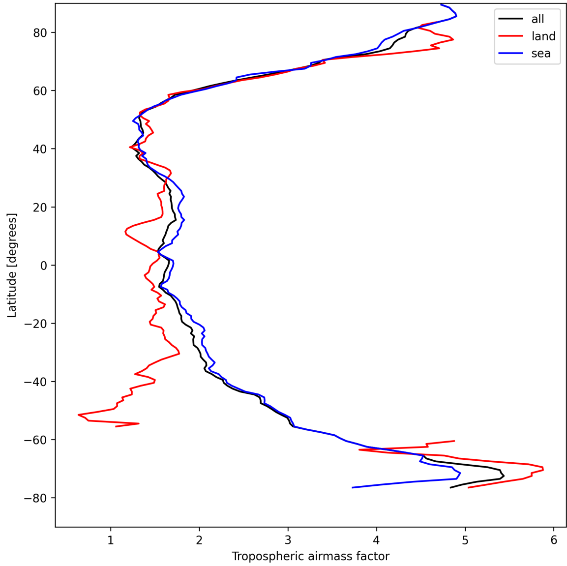
Figure 12: Zonal average of “Tropospheric airmass factor” for 2025-04-19 to 2025-04-20.
