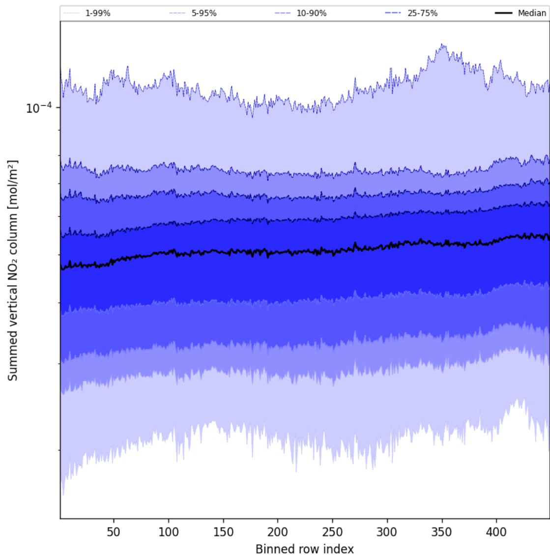
Figure 55: Along track statistics of “Summed vertical NO 2 column” for 2025-04-19 to 2025-04-20
