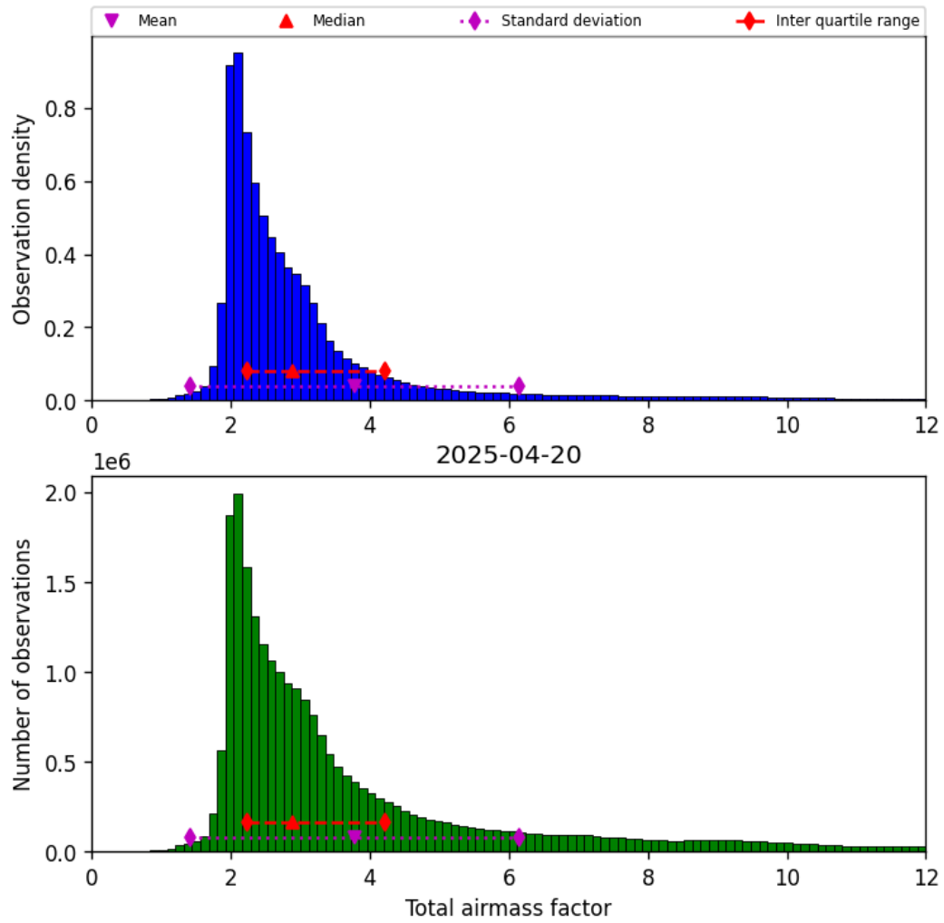
Figure 30: Histogram of “Total airmass factor” for 2025-04-20 to 2025-04-21
