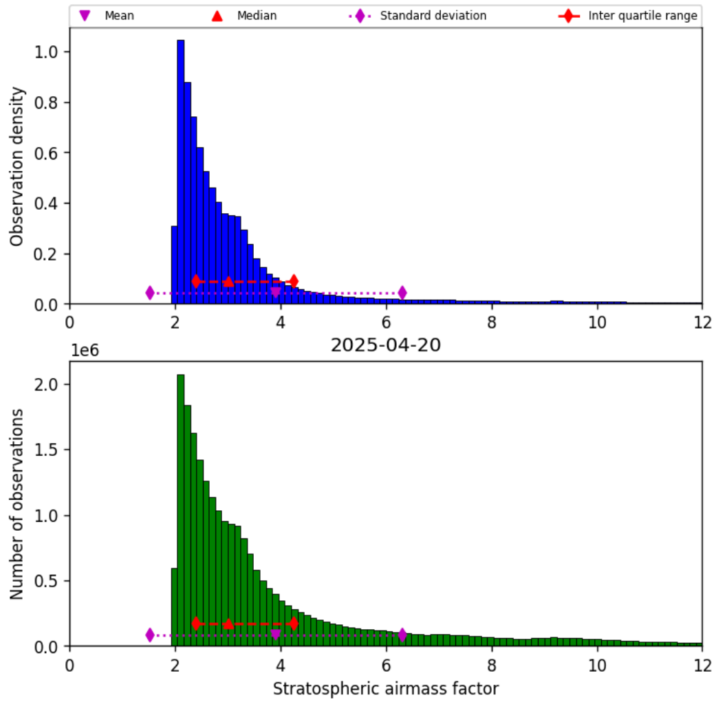
Figure 42: Histogram of “Stratospheric airmass factor” for 2025-04-20 to 2025-04-21
