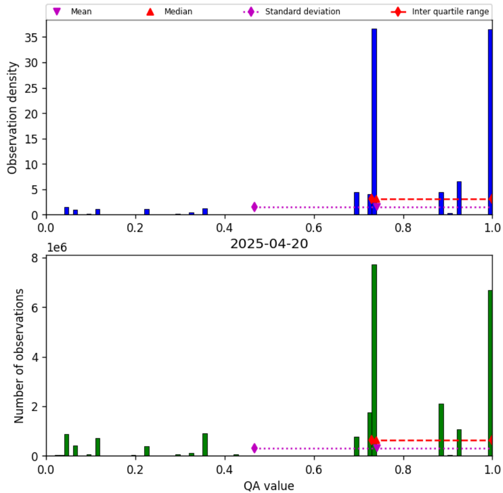
Figure 26: Histogram of “QA value” for 2025-04-20 to 2025-04-21
