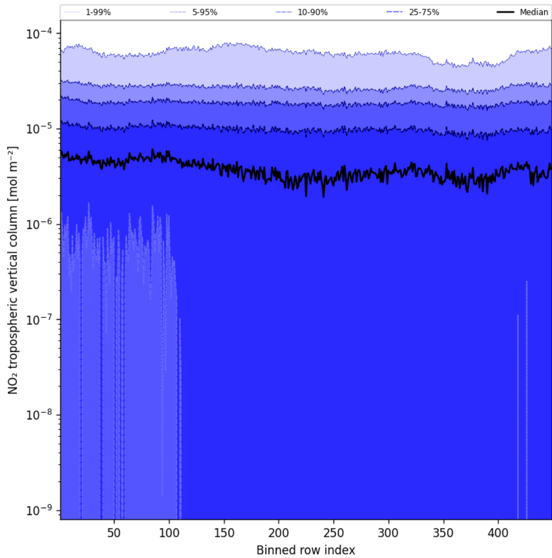
Figure 44: Along track statistics of “NO 2 tropospheric vertical column” for 2025-04-20 to 2025-04-21
