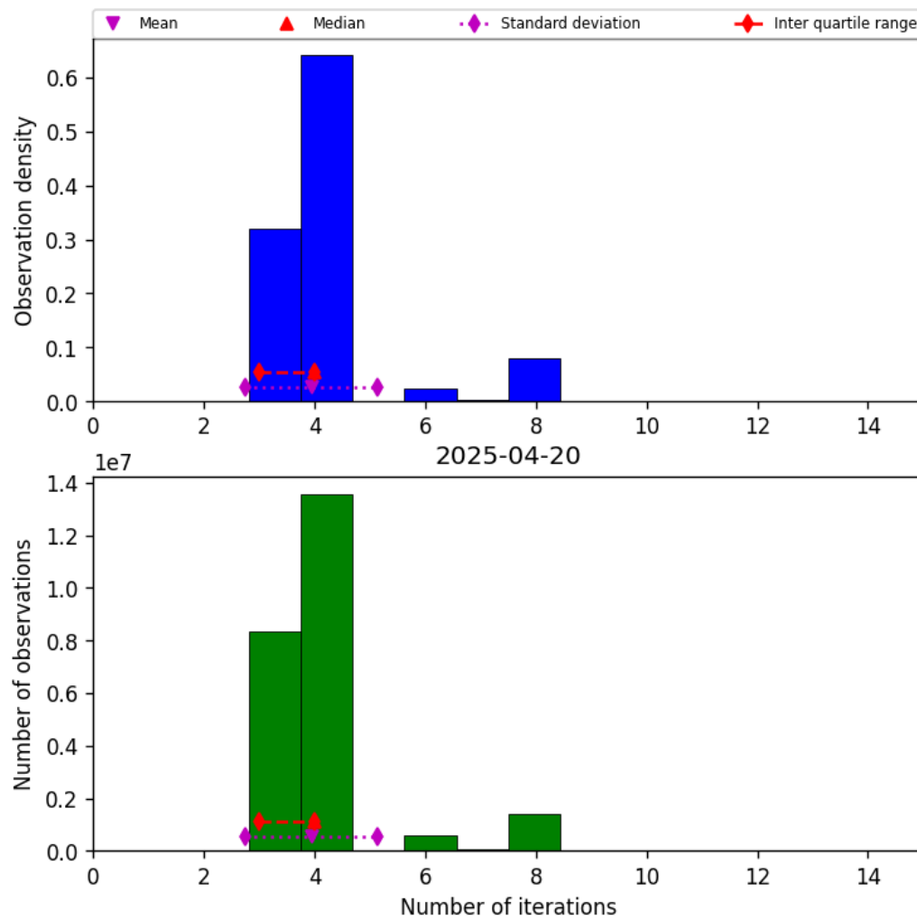
Figure 32: Histogram of “Number of iterations” for 2025-04-20 to 2025-04-21
