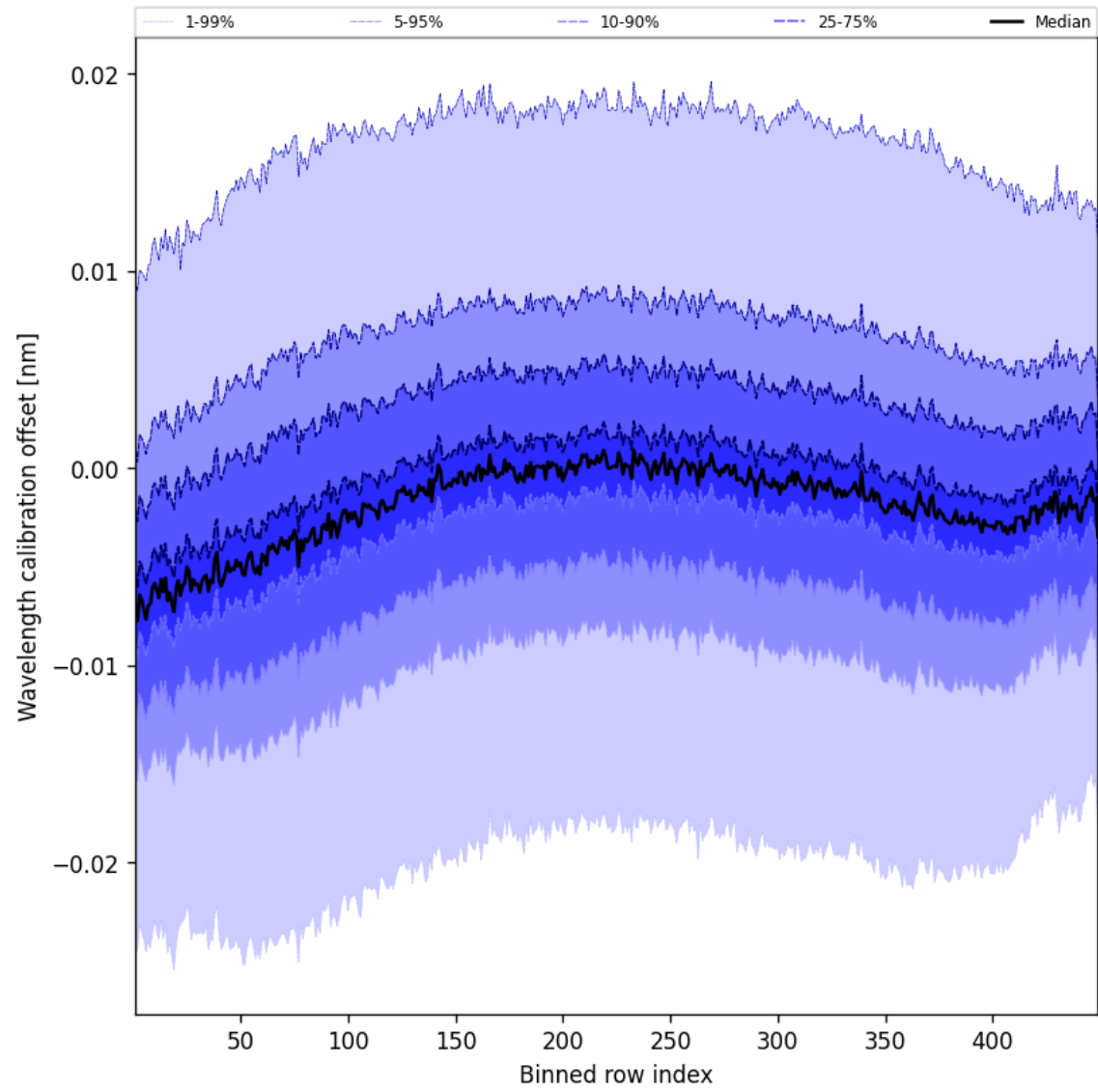
Figure 50: Along track statistics of “Wavelength calibration offset” for 2025-04-20 to 2025-04-21
