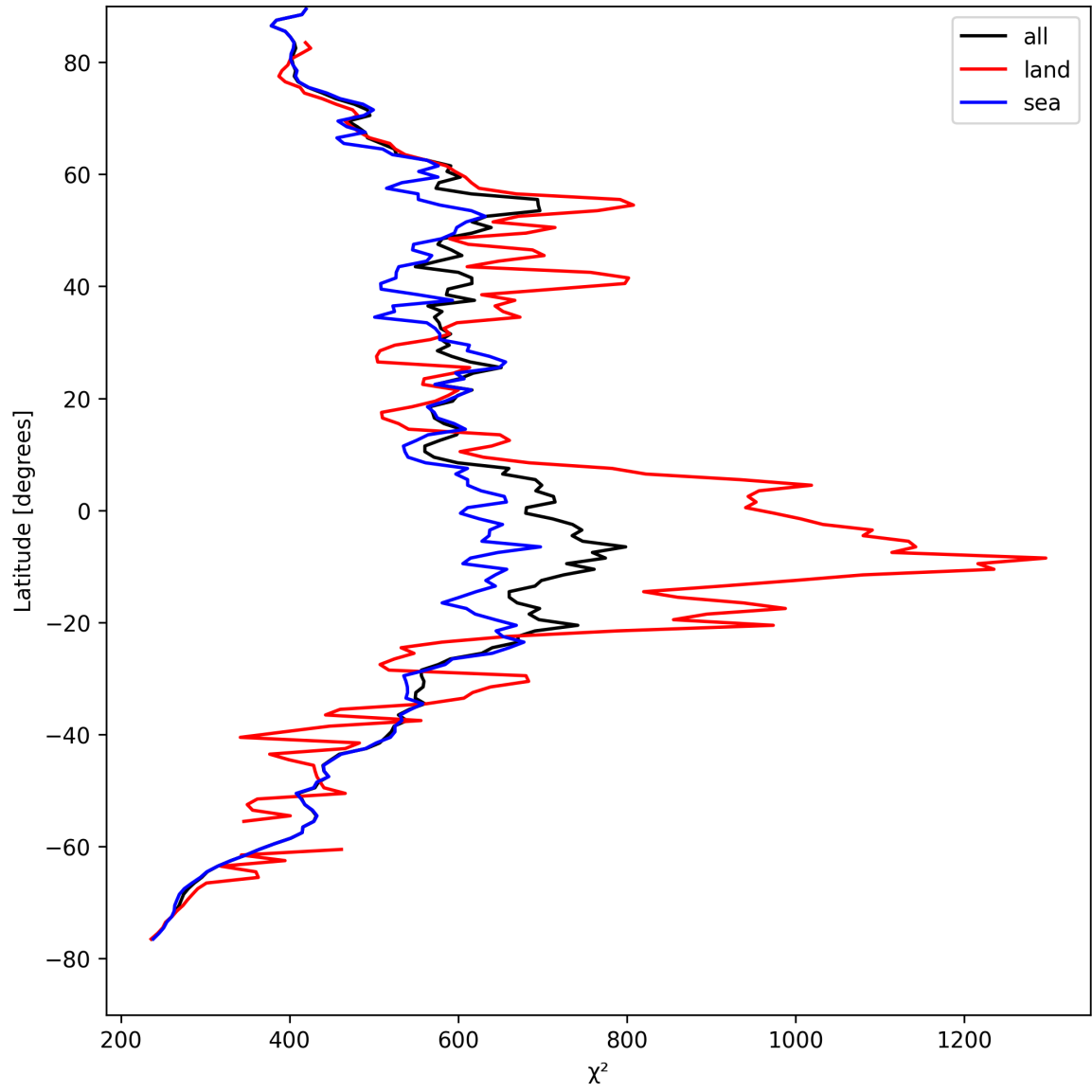
Figure 23: Zonal average of “ \chi^2 ” for 2025-04-20 to 2025-04-21.
