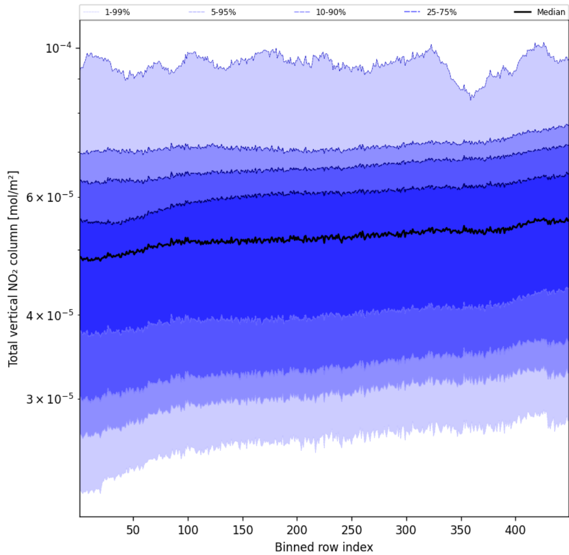
Figure 53: Along track statistics of “Total vertical NO 2 column” for 2025-04-20 to 2025-04-21
