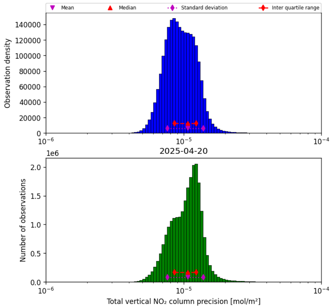
Figure 37: Histogram of “Total vertical NO 2 column precision” for 2025-04-20 to 2025-04-21
