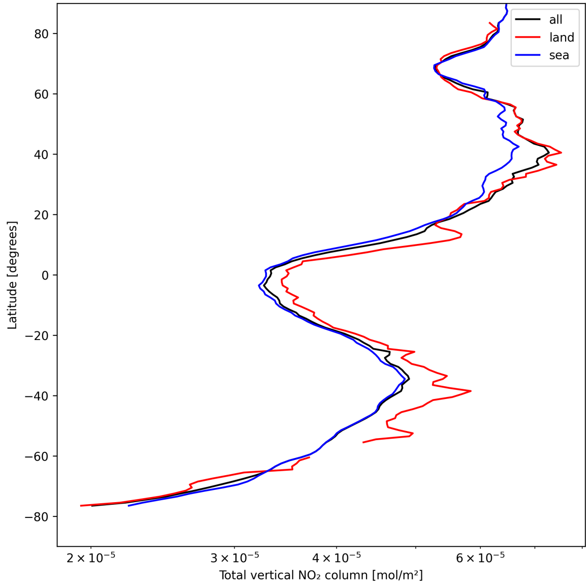
Figure 19: Zonal average of “Total vertical NO 2 column” for 2025-04-20 to 2025-04-21.
