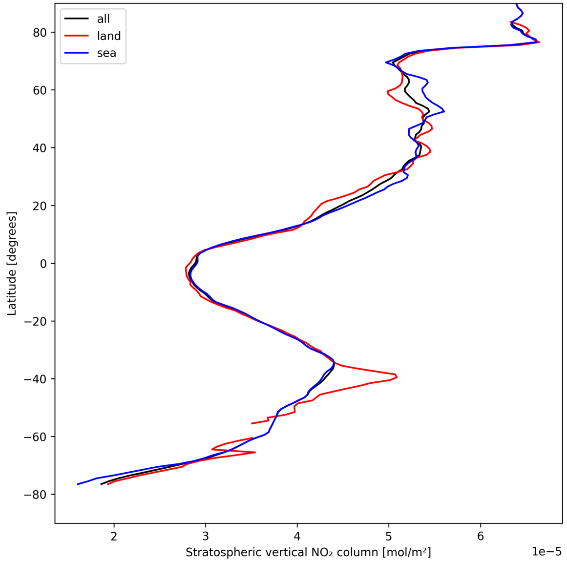
Figure 17: Zonal average of “Stratospheric vertical NO 2 column” for 2025-04-20 to 2025-04-21.
