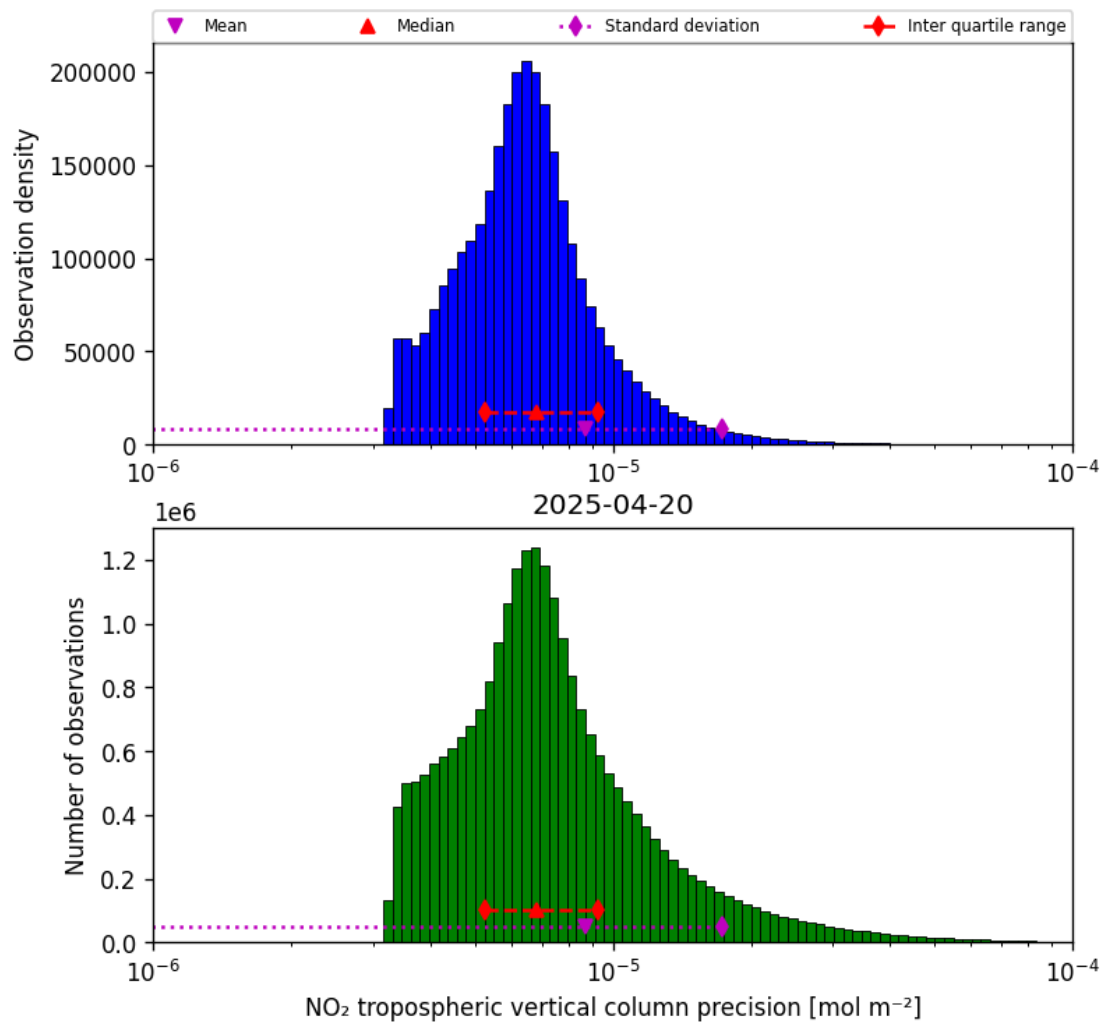
Figure 28: Histogram of “NO 2 tropospheric vertical column precision” for 2025-04-20 to 2025-04-21
