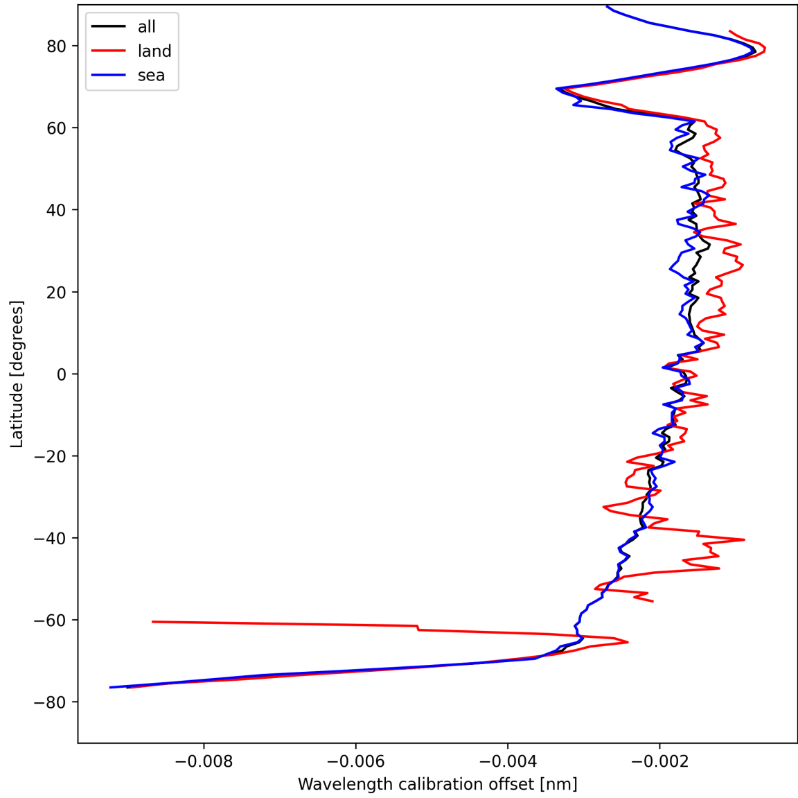
Figure 16: Zonal average of “Wavelength calibration offset” for 2025-04-20 to 2025-04-21.
