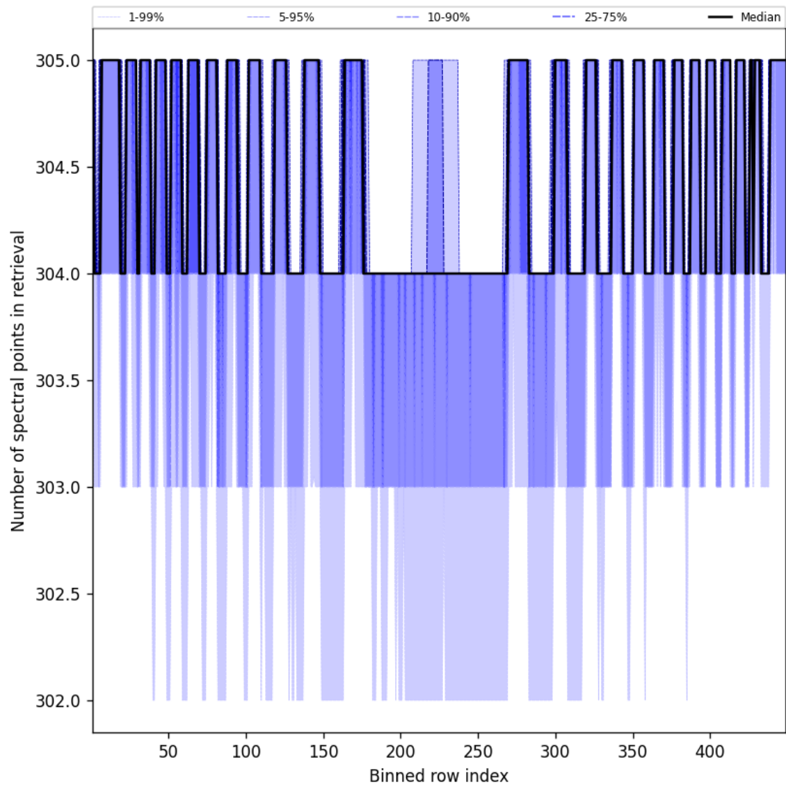
Figure 48: Along track statistics of “Number of spectral points in retrieval” for 2025-04-20 to 2025-04-21
