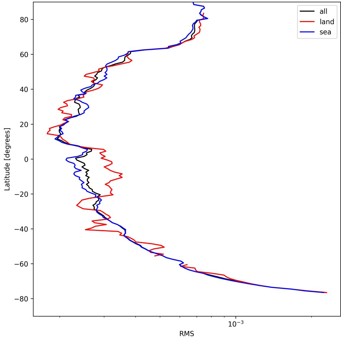
Figure 24: Zonal average of “RMS” for 2025-04-20 to 2025-04-21.
