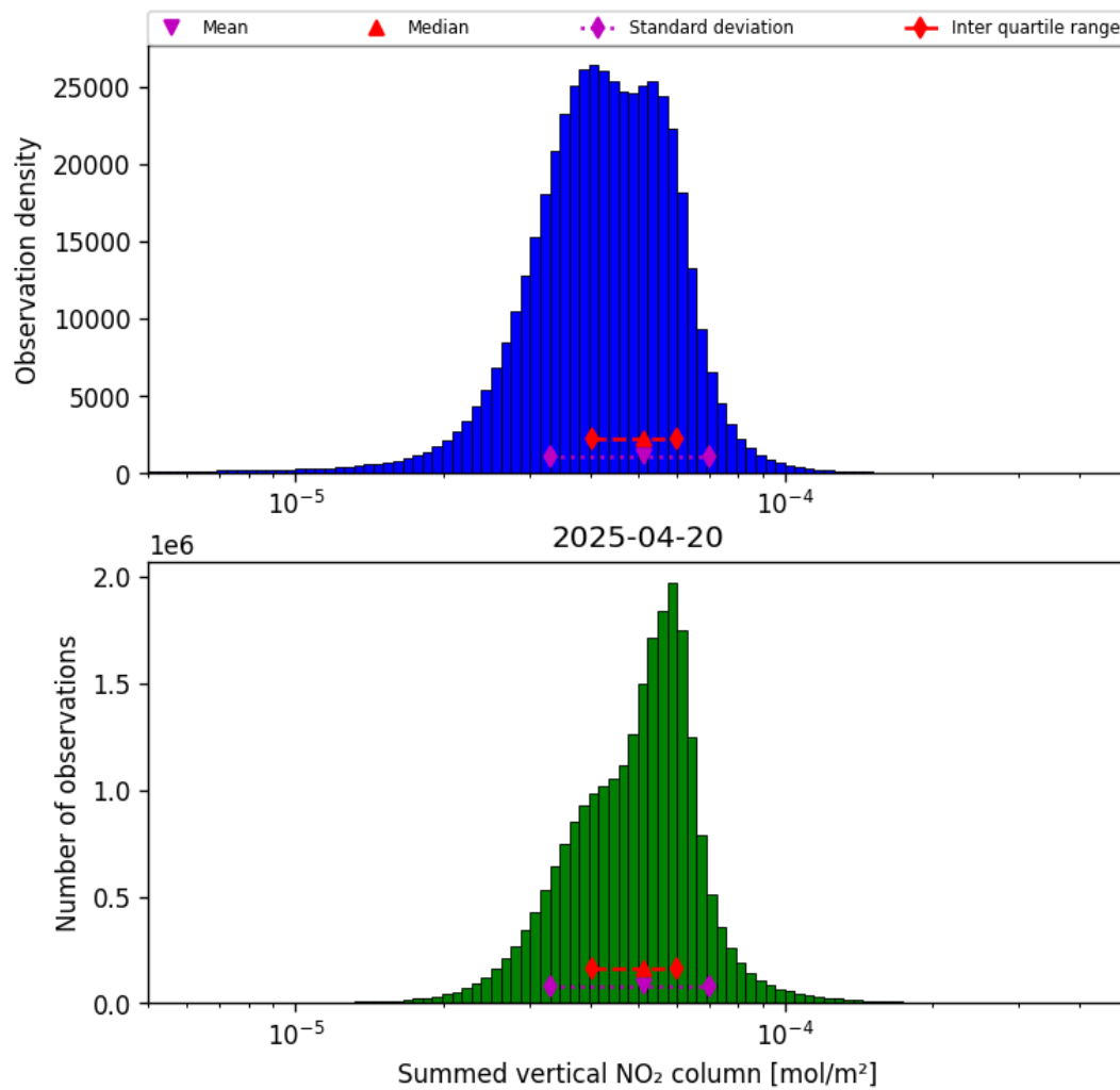
Figure 38: Histogram of “Summed vertical NO 2 column” for 2025-04-20 to 2025-04-21
