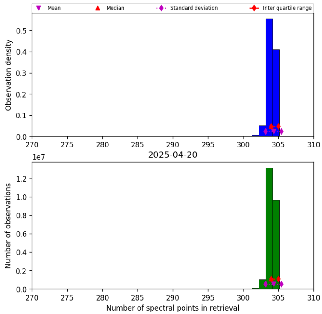
Figure 31: Histogram of “Number of spectral points in retrieval” for 2025-04-20 to 2025-04-21
