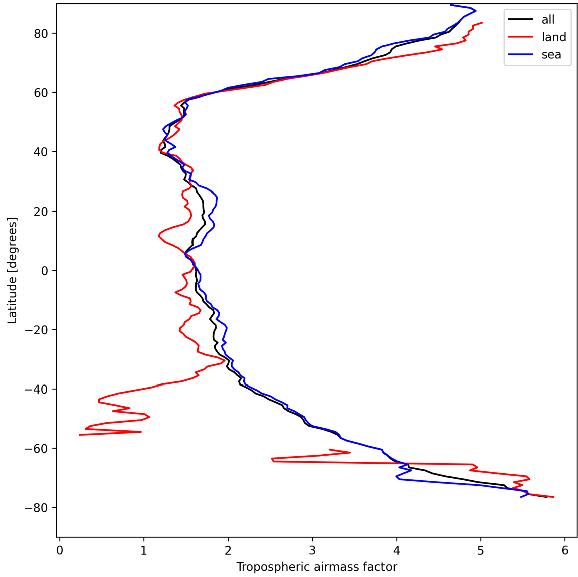
Figure 12: Zonal average of “Tropospheric airmass factor” for 2025-04-20 to 2025-04-21.
