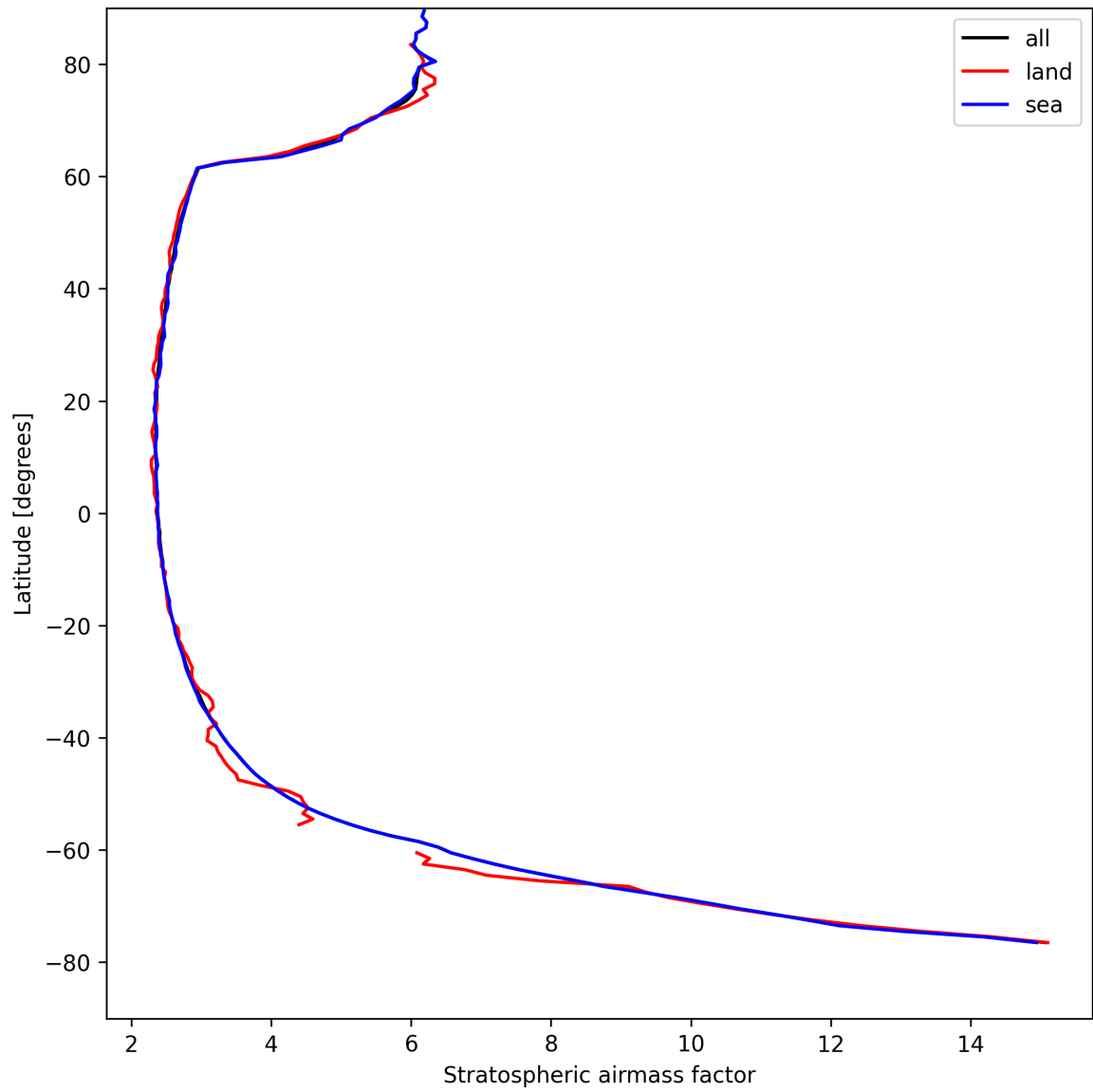
Figure 25: Zonal average of “Stratospheric airmass factor” for 2025-04-20 to 2025-04-21.
