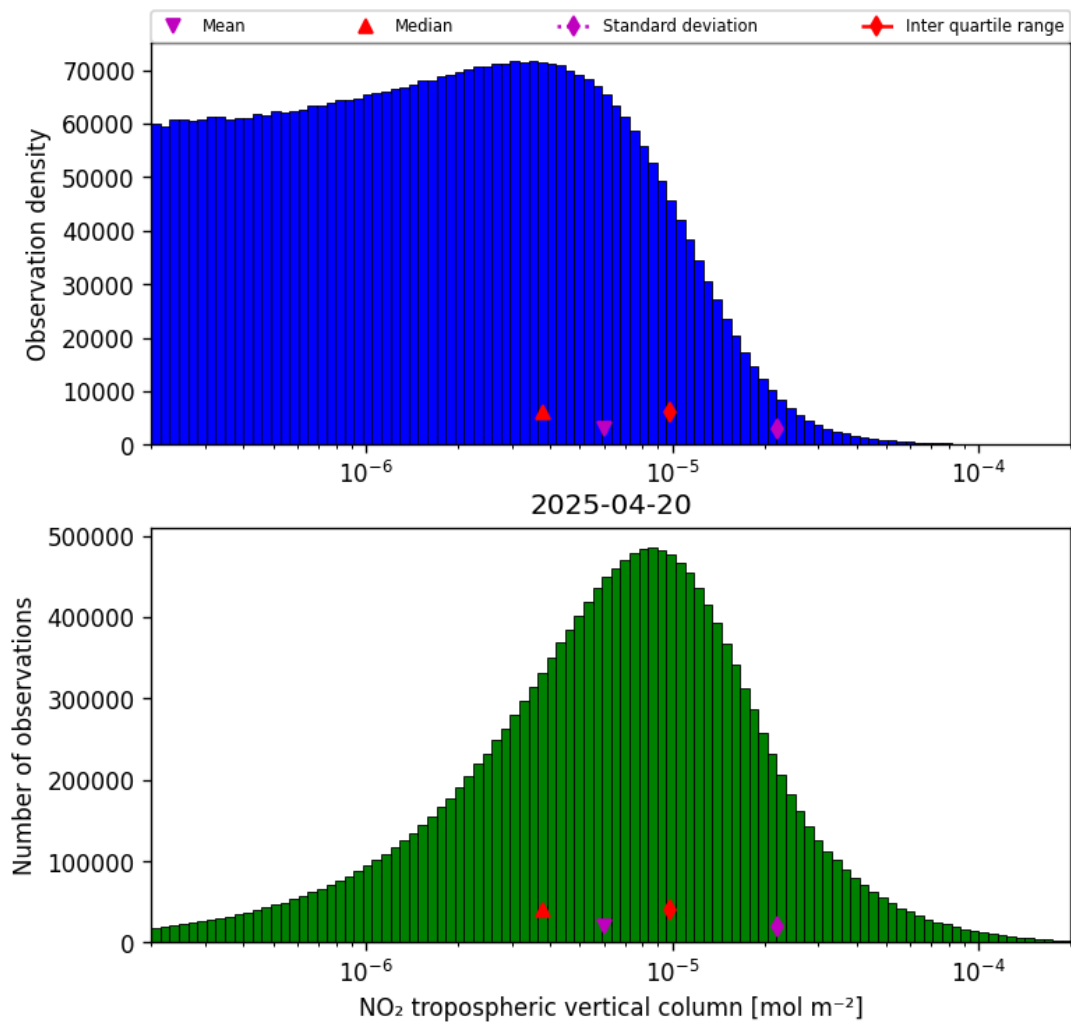
Figure 27: Histogram of “NO 2 tropospheric vertical column” for 2025-04-20 to 2025-04-21
