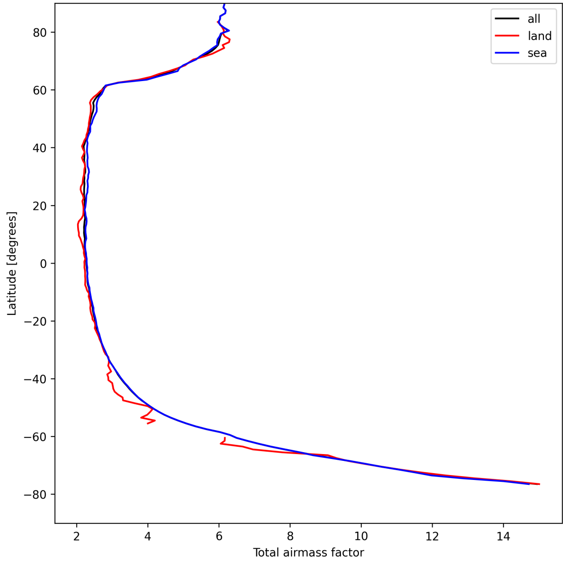
Figure 13: Zonal average of “Total airmass factor” for 2025-04-20 to 2025-04-21.
