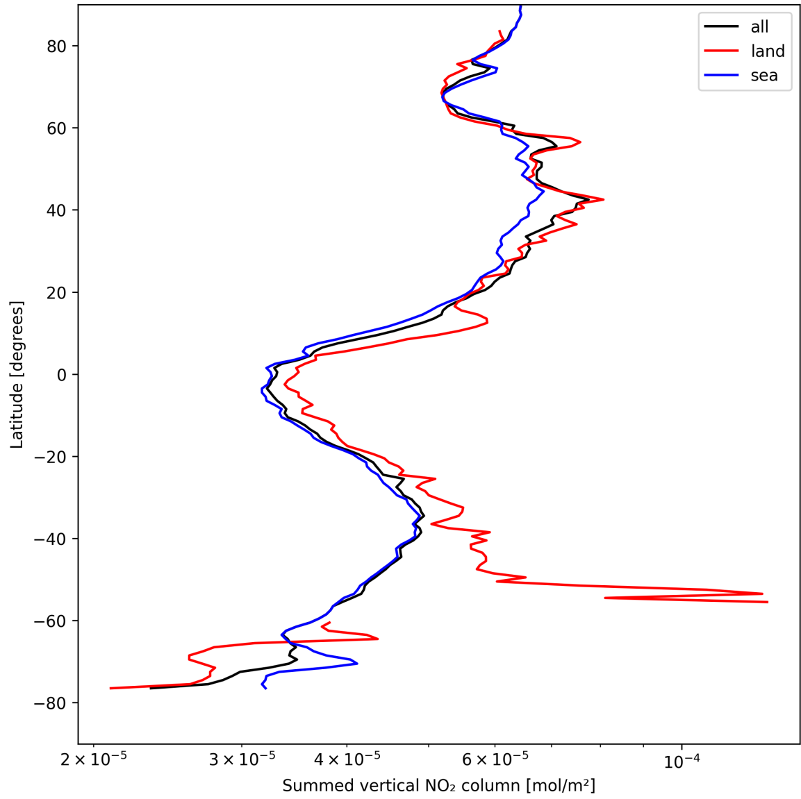
Figure 21: Zonal average of “Summed vertical NO 2 column” for 2025-04-20 to 2025-04-21.
