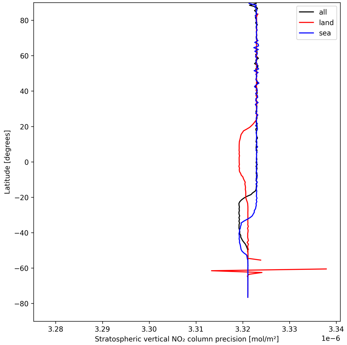
Figure 18: Zonal average of “Stratospheric vertical NO 2 column precision” for 2025-04-20 to 2025-04-21.
