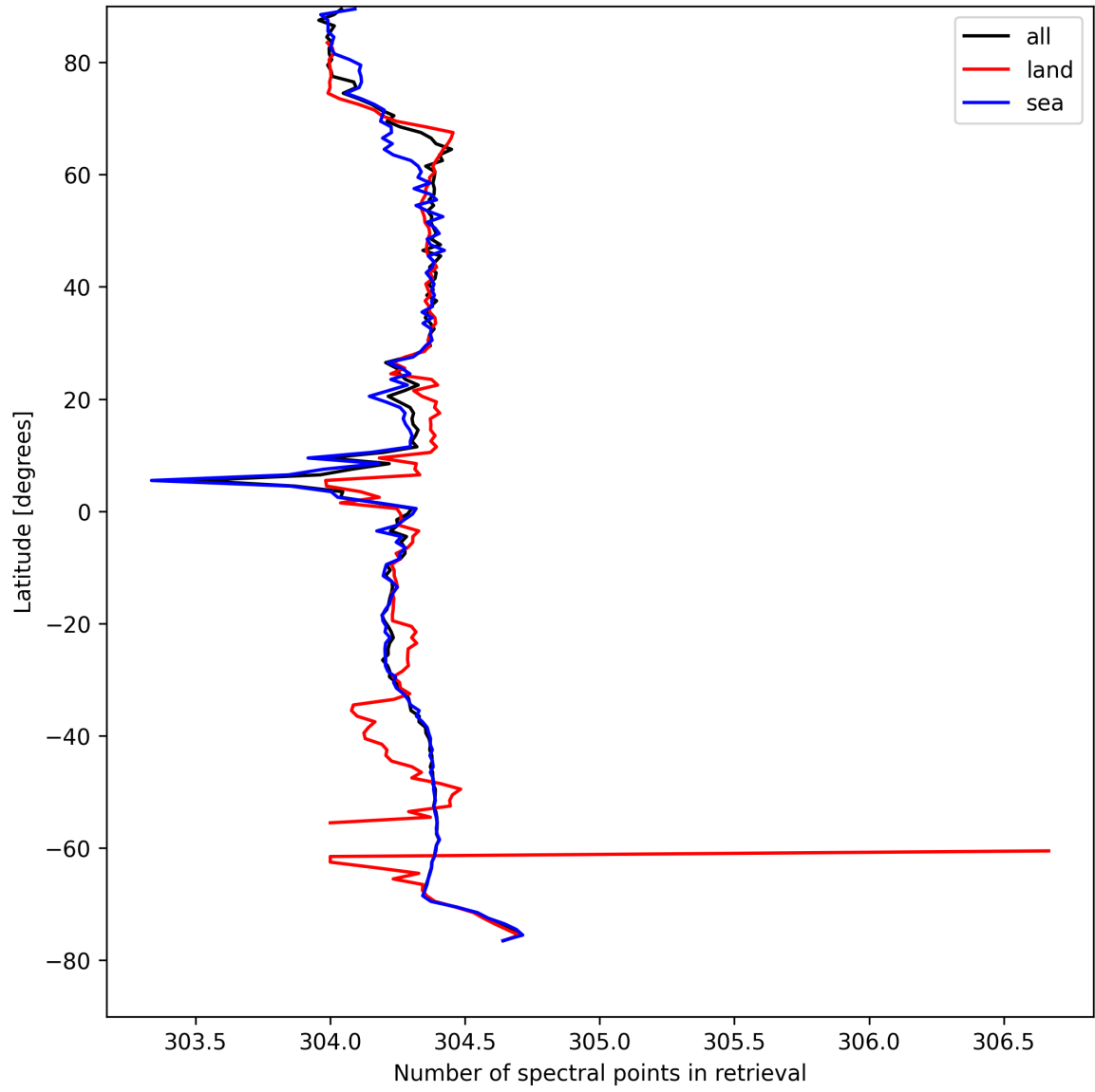
Figure 14: Zonal average of “Number of spectral points in retrieval” for 2025-04-20 to 2025-04-21.
