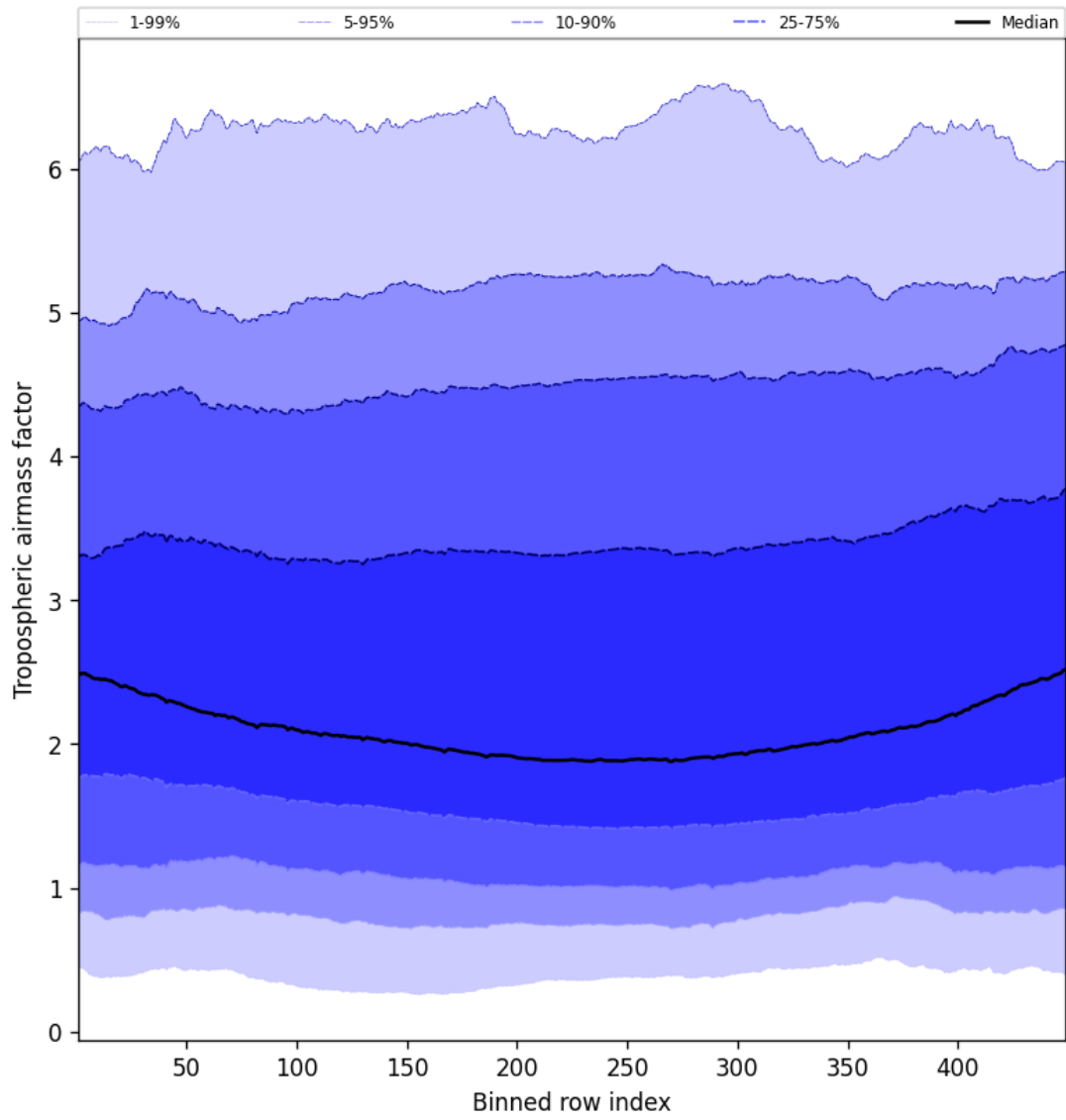
Figure 46: Along track statistics of “Tropospheric airmass factor” for 2025-04-20 to 2025-04-21
