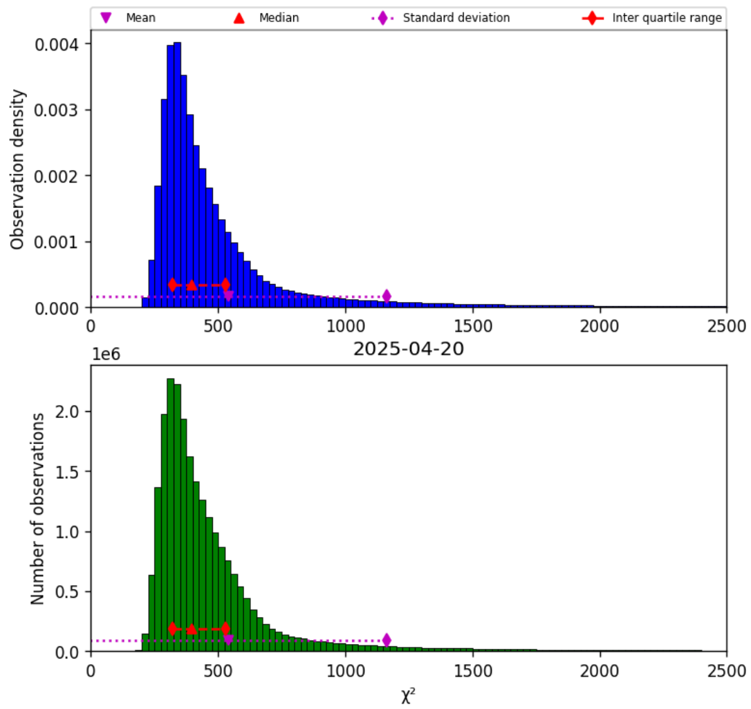
Figure 40: Histogram of " \chi^2 " for 2025-04-20 to 2025-04-21
