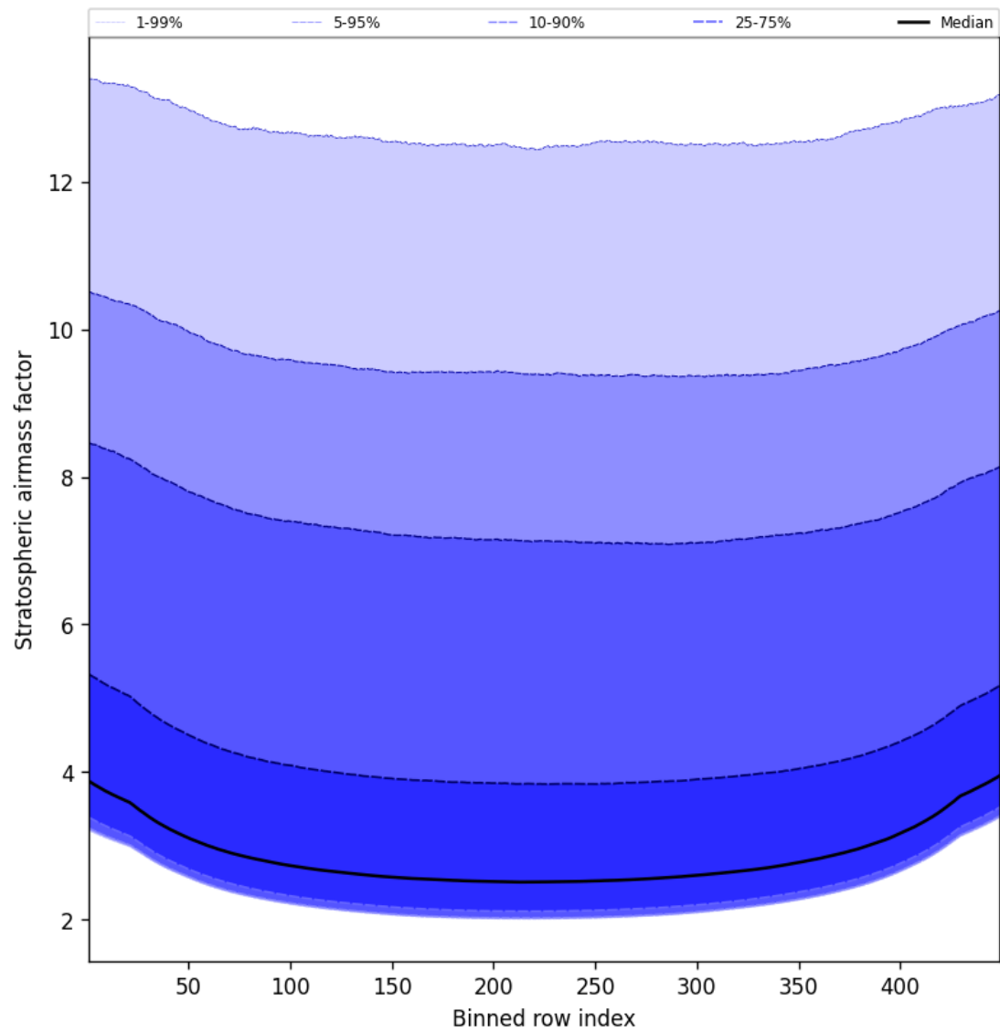
Figure 59: Along track statistics of “Stratospheric airmass factor” for 2025-04-20 to 2025-04-21
