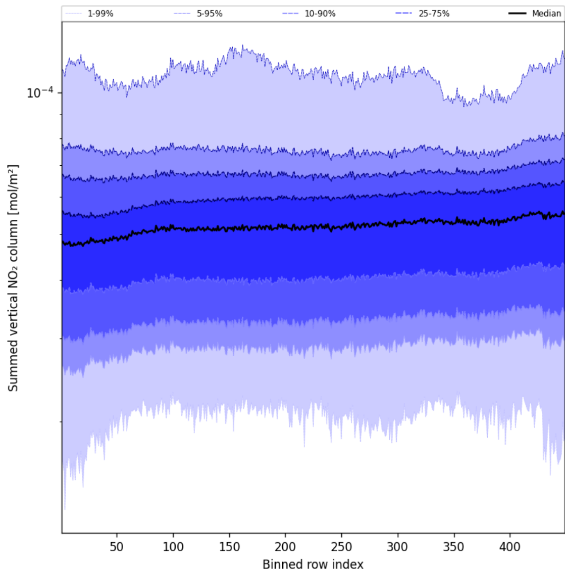
Figure 55: Along track statistics of “Summed vertical NO 2 column” for 2025-04-20 to 2025-04-21
