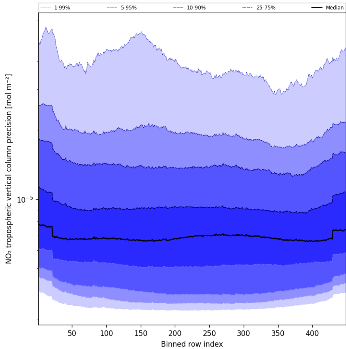
Figure 45: Along track statistics of “NO 2 tropospheric vertical column precision” for 2025-04-20 to 2025-04-21
