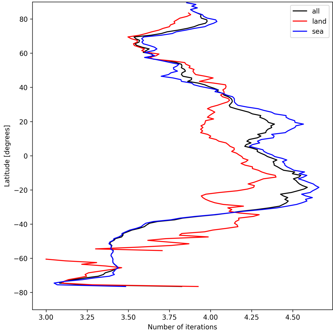
Figure 15: Zonal average of “Number of iterations” for 2025-04-20 to 2025-04-21.
