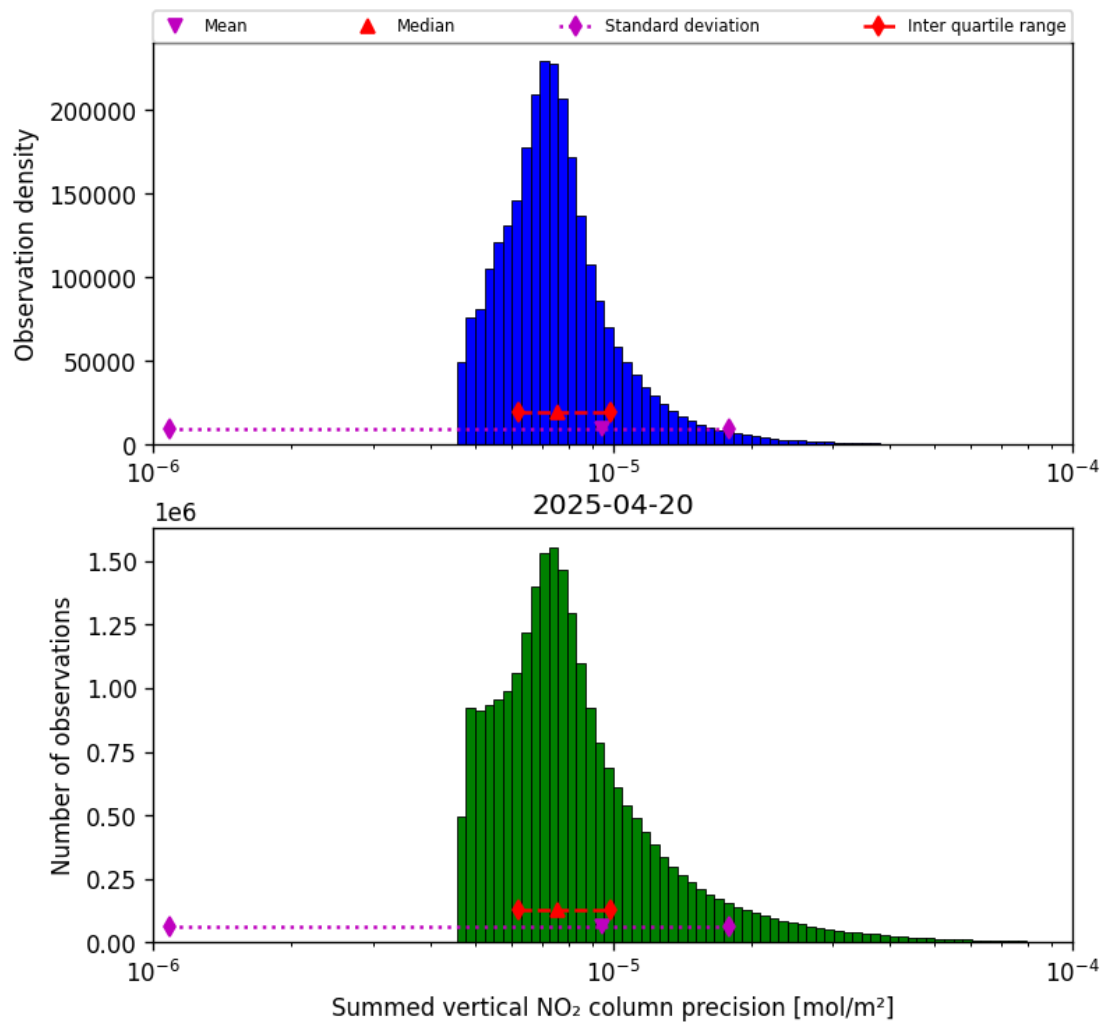
Figure 39: Histogram of “Summed vertical NO 2 column precision” for 2025-04-20 to 2025-04-21
