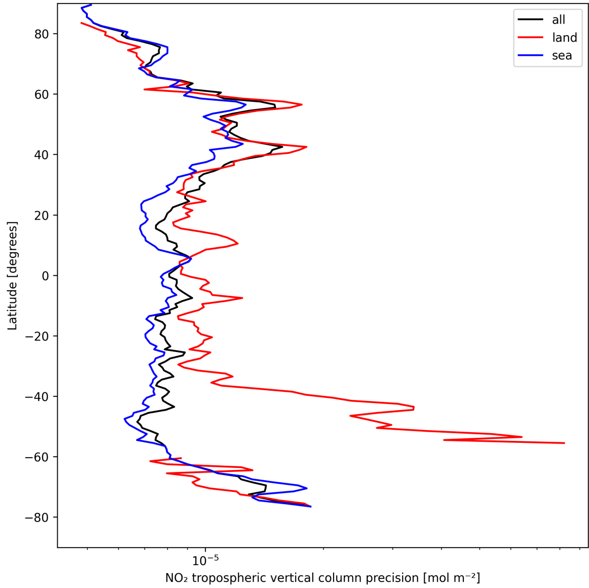
Figure 11: Zonal average of “NO 2 tropospheric vertical column precision” for 2025-04-20 to 2025-04-21.
