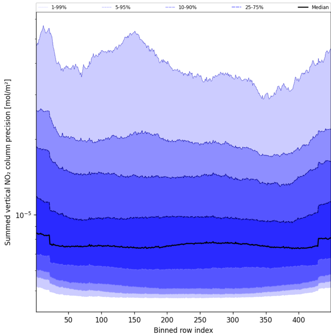
Figure 56: Along track statistics of “Summed vertical NO 2 column precision” for 2025-04-20 to 2025-04-21
