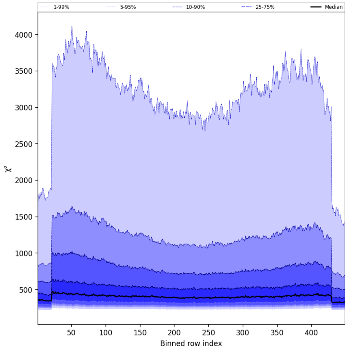
Figure 57: Along track statistics of “ \chi^2 ” for 2025-04-20 to 2025-04-21
