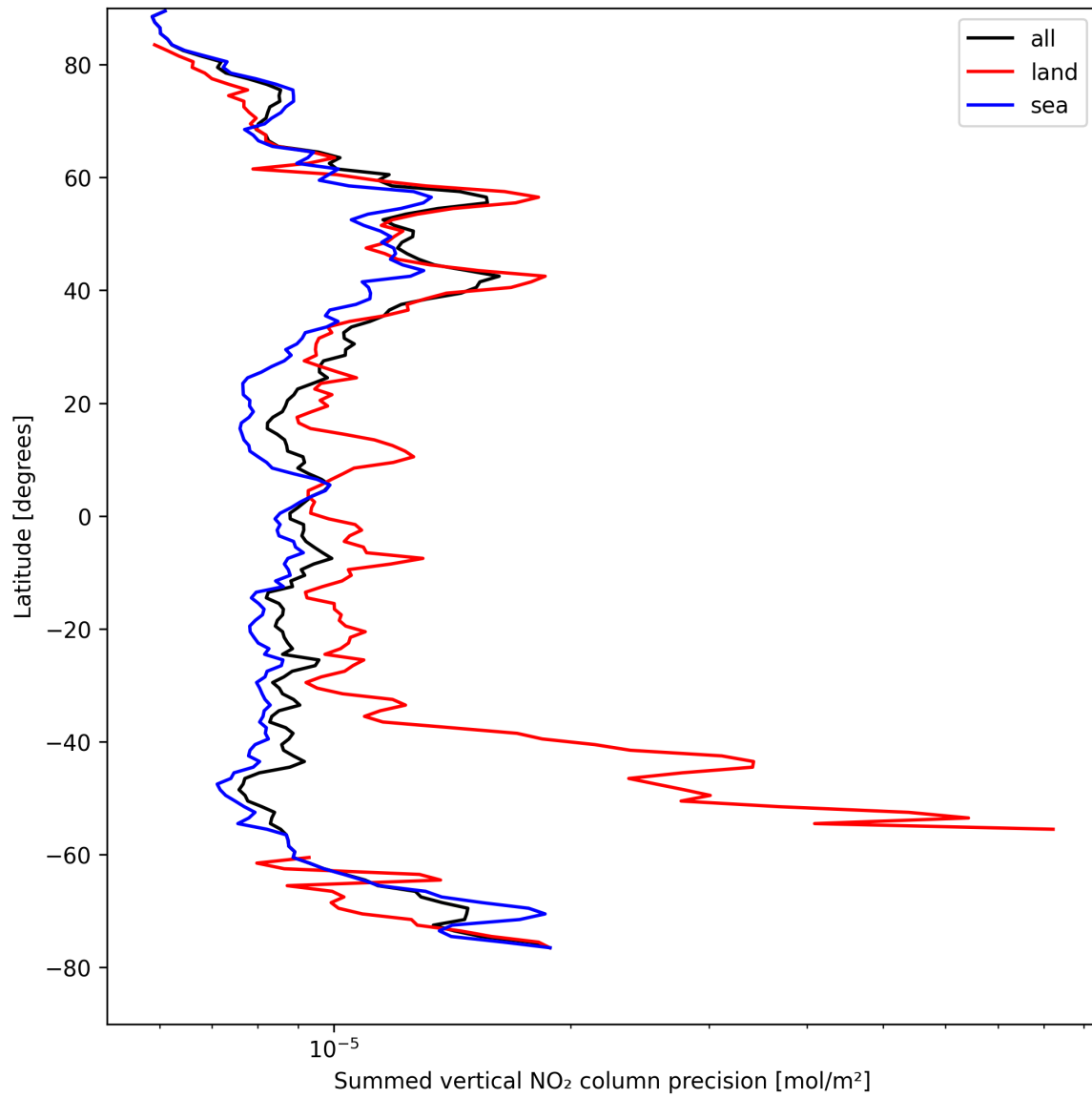
Figure 22: Zonal average of “Summed vertical NO 2 column precision” for 2025-04-20 to 2025-04-21.
