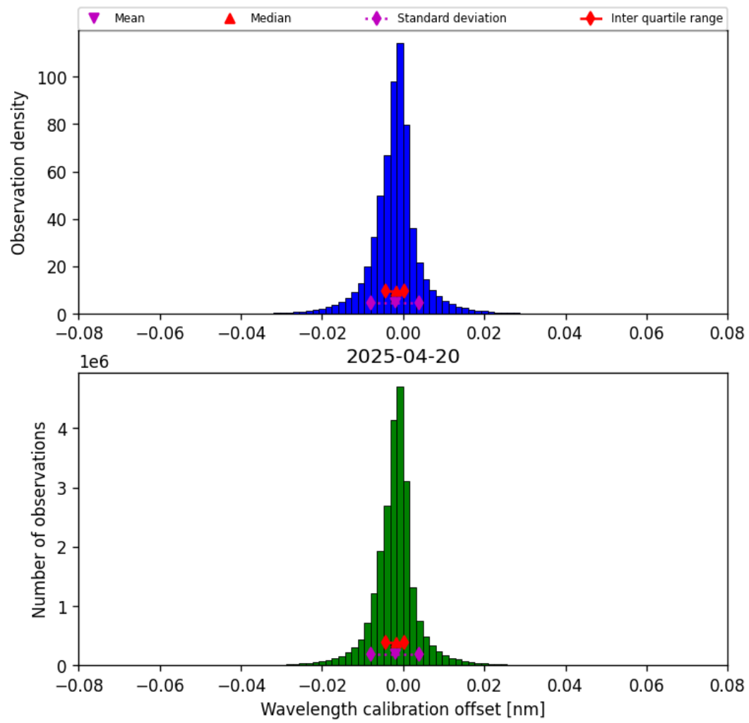
Figure 33: Histogram of “Wavelength calibration offset” for 2025-04-20 to 2025-04-21
