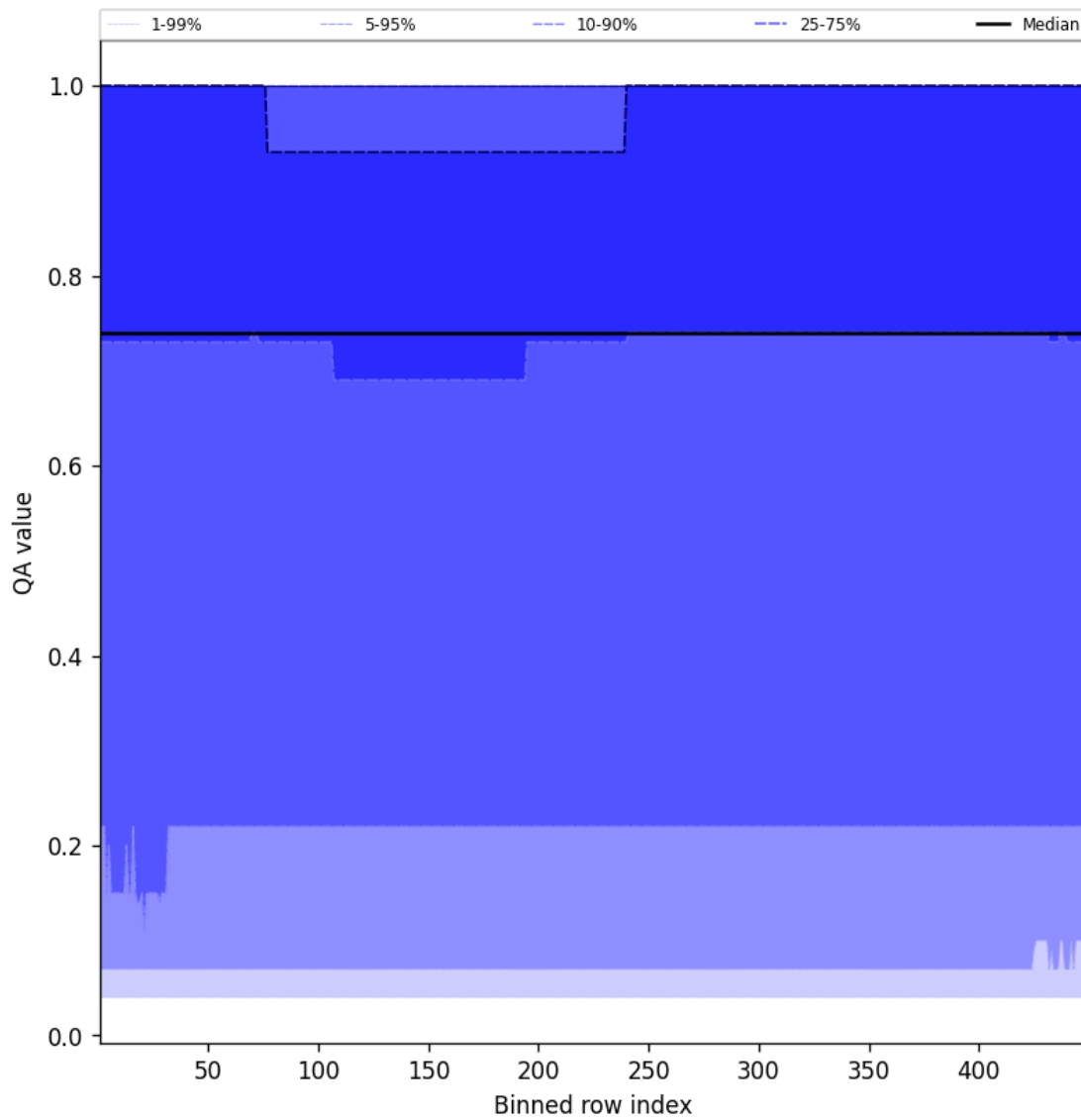
Figure 43: Along track statistics of “QA value” for 2025-04-20 to 2025-04-21
