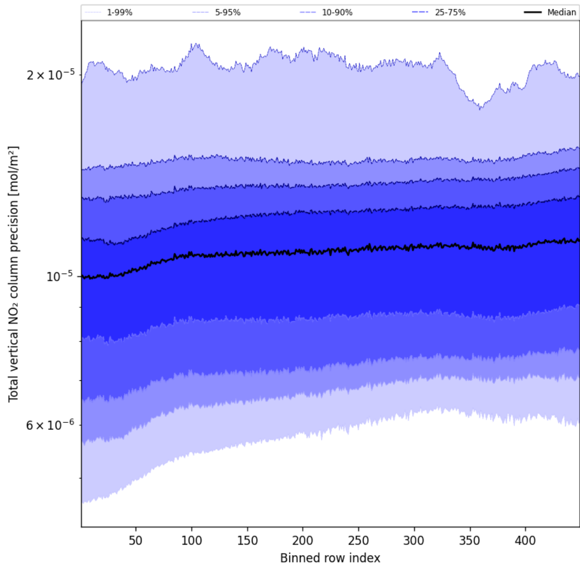
Figure 54: Along track statistics of "Total vertical NO 2 column precision" for 2025-04-20 to 2025-04-21
