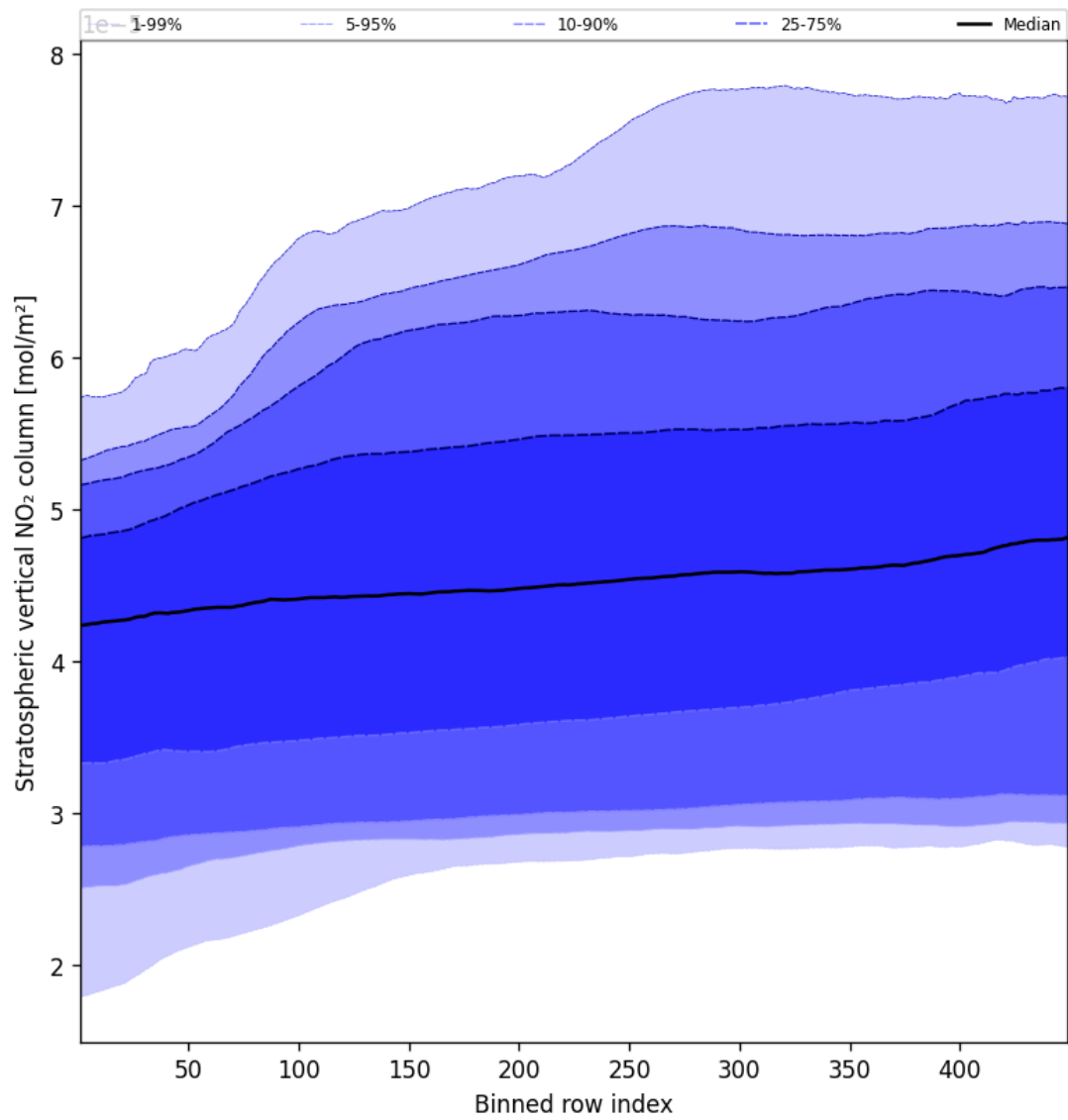
Figure 51: Along track statistics of “Stratospheric vertical NO 2 column” for 2025-04-20 to 2025-04-21
