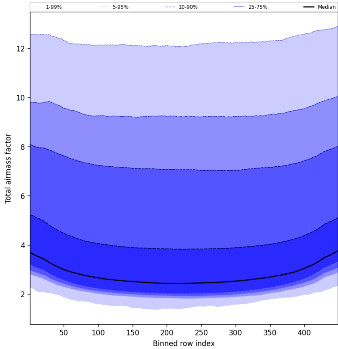
Figure 47: Along track statistics of “Total airmass factor” for 2025-04-20 to 2025-04-21
