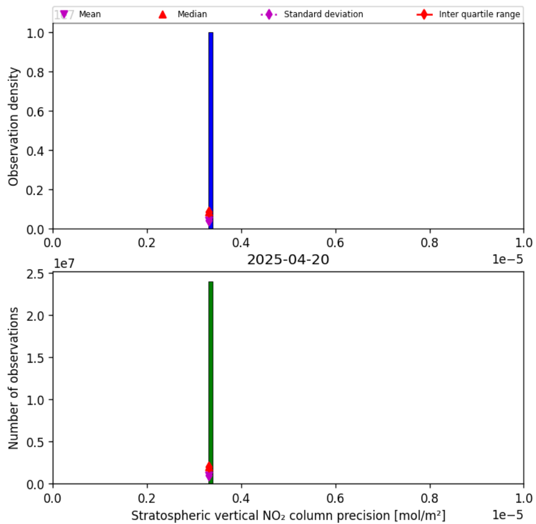
Figure 35: Histogram of “Stratospheric vertical NO 2 column precision” for 2025-04-20 to 2025-04-21
