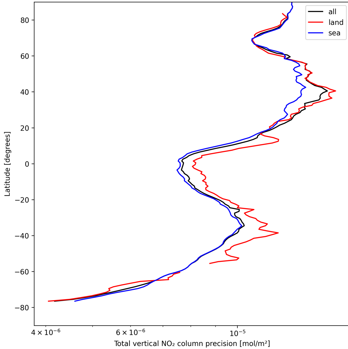
Figure 20: Zonal average of “Total vertical NO 2 column precision” for 2025-04-20 to 2025-04-21.
