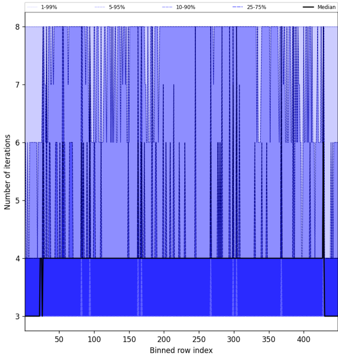
Figure 49: Along track statistics of “Number of iterations” for 2025-04-20 to 2025-04-21
