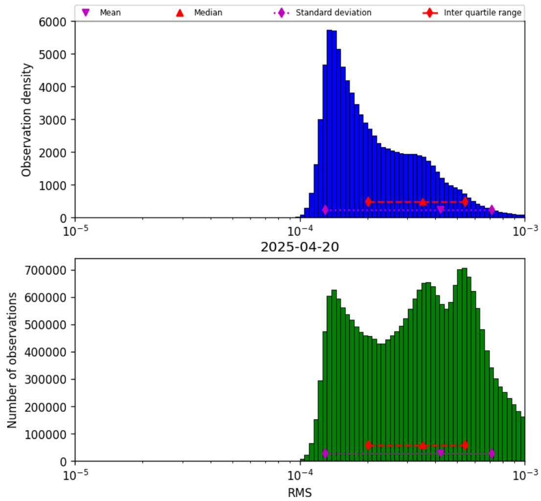
Figure 41: Histogram of “RMS” for 2025-04-20 to 2025-04-21
