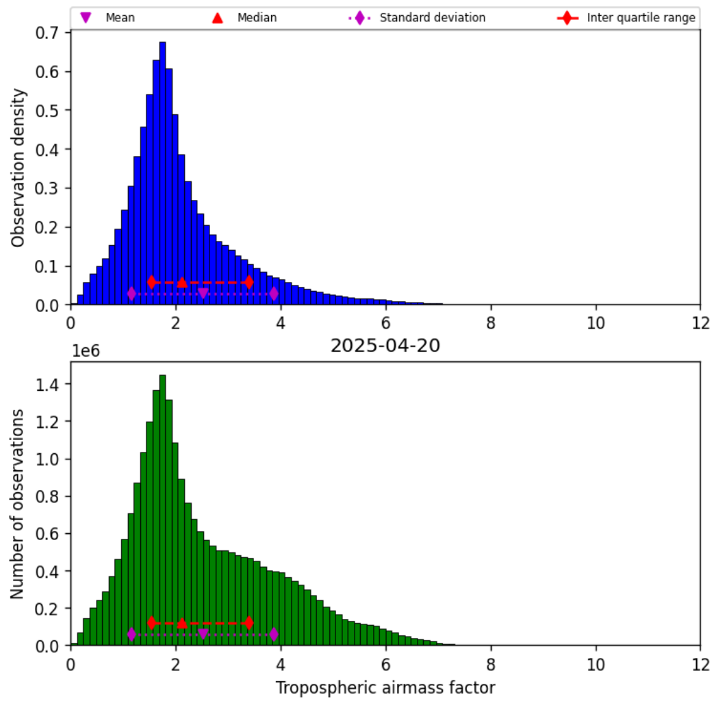
Figure 29: Histogram of “Tropospheric airmass factor” for 2025-04-20 to 2025-04-21
