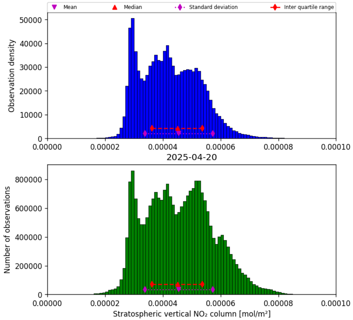
Figure 34: Histogram of “Stratospheric vertical NO 2 column” for 2025-04-20 to 2025-04-21
