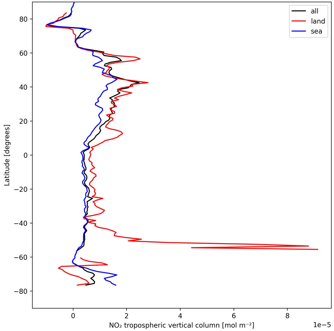
Figure 10: Zonal average of “NO 2 tropospheric vertical column” for 2025-04-20 to 2025-04-21.
