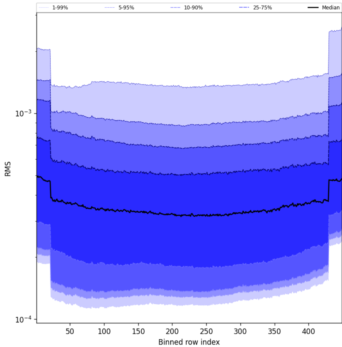
Figure 58: Along track statistics of “RMS” for 2025-04-20 to 2025-04-21
