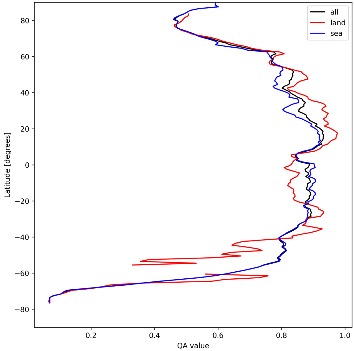
Figure 9: Zonal average of “QA value” for 2025-04-20 to 2025-04-21.
