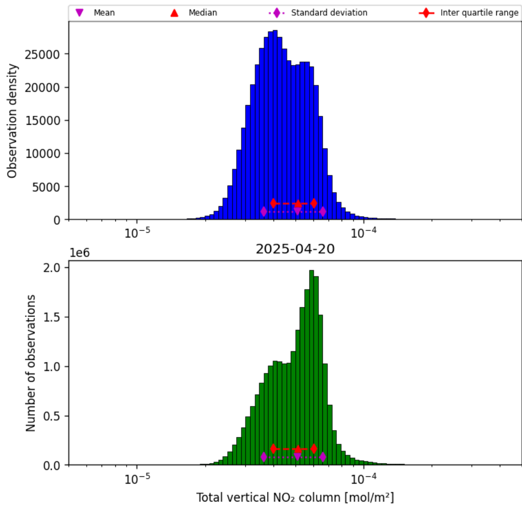
Figure 36: Histogram of “Total vertical NO 2 column” for 2025-04-20 to 2025-04-21
