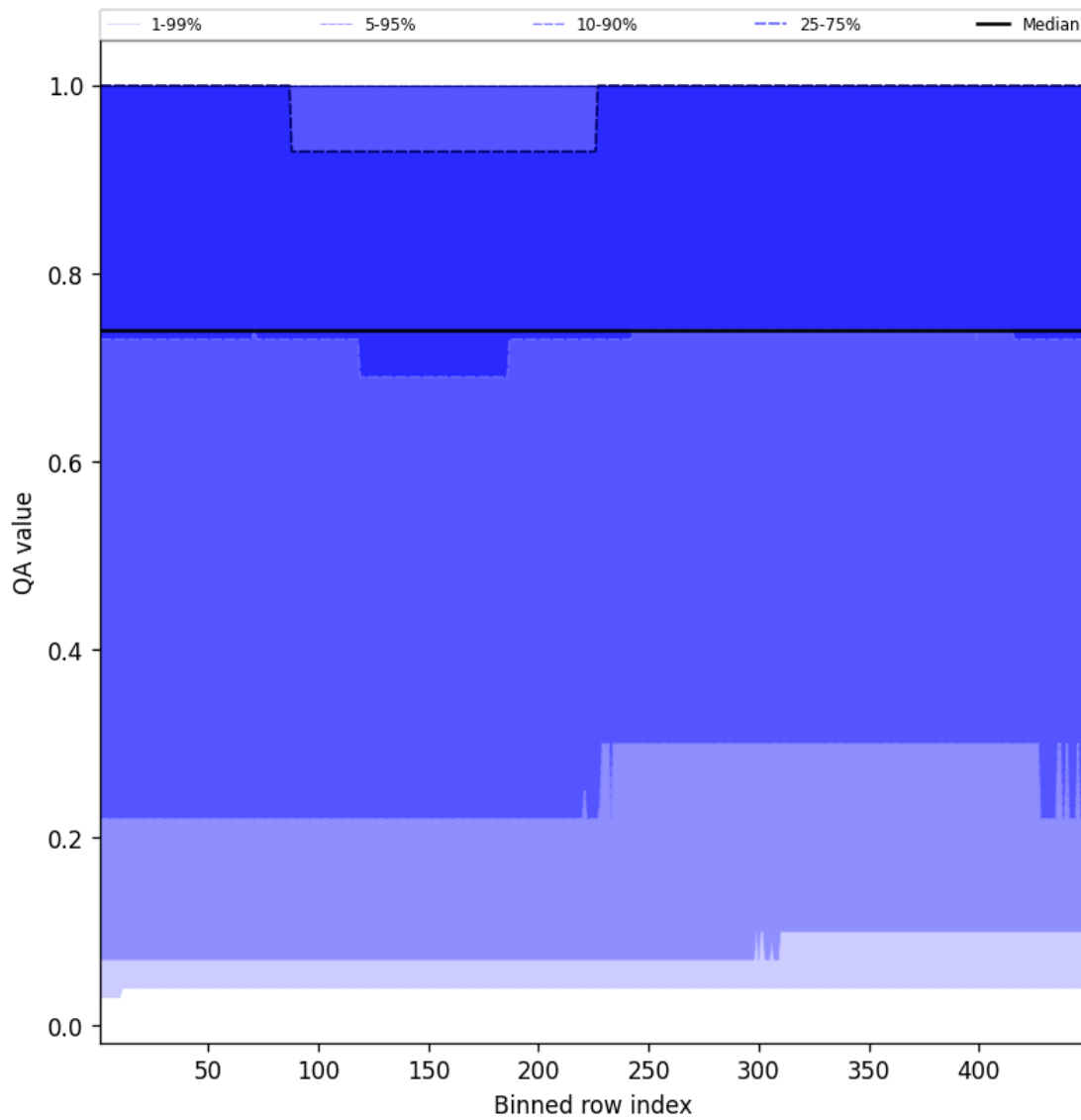
Figure 43: Along track statistics of “QA value” for 2025-04-22 to 2025-04-22
