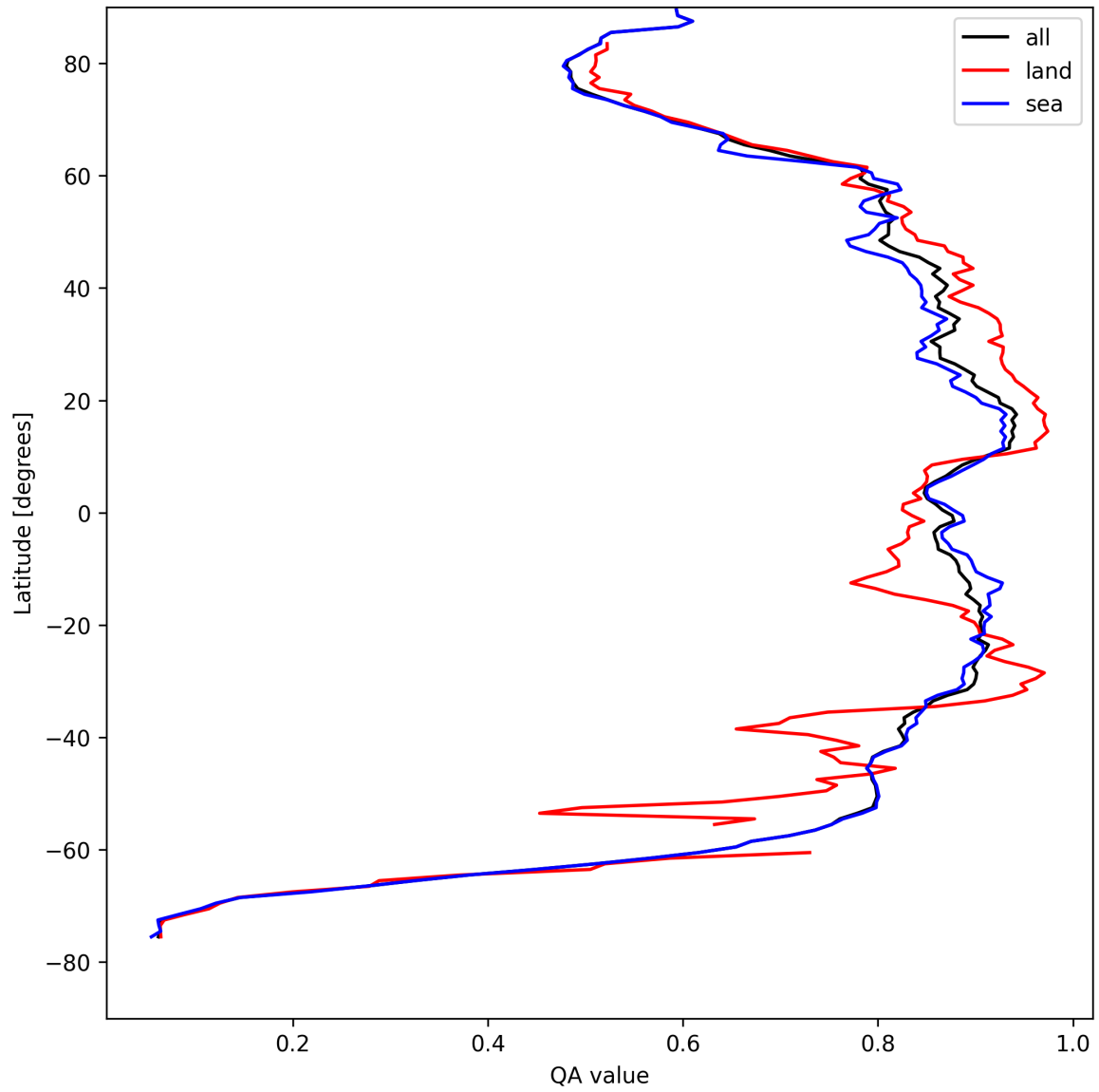
Figure 9: Zonal average of “QA value” for 2025-04-22 to 2025-04-22.
