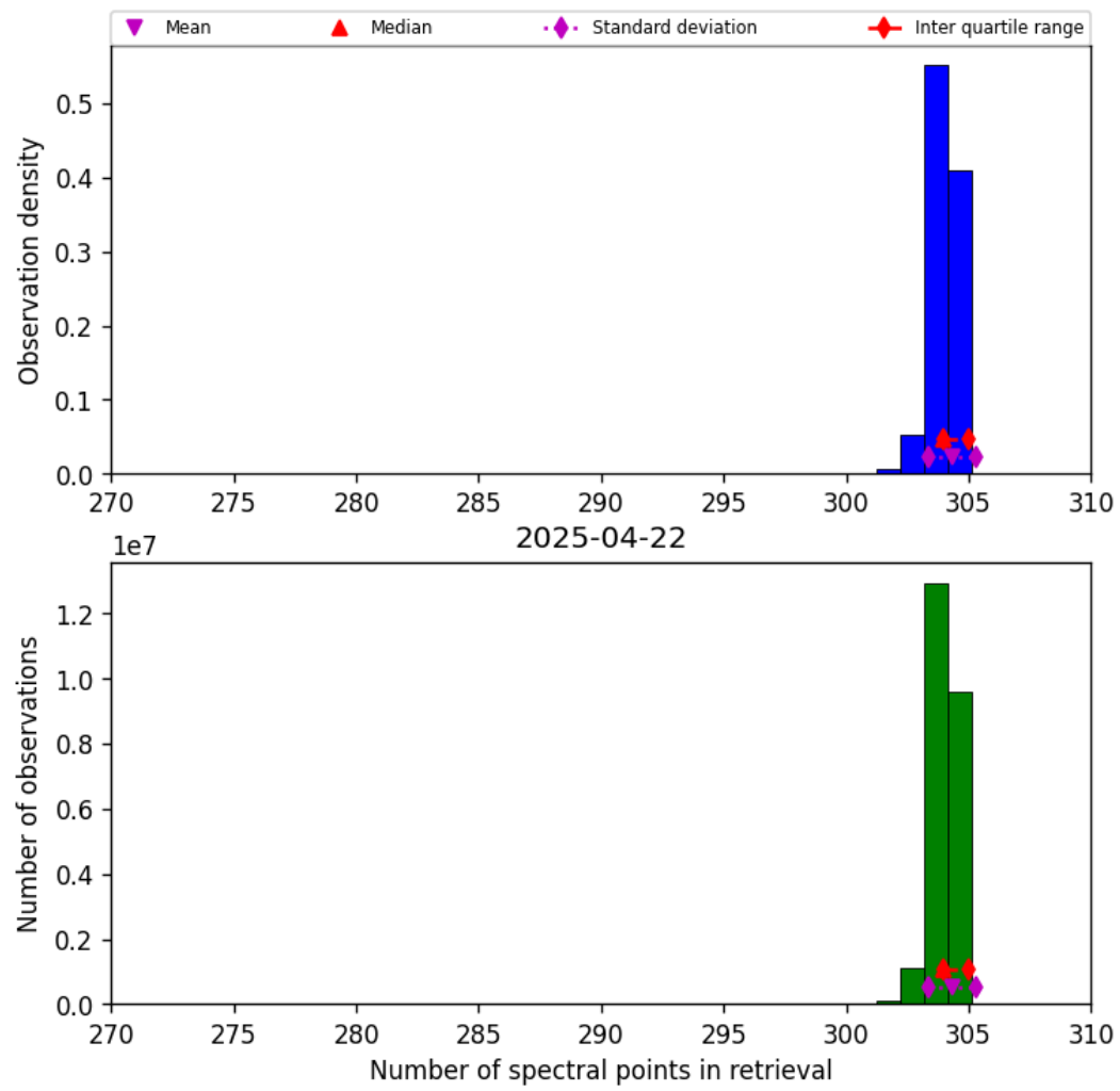
Figure 31: Histogram of “Number of spectral points in retrieval” for 2025-04-22 to 2025-04-22
