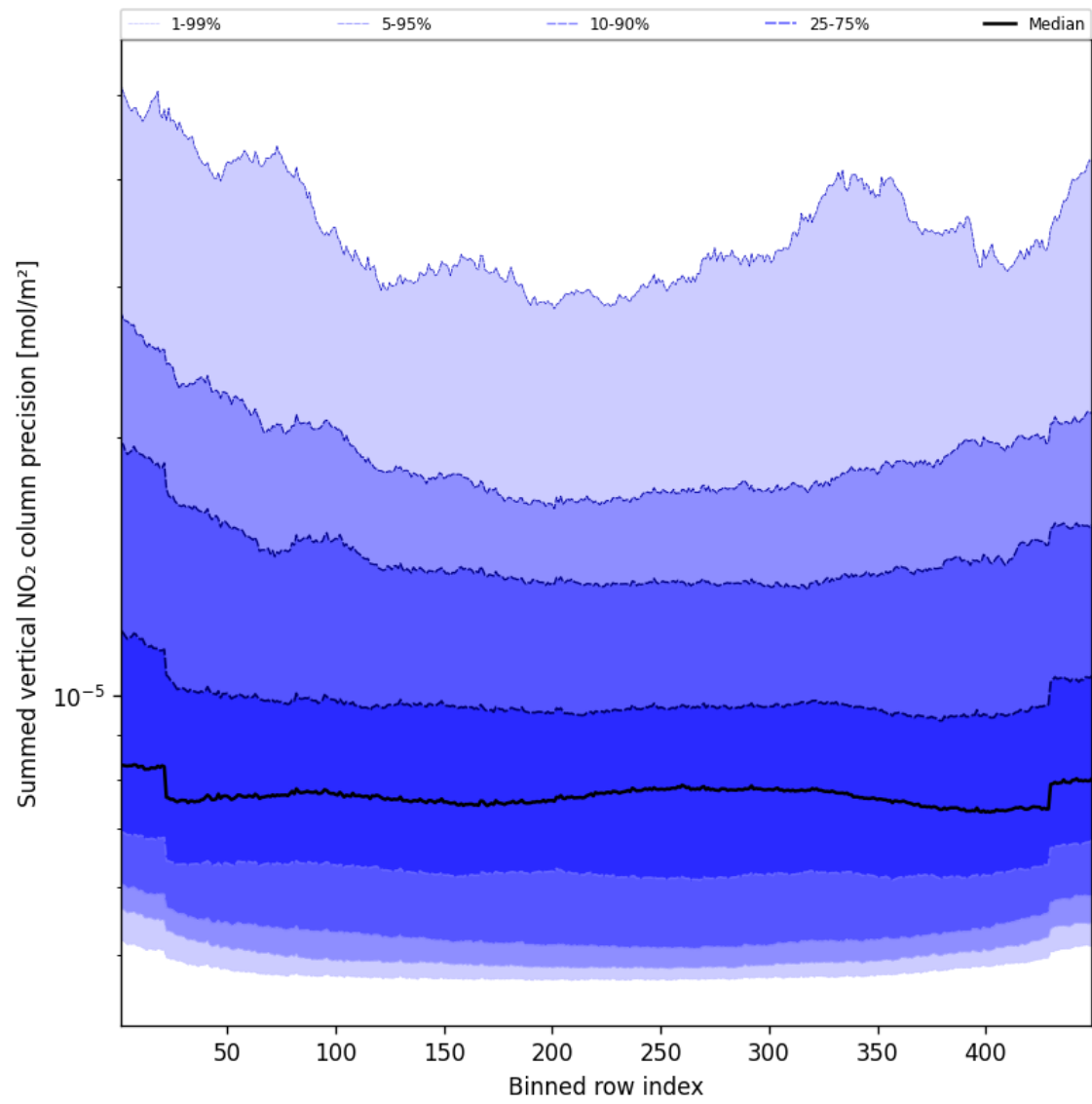
Figure 56: Along track statistics of “Summed vertical NO 2 column precision” for 2025-04-22 to 2025-04-22
