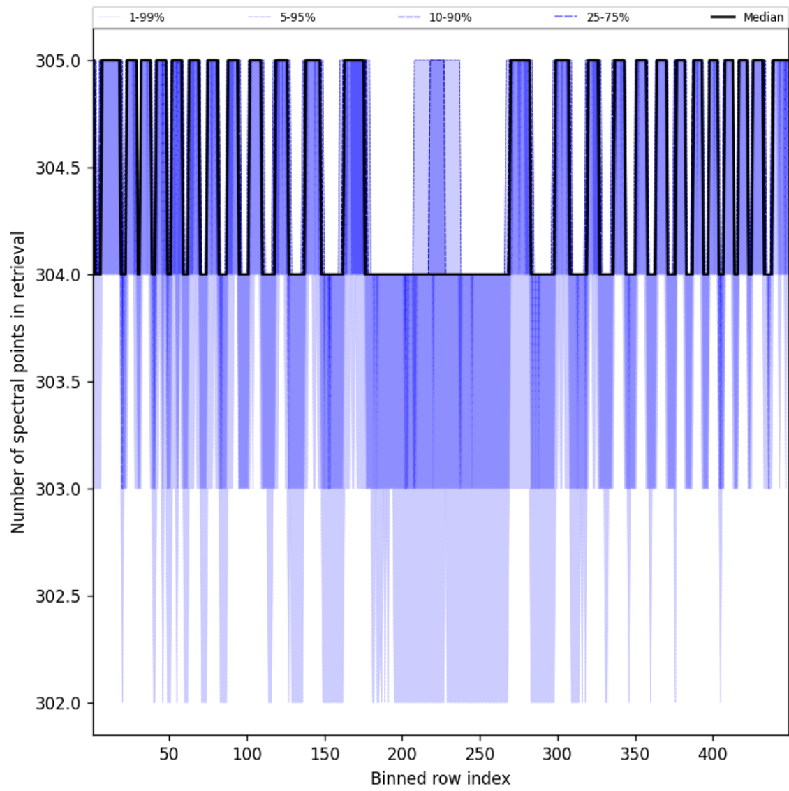
Figure 48: Along track statistics of “Number of spectral points in retrieval” for 2025-04-22 to 2025-04-22
