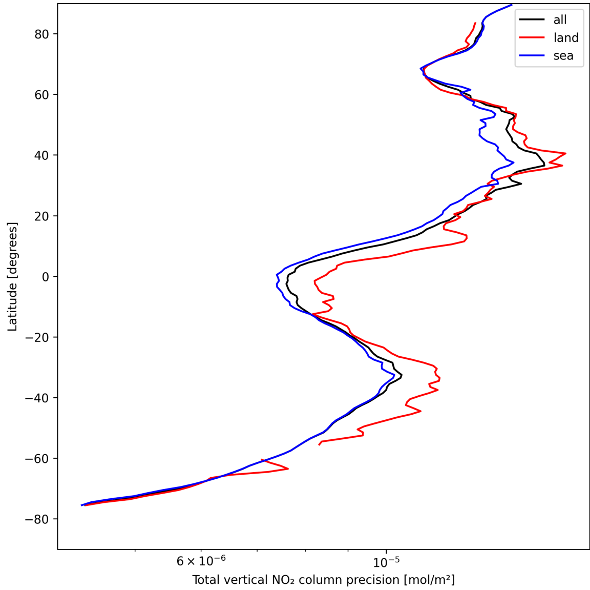
Figure 20: Zonal average of “Total vertical NO 2 column precision” for 2025-04-22 to 2025-04-22.
