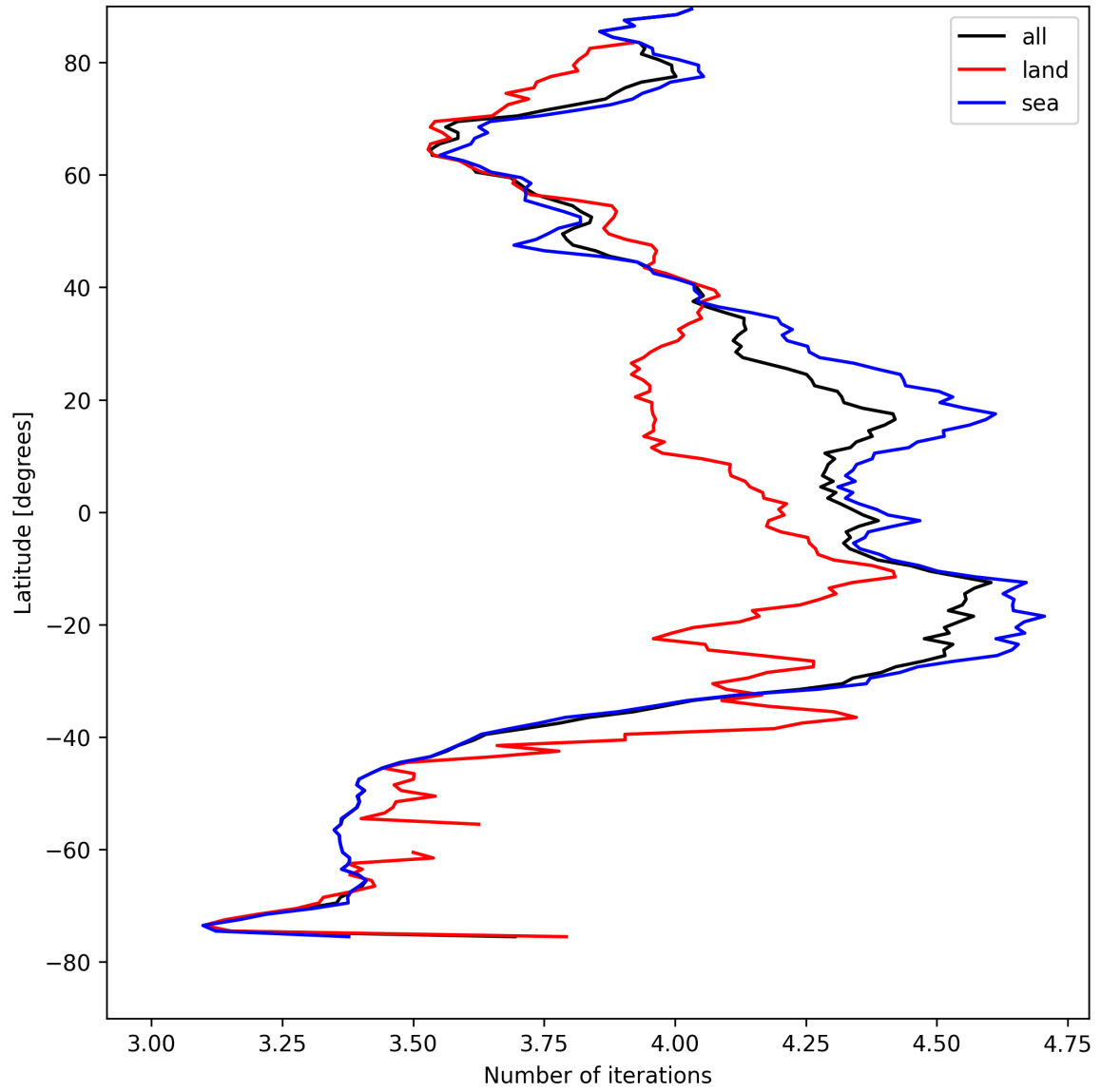
Figure 15: Zonal average of “Number of iterations” for 2025-04-22 to 2025-04-22.
