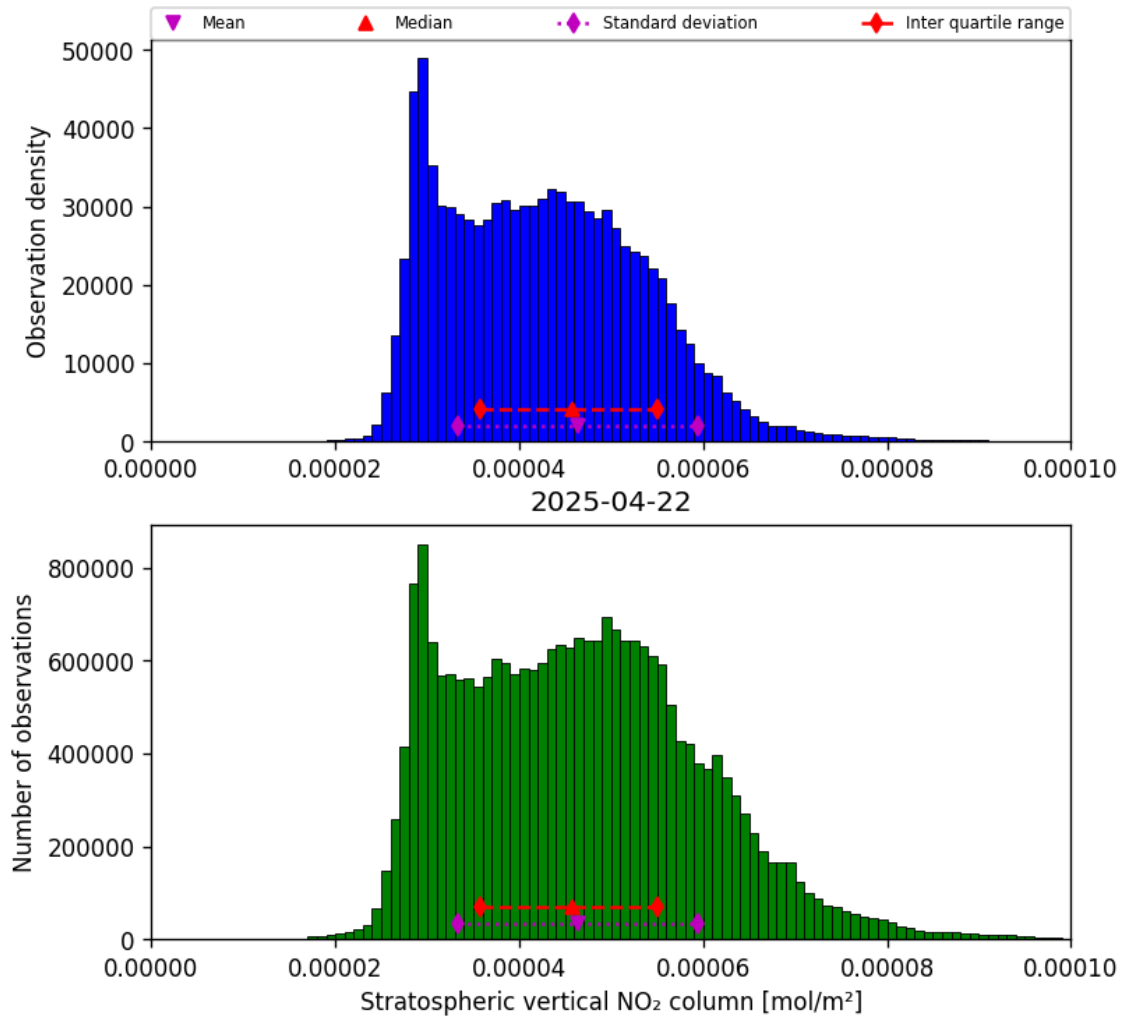
Figure 34: Histogram of “Stratospheric vertical NO 2 column” for 2025-04-22 to 2025-04-22
