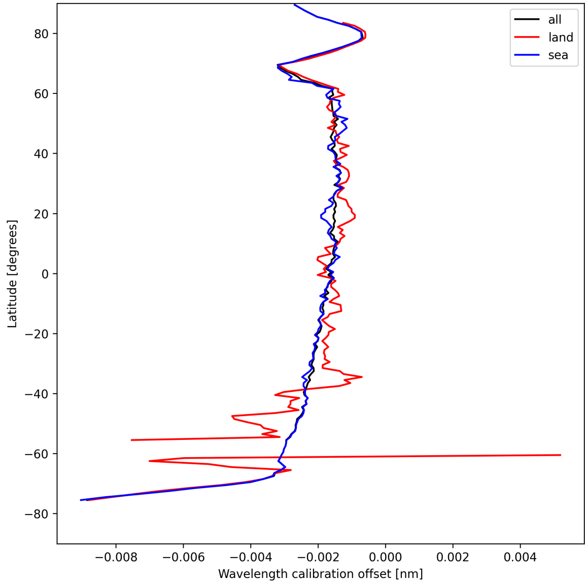
Figure 16: Zonal average of “Wavelength calibration offset” for 2025-04-22 to 2025-04-22.
