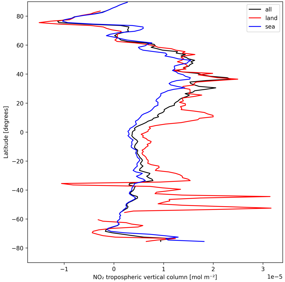
Figure 10: Zonal average of “NO 2 tropospheric vertical column” for 2025-04-22 to 2025-04-22.
