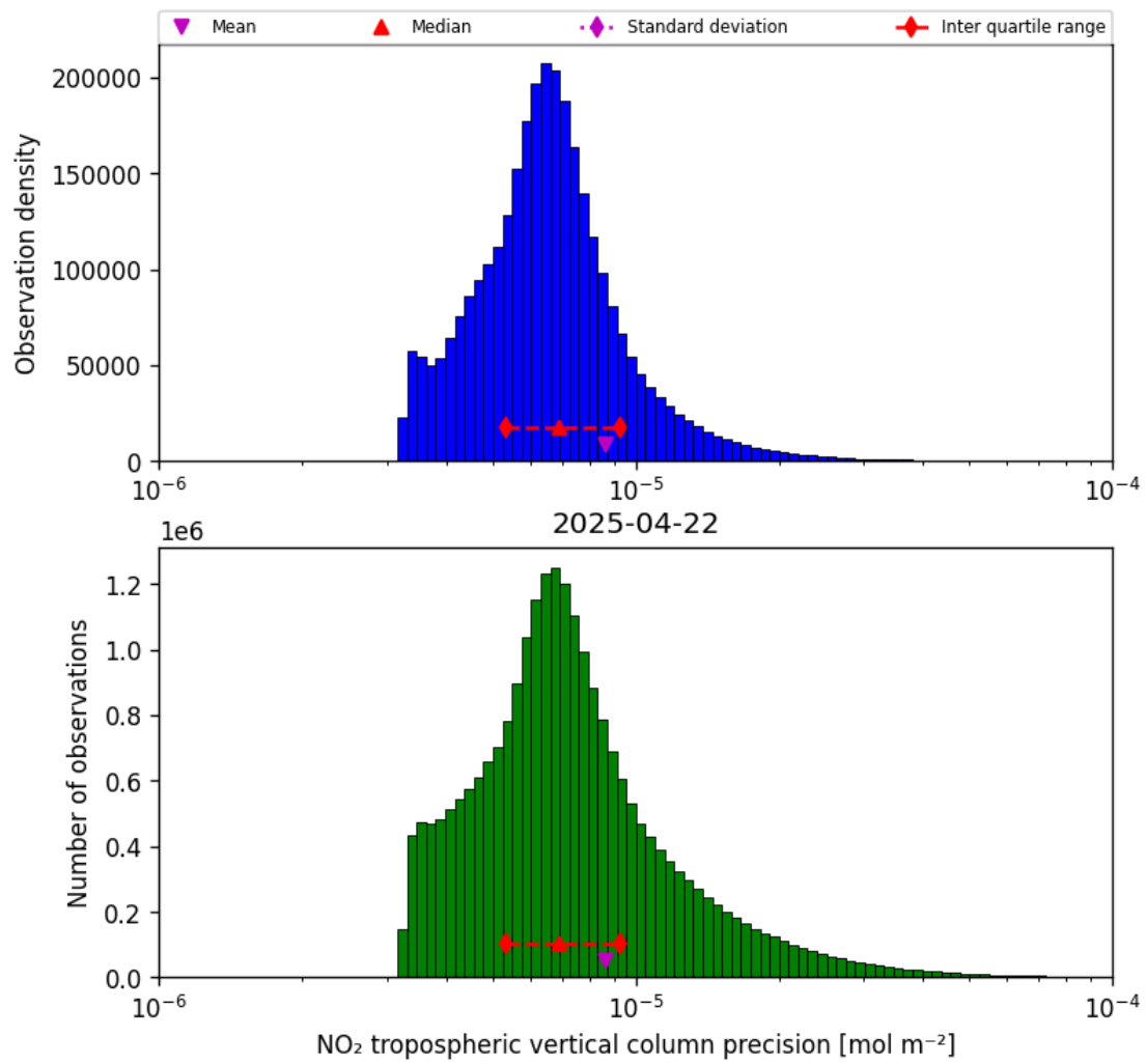
Figure 28: Histogram of “NO 2 tropospheric vertical column precision” for 2025-04-22 to 2025-04-22
