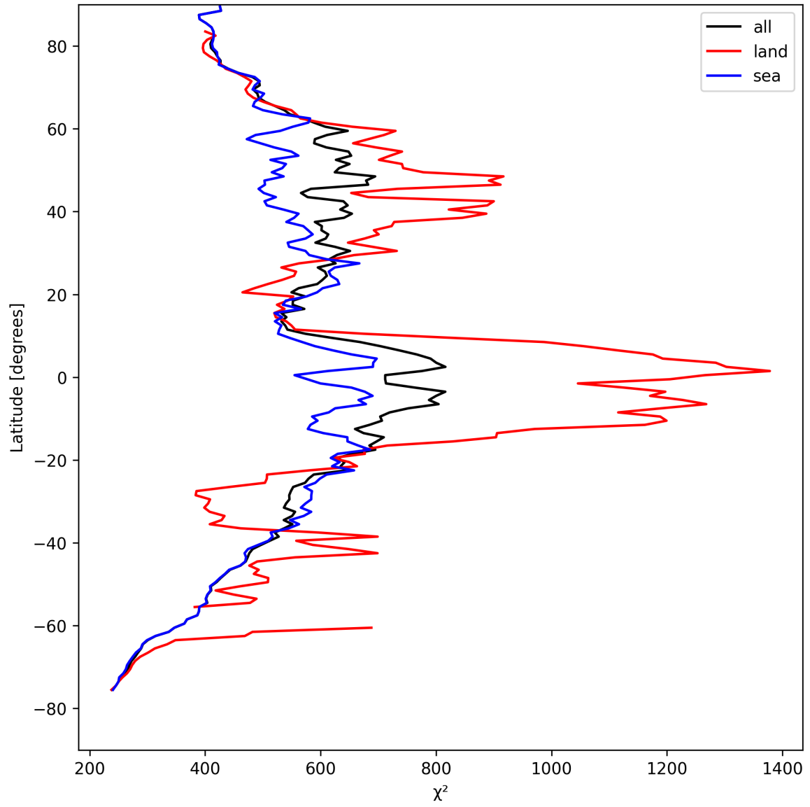
Figure 23: Zonal average of “ \chi^2 ” for 2025-04-22 to 2025-04-22.
