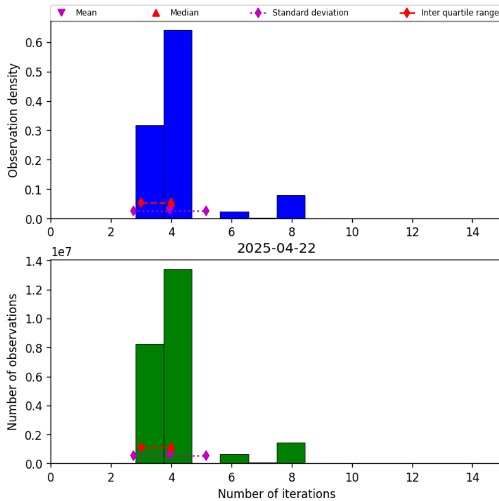
Figure 32: Histogram of “Number of iterations” for 2025-04-22 to 2025-04-22
