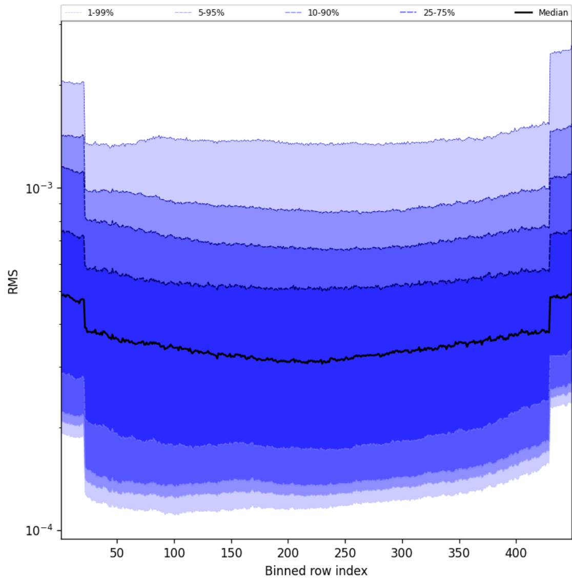
Figure 58: Along track statistics of “RMS” for 2025-04-22 to 2025-04-22
