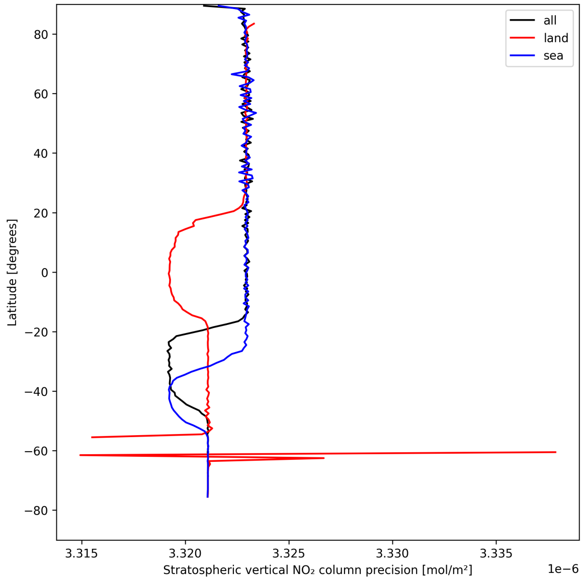
Figure 18: Zonal average of “Stratospheric vertical NO 2 column precision” for 2025-04-22 to 2025-04-22.
