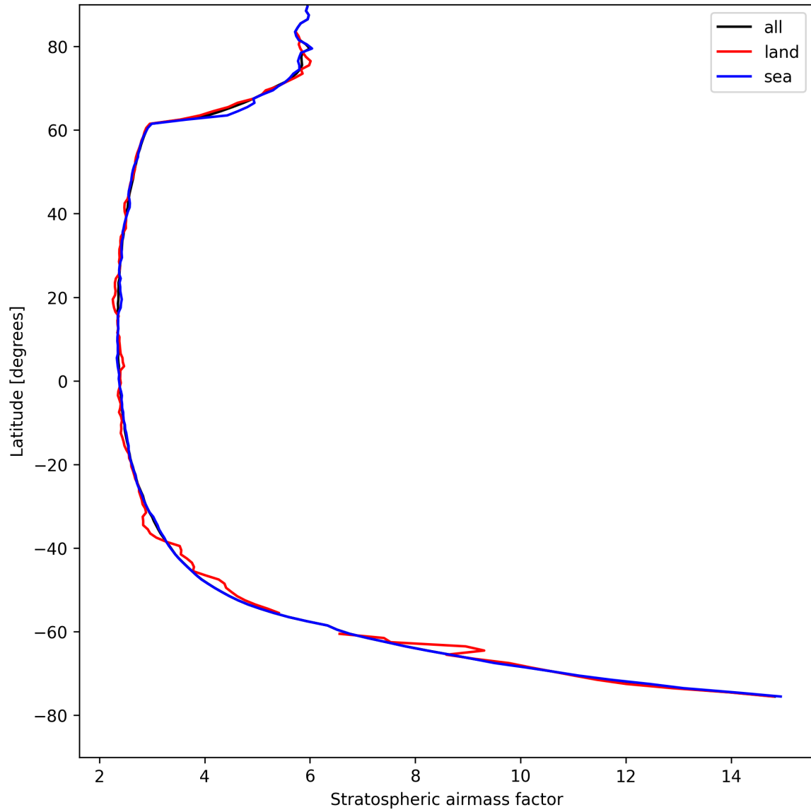
Figure 25: Zonal average of “Stratospheric airmass factor” for 2025-04-22 to 2025-04-22.
