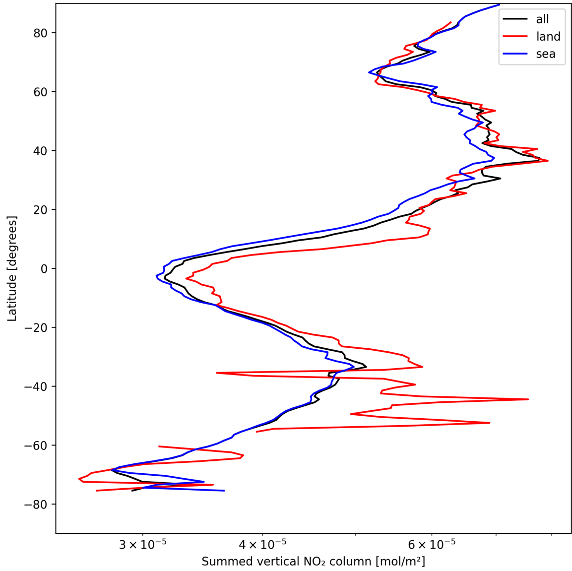
Figure 21: Zonal average of “Summed vertical NO 2 column” for 2025-04-22 to 2025-04-22.
