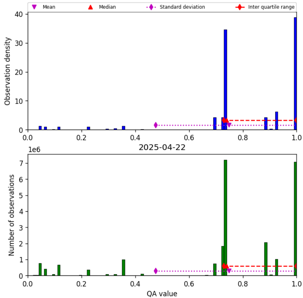
Figure 26: Histogram of “QA value” for 2025-04-22 to 2025-04-22
