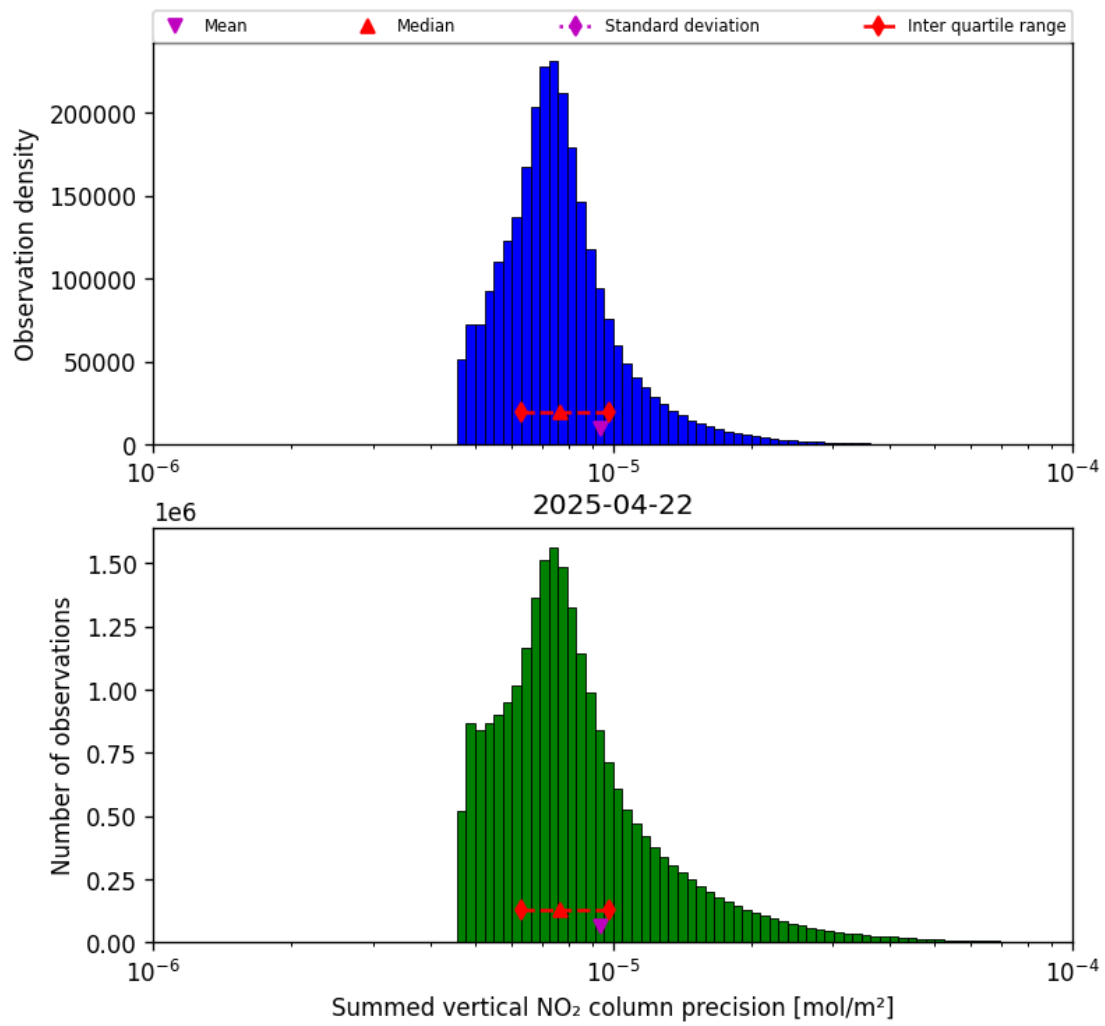
Figure 39: Histogram of "Summed vertical NO 2 column precision" for 2025-04-22 to 2025-04-22
