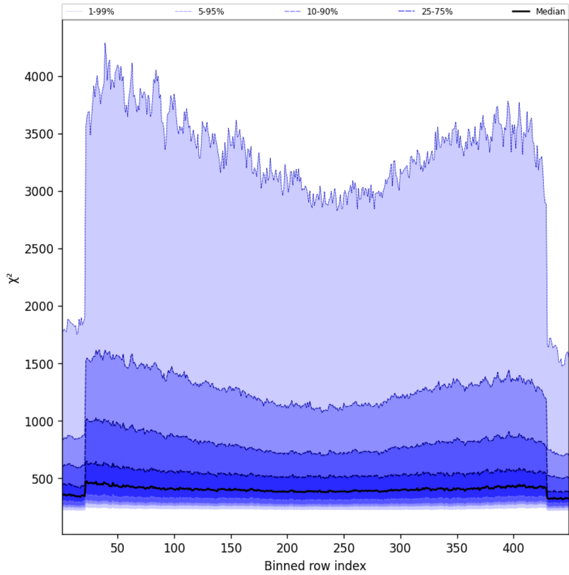
Figure 57: Along track statistics of “ \chi^2 ” for 2025-04-22 to 2025-04-22
