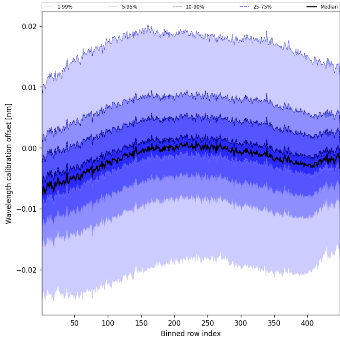
Figure 50: Along track statistics of “Wavelength calibration offset” for 2025-04-22 to 2025-04-22
