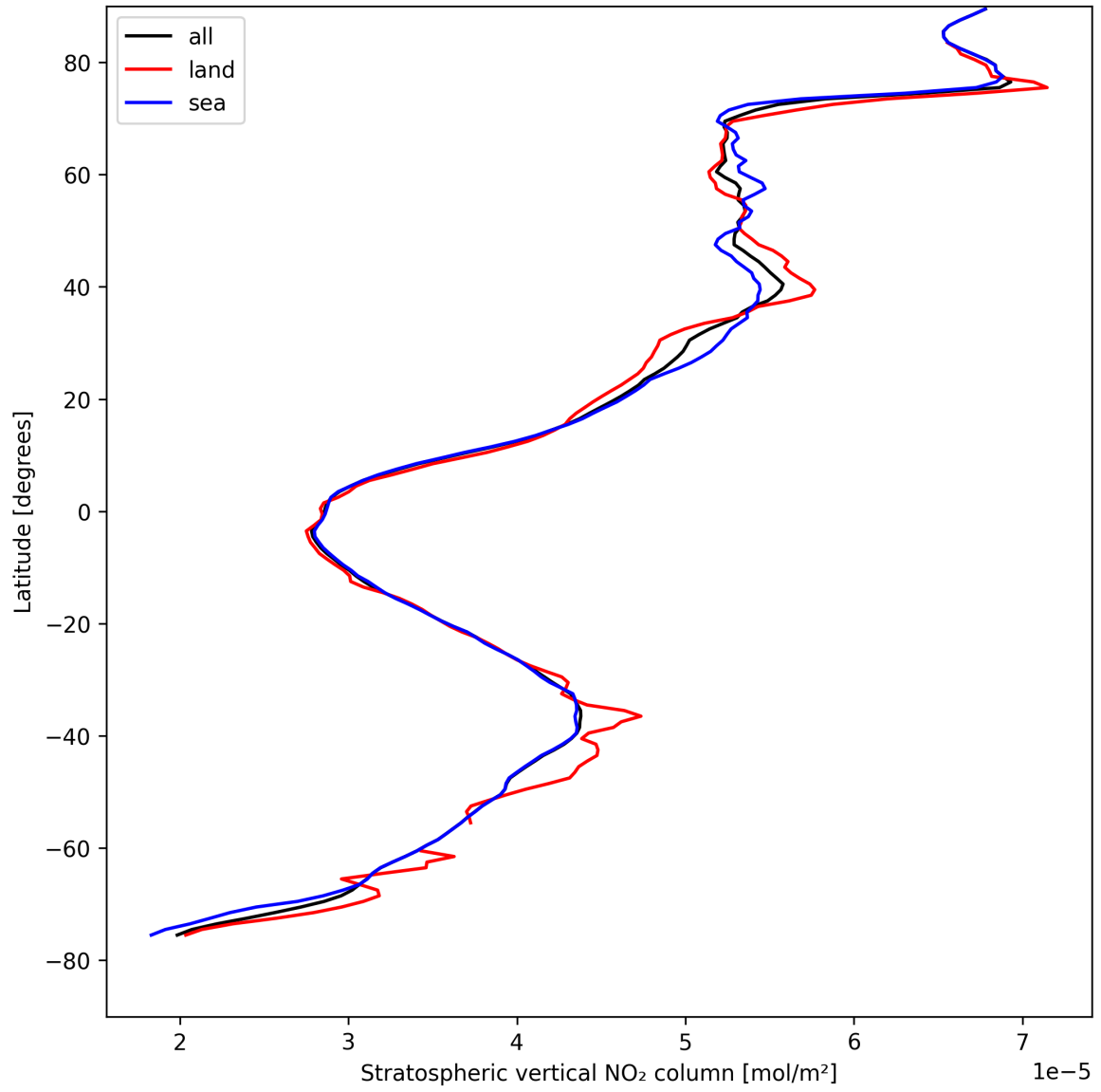
Figure 17: Zonal average of “Stratospheric vertical NO 2 column” for 2025-04-22 to 2025-04-22.
