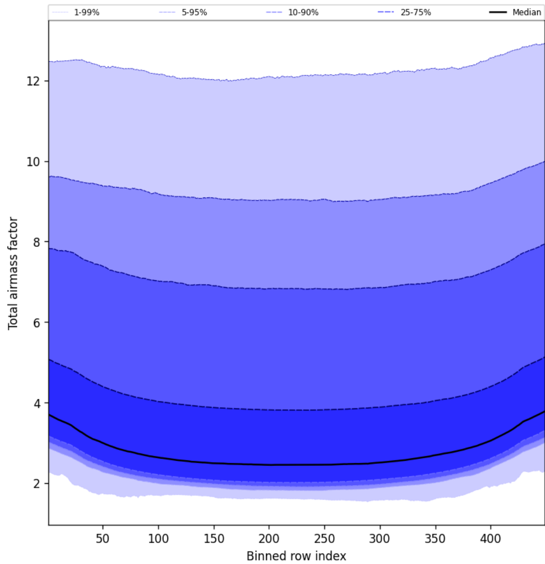
Figure 47: Along track statistics of “Total airmass factor” for 2025-04-22 to 2025-04-22
