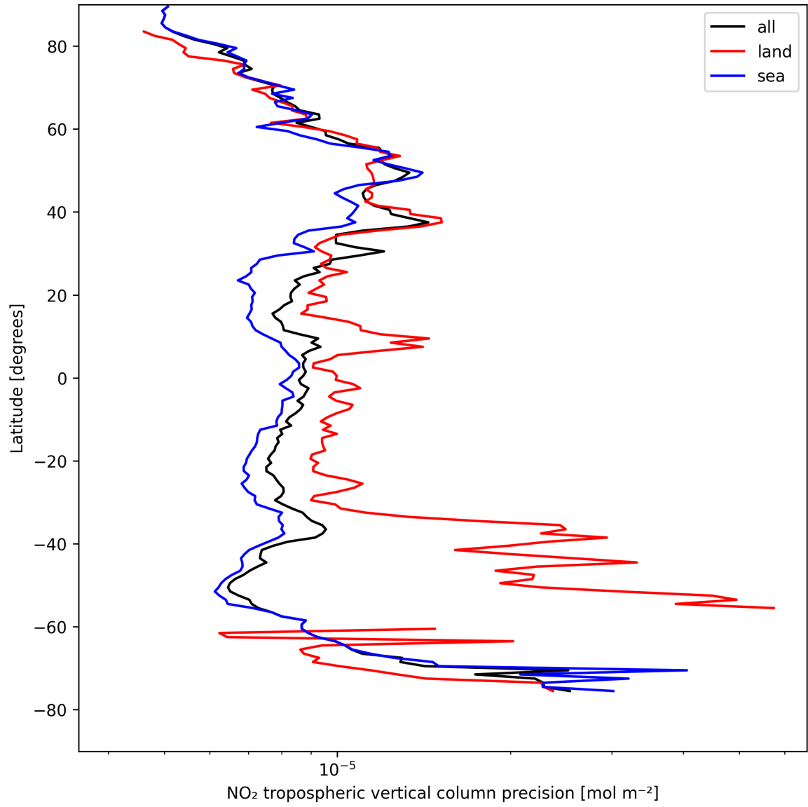
Figure 11: Zonal average of “NO 2 tropospheric vertical column precision” for 2025-04-22 to 2025-04-22.
