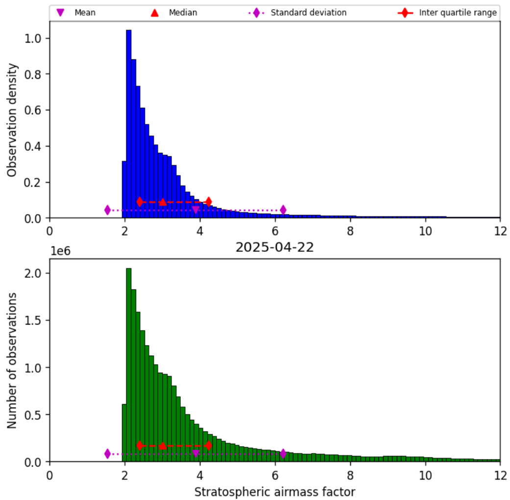
Figure 42: Histogram of “Stratospheric airmass factor” for 2025-04-22 to 2025-04-22
