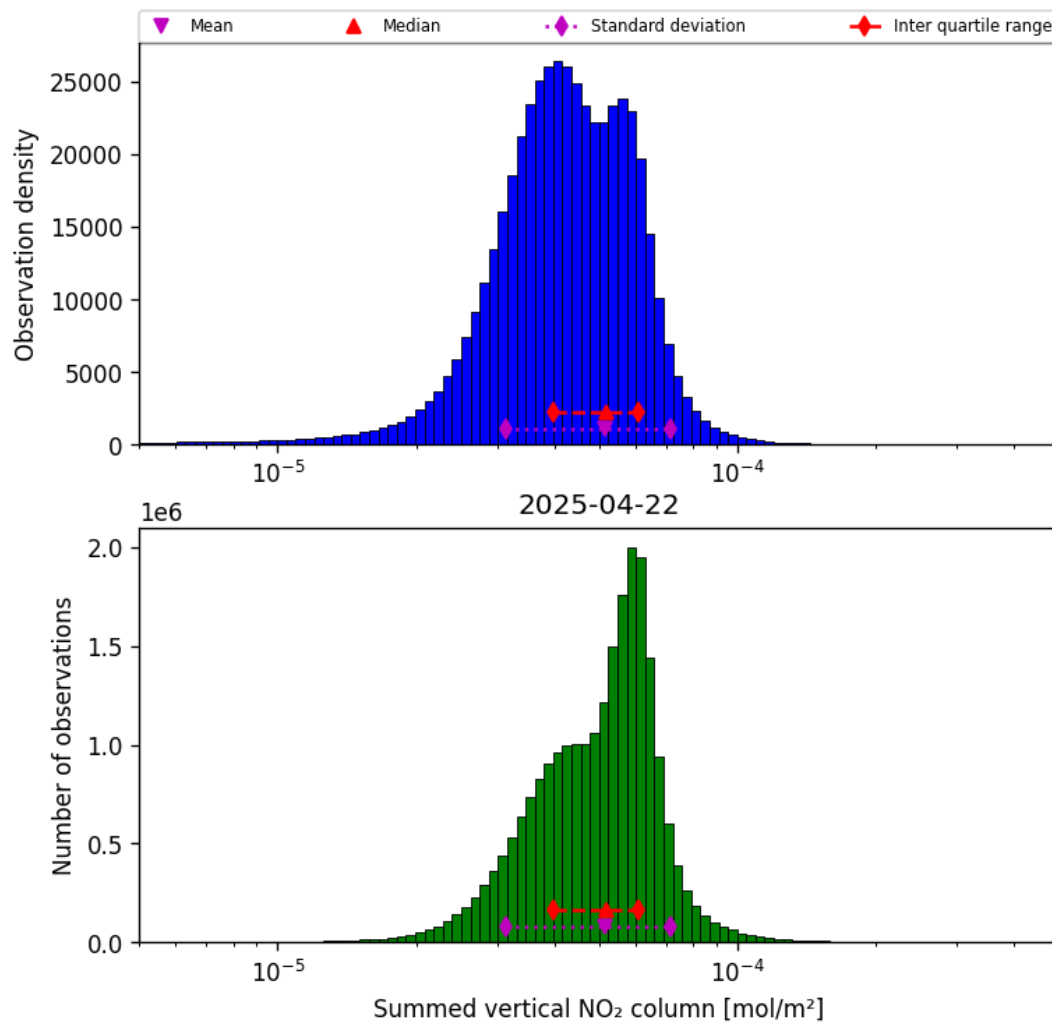
Figure 38: Histogram of “Summed vertical NO 2 column” for 2025-04-22 to 2025-04-22
