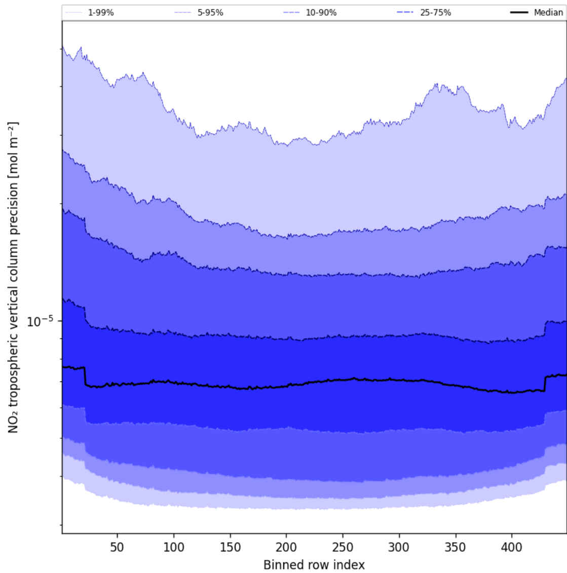
Figure 45: Along track statistics of “NO 2 tropospheric vertical column precision” for 2025-04-22 to 2025-04-22
