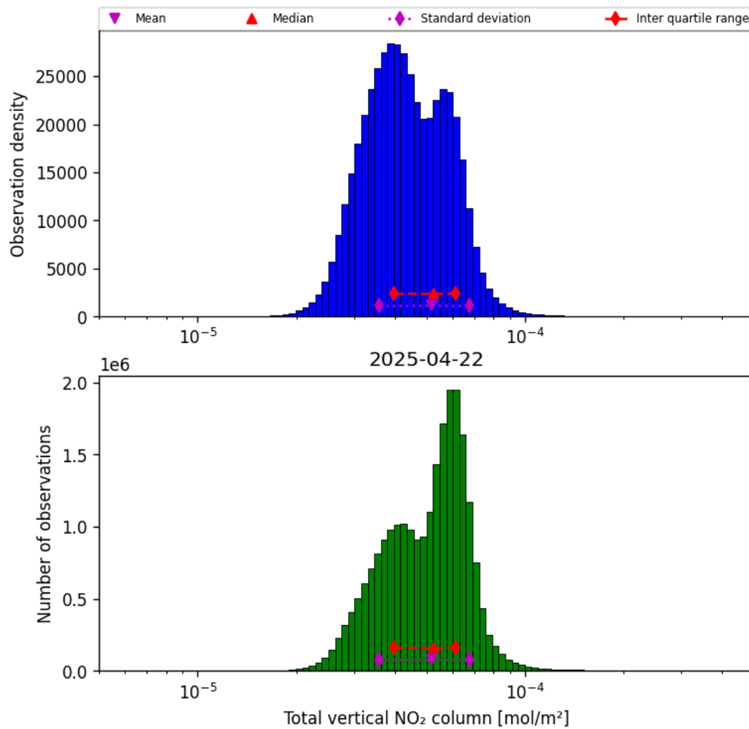
Figure 36: Histogram of “Total vertical NO 2 column” for 2025-04-22 to 2025-04-22
