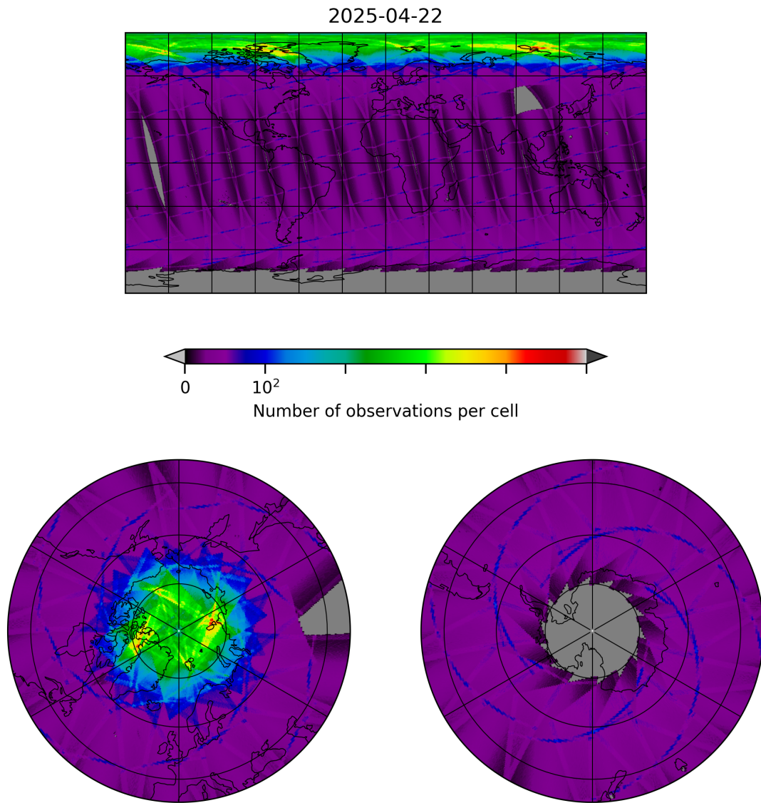
Figure 8: Map of the number of observations for 2025-04-22 to 2025-04-22
