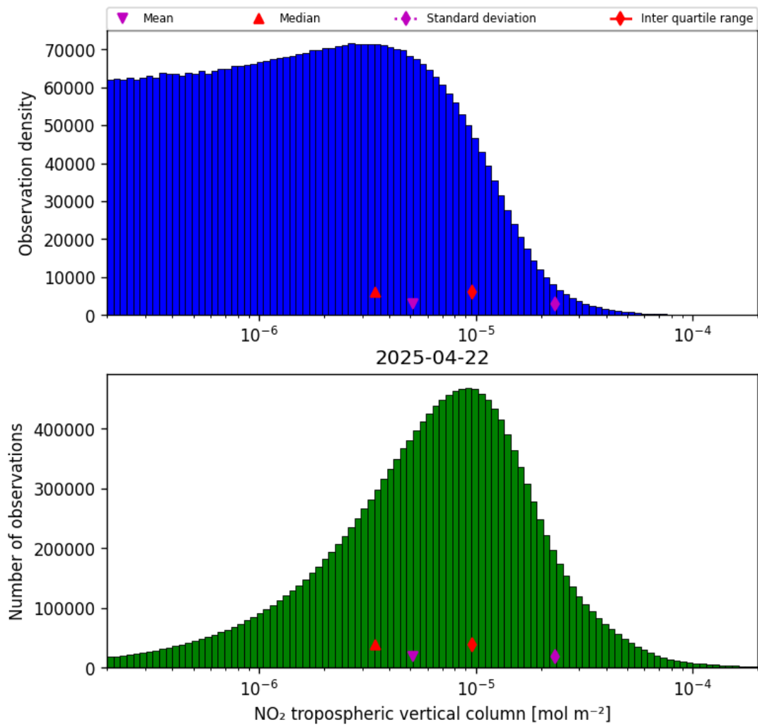
Figure 27: Histogram of “NO 2 tropospheric vertical column” for 2025-04-22 to 2025-04-22
