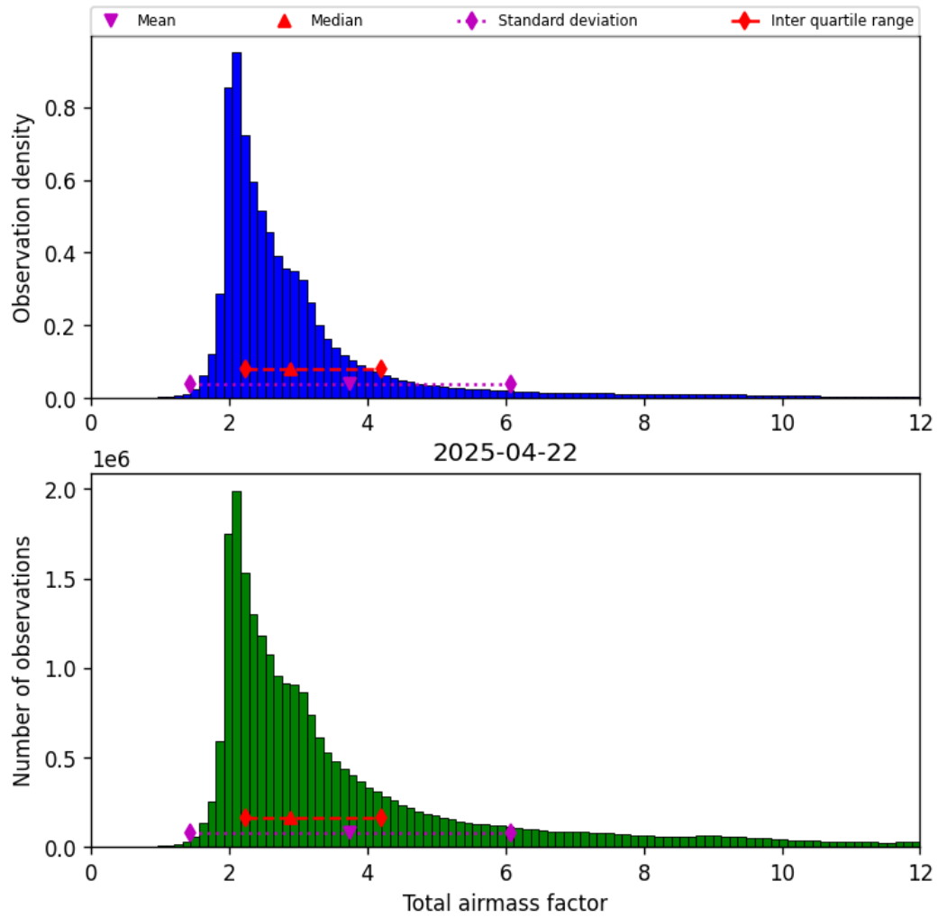
Figure 30: Histogram of “Total airmass factor” for 2025-04-22 to 2025-04-22
