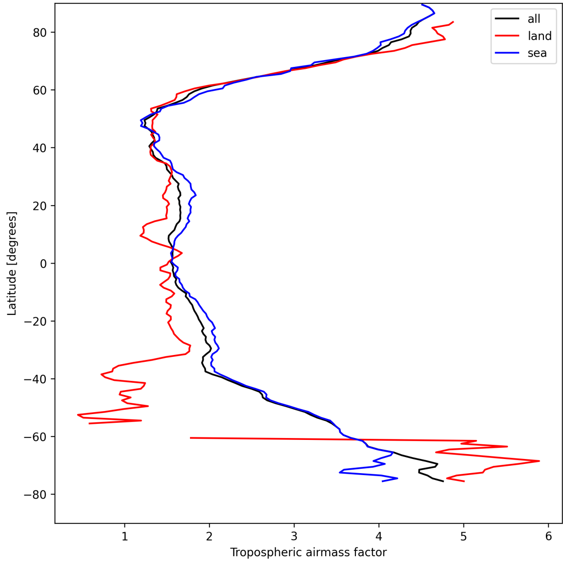
Figure 12: Zonal average of “Tropospheric airmass factor” for 2025-04-22 to 2025-04-22.
