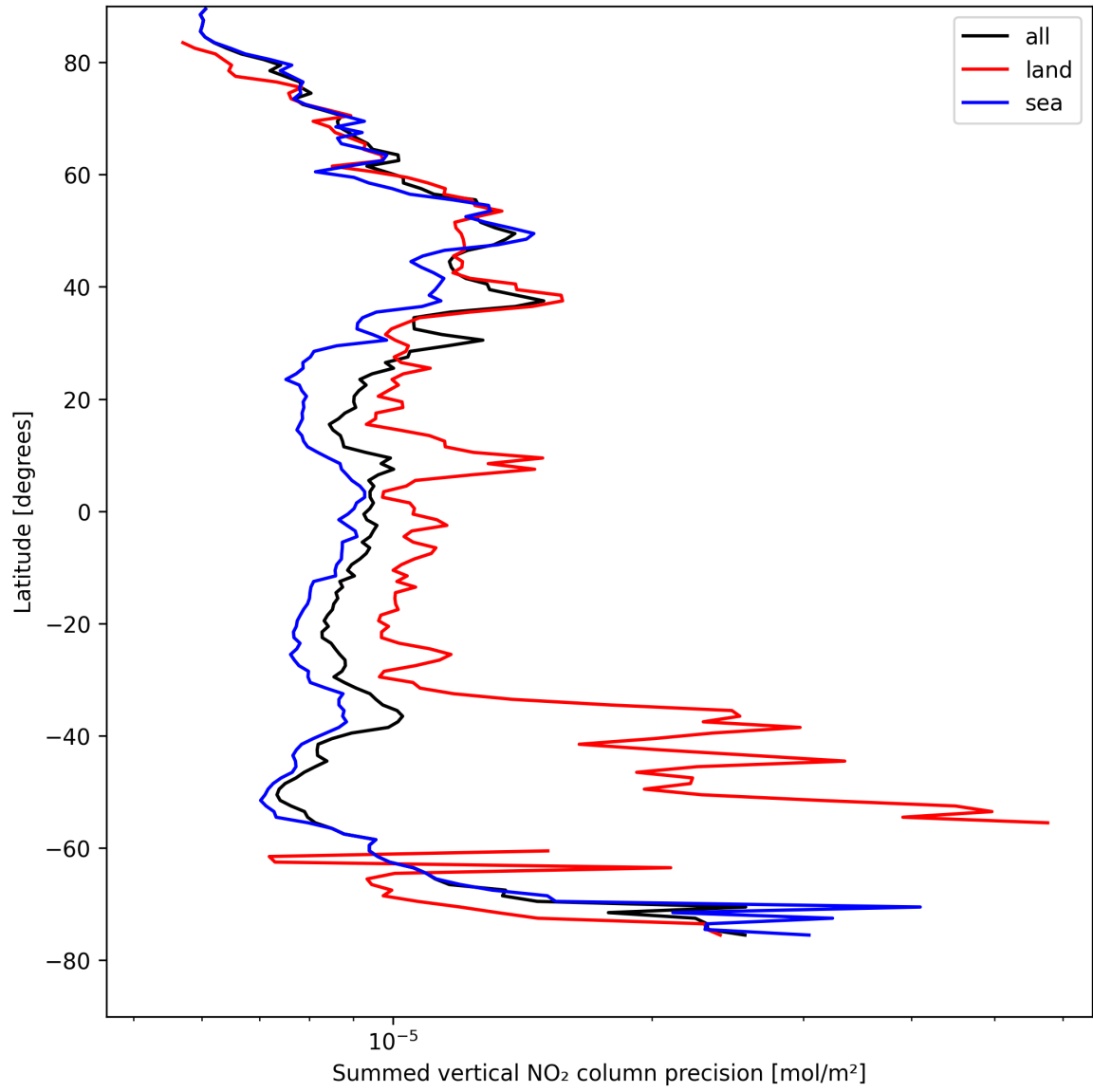
Figure 22: Zonal average of “Summed vertical NO 2 column precision” for 2025-04-22 to 2025-04-22.
