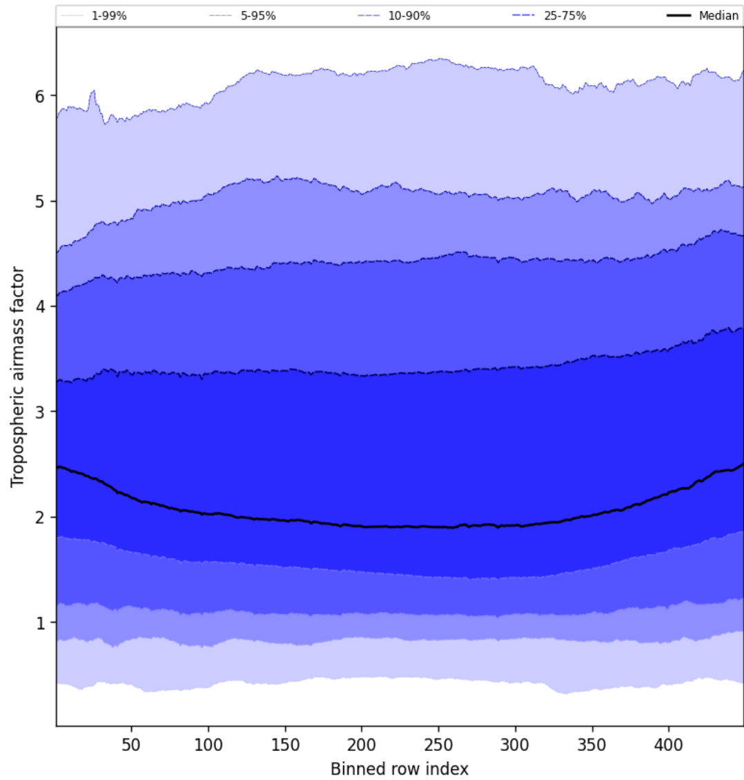
Figure 46: Along track statistics of “Tropospheric airmass factor” for 2025-04-22 to 2025-04-22
