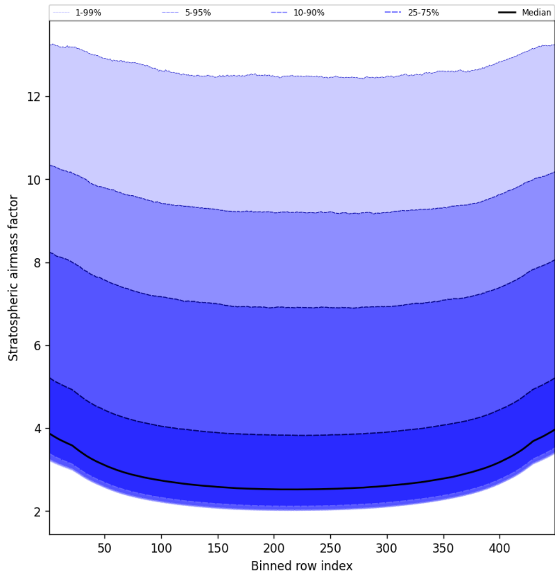
Figure 59: Along track statistics of “Stratospheric airmass factor” for 2025-04-22 to 2025-04-22
