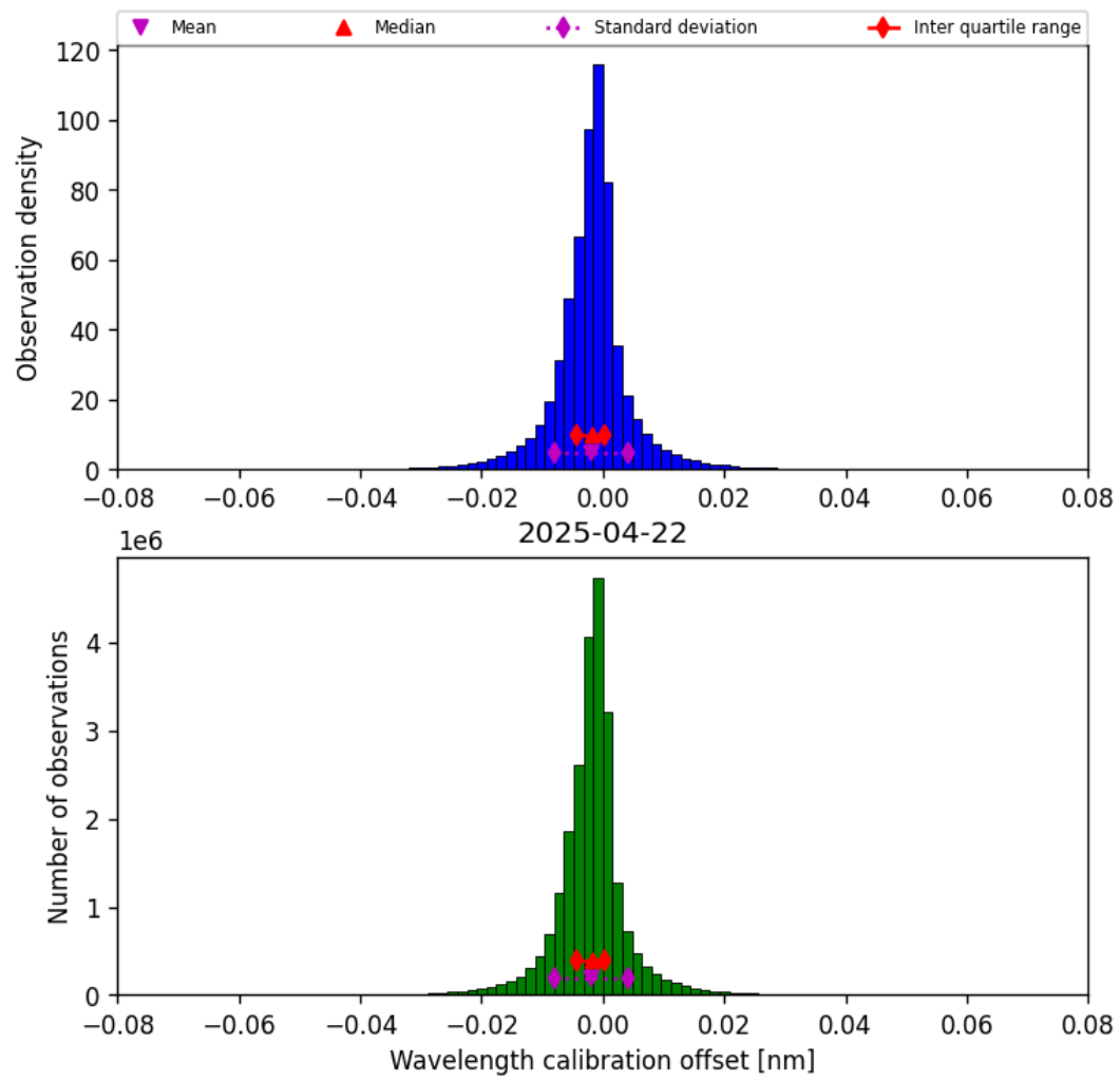
Figure 33: Histogram of “Wavelength calibration offset” for 2025-04-22 to 2025-04-22
