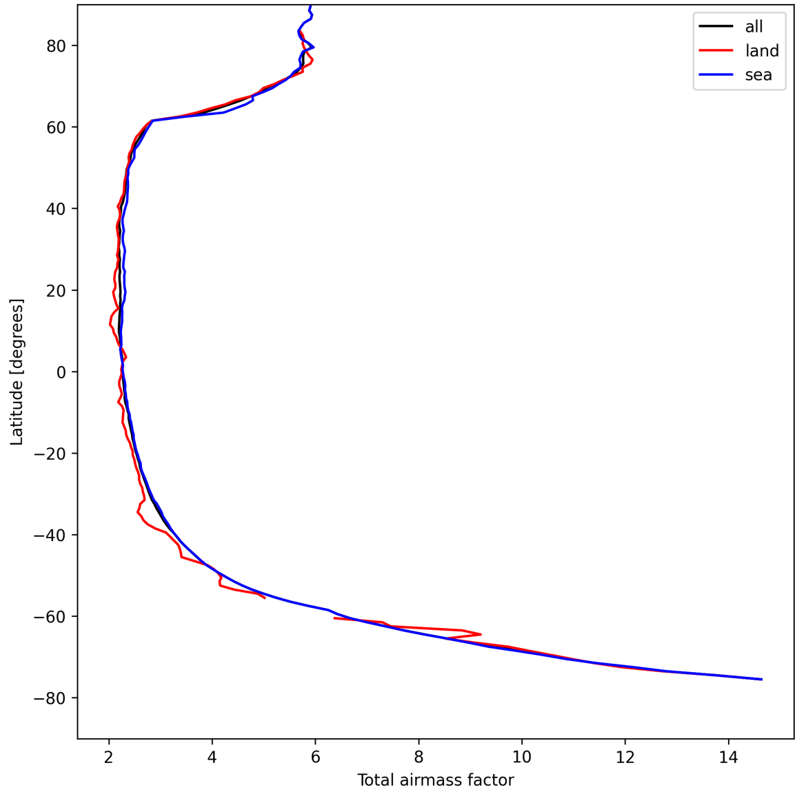
Figure 13: Zonal average of “Total airmass factor” for 2025-04-22 to 2025-04-22.
