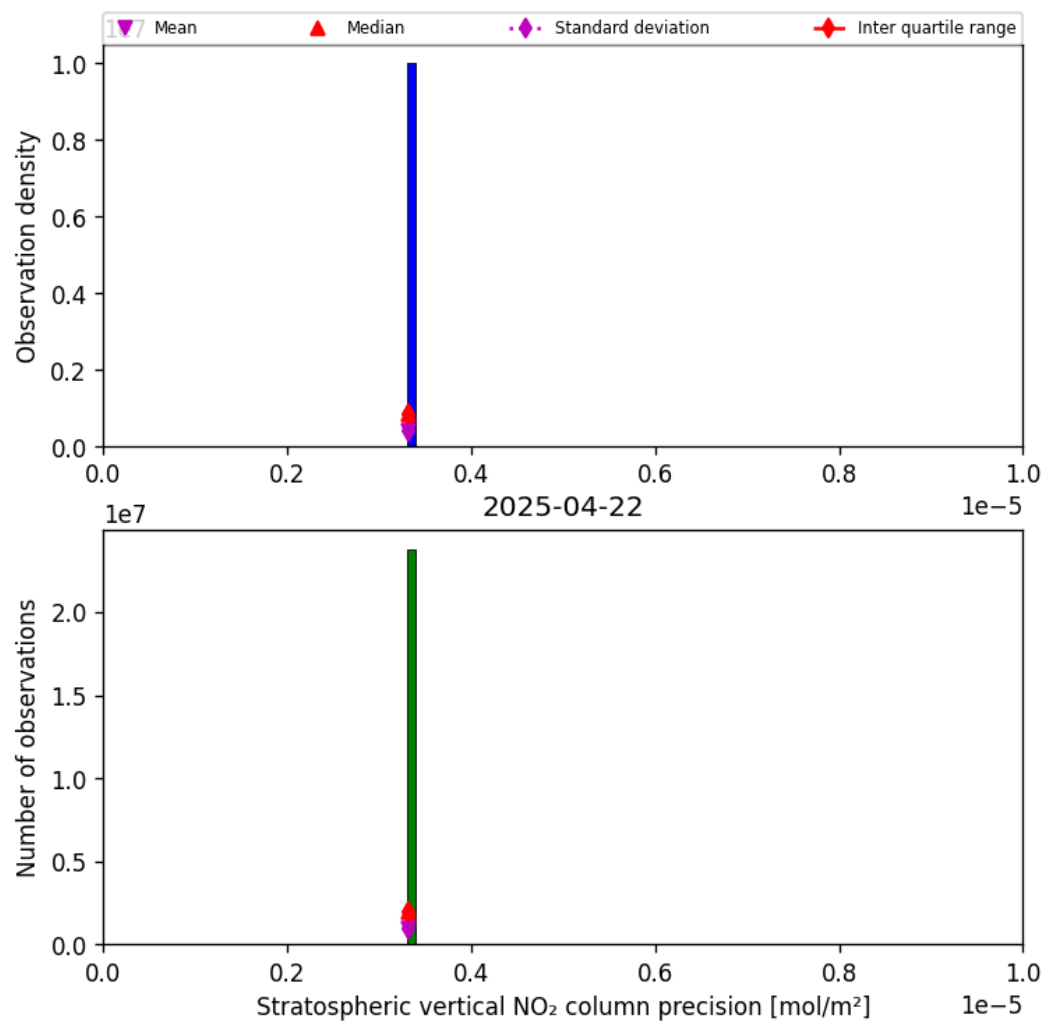
Figure 35: Histogram of “Stratospheric vertical NO 2 column precision” for 2025-04-22 to 2025-04-22
