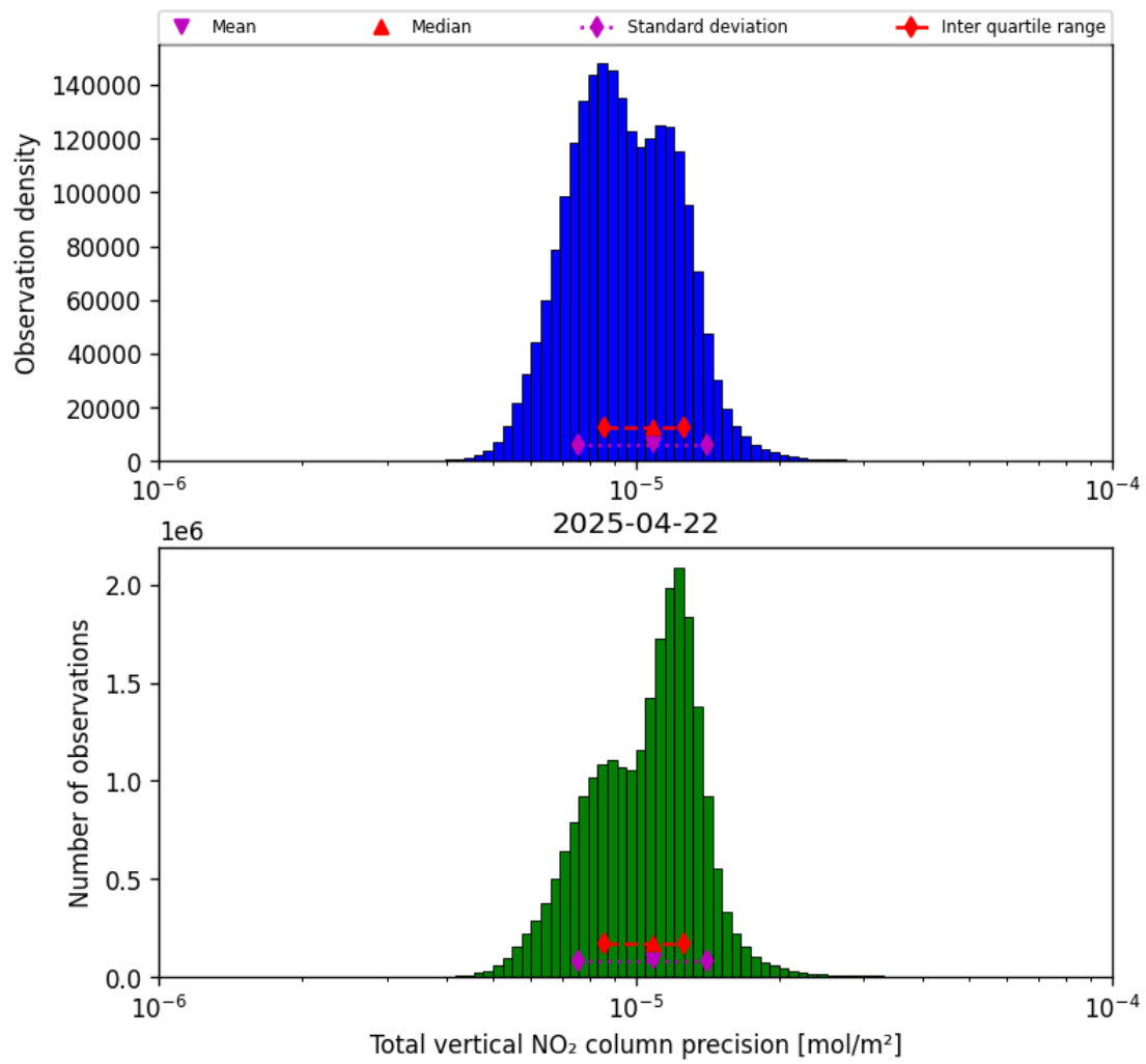
Figure 37: Histogram of "Total vertical NO 2 column precision" for 2025-04-22 to 2025-04-22
