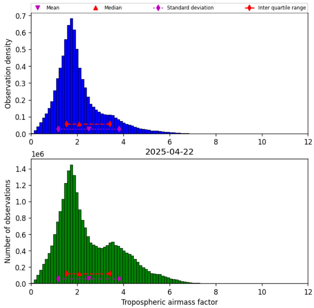
Figure 29: Histogram of “Tropospheric airmass factor” for 2025-04-22 to 2025-04-22
