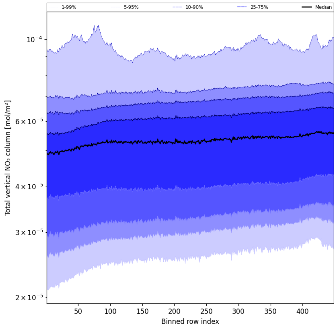
Figure 53: Along track statistics of “Total vertical NO 2 column” for 2025-04-22 to 2025-04-22
