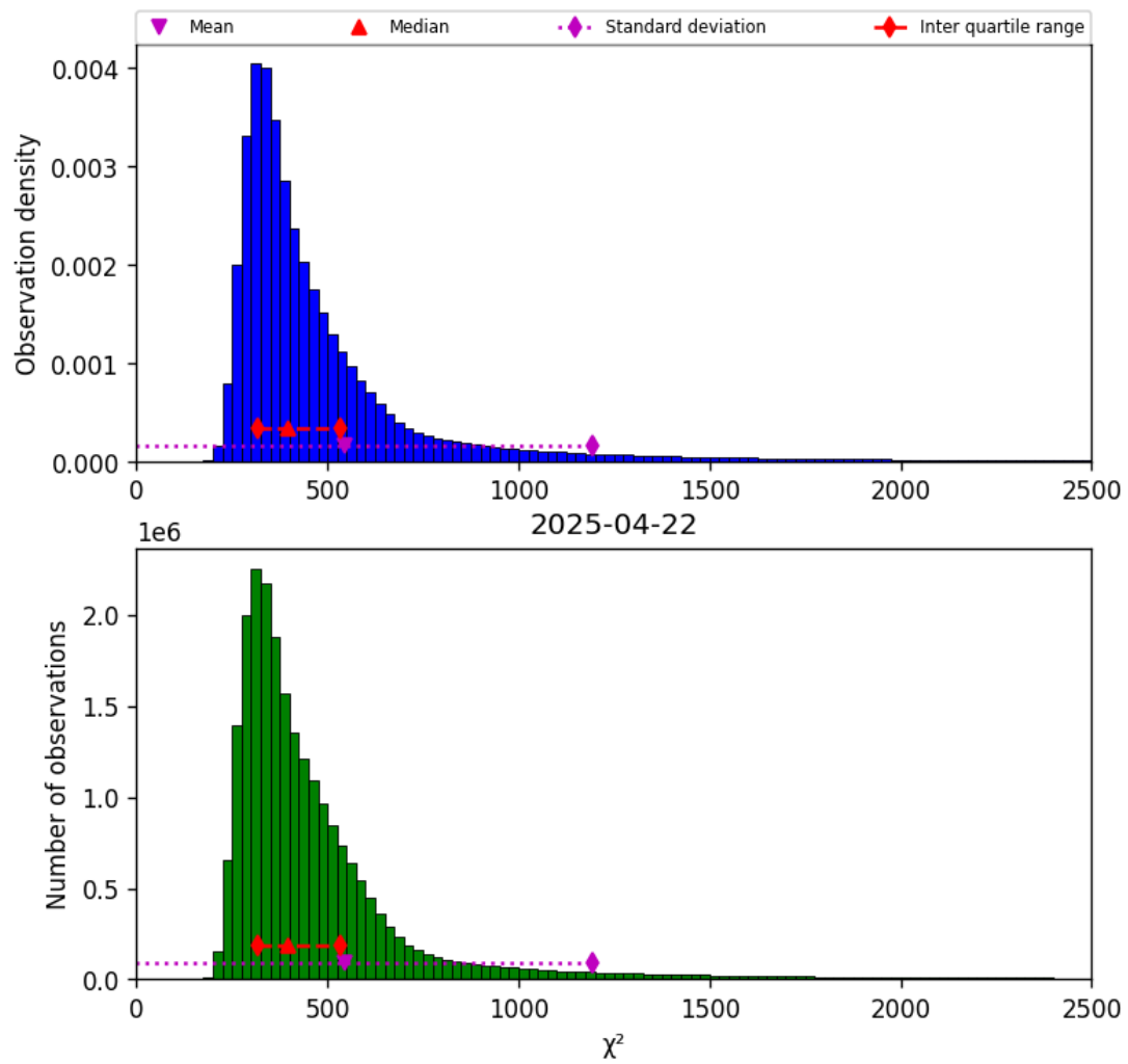
Figure 40: Histogram of “ \chi^2 ” for 2025-04-22 to 2025-04-22
