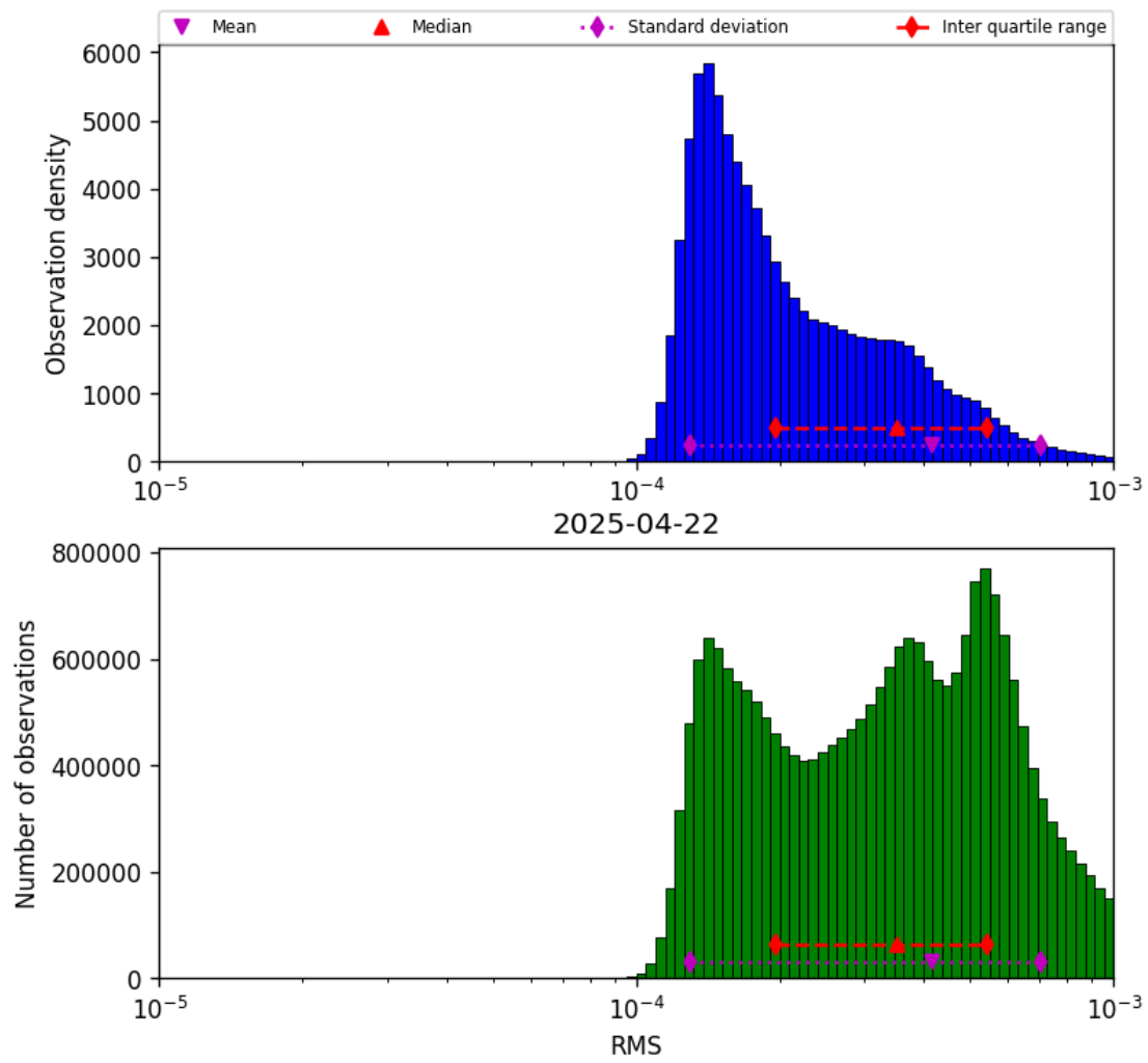
Figure 41: Histogram of “RMS” for 2025-04-22 to 2025-04-22
