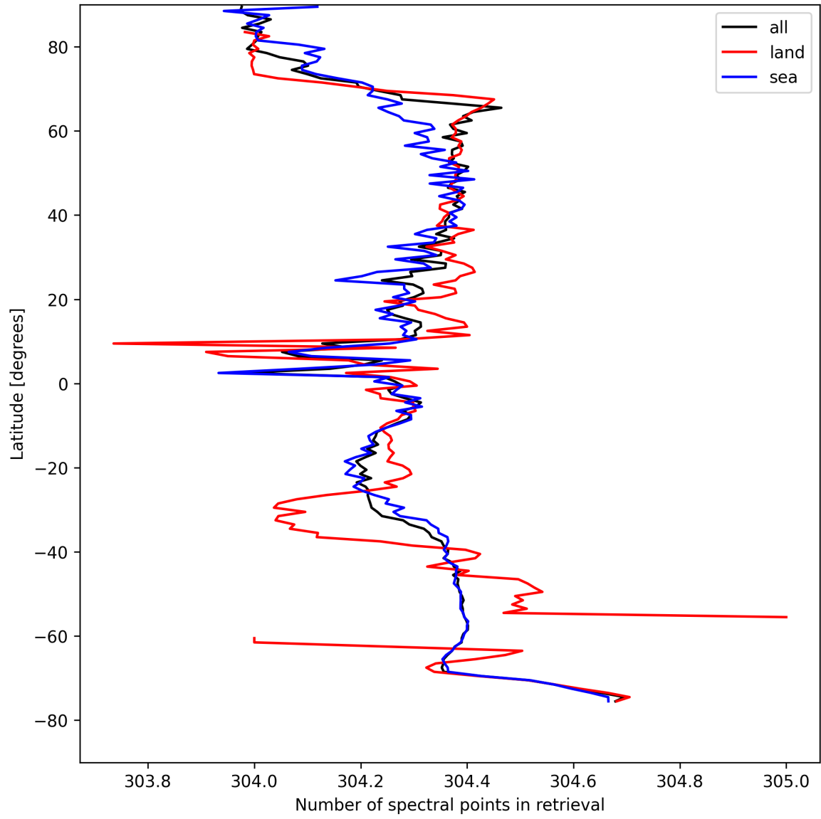
Figure 14: Zonal average of “Number of spectral points in retrieval” for 2025-04-22 to 2025-04-22.
