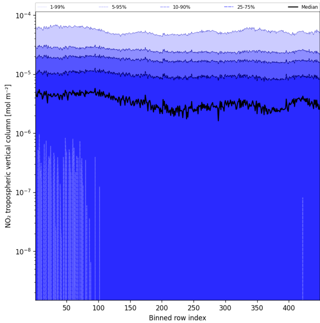
Figure 44: Along track statistics of “NO 2 tropospheric vertical column” for 2025-04-22 to 2025-04-22
