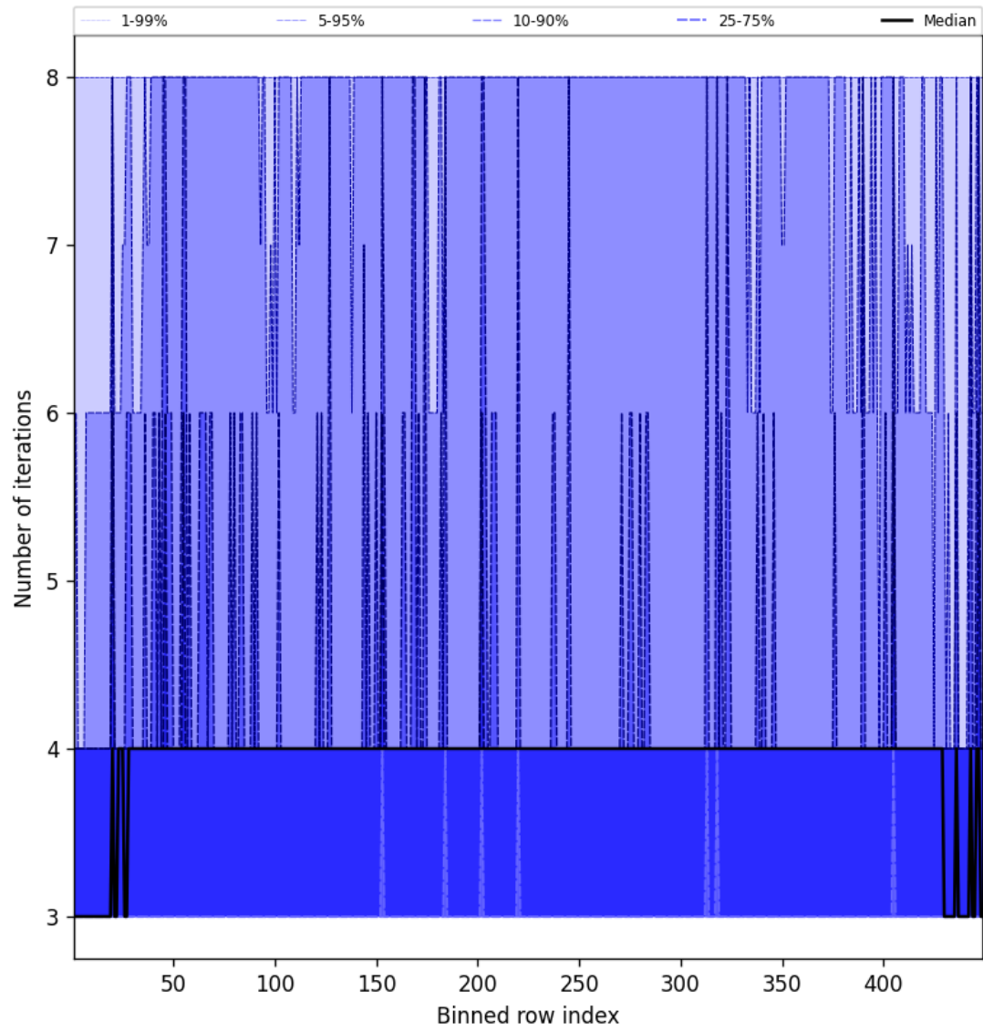
Figure 49: Along track statistics of “Number of iterations” for 2025-04-22 to 2025-04-22
