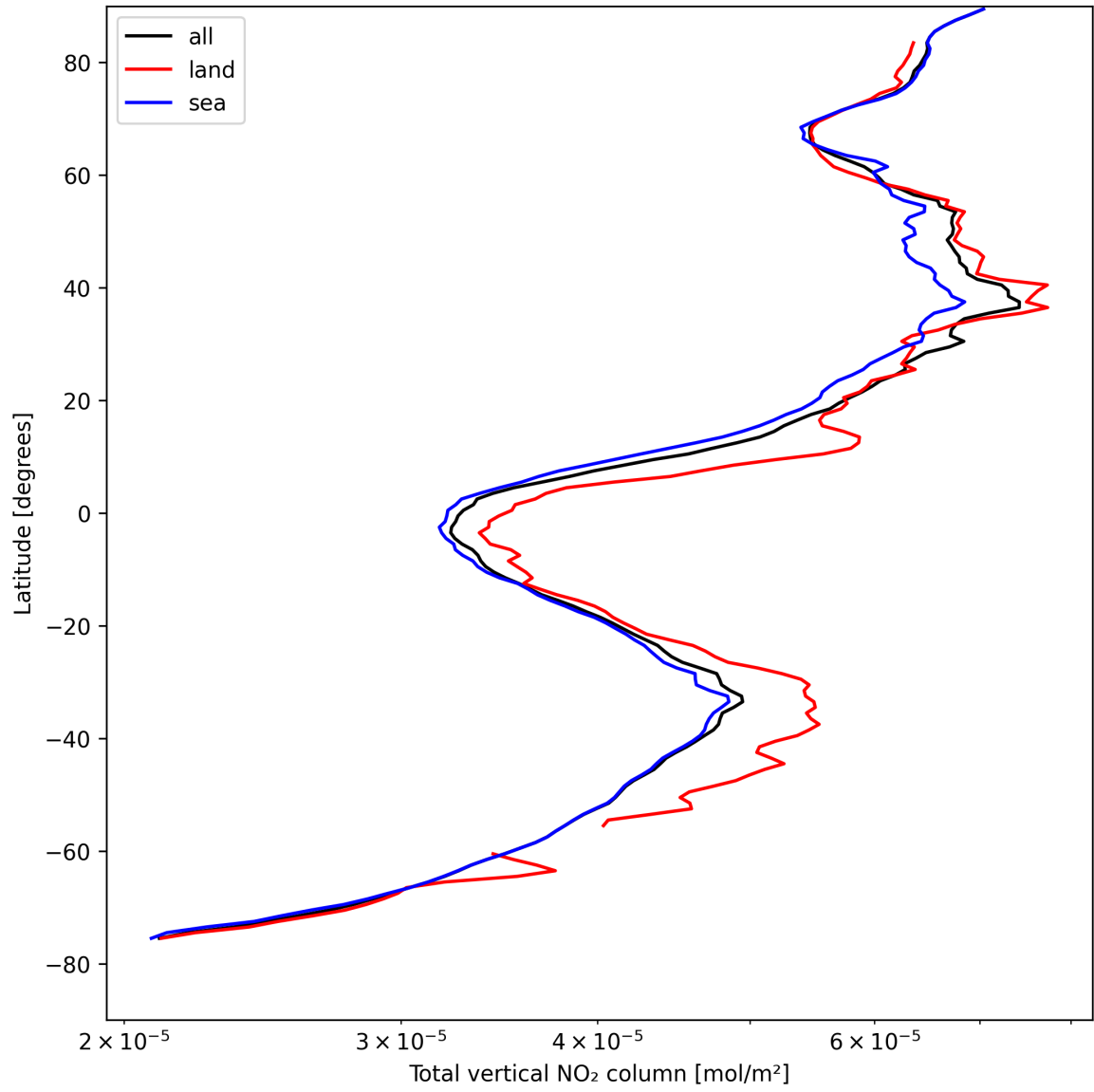
Figure 19: Zonal average of “Total vertical NO 2 column” for 2025-04-22 to 2025-04-22.
