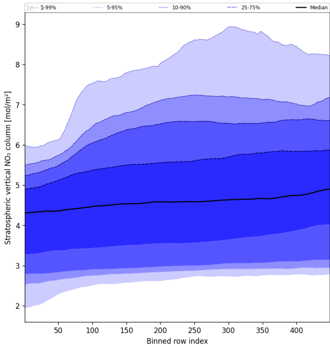
Figure 51: Along track statistics of “Stratospheric vertical NO 2 column” for 2025-04-22 to 2025-04-22
