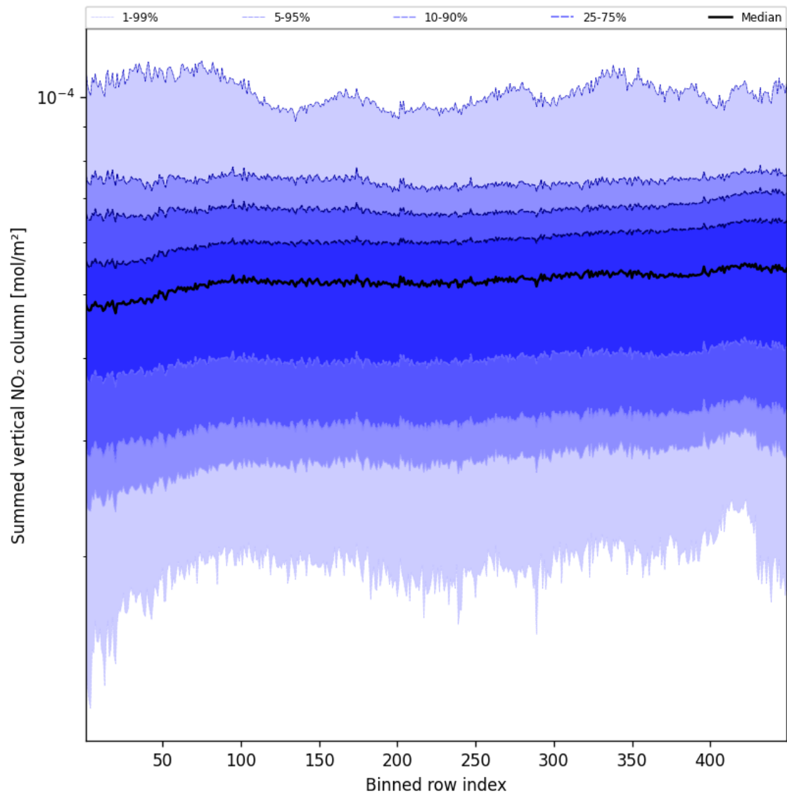
Figure 55: Along track statistics of “Summed vertical NO 2 column” for 2025-04-22 to 2025-04-22
