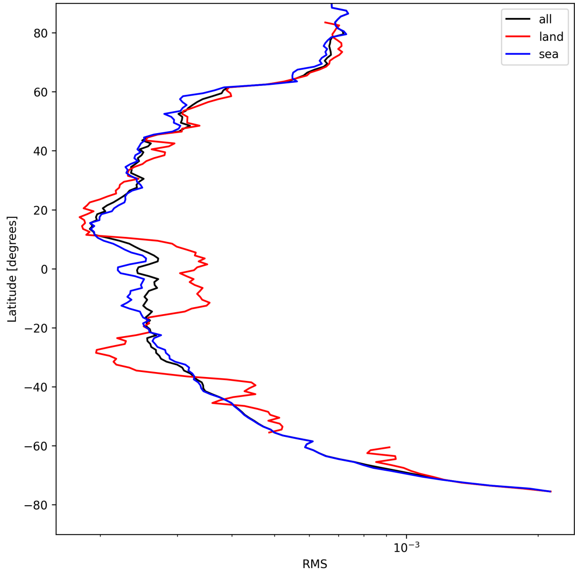
Figure 24: Zonal average of “RMS” for 2025-04-22 to 2025-04-22.
