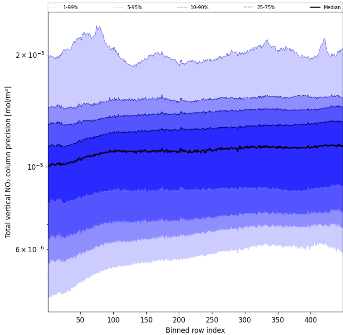
Figure 54: Along track statistics of “Total vertical NO 2 column precision” for 2025-04-22 to 2025-04-22
