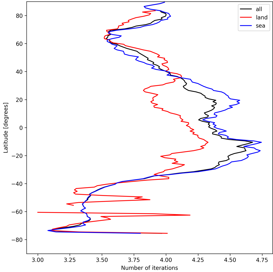
Figure 15: Zonal average of “Number of iterations” for 2025-04-23 to 2025-04-24.
