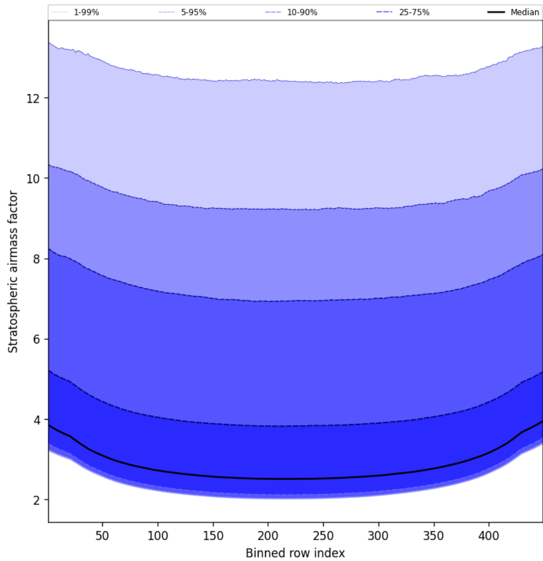
Figure 59: Along track statistics of “Stratospheric airmass factor” for 2025-04-23 to 2025-04-24
