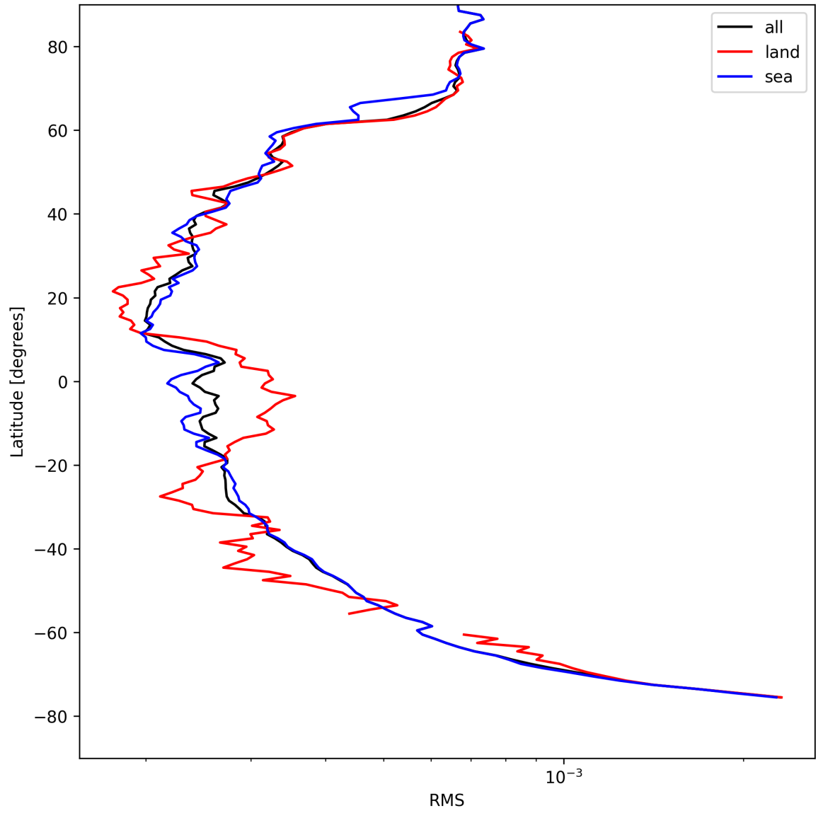
Figure 24: Zonal average of “RMS” for 2025-04-23 to 2025-04-24.
