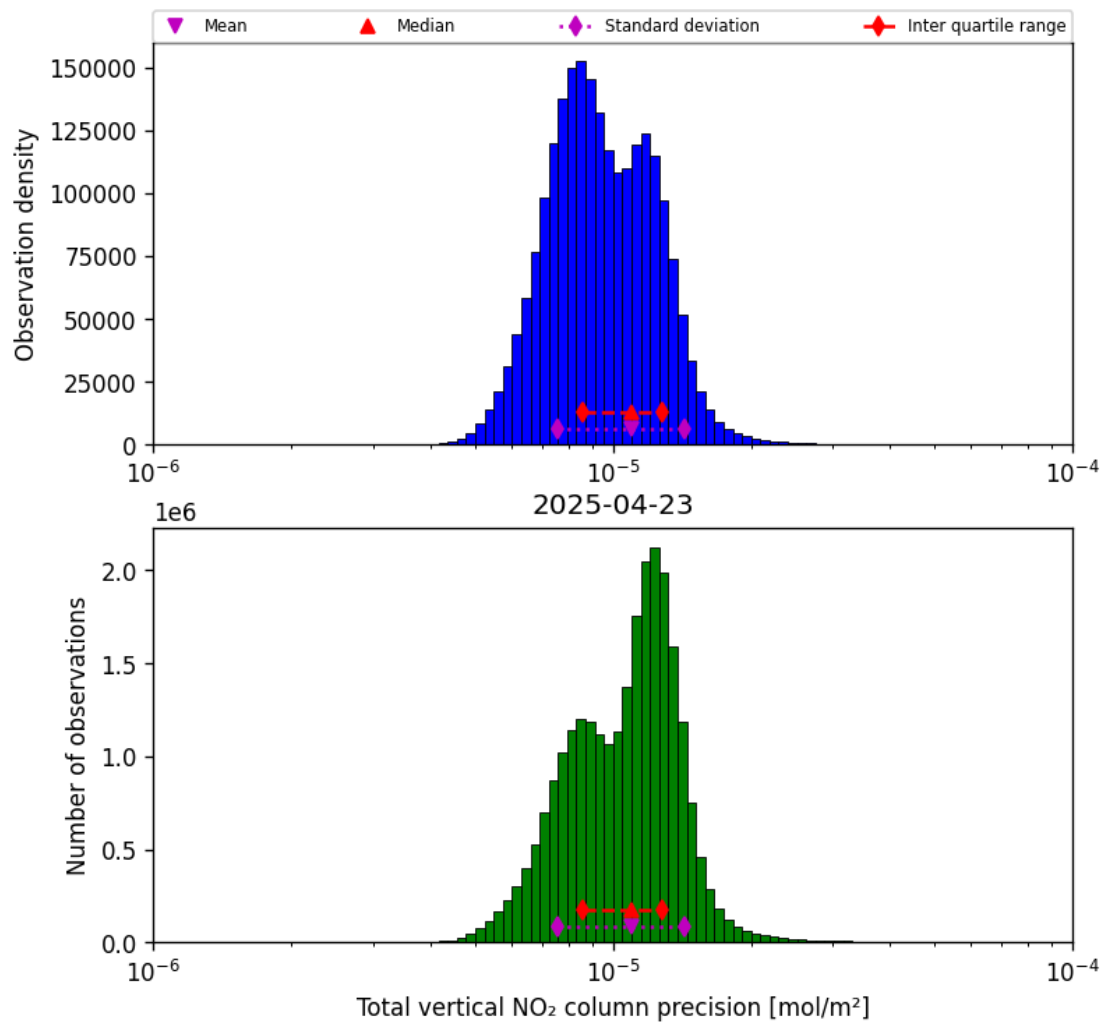
Figure 37: Histogram of “Total vertical NO 2 column precision” for 2025-04-23 to 2025-04-24
