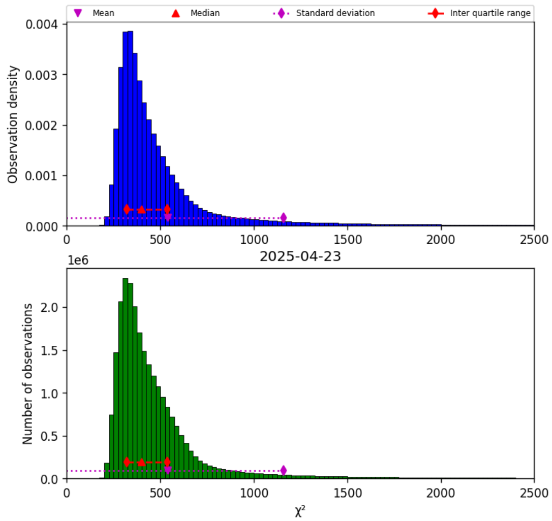
Figure 40: Histogram of “ \chi^2 ” for 2025-04-23 to 2025-04-24
