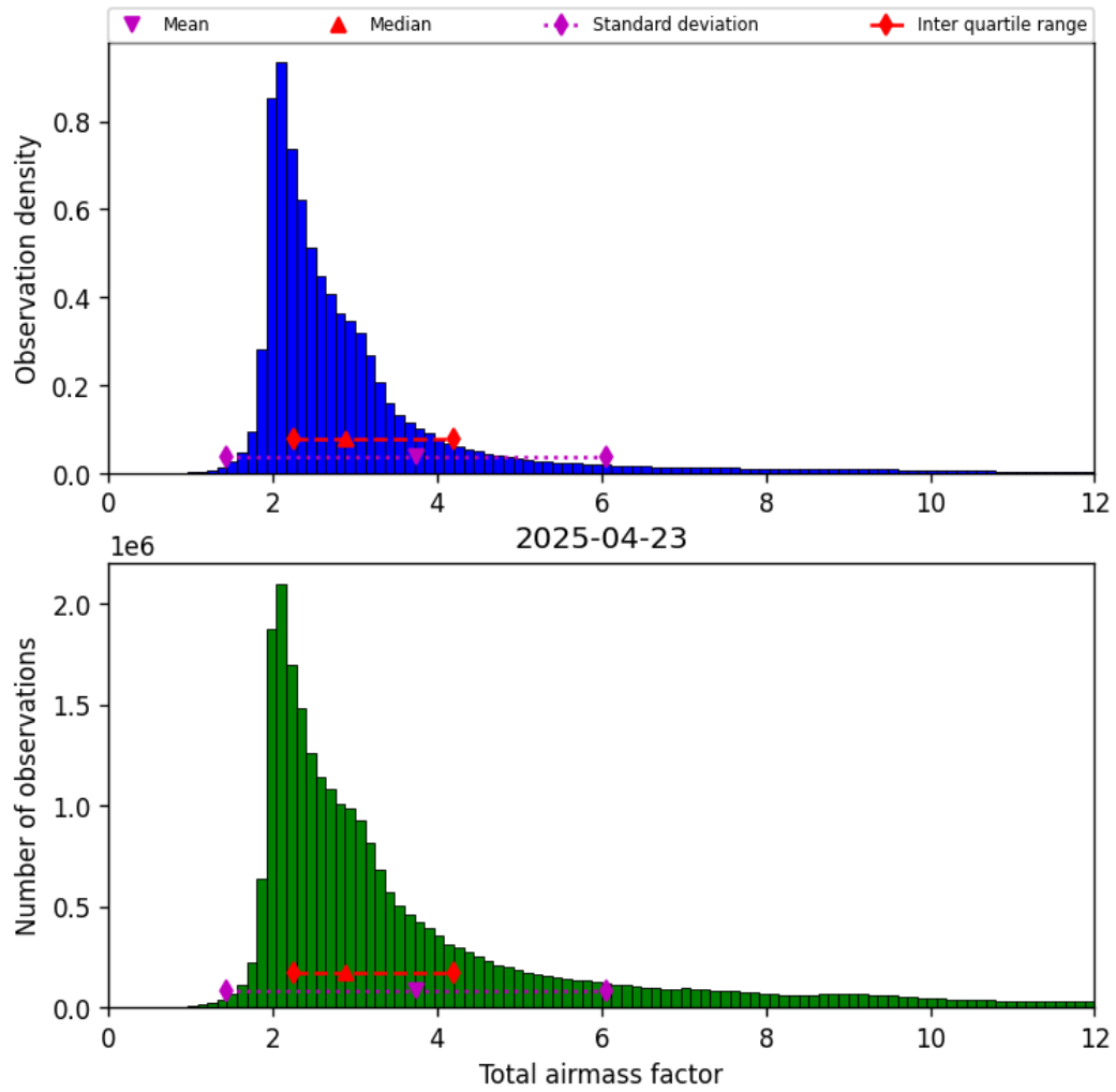
Figure 30: Histogram of “Total airmass factor” for 2025-04-23 to 2025-04-24
