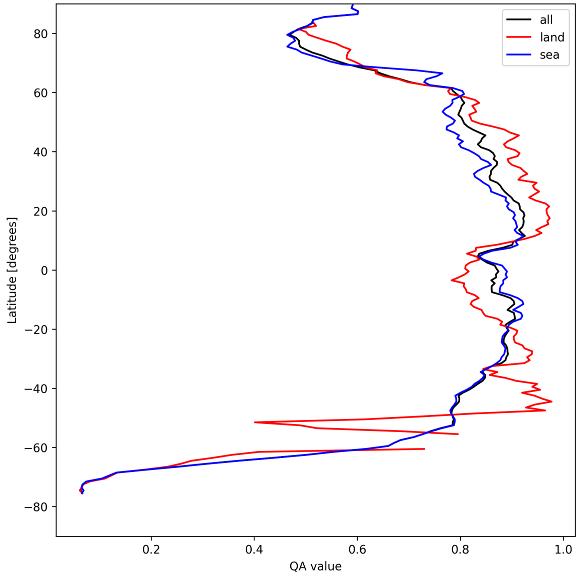
Figure 9: Zonal average of “QA value” for 2025-04-23 to 2025-04-24.
