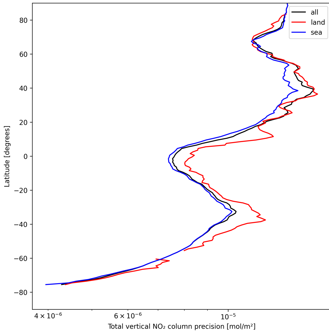
Figure 20: Zonal average of “Total vertical NO 2 column precision” for 2025-04-23 to 2025-04-24.
