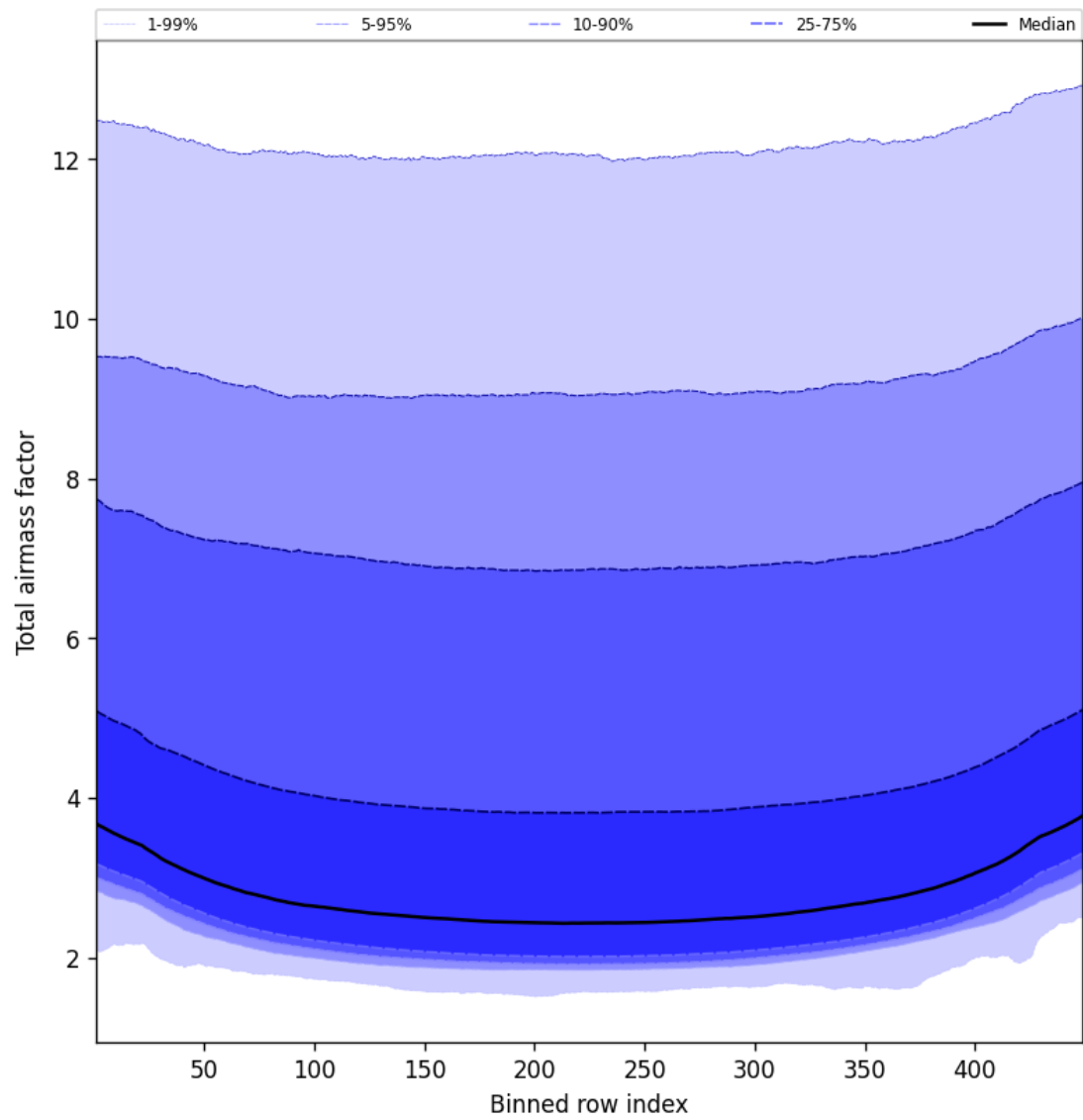
Figure 47: Along track statistics of “Total airmass factor” for 2025-04-23 to 2025-04-24
