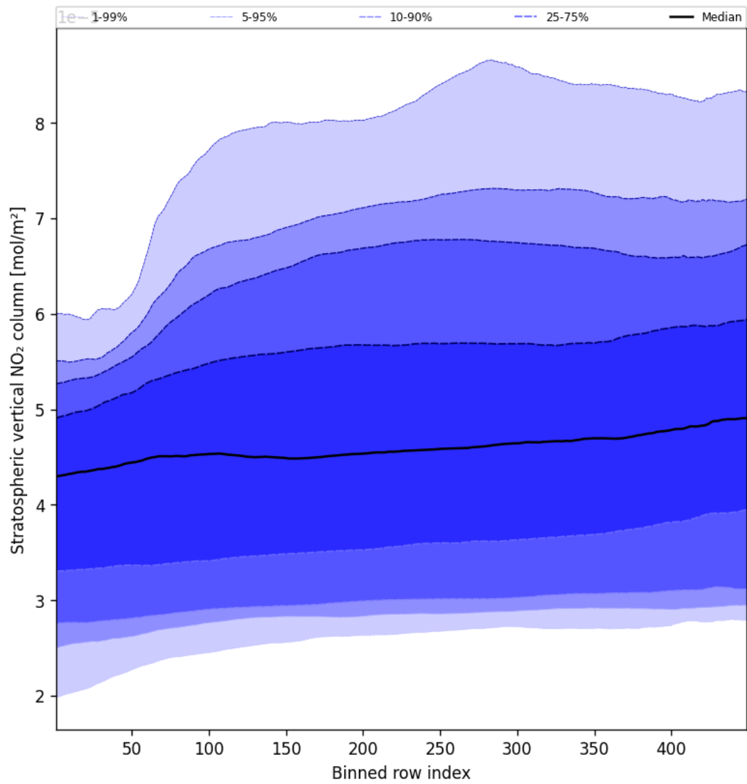
Figure 51: Along track statistics of “Stratospheric vertical NO 2 column” for 2025-04-23 to 2025-04-24
