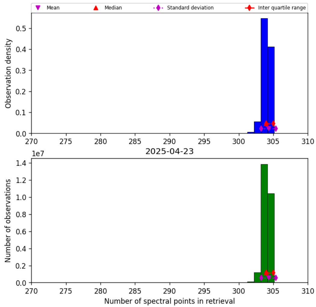
Figure 31: Histogram of “Number of spectral points in retrieval” for 2025-04-23 to 2025-04-24
