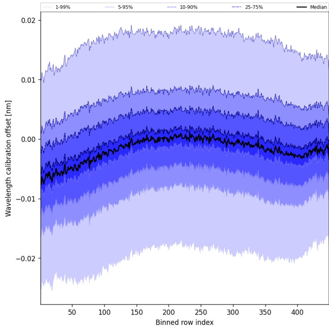
Figure 50: Along track statistics of “Wavelength calibration offset” for 2025-04-23 to 2025-04-24
