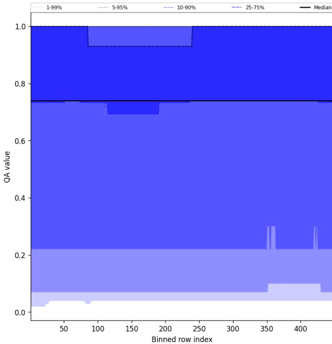
Figure 43: Along track statistics of “QA value” for 2025-04-23 to 2025-04-24
