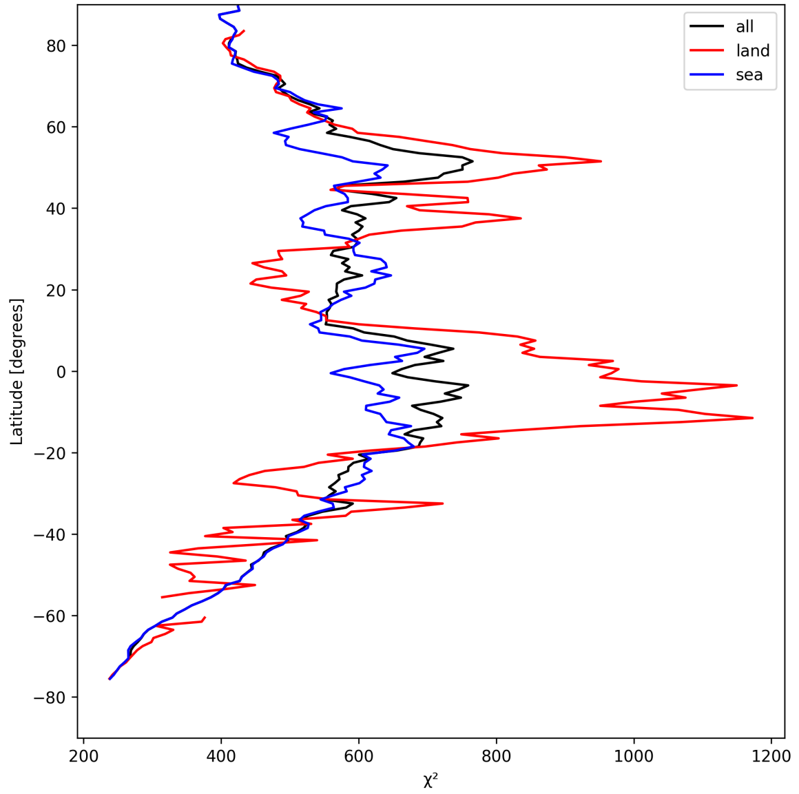
Figure 23: Zonal average of “ \chi^2 ” for 2025-04-23 to 2025-04-24.
