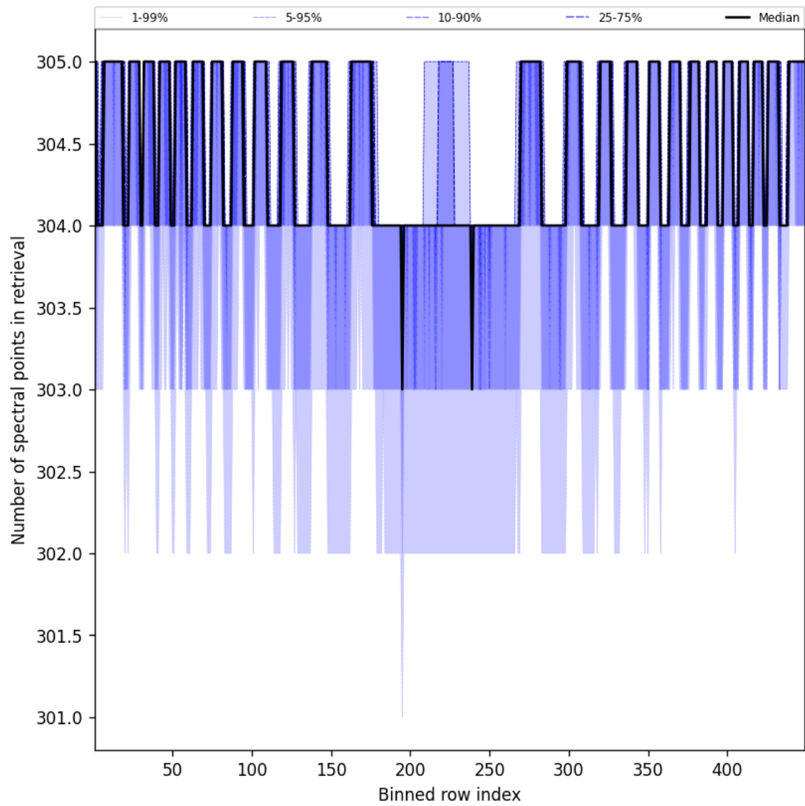
Figure 48: Along track statistics of “Number of spectral points in retrieval” for 2025-04-23 to 2025-04-24
