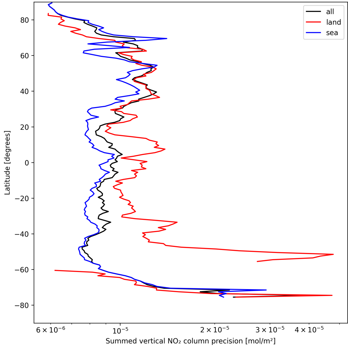
Figure 22: Zonal average of “Summed vertical NO 2 column precision” for 2025-04-23 to 2025-04-24.
