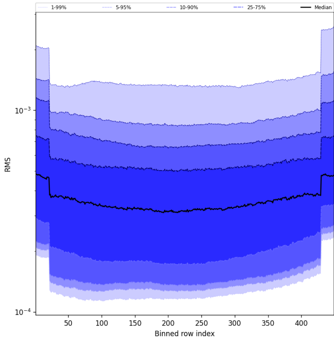
Figure 58: Along track statistics of “RMS” for 2025-04-23 to 2025-04-24
