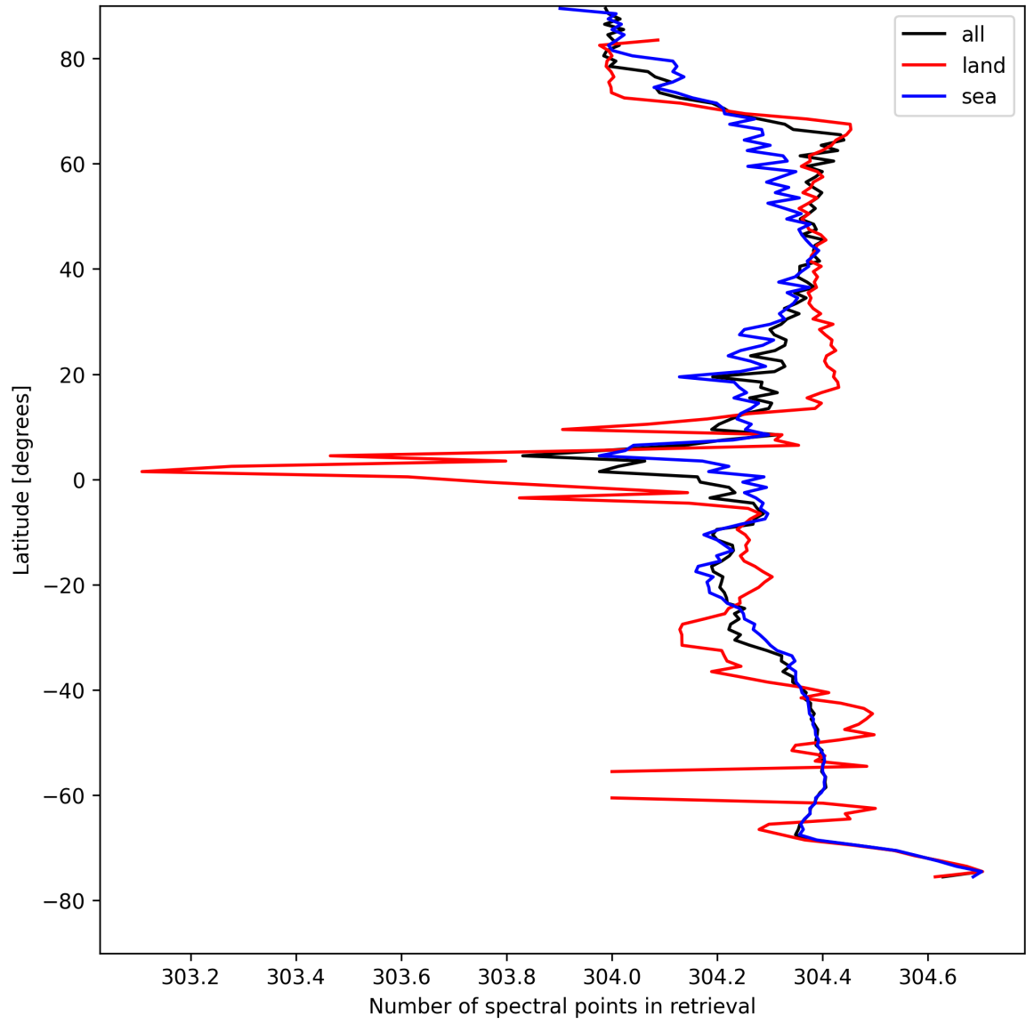
Figure 14: Zonal average of “Number of spectral points in retrieval” for 2025-04-23 to 2025-04-24.
