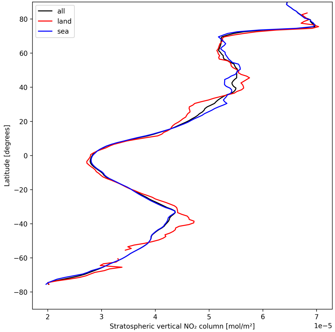
Figure 17: Zonal average of “Stratospheric vertical NO 2 column” for 2025-04-23 to 2025-04-24.
