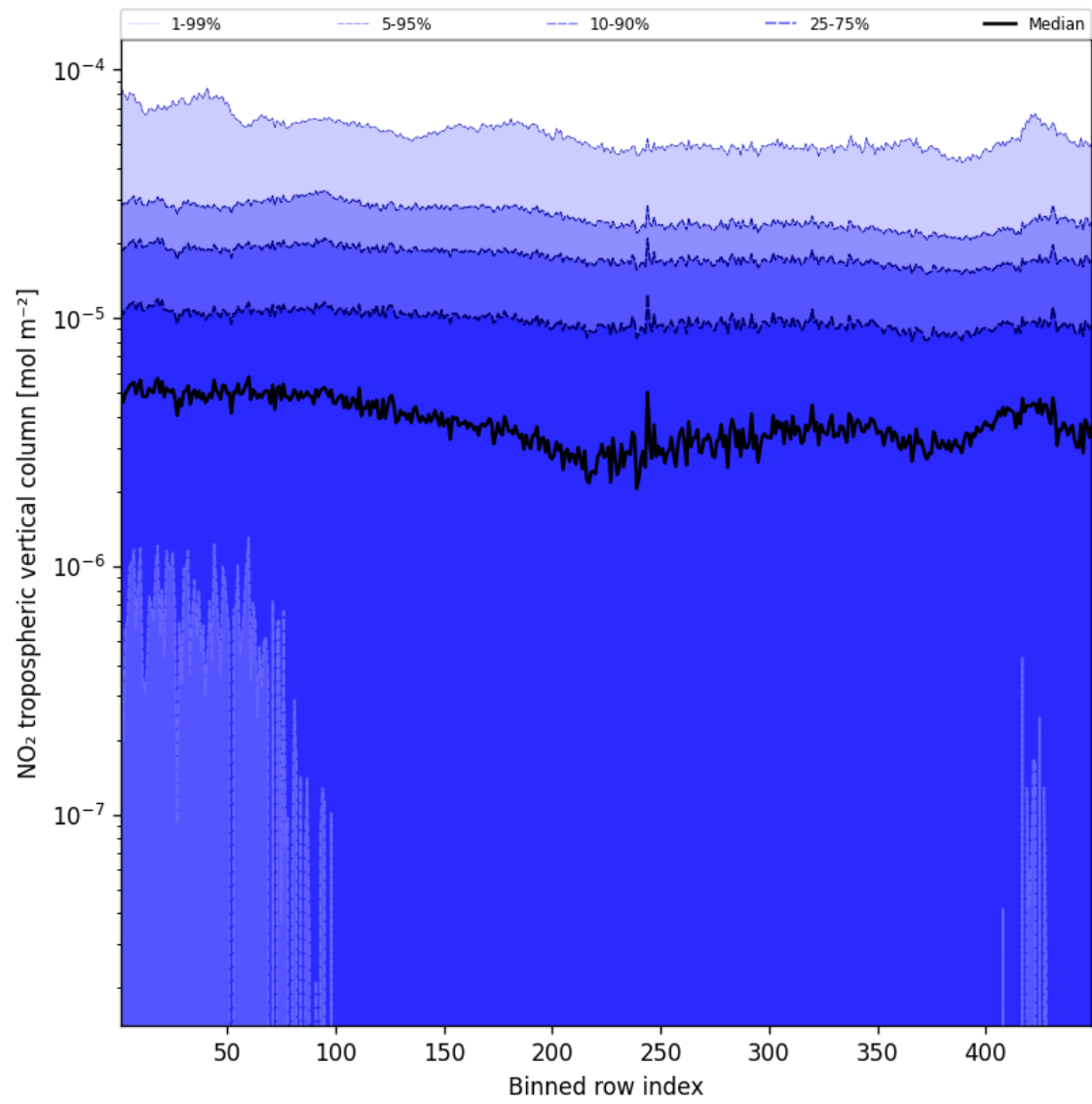
Figure 44: Along track statistics of “NO 2 tropospheric vertical column” for 2025-04-23 to 2025-04-24
