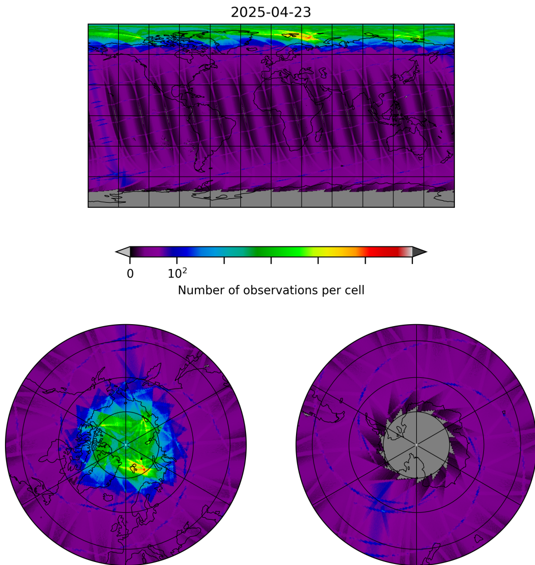
Figure 8: Map of the number of observations for 2025-04-23 to 2025-04-24
