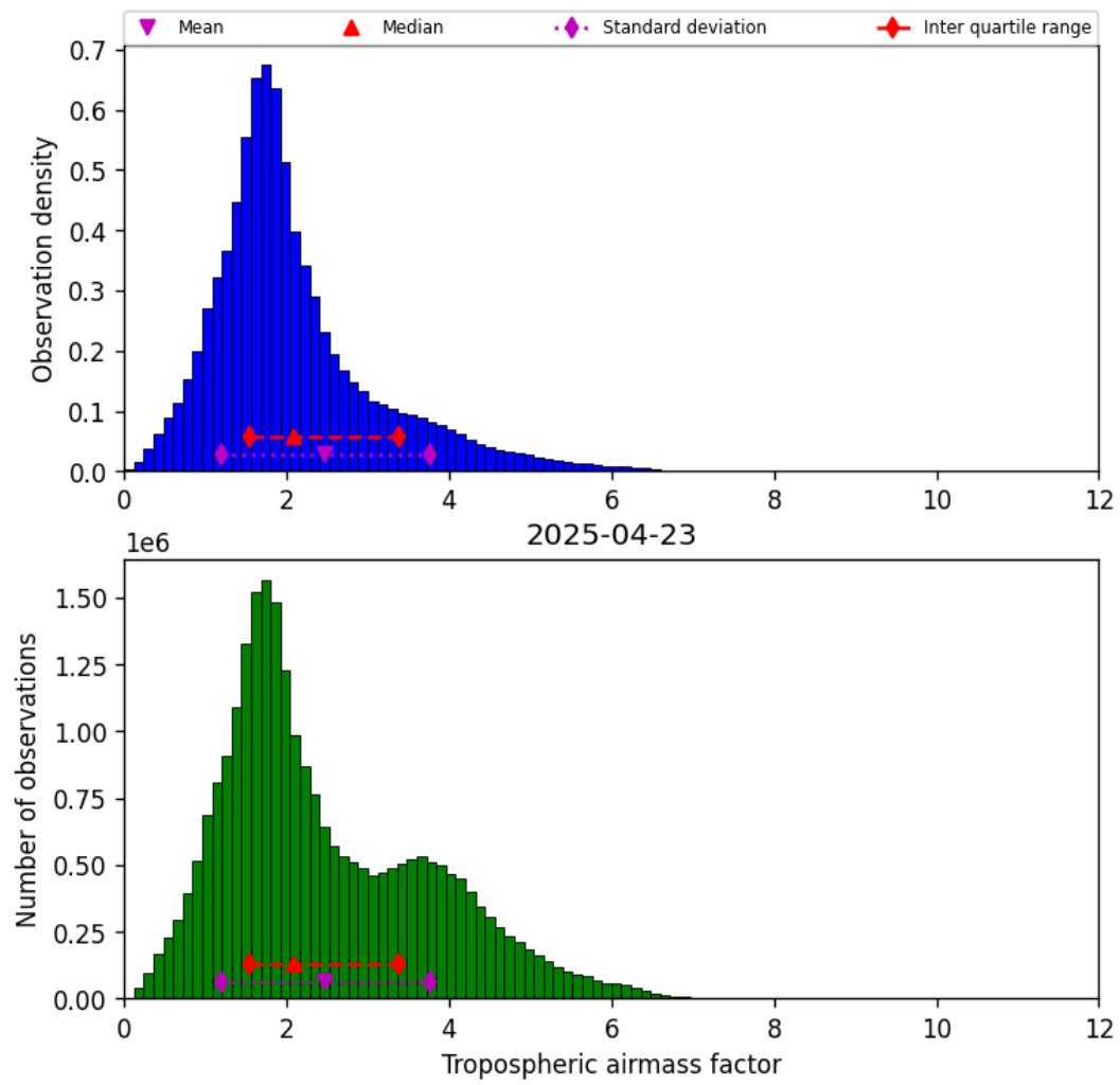
Figure 29: Histogram of “Tropospheric airmass factor” for 2025-04-23 to 2025-04-24
