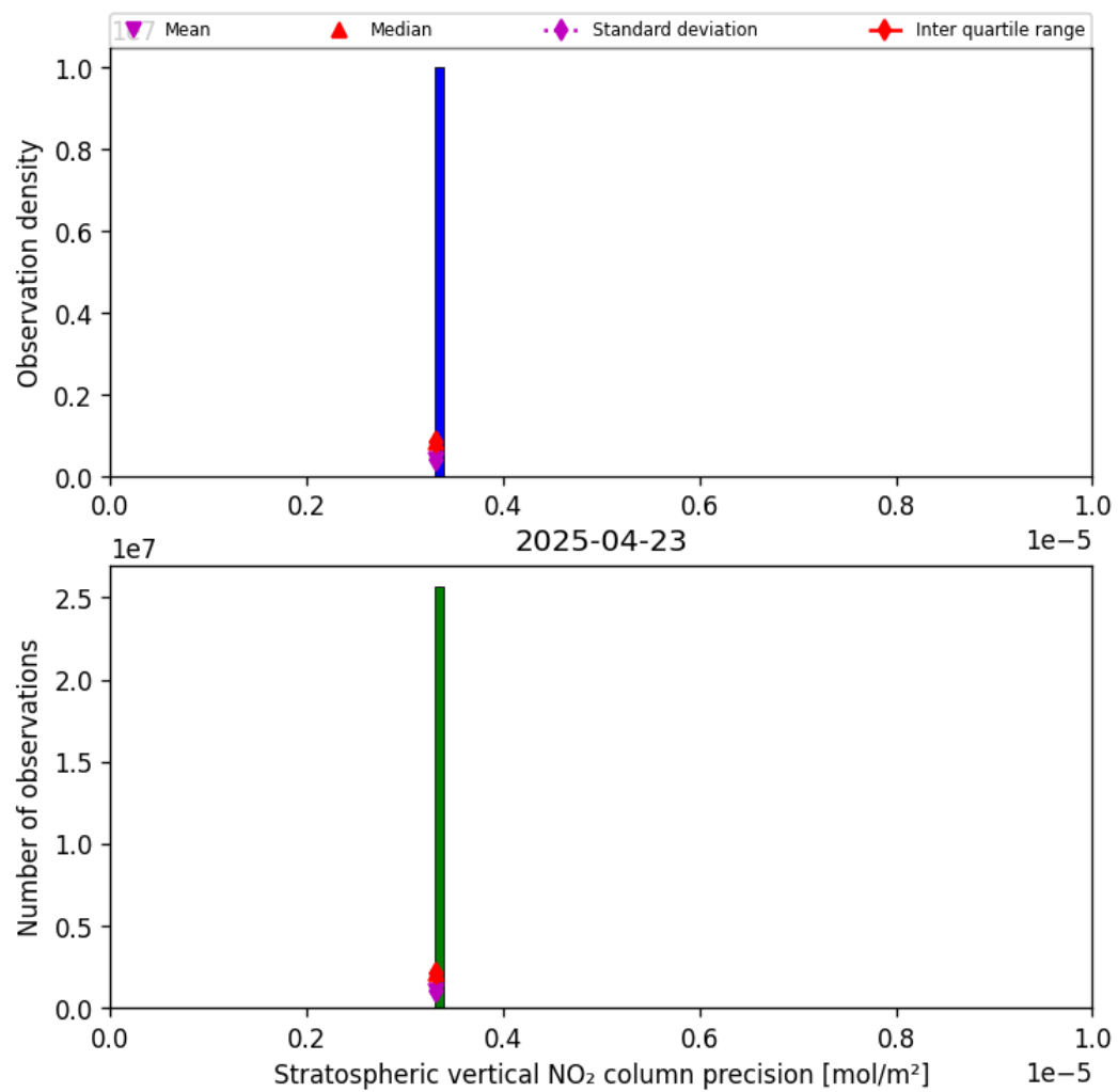
Figure 35: Histogram of “Stratospheric vertical NO 2 column precision” for 2025-04-23 to 2025-04-24
