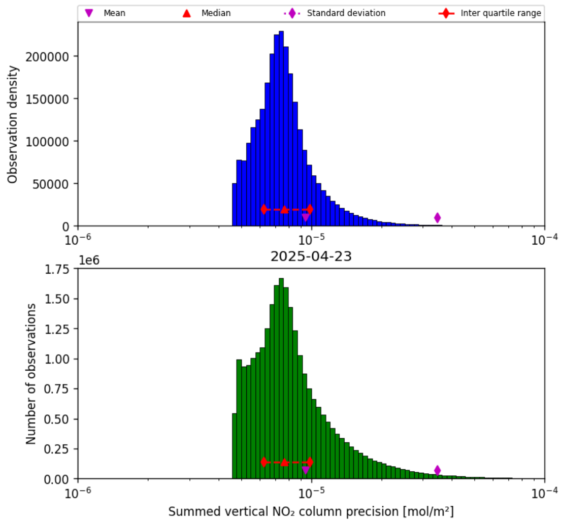
Figure 39: Histogram of “Summed vertical NO 2 column precision” for 2025-04-23 to 2025-04-24
