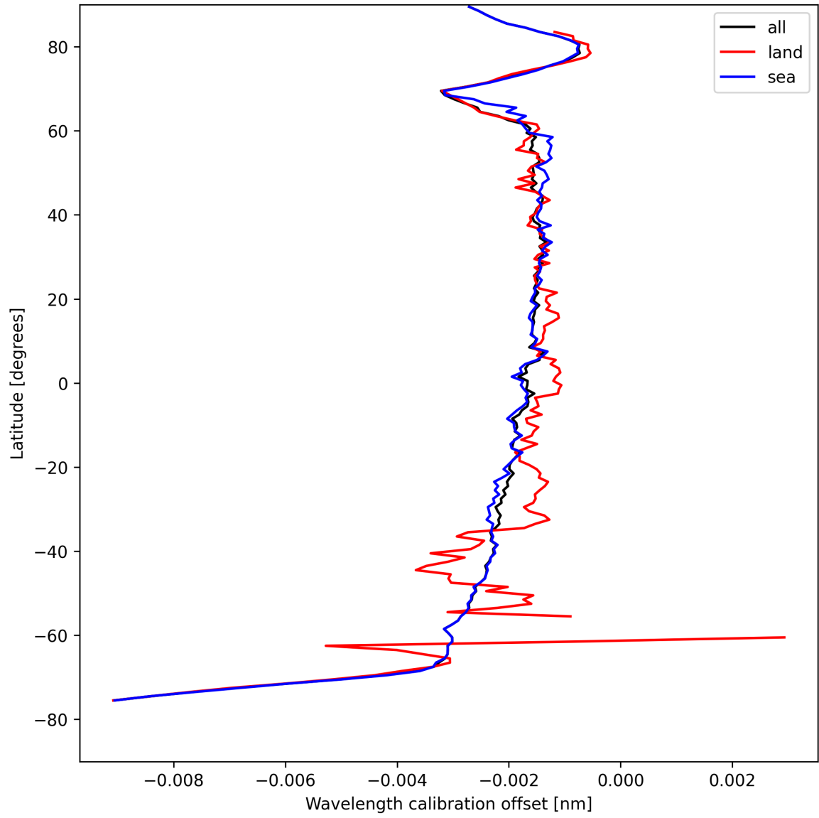
Figure 16: Zonal average of “Wavelength calibration offset” for 2025-04-23 to 2025-04-24.
