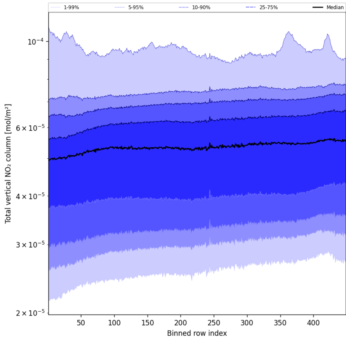
Figure 53: Along track statistics of “Total vertical NO 2 column” for 2025-04-23 to 2025-04-24
