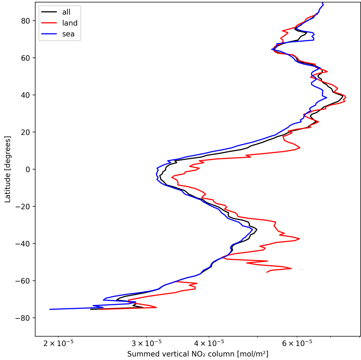
Figure 21: Zonal average of “Summed vertical NO 2 column” for 2025-04-23 to 2025-04-24.
