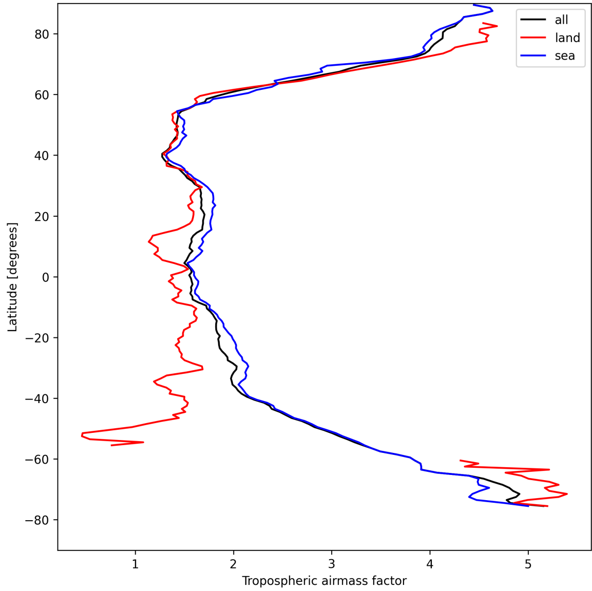
Figure 12: Zonal average of “Tropospheric air mass factor” for 2025-04-23 to 2025-04-24.
