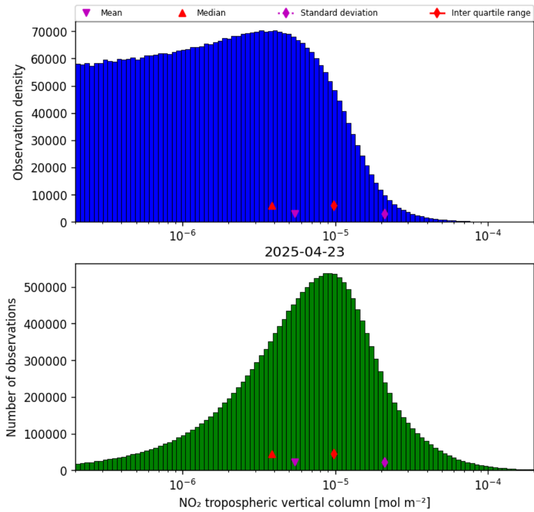
Figure 27: Histogram of “NO 2 tropospheric vertical column” for 2025-04-23 to 2025-04-24
