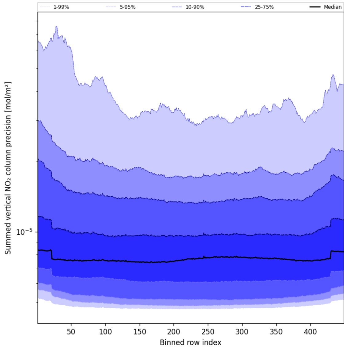
Figure 56: Along track statistics of “Summed vertical NO 2 column precision” for 2025-04-23 to 2025-04-24
