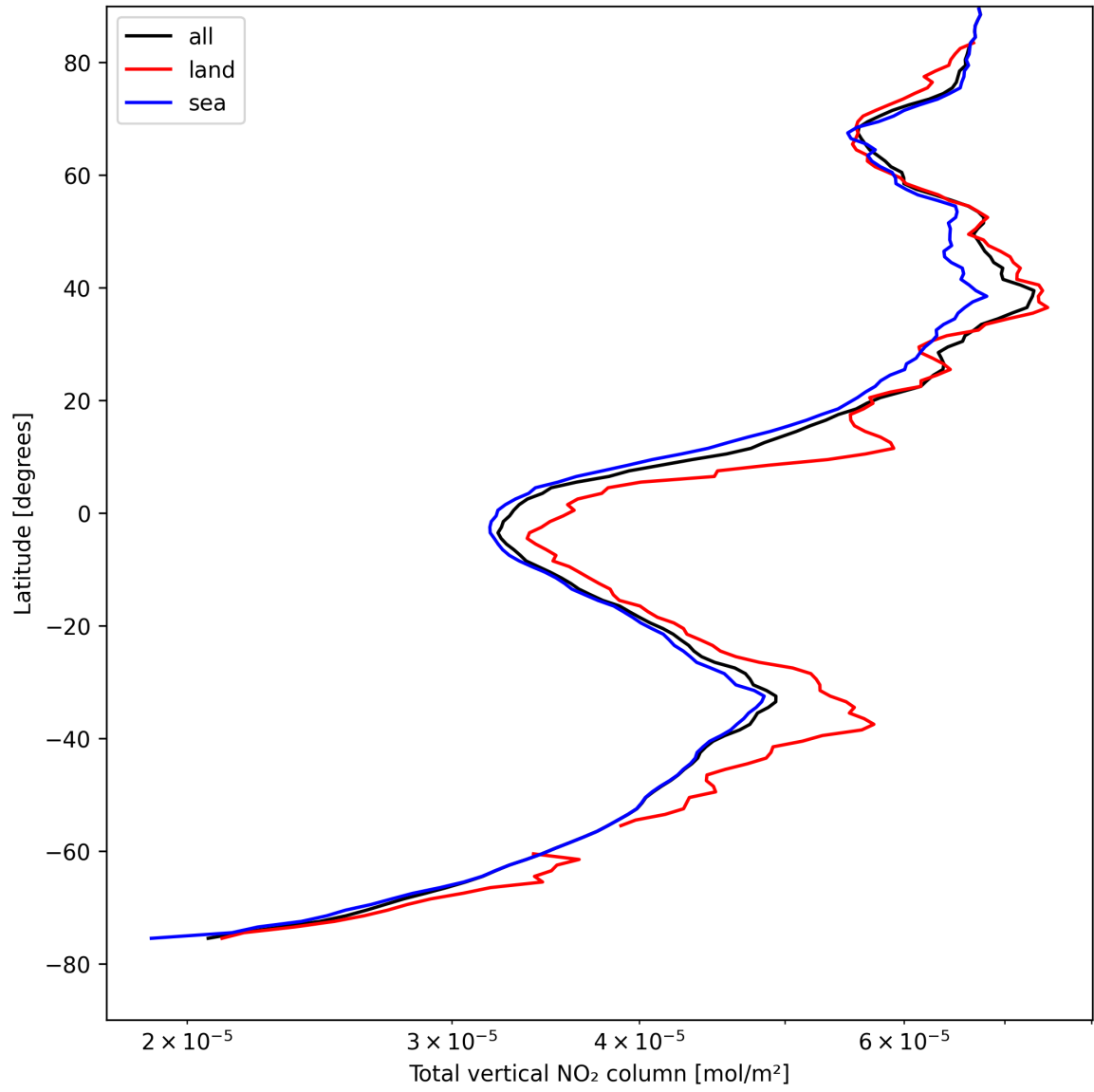
Figure 19: Zonal average of “Total vertical NO 2 column” for 2025-04-23 to 2025-04-24.
