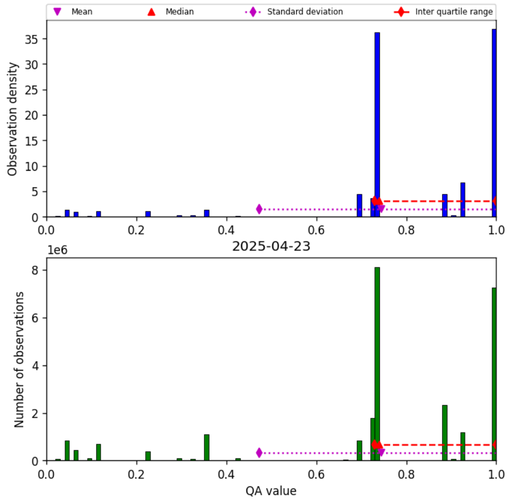
Figure 26: Histogram of “QA value” for 2025-04-23 to 2025-04-24
