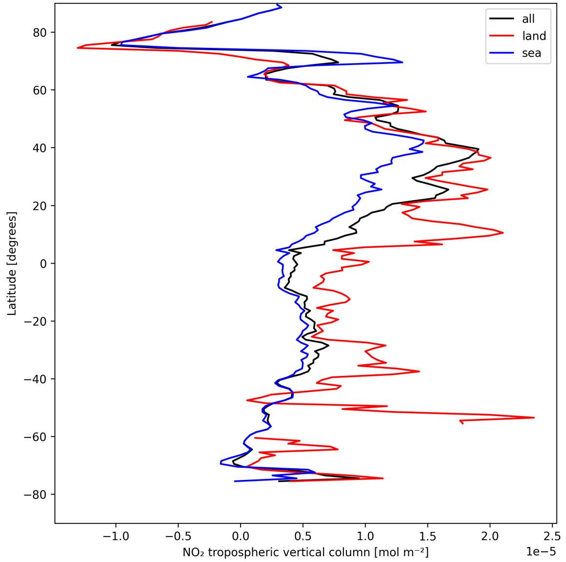
Figure 10: Zonal average of “NO 2 tropospheric vertical column” for 2025-04-23 to 2025-04-24.
