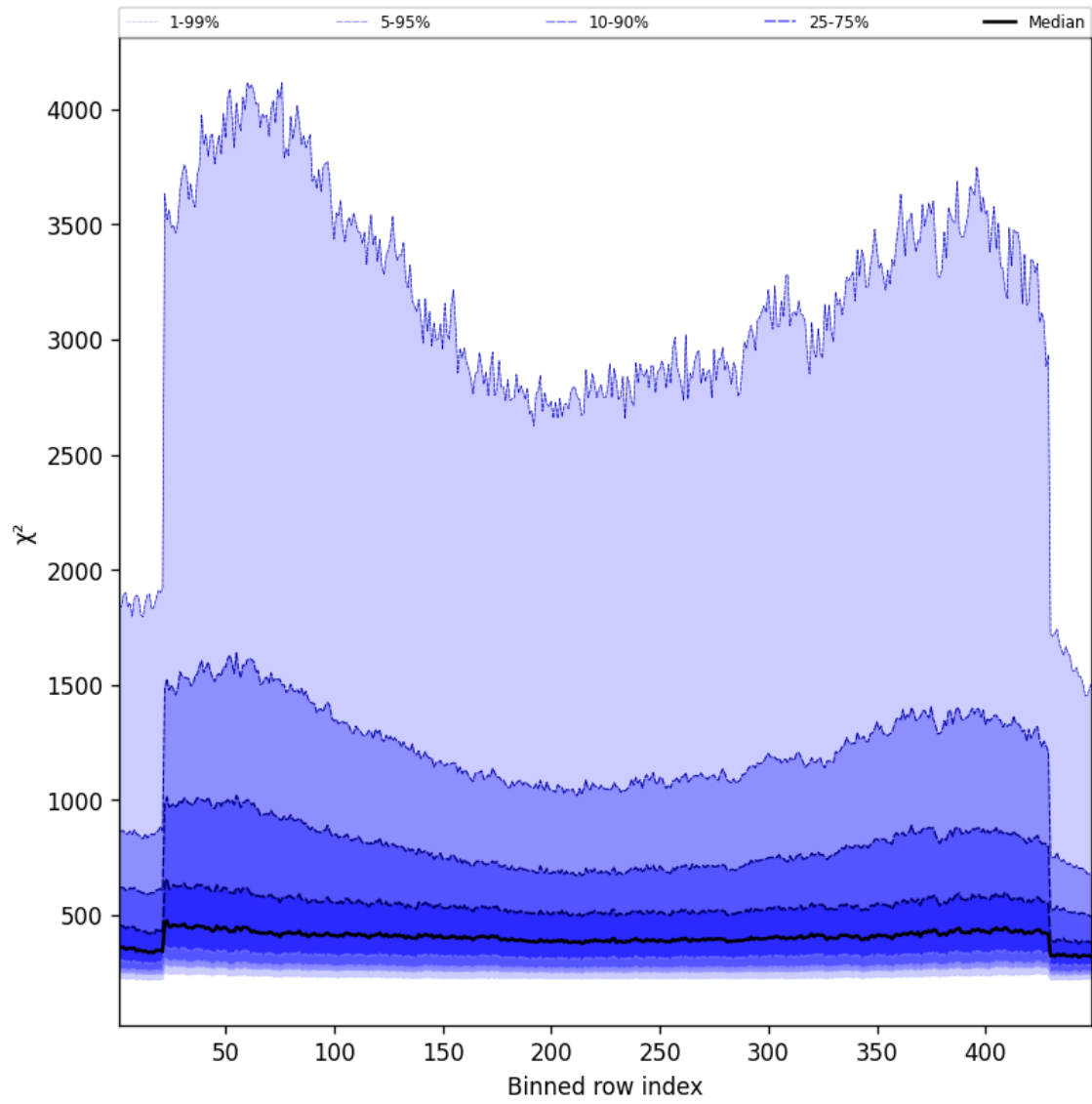
Figure 57: Along track statistics of “ \chi^2 ” for 2025-04-23 to 2025-04-24
