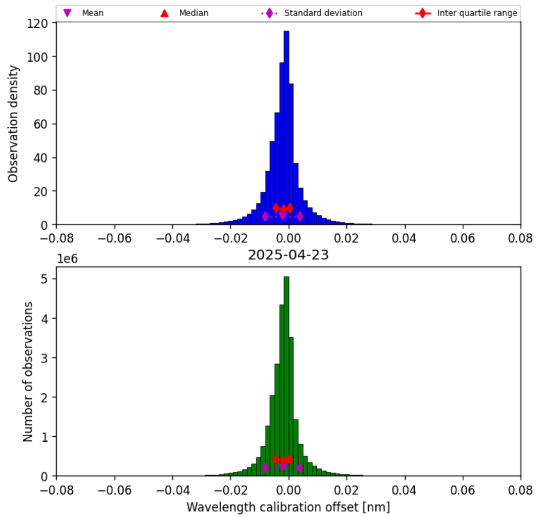
Figure 33: Histogram of “Wavelength calibration offset” for 2025-04-23 to 2025-04-24
