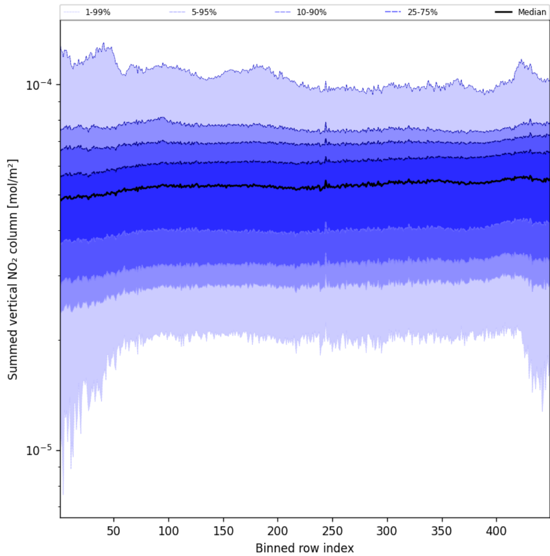
Figure 55: Along track statistics of “Summed vertical NO 2 column” for 2025-04-23 to 2025-04-24
