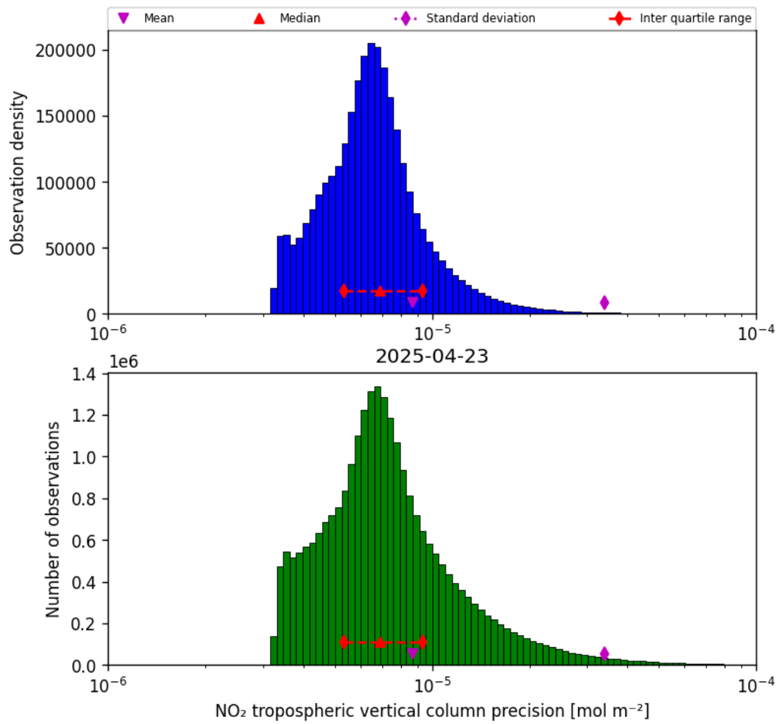
Figure 28: Histogram of “NO 2 tropospheric vertical column precision” for 2025-04-23 to 2025-04-24
