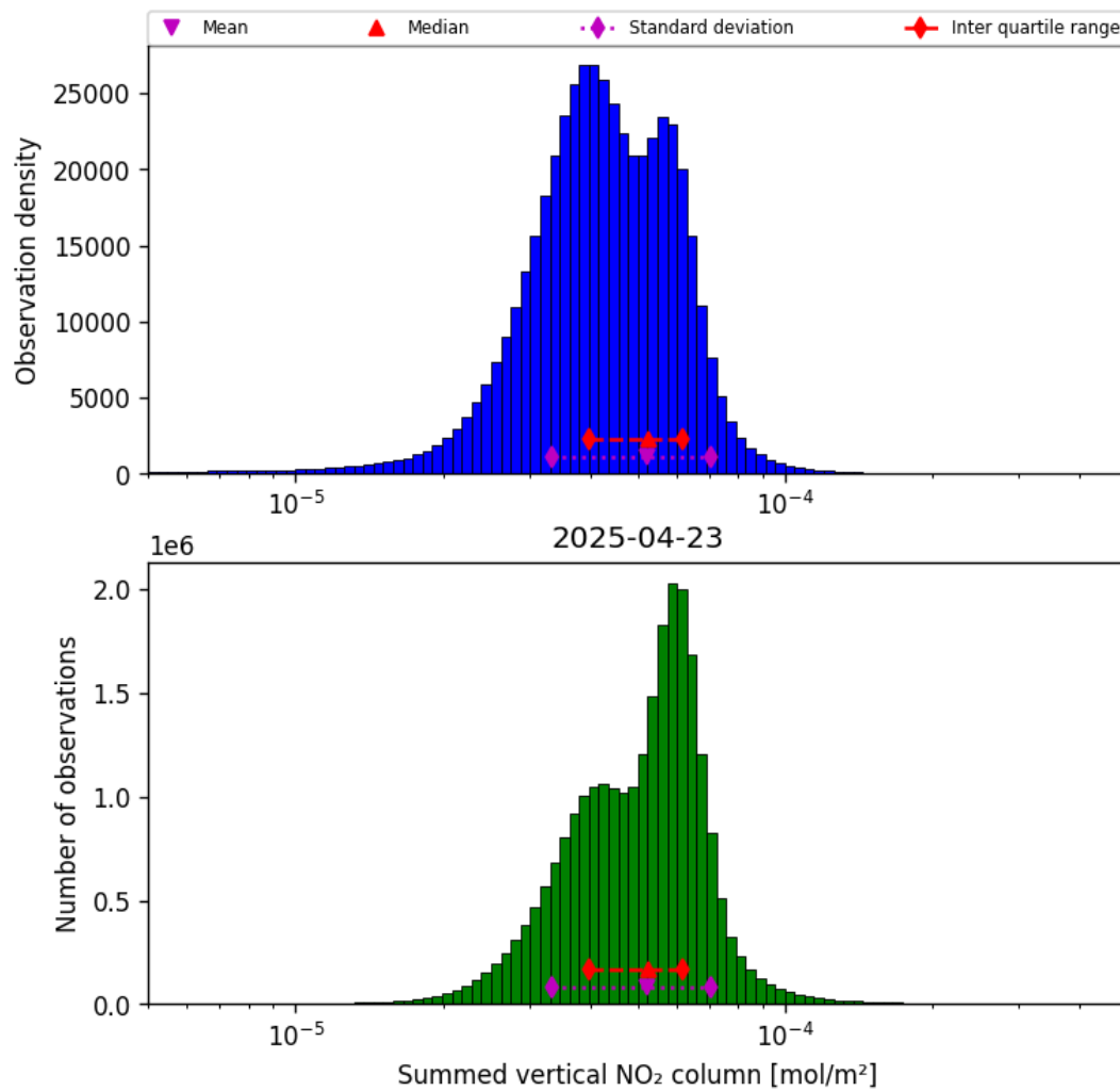
Figure 38: Histogram of “Summed vertical NO 2 column” for 2025-04-23 to 2025-04-24
