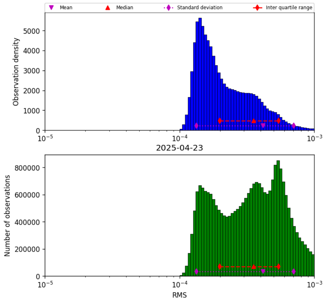
Figure 41: Histogram of “RMS” for 2025-04-23 to 2025-04-24
