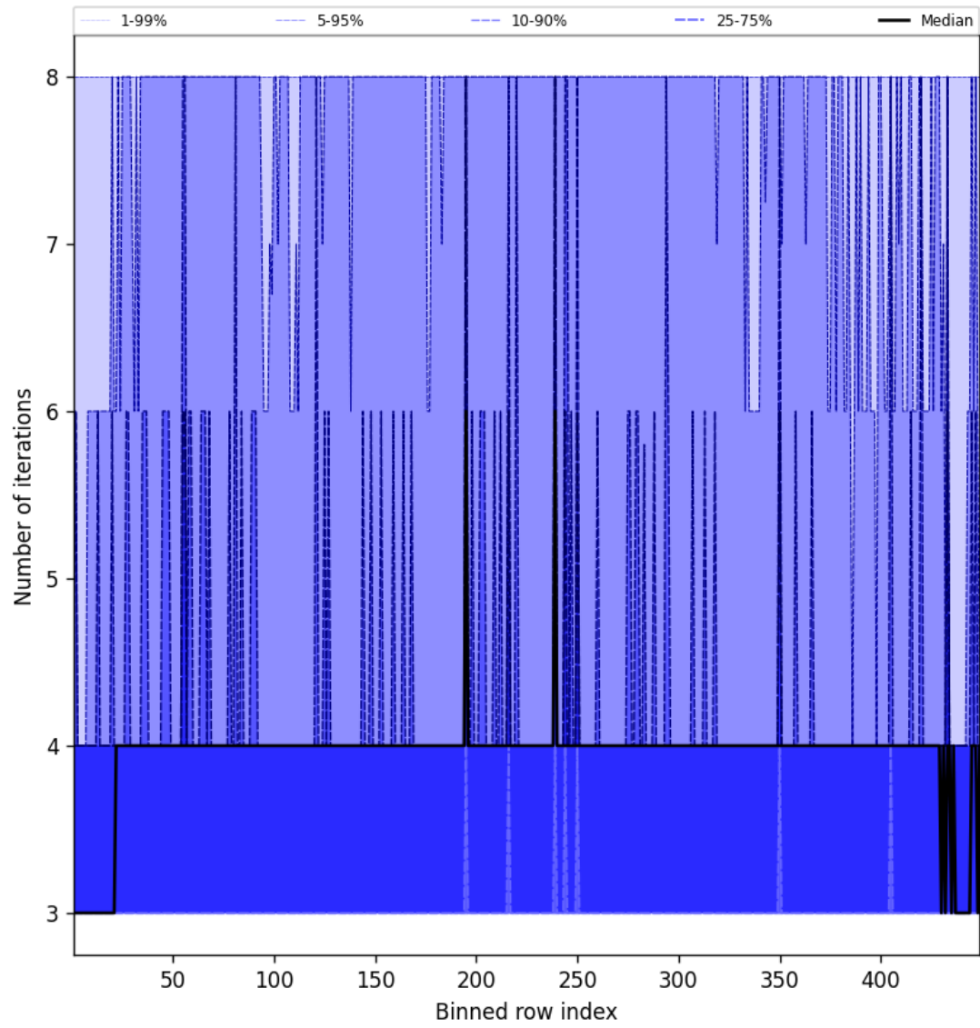
Figure 49: Along track statistics of “Number of iterations” for 2025-04-23 to 2025-04-24
