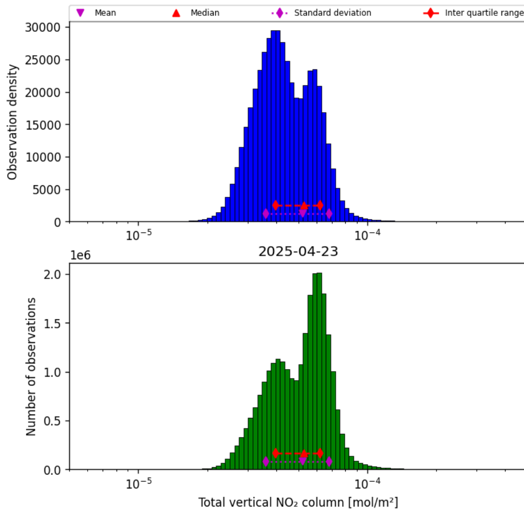
Figure 36: Histogram of “Total vertical NO 2 column” for 2025-04-23 to 2025-04-24
