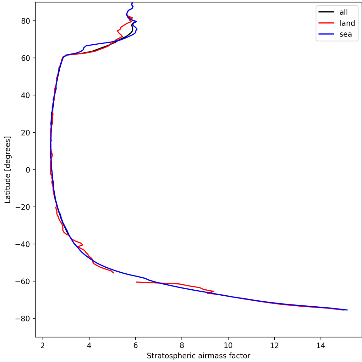
Figure 25: Zonal average of “Stratospheric airmass factor” for 2025-04-23 to 2025-04-24.
