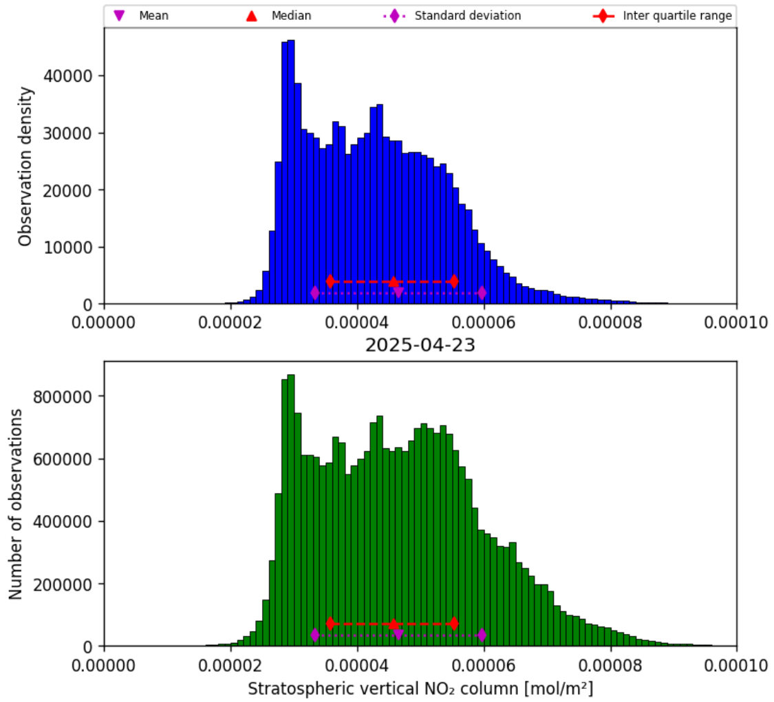
Figure 34: Histogram of “Stratospheric vertical NO 2 column” for 2025-04-23 to 2025-04-24
