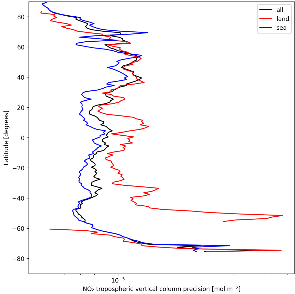
Figure 11: Zonal average of “NO 2 tropospheric vertical column precision” for 2025-04-23 to 2025-04-24.
