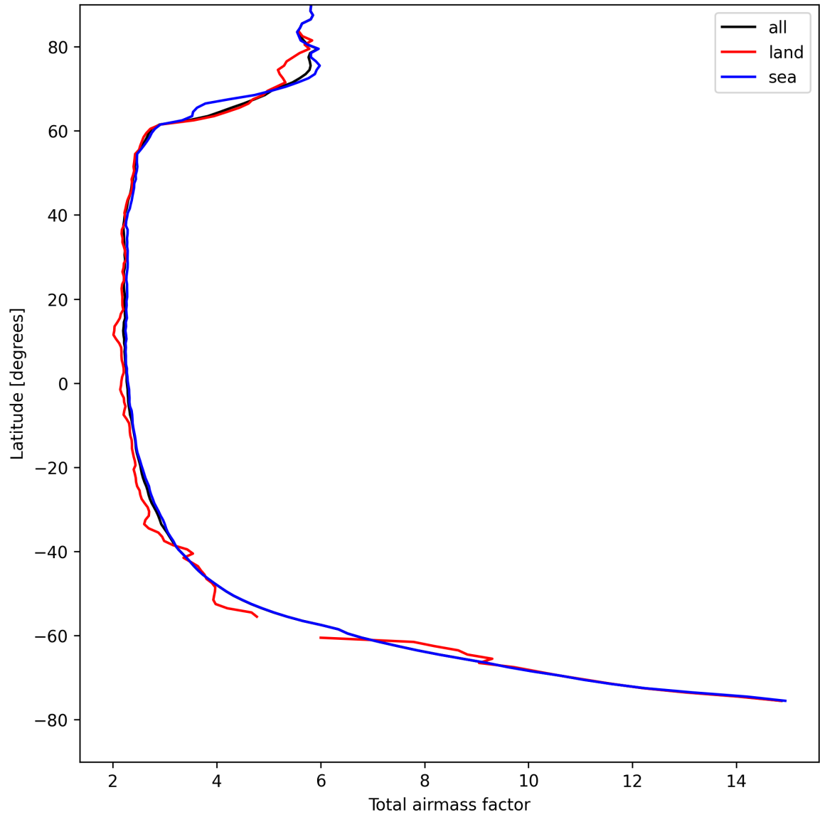
Figure 13: Zonal average of “Total airmass factor” for 2025-04-23 to 2025-04-24.
