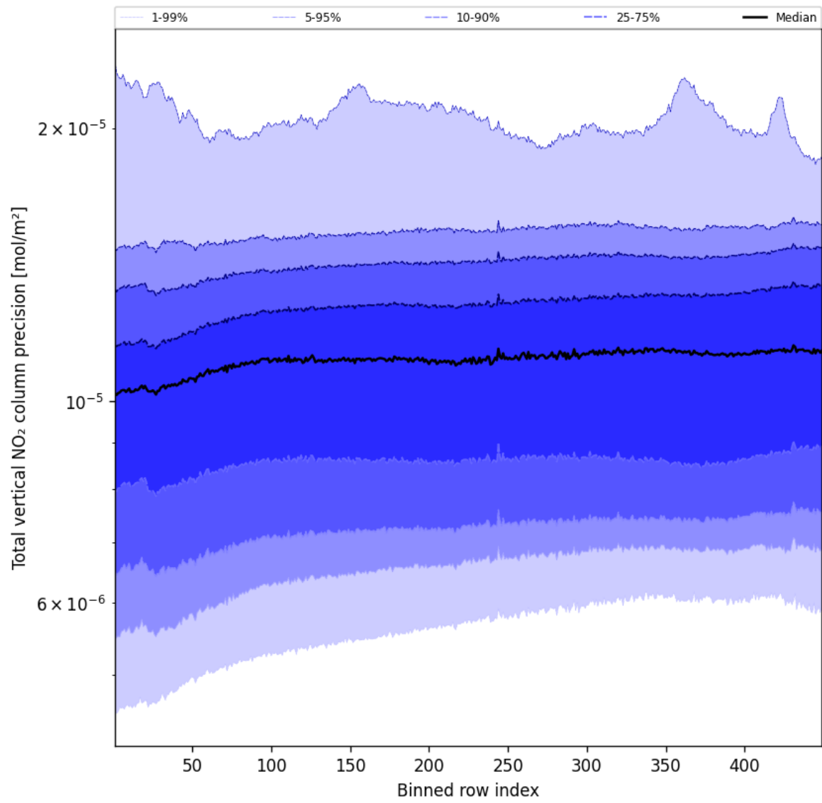
Figure 54: Along track statistics of “Total vertical NO 2 column precision” for 2025-04-23 to 2025-04-24
