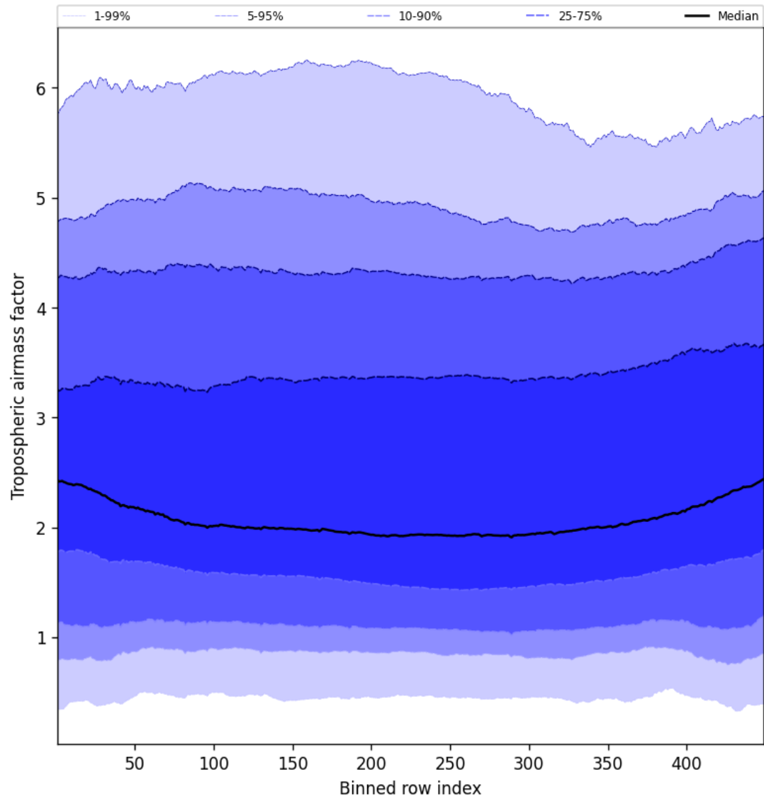
Figure 46: Along track statistics of “Tropospheric airmass factor” for 2025-04-23 to 2025-04-24
