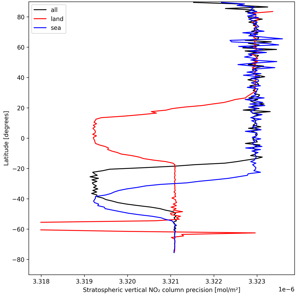
Figure 18: Zonal average of “Stratospheric vertical NO 2 column precision” for 2025-04-23 to 2025-04-24.
