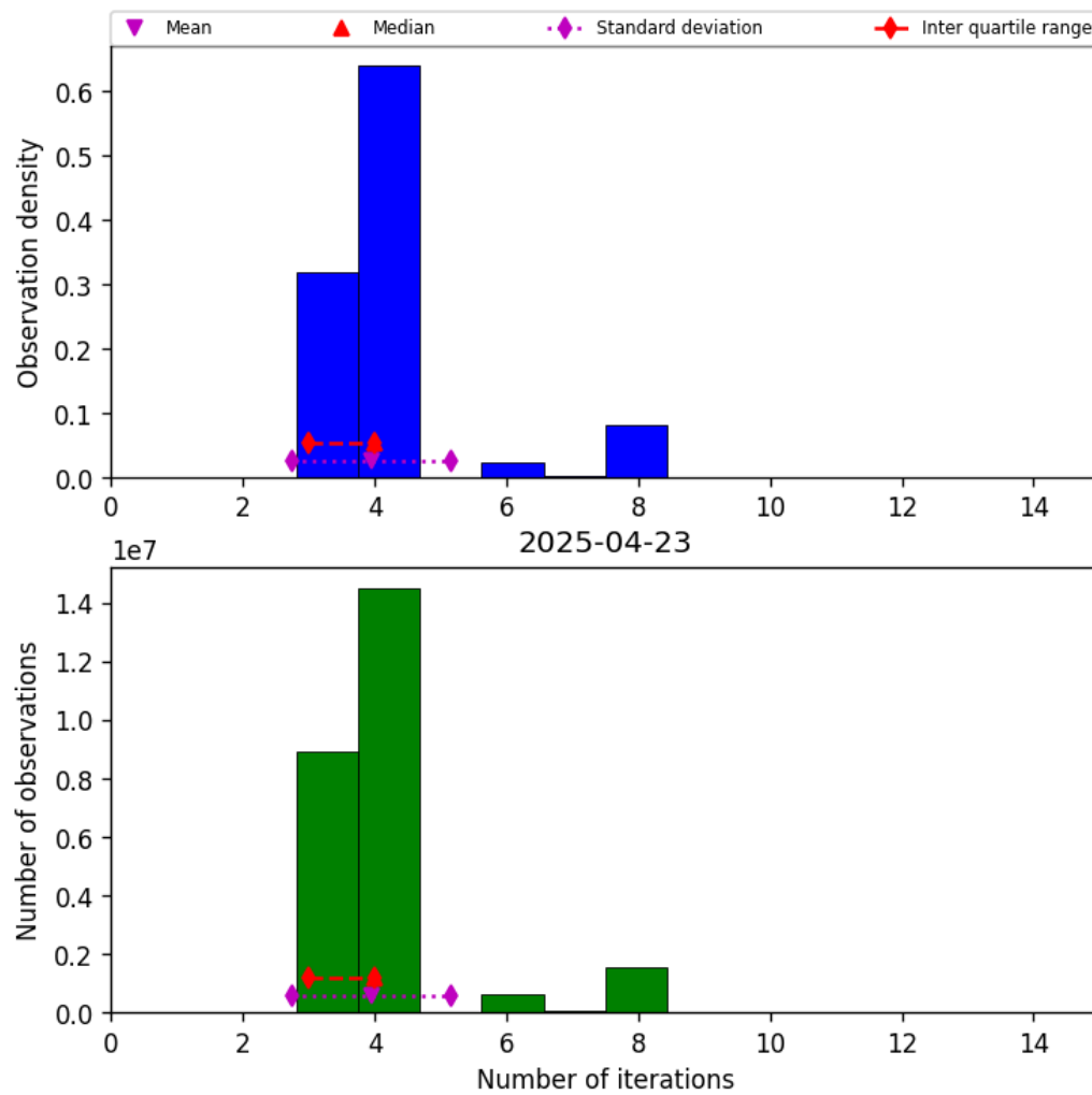
Figure 32: Histogram of “Number of iterations” for 2025-04-23 to 2025-04-24
