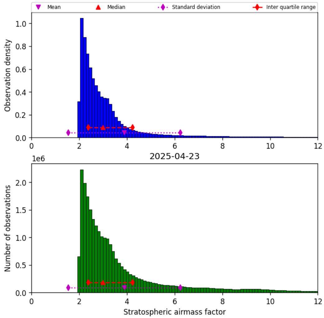
Figure 42: Histogram of “Stratospheric airmass factor” for 2025-04-23 to 2025-04-24
