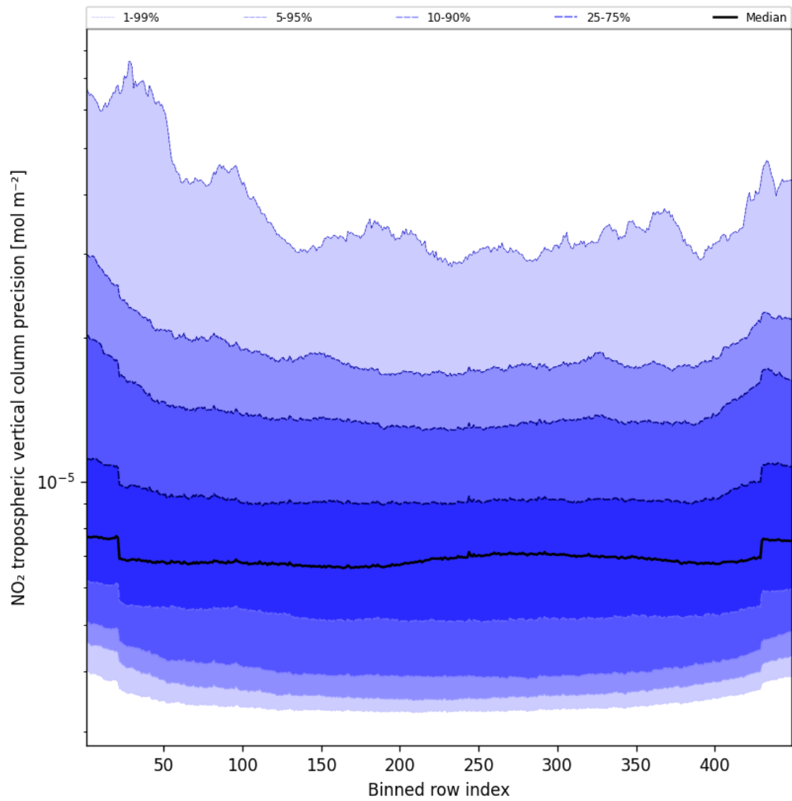
Figure 45: Along track statistics of “NO 2 tropospheric vertical column precision” for 2025-04-23 to 2025-04-24
