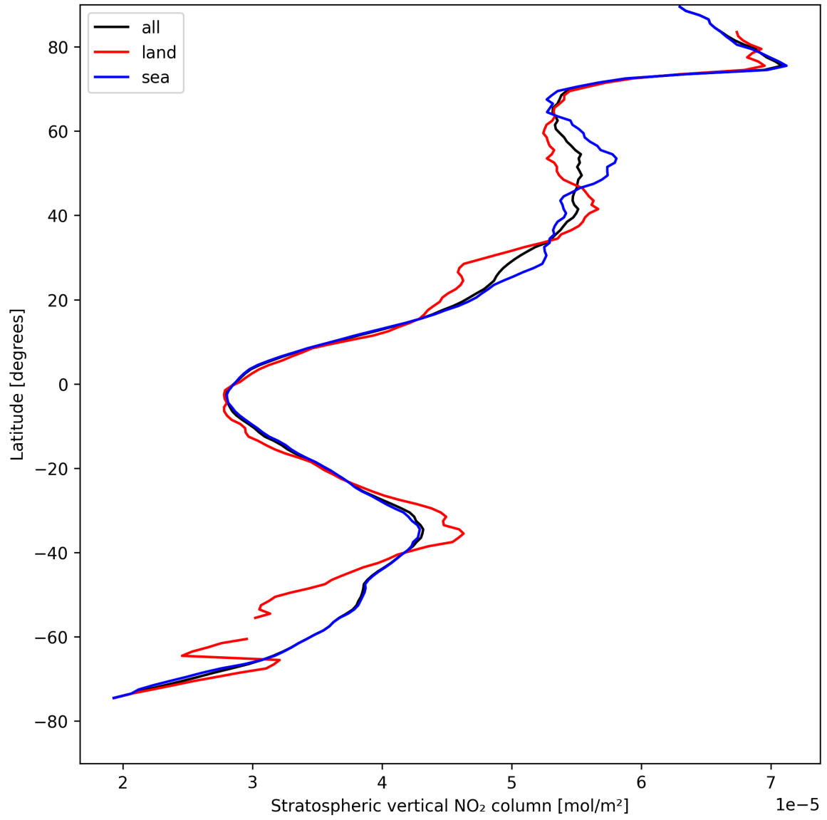
Figure 17: Zonal average of “Stratospheric vertical NO 2 column” for 2025-04-24 to 2025-04-25.
