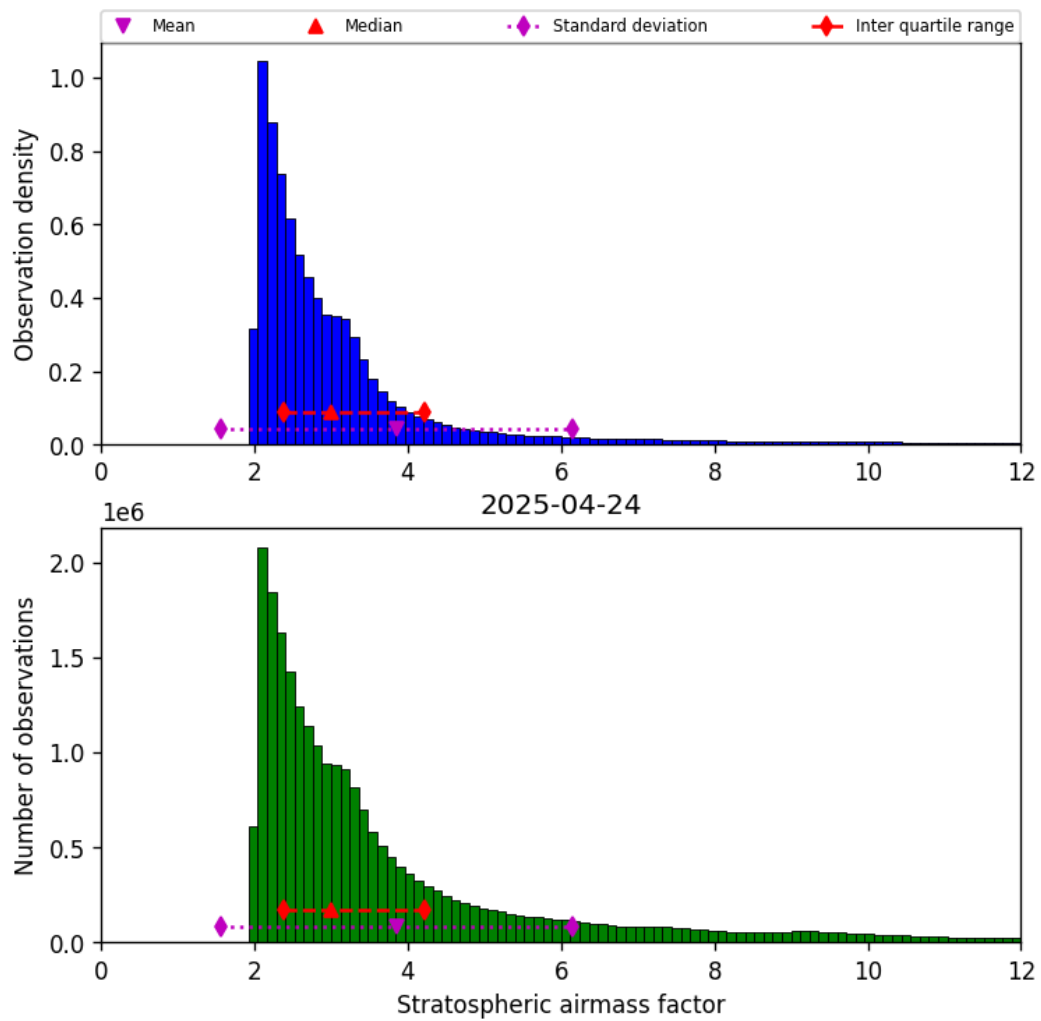
Figure 42: Histogram of “Stratospheric airmass factor” for 2025-04-24 to 2025-04-25
