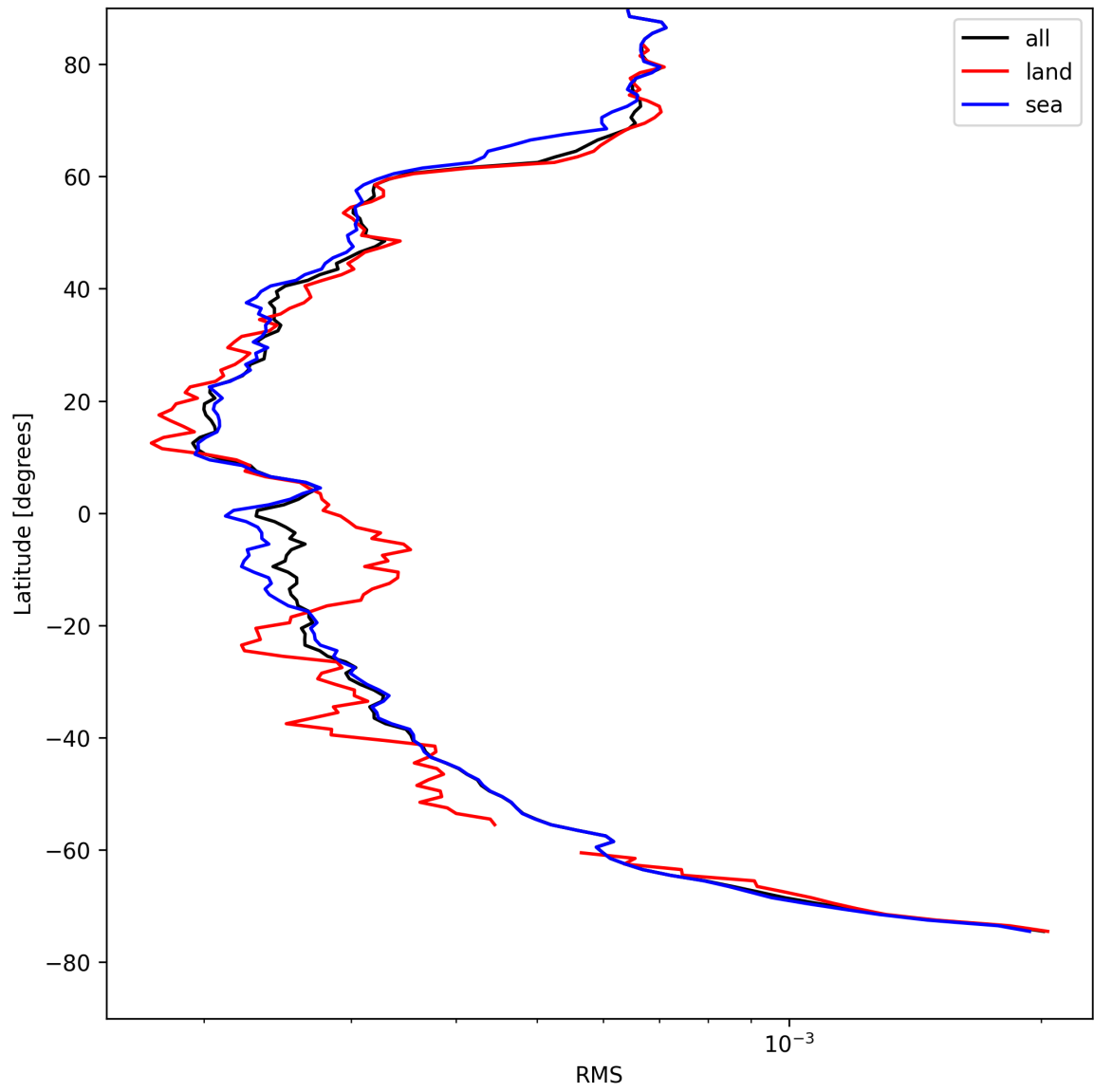
Figure 24: Zonal average of “RMS” for 2025-04-24 to 2025-04-25.
