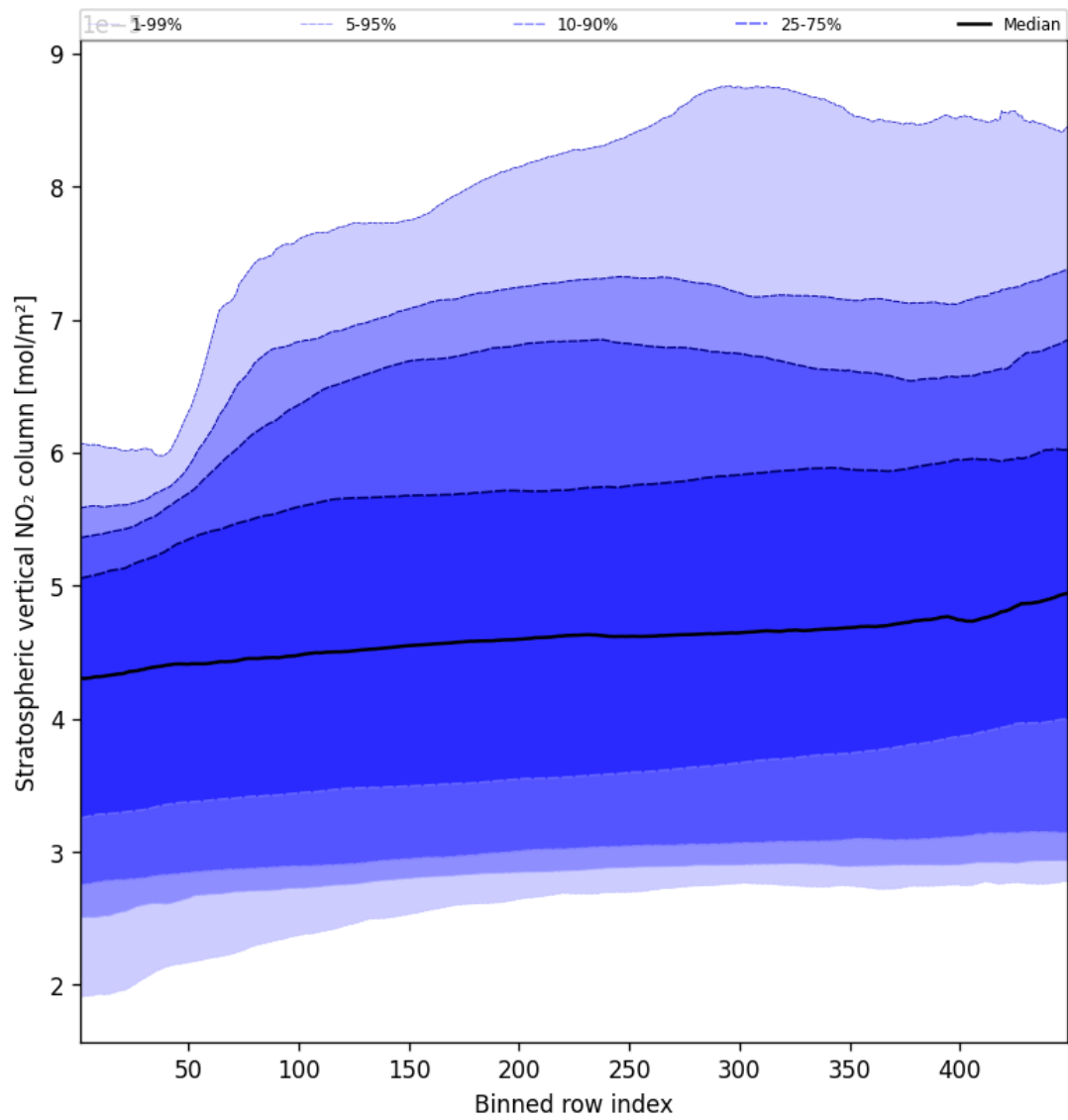
Figure 51: Along track statistics of “Stratospheric vertical NO 2 column” for 2025-04-24 to 2025-04-25
