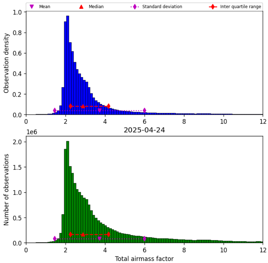
Figure 30: Histogram of “Total airmass factor” for 2025-04-24 to 2025-04-25
