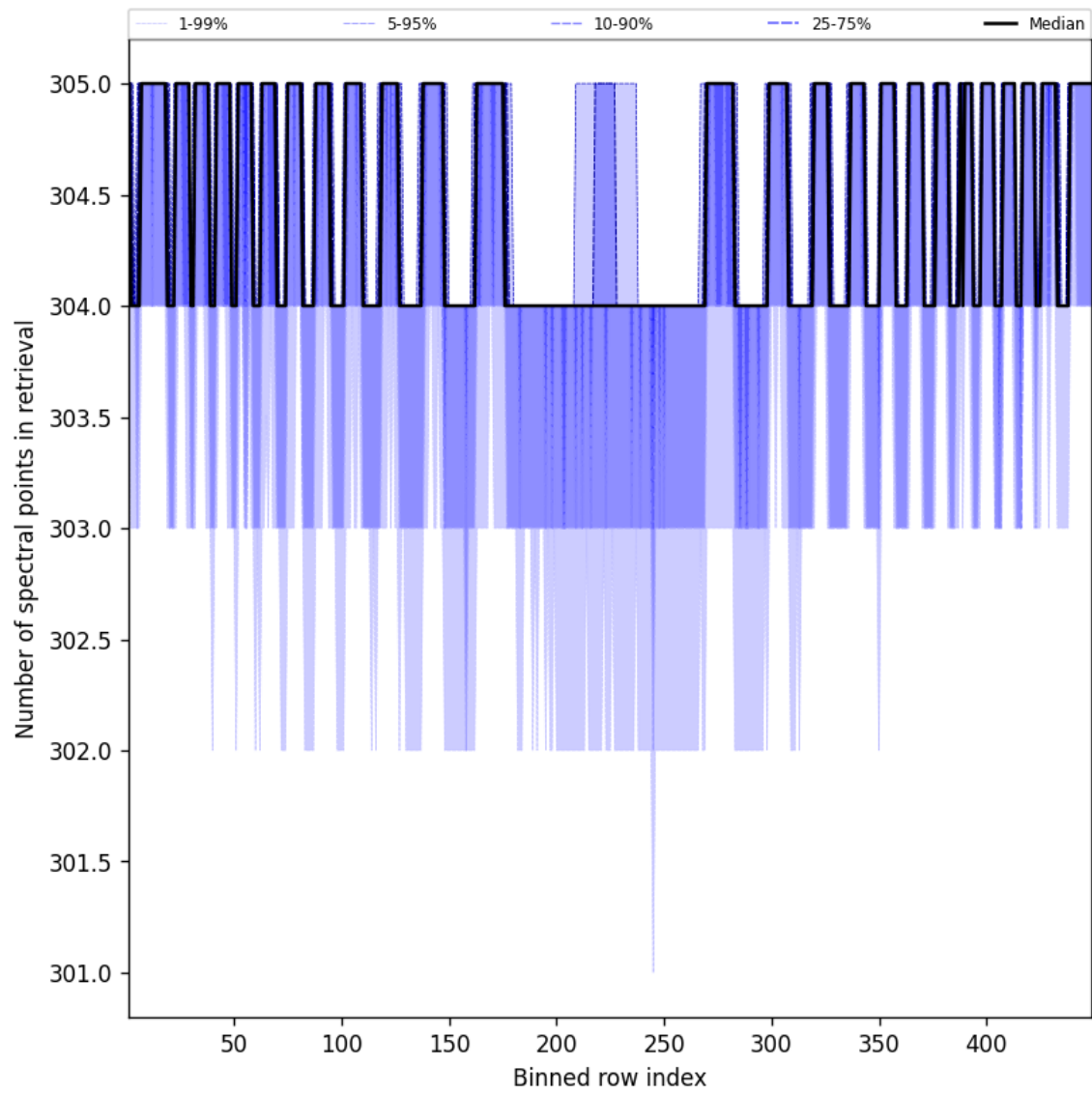
Figure 48: Along track statistics of “Number of spectral points in retrieval” for 2025-04-24 to 2025-04-25
