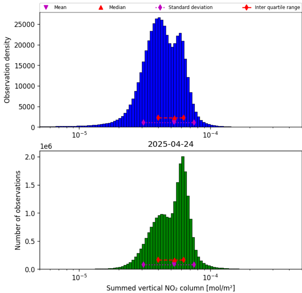
Figure 38: Histogram of “Summed vertical NO 2 column” for 2025-04-24 to 2025-04-25
