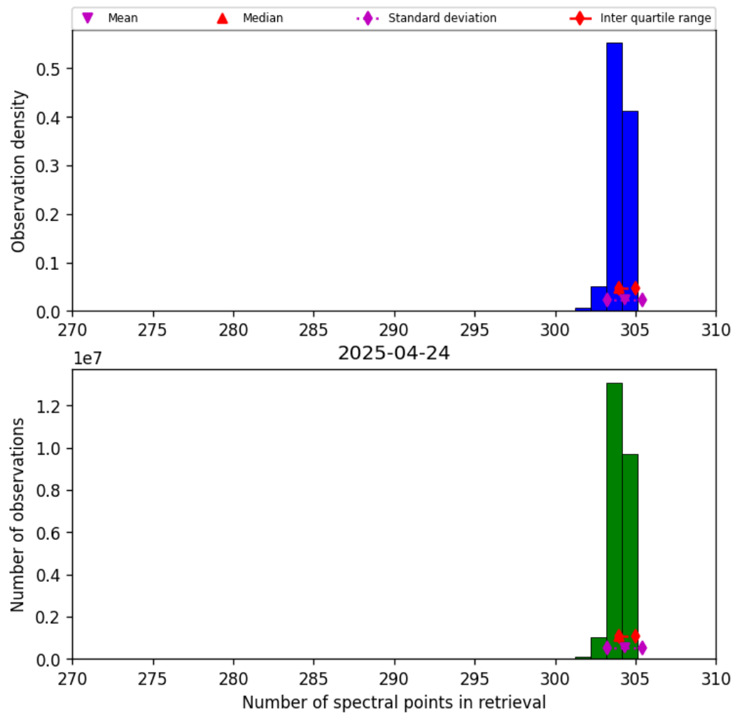
Figure 31: Histogram of “Number of spectral points in retrieval” for 2025-04-24 to 2025-04-25
