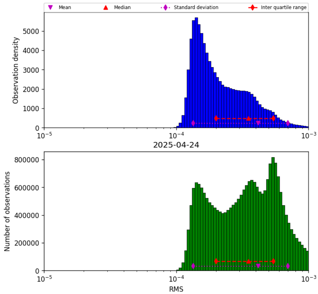
Figure 41: Histogram of “RMS” for 2025-04-24 to 2025-04-25
