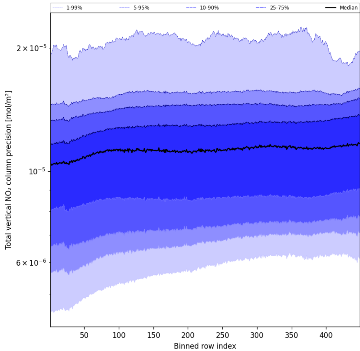
Figure 54: Along track statistics of “Total vertical NO 2 column precision” for 2025-04-24 to 2025-04-25
