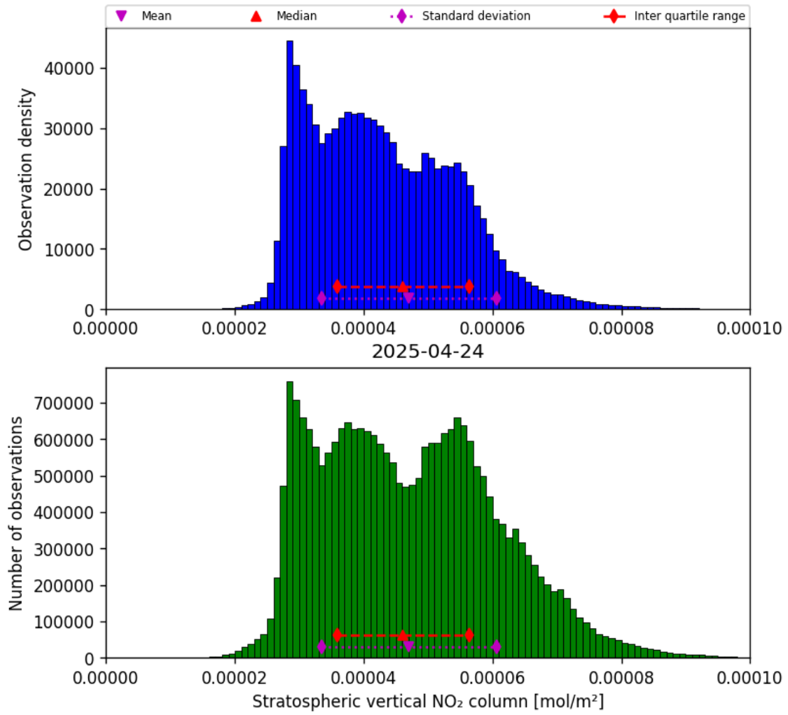
Figure 34: Histogram of “Stratospheric vertical NO 2 column” for 2025-04-24 to 2025-04-25
