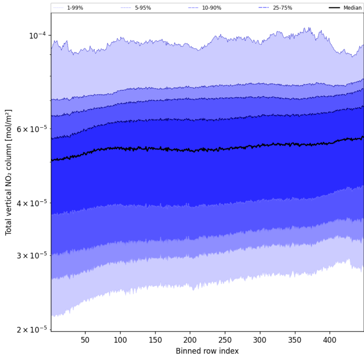
Figure 53: Along track statistics of “Total vertical NO 2 column” for 2025-04-24 to 2025-04-25
