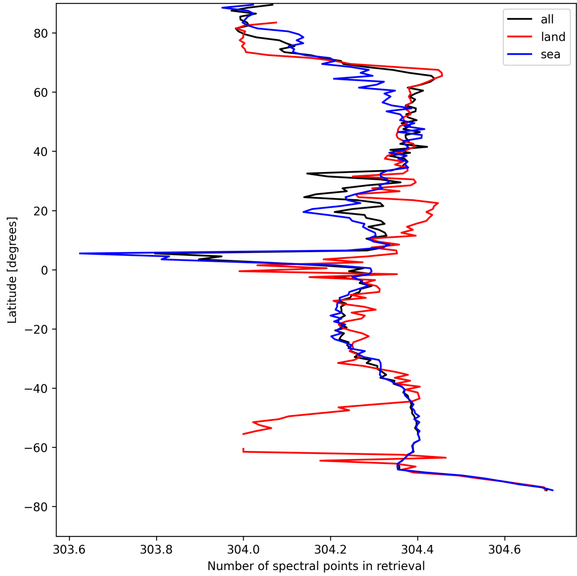
Figure 14: Zonal average of “Number of spectral points in retrieval” for 2025-04-24 to 2025-04-25.
