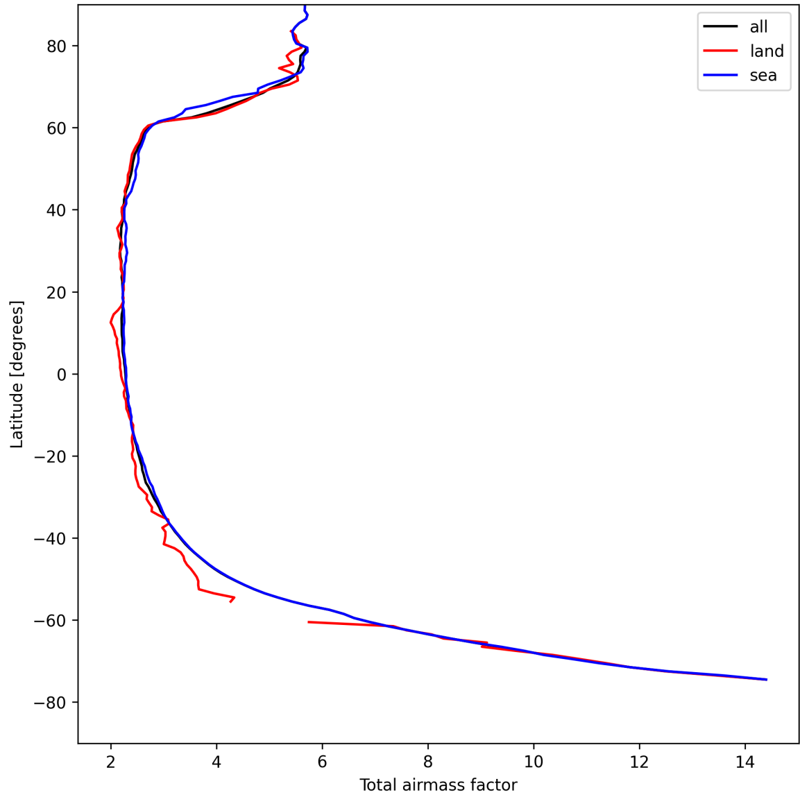
Figure 13: Zonal average of “Total airmass factor” for 2025-04-24 to 2025-04-25.
