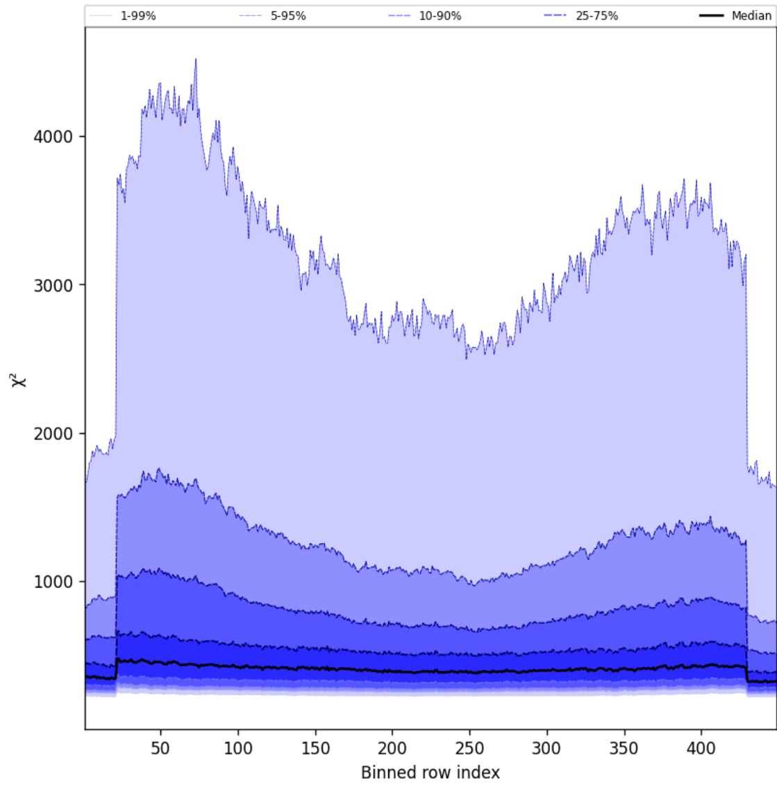
Figure 57: Along track statistics of “ \chi^2 ” for 2025-04-24 to 2025-04-25
