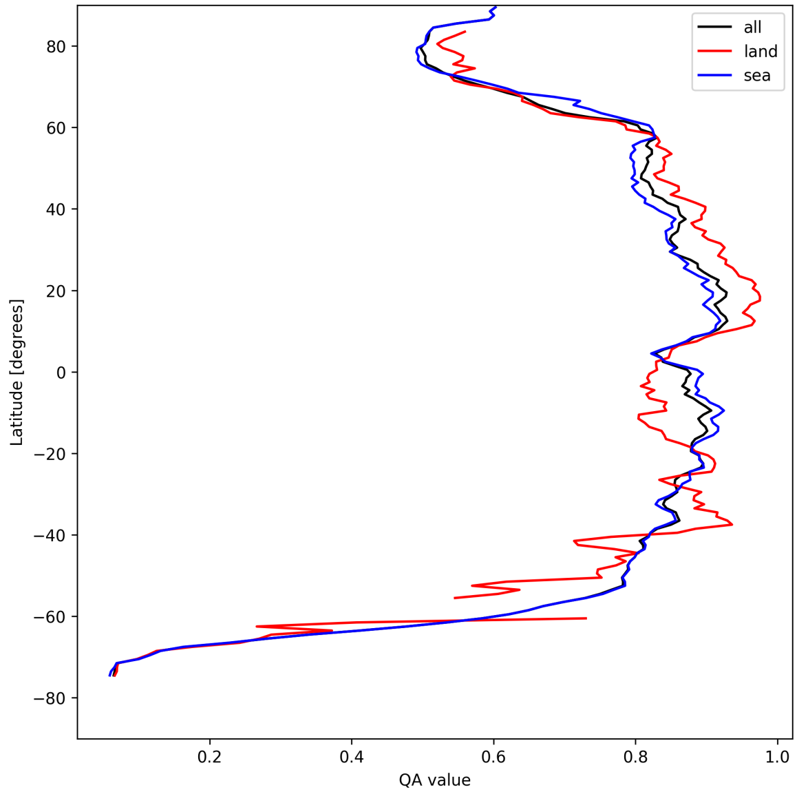
Figure 9: Zonal average of “QA value” for 2025-04-24 to 2025-04-25.
