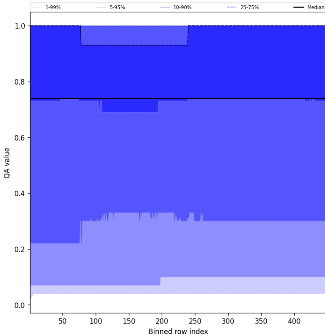
Figure 43: Along track statistics of “QA value” for 2025-04-24 to 2025-04-25
