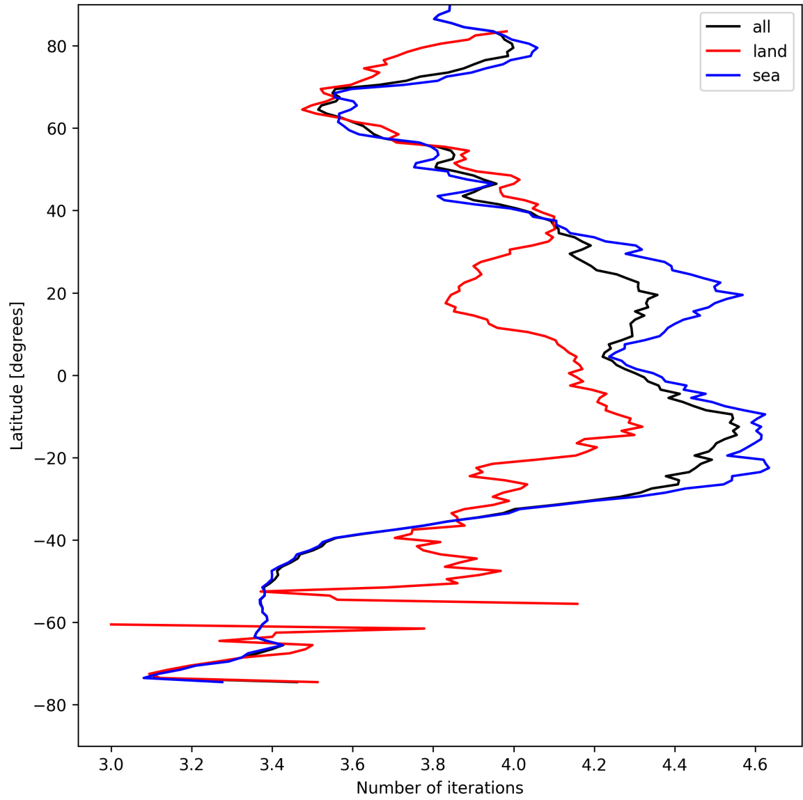
Figure 15: Zonal average of “Number of iterations” for 2025-04-24 to 2025-04-25.
