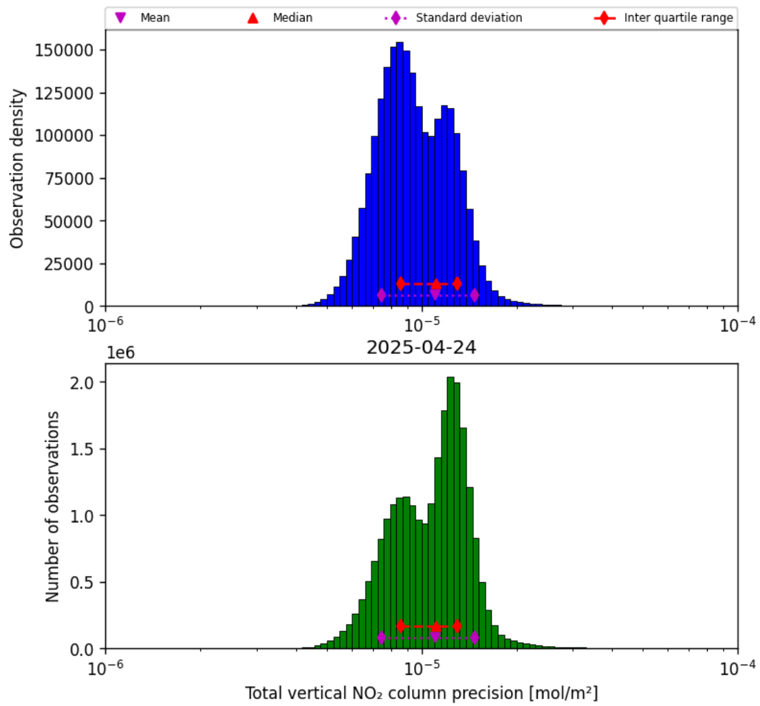
Figure 37: Histogram of “Total vertical NO 2 column precision” for 2025-04-24 to 2025-04-25
