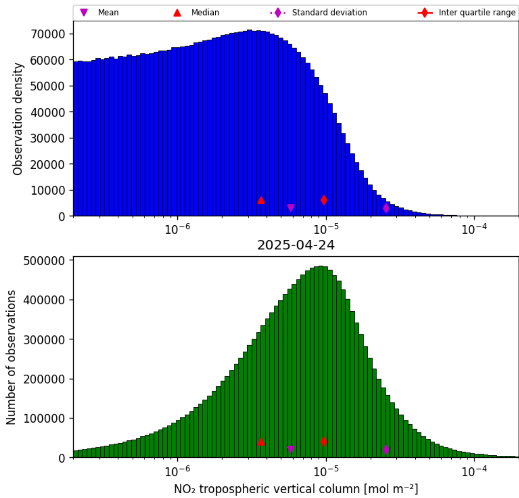
Figure 27: Histogram of “NO 2 tropospheric vertical column” for 2025-04-24 to 2025-04-25
