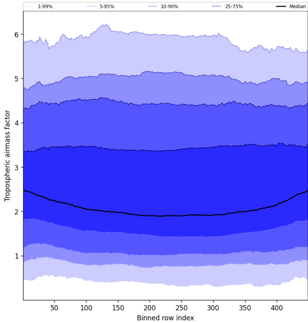
Figure 46: Along track statistics of “Tropospheric airmass factor” for 2025-04-24 to 2025-04-25
