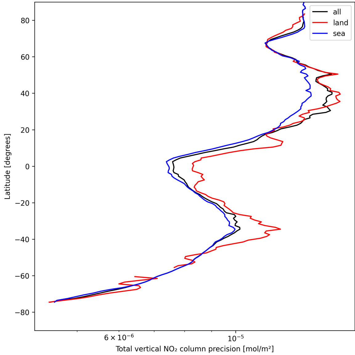
Figure 20: Zonal average of “Total vertical NO 2 column precision” for 2025-04-24 to 2025-04-25.
