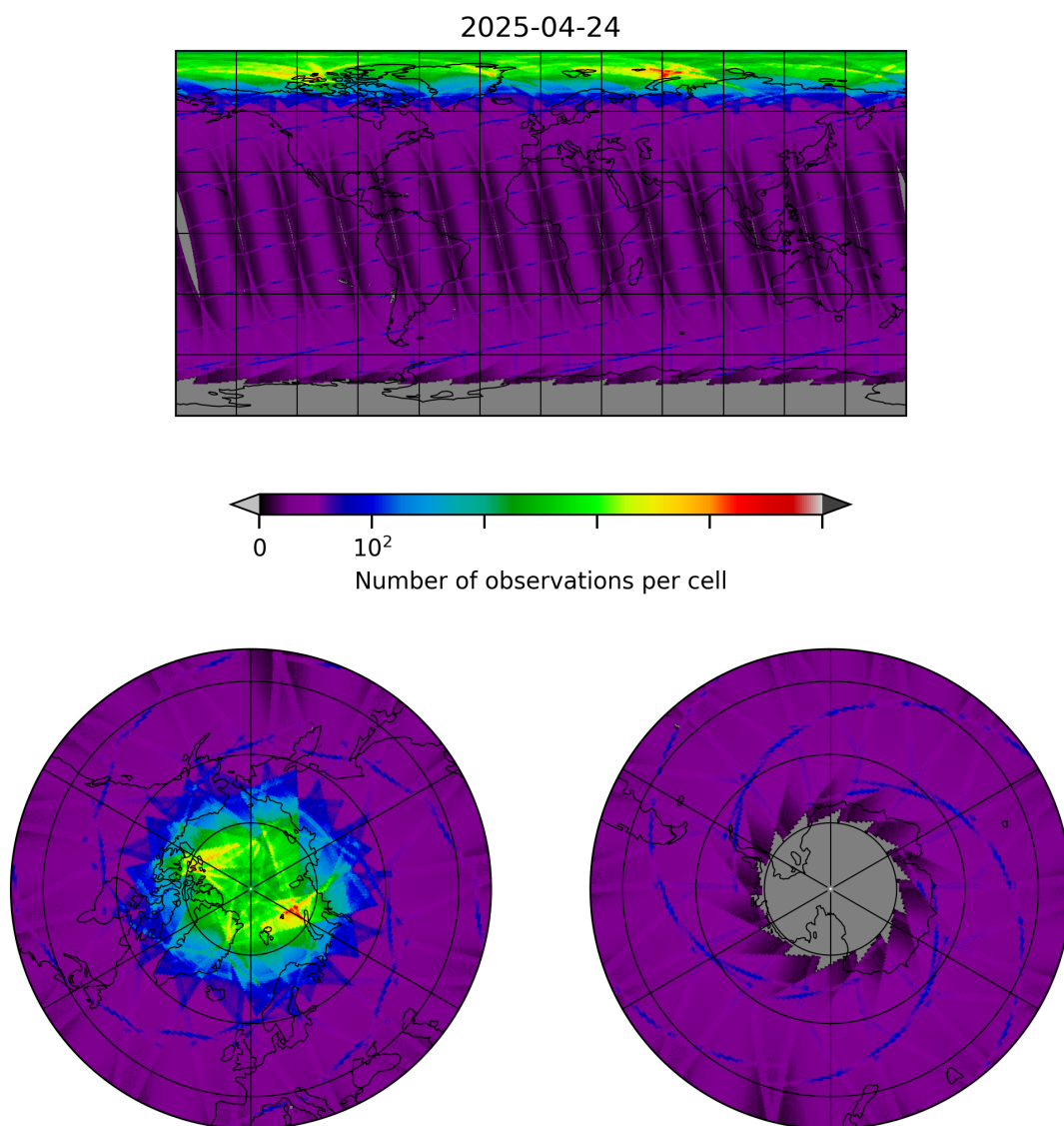
Figure 8: Map of the number of observations for 2025-04-24 to 2025-04-25
