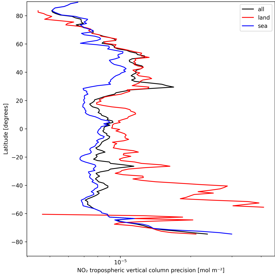
Figure 11: Zonal average of “NO 2 tropospheric vertical column precision” for 2025-04-24 to 2025-04-25.
