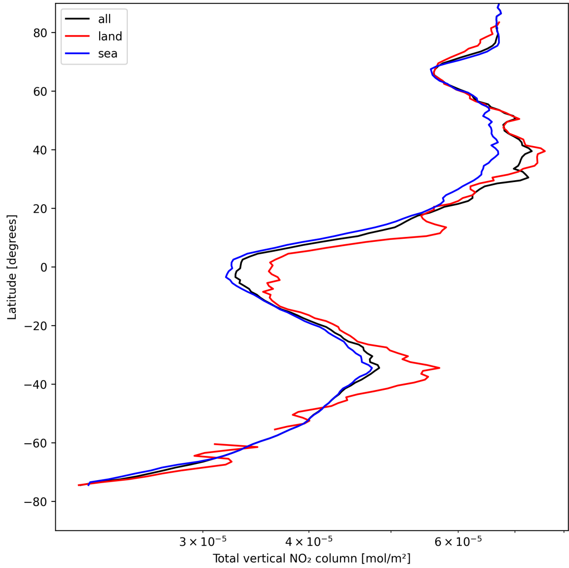
Figure 19: Zonal average of “Total vertical NO 2 column” for 2025-04-24 to 2025-04-25.
