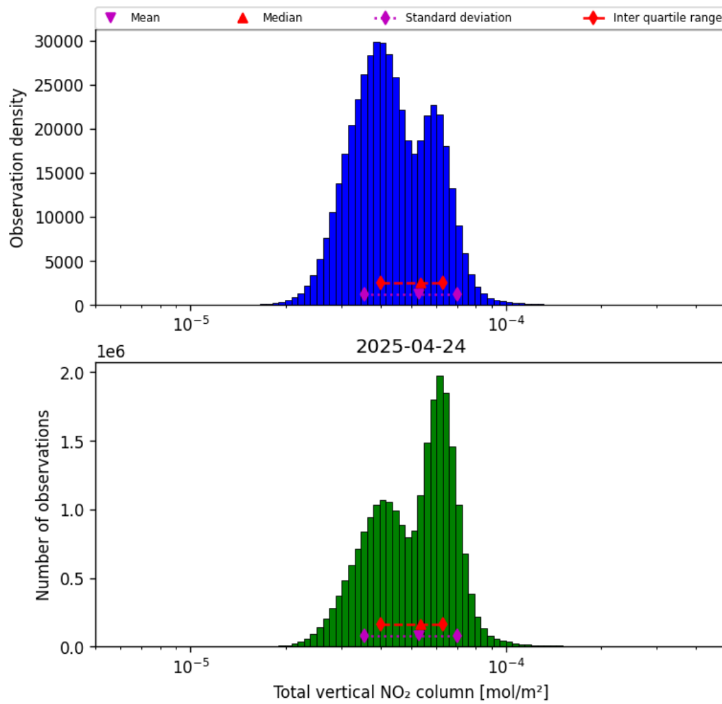
Figure 36: Histogram of "Total vertical NO 2 column" for 2025-04-24 to 2025-04-25
