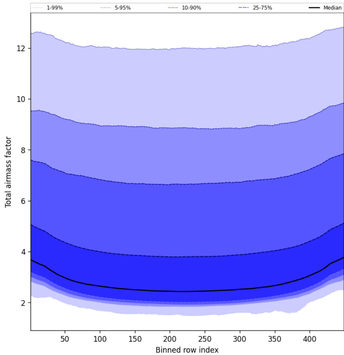
Figure 47: Along track statistics of “Total airmass factor” for 2025-04-24 to 2025-04-25
