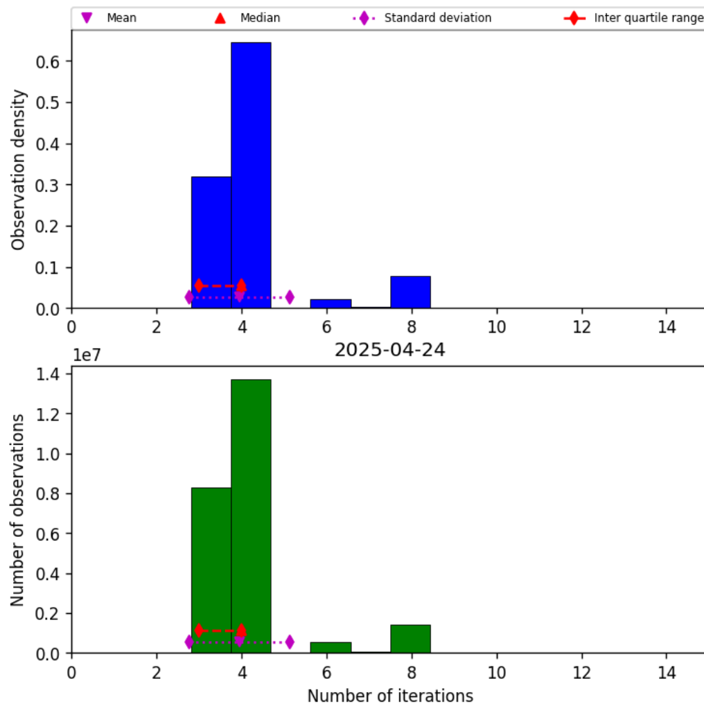
Figure 32: Histogram of “Number of iterations” for 2025-04-24 to 2025-04-25
