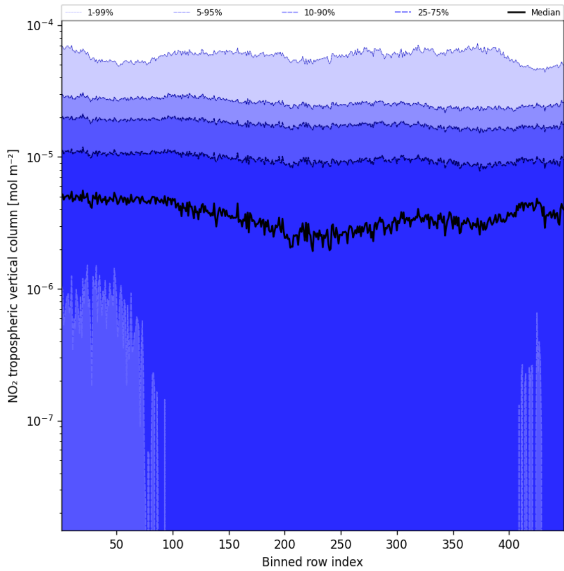
Figure 44: Along track statistics of “NO 2 tropospheric vertical column” for 2025-04-24 to 2025-04-25
