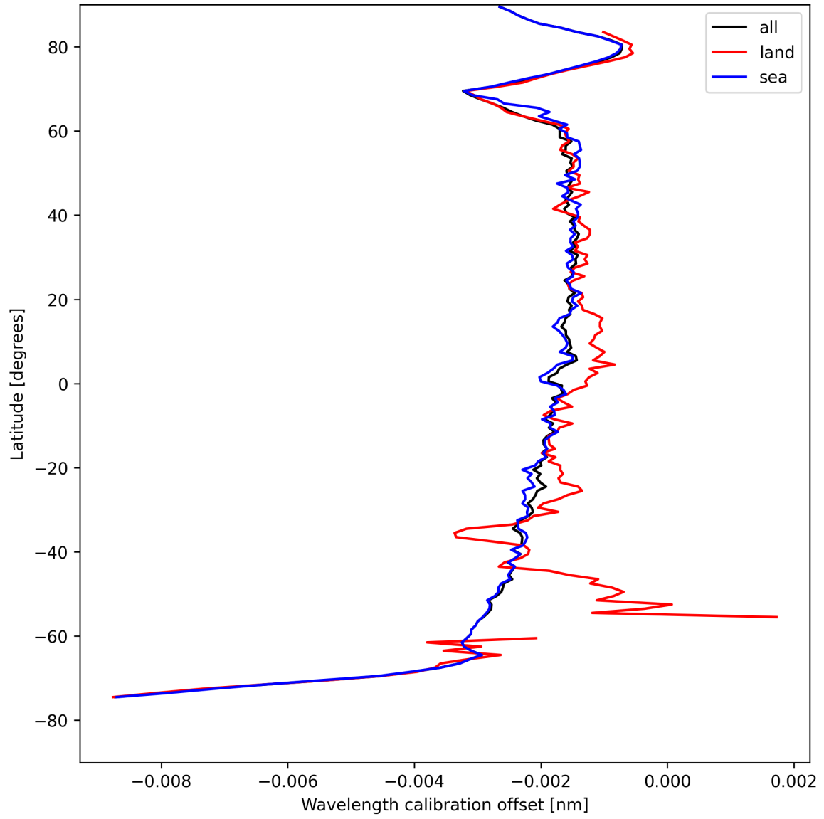
Figure 16: Zonal average of “Wavelength calibration offset” for 2025-04-24 to 2025-04-25.
