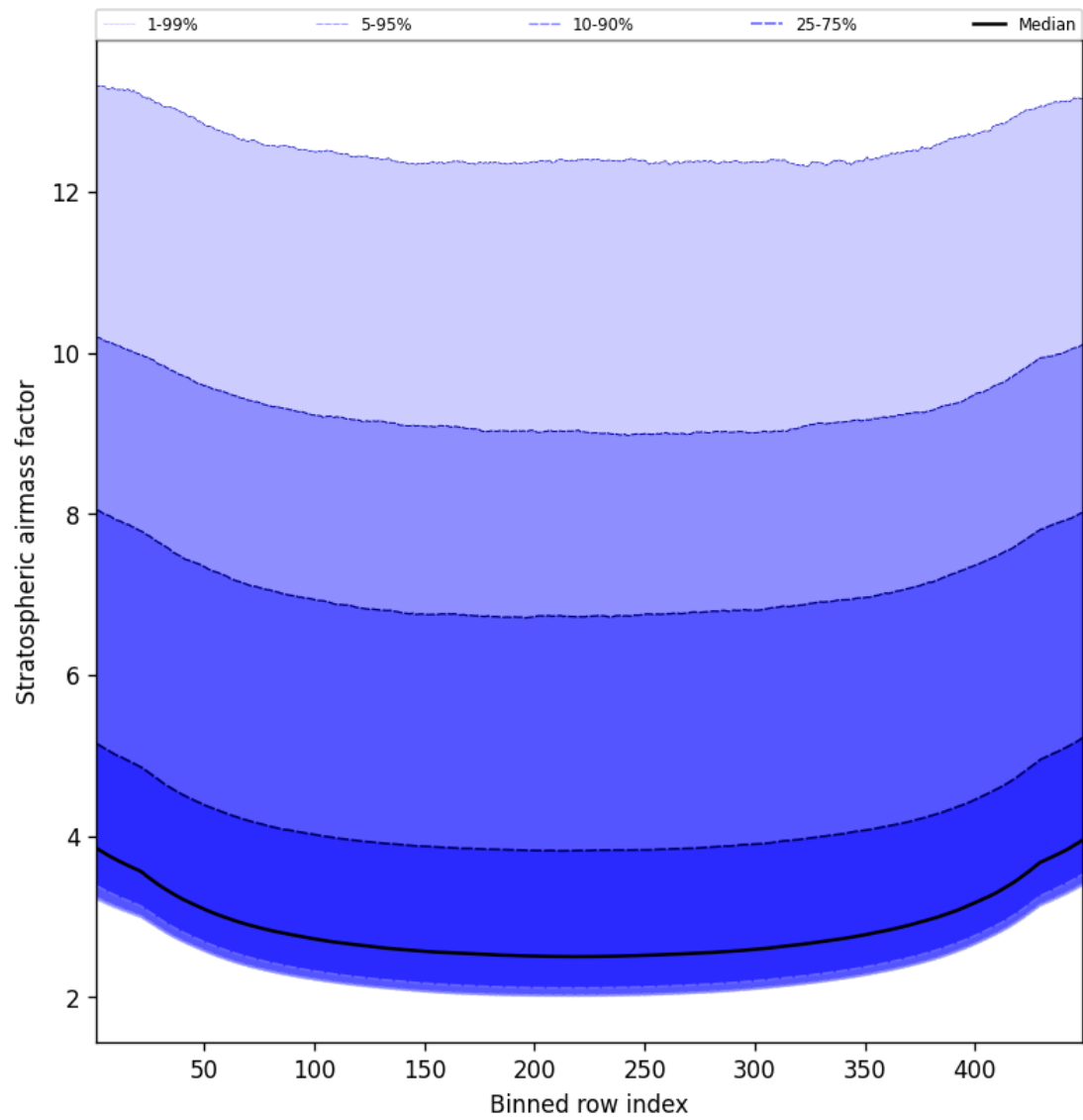
Figure 59: Along track statistics of “Stratospheric airmass factor” for 2025-04-24 to 2025-04-25
