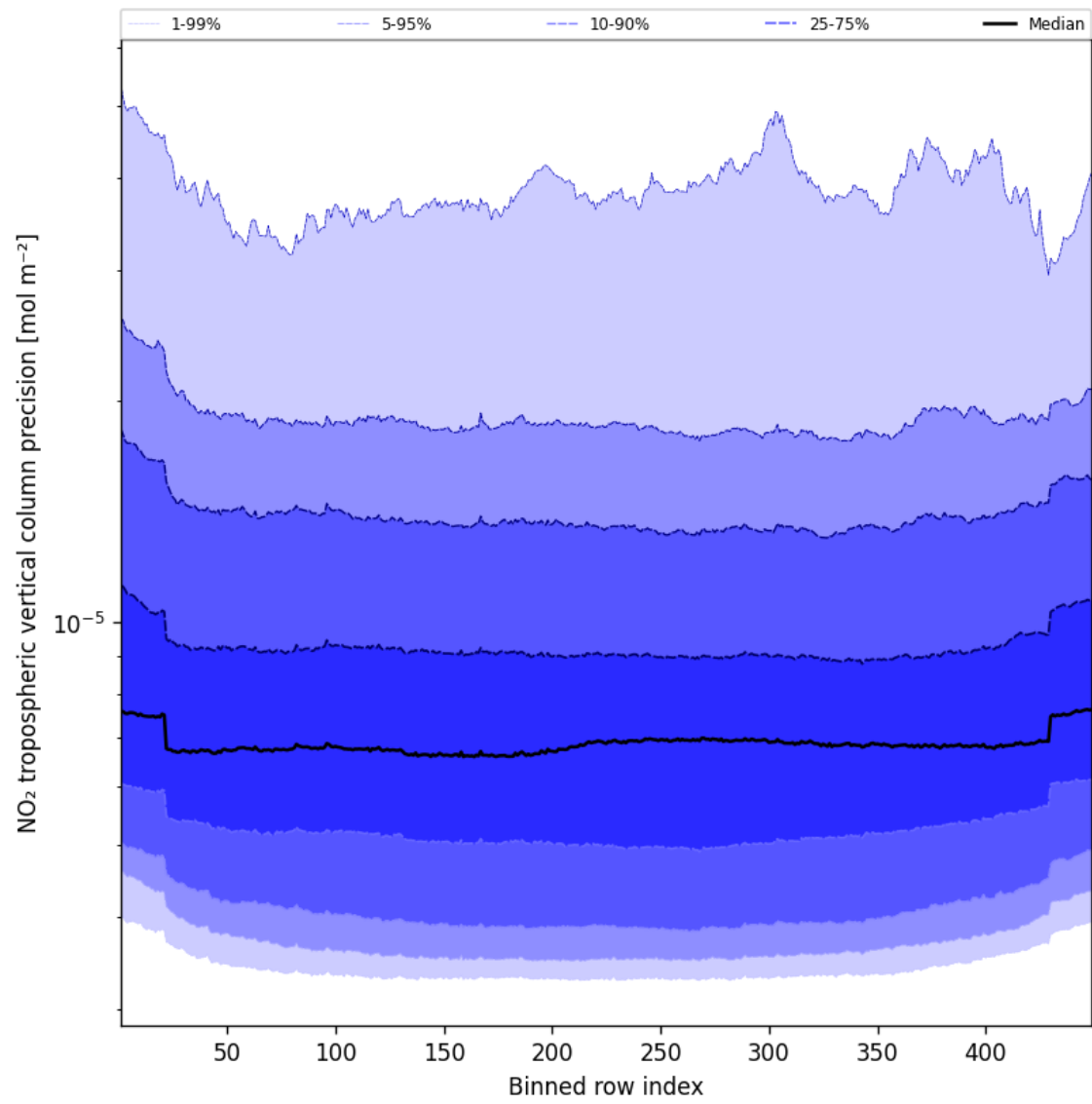
Figure 45: Along track statistics of “NO 2 tropospheric vertical column precision” for 2025-04-24 to 2025-04-25
