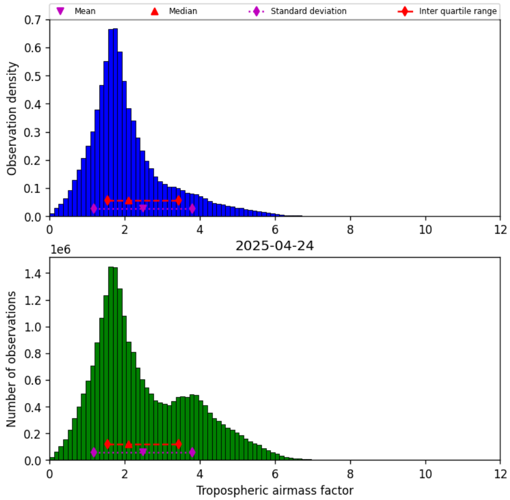
Figure 29: Histogram of “Tropospheric airmass factor” for 2025-04-24 to 2025-04-25
