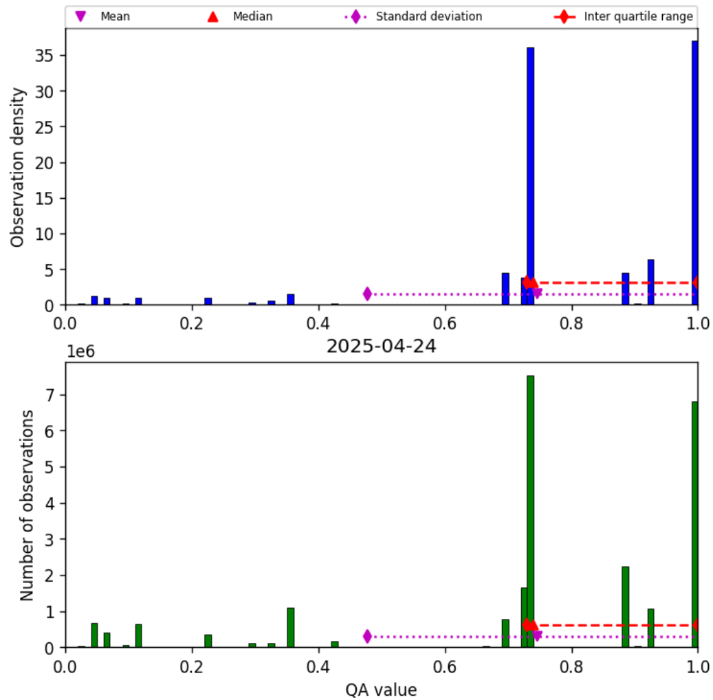
Figure 26: Histogram of “QA value” for 2025-04-24 to 2025-04-25
