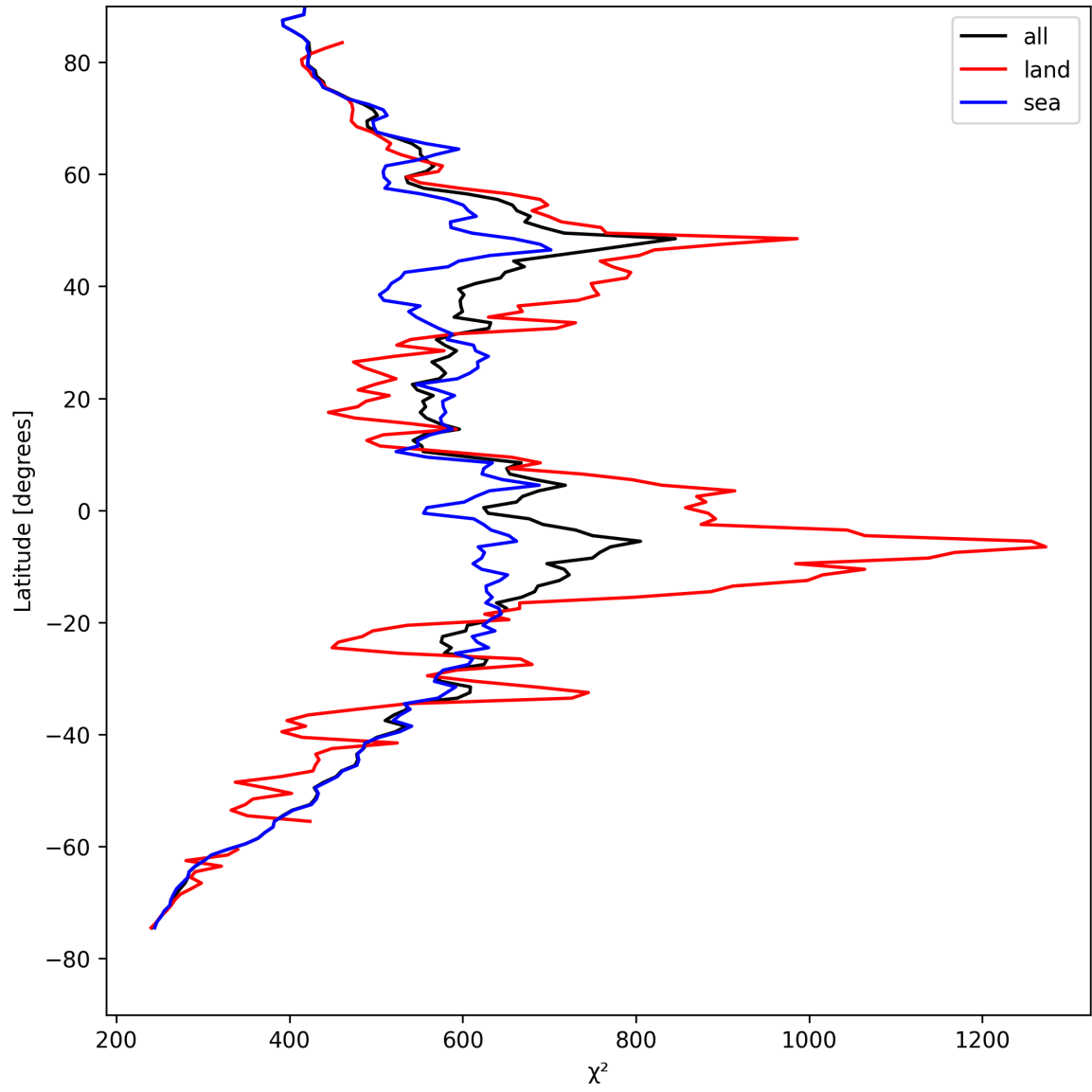
Figure 23: Zonal average of “ \chi^2 ” for 2025-04-24 to 2025-04-25.
