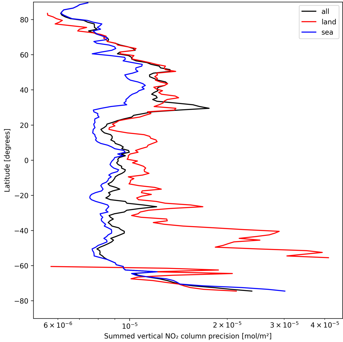
Figure 22: Zonal average of “Summed vertical NO 2 column precision” for 2025-04-24 to 2025-04-25.
