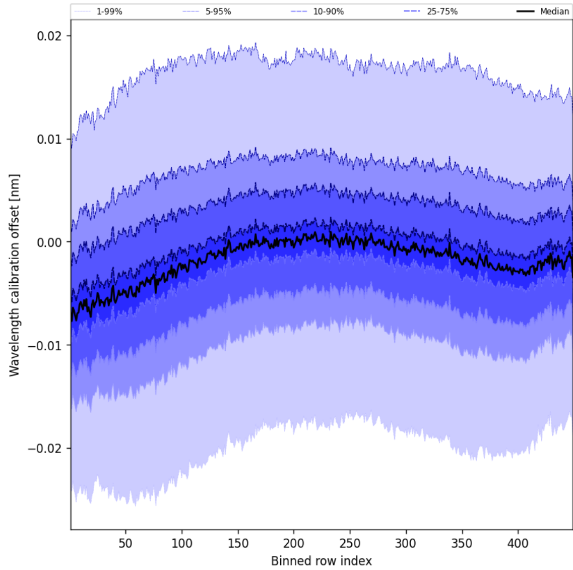
Figure 50: Along track statistics of “Wavelength calibration offset” for 2025-04-24 to 2025-04-25
