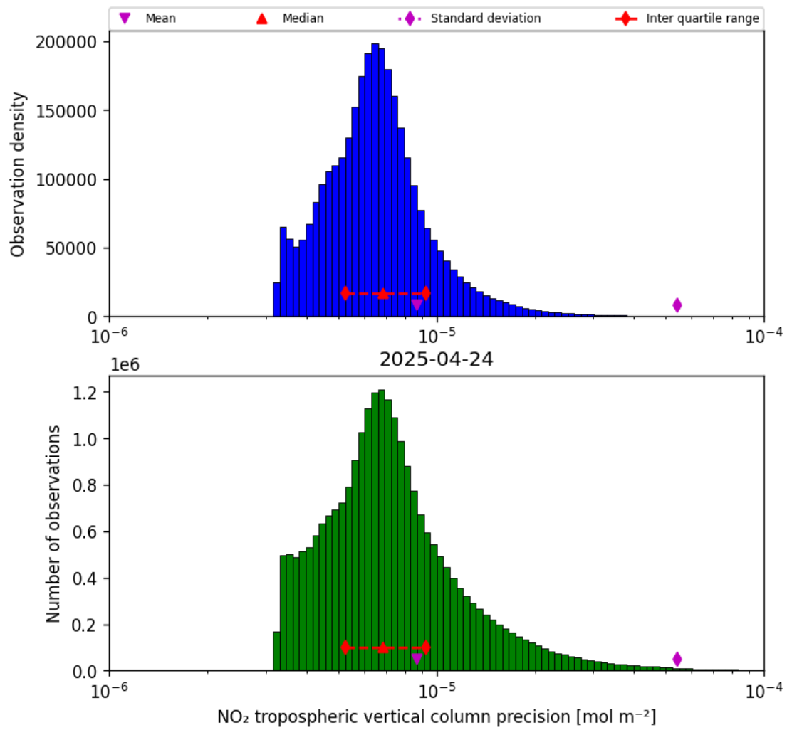
Figure 28: Histogram of “NO 2 tropospheric vertical column precision” for 2025-04-24 to 2025-04-25
