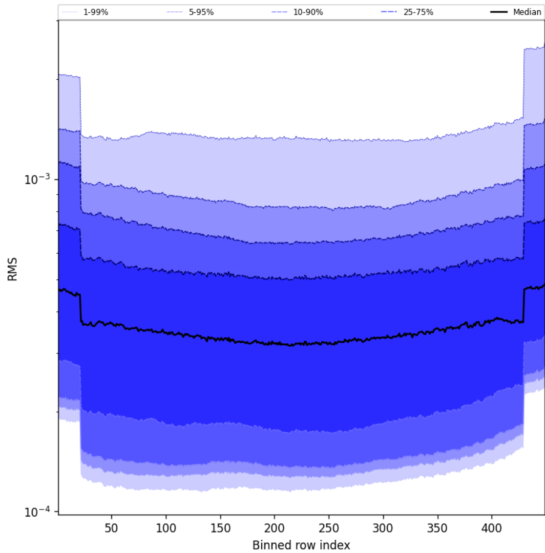
Figure 58: Along track statistics of “RMS” for 2025-04-24 to 2025-04-25
