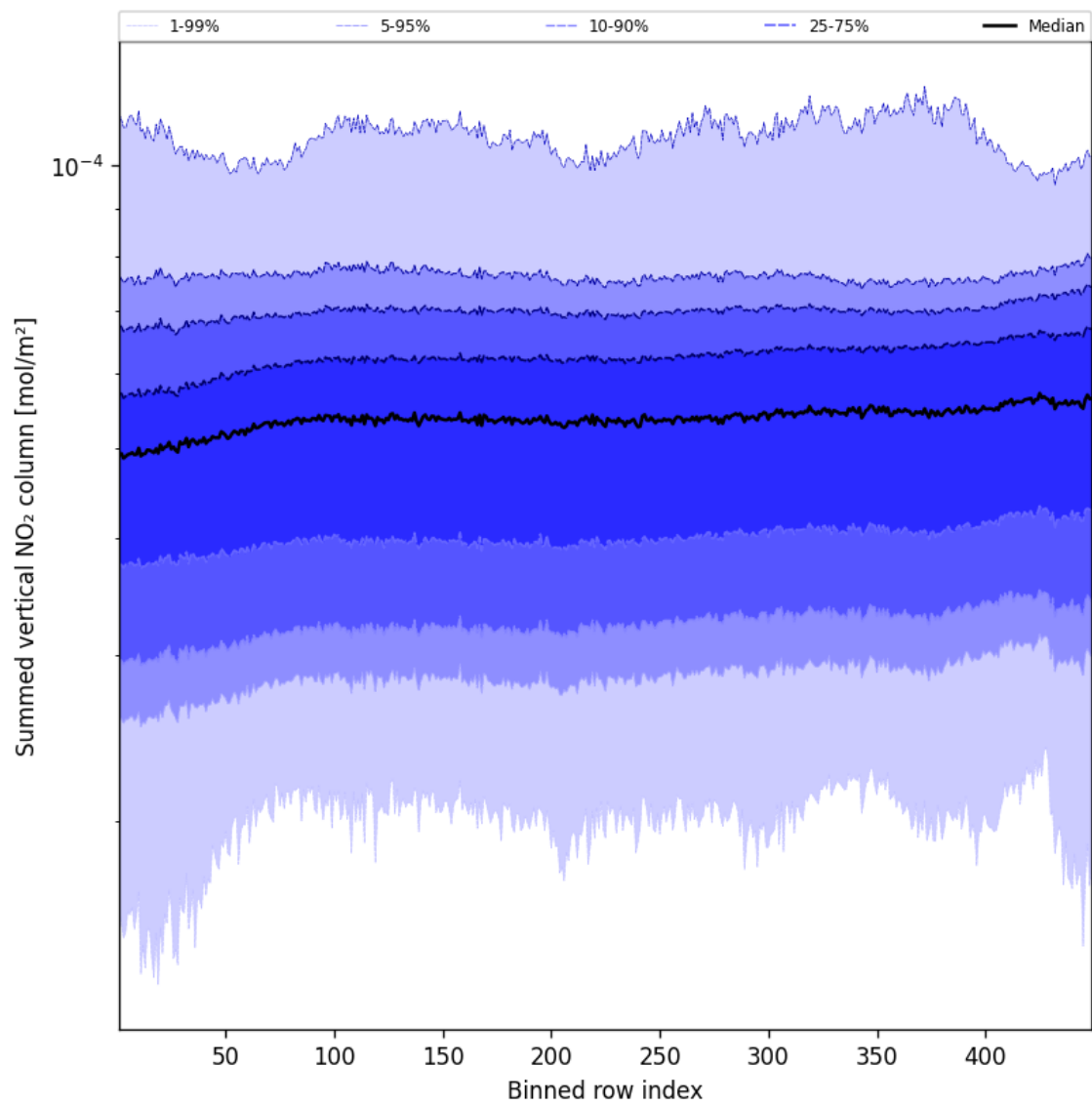
Figure 55: Along track statistics of “Summed vertical NO 2 column” for 2025-04-24 to 2025-04-25
