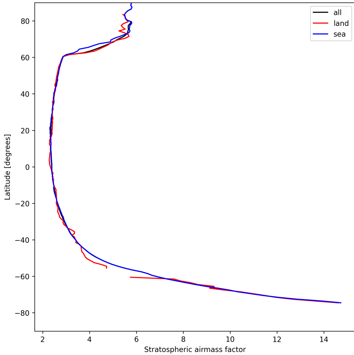
Figure 25: Zonal average of “Stratospheric airmass factor” for 2025-04-24 to 2025-04-25.
