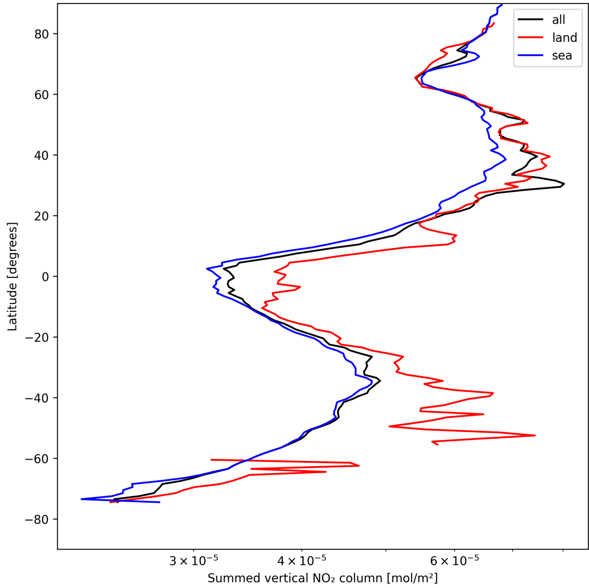
Figure 21: Zonal average of “Summed vertical NO 2 column” for 2025-04-24 to 2025-04-25.
