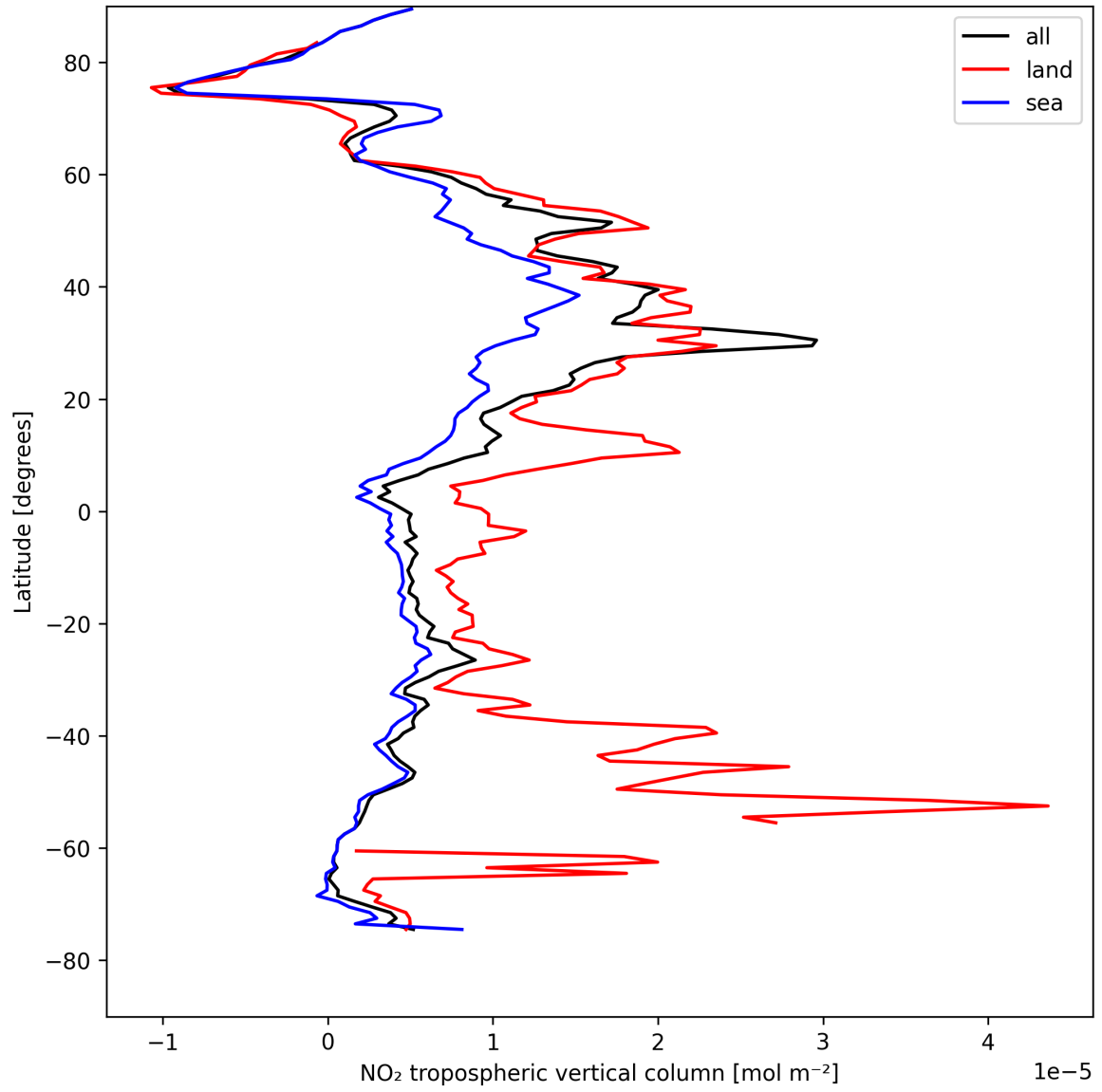
Figure 10: Zonal average of “NO 2 tropospheric vertical column” for 2025-04-24 to 2025-04-25.
