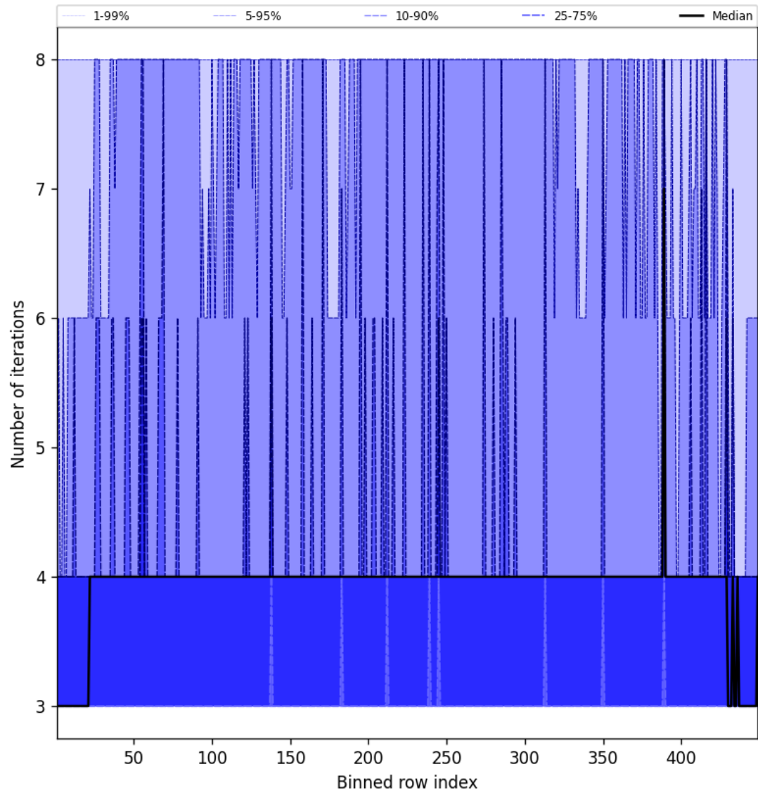
Figure 49: Along track statistics of “Number of iterations” for 2025-04-24 to 2025-04-25
