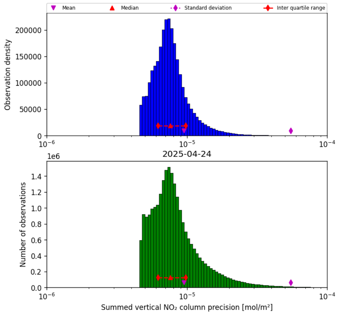
Figure 39: Histogram of "Summed vertical NO 2 column precision" for 2025-04-24 to 2025-04-25
