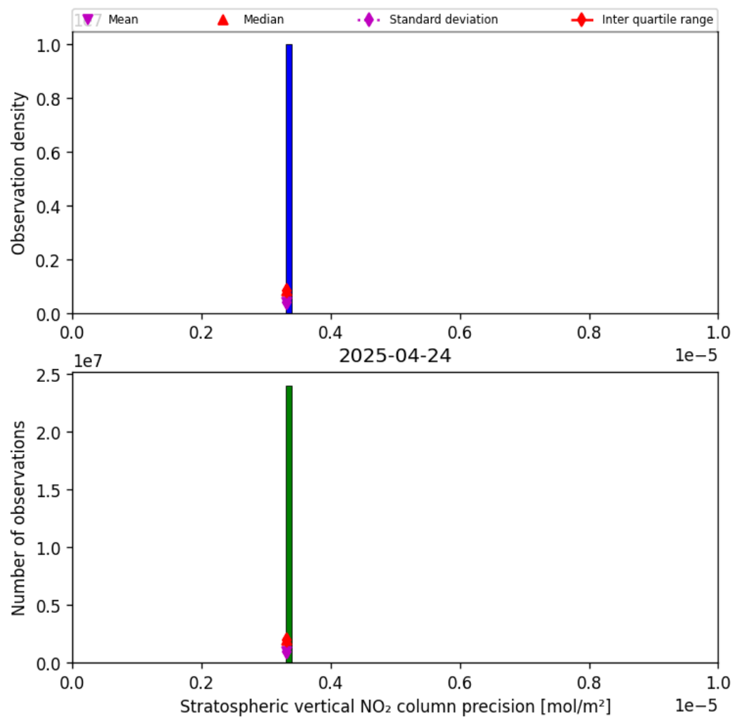
Figure 35: Histogram of “Stratospheric vertical NO 2 column precision” for 2025-04-24 to 2025-04-25
