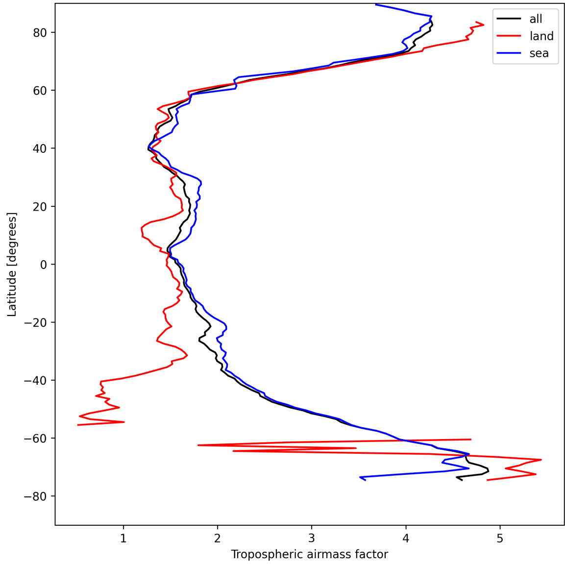
Figure 12: Zonal average of “Tropospheric air mass factor” for 2025-04-24 to 2025-04-25.
