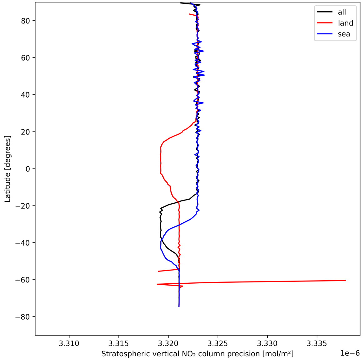
Figure 18: Zonal average of “Stratospheric vertical NO 2 column precision” for 2025-04-24 to 2025-04-25.
