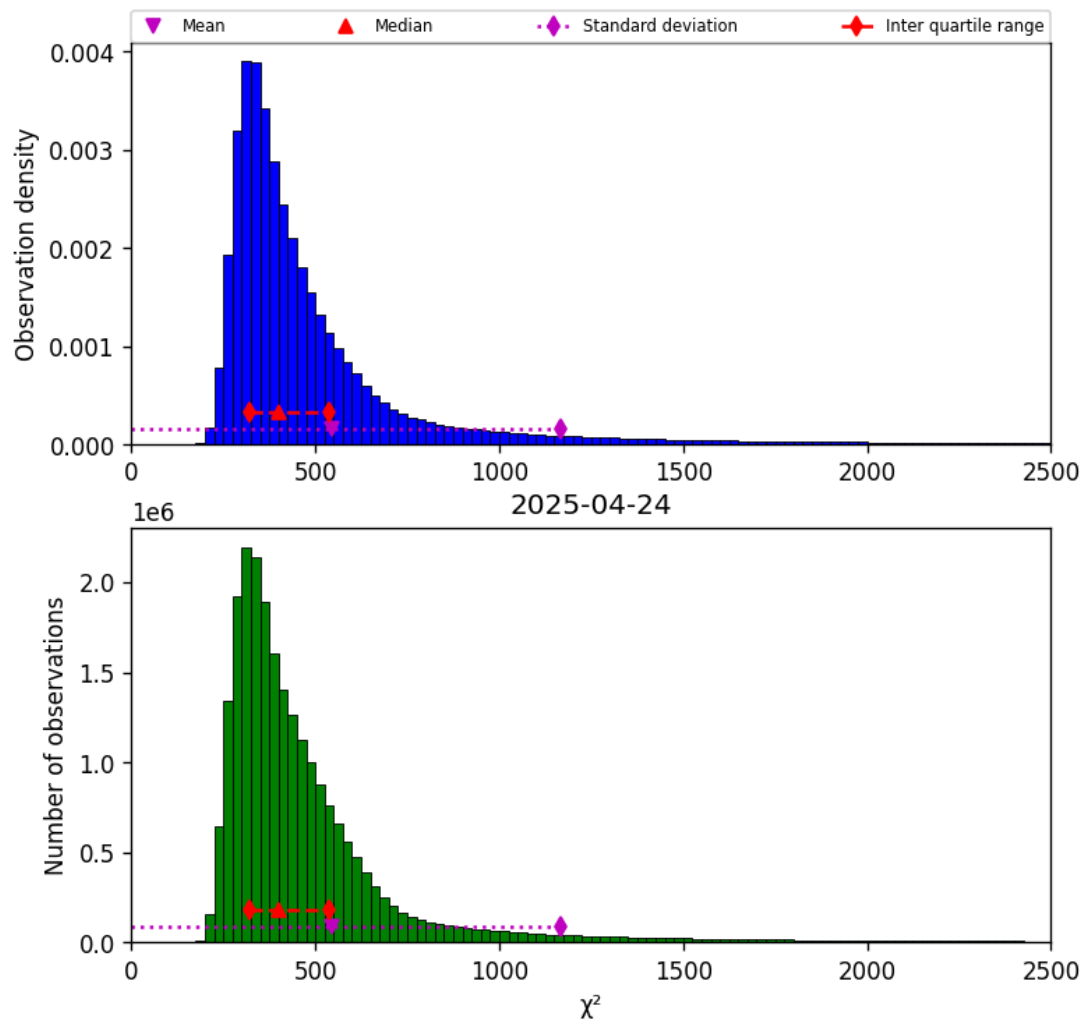
Figure 40: Histogram of “ \chi^2 ” for 2025-04-24 to 2025-04-25
