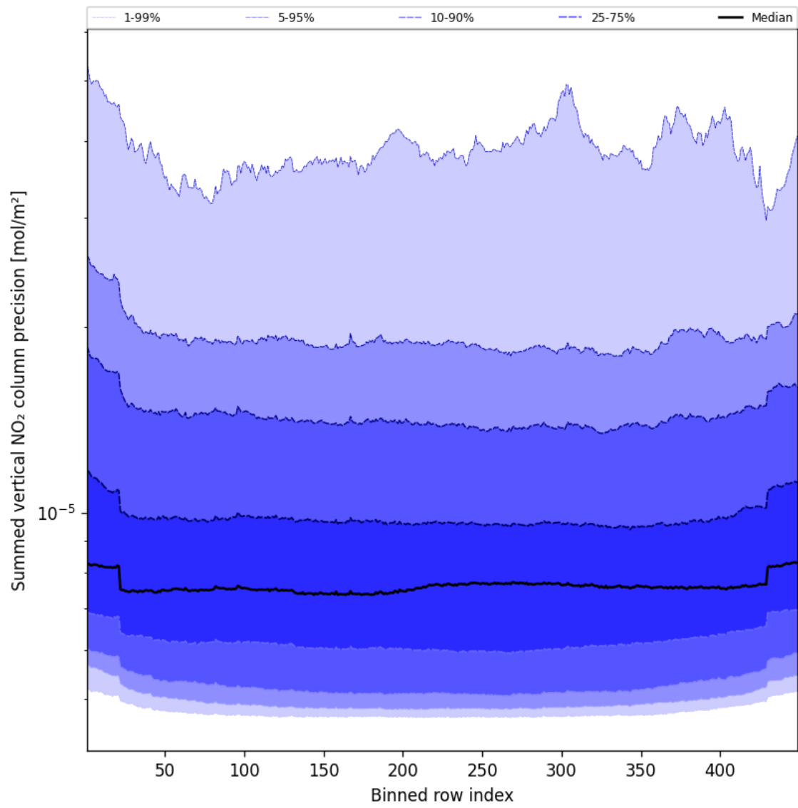
Figure 56: Along track statistics of “Summed vertical NO 2 column precision” for 2025-04-24 to 2025-04-25
