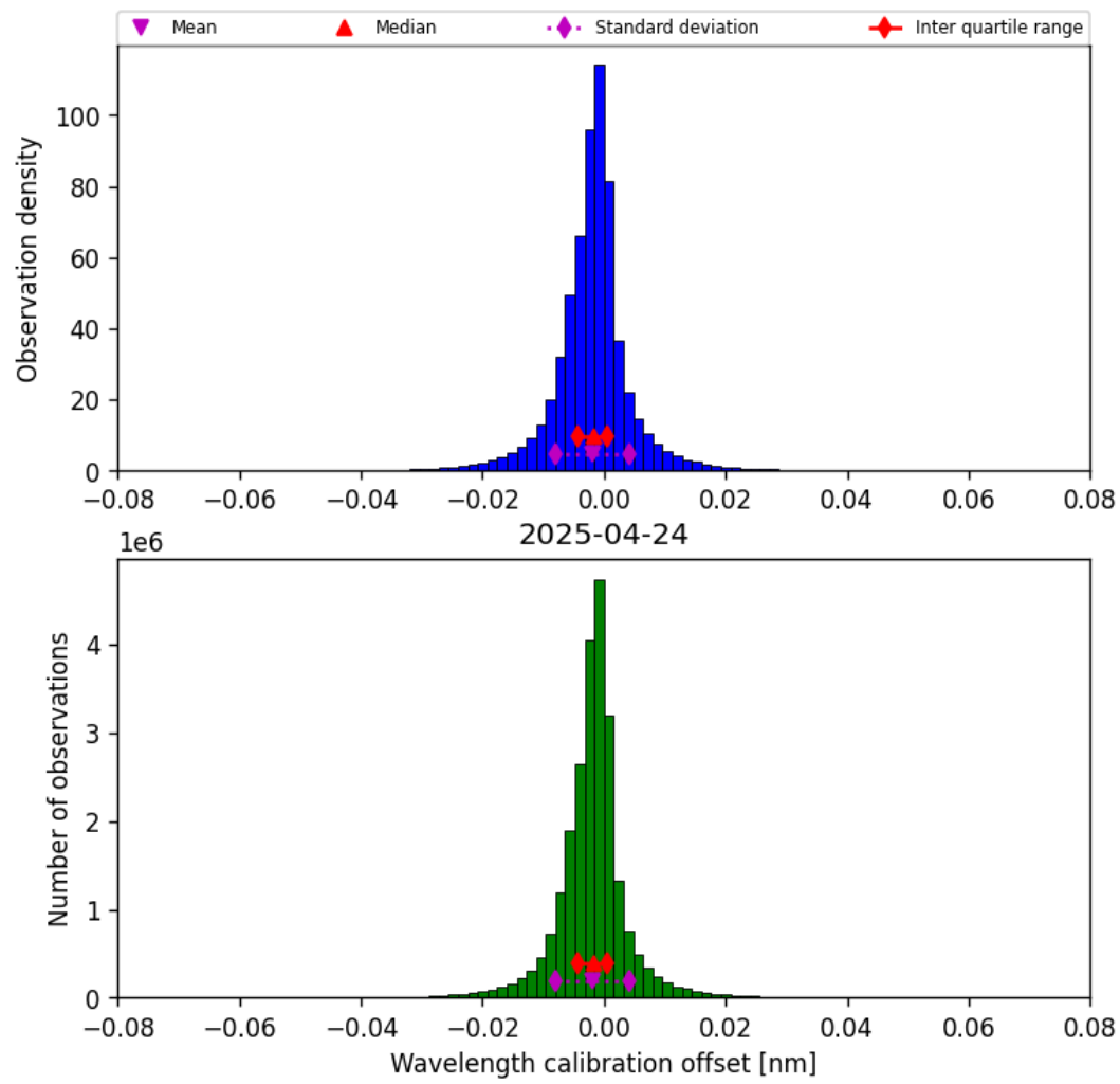
Figure 33: Histogram of “Wavelength calibration offset” for 2025-04-24 to 2025-04-25
