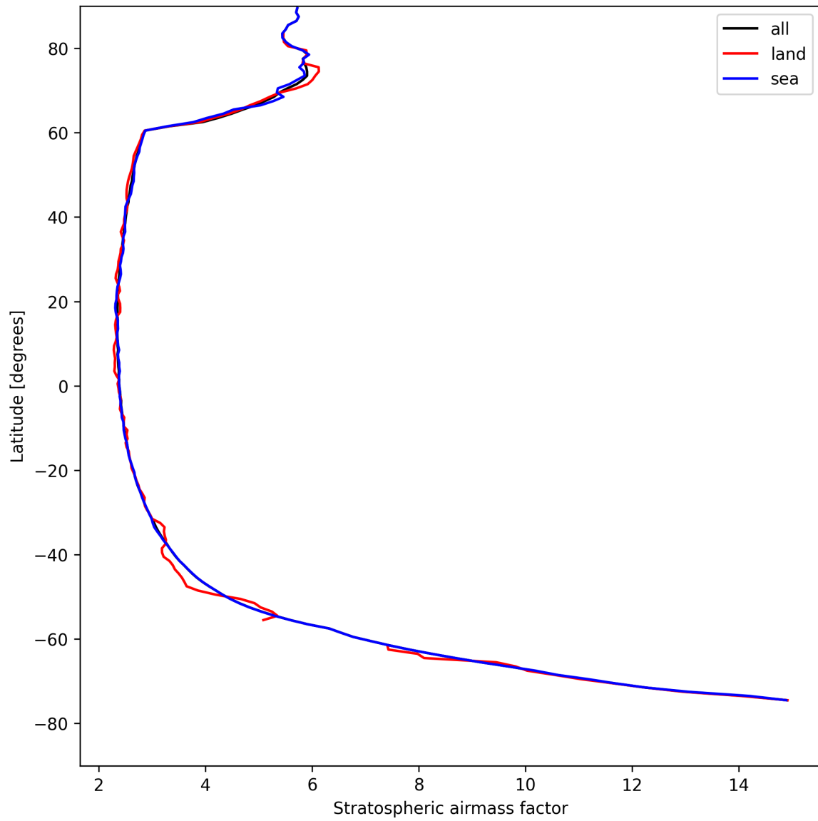
Figure 25: Zonal average of “Stratospheric airmass factor” for 2025-04-25 to 2025-04-26.
