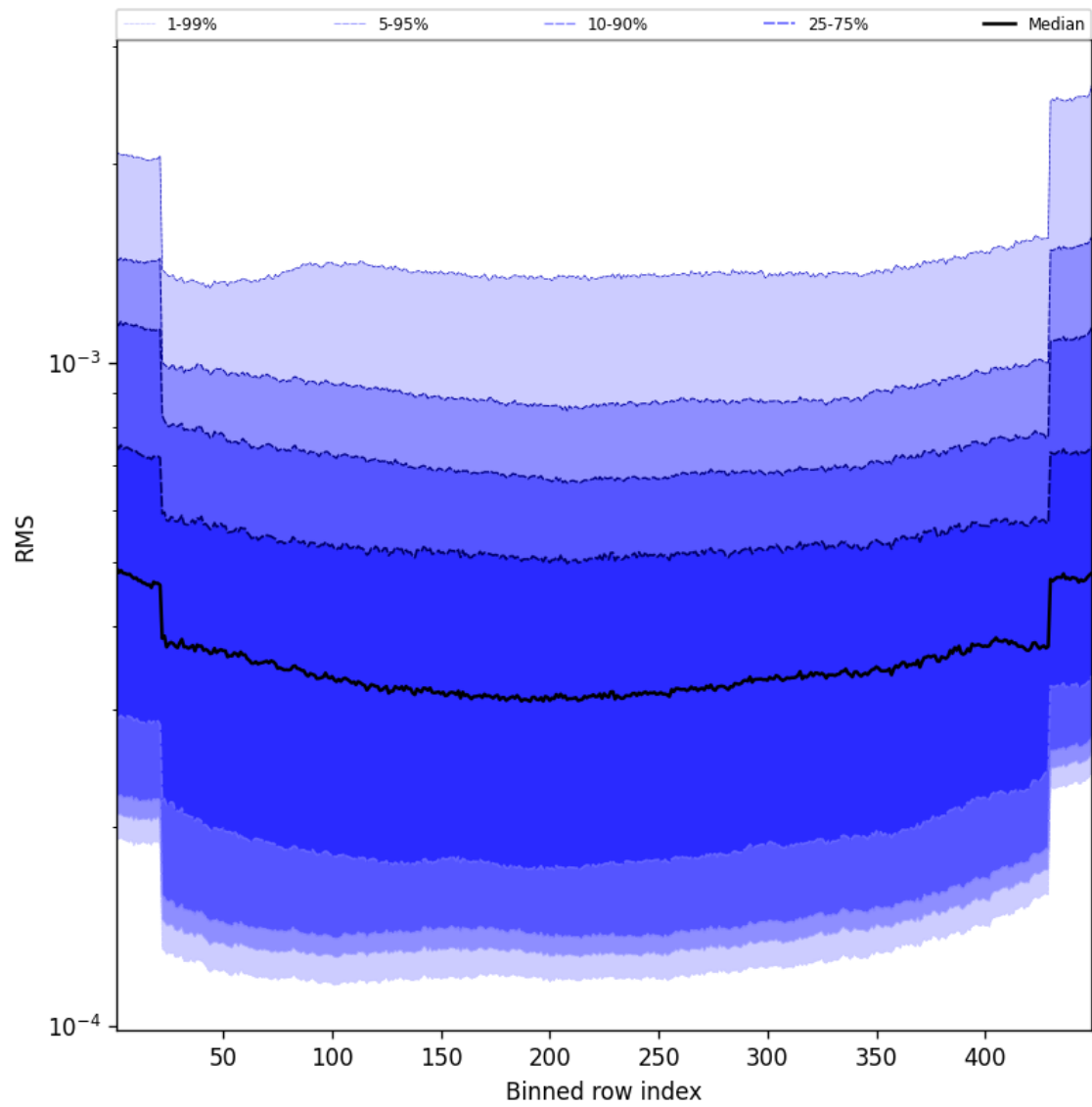
Figure 58: Along track statistics of “RMS” for 2025-04-25 to 2025-04-26
