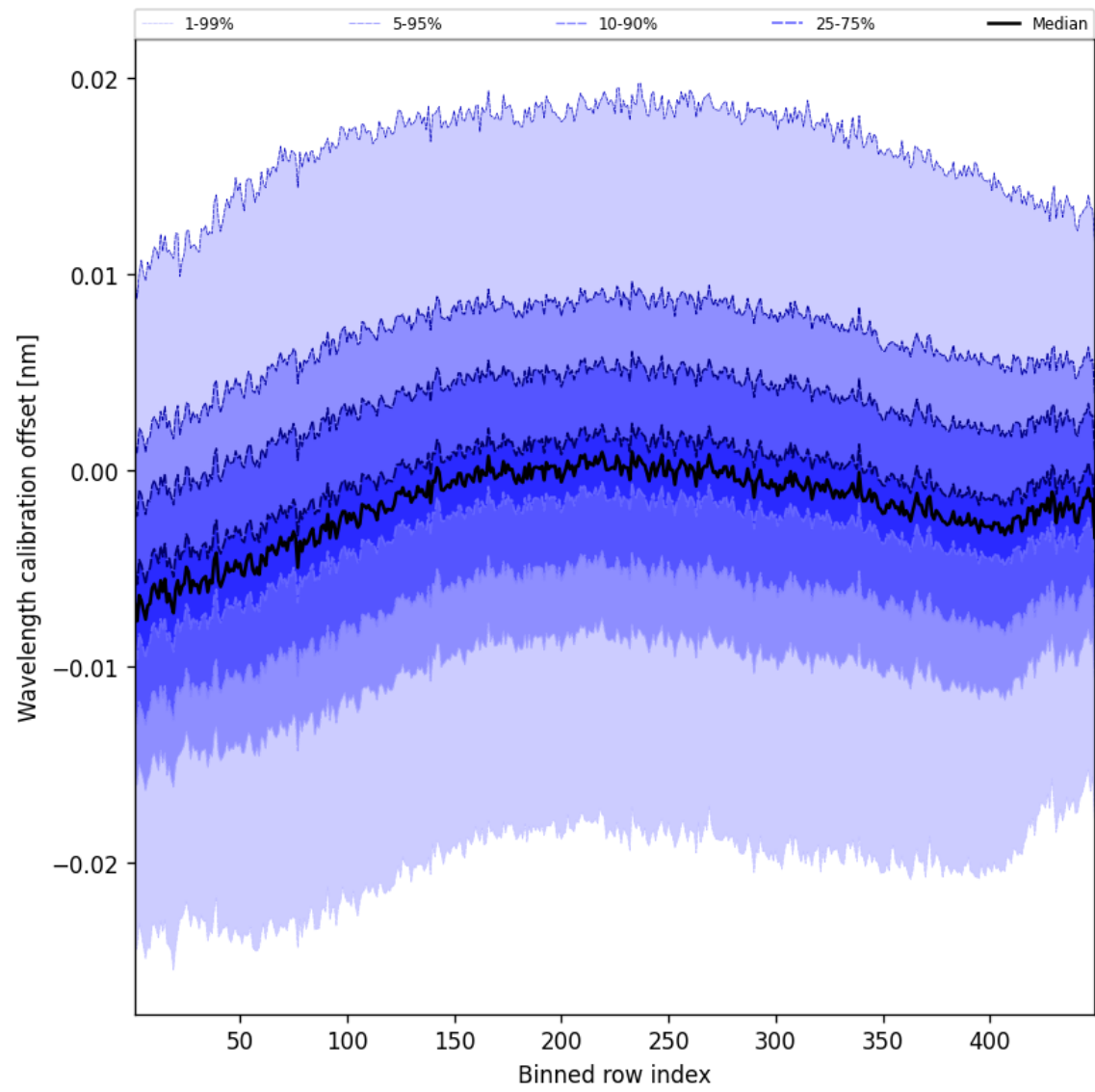
Figure 50: Along track statistics of “Wavelength calibration offset” for 2025-04-25 to 2025-04-26
