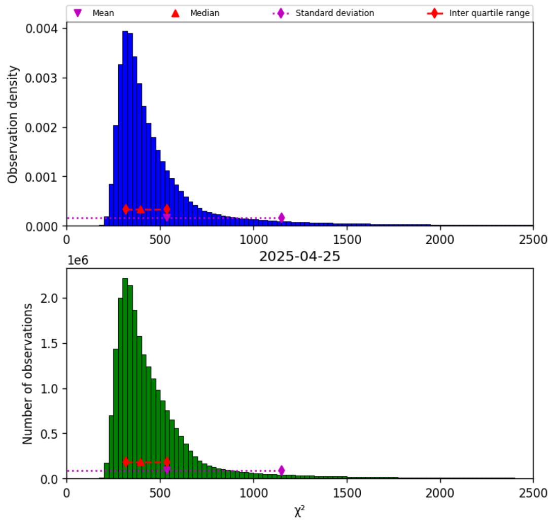
Figure 40: Histogram of “ \chi^2 ” for 2025-04-25 to 2025-04-26
