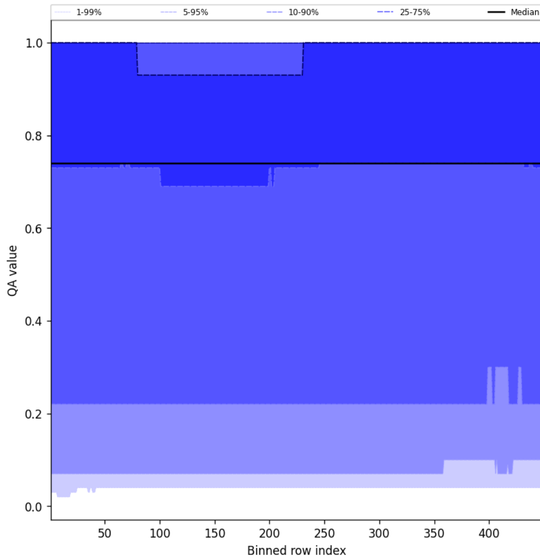
Figure 43: Along track statistics of “QA value” for 2025-04-25 to 2025-04-26
