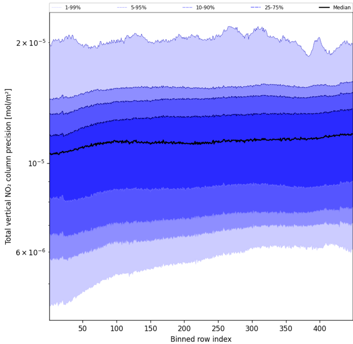
Figure 54: Along track statistics of "Total vertical NO 2 column precision" for 2025-04-25 to 2025-04-26
