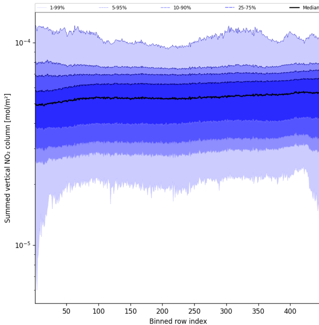
Figure 55: Along track statistics of “Summed vertical NO 2 column” for 2025-04-25 to 2025-04-26
