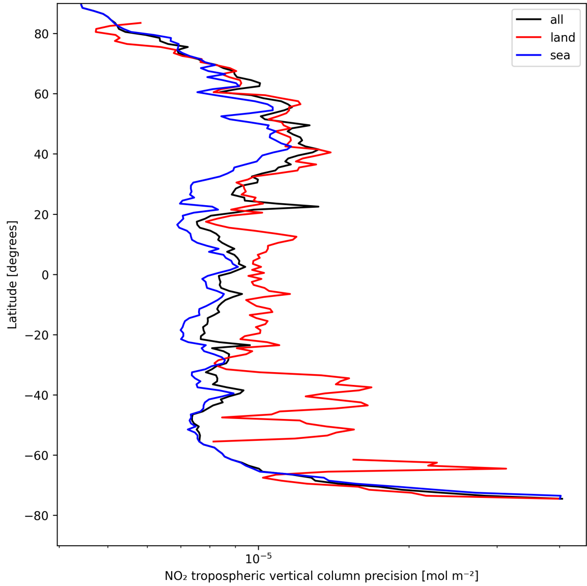
Figure 11: Zonal average of “NO 2 tropospheric vertical column precision” for 2025-04-25 to 2025-04-26.
