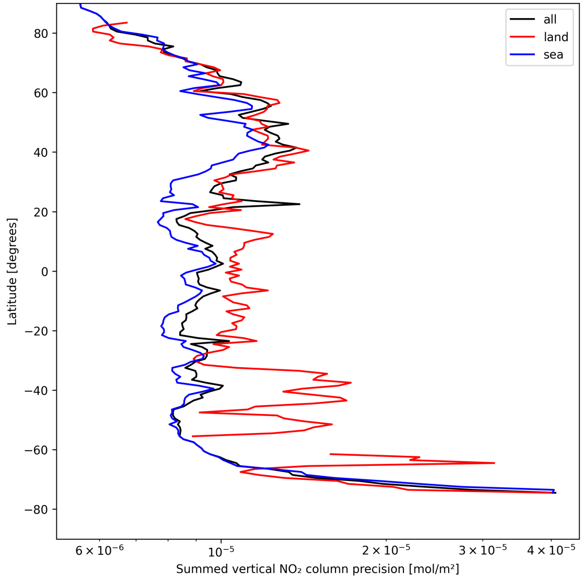
Figure 22: Zonal average of “Summed vertical NO 2 column precision” for 2025-04-25 to 2025-04-26.
