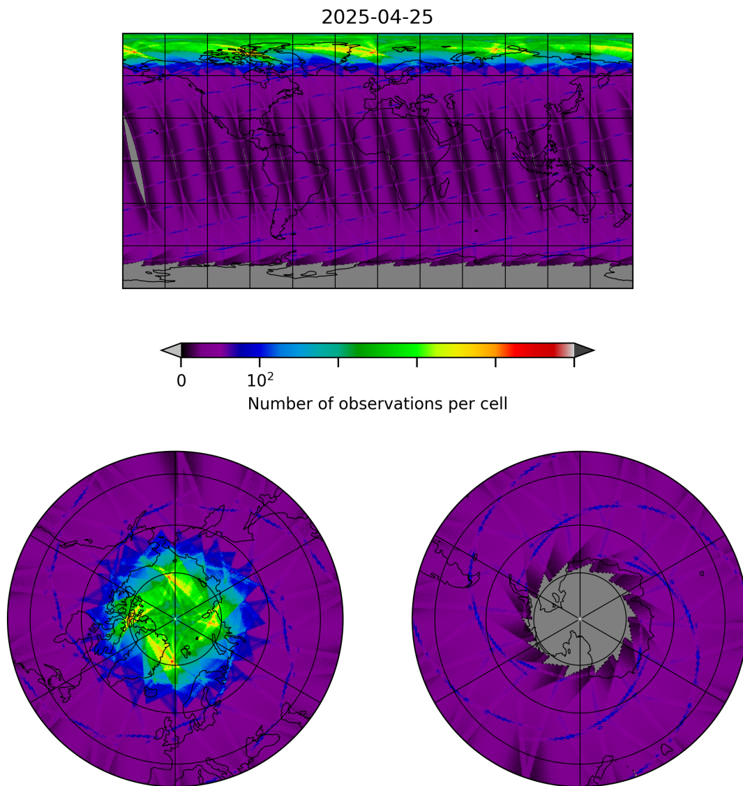
Figure 8: Map of the number of observations for 2025-04-25 to 2025-04-26
