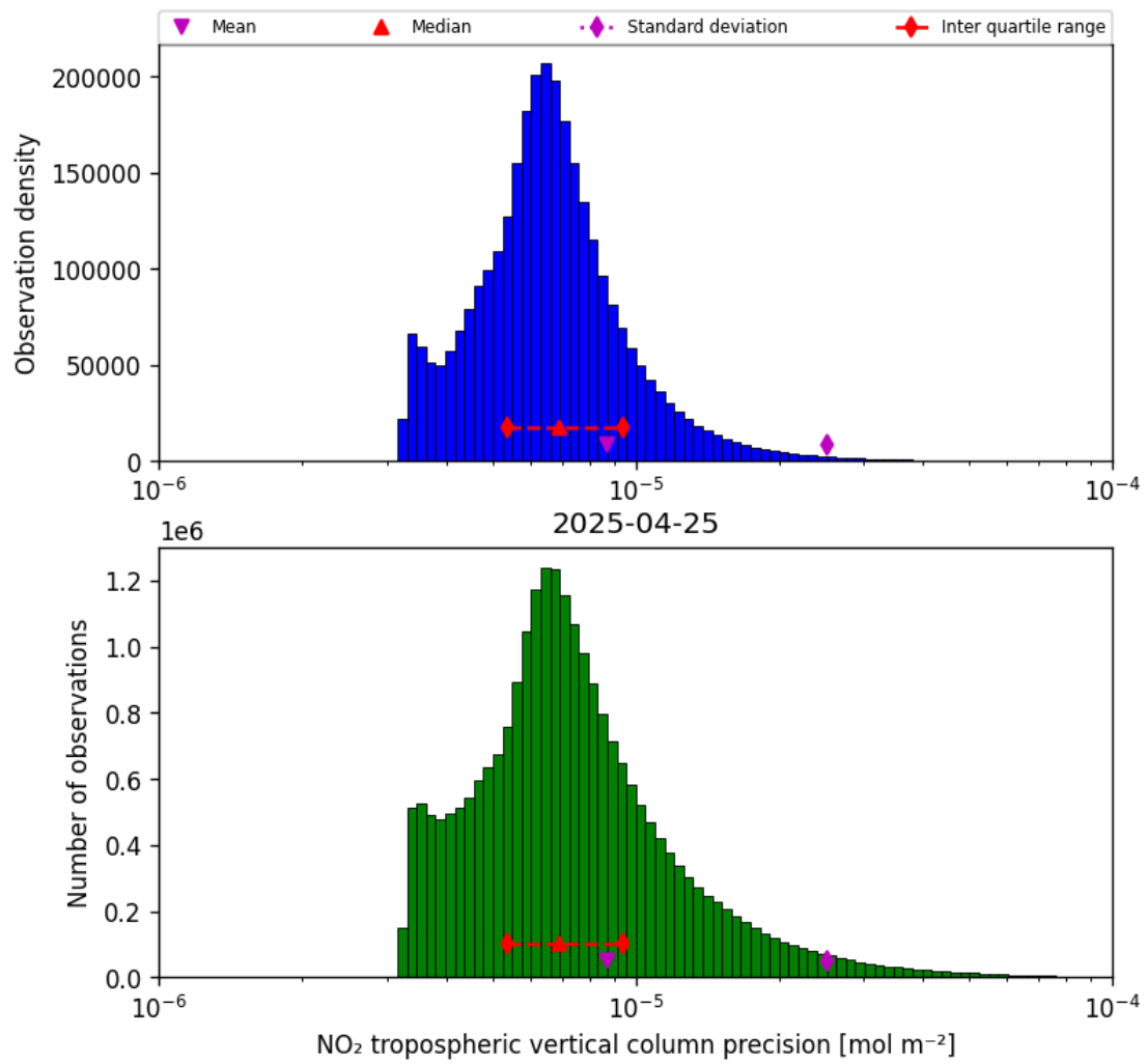
Figure 28: Histogram of “NO 2 tropospheric vertical column precision” for 2025-04-25 to 2025-04-26
