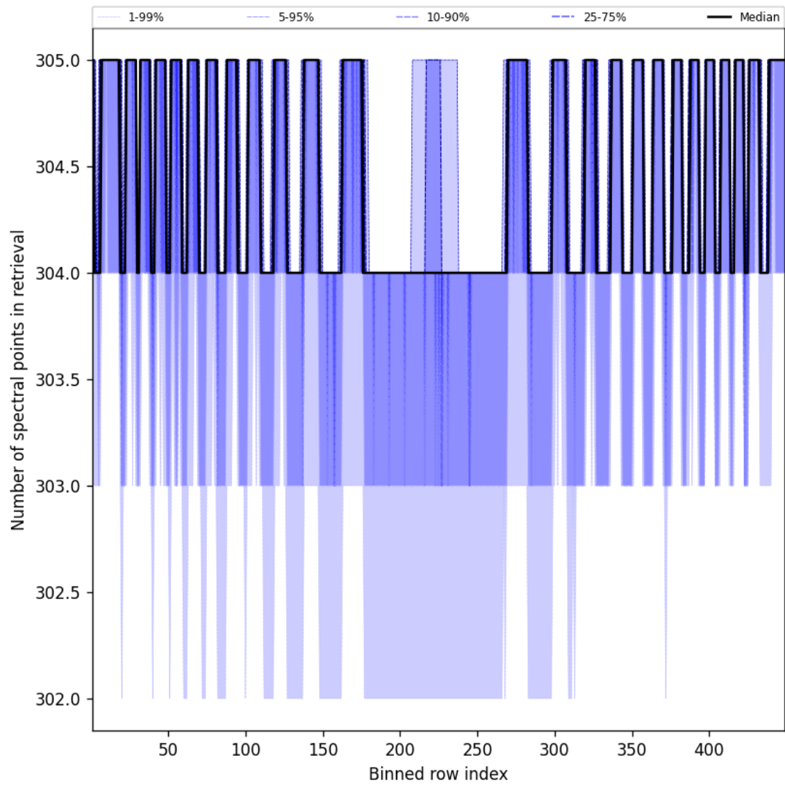
Figure 48: Along track statistics of “Number of spectral points in retrieval” for 2025-04-25 to 2025-04-26
