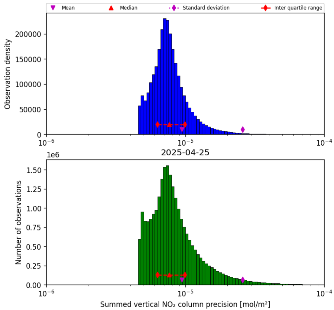
Figure 39: Histogram of "Summed vertical NO 2 column precision" for 2025-04-25 to 2025-04-26
