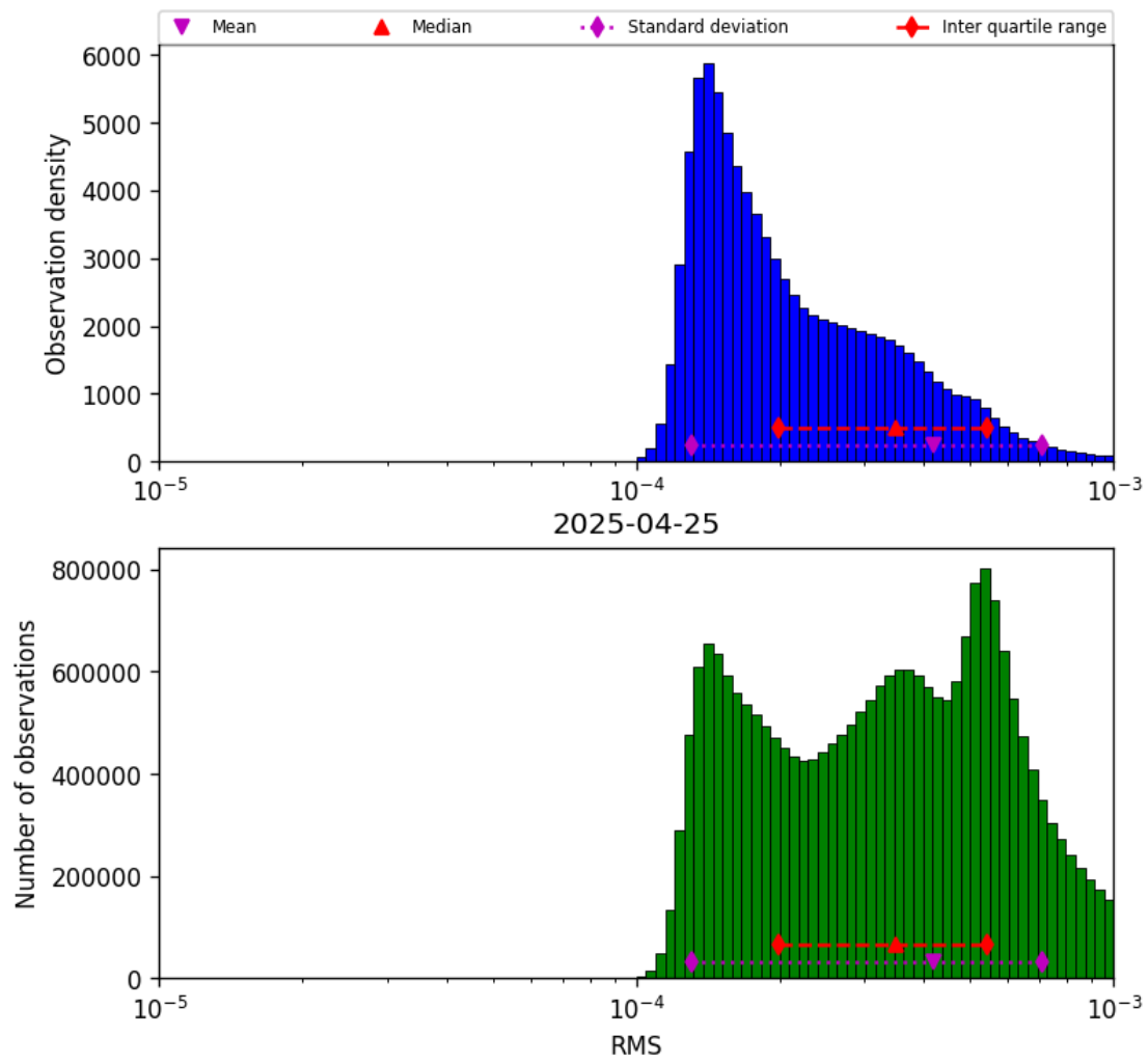
Figure 41: Histogram of “RMS” for 2025-04-25 to 2025-04-26
