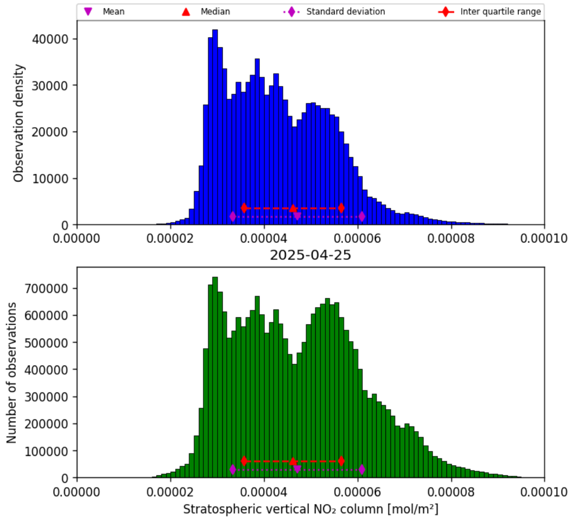
Figure 34: Histogram of “Stratospheric vertical NO 2 column” for 2025-04-25 to 2025-04-26
