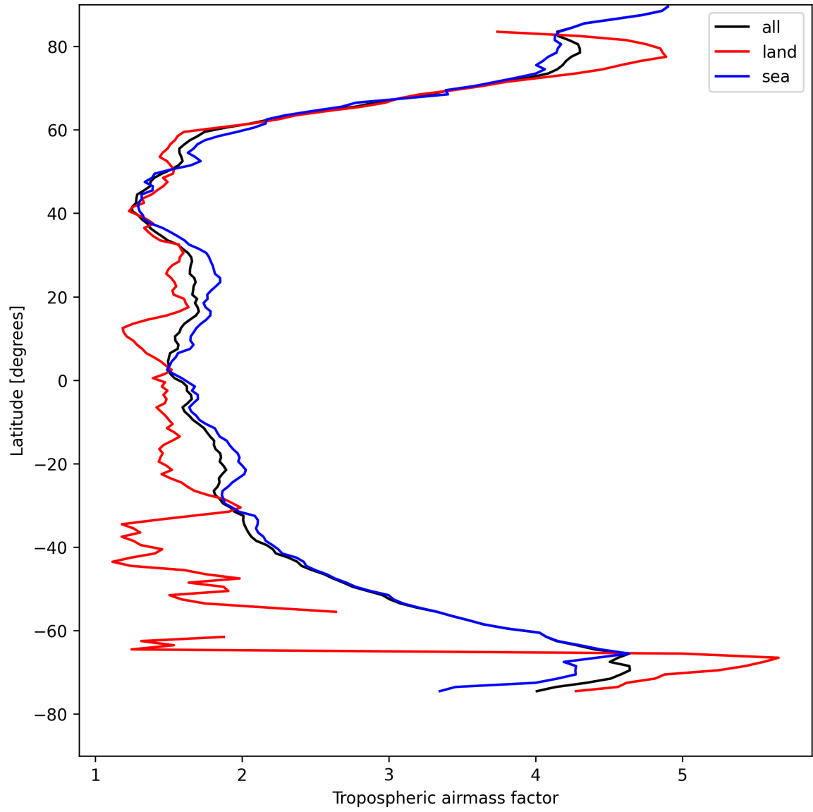
Figure 12: Zonal average of “Tropospheric airmass factor” for 2025-04-25 to 2025-04-26.
