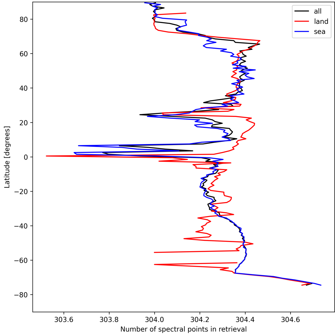
Figure 14: Zonal average of “Number of spectral points in retrieval” for 2025-04-25 to 2025-04-26.
