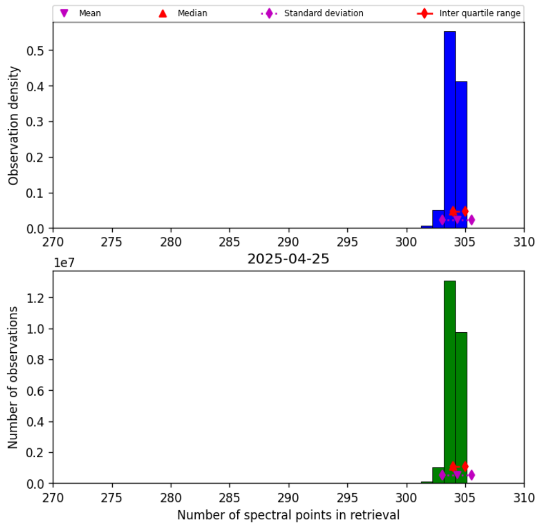
Figure 31: Histogram of “Number of spectral points in retrieval” for 2025-04-25 to 2025-04-26
