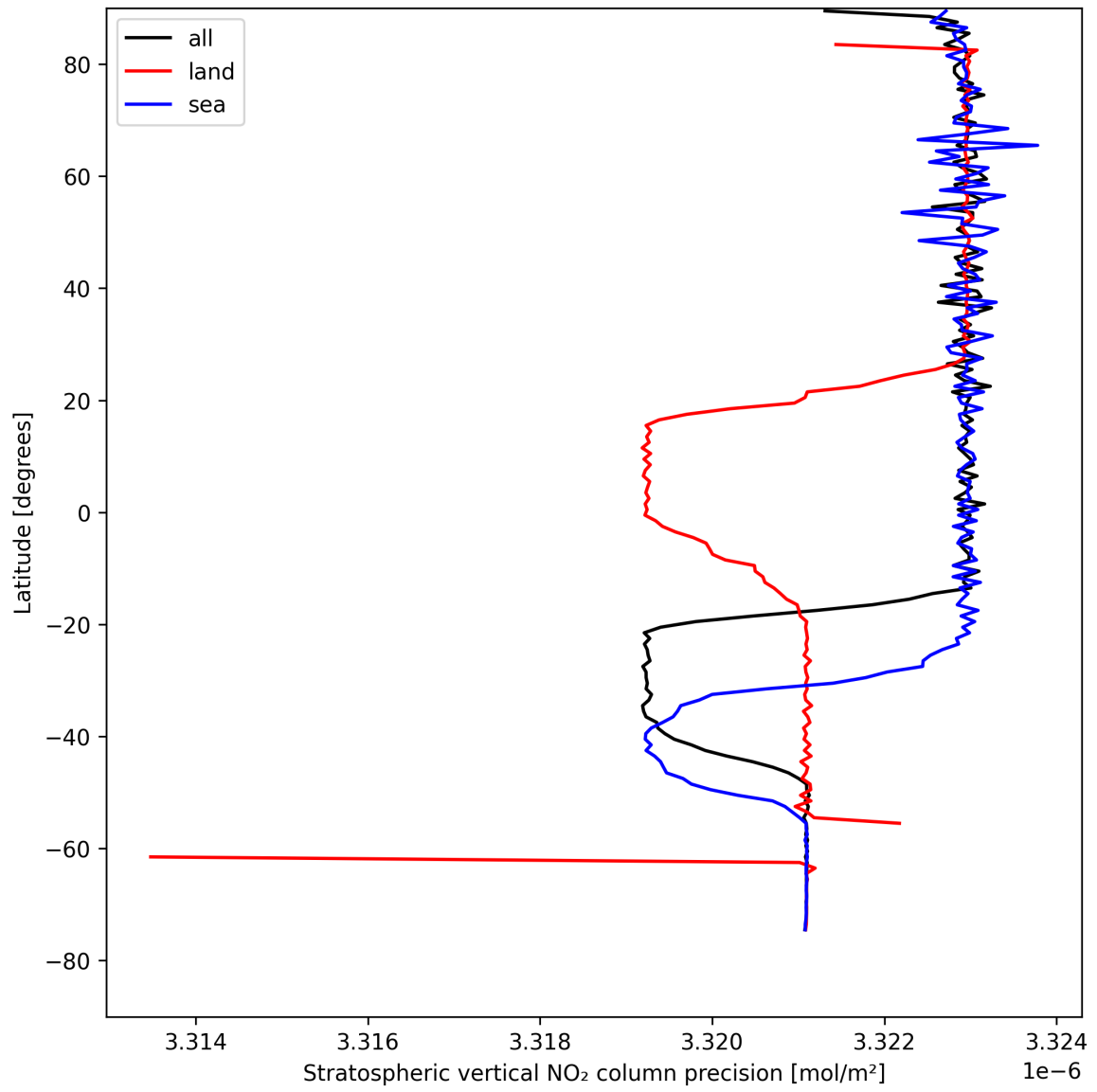
Figure 18: Zonal average of “Stratospheric vertical NO 2 column precision” for 2025-04-25 to 2025-04-26.
