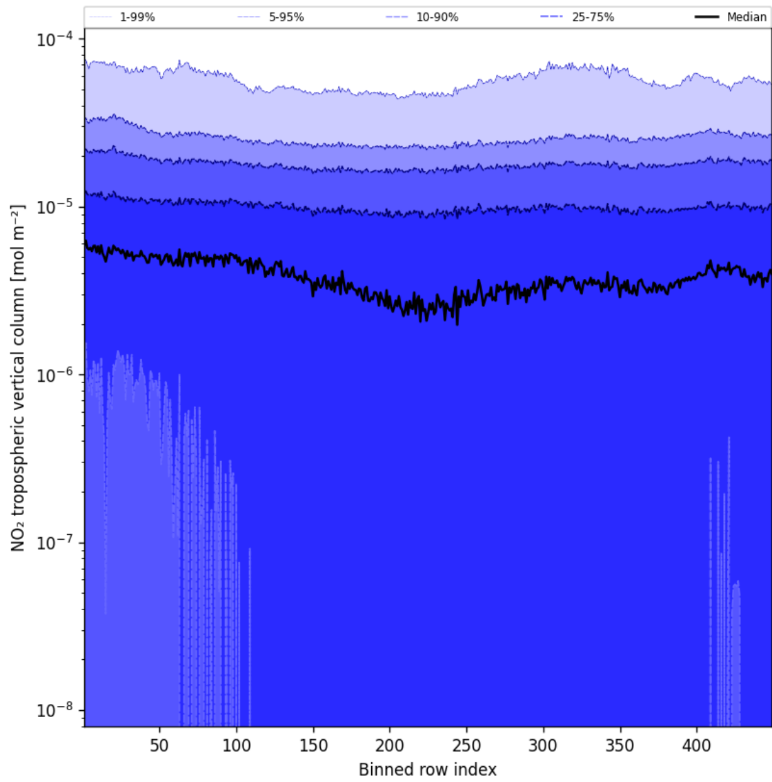
Figure 44: Along track statistics of “NO 2 tropospheric vertical column” for 2025-04-25 to 2025-04-26
