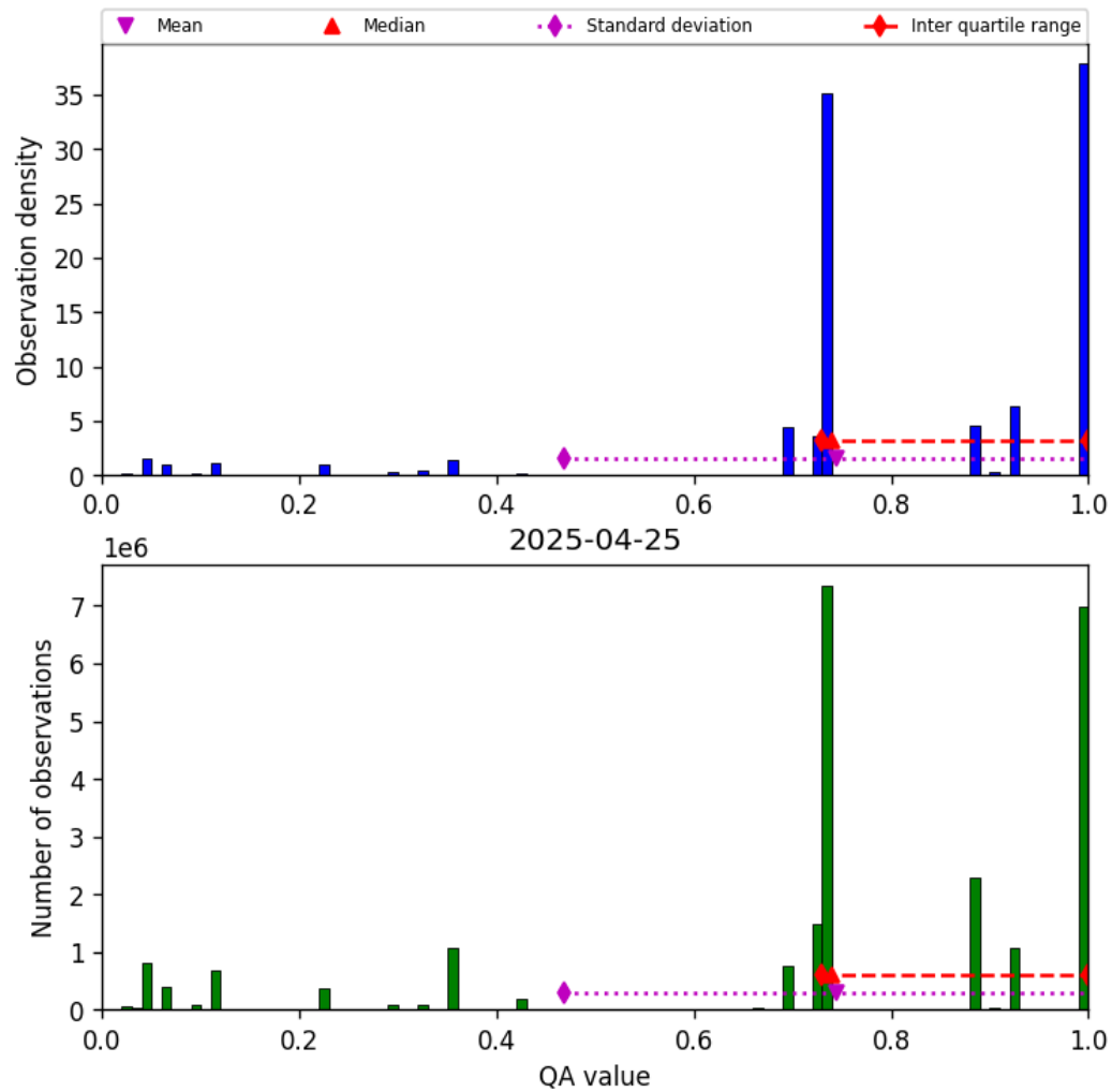
Figure 26: Histogram of “QA value” for 2025-04-25 to 2025-04-26
