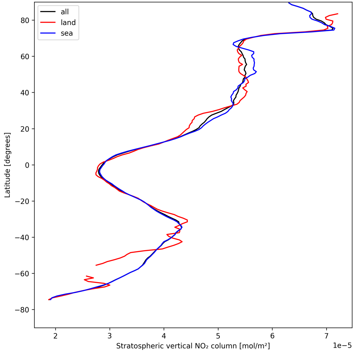
Figure 17: Zonal average of “Stratospheric vertical NO 2 column” for 2025-04-25 to 2025-04-26.
