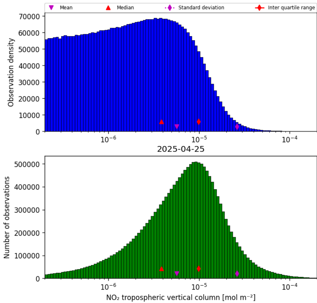
Figure 27: Histogram of “NO 2 tropospheric vertical column” for 2025-04-25 to 2025-04-26
