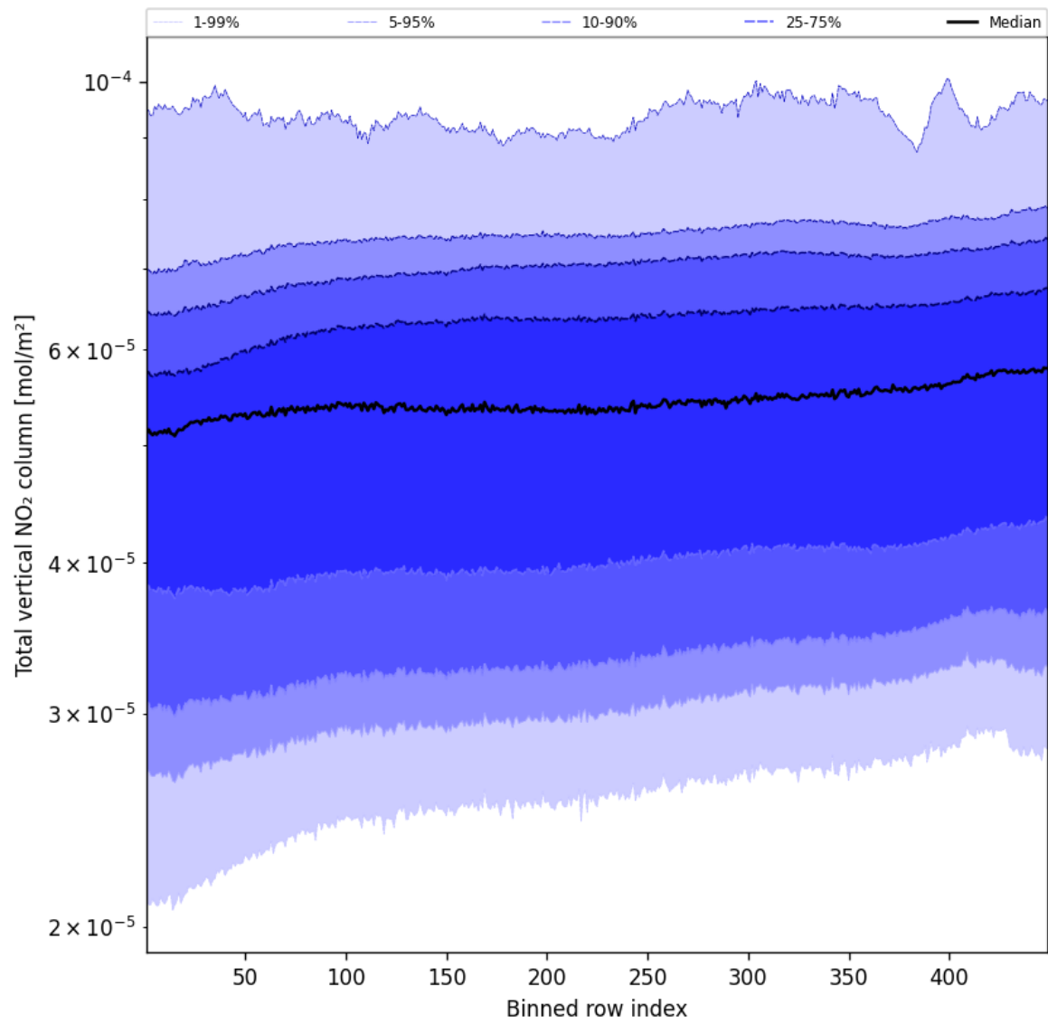
Figure 53: Along track statistics of “Total vertical NO 2 column” for 2025-04-25 to 2025-04-26
