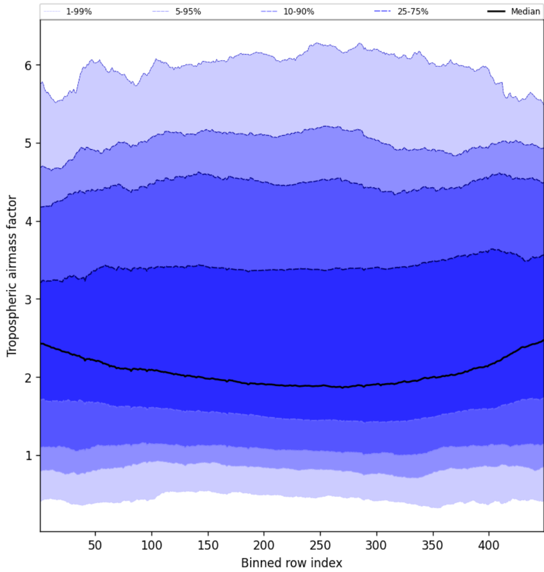
Figure 46: Along track statistics of “Tropospheric airmass factor” for 2025-04-25 to 2025-04-26
