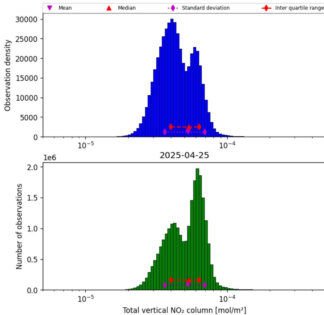
Figure 36: Histogram of "Total vertical NO 2 column" for 2025-04-25 to 2025-04-26
