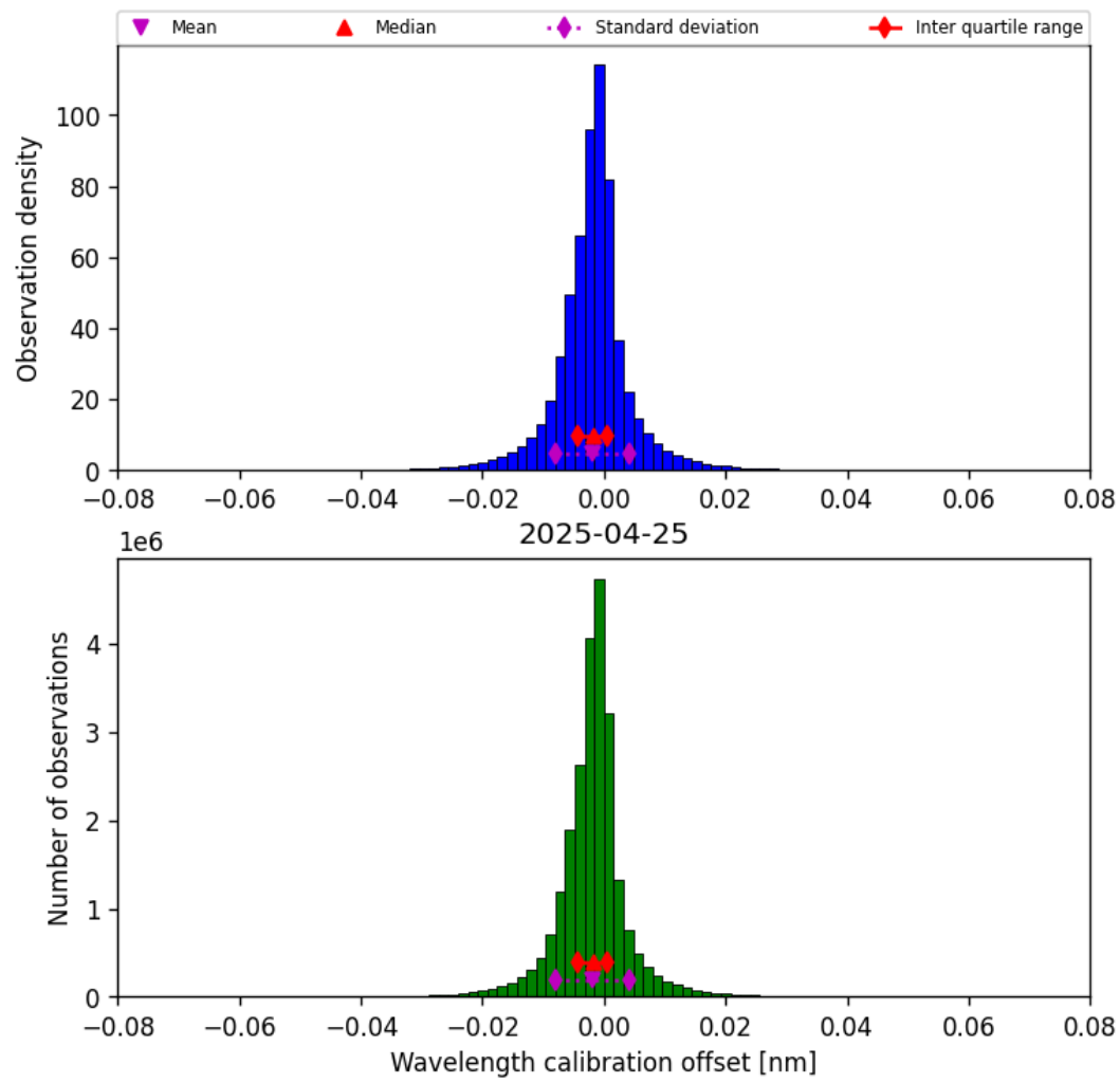
Figure 33: Histogram of “Wavelength calibration offset” for 2025-04-25 to 2025-04-26
