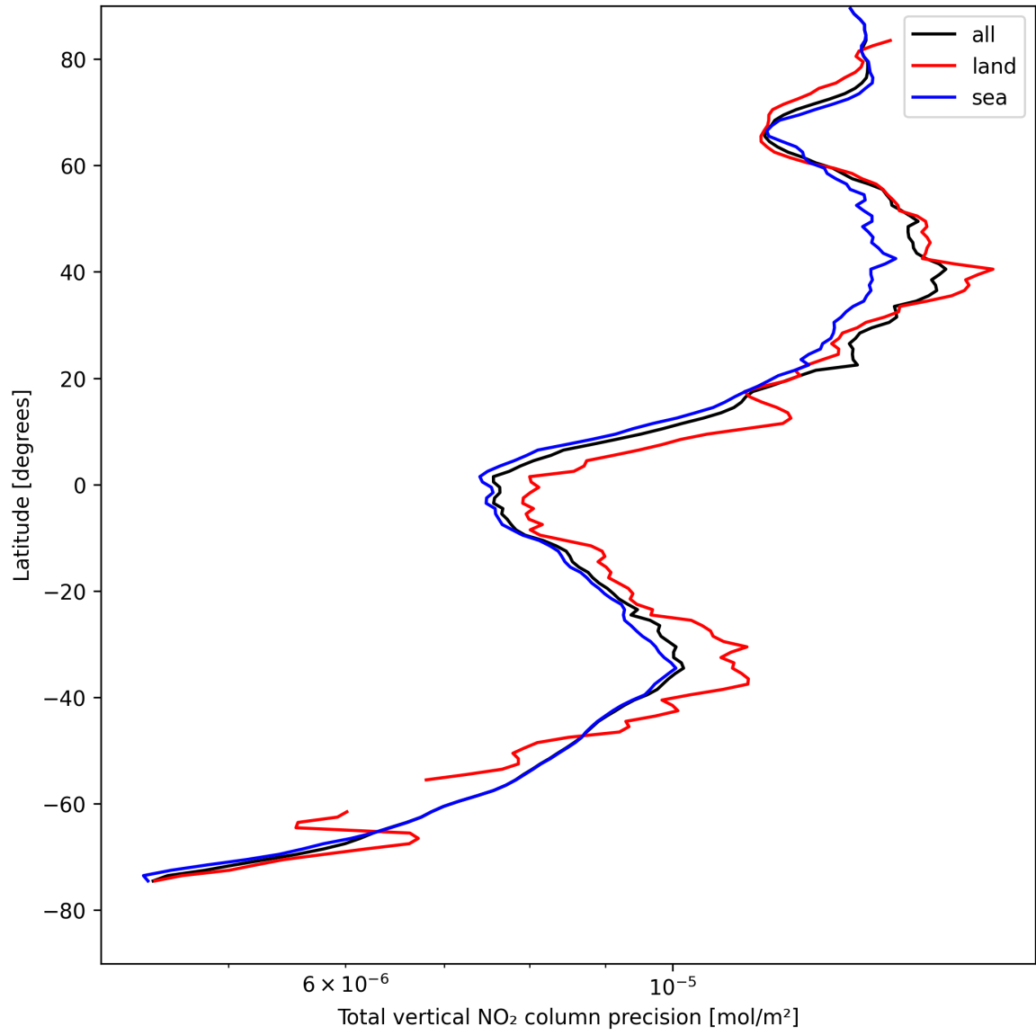
Figure 20: Zonal average of “Total vertical NO 2 column precision” for 2025-04-25 to 2025-04-26.
