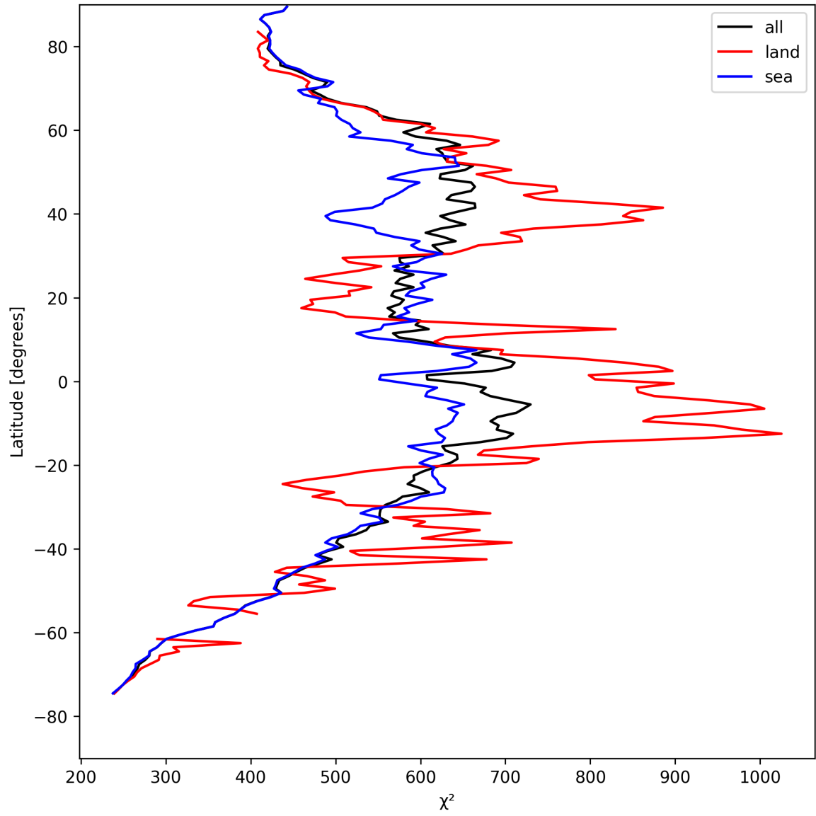
Figure 23: Zonal average of “ \chi^2 ” for 2025-04-25 to 2025-04-26.
