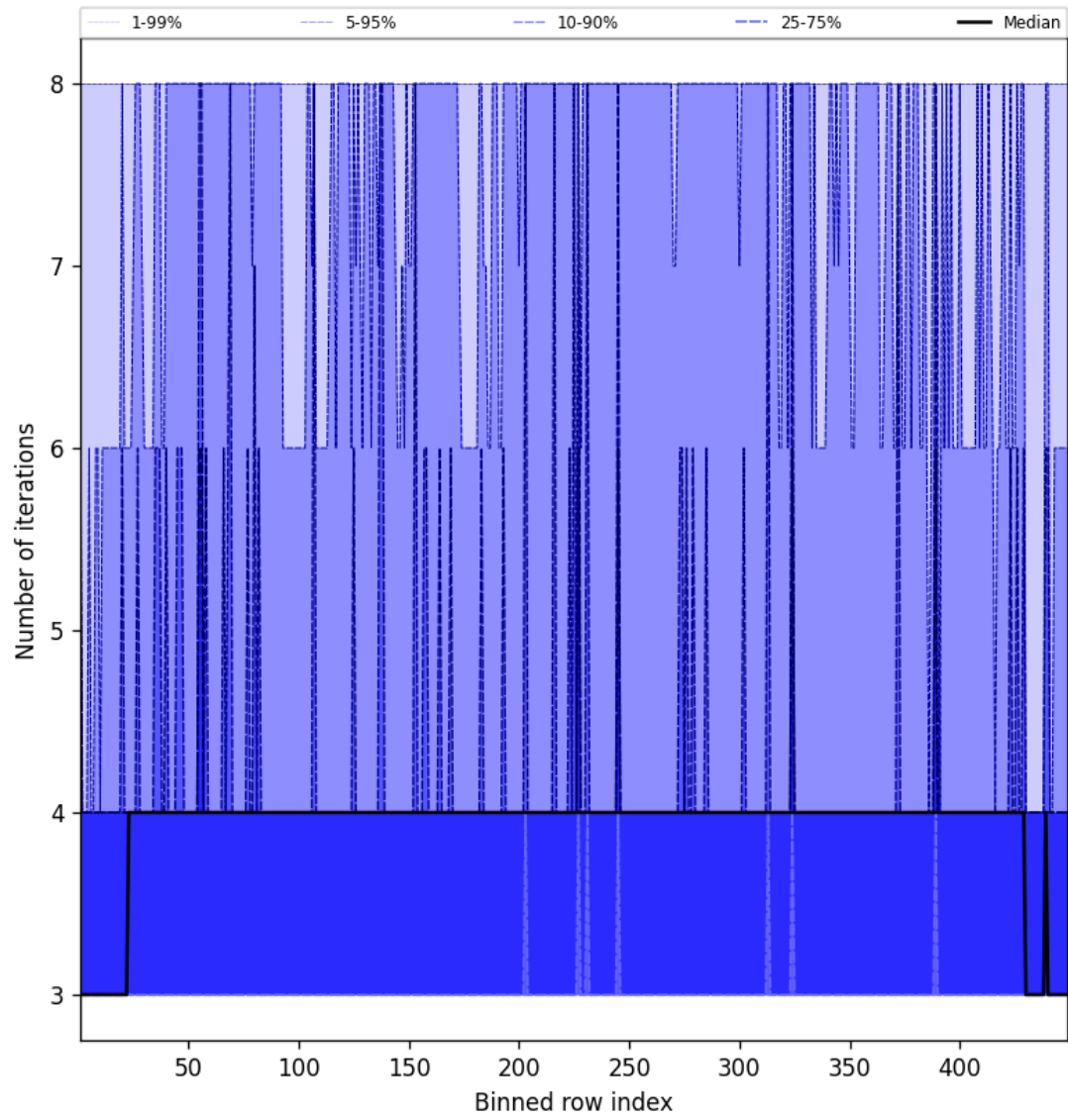
Figure 49: Along track statistics of “Number of iterations” for 2025-04-25 to 2025-04-26
