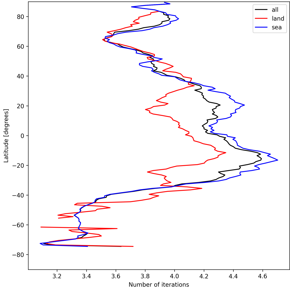
Figure 15: Zonal average of “Number of iterations” for 2025-04-25 to 2025-04-26.
