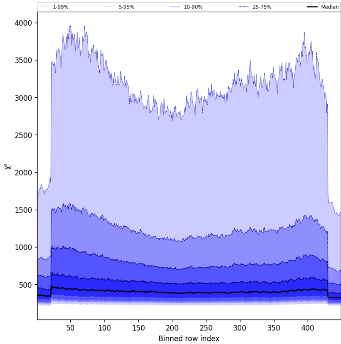
Figure 57: Along track statistics of “ \chi^2 ” for 2025-04-25 to 2025-04-26
