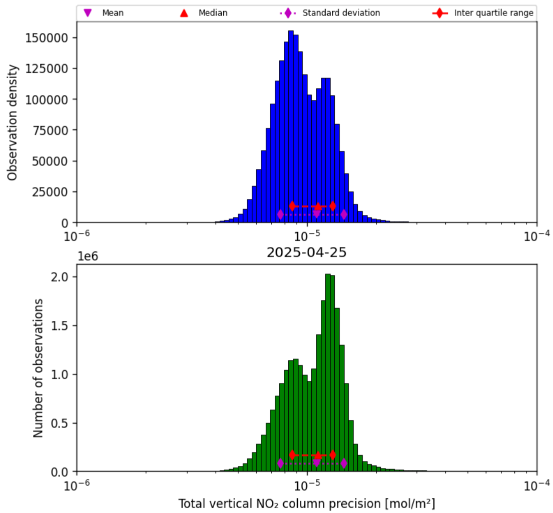
Figure 37: Histogram of “Total vertical NO 2 column precision” for 2025-04-25 to 2025-04-26
