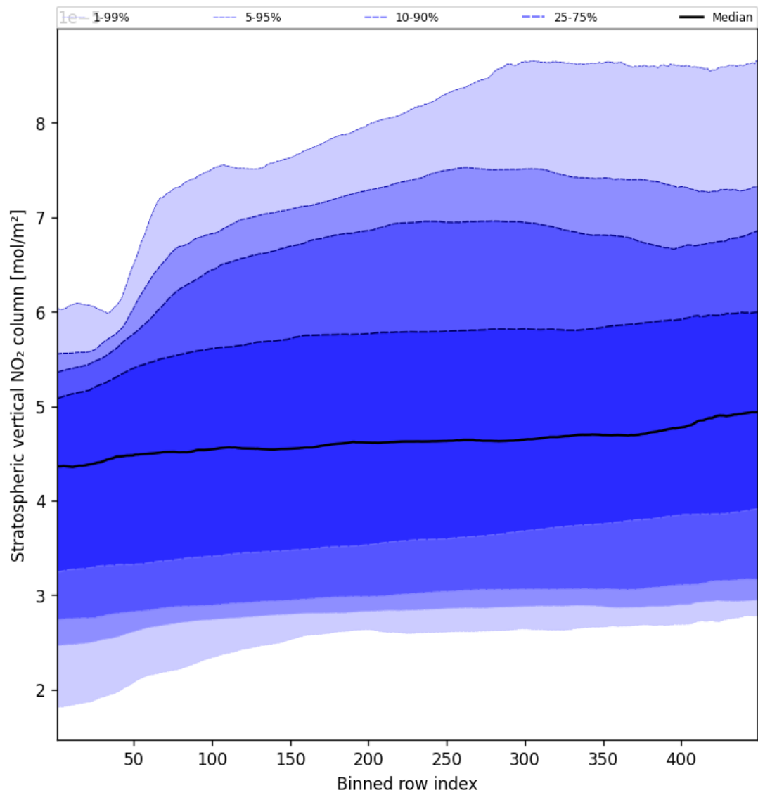
Figure 51: Along track statistics of “Stratospheric vertical NO 2 column” for 2025-04-25 to 2025-04-26
