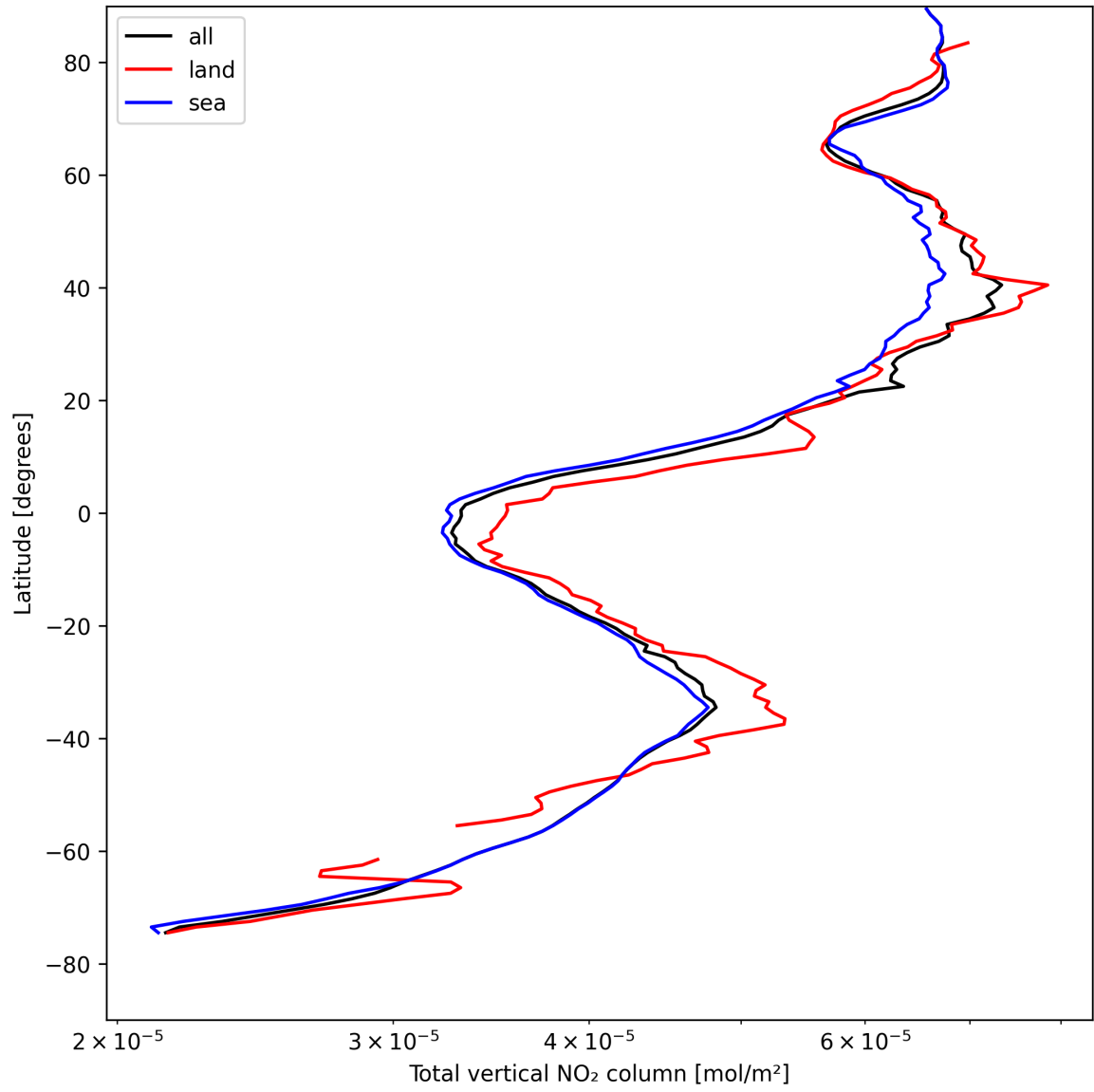
Figure 19: Zonal average of “Total vertical NO 2 column” for 2025-04-25 to 2025-04-26.
