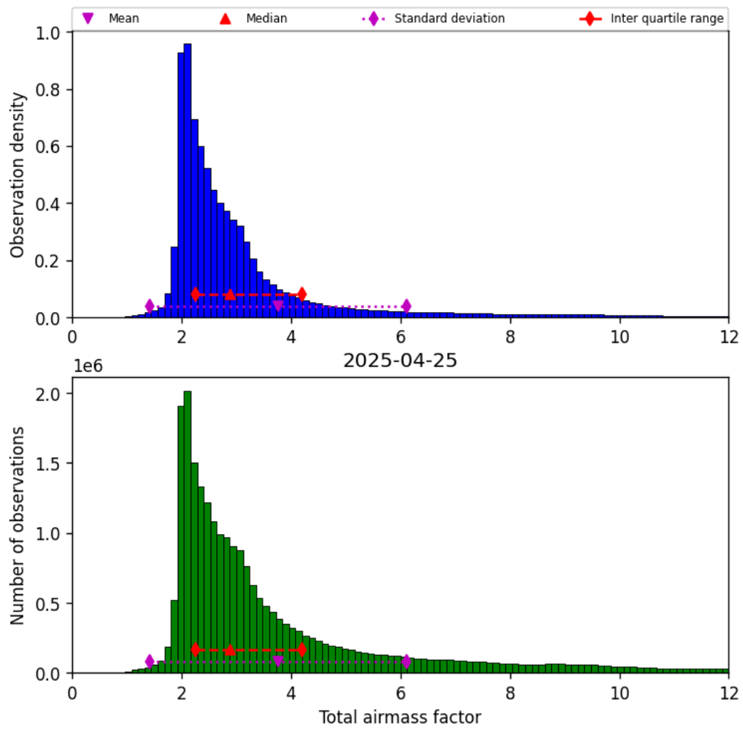
Figure 30: Histogram of “Total airmass factor” for 2025-04-25 to 2025-04-26
