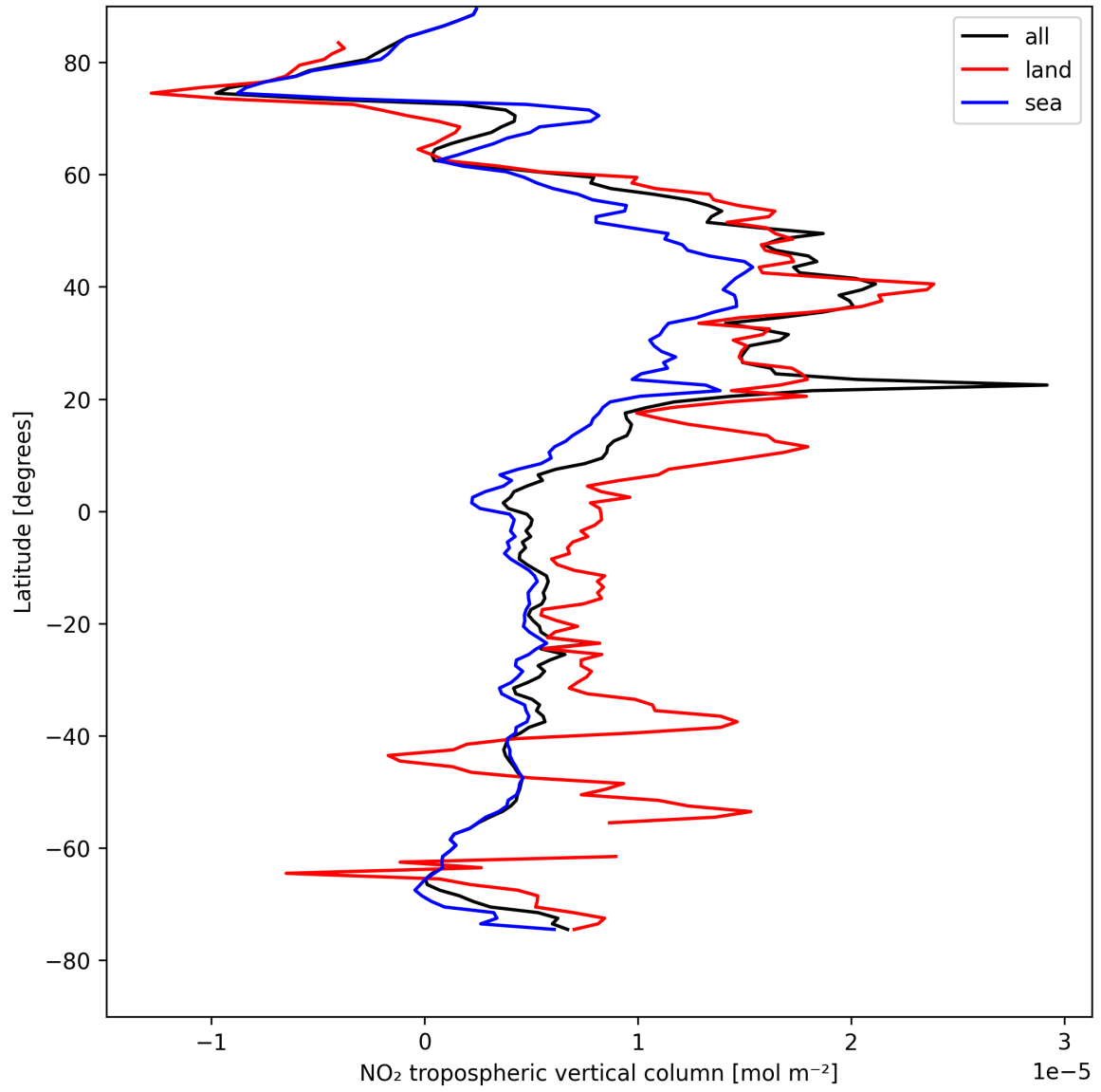
Figure 10: Zonal average of “NO 2 tropospheric vertical column” for 2025-04-25 to 2025-04-26.
