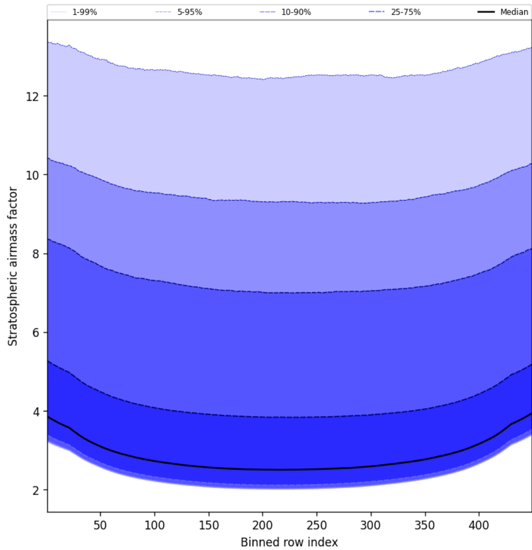
Figure 59: Along track statistics of “Stratospheric airmass factor” for 2025-04-25 to 2025-04-26
