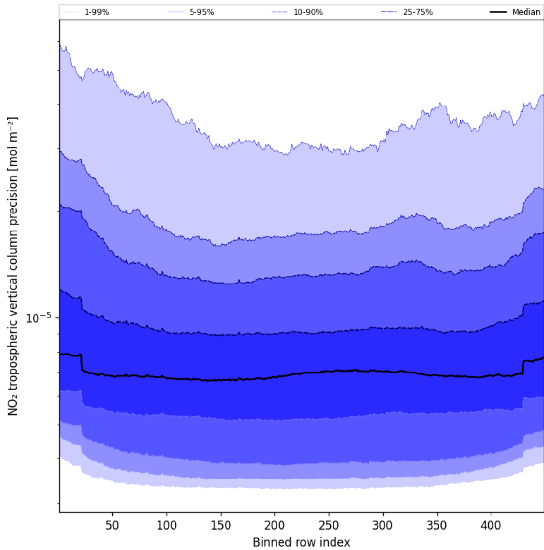
Figure 45: Along track statistics of “NO 2 tropospheric vertical column precision” for 2025-04-25 to 2025-04-26
