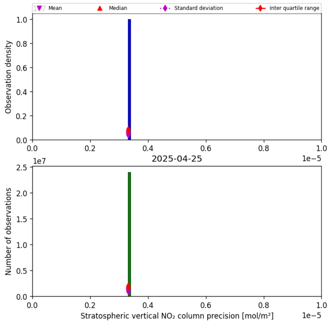
Figure 35: Histogram of “Stratospheric vertical NO 2 column precision” for 2025-04-25 to 2025-04-26
