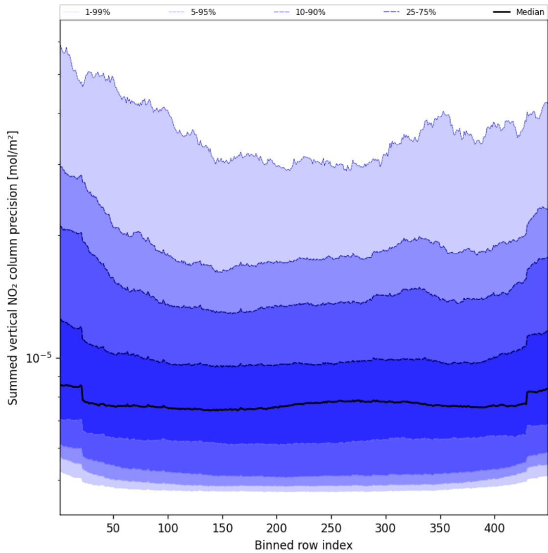
Figure 56: Along track statistics of “Summed vertical NO 2 column precision” for 2025-04-25 to 2025-04-26
