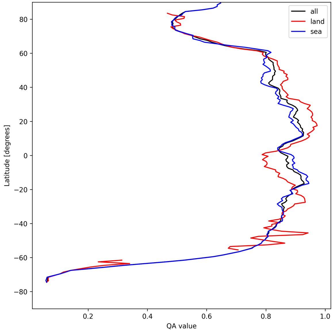
Figure 9: Zonal average of “QA value” for 2025-04-25 to 2025-04-26.
