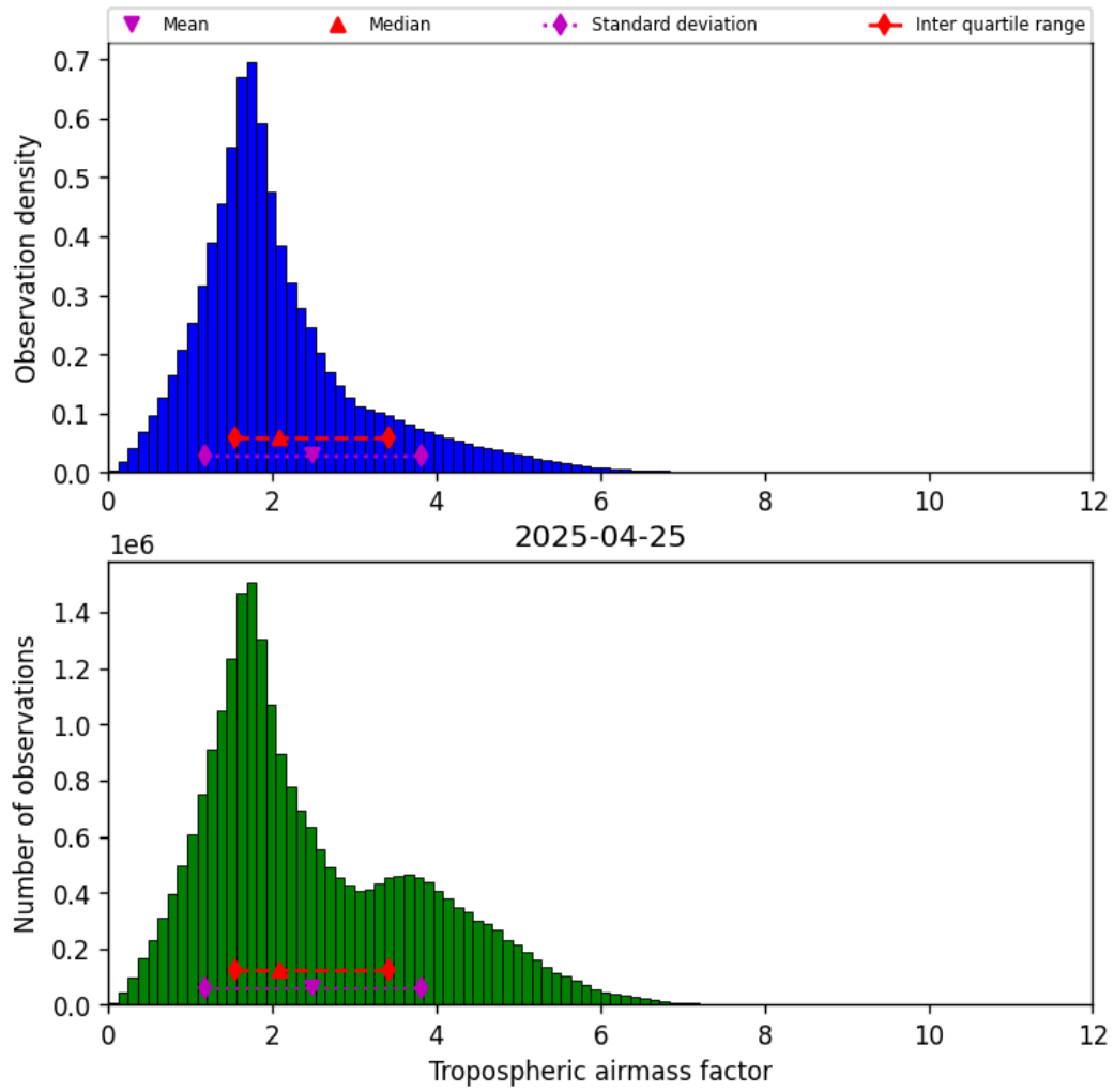
Figure 29: Histogram of “Tropospheric airmass factor” for 2025-04-25 to 2025-04-26
