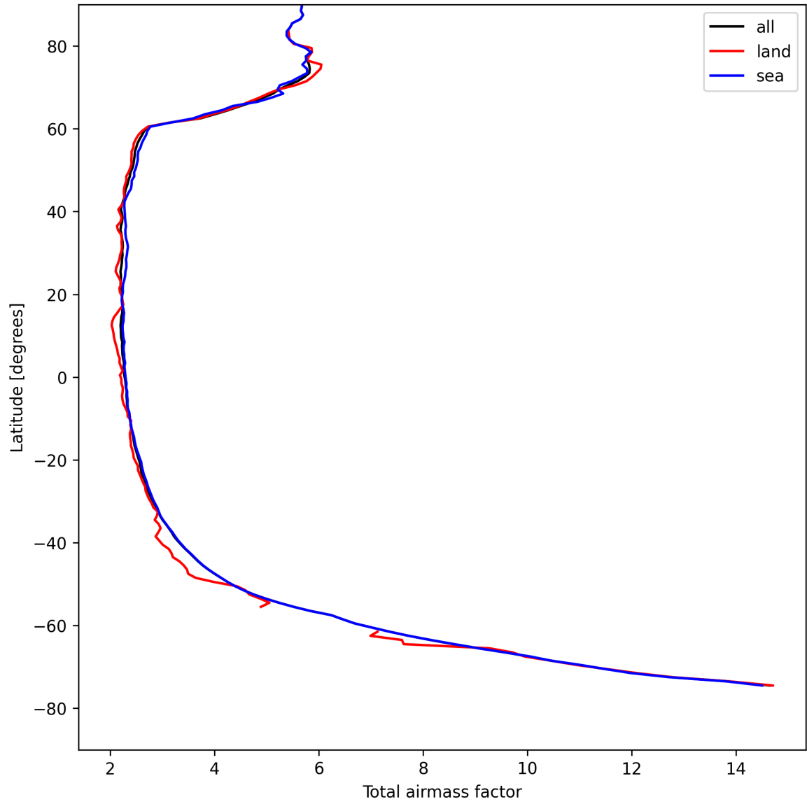
Figure 13: Zonal average of “Total airmass factor” for 2025-04-25 to 2025-04-26.
