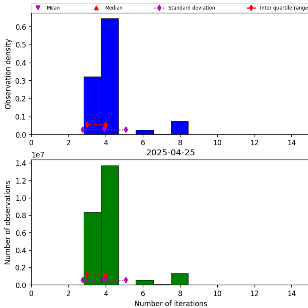
Figure 32: Histogram of “Number of iterations” for 2025-04-25 to 2025-04-26
