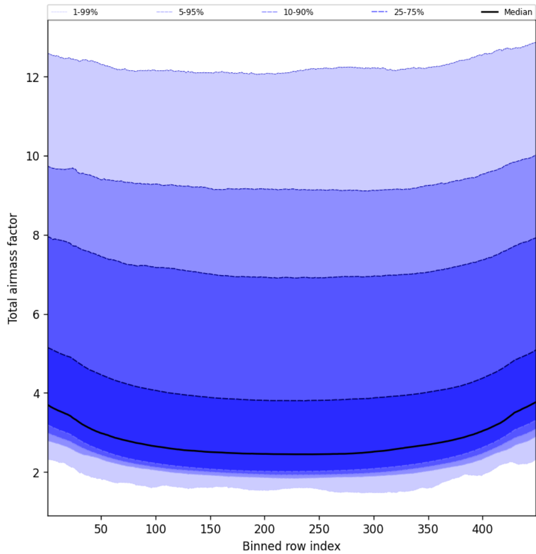
Figure 47: Along track statistics of “Total airmass factor” for 2025-04-25 to 2025-04-26
