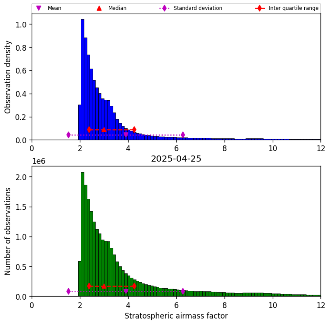
Figure 42: Histogram of “Stratospheric airmass factor” for 2025-04-25 to 2025-04-26
