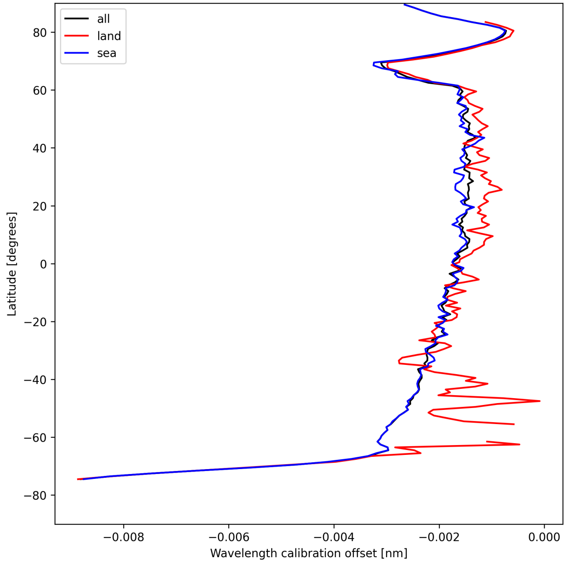
Figure 16: Zonal average of “Wavelength calibration offset” for 2025-04-25 to 2025-04-26.
