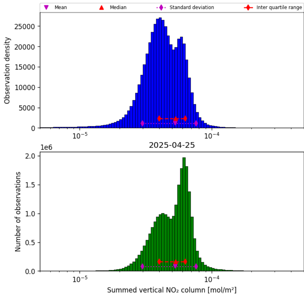
Figure 38: Histogram of “Summed vertical NO 2 column” for 2025-04-25 to 2025-04-26
