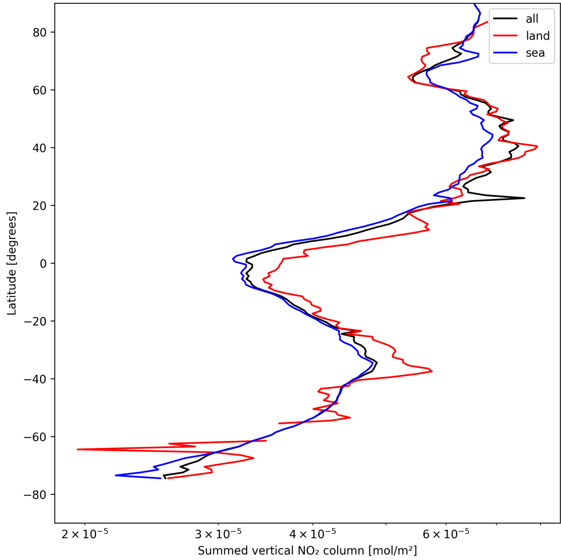
Figure 21: Zonal average of “Summed vertical NO 2 column” for 2025-04-25 to 2025-04-26.
