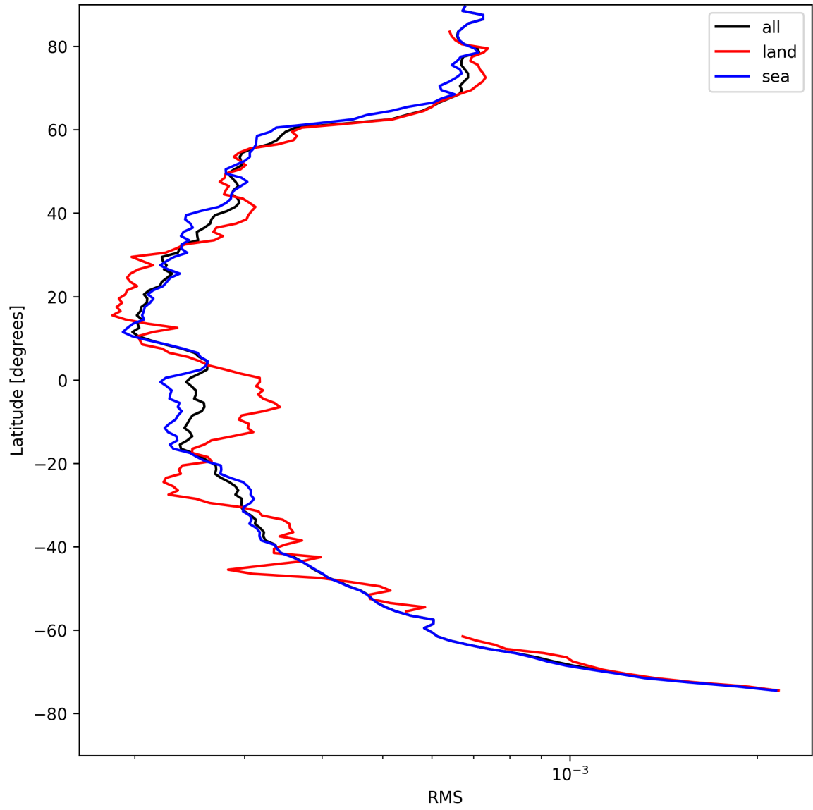
Figure 24: Zonal average of “RMS” for 2025-04-25 to 2025-04-26.
