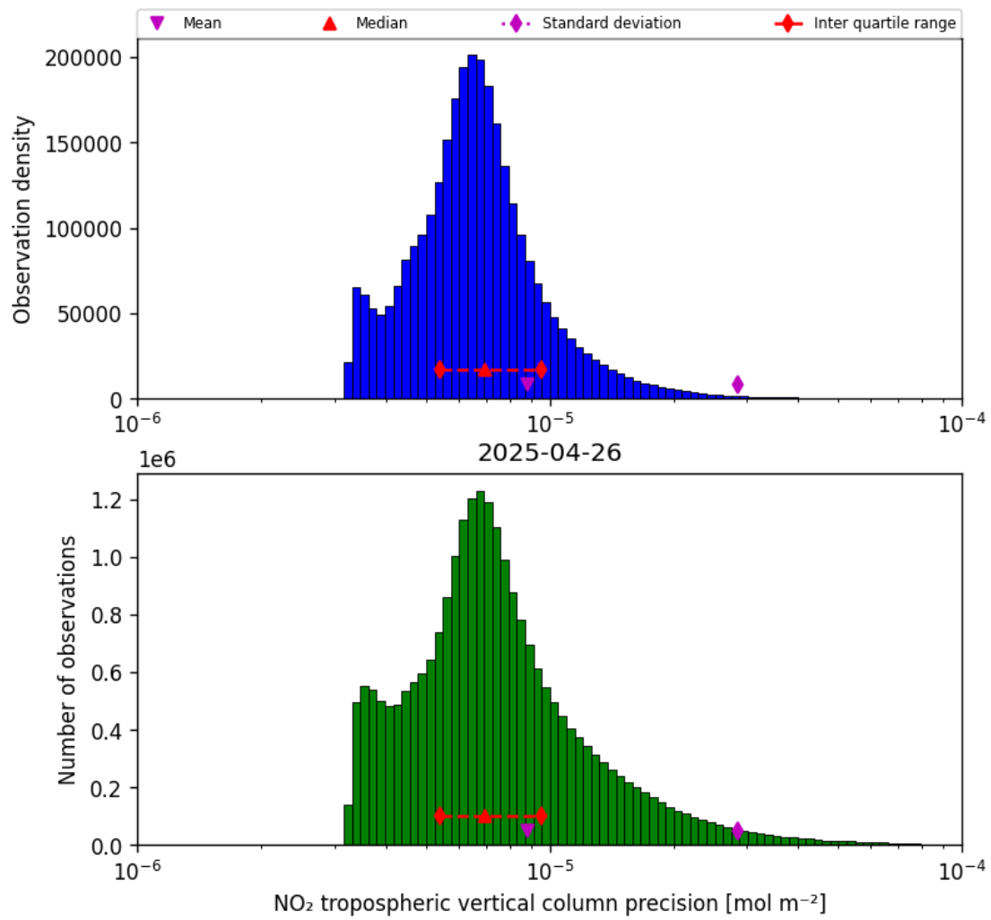
Figure 28: Histogram of “NO 2 tropospheric vertical column precision” for 2025-04-26 to 2025-04-27
