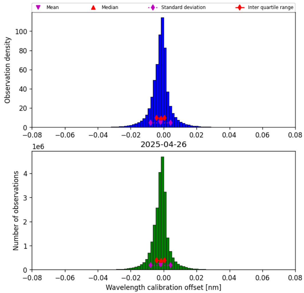
Figure 33: Histogram of “Wavelength calibration offset” for 2025-04-26 to 2025-04-27
