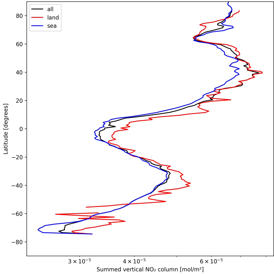
Figure 21: Zonal average of “Summed vertical NO 2 column” for 2025-04-26 to 2025-04-27.
