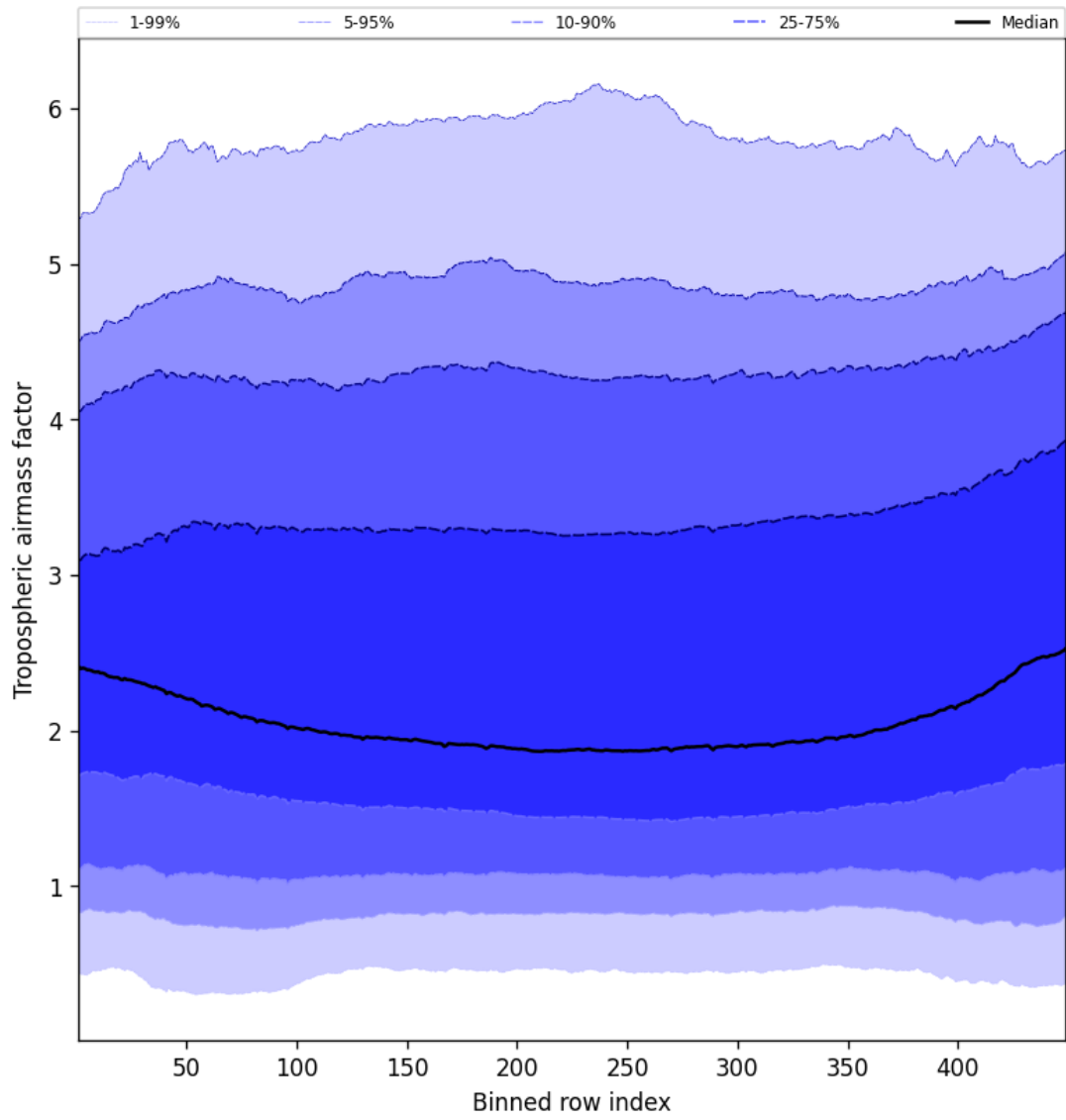
Figure 46: Along track statistics of “Tropospheric airmass factor” for 2025-04-26 to 2025-04-27
