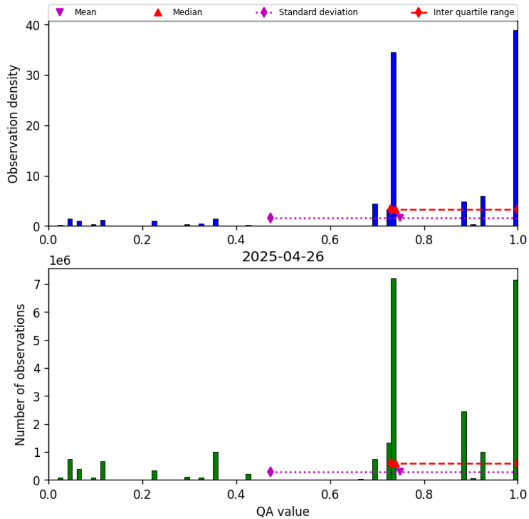
Figure 26: Histogram of “QA value” for 2025-04-26 to 2025-04-27
