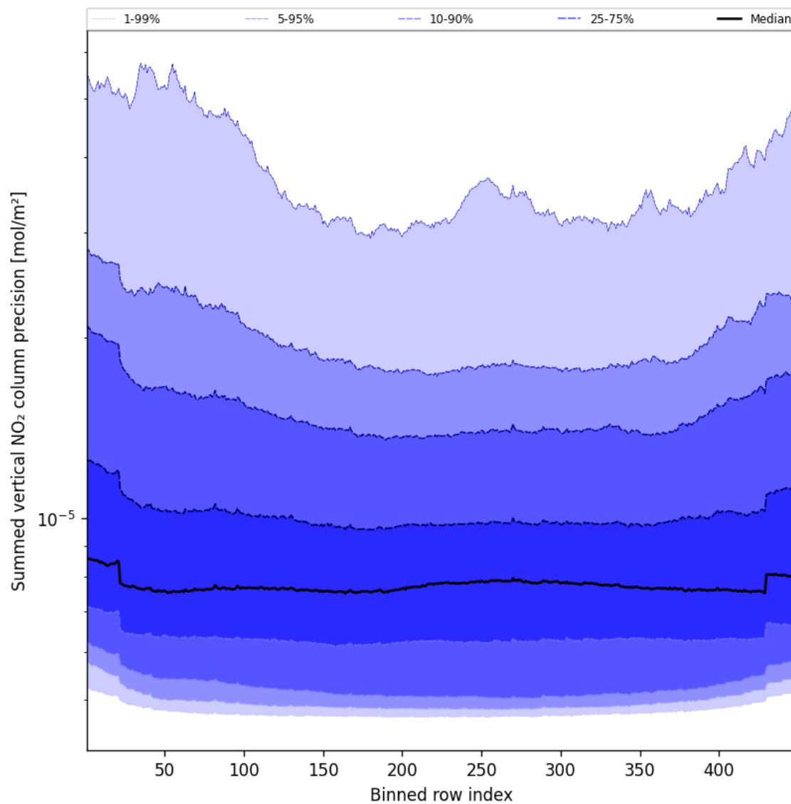
Figure 56: Along track statistics of “Summed vertical NO 2 column precision” for 2025-04-26 to 2025-04-27
