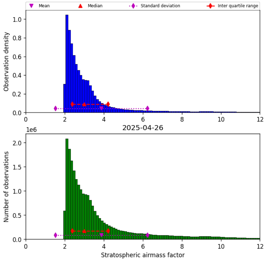
Figure 42: Histogram of “Stratospheric airmass factor” for 2025-04-26 to 2025-04-27
