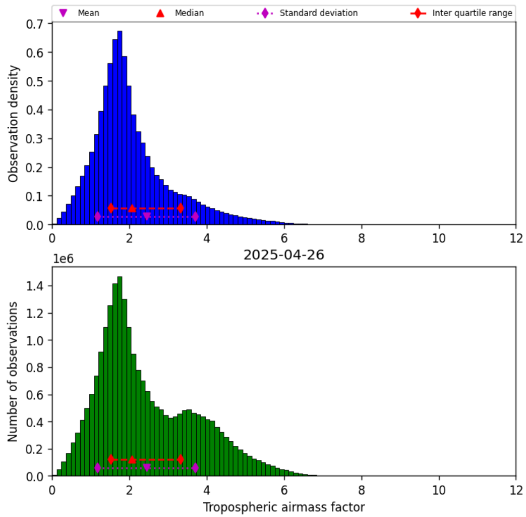
Figure 29: Histogram of “Tropospheric airmass factor” for 2025-04-26 to 2025-04-27
