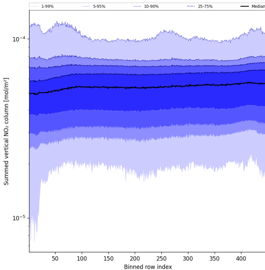
Figure 55: Along track statistics of “Summed vertical NO 2 column” for 2025-04-26 to 2025-04-27
