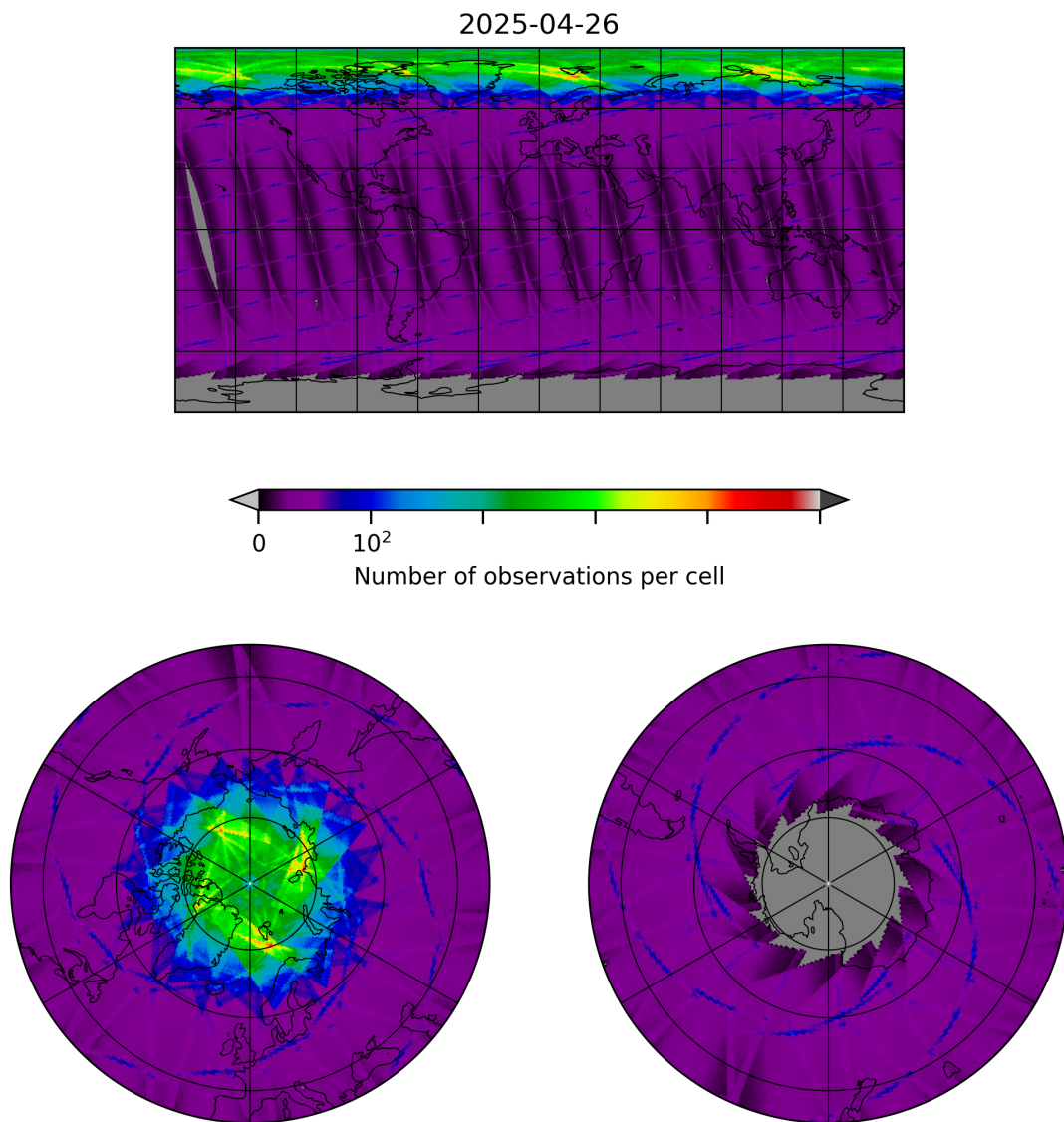
Figure 8: Map of the number of observations for 2025-04-26 to 2025-04-27
