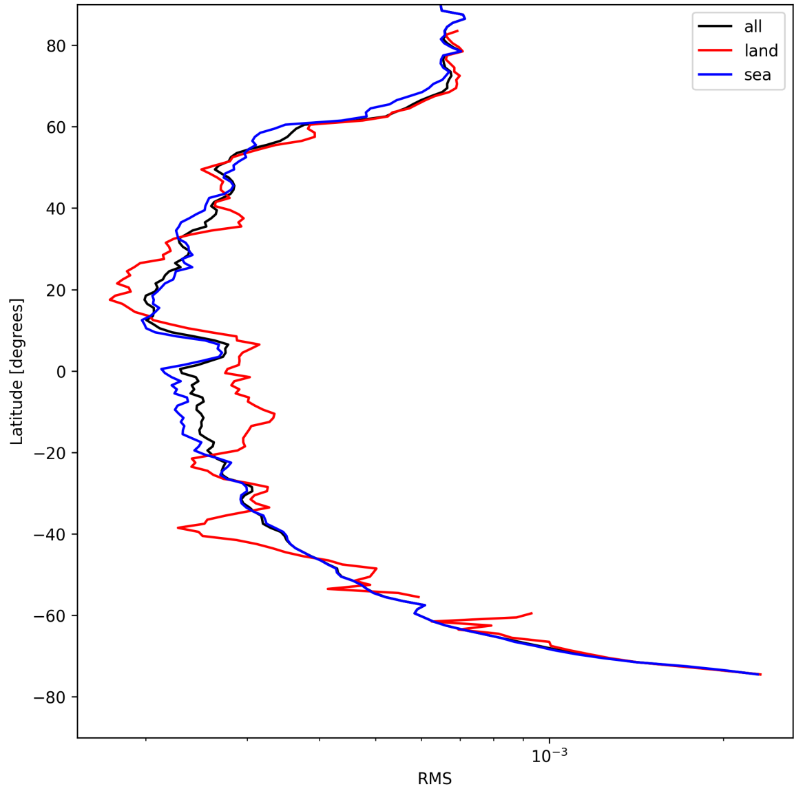
Figure 24: Zonal average of “RMS” for 2025-04-26 to 2025-04-27.
