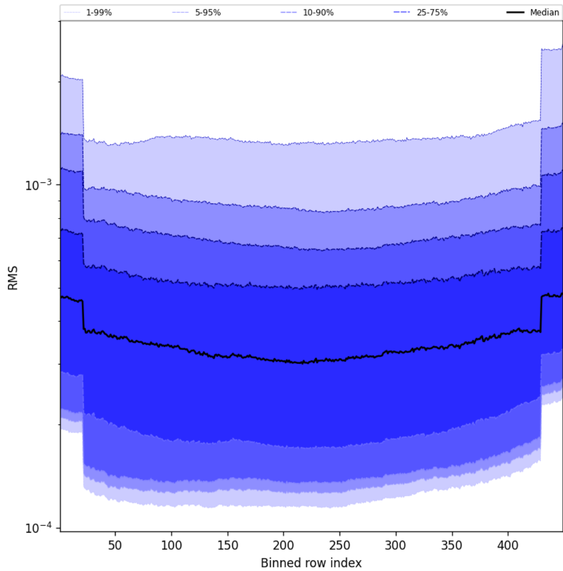
Figure 58: Along track statistics of “RMS” for 2025-04-26 to 2025-04-27
