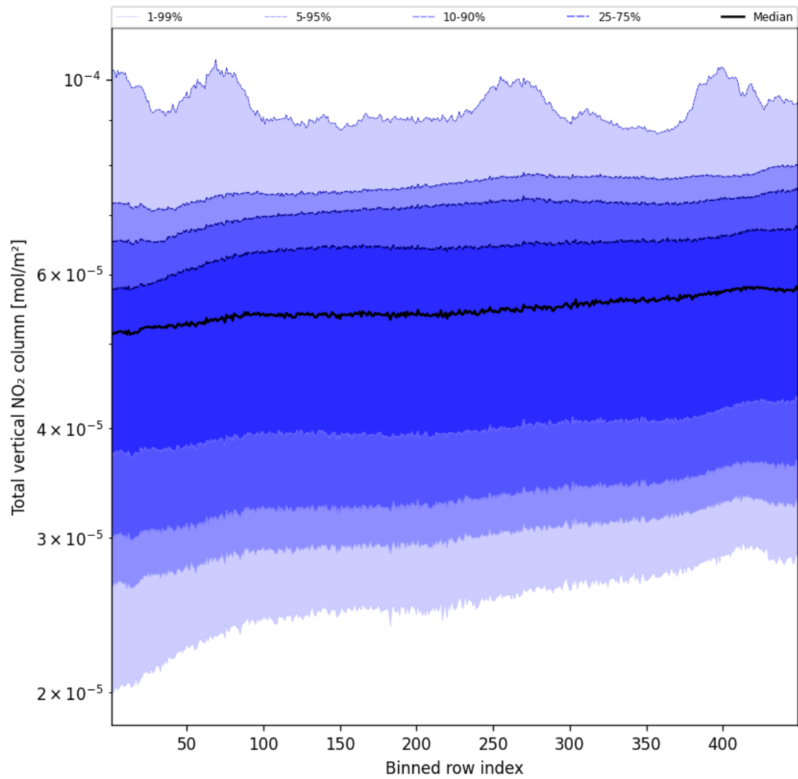
Figure 53: Along track statistics of “Total vertical NO 2 column” for 2025-04-26 to 2025-04-27
