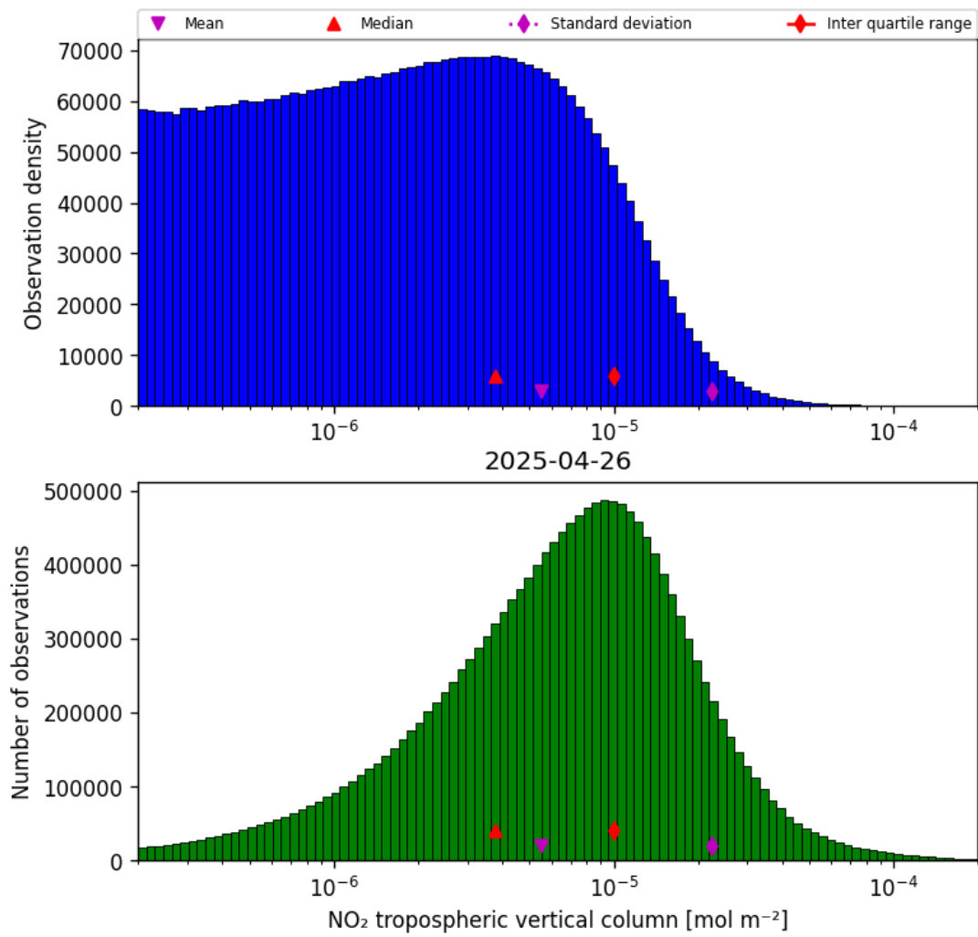
Figure 27: Histogram of “NO 2 tropospheric vertical column” for 2025-04-26 to 2025-04-27
