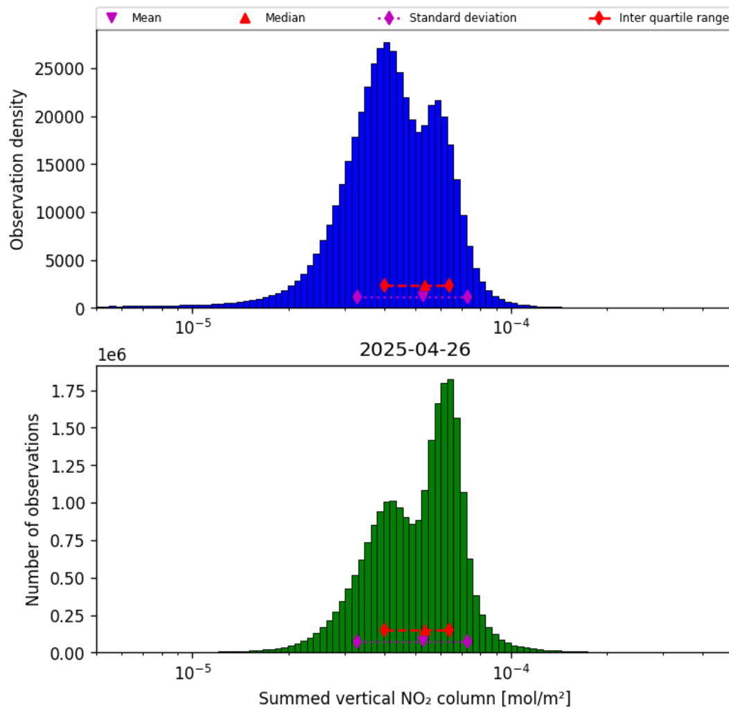
Figure 38: Histogram of “Summed vertical NO 2 column” for 2025-04-26 to 2025-04-27
