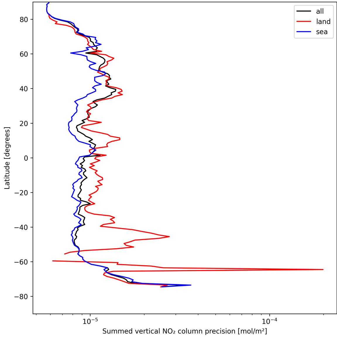
Figure 22: Zonal average of “Summed vertical NO 2 column precision” for 2025-04-26 to 2025-04-27.
