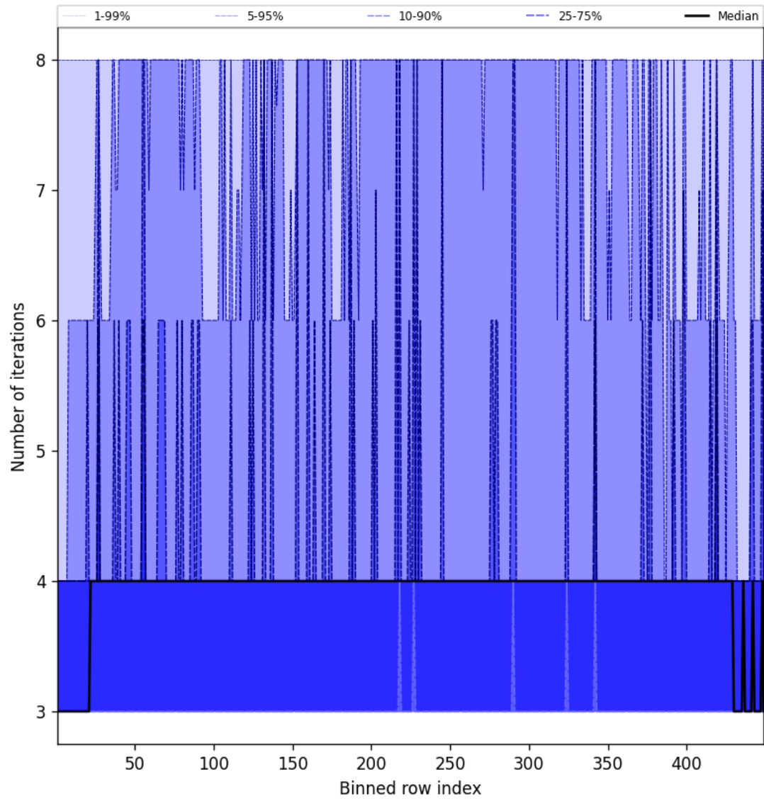
Figure 49: Along track statistics of “Number of iterations” for 2025-04-26 to 2025-04-27
