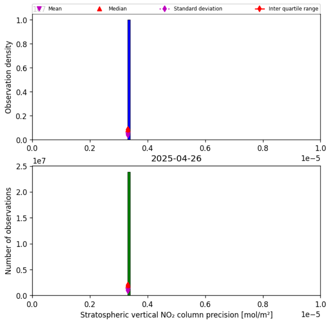
Figure 35: Histogram of “Stratospheric vertical NO 2 column precision” for 2025-04-26 to 2025-04-27
