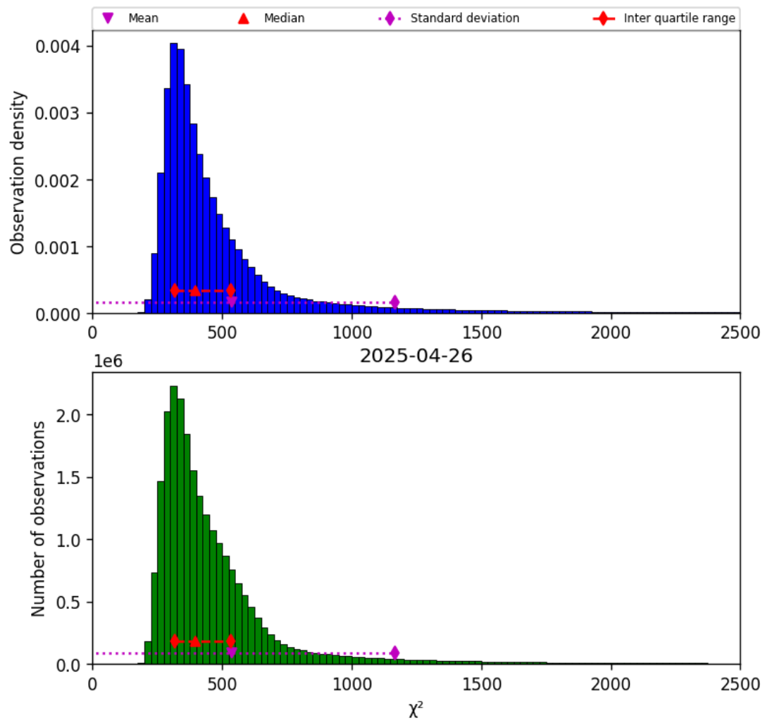
Figure 40: Histogram of “ \chi^2 ” for 2025-04-26 to 2025-04-27
