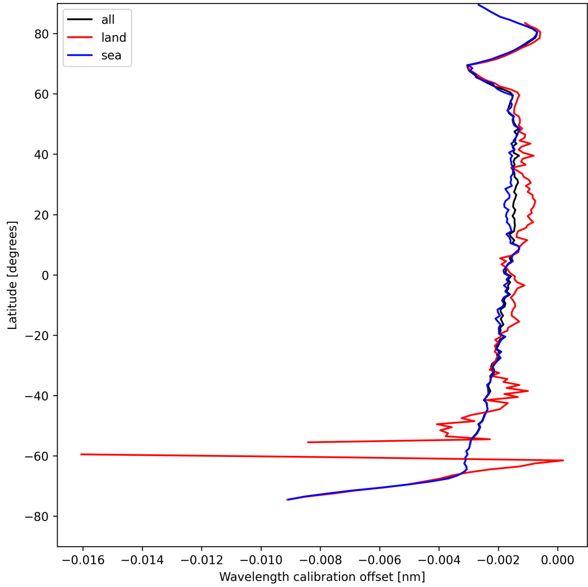
Figure 16: Zonal average of “Wavelength calibration offset” for 2025-04-26 to 2025-04-27.
