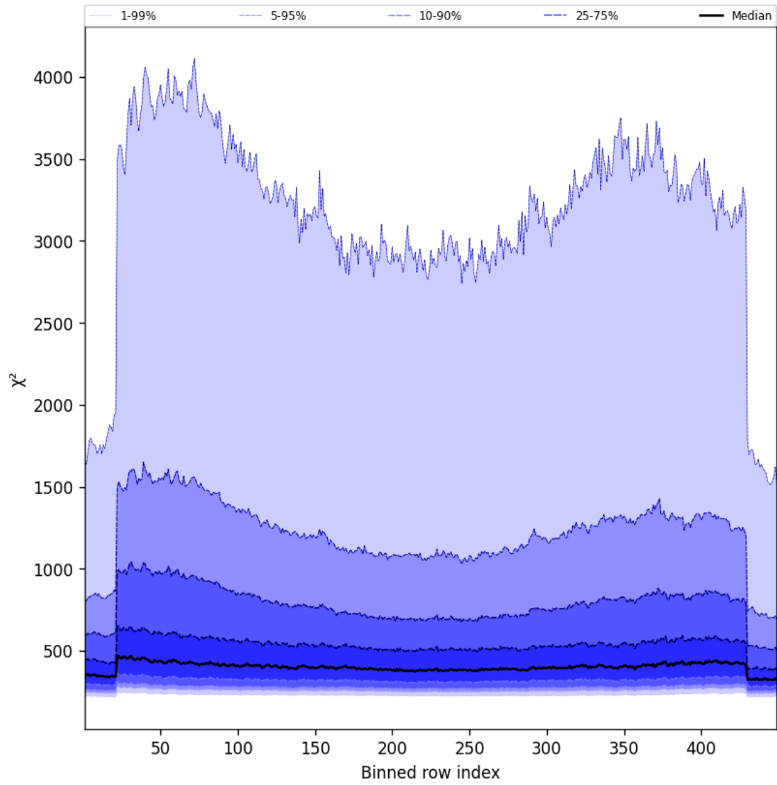
Figure 57: Along track statistics of “ \chi^2 ” for 2025-04-26 to 2025-04-27
