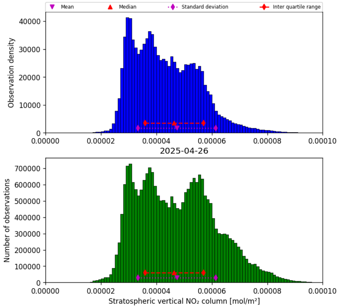
Figure 34: Histogram of “Stratospheric vertical NO 2 column” for 2025-04-26 to 2025-04-27
