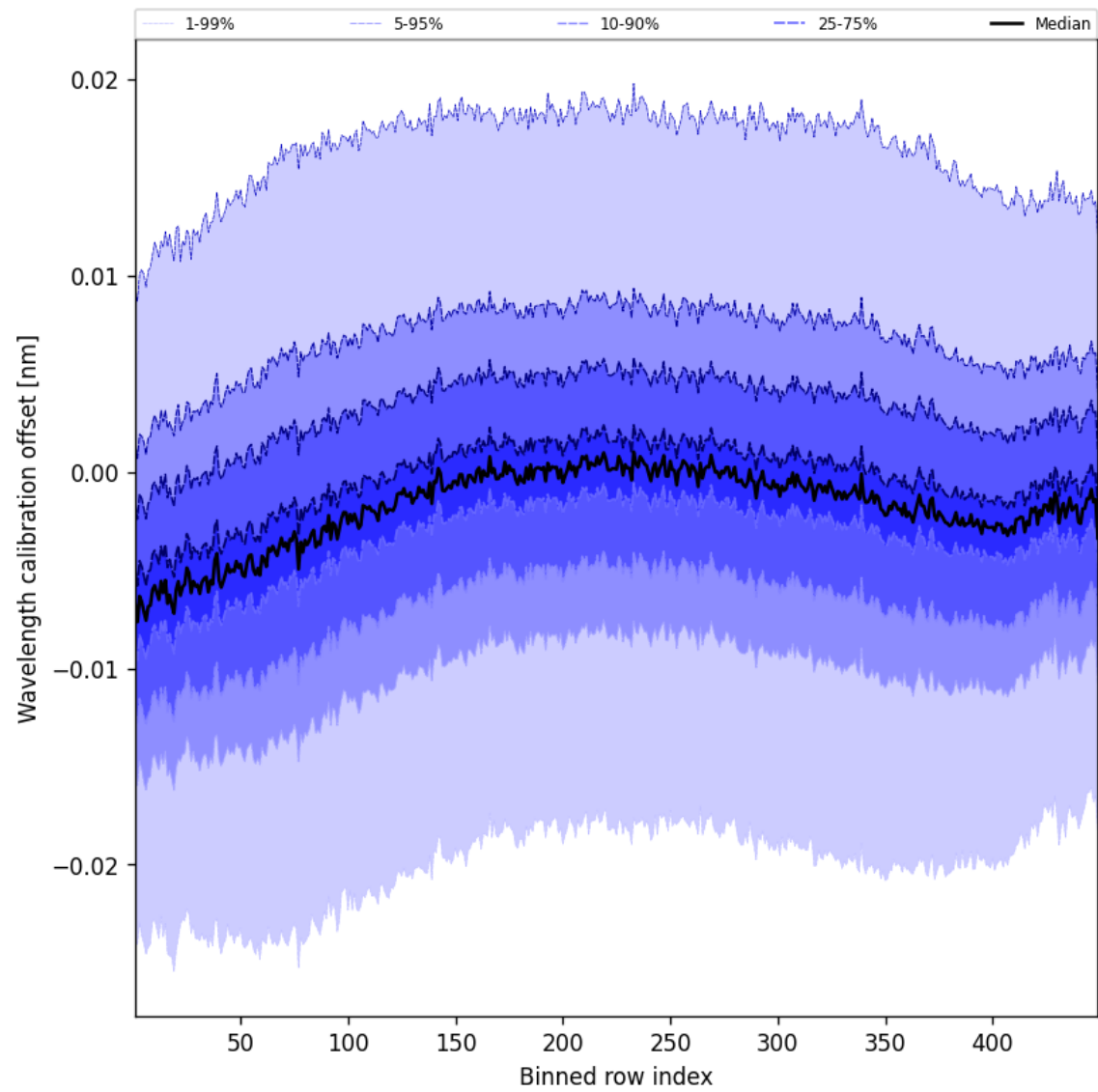
Figure 50: Along track statistics of “Wavelength calibration offset” for 2025-04-26 to 2025-04-27
