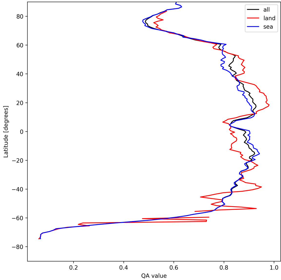
Figure 9: Zonal average of “QA value” for 2025-04-26 to 2025-04-27.
