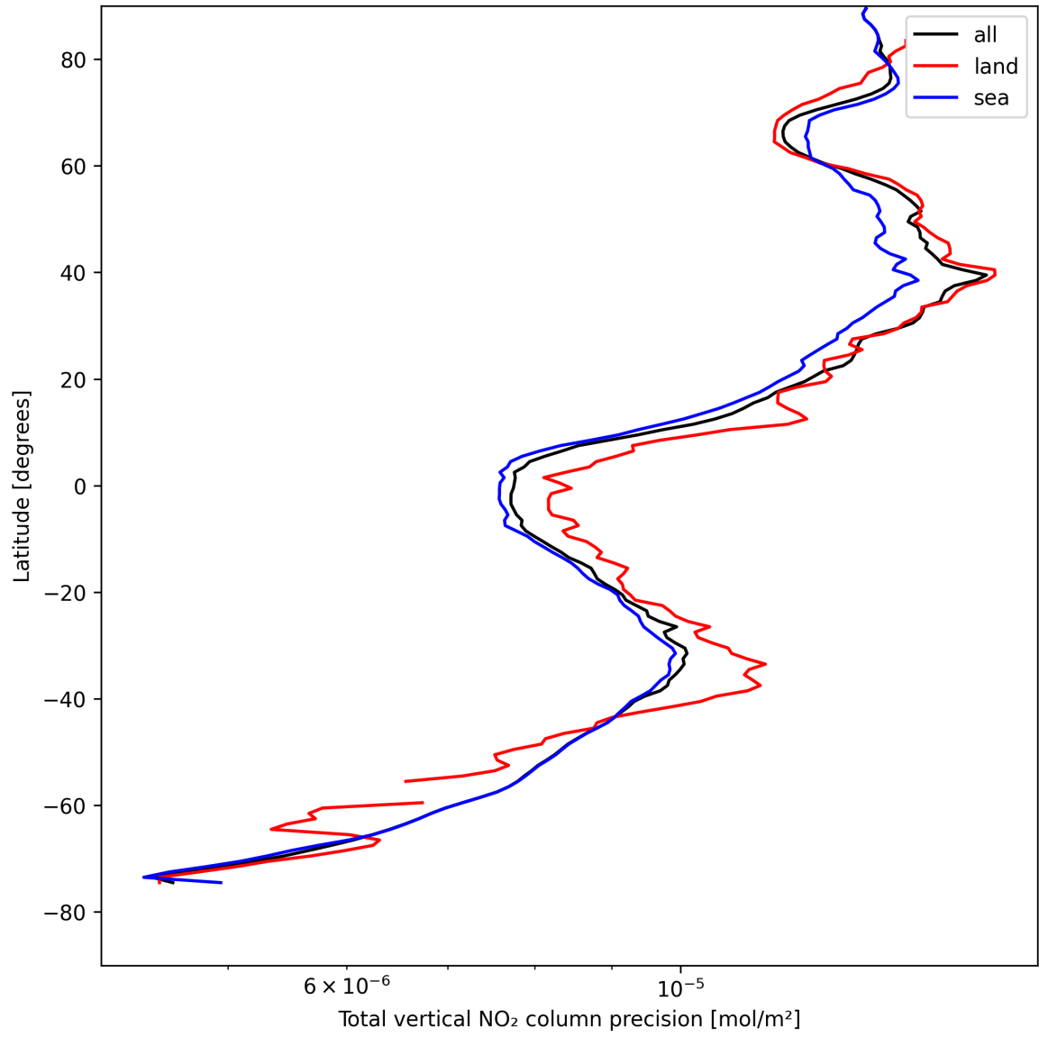
Figure 20: Zonal average of “Total vertical NO 2 column precision” for 2025-04-26 to 2025-04-27.
