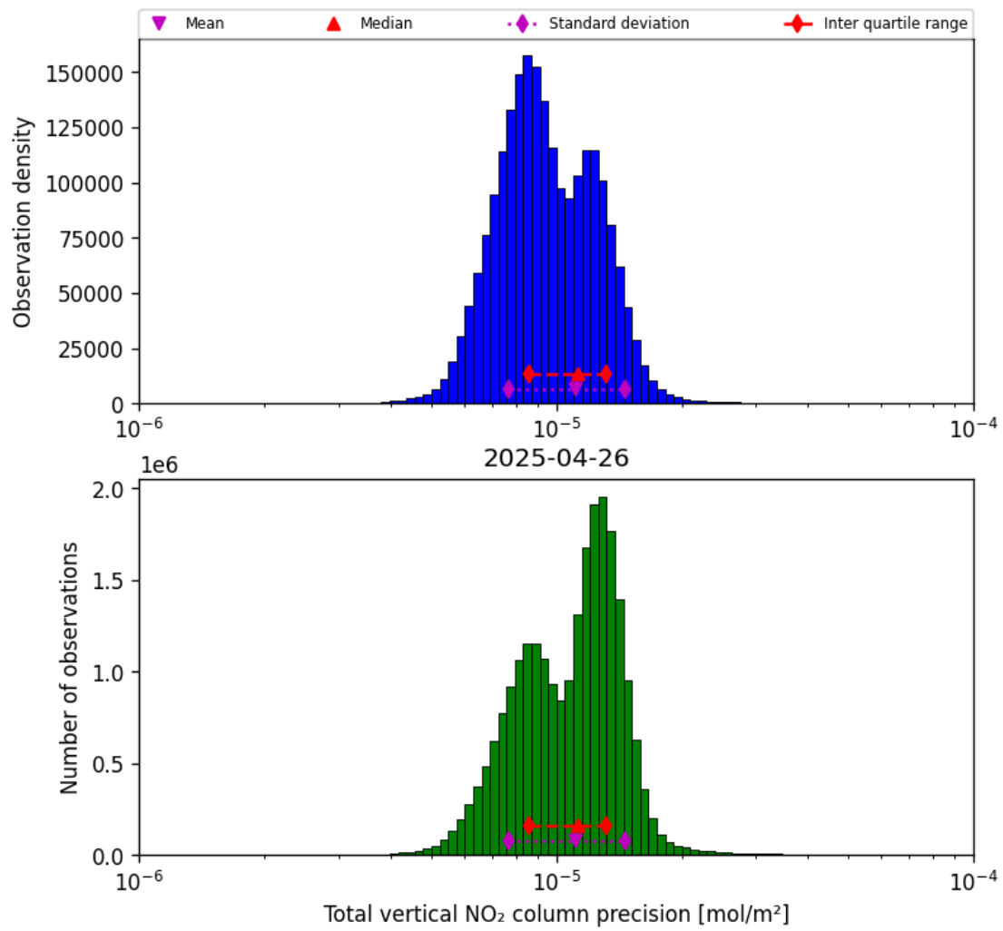
Figure 37: Histogram of “Total vertical NO 2 column precision” for 2025-04-26 to 2025-04-27
