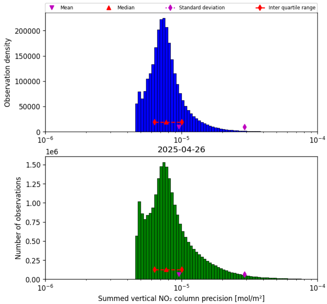
Figure 39: Histogram of “Summed vertical NO 2 column precision” for 2025-04-26 to 2025-04-27
