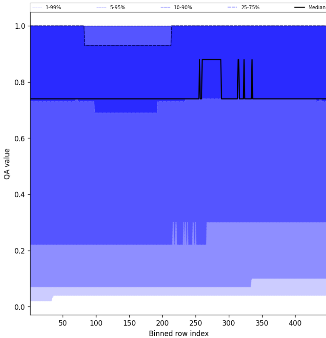
Figure 43: Along track statistics of “QA value” for 2025-04-26 to 2025-04-27
