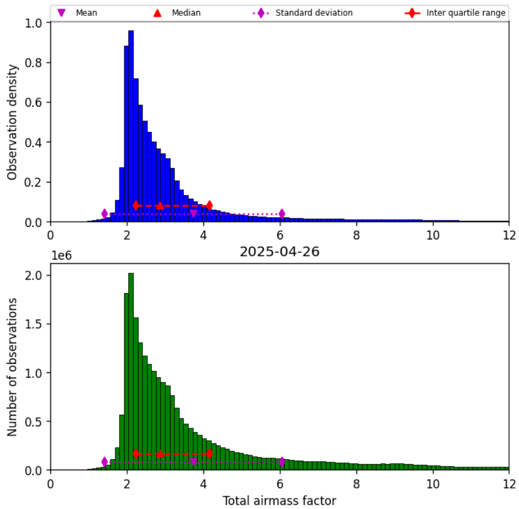
Figure 30: Histogram of “Total airmass factor” for 2025-04-26 to 2025-04-27
