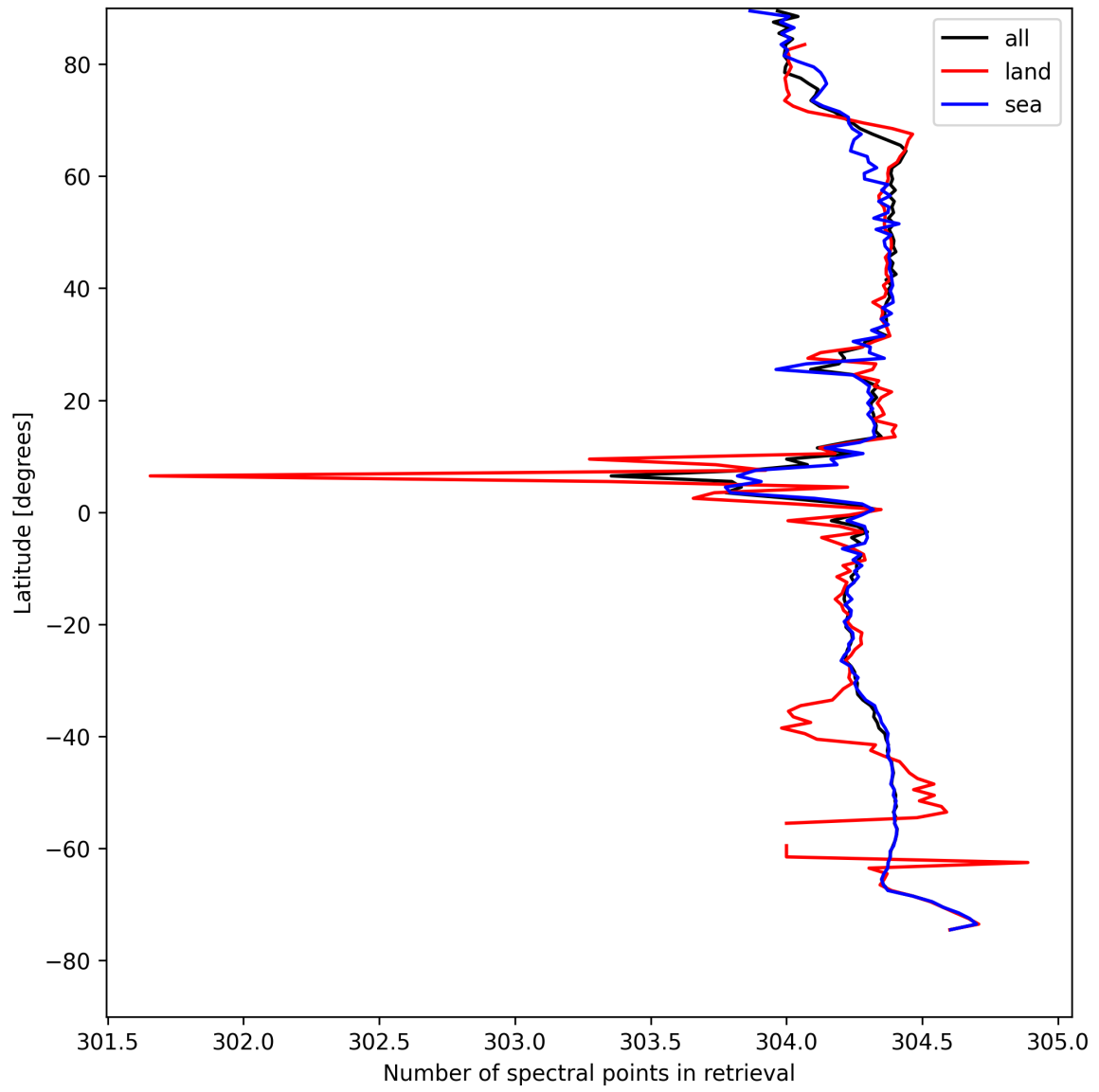
Figure 14: Zonal average of “Number of spectral points in retrieval” for 2025-04-26 to 2025-04-27.
