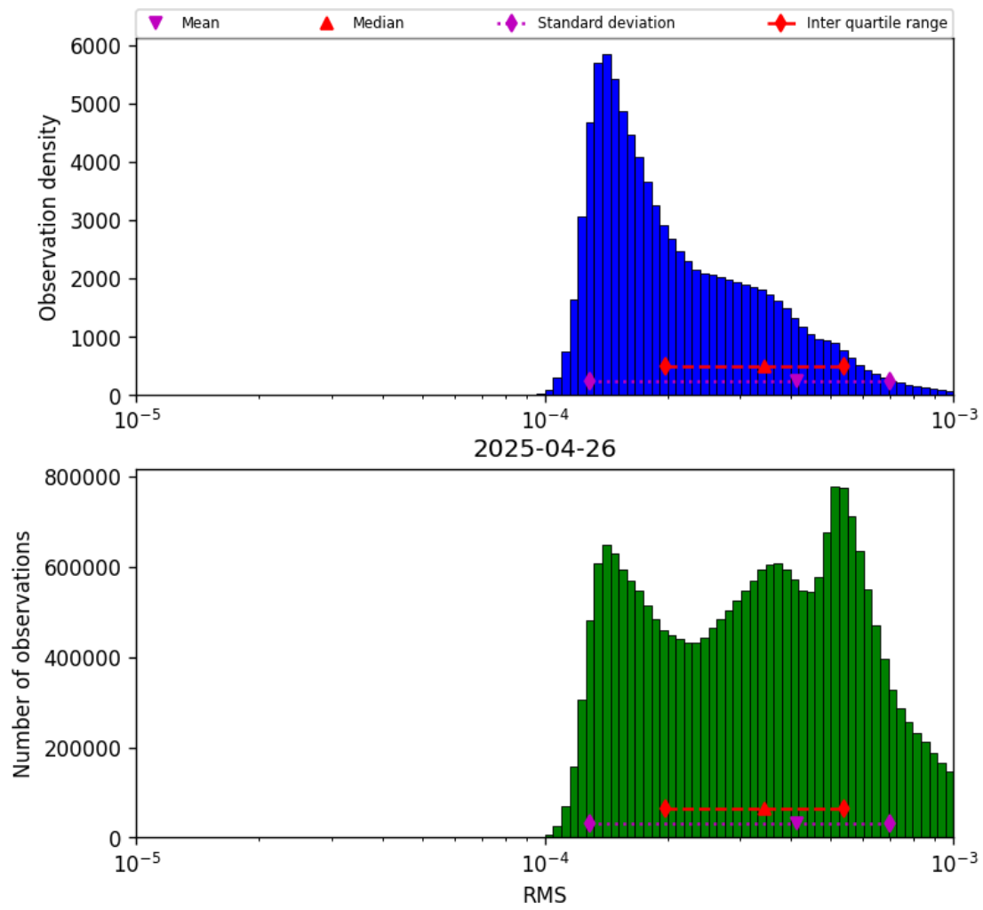
Figure 41: Histogram of “RMS” for 2025-04-26 to 2025-04-27
