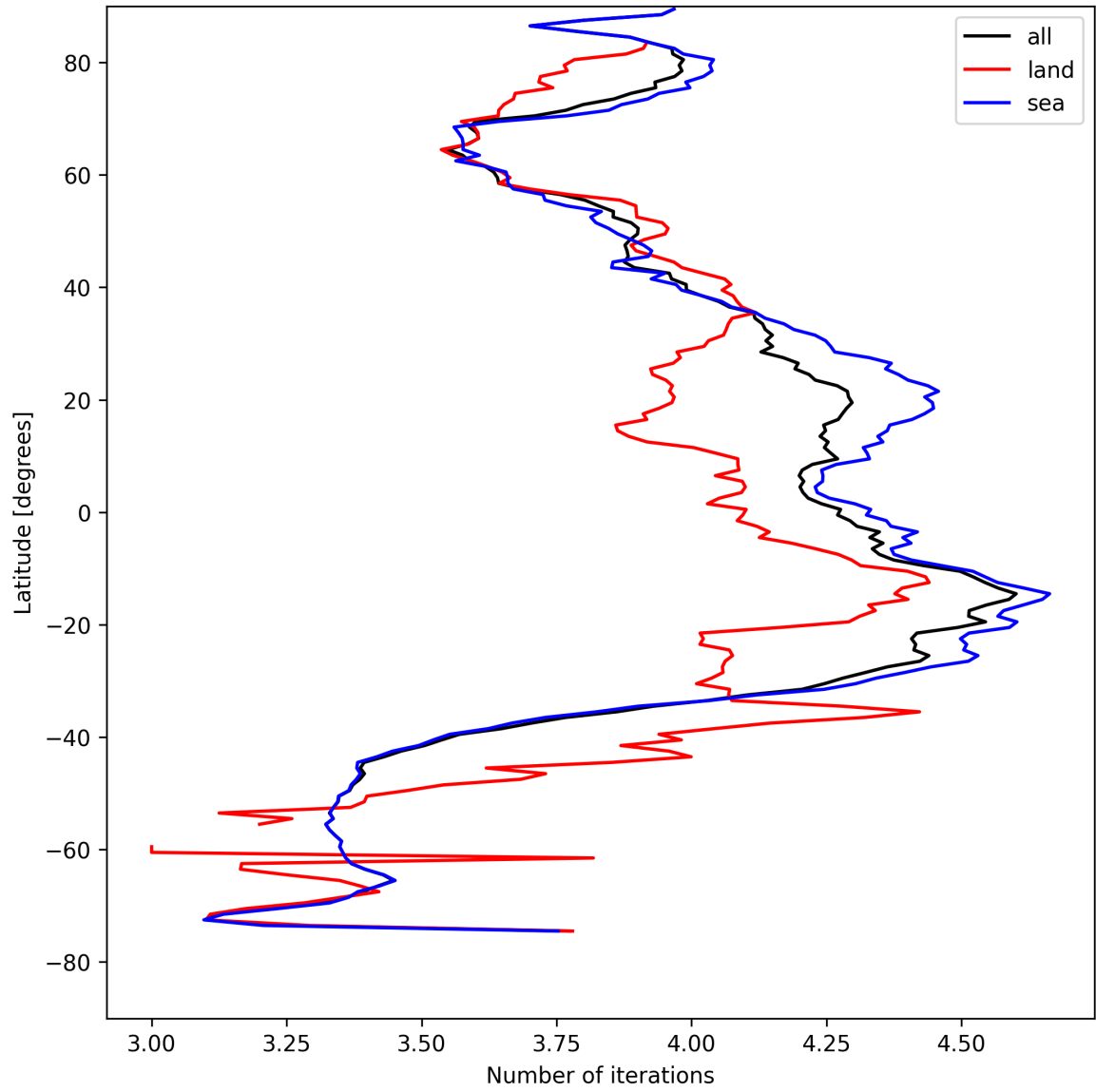
Figure 15: Zonal average of “Number of iterations” for 2025-04-26 to 2025-04-27.
