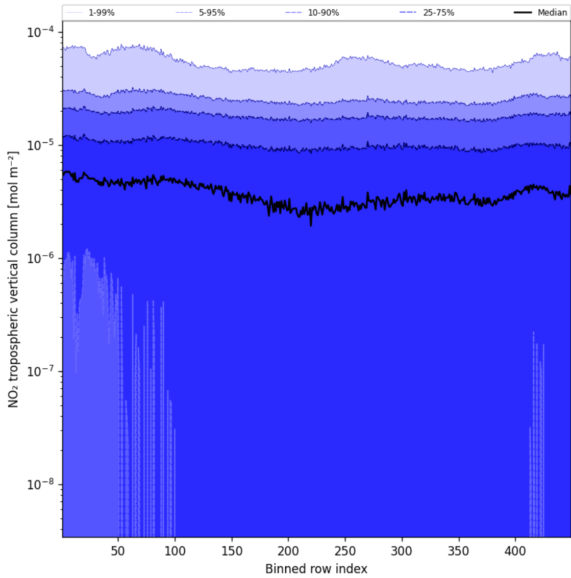
Figure 44: Along track statistics of “NO 2 tropospheric vertical column” for 2025-04-26 to 2025-04-27
