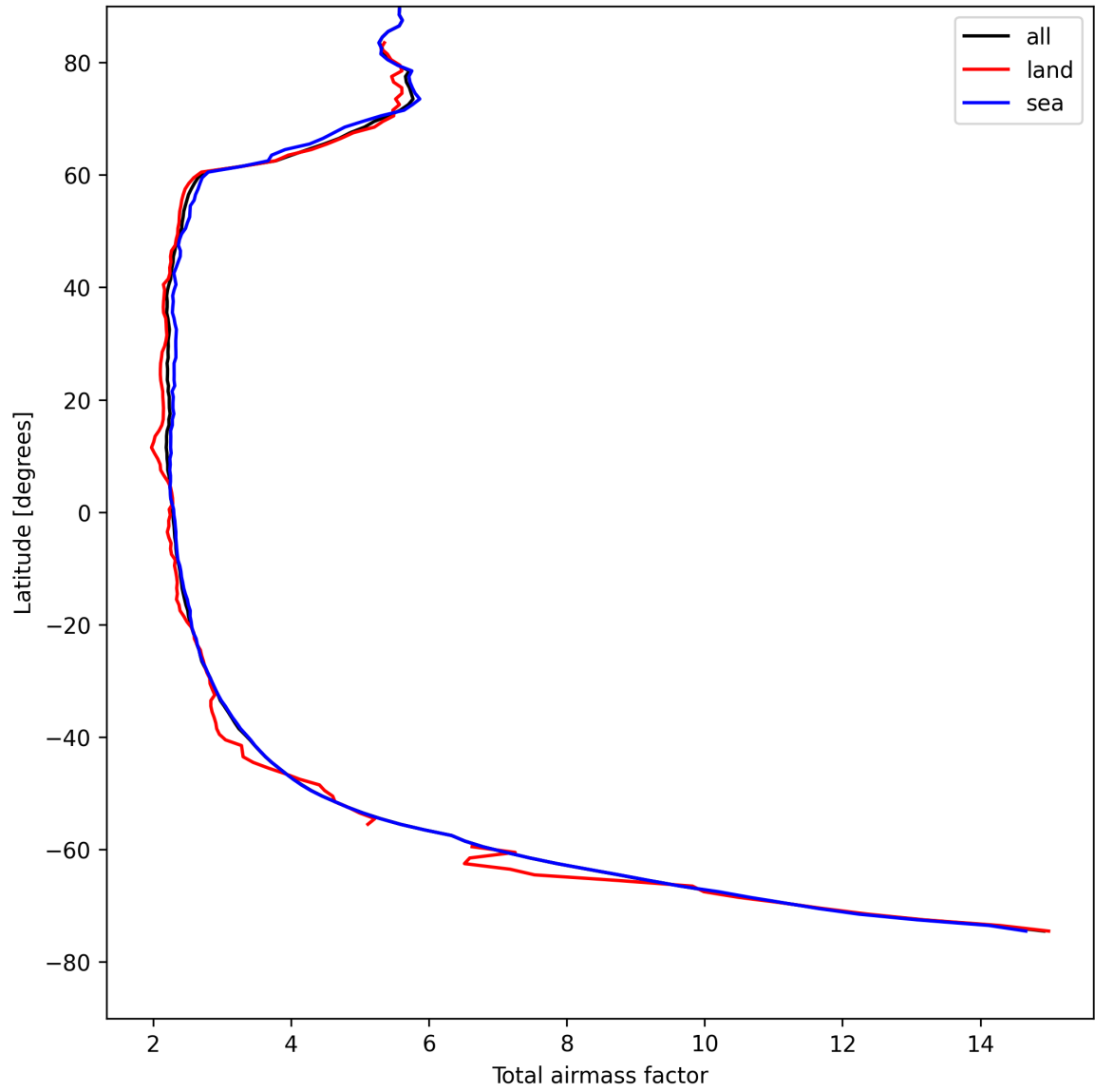
Figure 13: Zonal average of “Total airmass factor” for 2025-04-26 to 2025-04-27.
