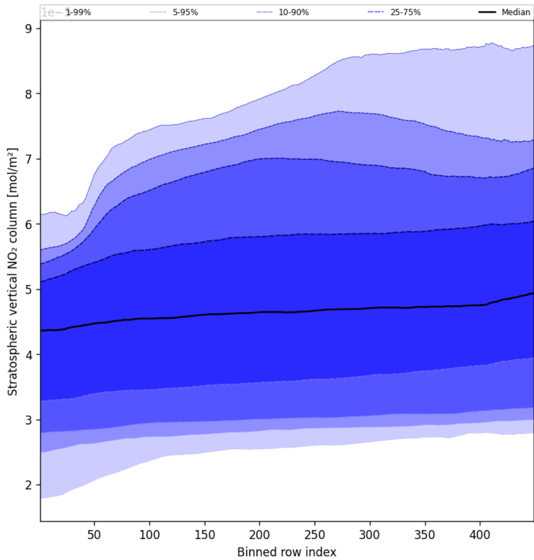
Figure 51: Along track statistics of “Stratospheric vertical NO 2 column” for 2025-04-26 to 2025-04-27
