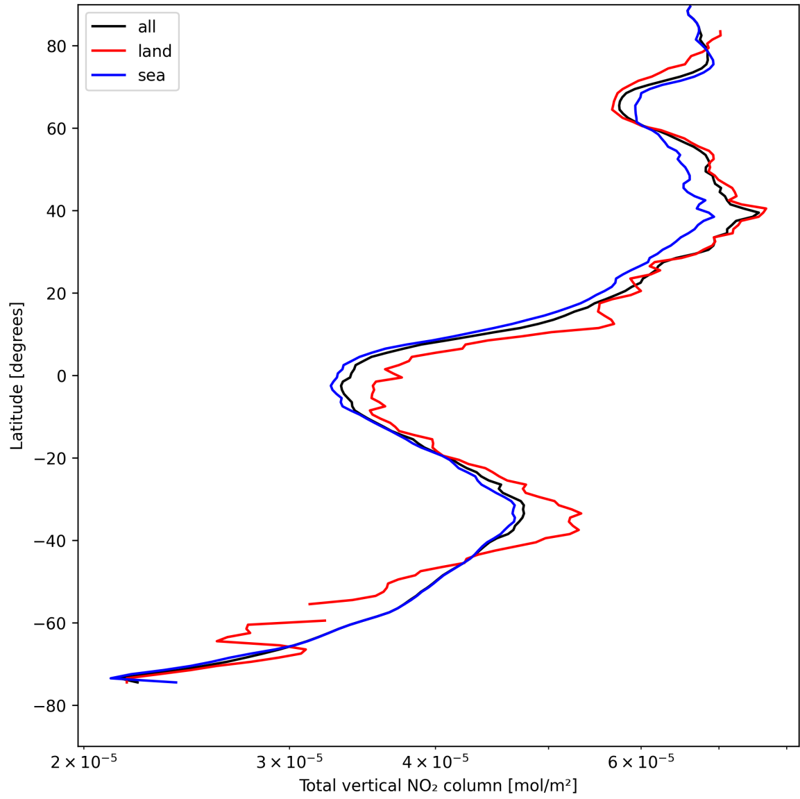
Figure 19: Zonal average of “Total vertical NO 2 column” for 2025-04-26 to 2025-04-27.
