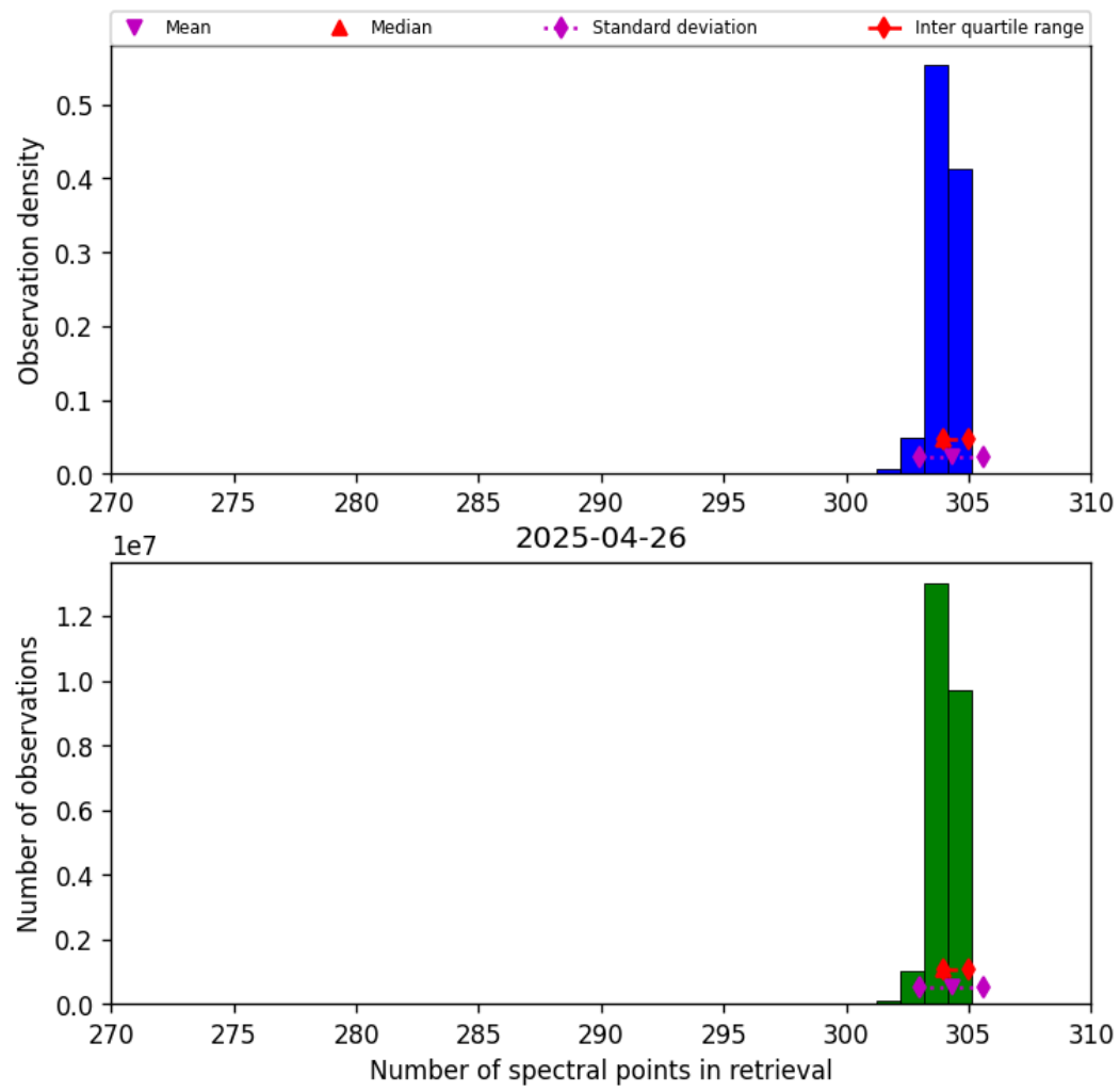
Figure 31: Histogram of “Number of spectral points in retrieval” for 2025-04-26 to 2025-04-27
