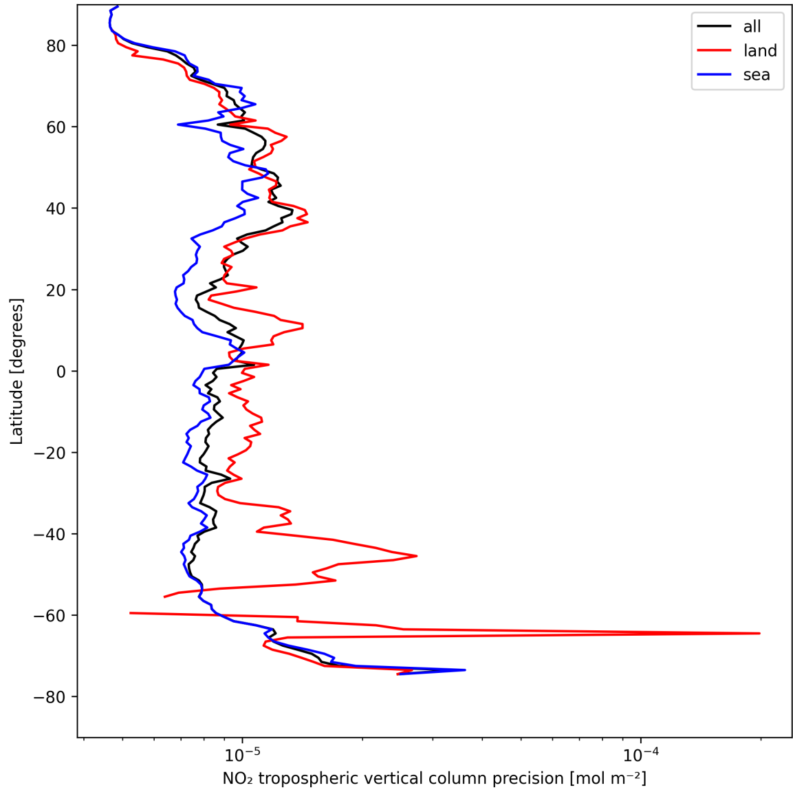
Figure 11: Zonal average of “NO 2 tropospheric vertical column precision” for 2025-04-26 to 2025-04-27.
