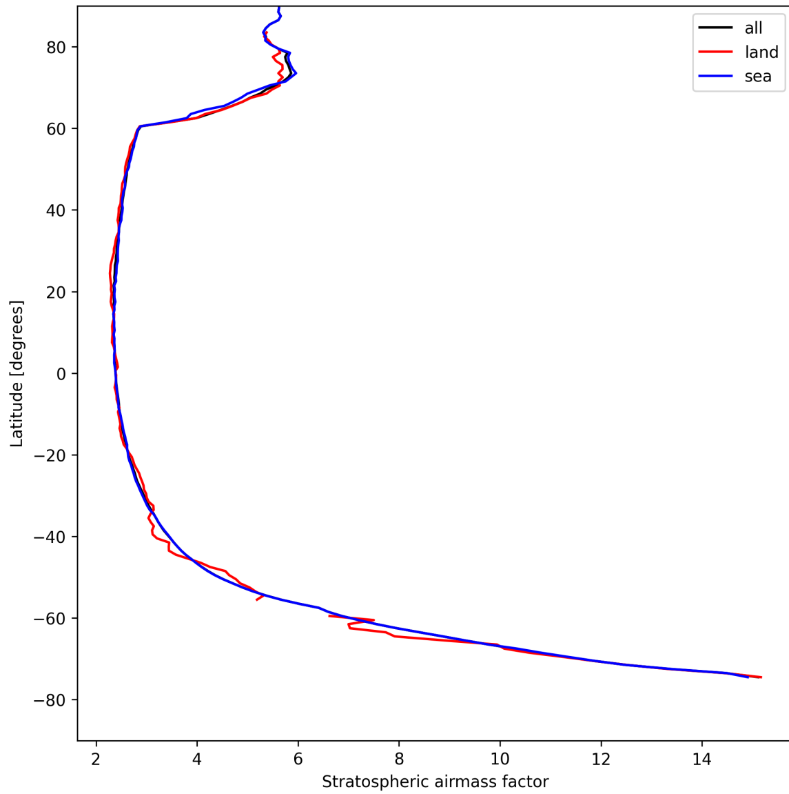
Figure 25: Zonal average of “Stratospheric airmass factor” for 2025-04-26 to 2025-04-27.
