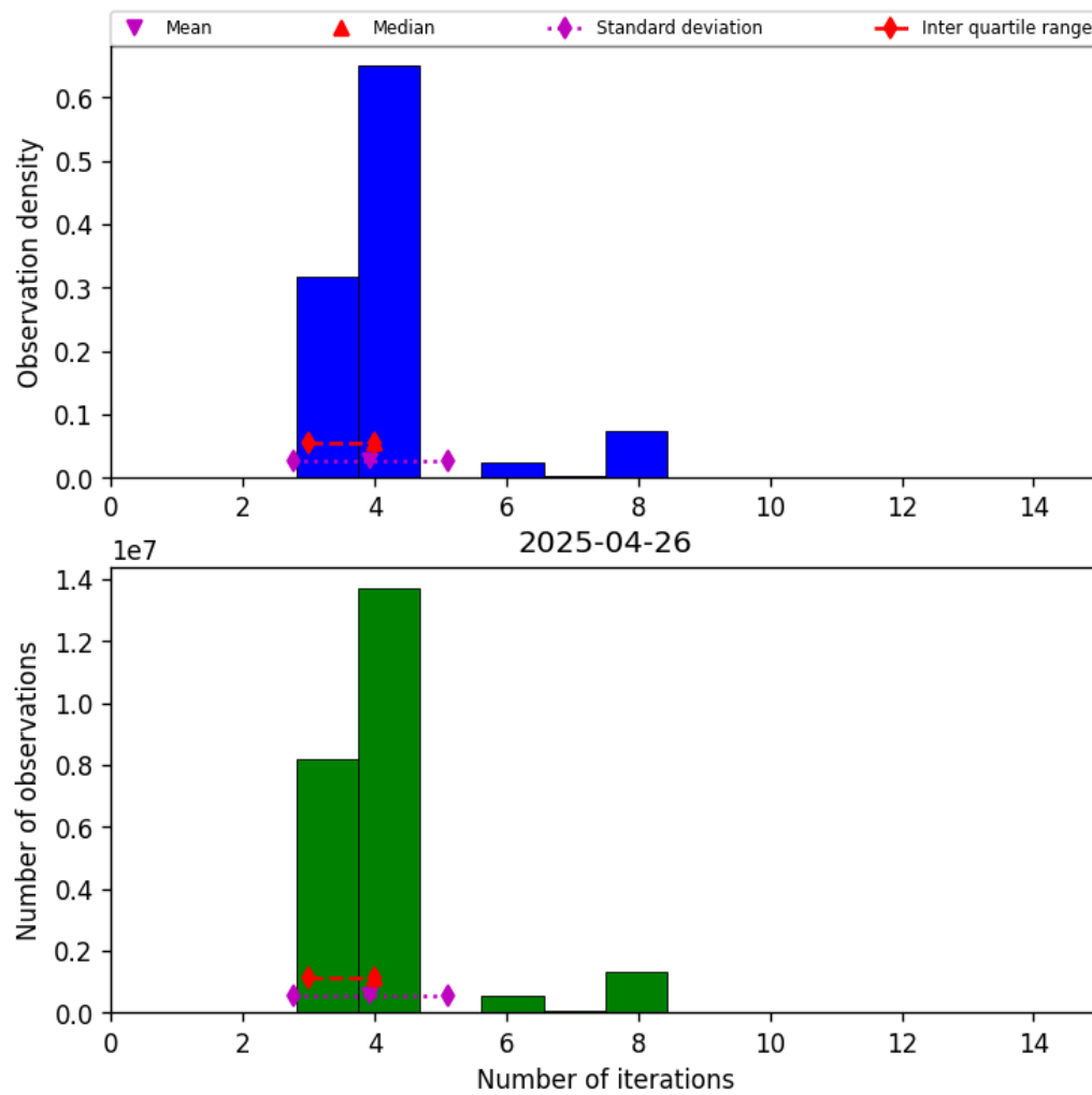
Figure 32: Histogram of “Number of iterations” for 2025-04-26 to 2025-04-27
