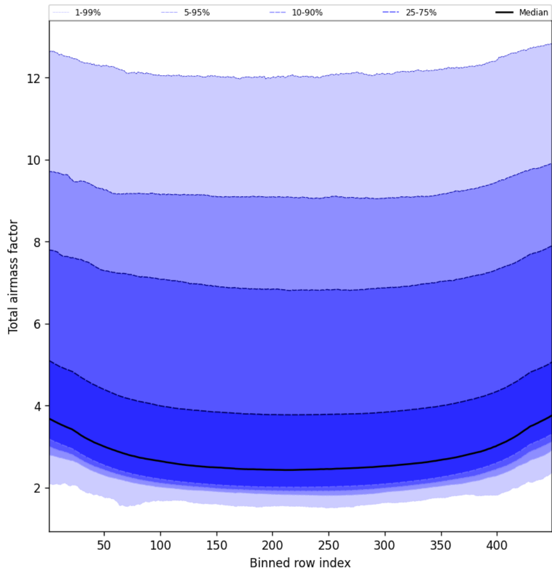
Figure 47: Along track statistics of “Total airmass factor” for 2025-04-26 to 2025-04-27
