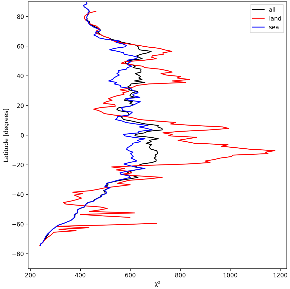
Figure 23: Zonal average of “ \chi^2 ” for 2025-04-26 to 2025-04-27.
