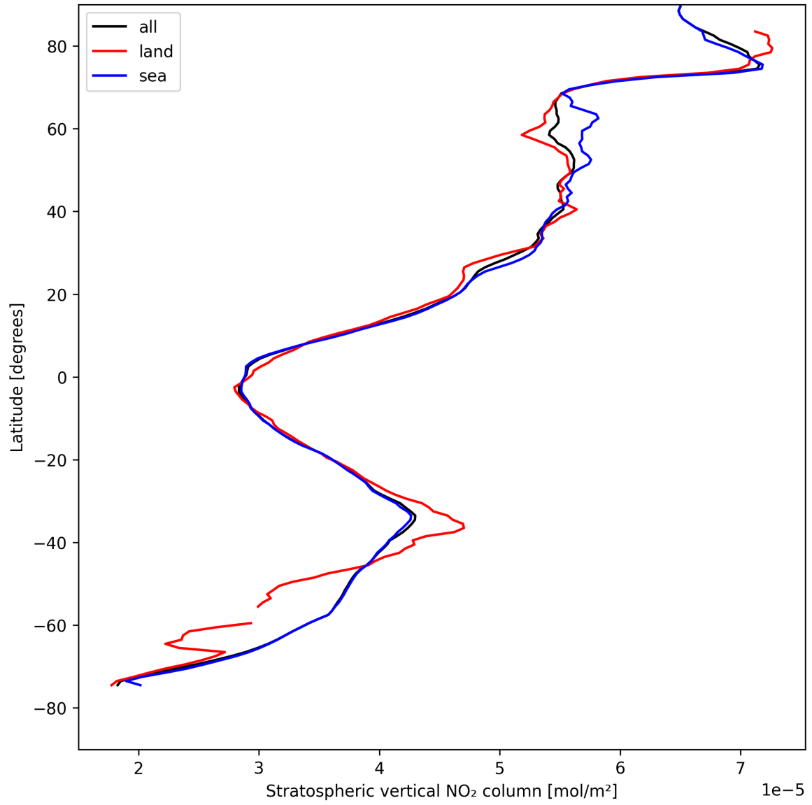
Figure 17: Zonal average of “Stratospheric vertical NO 2 column” for 2025-04-26 to 2025-04-27.
