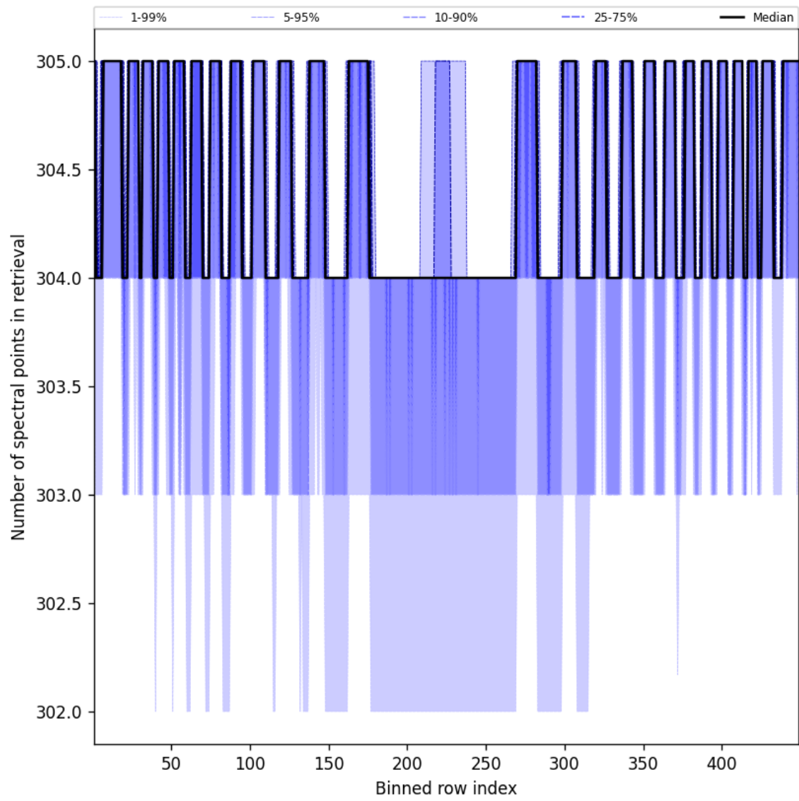
Figure 48: Along track statistics of “Number of spectral points in retrieval” for 2025-04-26 to 2025-04-27
