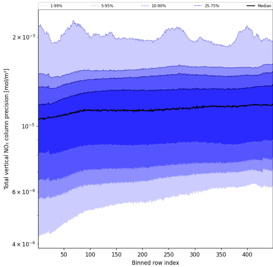
Figure 54: Along track statistics of “Total vertical NO 2 column precision” for 2025-04-26 to 2025-04-27
