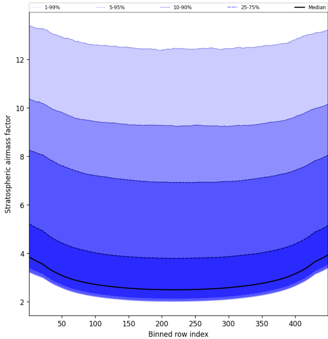
Figure 59: Along track statistics of “Stratospheric airmass factor” for 2025-04-26 to 2025-04-27
