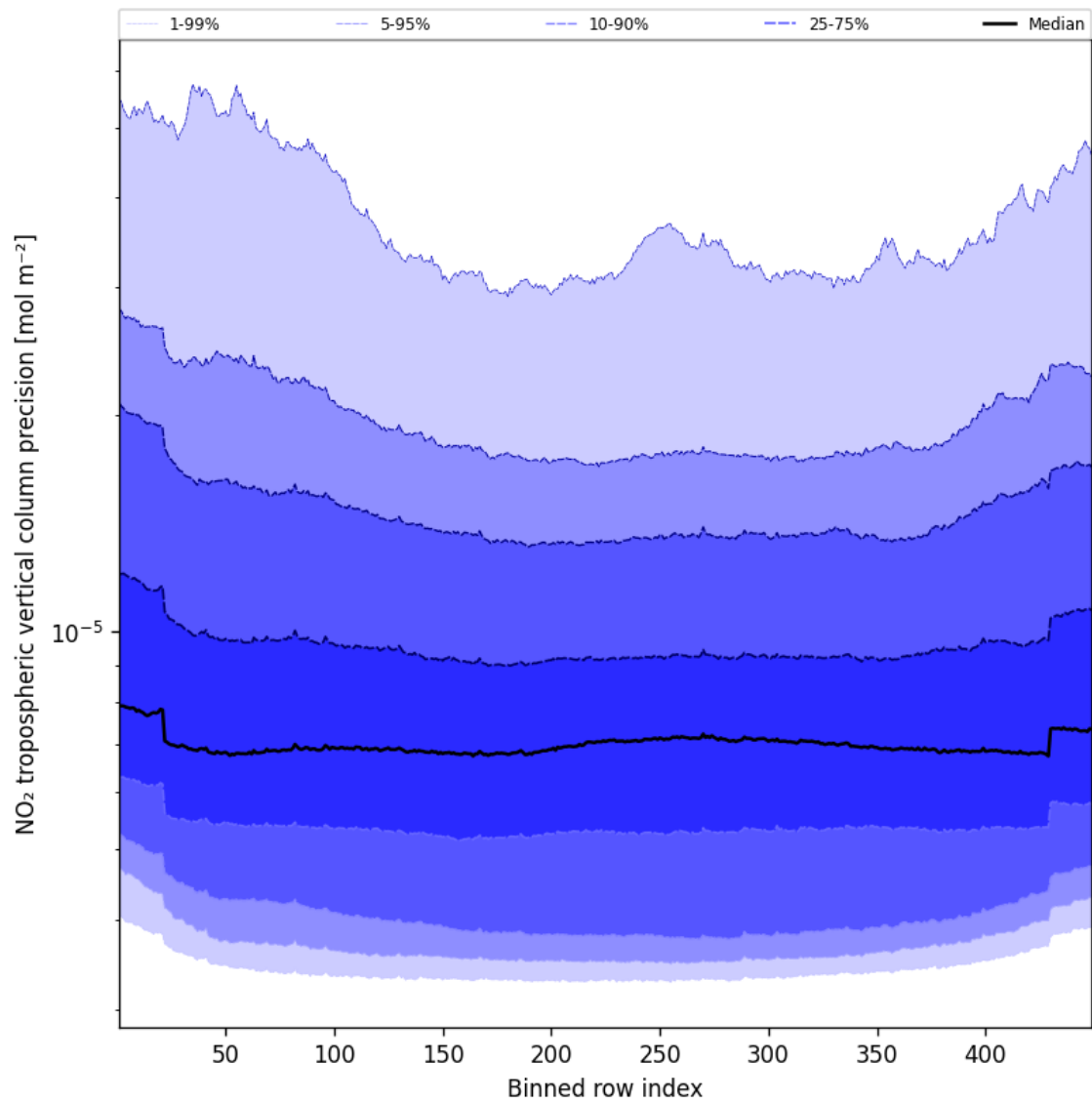
Figure 45: Along track statistics of “NO 2 tropospheric vertical column precision” for 2025-04-26 to 2025-04-27
