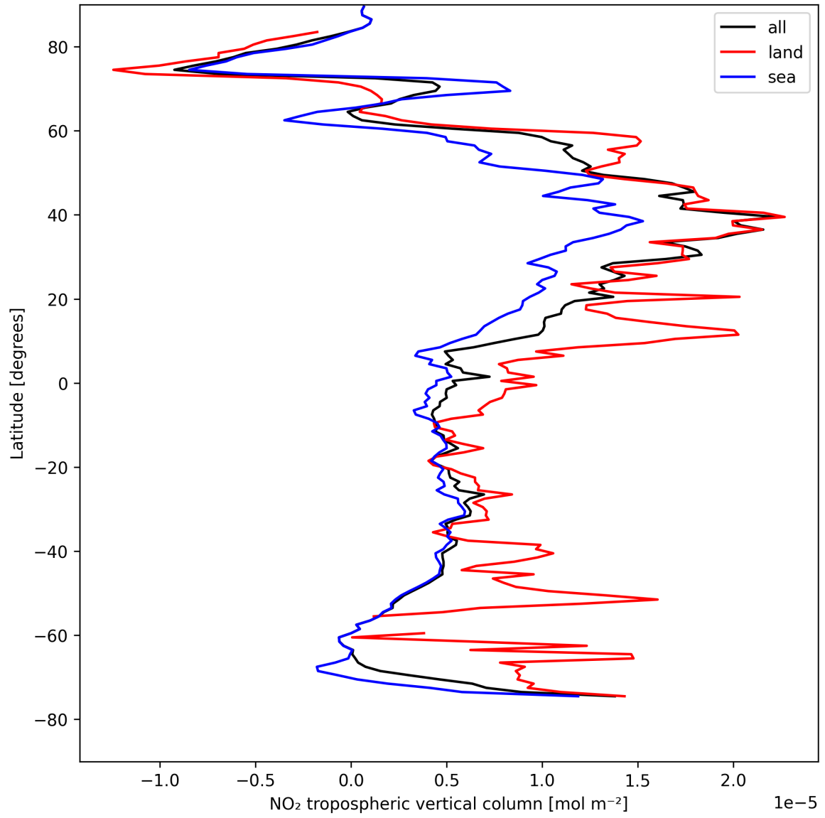
Figure 10: Zonal average of “NO 2 tropospheric vertical column” for 2025-04-26 to 2025-04-27.
