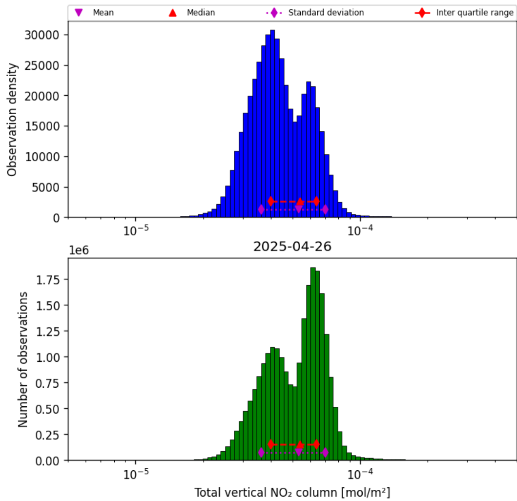
Figure 36: Histogram of "Total vertical NO 2 column" for 2025-04-26 to 2025-04-27
