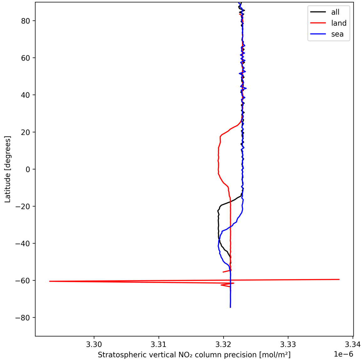
Figure 18: Zonal average of “Stratospheric vertical NO 2 column precision” for 2025-04-26 to 2025-04-27.
