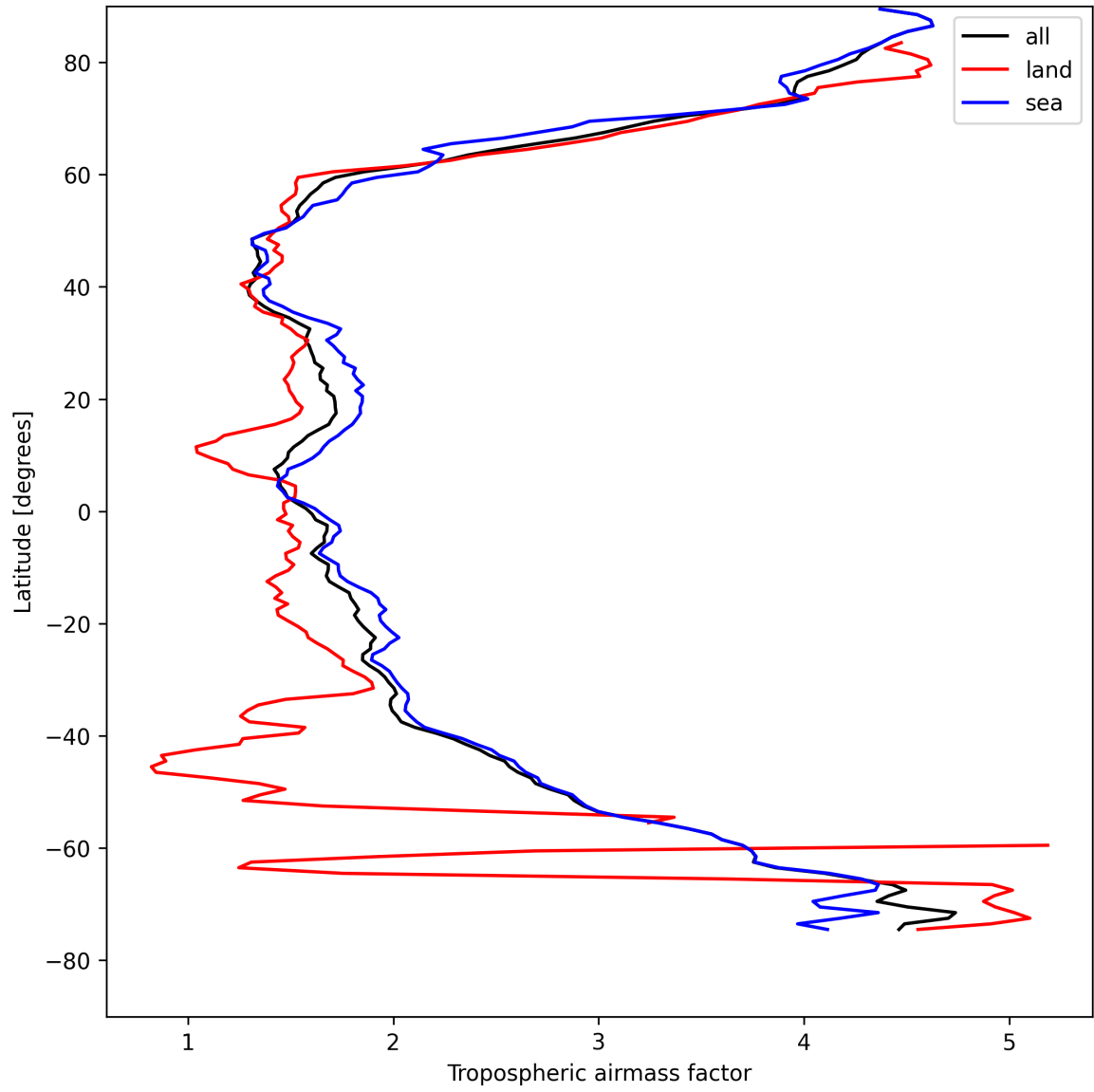
Figure 12: Zonal average of “Tropospheric airmass factor” for 2025-04-26 to 2025-04-27.
