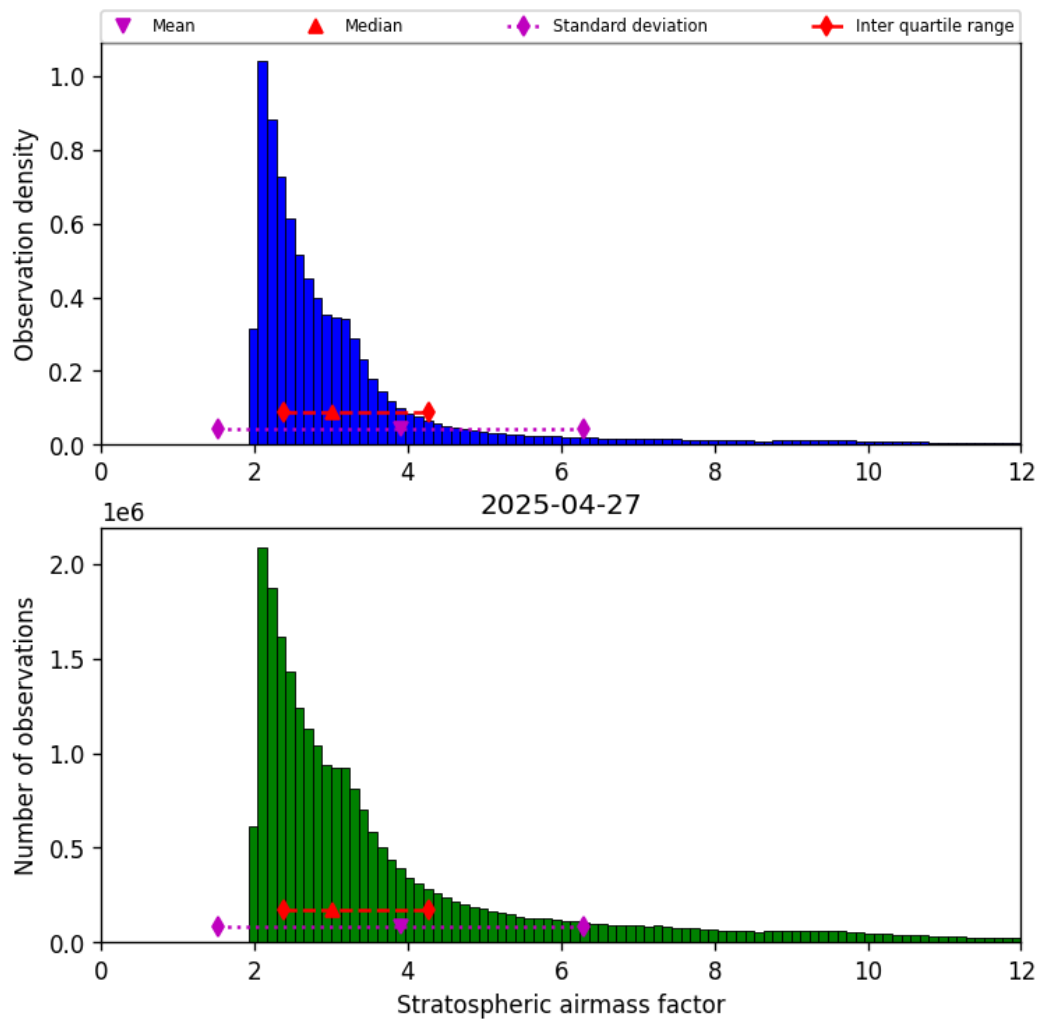
Figure 42: Histogram of “Stratospheric airmass factor” for 2025-04-27 to 2025-04-27
