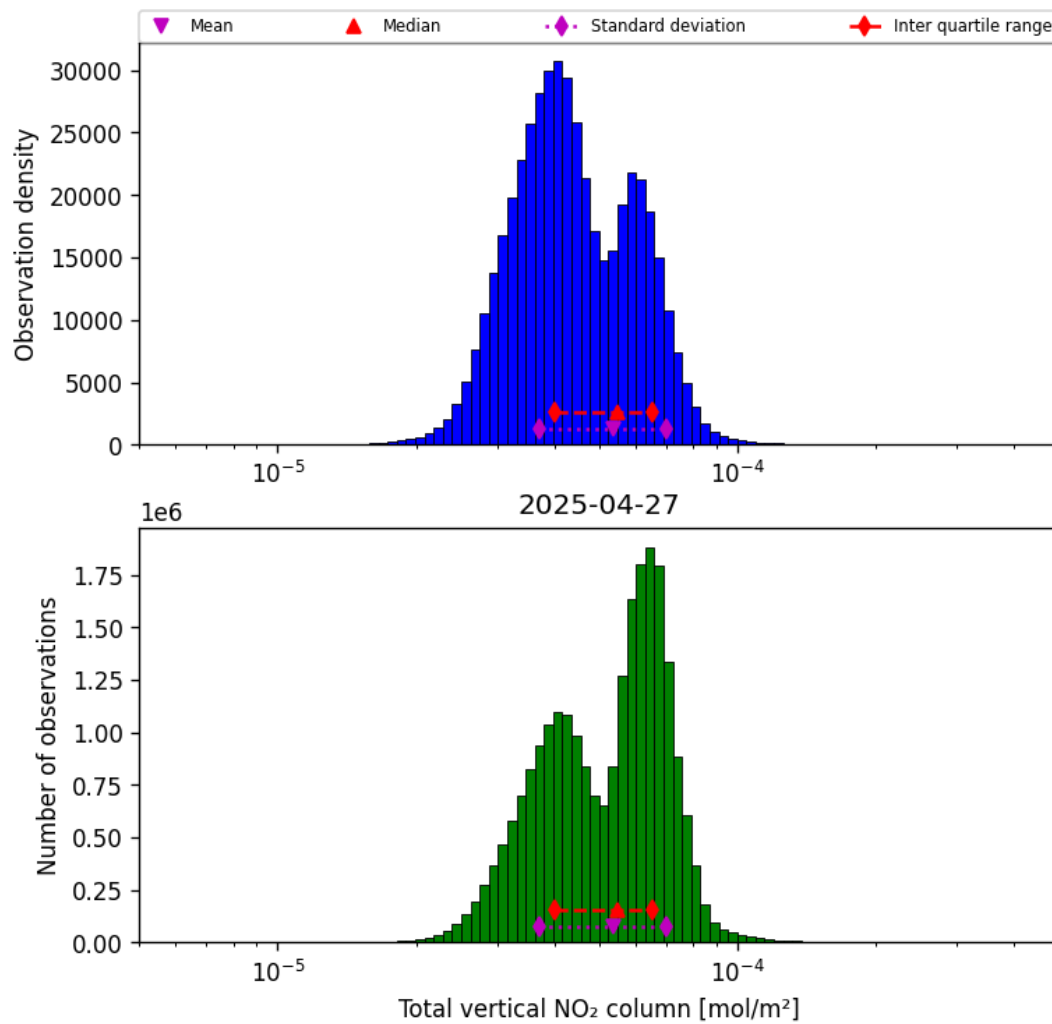
Figure 36: Histogram of “Total vertical NO 2 column” for 2025-04-27 to 2025-04-27
