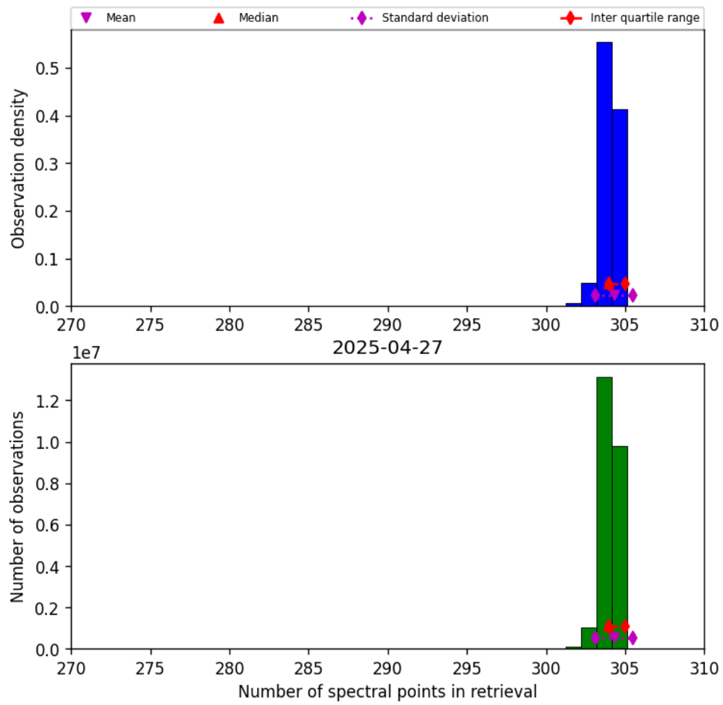
Figure 31: Histogram of “Number of spectral points in retrieval” for 2025-04-27 to 2025-04-27
