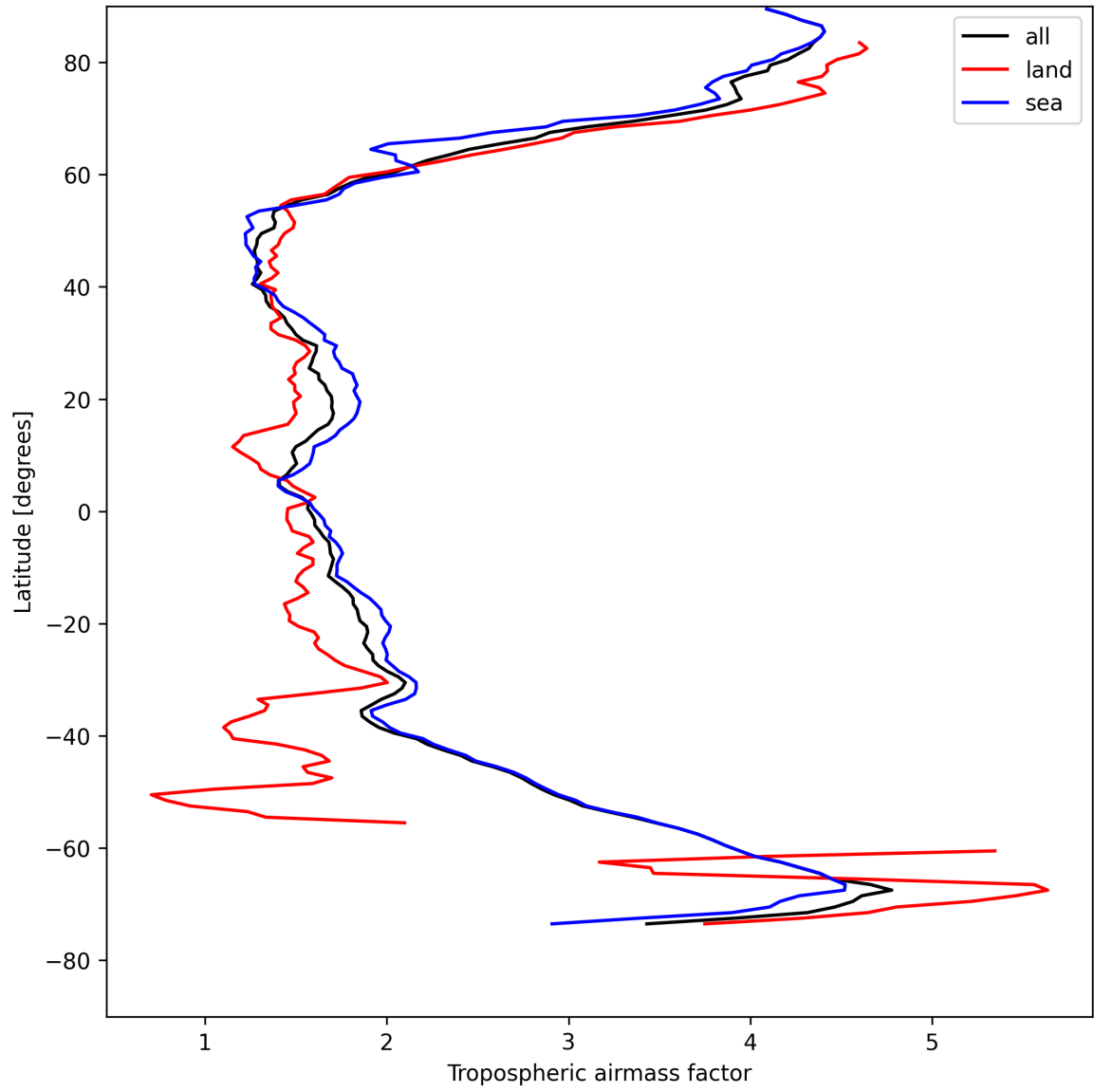
Figure 12: Zonal average of “Tropospheric airmass factor” for 2025-04-27 to 2025-04-27.
