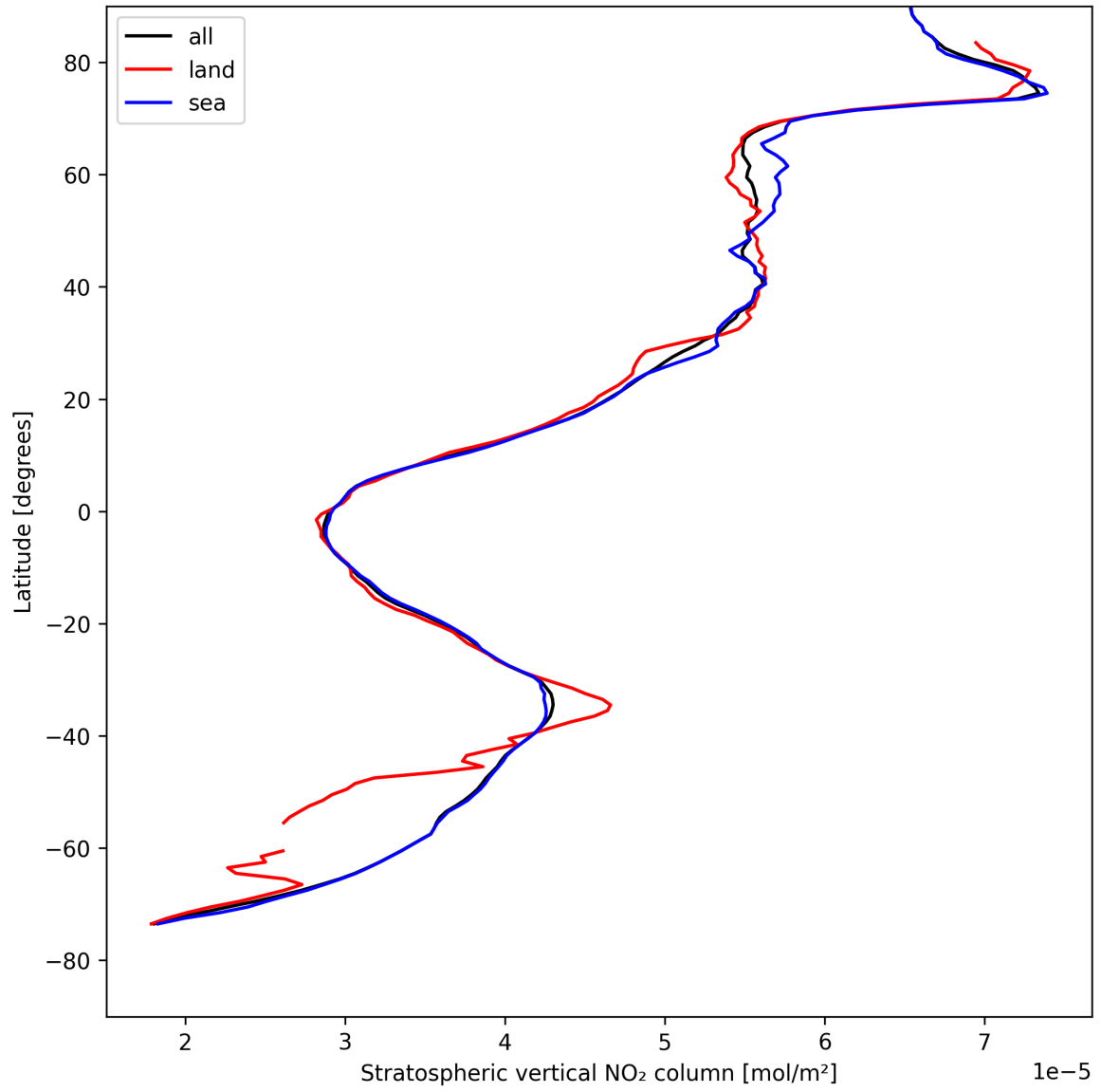
Figure 17: Zonal average of “Stratospheric vertical NO 2 column” for 2025-04-27 to 2025-04-27.
