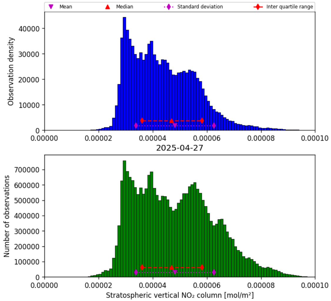
Figure 34: Histogram of “Stratospheric vertical NO 2 column” for 2025-04-27 to 2025-04-27
