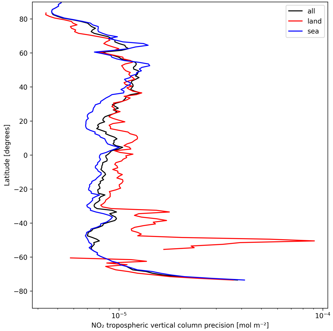
Figure 11: Zonal average of “NO 2 tropospheric vertical column precision” for 2025-04-27 to 2025-04-27.
