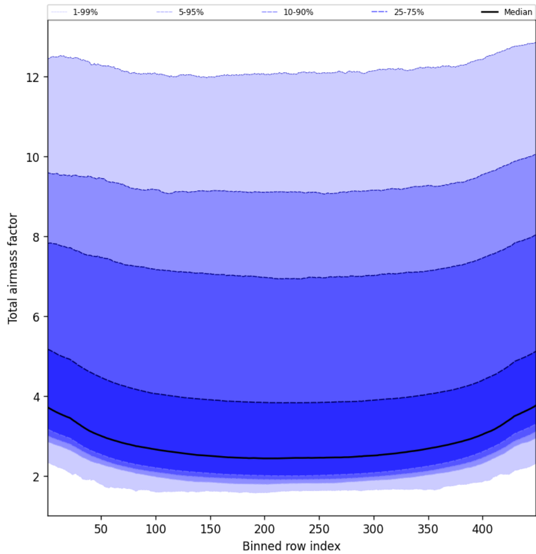
Figure 47: Along track statistics of “Total airmass factor” for 2025-04-27 to 2025-04-27
