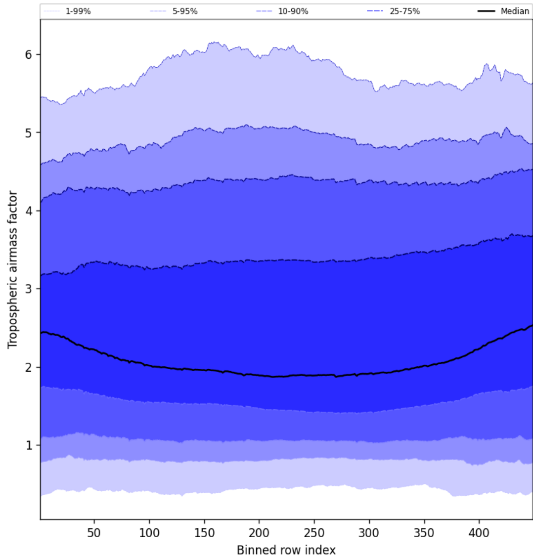
Figure 46: Along track statistics of “Tropospheric airmass factor” for 2025-04-27 to 2025-04-27
