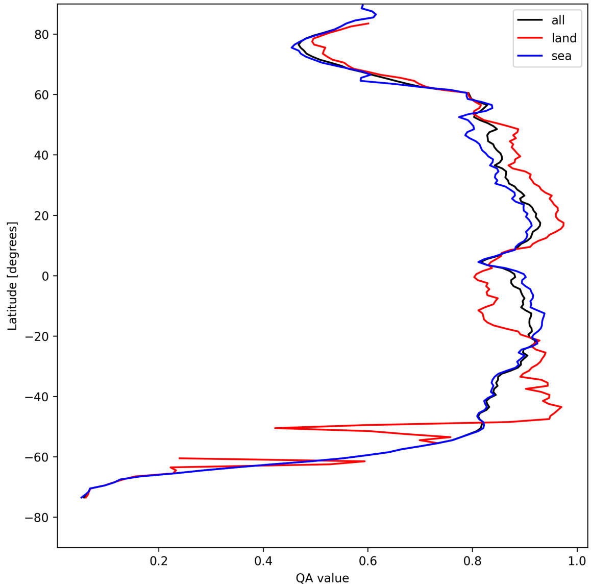
Figure 9: Zonal average of “QA value” for 2025-04-27 to 2025-04-27.
