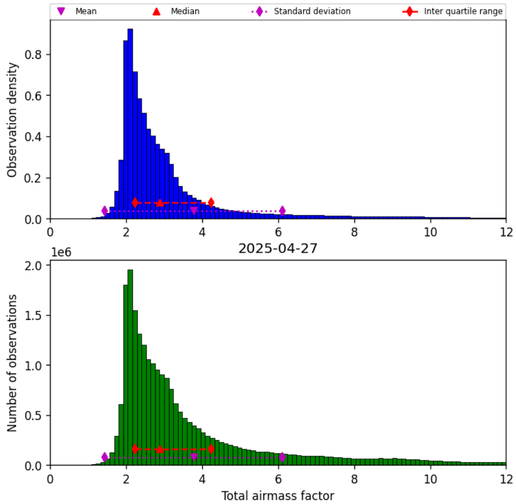
Figure 30: Histogram of “Total airmass factor” for 2025-04-27 to 2025-04-27
