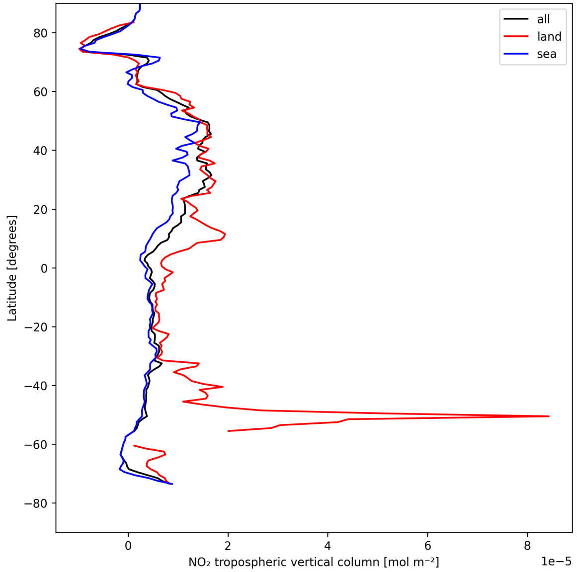
Figure 10: Zonal average of “NO 2 tropospheric vertical column” for 2025-04-27 to 2025-04-27.
