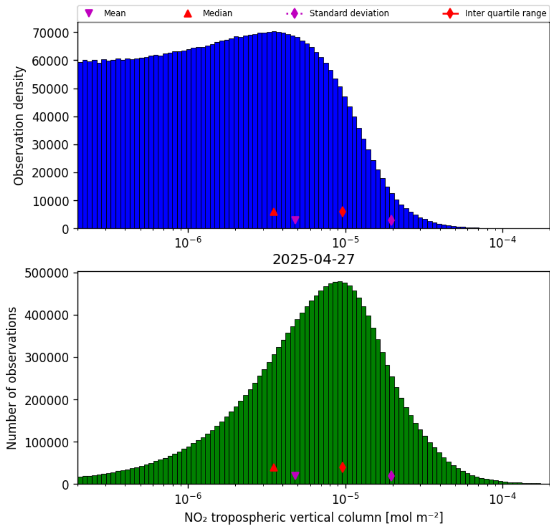
Figure 27: Histogram of “NO 2 tropospheric vertical column” for 2025-04-27 to 2025-04-27
