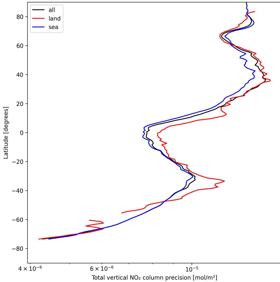
Figure 20: Zonal average of “Total vertical NO 2 column precision” for 2025-04-27 to 2025-04-27.
