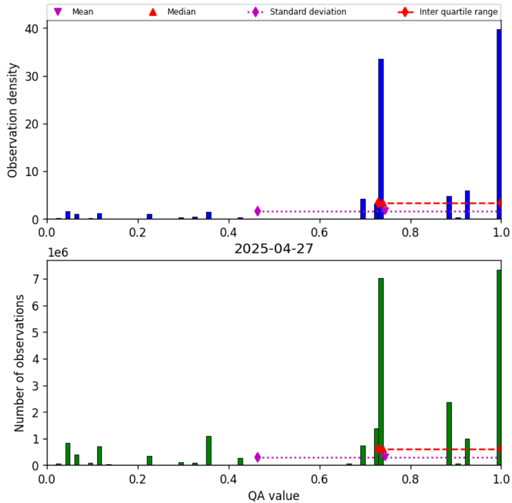
Figure 26: Histogram of “QA value” for 2025-04-27 to 2025-04-27
