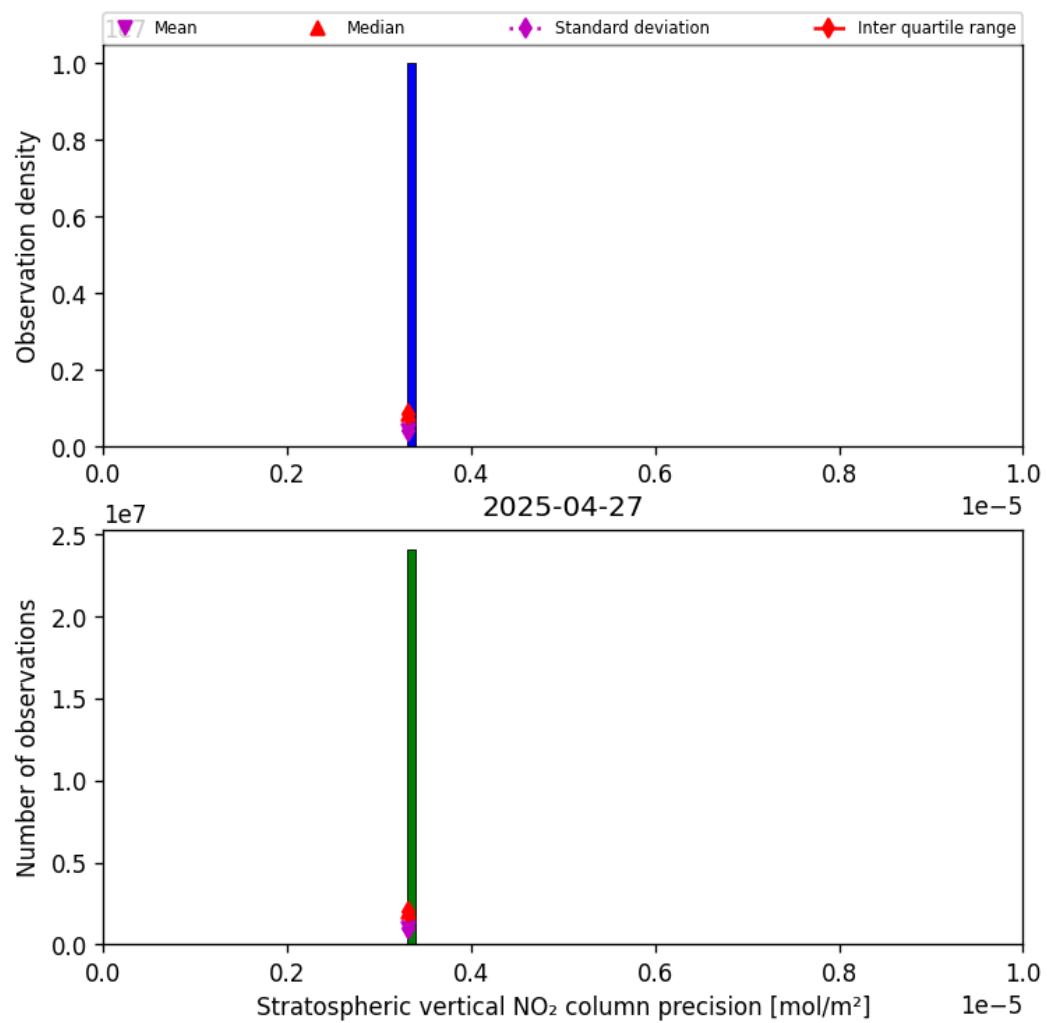
Figure 35: Histogram of “Stratospheric vertical NO 2 column precision” for 2025-04-27 to 2025-04-27
