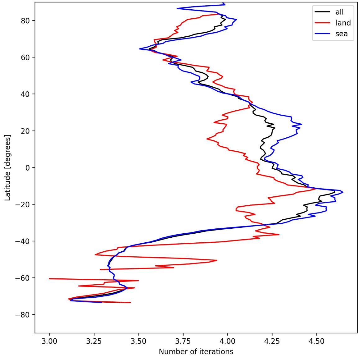
Figure 15: Zonal average of “Number of iterations” for 2025-04-27 to 2025-04-27.
