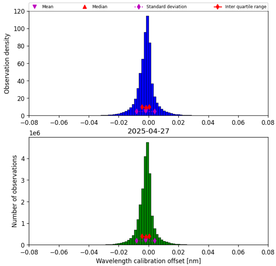
Figure 33: Histogram of “Wavelength calibration offset” for 2025-04-27 to 2025-04-27
