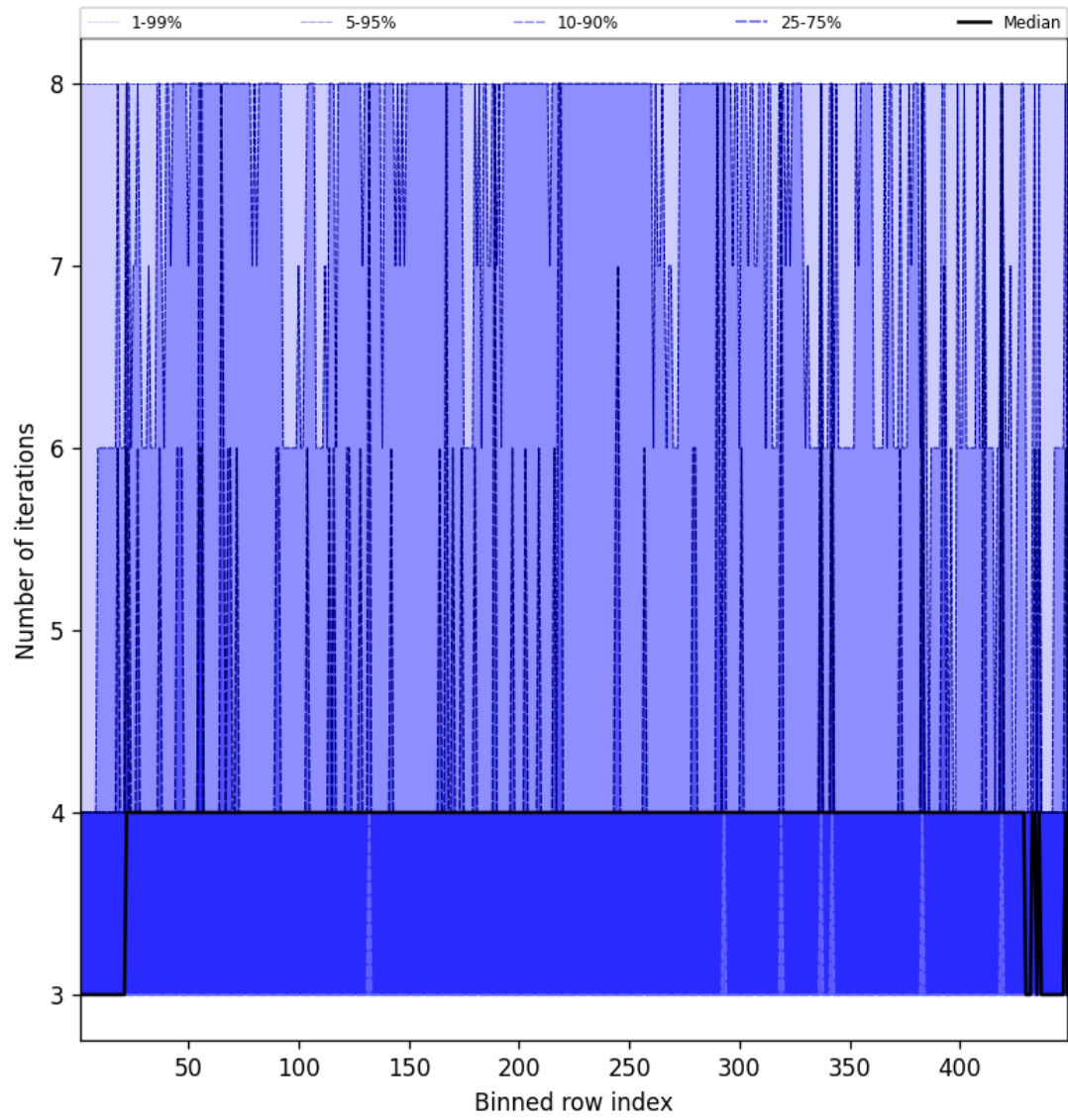
Figure 49: Along track statistics of “Number of iterations” for 2025-04-27 to 2025-04-27
