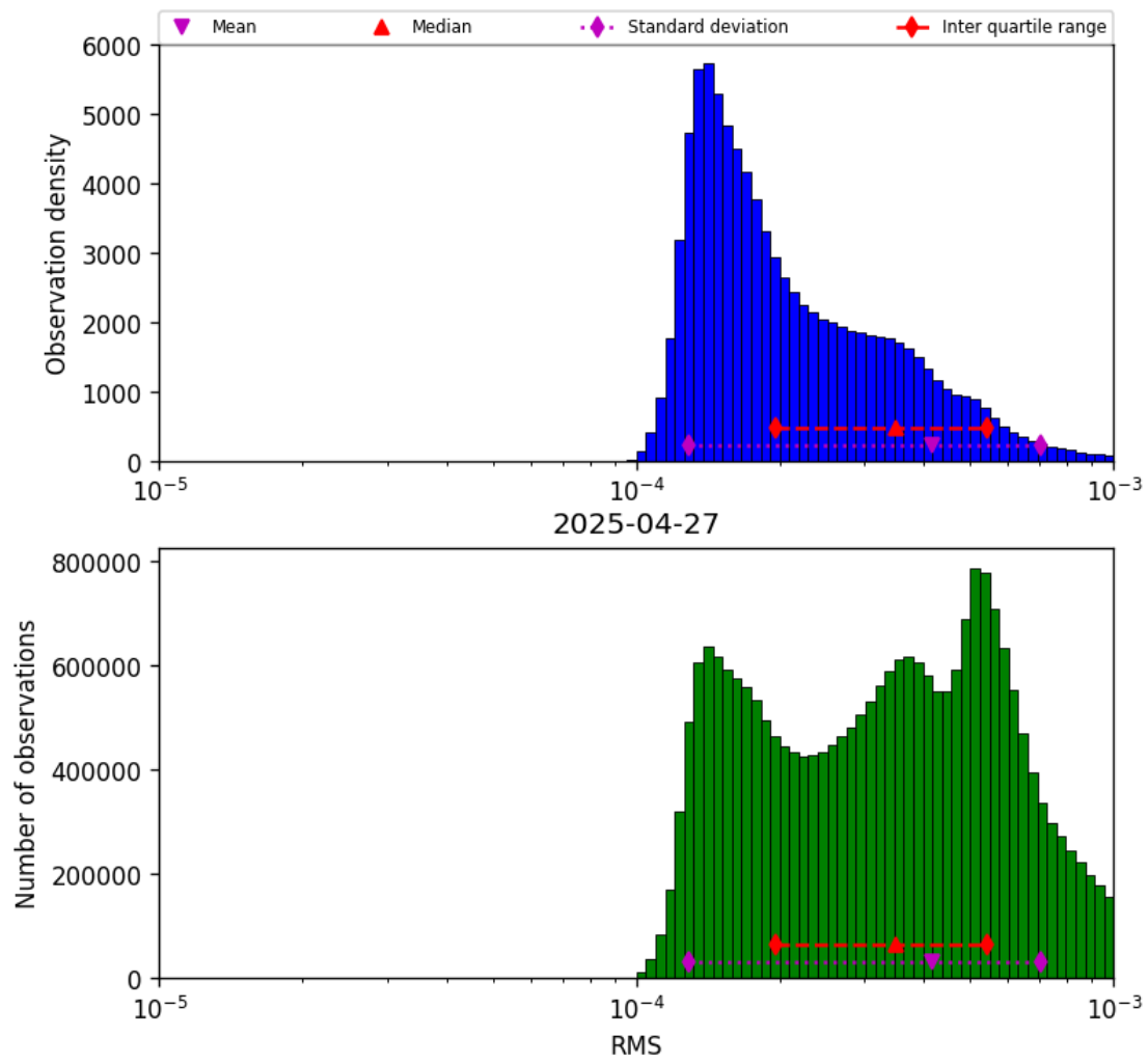
Figure 41: Histogram of “RMS” for 2025-04-27 to 2025-04-27
