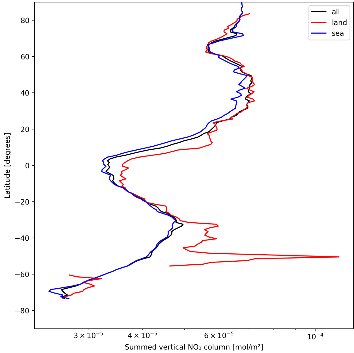
Figure 21: Zonal average of “Summed vertical NO 2 column” for 2025-04-27 to 2025-04-27.
