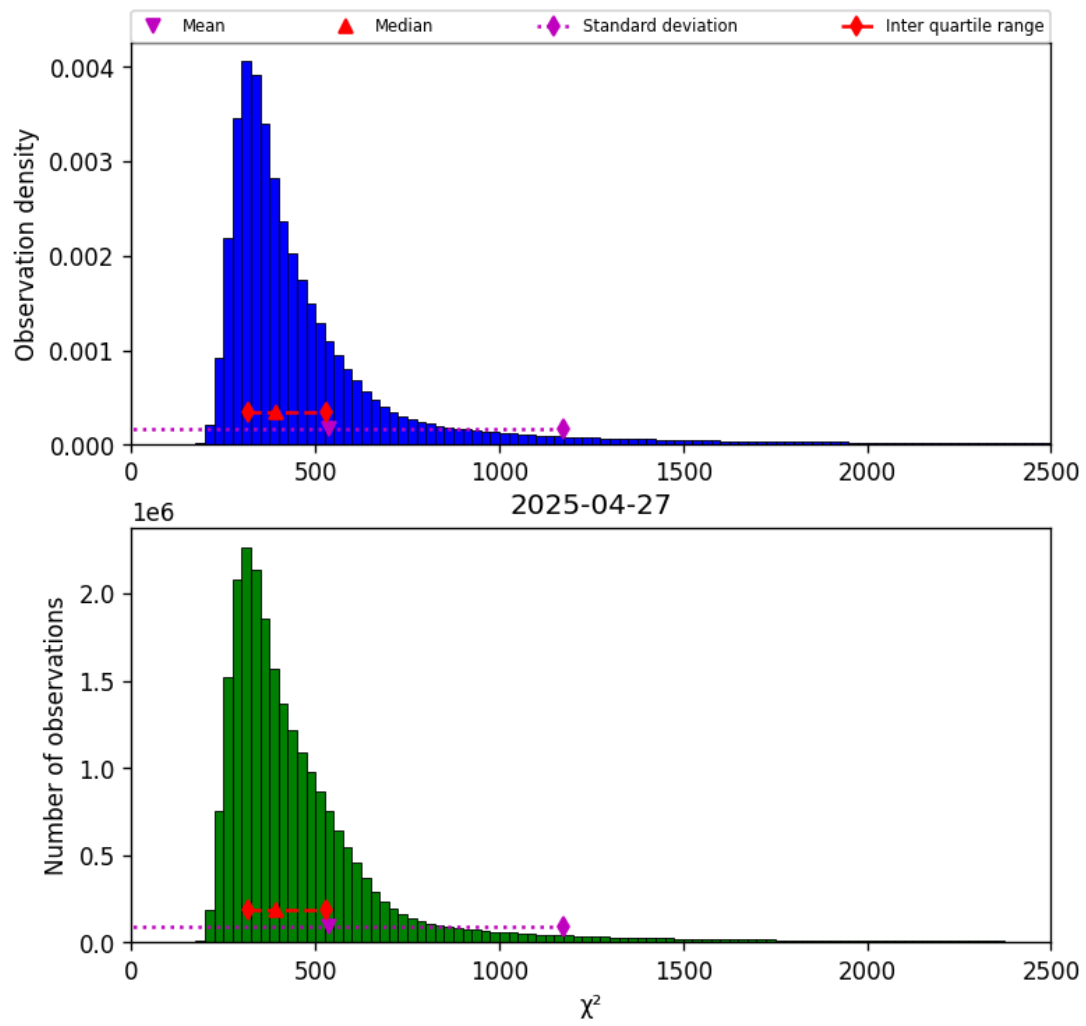
Figure 40: Histogram of " \chi^2 " for 2025-04-27 to 2025-04-27
