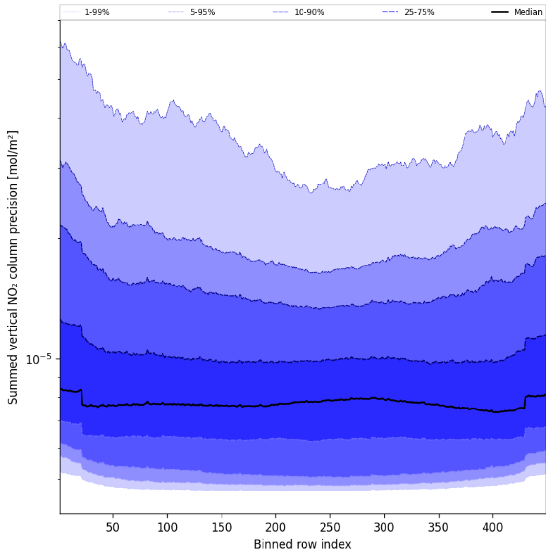
Figure 56: Along track statistics of “Summed vertical NO 2 column precision” for 2025-04-27 to 2025-04-27
