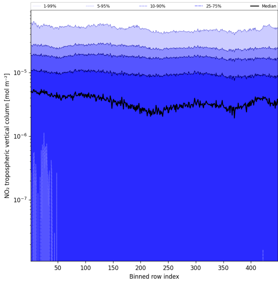
Figure 44: Along track statistics of “NO 2 tropospheric vertical column” for 2025-04-27 to 2025-04-27
