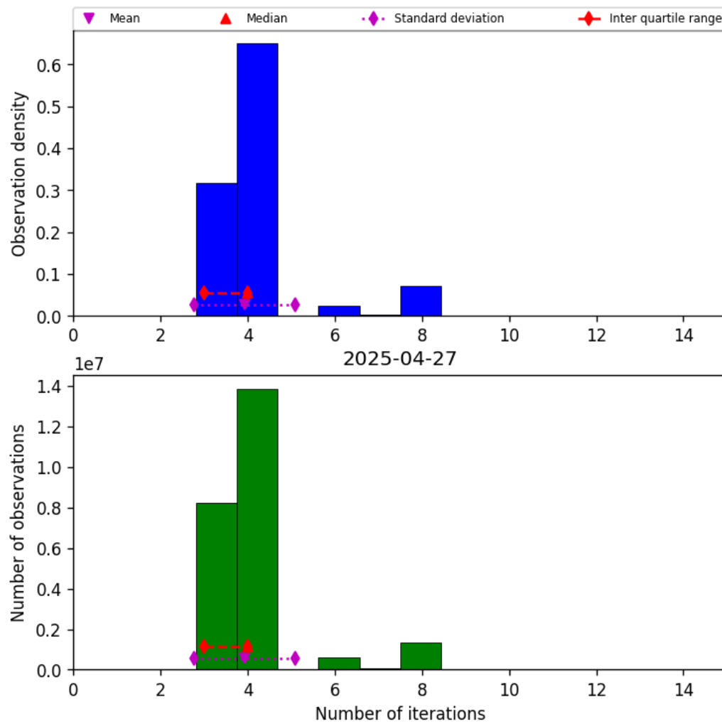
Figure 32: Histogram of “Number of iterations” for 2025-04-27 to 2025-04-27
