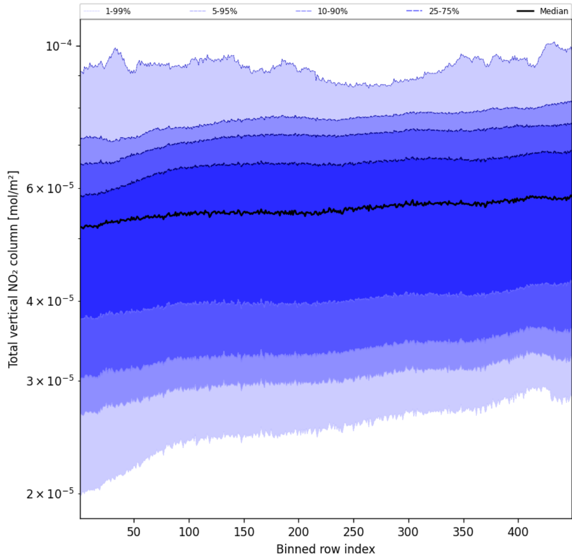
Figure 53: Along track statistics of “Total vertical NO 2 column” for 2025-04-27 to 2025-04-27
