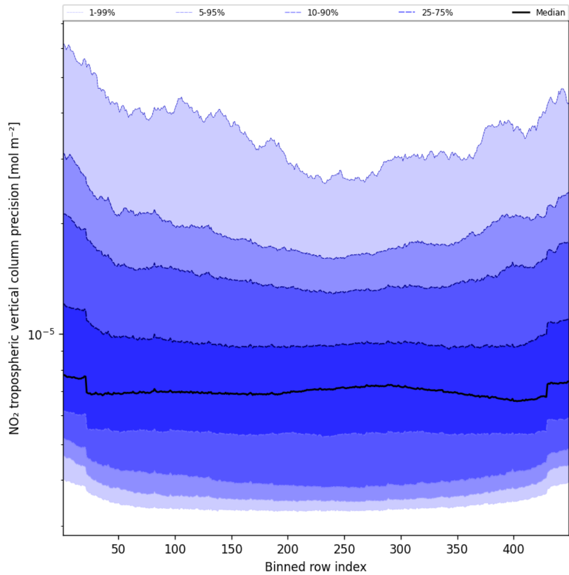
Figure 45: Along track statistics of “NO 2 tropospheric vertical column precision” for 2025-04-27 to 2025-04-27
