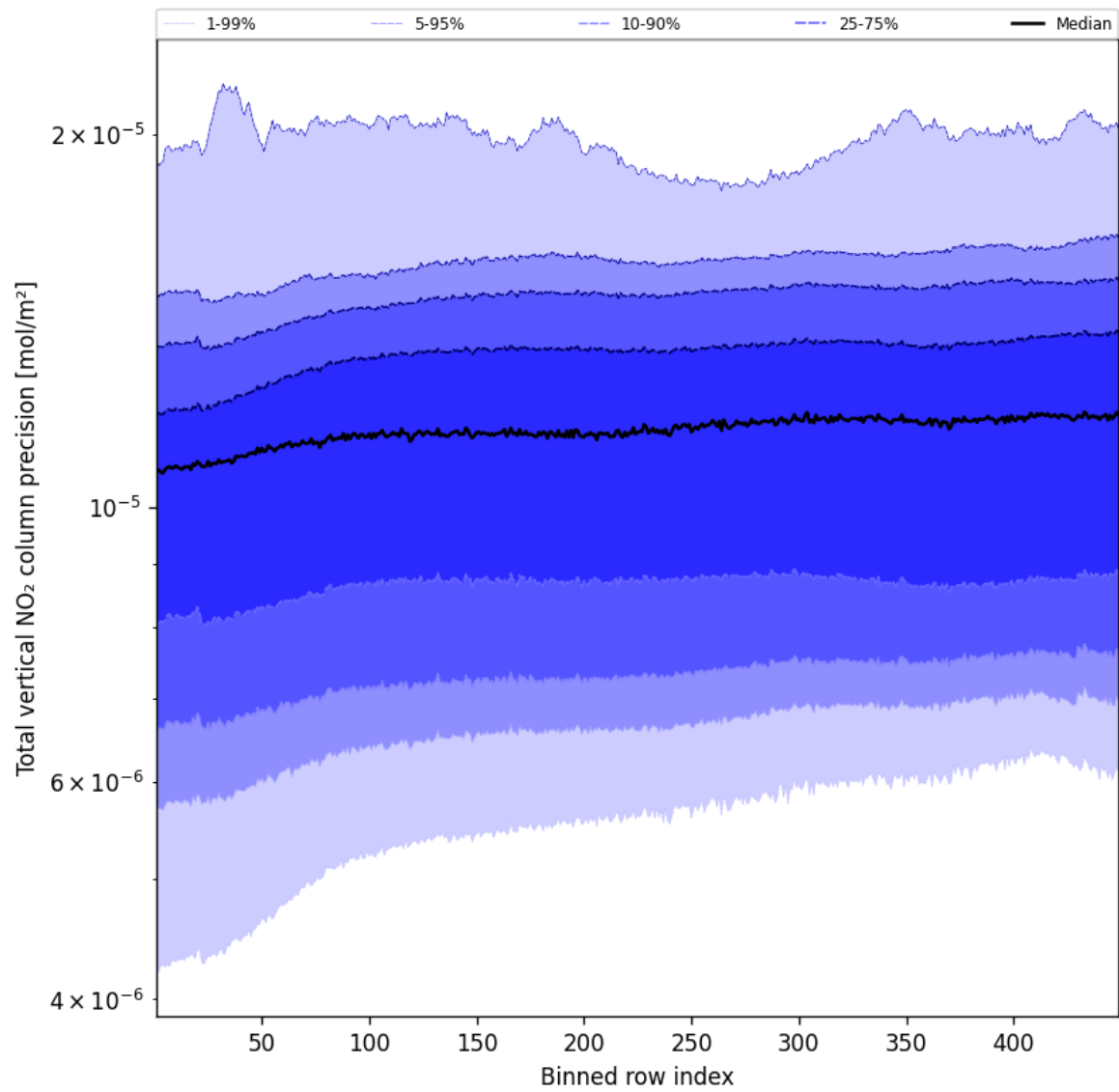
Figure 54: Along track statistics of “Total vertical NO 2 column precision” for 2025-04-27 to 2025-04-27
