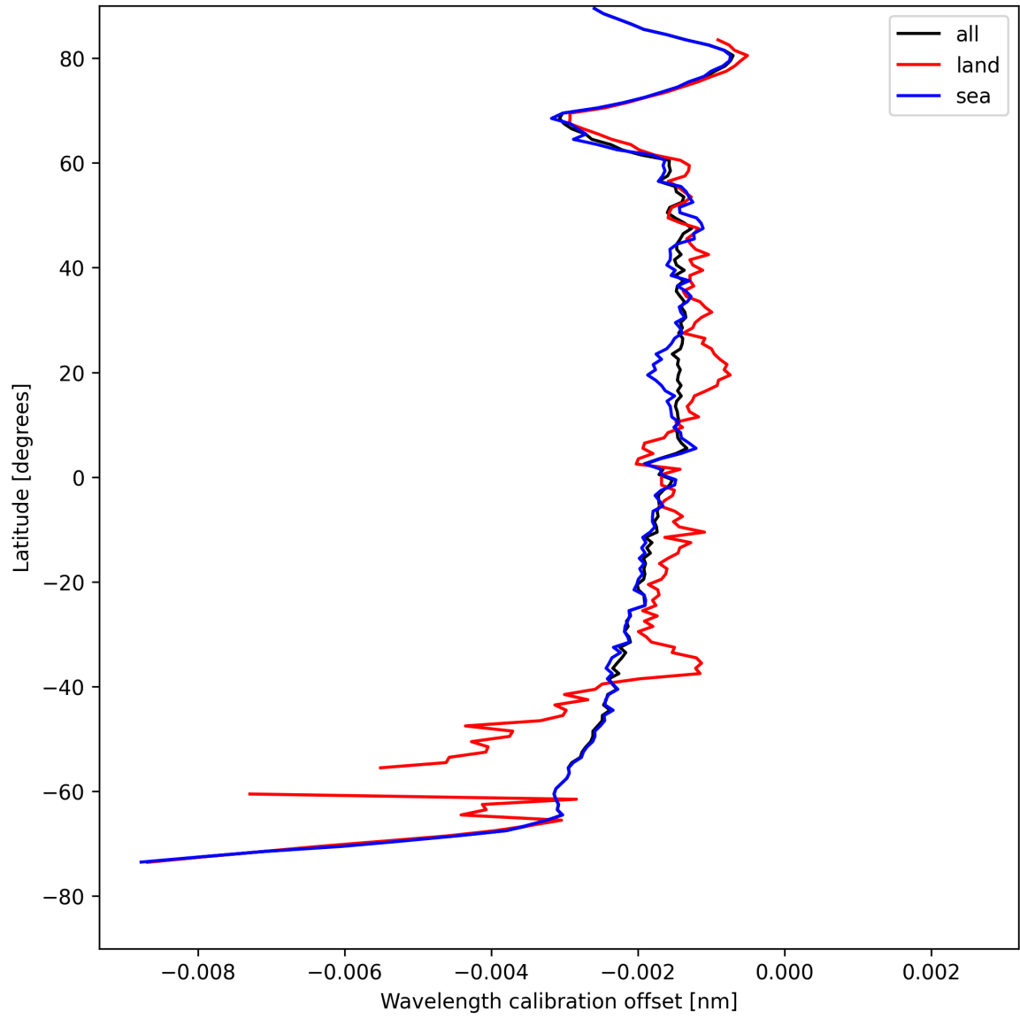
Figure 16: Zonal average of “Wavelength calibration offset” for 2025-04-27 to 2025-04-27.
