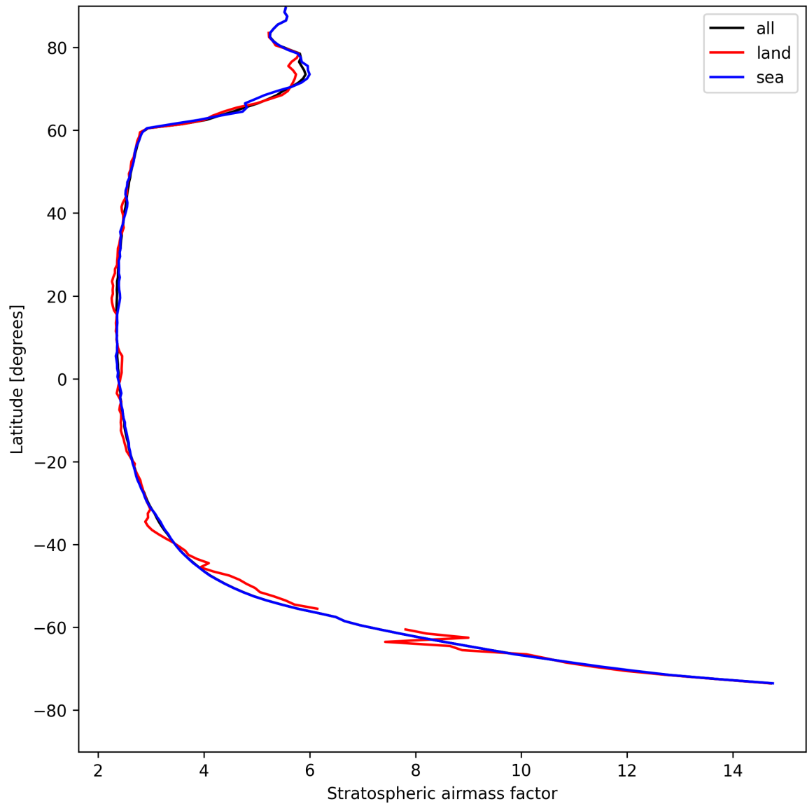
Figure 25: Zonal average of “Stratospheric air mass factor” for 2025-04-27 to 2025-04-27.
