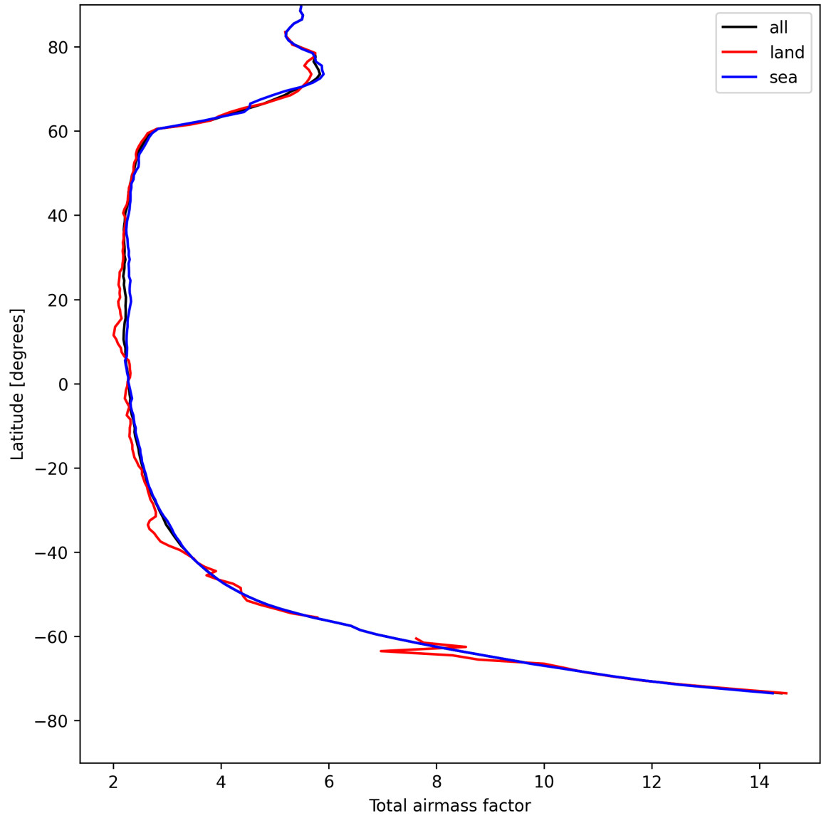
Figure 13: Zonal average of “Total airmass factor” for 2025-04-27 to 2025-04-27.
