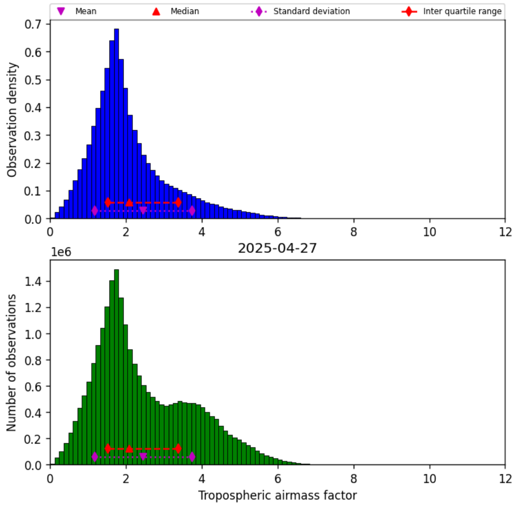
Figure 29: Histogram of “Tropospheric airmass factor” for 2025-04-27 to 2025-04-27
