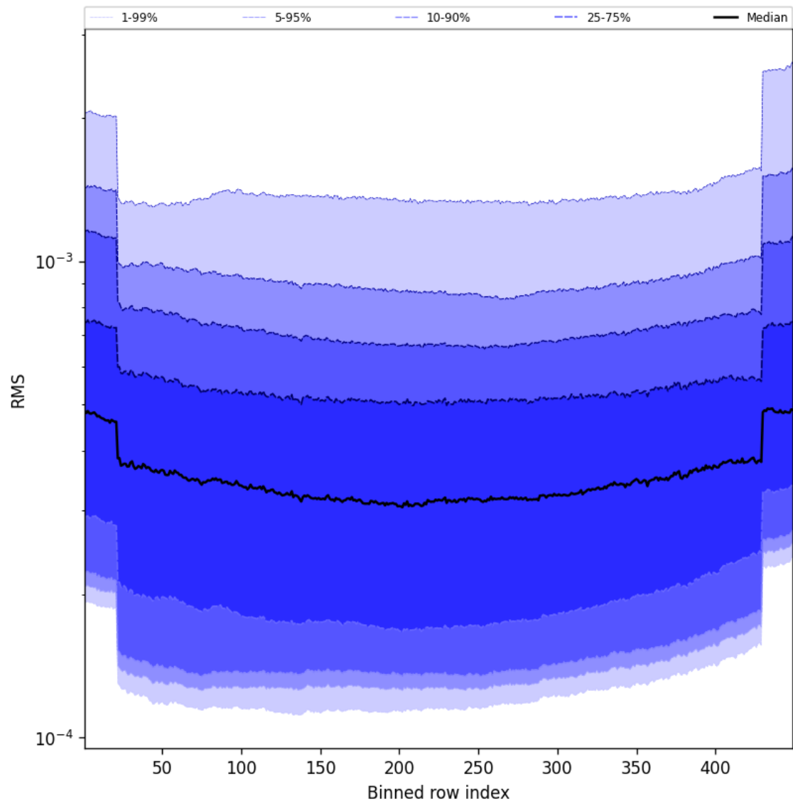
Figure 58: Along track statistics of “RMS” for 2025-04-27 to 2025-04-27
