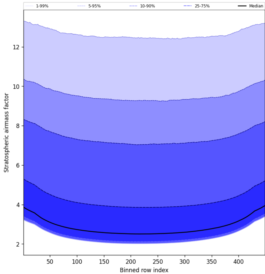
Figure 59: Along track statistics of “Stratospheric airmass factor” for 2025-04-27 to 2025-04-27
