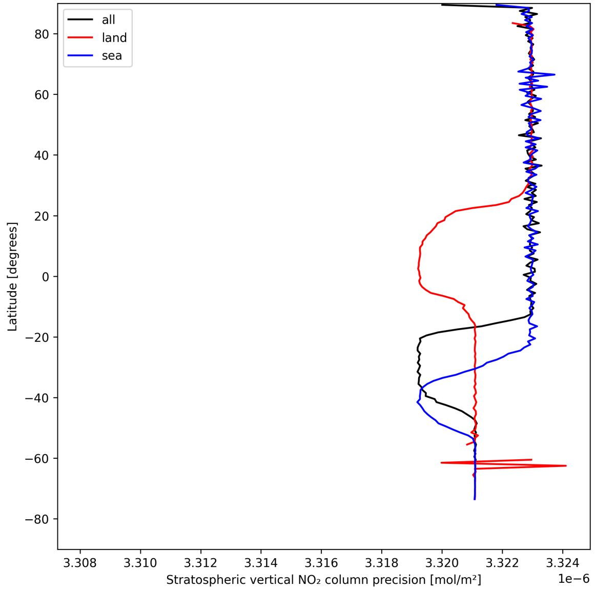
Figure 18: Zonal average of “Stratospheric vertical NO 2 column precision” for 2025-04-27 to 2025-04-27.
