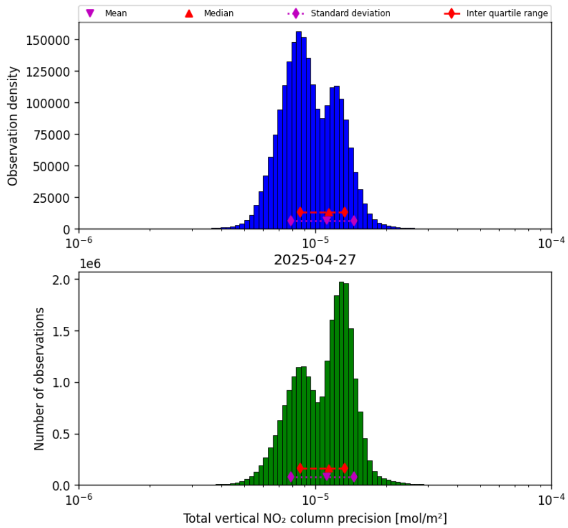
Figure 37: Histogram of "Total vertical NO 2 column precision" for 2025-04-27 to 2025-04-27
