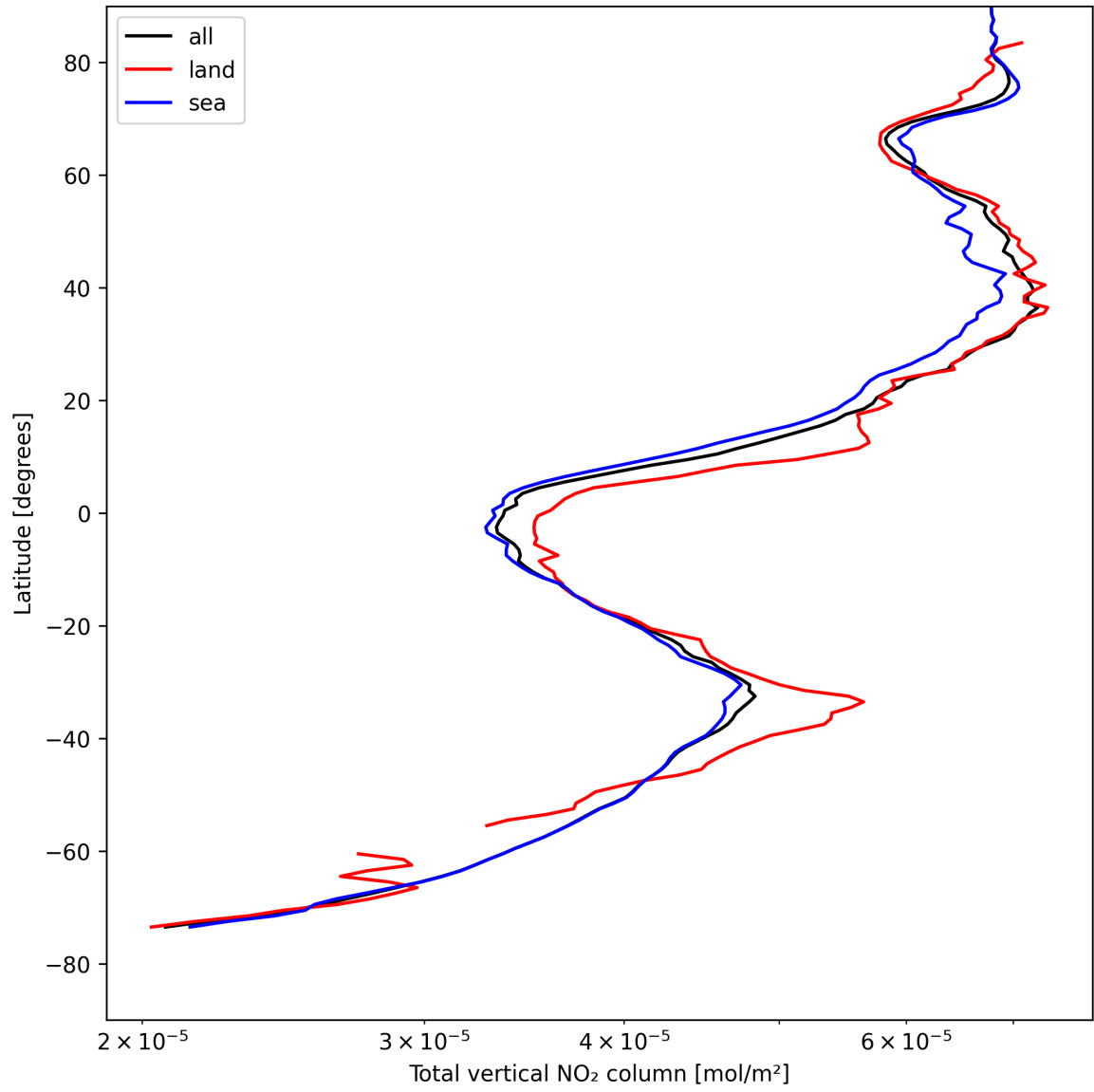
Figure 19: Zonal average of “Total vertical NO 2 column” for 2025-04-27 to 2025-04-27.
