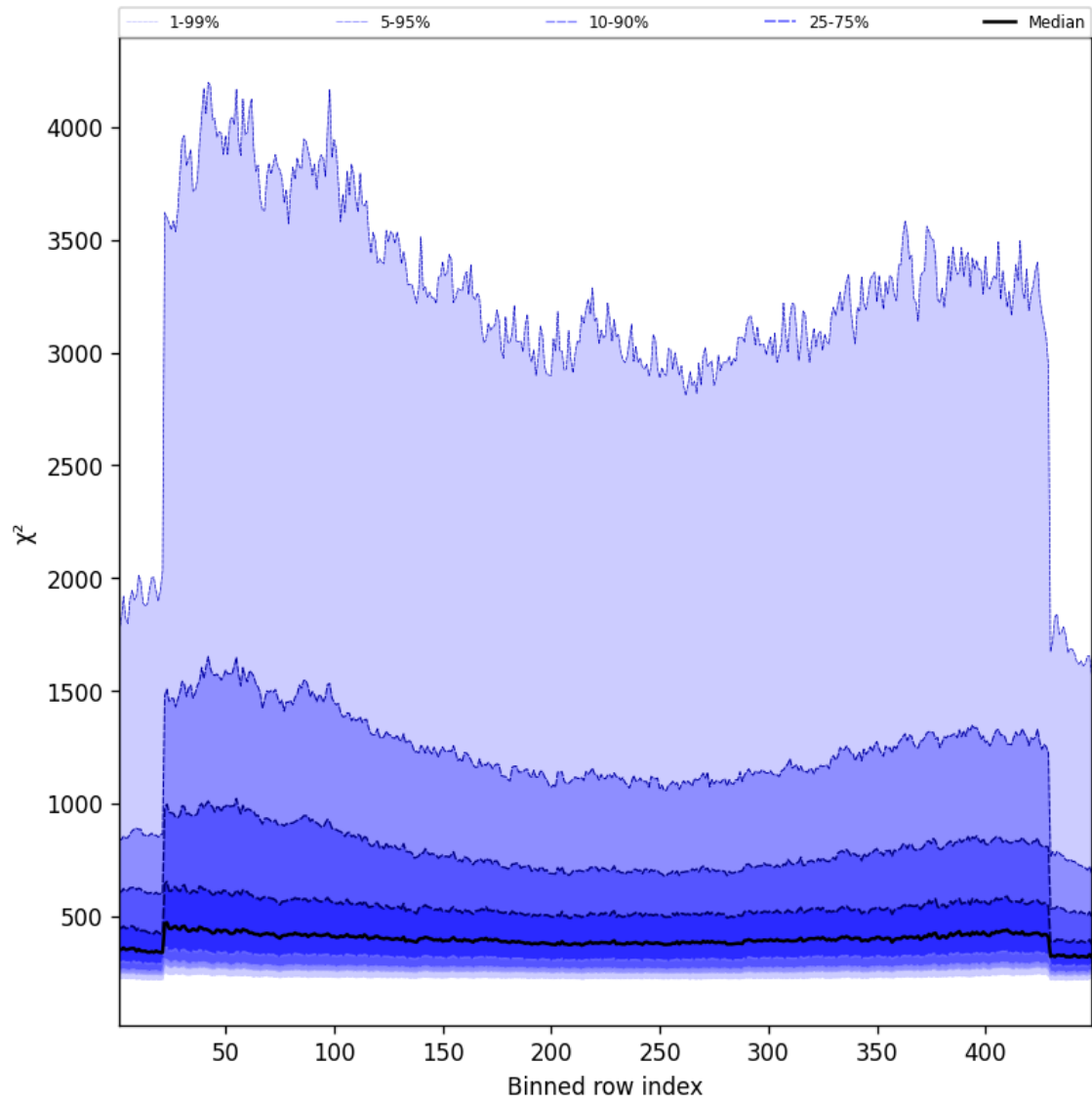
Figure 57: Along track statistics of “ \chi^2 ” for 2025-04-27 to 2025-04-27
