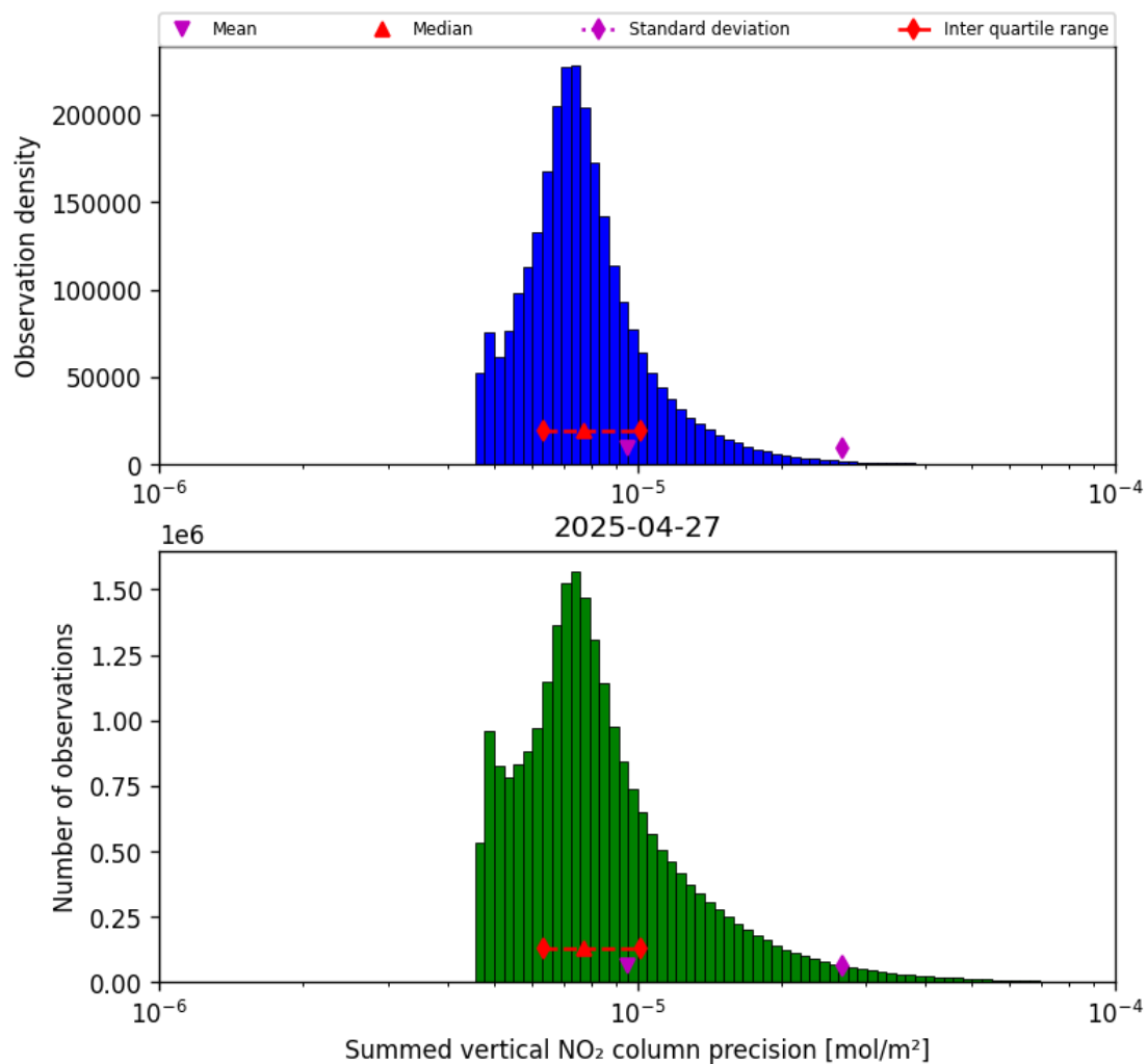
Figure 39: Histogram of "Summed vertical NO 2 column precision" for 2025-04-27 to 2025-04-27
