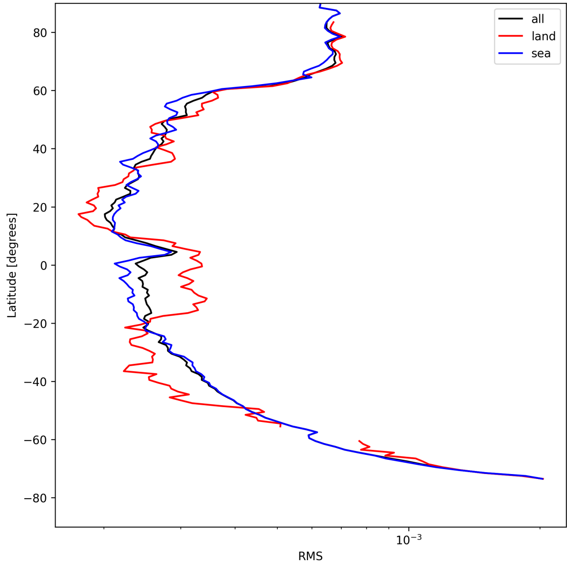
Figure 24: Zonal average of “RMS” for 2025-04-27 to 2025-04-27.
