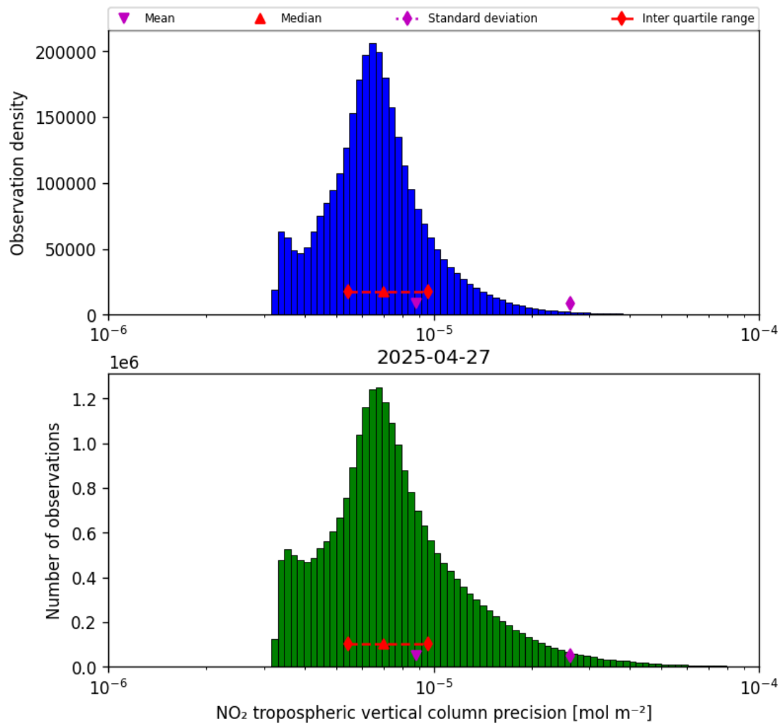
Figure 28: Histogram of “NO 2 tropospheric vertical column precision” for 2025-04-27 to 2025-04-27
