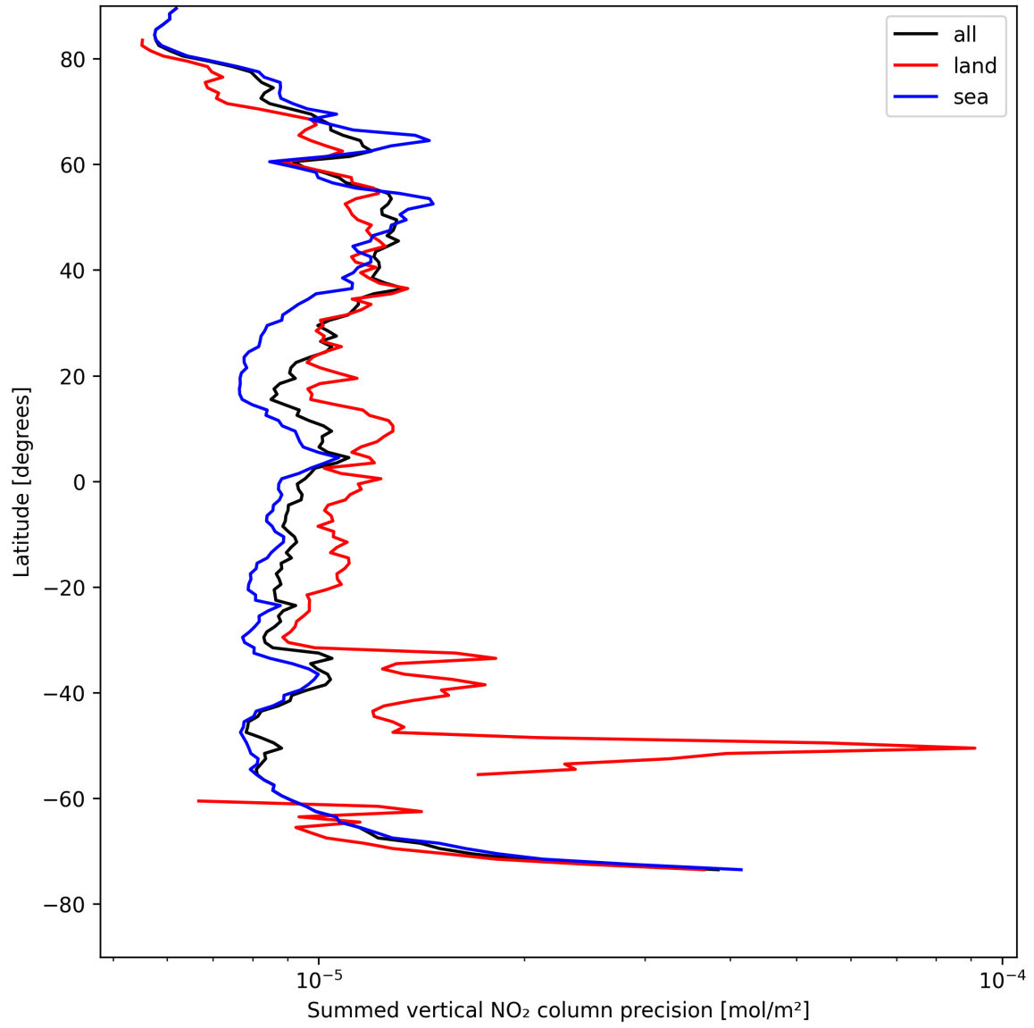
Figure 22: Zonal average of “Summed vertical NO 2 column precision” for 2025-04-27 to 2025-04-27.
