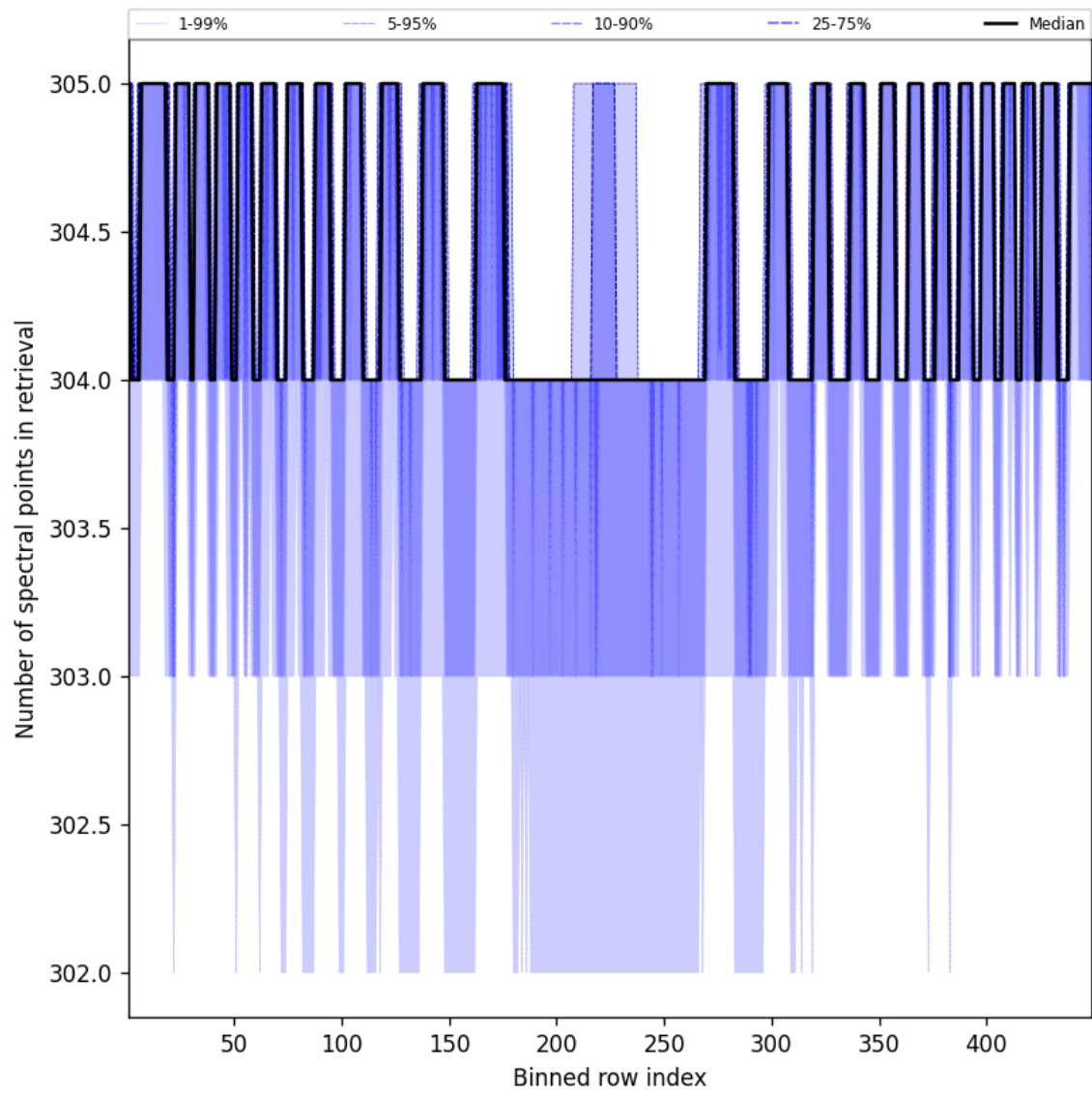
Figure 48: Along track statistics of “Number of spectral points in retrieval” for 2025-04-27 to 2025-04-27
