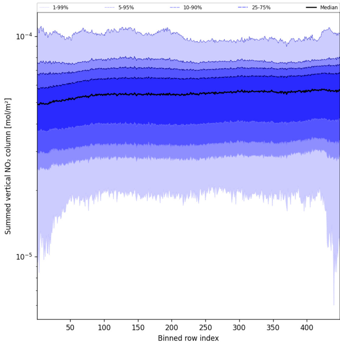
Figure 55: Along track statistics of “Summed vertical NO 2 column” for 2025-04-27 to 2025-04-27
