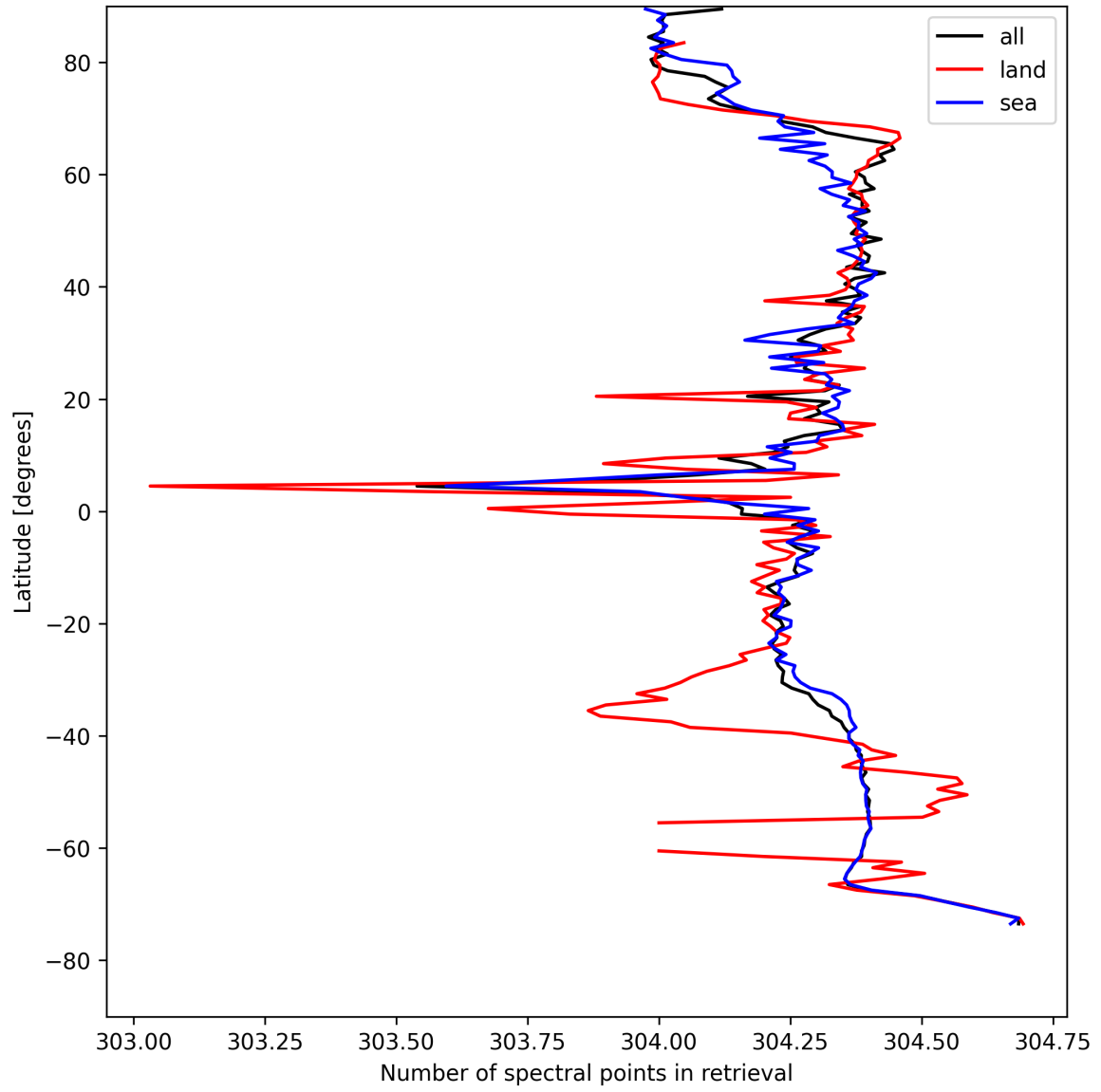
Figure 14: Zonal average of “Number of spectral points in retrieval” for 2025-04-27 to 2025-04-27.
