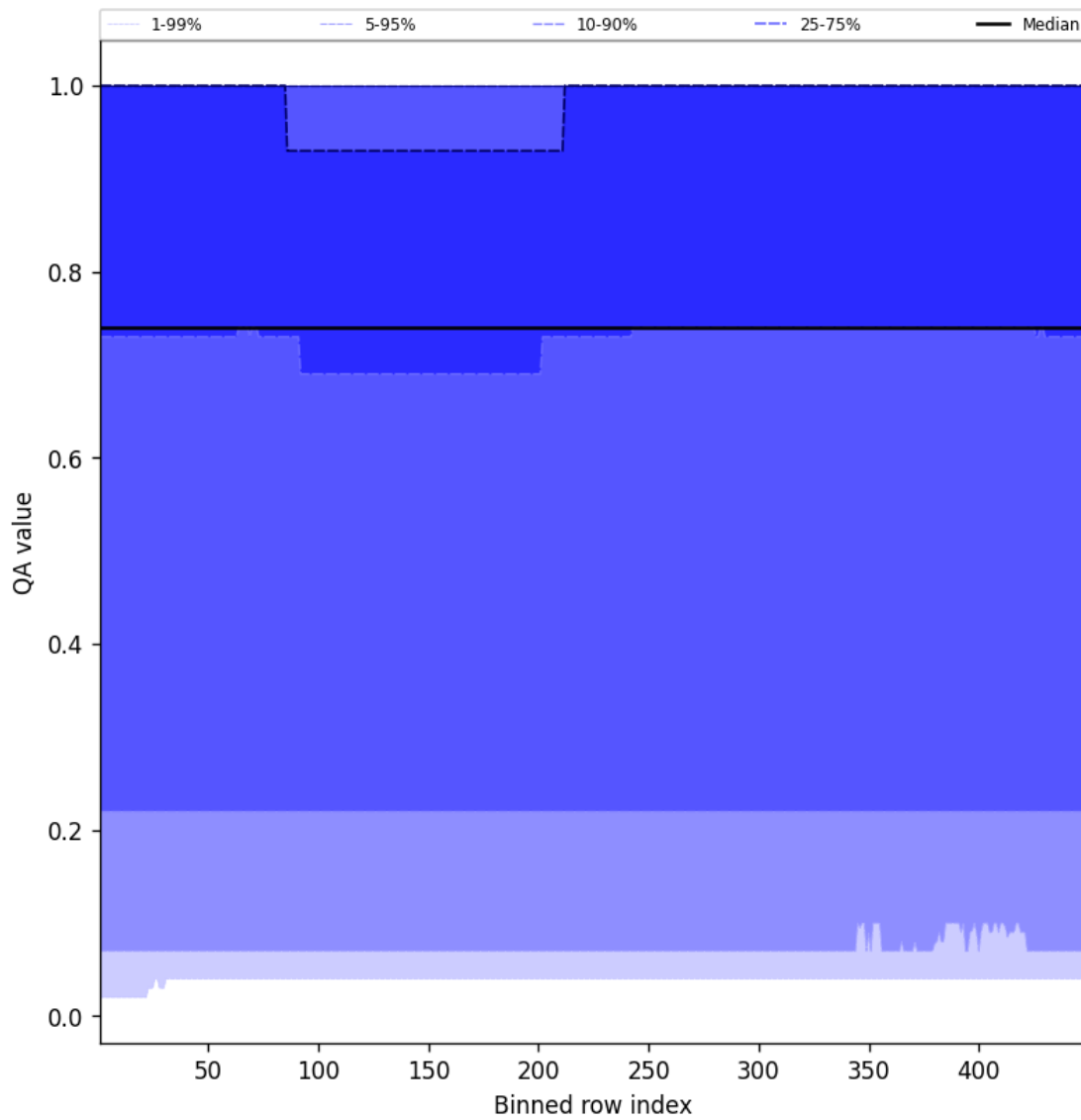
Figure 43: Along track statistics of "QA value" for 2025-04-27 to 2025-04-27
