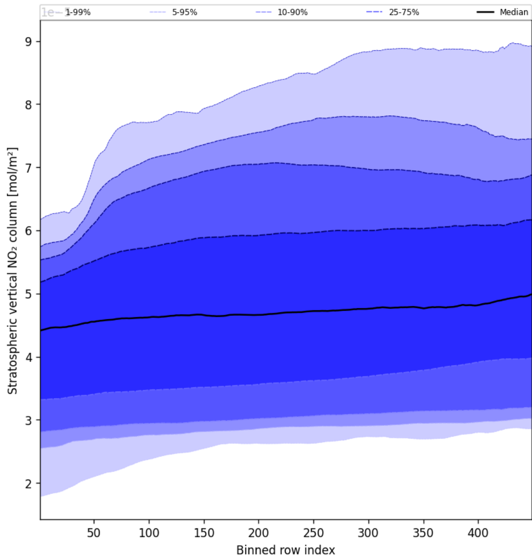
Figure 51: Along track statistics of “Stratospheric vertical NO 2 column” for 2025-04-27 to 2025-04-27
