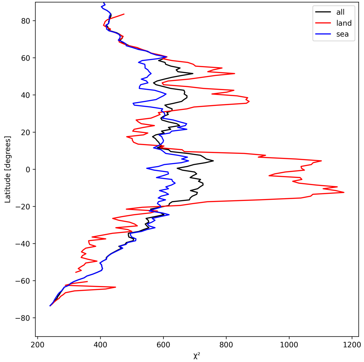
Figure 23: Zonal average of “ \chi^2 ” for 2025-04-27 to 2025-04-27.
