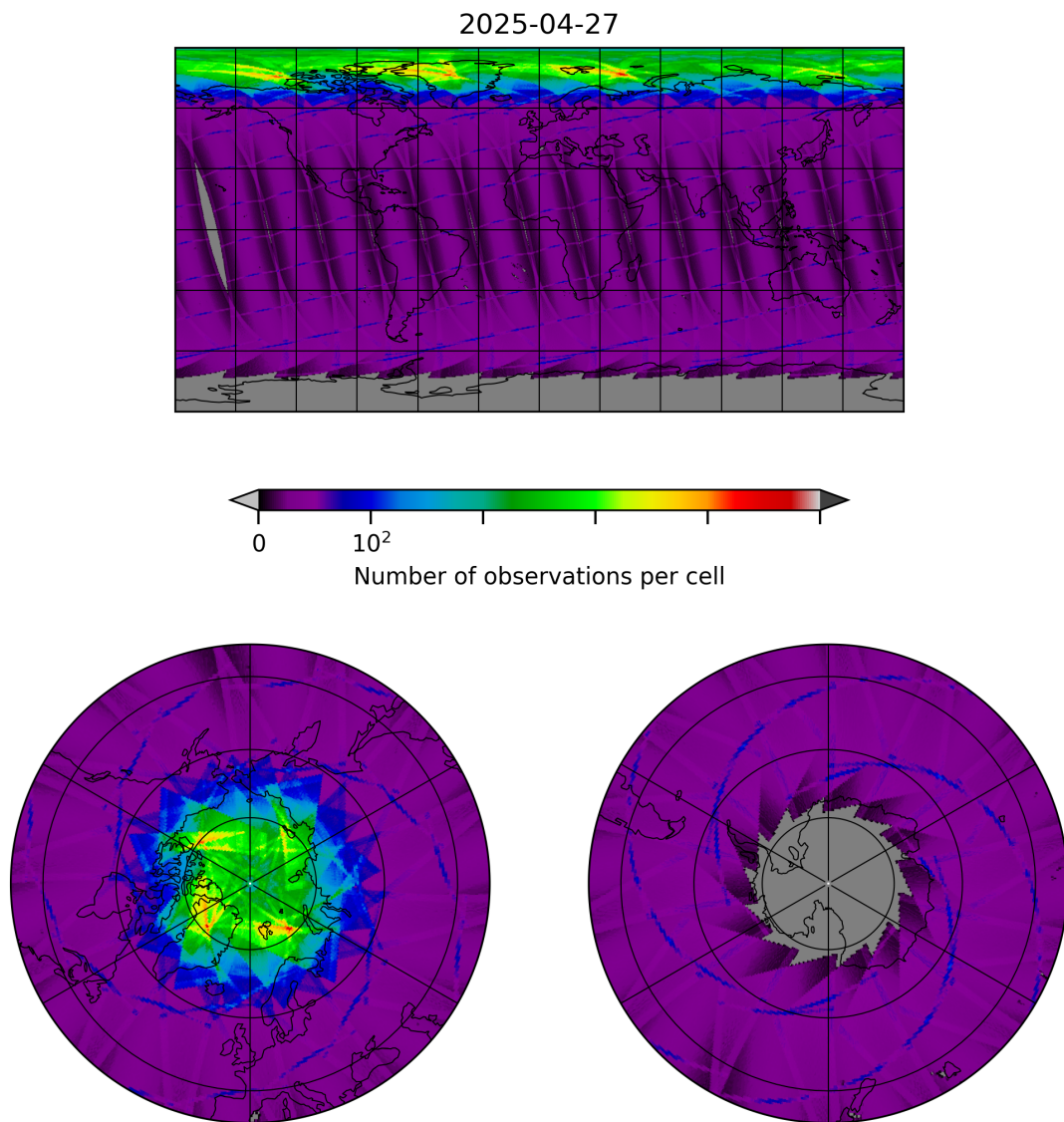
Figure 8: Map of the number of observations for 2025-04-27 to 2025-04-27
