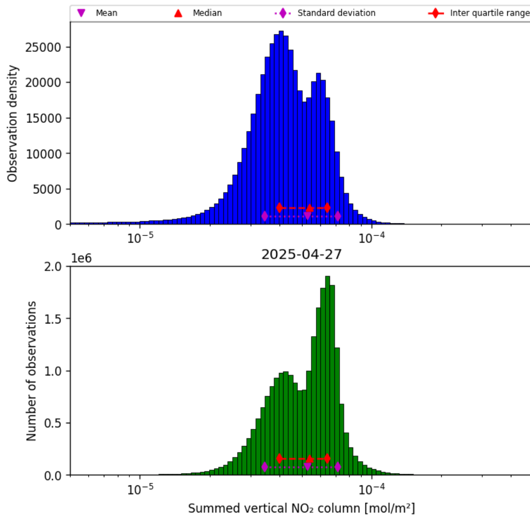
Figure 38: Histogram of “Summed vertical NO 2 column” for 2025-04-27 to 2025-04-27
