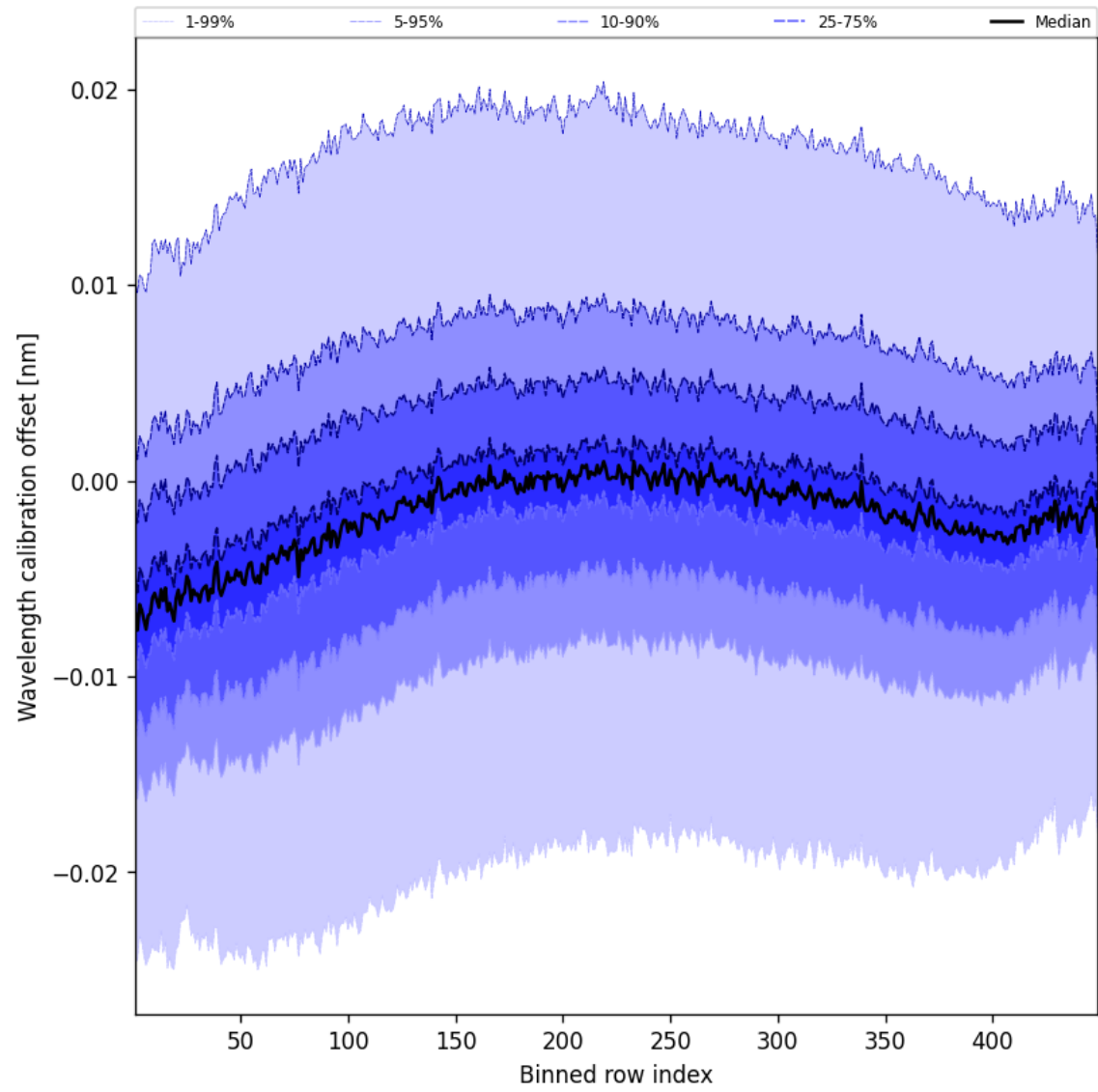
Figure 50: Along track statistics of “Wavelength calibration offset” for 2025-04-27 to 2025-04-27
