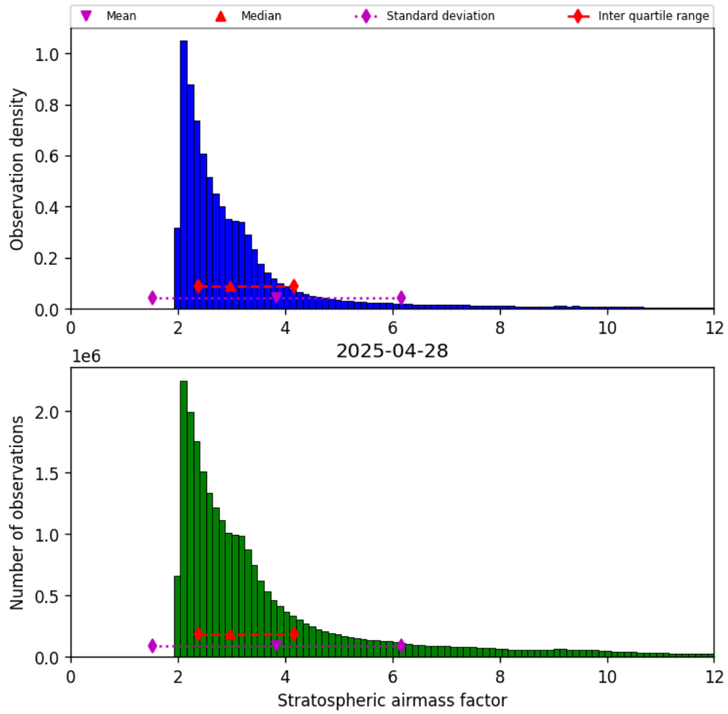
Figure 42: Histogram of “Stratospheric airmass factor” for 2025-04-28 to 2025-04-29
