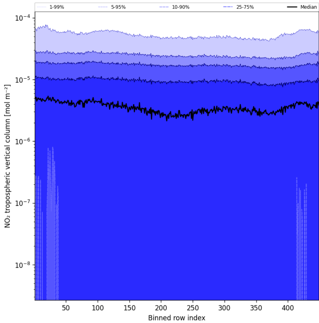
Figure 44: Along track statistics of “NO 2 tropospheric vertical column” for 2025-04-28 to 2025-04-29
