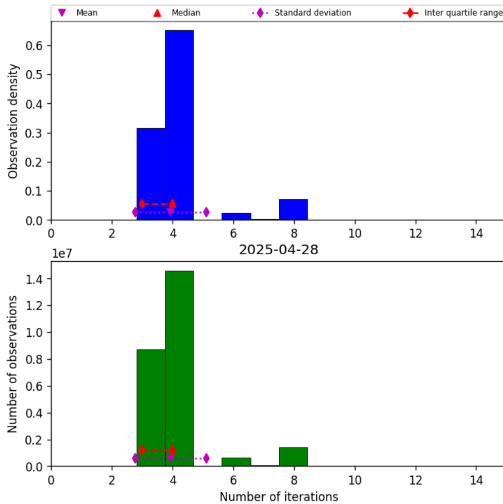
Figure 32: Histogram of “Number of iterations” for 2025-04-28 to 2025-04-29
