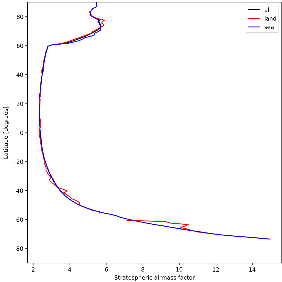
Figure 25: Zonal average of “Stratospheric air mass factor” for 2025-04-28 to 2025-04-29.
