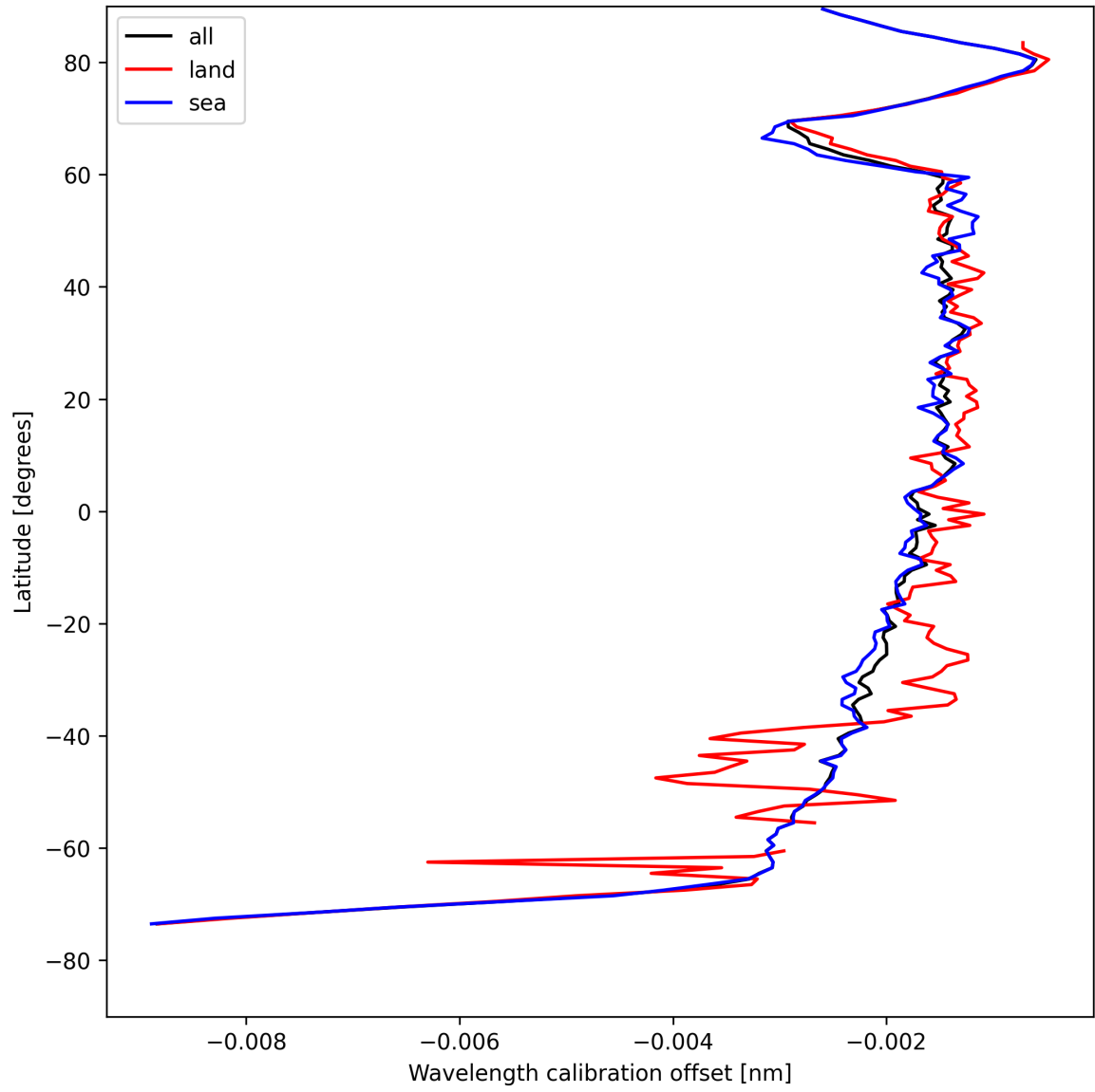
Figure 16: Zonal average of “Wavelength calibration offset” for 2025-04-28 to 2025-04-29.
