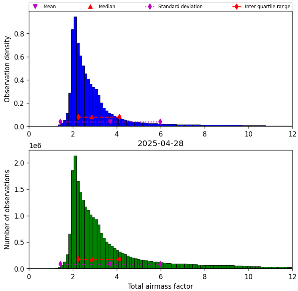
Figure 30: Histogram of “Total airmass factor” for 2025-04-28 to 2025-04-29
