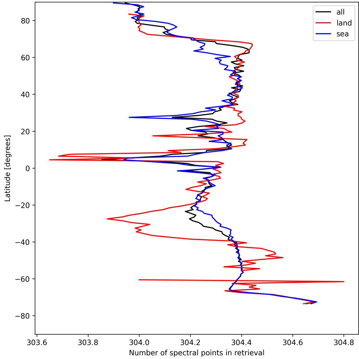
Figure 14: Zonal average of “Number of spectral points in retrieval” for 2025-04-28 to 2025-04-29.
