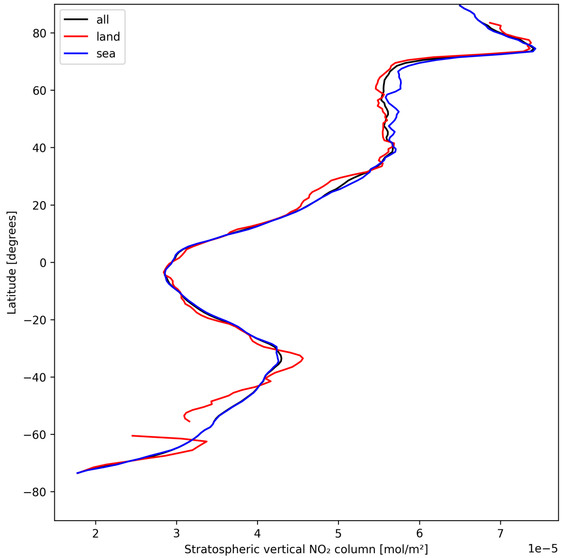
Figure 17: Zonal average of “Stratospheric vertical NO 2 column” for 2025-04-28 to 2025-04-29.
