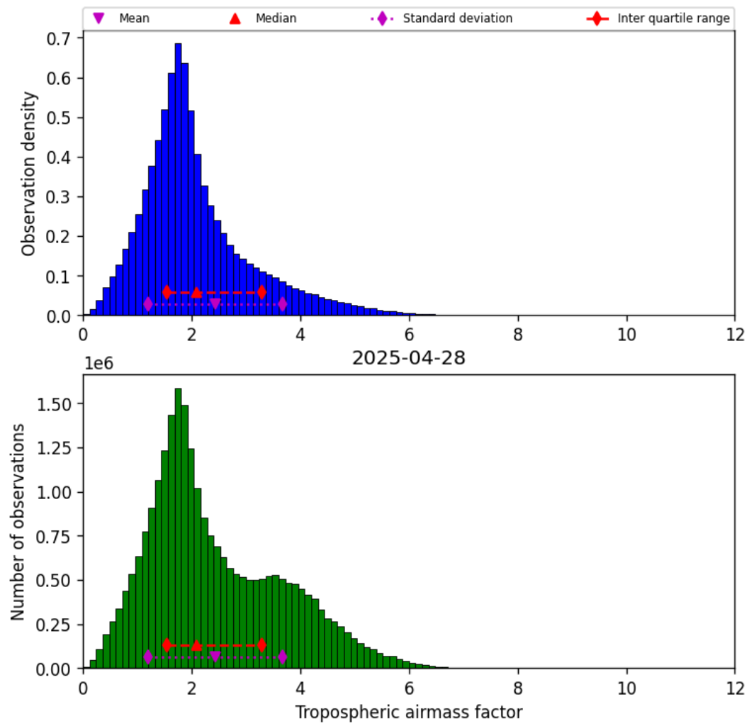
Figure 29: Histogram of “Tropospheric airmass factor” for 2025-04-28 to 2025-04-29
