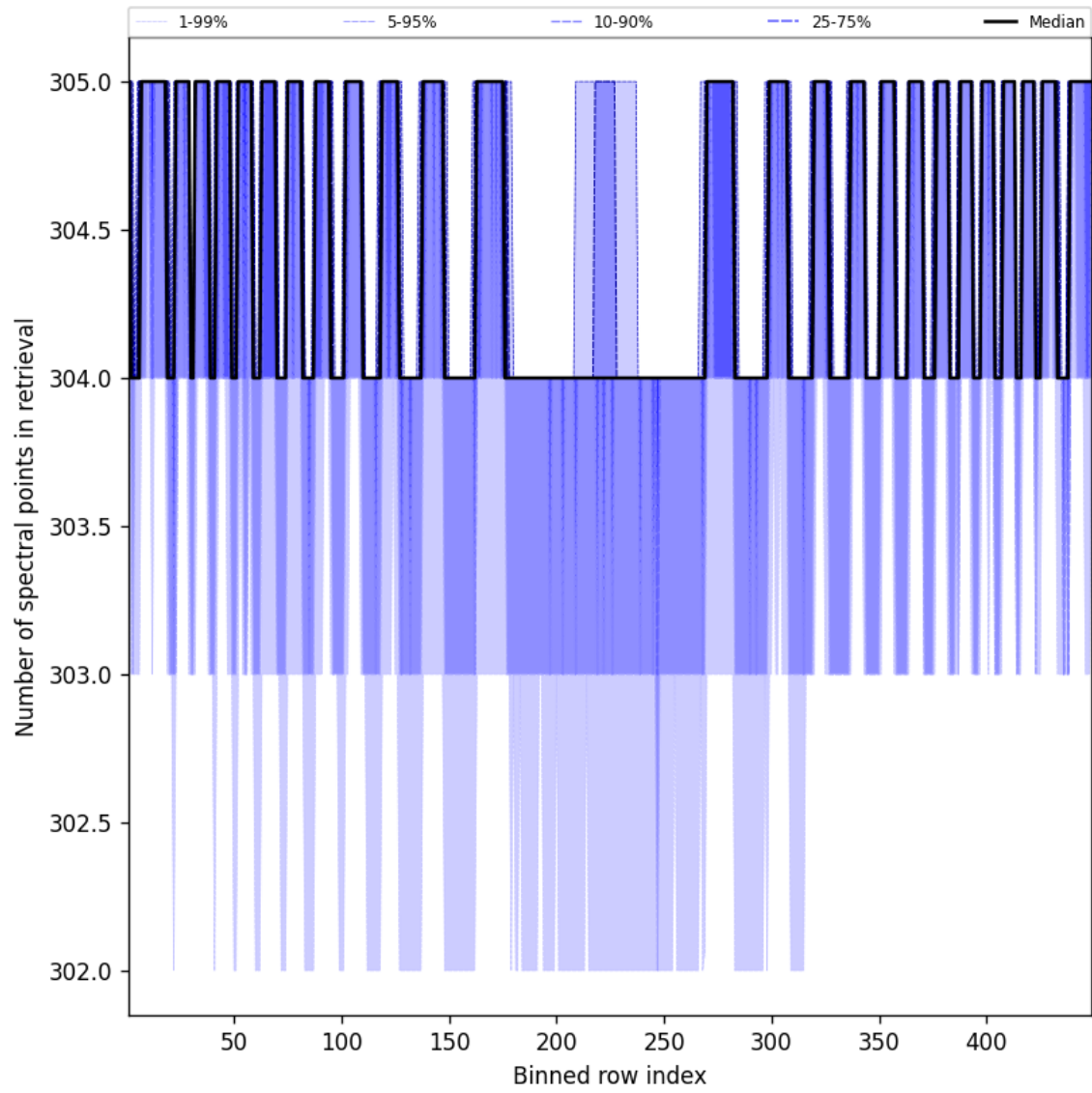
Figure 48: Along track statistics of “Number of spectral points in retrieval” for 2025-04-28 to 2025-04-29
