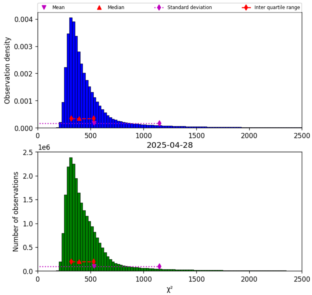
Figure 40: Histogram of “ \chi^2 ” for 2025-04-28 to 2025-04-29
