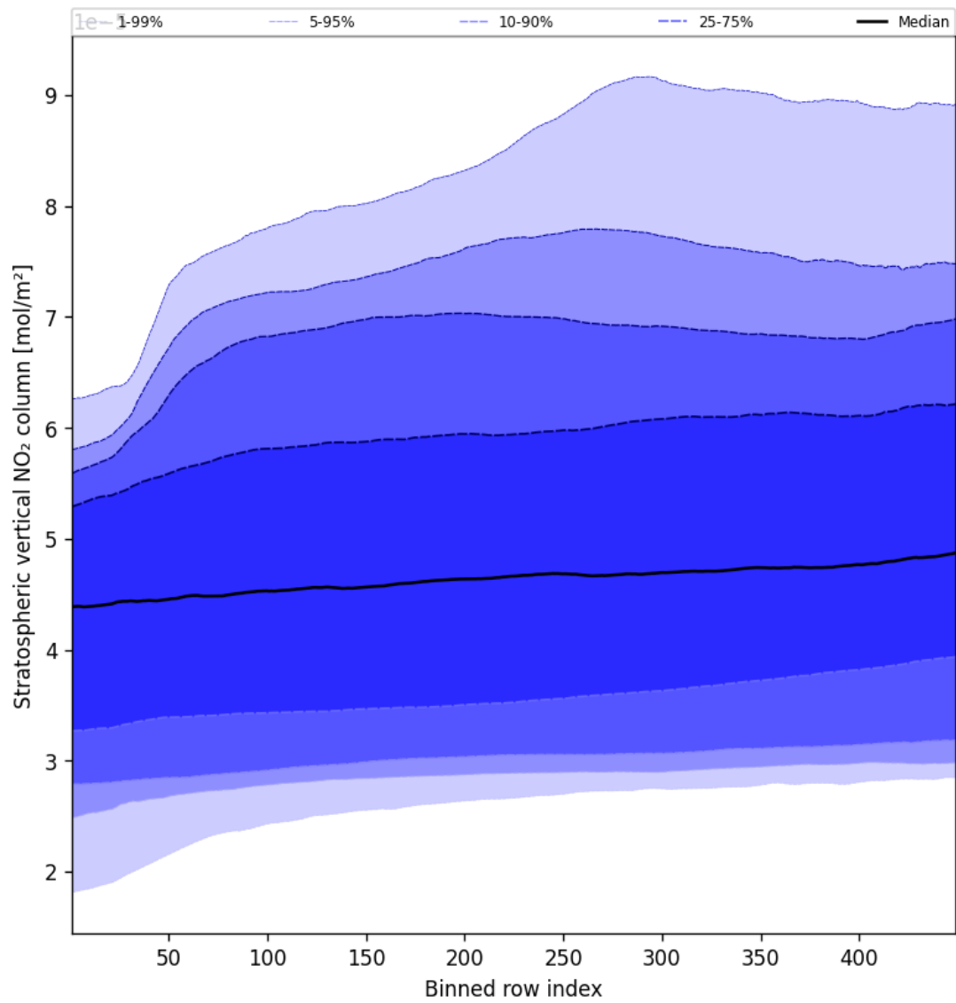
Figure 51: Along track statistics of “Stratospheric vertical NO 2 column” for 2025-04-28 to 2025-04-29
