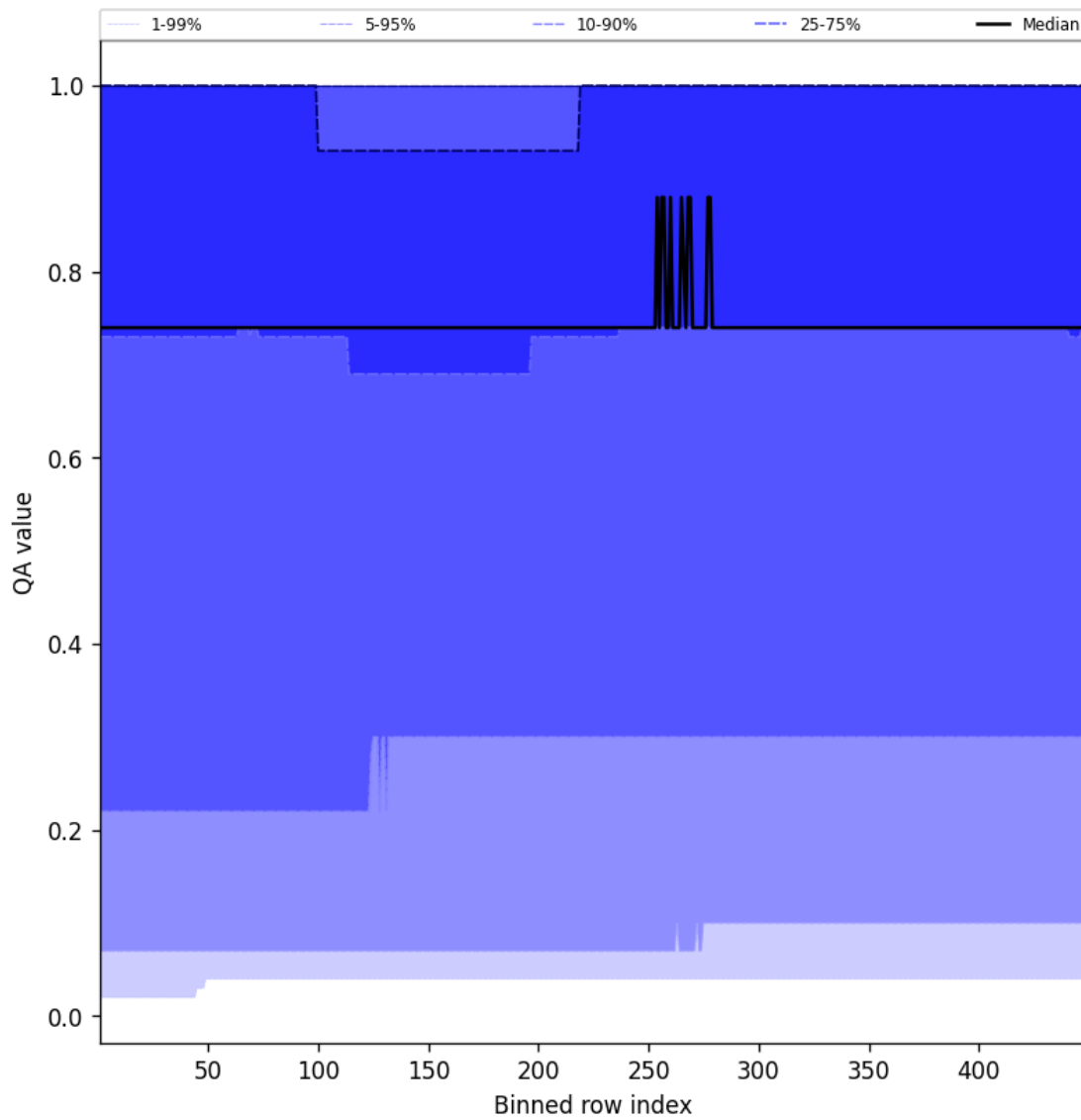
Figure 43: Along track statistics of “QA value” for 2025-04-28 to 2025-04-29
