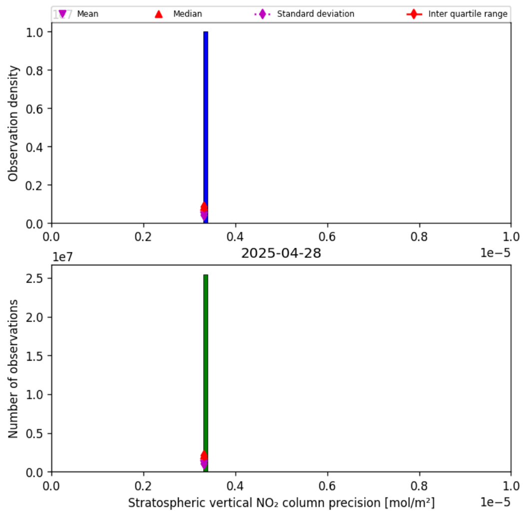
Figure 35: Histogram of “Stratospheric vertical NO 2 column precision” for 2025-04-28 to 2025-04-29
