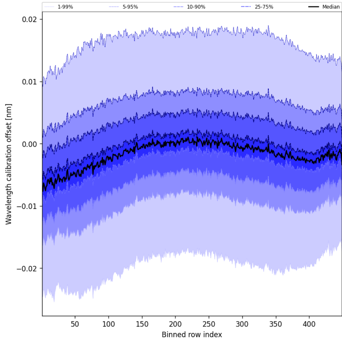
Figure 50: Along track statistics of “Wavelength calibration offset” for 2025-04-28 to 2025-04-29
