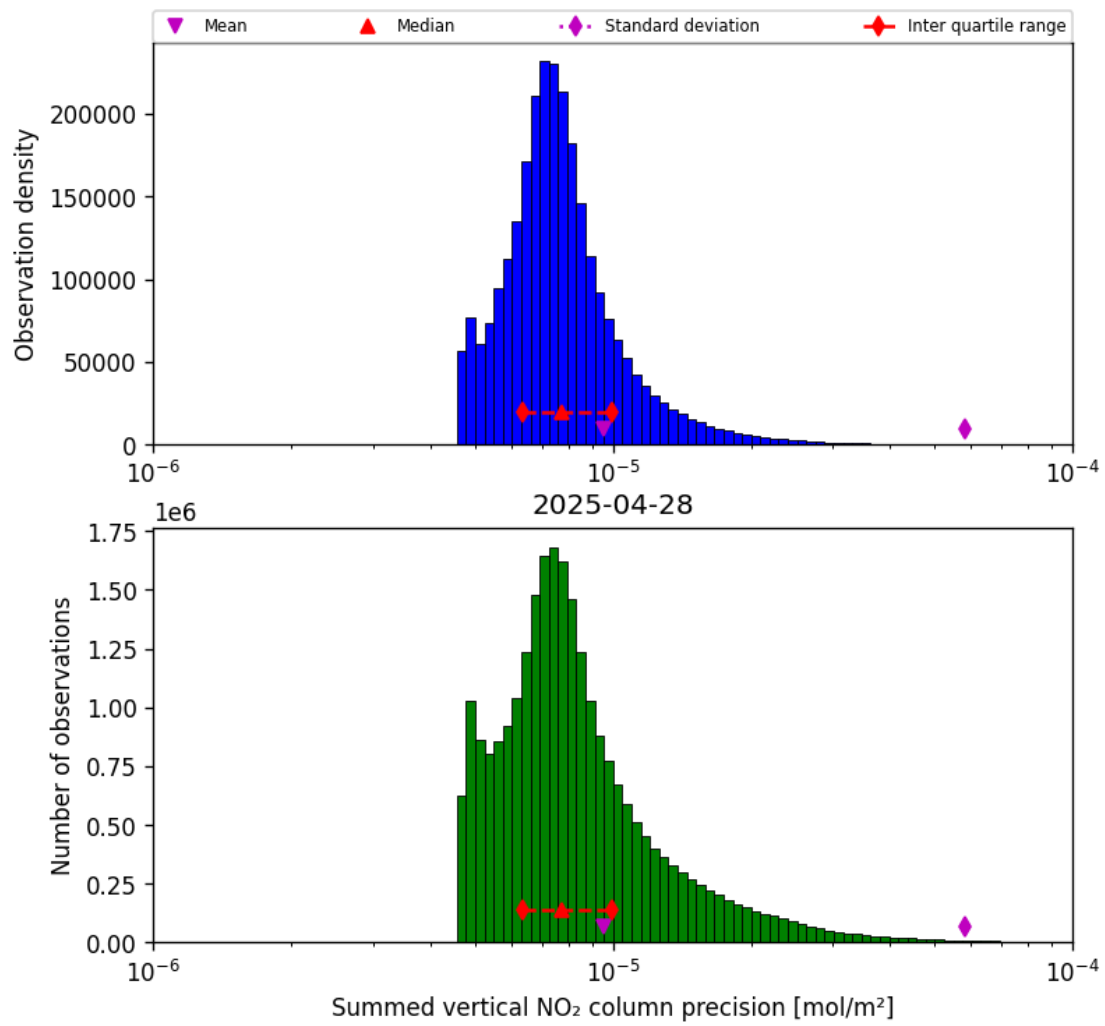
Figure 39: Histogram of “Summed vertical NO 2 column precision” for 2025-04-28 to 2025-04-29
