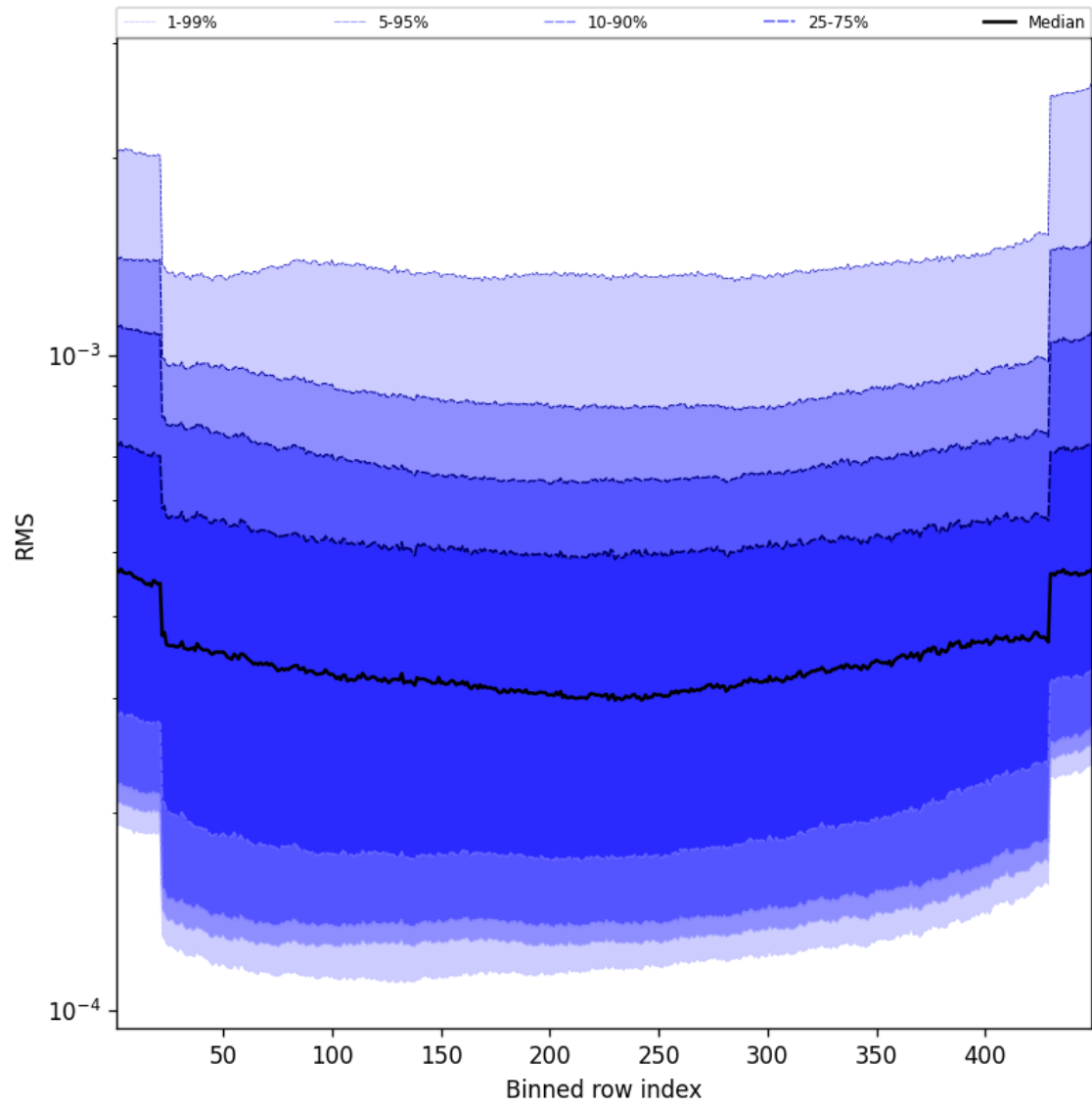
Figure 58: Along track statistics of “RMS” for 2025-04-28 to 2025-04-29
