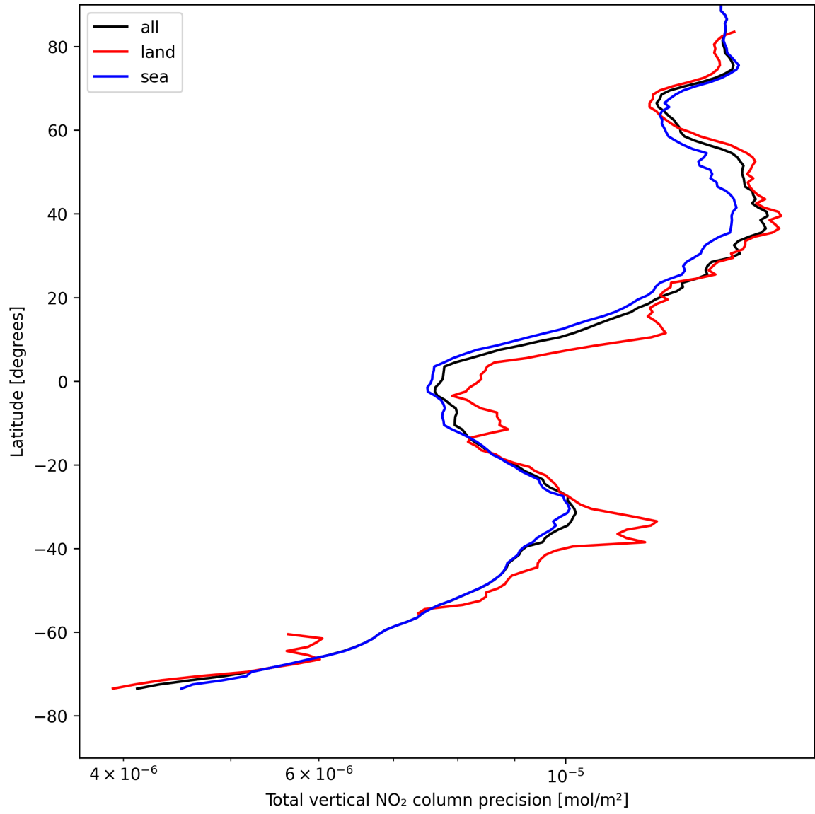
Figure 20: Zonal average of “Total vertical NO 2 column precision” for 2025-04-28 to 2025-04-29.
