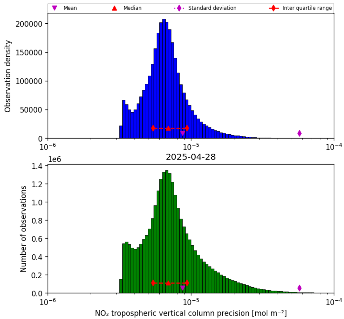
Figure 28: Histogram of “NO 2 tropospheric vertical column precision” for 2025-04-28 to 2025-04-29
