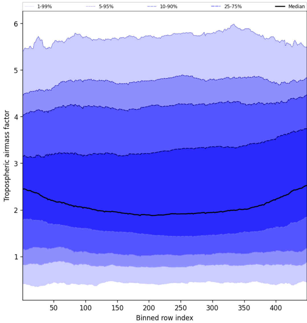
Figure 46: Along track statistics of "Tropospheric airmass factor" for 2025-04-28 to 2025-04-29
