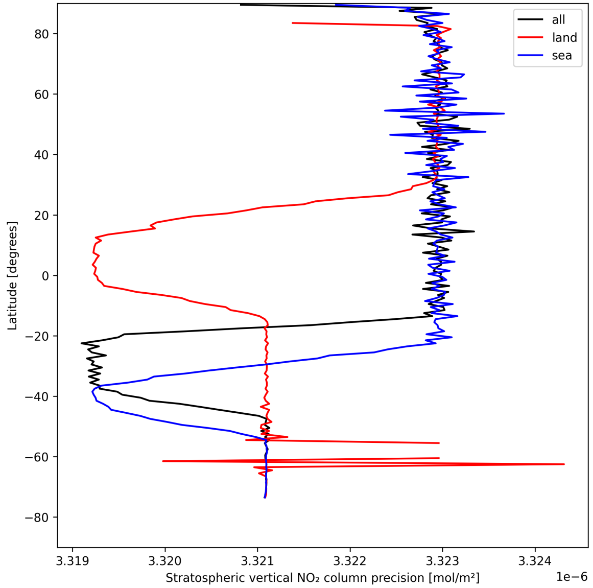
Figure 18: Zonal average of “Stratospheric vertical NO 2 column precision” for 2025-04-28 to 2025-04-29.
