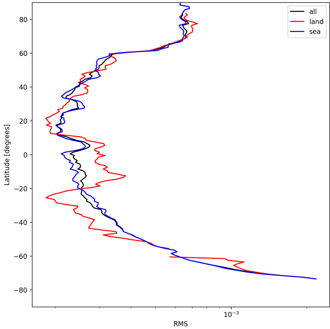
Figure 24: Zonal average of “RMS” for 2025-04-28 to 2025-04-29.
