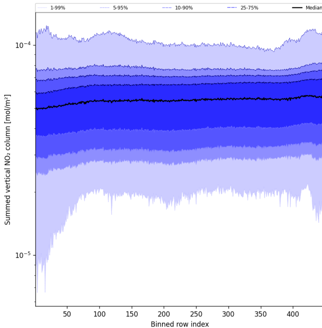
Figure 55: Along track statistics of “Summed vertical NO 2 column” for 2025-04-28 to 2025-04-29
