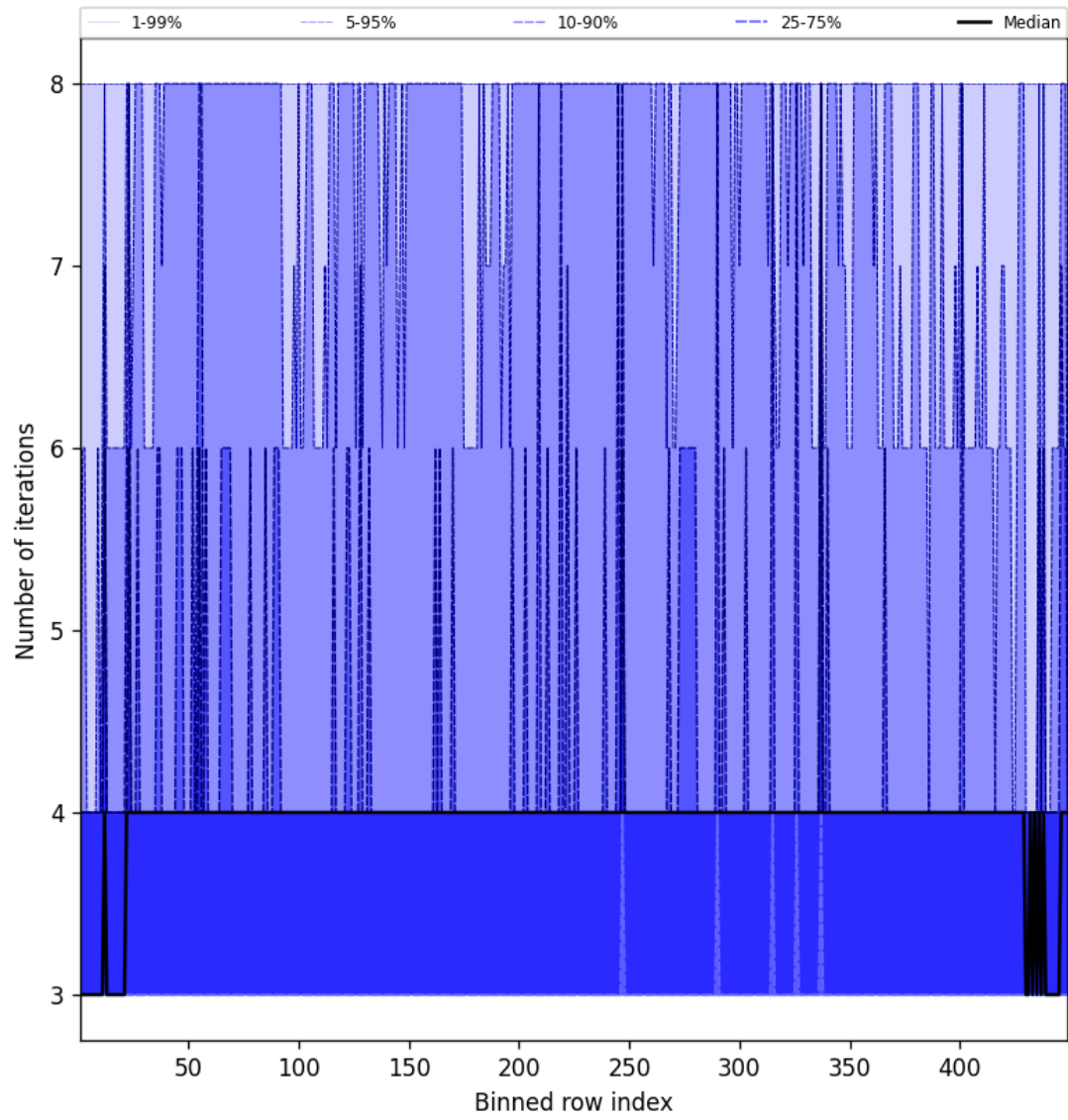
Figure 49: Along track statistics of “Number of iterations” for 2025-04-28 to 2025-04-29
