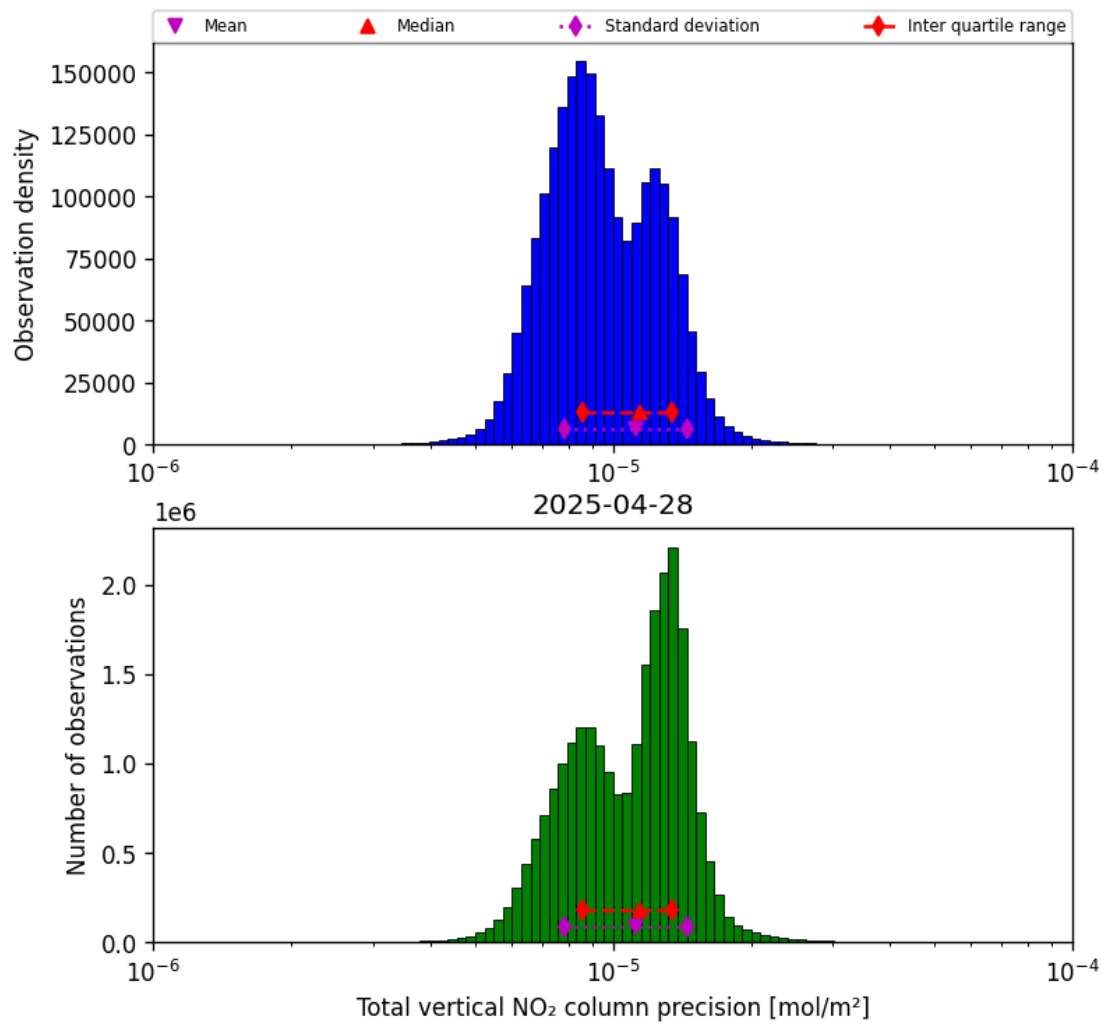
Figure 37: Histogram of "Total vertical NO 2 column precision" for 2025-04-28 to 2025-04-29
