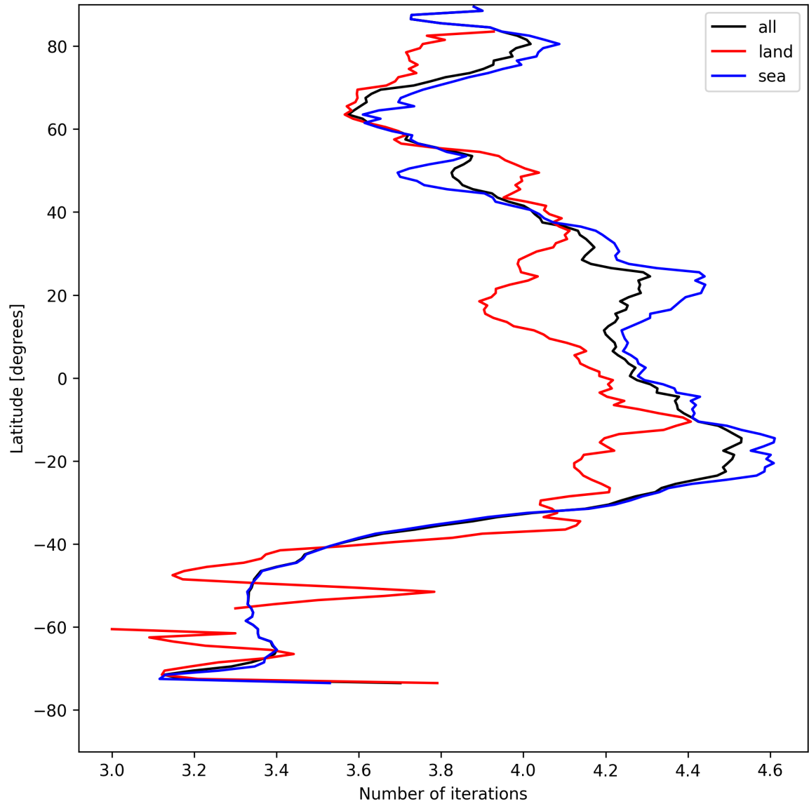
Figure 15: Zonal average of “Number of iterations” for 2025-04-28 to 2025-04-29.
