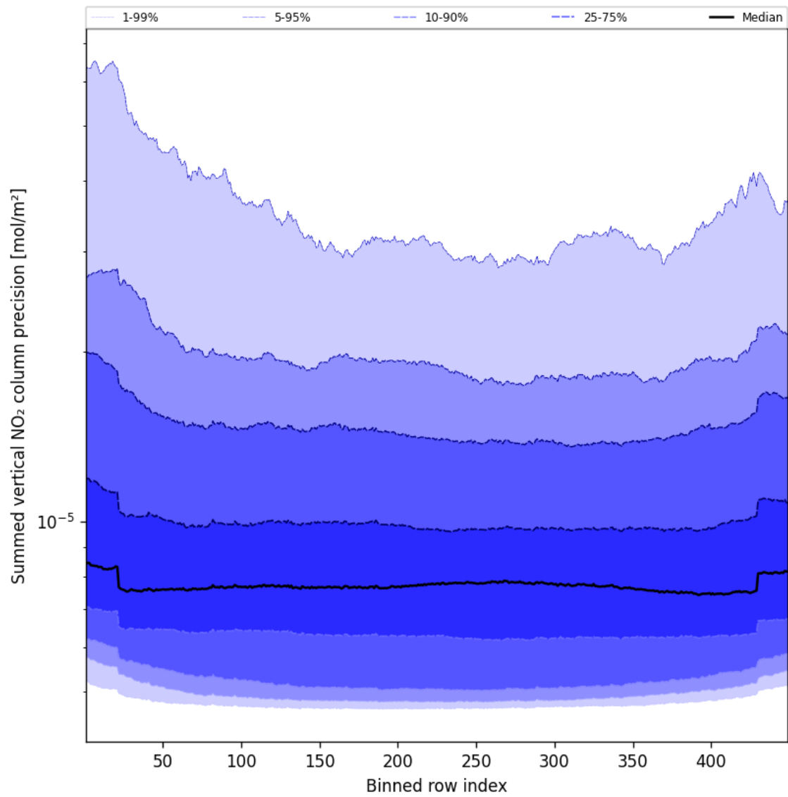
Figure 56: Along track statistics of “Summed vertical NO 2 column precision” for 2025-04-28 to 2025-04-29
