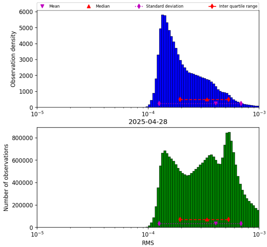
Figure 41: Histogram of “RMS” for 2025-04-28 to 2025-04-29
