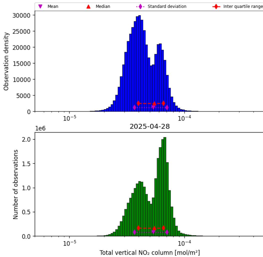
Figure 36: Histogram of "Total vertical NO 2 column" for 2025-04-28 to 2025-04-29
