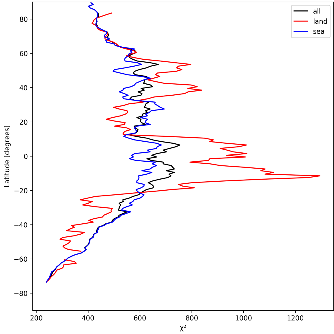
Figure 23: Zonal average of “ \chi^2 ” for 2025-04-28 to 2025-04-29.
