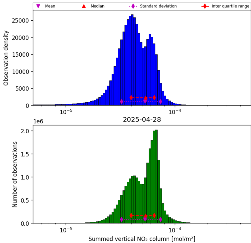
Figure 38: Histogram of “Summed vertical NO 2 column” for 2025-04-28 to 2025-04-29
