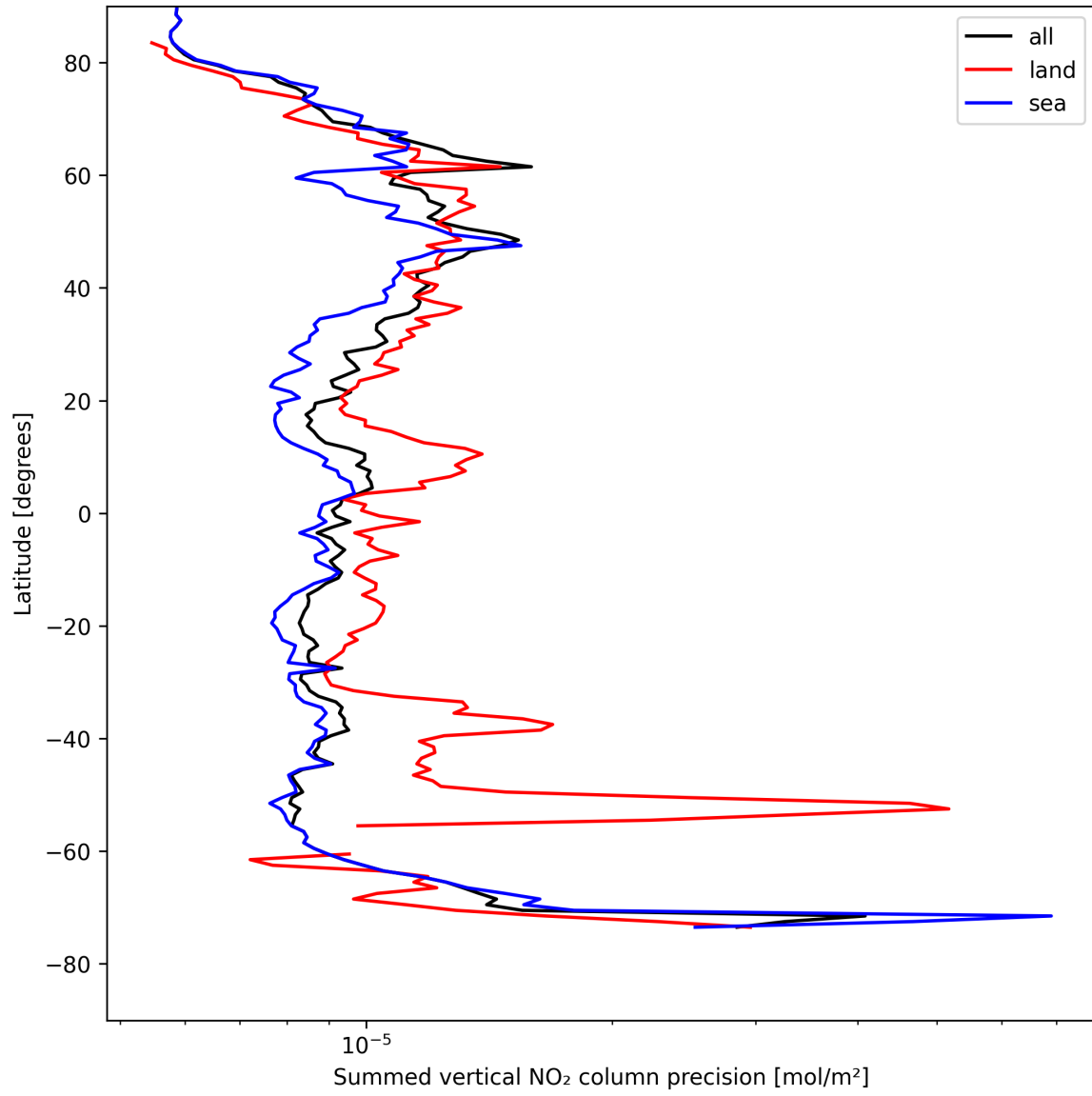
Figure 22: Zonal average of “Summed vertical NO 2 column precision” for 2025-04-28 to 2025-04-29.
