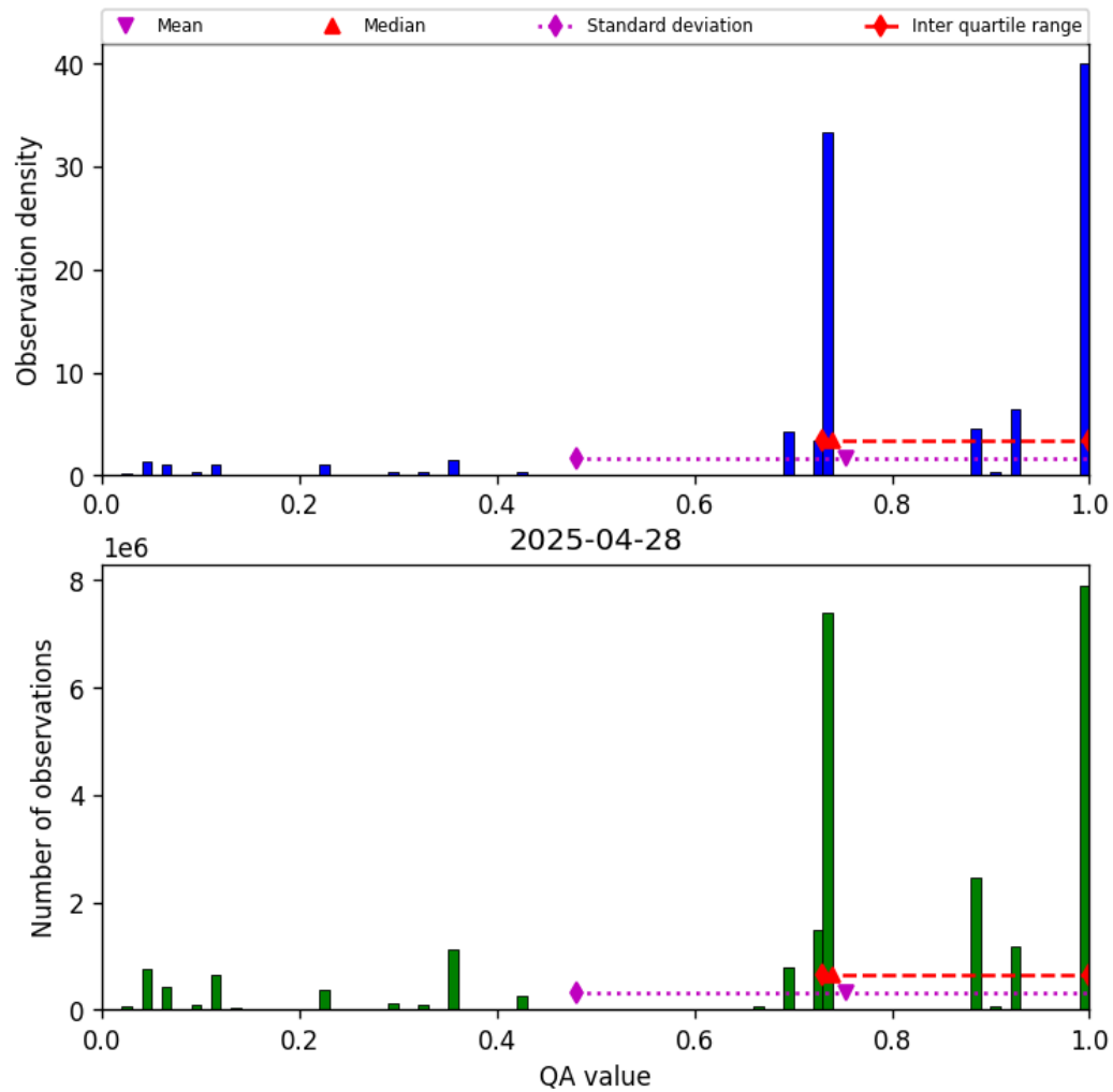
Figure 26: Histogram of “QA value” for 2025-04-28 to 2025-04-29
