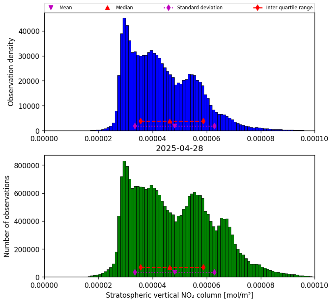
Figure 34: Histogram of “Stratospheric vertical NO 2 column” for 2025-04-28 to 2025-04-29
