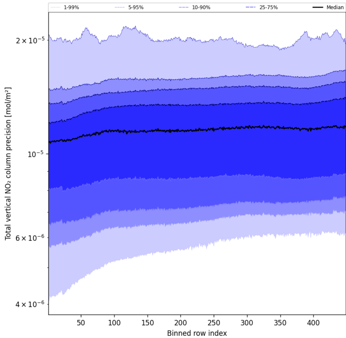
Figure 54: Along track statistics of “Total vertical NO 2 column precision” for 2025-04-28 to 2025-04-29
