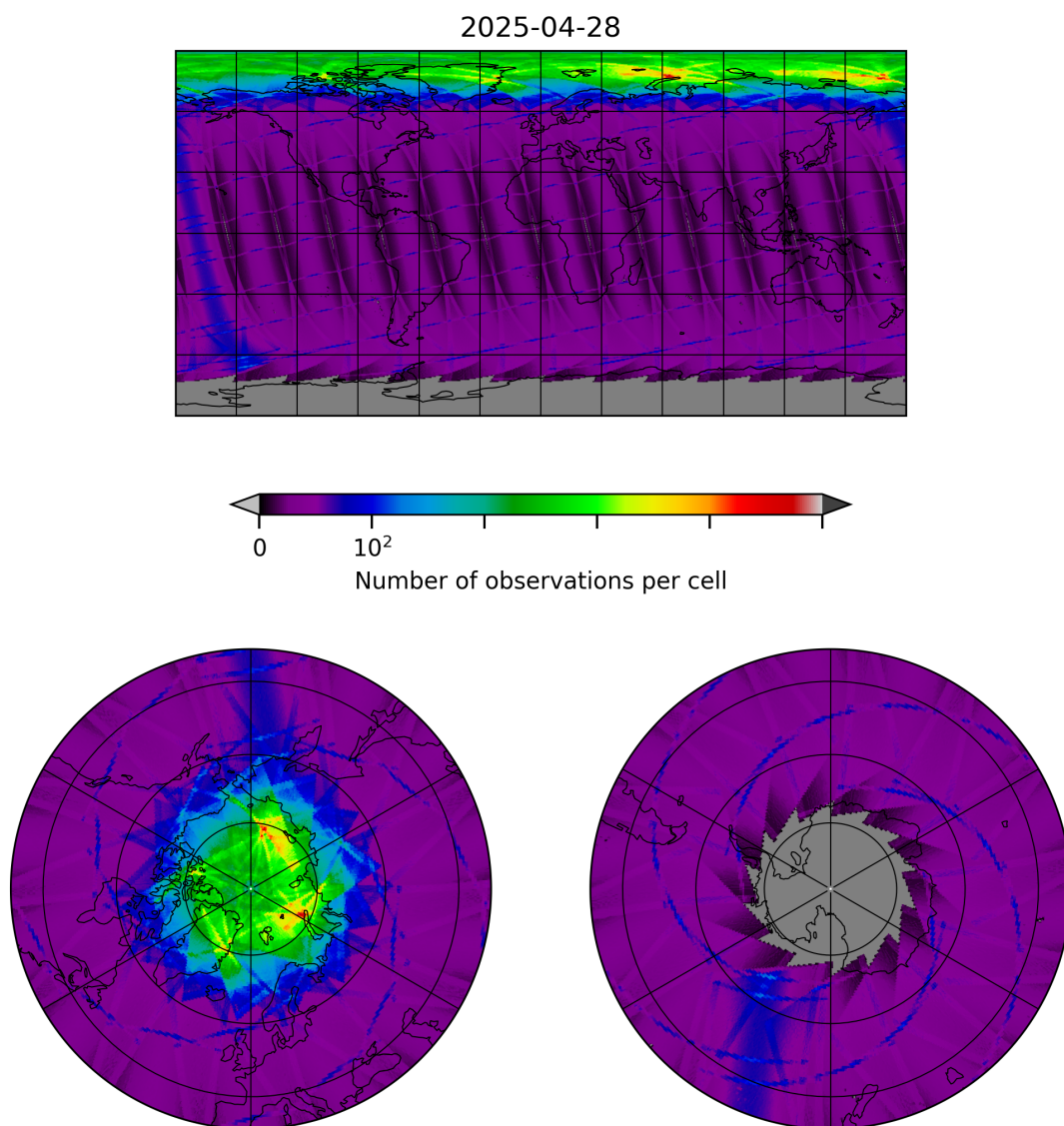
Figure 8: Map of the number of observations for 2025-04-28 to 2025-04-29
