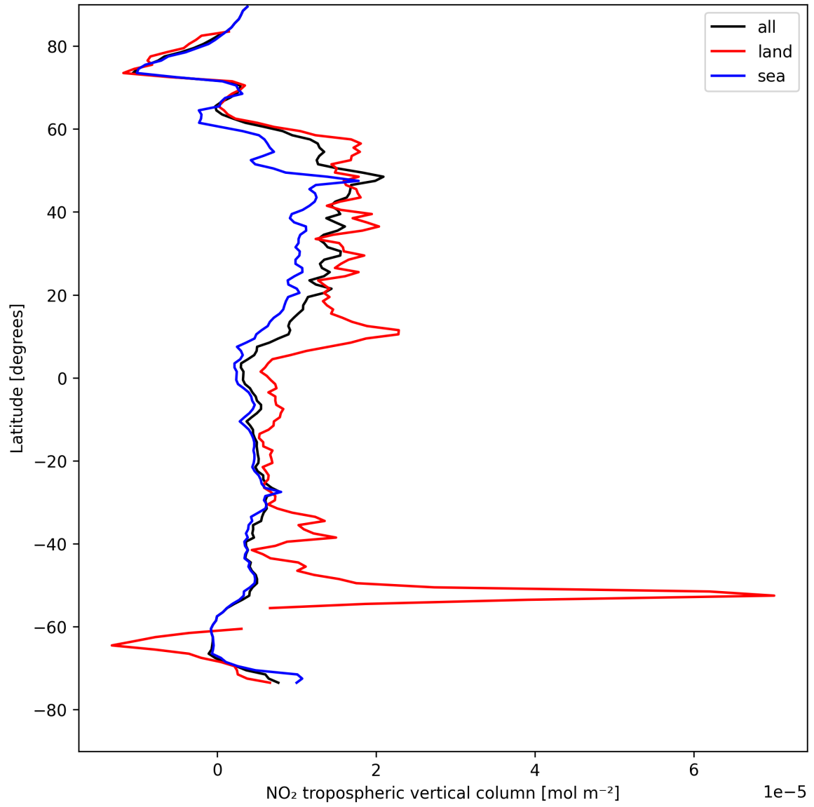
Figure 10: Zonal average of “NO 2 tropospheric vertical column” for 2025-04-28 to 2025-04-29.
