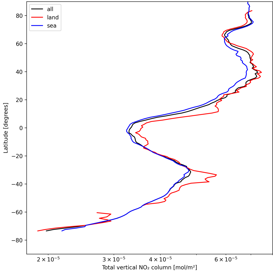
Figure 19: Zonal average of “Total vertical NO 2 column” for 2025-04-28 to 2025-04-29.
