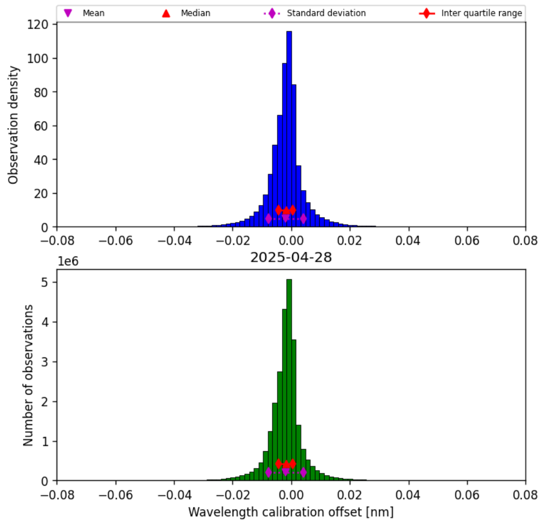
Figure 33: Histogram of “Wavelength calibration offset” for 2025-04-28 to 2025-04-29
