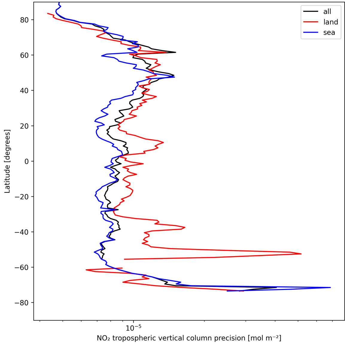
Figure 11: Zonal average of “NO 2 tropospheric vertical column precision” for 2025-04-28 to 2025-04-29.
