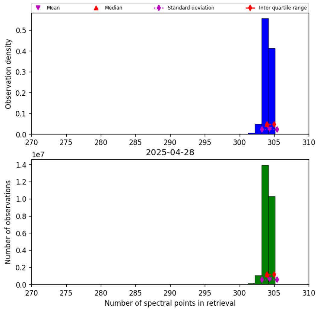
Figure 31: Histogram of “Number of spectral points in retrieval” for 2025-04-28 to 2025-04-29
