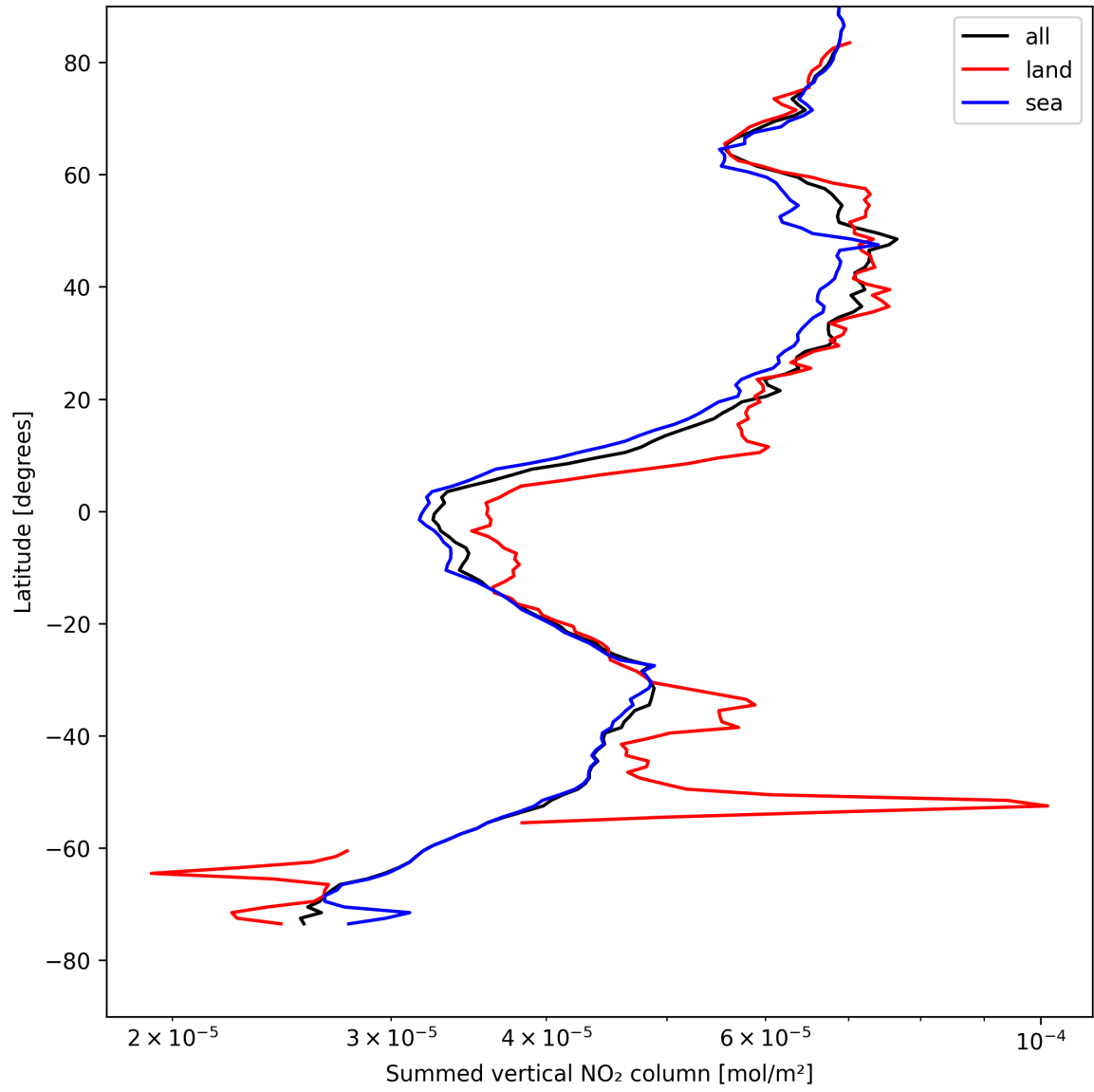
Figure 21: Zonal average of “Summed vertical NO 2 column” for 2025-04-28 to 2025-04-29.
