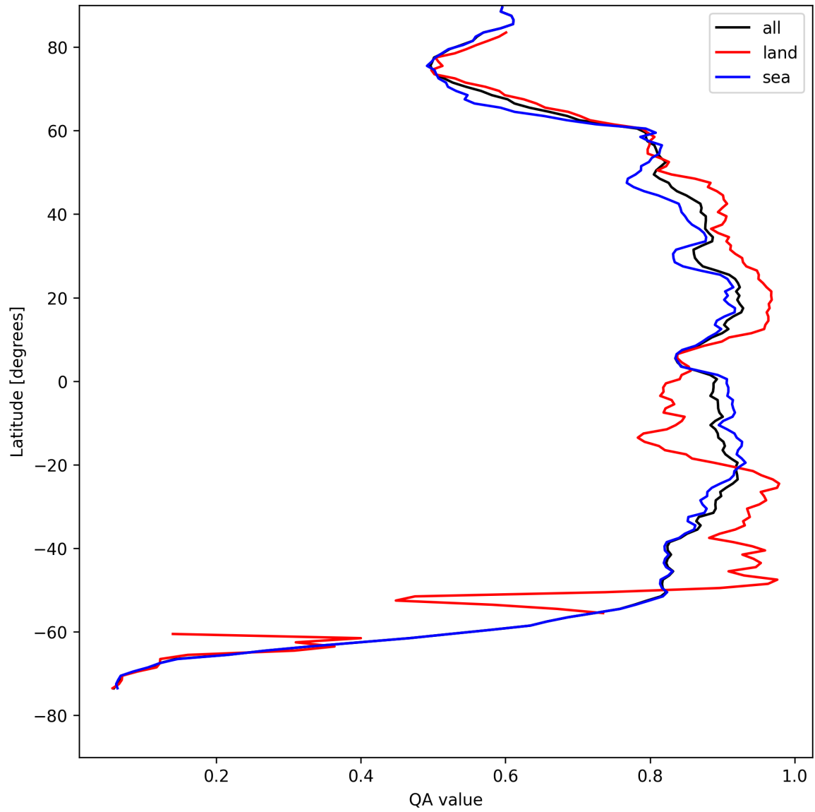
Figure 9: Zonal average of “QA value” for 2025-04-28 to 2025-04-29.
