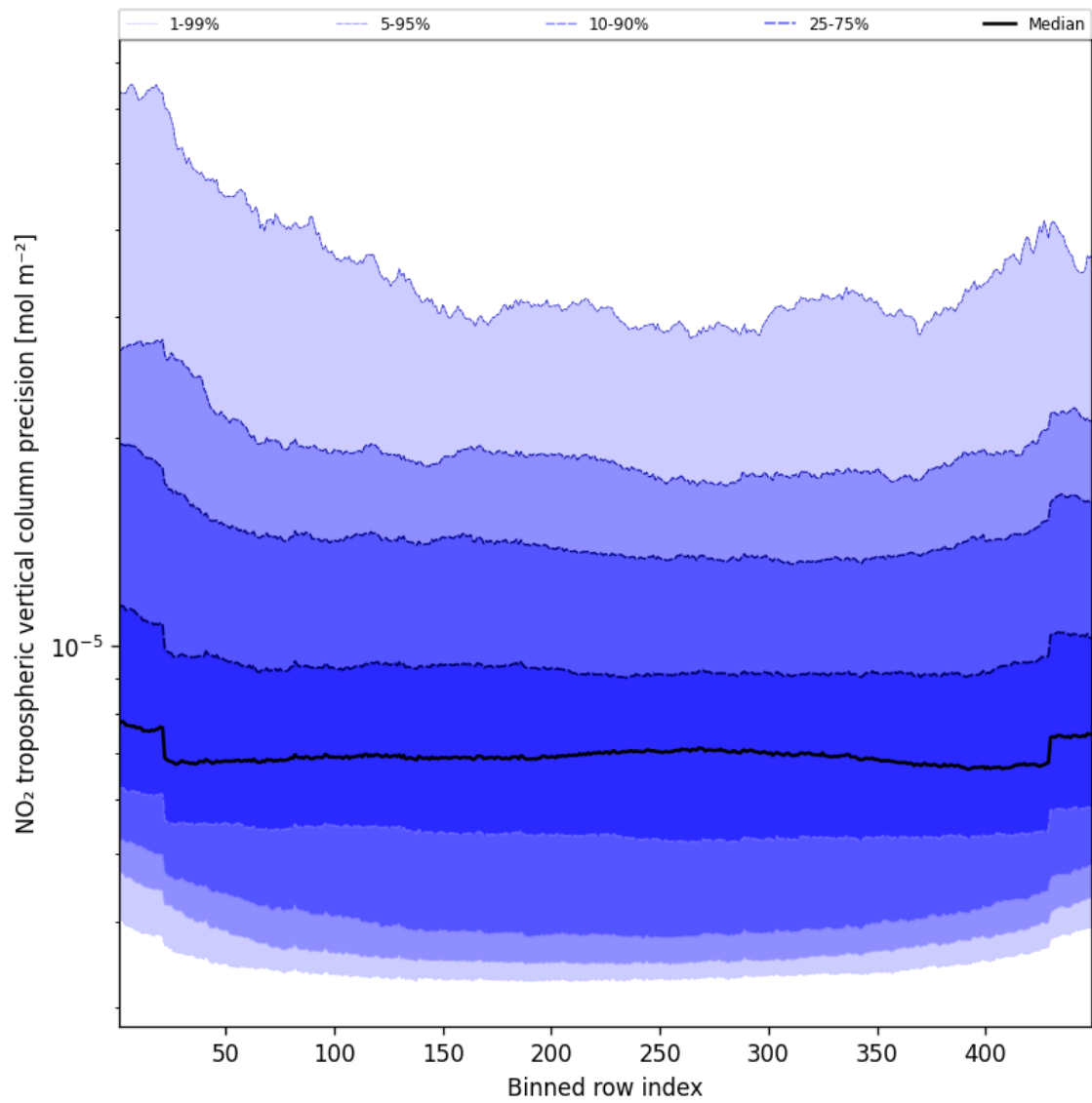
Figure 45: Along track statistics of “NO 2 tropospheric vertical column precision” for 2025-04-28 to 2025-04-29
