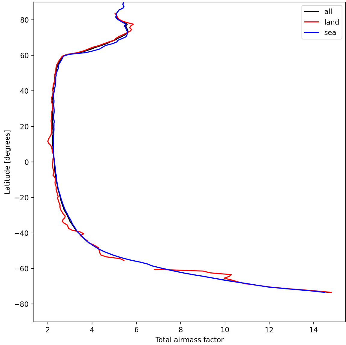
Figure 13: Zonal average of “Total airmass factor” for 2025-04-28 to 2025-04-29.
