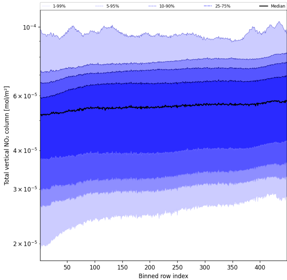
Figure 53: Along track statistics of “Total vertical NO 2 column” for 2025-04-28 to 2025-04-29
