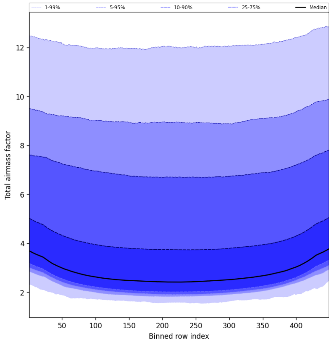
Figure 47: Along track statistics of “Total airmass factor” for 2025-04-28 to 2025-04-29
