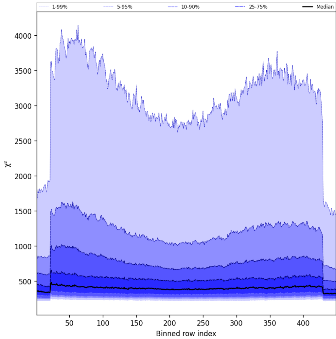
Figure 57: Along track statistics of “ \chi^2 ” for 2025-04-28 to 2025-04-29
