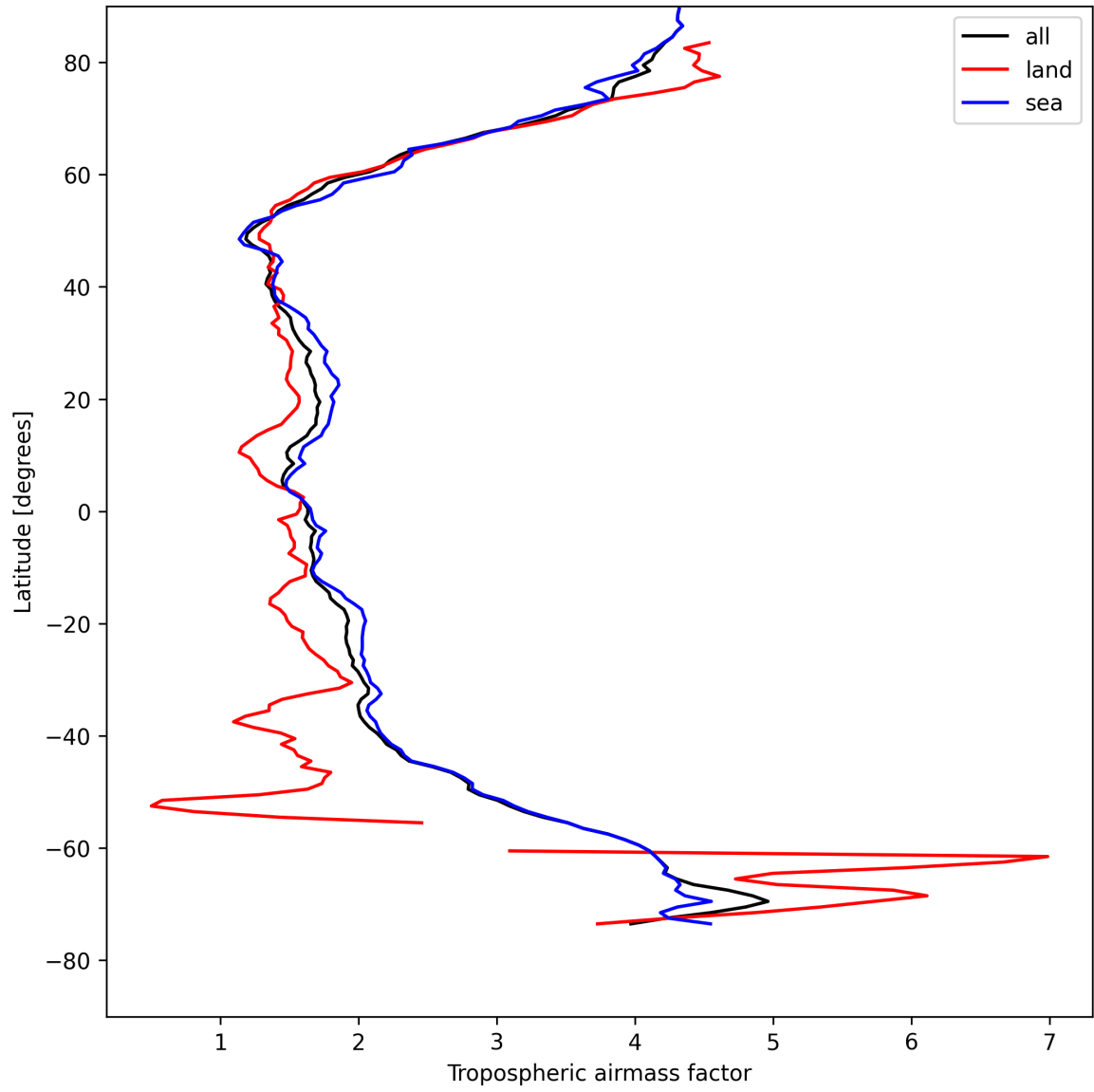
Figure 12: Zonal average of “Tropospheric air mass factor” for 2025-04-28 to 2025-04-29.
