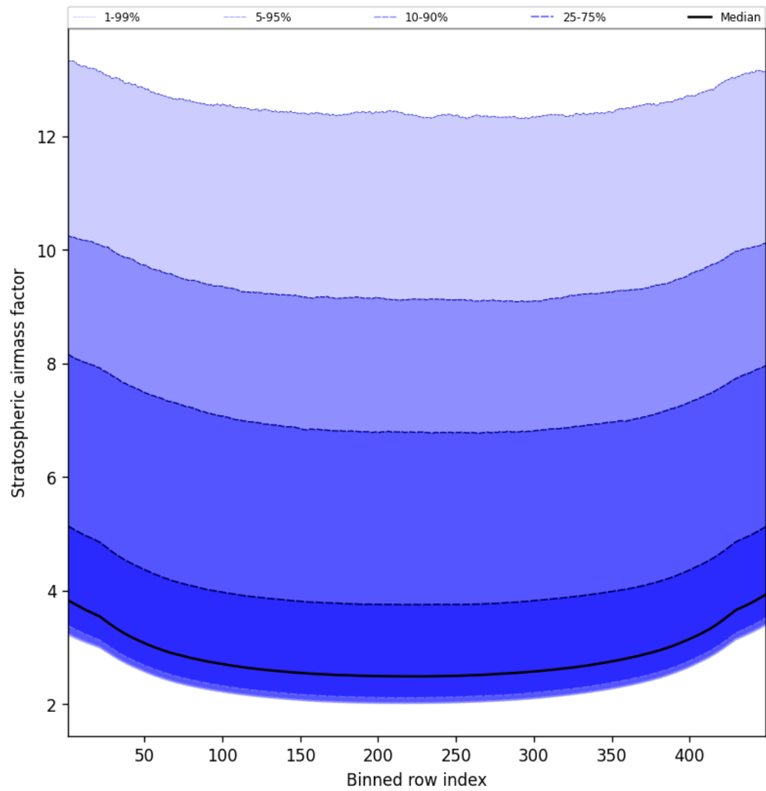
Figure 59: Along track statistics of “Stratospheric airmass factor” for 2025-04-28 to 2025-04-29
