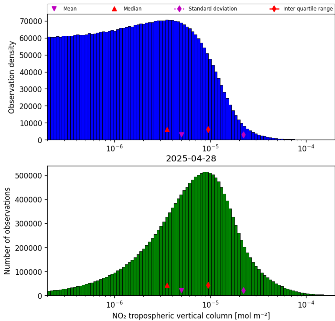
Figure 27: Histogram of “NO 2 tropospheric vertical column” for 2025-04-28 to 2025-04-29
