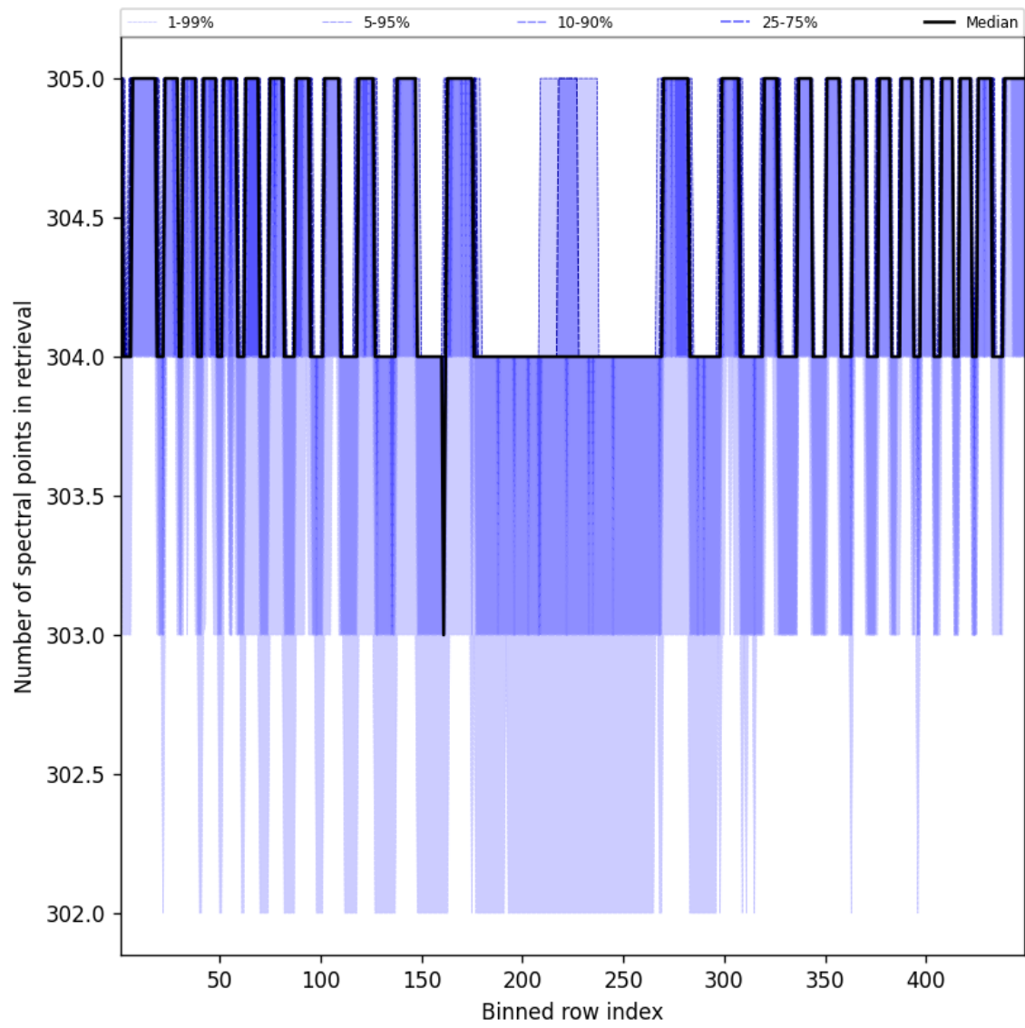
Figure 48: Along track statistics of “Number of spectral points in retrieval” for 2025-04-29 to 2025-04-30
