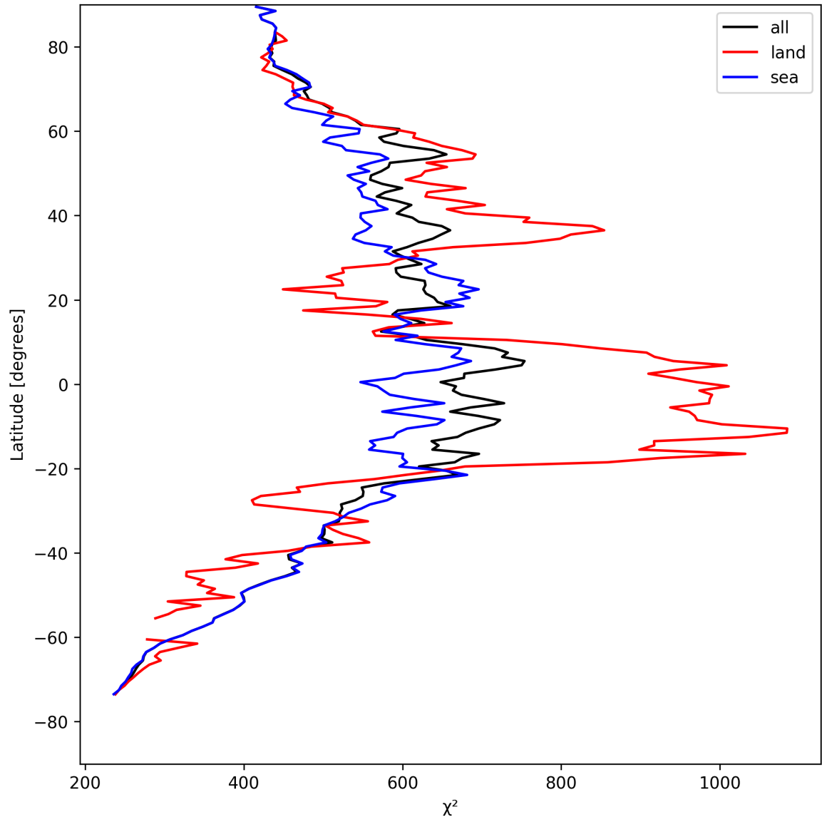
Figure 23: Zonal average of “ \chi^2 ” for 2025-04-29 to 2025-04-30.
