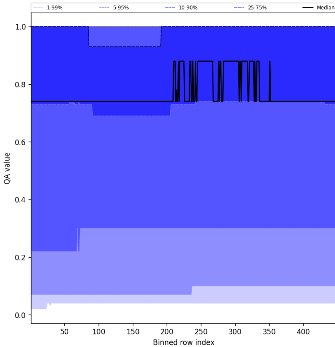
Figure 43: Along track statistics of “QA value” for 2025-04-29 to 2025-04-30
