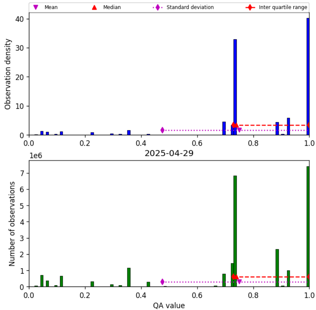
Figure 26: Histogram of “QA value” for 2025-04-29 to 2025-04-30
