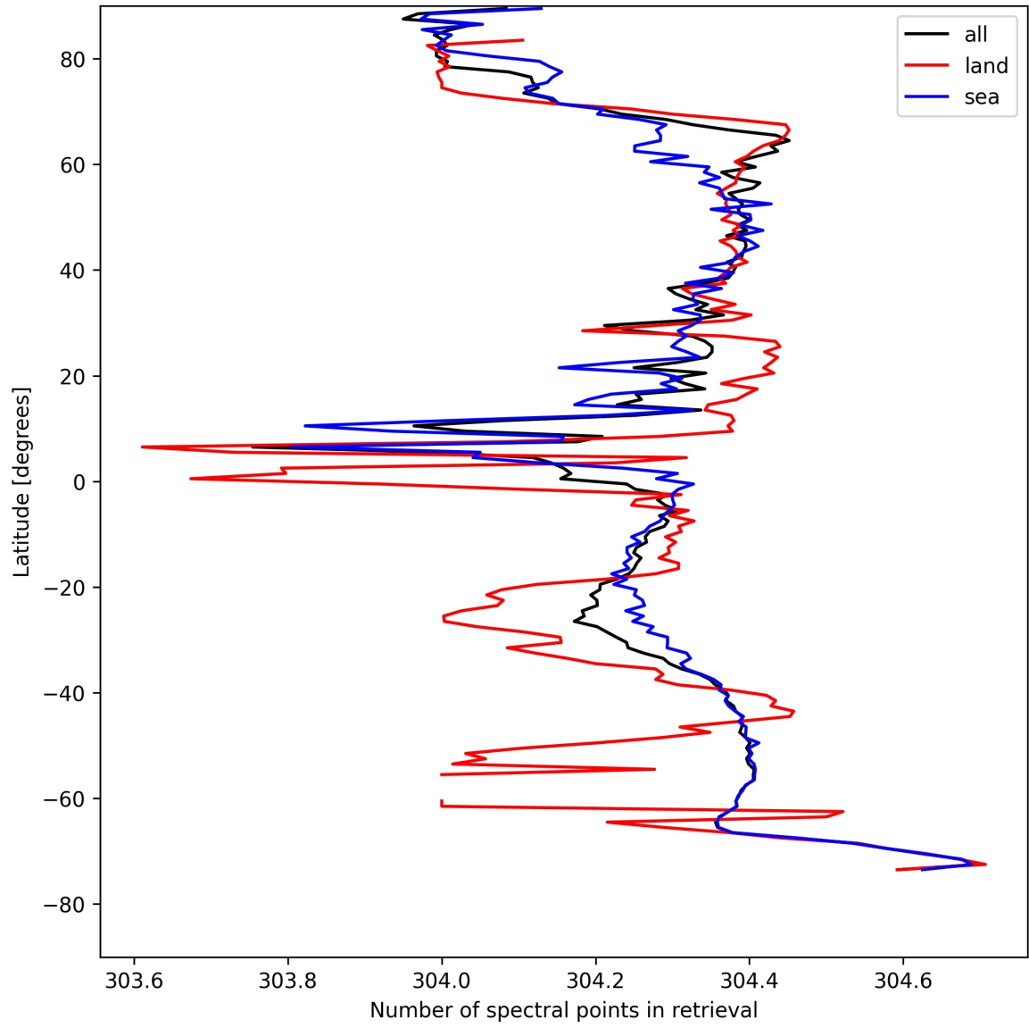
Figure 14: Zonal average of “Number of spectral points in retrieval” for 2025-04-29 to 2025-04-30.
