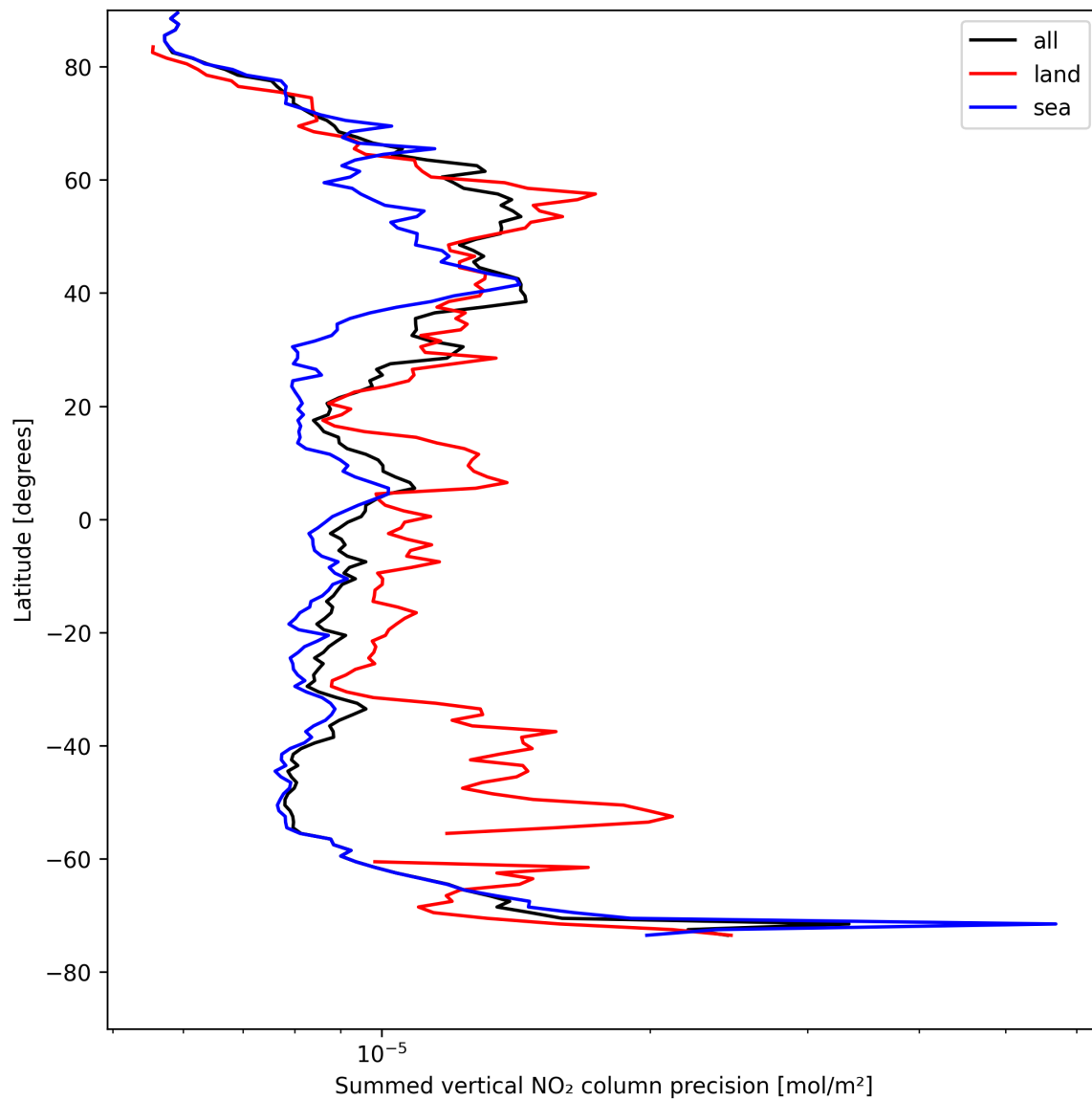
Figure 22: Zonal average of “Summed vertical NO 2 column precision” for 2025-04-29 to 2025-04-30.
