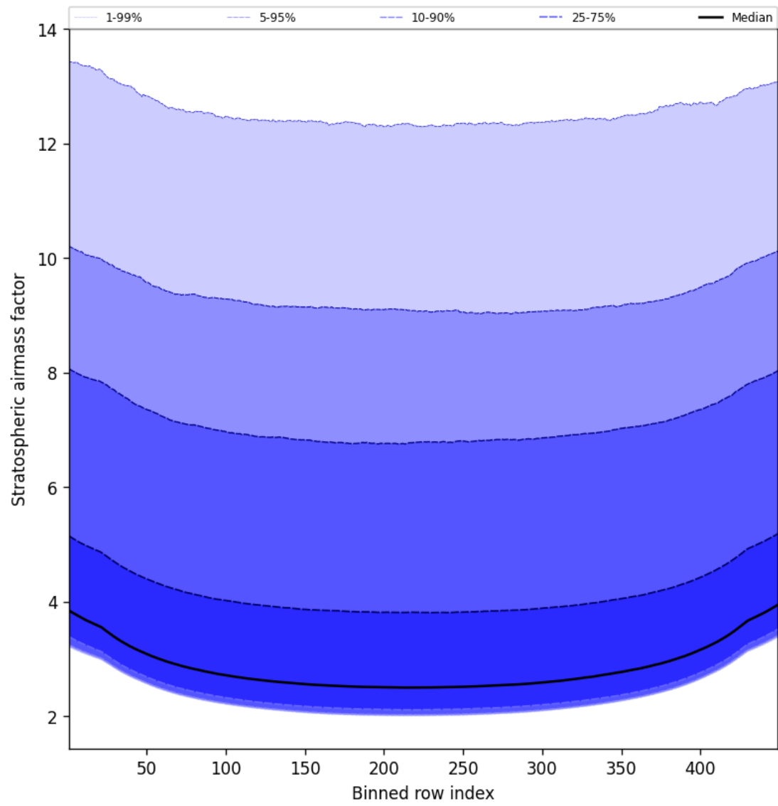
Figure 59: Along track statistics of “Stratospheric airmass factor” for 2025-04-29 to 2025-04-30
