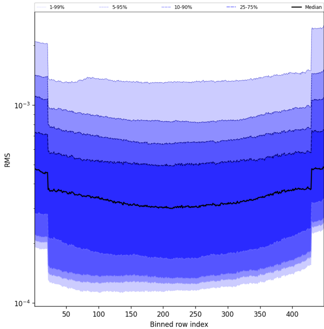
Figure 58: Along track statistics of “RMS” for 2025-04-29 to 2025-04-30
