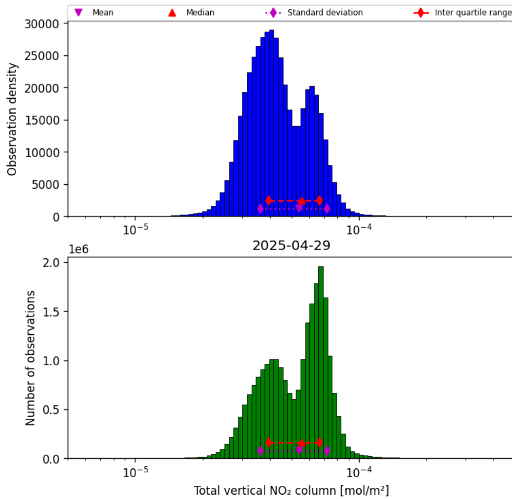
Figure 36: Histogram of “Total vertical NO 2 column” for 2025-04-29 to 2025-04-30
