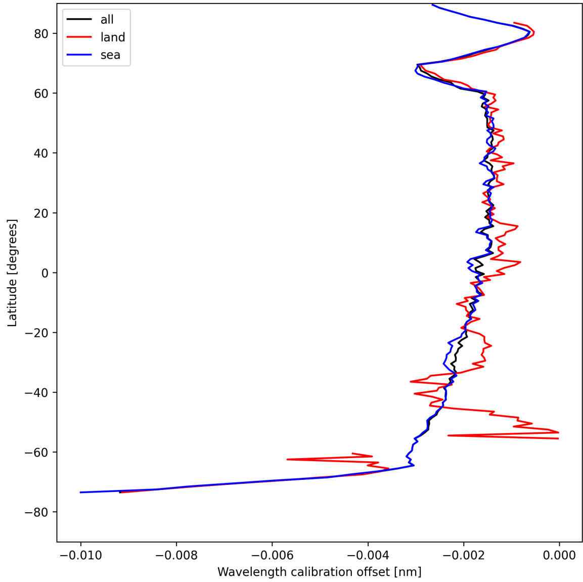
Figure 16: Zonal average of “Wavelength calibration offset” for 2025-04-29 to 2025-04-30.
