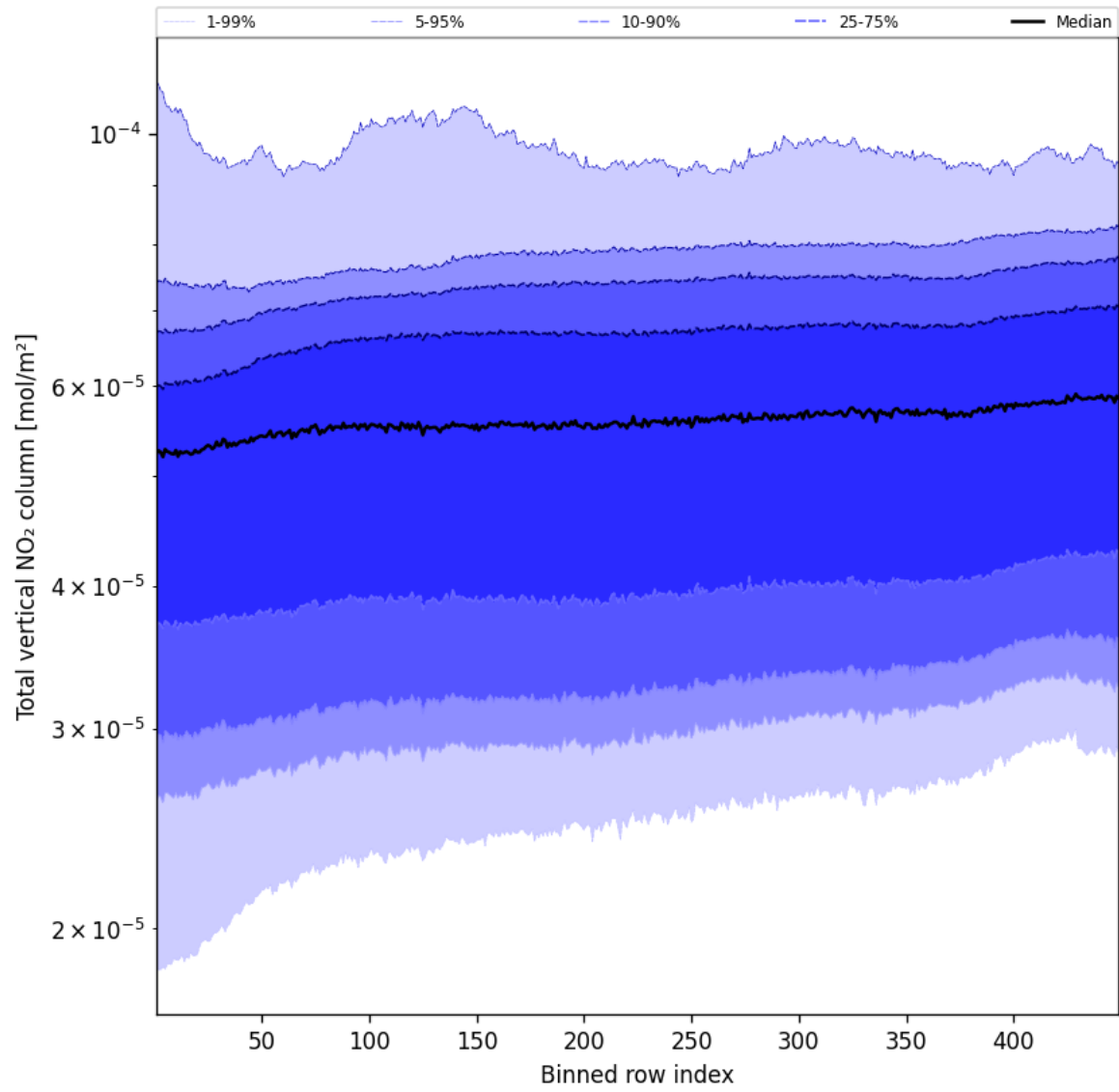
Figure 53: Along track statistics of “Total vertical NO 2 column” for 2025-04-29 to 2025-04-30
