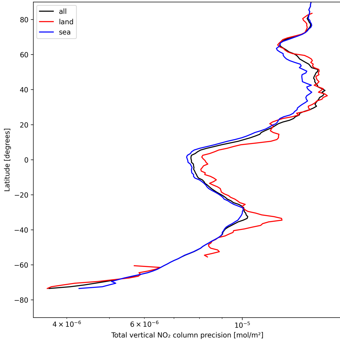
Figure 20: Zonal average of “Total vertical NO 2 column precision” for 2025-04-29 to 2025-04-30.
