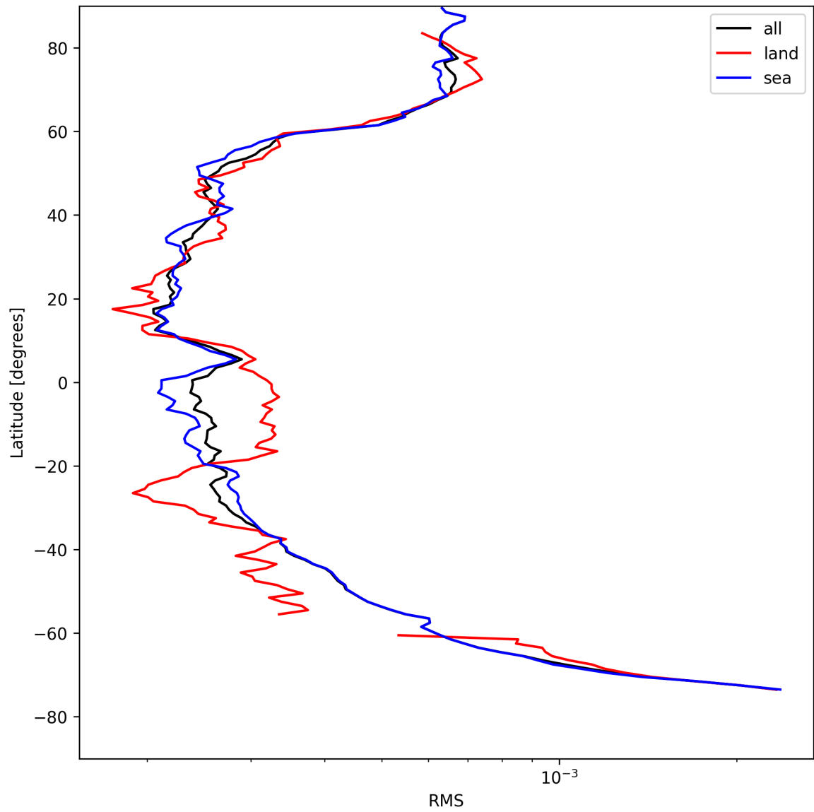
Figure 24: Zonal average of “RMS” for 2025-04-29 to 2025-04-30.
