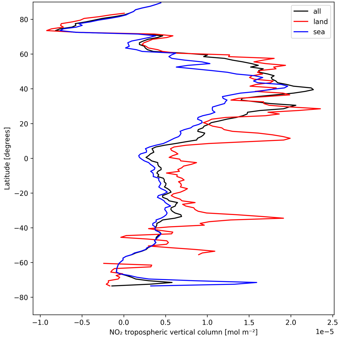
Figure 10: Zonal average of “NO 2 tropospheric vertical column” for 2025-04-29 to 2025-04-30.
