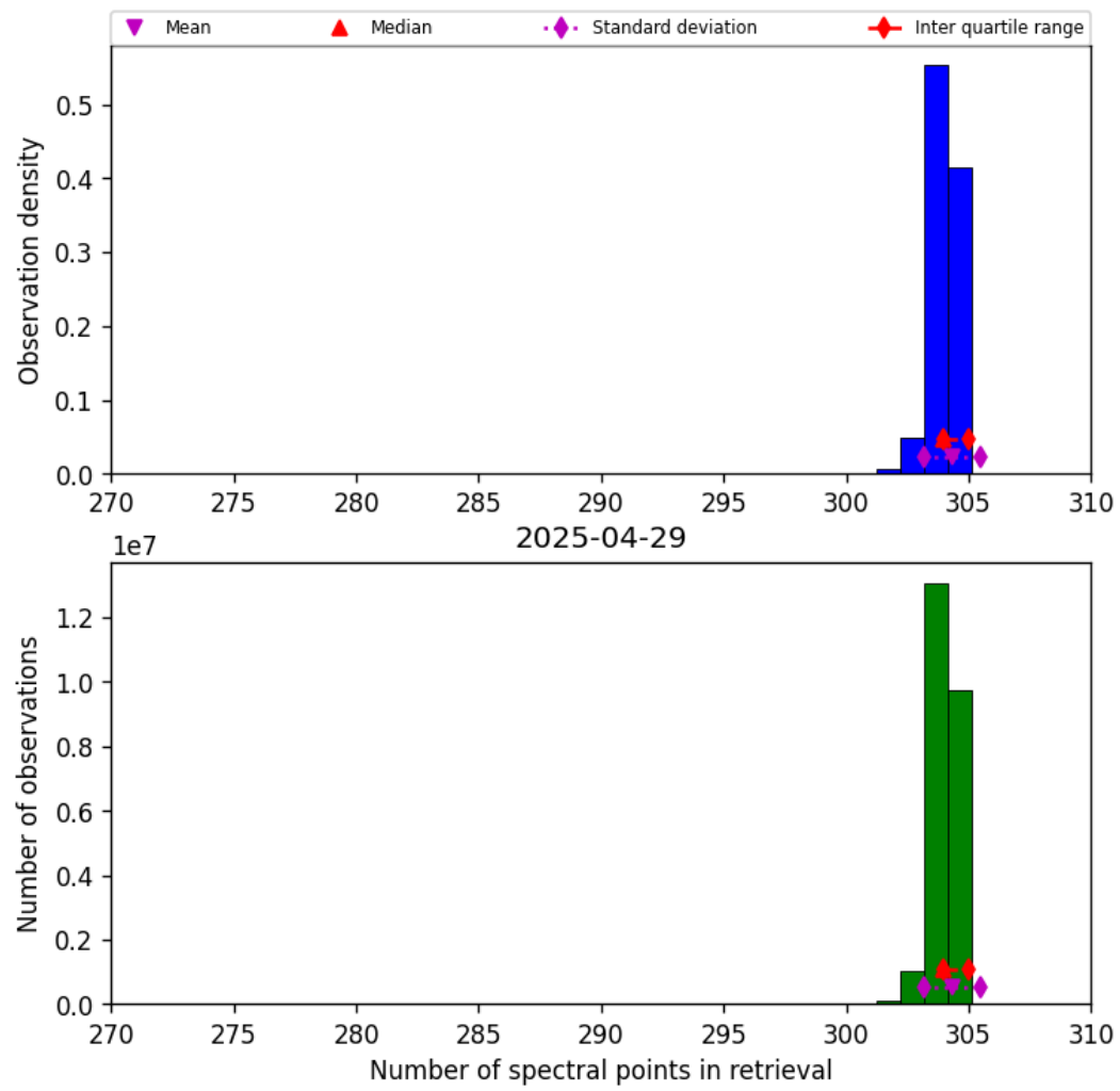
Figure 31: Histogram of “Number of spectral points in retrieval” for 2025-04-29 to 2025-04-30
