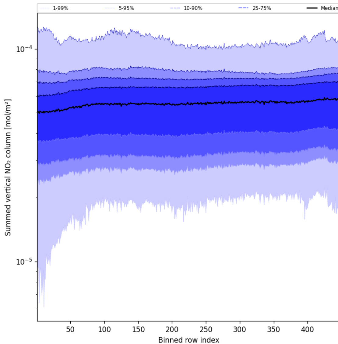
Figure 55: Along track statistics of “Summed vertical NO 2 column” for 2025-04-29 to 2025-04-30
