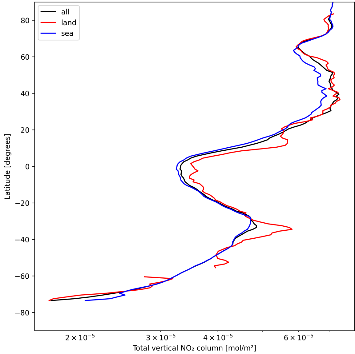
Figure 19: Zonal average of “Total vertical NO 2 column” for 2025-04-29 to 2025-04-30.
