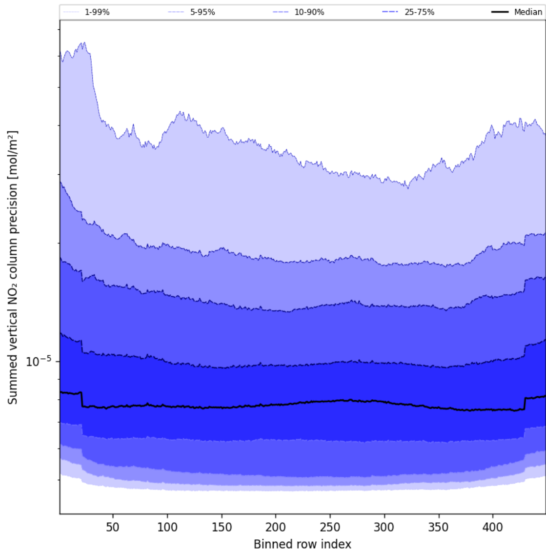
Figure 56: Along track statistics of “Summed vertical NO 2 column precision” for 2025-04-29 to 2025-04-30
