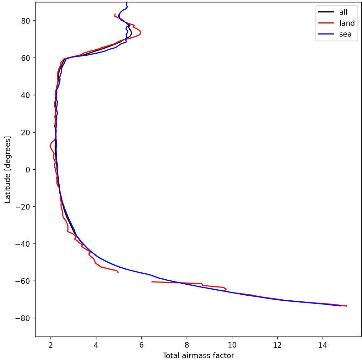
Figure 13: Zonal average of “Total airmass factor” for 2025-04-29 to 2025-04-30.
