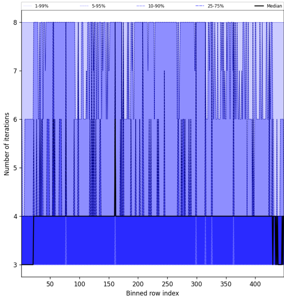
Figure 49: Along track statistics of “Number of iterations” for 2025-04-29 to 2025-04-30
