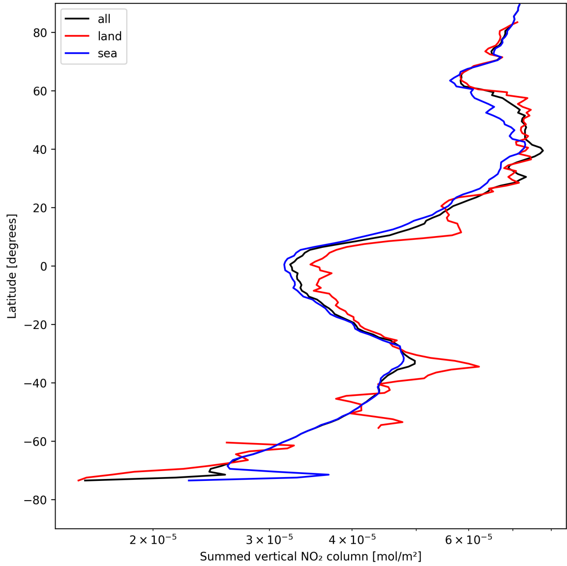
Figure 21: Zonal average of “Summed vertical NO 2 column” for 2025-04-29 to 2025-04-30.
