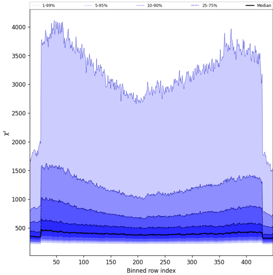
Figure 57: Along track statistics of “ \chi^2 ” for 2025-04-29 to 2025-04-30
