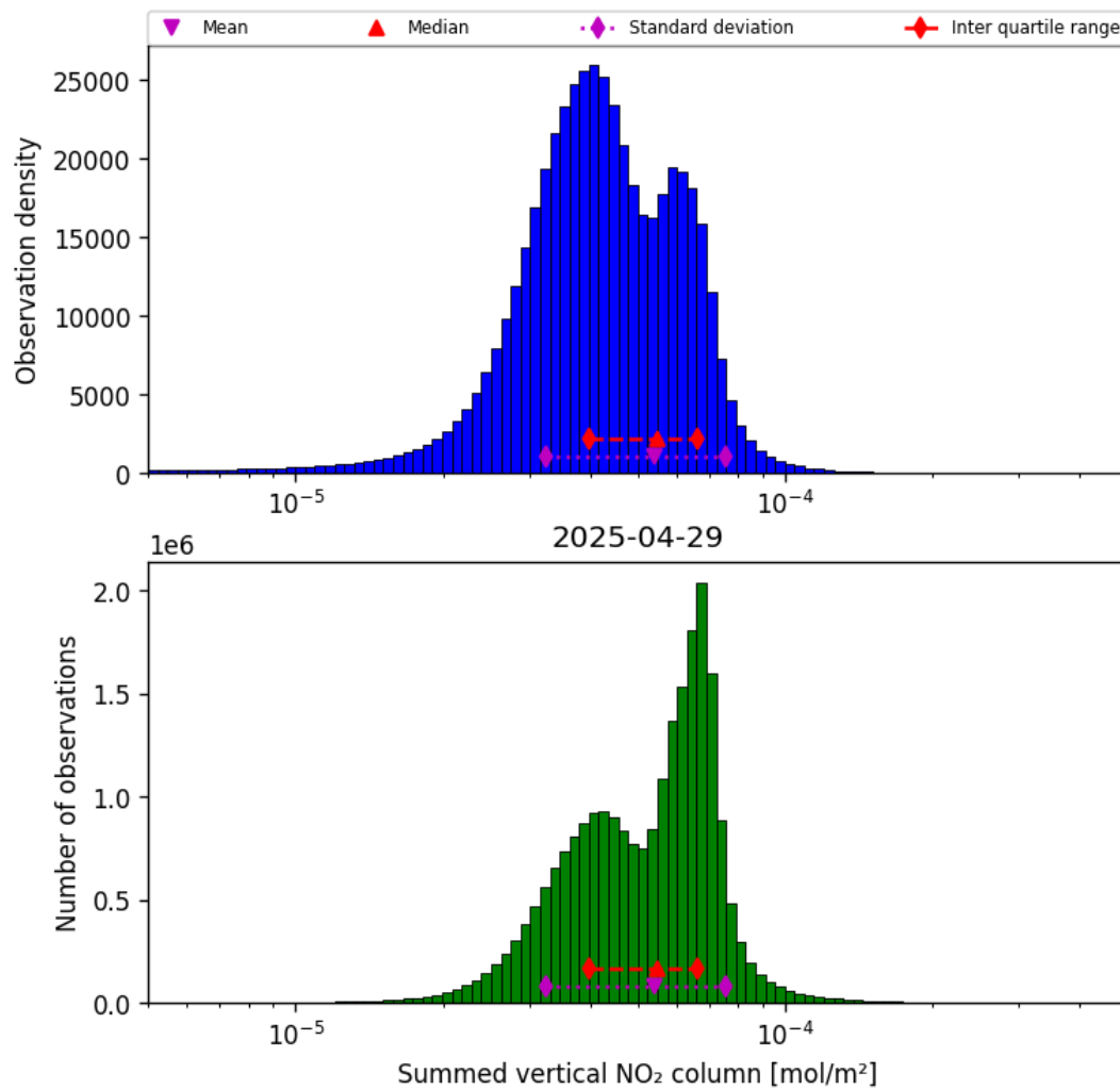
Figure 38: Histogram of “Summed vertical NO 2 column” for 2025-04-29 to 2025-04-30
