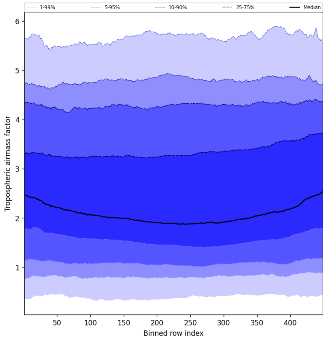
Figure 46: Along track statistics of “Tropospheric airmass factor” for 2025-04-29 to 2025-04-30
