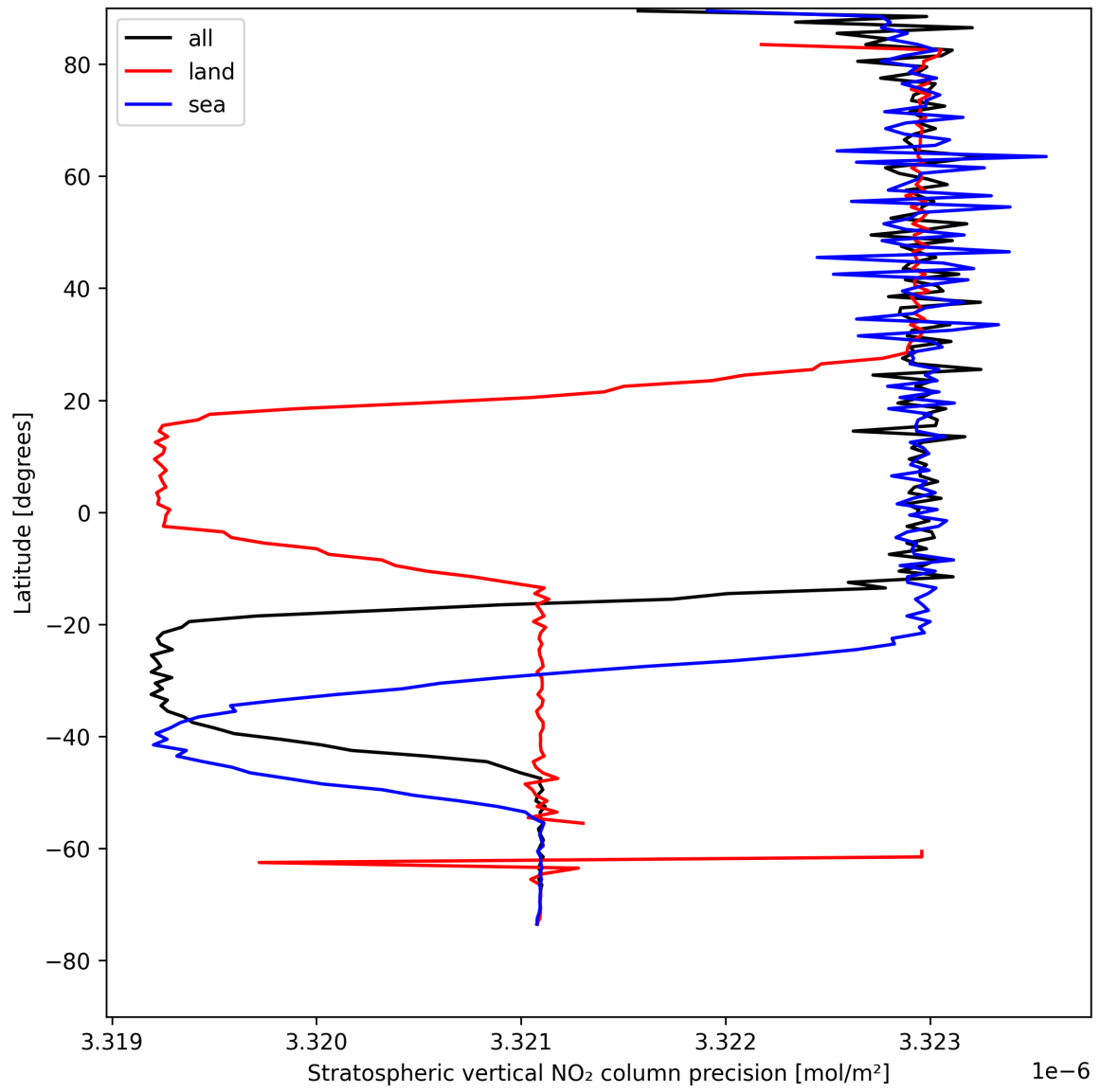
Figure 18: Zonal average of “Stratospheric vertical NO 2 column precision” for 2025-04-29 to 2025-04-30.
