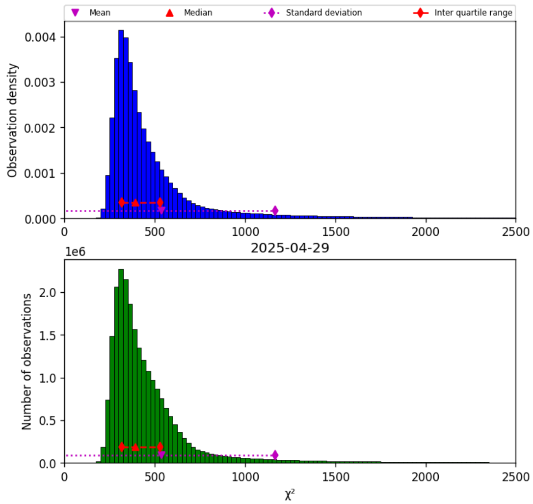
Figure 40: Histogram of “ \chi^2 ” for 2025-04-29 to 2025-04-30
