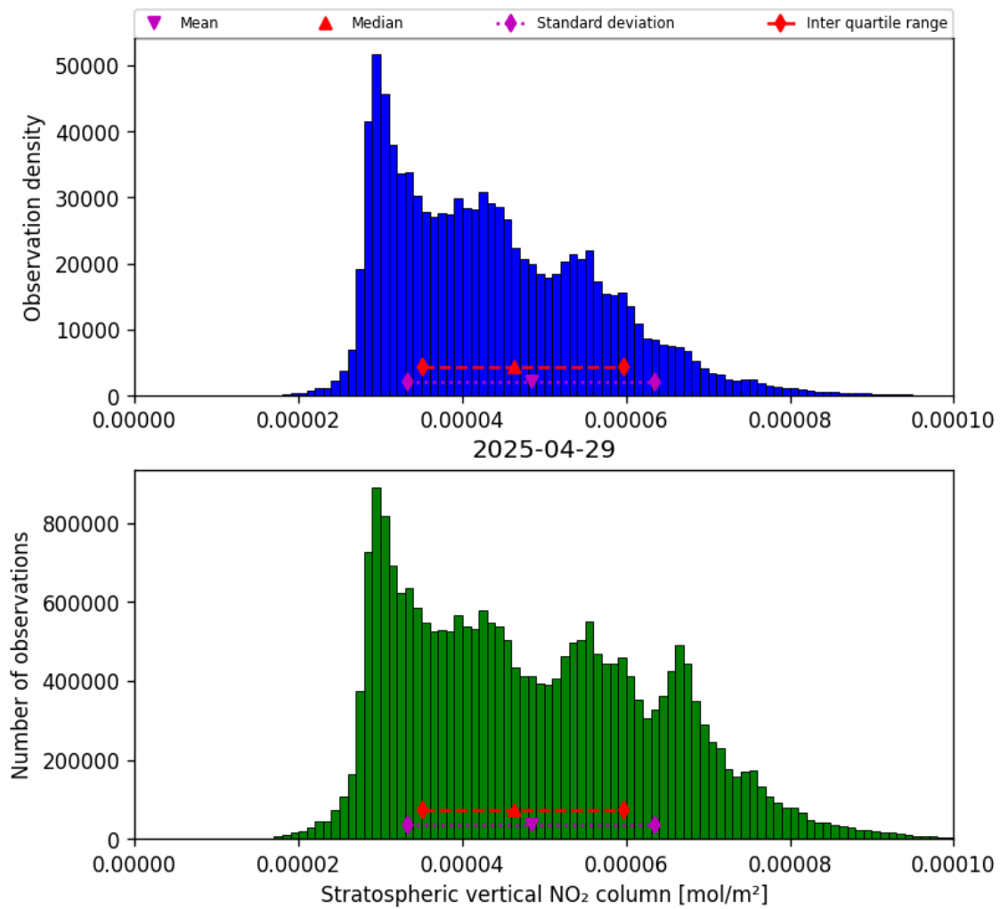
Figure 34: Histogram of “Stratospheric vertical NO 2 column” for 2025-04-29 to 2025-04-30
