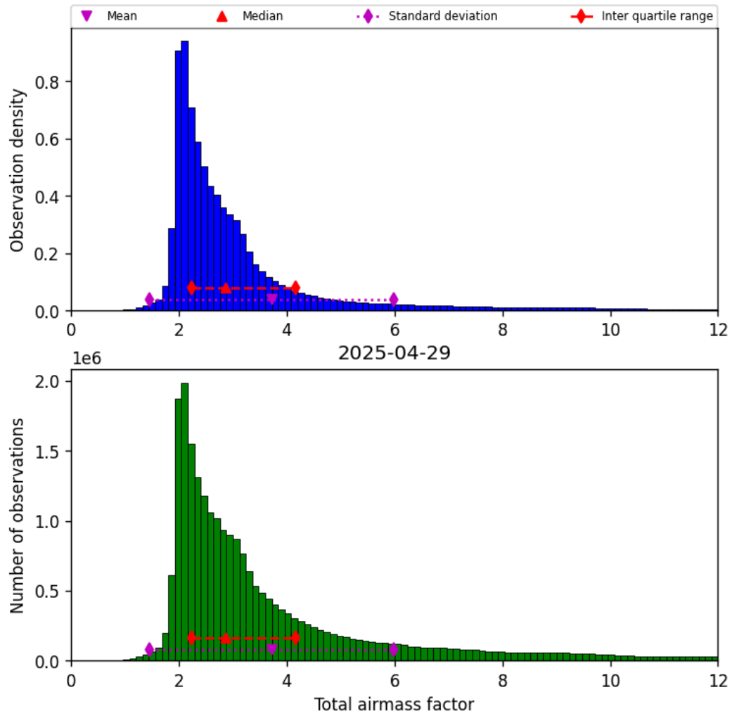
Figure 30: Histogram of “Total airmass factor” for 2025-04-29 to 2025-04-30
