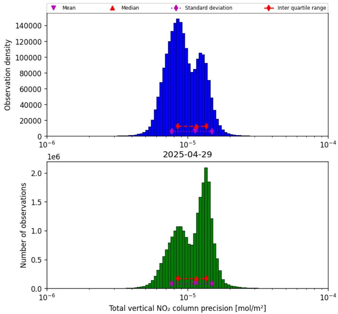
Figure 37: Histogram of "Total vertical NO 2 column precision" for 2025-04-29 to 2025-04-30
