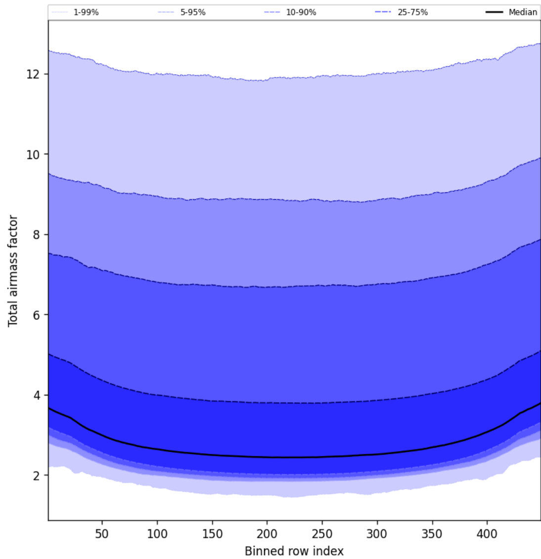
Figure 47: Along track statistics of “Total airmass factor” for 2025-04-29 to 2025-04-30
