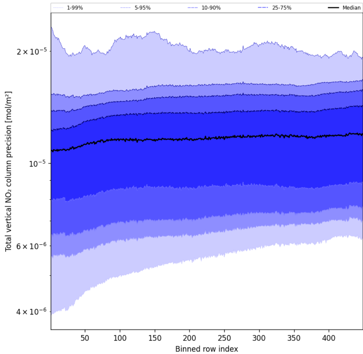
Figure 54: Along track statistics of “Total vertical NO 2 column precision” for 2025-04-29 to 2025-04-30
