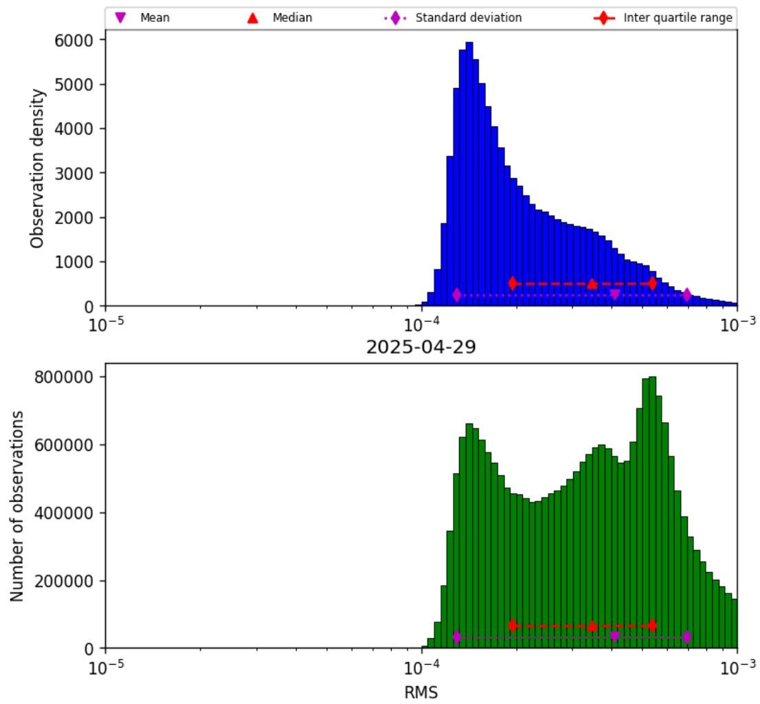
Figure 41: Histogram of “RMS” for 2025-04-29 to 2025-04-30
