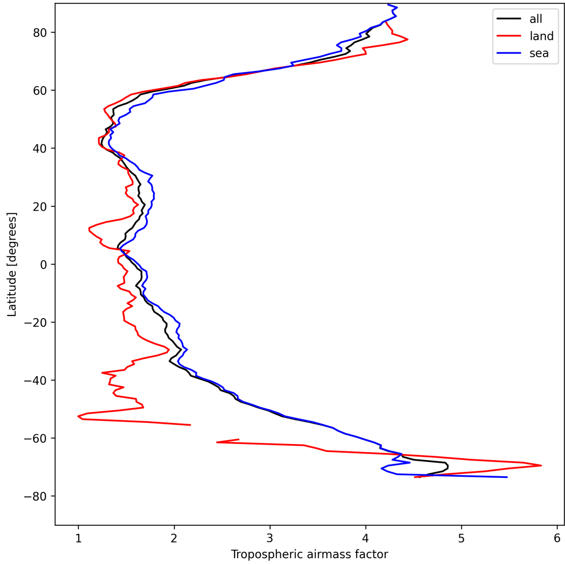
Figure 12: Zonal average of “Tropospheric air mass factor” for 2025-04-29 to 2025-04-30.
