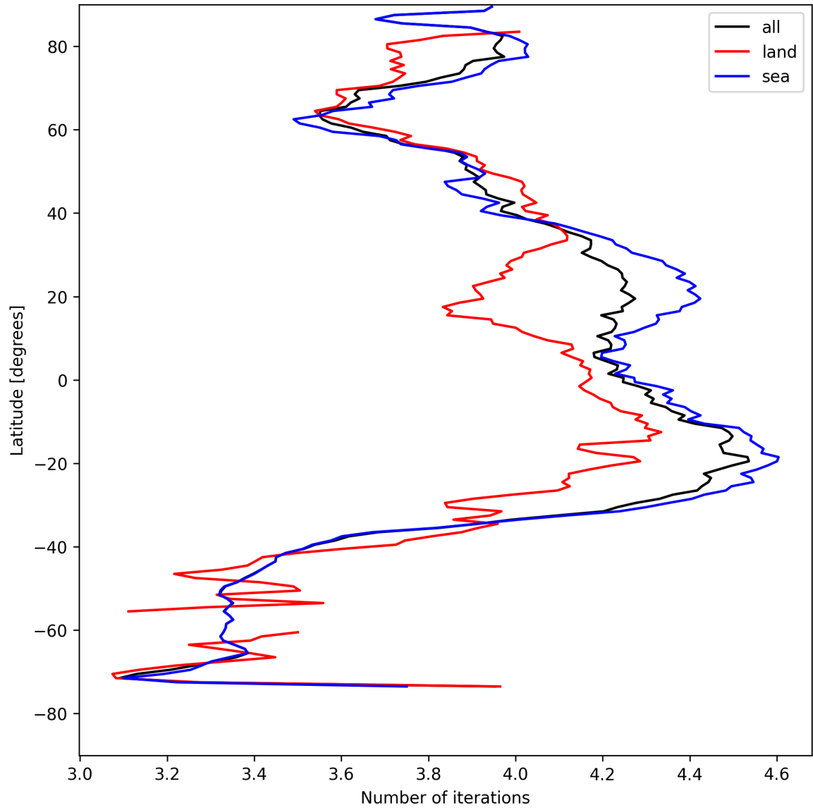
Figure 15: Zonal average of “Number of iterations” for 2025-04-29 to 2025-04-30.
