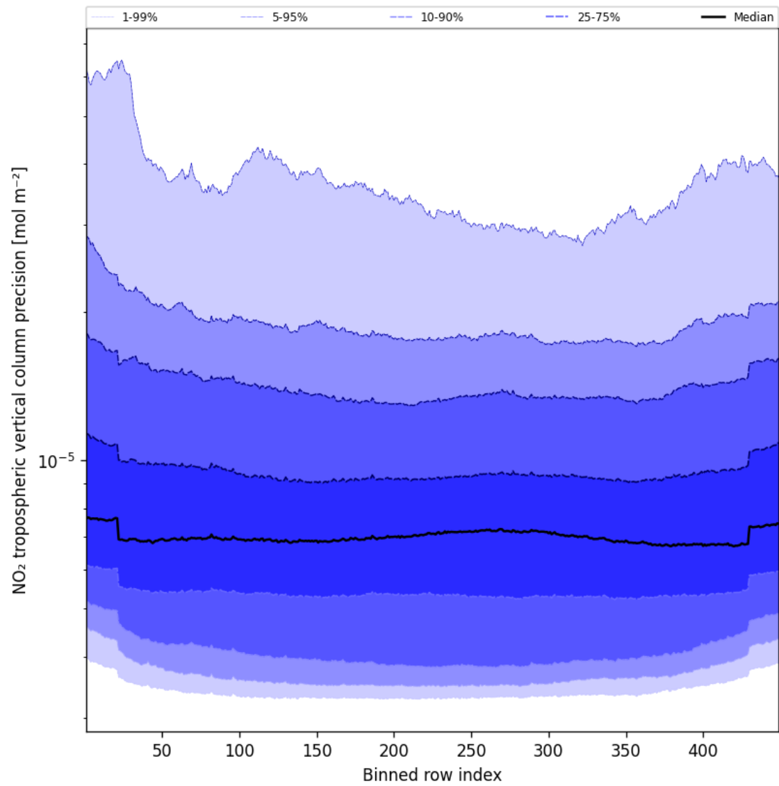
Figure 45: Along track statistics of “NO 2 tropospheric vertical column precision” for 2025-04-29 to 2025-04-30
