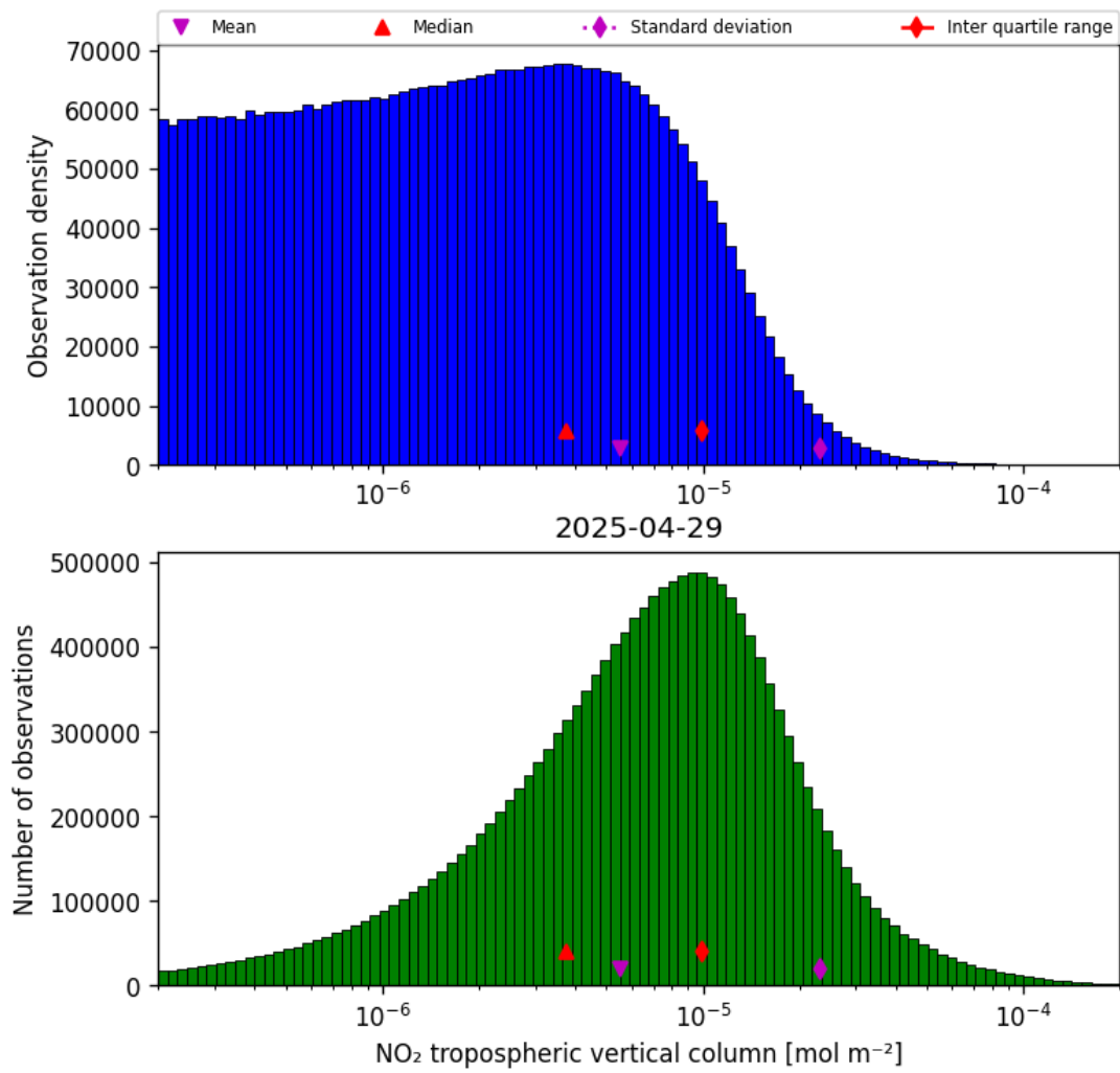
Figure 27: Histogram of “NO 2 tropospheric vertical column” for 2025-04-29 to 2025-04-30
