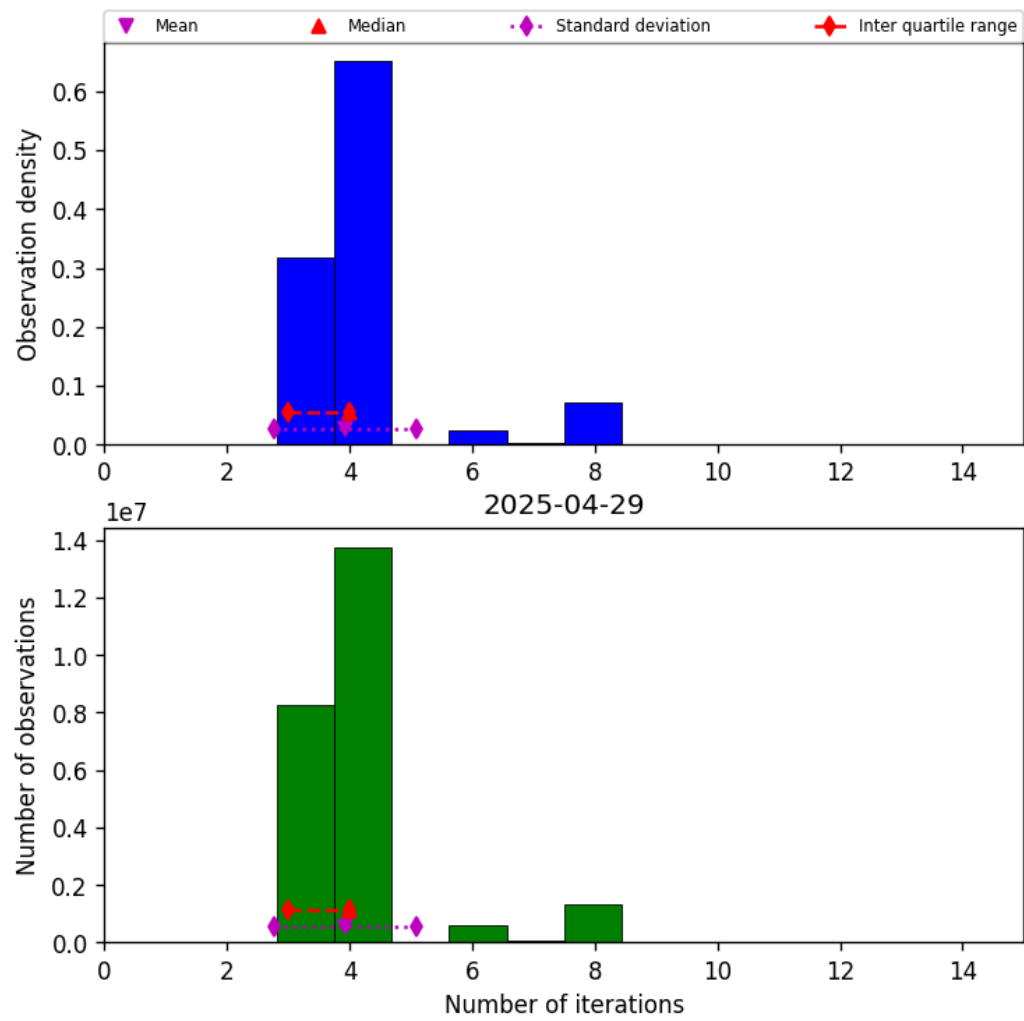
Figure 32: Histogram of “Number of iterations” for 2025-04-29 to 2025-04-30
