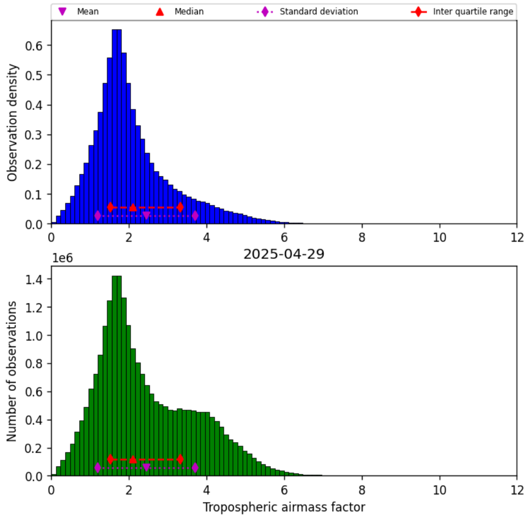
Figure 29: Histogram of “Tropospheric airmass factor” for 2025-04-29 to 2025-04-30
