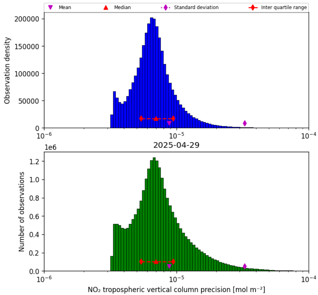
Figure 28: Histogram of “NO 2 tropospheric vertical column precision” for 2025-04-29 to 2025-04-30
