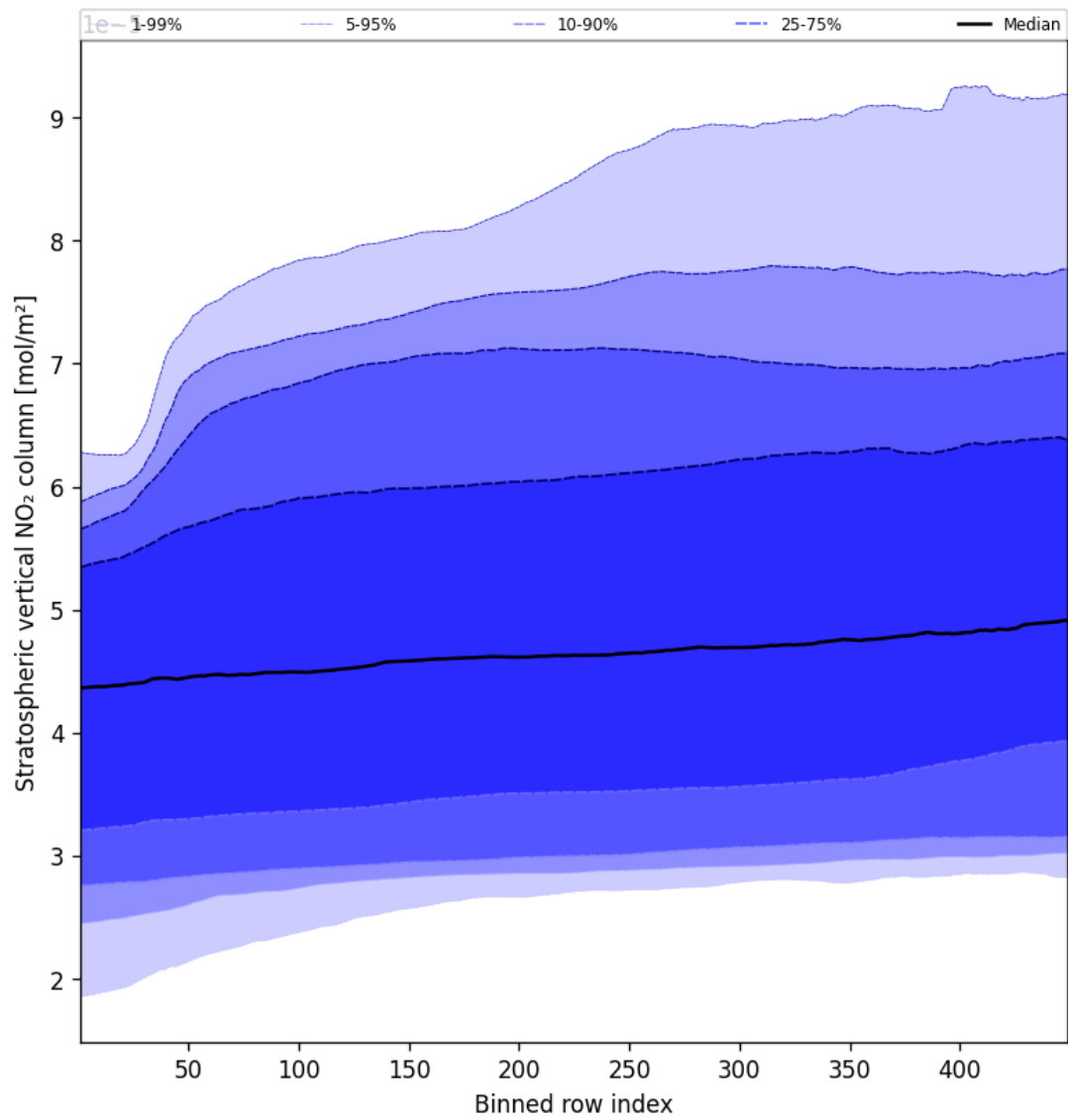
Figure 51: Along track statistics of “Stratospheric vertical NO 2 column” for 2025-04-29 to 2025-04-30
