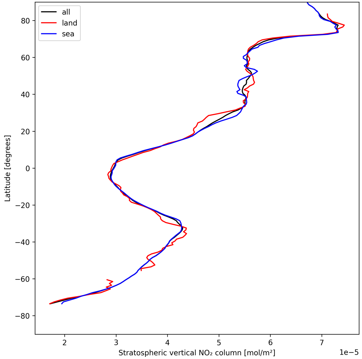
Figure 17: Zonal average of “Stratospheric vertical NO 2 column” for 2025-04-29 to 2025-04-30.
