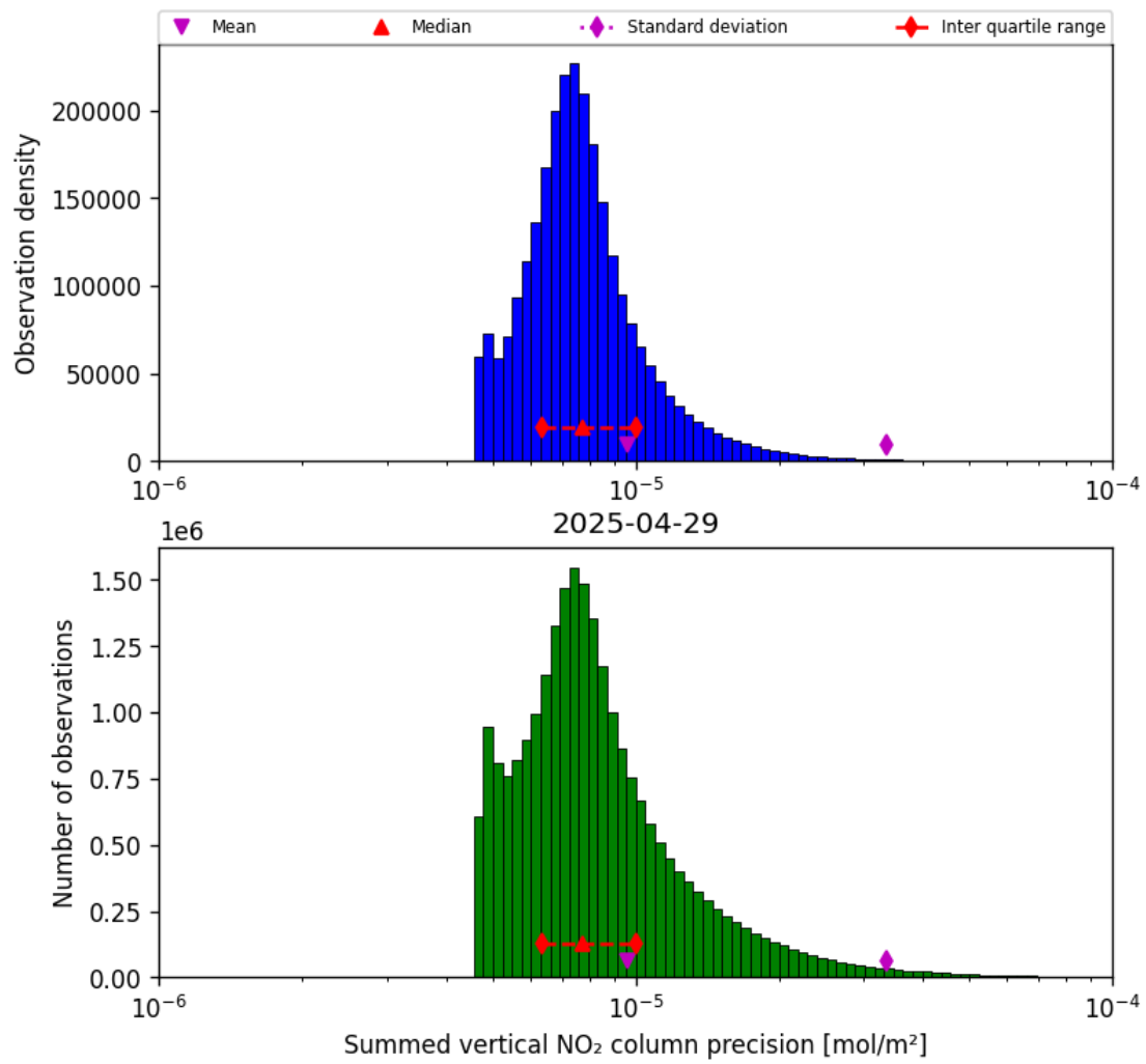
Figure 39: Histogram of "Summed vertical NO 2 column precision" for 2025-04-29 to 2025-04-30
