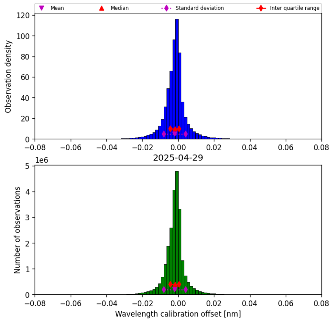
Figure 33: Histogram of “Wavelength calibration offset” for 2025-04-29 to 2025-04-30
