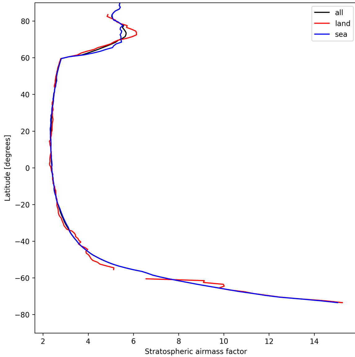
Figure 25: Zonal average of “Stratospheric air mass factor” for 2025-04-29 to 2025-04-30.
