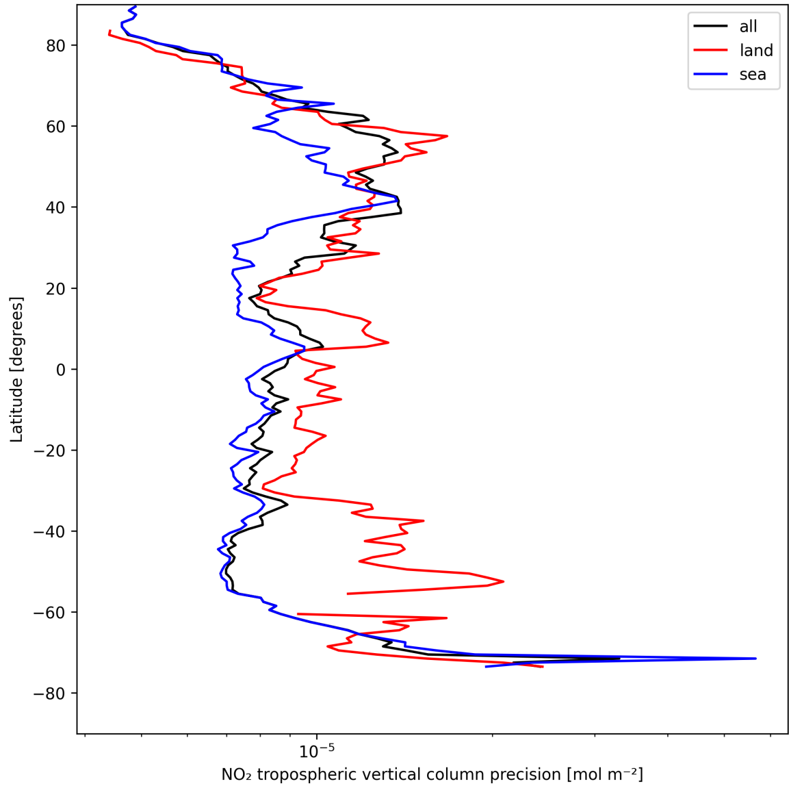
Figure 11: Zonal average of “NO 2 tropospheric vertical column precision” for 2025-04-29 to 2025-04-30.
