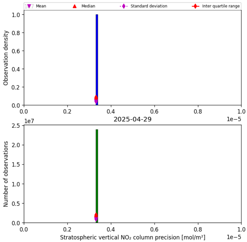
Figure 35: Histogram of “Stratospheric vertical NO 2 column precision” for 2025-04-29 to 2025-04-30
