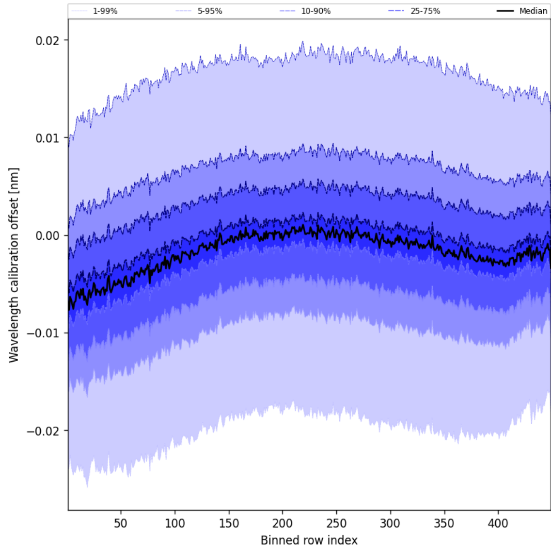
Figure 50: Along track statistics of “Wavelength calibration offset” for 2025-04-29 to 2025-04-30
