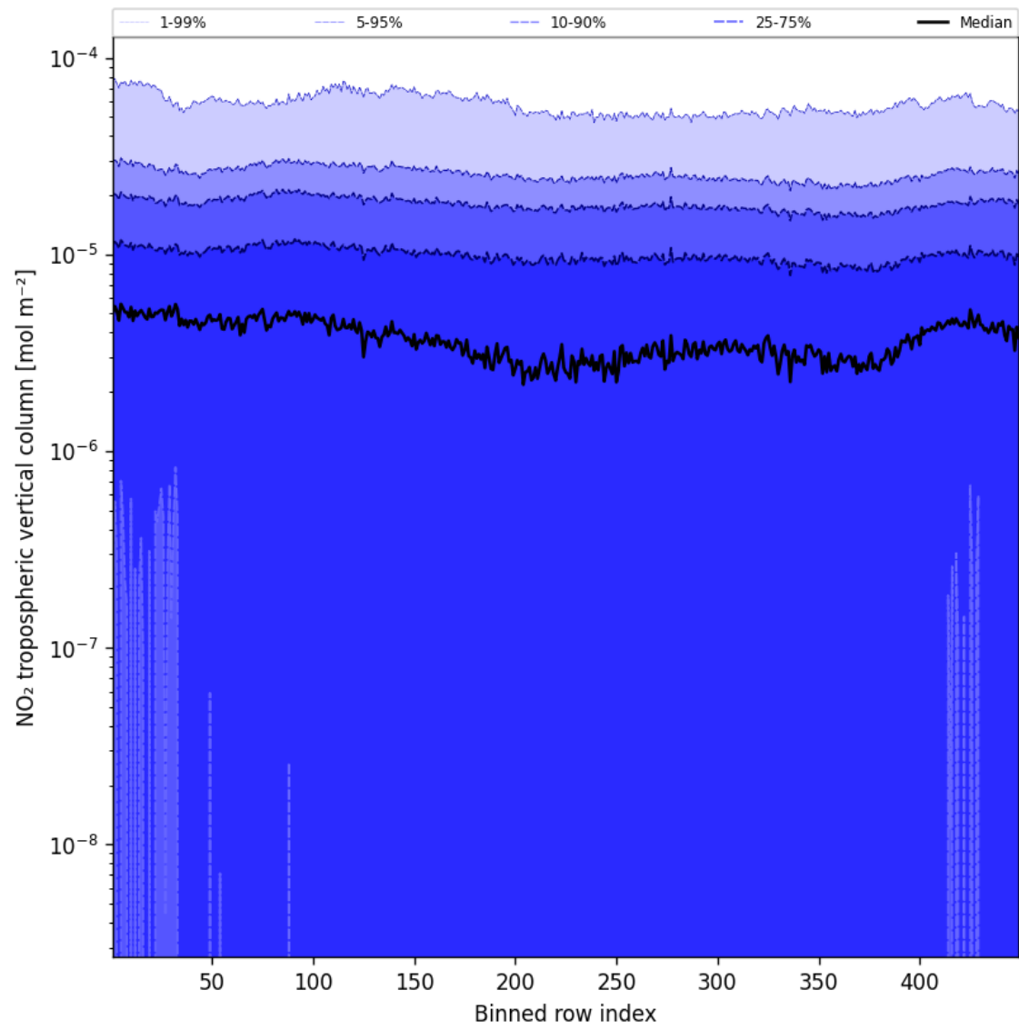
Figure 44: Along track statistics of “NO 2 tropospheric vertical column” for 2025-04-29 to 2025-04-30
