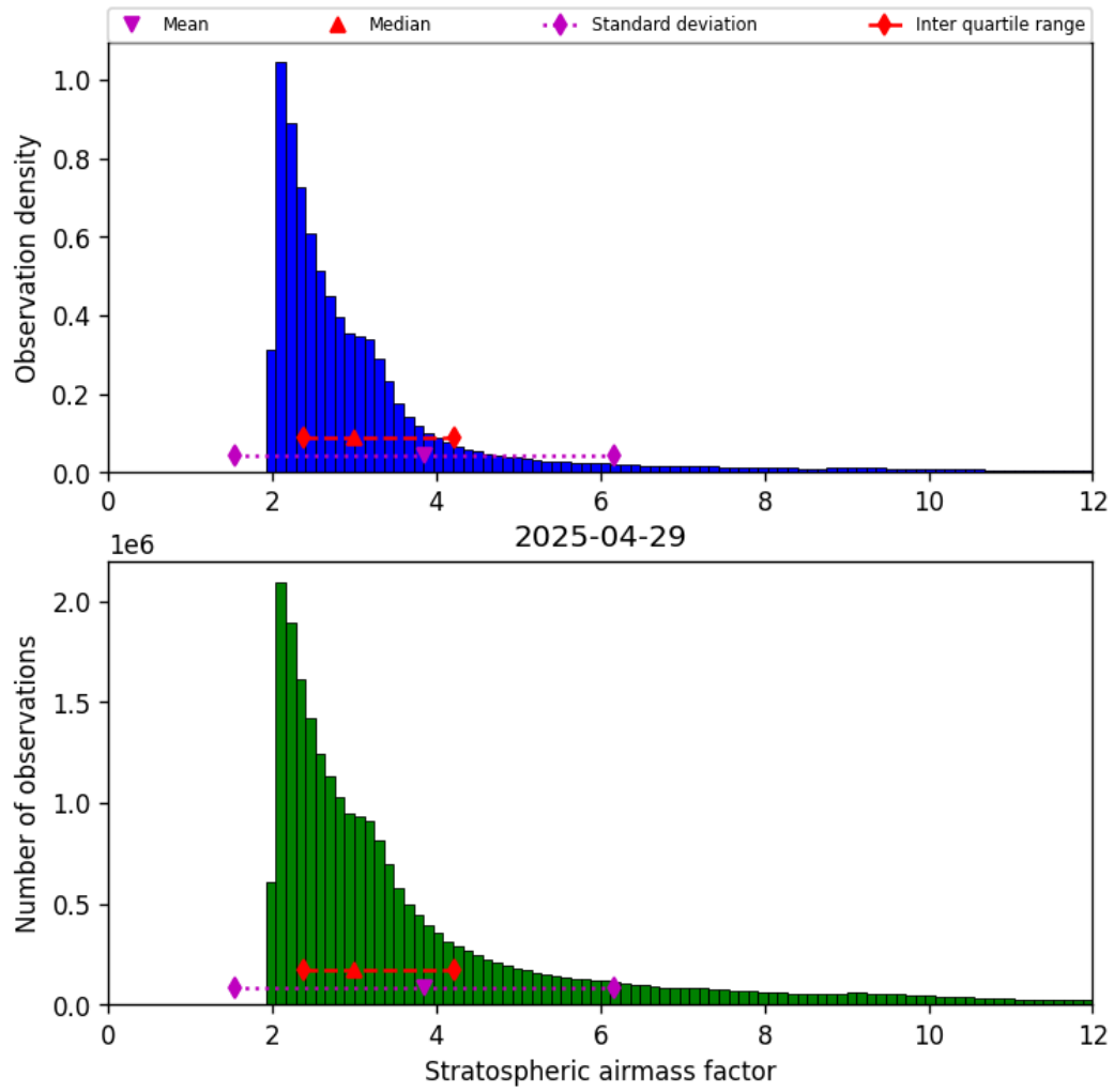
Figure 42: Histogram of “Stratospheric airmass factor” for 2025-04-29 to 2025-04-30
