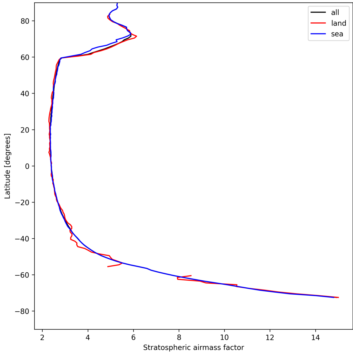
Figure 25: Zonal average of “Stratospheric air mass factor” for 2025-05-01 to 2025-05-02.
