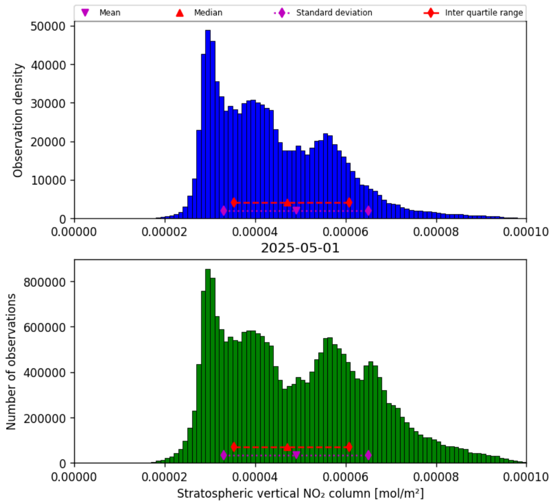
Figure 34: Histogram of “Stratospheric vertical NO 2 column” for 2025-05-01 to 2025-05-02
