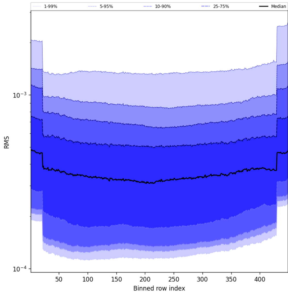
Figure 58: Along track statistics of “RMS” for 2025-05-01 to 2025-05-02
