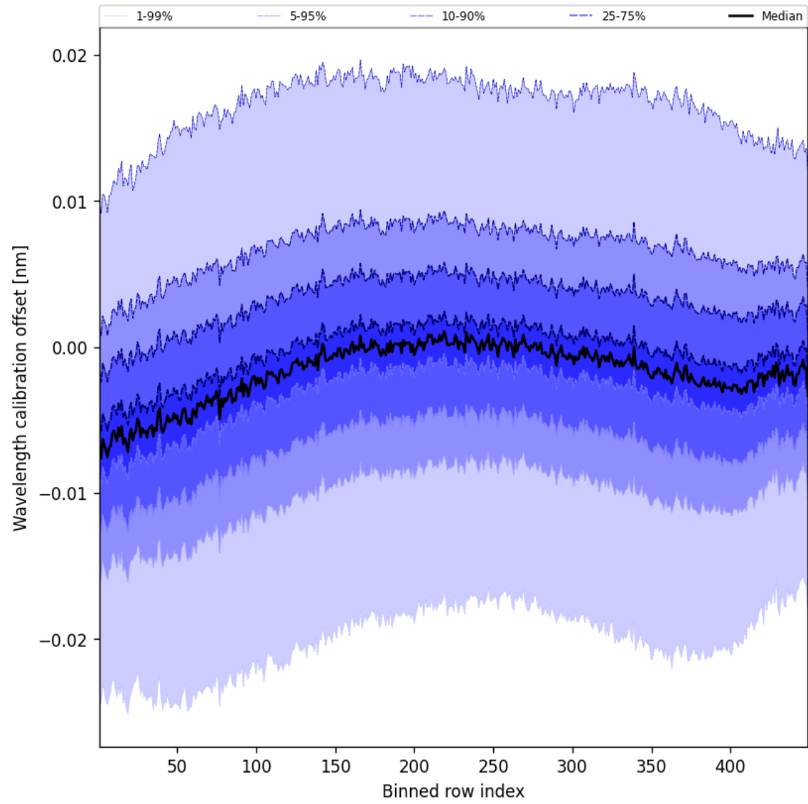
Figure 50: Along track statistics of “Wavelength calibration offset” for 2025-05-01 to 2025-05-02
