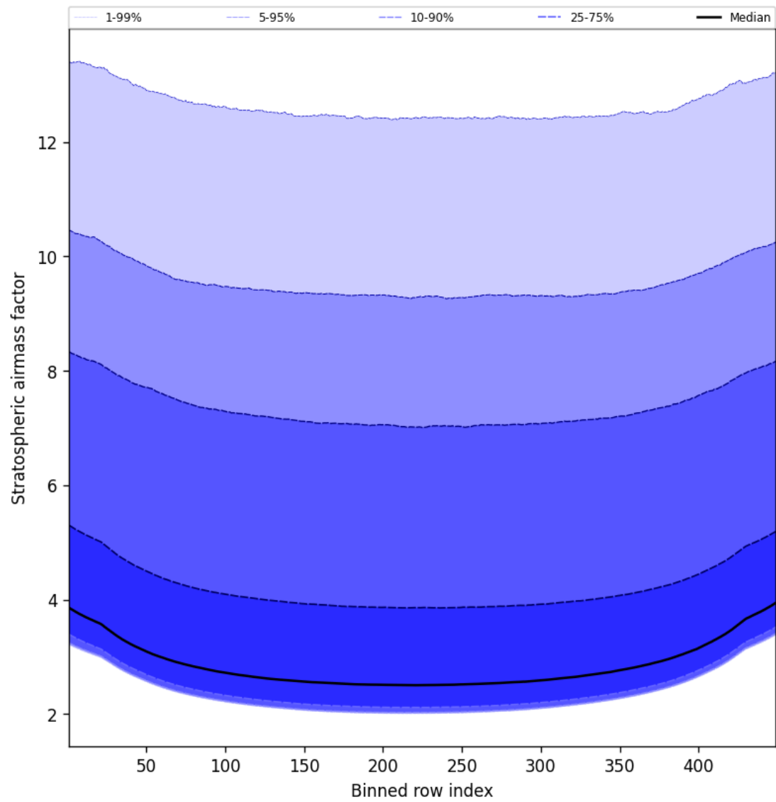
Figure 59: Along track statistics of “Stratospheric airmass factor” for 2025-05-01 to 2025-05-02
