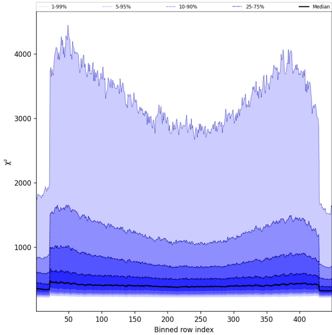
Figure 57: Along track statistics of “ \chi^2 ” for 2025-05-01 to 2025-05-02
