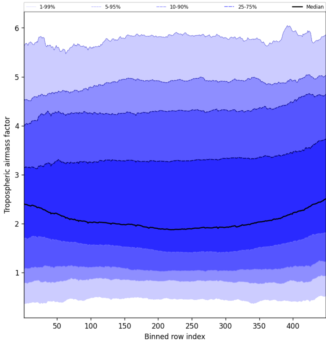
Figure 46: Along track statistics of “Tropospheric airmass factor” for 2025-05-01 to 2025-05-02
