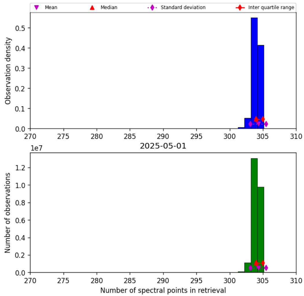
Figure 31: Histogram of “Number of spectral points in retrieval” for 2025-05-01 to 2025-05-02
