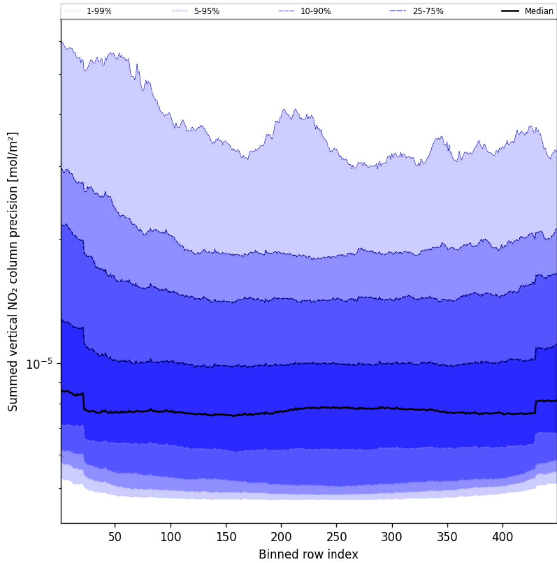
Figure 56: Along track statistics of “Summed vertical NO 2 column precision” for 2025-05-01 to 2025-05-02
