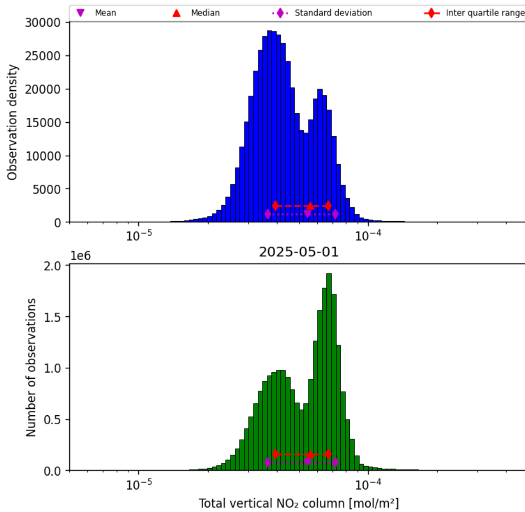
Figure 36: Histogram of “Total vertical NO 2 column” for 2025-05-01 to 2025-05-02
