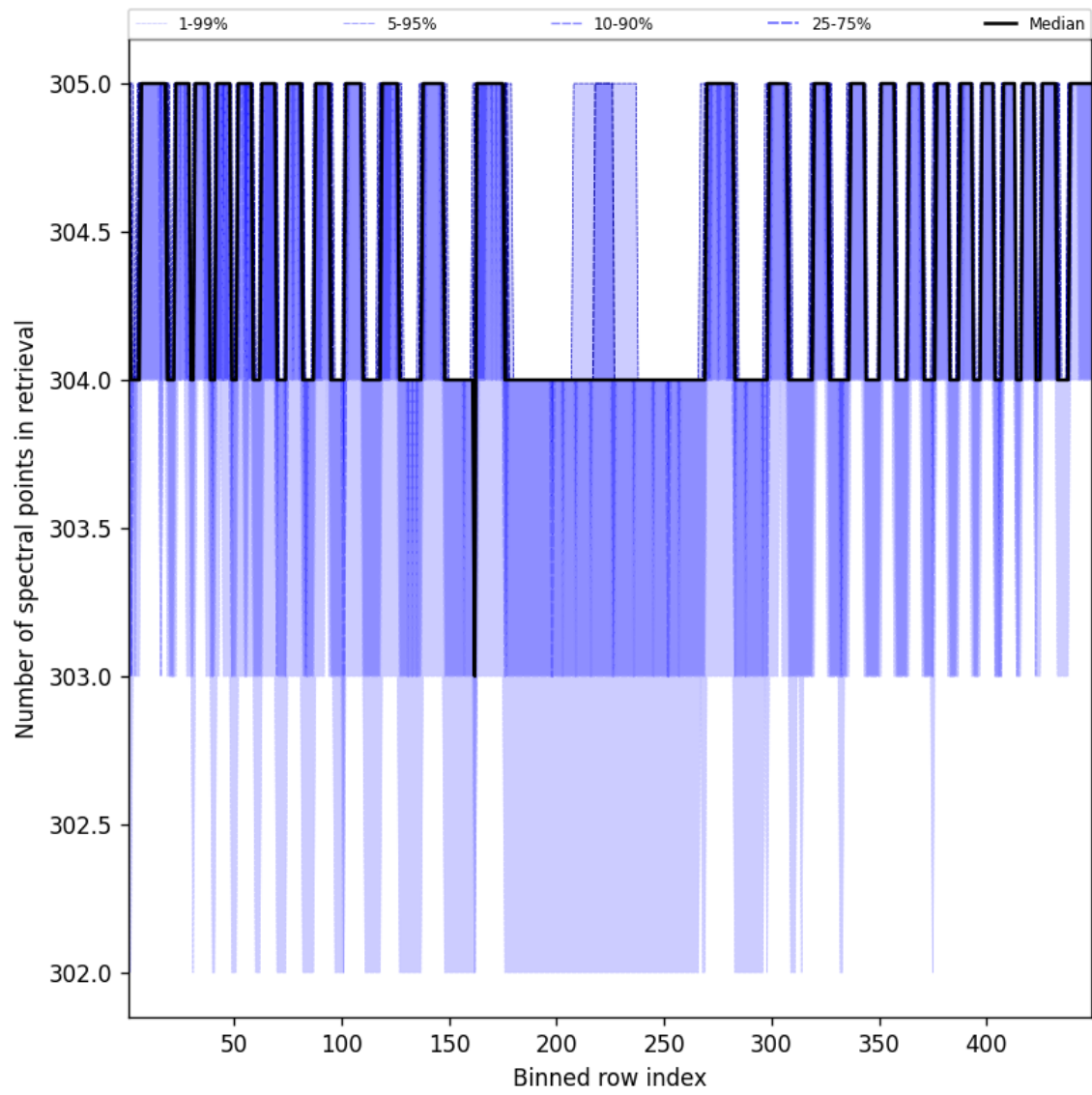
Figure 48: Along track statistics of “Number of spectral points in retrieval” for 2025-05-01 to 2025-05-02
