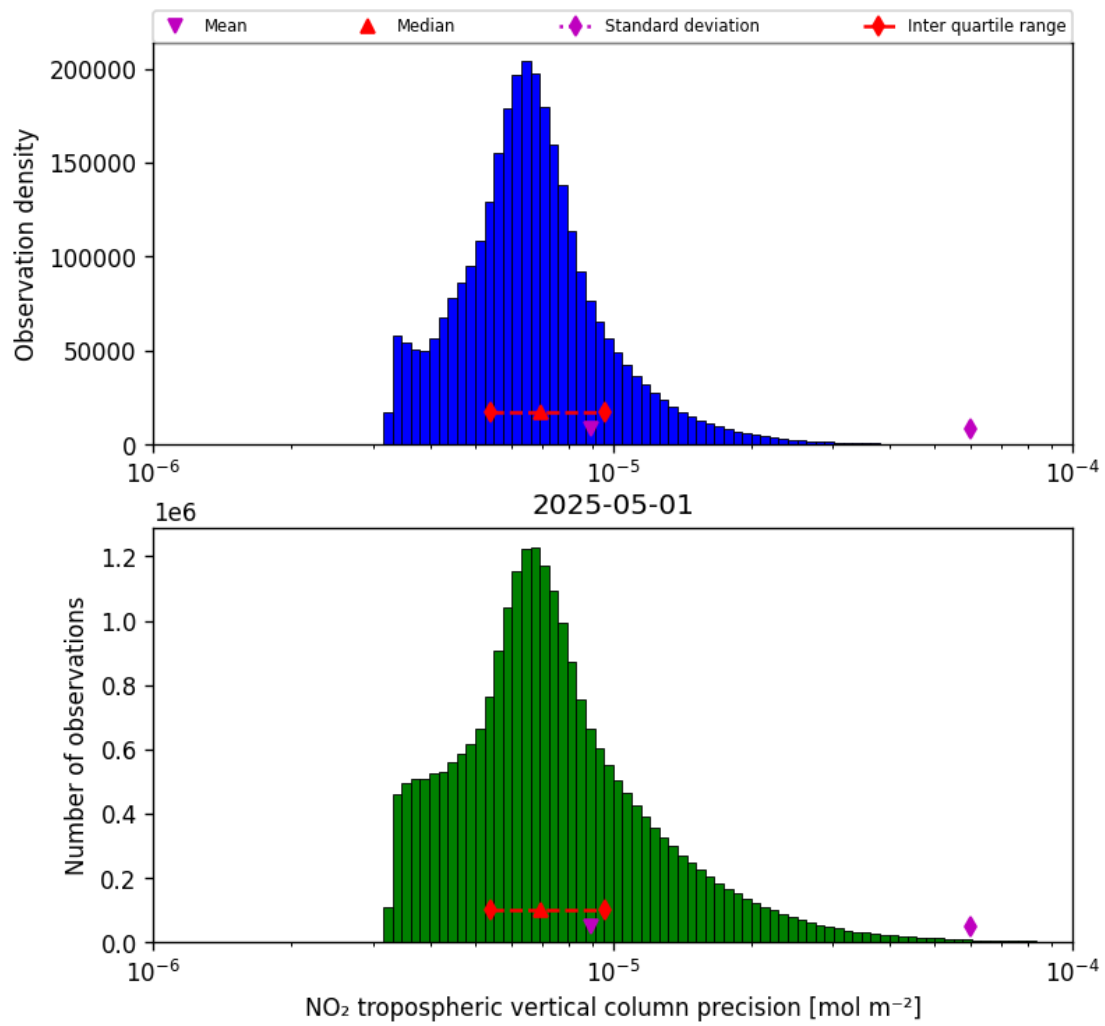
Figure 28: Histogram of “NO 2 tropospheric vertical column precision” for 2025-05-01 to 2025-05-02
