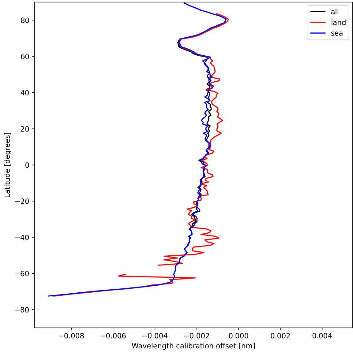
Figure 16: Zonal average of “Wavelength calibration offset” for 2025-05-01 to 2025-05-02.
