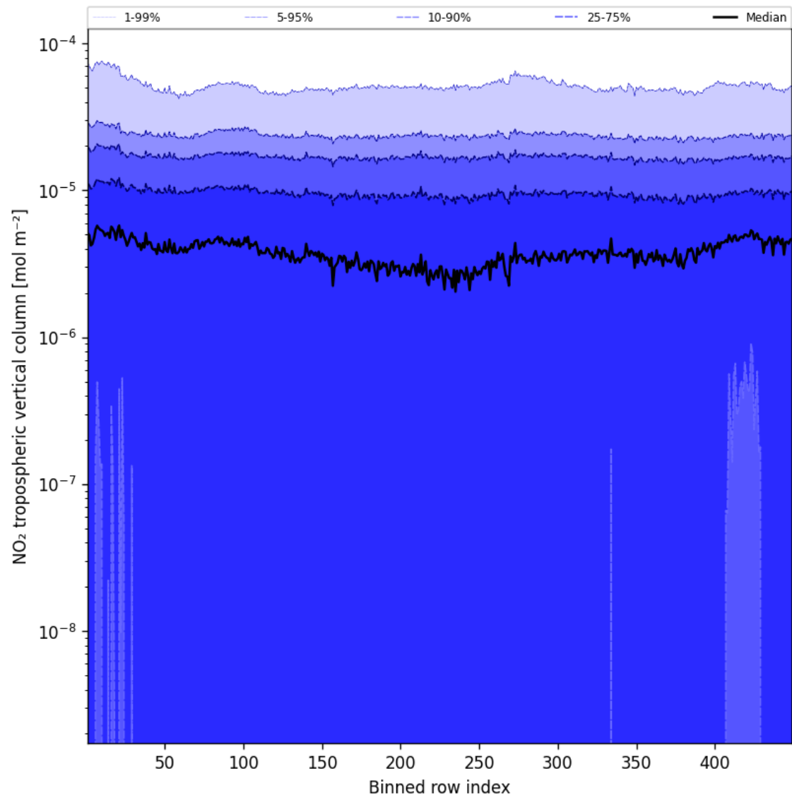
Figure 44: Along track statistics of “NO 2 tropospheric vertical column” for 2025-05-01 to 2025-05-02
