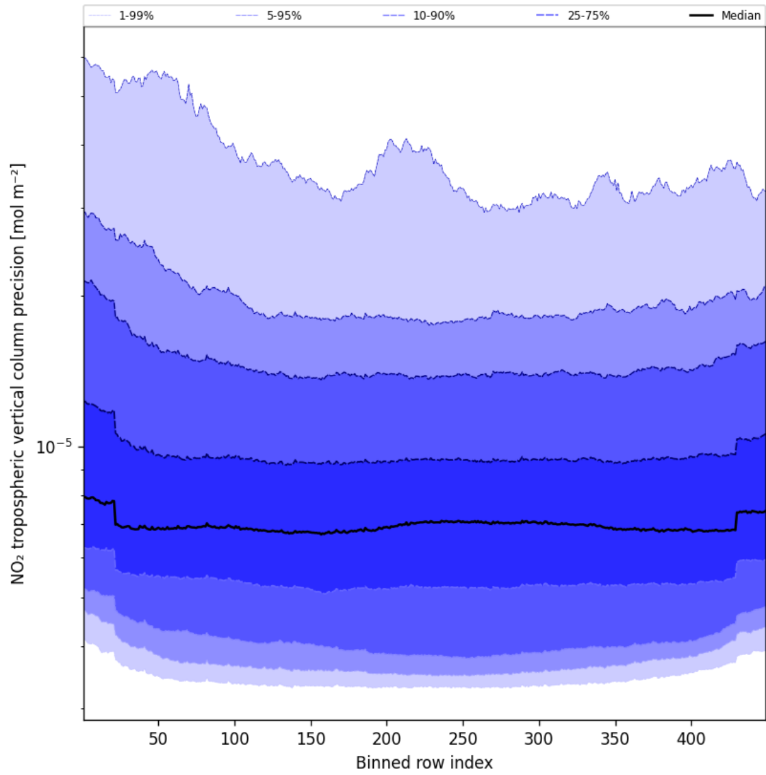
Figure 45: Along track statistics of “NO 2 tropospheric vertical column precision” for 2025-05-01 to 2025-05-02
