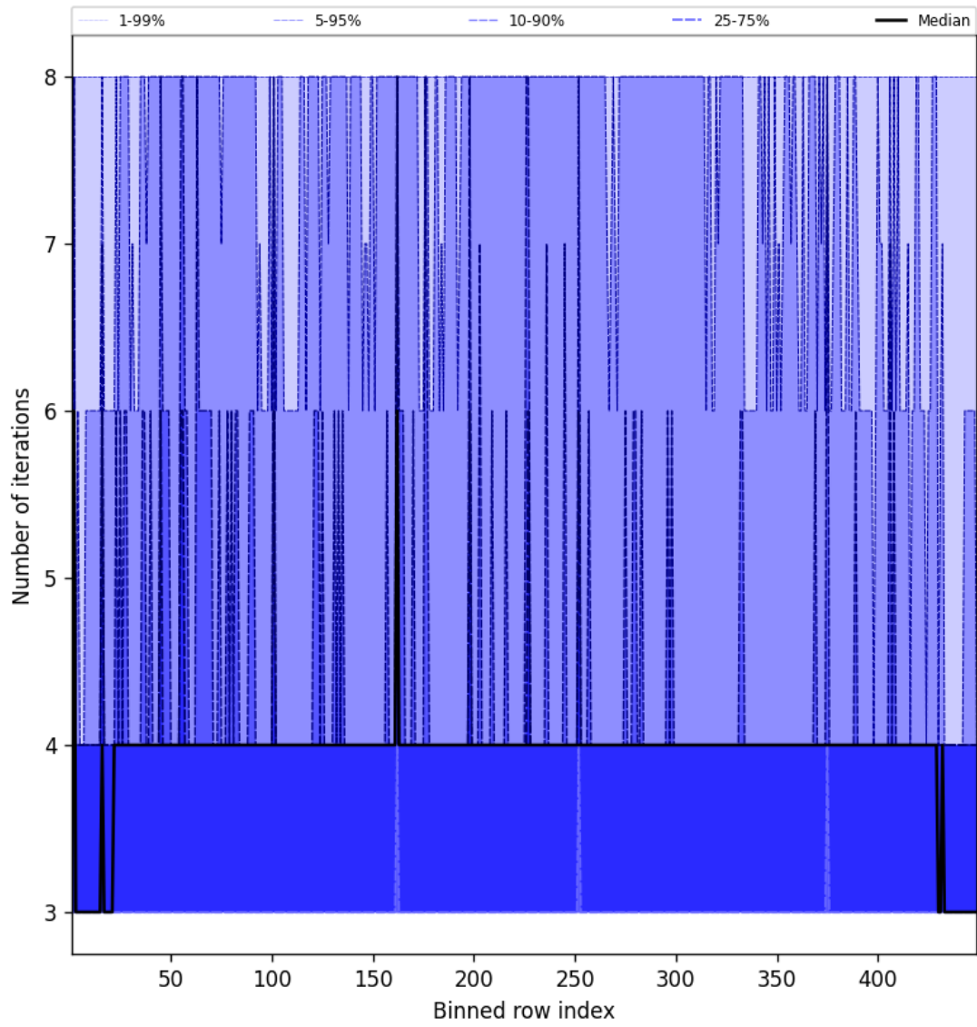
Figure 49: Along track statistics of “Number of iterations” for 2025-05-01 to 2025-05-02
