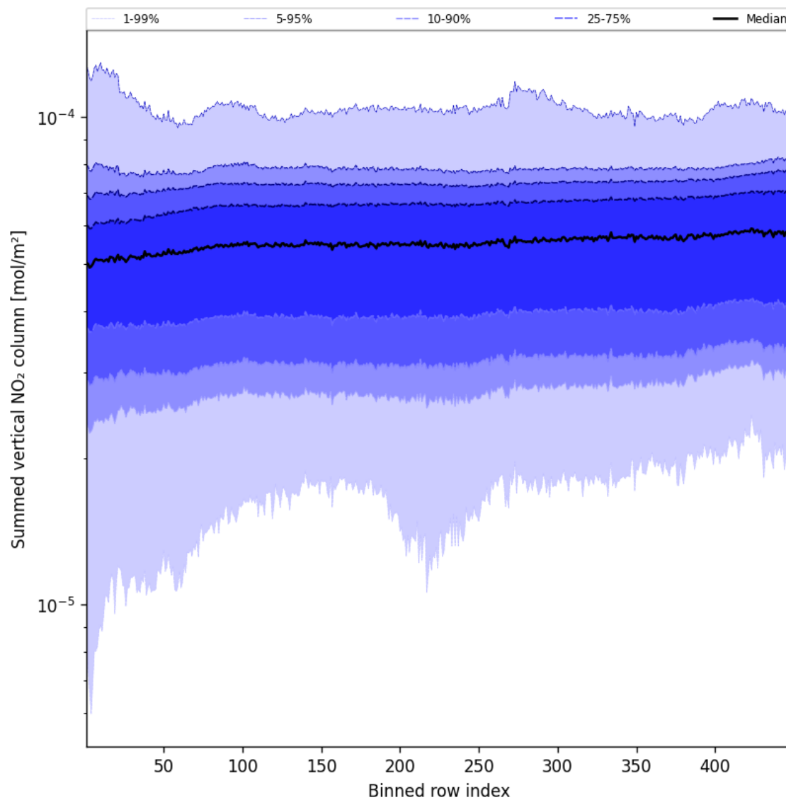
Figure 55: Along track statistics of “Summed vertical NO 2 column” for 2025-05-01 to 2025-05-02
