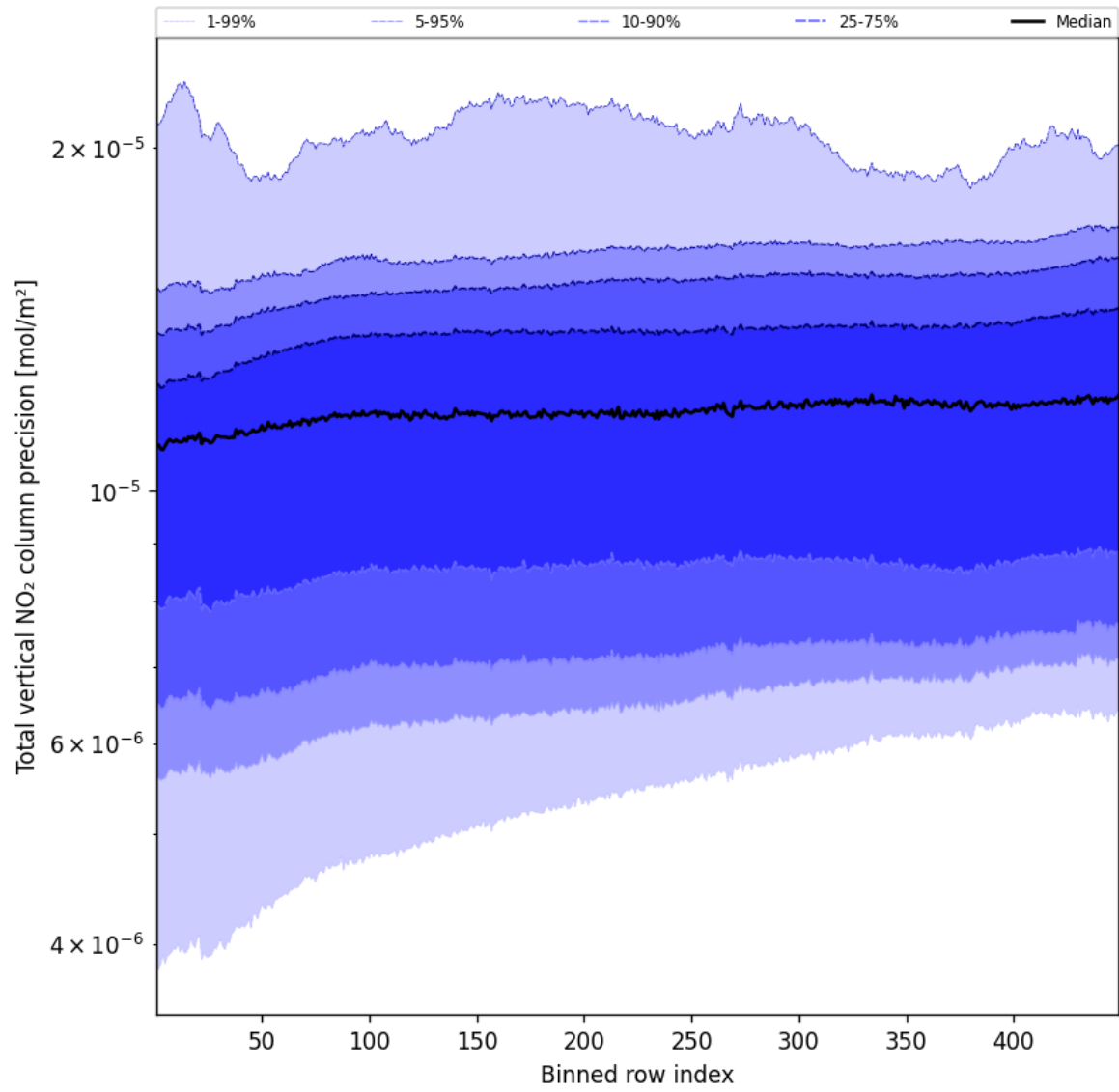
Figure 54: Along track statistics of “Total vertical NO 2 column precision” for 2025-05-01 to 2025-05-02
