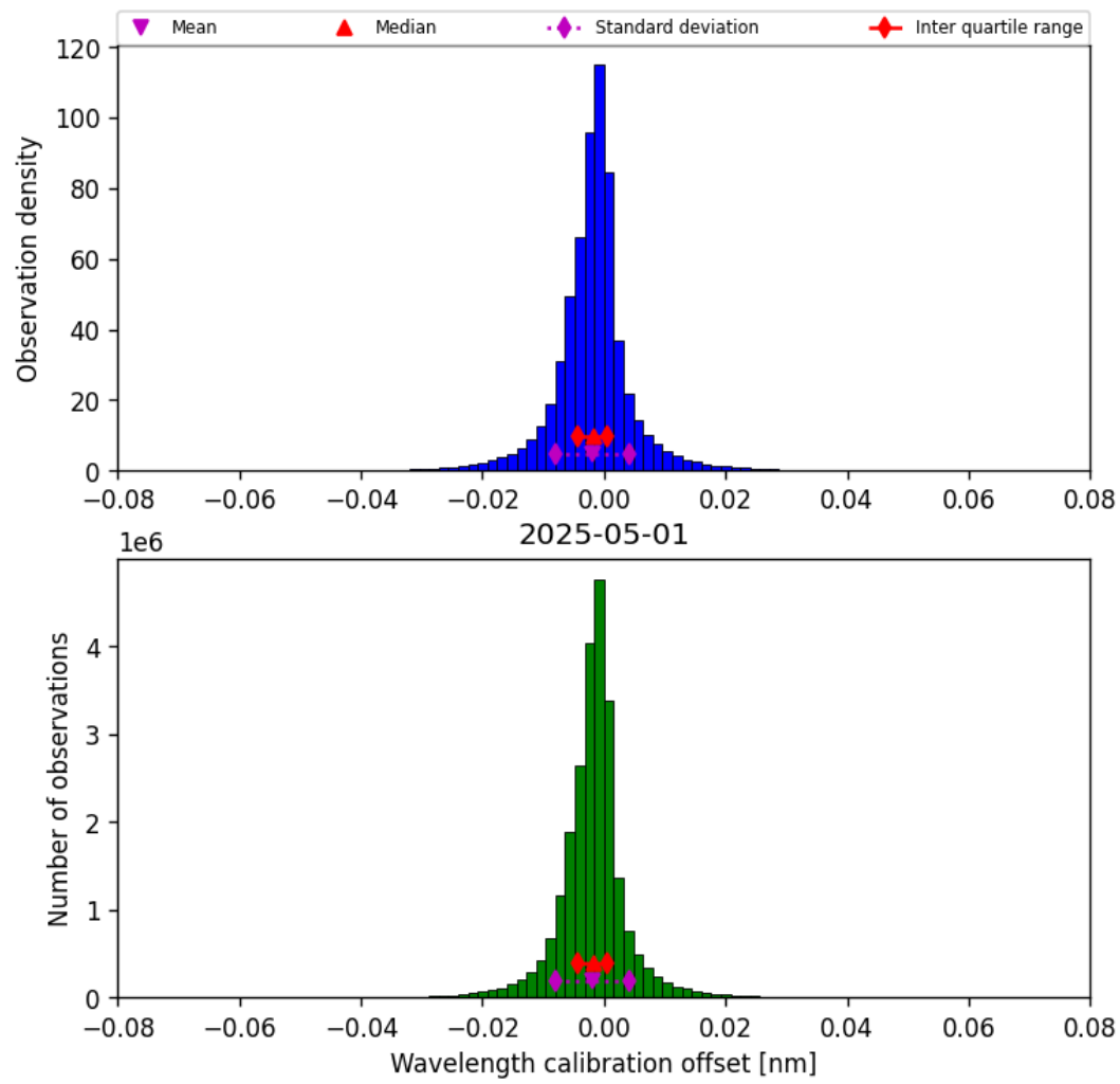
Figure 33: Histogram of “Wavelength calibration offset” for 2025-05-01 to 2025-05-02
