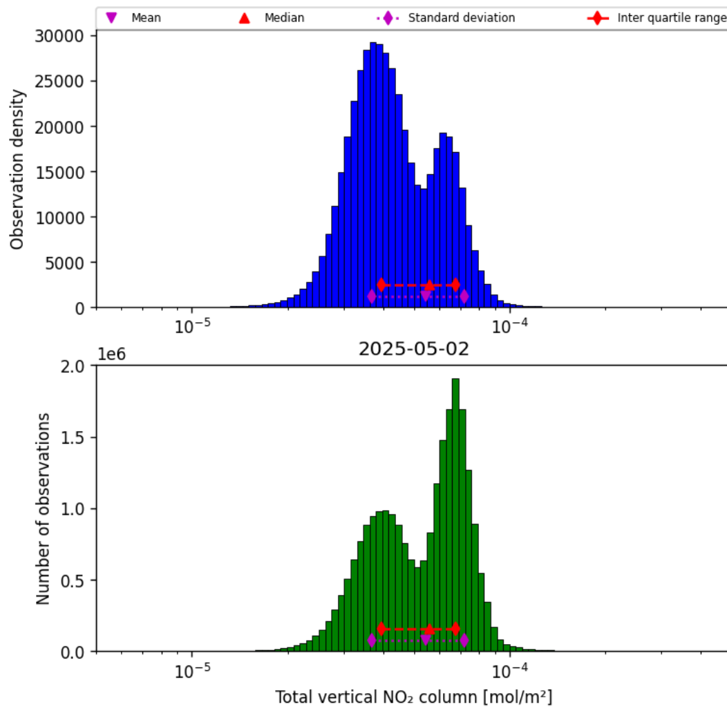
Figure 36: Histogram of "Total vertical NO 2 column" for 2025-05-02 to 2025-05-02
