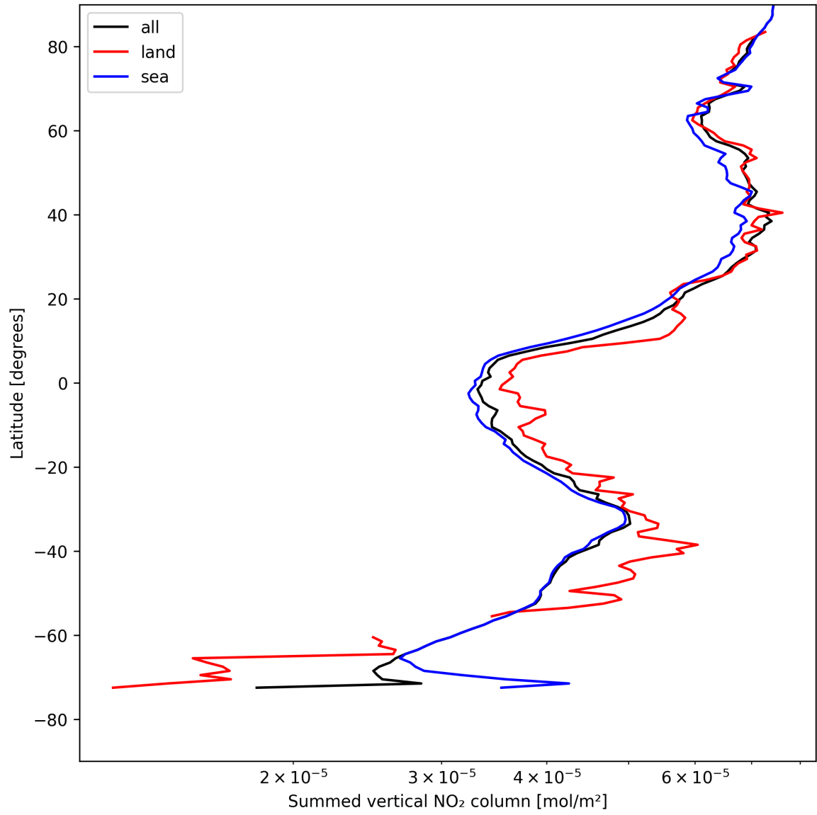
Figure 21: Zonal average of “Summed vertical NO 2 column” for 2025-05-02 to 2025-05-02.
