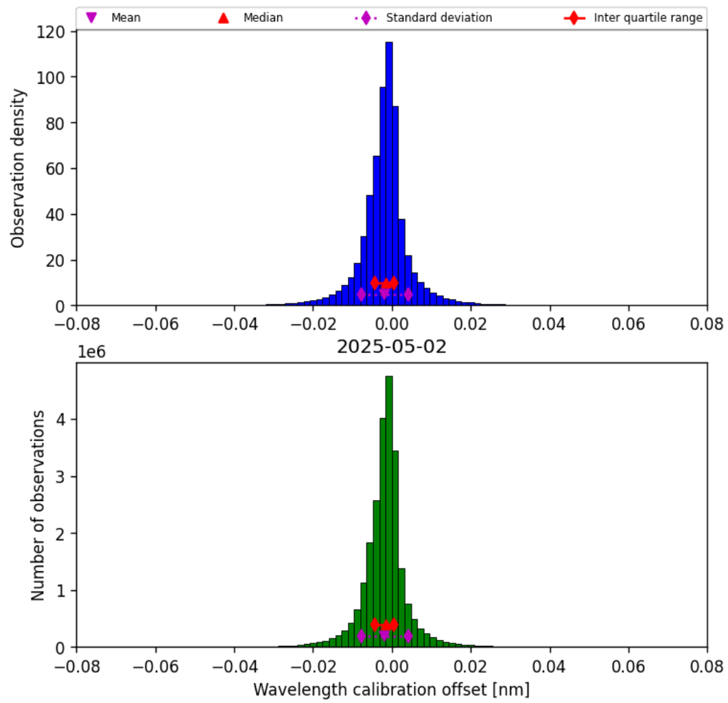
Figure 33: Histogram of “Wavelength calibration offset” for 2025-05-02 to 2025-05-02
