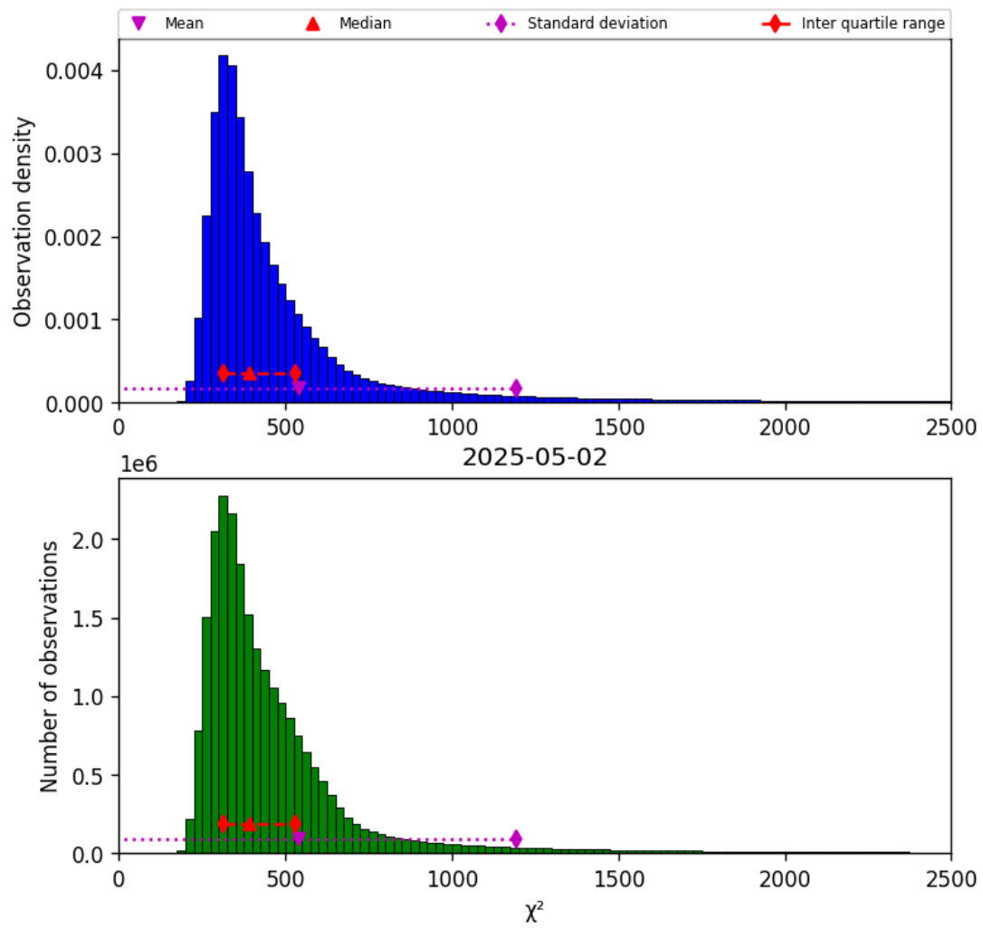
Figure 40: Histogram of “ \chi^2 ” for 2025-05-02 to 2025-05-02
