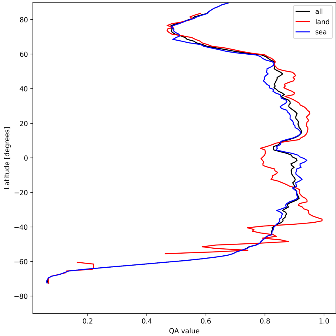
Figure 9: Zonal average of “QA value” for 2025-05-02 to 2025-05-02.
