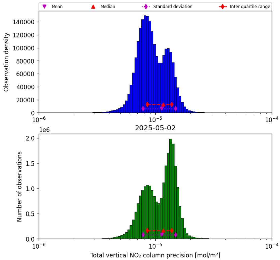
Figure 37: Histogram of "Total vertical NO 2 column precision" for 2025-05-02 to 2025-05-02
