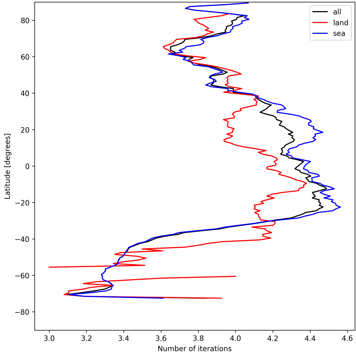
Figure 15: Zonal average of “Number of iterations” for 2025-05-02 to 2025-05-02.
