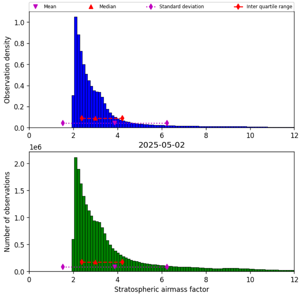
Figure 42: Histogram of “Stratospheric airmass factor” for 2025-05-02 to 2025-05-02
