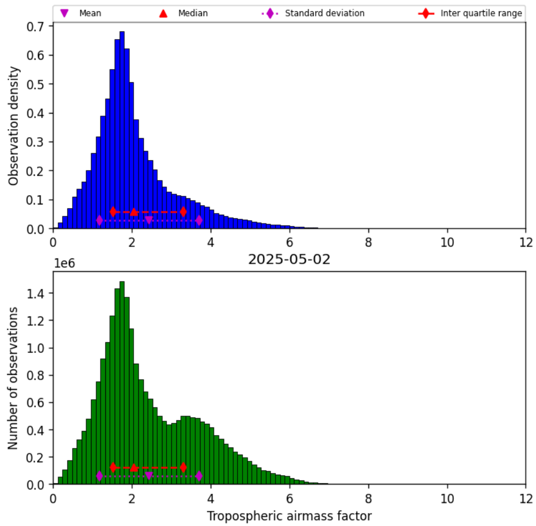
Figure 29: Histogram of “Tropospheric airmass factor” for 2025-05-02 to 2025-05-02
