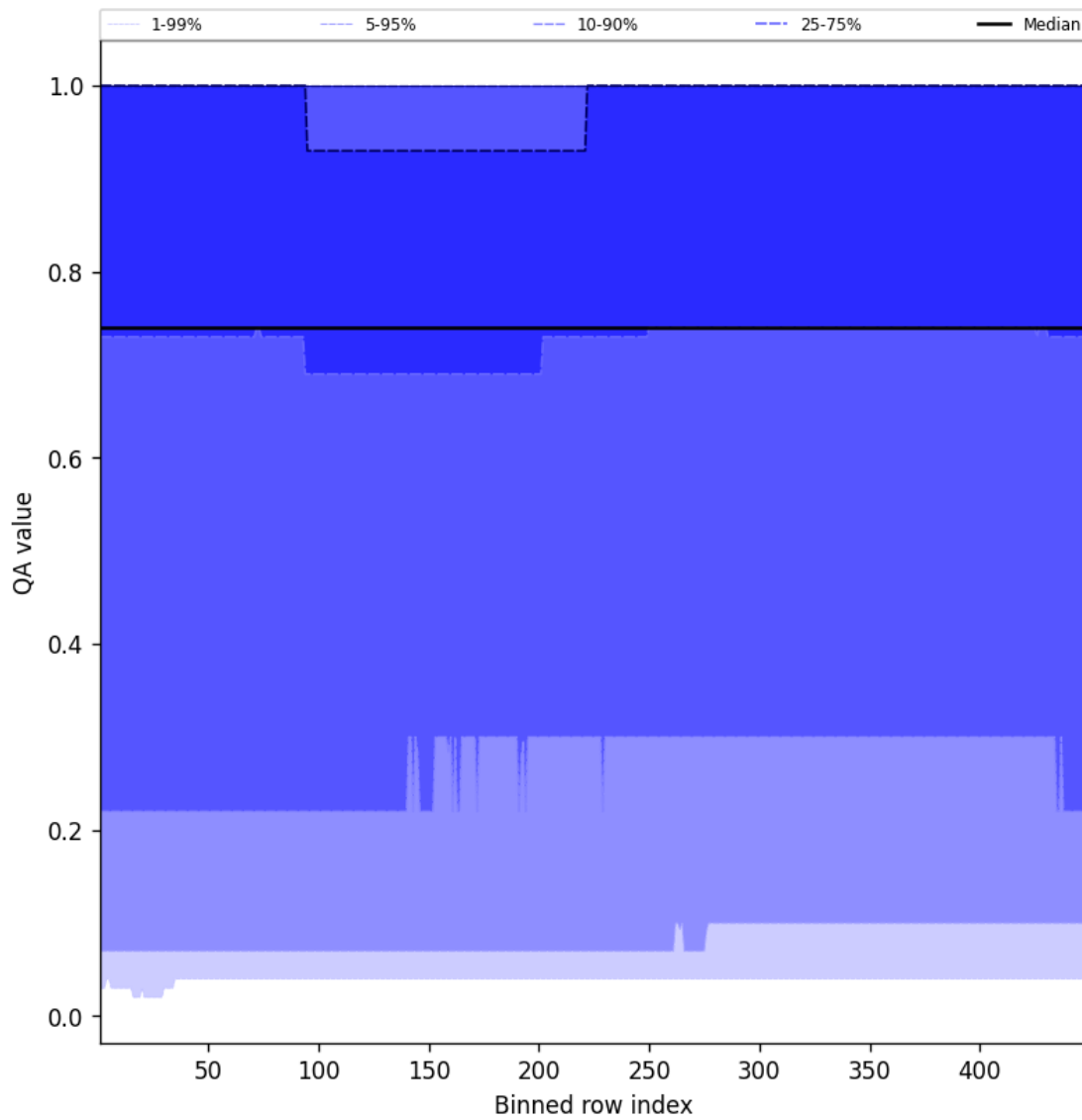
Figure 43: Along track statistics of “QA value” for 2025-05-02 to 2025-05-02
