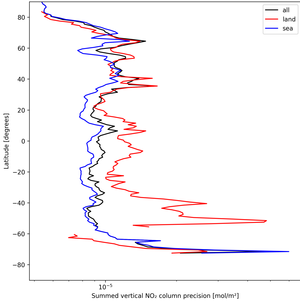
Figure 22: Zonal average of “Summed vertical NO 2 column precision” for 2025-05-02 to 2025-05-02.
