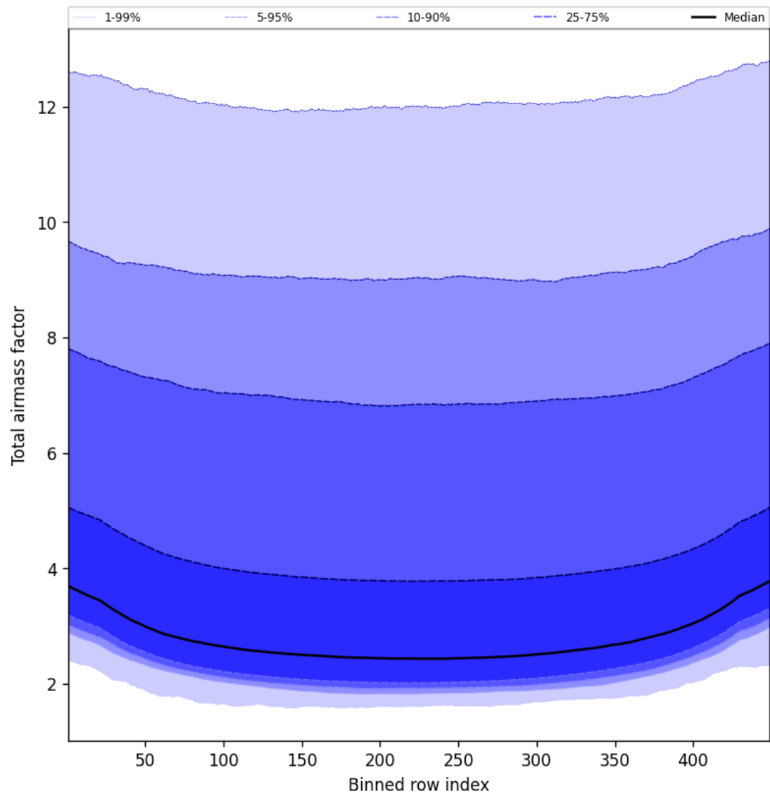
Figure 47: Along track statistics of “Total airmass factor” for 2025-05-02 to 2025-05-02
