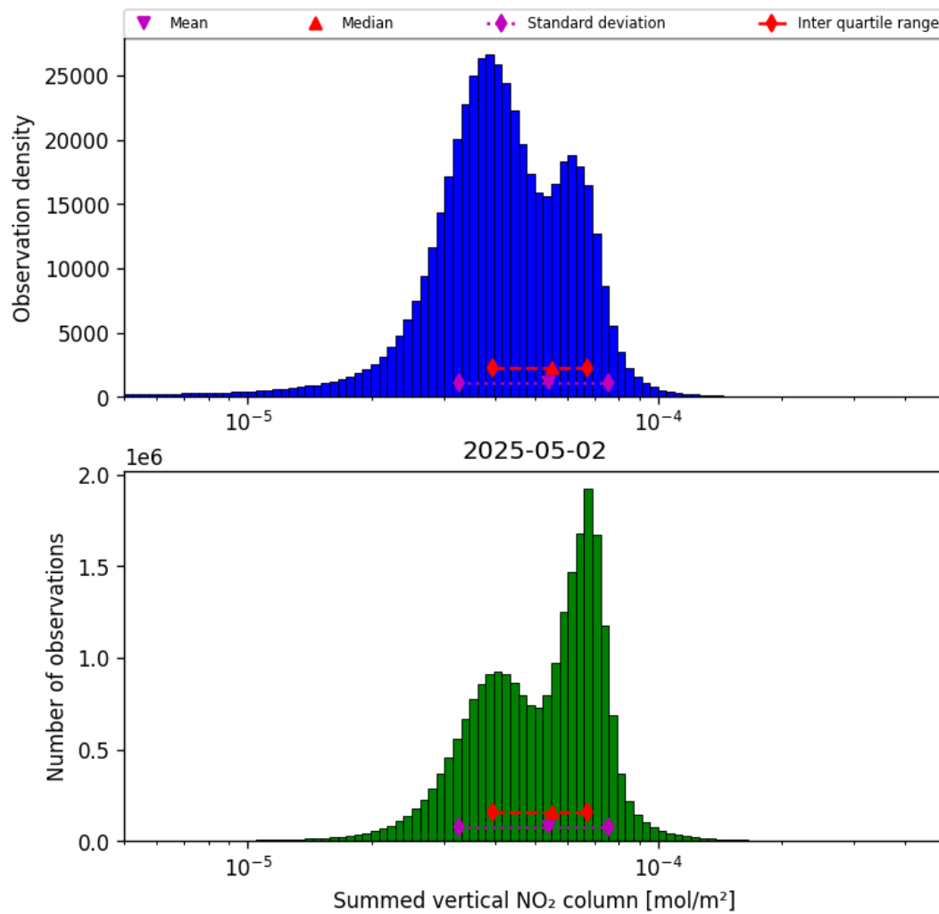
Figure 38: Histogram of "Summed vertical NO 2 column" for 2025-05-02 to 2025-05-02
