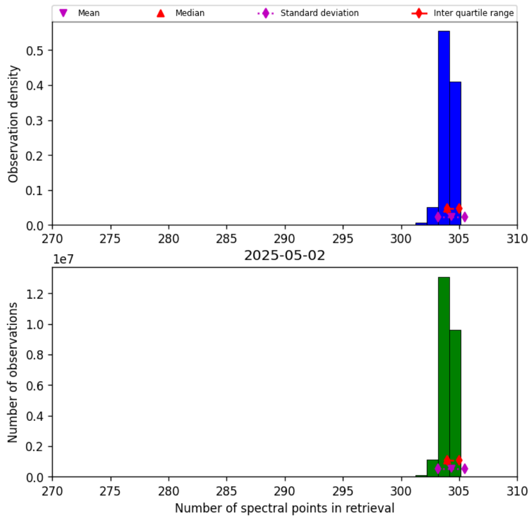
Figure 31: Histogram of “Number of spectral points in retrieval” for 2025-05-02 to 2025-05-02
