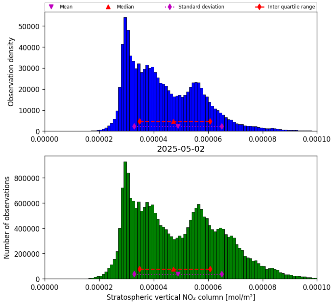
Figure 34: Histogram of “Stratospheric vertical NO 2 column” for 2025-05-02 to 2025-05-02
