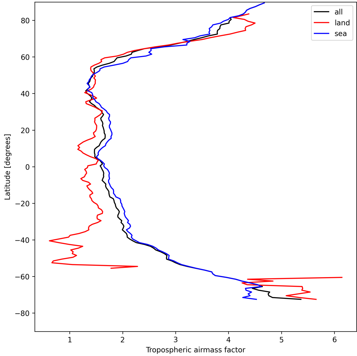
Figure 12: Zonal average of “Tropospheric air mass factor” for 2025-05-02 to 2025-05-02.
