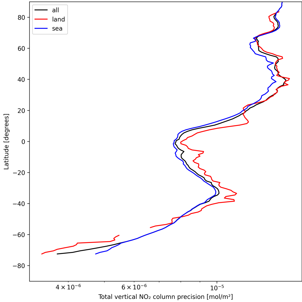
Figure 20: Zonal average of “Total vertical NO 2 column precision” for 2025-05-02 to 2025-05-02.
