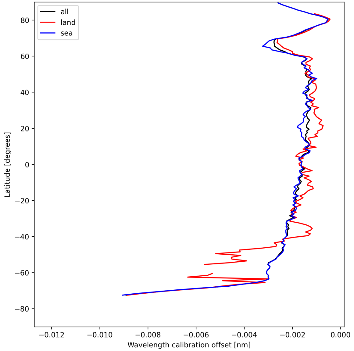
Figure 16: Zonal average of “Wavelength calibration offset” for 2025-05-02 to 2025-05-02.
