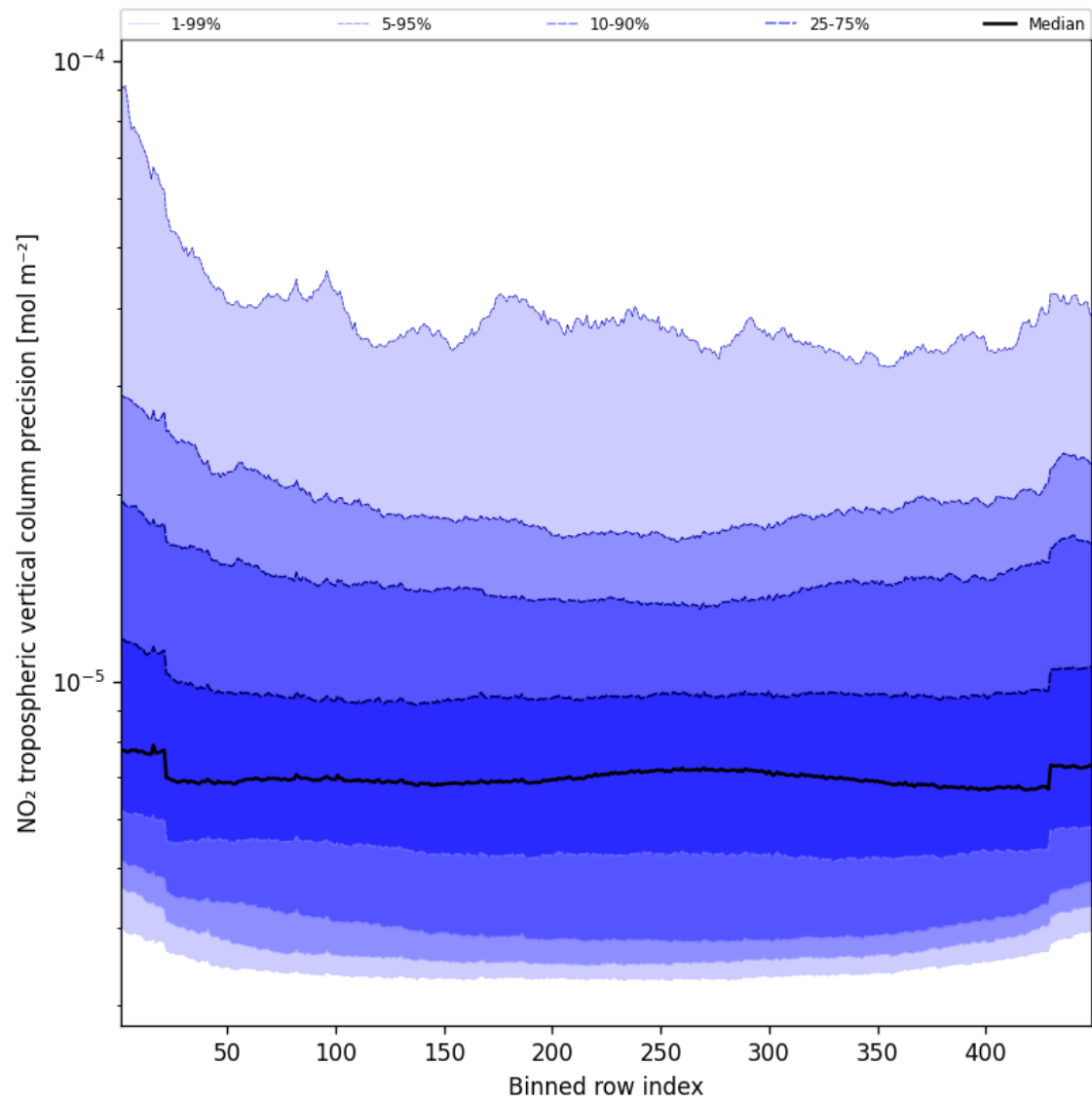
Figure 45: Along track statistics of “NO 2 tropospheric vertical column precision” for 2025-05-02 to 2025-05-02
