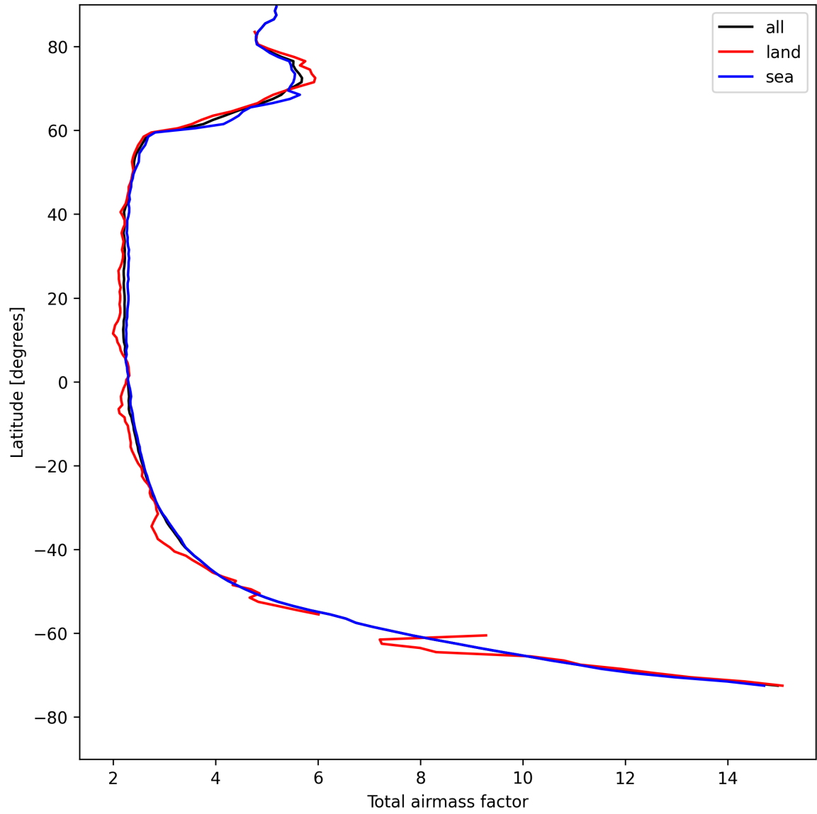
Figure 13: Zonal average of “Total airmass factor” for 2025-05-02 to 2025-05-02.
