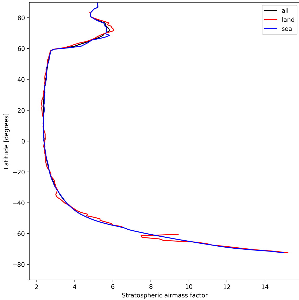
Figure 25: Zonal average of “Stratospheric airmass factor” for 2025-05-02 to 2025-05-02.
