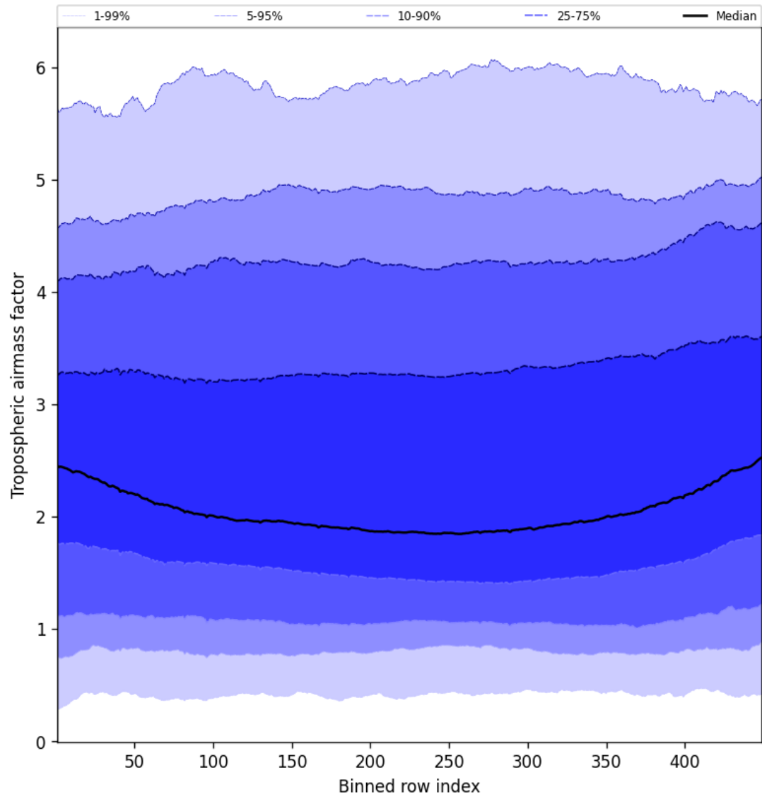
Figure 46: Along track statistics of “Tropospheric airmass factor” for 2025-05-02 to 2025-05-02
