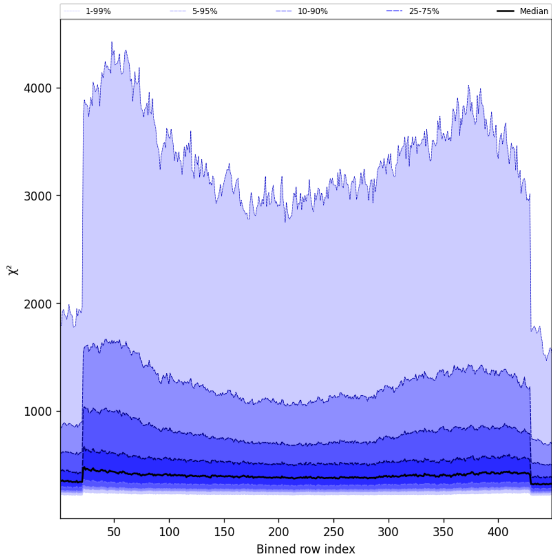
Figure 57: Along track statistics of “ \chi^2 ” for 2025-05-02 to 2025-05-02
