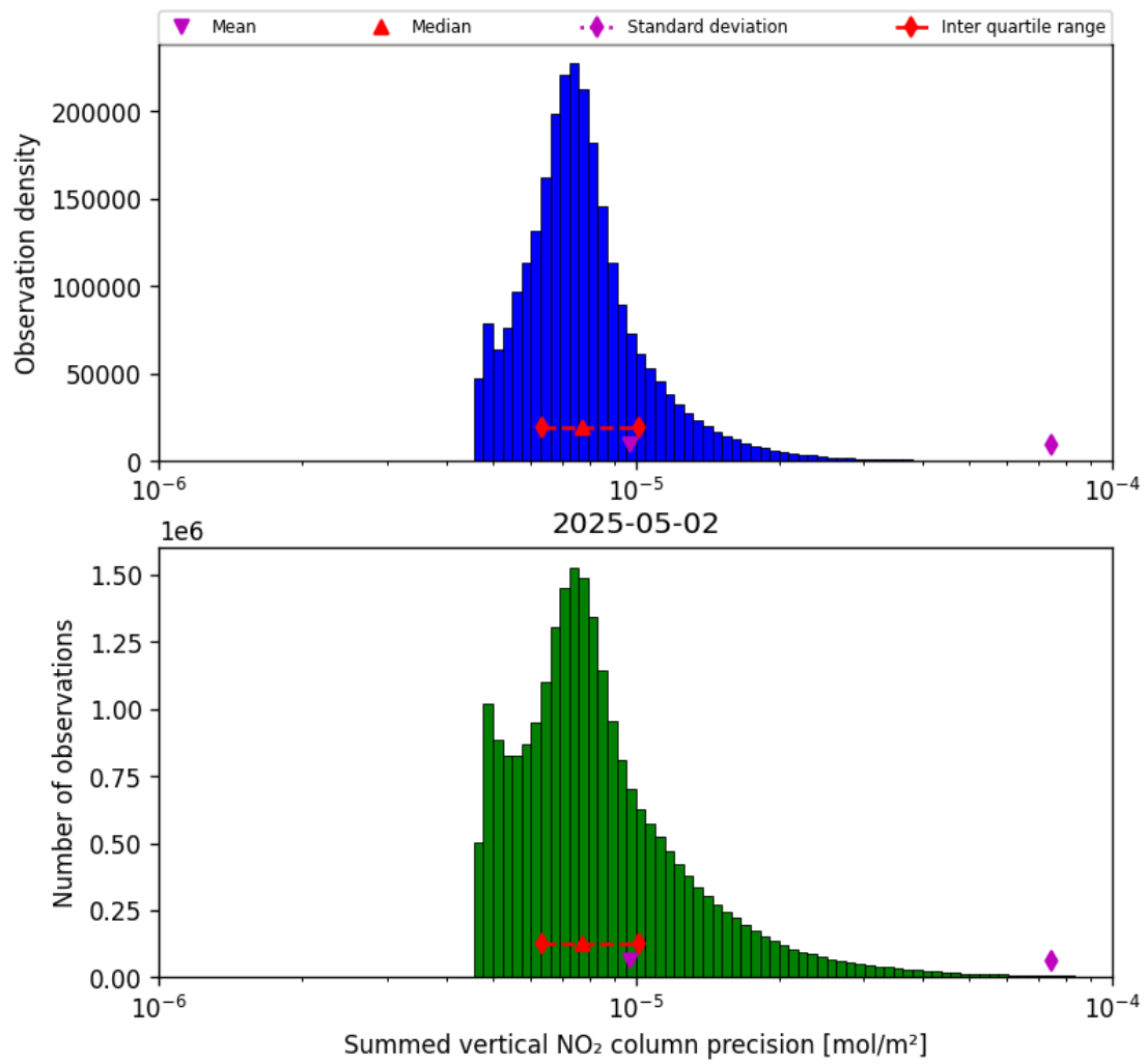
Figure 39: Histogram of "Summed vertical NO 2 column precision" for 2025-05-02 to 2025-05-02
