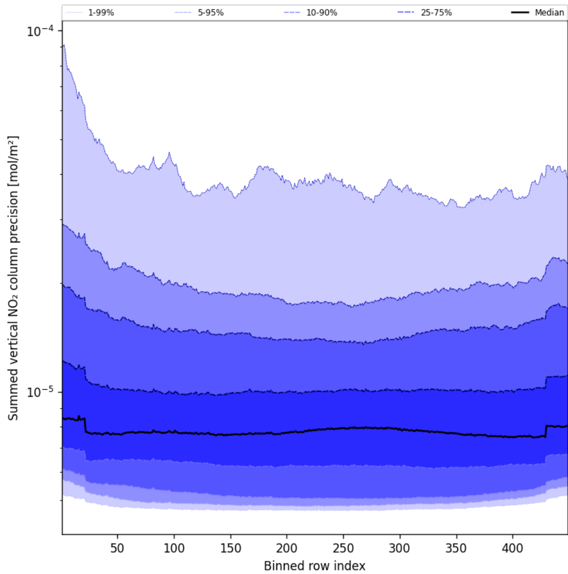
Figure 56: Along track statistics of “Summed vertical NO 2 column precision” for 2025-05-02 to 2025-05-02
