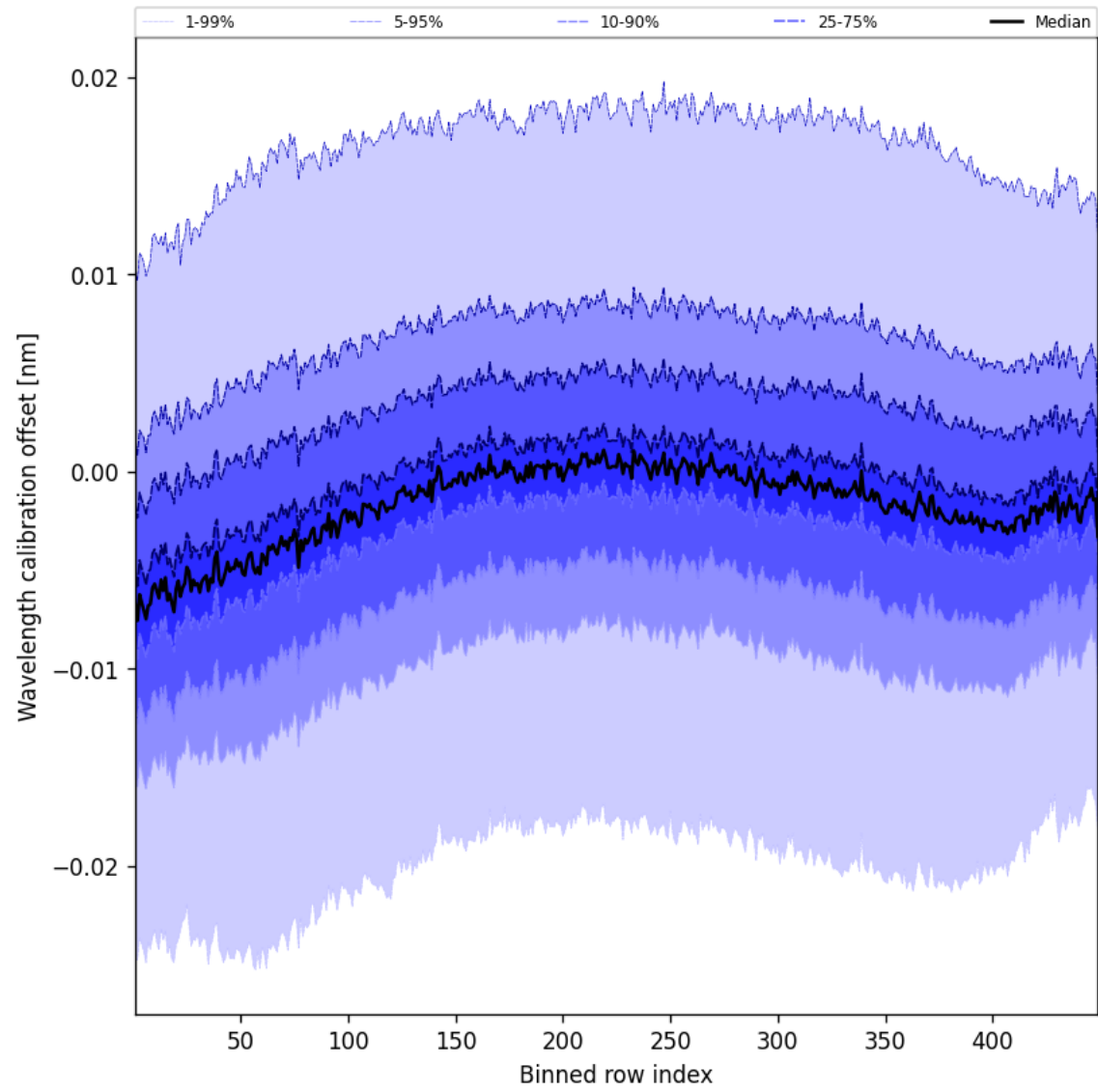
Figure 50: Along track statistics of “Wavelength calibration offset” for 2025-05-02 to 2025-05-02
