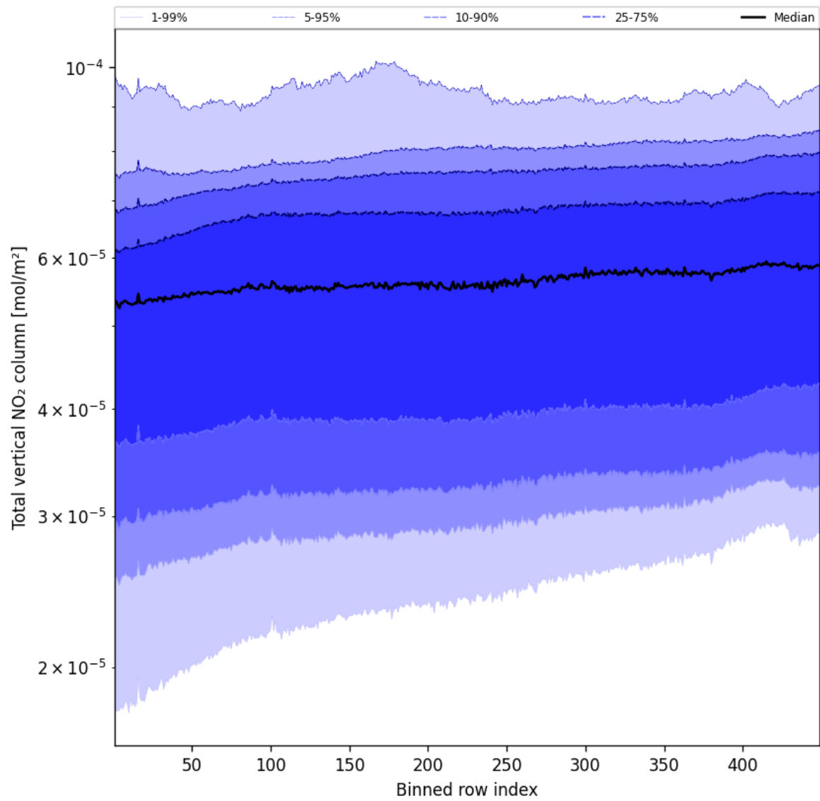
Figure 53: Along track statistics of “Total vertical NO 2 column” for 2025-05-02 to 2025-05-02
