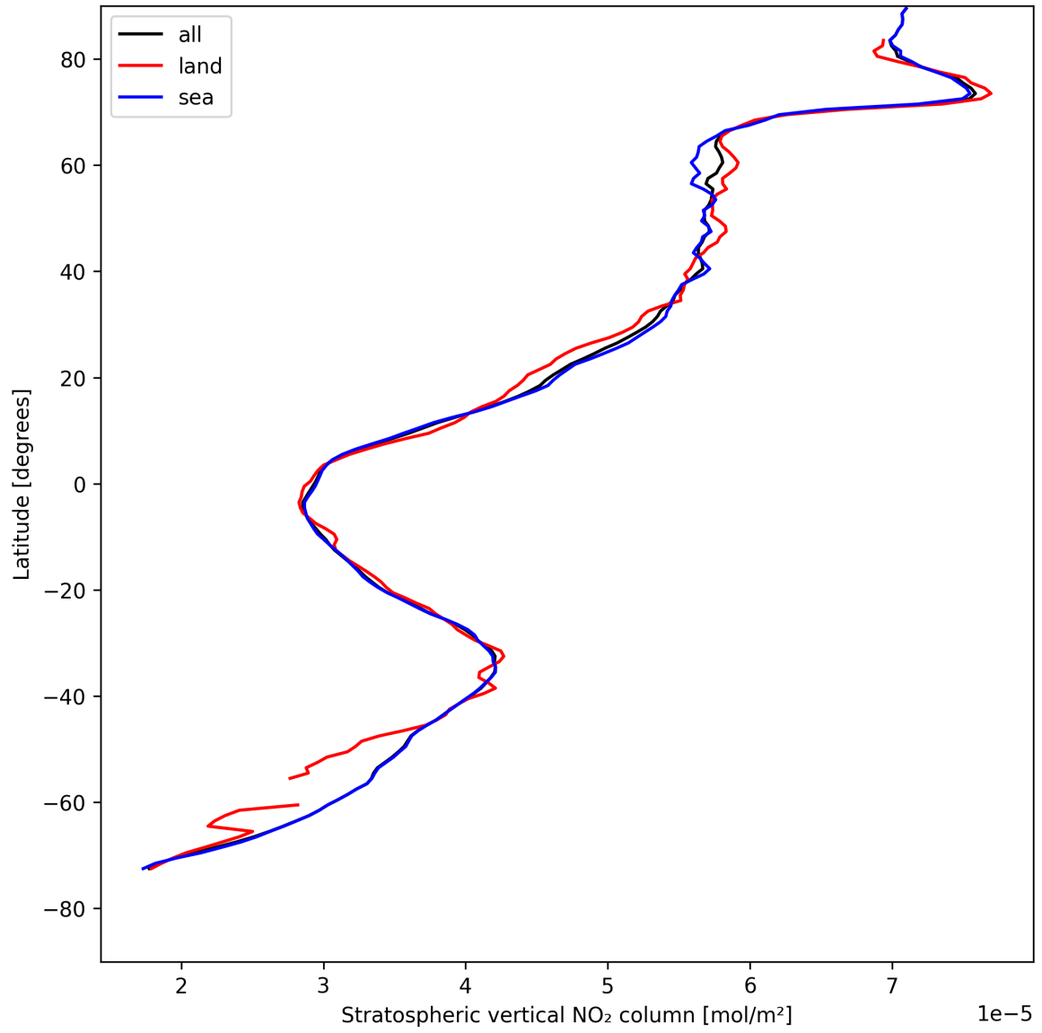
Figure 17: Zonal average of “Stratospheric vertical NO 2 column” for 2025-05-02 to 2025-05-02.
