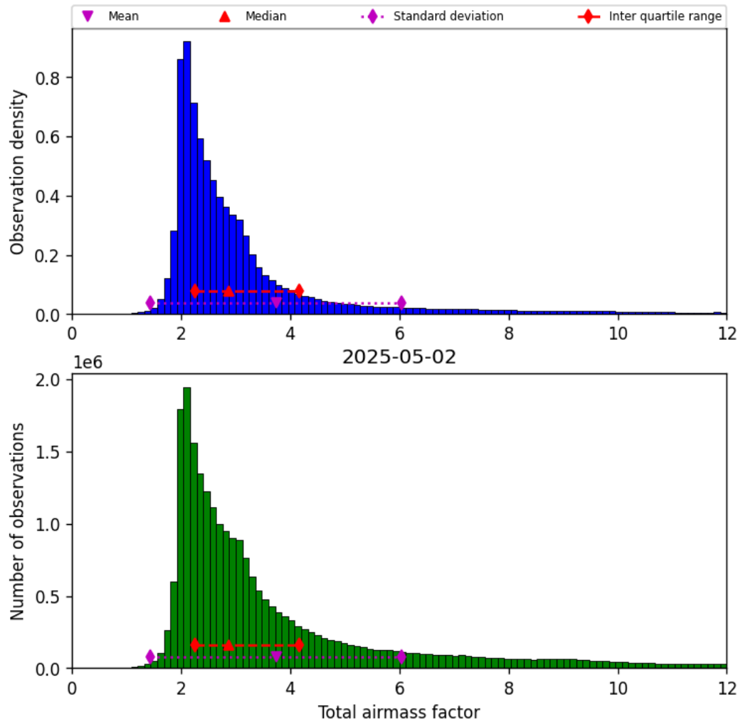
Figure 30: Histogram of “Total airmass factor” for 2025-05-02 to 2025-05-02
