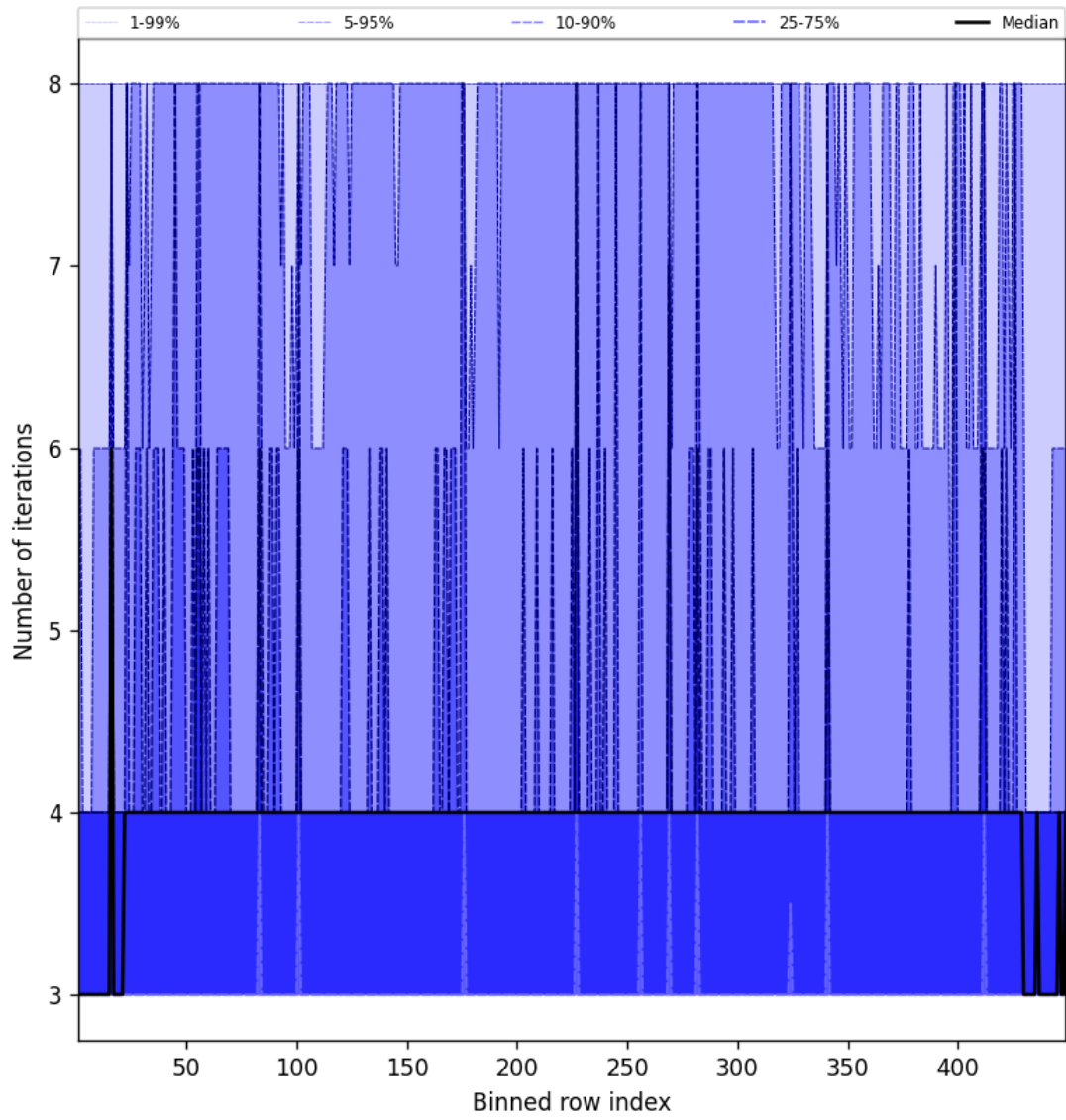
Figure 49: Along track statistics of “Number of iterations” for 2025-05-02 to 2025-05-02
