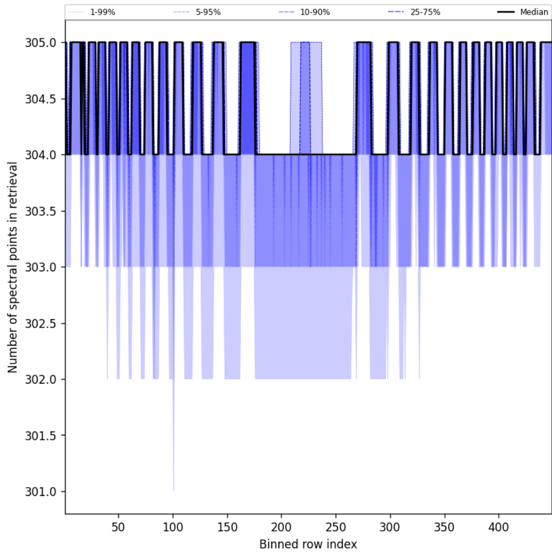
Figure 48: Along track statistics of “Number of spectral points in retrieval” for 2025-05-02 to 2025-05-02
