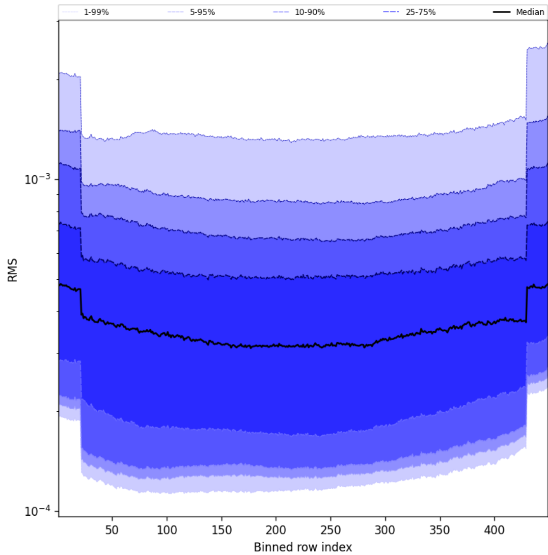
Figure 58: Along track statistics of “RMS” for 2025-05-02 to 2025-05-02
