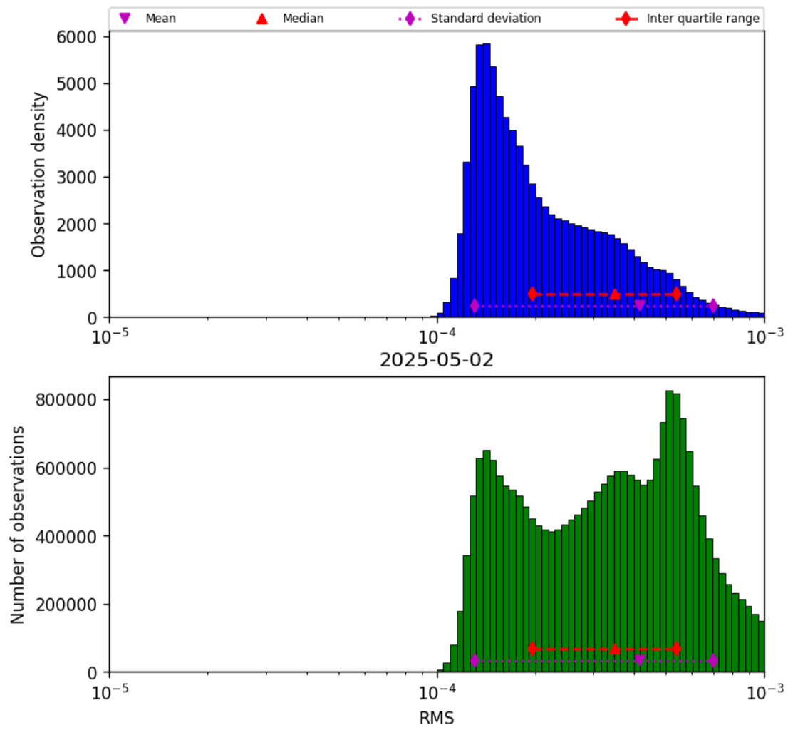
Figure 41: Histogram of “RMS” for 2025-05-02 to 2025-05-02
