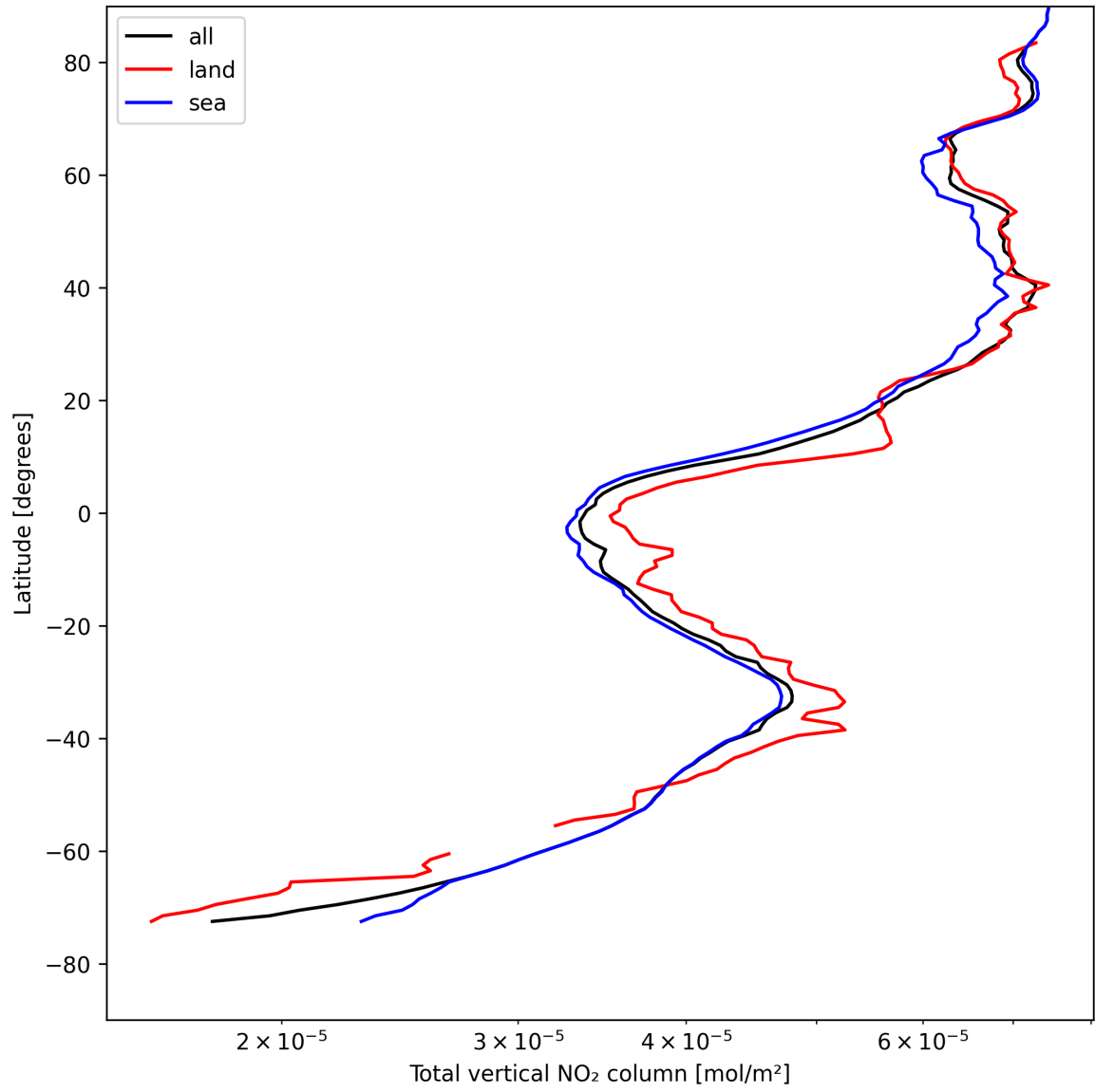
Figure 19: Zonal average of “Total vertical NO 2 column” for 2025-05-02 to 2025-05-02.
