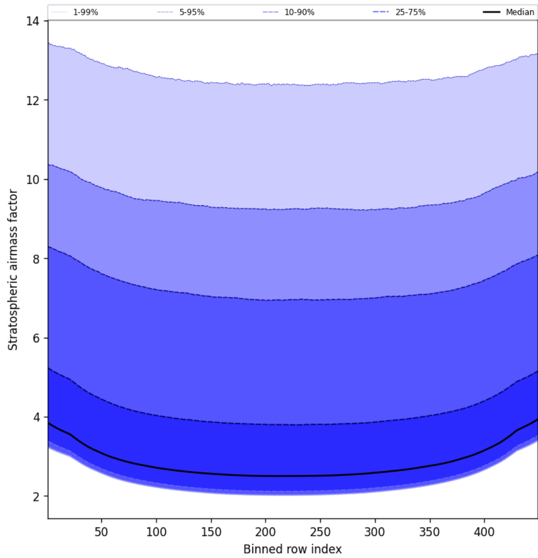
Figure 59: Along track statistics of “Stratospheric airmass factor” for 2025-05-02 to 2025-05-02
