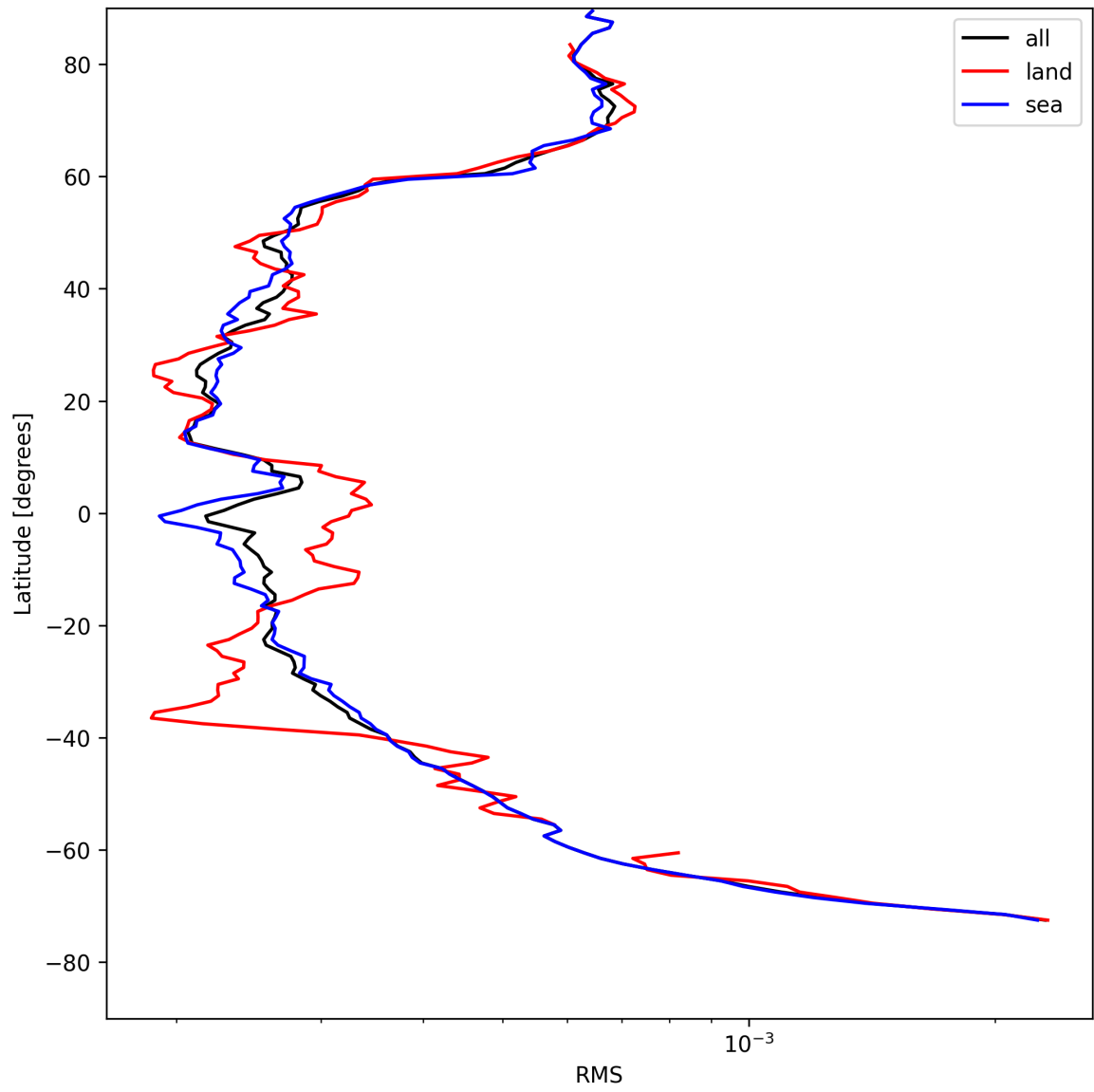
Figure 24: Zonal average of “RMS” for 2025-05-02 to 2025-05-02.
