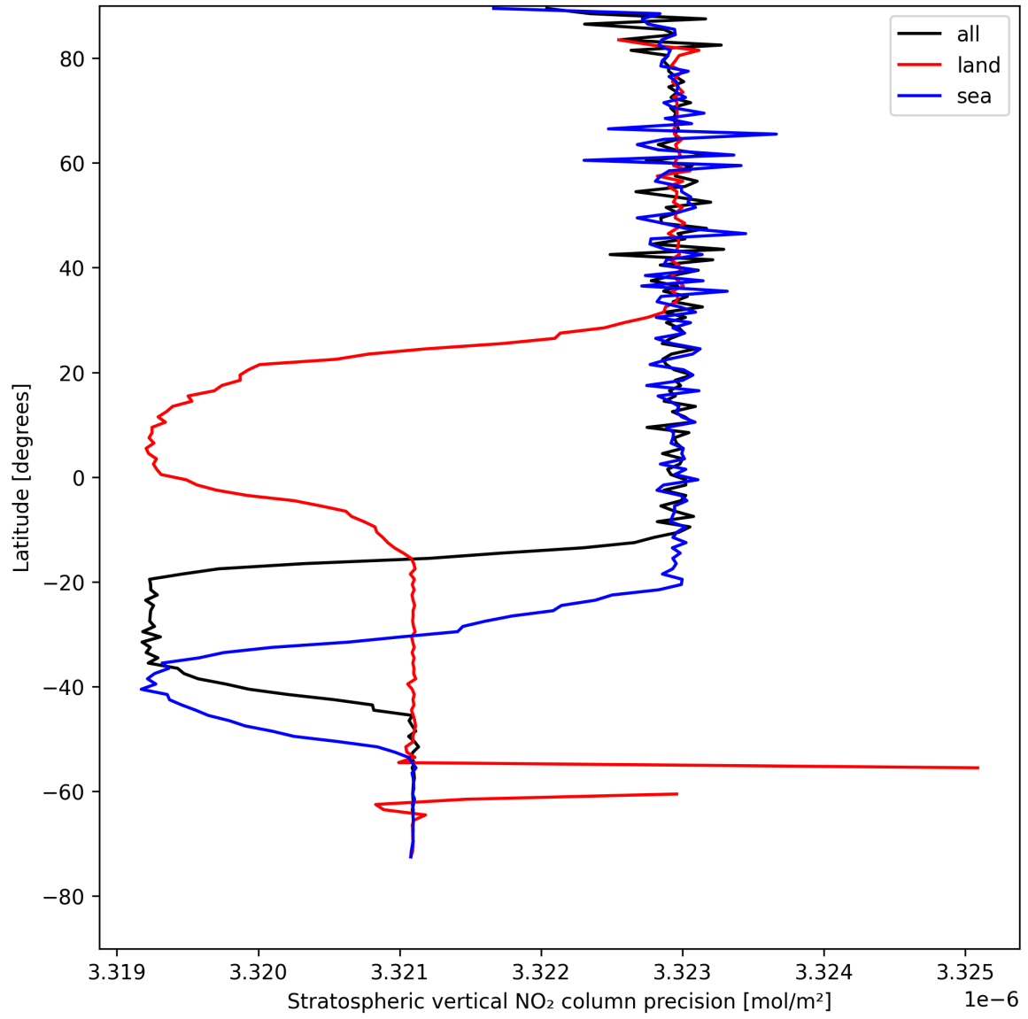
Figure 18: Zonal average of “Stratospheric vertical NO 2 column precision” for 2025-05-02 to 2025-05-02.
