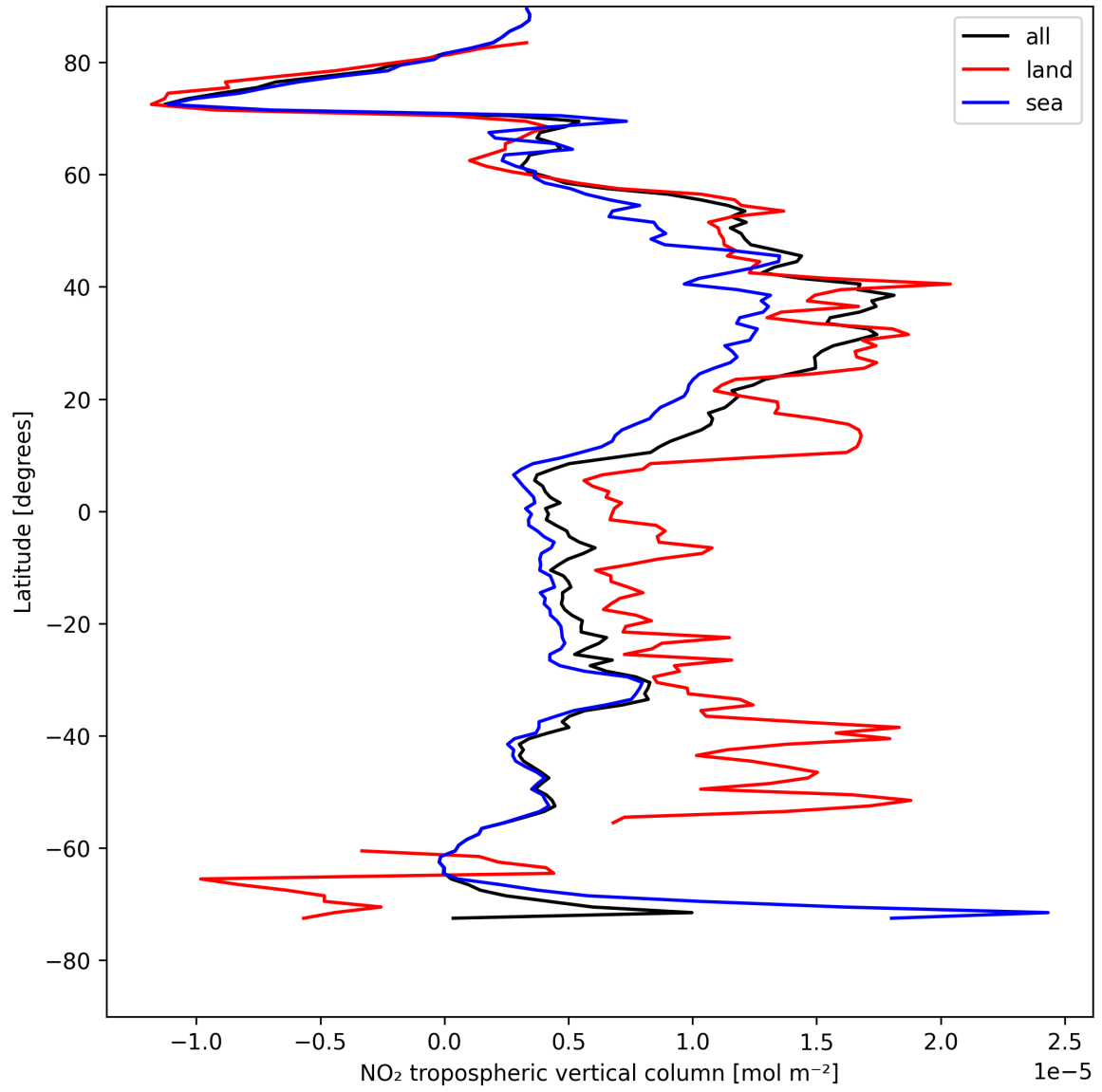
Figure 10: Zonal average of “NO 2 tropospheric vertical column” for 2025-05-02 to 2025-05-02.
