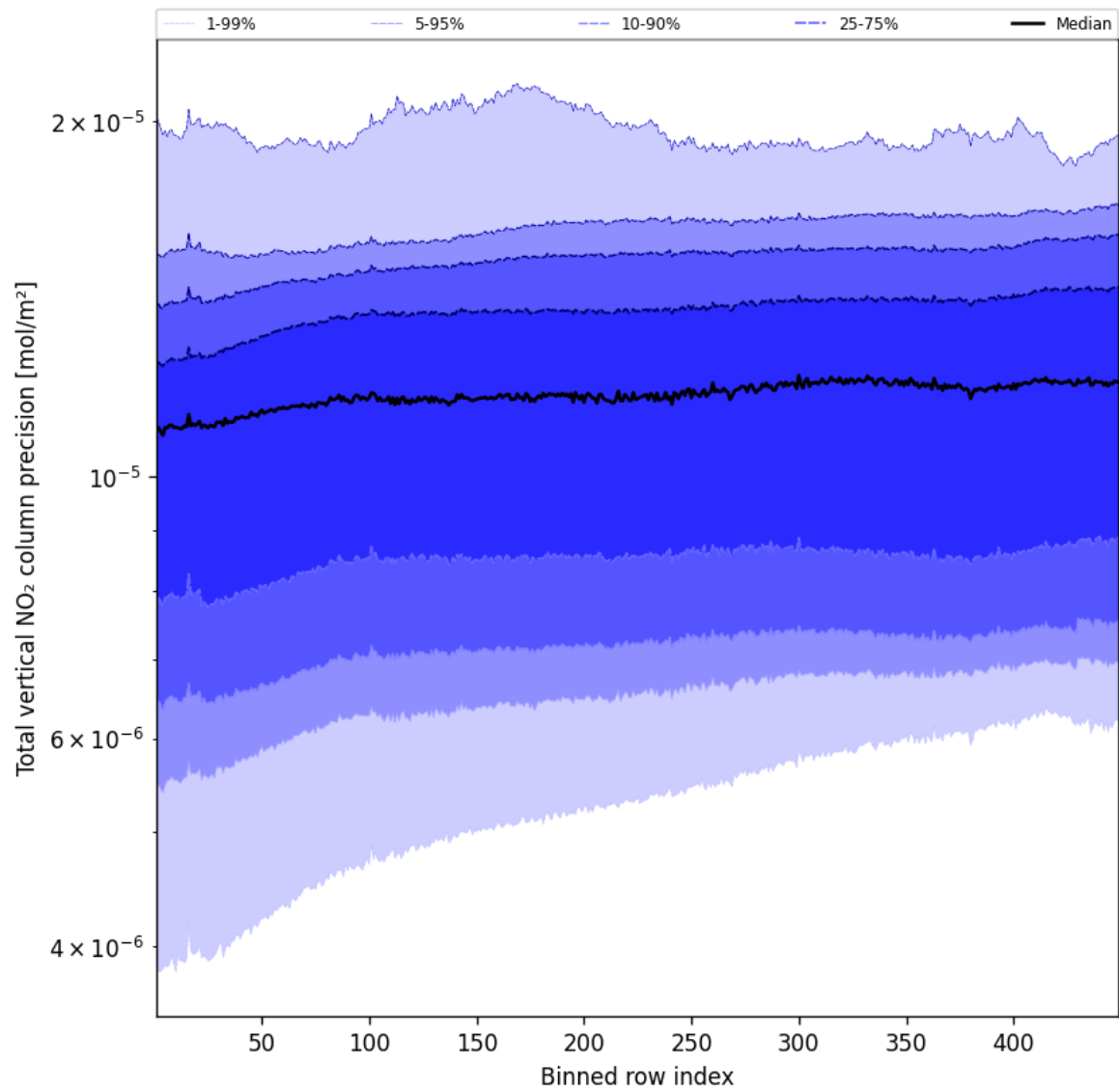
Figure 54: Along track statistics of "Total vertical NO 2 column precision" for 2025-05-02 to 2025-05-02
