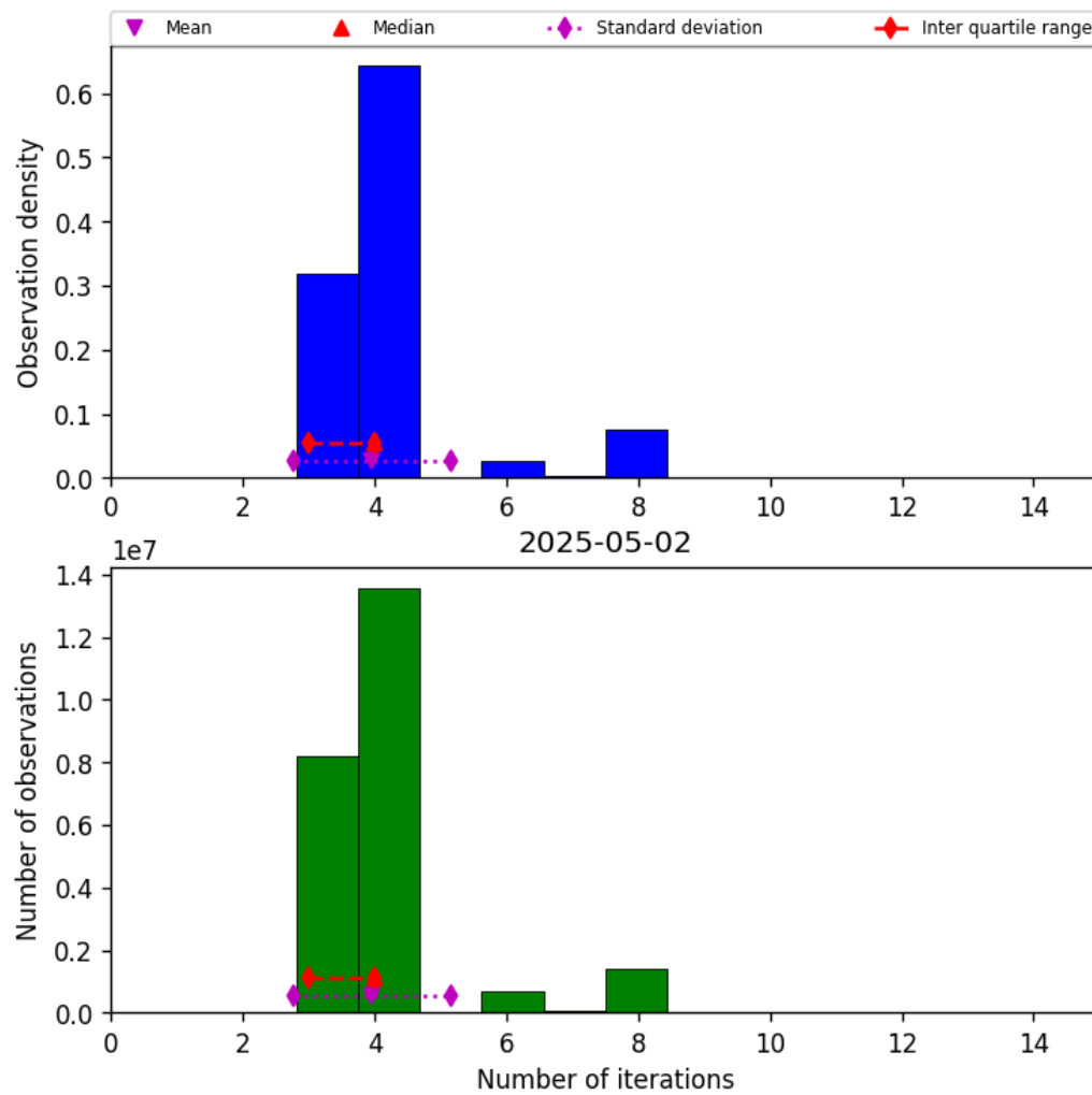
Figure 32: Histogram of “Number of iterations” for 2025-05-02 to 2025-05-02
