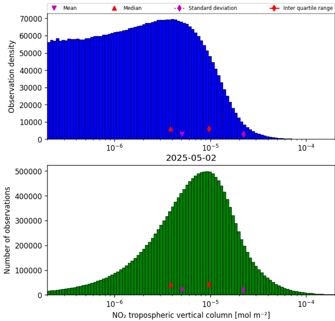
Figure 27: Histogram of “ \text{NO}_2 tropospheric vertical column” for 2025-05-02 to 2025-05-02
