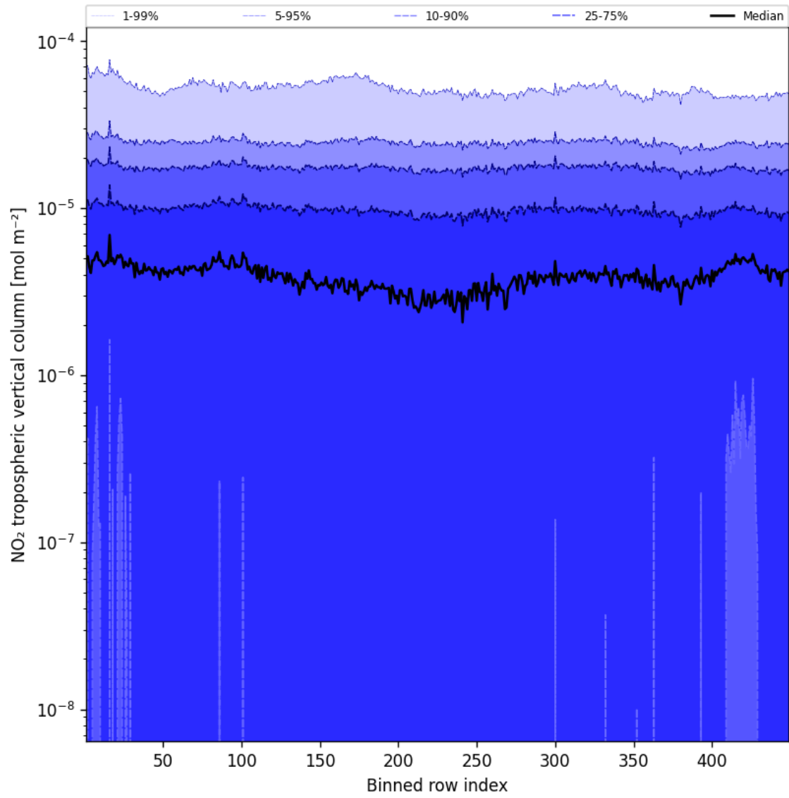
Figure 44: Along track statistics of “NO 2 tropospheric vertical column” for 2025-05-02 to 2025-05-02
