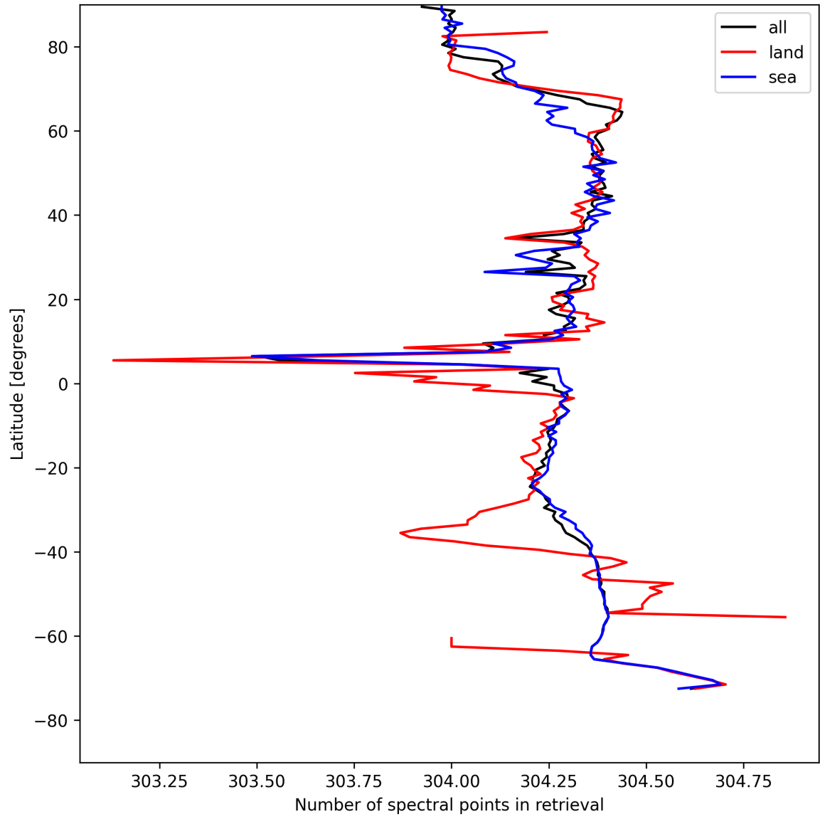
Figure 14: Zonal average of “Number of spectral points in retrieval” for 2025-05-02 to 2025-05-02.
