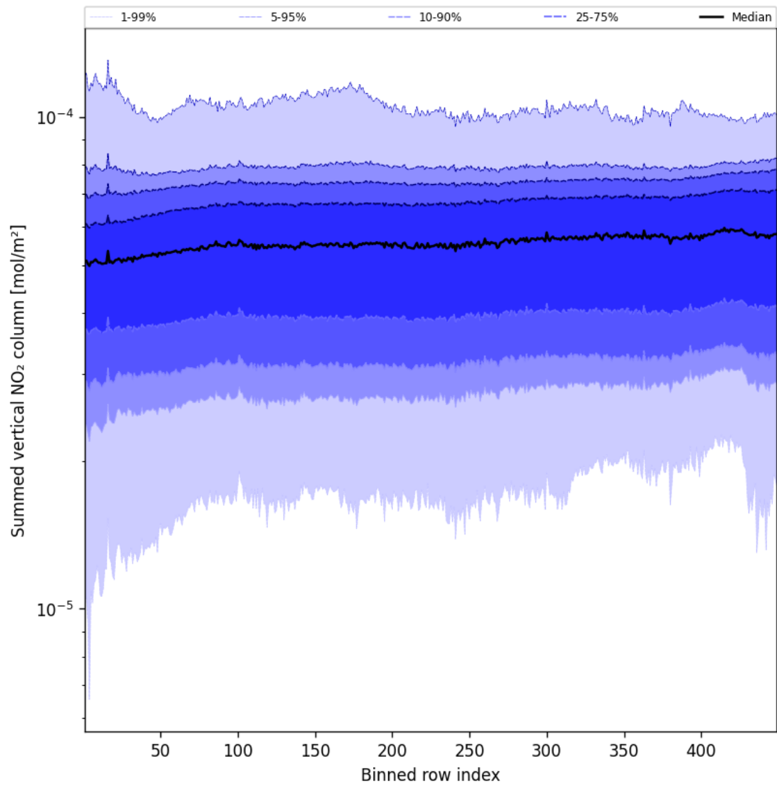
Figure 55: Along track statistics of “Summed vertical NO 2 column” for 2025-05-02 to 2025-05-02
