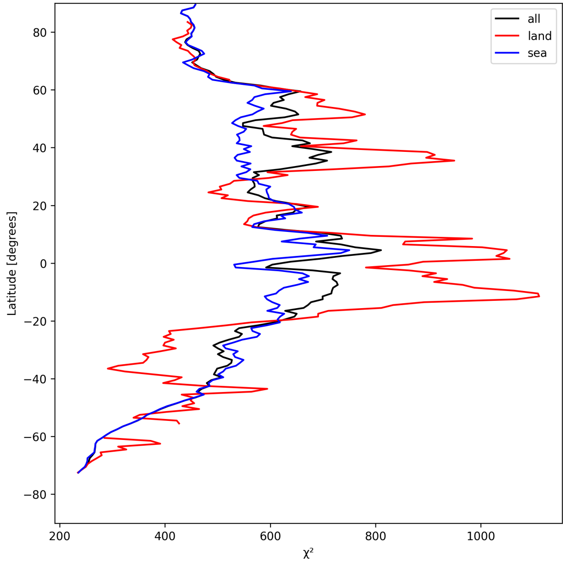
Figure 23: Zonal average of “ \chi^2 ” for 2025-05-02 to 2025-05-02.
