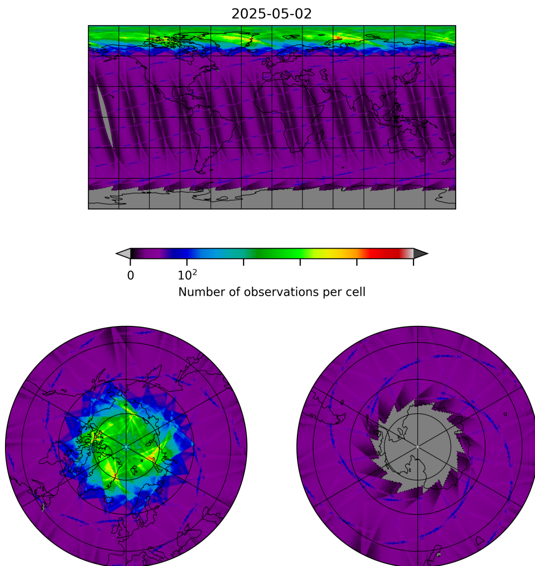
Figure 8: Map of the number of observations for 2025-05-02 to 2025-05-02
