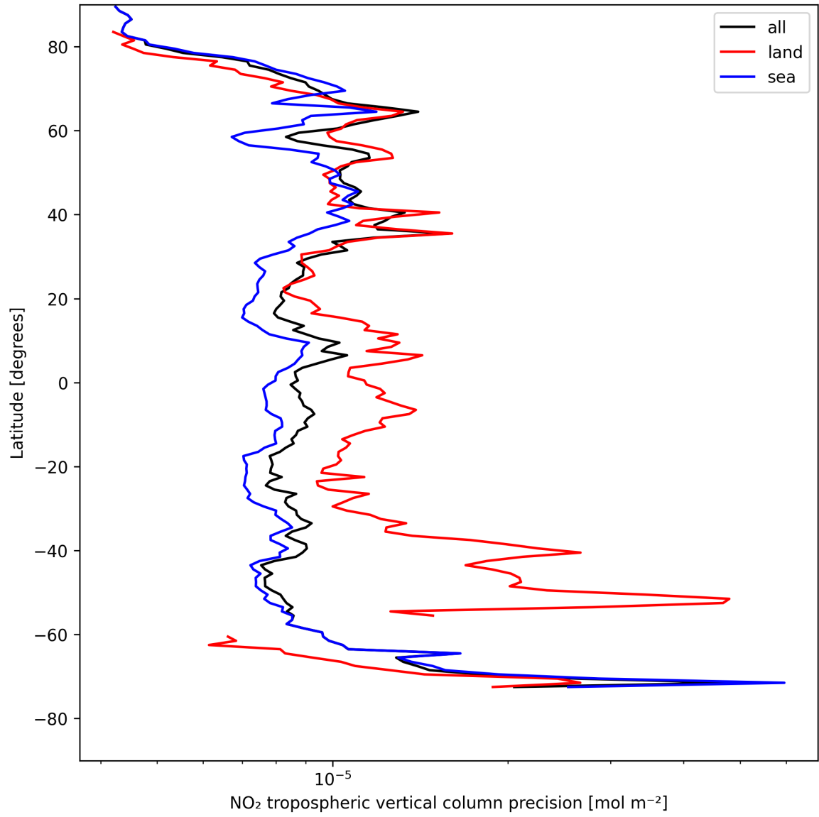
Figure 11: Zonal average of “NO 2 tropospheric vertical column precision” for 2025-05-02 to 2025-05-02.
