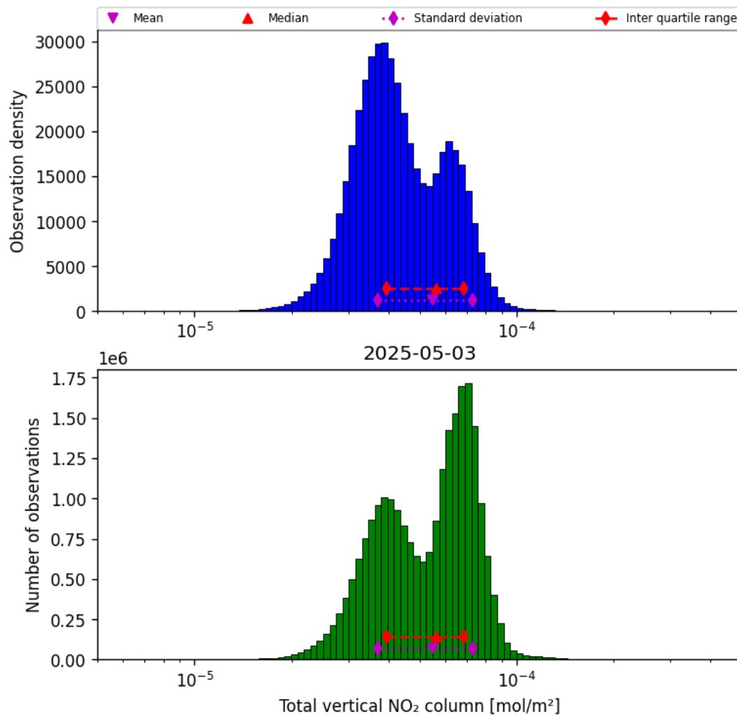
Figure 36: Histogram of "Total vertical NO 2 column" for 2025-05-03 to 2025-05-03
