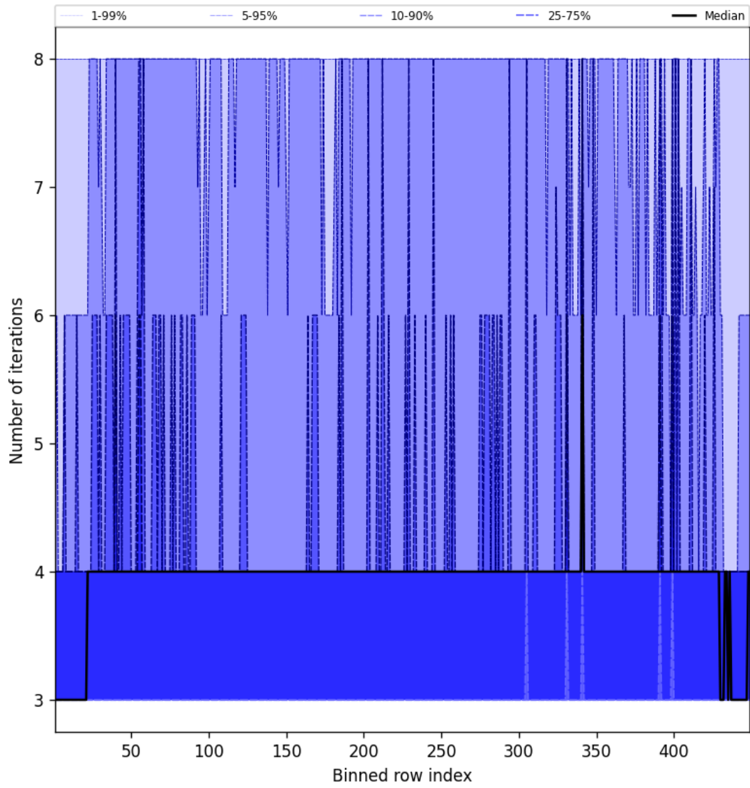
Figure 49: Along track statistics of “Number of iterations” for 2025-05-03 to 2025-05-03
