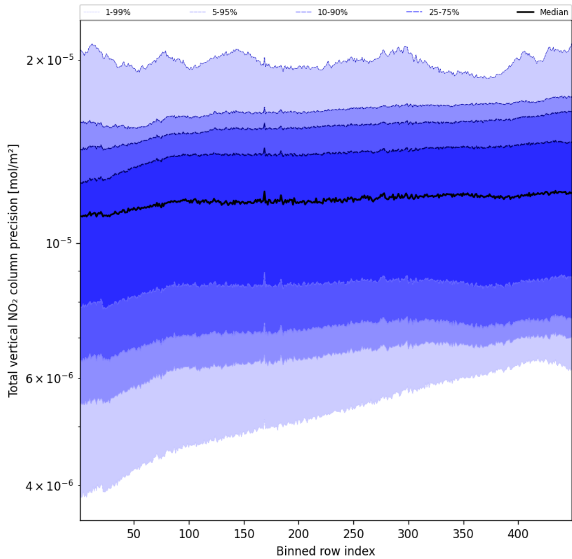
Figure 54: Along track statistics of "Total vertical NO 2 column precision" for 2025-05-03 to 2025-05-03
