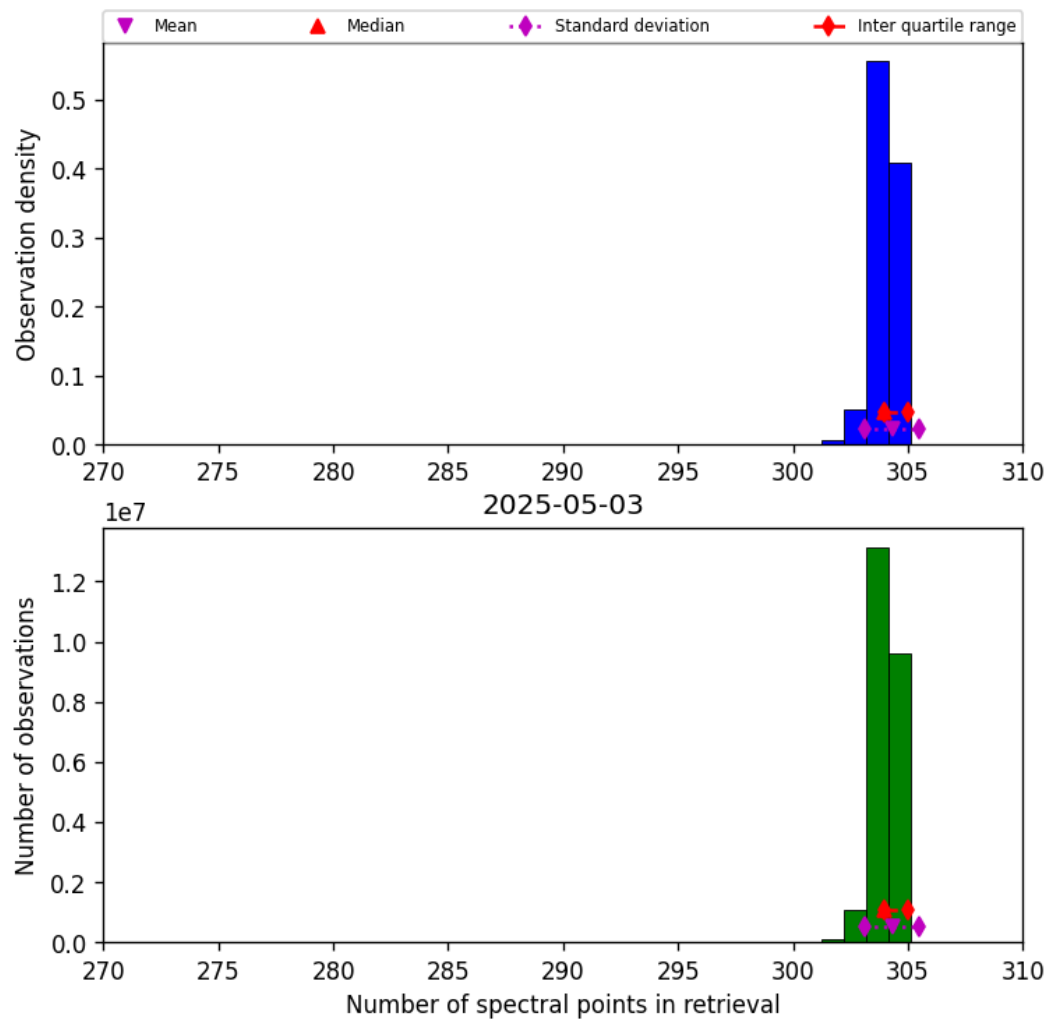
Figure 31: Histogram of “Number of spectral points in retrieval” for 2025-05-03 to 2025-05-03
