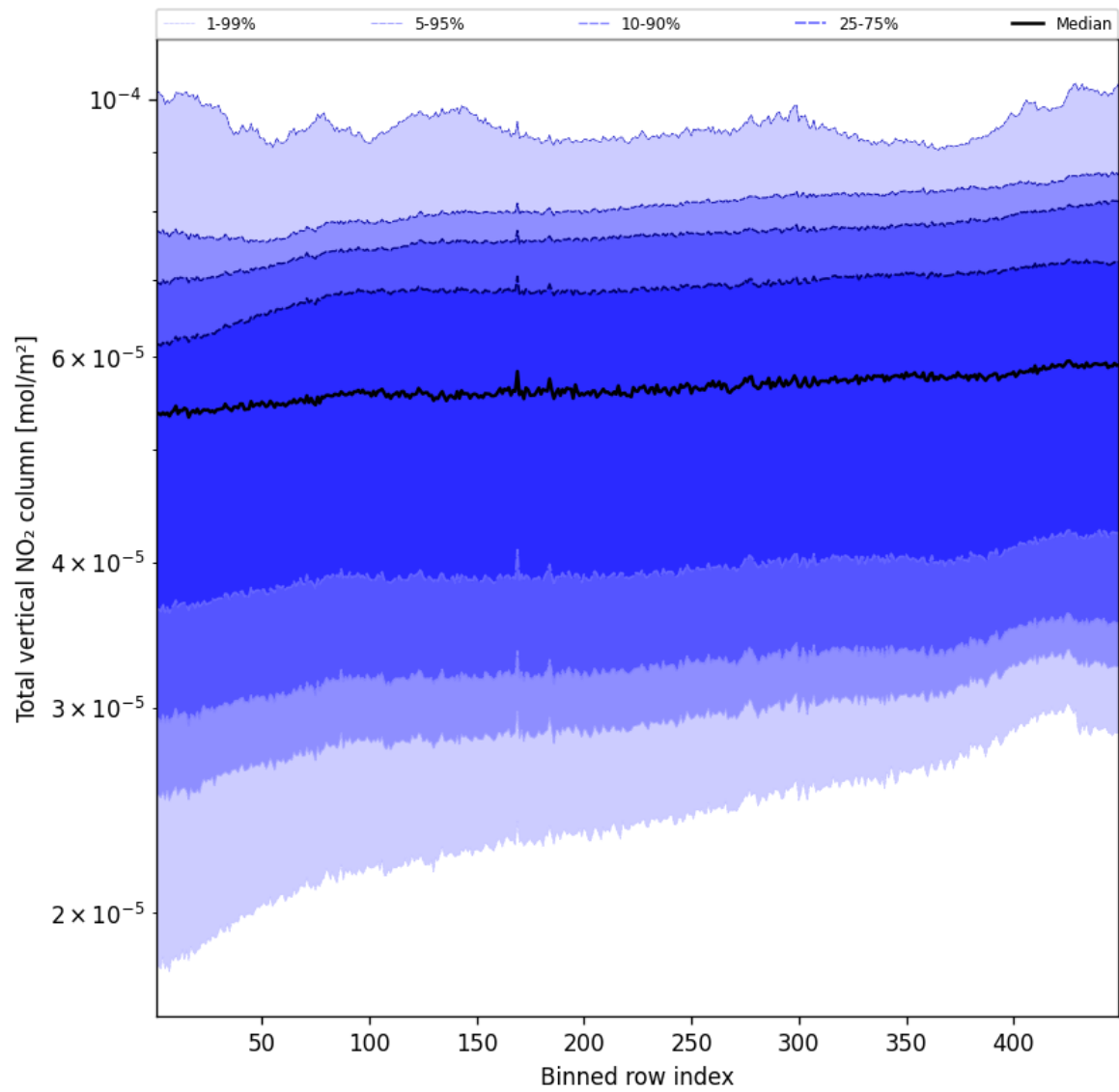
Figure 53: Along track statistics of “Total vertical NO 2 column” for 2025-05-03 to 2025-05-03
