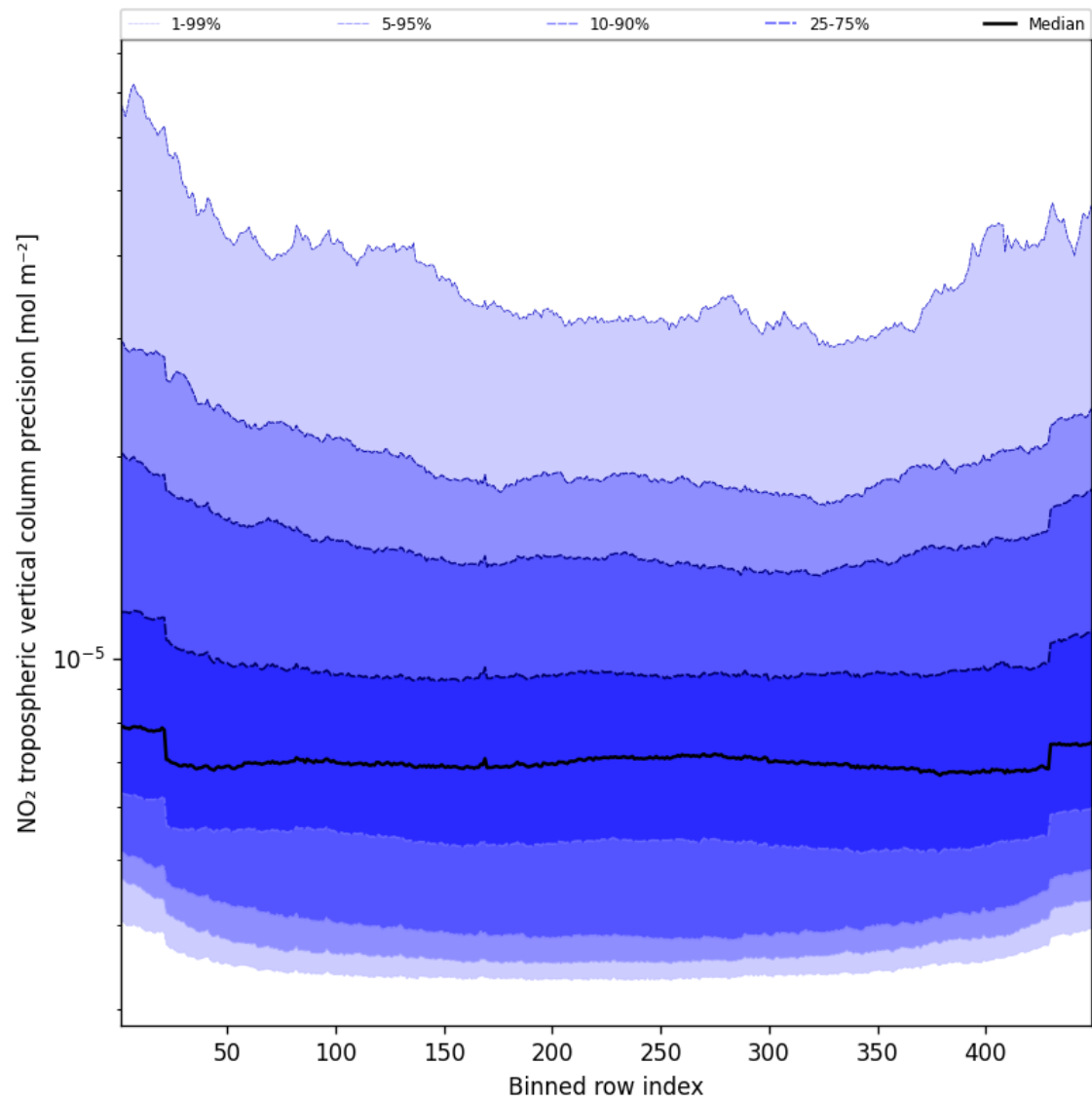
Figure 45: Along track statistics of “NO 2 tropospheric vertical column precision” for 2025-05-03 to 2025-05-03
