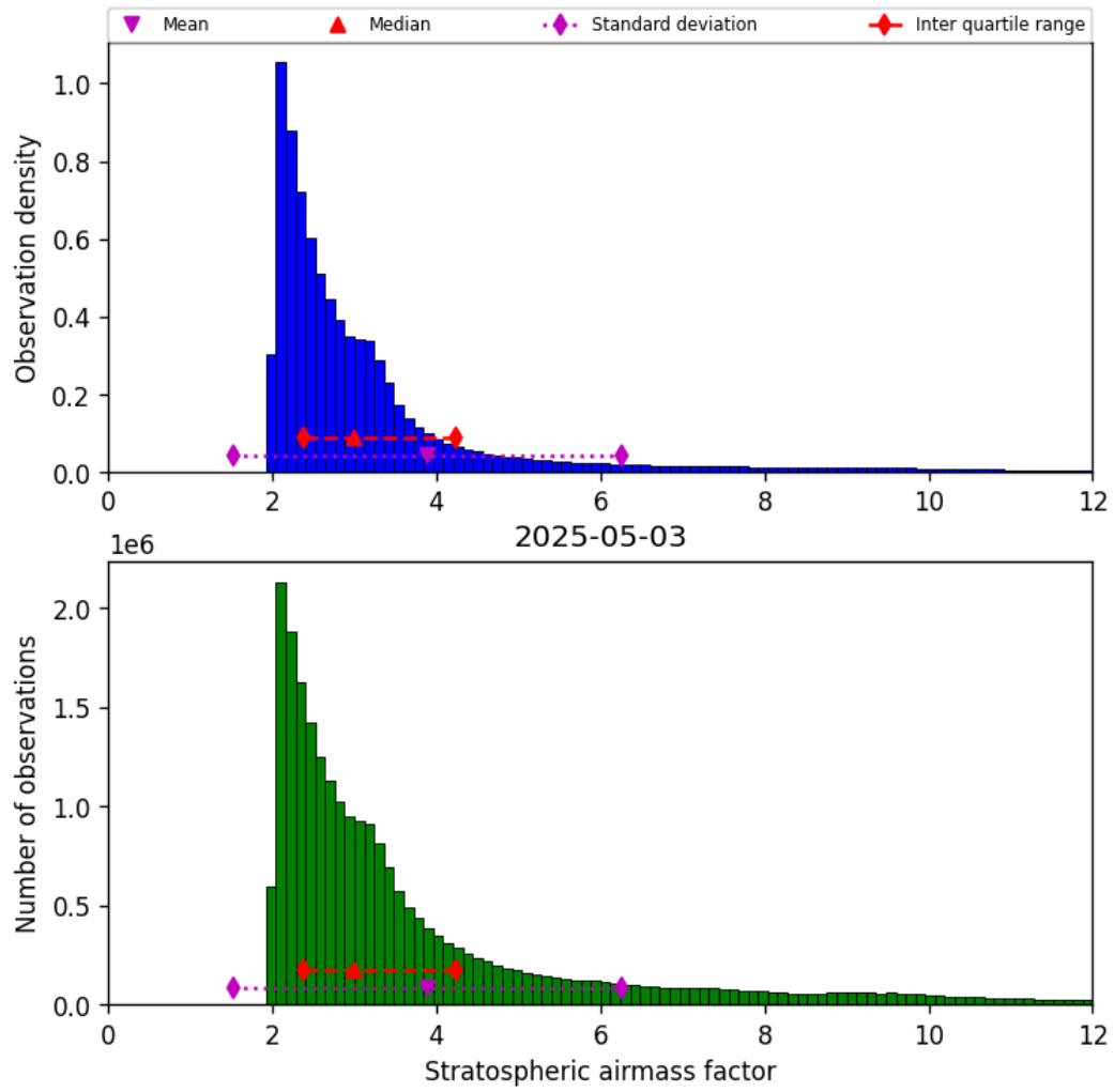
Figure 42: Histogram of “Stratospheric airmass factor” for 2025-05-03 to 2025-05-03
