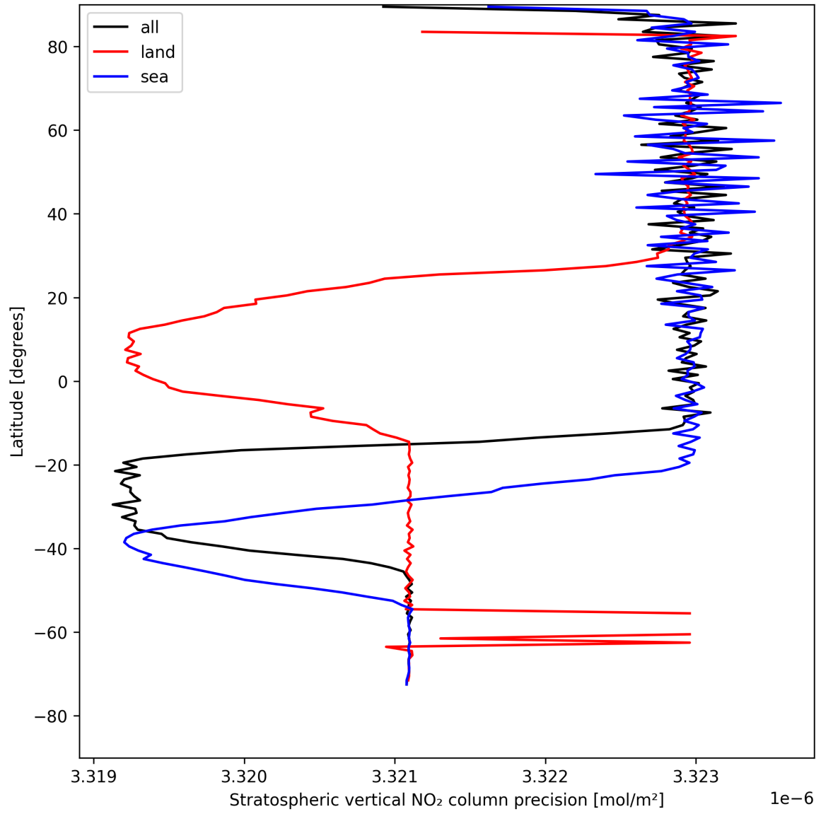
Figure 18: Zonal average of “Stratospheric vertical NO 2 column precision” for 2025-05-03 to 2025-05-03.
