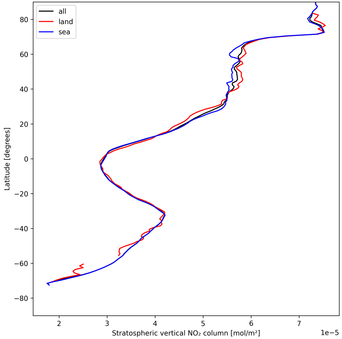
Figure 17: Zonal average of “Stratospheric vertical NO 2 column” for 2025-05-03 to 2025-05-03.
