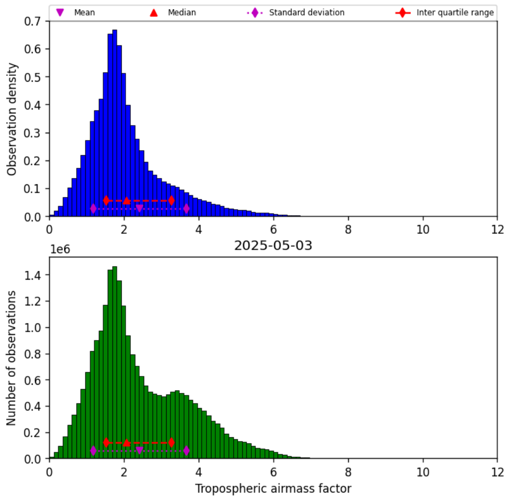
Figure 29: Histogram of “Tropospheric airmass factor” for 2025-05-03 to 2025-05-03
