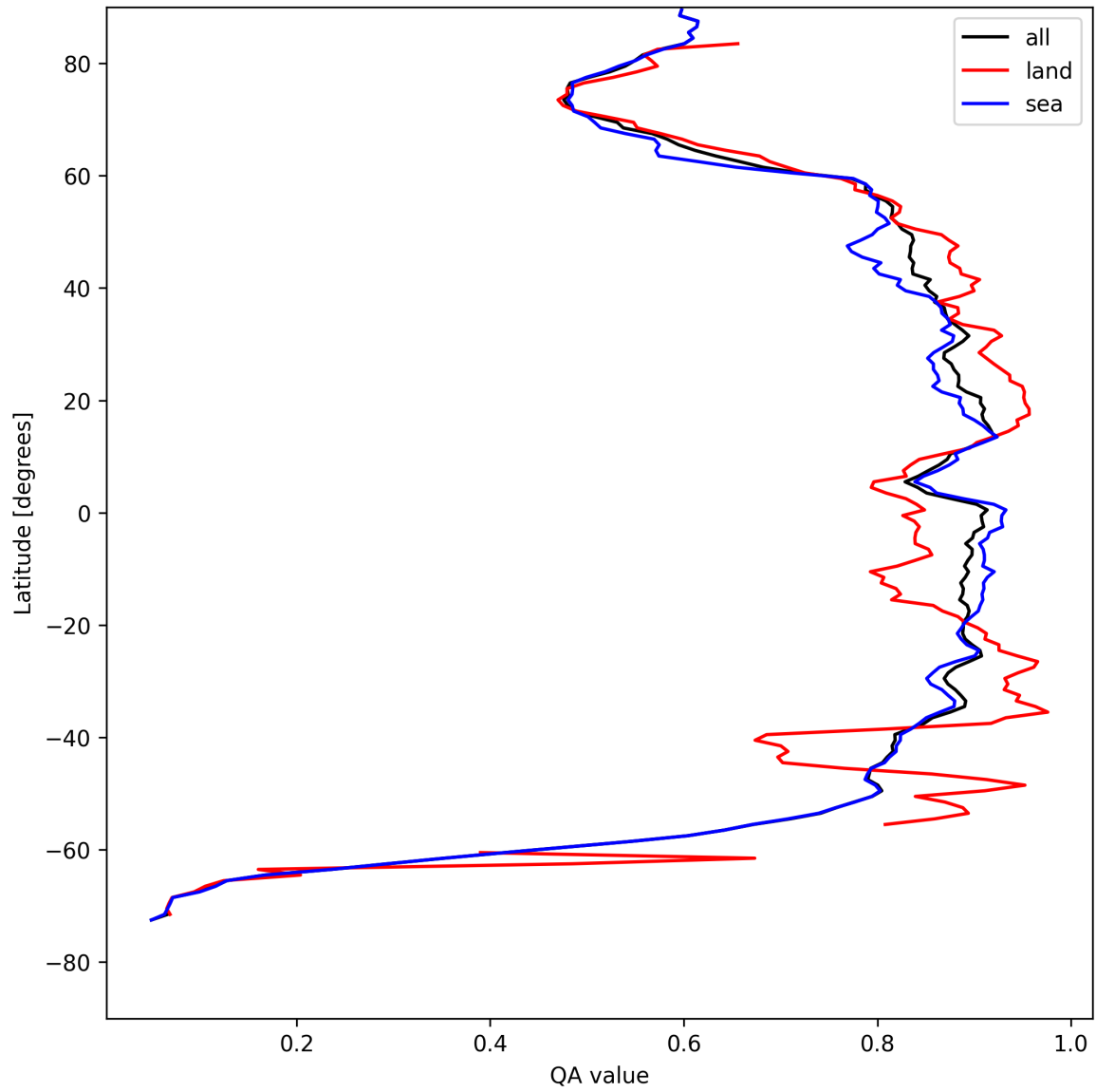
Figure 9: Zonal average of “QA value” for 2025-05-03 to 2025-05-03.
