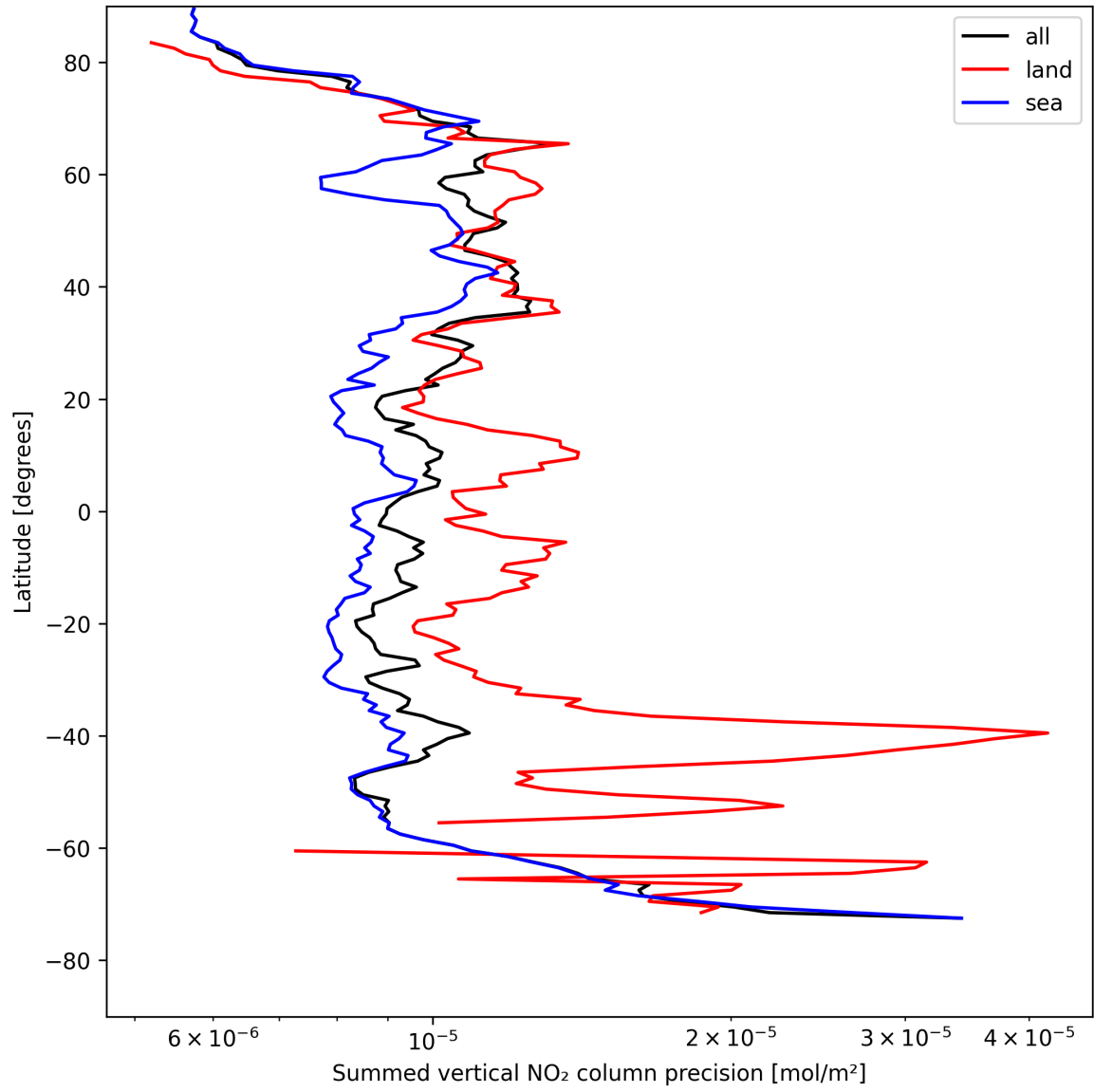
Figure 22: Zonal average of “Summed vertical NO 2 column precision” for 2025-05-03 to 2025-05-03.
