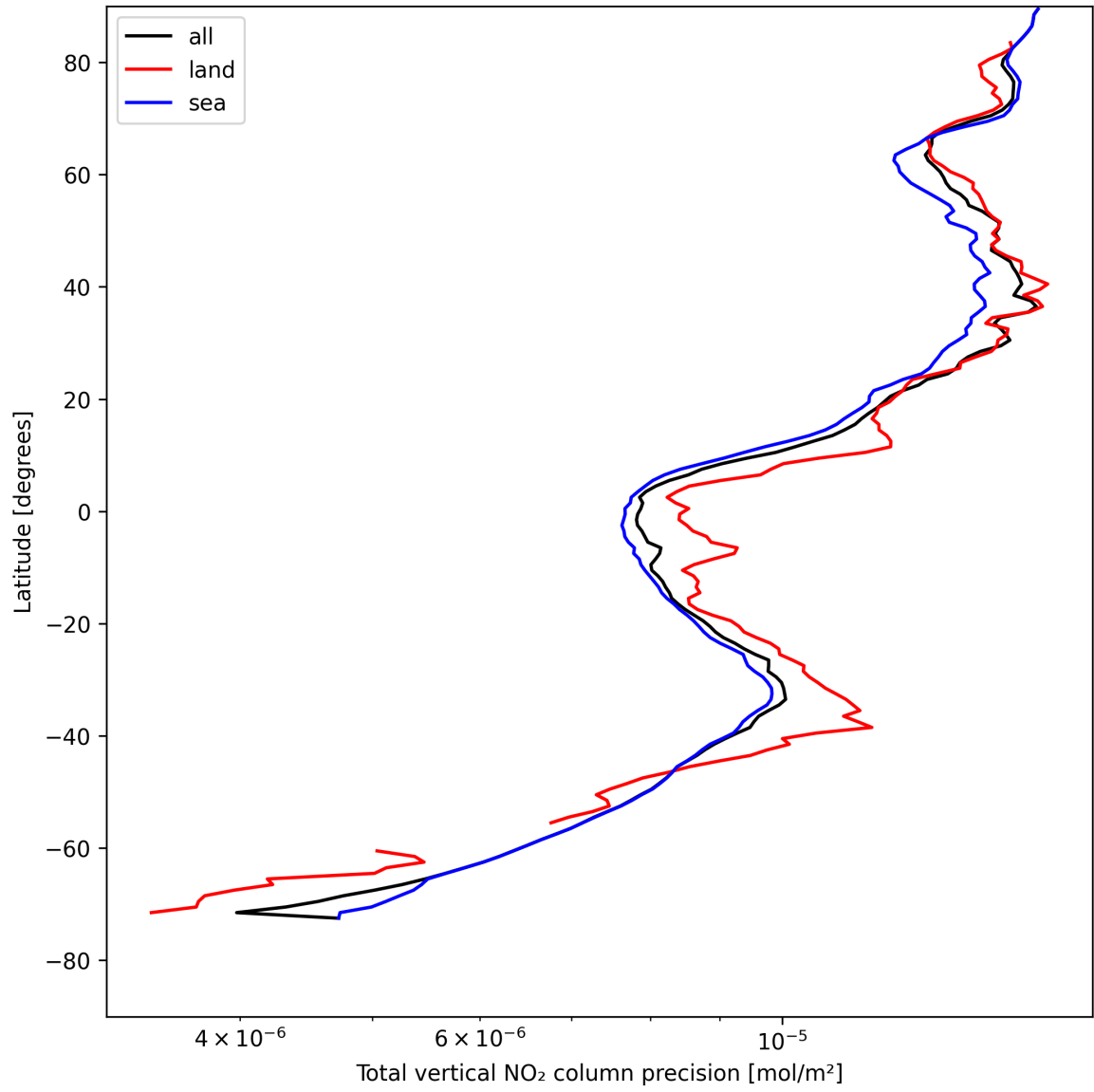
Figure 20: Zonal average of “Total vertical NO 2 column precision” for 2025-05-03 to 2025-05-03.
