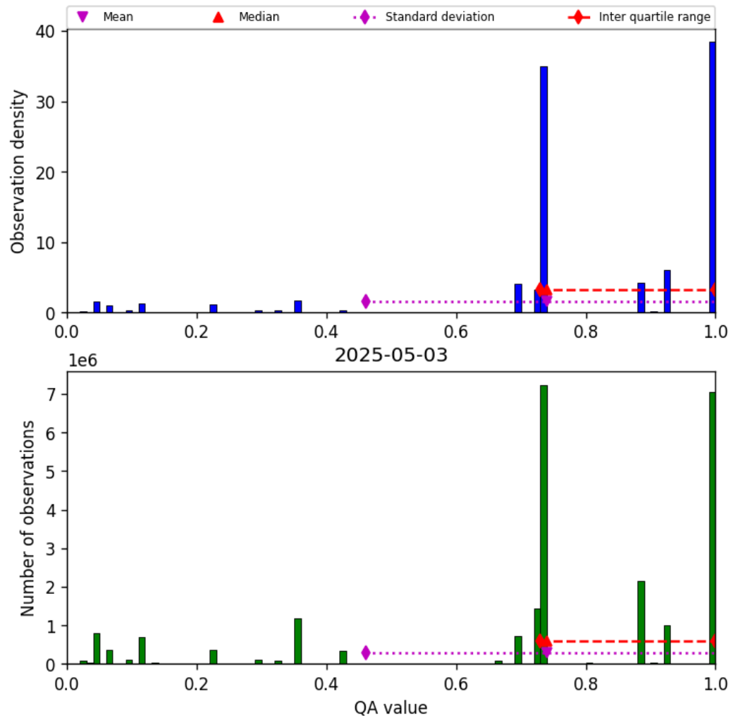
Figure 26: Histogram of “QA value” for 2025-05-03 to 2025-05-03
