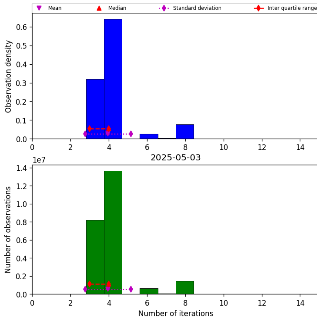
Figure 32: Histogram of “Number of iterations” for 2025-05-03 to 2025-05-03
