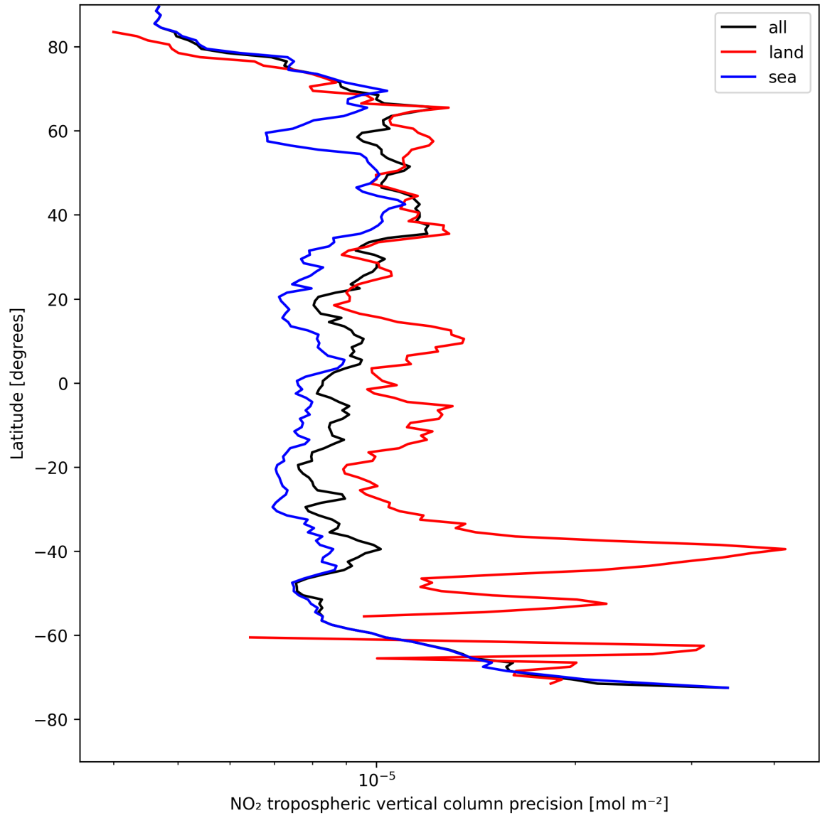
Figure 11: Zonal average of “NO 2 tropospheric vertical column precision” for 2025-05-03 to 2025-05-03.
