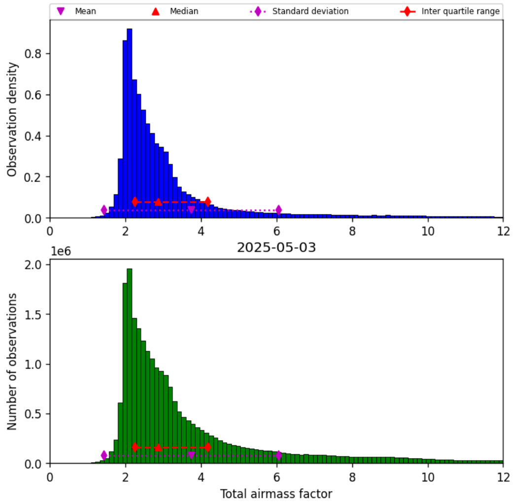
Figure 30: Histogram of “Total airmass factor” for 2025-05-03 to 2025-05-03
