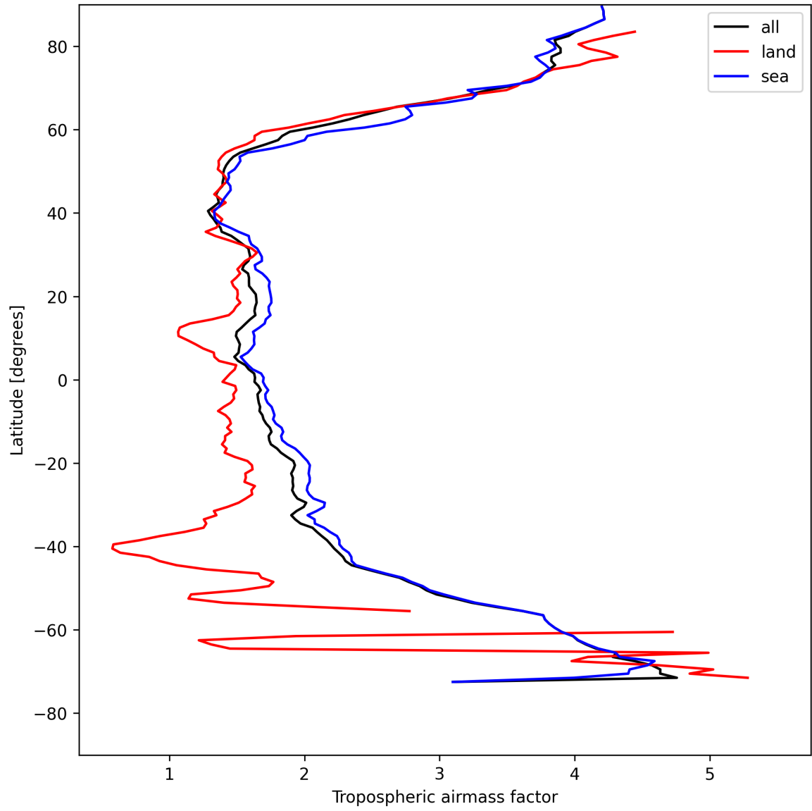
Figure 12: Zonal average of “Tropospheric airmass factor” for 2025-05-03 to 2025-05-03.
