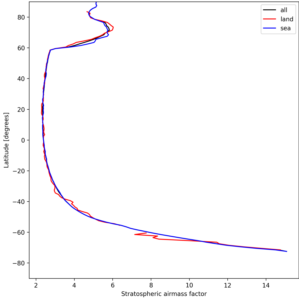
Figure 25: Zonal average of “Stratospheric air mass factor” for 2025-05-03 to 2025-05-03.
