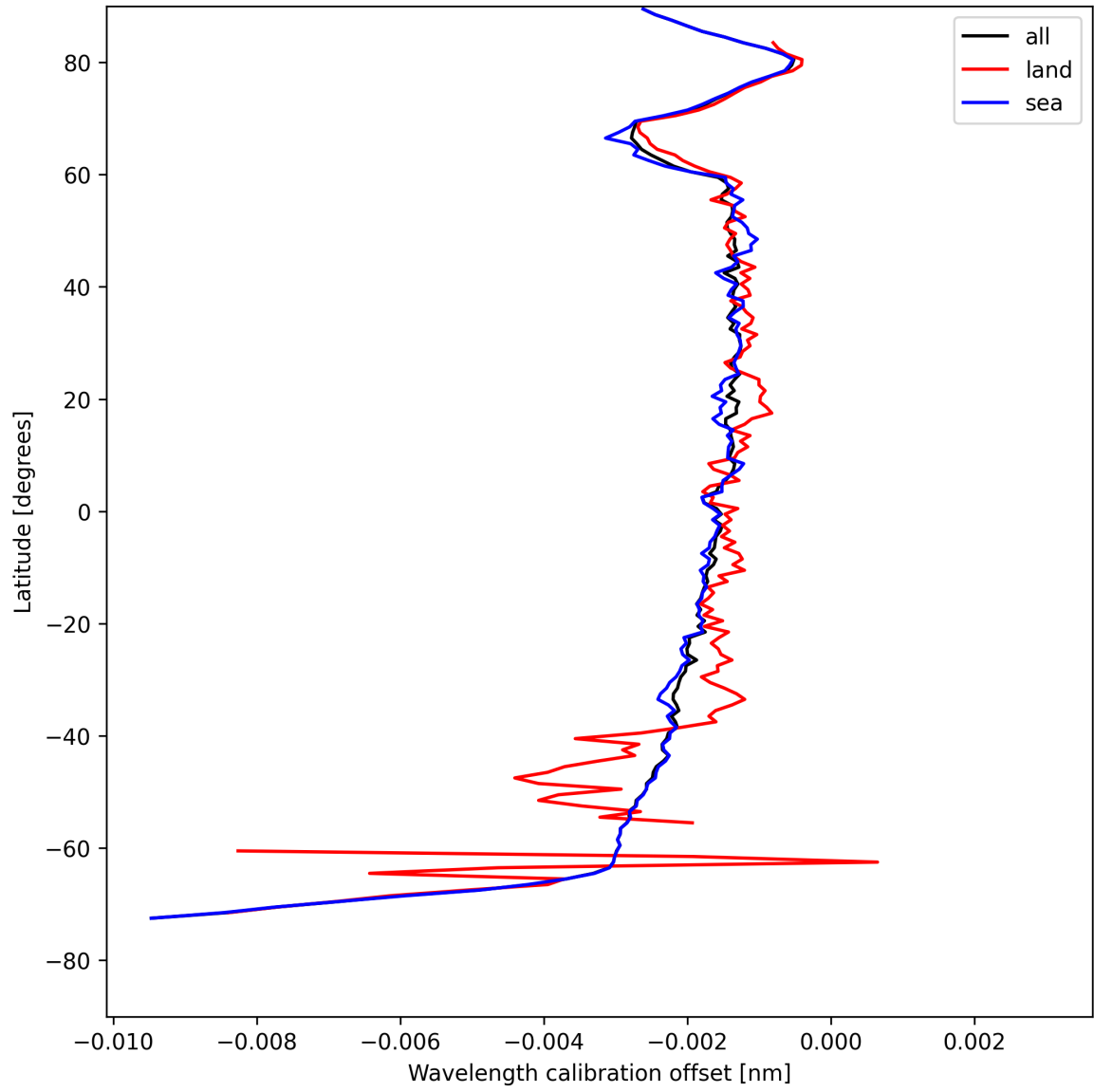
Figure 16: Zonal average of “Wavelength calibration offset” for 2025-05-03 to 2025-05-03.
