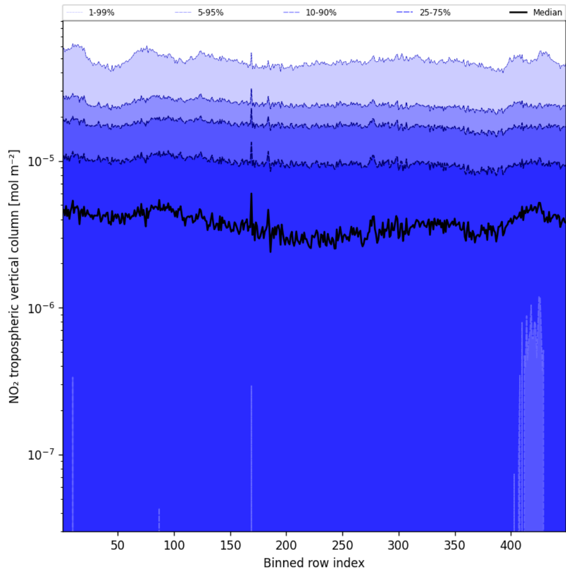
Figure 44: Along track statistics of “NO 2 tropospheric vertical column” for 2025-05-03 to 2025-05-03
