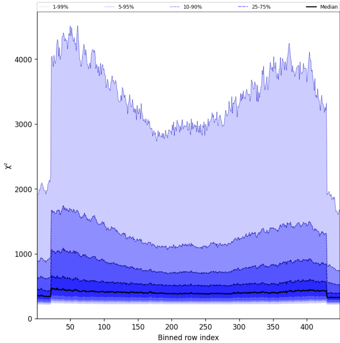
Figure 57: Along track statistics of “ \chi^2 ” for 2025-05-03 to 2025-05-03
