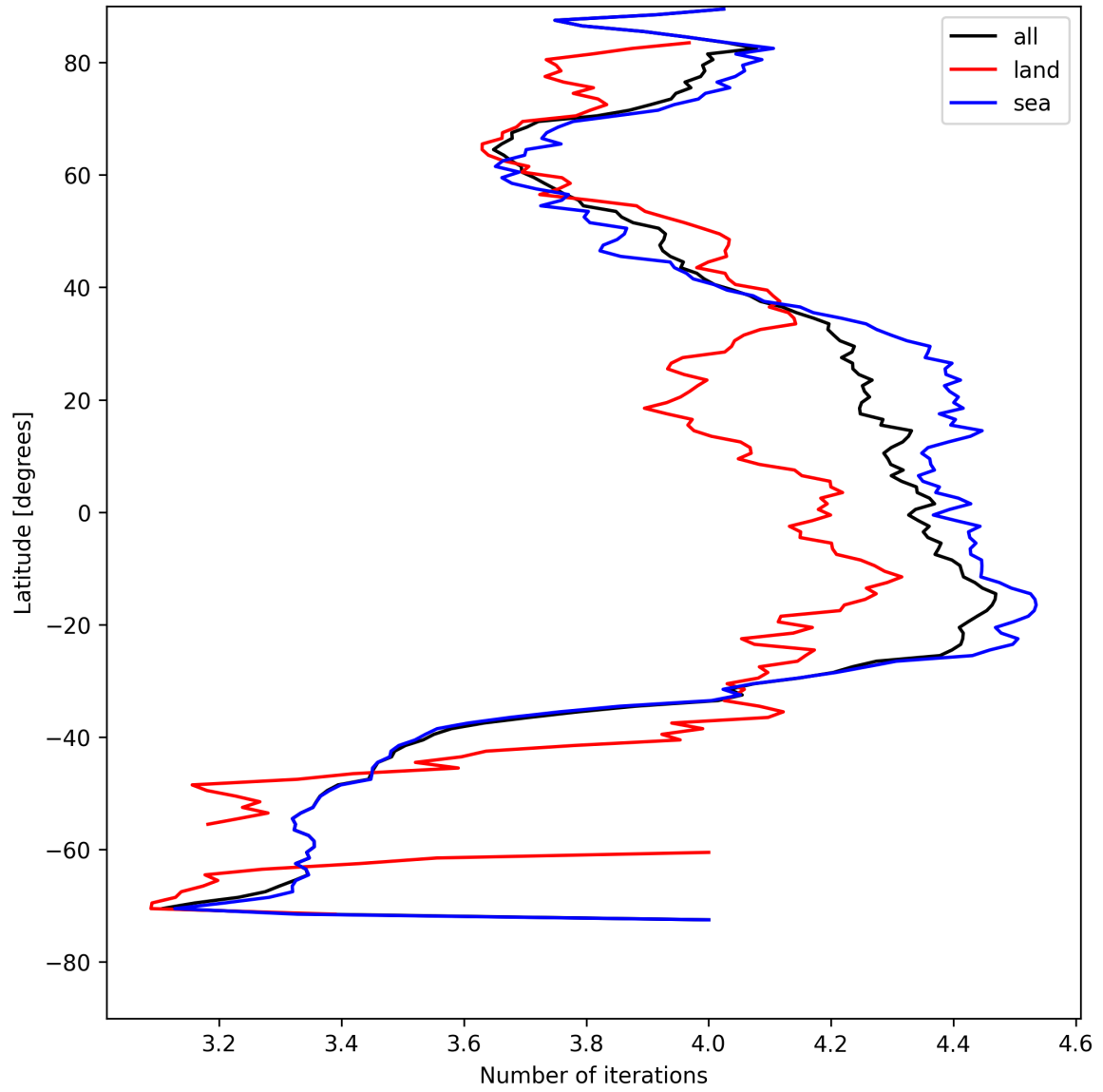
Figure 15: Zonal average of “Number of iterations” for 2025-05-03 to 2025-05-03.
