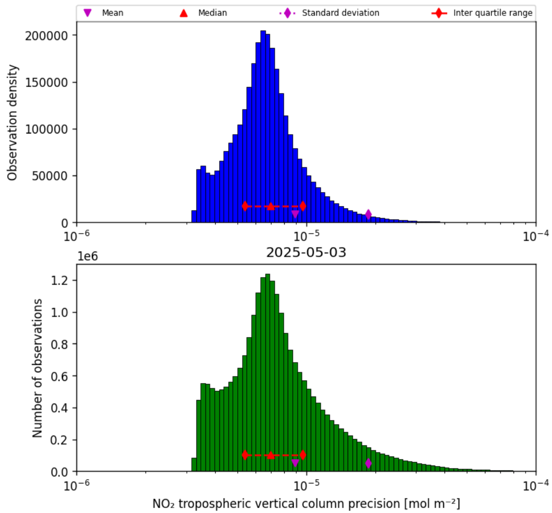
Figure 28: Histogram of “NO 2 tropospheric vertical column precision” for 2025-05-03 to 2025-05-03
