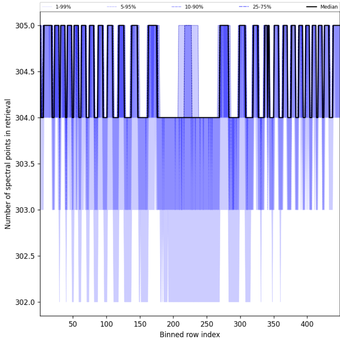
Figure 48: Along track statistics of “Number of spectral points in retrieval” for 2025-05-03 to 2025-05-03
