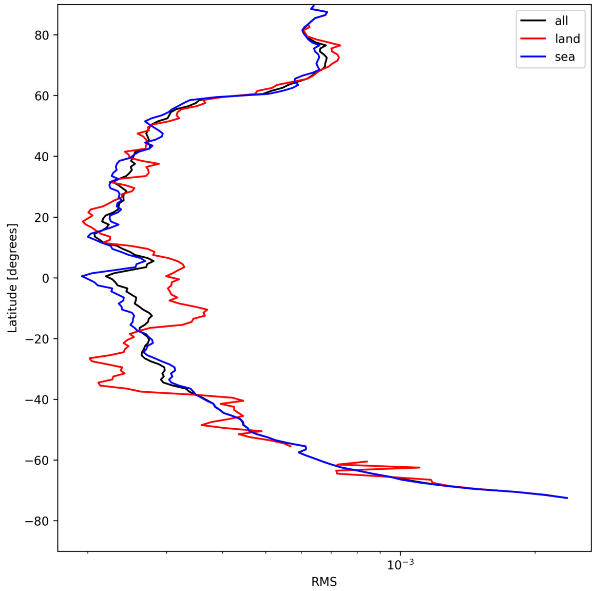
Figure 24: Zonal average of “RMS” for 2025-05-03 to 2025-05-03.
