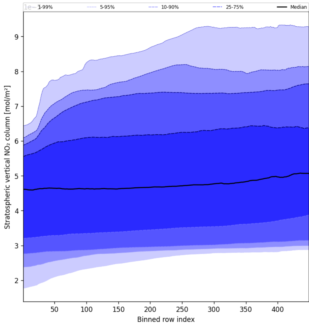
Figure 51: Along track statistics of “Stratospheric vertical NO 2 column” for 2025-05-03 to 2025-05-03
