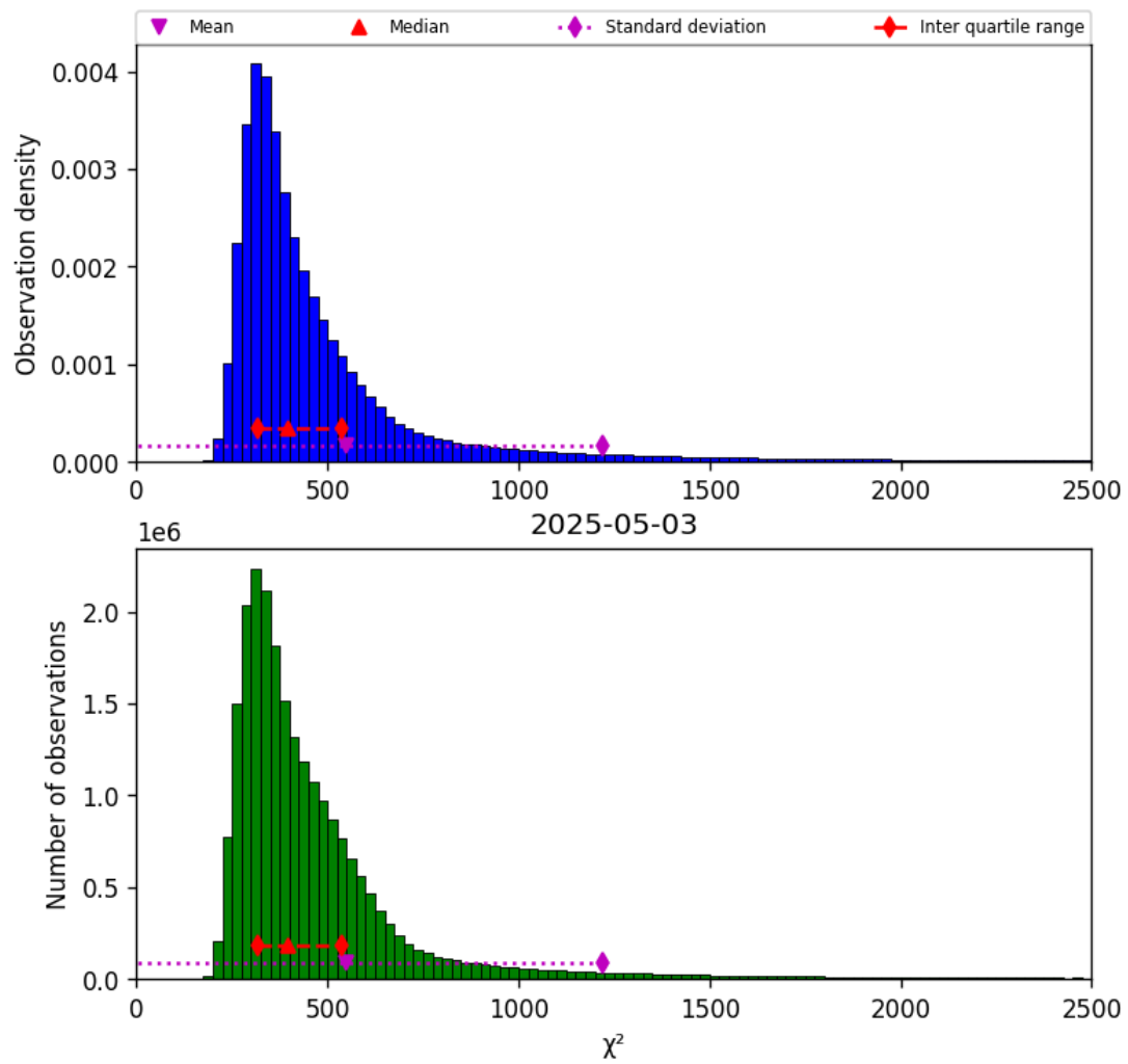
Figure 40: Histogram of “ \chi^2 ” for 2025-05-03 to 2025-05-03
