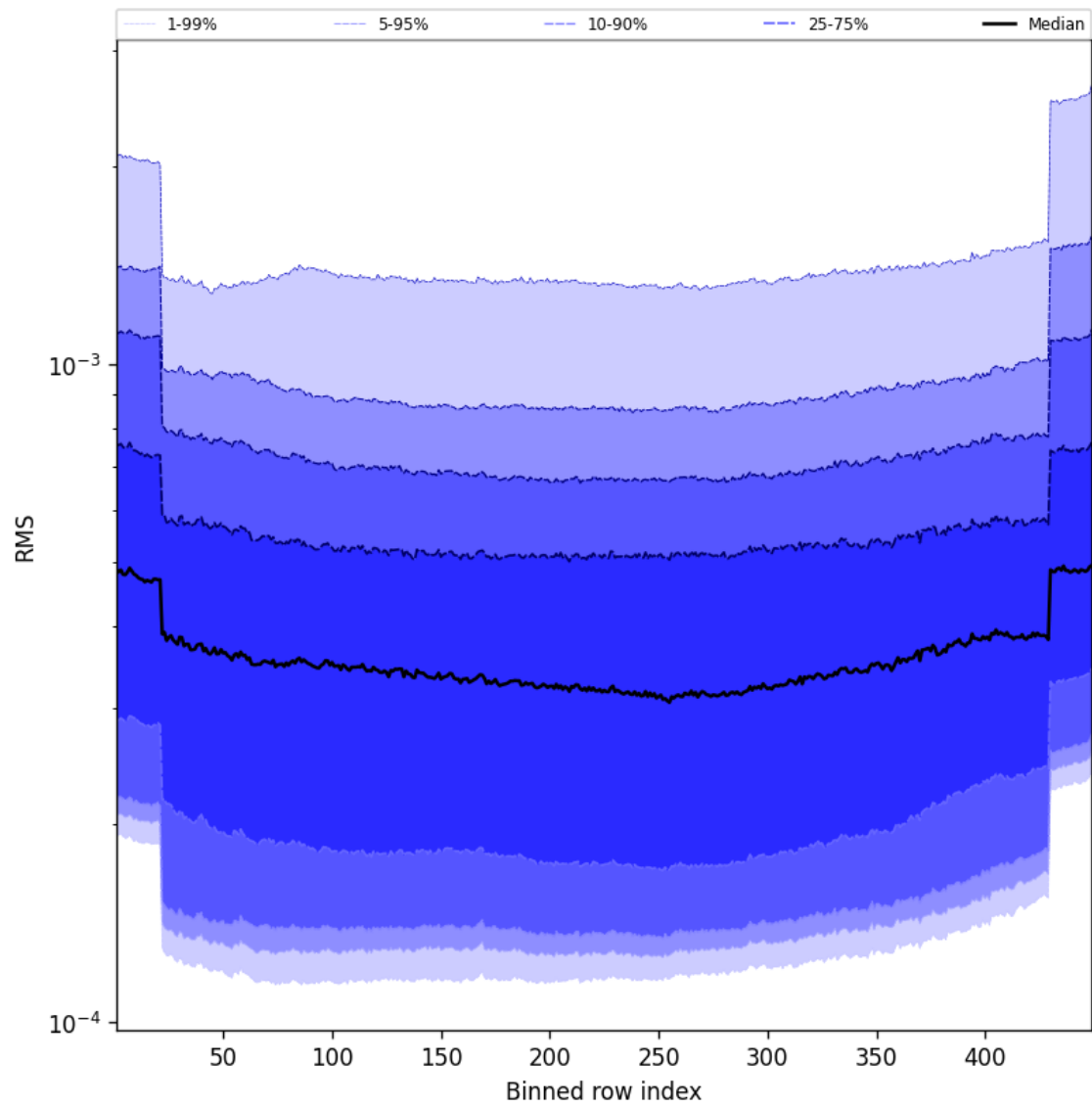
Figure 58: Along track statistics of “RMS” for 2025-05-03 to 2025-05-03
