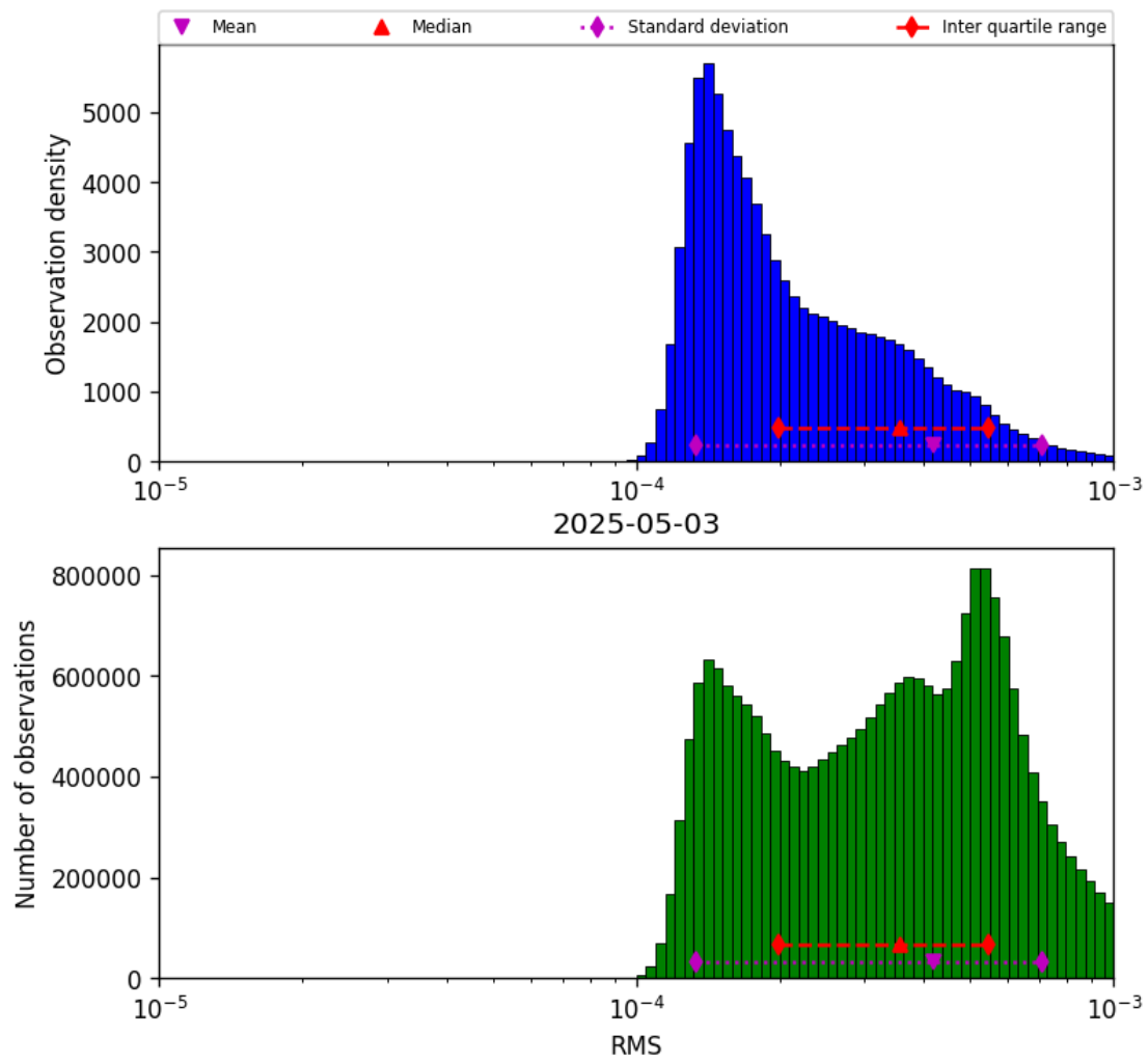
Figure 41: Histogram of “RMS” for 2025-05-03 to 2025-05-03
