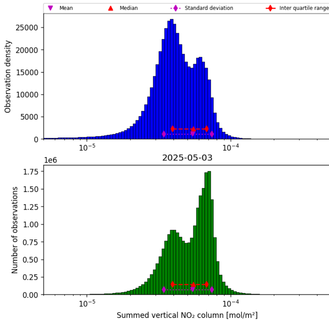
Figure 38: Histogram of “Summed vertical NO 2 column” for 2025-05-03 to 2025-05-03
