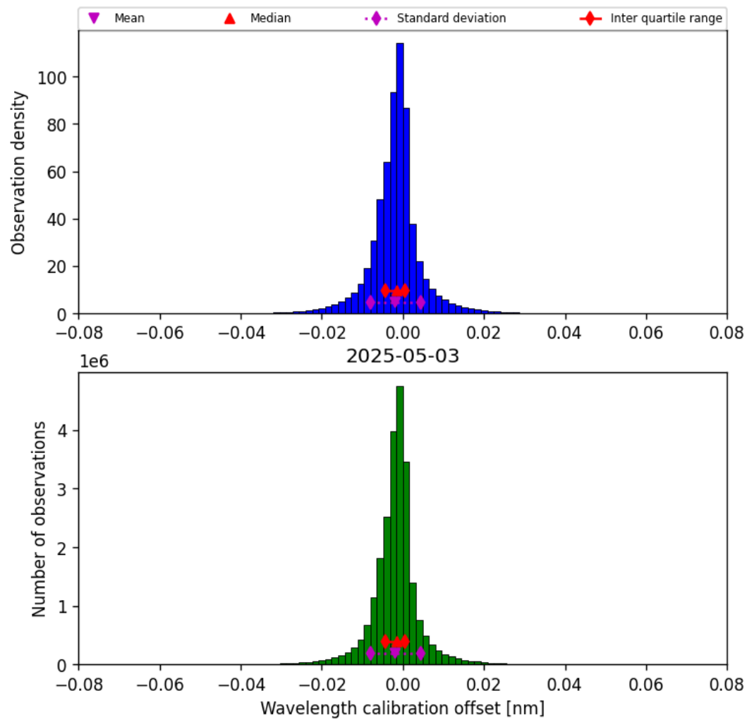
Figure 33: Histogram of “Wavelength calibration offset” for 2025-05-03 to 2025-05-03
