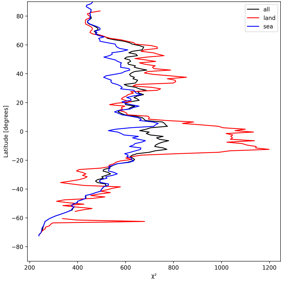
Figure 23: Zonal average of “ \chi^2 ” for 2025-05-03 to 2025-05-03.
