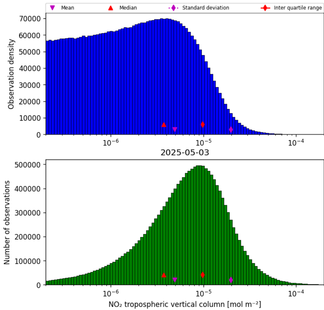
Figure 27: Histogram of “NO 2 tropospheric vertical column” for 2025-05-03 to 2025-05-03
