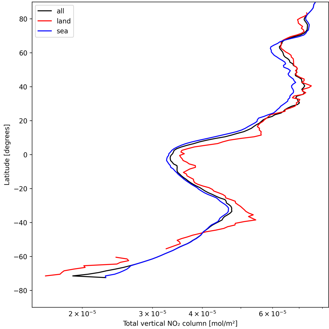
Figure 19: Zonal average of “Total vertical NO 2 column” for 2025-05-03 to 2025-05-03.
