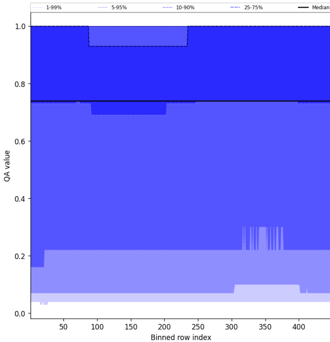
Figure 43: Along track statistics of “QA value” for 2025-05-03 to 2025-05-03
