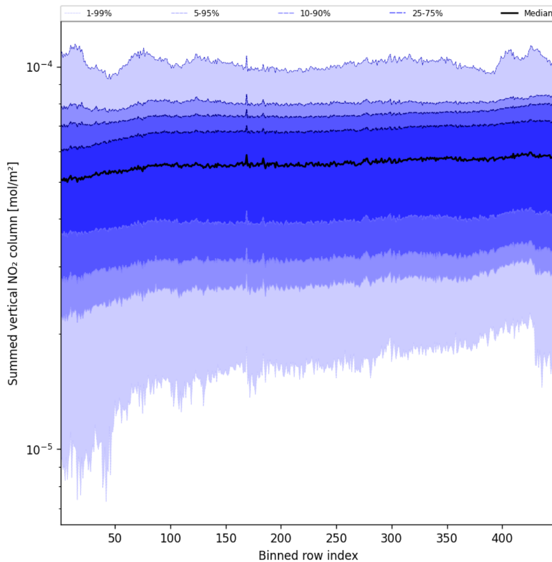
Figure 55: Along track statistics of “Summed vertical NO 2 column” for 2025-05-03 to 2025-05-03
