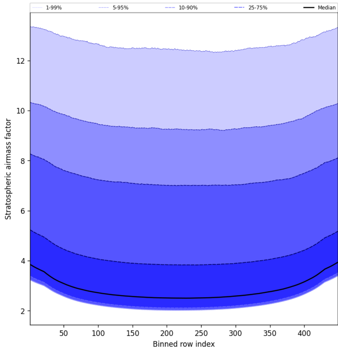
Figure 59: Along track statistics of “Stratospheric airmass factor” for 2025-05-03 to 2025-05-03
