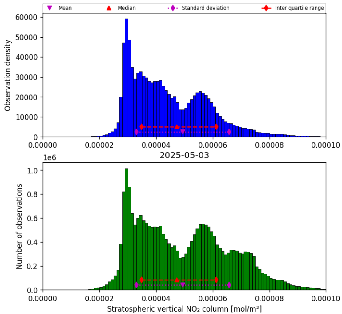
Figure 34: Histogram of “Stratospheric vertical NO 2 column” for 2025-05-03 to 2025-05-03
