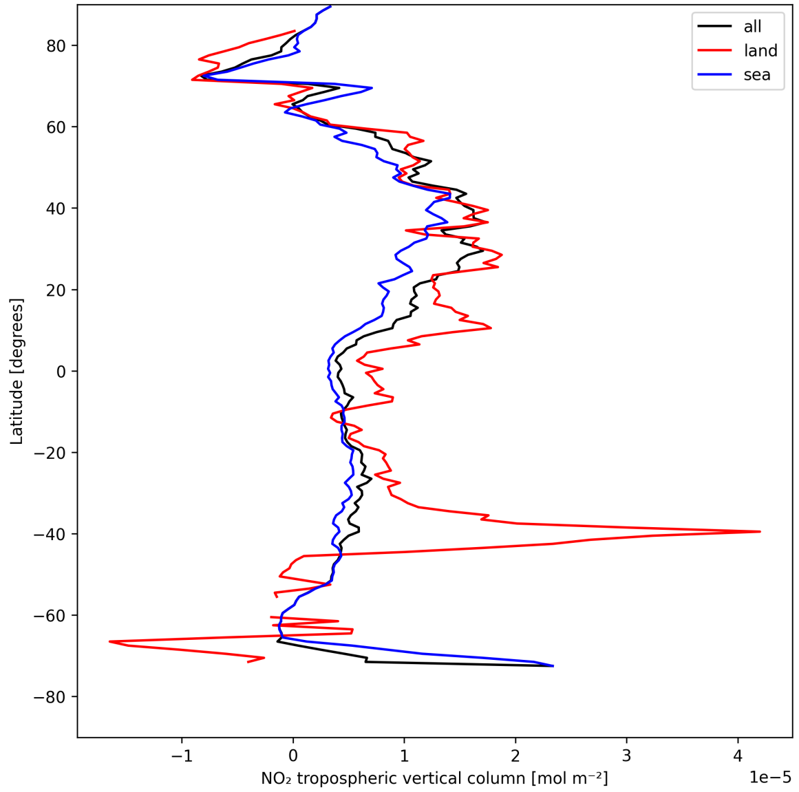
Figure 10: Zonal average of “NO 2 tropospheric vertical column” for 2025-05-03 to 2025-05-03.
