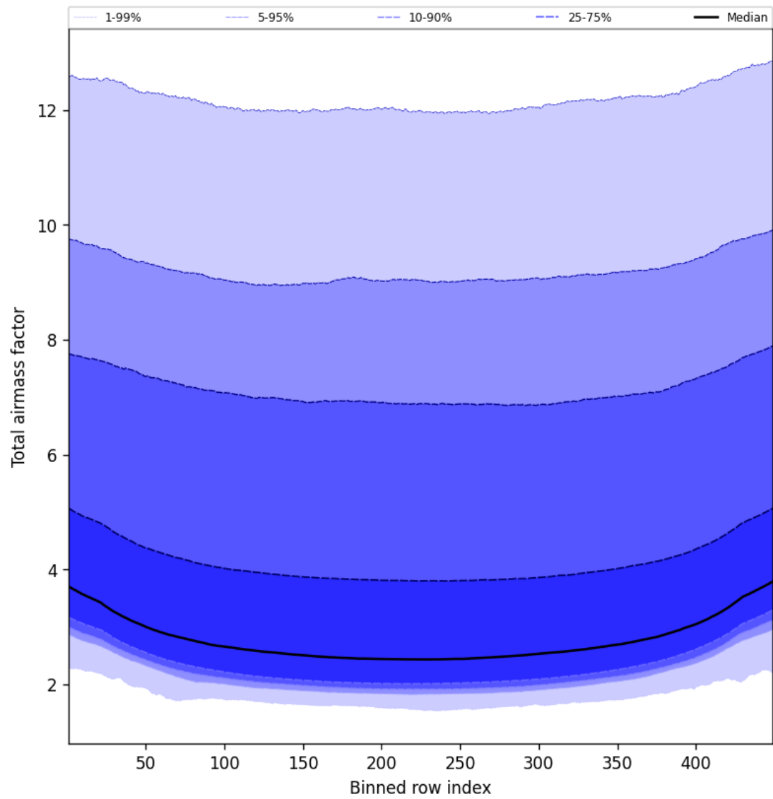
Figure 47: Along track statistics of “Total airmass factor” for 2025-05-03 to 2025-05-03
