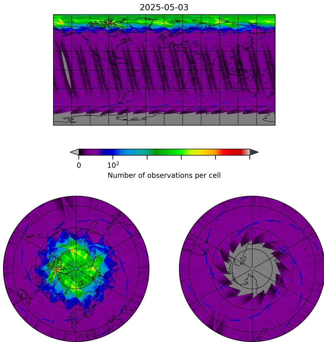
Figure 8: Map of the number of observations for 2025-05-03 to 2025-05-03
