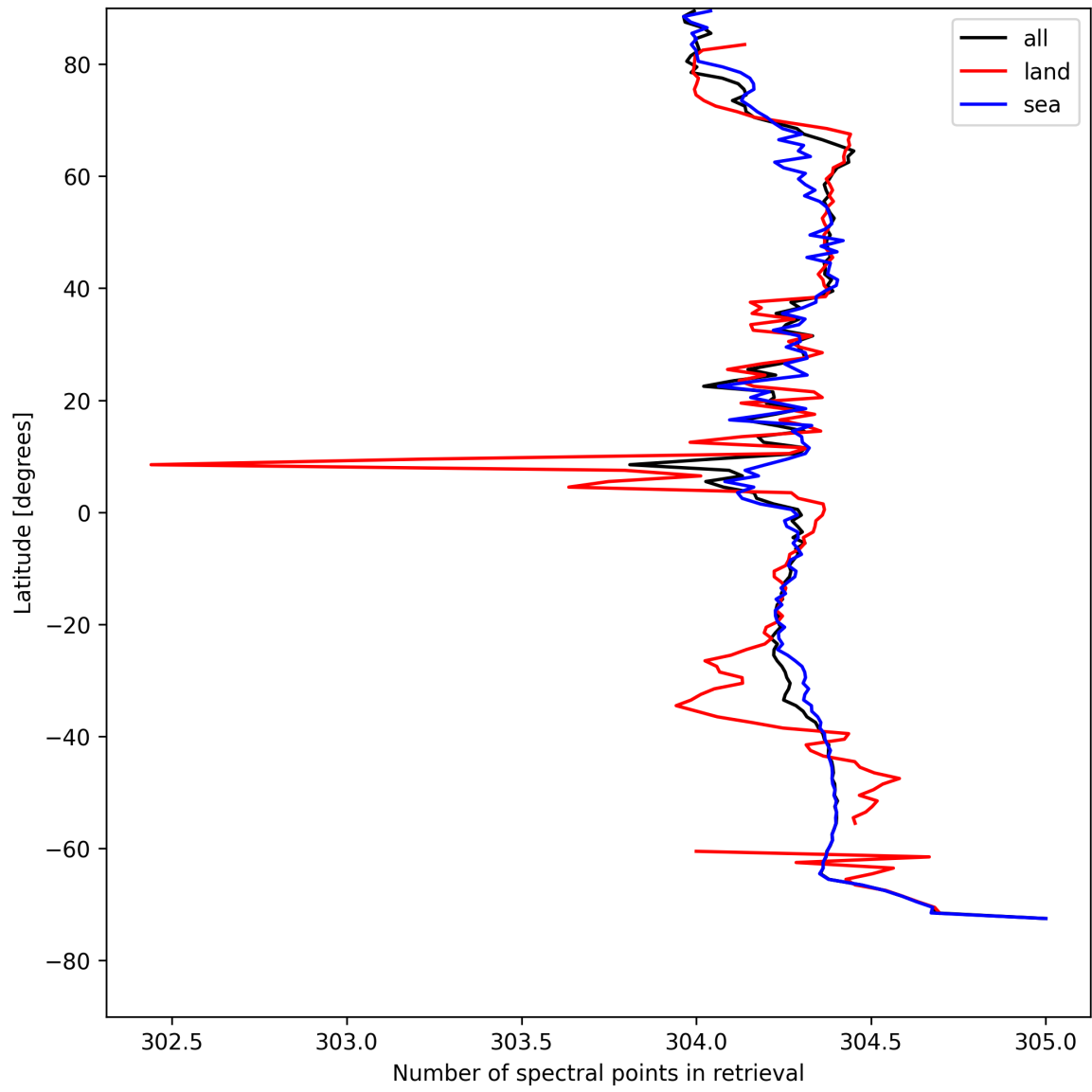
Figure 14: Zonal average of “Number of spectral points in retrieval” for 2025-05-03 to 2025-05-03.
