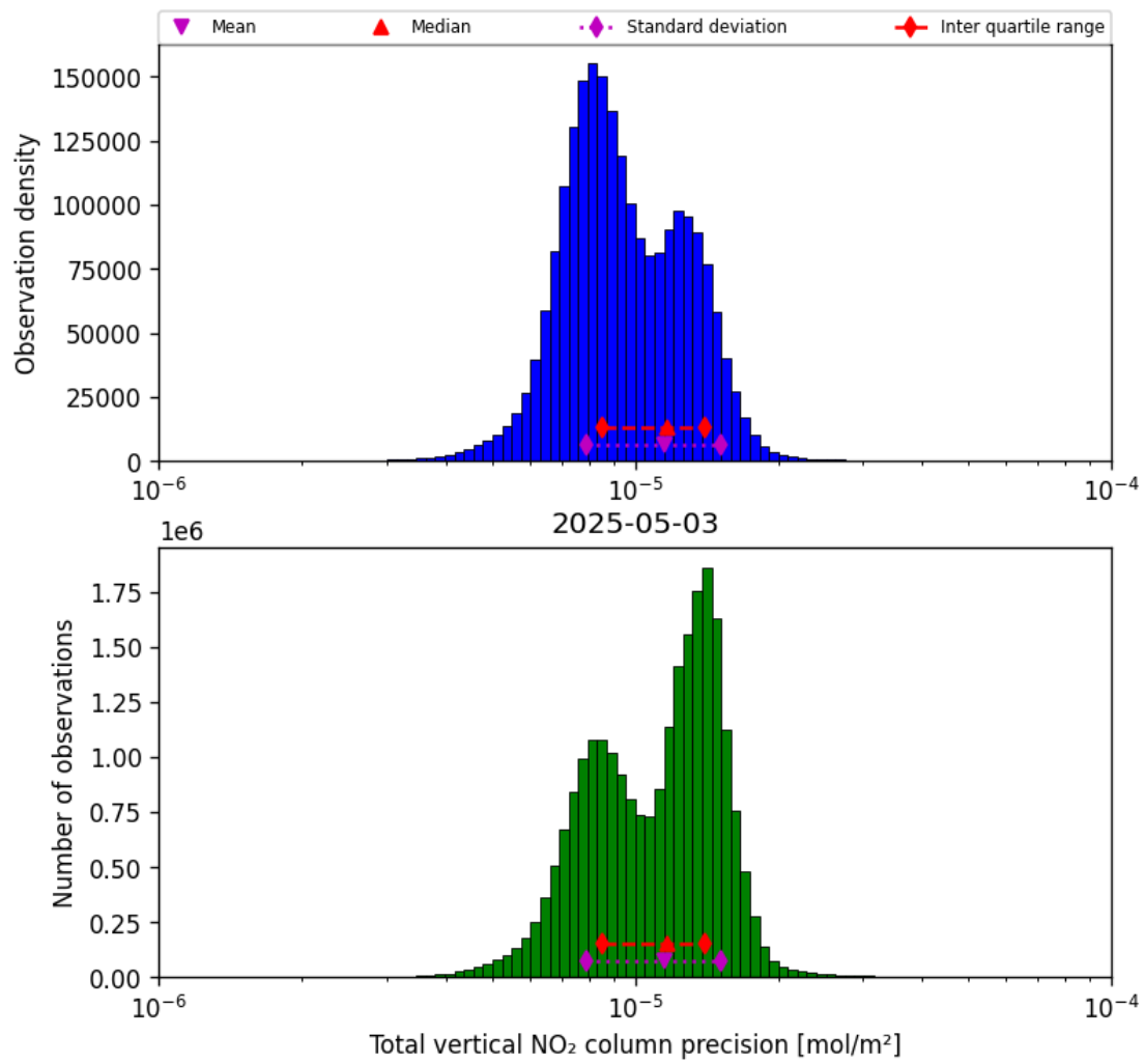
Figure 37: Histogram of "Total vertical NO 2 column precision" for 2025-05-03 to 2025-05-03
