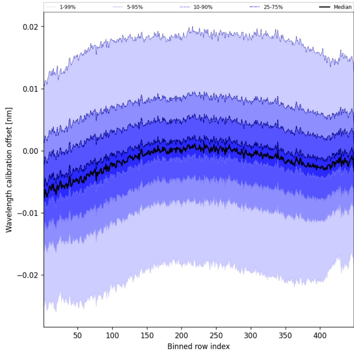
Figure 50: Along track statistics of “Wavelength calibration offset” for 2025-05-03 to 2025-05-03
