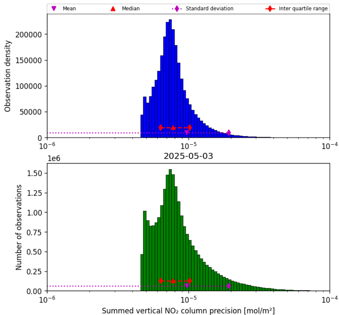
Figure 39: Histogram of "Summed vertical NO 2 column precision" for 2025-05-03 to 2025-05-03
