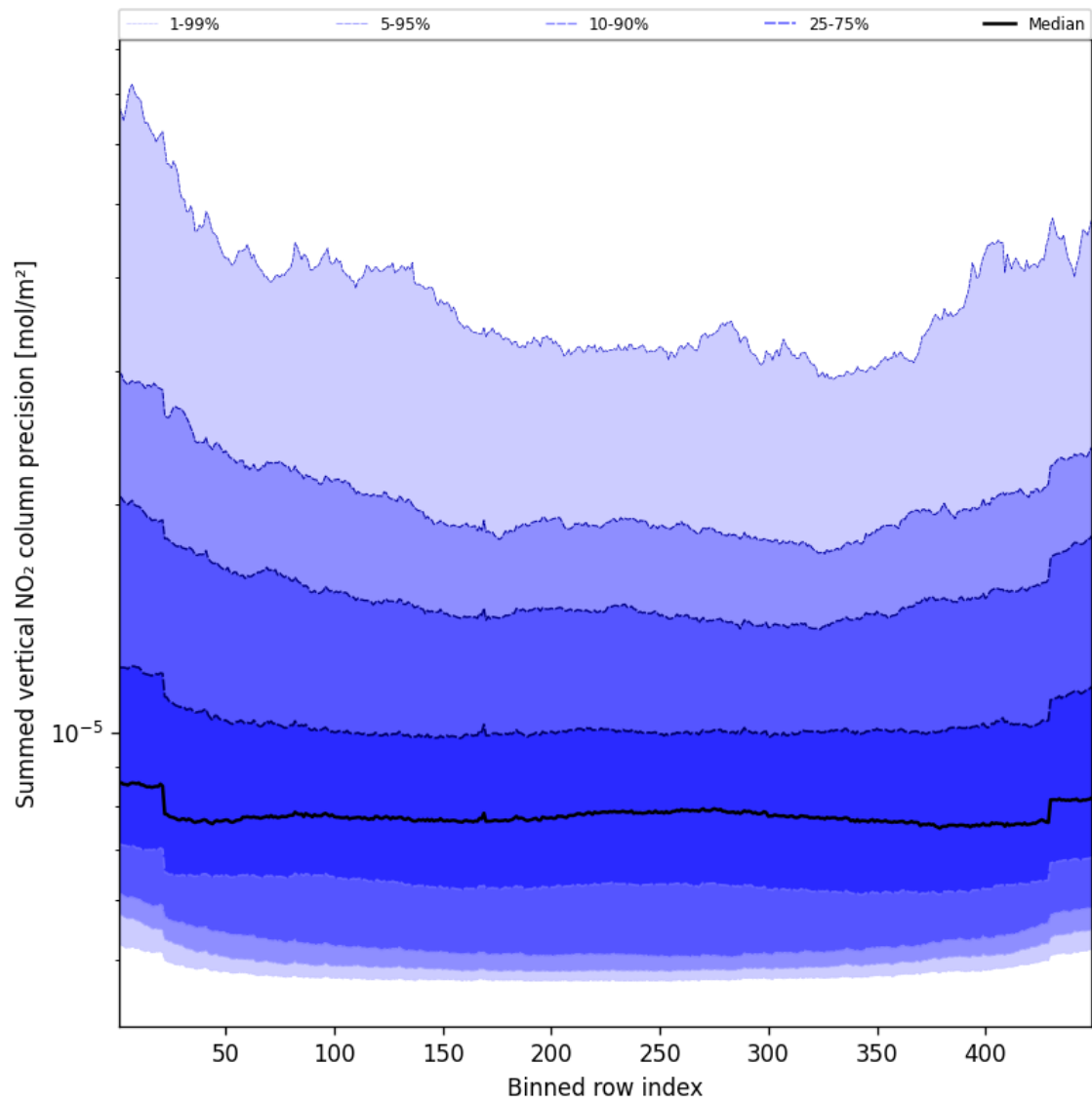
Figure 56: Along track statistics of “Summed vertical NO 2 column precision” for 2025-05-03 to 2025-05-03
