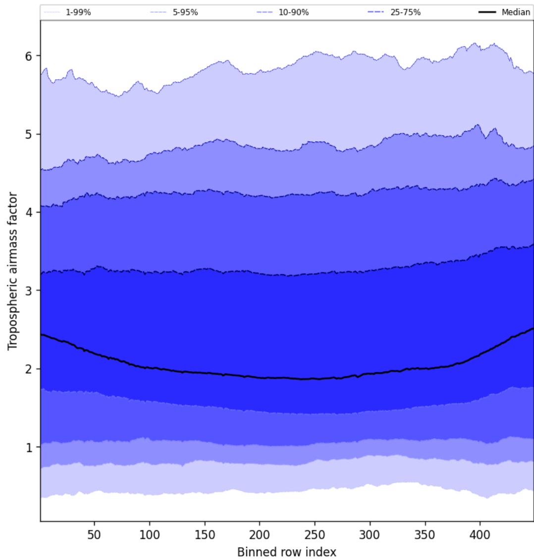
Figure 46: Along track statistics of “Tropospheric airmass factor” for 2025-05-03 to 2025-05-03
