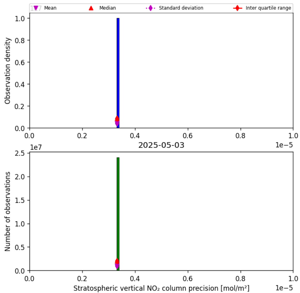
Figure 35: Histogram of “Stratospheric vertical NO 2 column precision” for 2025-05-03 to 2025-05-03
