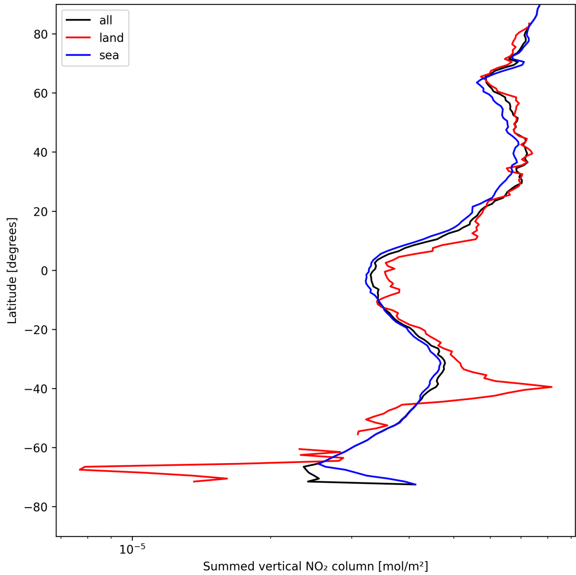
Figure 21: Zonal average of “Summed vertical NO 2 column” for 2025-05-03 to 2025-05-03.
