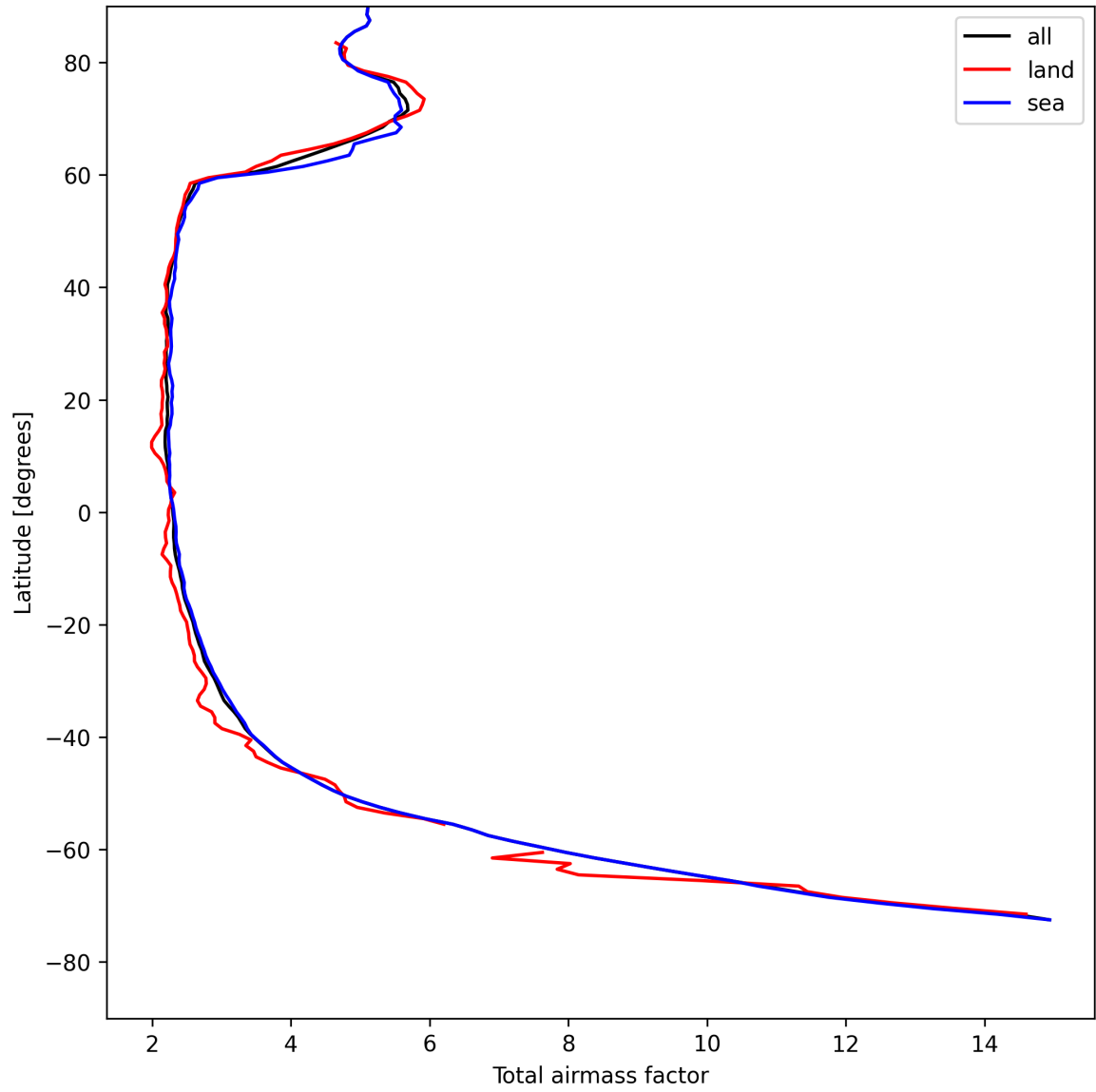
Figure 13: Zonal average of “Total airmass factor” for 2025-05-03 to 2025-05-03.
