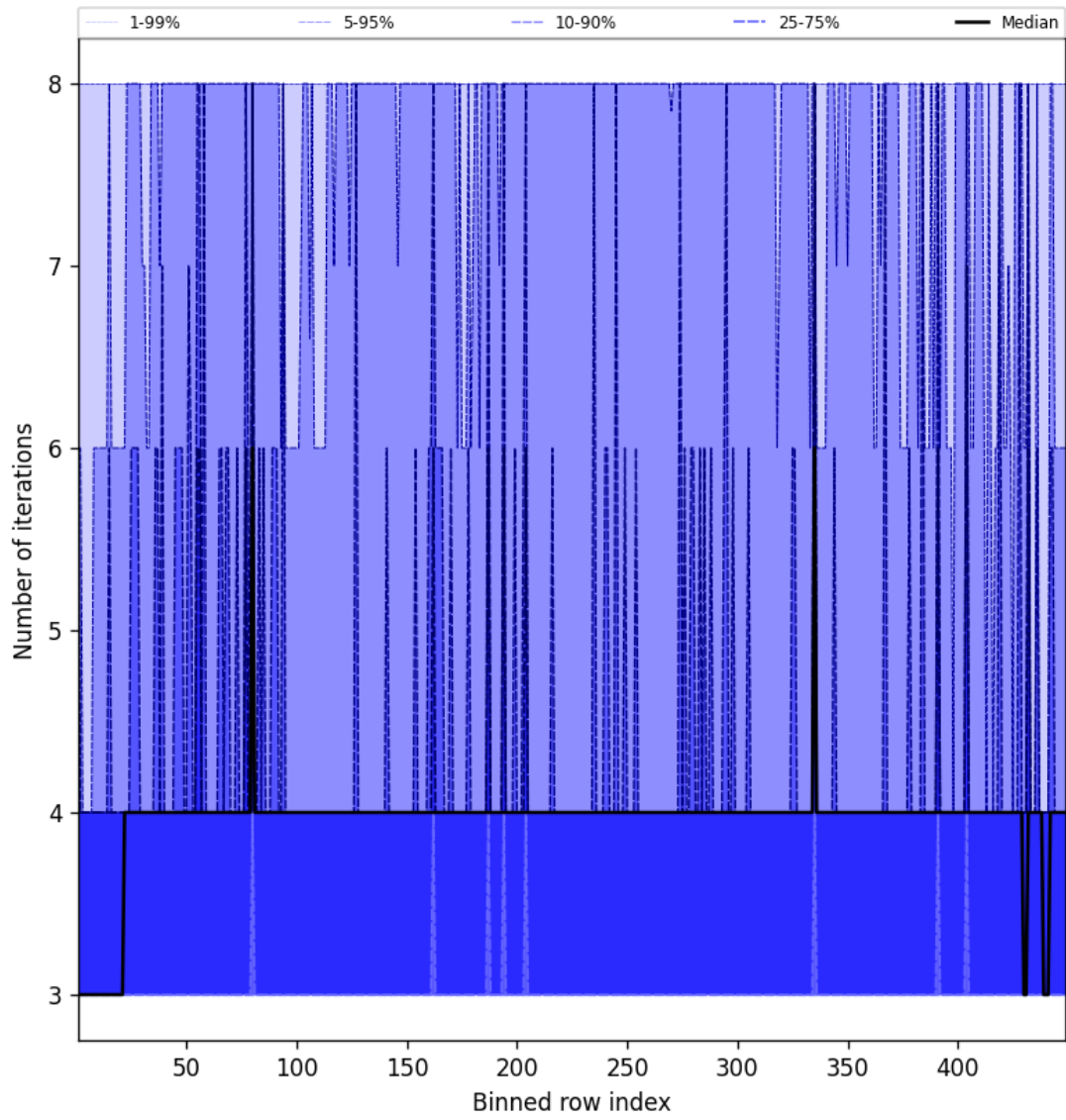
Figure 49: Along track statistics of “Number of iterations” for 2025-05-04 to 2025-05-05
