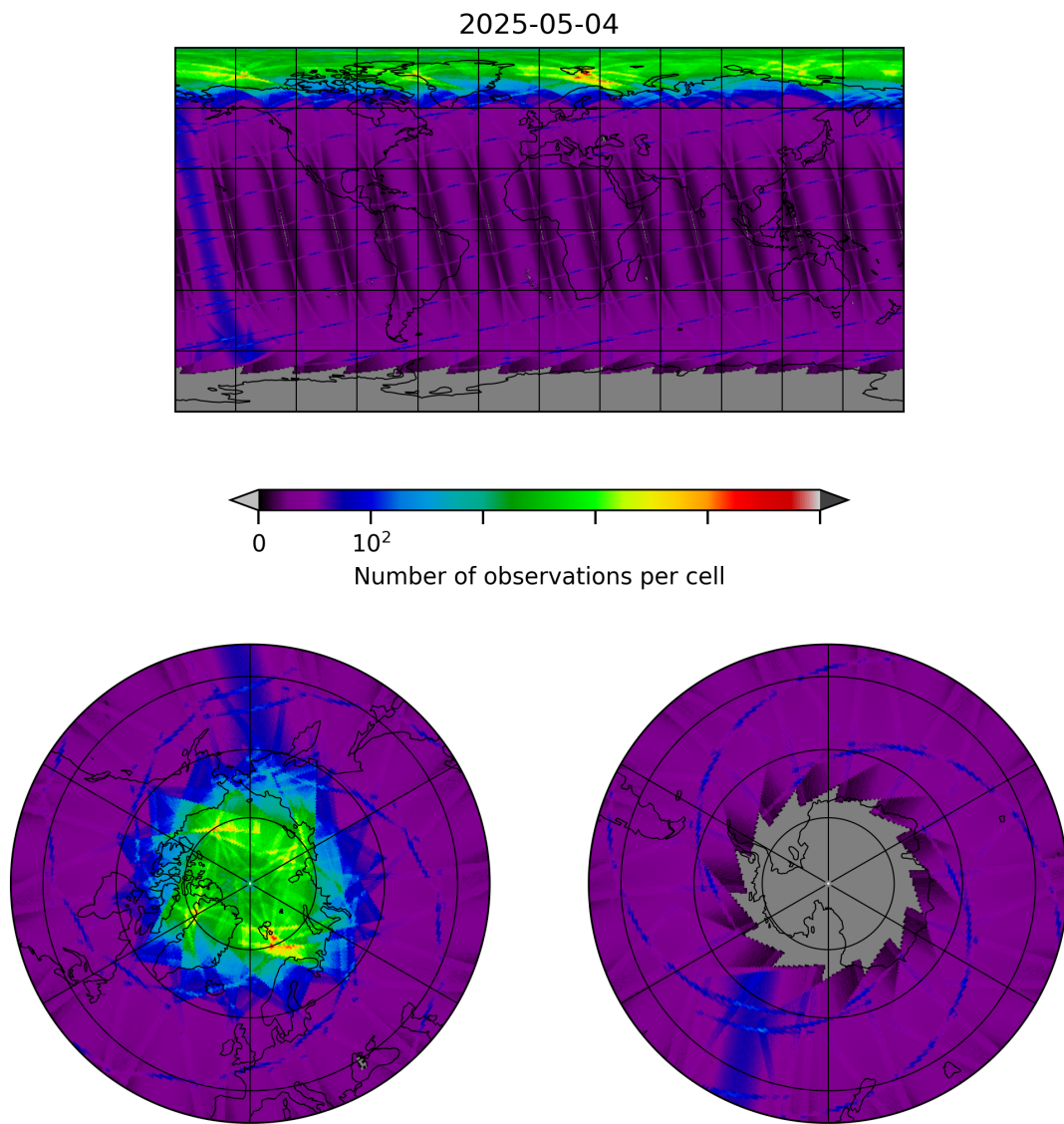
Figure 8: Map of the number of observations for 2025-05-04 to 2025-05-05
