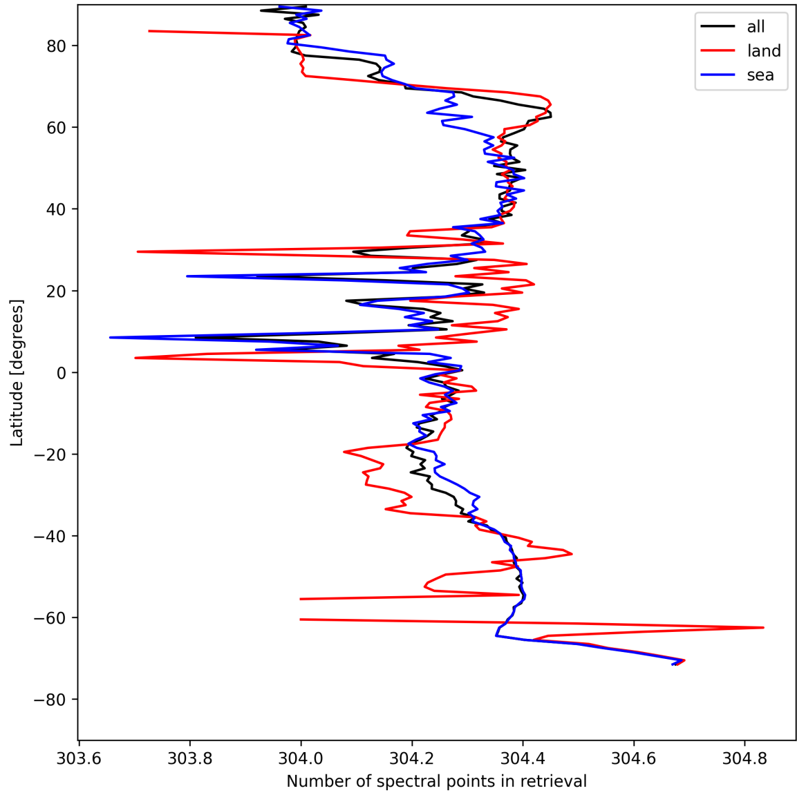
Figure 14: Zonal average of “Number of spectral points in retrieval” for 2025-05-04 to 2025-05-05.
