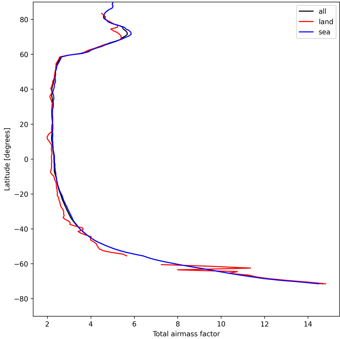
Figure 13: Zonal average of “Total airmass factor” for 2025-05-04 to 2025-05-05.
