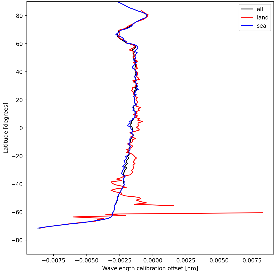
Figure 16: Zonal average of “Wavelength calibration offset” for 2025-05-04 to 2025-05-05.
