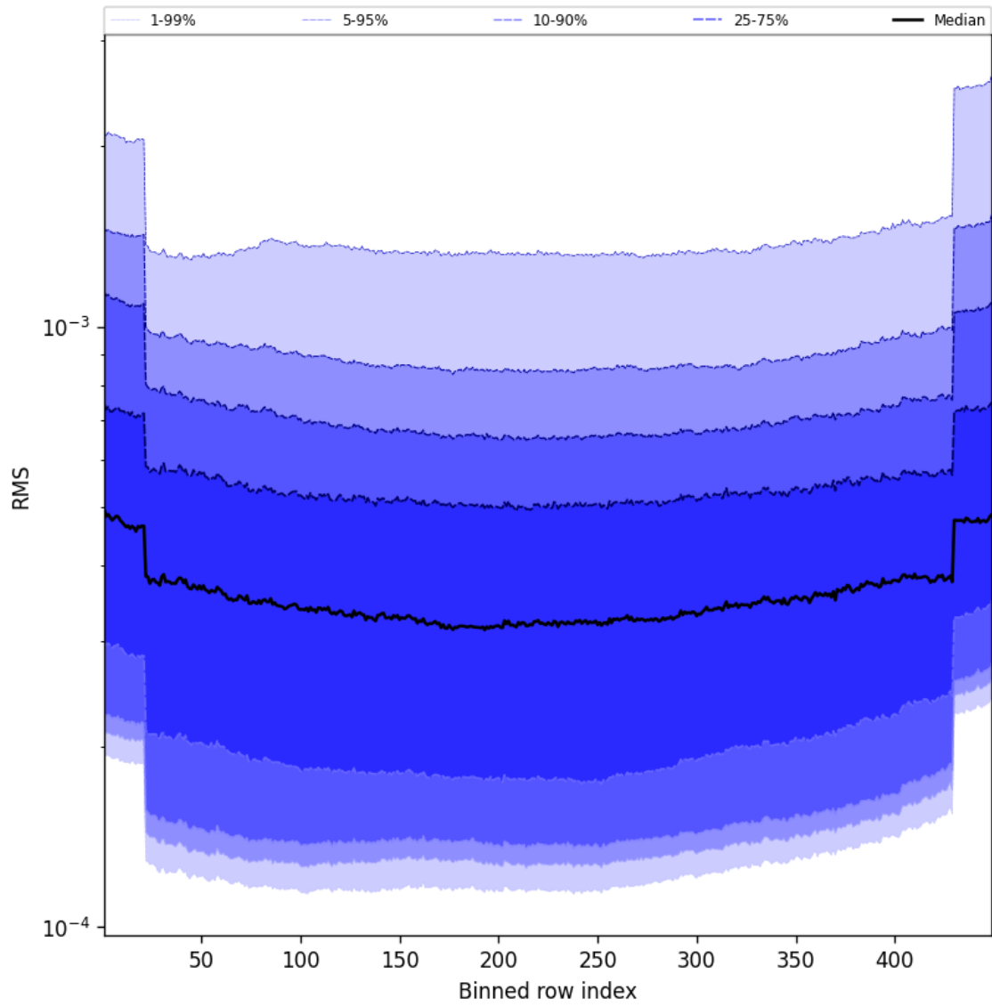
Figure 58: Along track statistics of “RMS” for 2025-05-04 to 2025-05-05
