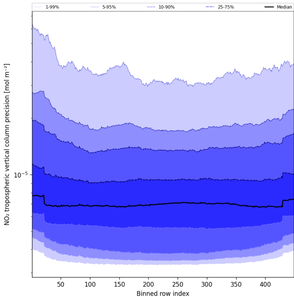
Figure 45: Along track statistics of “NO 2 tropospheric vertical column precision” for 2025-05-04 to 2025-05-05
