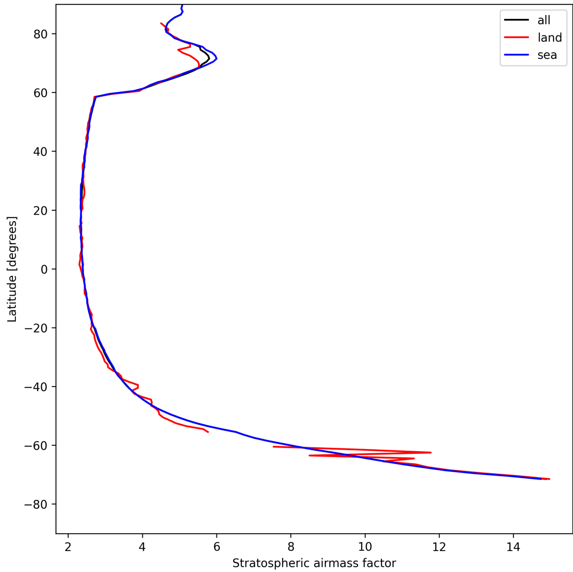
Figure 25: Zonal average of “Stratospheric air mass factor” for 2025-05-04 to 2025-05-05.
