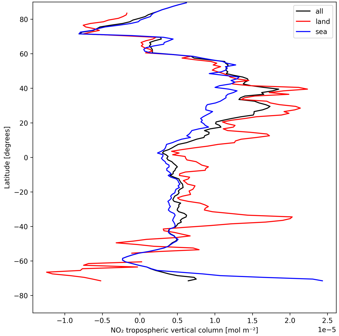
Figure 10: Zonal average of “NO 2 tropospheric vertical column” for 2025-05-04 to 2025-05-05.
