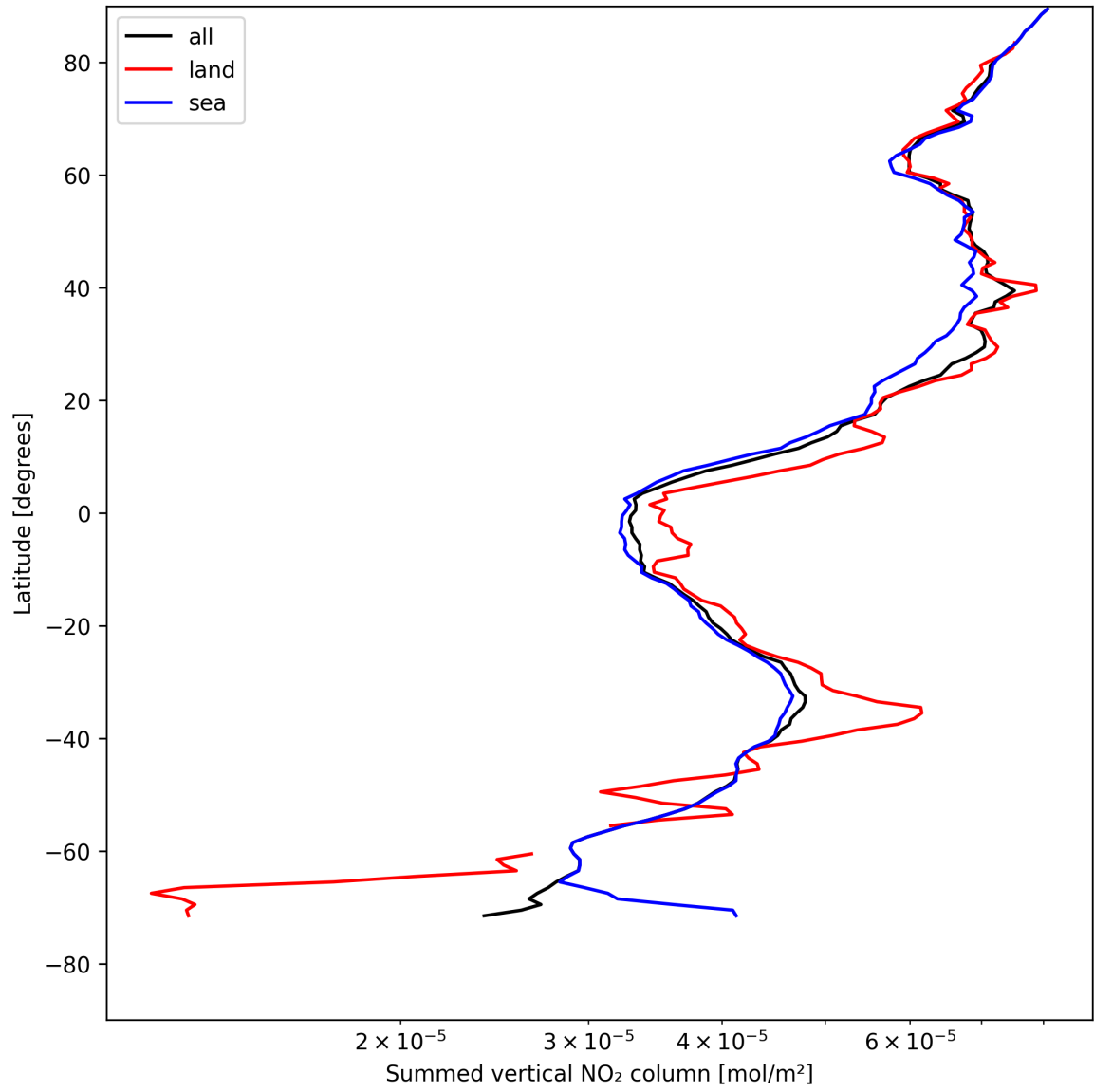
Figure 21: Zonal average of “Summed vertical NO 2 column” for 2025-05-04 to 2025-05-05.
