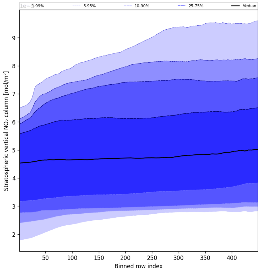
Figure 51: Along track statistics of “Stratospheric vertical NO 2 column” for 2025-05-04 to 2025-05-05
