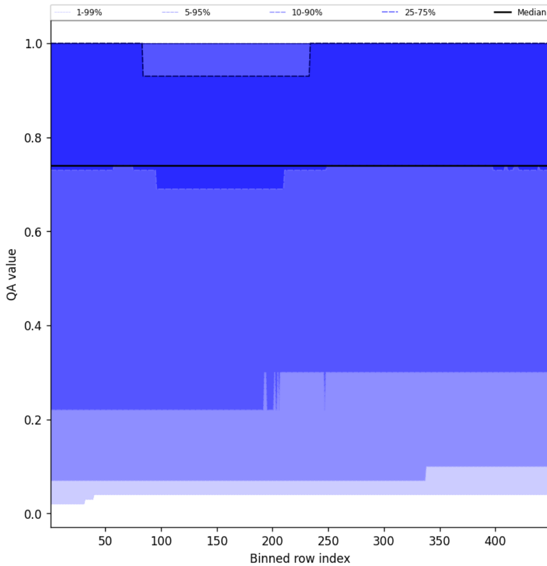
Figure 43: Along track statistics of “QA value” for 2025-05-04 to 2025-05-05
