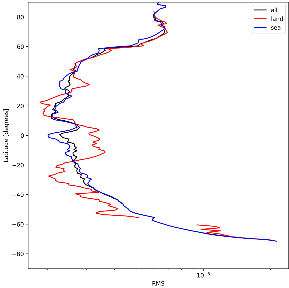
Figure 24: Zonal average of “RMS” for 2025-05-04 to 2025-05-05.
