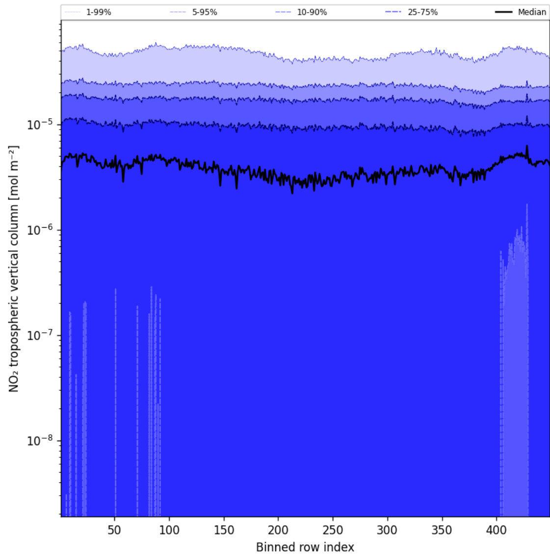
Figure 44: Along track statistics of “NO 2 tropospheric vertical column” for 2025-05-04 to 2025-05-05
