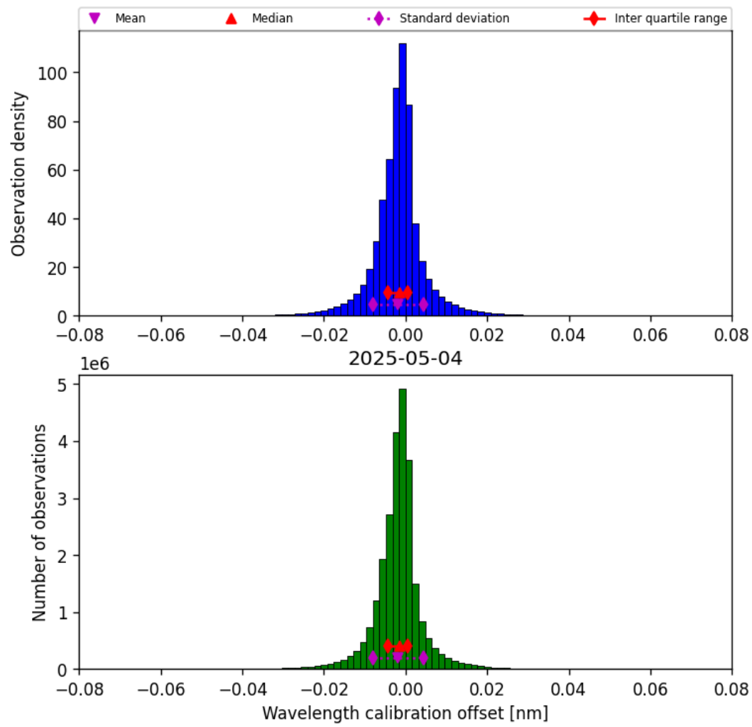
Figure 33: Histogram of “Wavelength calibration offset” for 2025-05-04 to 2025-05-05
