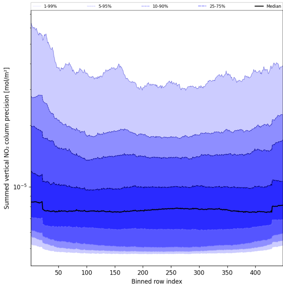
Figure 56: Along track statistics of “Summed vertical NO 2 column precision” for 2025-05-04 to 2025-05-05
