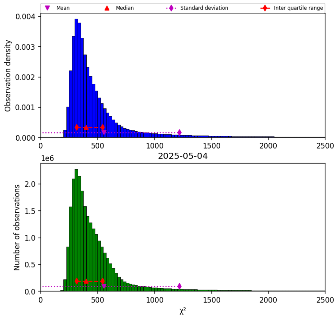
Figure 40: Histogram of “ \chi^2 ” for 2025-05-04 to 2025-05-05
