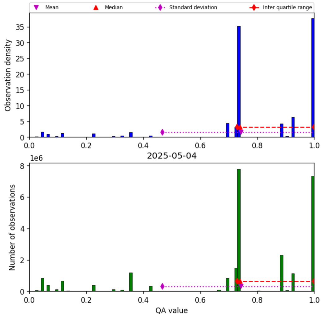
Figure 26: Histogram of “QA value” for 2025-05-04 to 2025-05-05
