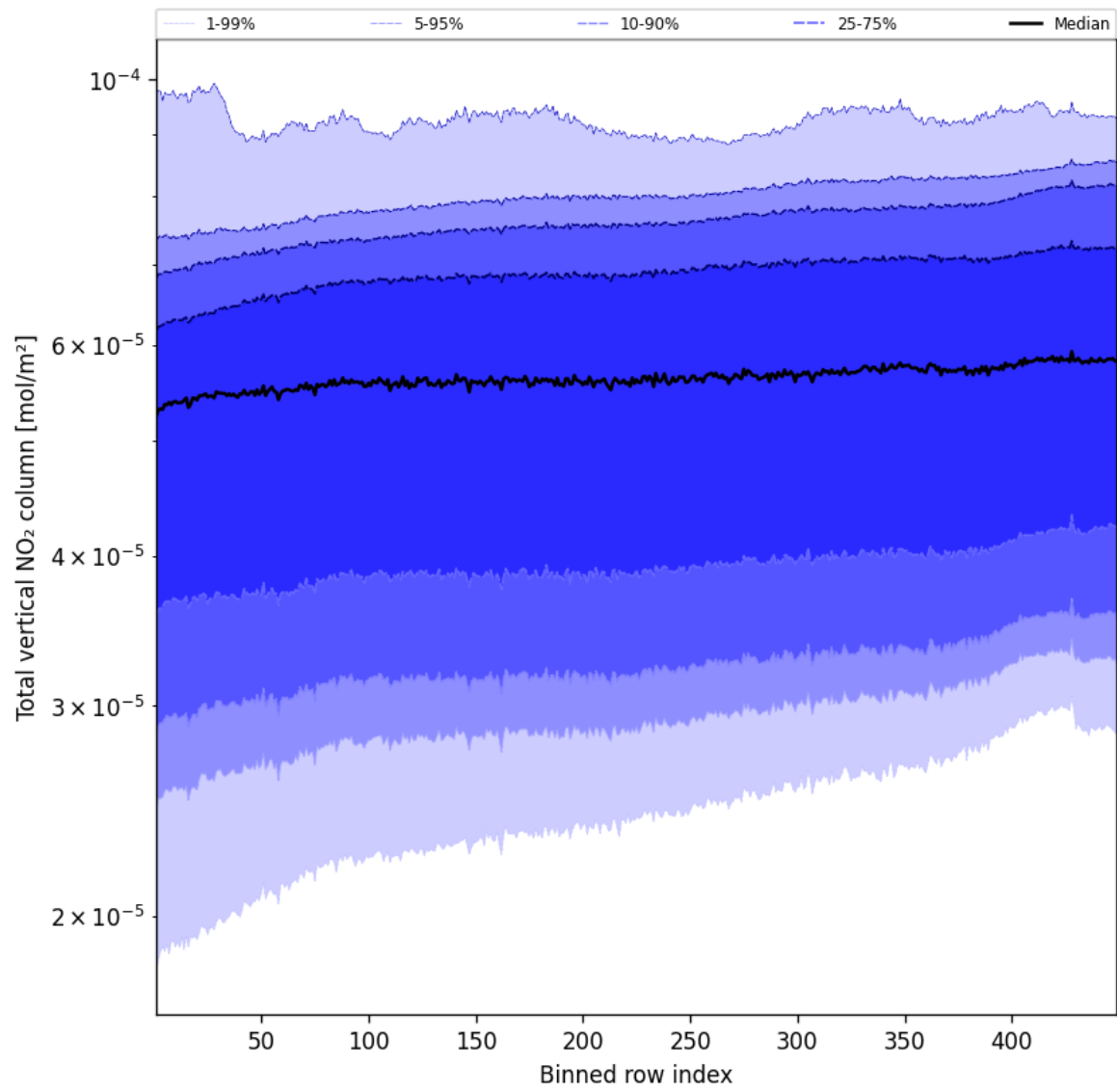
Figure 53: Along track statistics of “Total vertical NO 2 column” for 2025-05-04 to 2025-05-05
