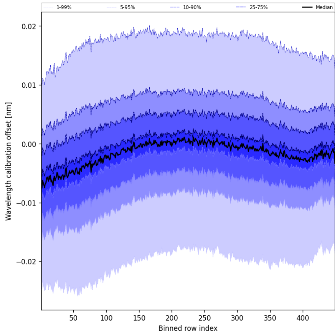
Figure 50: Along track statistics of “Wavelength calibration offset” for 2025-05-04 to 2025-05-05
