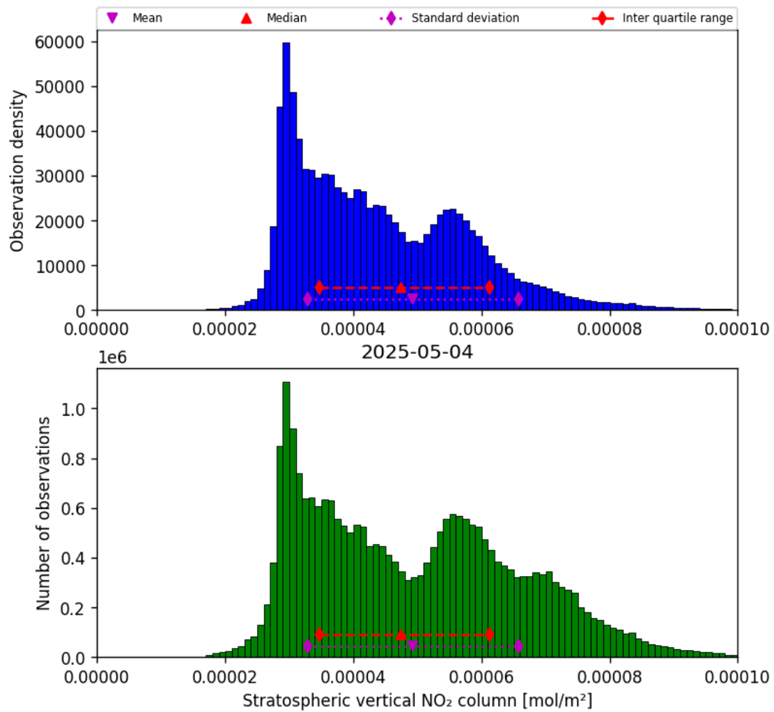
Figure 34: Histogram of “Stratospheric vertical NO 2 column” for 2025-05-04 to 2025-05-05
