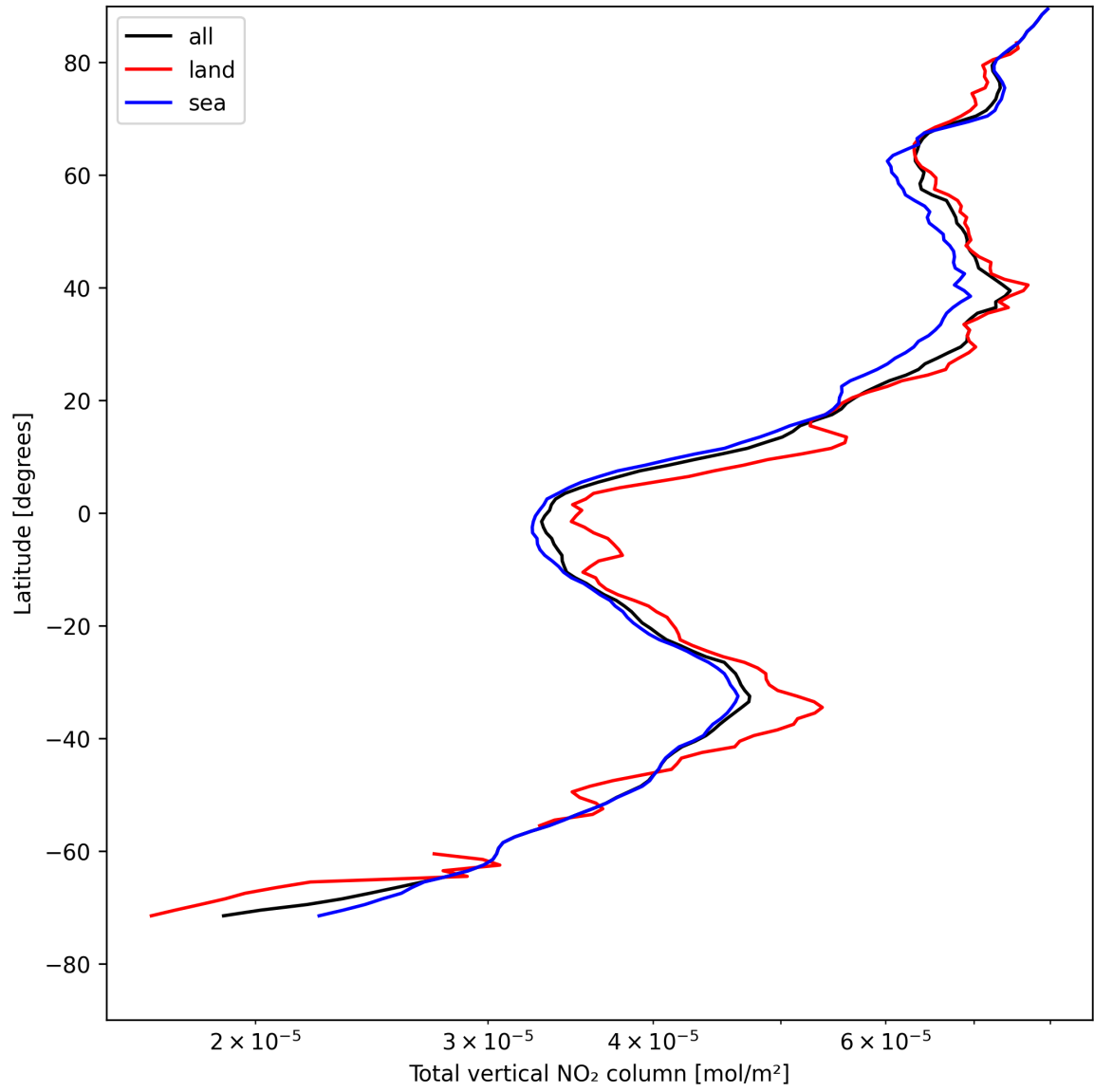
Figure 19: Zonal average of “Total vertical NO 2 column” for 2025-05-04 to 2025-05-05.
