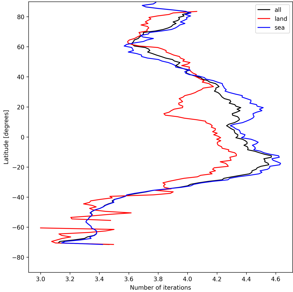
Figure 15: Zonal average of “Number of iterations” for 2025-05-04 to 2025-05-05.
