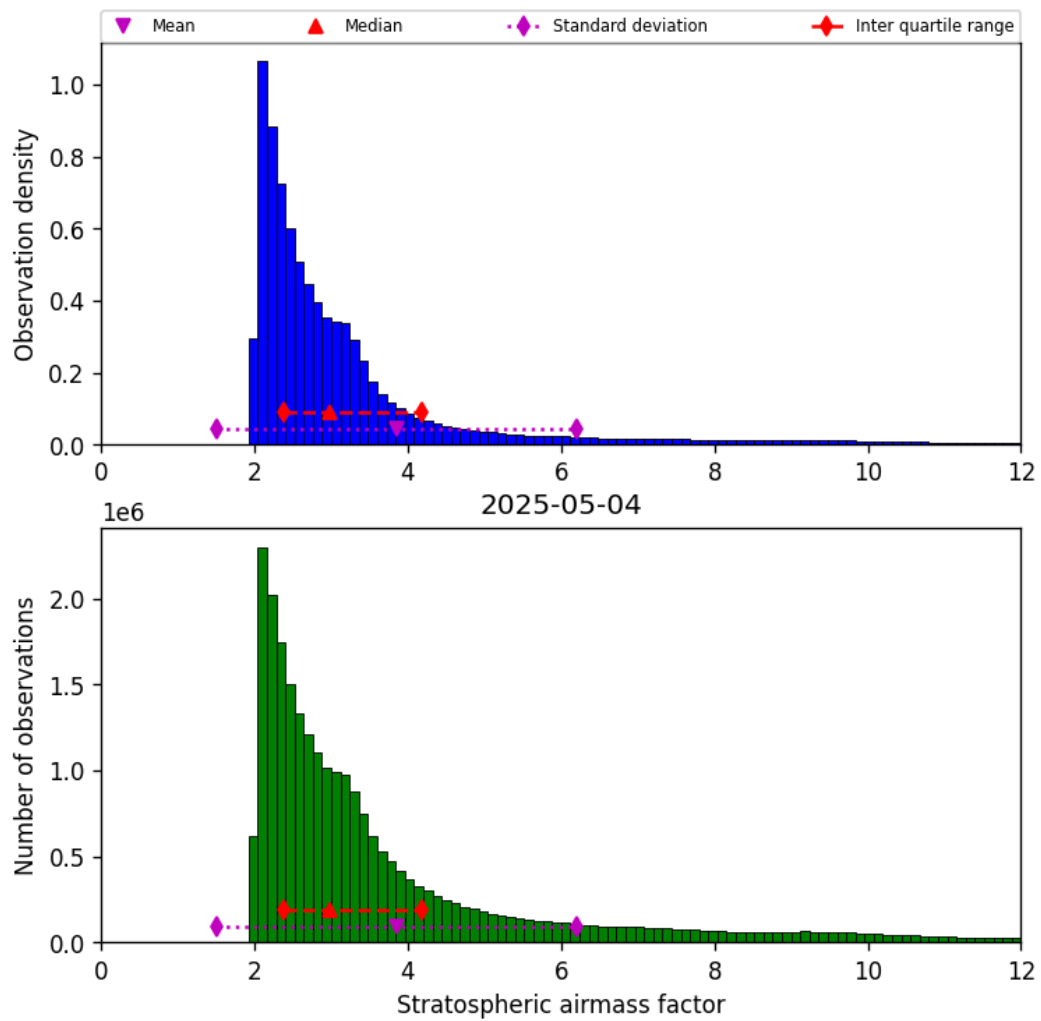
Figure 42: Histogram of “Stratospheric airmass factor” for 2025-05-04 to 2025-05-05
