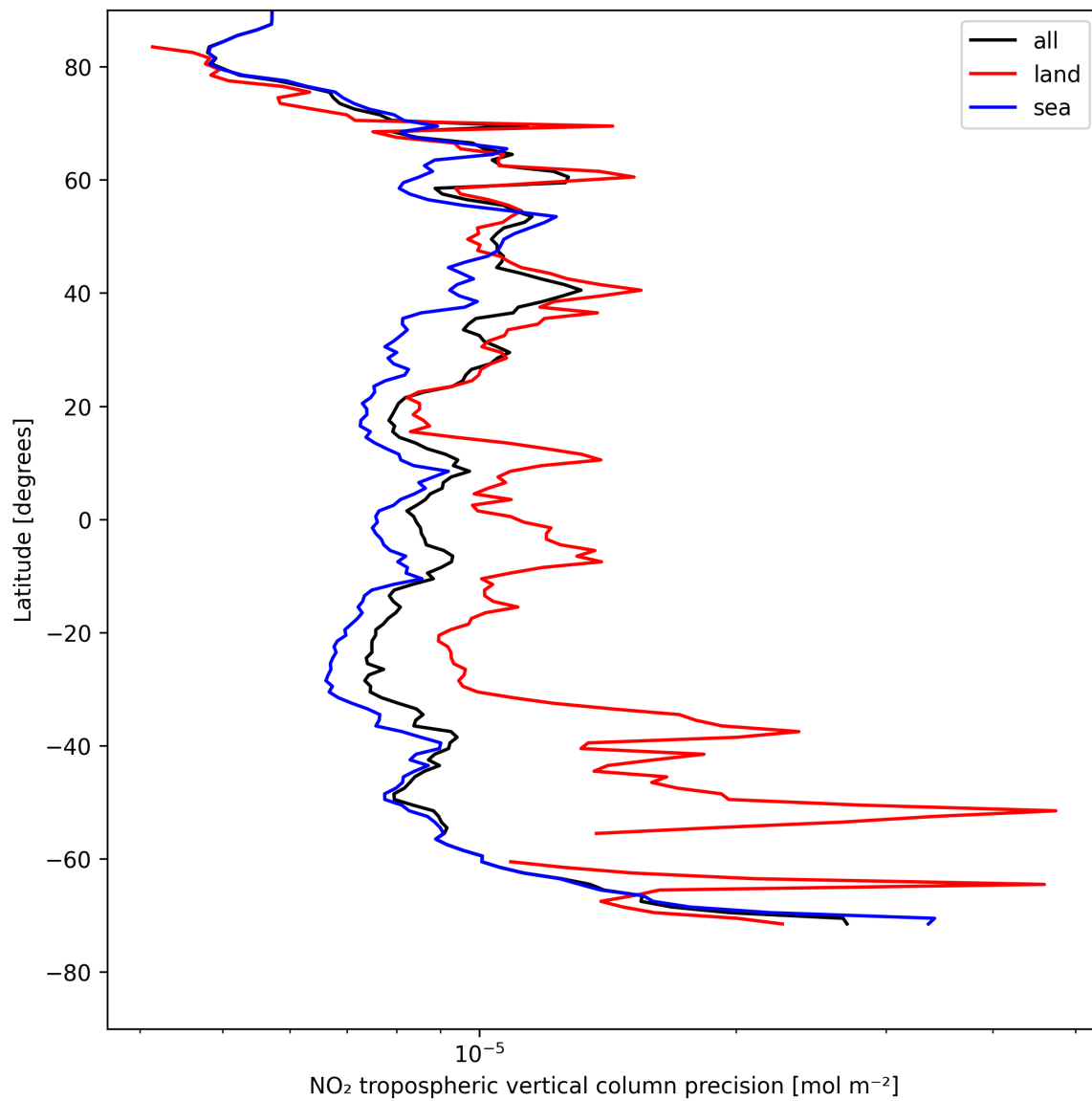
Figure 11: Zonal average of “NO 2 tropospheric vertical column precision” for 2025-05-04 to 2025-05-05.
