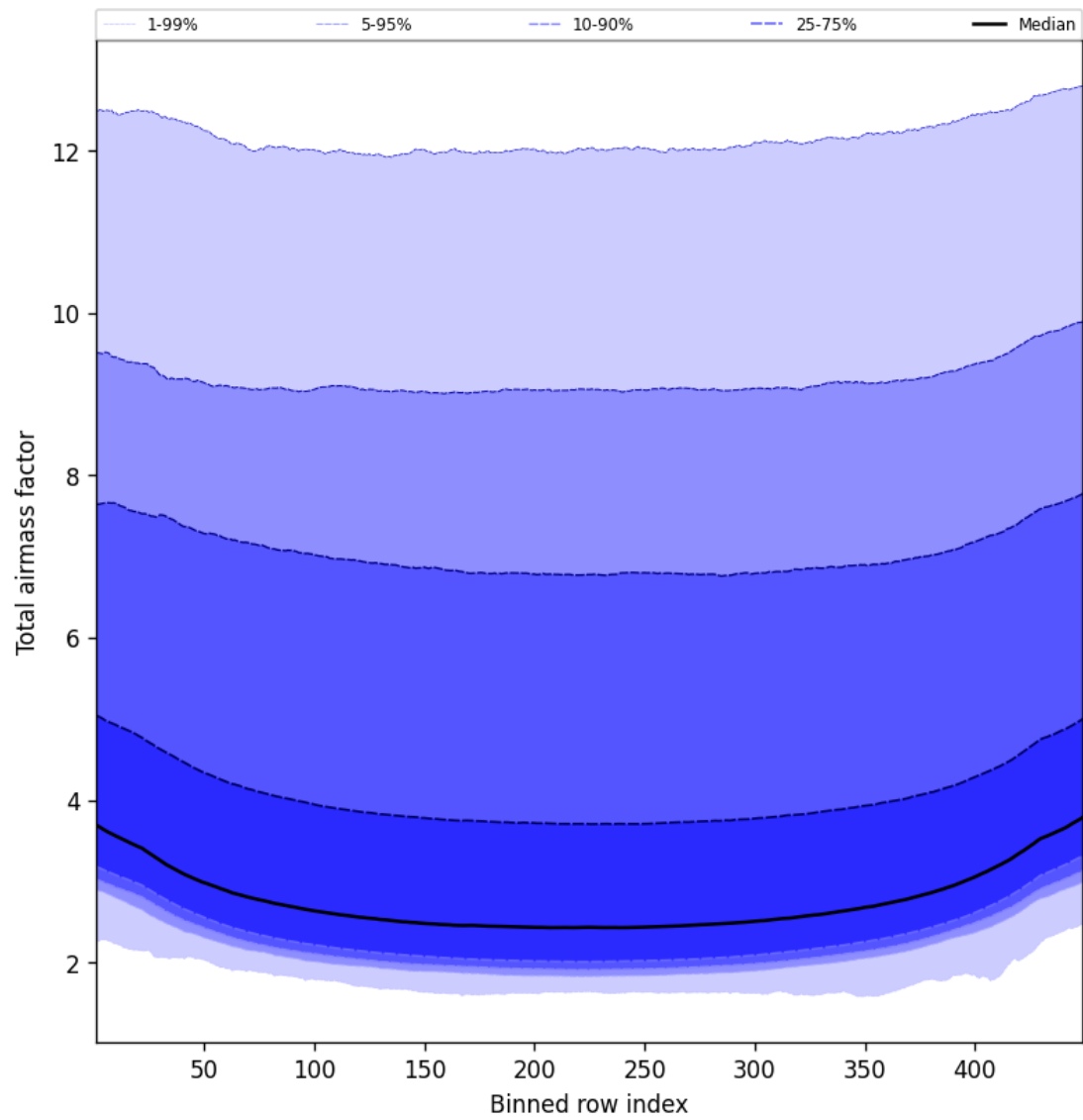
Figure 47: Along track statistics of “Total airmass factor” for 2025-05-04 to 2025-05-05
