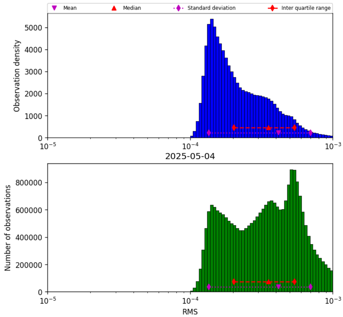
Figure 41: Histogram of “RMS” for 2025-05-04 to 2025-05-05
