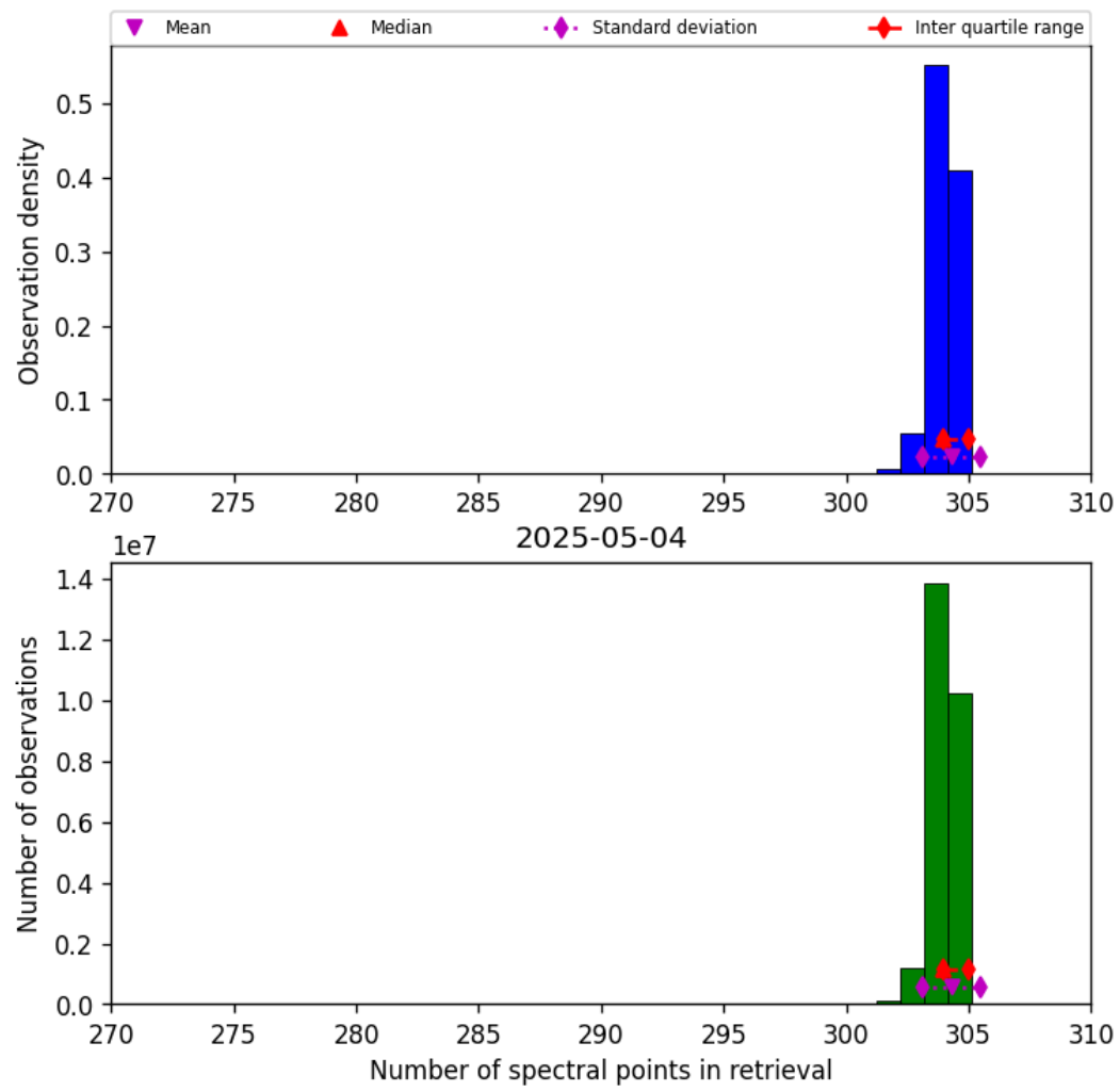
Figure 31: Histogram of “Number of spectral points in retrieval” for 2025-05-04 to 2025-05-05
