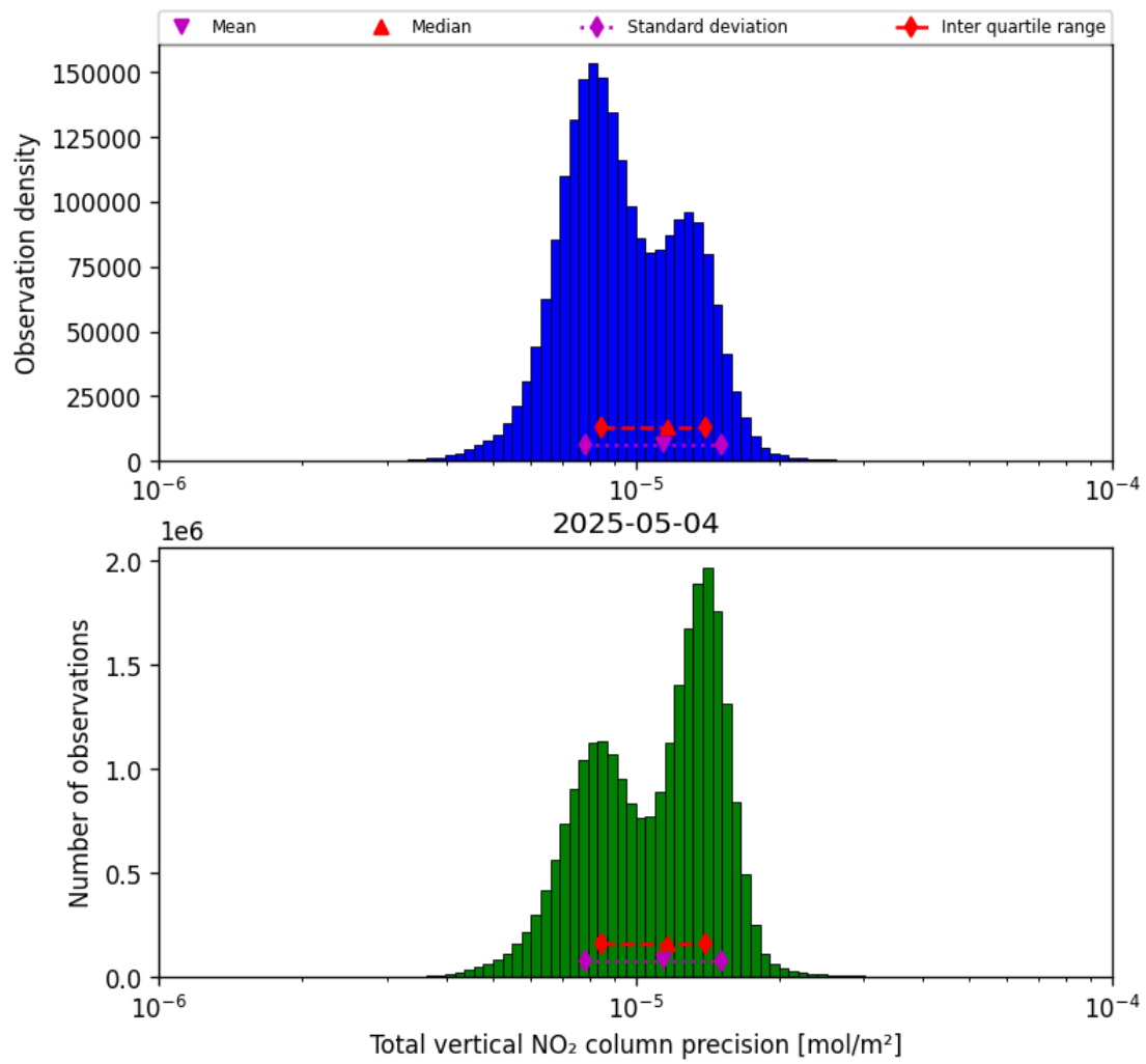
Figure 37: Histogram of “Total vertical NO 2 column precision” for 2025-05-04 to 2025-05-05
