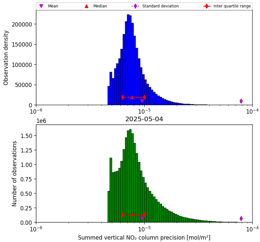
Figure 39: Histogram of "Summed vertical NO 2 column precision" for 2025-05-04 to 2025-05-05
