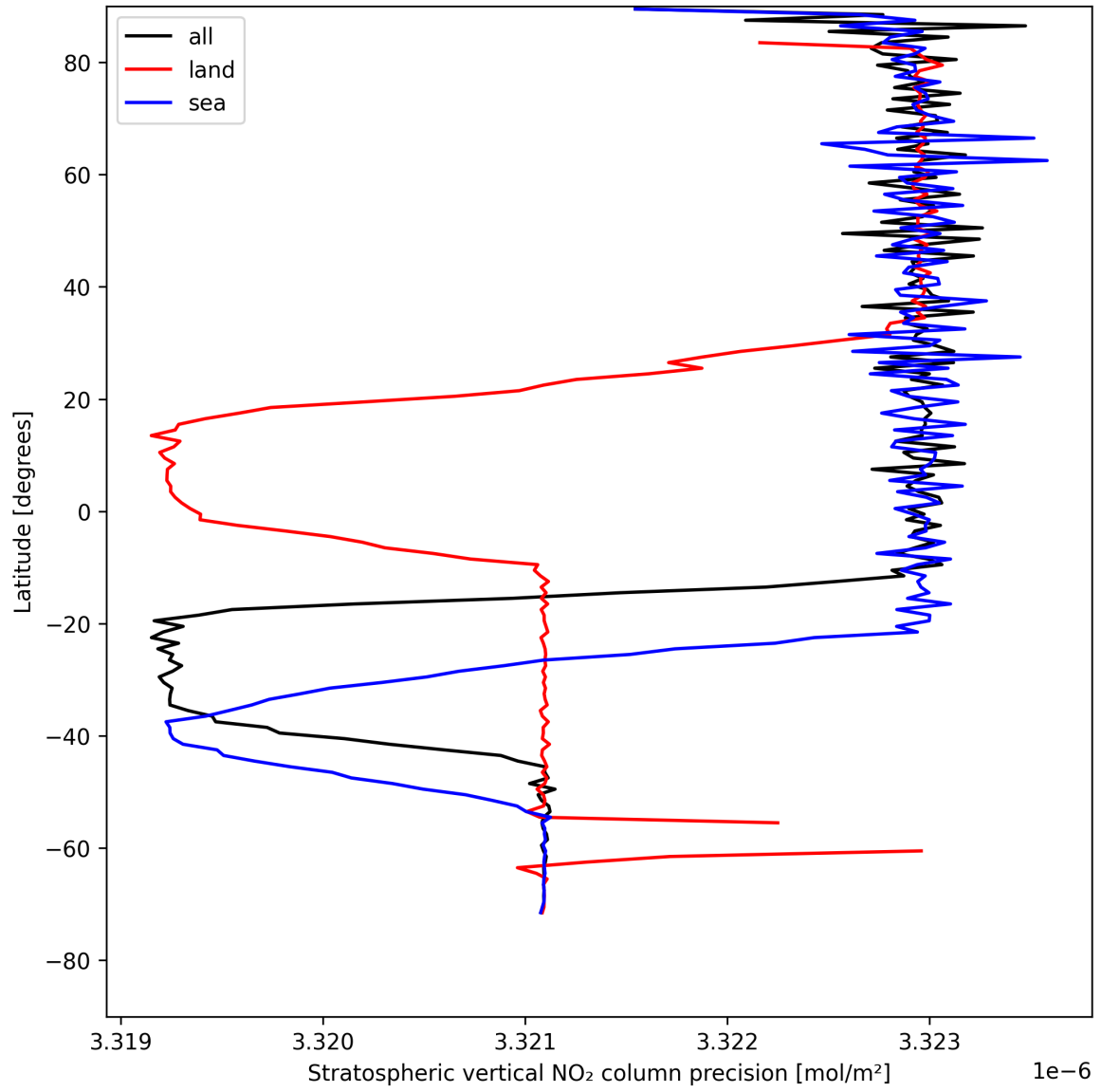
Figure 18: Zonal average of “Stratospheric vertical NO 2 column precision” for 2025-05-04 to 2025-05-05.
