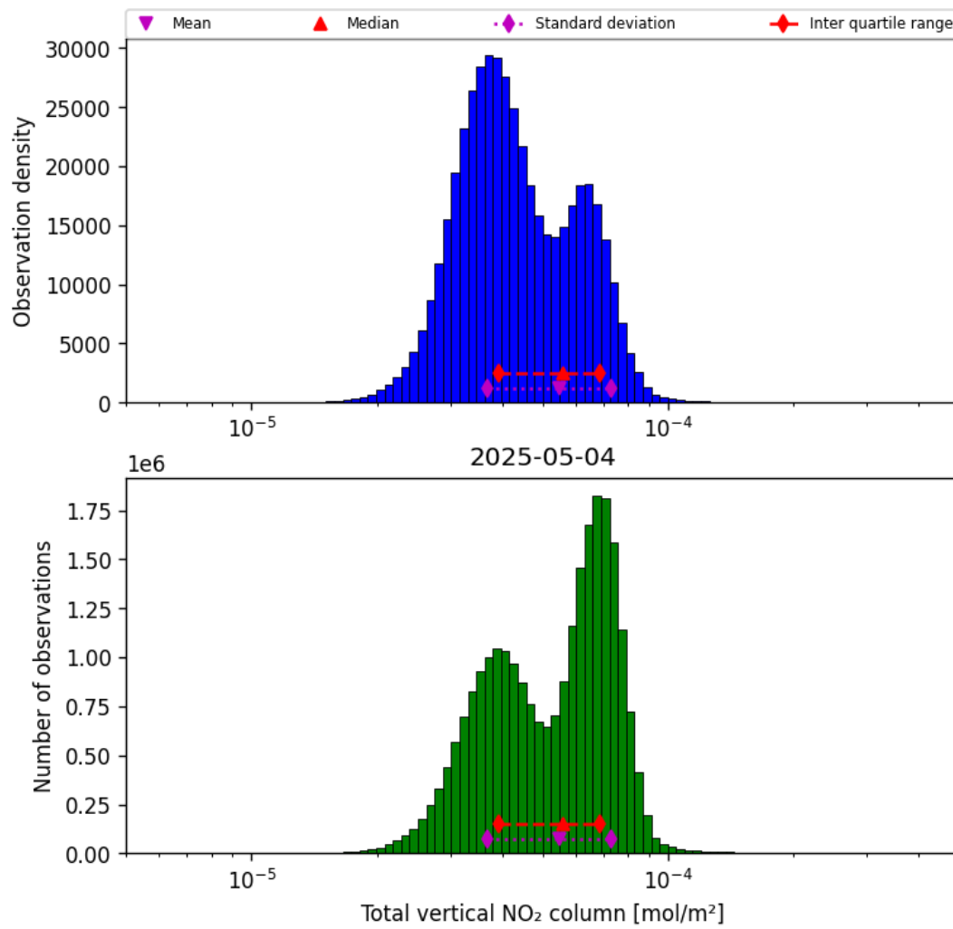
Figure 36: Histogram of "Total vertical NO 2 column" for 2025-05-04 to 2025-05-05
