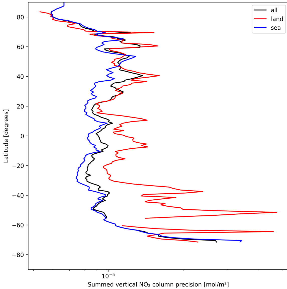
Figure 22: Zonal average of “Summed vertical NO 2 column precision” for 2025-05-04 to 2025-05-05.
