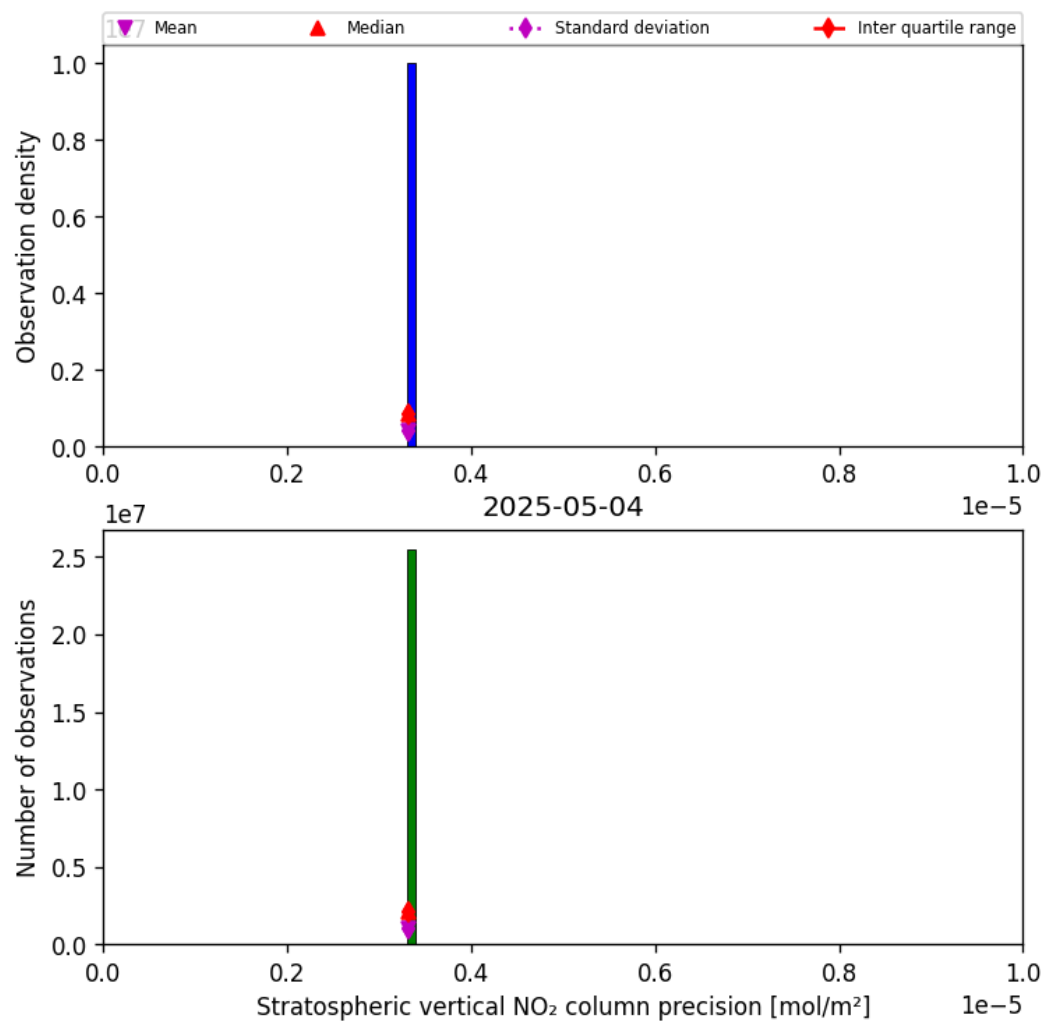
Figure 35: Histogram of “Stratospheric vertical NO 2 column precision” for 2025-05-04 to 2025-05-05
