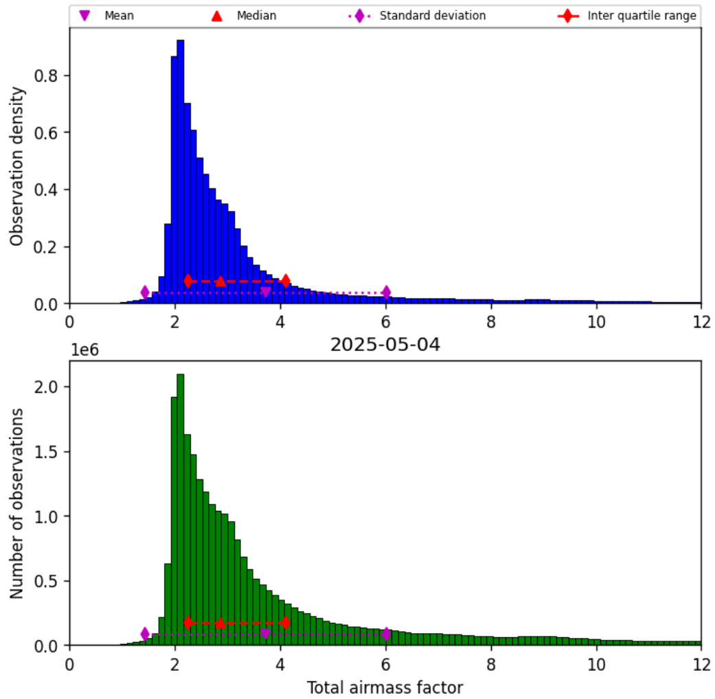
Figure 30: Histogram of “Total airmass factor” for 2025-05-04 to 2025-05-05
