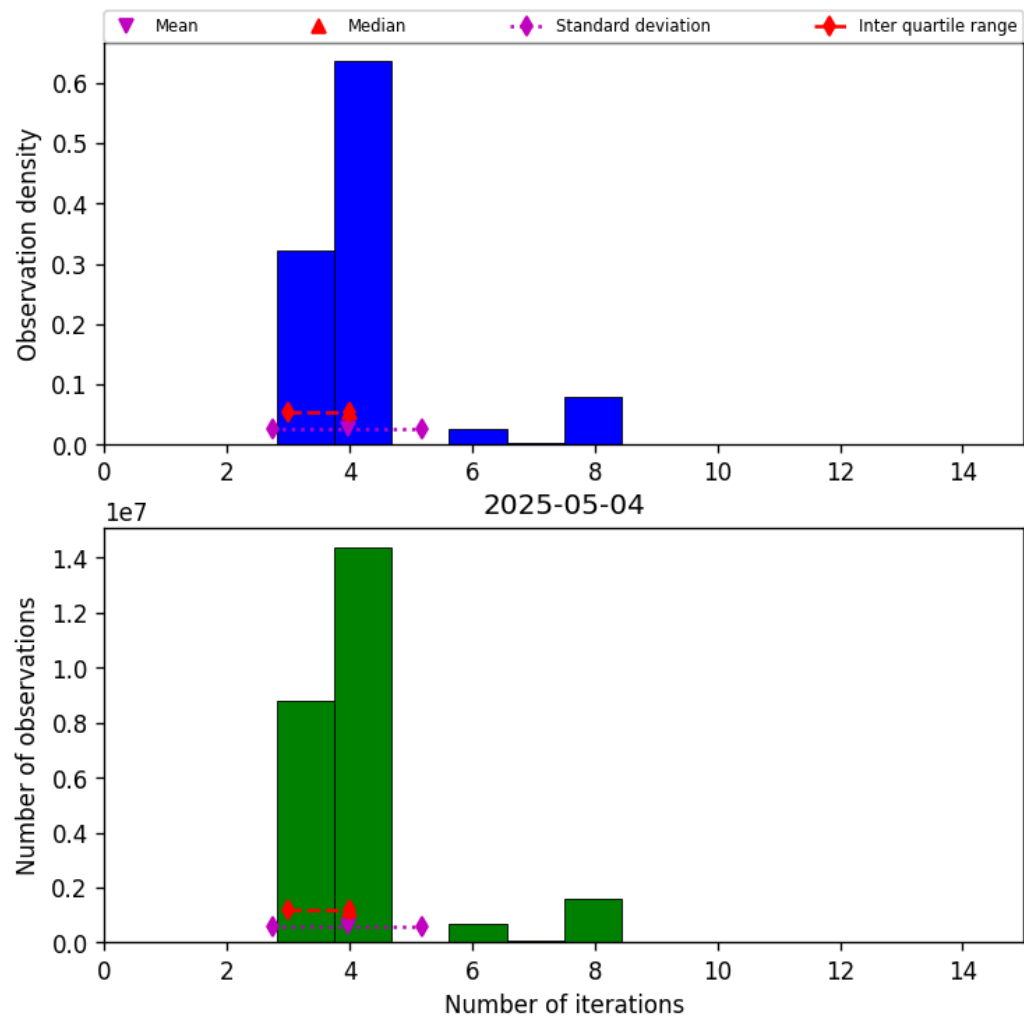
Figure 32: Histogram of “Number of iterations” for 2025-05-04 to 2025-05-05
