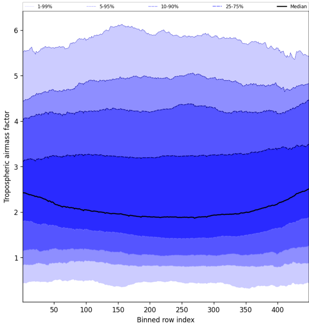
Figure 46: Along track statistics of “Tropospheric airmass factor” for 2025-05-04 to 2025-05-05
