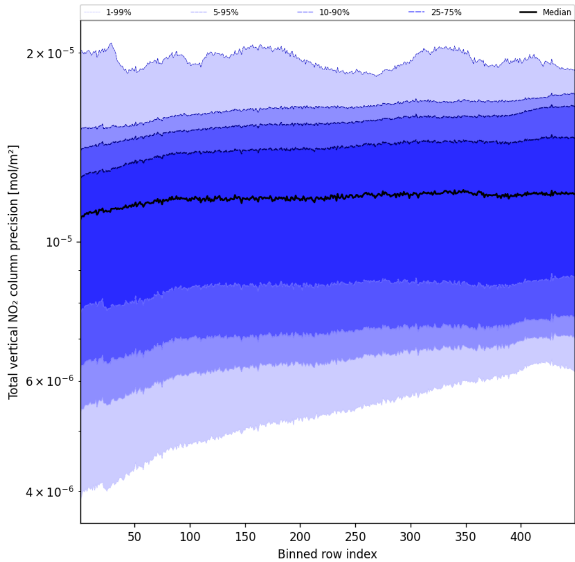
Figure 54: Along track statistics of “Total vertical NO 2 column precision” for 2025-05-04 to 2025-05-05
