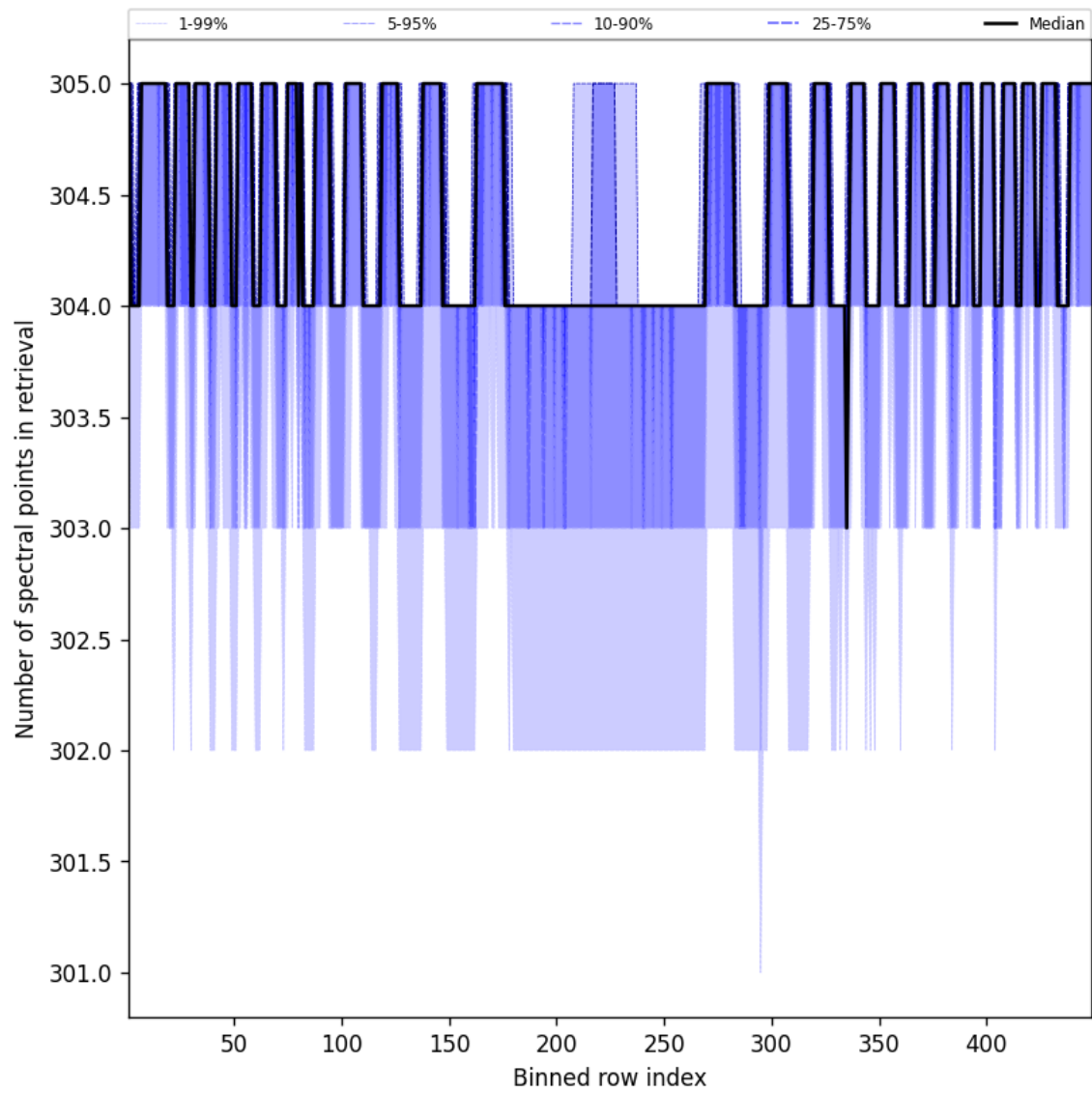
Figure 48: Along track statistics of “Number of spectral points in retrieval” for 2025-05-04 to 2025-05-05
