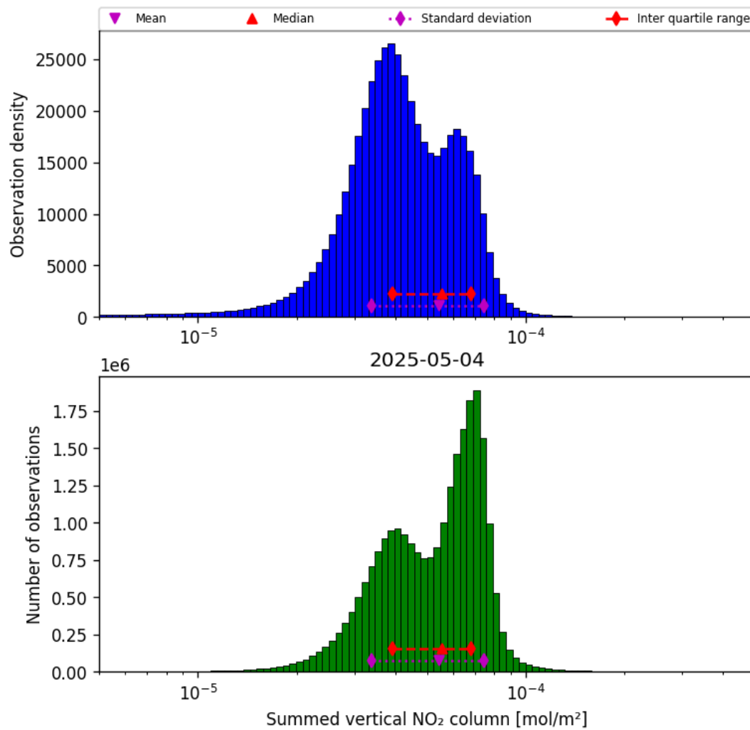
Figure 38: Histogram of “Summed vertical NO 2 column” for 2025-05-04 to 2025-05-05
