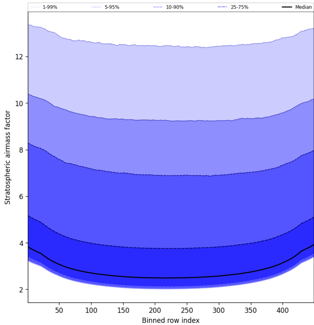
Figure 59: Along track statistics of “Stratospheric airmass factor” for 2025-05-04 to 2025-05-05
