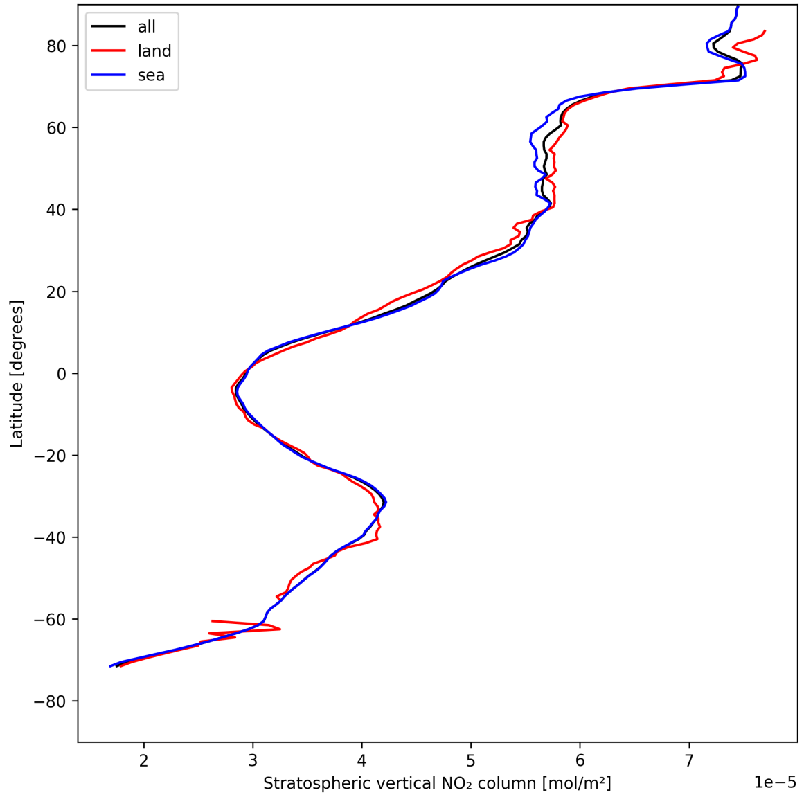
Figure 17: Zonal average of “Stratospheric vertical NO 2 column” for 2025-05-04 to 2025-05-05.
