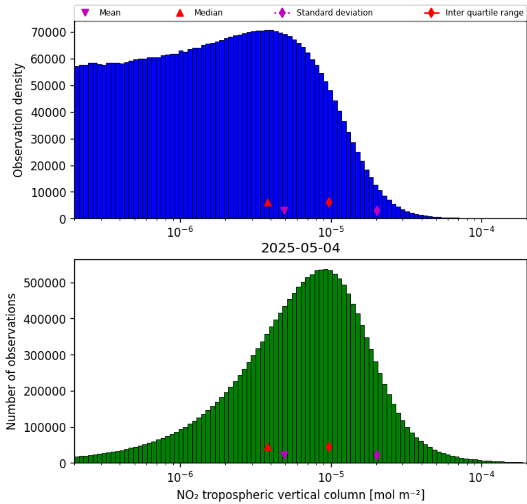
Figure 27: Histogram of “NO 2 tropospheric vertical column” for 2025-05-04 to 2025-05-05
