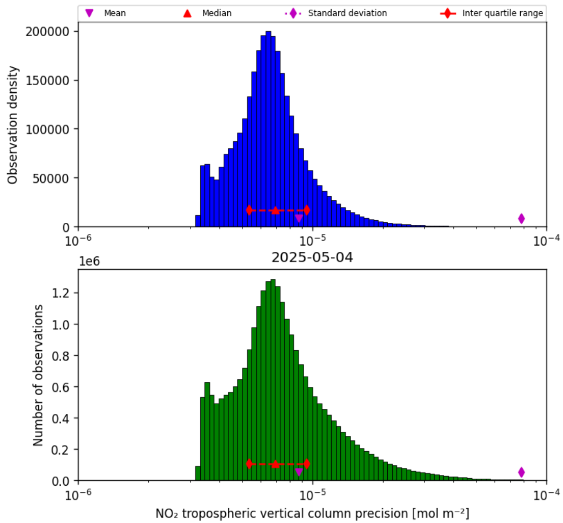
Figure 28: Histogram of “NO 2 tropospheric vertical column precision” for 2025-05-04 to 2025-05-05
