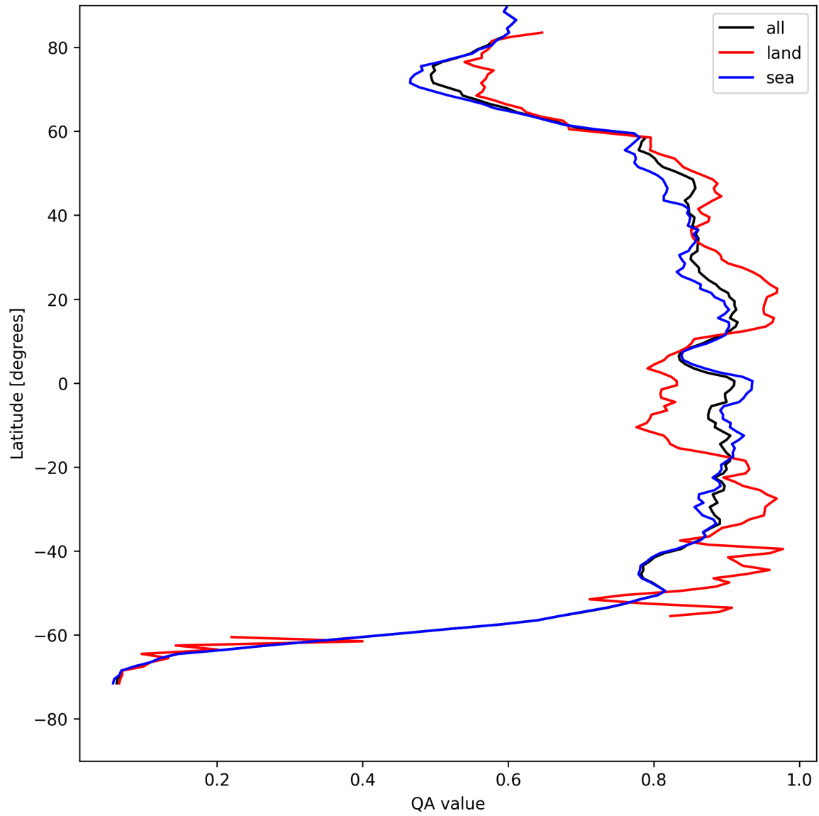
Figure 9: Zonal average of “QA value” for 2025-05-04 to 2025-05-05.
