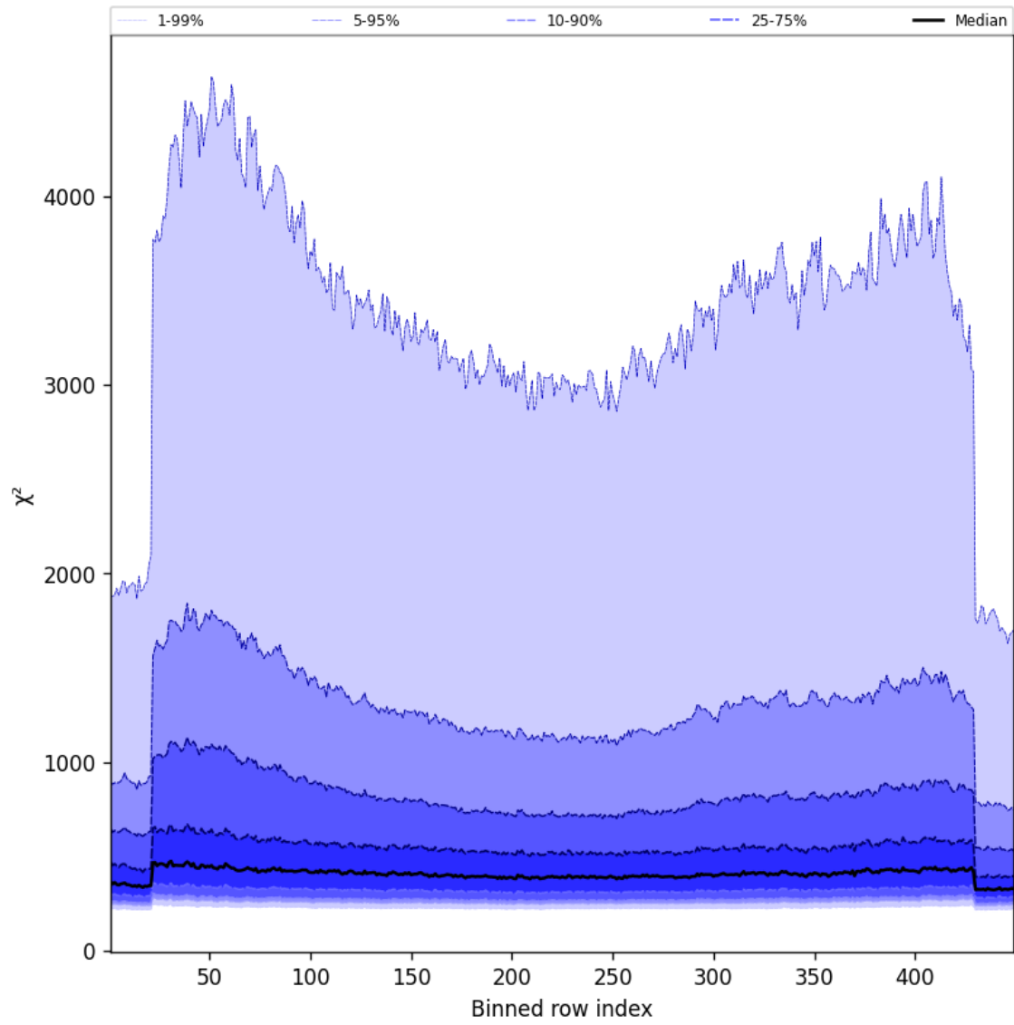
Figure 57: Along track statistics of “ \chi^2 ” for 2025-05-04 to 2025-05-05
