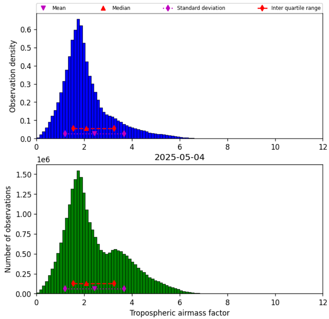
Figure 29: Histogram of “Tropospheric airmass factor” for 2025-05-04 to 2025-05-05
