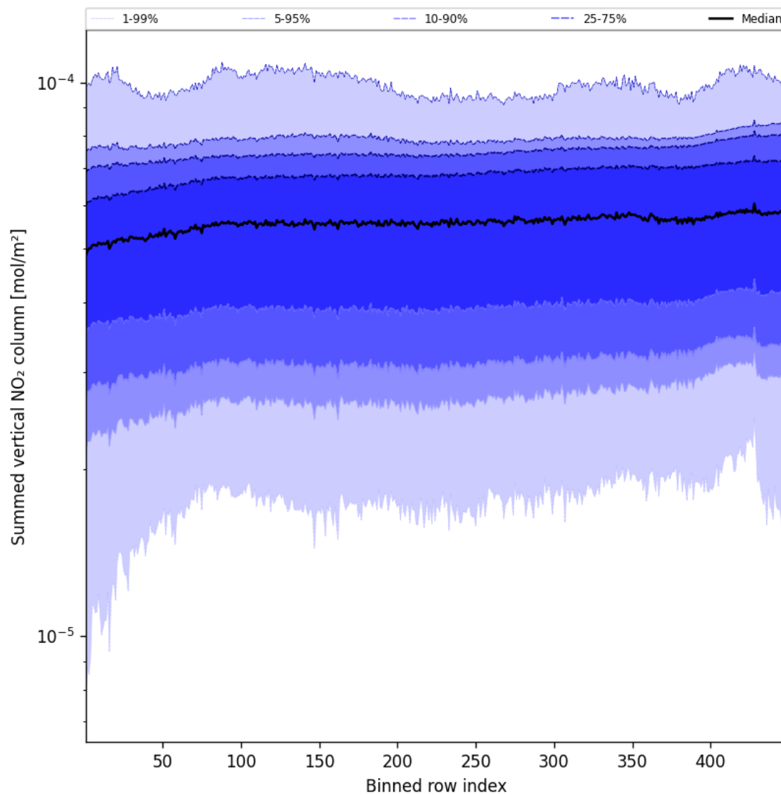
Figure 55: Along track statistics of “Summed vertical NO 2 column” for 2025-05-04 to 2025-05-05
