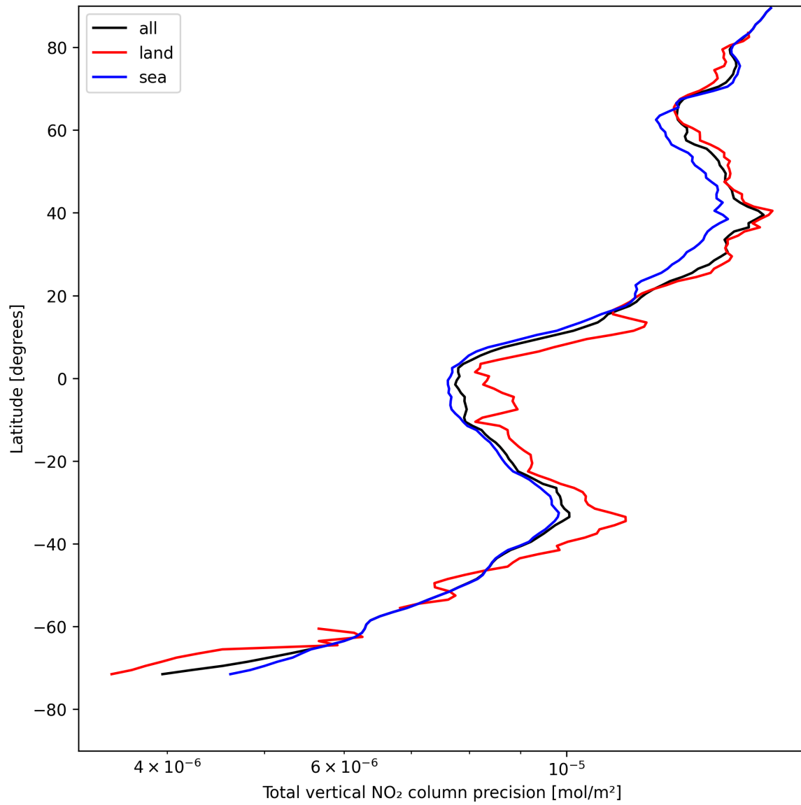
Figure 20: Zonal average of “Total vertical NO 2 column precision” for 2025-05-04 to 2025-05-05.
