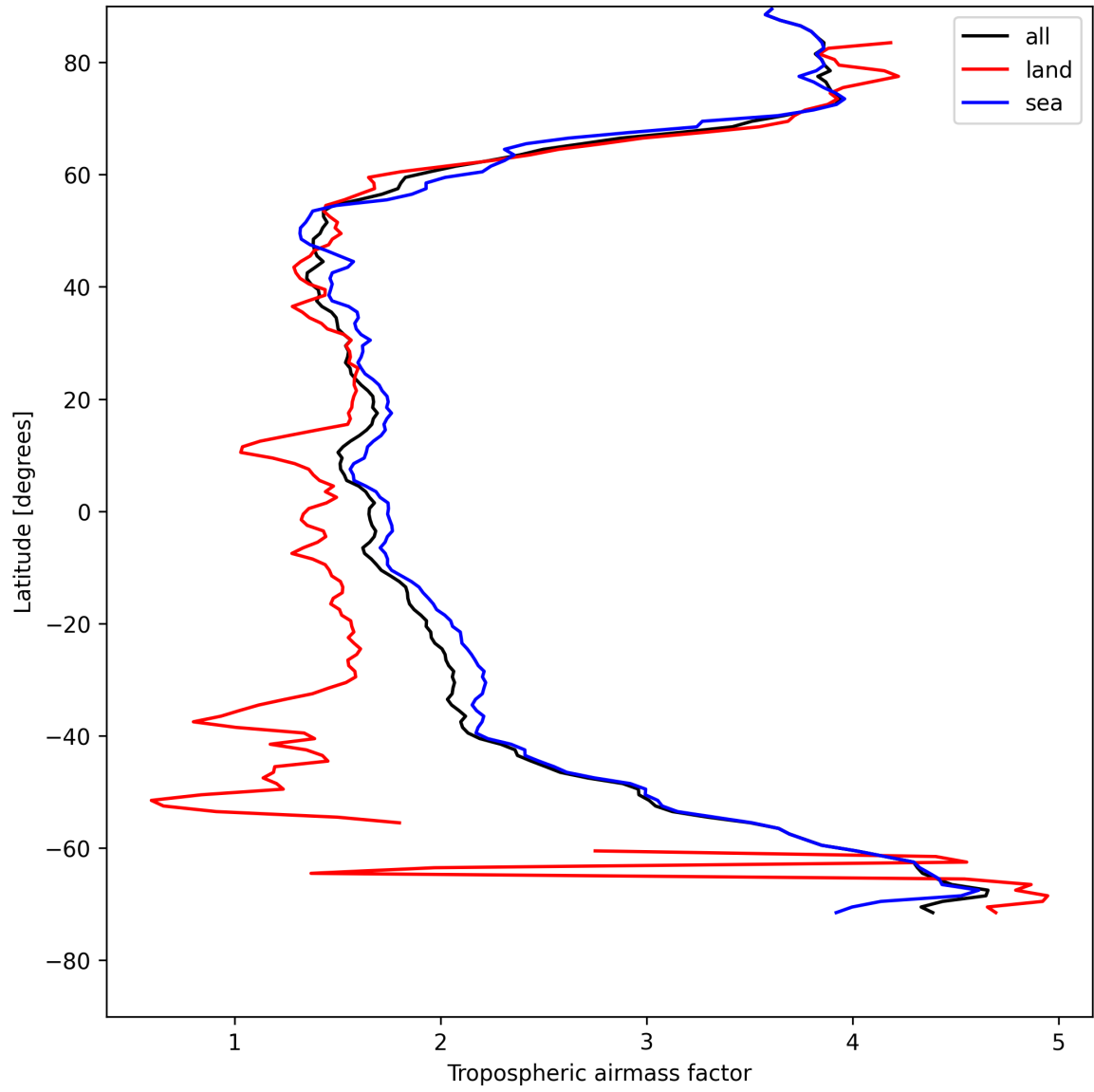
Figure 12: Zonal average of “Tropospheric airmass factor” for 2025-05-04 to 2025-05-05.
