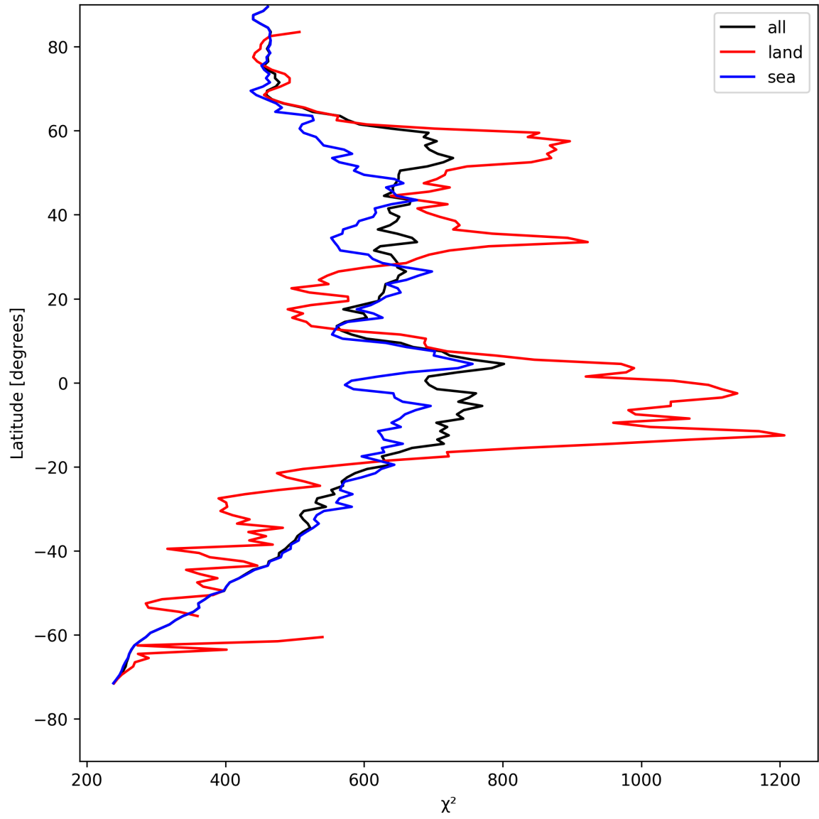
Figure 23: Zonal average of “ \chi^2 ” for 2025-05-04 to 2025-05-05.
