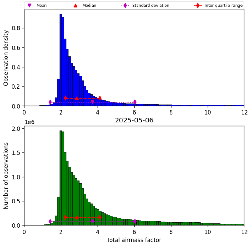
Figure 30: Histogram of “Total airmass factor” for 2025-05-06 to 2025-05-07
