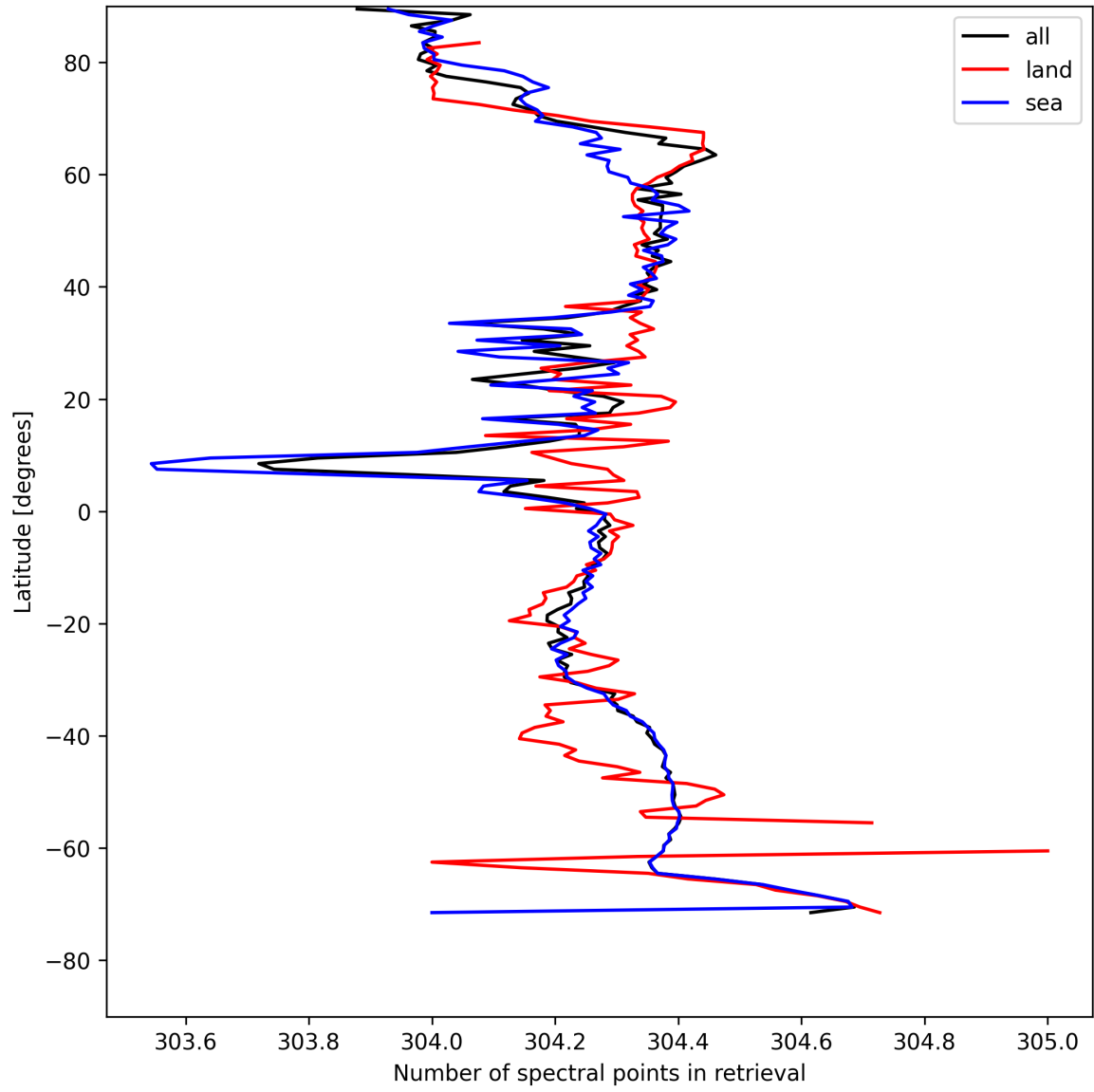
Figure 14: Zonal average of “Number of spectral points in retrieval” for 2025-05-06 to 2025-05-07.
