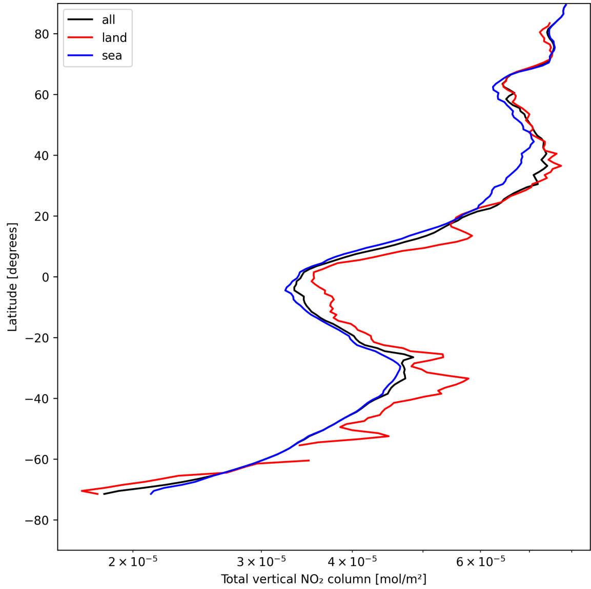
Figure 19: Zonal average of “Total vertical NO 2 column” for 2025-05-06 to 2025-05-07.
