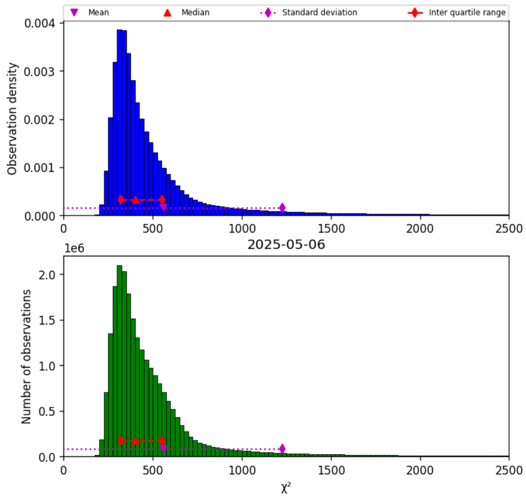
Figure 40: Histogram of “ \chi^2 ” for 2025-05-06 to 2025-05-07
