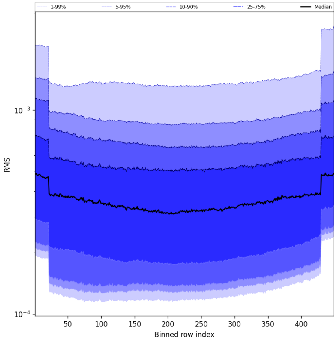
Figure 58: Along track statistics of “RMS” for 2025-05-06 to 2025-05-07
