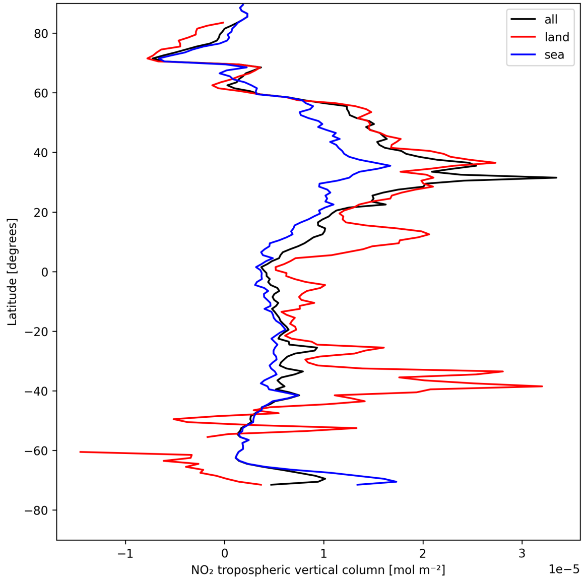
Figure 10: Zonal average of “NO 2 tropospheric vertical column” for 2025-05-06 to 2025-05-07.
