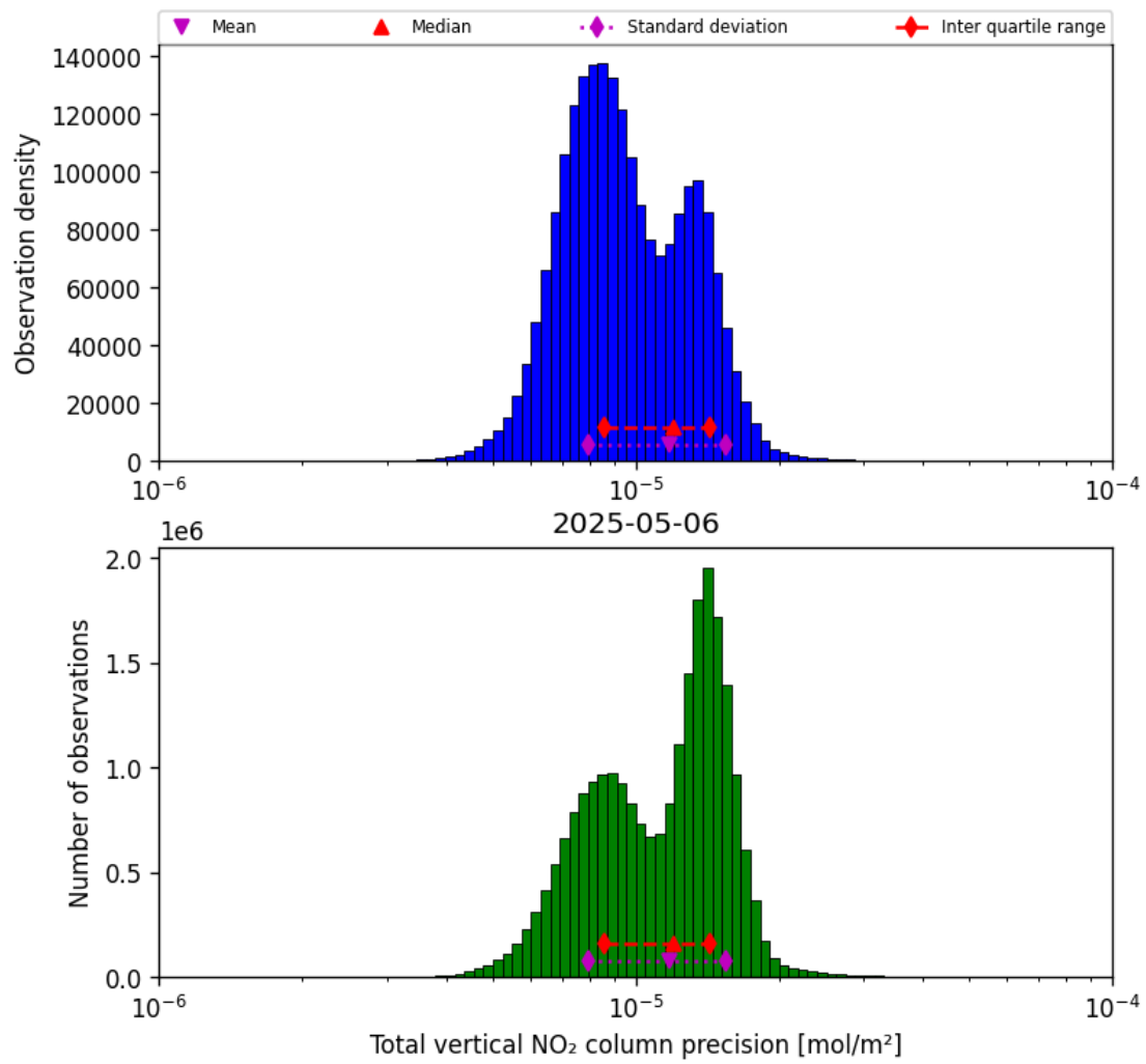
Figure 37: Histogram of “Total vertical NO 2 column precision” for 2025-05-06 to 2025-05-07
