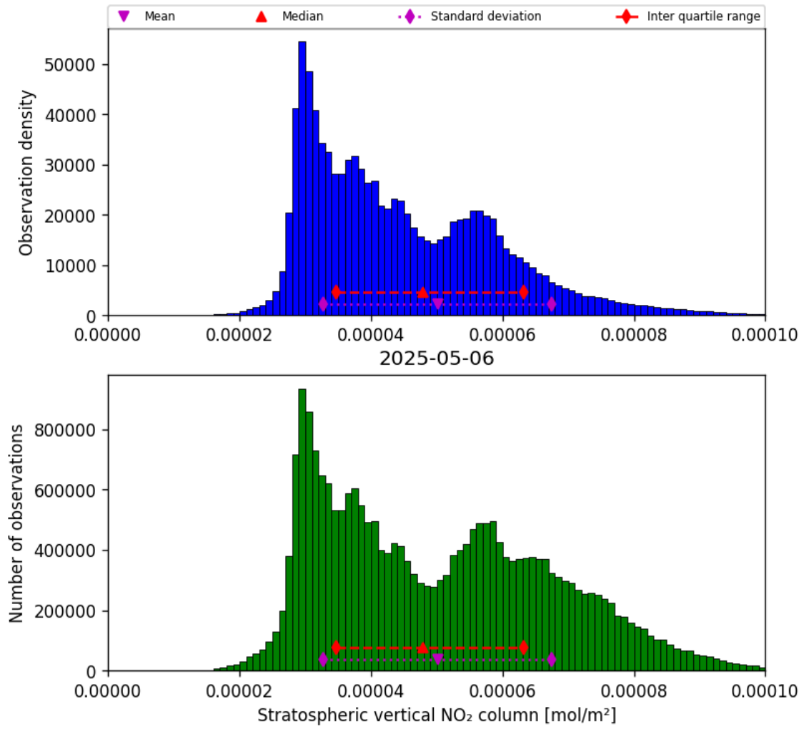
Figure 34: Histogram of “Stratospheric vertical NO 2 column” for 2025-05-06 to 2025-05-07
