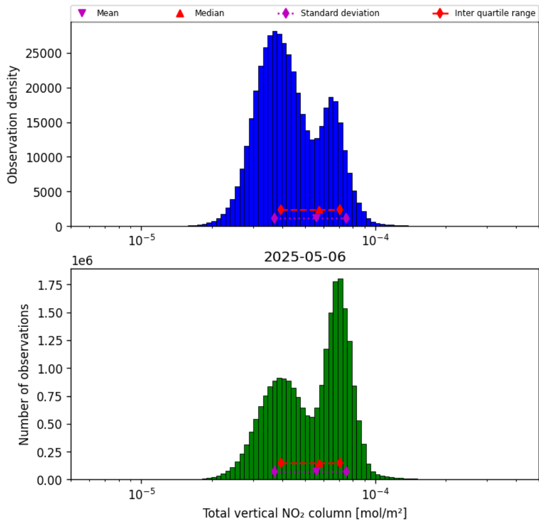
Figure 36: Histogram of “Total vertical NO 2 column” for 2025-05-06 to 2025-05-07
