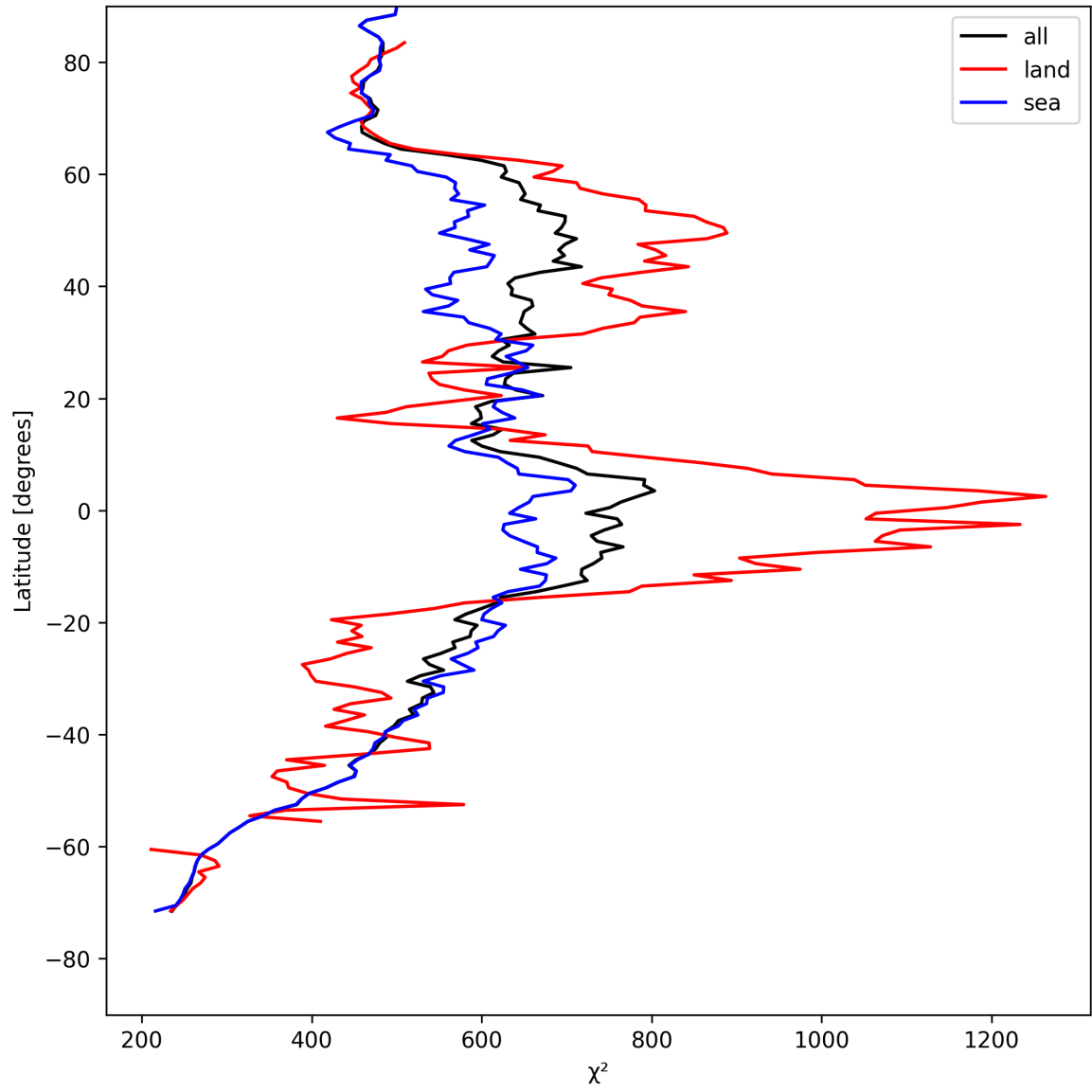
Figure 23: Zonal average of “ \chi^2 ” for 2025-05-06 to 2025-05-07.
