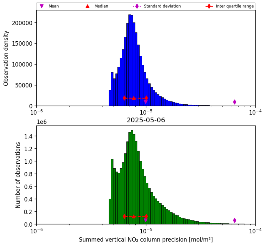
Figure 39: Histogram of “Summed vertical NO 2 column precision” for 2025-05-06 to 2025-05-07
