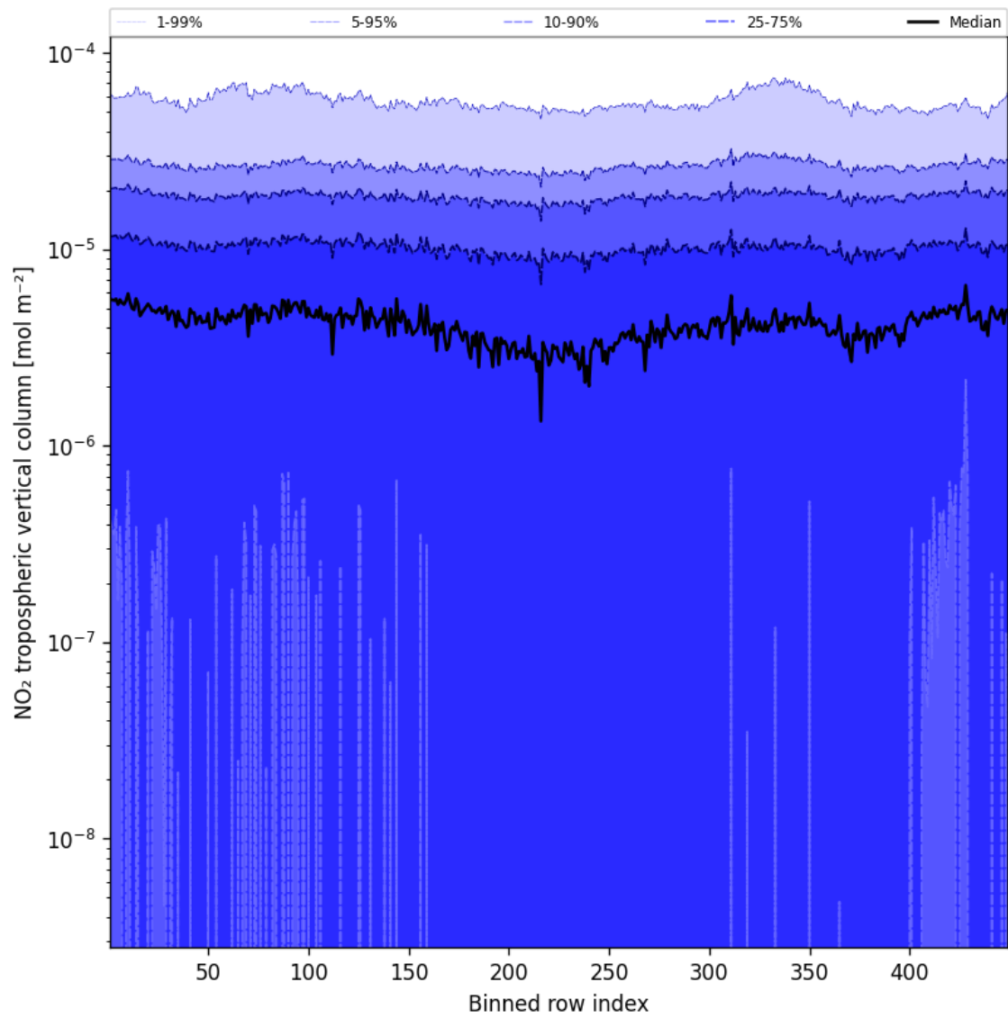
Figure 44: Along track statistics of “NO 2 tropospheric vertical column” for 2025-05-06 to 2025-05-07
