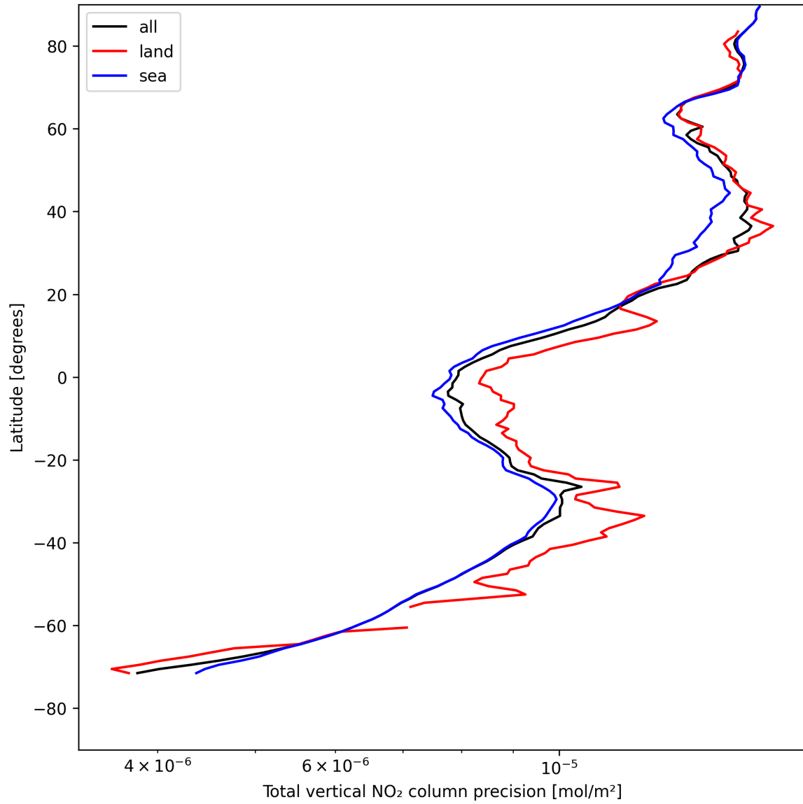
Figure 20: Zonal average of “Total vertical NO 2 column precision” for 2025-05-06 to 2025-05-07.
