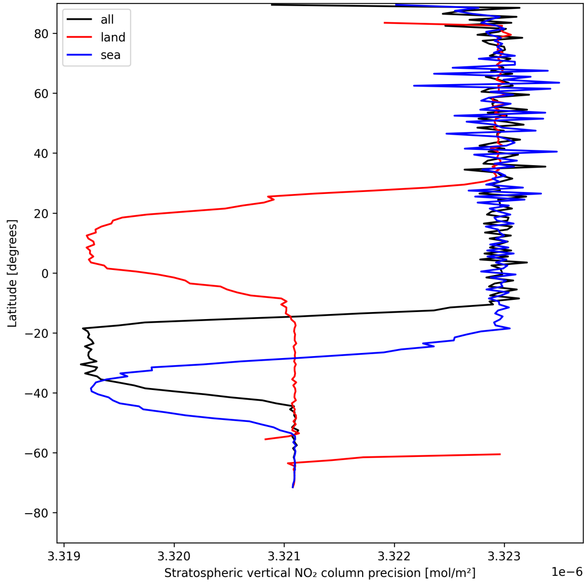
Figure 18: Zonal average of “Stratospheric vertical NO 2 column precision” for 2025-05-06 to 2025-05-07.
