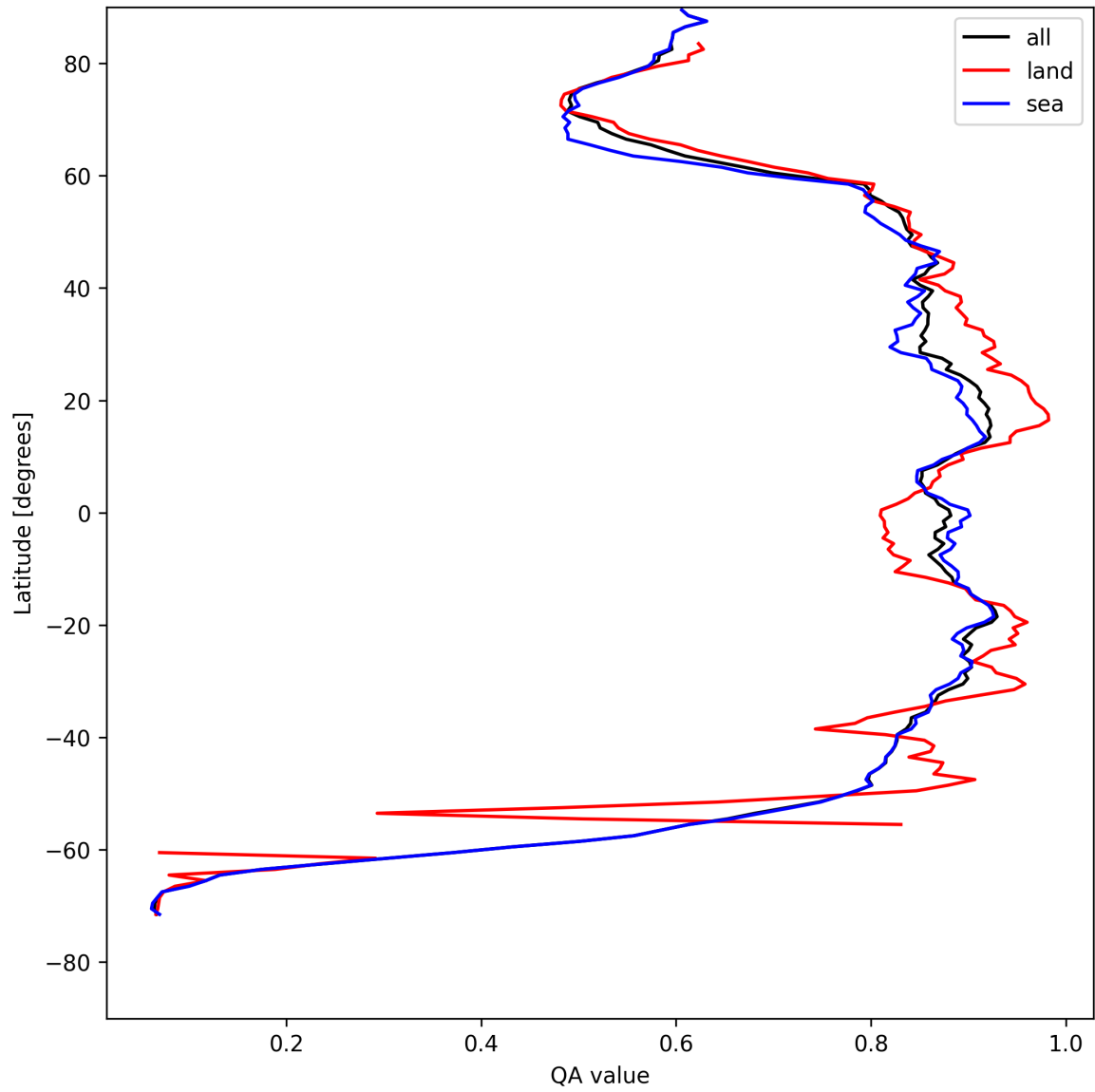
Figure 9: Zonal average of “QA value” for 2025-05-06 to 2025-05-07.
