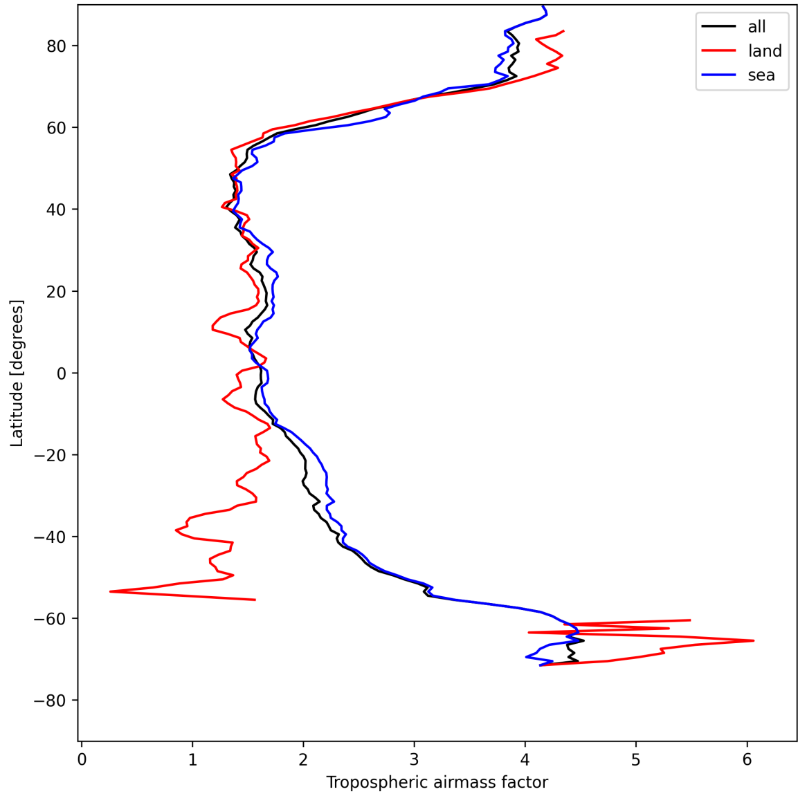
Figure 12: Zonal average of “Tropospheric airmass factor” for 2025-05-06 to 2025-05-07.
