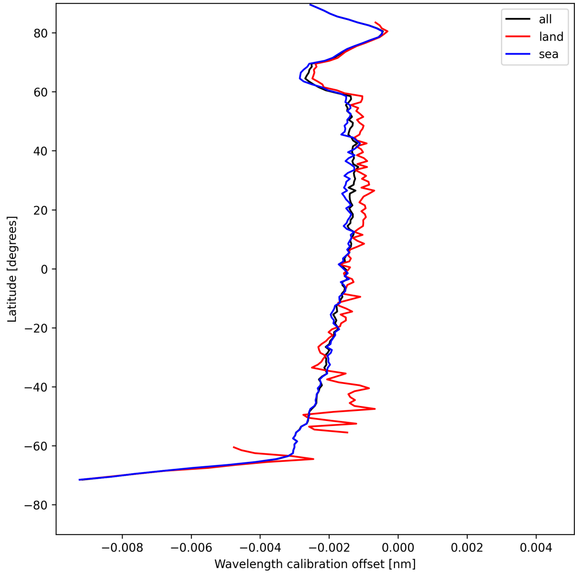
Figure 16: Zonal average of “Wavelength calibration offset” for 2025-05-06 to 2025-05-07.
