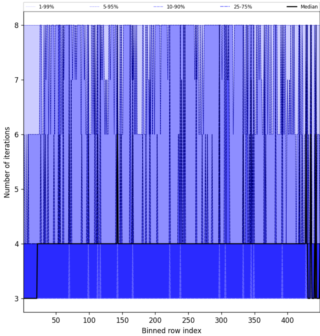
Figure 49: Along track statistics of “Number of iterations” for 2025-05-06 to 2025-05-07
