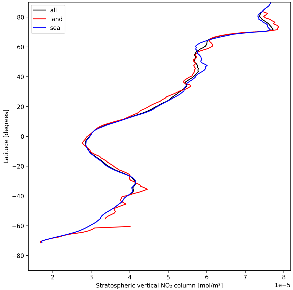
Figure 17: Zonal average of “Stratospheric vertical NO 2 column” for 2025-05-06 to 2025-05-07.
