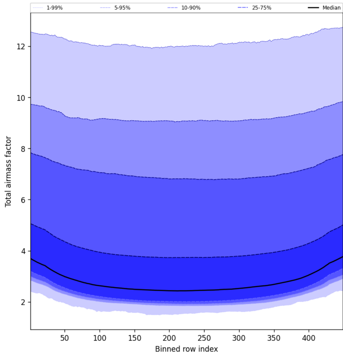
Figure 47: Along track statistics of “Total airmass factor” for 2025-05-06 to 2025-05-07
