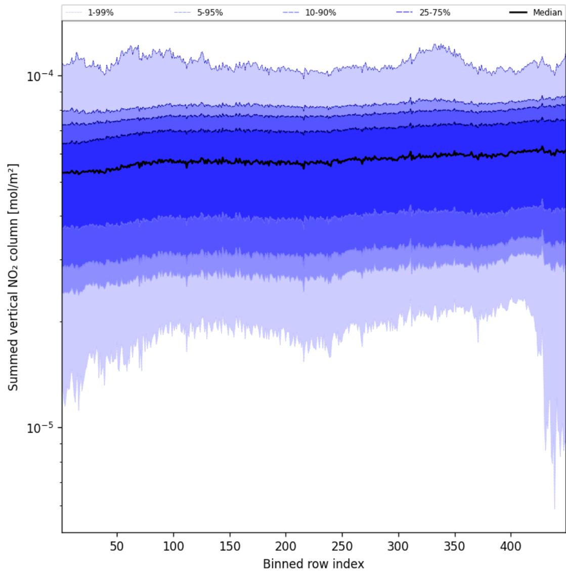
Figure 55: Along track statistics of “Summed vertical NO 2 column” for 2025-05-06 to 2025-05-07
