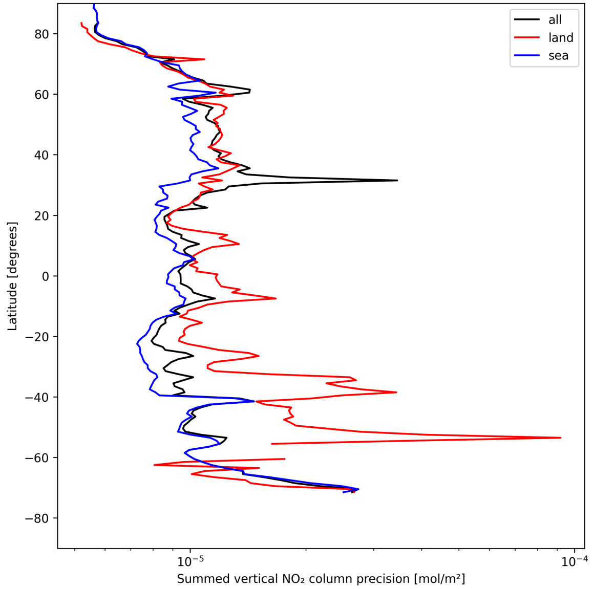
Figure 22: Zonal average of “Summed vertical NO 2 column precision” for 2025-05-06 to 2025-05-07.
