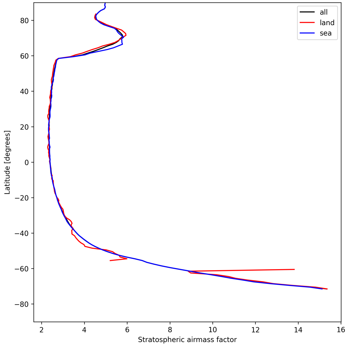
Figure 25: Zonal average of “Stratospheric airmass factor” for 2025-05-06 to 2025-05-07.
