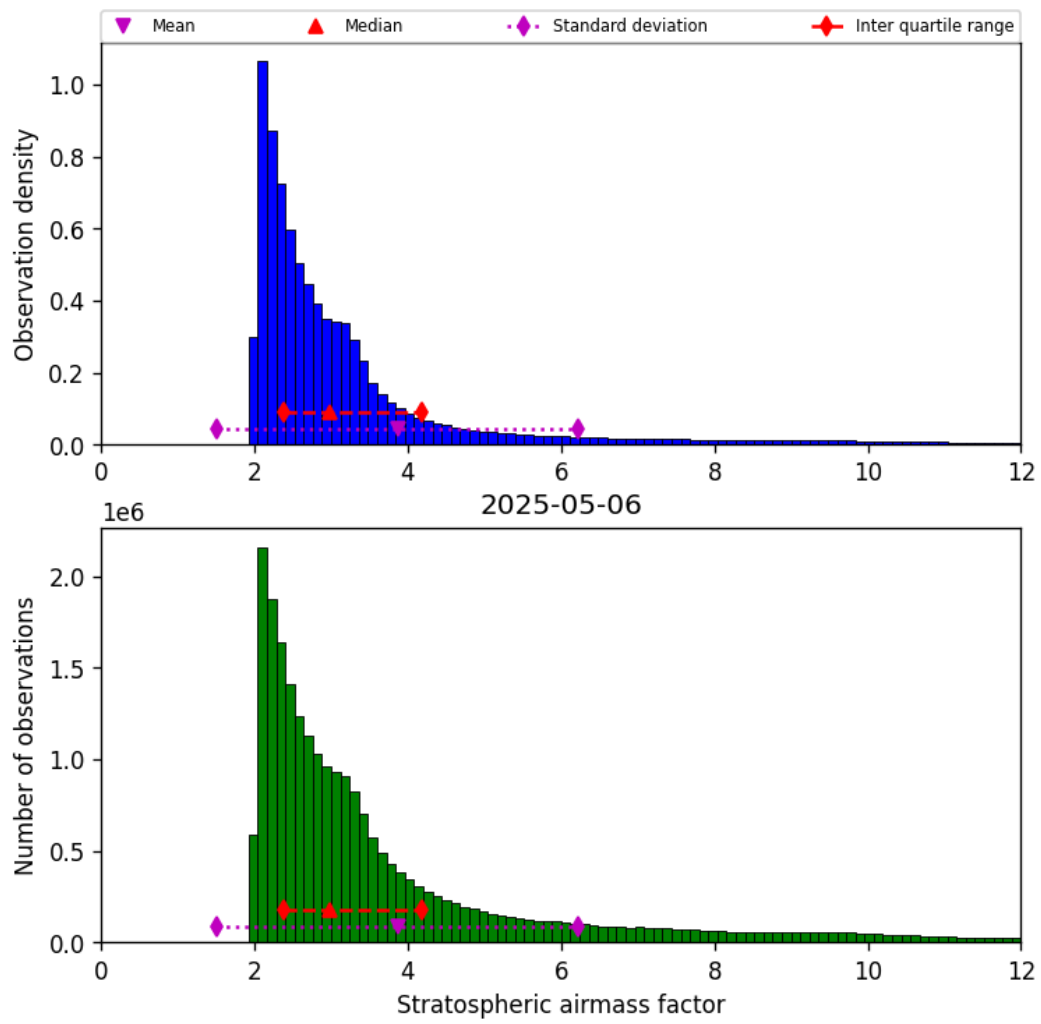
Figure 42: Histogram of “Stratospheric airmass factor” for 2025-05-06 to 2025-05-07
