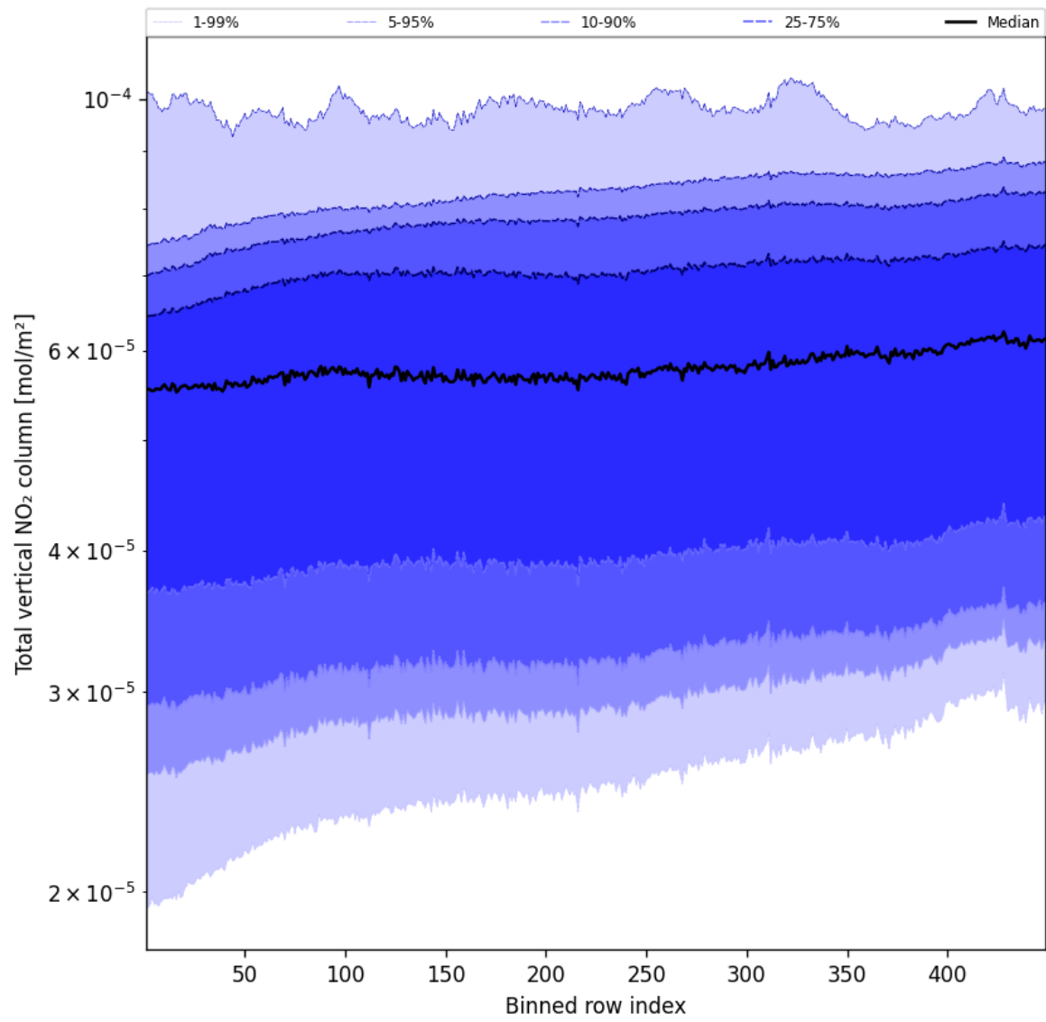
Figure 53: Along track statistics of “Total vertical NO 2 column” for 2025-05-06 to 2025-05-07
