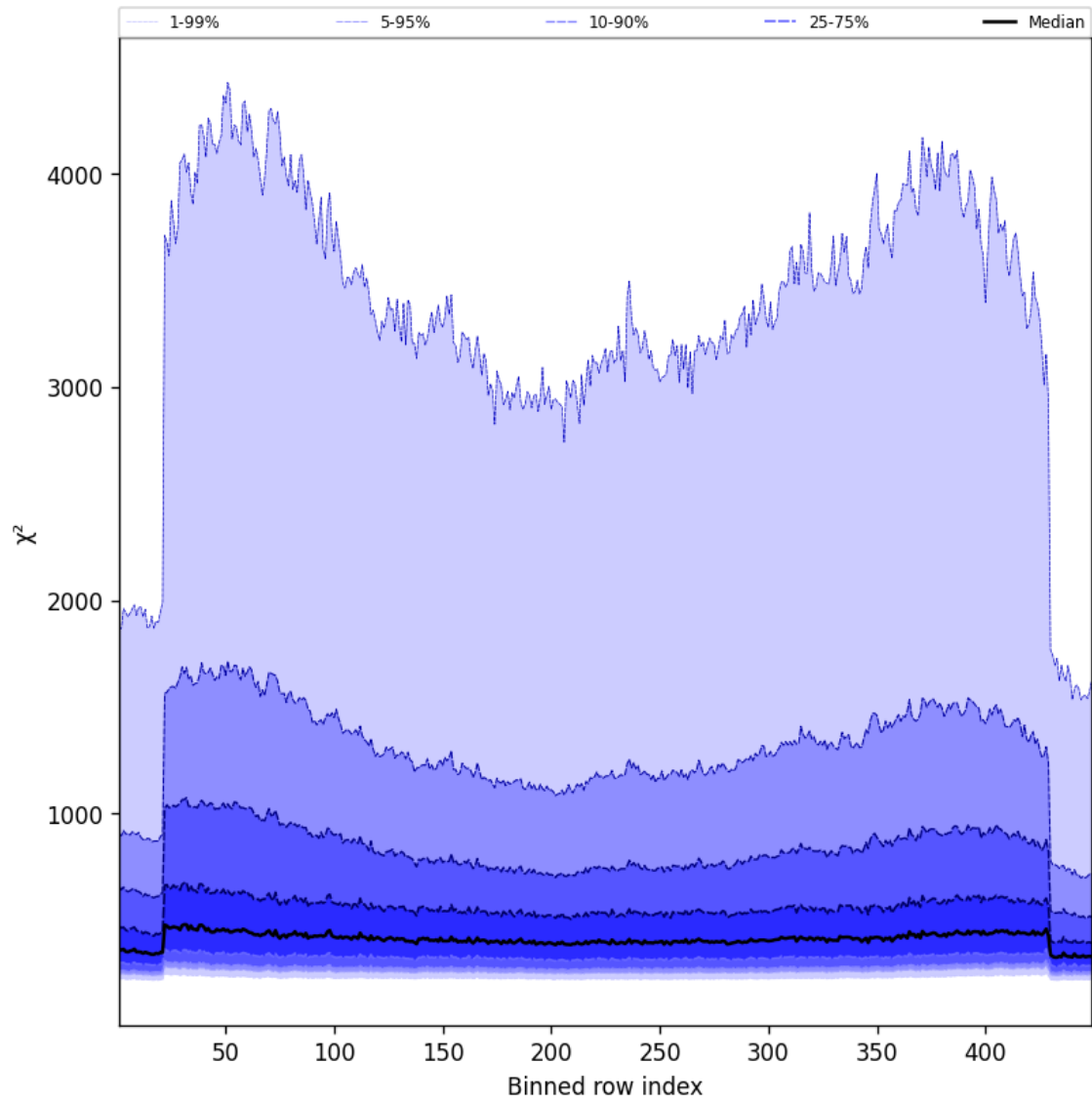
Figure 57: Along track statistics of “ \chi^2 ” for 2025-05-06 to 2025-05-07
