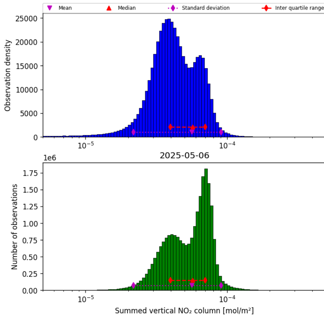
Figure 38: Histogram of “Summed vertical NO 2 column” for 2025-05-06 to 2025-05-07
