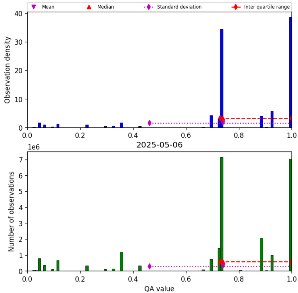
Figure 26: Histogram of “QA value” for 2025-05-06 to 2025-05-07
