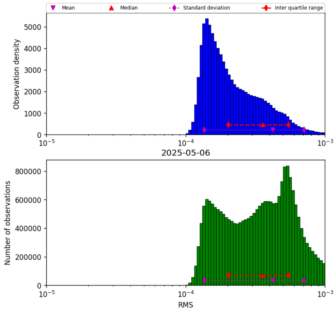
Figure 41: Histogram of “RMS” for 2025-05-06 to 2025-05-07
