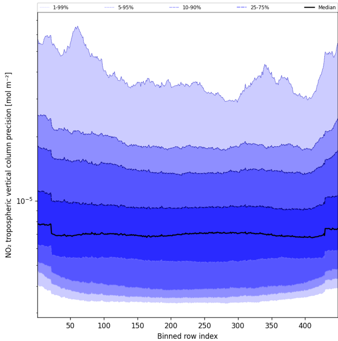
Figure 45: Along track statistics of “NO 2 tropospheric vertical column precision” for 2025-05-06 to 2025-05-07
