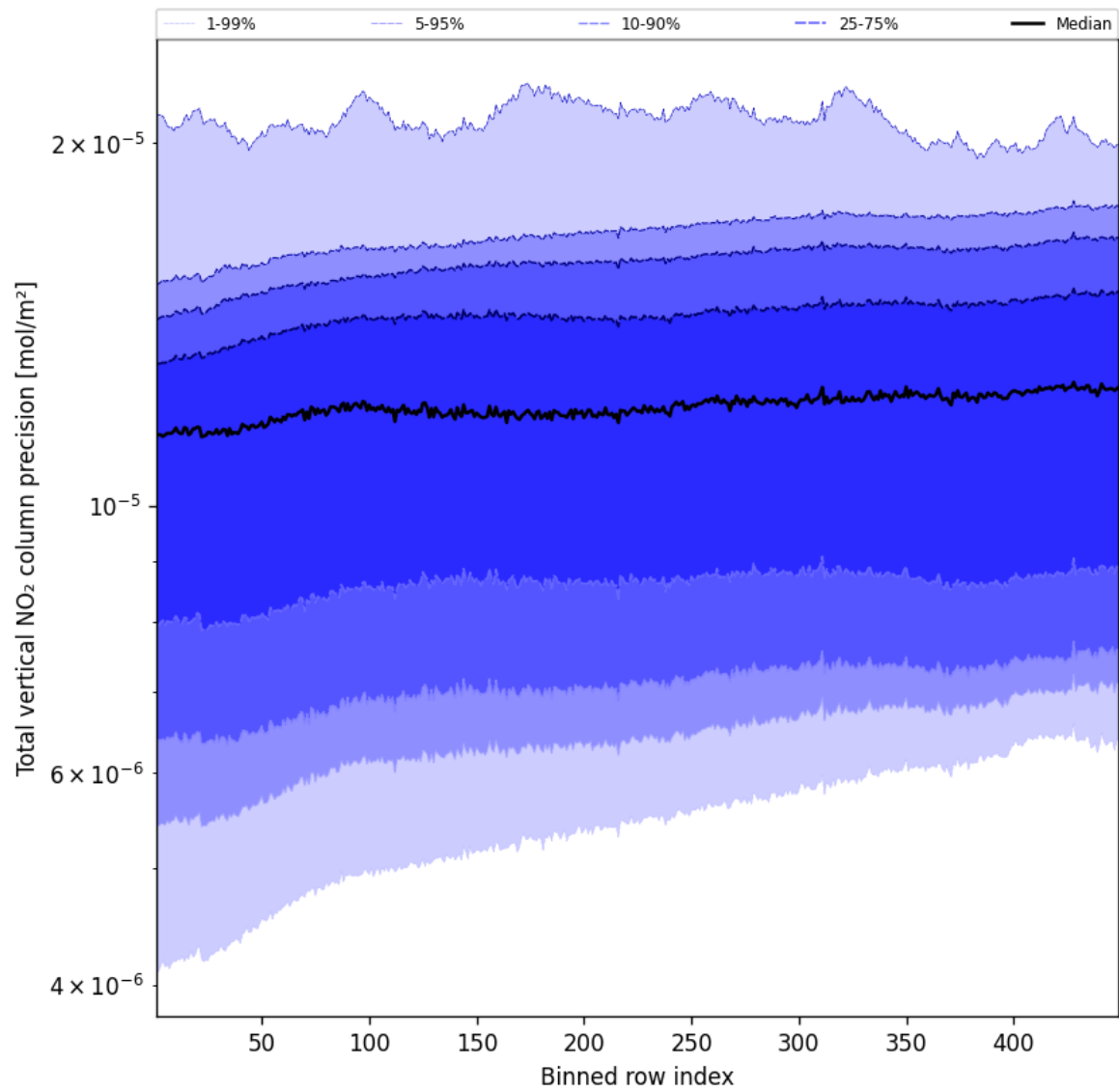
Figure 54: Along track statistics of “Total vertical NO 2 column precision” for 2025-05-06 to 2025-05-07
