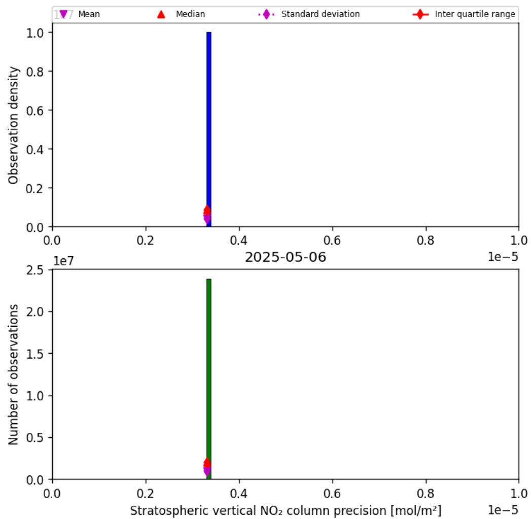
Figure 35: Histogram of “Stratospheric vertical NO 2 column precision” for 2025-05-06 to 2025-05-07
