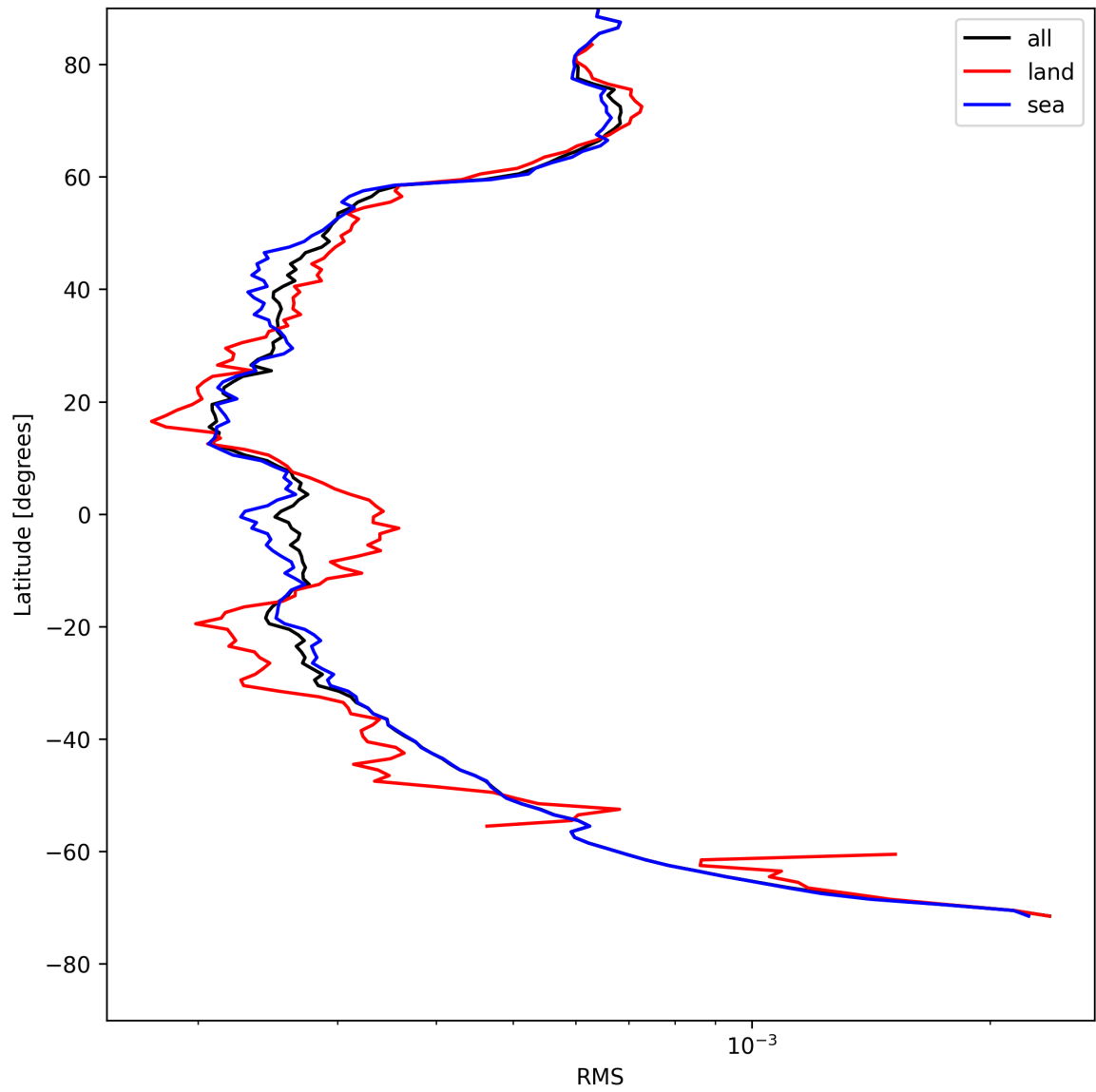
Figure 24: Zonal average of “RMS” for 2025-05-06 to 2025-05-07.
