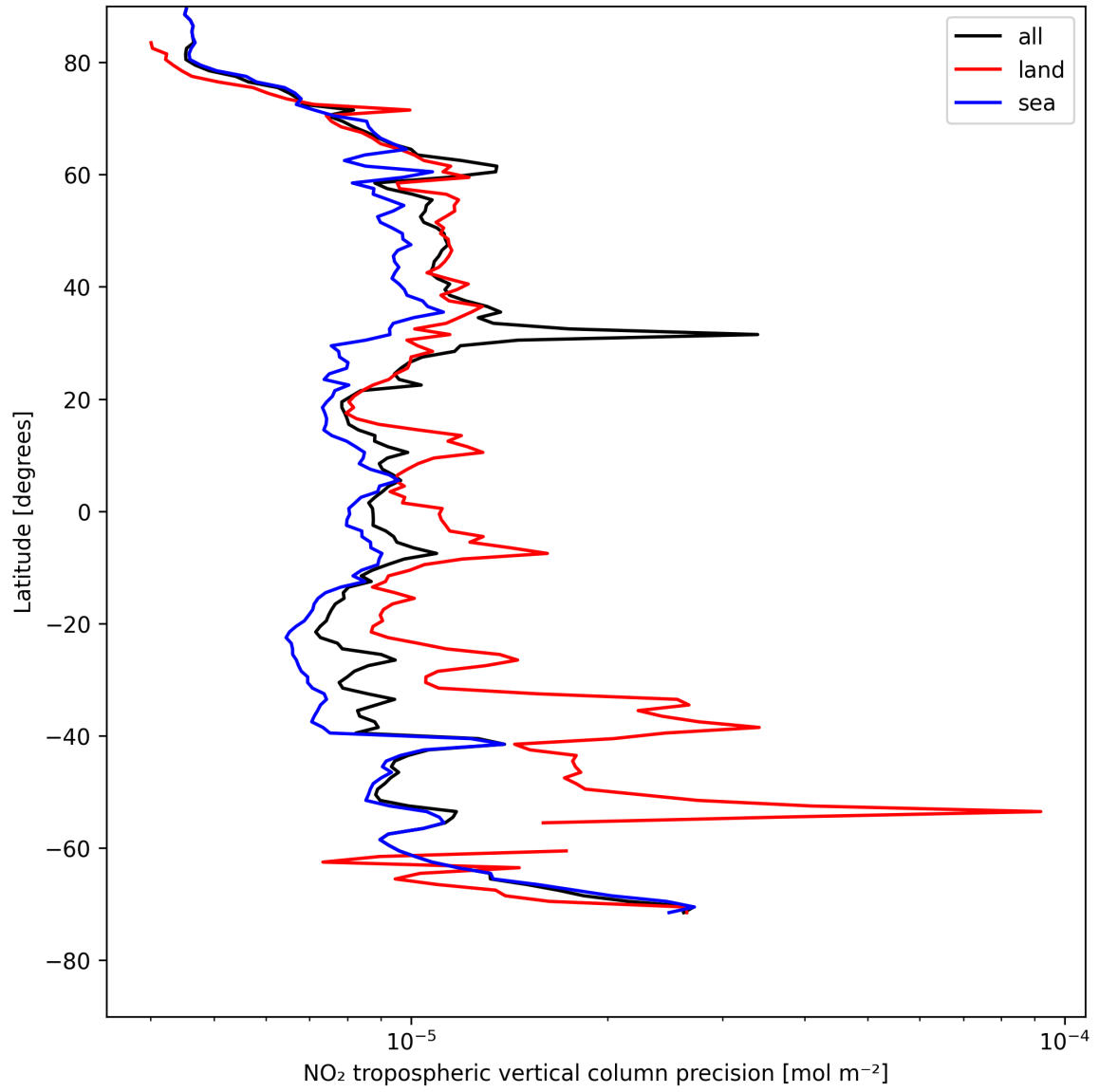
Figure 11: Zonal average of “NO 2 tropospheric vertical column precision” for 2025-05-06 to 2025-05-07.
