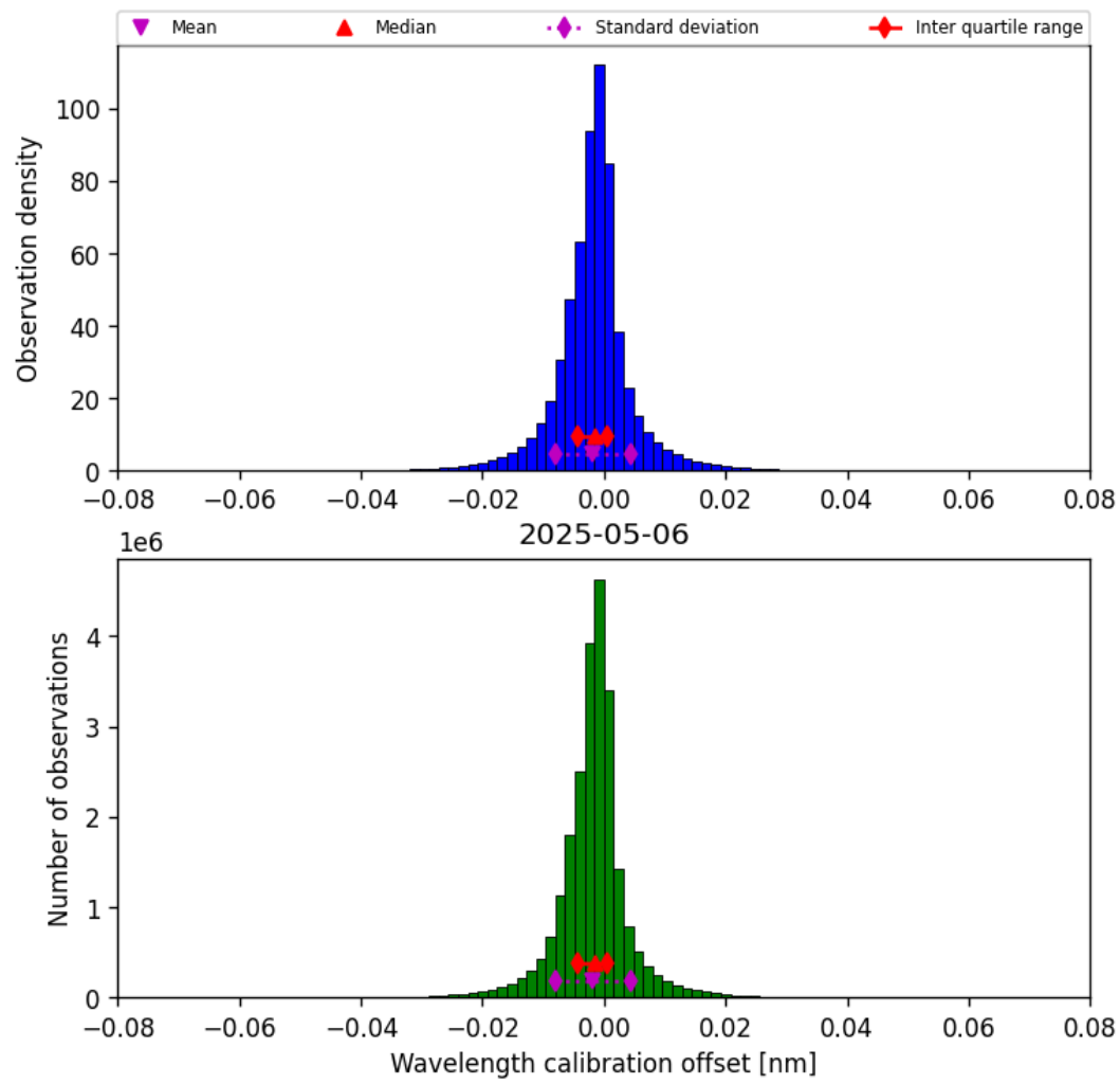
Figure 33: Histogram of “Wavelength calibration offset” for 2025-05-06 to 2025-05-07
