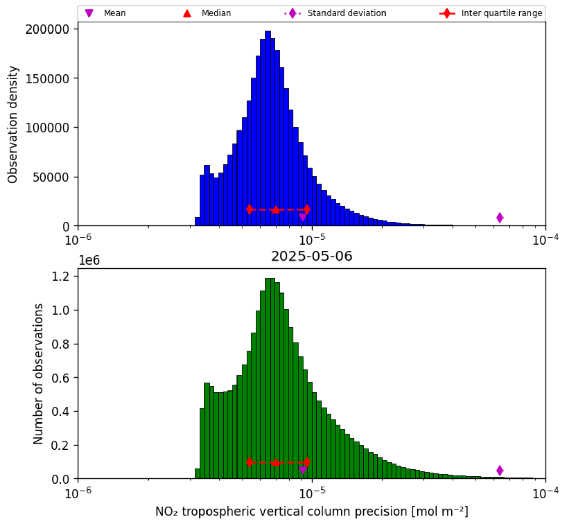
Figure 28: Histogram of “NO 2 tropospheric vertical column precision” for 2025-05-06 to 2025-05-07
