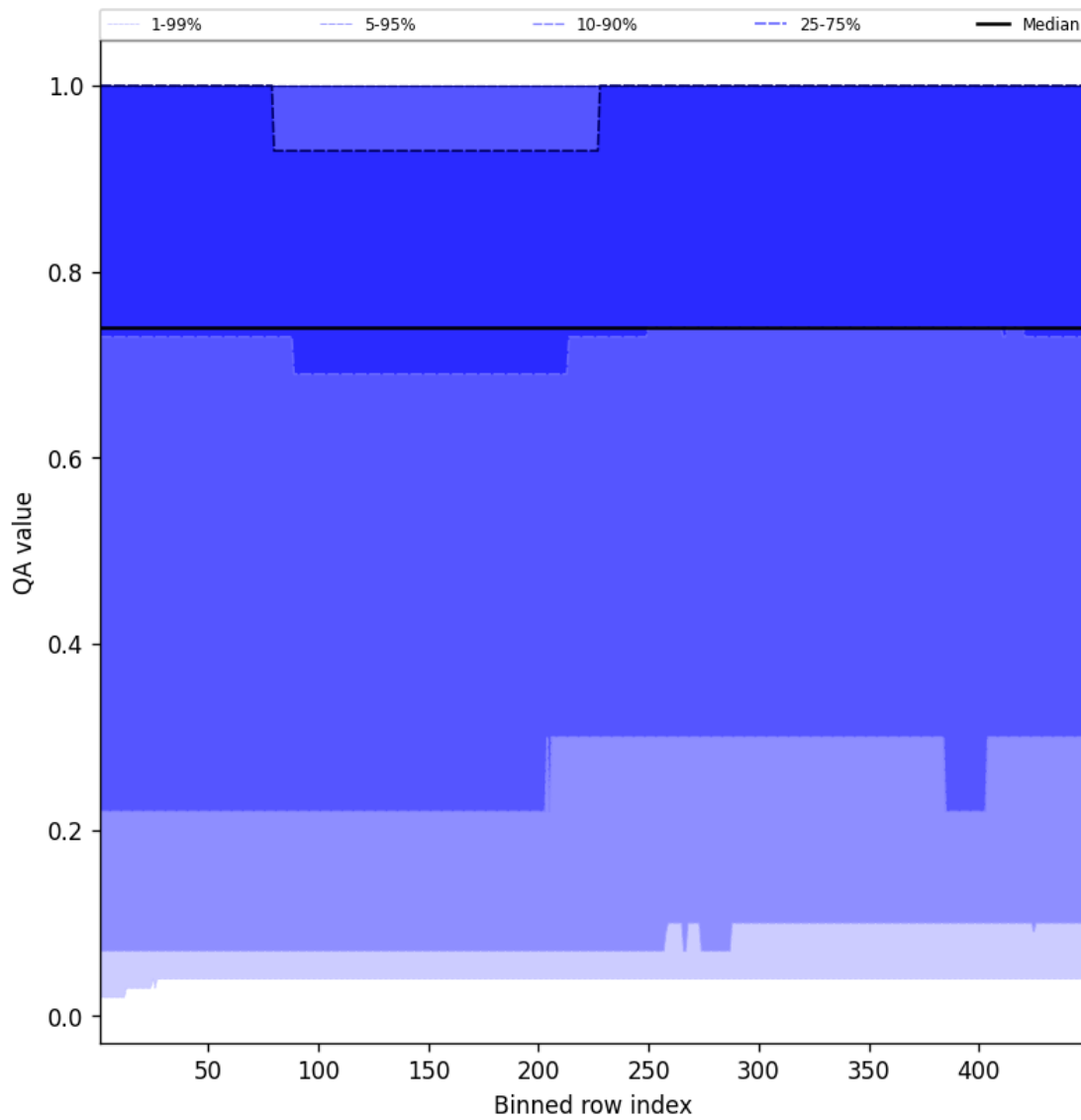
Figure 43: Along track statistics of “QA value” for 2025-05-06 to 2025-05-07
