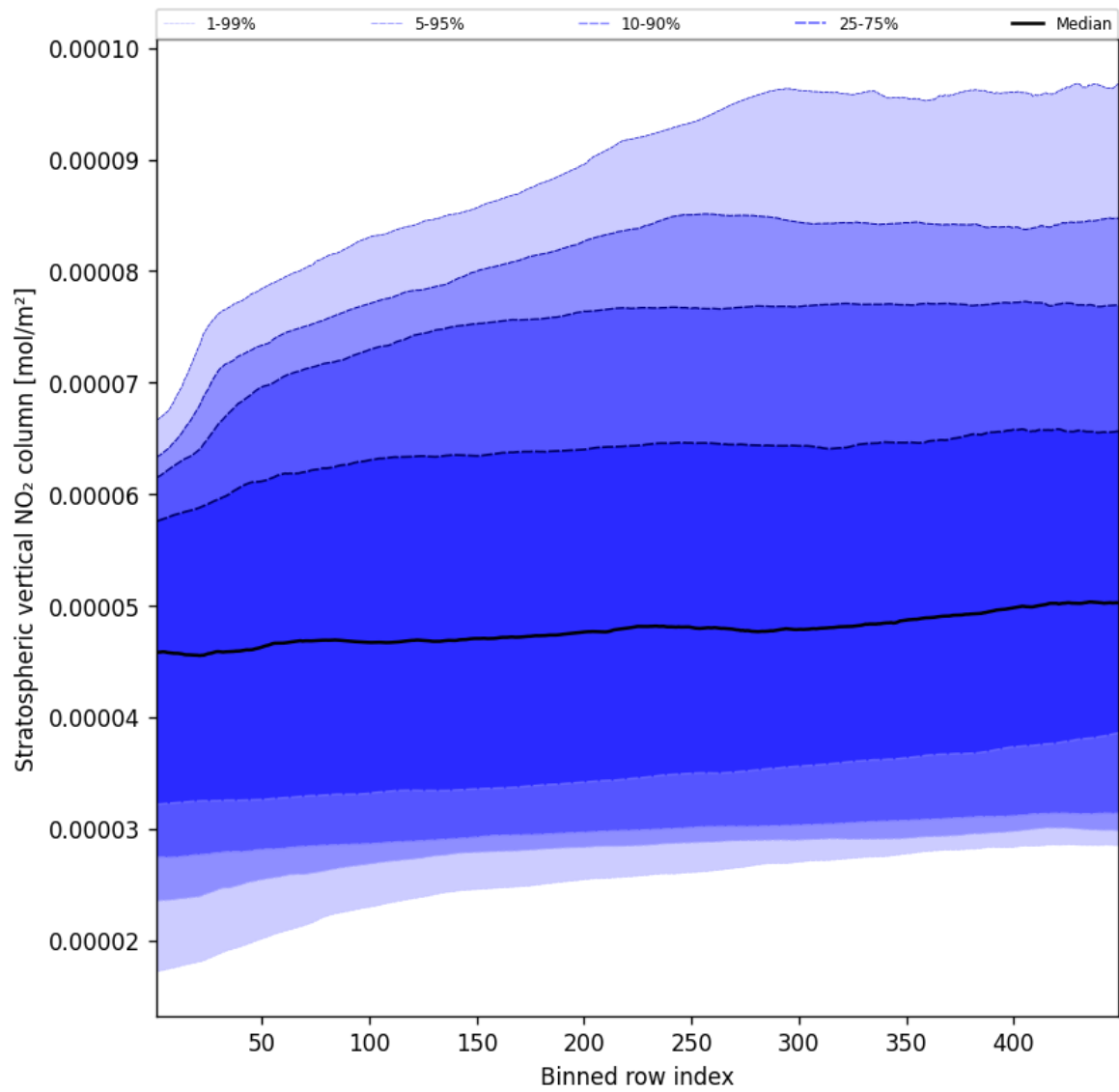
Figure 51: Along track statistics of “Stratospheric vertical NO 2 column” for 2025-05-06 to 2025-05-07
