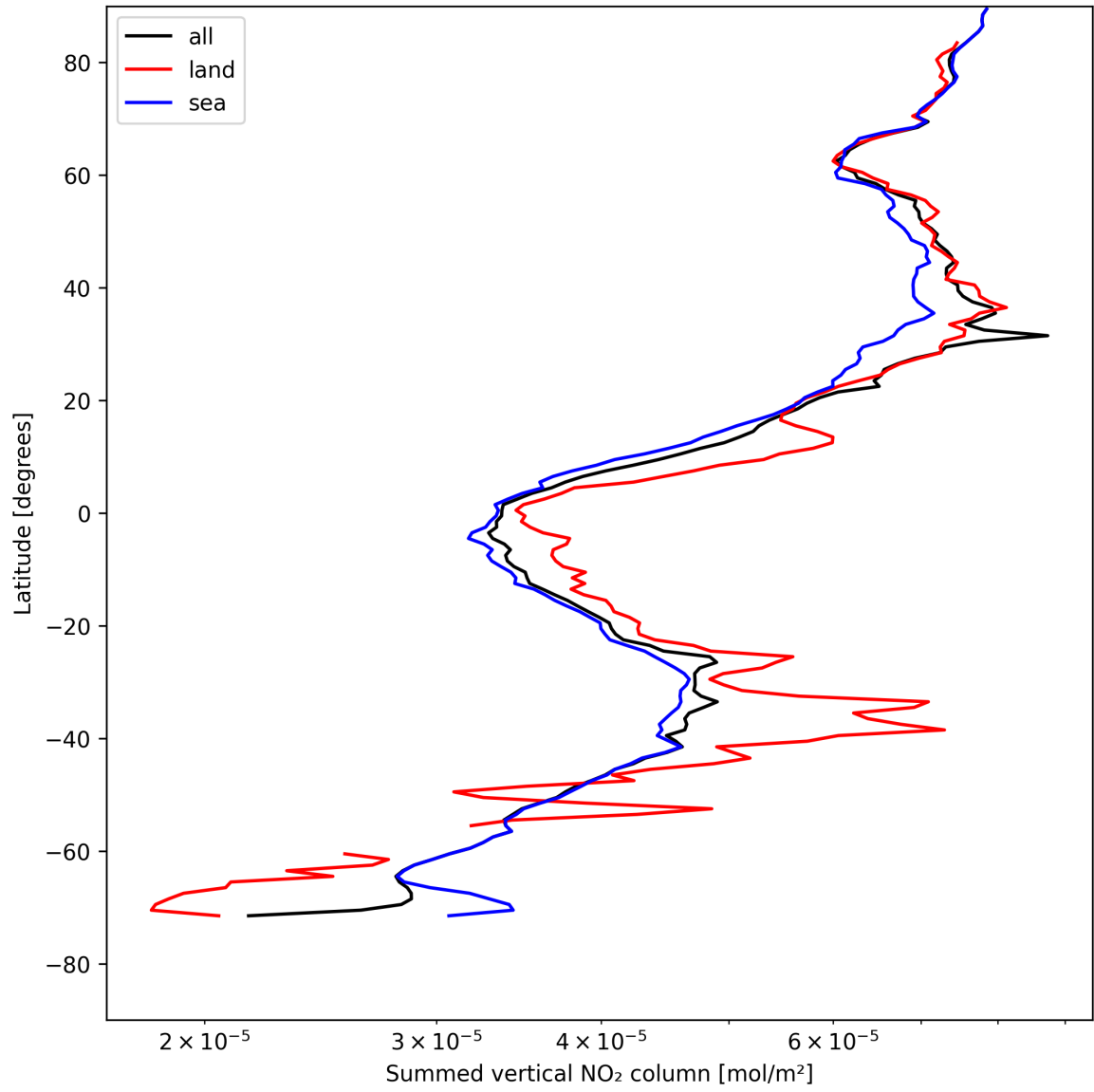
Figure 21: Zonal average of “Summed vertical NO 2 column” for 2025-05-06 to 2025-05-07.
