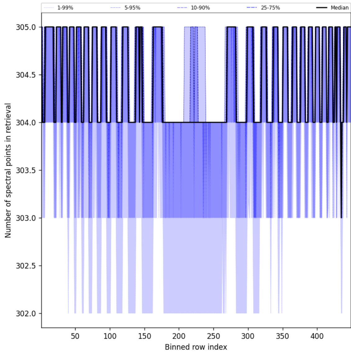
Figure 48: Along track statistics of “Number of spectral points in retrieval” for 2025-05-06 to 2025-05-07
