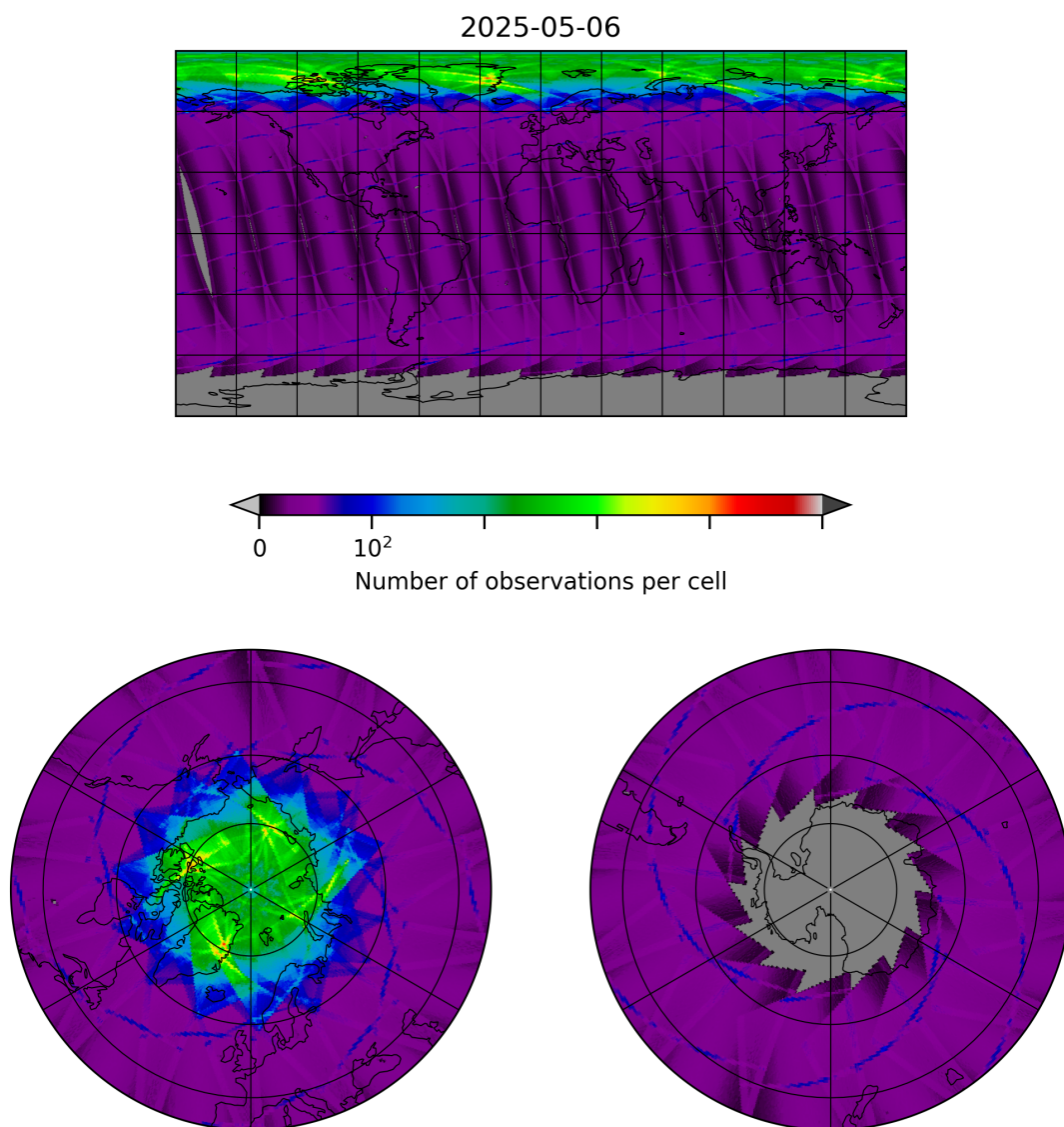
Figure 8: Map of the number of observations for 2025-05-06 to 2025-05-07
