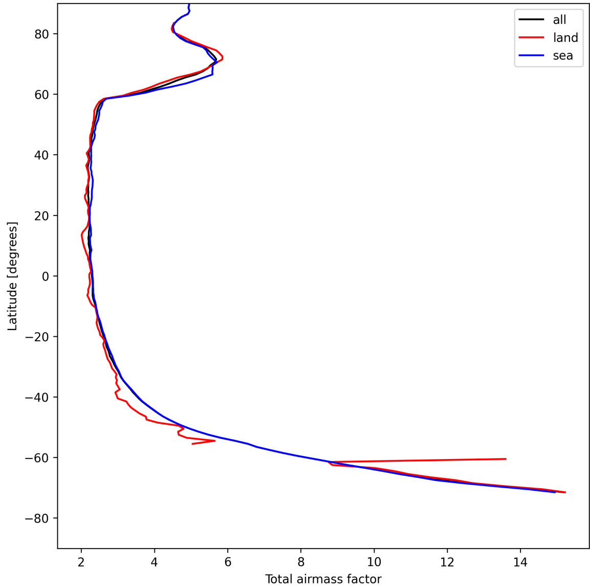
Figure 13: Zonal average of “Total airmass factor” for 2025-05-06 to 2025-05-07.
