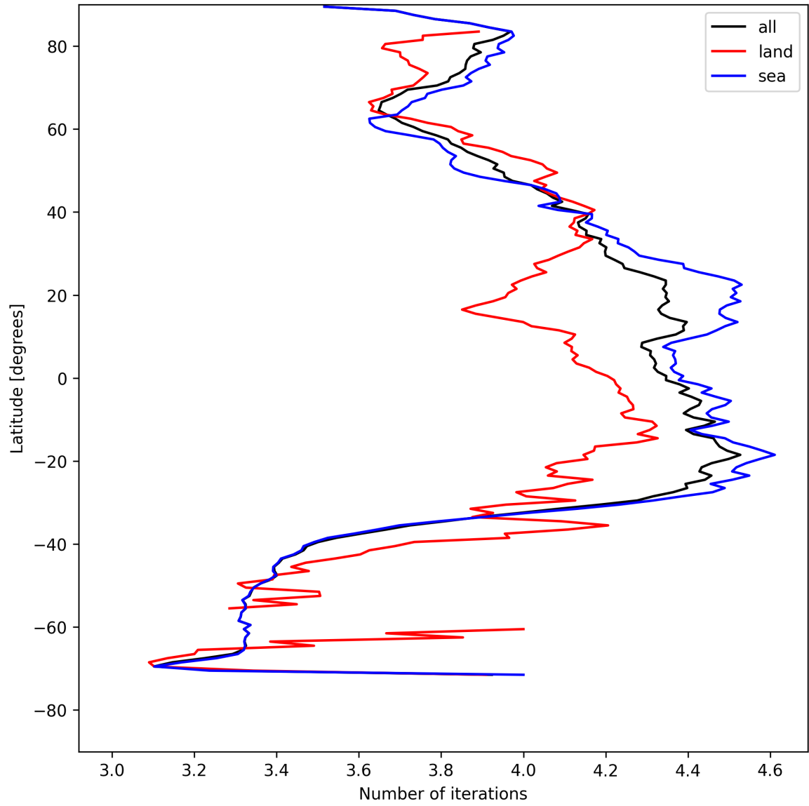
Figure 15: Zonal average of “Number of iterations” for 2025-05-06 to 2025-05-07.
