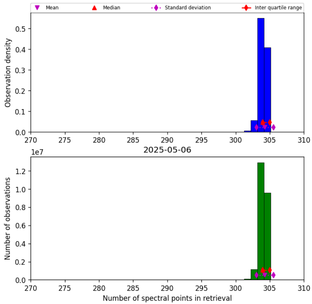
Figure 31: Histogram of “Number of spectral points in retrieval” for 2025-05-06 to 2025-05-07
