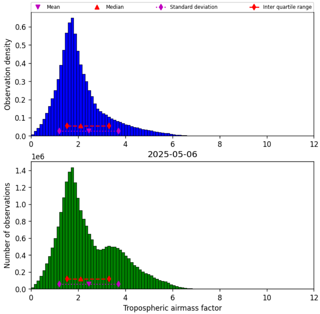
Figure 29: Histogram of “Tropospheric airmass factor” for 2025-05-06 to 2025-05-07
