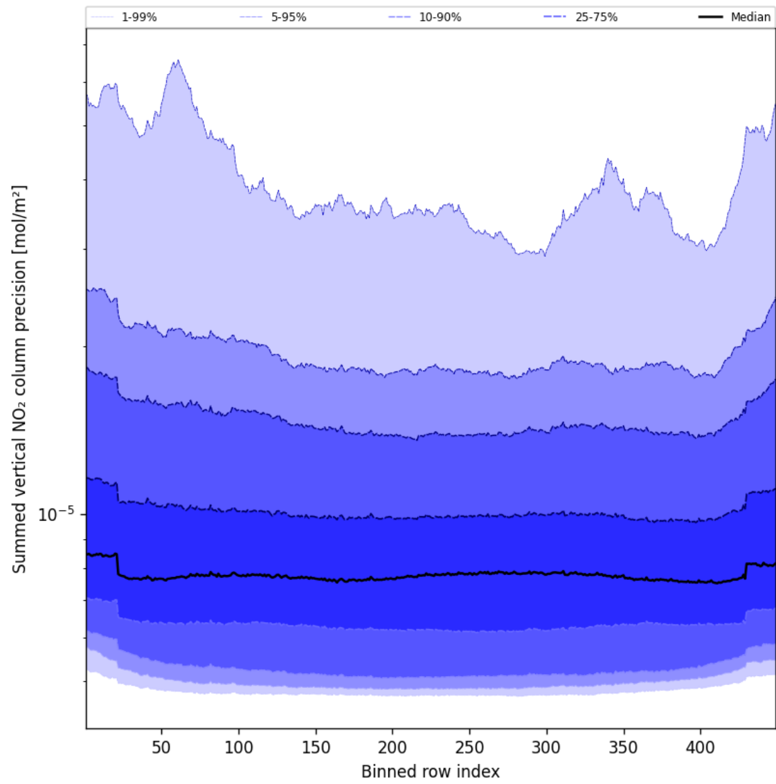
Figure 56: Along track statistics of “Summed vertical NO 2 column precision” for 2025-05-06 to 2025-05-07
