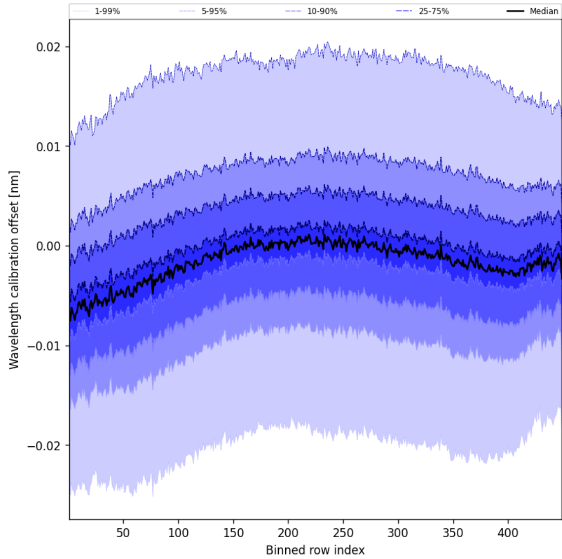
Figure 50: Along track statistics of “Wavelength calibration offset” for 2025-05-06 to 2025-05-07
