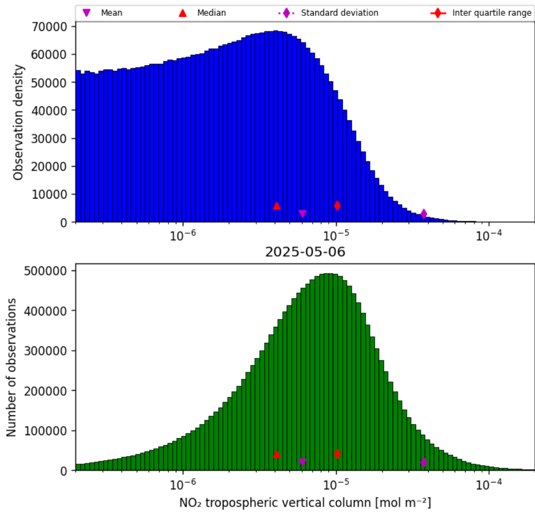
Figure 27: Histogram of “NO 2 tropospheric vertical column” for 2025-05-06 to 2025-05-07
