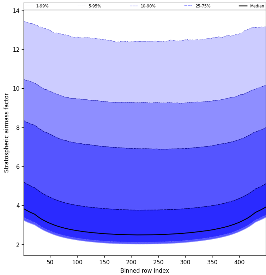
Figure 59: Along track statistics of “Stratospheric airmass factor” for 2025-05-06 to 2025-05-07
