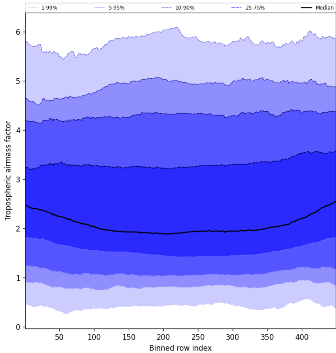
Figure 46: Along track statistics of “Tropospheric airmass factor” for 2025-05-06 to 2025-05-07
