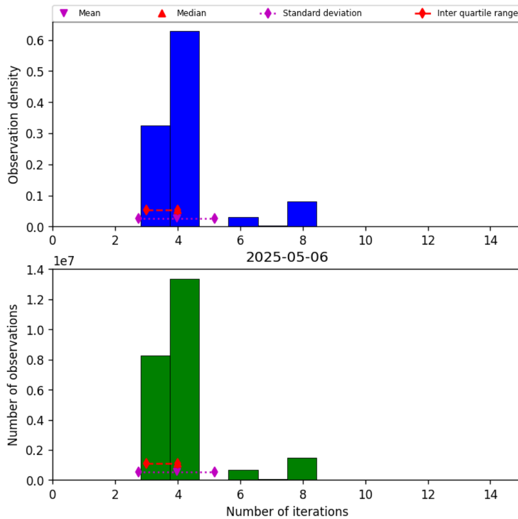
Figure 32: Histogram of “Number of iterations” for 2025-05-06 to 2025-05-07
