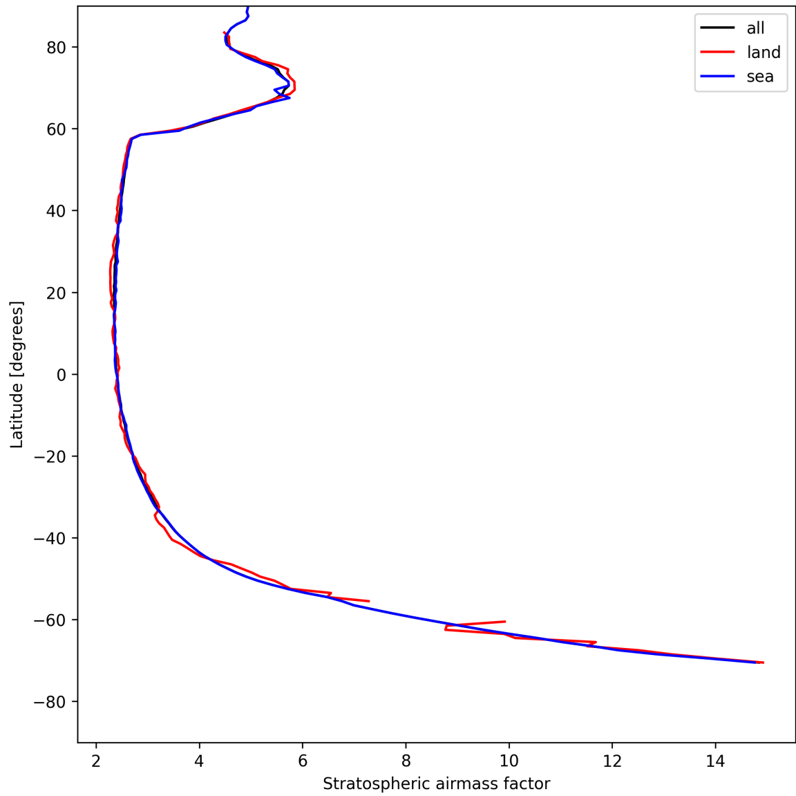
Figure 25: Zonal average of “Stratospheric air mass factor” for 2025-05-07 to 2025-05-08.
