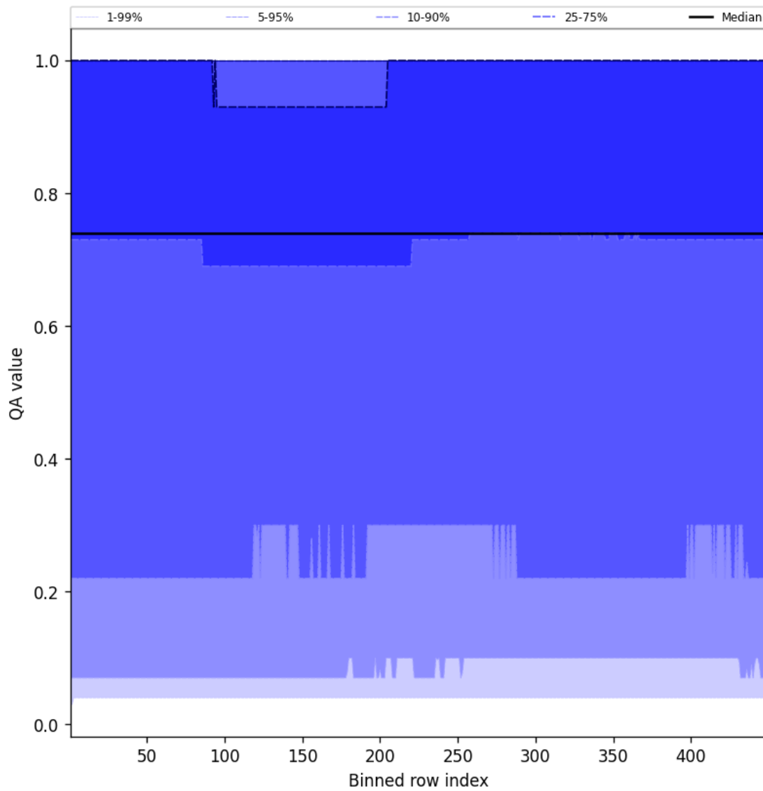
Figure 43: Along track statistics of “QA value” for 2025-05-07 to 2025-05-08
