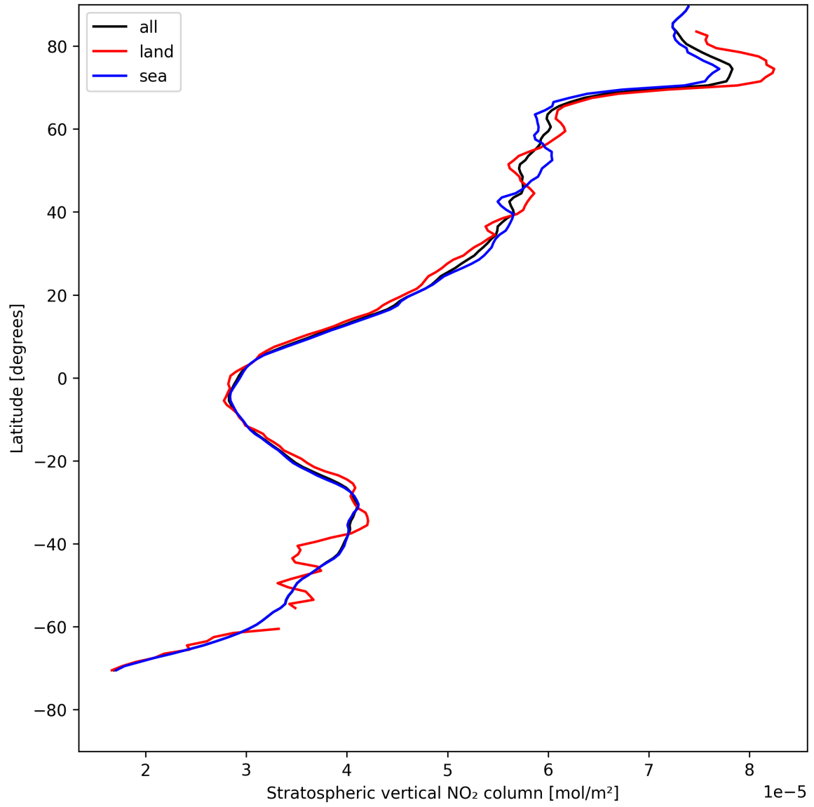
Figure 17: Zonal average of “Stratospheric vertical NO 2 column” for 2025-05-07 to 2025-05-08.
