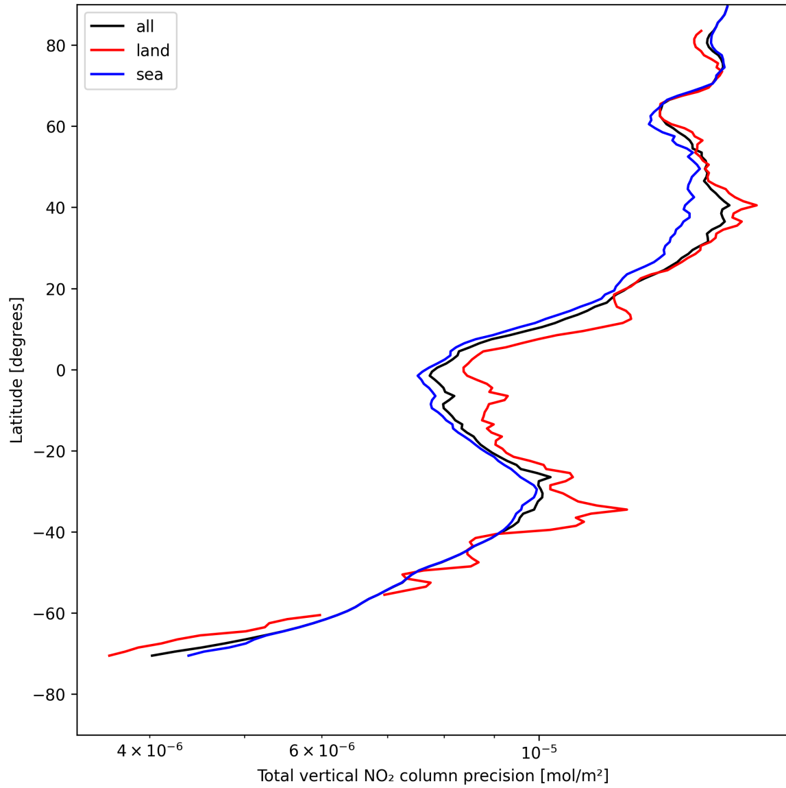
Figure 20: Zonal average of “Total vertical NO 2 column precision” for 2025-05-07 to 2025-05-08.
