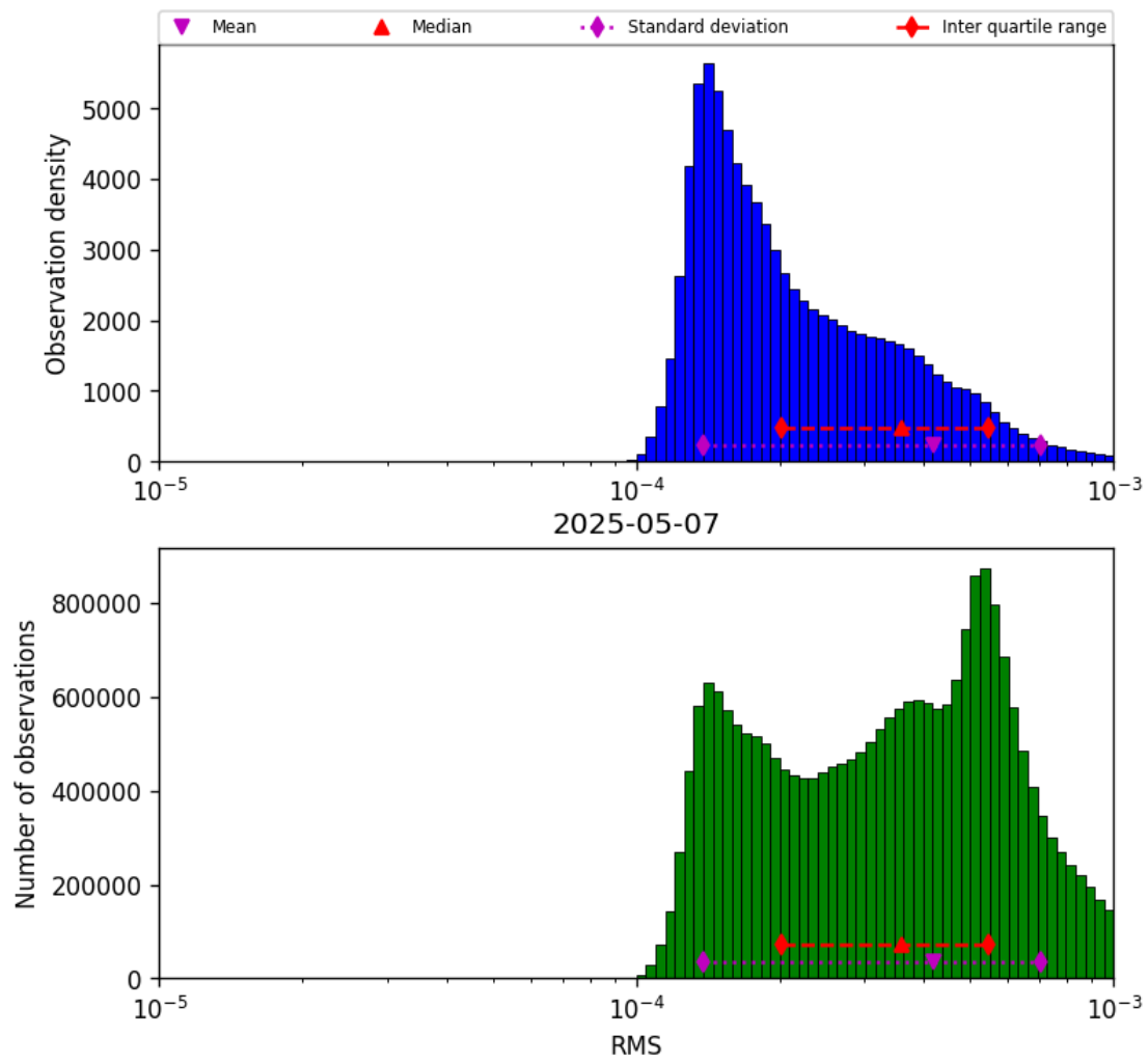
Figure 41: Histogram of “RMS” for 2025-05-07 to 2025-05-08
