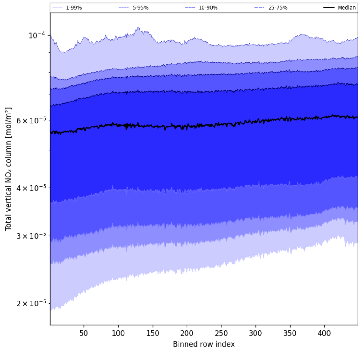
Figure 53: Along track statistics of “Total vertical NO 2 column” for 2025-05-07 to 2025-05-08
