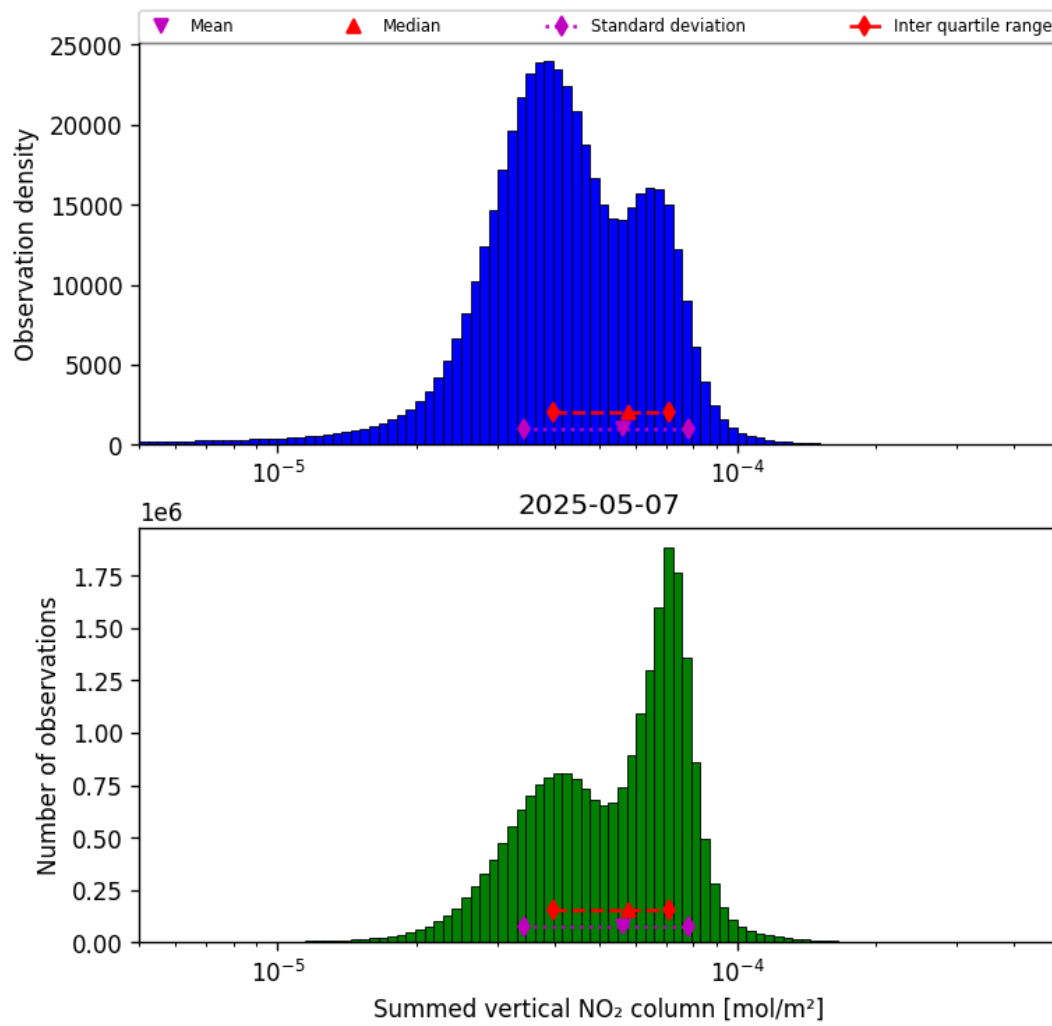
Figure 38: Histogram of “Summed vertical NO 2 column” for 2025-05-07 to 2025-05-08
