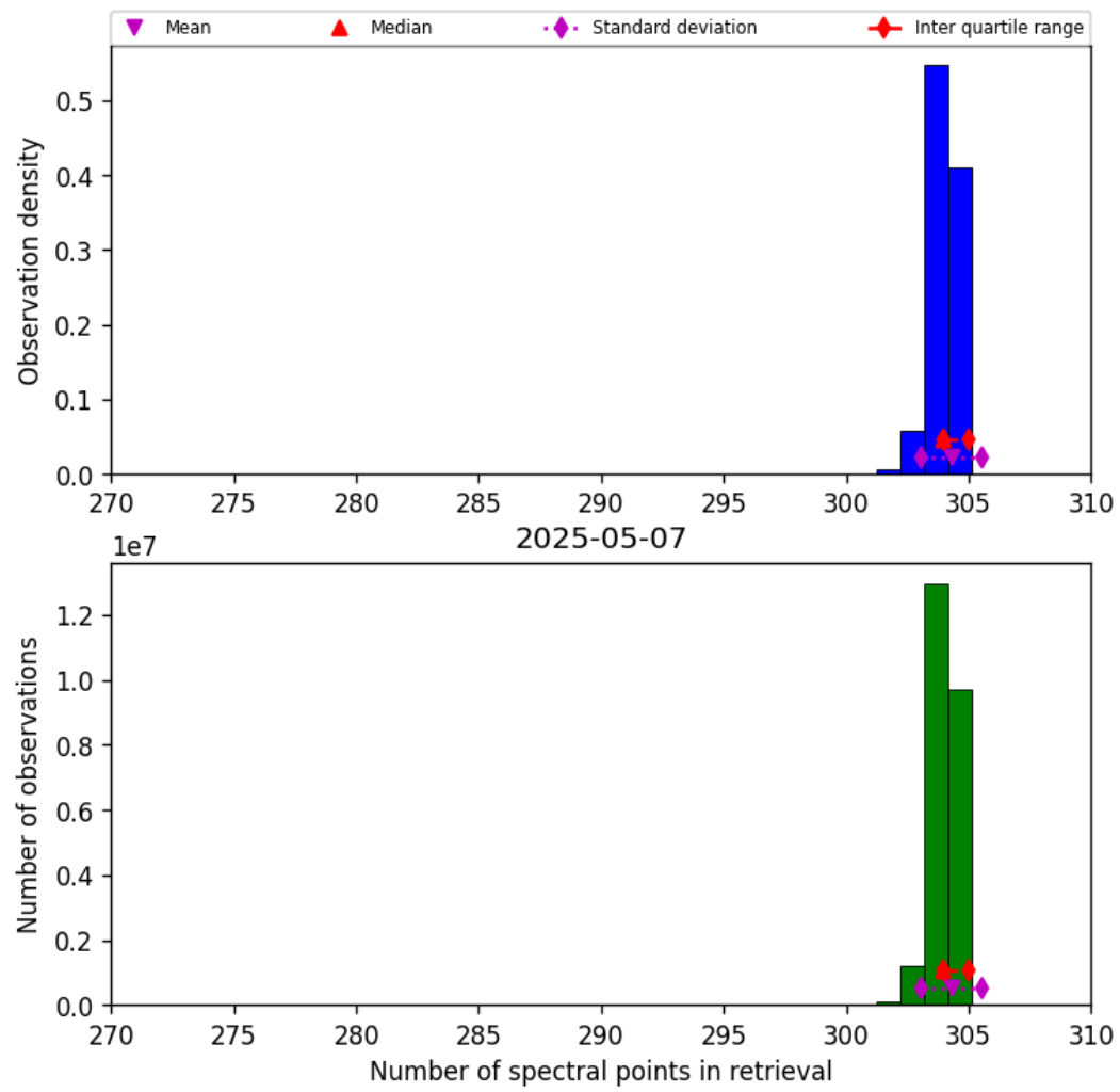
Figure 31: Histogram of “Number of spectral points in retrieval” for 2025-05-07 to 2025-05-08
