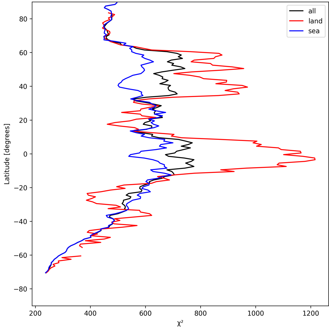
Figure 23: Zonal average of “ \chi^2 ” for 2025-05-07 to 2025-05-08.
