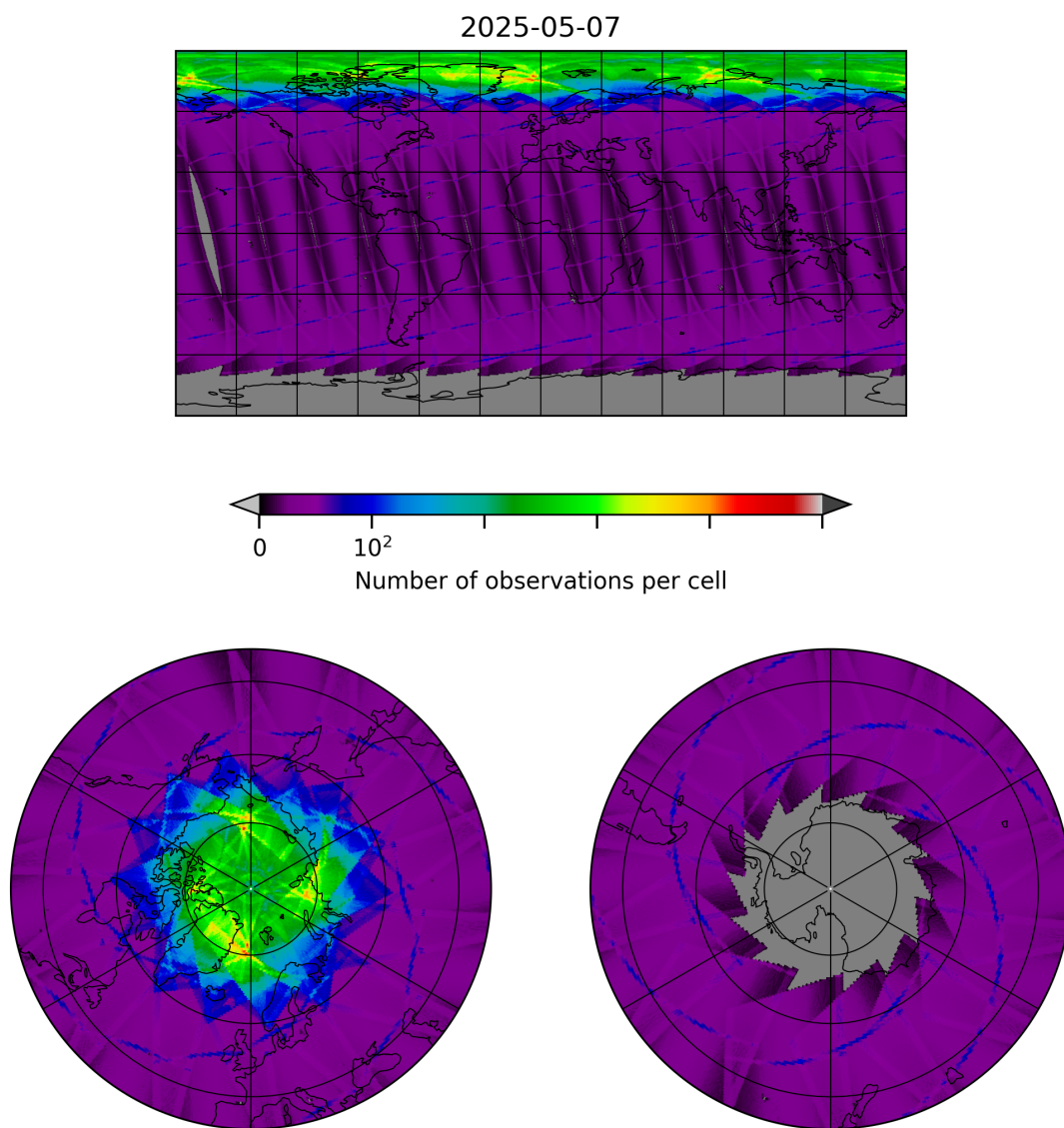
Figure 8: Map of the number of observations for 2025-05-07 to 2025-05-08
