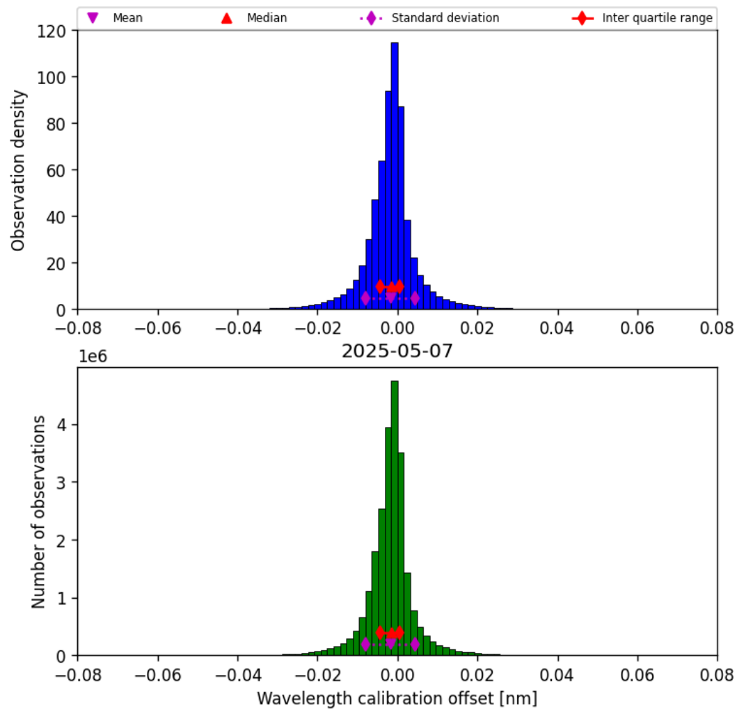
Figure 33: Histogram of “Wavelength calibration offset” for 2025-05-07 to 2025-05-08
