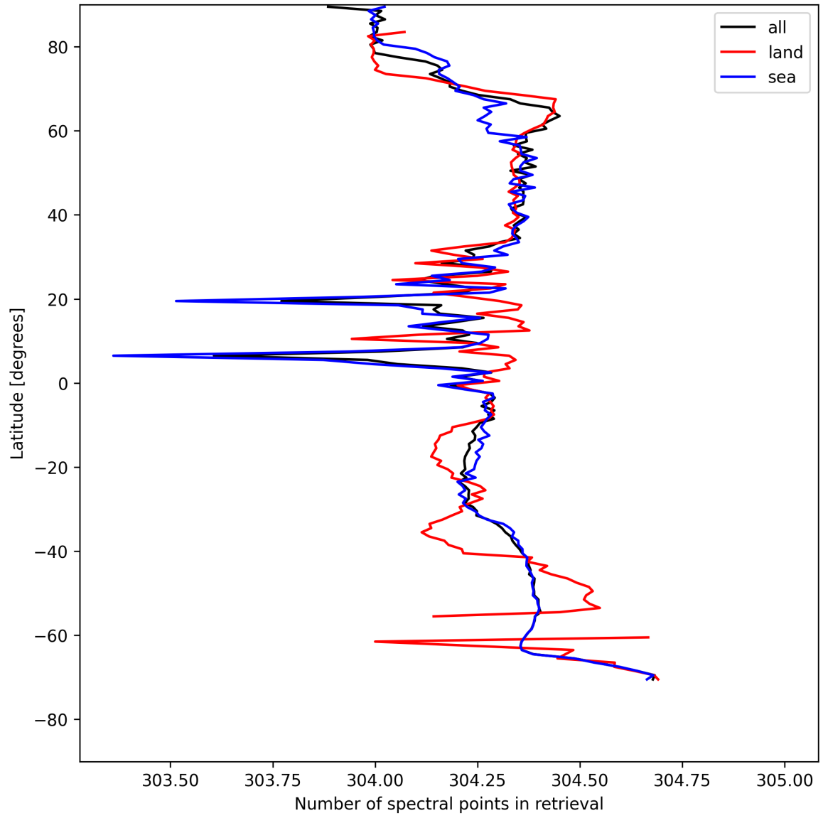
Figure 14: Zonal average of “Number of spectral points in retrieval” for 2025-05-07 to 2025-05-08.
