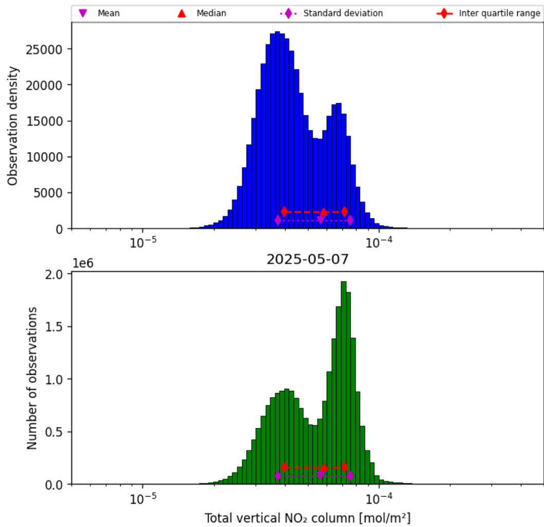
Figure 36: Histogram of “Total vertical NO 2 column” for 2025-05-07 to 2025-05-08
