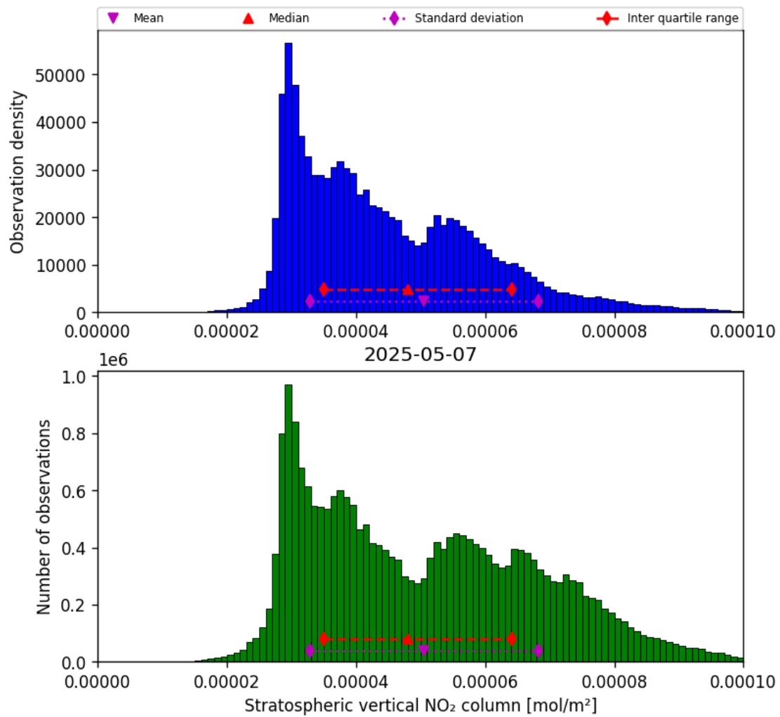
Figure 34: Histogram of “Stratospheric vertical NO 2 column” for 2025-05-07 to 2025-05-08
