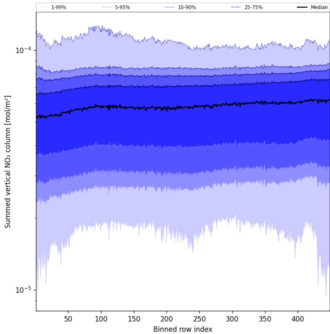
Figure 55: Along track statistics of “Summed vertical NO 2 column” for 2025-05-07 to 2025-05-08
