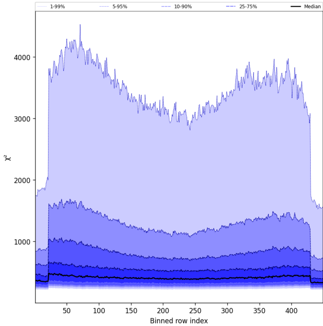
Figure 57: Along track statistics of “ \chi^2 ” for 2025-05-07 to 2025-05-08
