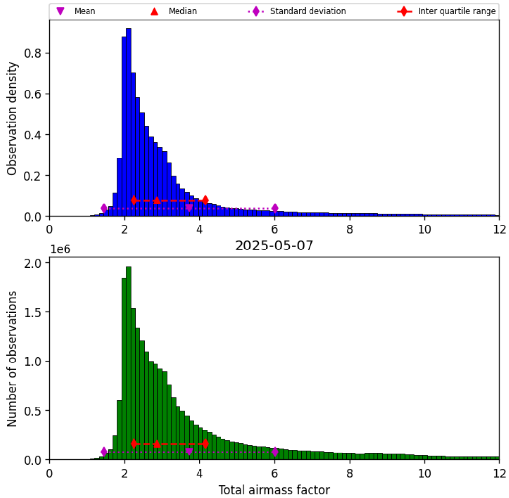
Figure 30: Histogram of “Total airmass factor” for 2025-05-07 to 2025-05-08
