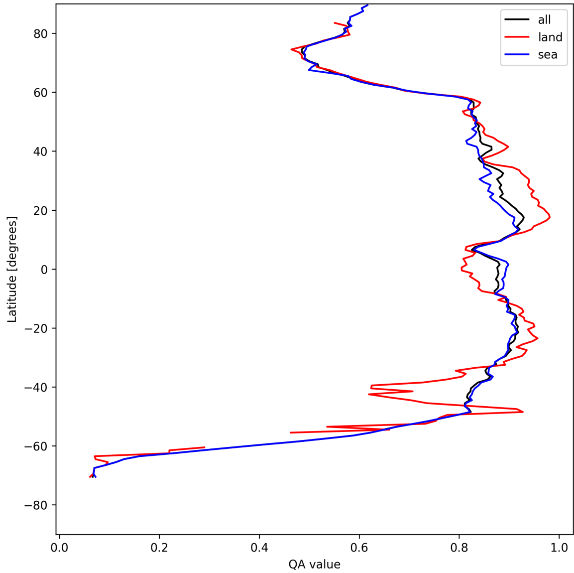
Figure 9: Zonal average of “QA value” for 2025-05-07 to 2025-05-08.
