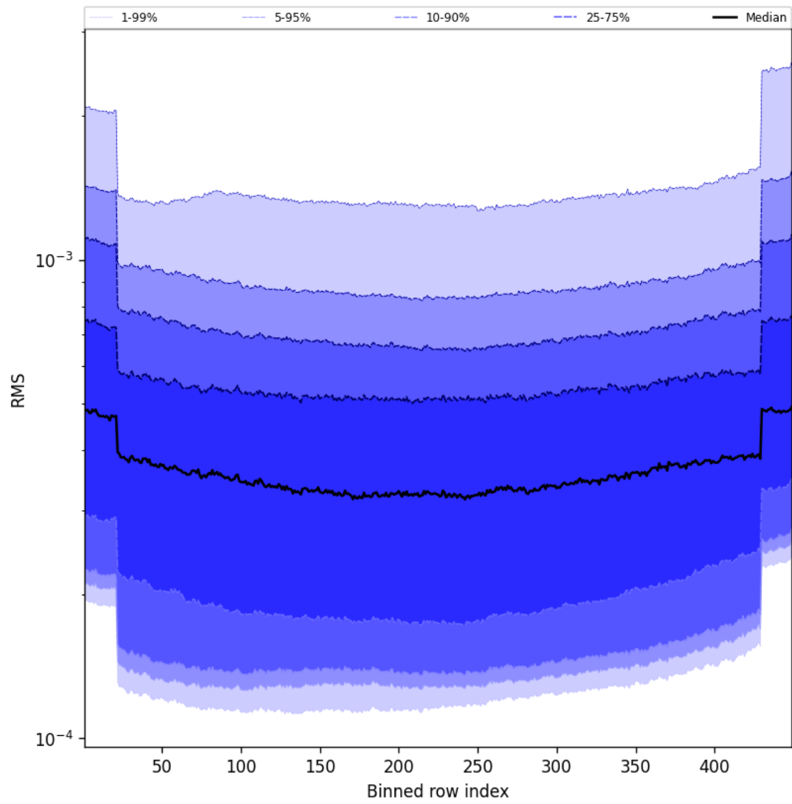
Figure 58: Along track statistics of “RMS” for 2025-05-07 to 2025-05-08
