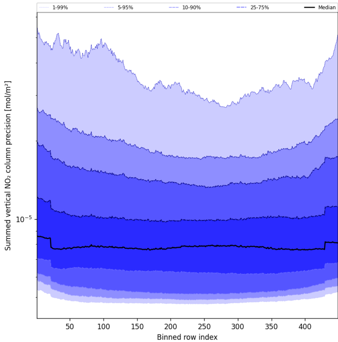
Figure 56: Along track statistics of “Summed vertical NO 2 column precision” for 2025-05-07 to 2025-05-08
