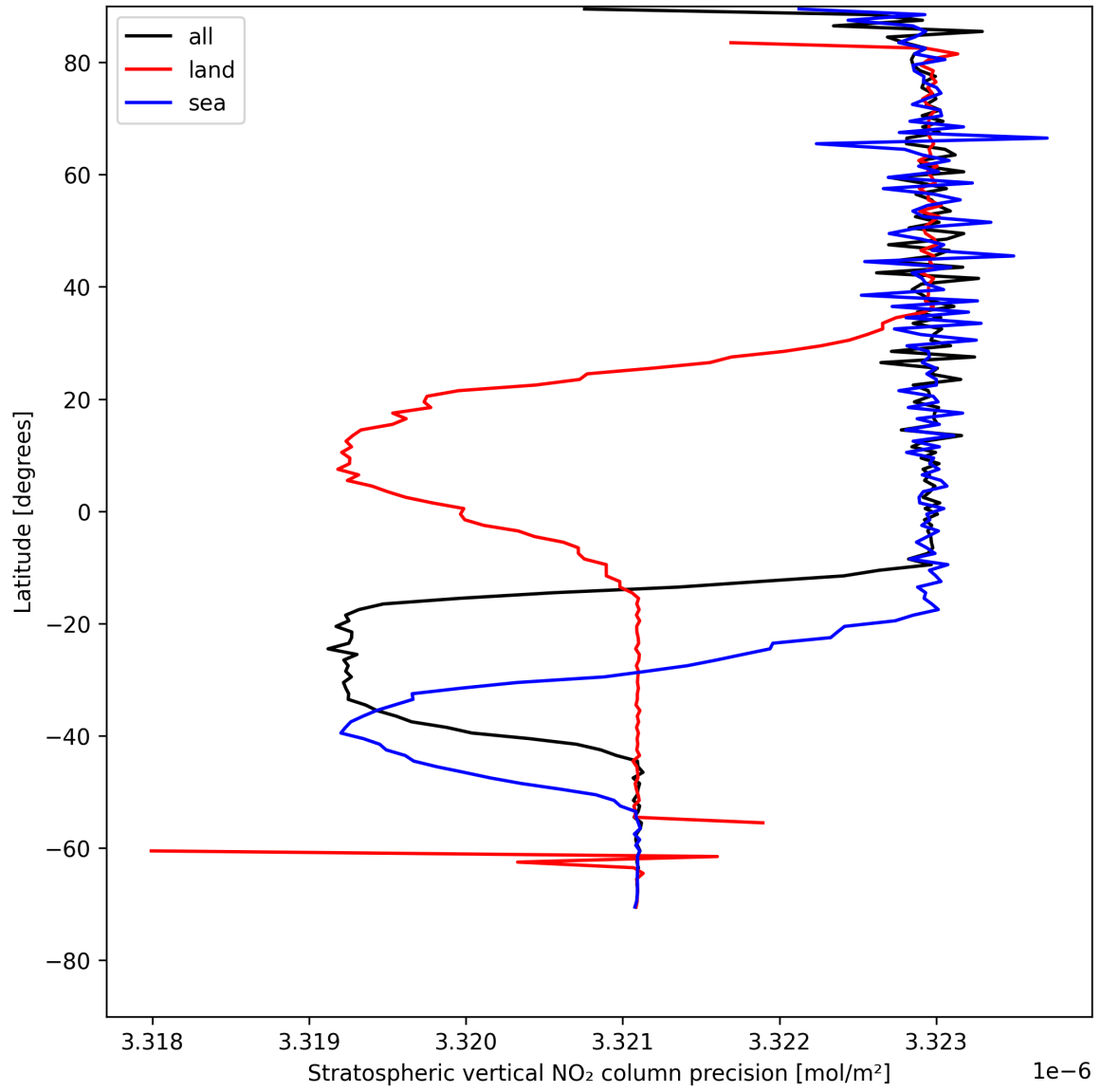
Figure 18: Zonal average of “Stratospheric vertical NO 2 column precision” for 2025-05-07 to 2025-05-08.
