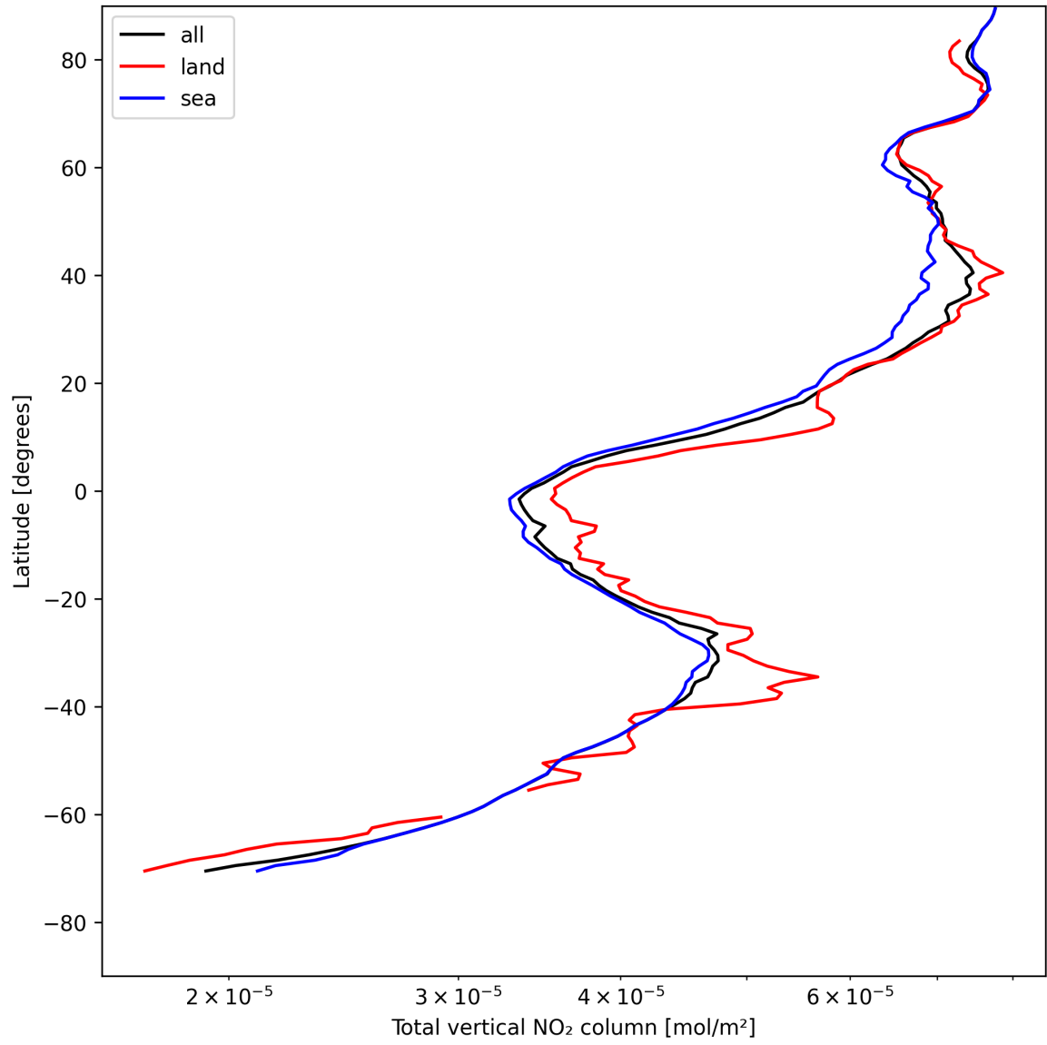
Figure 19: Zonal average of “Total vertical NO 2 column” for 2025-05-07 to 2025-05-08.
