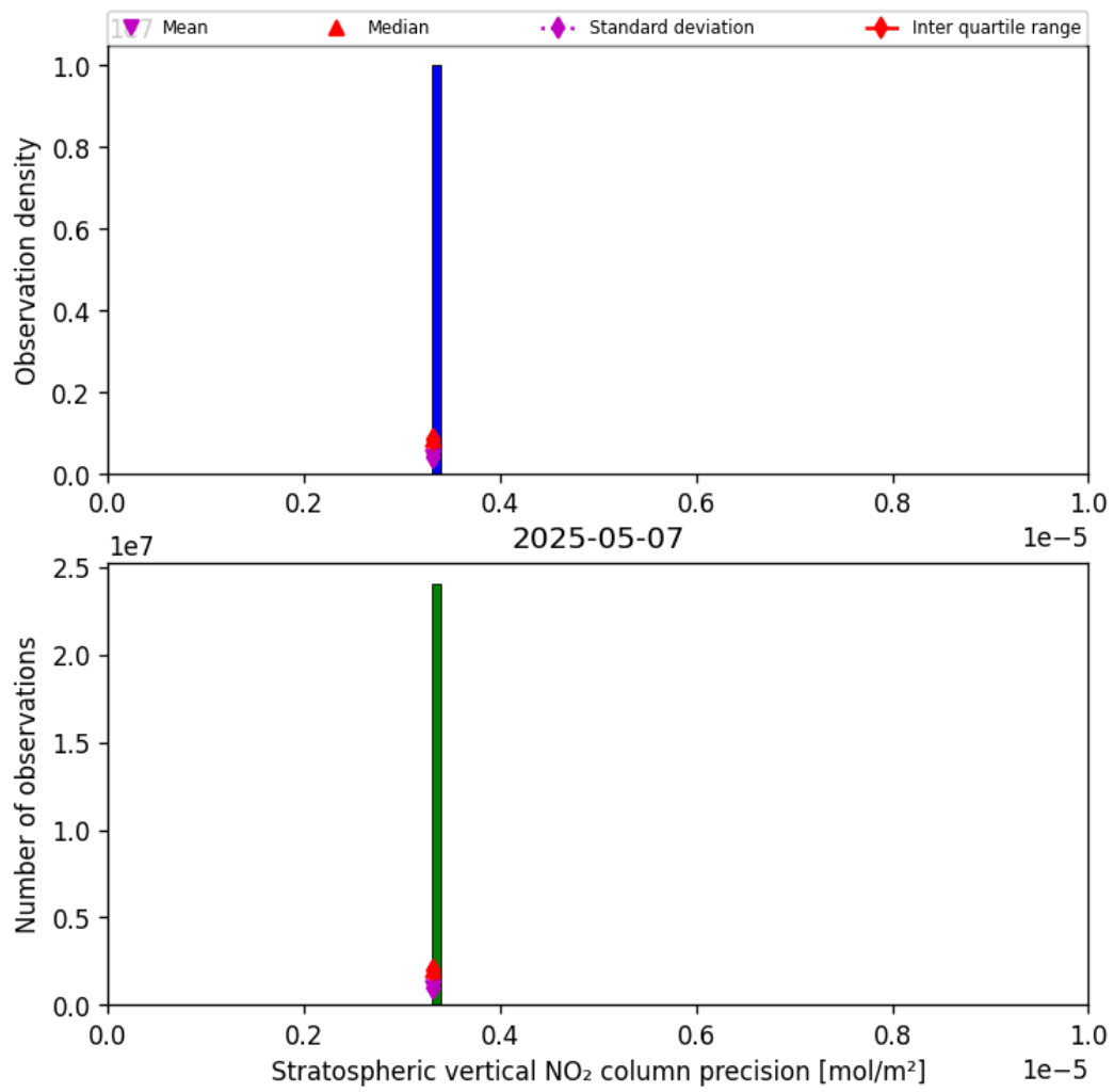
Figure 35: Histogram of “Stratospheric vertical NO 2 column precision” for 2025-05-07 to 2025-05-08
