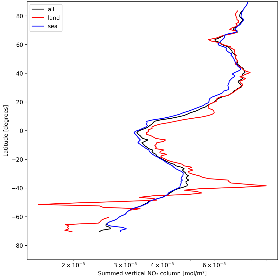
Figure 21: Zonal average of “Summed vertical NO 2 column” for 2025-05-07 to 2025-05-08.
