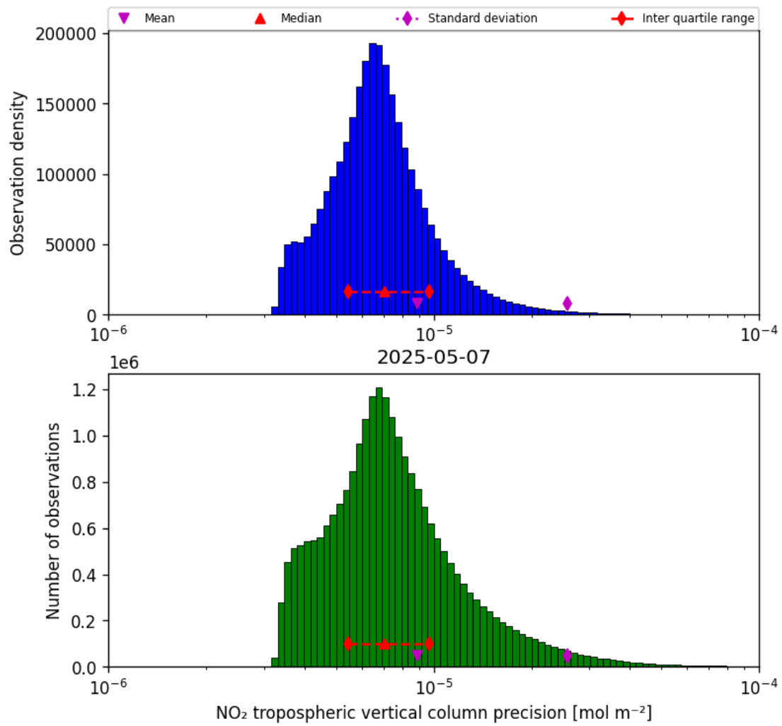
Figure 28: Histogram of “NO 2 tropospheric vertical column precision” for 2025-05-07 to 2025-05-08
