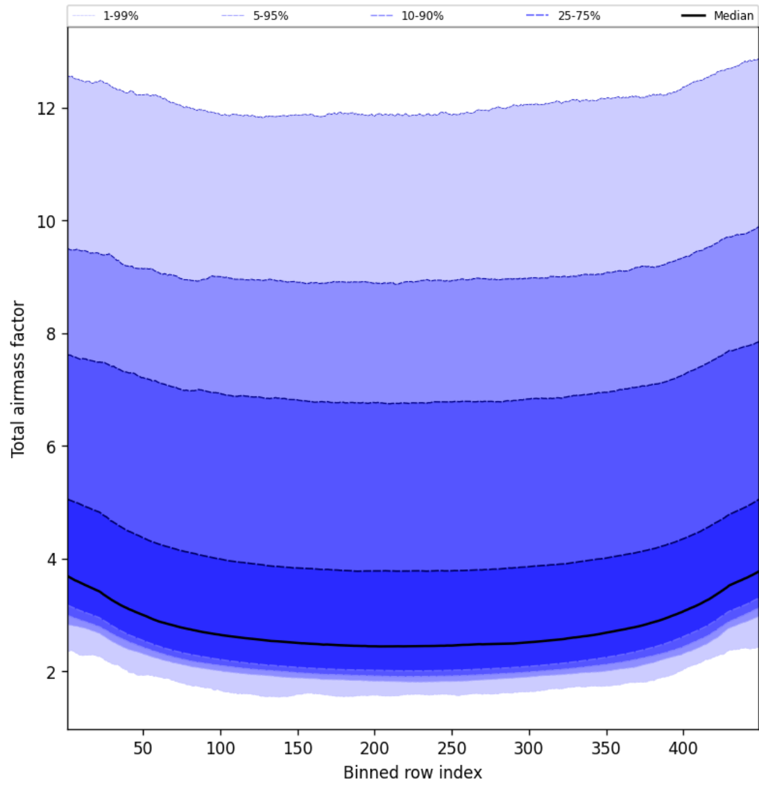
Figure 47: Along track statistics of “Total airmass factor” for 2025-05-07 to 2025-05-08
