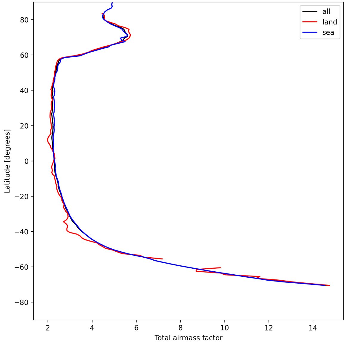
Figure 13: Zonal average of “Total airmass factor” for 2025-05-07 to 2025-05-08.
