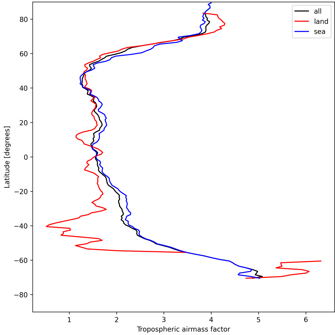
Figure 12: Zonal average of “Tropospheric air mass factor” for 2025-05-07 to 2025-05-08.
