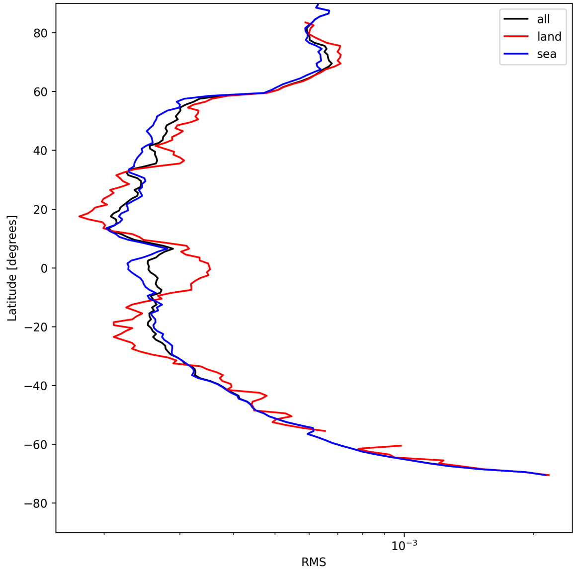
Figure 24: Zonal average of “RMS” for 2025-05-07 to 2025-05-08.
