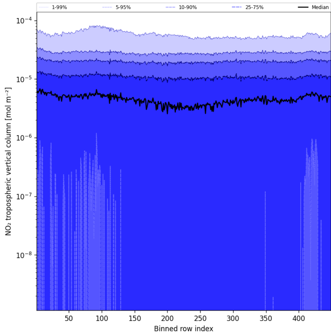
Figure 44: Along track statistics of “NO 2 tropospheric vertical column” for 2025-05-07 to 2025-05-08
