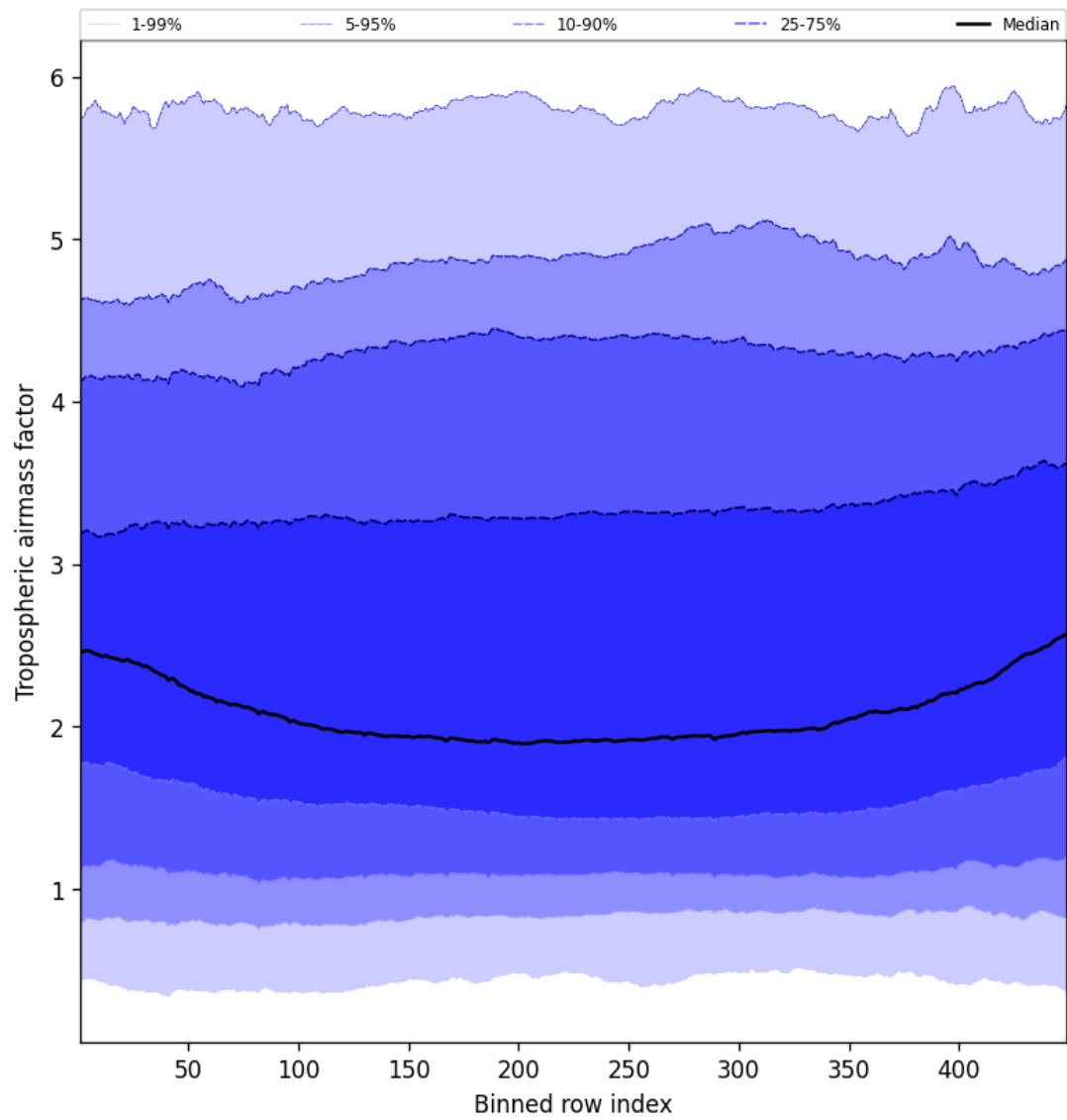
Figure 46: Along track statistics of “Tropospheric airmass factor” for 2025-05-07 to 2025-05-08
