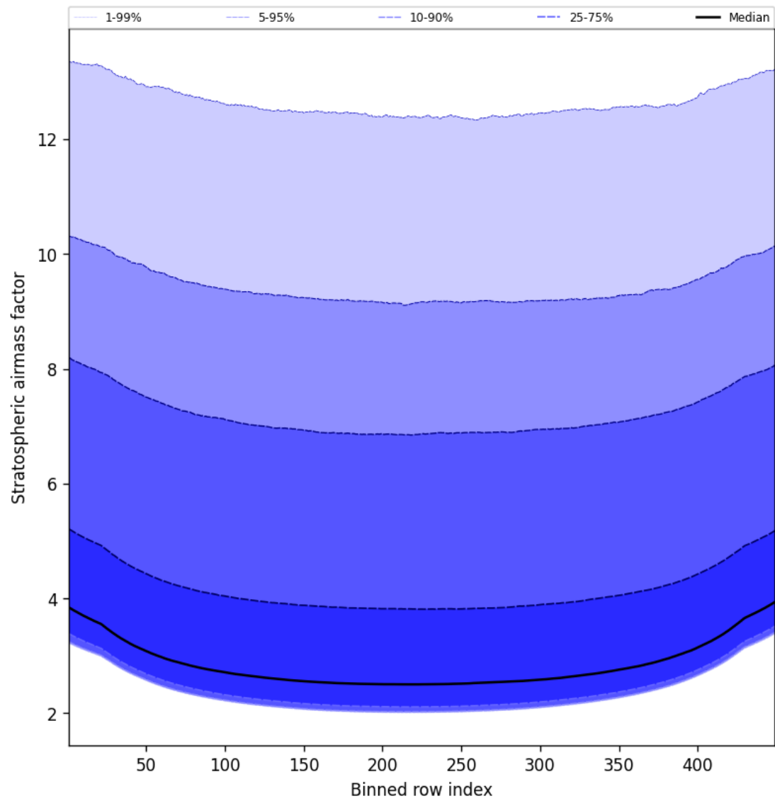
Figure 59: Along track statistics of “Stratospheric airmass factor” for 2025-05-07 to 2025-05-08
