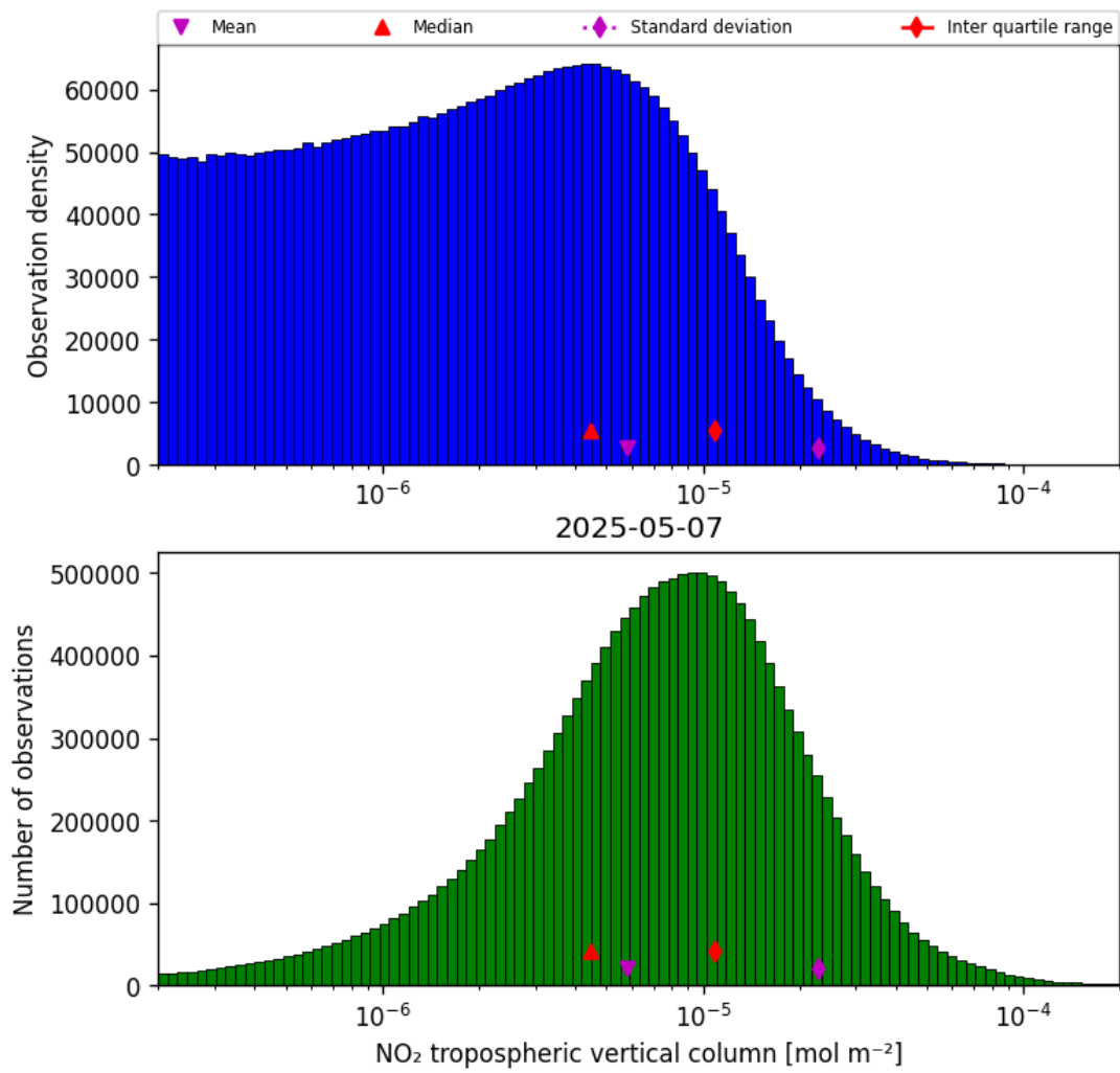
Figure 27: Histogram of “NO 2 tropospheric vertical column” for 2025-05-07 to 2025-05-08
