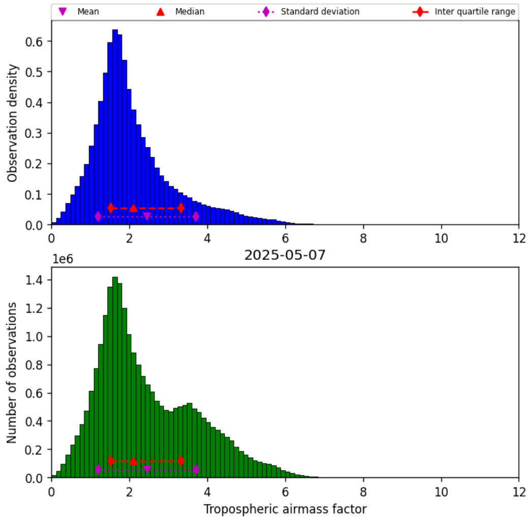
Figure 29: Histogram of “Tropospheric airmass factor” for 2025-05-07 to 2025-05-08
