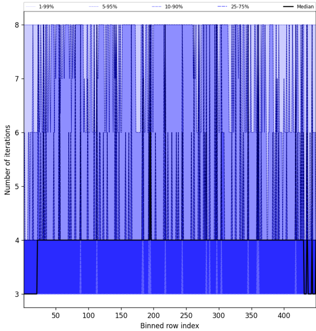
Figure 49: Along track statistics of “Number of iterations” for 2025-05-07 to 2025-05-08
