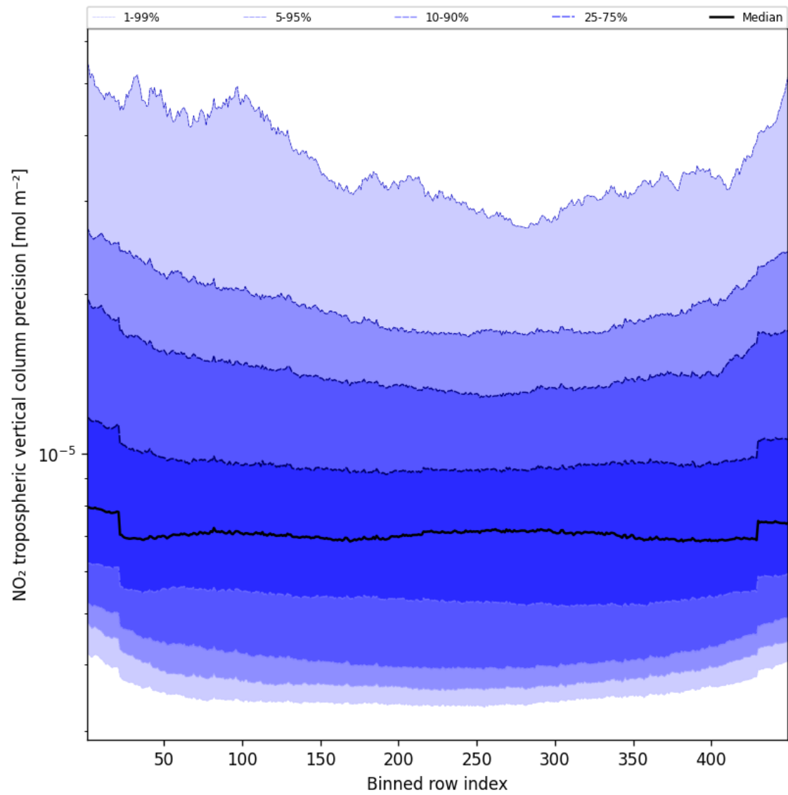
Figure 45: Along track statistics of “NO 2 tropospheric vertical column precision” for 2025-05-07 to 2025-05-08
