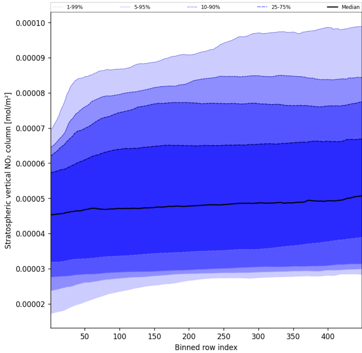
Figure 51: Along track statistics of “Stratospheric vertical NO 2 column” for 2025-05-07 to 2025-05-08
