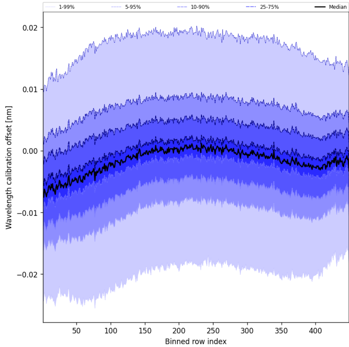
Figure 50: Along track statistics of “Wavelength calibration offset” for 2025-05-07 to 2025-05-08
