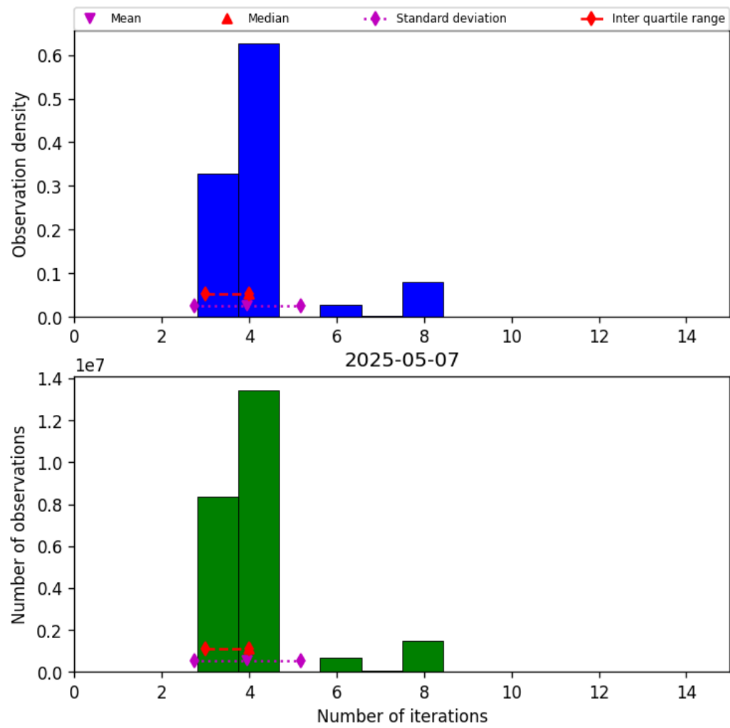
Figure 32: Histogram of “Number of iterations” for 2025-05-07 to 2025-05-08
