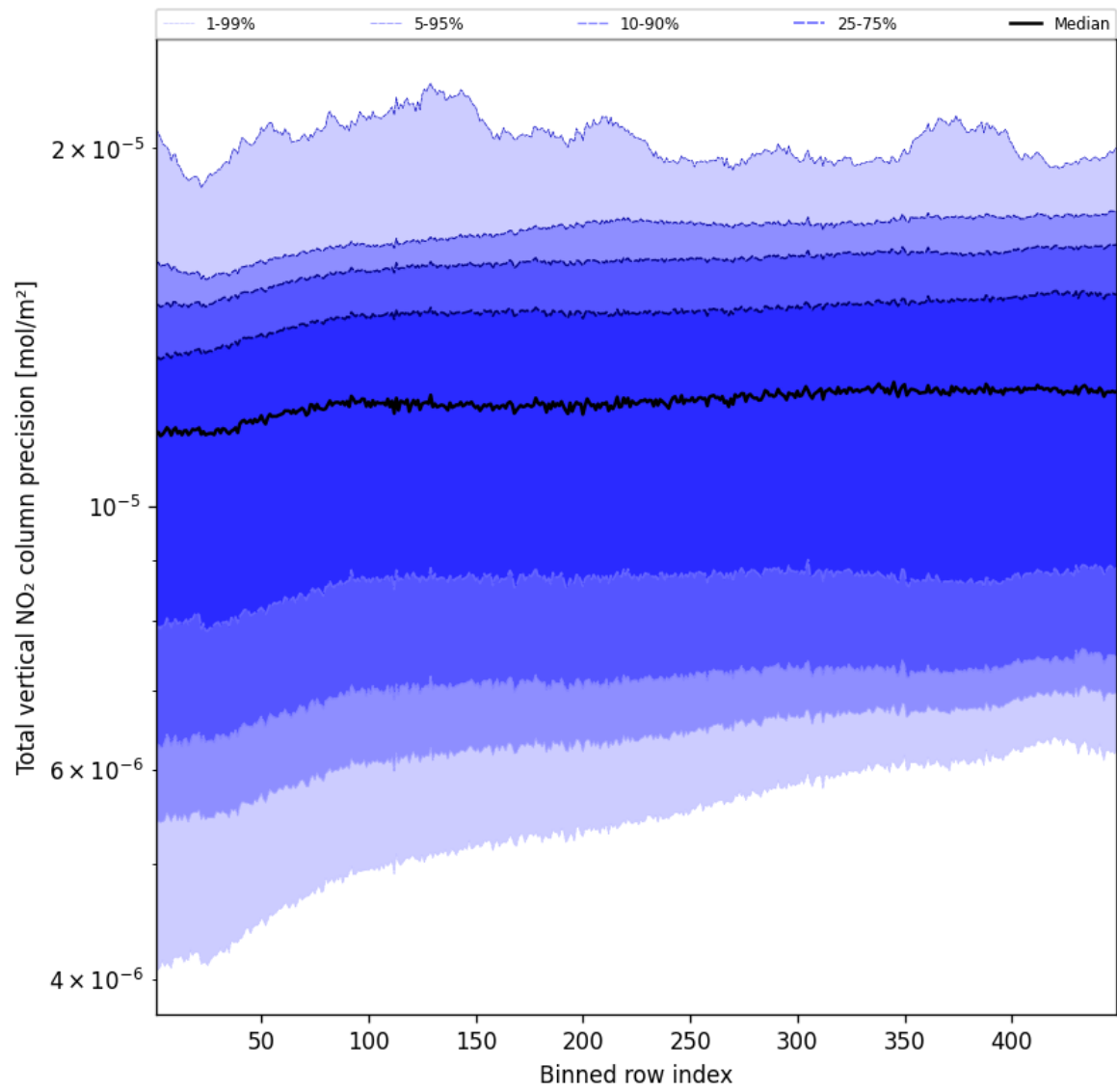
Figure 54: Along track statistics of “Total vertical NO 2 column precision” for 2025-05-07 to 2025-05-08
