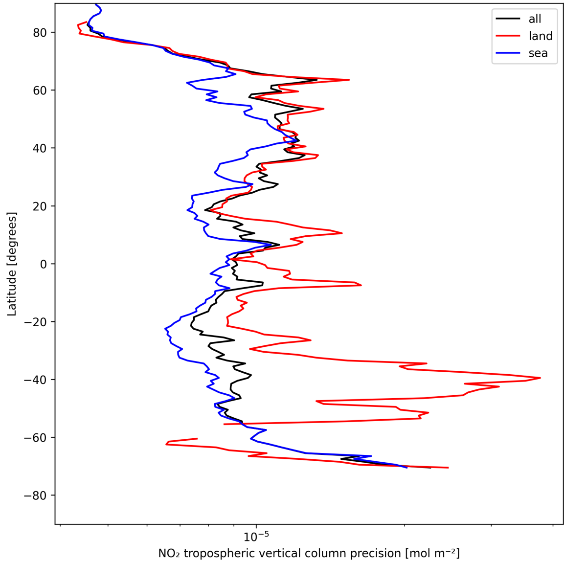
Figure 11: Zonal average of “NO 2 tropospheric vertical column precision” for 2025-05-07 to 2025-05-08.
