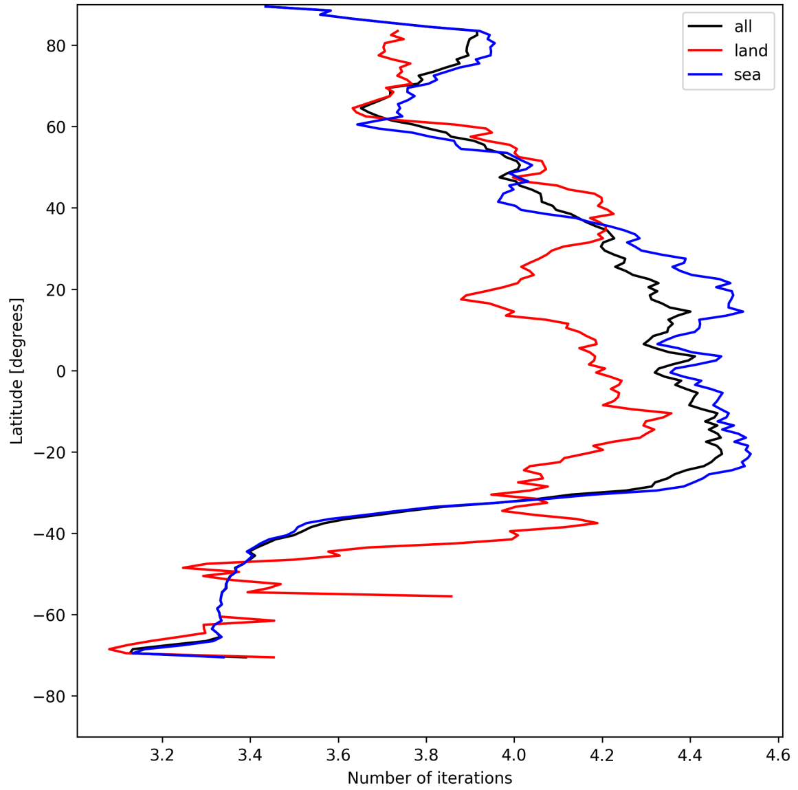
Figure 15: Zonal average of “Number of iterations” for 2025-05-07 to 2025-05-08.
