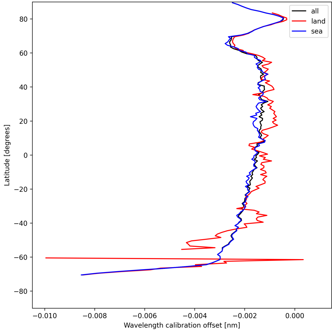
Figure 16: Zonal average of “Wavelength calibration offset” for 2025-05-07 to 2025-05-08.
