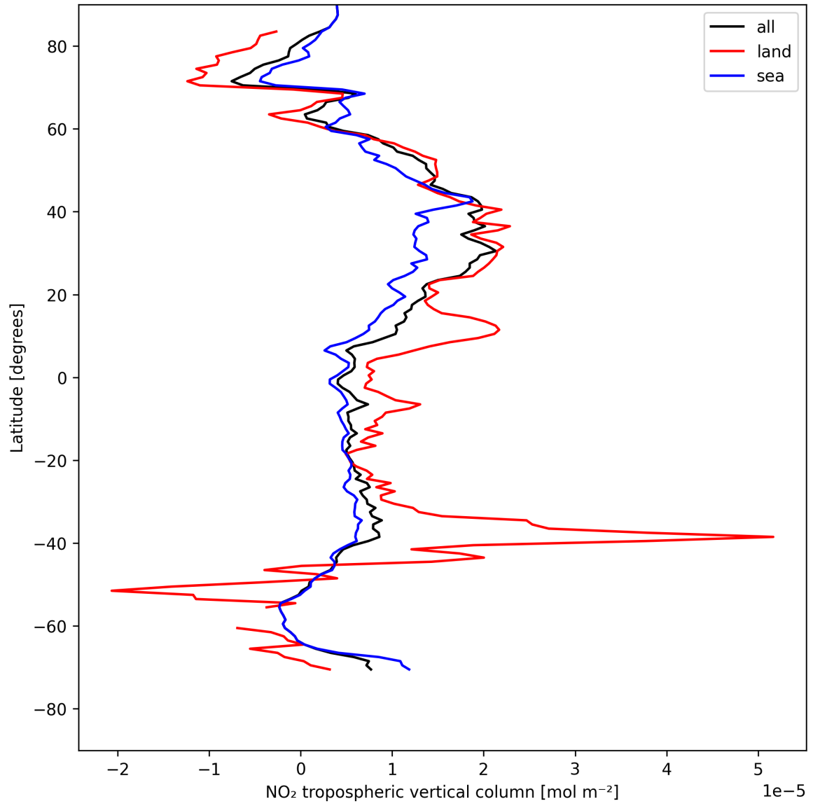
Figure 10: Zonal average of “NO 2 tropospheric vertical column” for 2025-05-07 to 2025-05-08.
