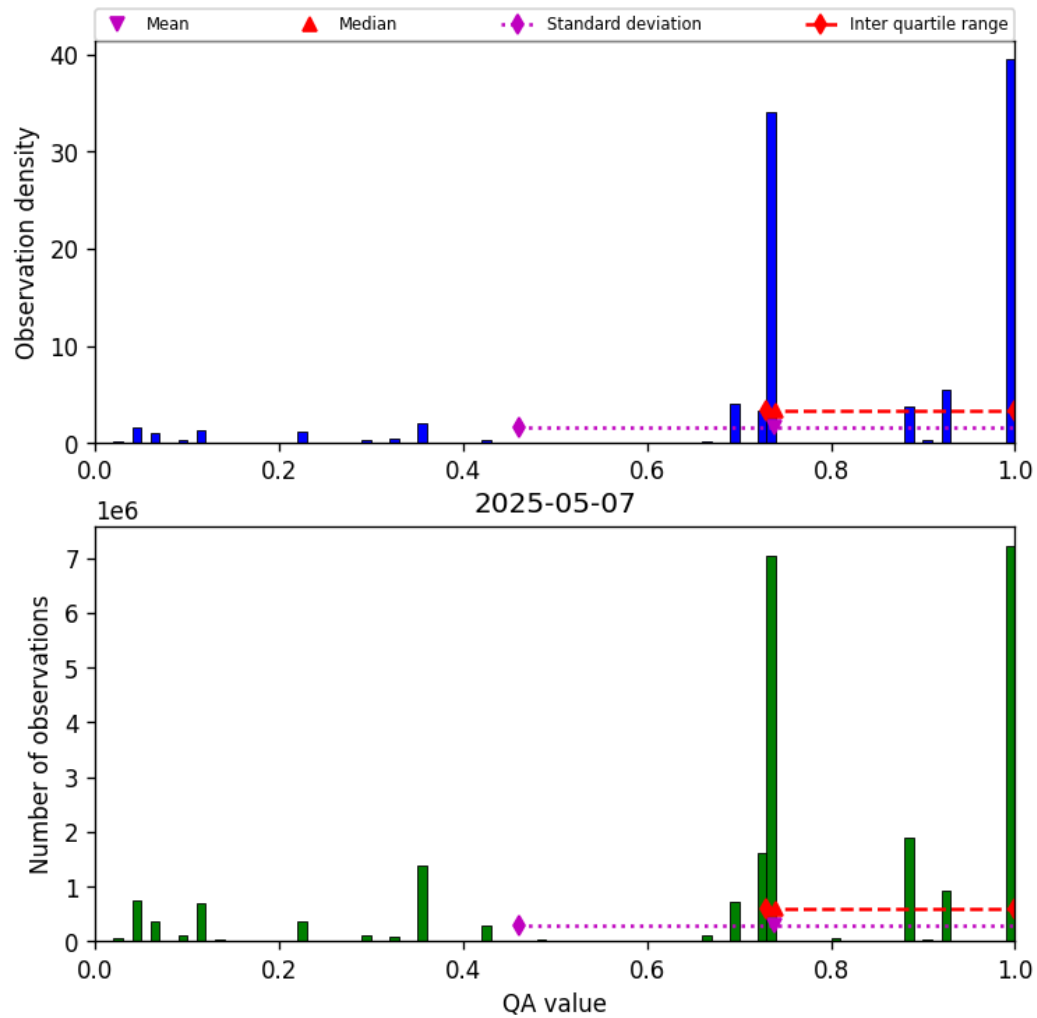
Figure 26: Histogram of “QA value” for 2025-05-07 to 2025-05-08
