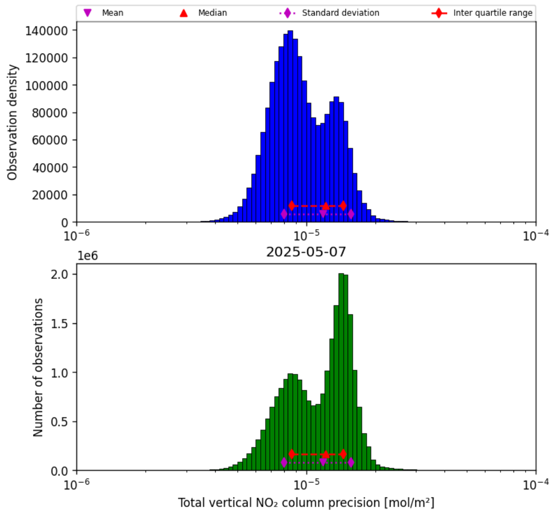
Figure 37: Histogram of “Total vertical NO 2 column precision” for 2025-05-07 to 2025-05-08
