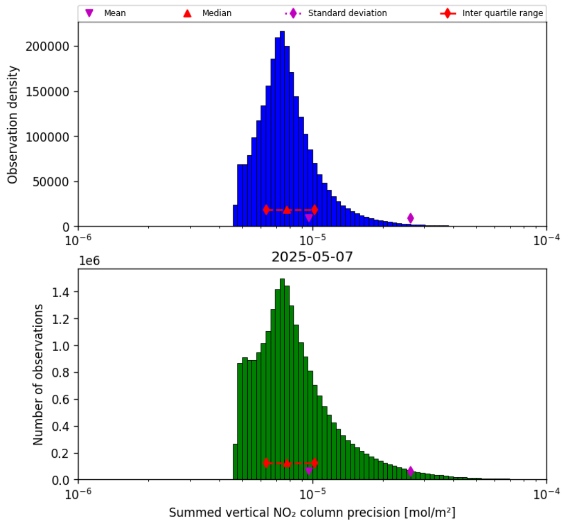
Figure 39: Histogram of “Summed vertical NO 2 column precision” for 2025-05-07 to 2025-05-08
