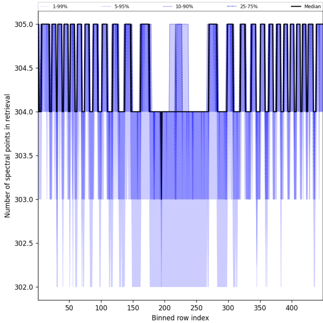
Figure 48: Along track statistics of “Number of spectral points in retrieval” for 2025-05-07 to 2025-05-08
