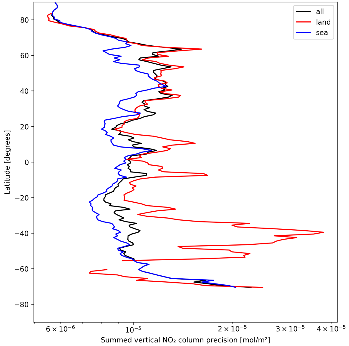
Figure 22: Zonal average of “Summed vertical NO 2 column precision” for 2025-05-07 to 2025-05-08.
