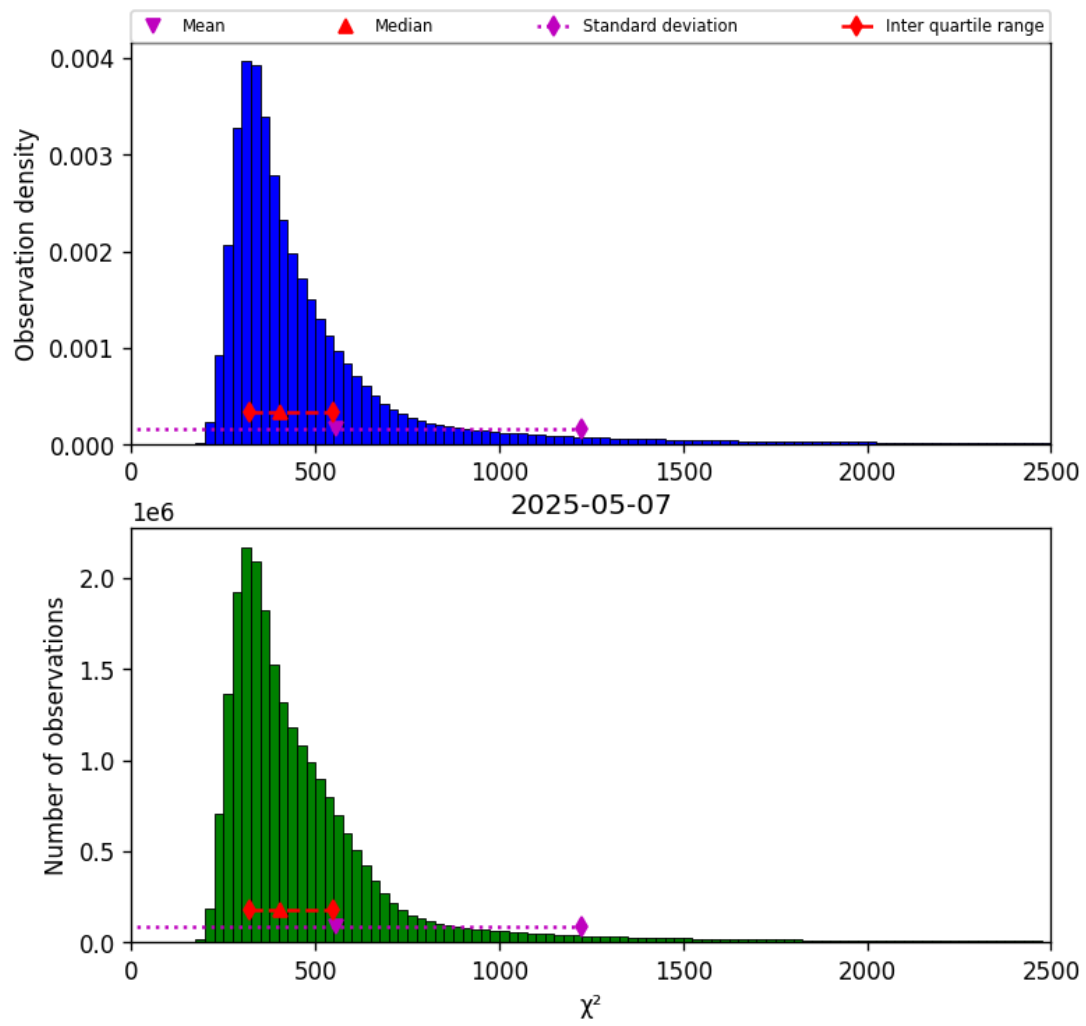
Figure 40: Histogram of “ \chi^2 ” for 2025-05-07 to 2025-05-08
