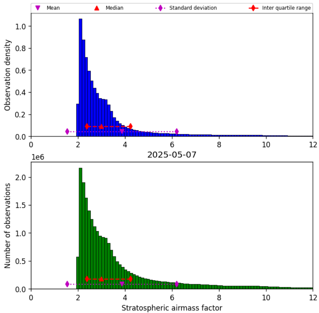
Figure 42: Histogram of “Stratospheric airmass factor” for 2025-05-07 to 2025-05-08
