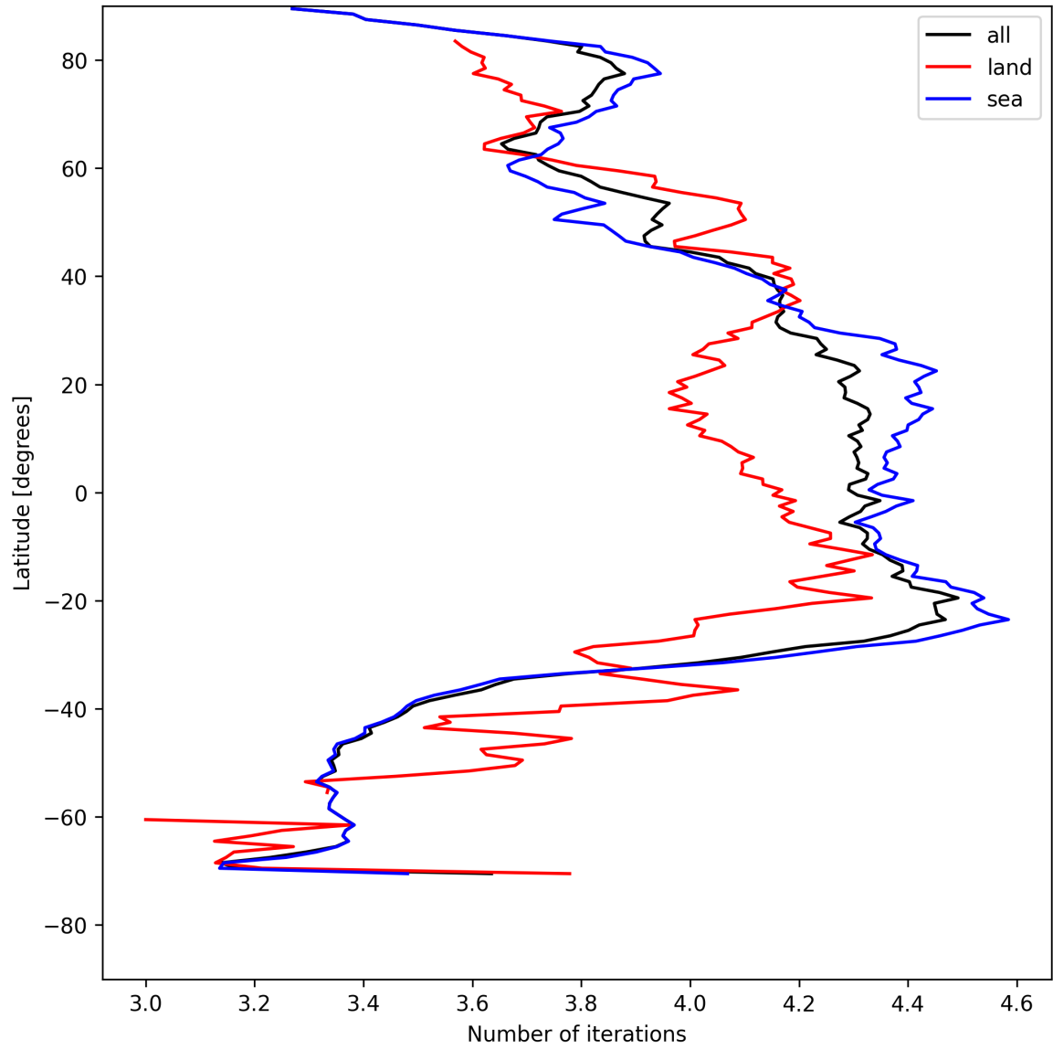
Figure 15: Zonal average of “Number of iterations” for 2025-05-08 to 2025-05-08.
