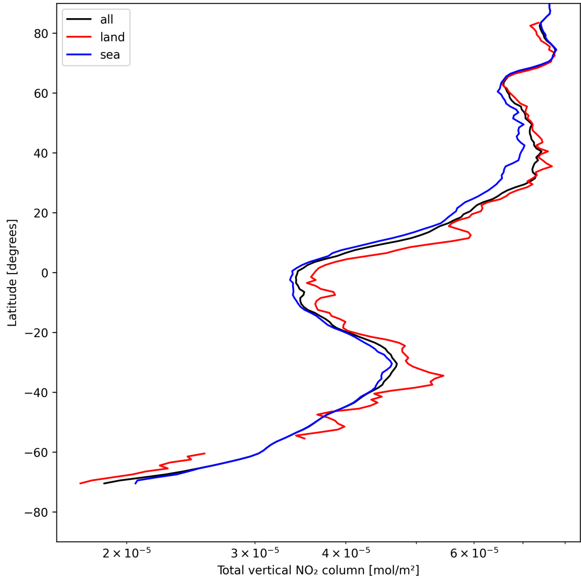
Figure 19: Zonal average of “Total vertical NO 2 column” for 2025-05-08 to 2025-05-08.
