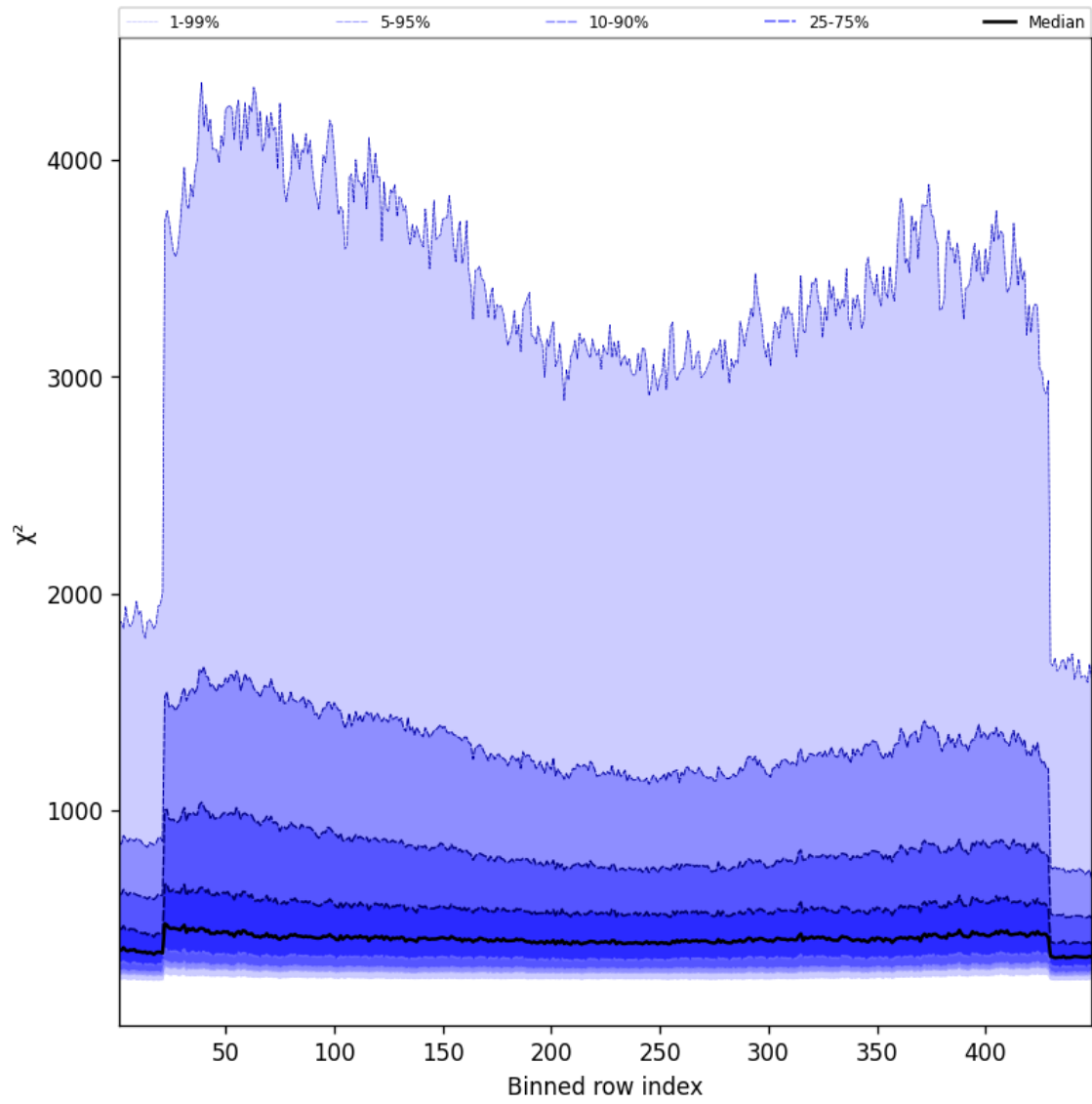
Figure 57: Along track statistics of “ \chi^2 ” for 2025-05-08 to 2025-05-08
