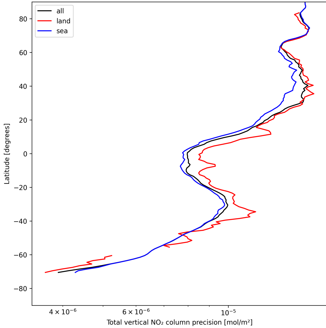
Figure 20: Zonal average of “Total vertical NO 2 column precision” for 2025-05-08 to 2025-05-08.
