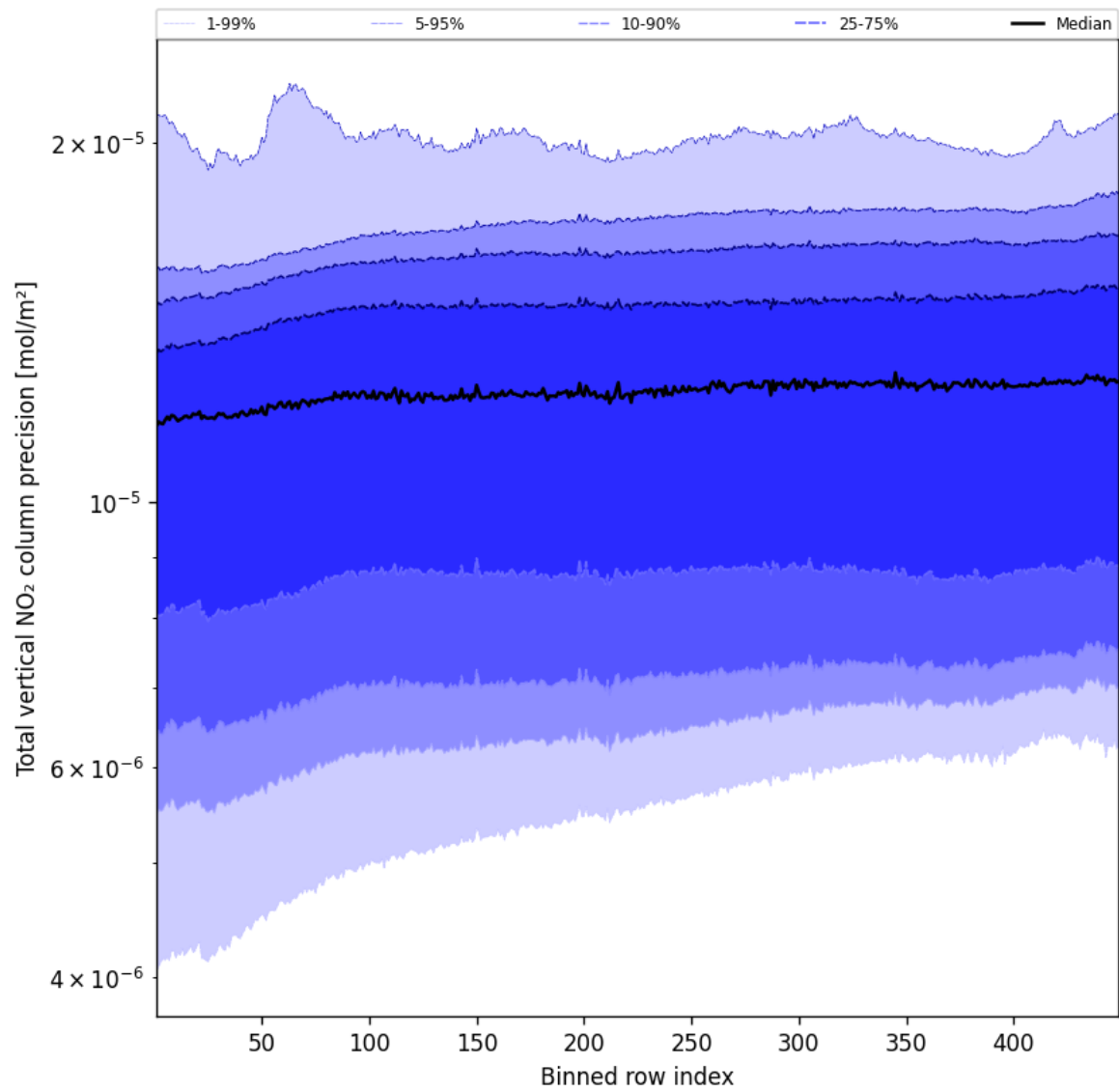
Figure 54: Along track statistics of “Total vertical NO 2 column precision” for 2025-05-08 to 2025-05-08
