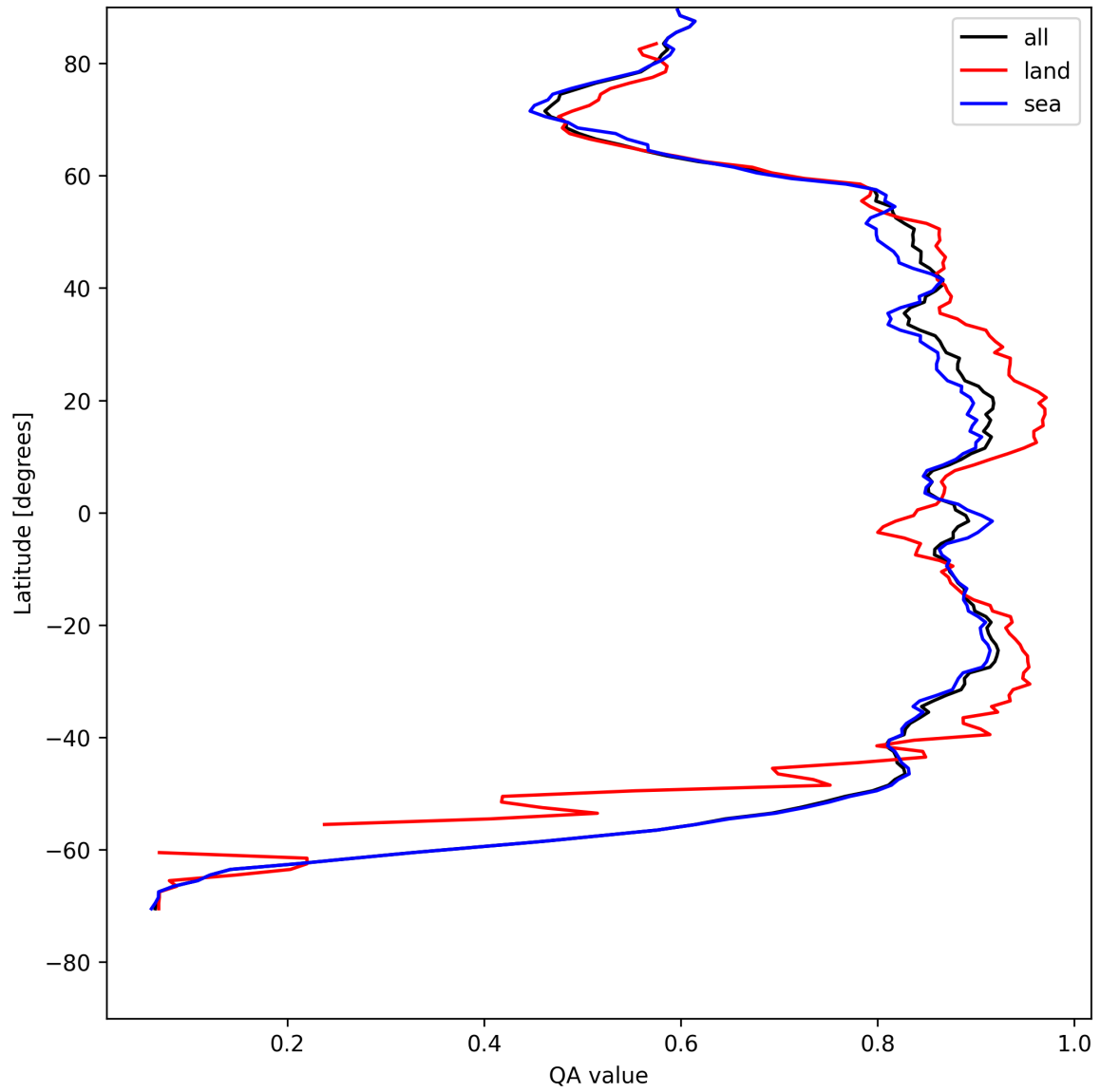
Figure 9: Zonal average of “QA value” for 2025-05-08 to 2025-05-08.
