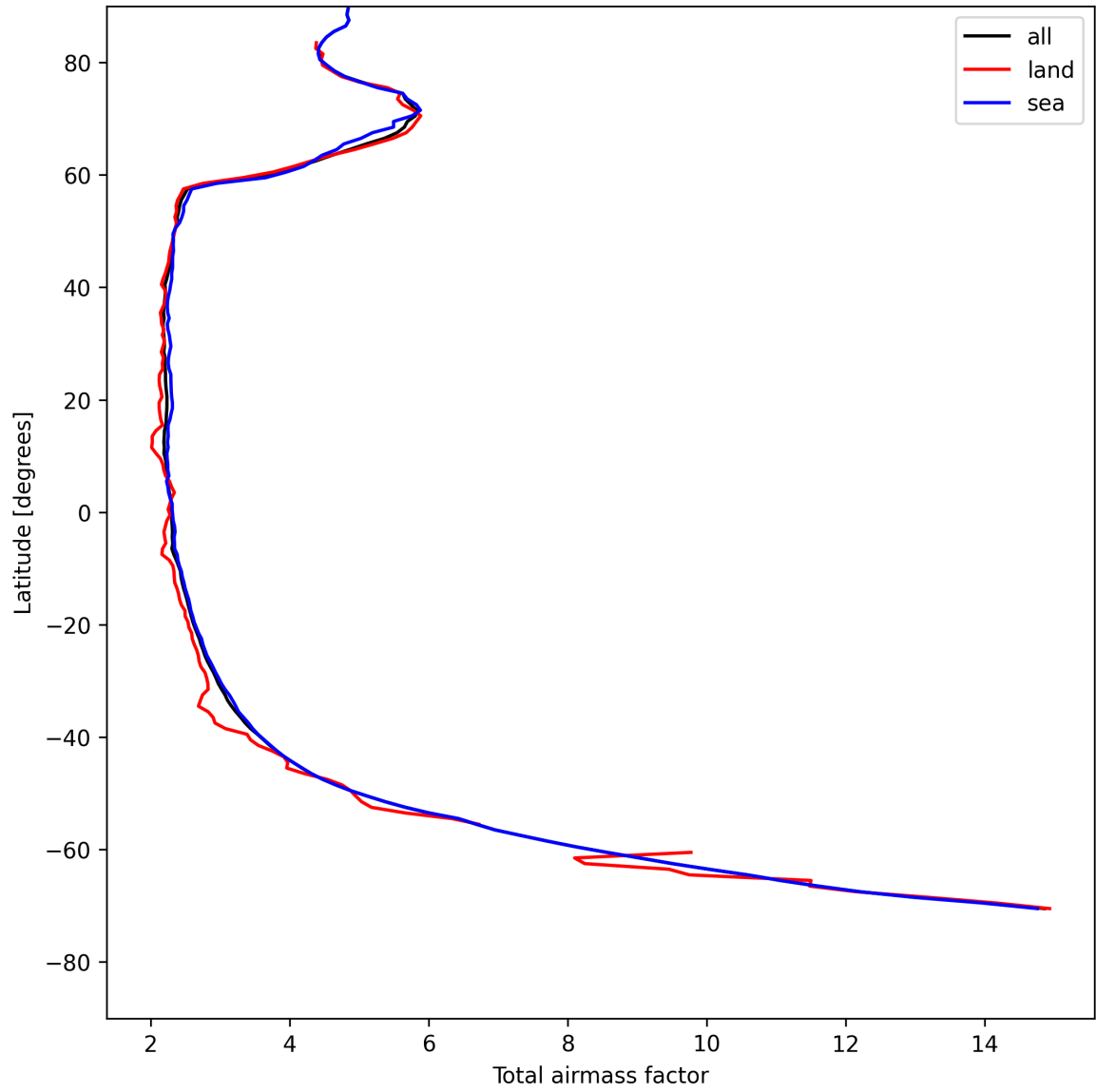
Figure 13: Zonal average of “Total airmass factor” for 2025-05-08 to 2025-05-08.
