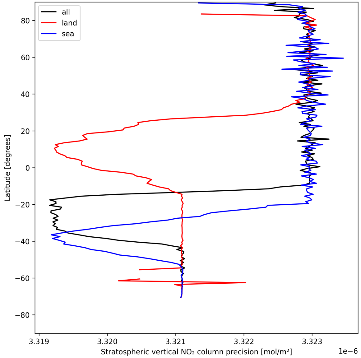
Figure 18: Zonal average of “Stratospheric vertical NO 2 column precision” for 2025-05-08 to 2025-05-08.
