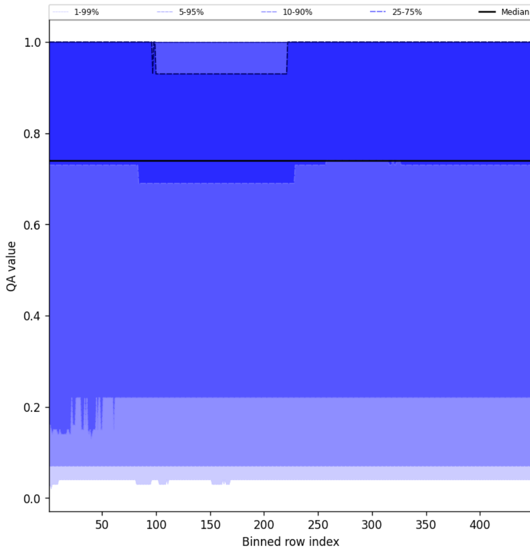
Figure 43: Along track statistics of “QA value” for 2025-05-08 to 2025-05-08
