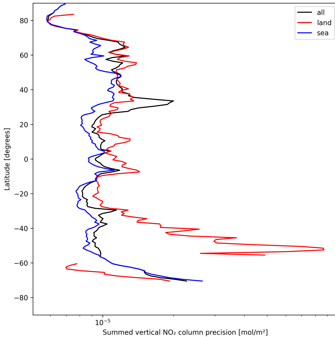
Figure 22: Zonal average of “Summed vertical NO 2 column precision” for 2025-05-08 to 2025-05-08.
