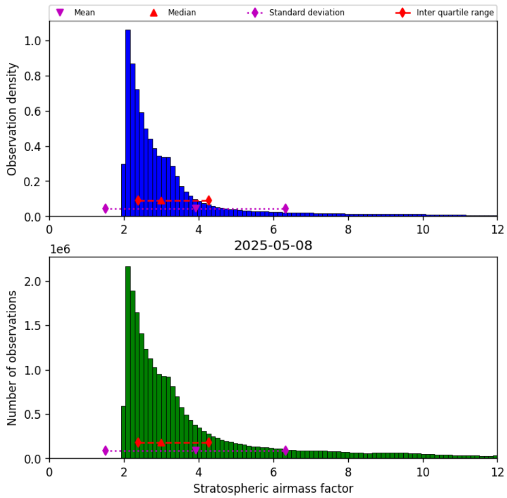
Figure 42: Histogram of “Stratospheric airmass factor” for 2025-05-08 to 2025-05-08
