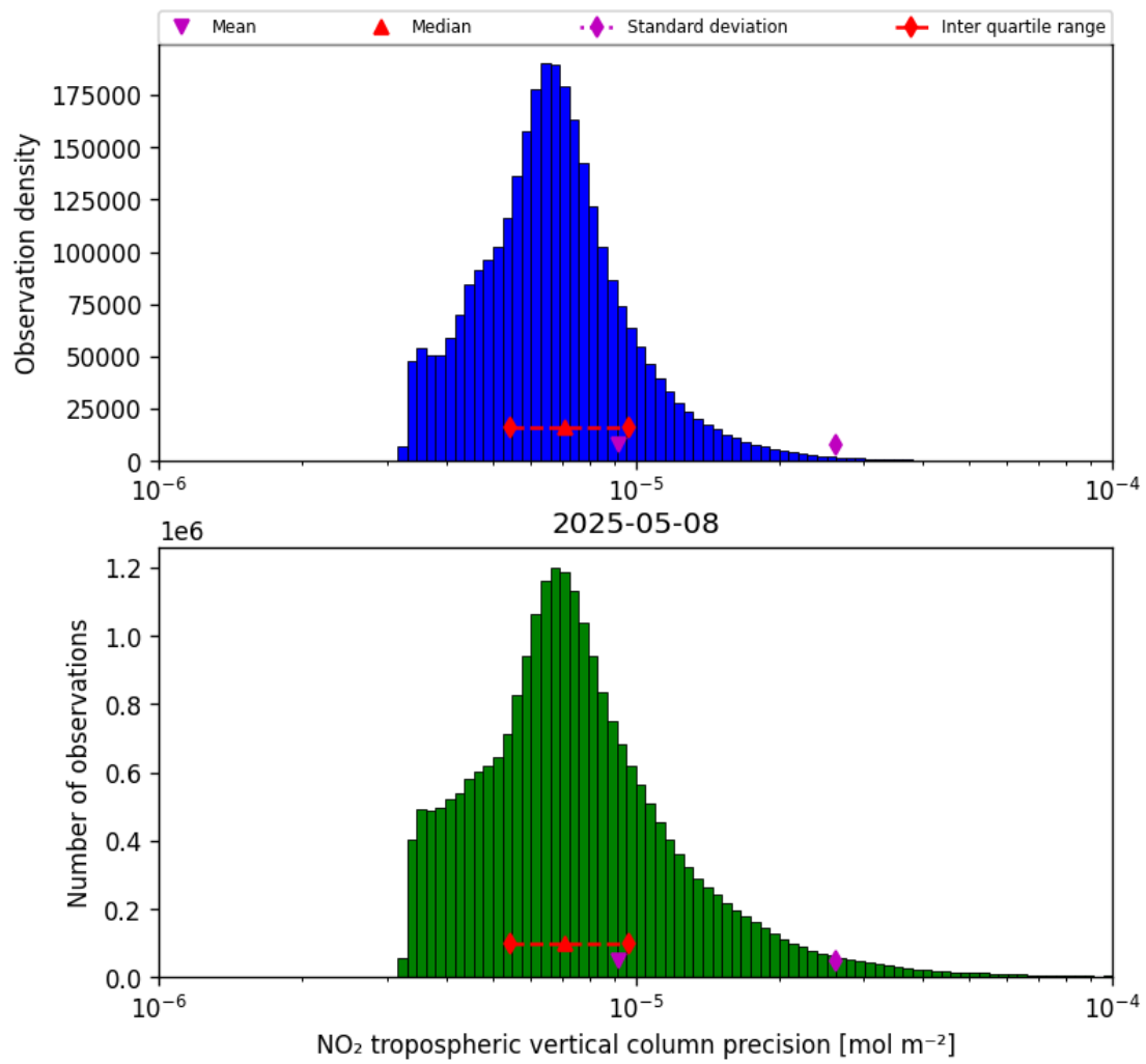
Figure 28: Histogram of “NO 2 tropospheric vertical column precision” for 2025-05-08 to 2025-05-08
