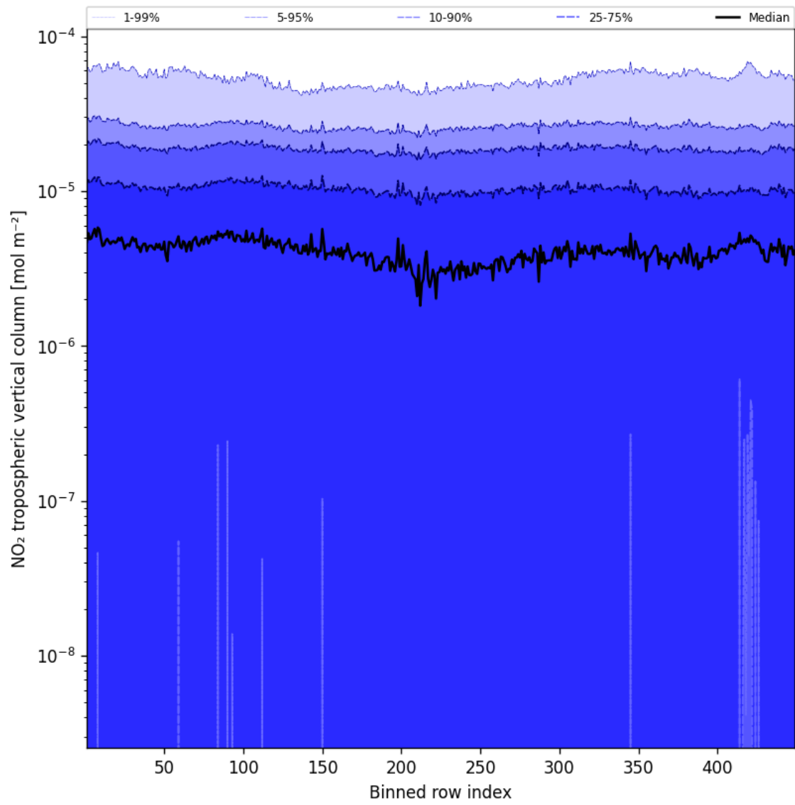
Figure 44: Along track statistics of “NO 2 tropospheric vertical column” for 2025-05-08 to 2025-05-08
