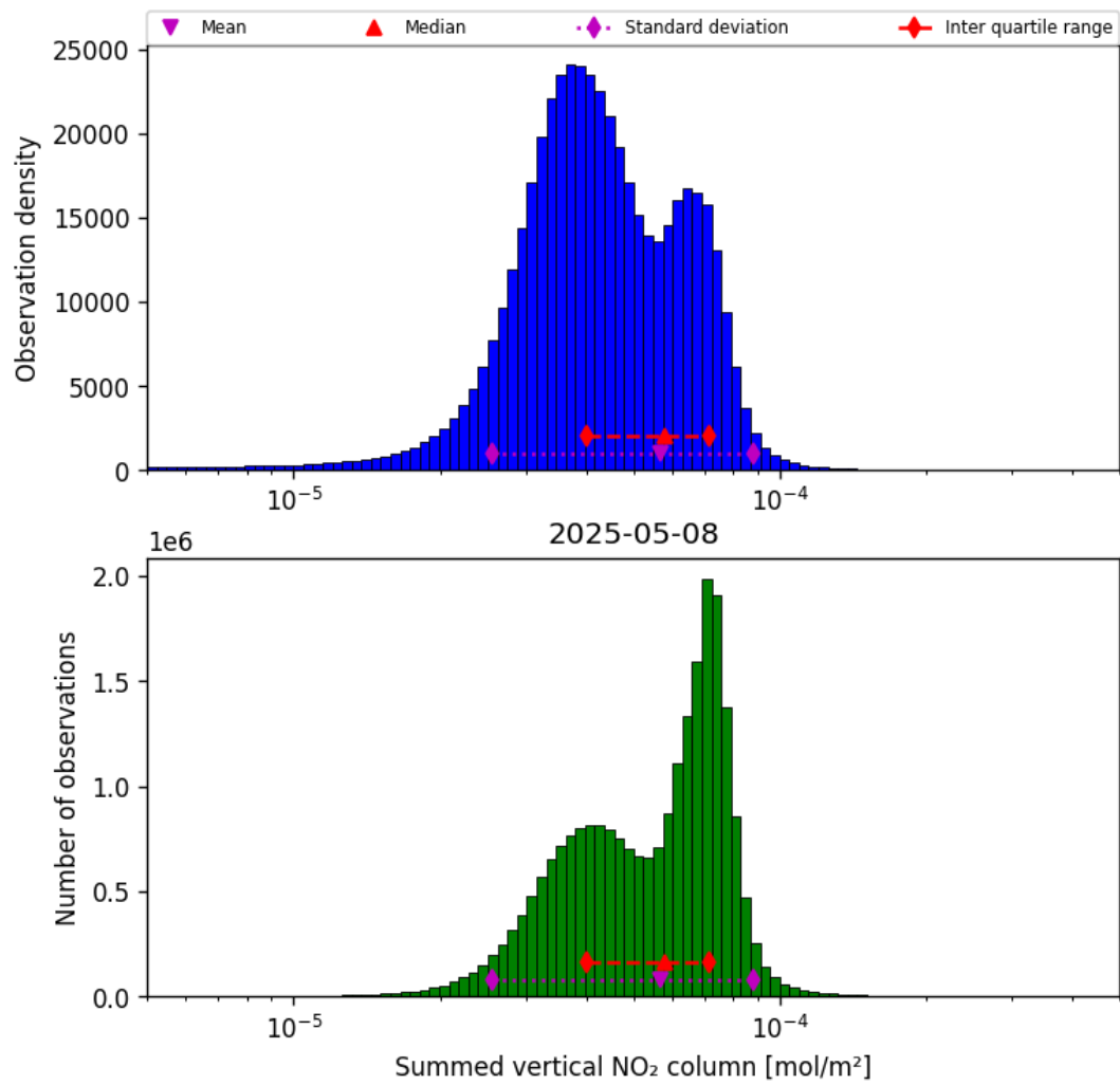
Figure 38: Histogram of “Summed vertical NO 2 column” for 2025-05-08 to 2025-05-08
