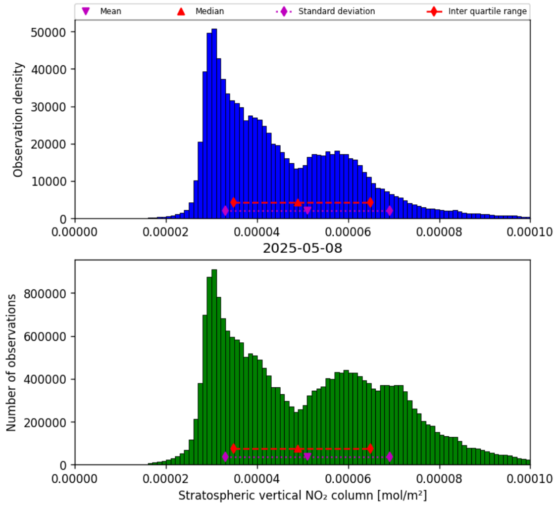
Figure 34: Histogram of “Stratospheric vertical NO 2 column” for 2025-05-08 to 2025-05-08
