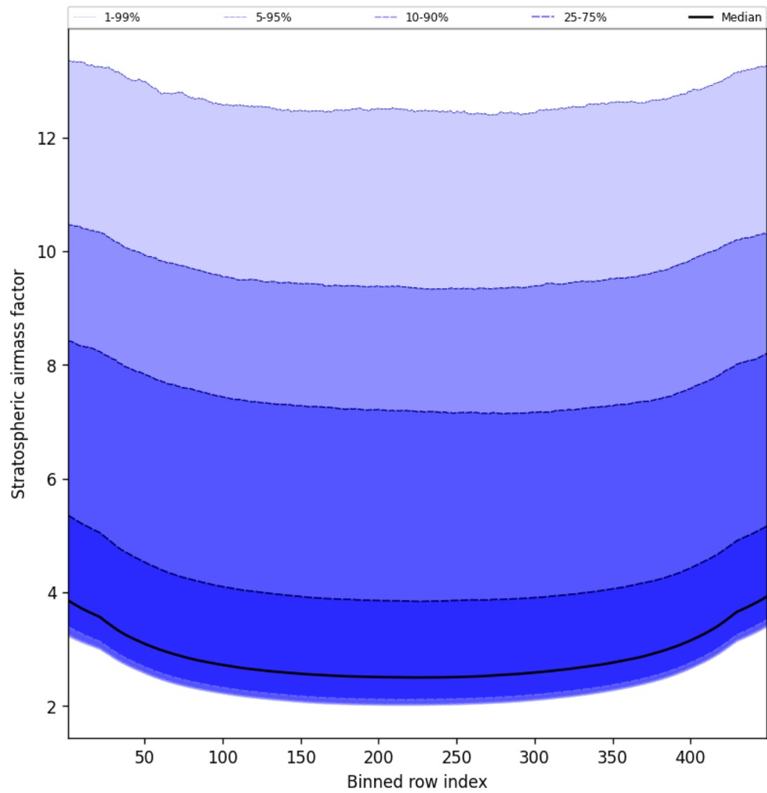
Figure 59: Along track statistics of “Stratospheric airmass factor” for 2025-05-08 to 2025-05-08
