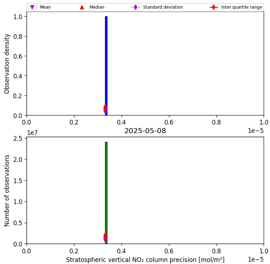
Figure 35: Histogram of “Stratospheric vertical NO 2 column precision” for 2025-05-08 to 2025-05-08
