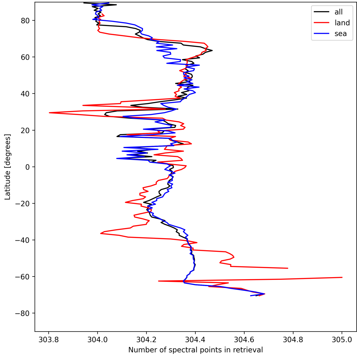
Figure 14: Zonal average of “Number of spectral points in retrieval” for 2025-05-08 to 2025-05-08.
