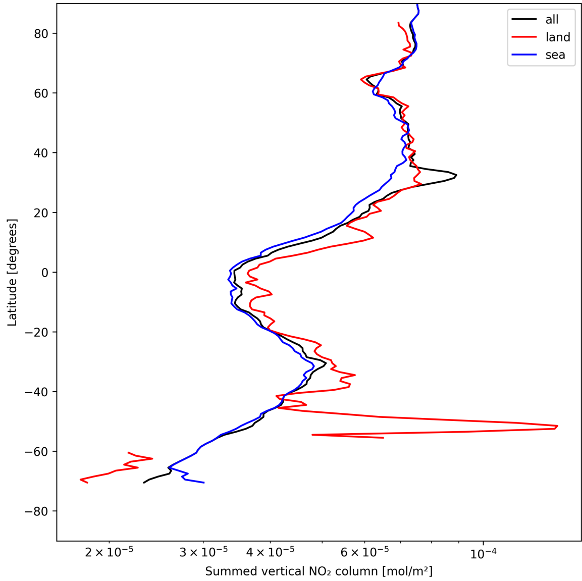
Figure 21: Zonal average of “Summed vertical NO 2 column” for 2025-05-08 to 2025-05-08.
