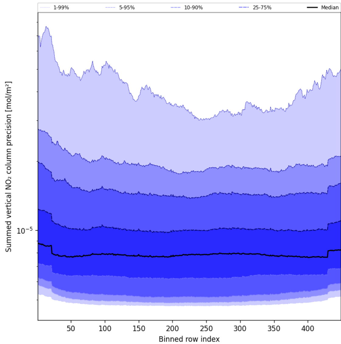
Figure 56: Along track statistics of “Summed vertical NO 2 column precision” for 2025-05-08 to 2025-05-08
