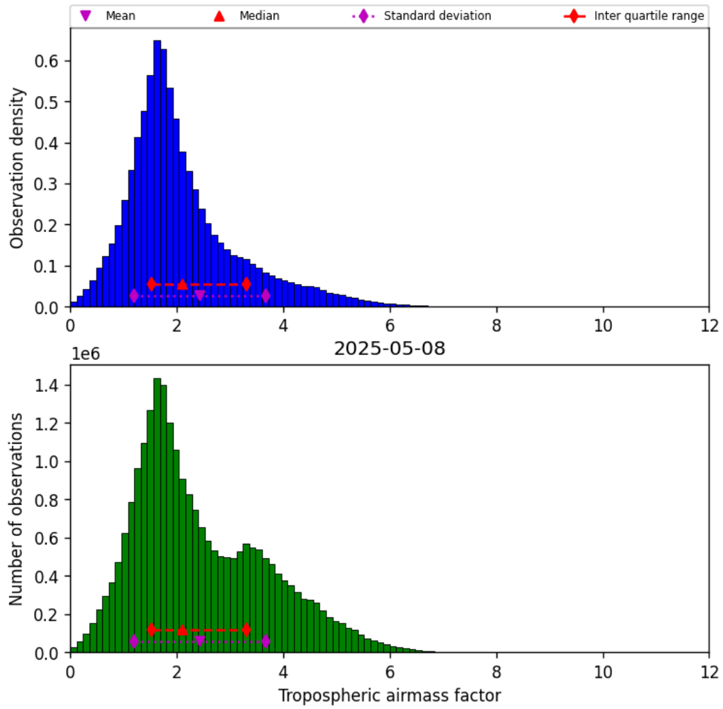
Figure 29: Histogram of “Tropospheric airmass factor” for 2025-05-08 to 2025-05-08
