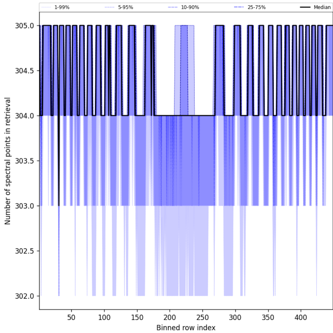
Figure 48: Along track statistics of “Number of spectral points in retrieval” for 2025-05-08 to 2025-05-08
