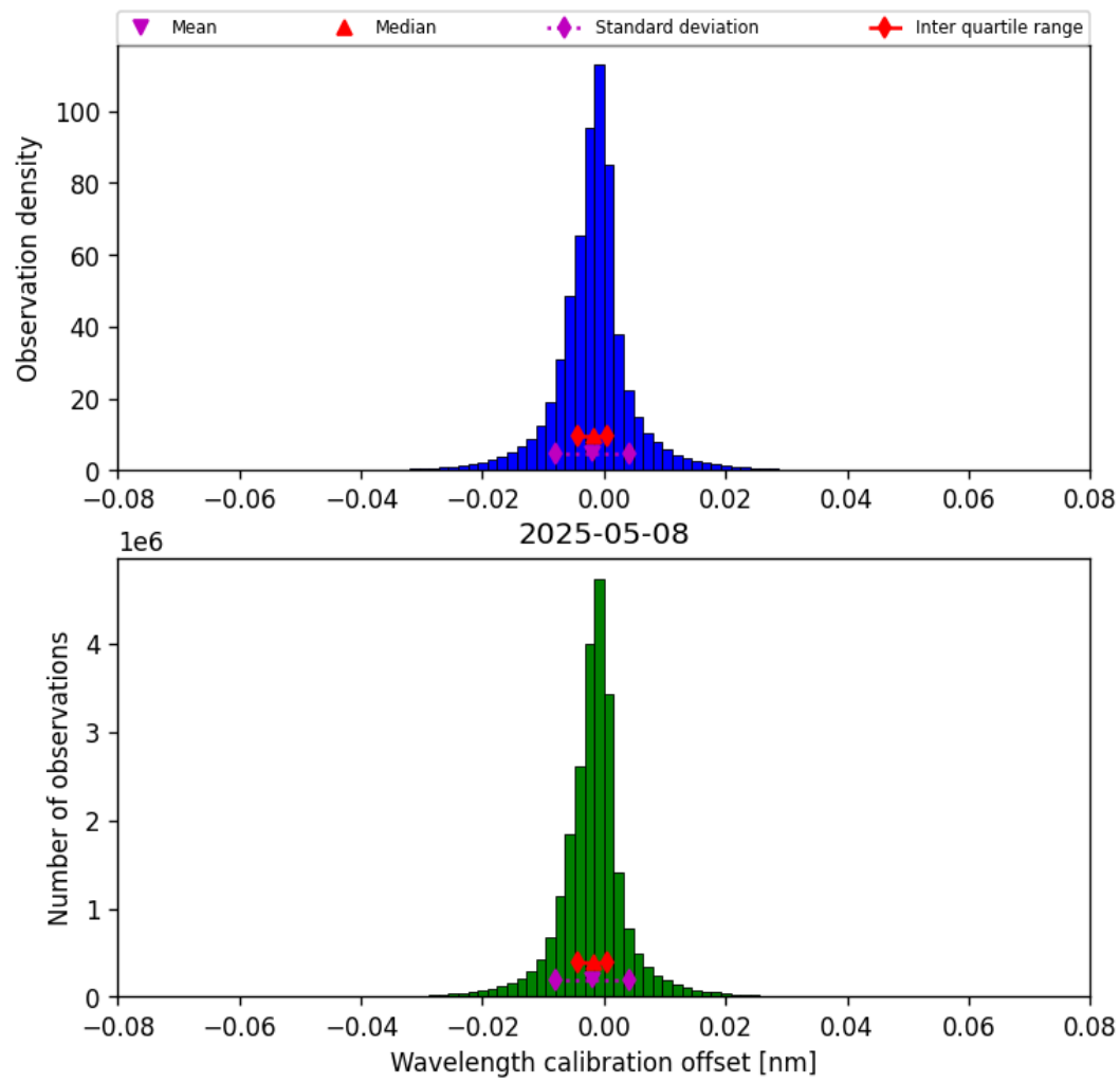
Figure 33: Histogram of “Wavelength calibration offset” for 2025-05-08 to 2025-05-08
