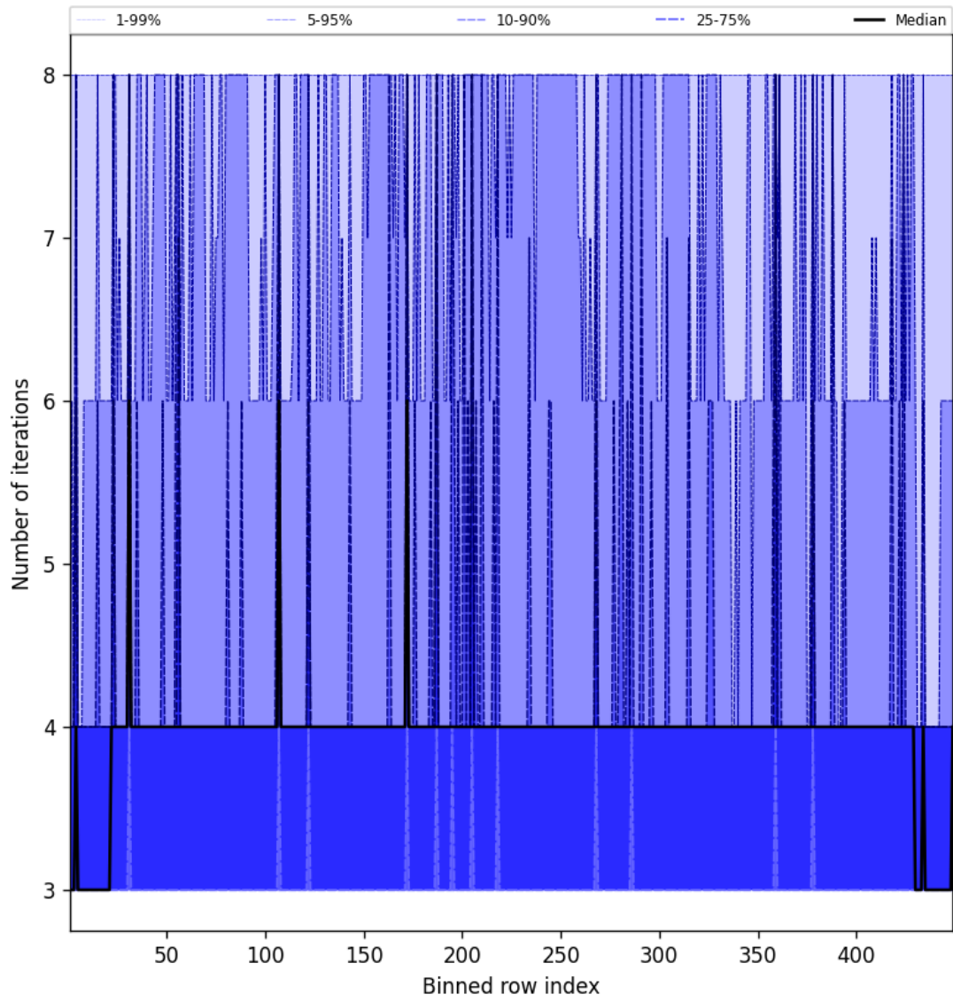
Figure 49: Along track statistics of “Number of iterations” for 2025-05-08 to 2025-05-08
