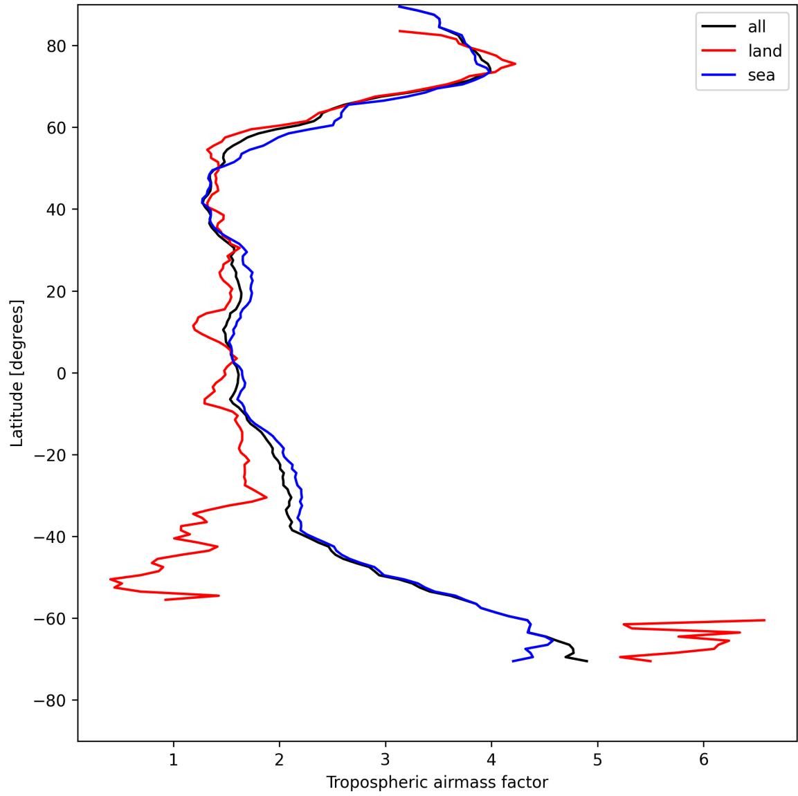
Figure 12: Zonal average of “Tropospheric airmass factor” for 2025-05-08 to 2025-05-08.
