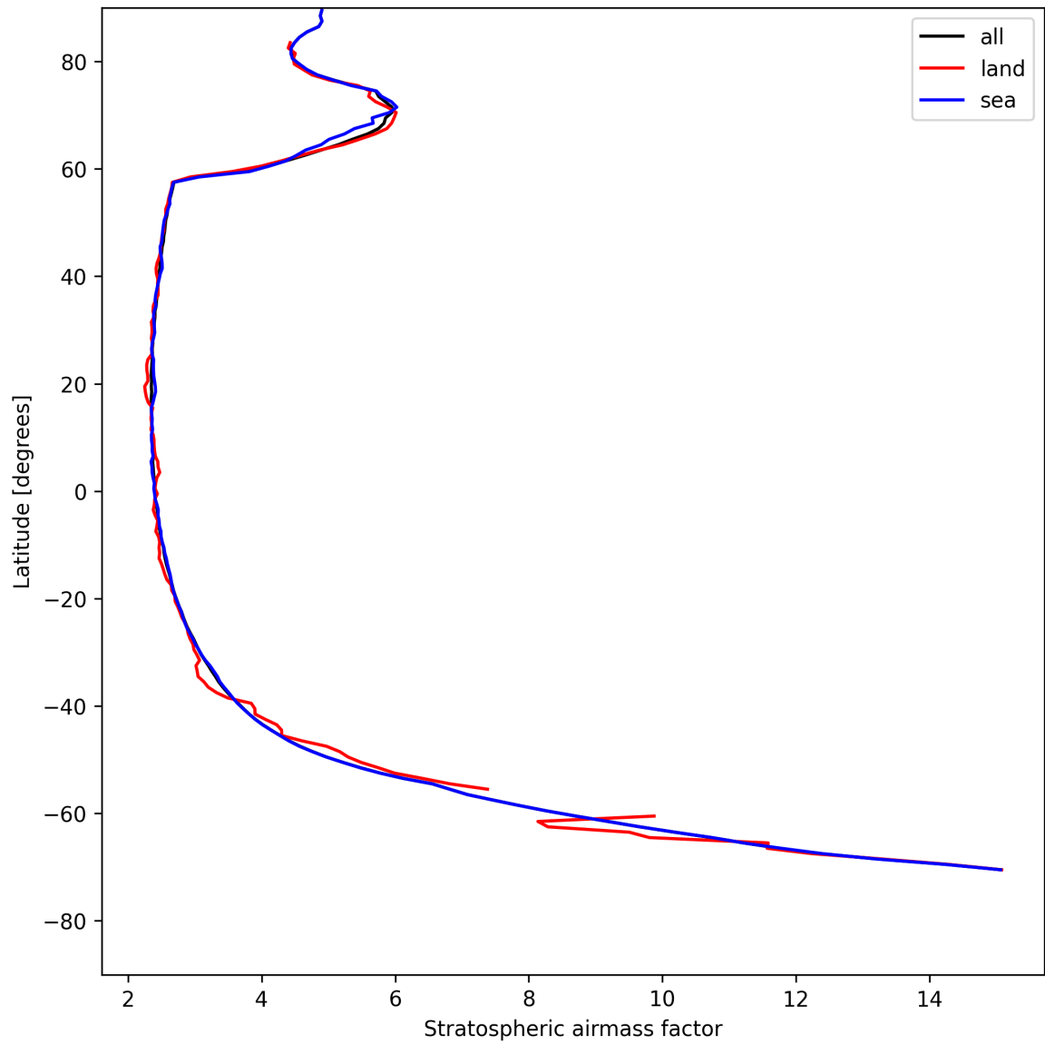
Figure 25: Zonal average of “Stratospheric airmass factor” for 2025-05-08 to 2025-05-08.
