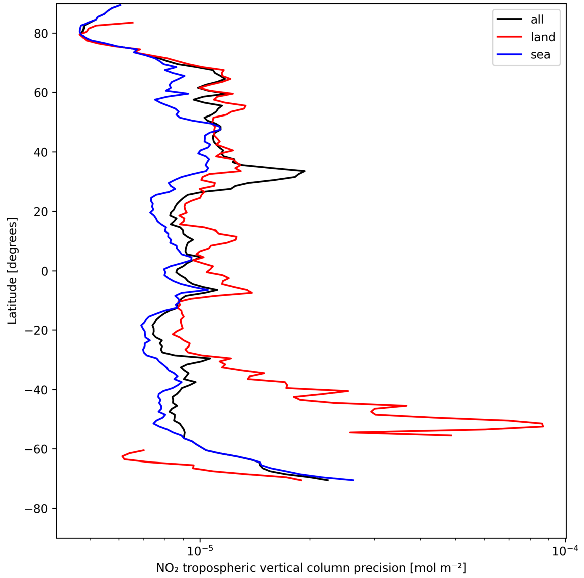
Figure 11: Zonal average of “NO 2 tropospheric vertical column precision” for 2025-05-08 to 2025-05-08.
