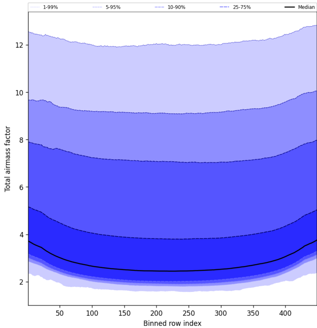
Figure 47: Along track statistics of “Total airmass factor” for 2025-05-08 to 2025-05-08
