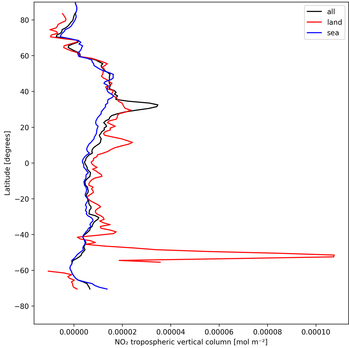
Figure 10: Zonal average of “NO 2 tropospheric vertical column” for 2025-05-08 to 2025-05-08.
