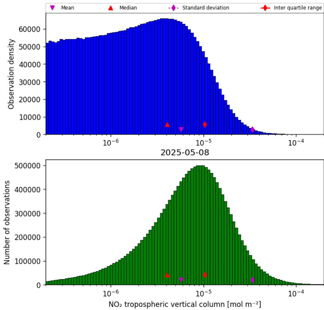
Figure 27: Histogram of “ \text{NO}_2 tropospheric vertical column” for 2025-05-08 to 2025-05-08
