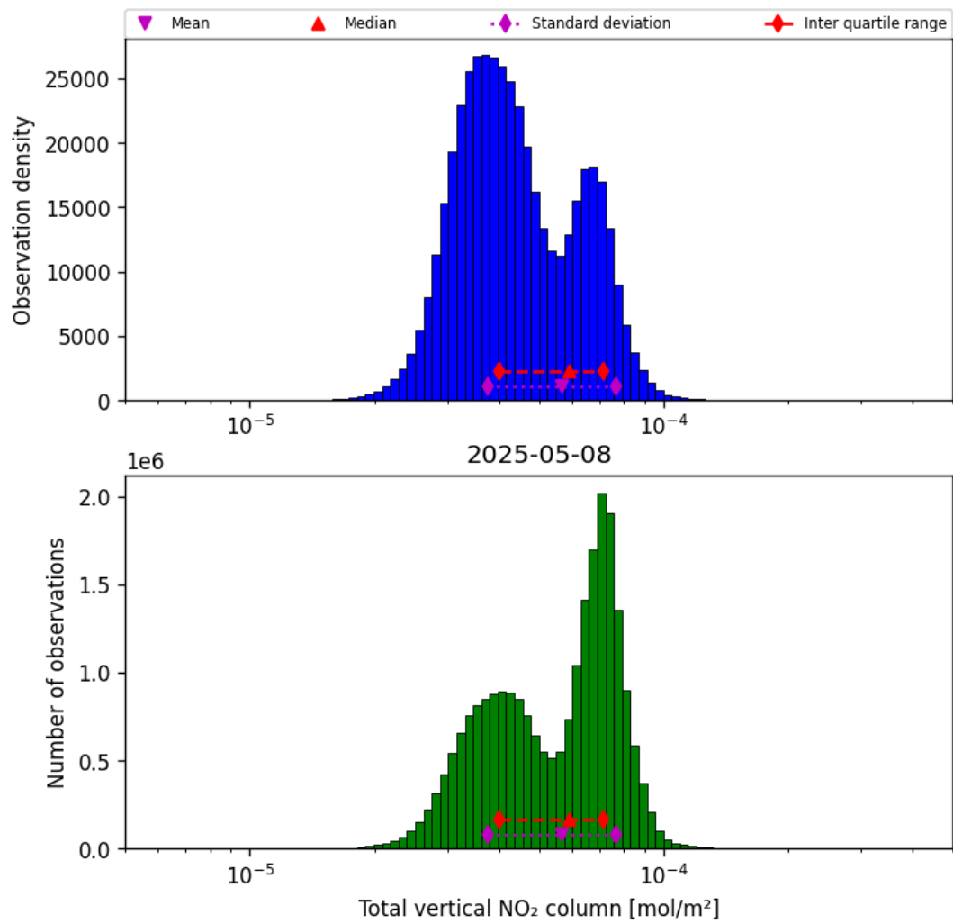
Figure 36: Histogram of “Total vertical NO 2 column” for 2025-05-08 to 2025-05-08
