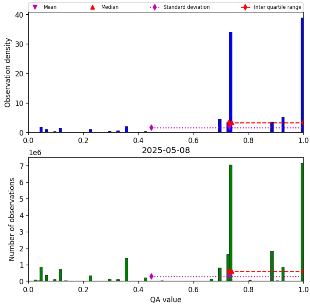
Figure 26: Histogram of “QA value” for 2025-05-08 to 2025-05-08
