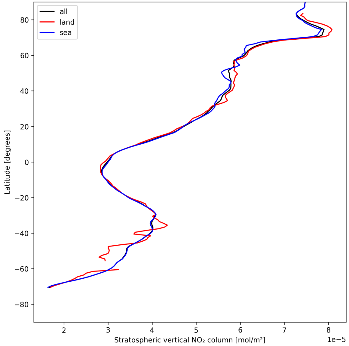
Figure 17: Zonal average of “Stratospheric vertical NO 2 column” for 2025-05-08 to 2025-05-08.
