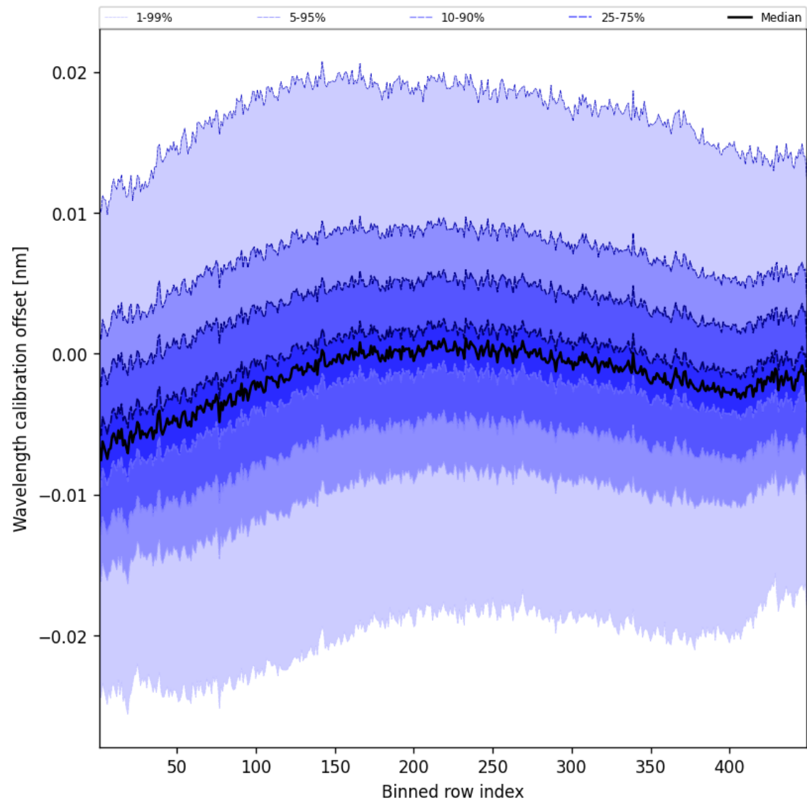
Figure 50: Along track statistics of “Wavelength calibration offset” for 2025-05-08 to 2025-05-08
