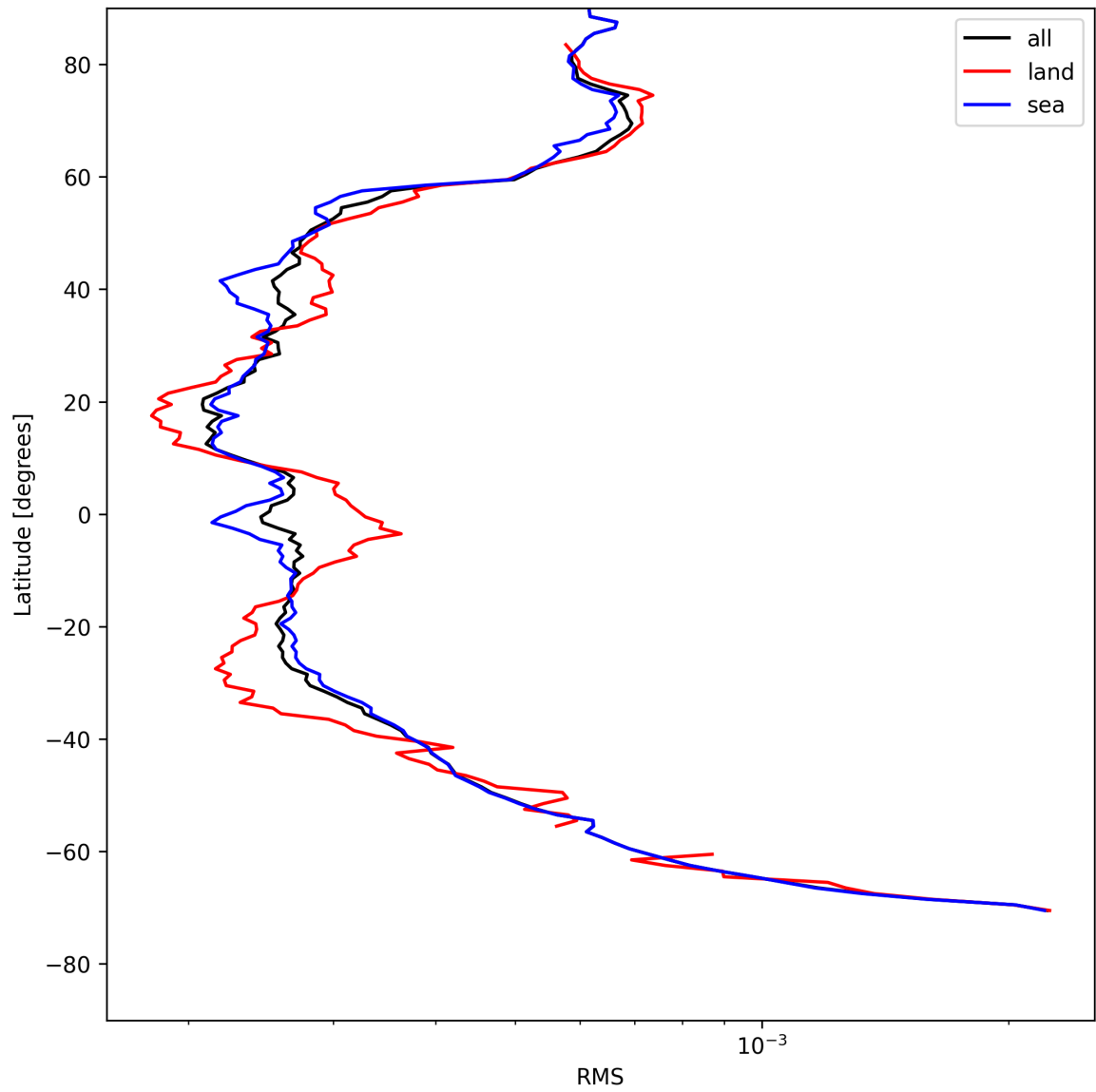
Figure 24: Zonal average of “RMS” for 2025-05-08 to 2025-05-08.
