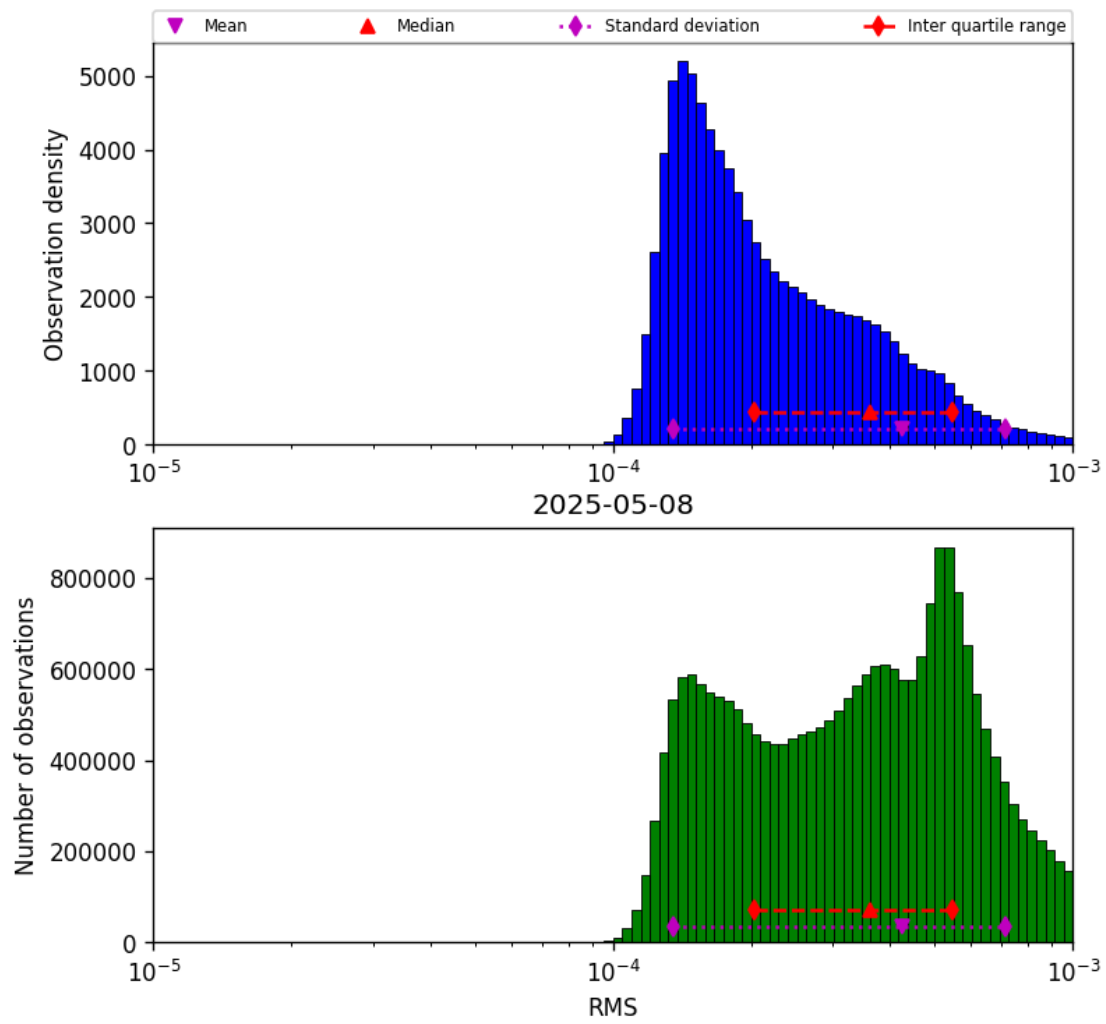
Figure 41: Histogram of “RMS” for 2025-05-08 to 2025-05-08
