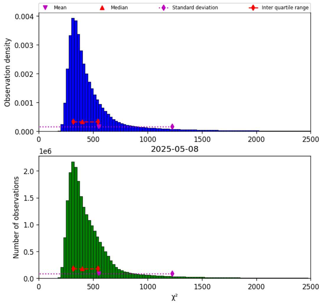
Figure 40: Histogram of “ \chi^2 ” for 2025-05-08 to 2025-05-08
