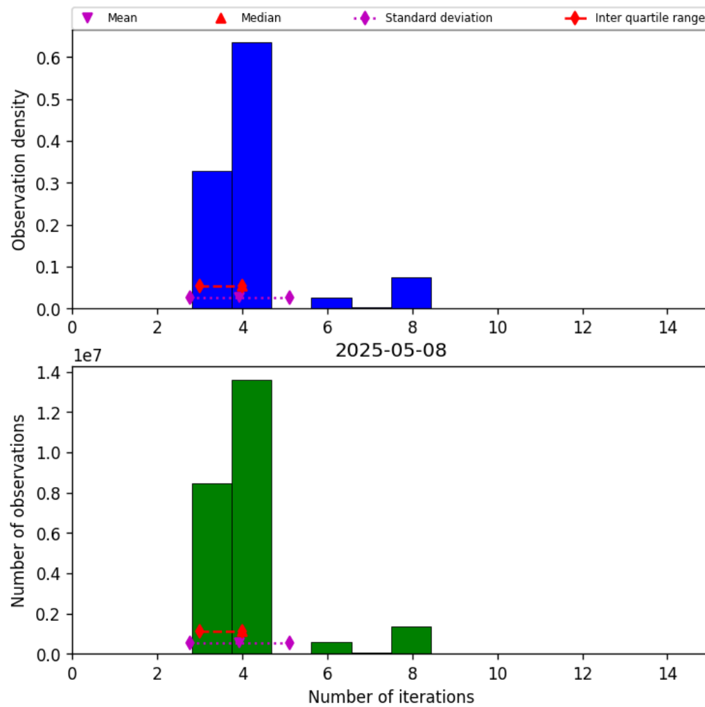
Figure 32: Histogram of “Number of iterations” for 2025-05-08 to 2025-05-08
