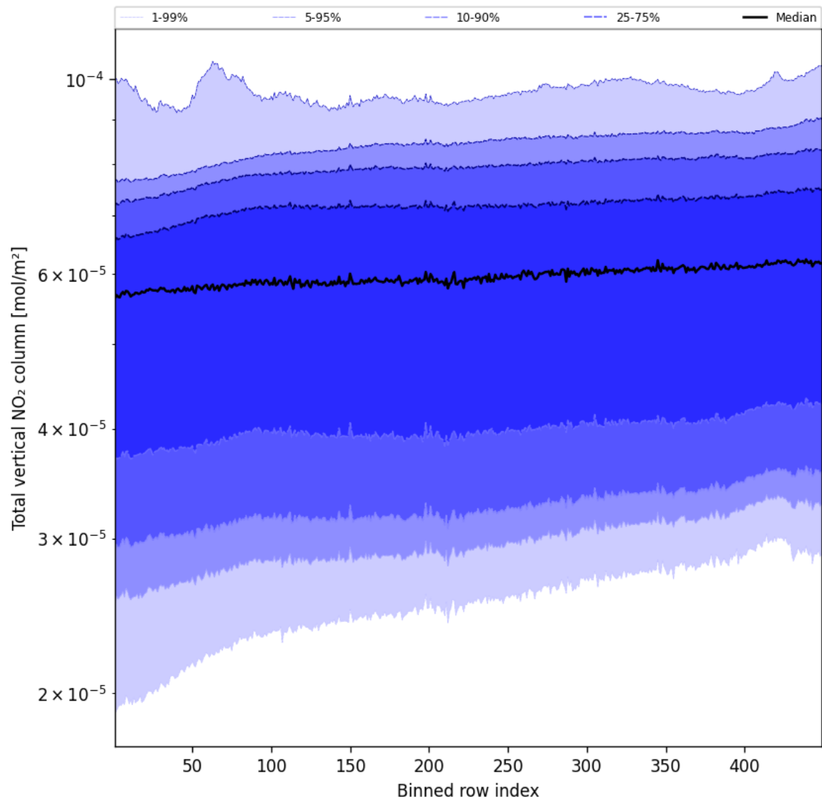
Figure 53: Along track statistics of “Total vertical NO 2 column” for 2025-05-08 to 2025-05-08
