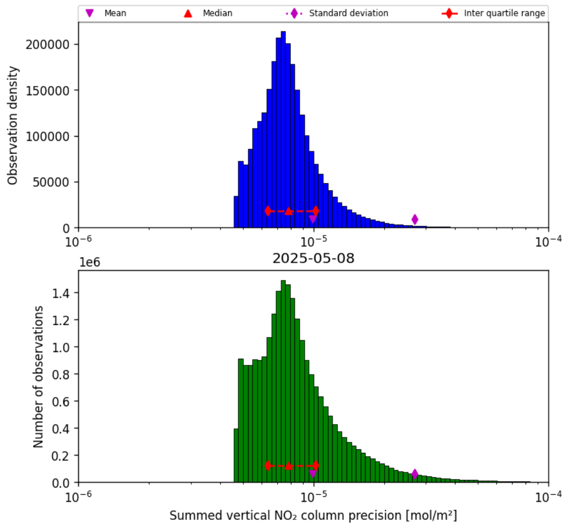
Figure 39: Histogram of "Summed vertical NO 2 column precision" for 2025-05-08 to 2025-05-08
