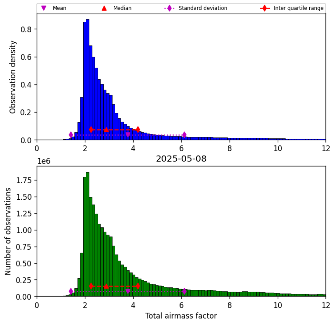
Figure 30: Histogram of “Total airmass factor” for 2025-05-08 to 2025-05-08
