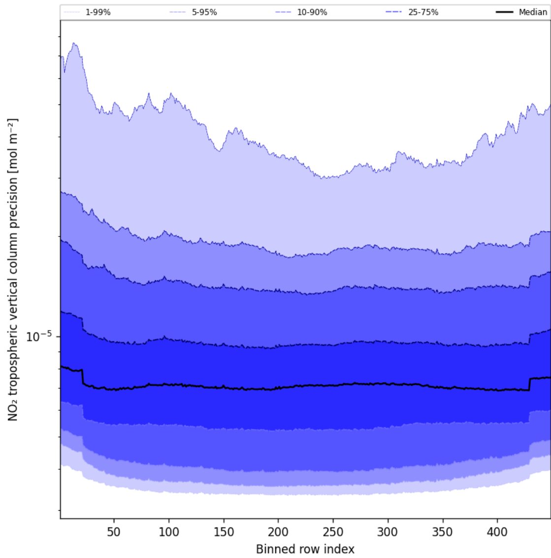
Figure 45: Along track statistics of “NO 2 tropospheric vertical column precision” for 2025-05-08 to 2025-05-08
