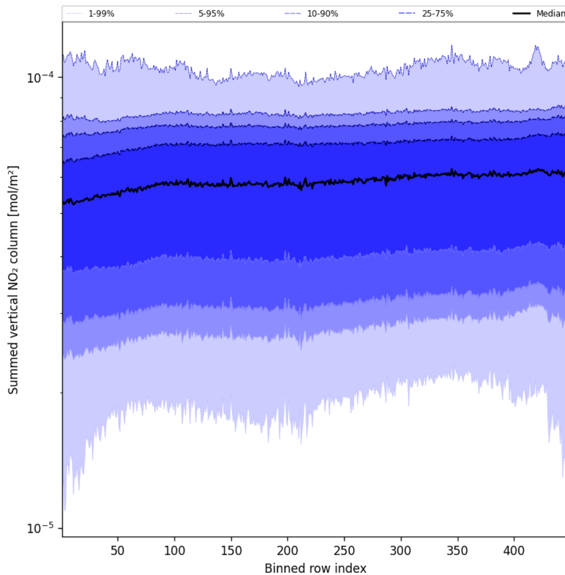
Figure 55: Along track statistics of “Summed vertical NO 2 column” for 2025-05-08 to 2025-05-08
