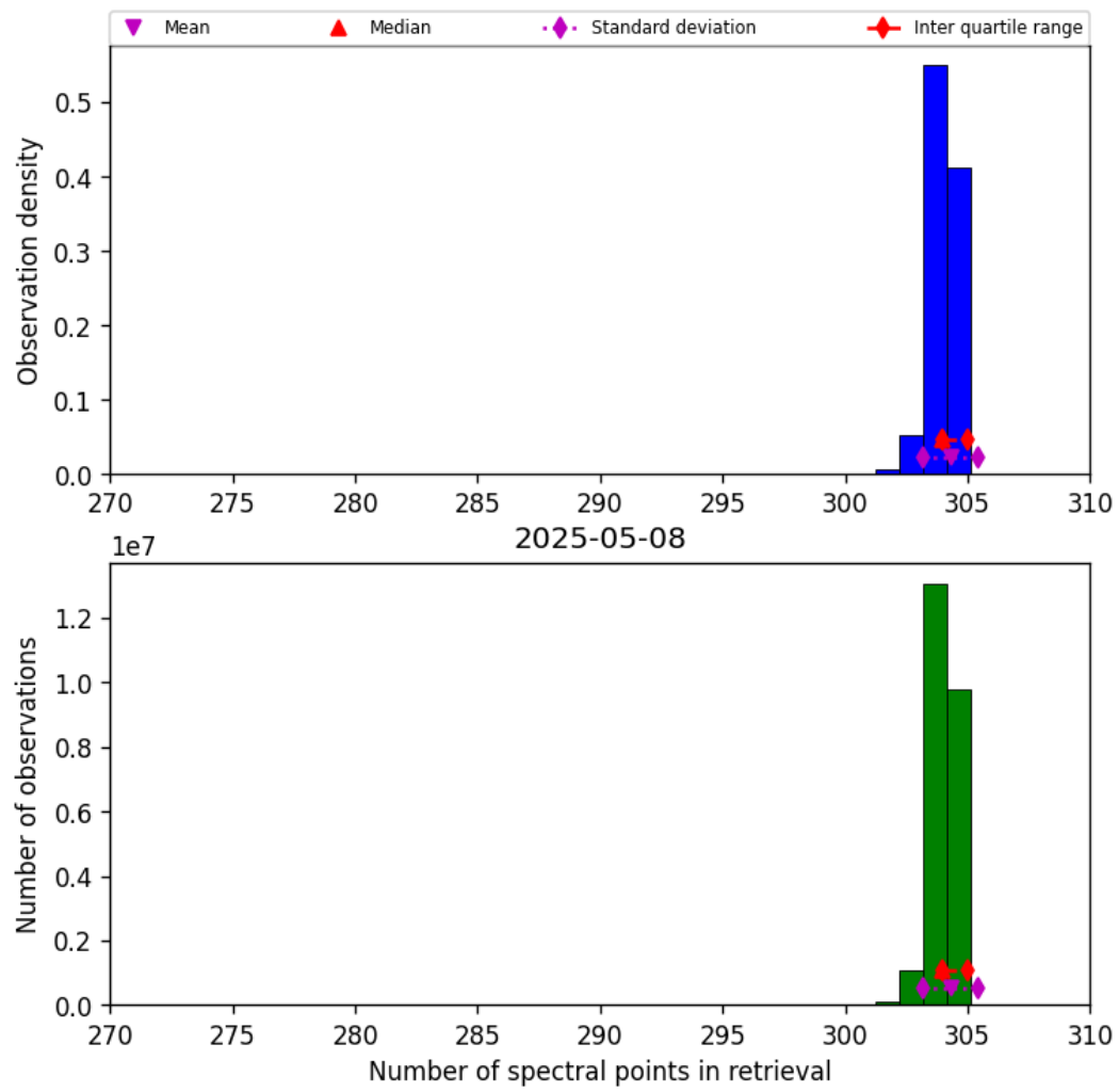
Figure 31: Histogram of “Number of spectral points in retrieval” for 2025-05-08 to 2025-05-08
