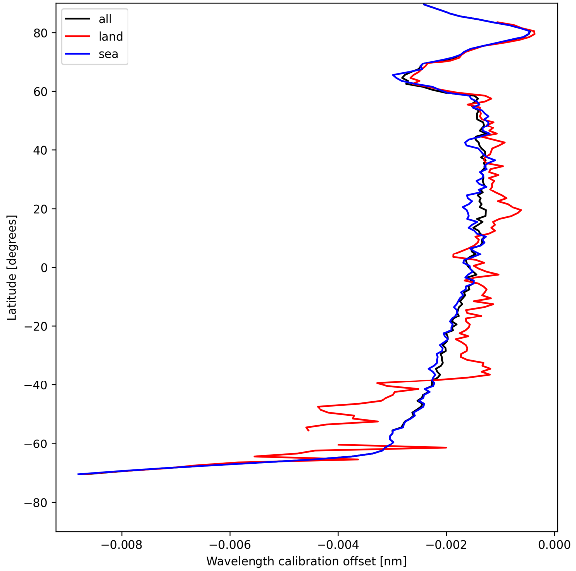
Figure 16: Zonal average of “Wavelength calibration offset” for 2025-05-08 to 2025-05-08.
