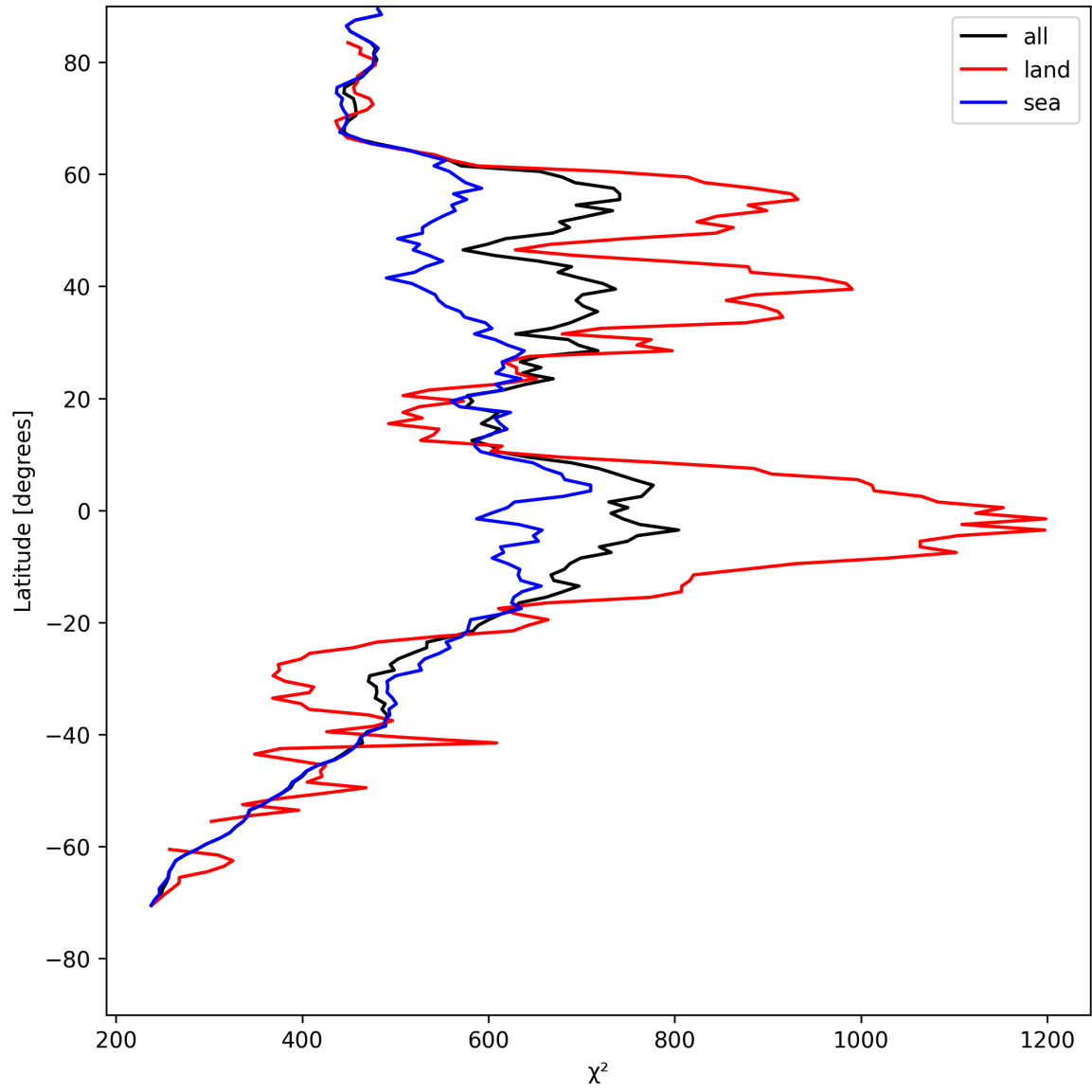
Figure 23: Zonal average of “ \chi^2 ” for 2025-05-08 to 2025-05-08.
