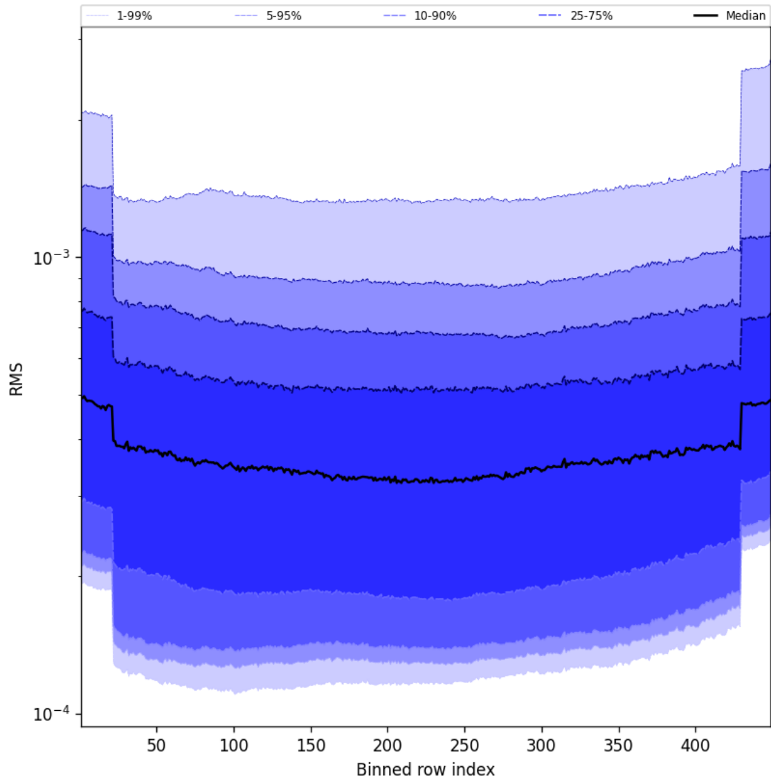
Figure 58: Along track statistics of “RMS” for 2025-05-08 to 2025-05-08
