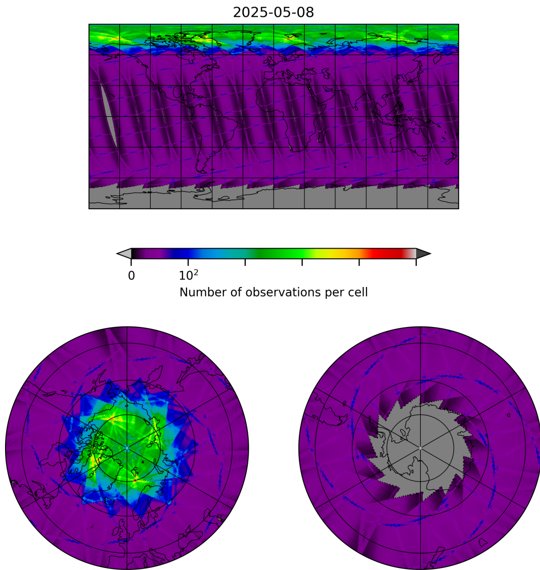
Figure 8: Map of the number of observations for 2025-05-08 to 2025-05-08
