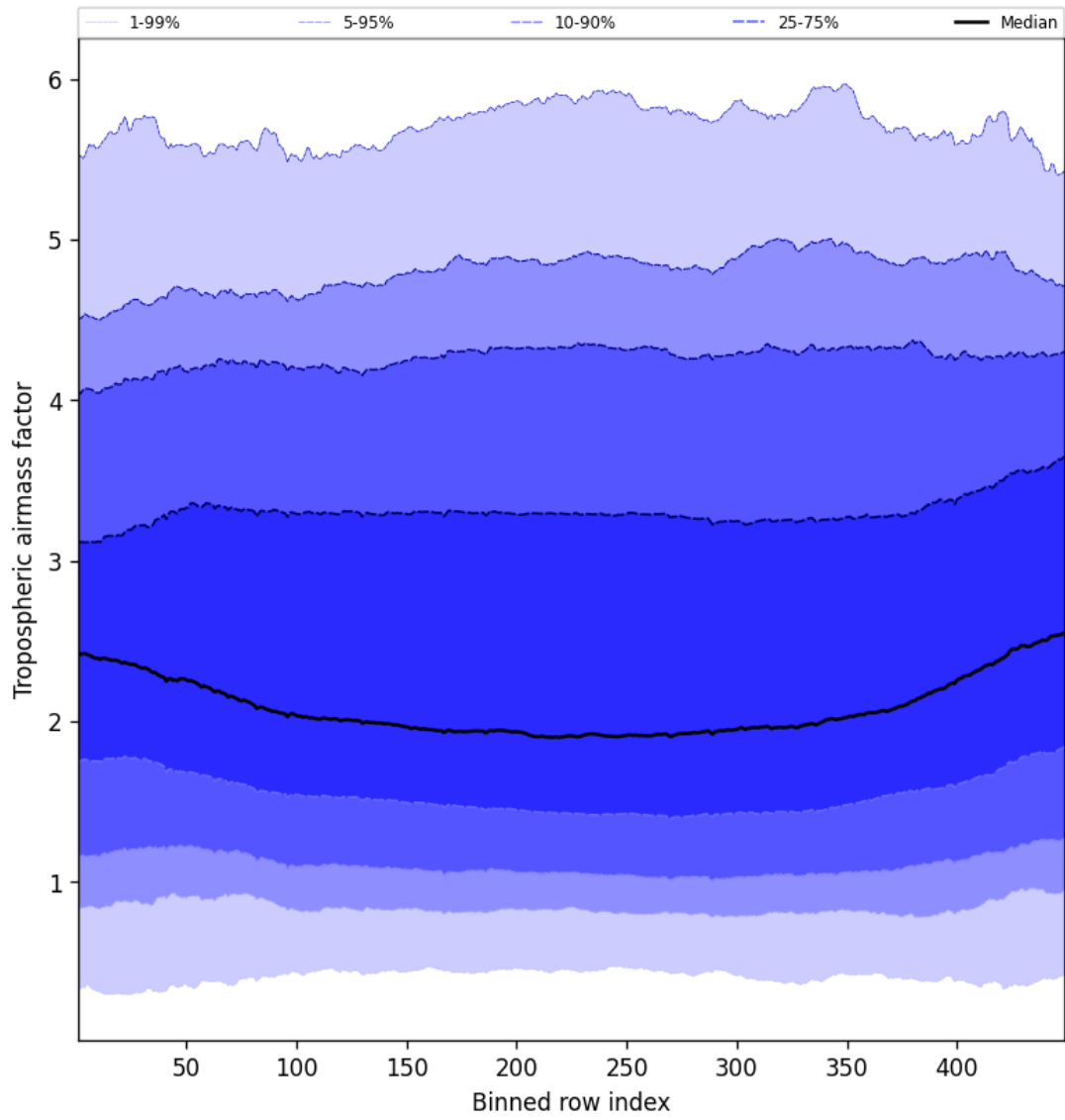
Figure 46: Along track statistics of “Tropospheric airmass factor” for 2025-05-08 to 2025-05-08
