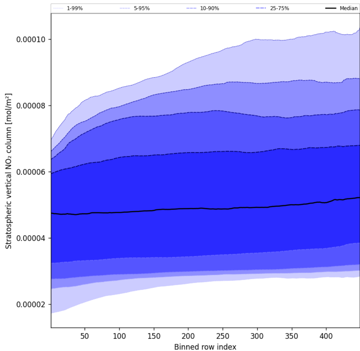
Figure 51: Along track statistics of “Stratospheric vertical NO 2 column” for 2025-05-08 to 2025-05-08
