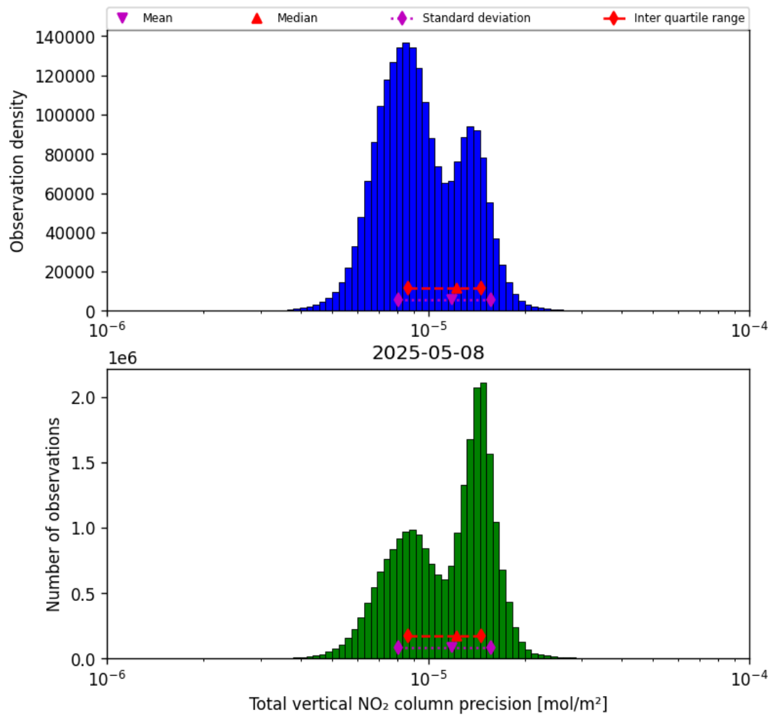
Figure 37: Histogram of "Total vertical NO 2 column precision" for 2025-05-08 to 2025-05-08
