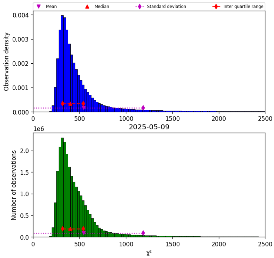
Figure 40: Histogram of “ \chi^2 ” for 2025-05-09 to 2025-05-10
