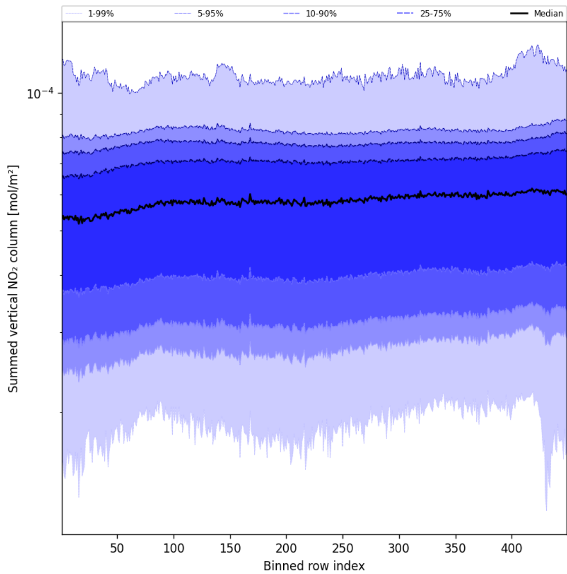
Figure 55: Along track statistics of “Summed vertical NO 2 column” for 2025-05-09 to 2025-05-10
