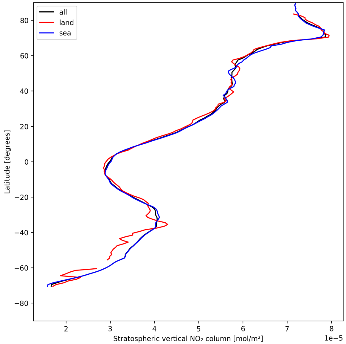
Figure 17: Zonal average of “Stratospheric vertical NO 2 column” for 2025-05-09 to 2025-05-10.
