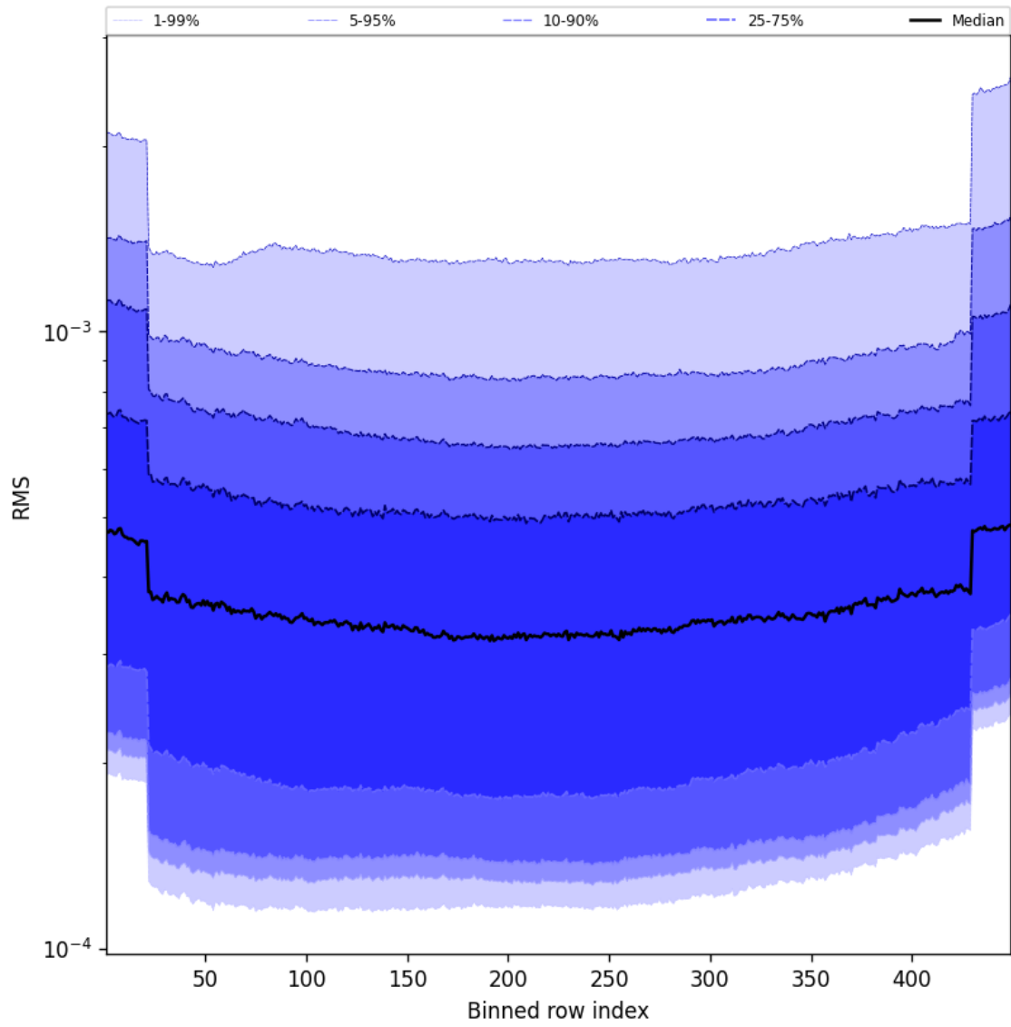
Figure 58: Along track statistics of “RMS” for 2025-05-09 to 2025-05-10
