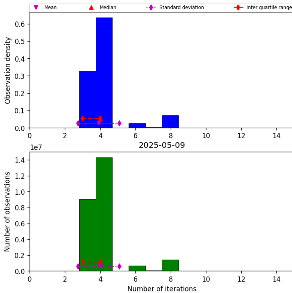
Figure 32: Histogram of “Number of iterations” for 2025-05-09 to 2025-05-10
