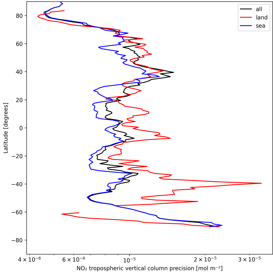
Figure 11: Zonal average of “NO 2 tropospheric vertical column precision” for 2025-05-09 to 2025-05-10.
