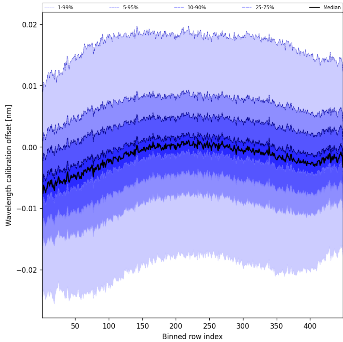
Figure 50: Along track statistics of “Wavelength calibration offset” for 2025-05-09 to 2025-05-10
