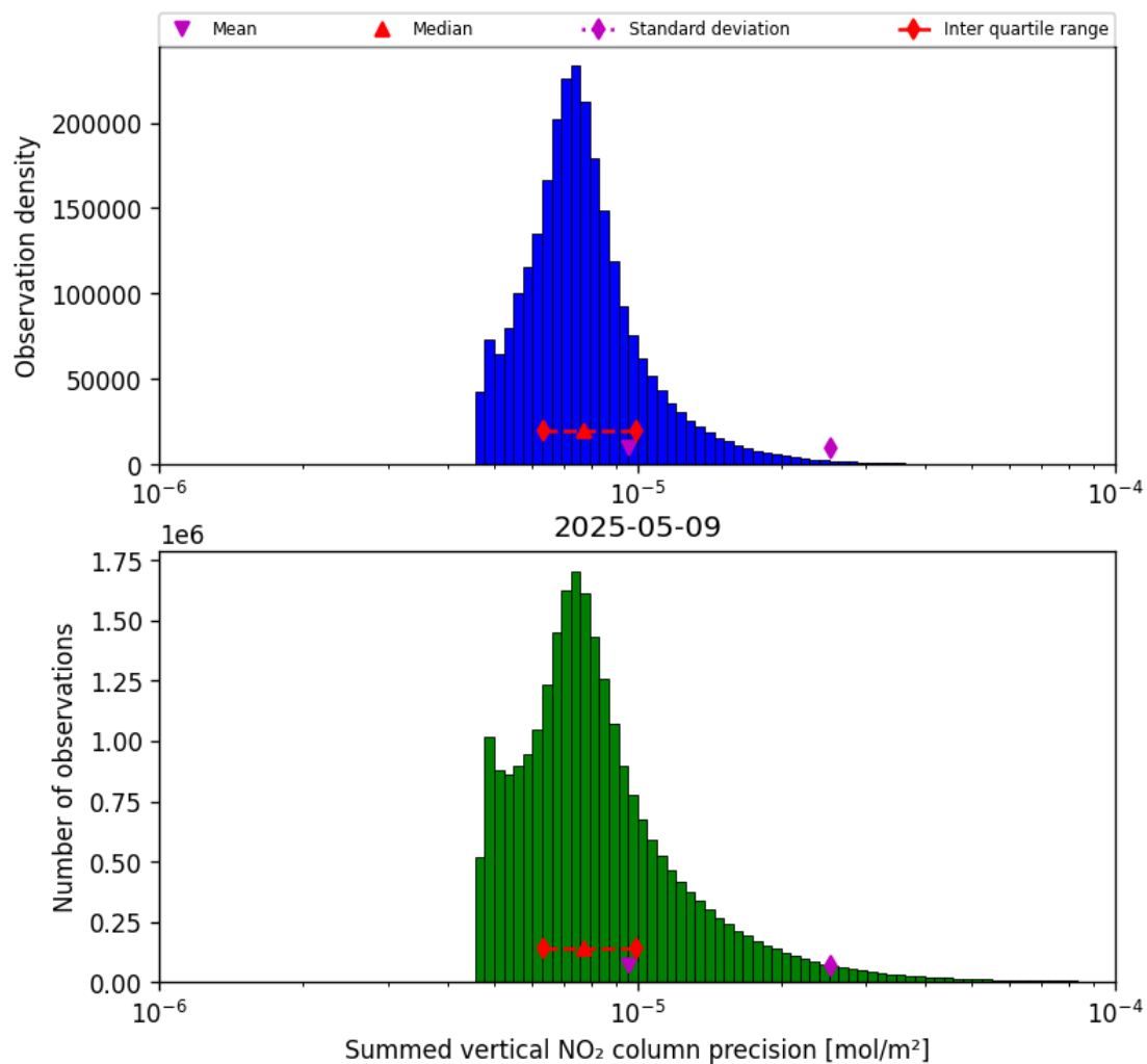
Figure 39: Histogram of “Summed vertical NO 2 column precision” for 2025-05-09 to 2025-05-10
