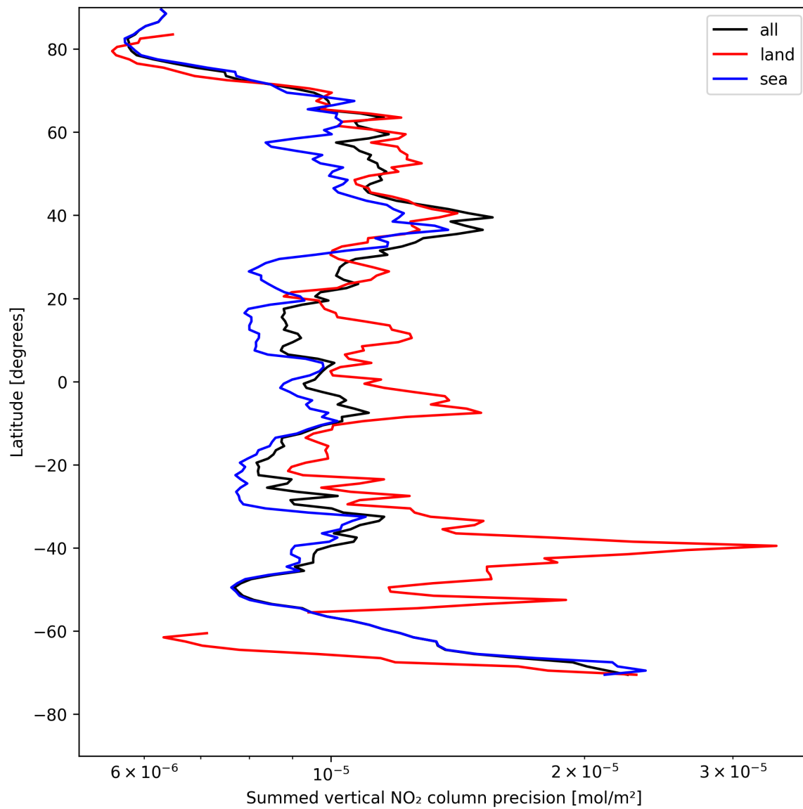
Figure 22: Zonal average of “Summed vertical NO 2 column precision” for 2025-05-09 to 2025-05-10.
