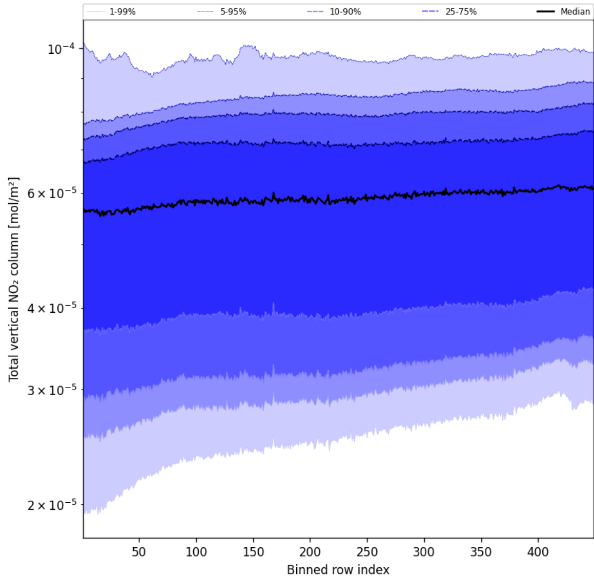
Figure 53: Along track statistics of “Total vertical NO 2 column” for 2025-05-09 to 2025-05-10
