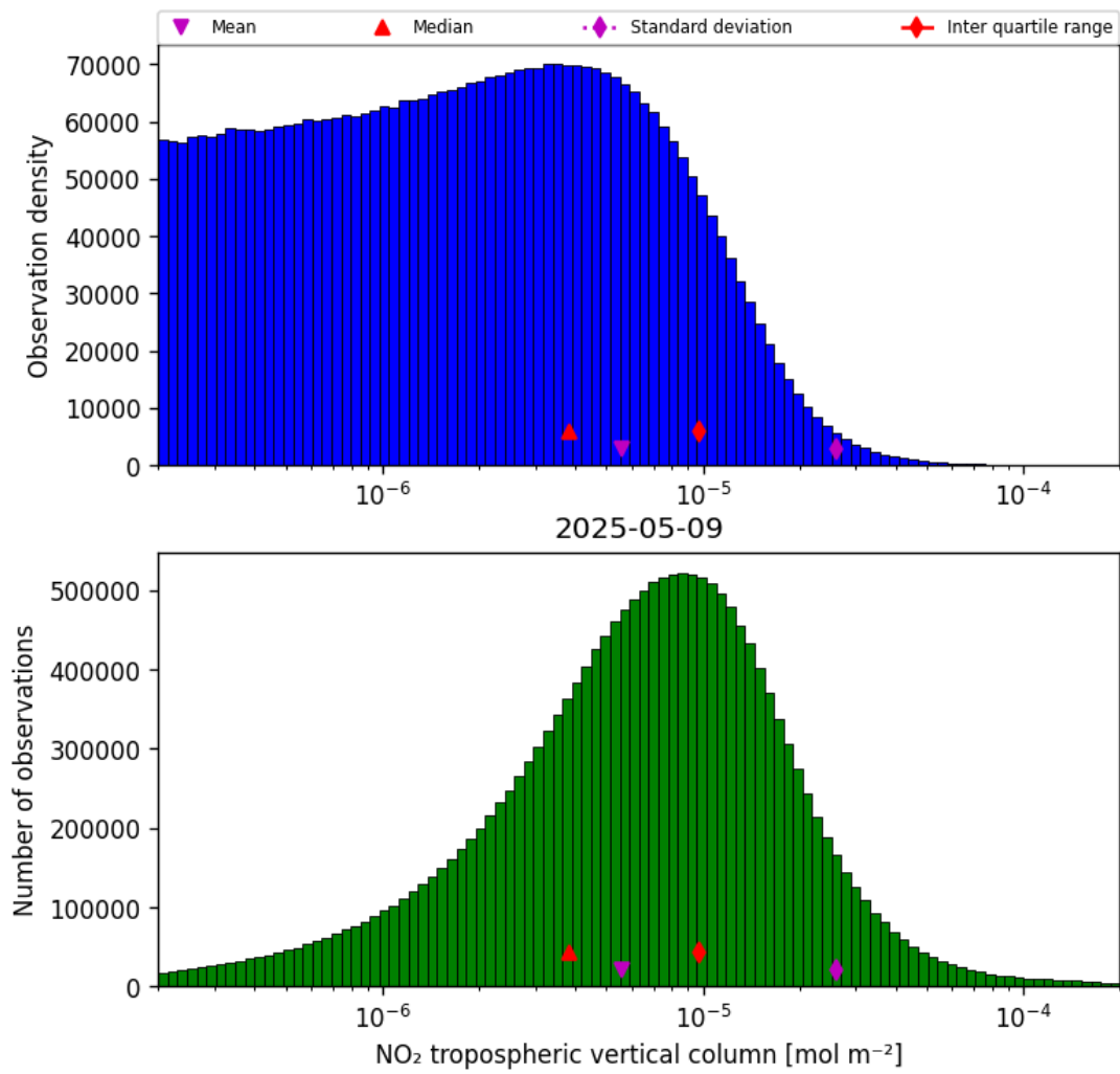
Figure 27: Histogram of “NO 2 tropospheric vertical column” for 2025-05-09 to 2025-05-10
