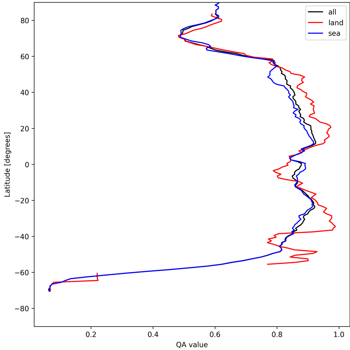
Figure 9: Zonal average of “QA value” for 2025-05-09 to 2025-05-10.
