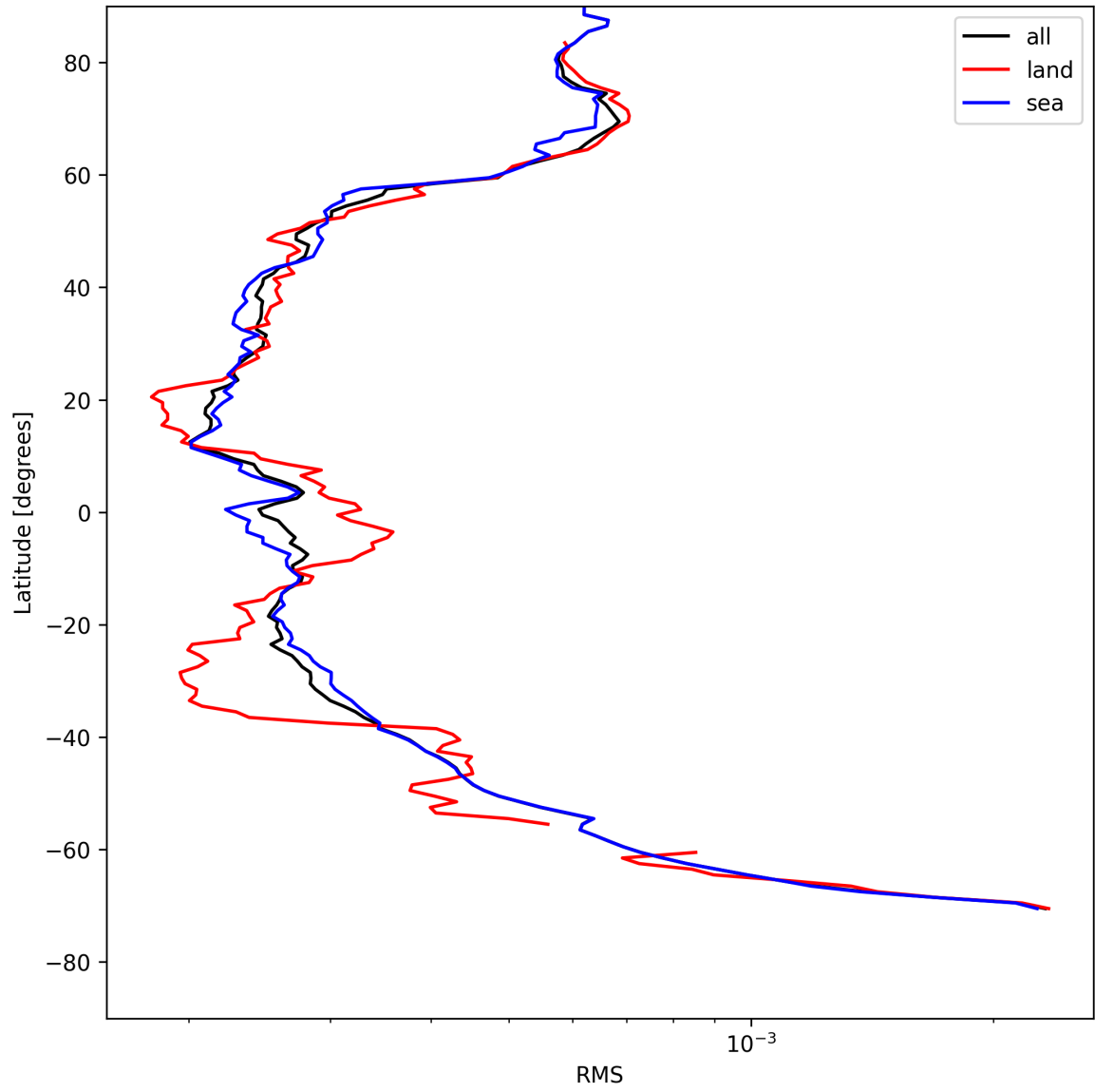
Figure 24: Zonal average of “RMS” for 2025-05-09 to 2025-05-10.
