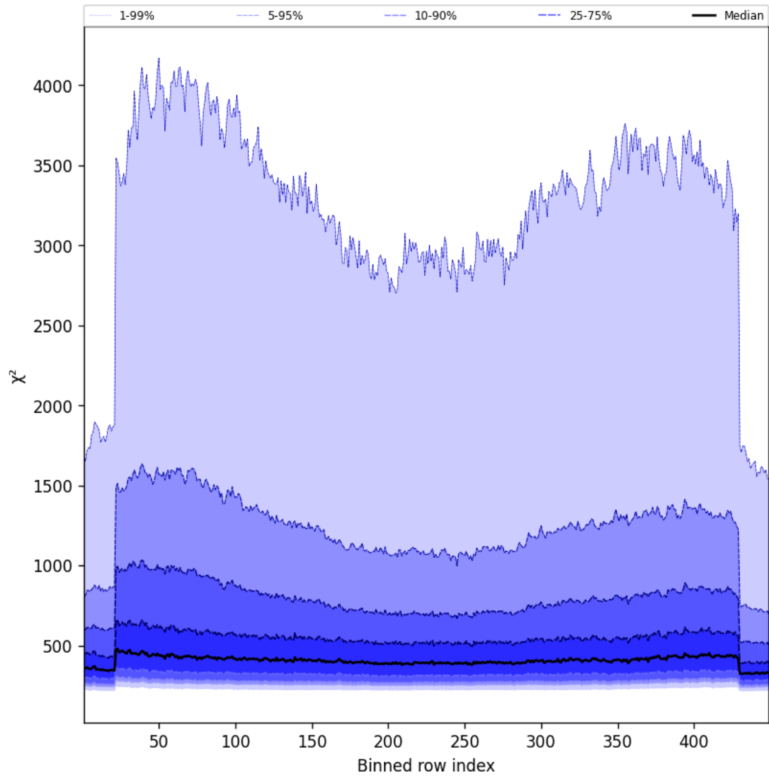
Figure 57: Along track statistics of “ \chi^2 ” for 2025-05-09 to 2025-05-10
