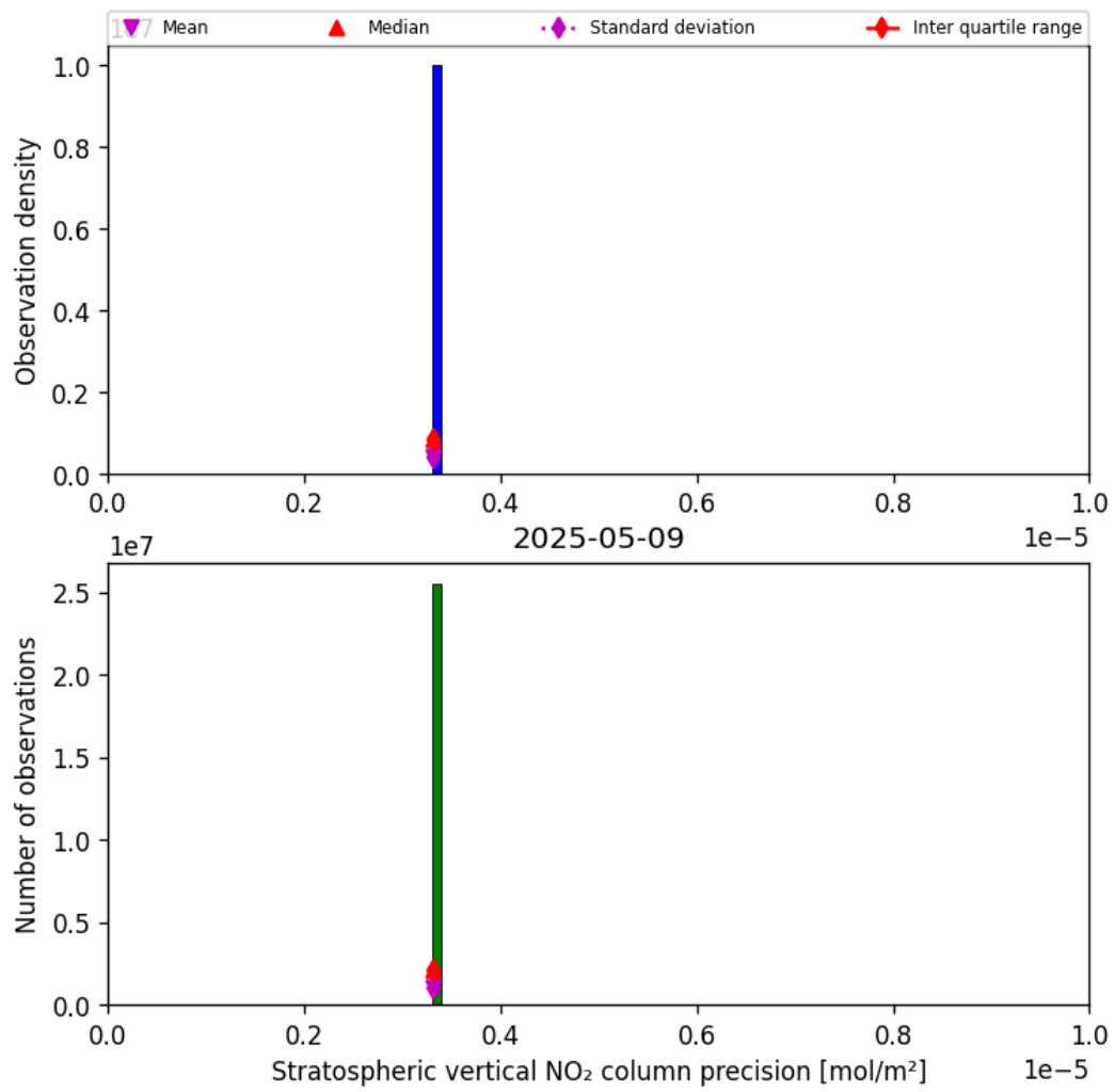
Figure 35: Histogram of “Stratospheric vertical NO 2 column precision” for 2025-05-09 to 2025-05-10
