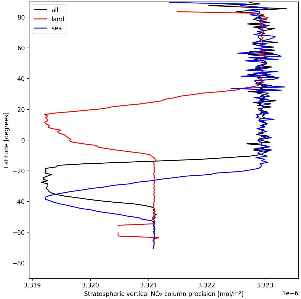
Figure 18: Zonal average of “Stratospheric vertical NO 2 column precision” for 2025-05-09 to 2025-05-10.
