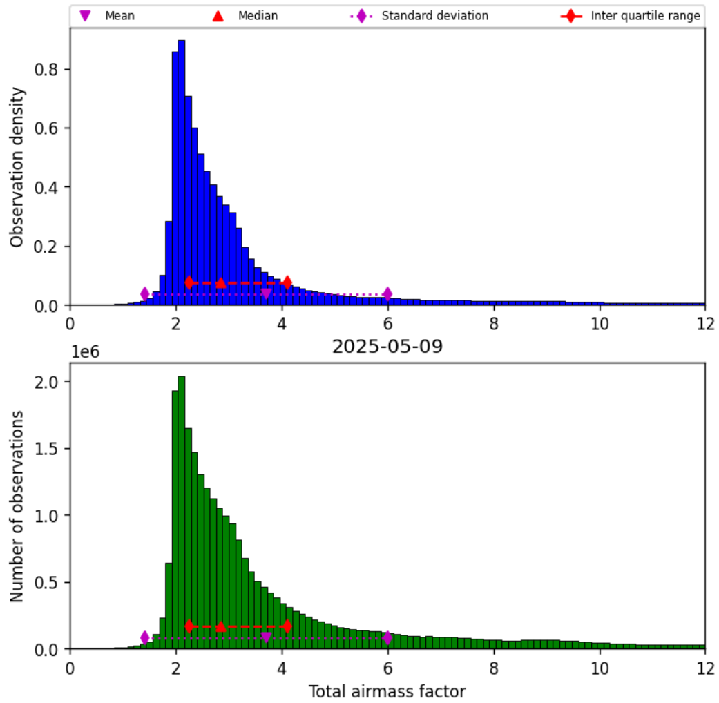
Figure 30: Histogram of “Total airmass factor” for 2025-05-09 to 2025-05-10
