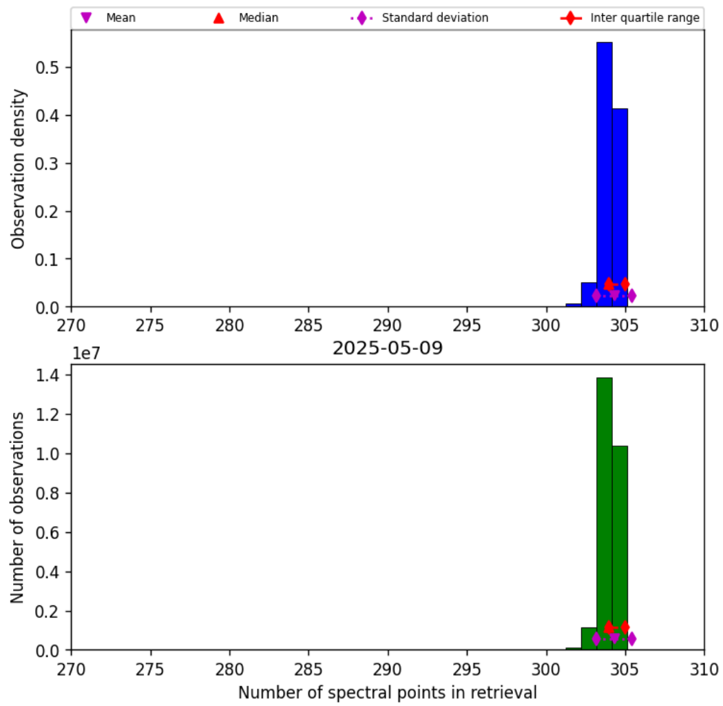
Figure 31: Histogram of “Number of spectral points in retrieval” for 2025-05-09 to 2025-05-10
