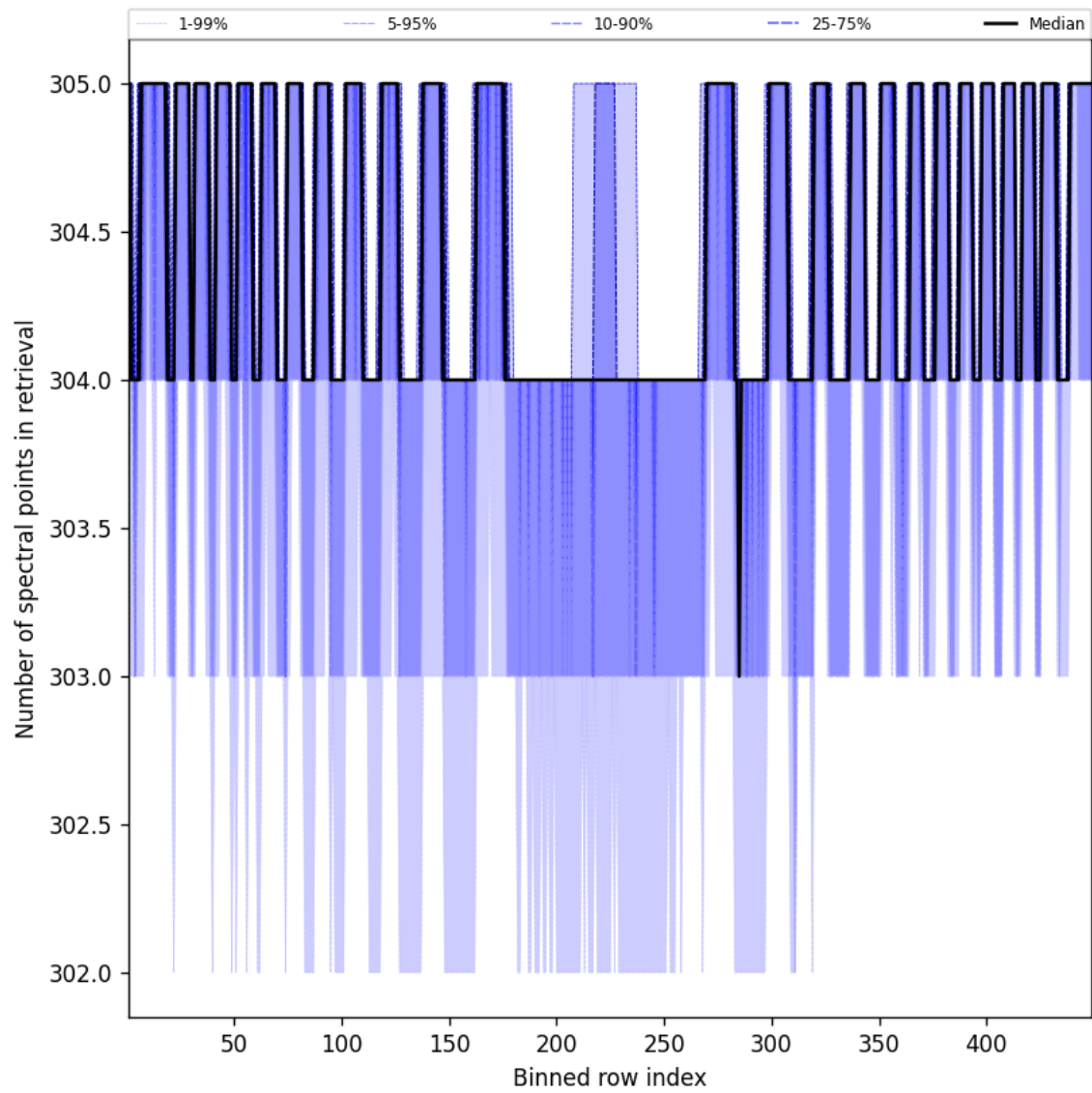
Figure 48: Along track statistics of “Number of spectral points in retrieval” for 2025-05-09 to 2025-05-10
