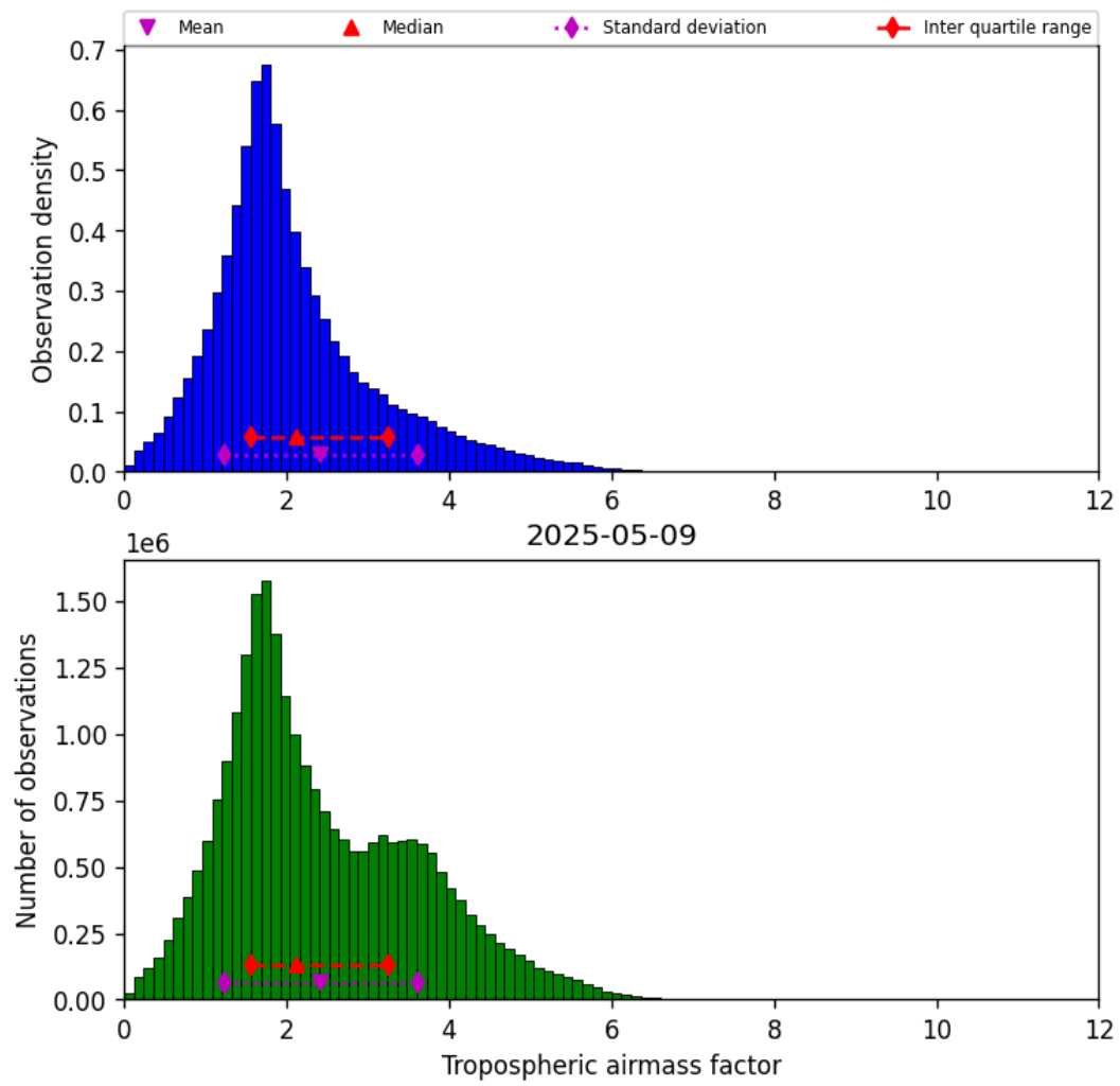
Figure 29: Histogram of “Tropospheric airmass factor” for 2025-05-09 to 2025-05-10
