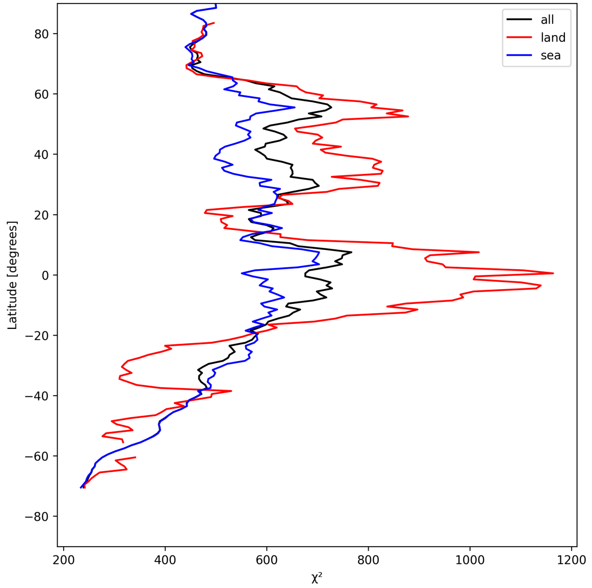
Figure 23: Zonal average of “ \chi^2 ” for 2025-05-09 to 2025-05-10.
