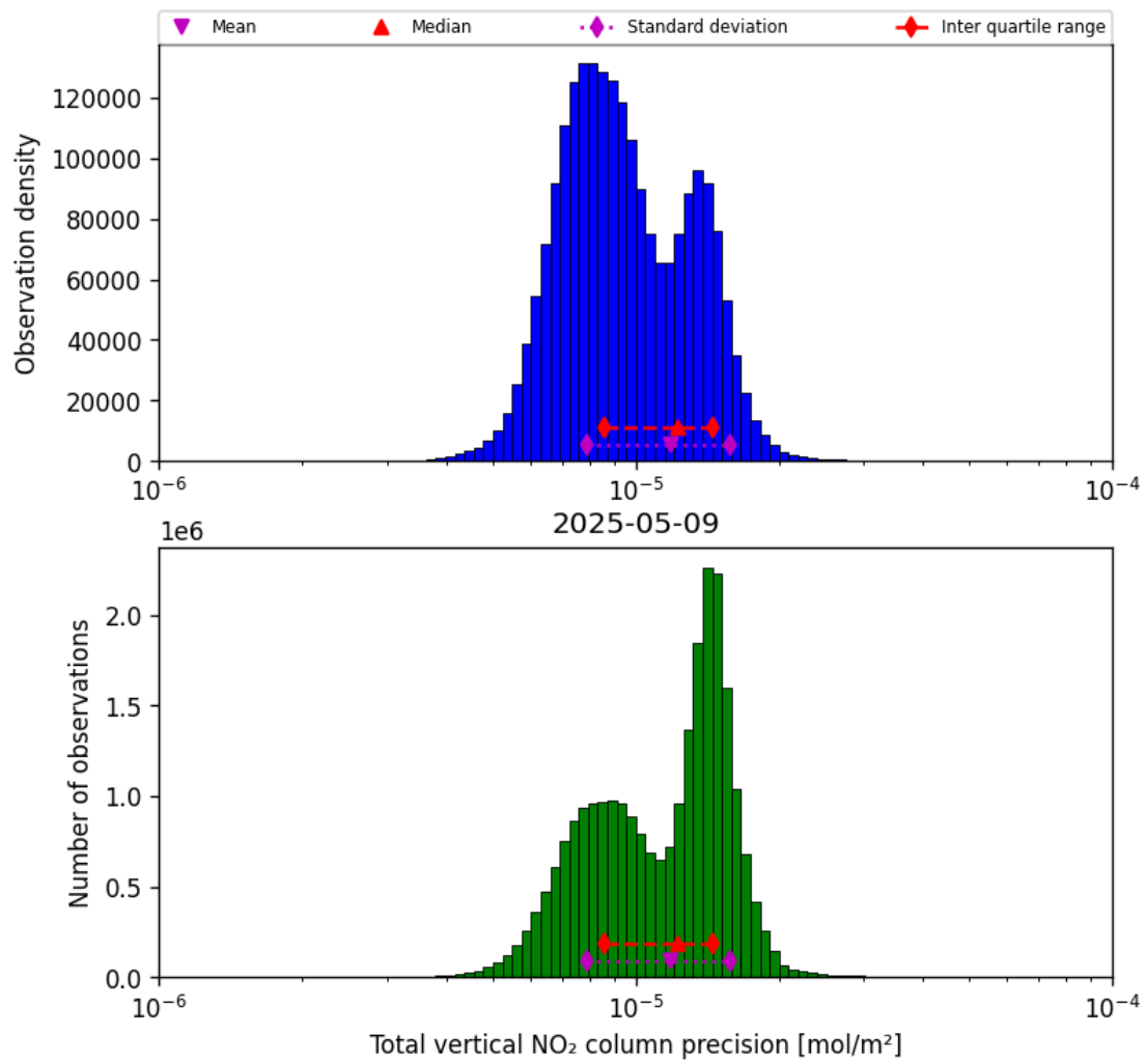
Figure 37: Histogram of “Total vertical NO 2 column precision” for 2025-05-09 to 2025-05-10
