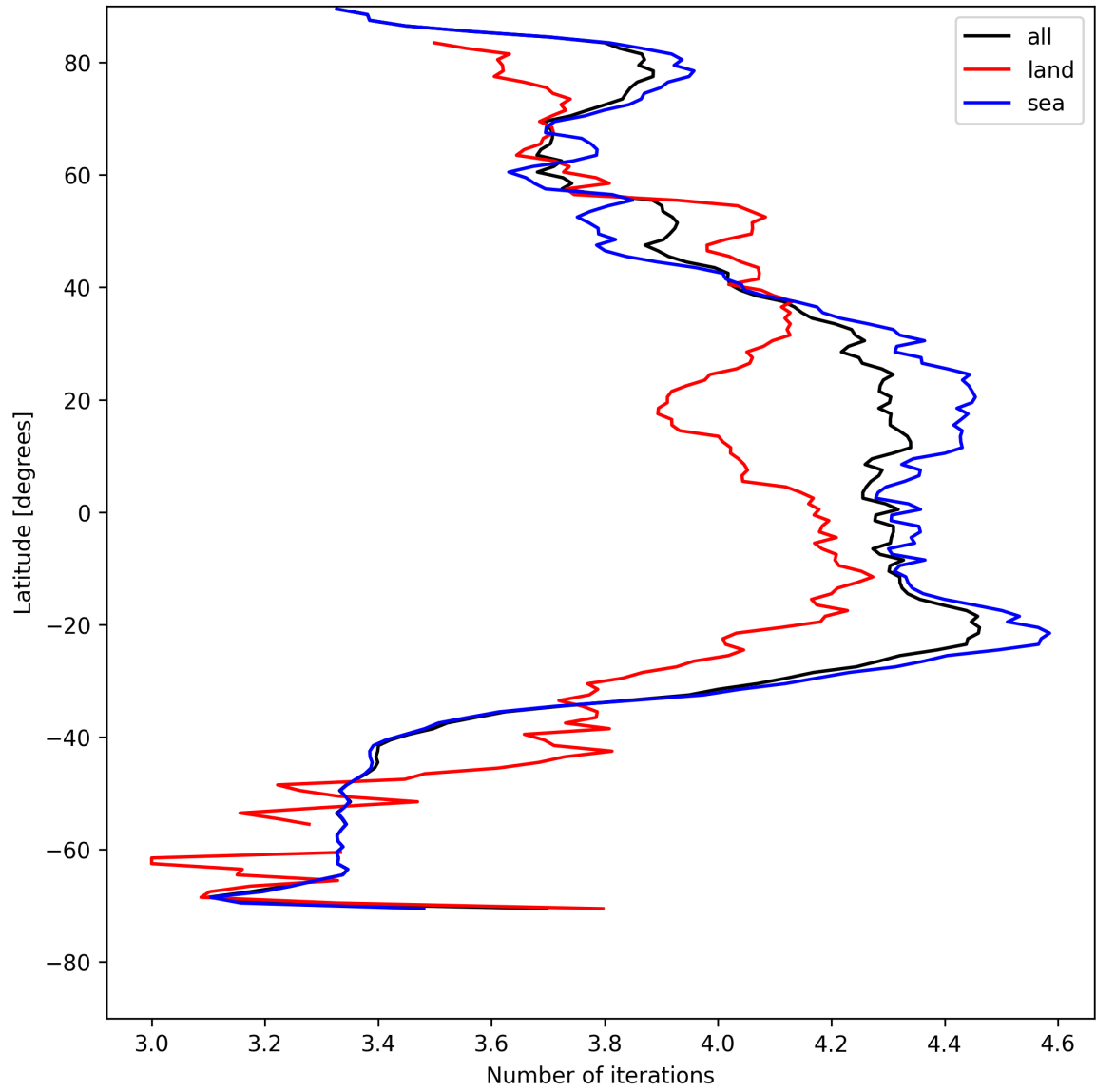
Figure 15: Zonal average of “Number of iterations” for 2025-05-09 to 2025-05-10.
