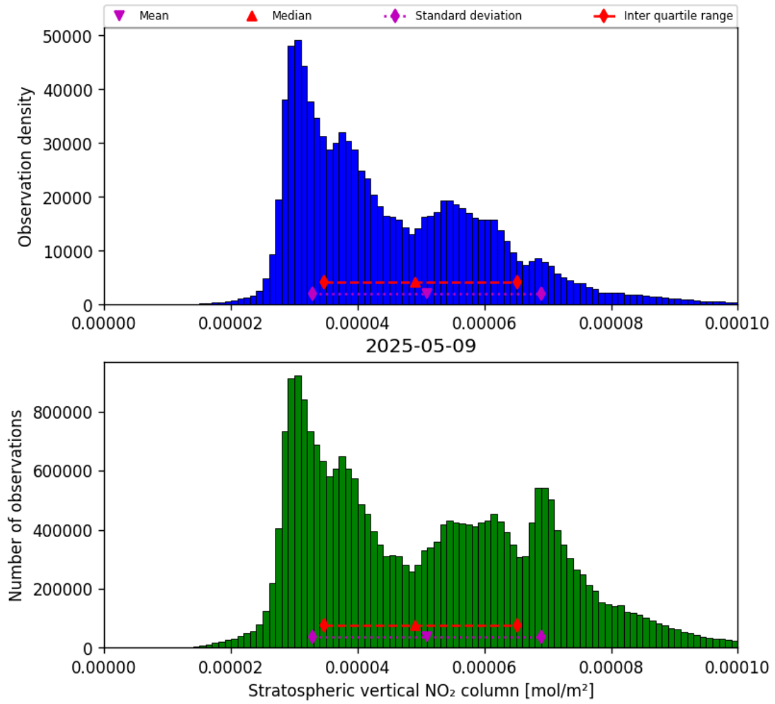
Figure 34: Histogram of “Stratospheric vertical NO 2 column” for 2025-05-09 to 2025-05-10
