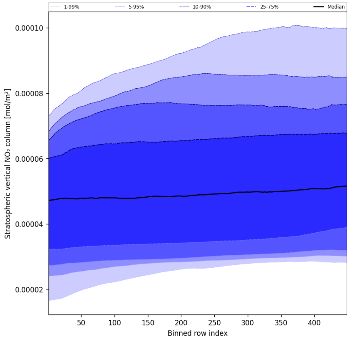
Figure 51: Along track statistics of “Stratospheric vertical NO 2 column” for 2025-05-09 to 2025-05-10
