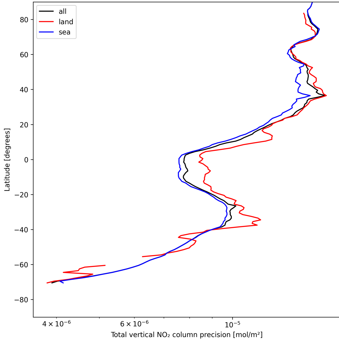
Figure 20: Zonal average of “Total vertical NO 2 column precision” for 2025-05-09 to 2025-05-10.
