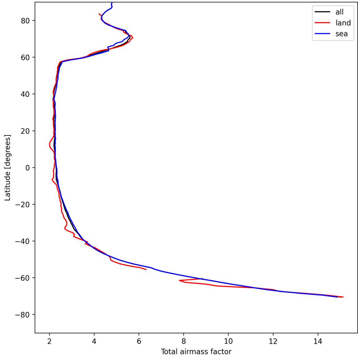
Figure 13: Zonal average of “Total airmass factor” for 2025-05-09 to 2025-05-10.
