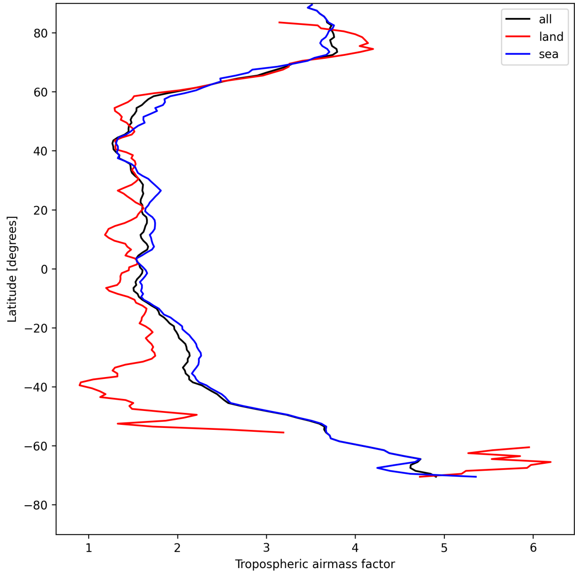
Figure 12: Zonal average of “Tropospheric airmass factor” for 2025-05-09 to 2025-05-10.
