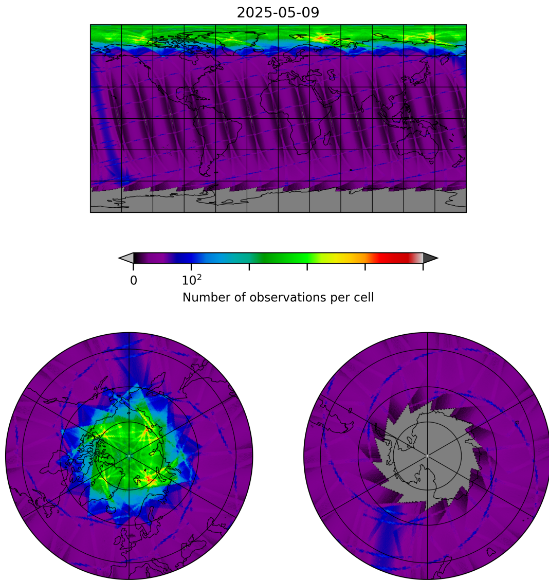
Figure 8: Map of the number of observations for 2025-05-09 to 2025-05-10
