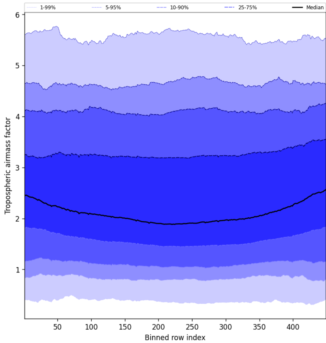
Figure 46: Along track statistics of “Tropospheric airmass factor” for 2025-05-09 to 2025-05-10
