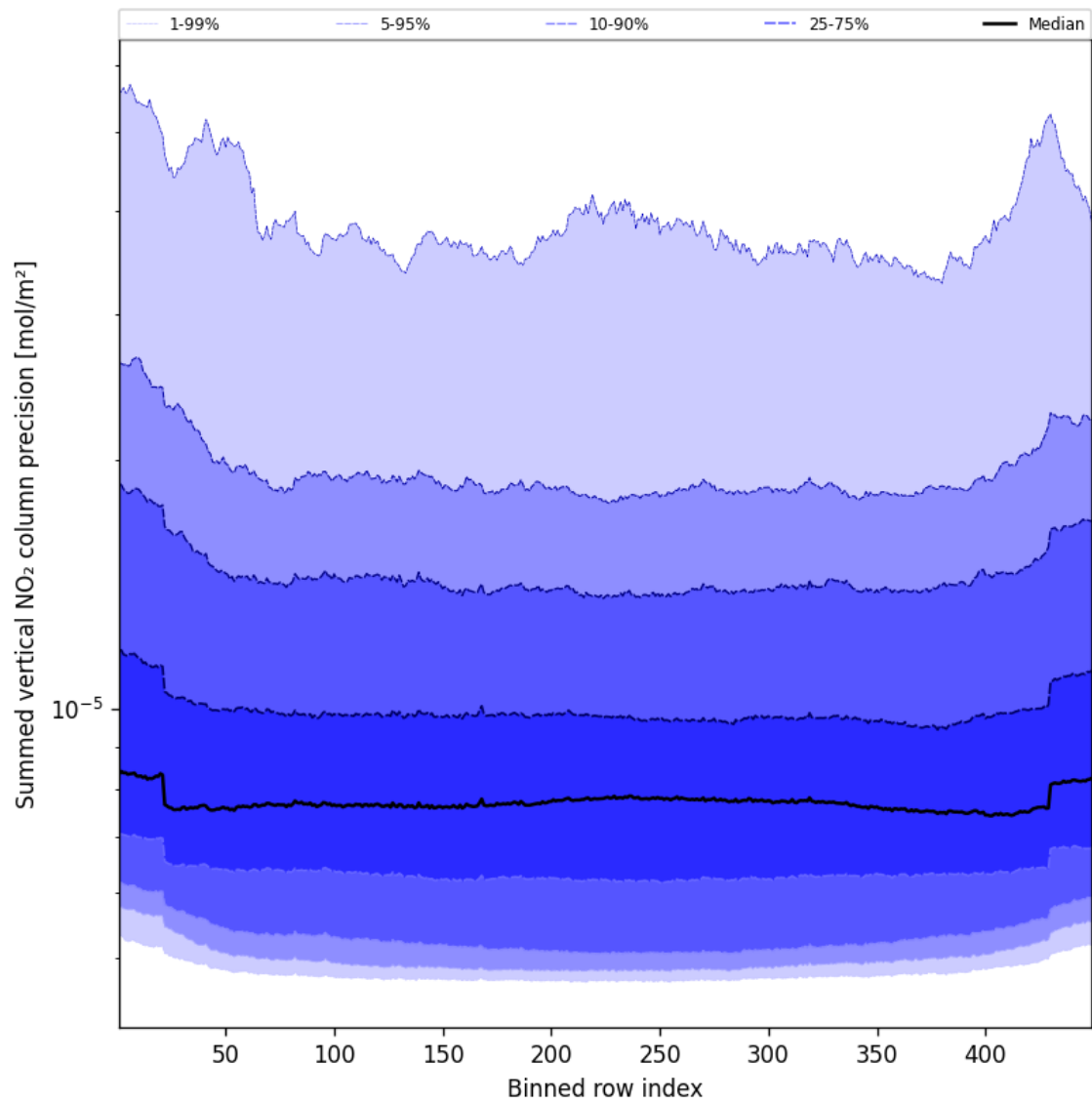
Figure 56: Along track statistics of “Summed vertical NO 2 column precision” for 2025-05-09 to 2025-05-10
