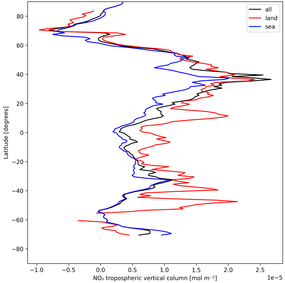
Figure 10: Zonal average of “NO 2 tropospheric vertical column” for 2025-05-09 to 2025-05-10.
