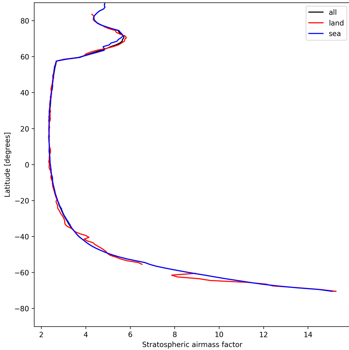
Figure 25: Zonal average of “Stratospheric air mass factor” for 2025-05-09 to 2025-05-10.
