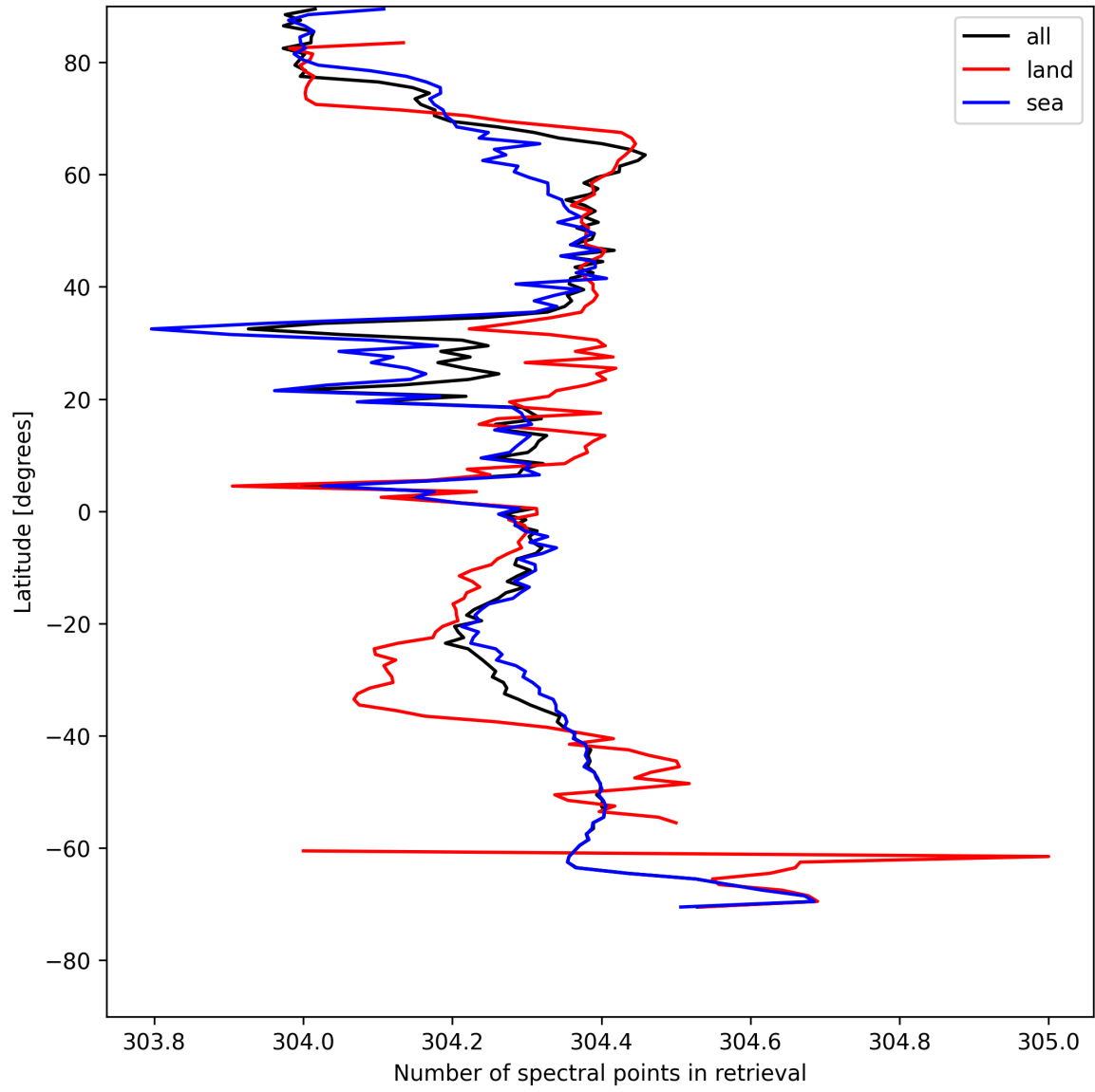
Figure 14: Zonal average of “Number of spectral points in retrieval” for 2025-05-09 to 2025-05-10.
