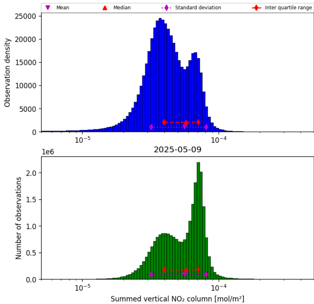
Figure 38: Histogram of “Summed vertical NO 2 column” for 2025-05-09 to 2025-05-10
