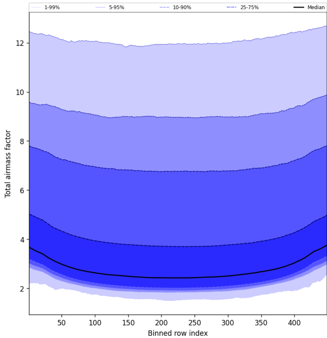
Figure 47: Along track statistics of “Total airmass factor” for 2025-05-09 to 2025-05-10
