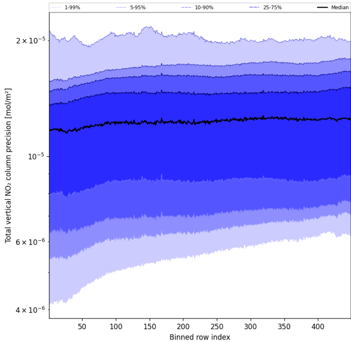
Figure 54: Along track statistics of “Total vertical NO 2 column precision” for 2025-05-09 to 2025-05-10
