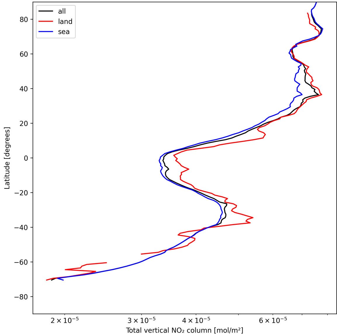
Figure 19: Zonal average of “Total vertical NO 2 column” for 2025-05-09 to 2025-05-10.
