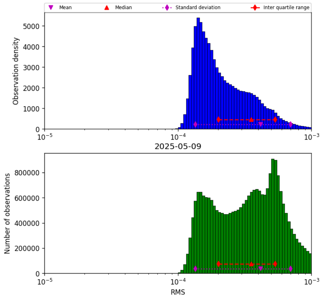
Figure 41: Histogram of “RMS” for 2025-05-09 to 2025-05-10
