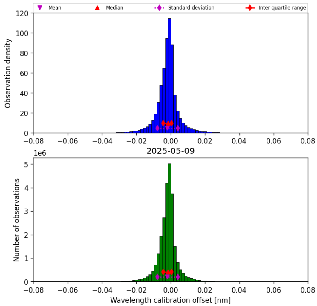
Figure 33: Histogram of “Wavelength calibration offset” for 2025-05-09 to 2025-05-10
