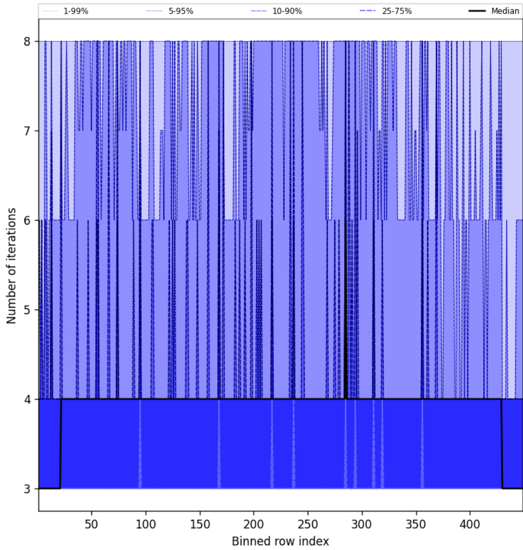
Figure 49: Along track statistics of “Number of iterations” for 2025-05-09 to 2025-05-10
