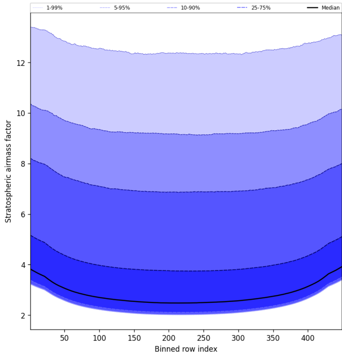
Figure 59: Along track statistics of “Stratospheric airmass factor” for 2025-05-09 to 2025-05-10
