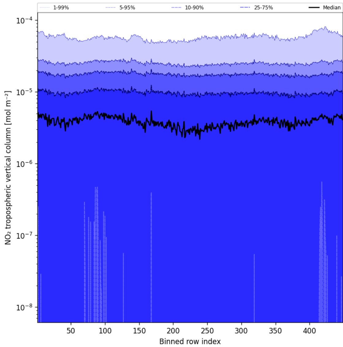
Figure 44: Along track statistics of “NO 2 tropospheric vertical column” for 2025-05-09 to 2025-05-10
