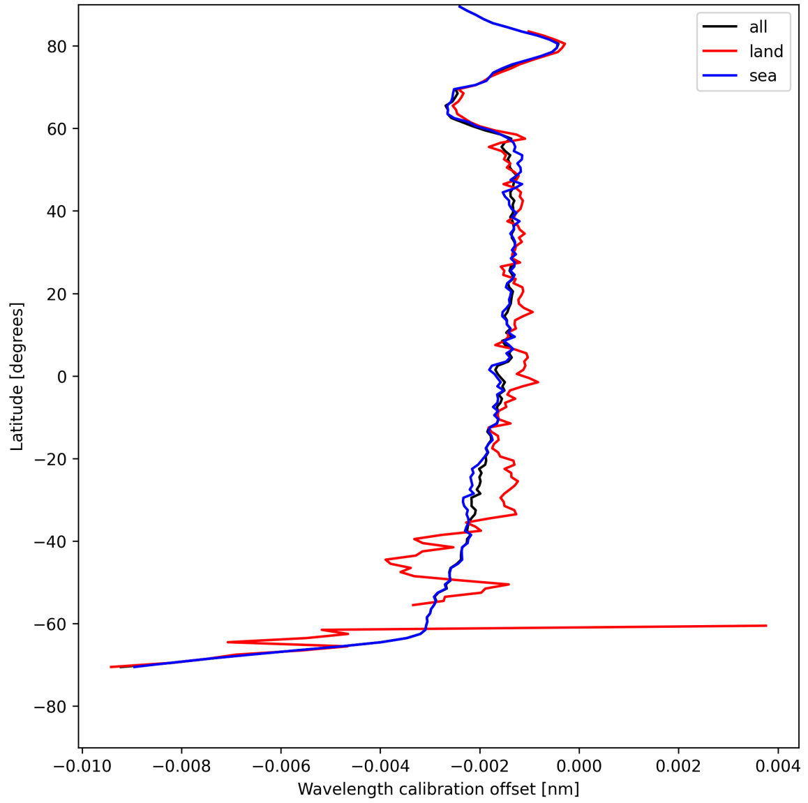
Figure 16: Zonal average of “Wavelength calibration offset” for 2025-05-09 to 2025-05-10.
