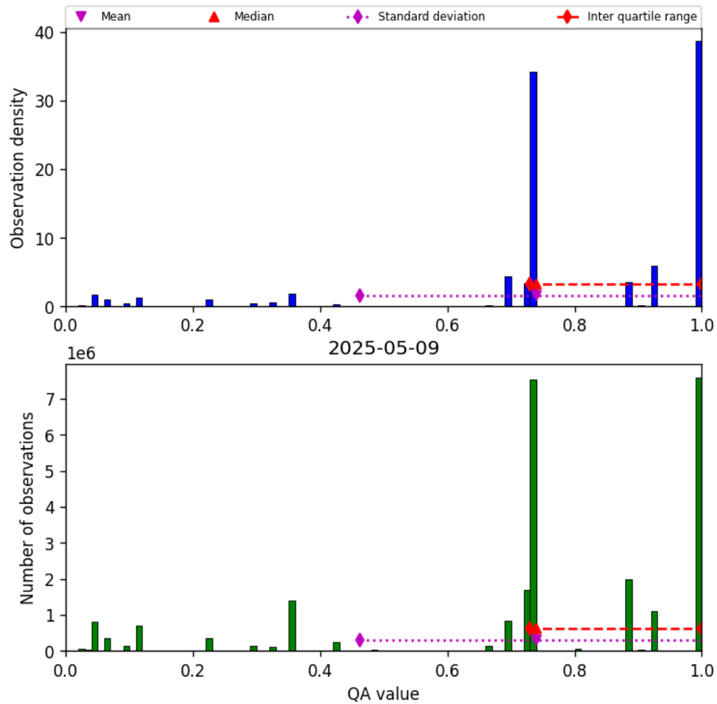
Figure 26: Histogram of “QA value” for 2025-05-09 to 2025-05-10
