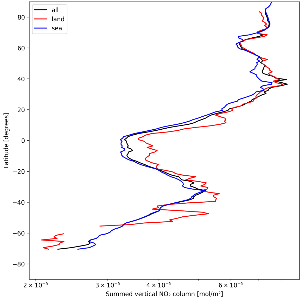
Figure 21: Zonal average of “Summed vertical NO 2 column” for 2025-05-09 to 2025-05-10.
