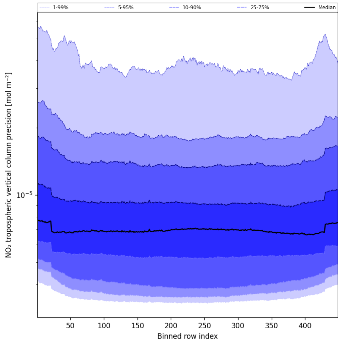
Figure 45: Along track statistics of “NO 2 tropospheric vertical column precision” for 2025-05-09 to 2025-05-10
