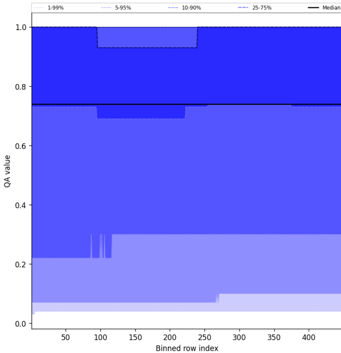
Figure 43: Along track statistics of “QA value” for 2025-05-09 to 2025-05-10
