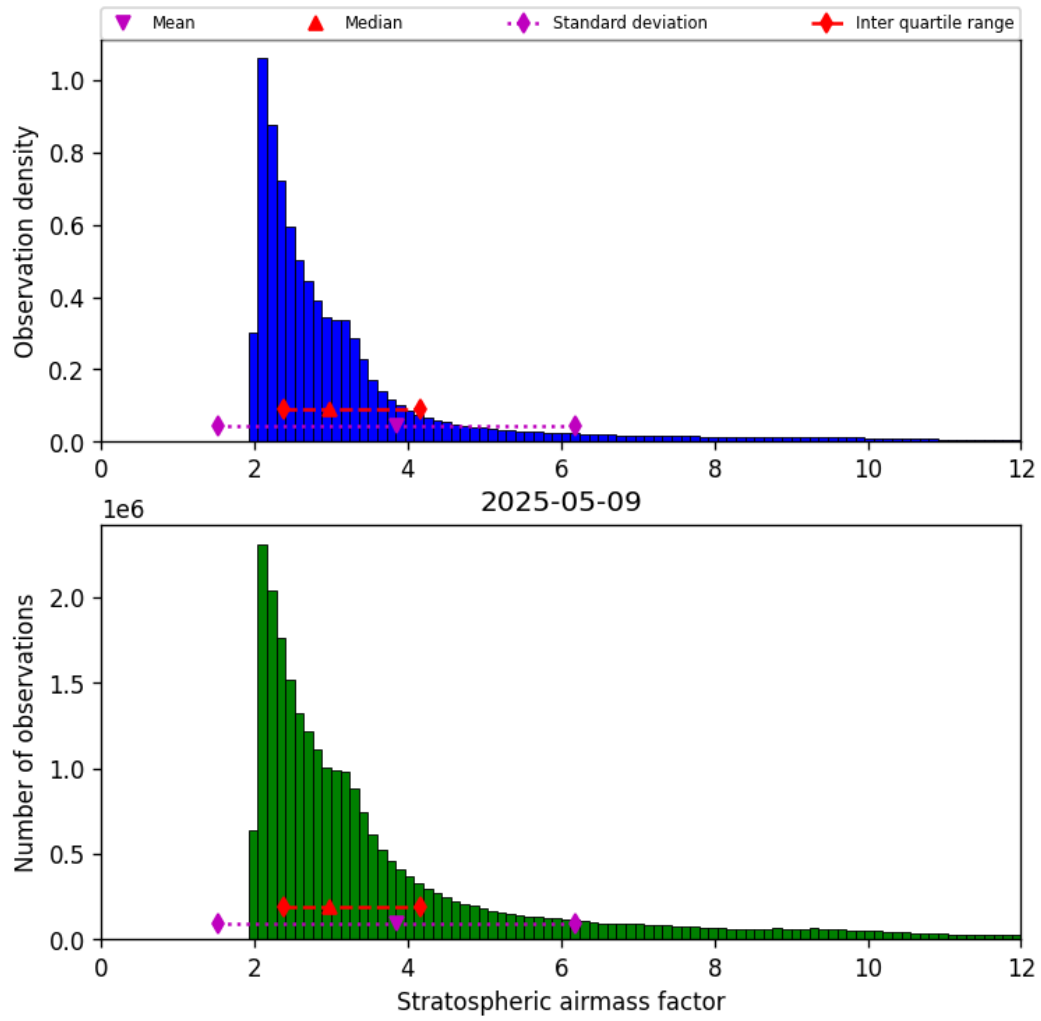
Figure 42: Histogram of “Stratospheric airmass factor” for 2025-05-09 to 2025-05-10
