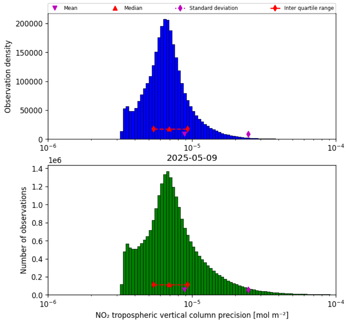
Figure 28: Histogram of “NO 2 tropospheric vertical column precision” for 2025-05-09 to 2025-05-10
