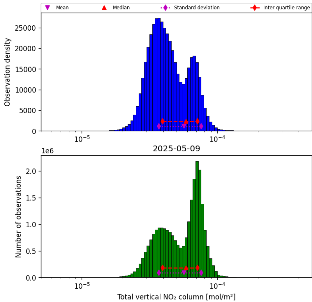
Figure 36: Histogram of “Total vertical NO 2 column” for 2025-05-09 to 2025-05-10
