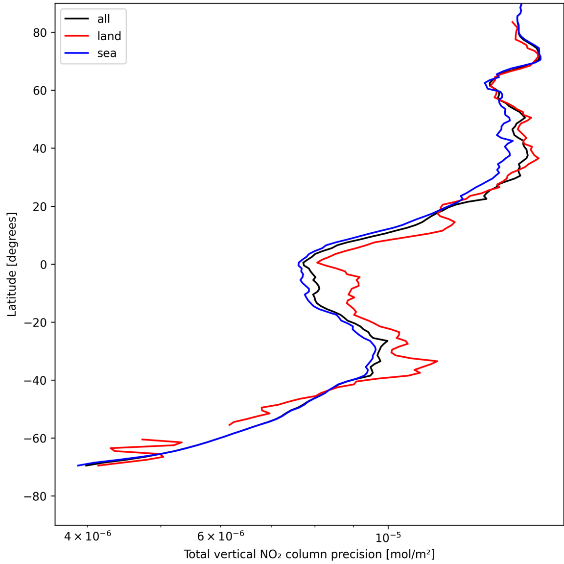
Figure 20: Zonal average of “Total vertical NO 2 column precision” for 2025-05-10 to 2025-05-11.
