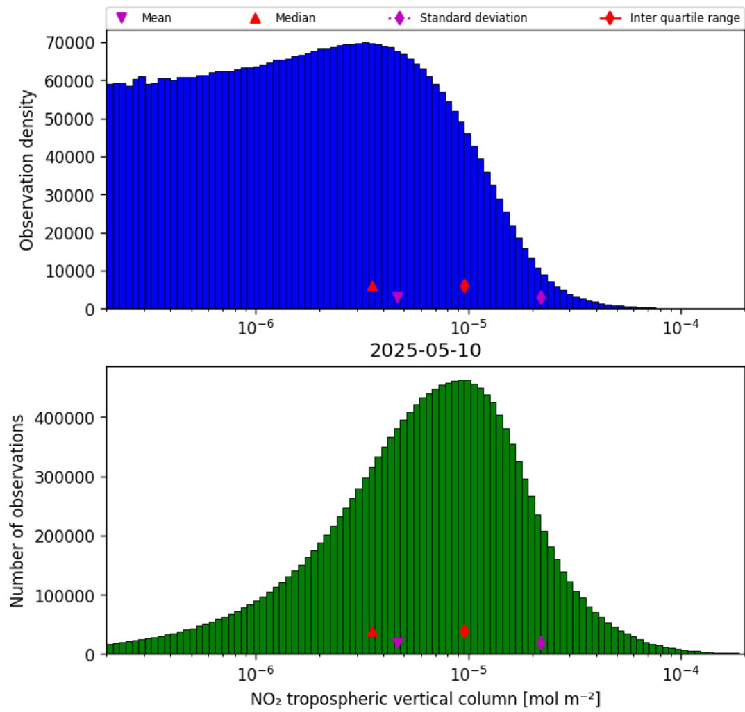
Figure 27: Histogram of “NO 2 tropospheric vertical column” for 2025-05-10 to 2025-05-11
