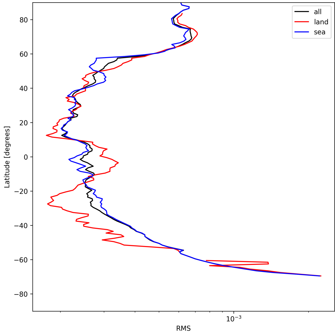
Figure 24: Zonal average of “RMS” for 2025-05-10 to 2025-05-11.
