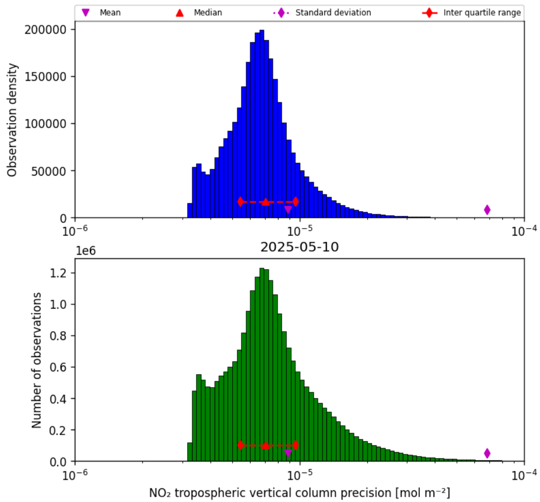
Figure 28: Histogram of “NO 2 tropospheric vertical column precision” for 2025-05-10 to 2025-05-11
