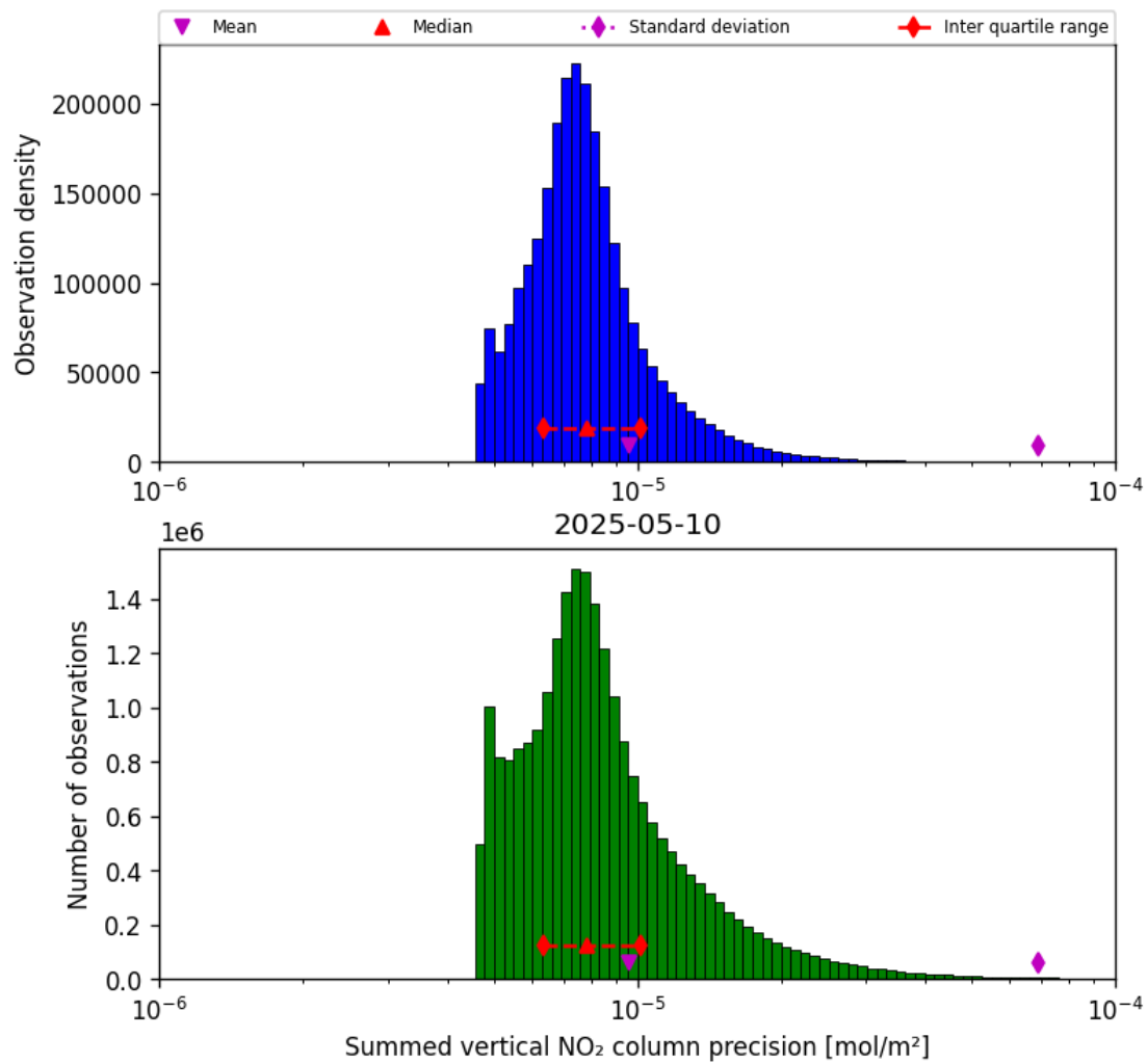
Figure 39: Histogram of “Summed vertical NO 2 column precision” for 2025-05-10 to 2025-05-11
