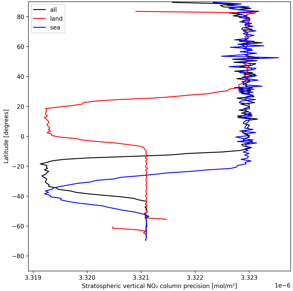
Figure 18: Zonal average of “Stratospheric vertical NO 2 column precision” for 2025-05-10 to 2025-05-11.
