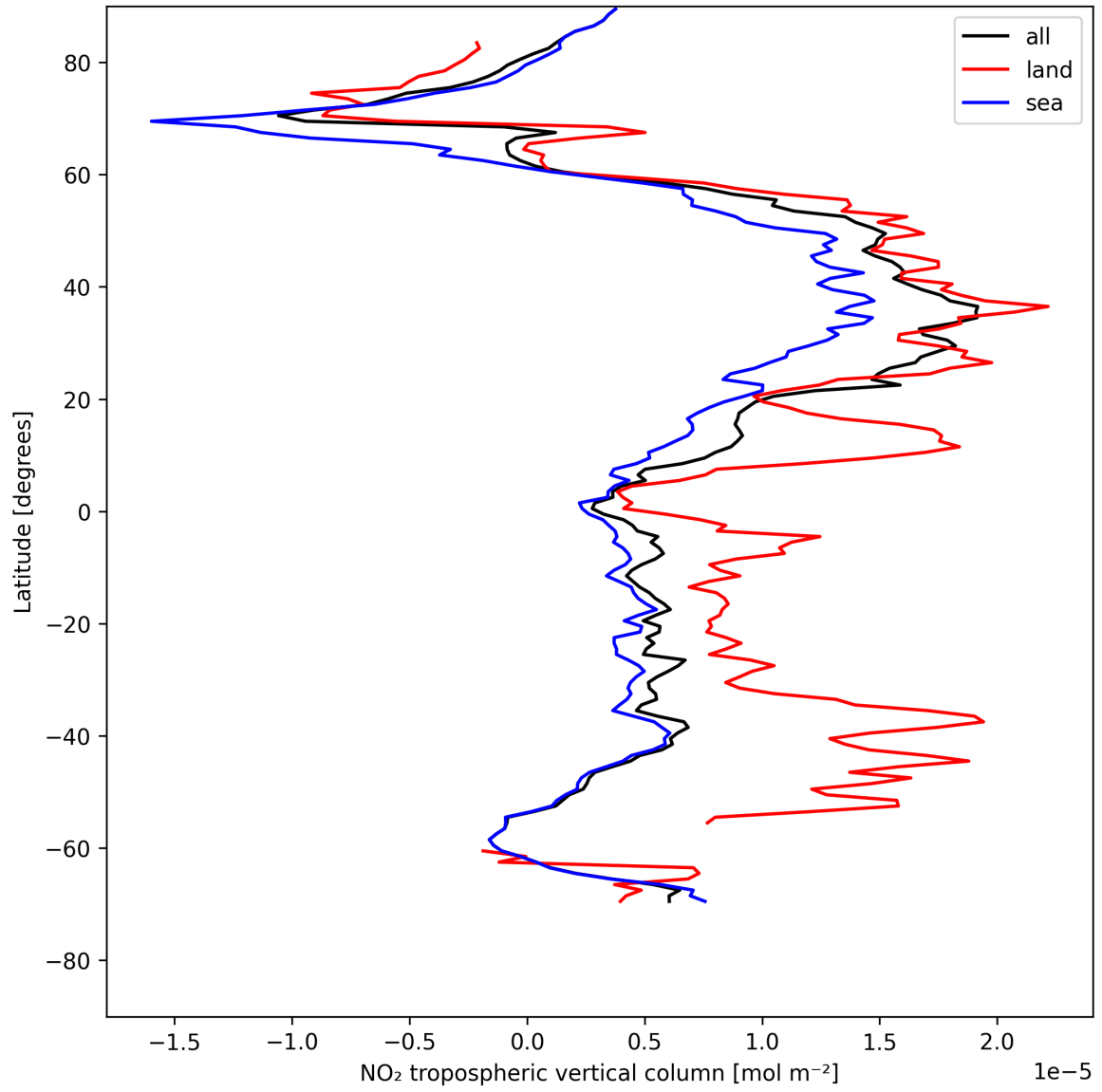
Figure 10: Zonal average of “NO 2 tropospheric vertical column” for 2025-05-10 to 2025-05-11.
