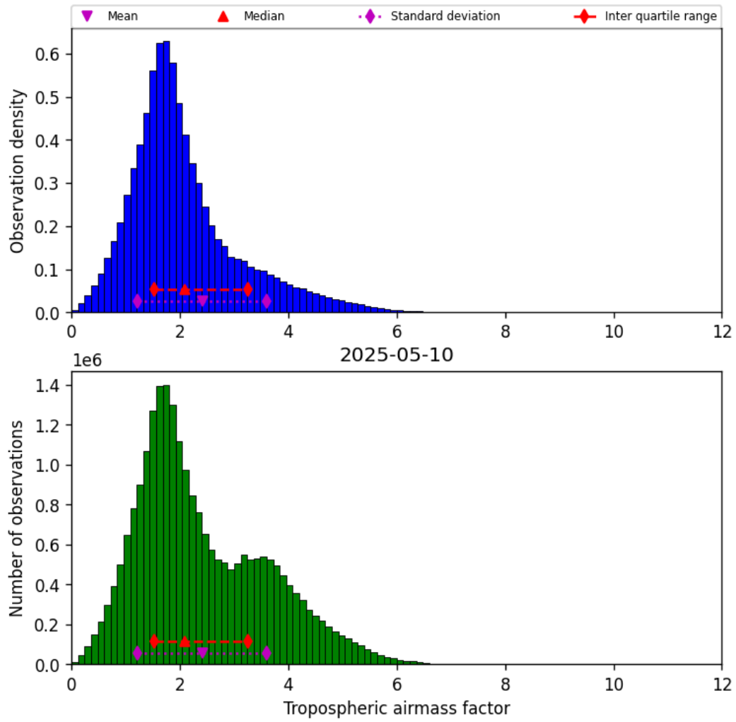
Figure 29: Histogram of “Tropospheric airmass factor” for 2025-05-10 to 2025-05-11
