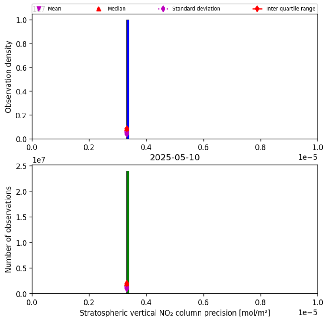
Figure 35: Histogram of “Stratospheric vertical NO 2 column precision” for 2025-05-10 to 2025-05-11
