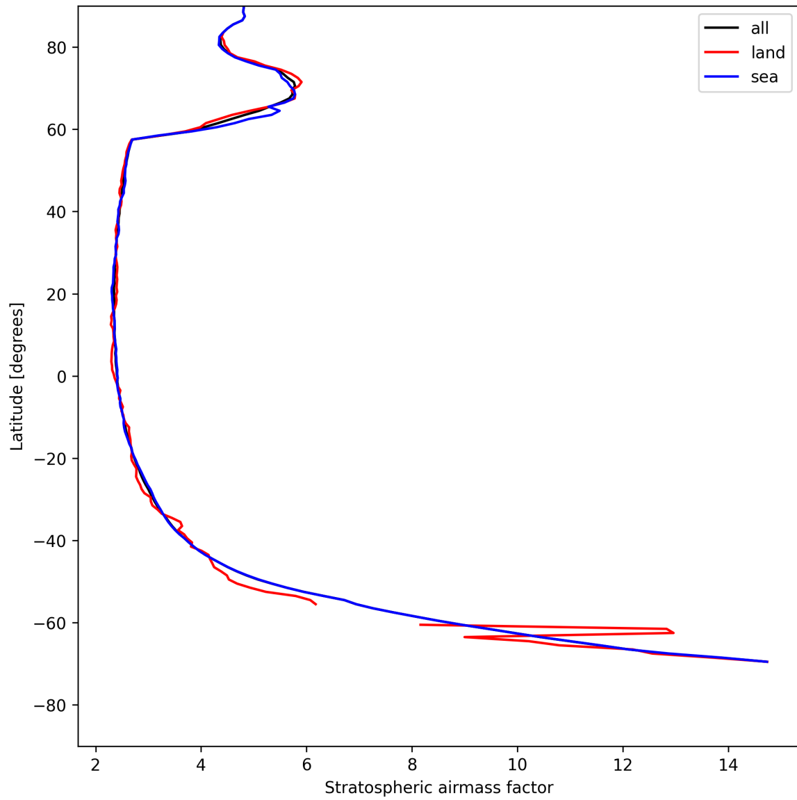
Figure 25: Zonal average of “Stratospheric air mass factor” for 2025-05-10 to 2025-05-11.
