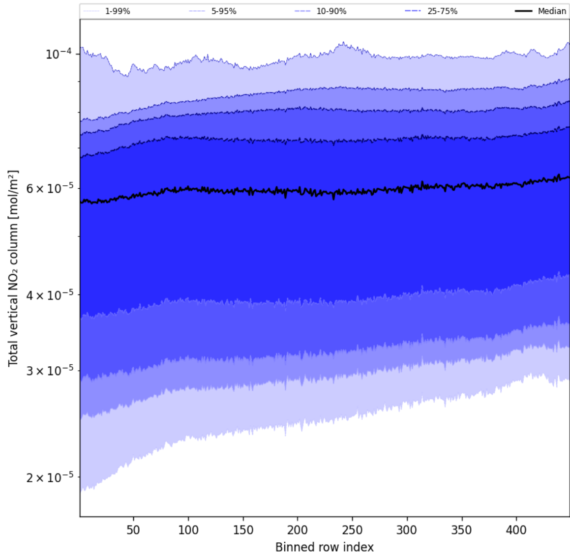
Figure 53: Along track statistics of “Total vertical NO 2 column” for 2025-05-10 to 2025-05-11
