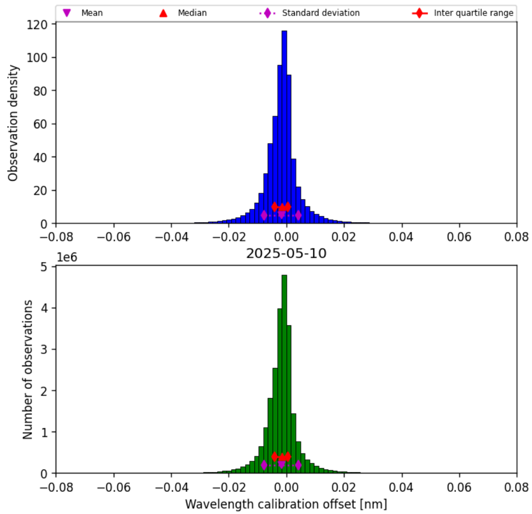
Figure 33: Histogram of “Wavelength calibration offset” for 2025-05-10 to 2025-05-11
