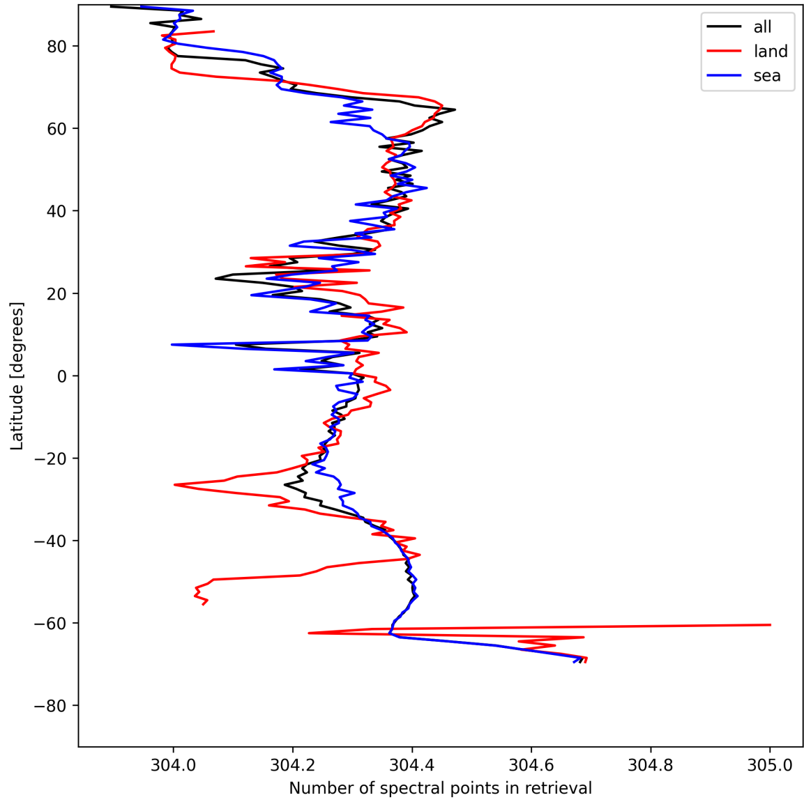
Figure 14: Zonal average of “Number of spectral points in retrieval” for 2025-05-10 to 2025-05-11.
