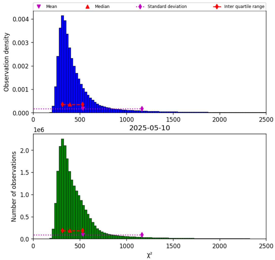
Figure 40: Histogram of “ \chi^2 ” for 2025-05-10 to 2025-05-11
