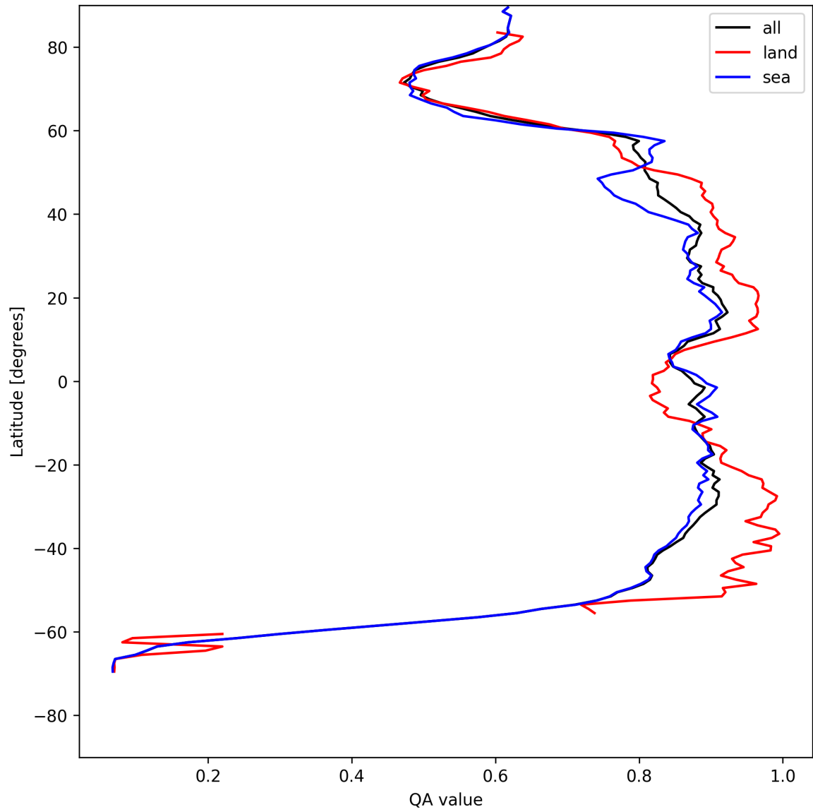
Figure 9: Zonal average of “QA value” for 2025-05-10 to 2025-05-11.
