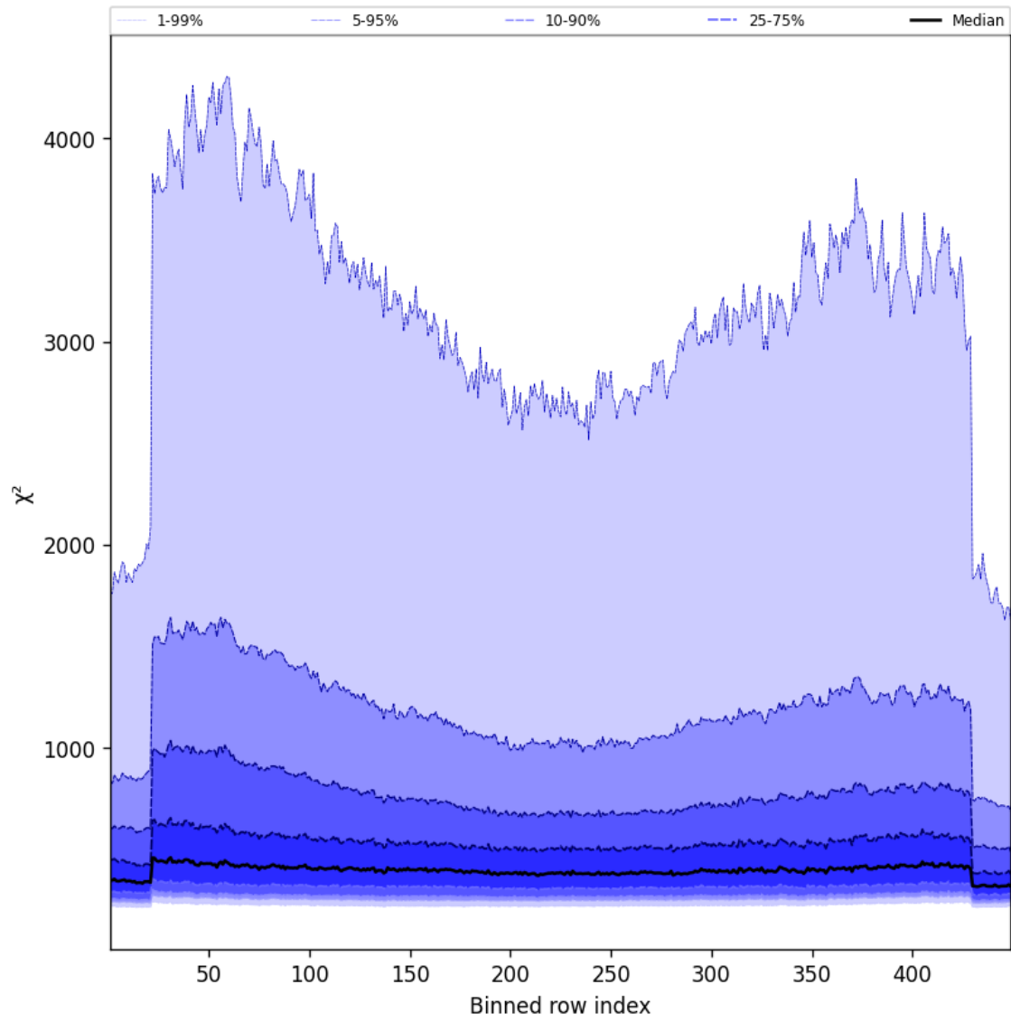
Figure 57: Along track statistics of “ \chi^2 ” for 2025-05-10 to 2025-05-11
