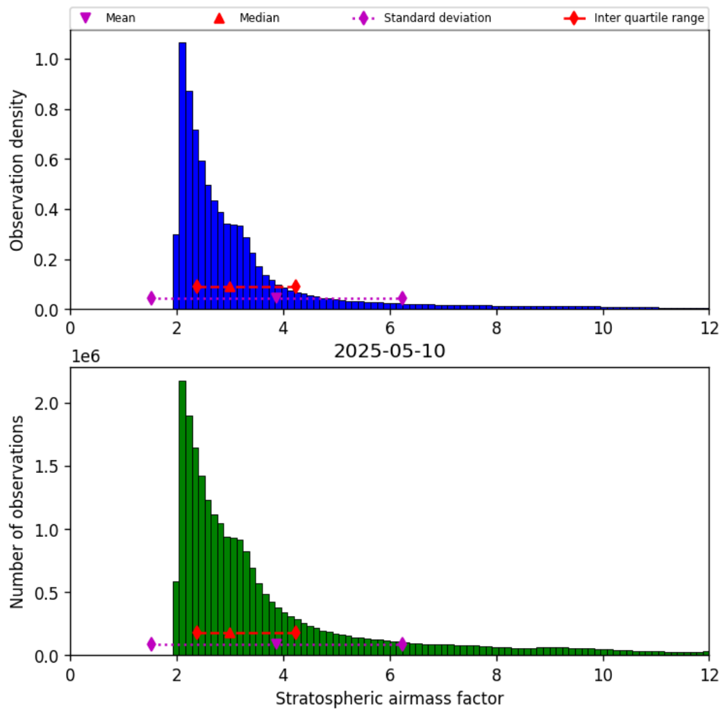
Figure 42: Histogram of “Stratospheric airmass factor” for 2025-05-10 to 2025-05-11
