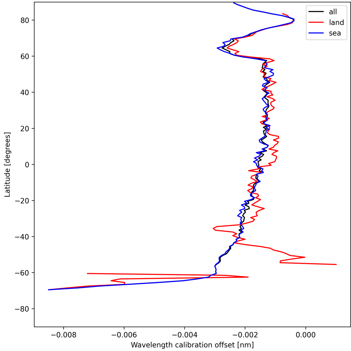
Figure 16: Zonal average of “Wavelength calibration offset” for 2025-05-10 to 2025-05-11.
