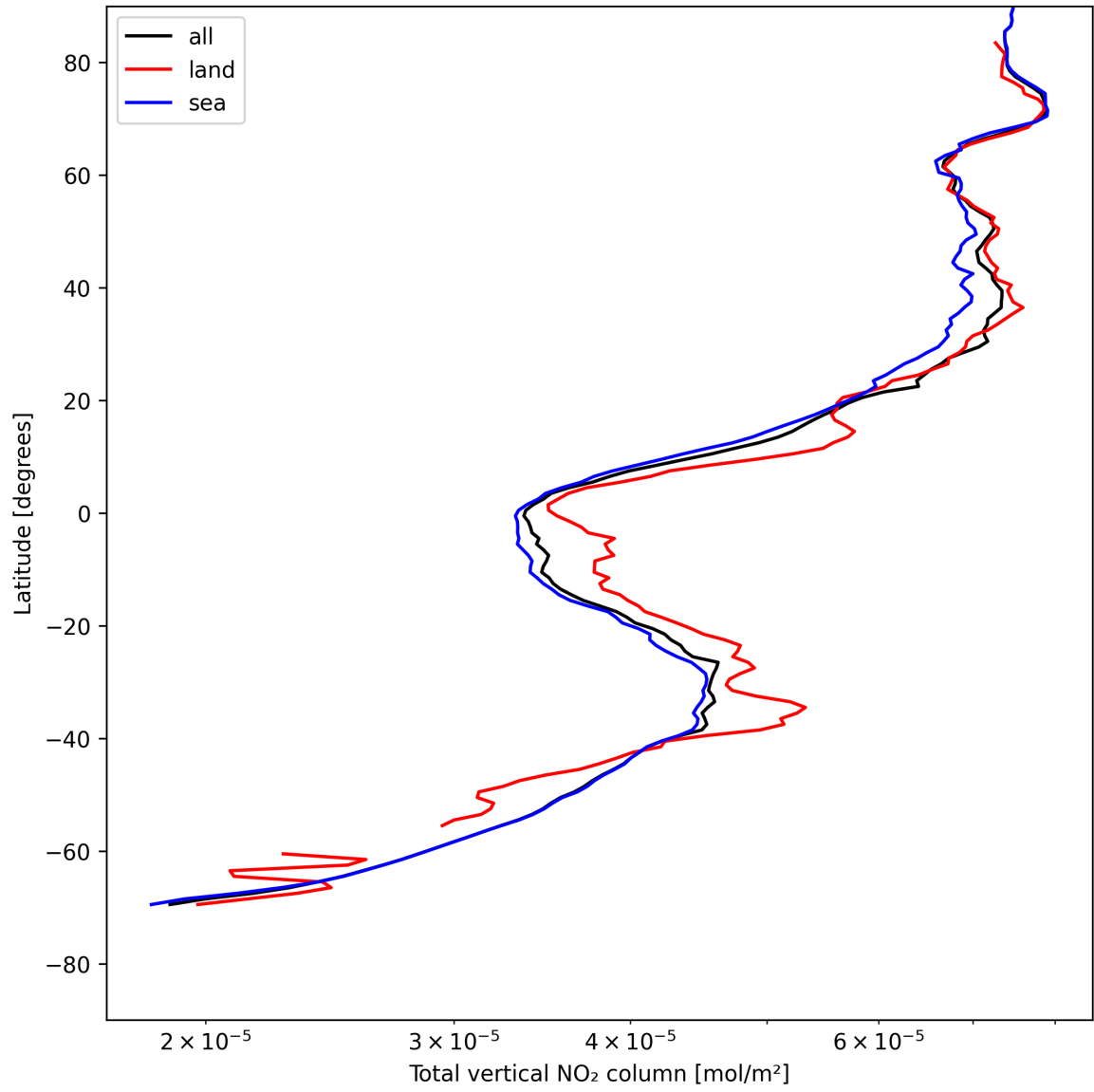
Figure 19: Zonal average of “Total vertical NO 2 column” for 2025-05-10 to 2025-05-11.
