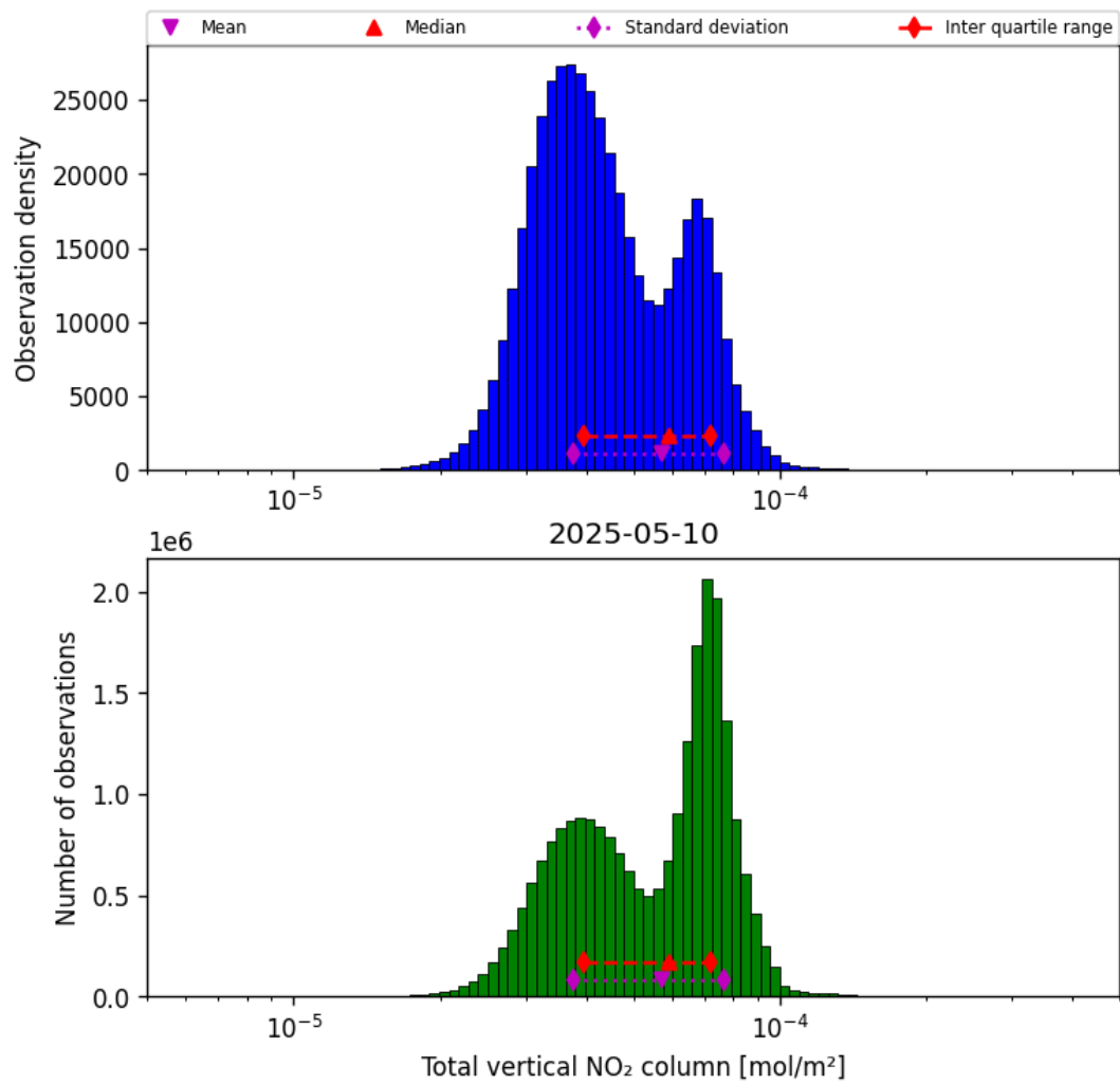
Figure 36: Histogram of “Total vertical NO 2 column” for 2025-05-10 to 2025-05-11
