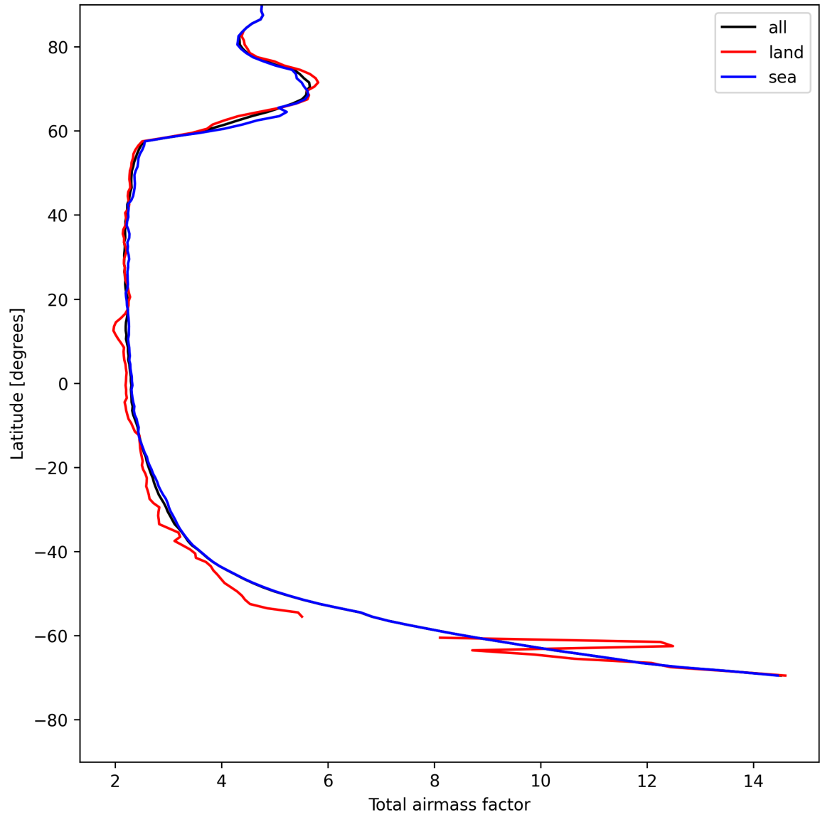
Figure 13: Zonal average of “Total airmass factor” for 2025-05-10 to 2025-05-11.
