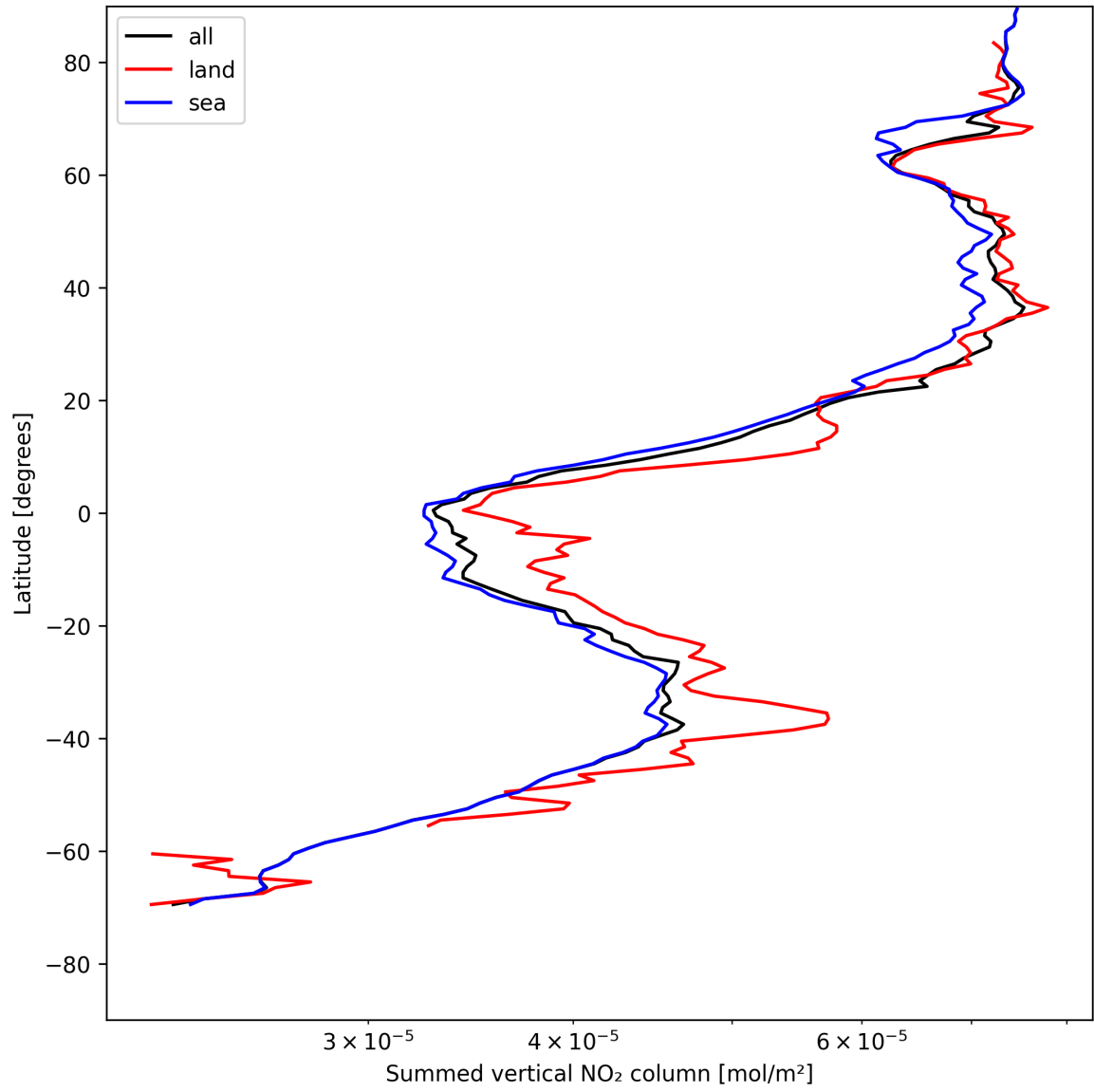
Figure 21: Zonal average of “Summed vertical NO 2 column” for 2025-05-10 to 2025-05-11.
