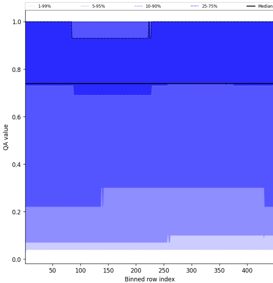
Figure 43: Along track statistics of “QA value” for 2025-05-10 to 2025-05-11
