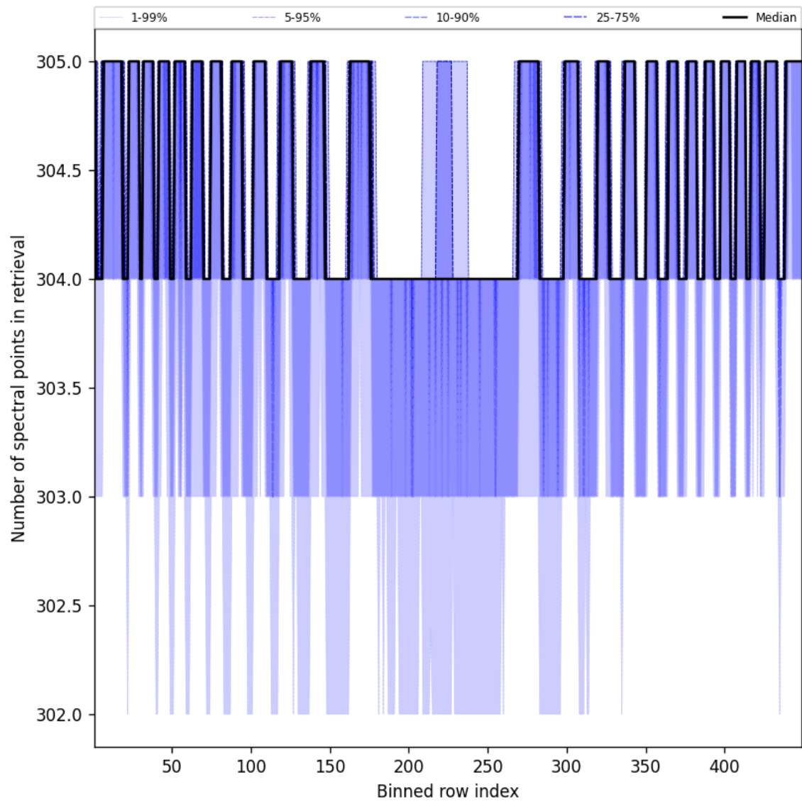
Figure 48: Along track statistics of “Number of spectral points in retrieval” for 2025-05-10 to 2025-05-11
