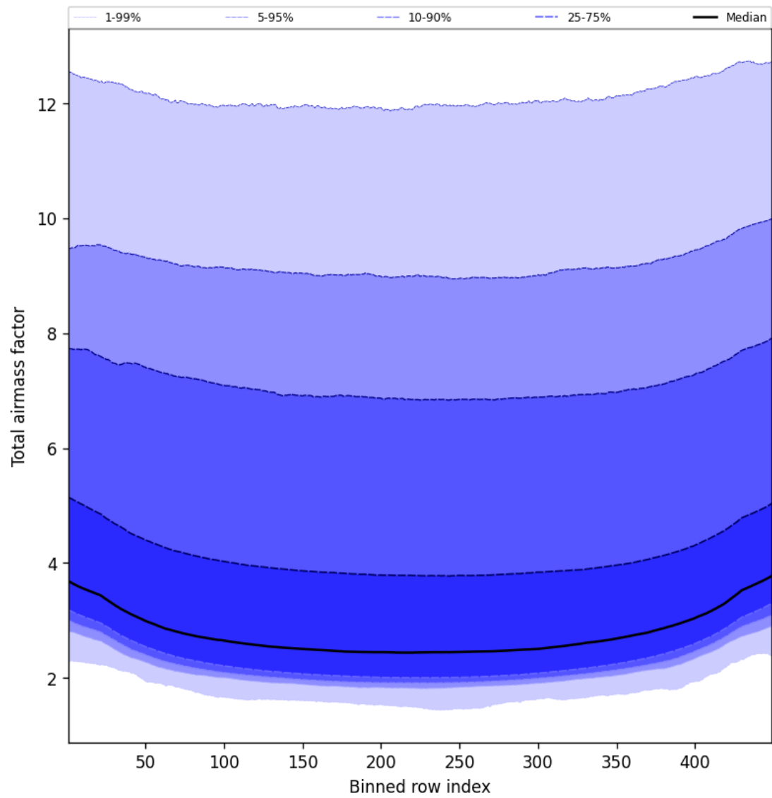
Figure 47: Along track statistics of “Total airmass factor” for 2025-05-10 to 2025-05-11
