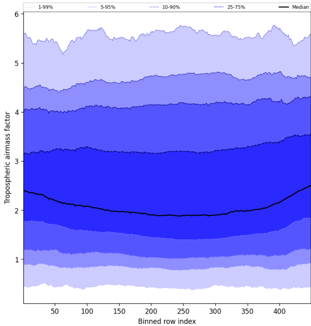
Figure 46: Along track statistics of “Tropospheric airmass factor” for 2025-05-10 to 2025-05-11
