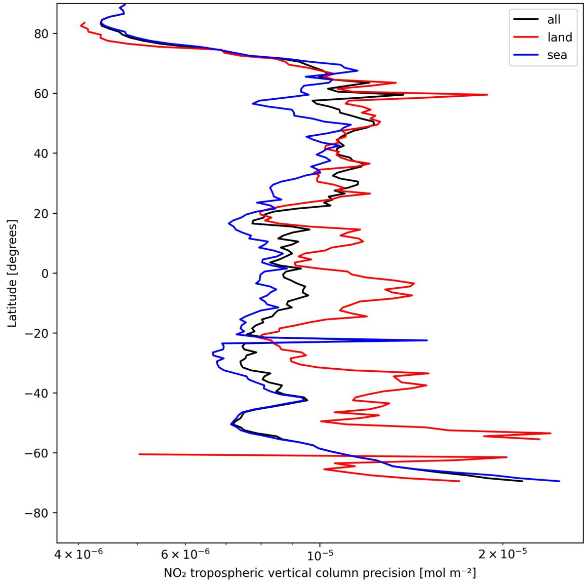
Figure 11: Zonal average of “NO 2 tropospheric vertical column precision” for 2025-05-10 to 2025-05-11.
