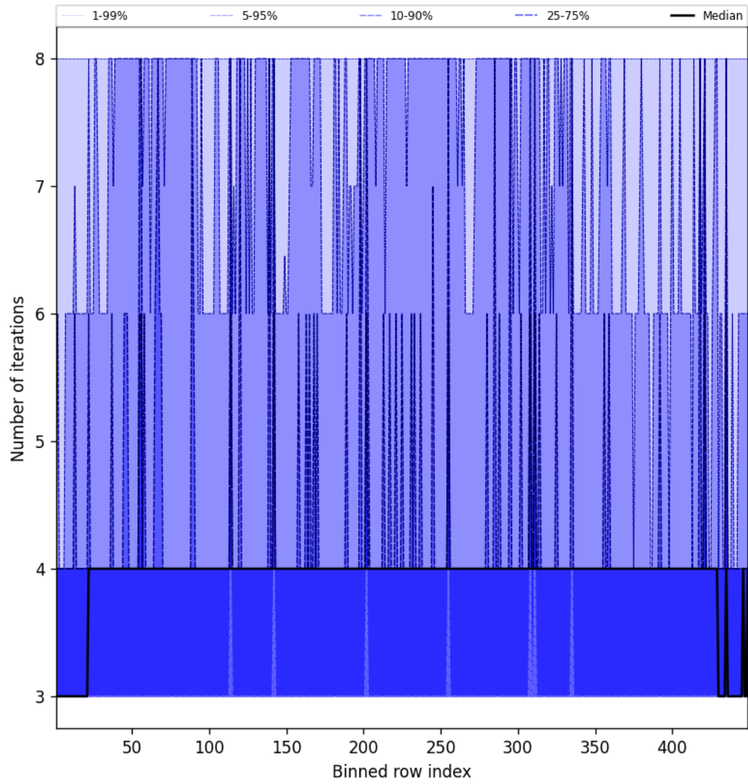
Figure 49: Along track statistics of “Number of iterations” for 2025-05-10 to 2025-05-11
