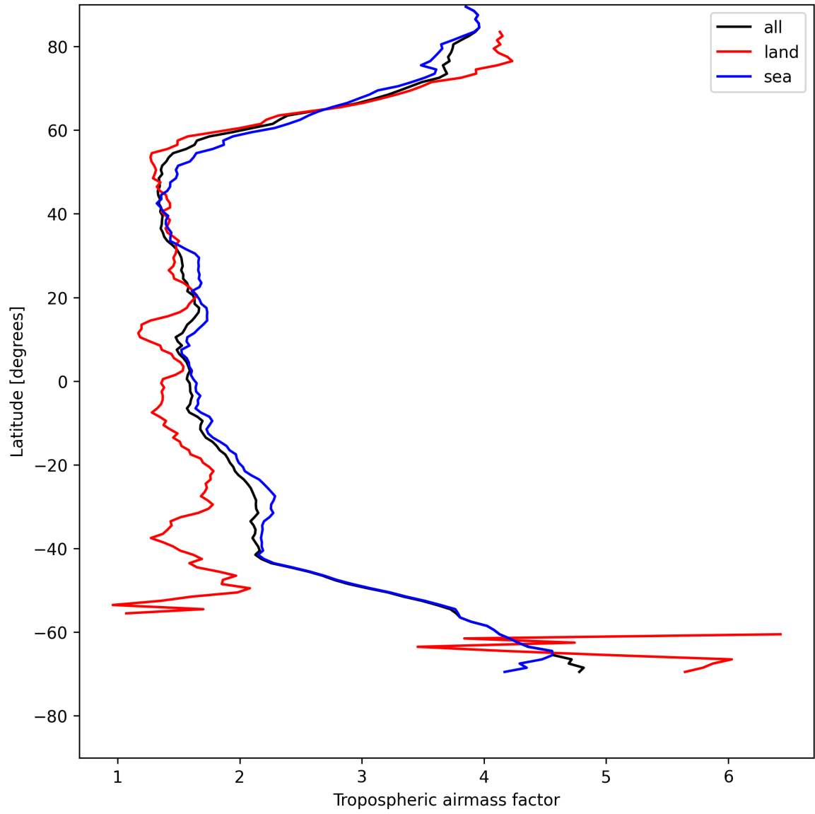
Figure 12: Zonal average of “Tropospheric airmass factor” for 2025-05-10 to 2025-05-11.
