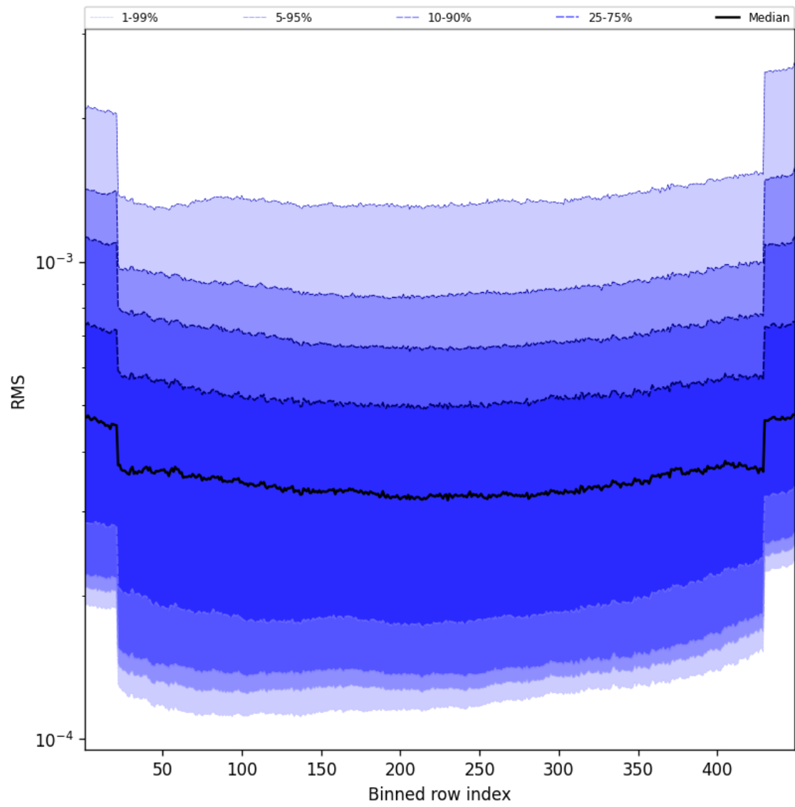
Figure 58: Along track statistics of “RMS” for 2025-05-10 to 2025-05-11
