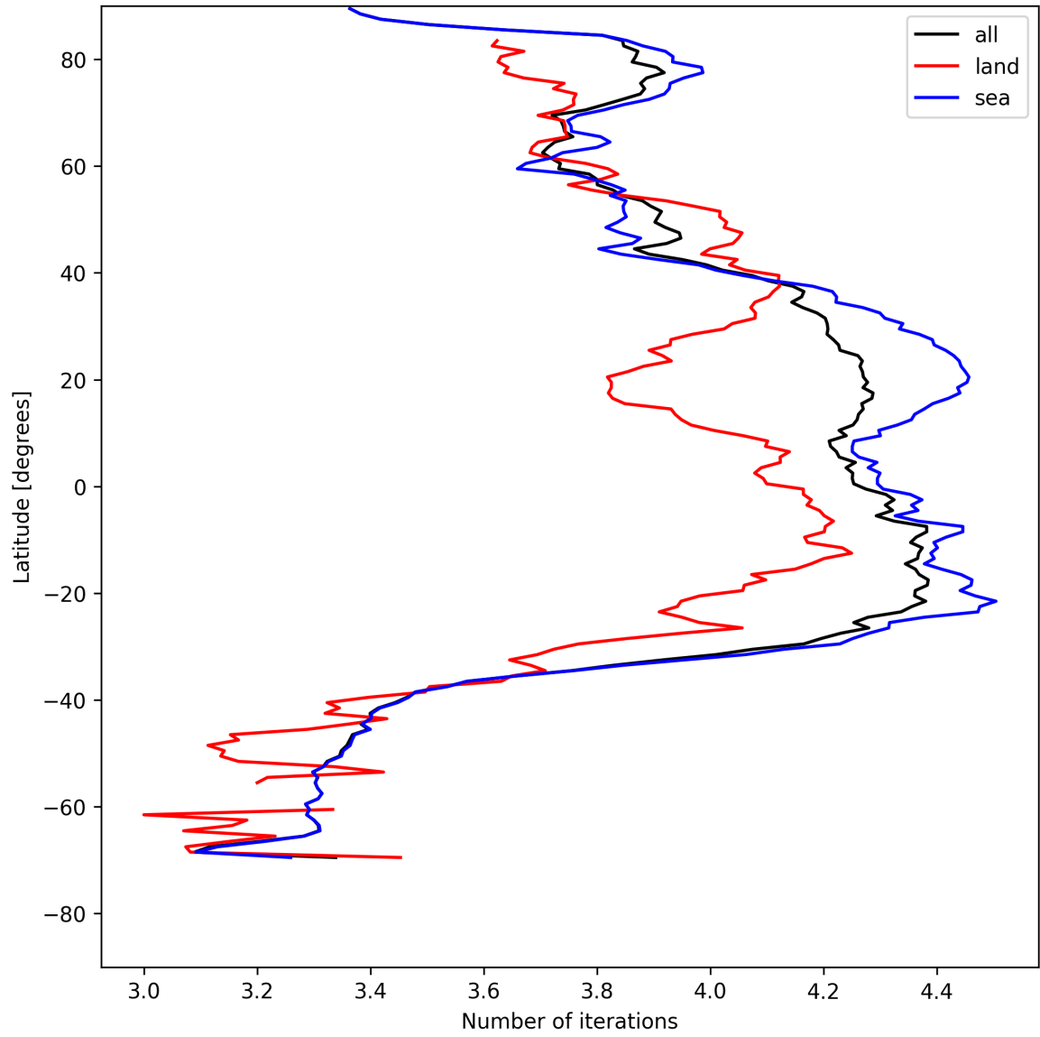
Figure 15: Zonal average of “Number of iterations” for 2025-05-10 to 2025-05-11.
