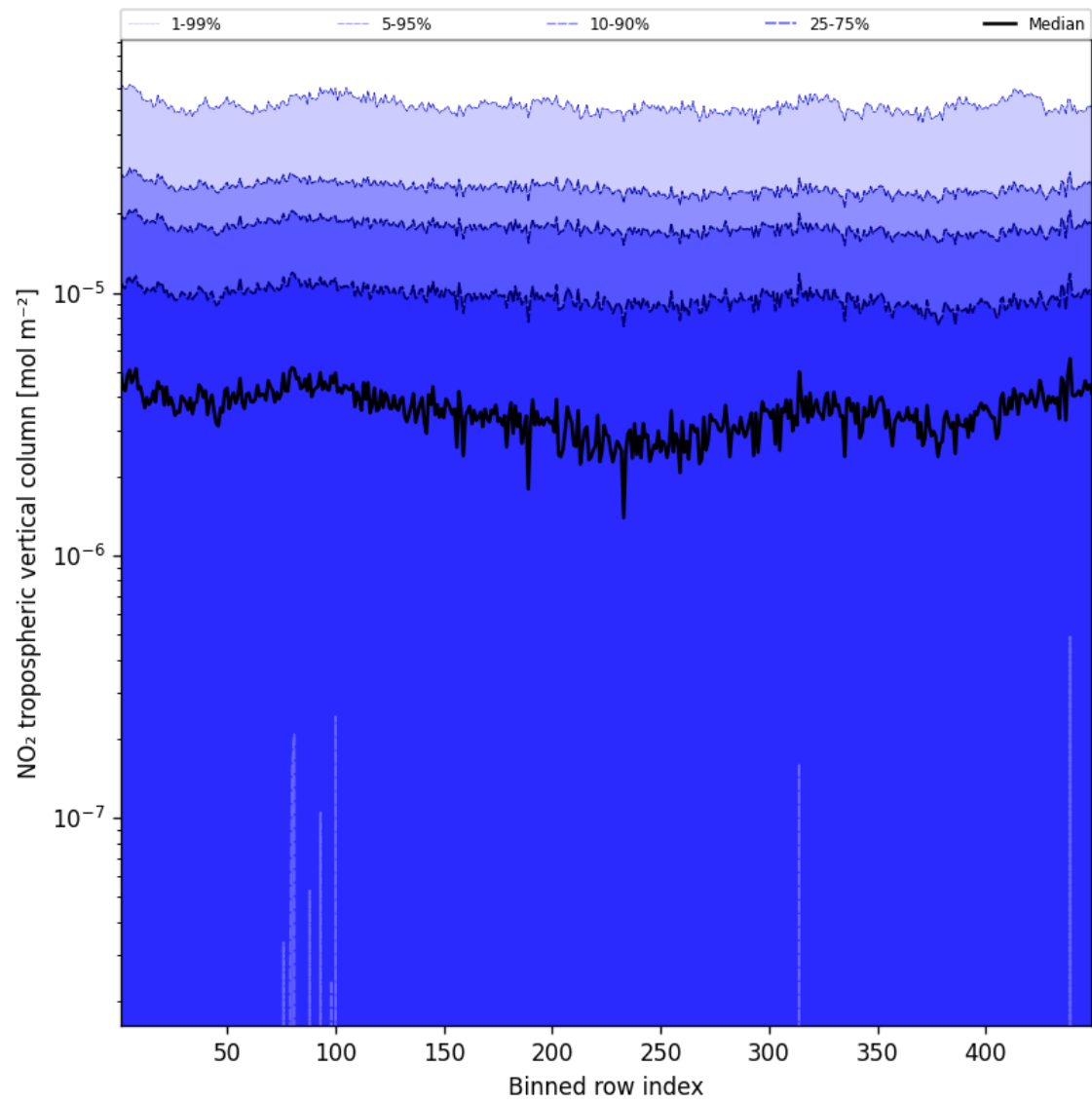
Figure 44: Along track statistics of “NO 2 tropospheric vertical column” for 2025-05-10 to 2025-05-11
