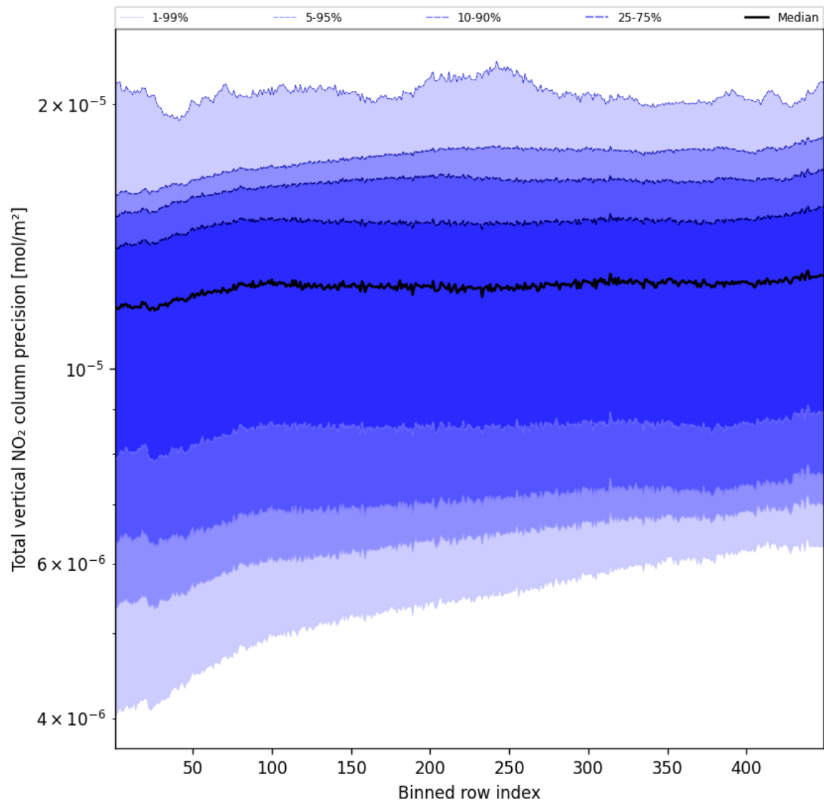
Figure 54: Along track statistics of “Total vertical NO 2 column precision” for 2025-05-10 to 2025-05-11
