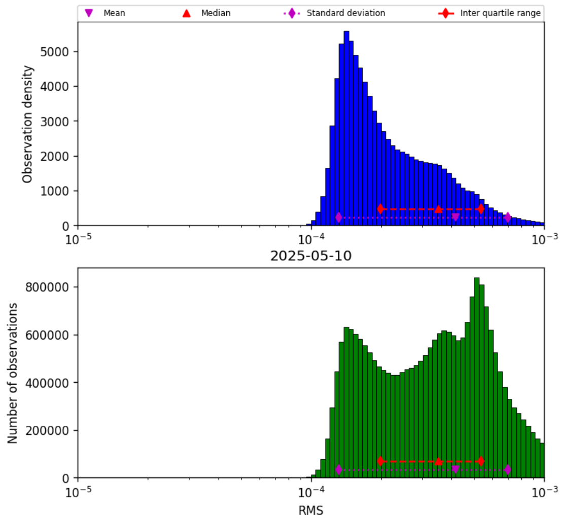
Figure 41: Histogram of “RMS” for 2025-05-10 to 2025-05-11
