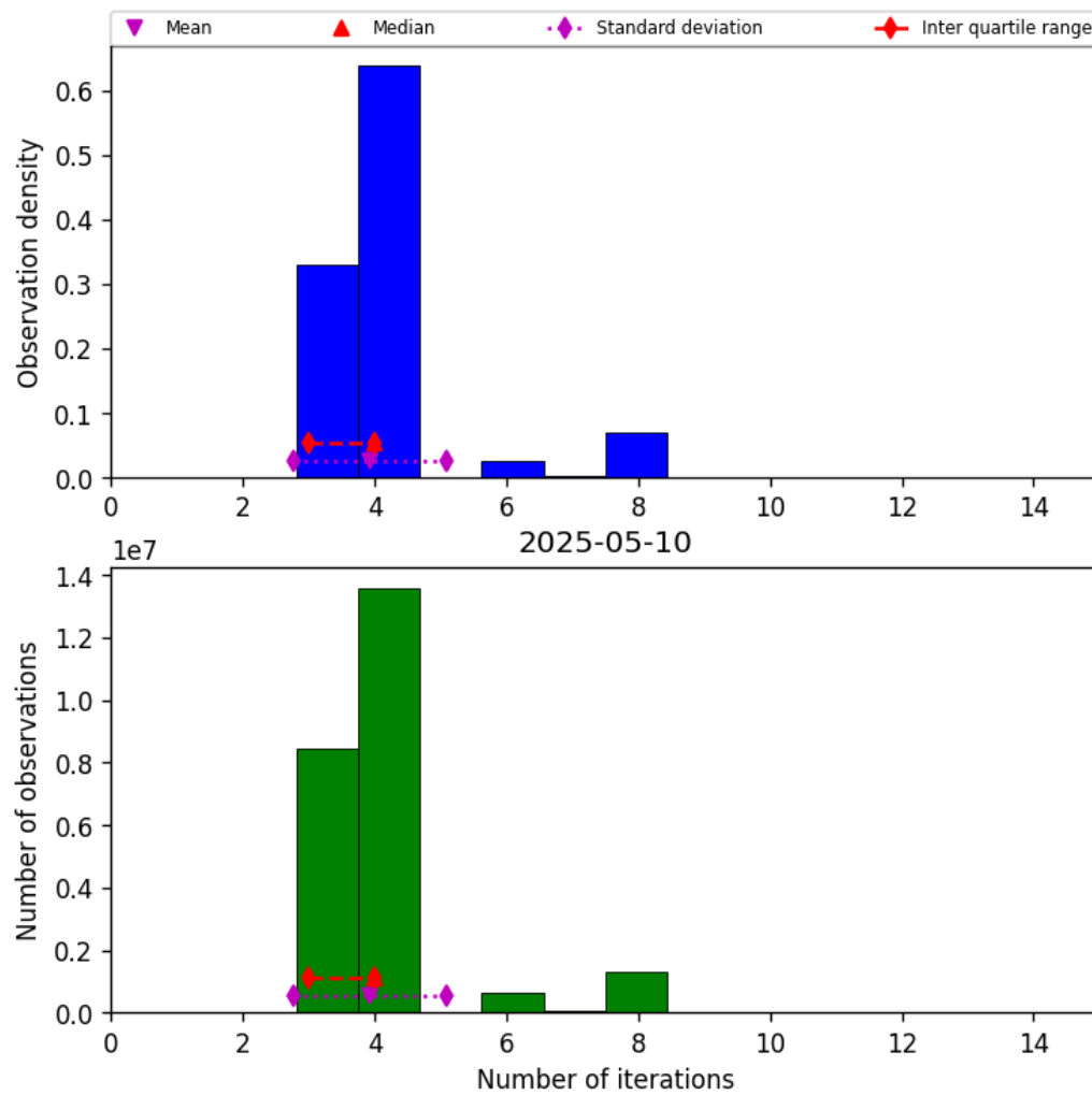
Figure 32: Histogram of “Number of iterations” for 2025-05-10 to 2025-05-11
