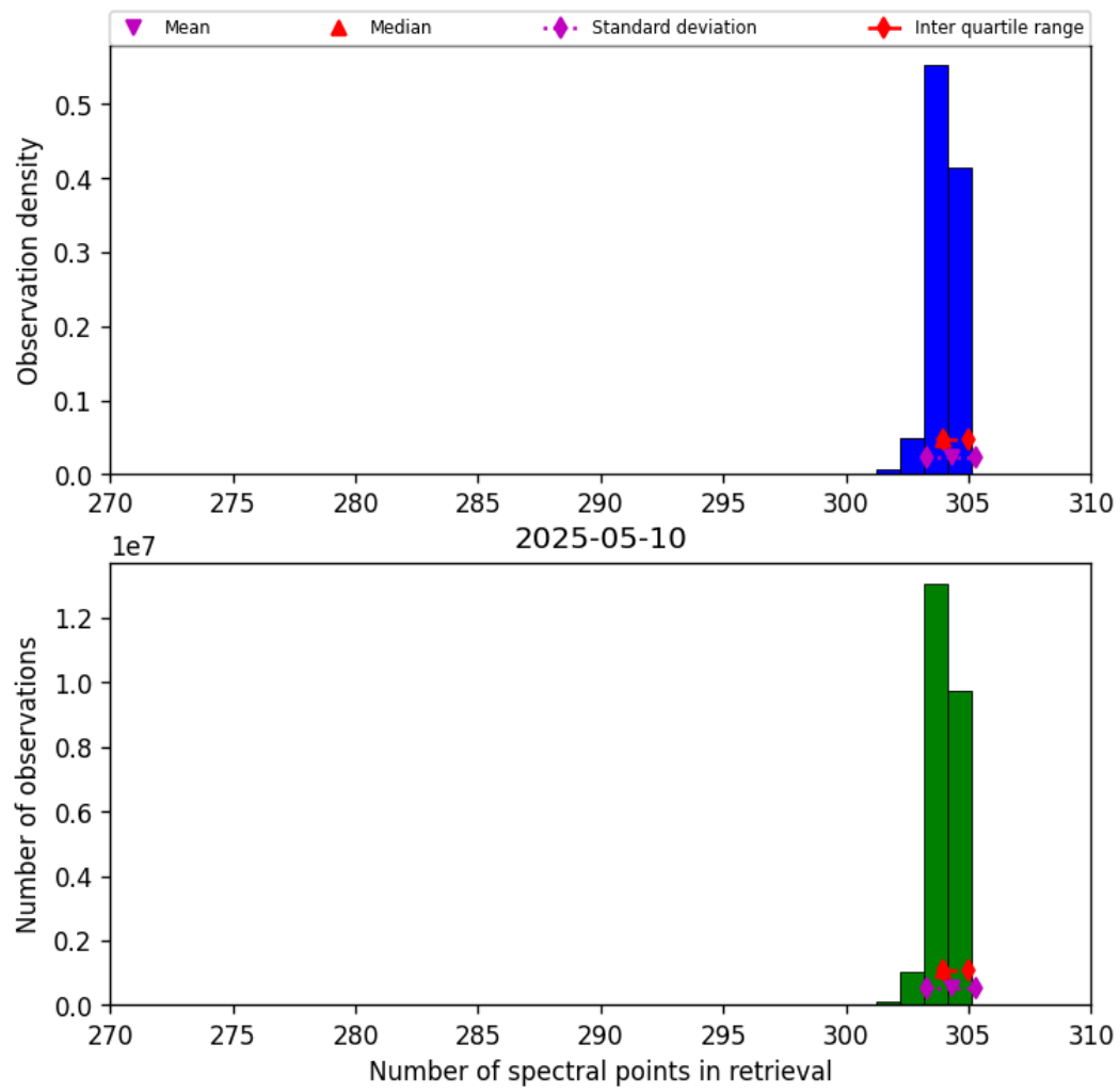
Figure 31: Histogram of “Number of spectral points in retrieval” for 2025-05-10 to 2025-05-11
