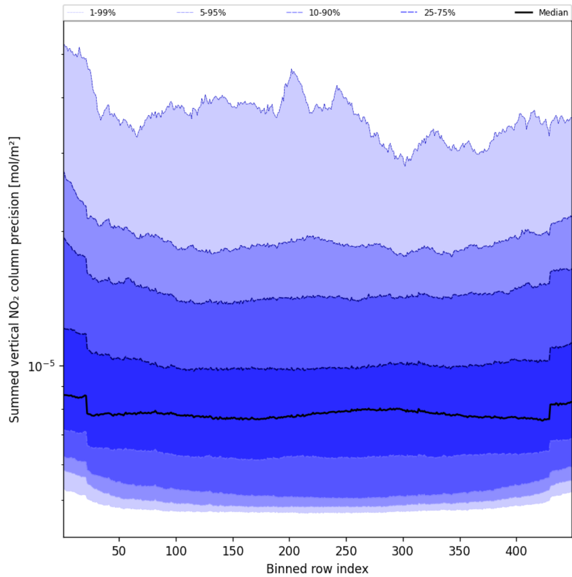
Figure 56: Along track statistics of “Summed vertical NO 2 column precision” for 2025-05-10 to 2025-05-11
