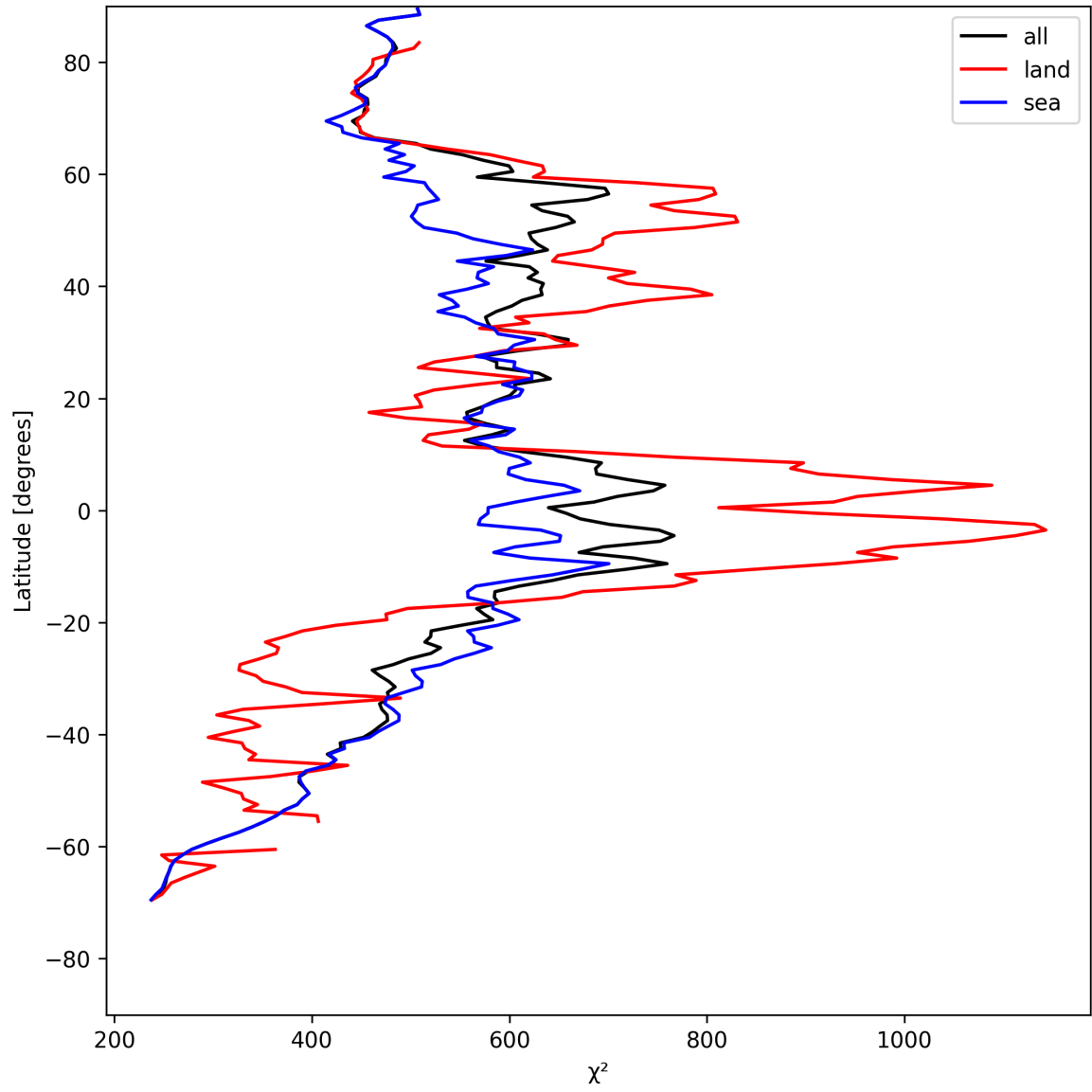
Figure 23: Zonal average of “ \chi^2 ” for 2025-05-10 to 2025-05-11.
