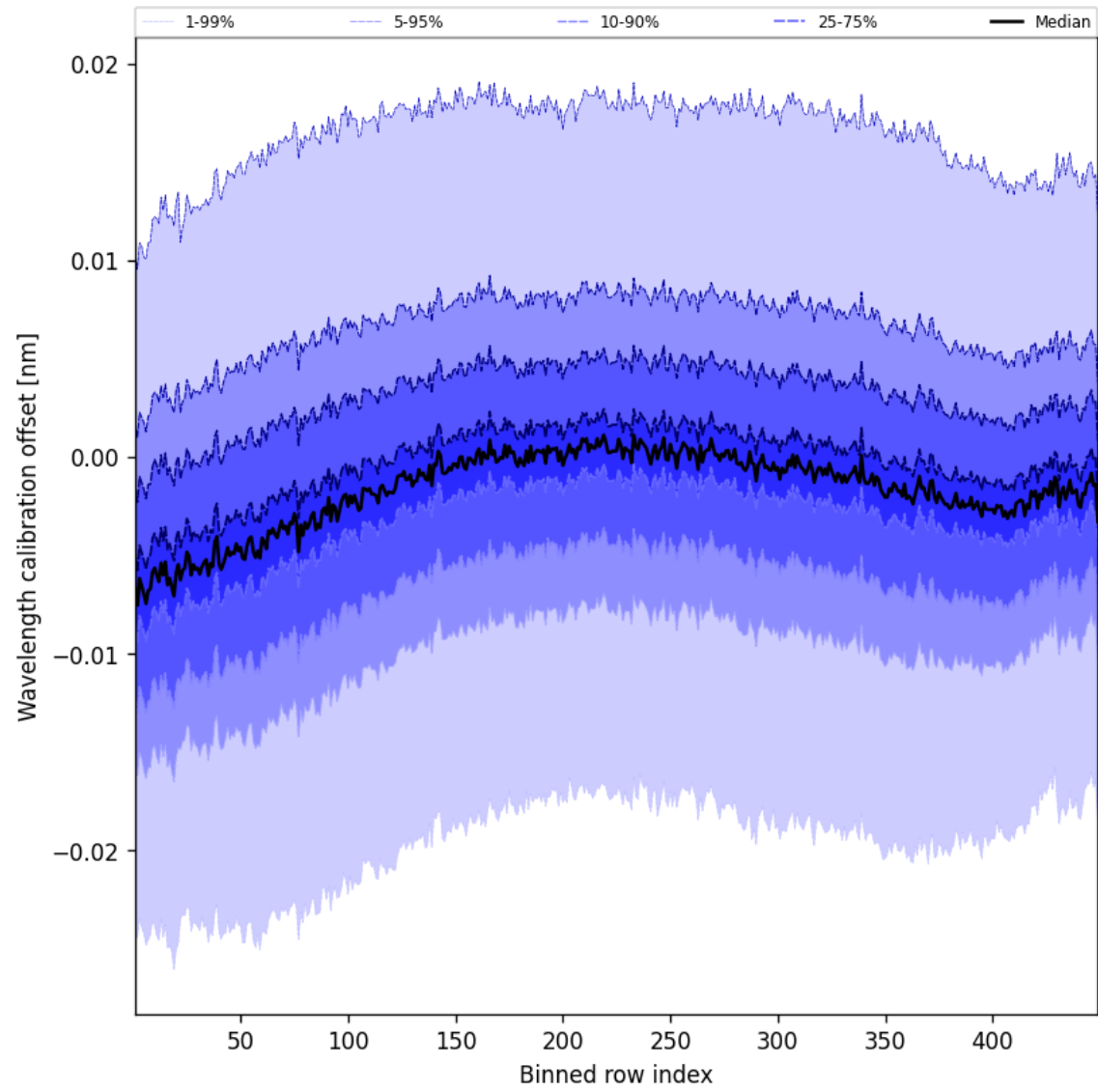
Figure 50: Along track statistics of “Wavelength calibration offset” for 2025-05-10 to 2025-05-11
