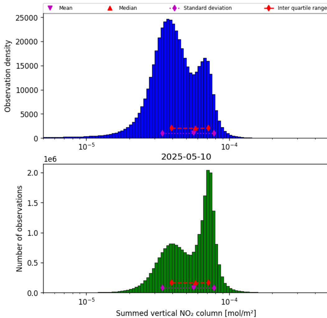
Figure 38: Histogram of “Summed vertical NO 2 column” for 2025-05-10 to 2025-05-11
