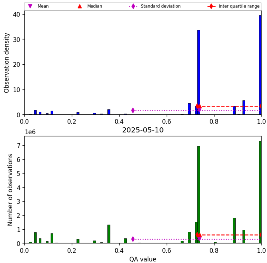
Figure 26: Histogram of “QA value” for 2025-05-10 to 2025-05-11
