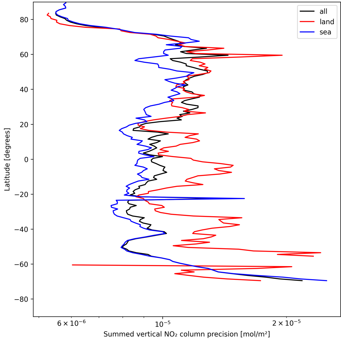
Figure 22: Zonal average of “Summed vertical NO 2 column precision” for 2025-05-10 to 2025-05-11.
