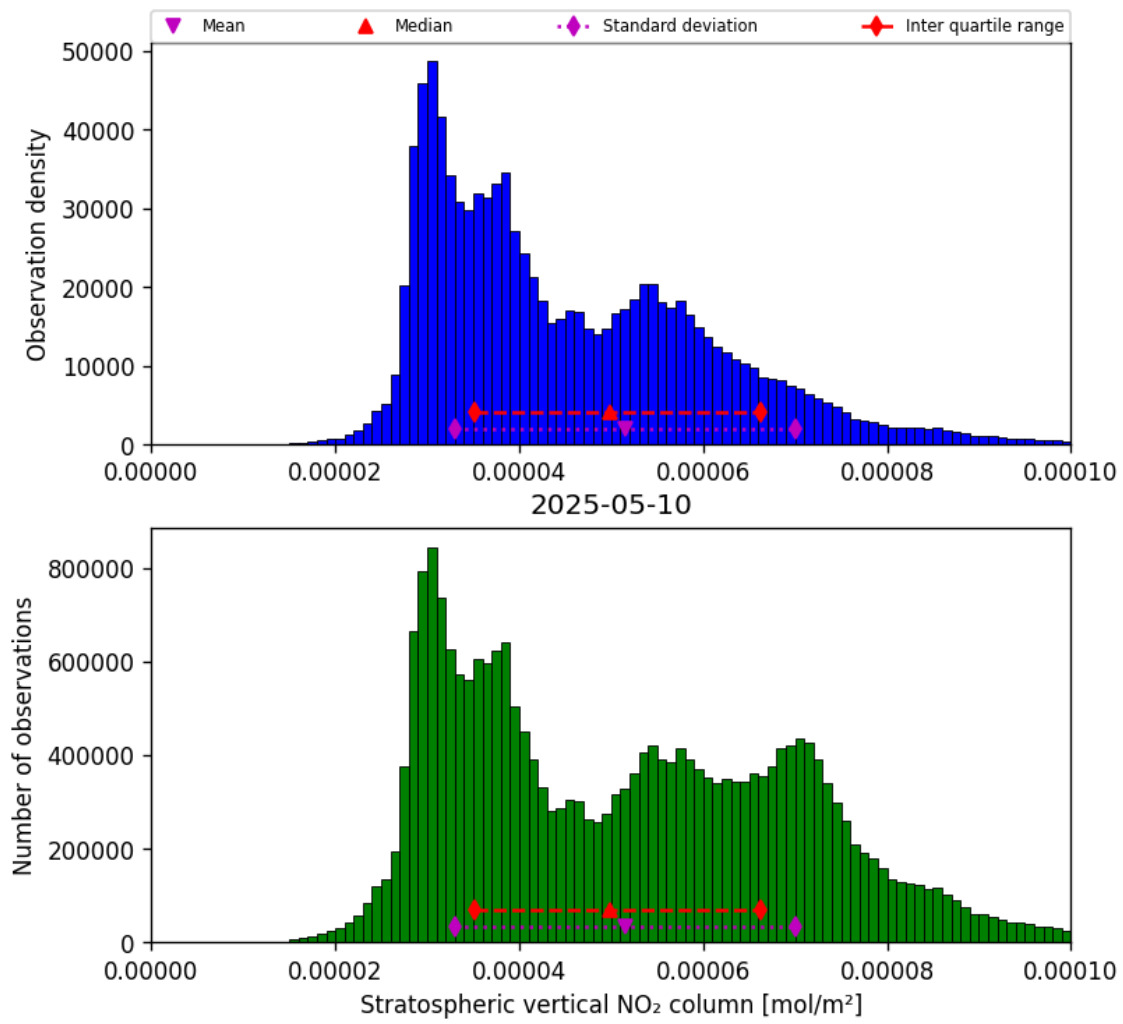
Figure 34: Histogram of “Stratospheric vertical NO 2 column” for 2025-05-10 to 2025-05-11
