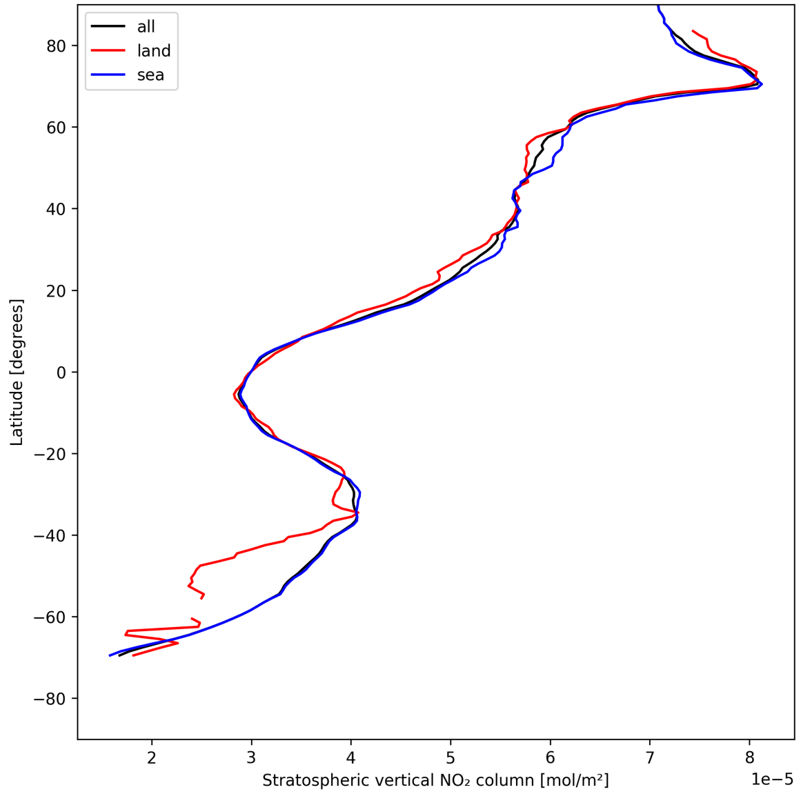
Figure 17: Zonal average of “Stratospheric vertical NO 2 column” for 2025-05-10 to 2025-05-11.
