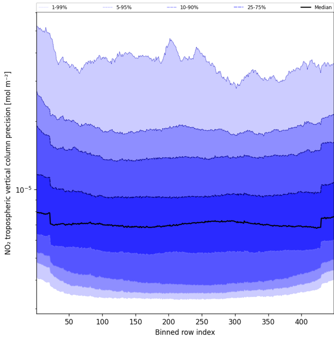
Figure 45: Along track statistics of “NO 2 tropospheric vertical column precision” for 2025-05-10 to 2025-05-11
