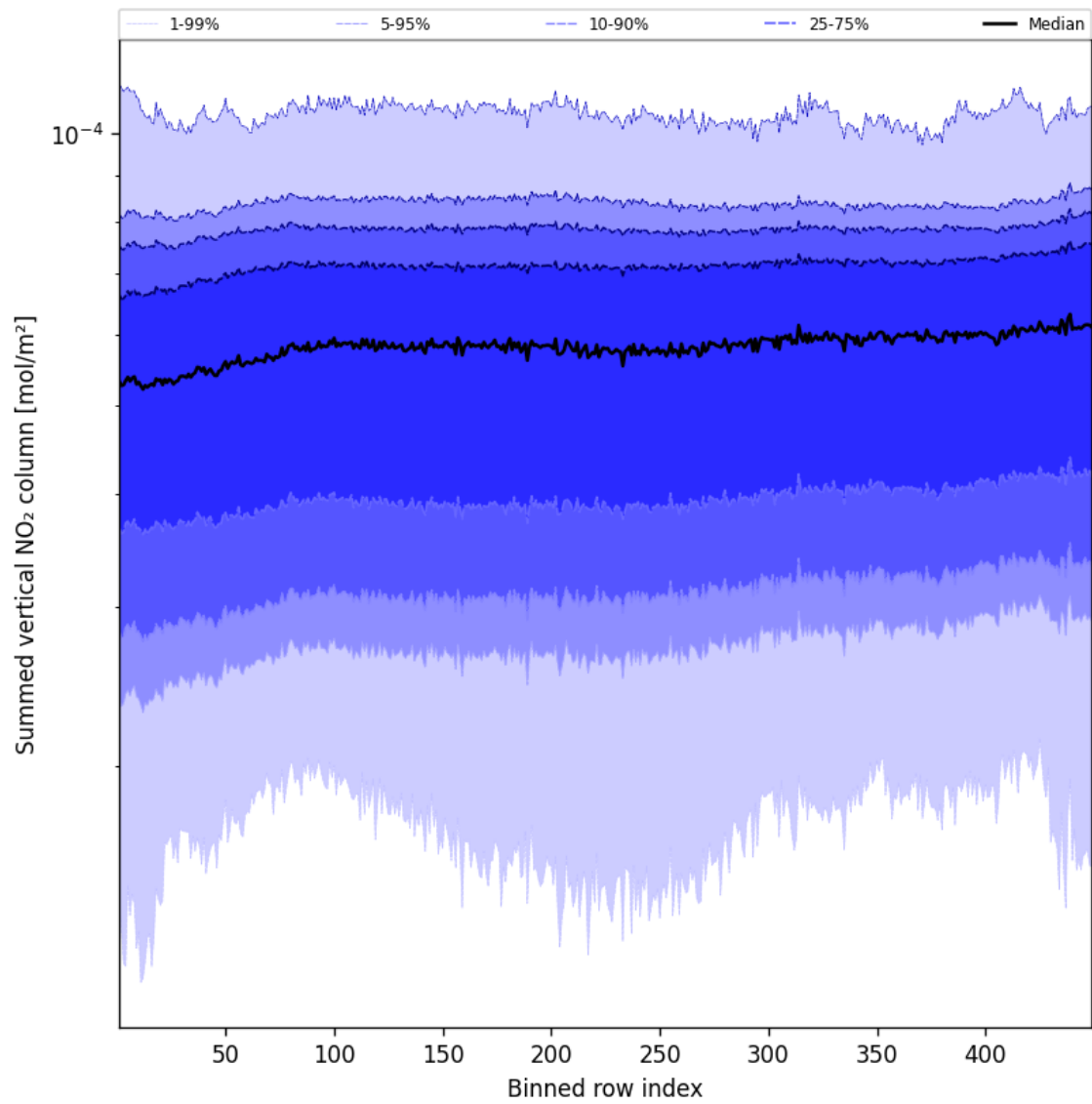
Figure 55: Along track statistics of “Summed vertical NO 2 column” for 2025-05-10 to 2025-05-11
