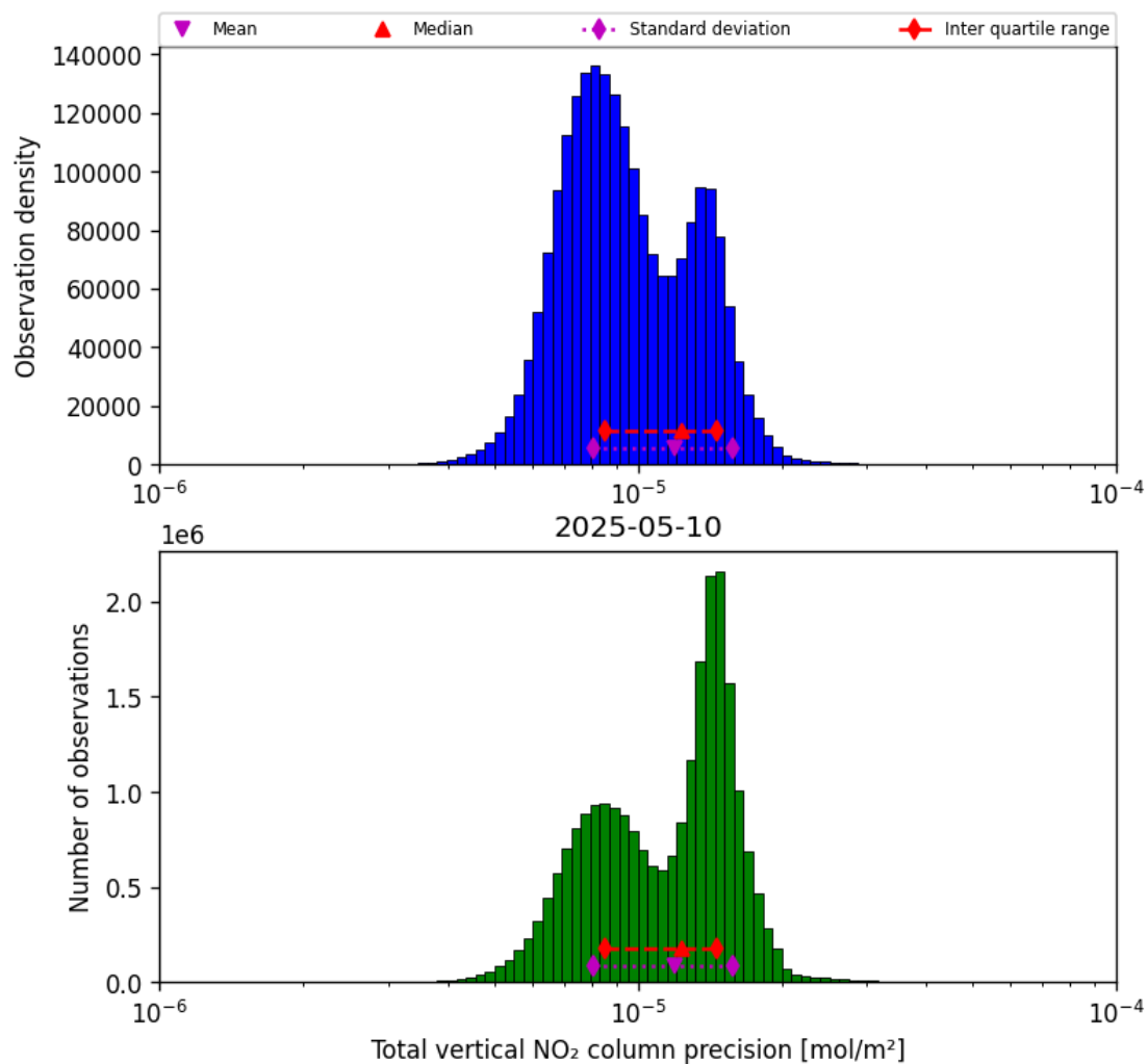
Figure 37: Histogram of “Total vertical NO 2 column precision” for 2025-05-10 to 2025-05-11
