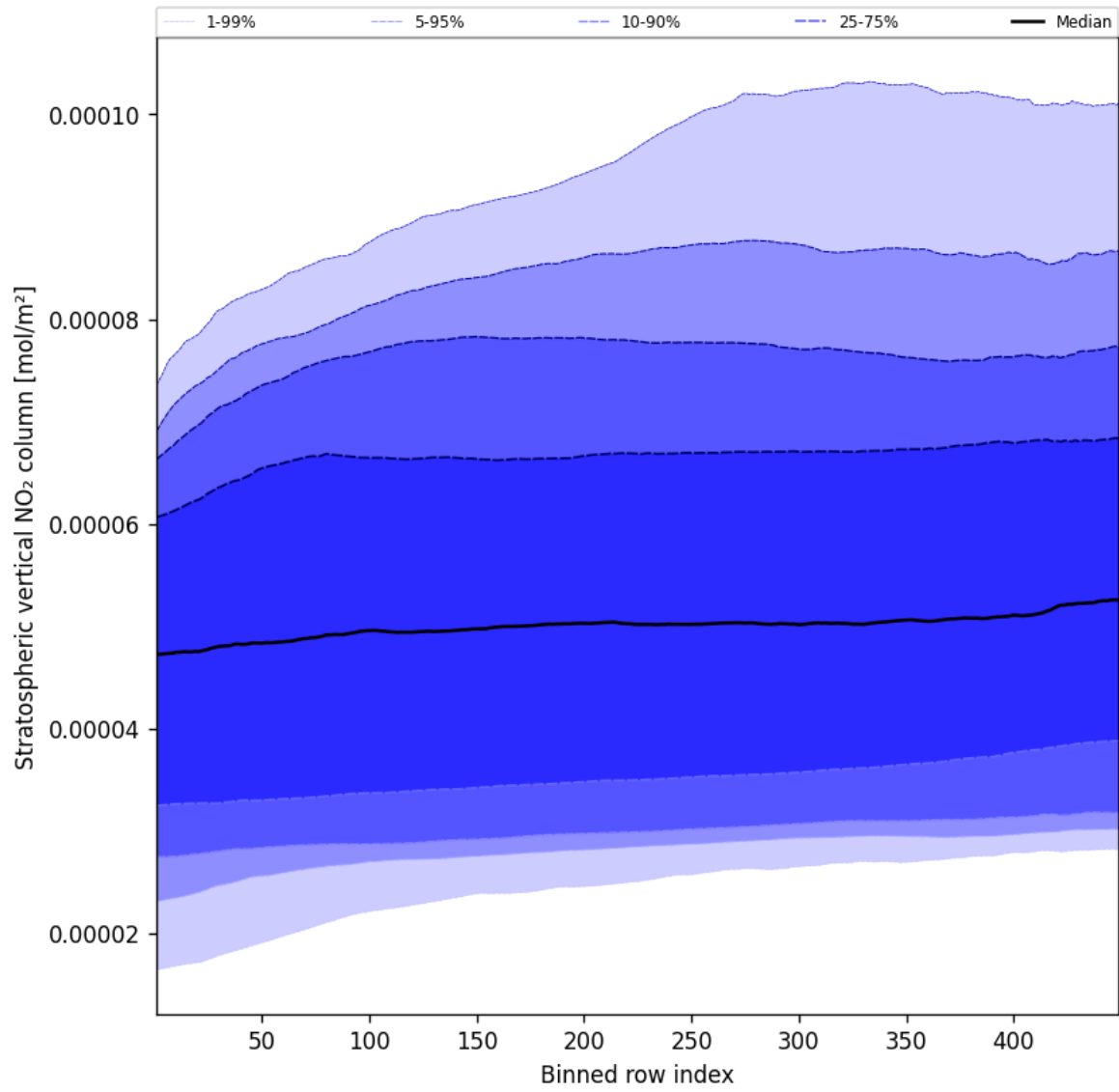
Figure 51: Along track statistics of “Stratospheric vertical NO 2 column” for 2025-05-10 to 2025-05-11
