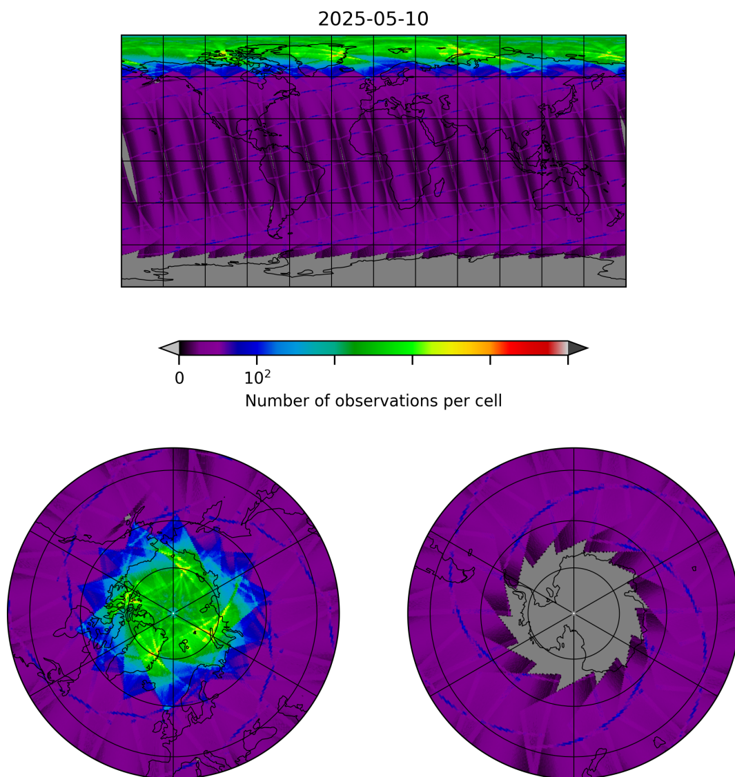
Figure 8: Map of the number of observations for 2025-05-10 to 2025-05-11
