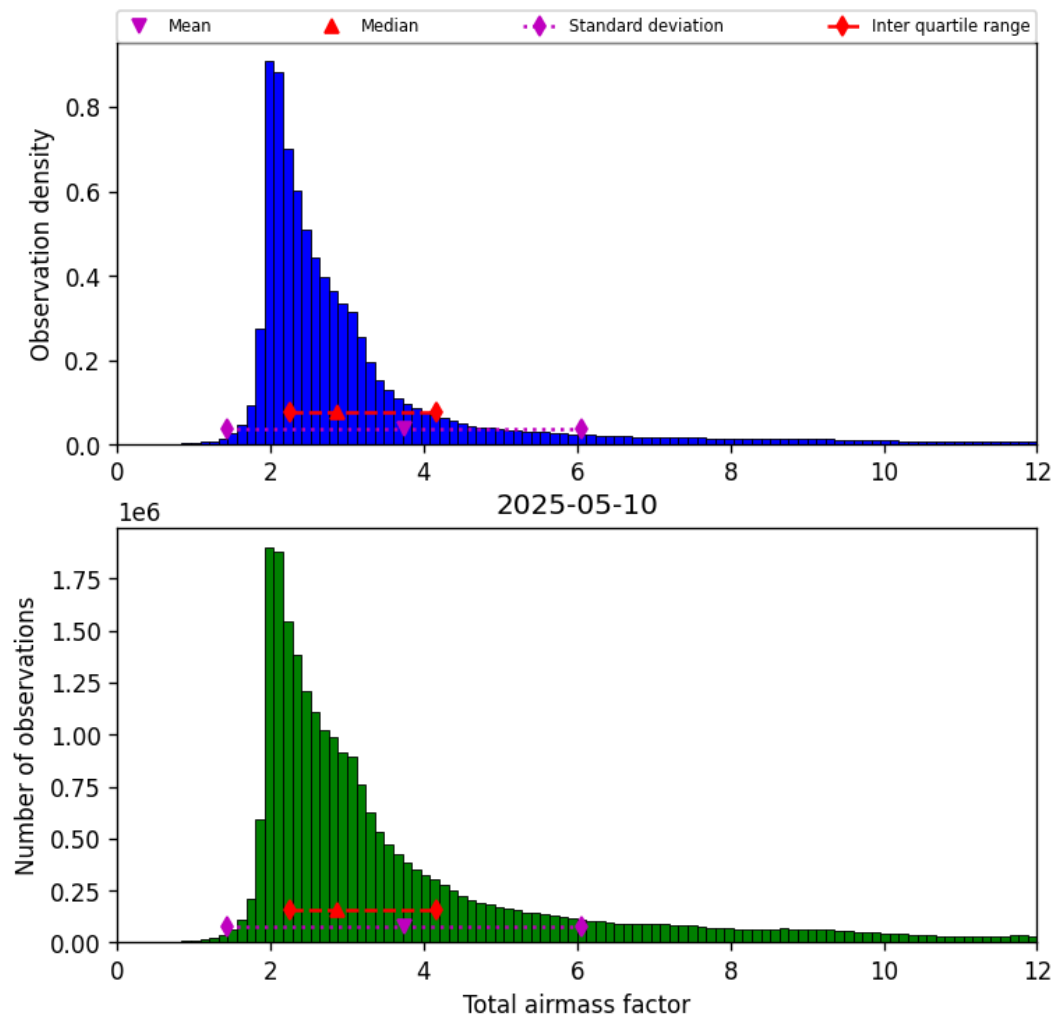
Figure 30: Histogram of “Total airmass factor” for 2025-05-10 to 2025-05-11
