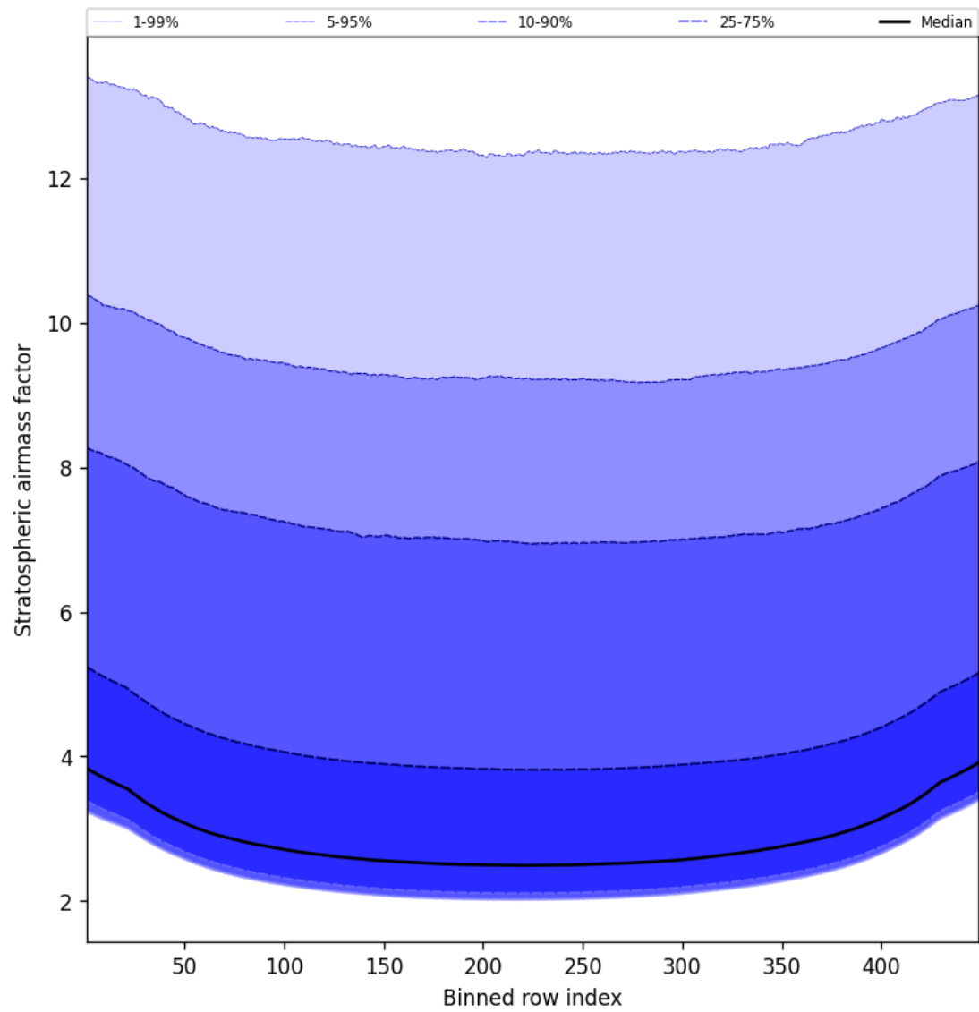
Figure 59: Along track statistics of “Stratospheric airmass factor” for 2025-05-10 to 2025-05-11
