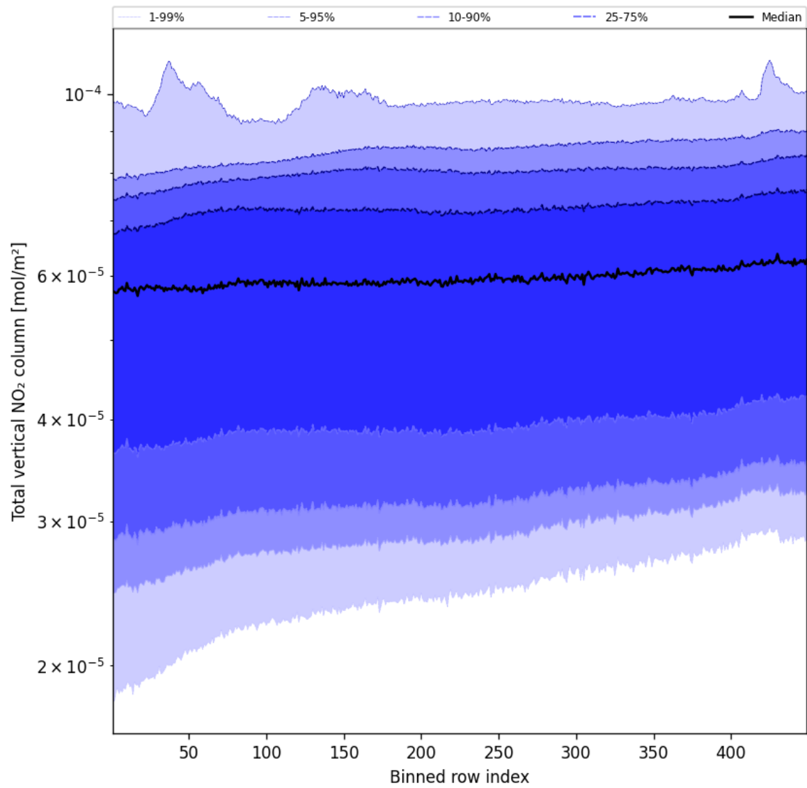
Figure 53: Along track statistics of “Total vertical NO 2 column” for 2025-05-11 to 2025-05-12
