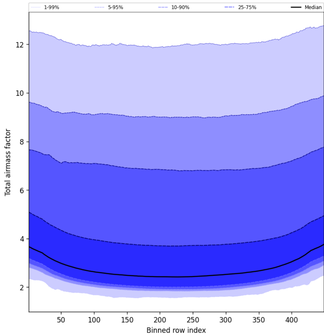
Figure 47: Along track statistics of “Total airmass factor” for 2025-05-11 to 2025-05-12
