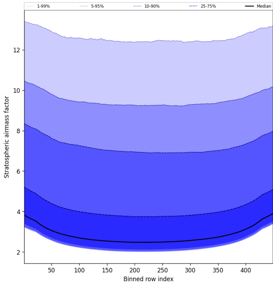
Figure 59: Along track statistics of “Stratospheric airmass factor” for 2025-05-11 to 2025-05-12
