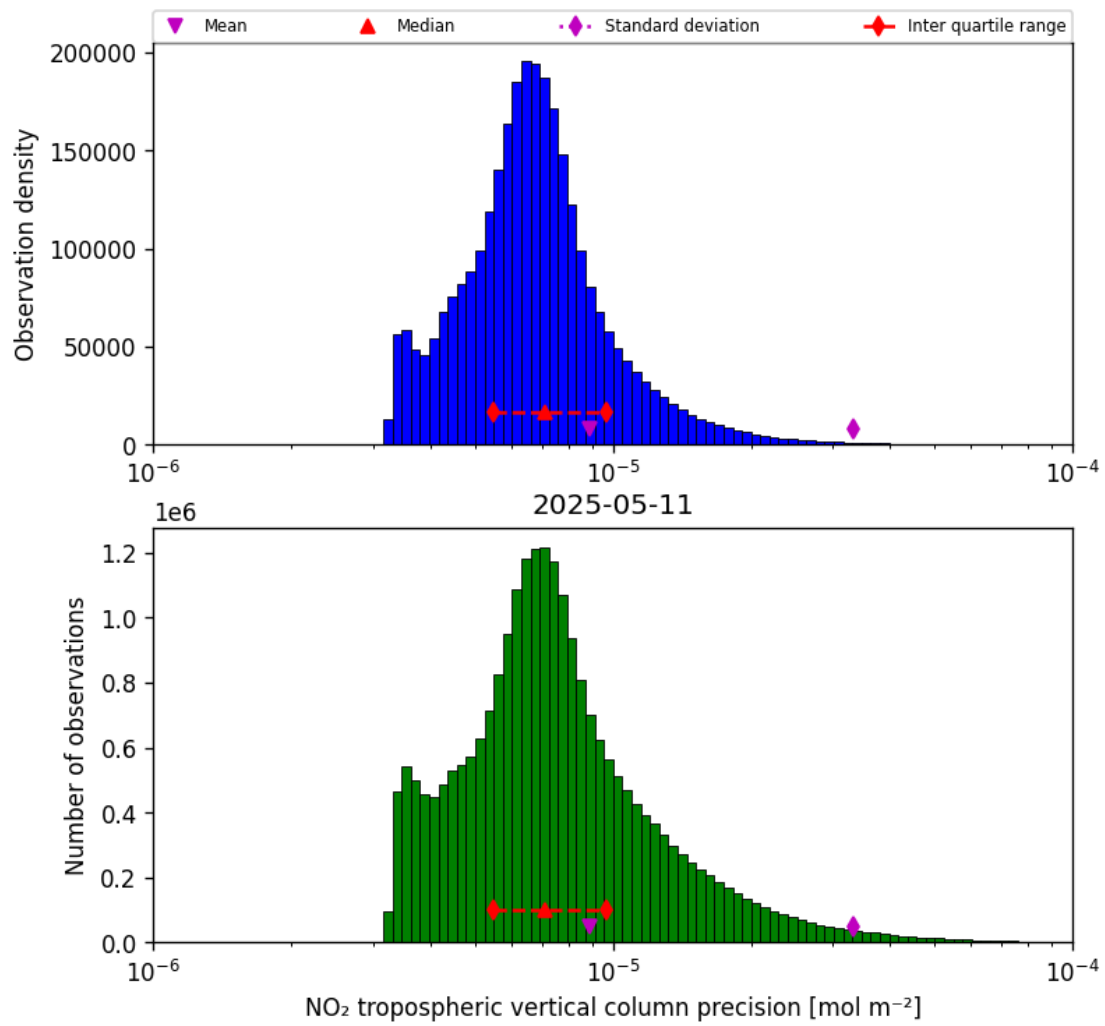
Figure 28: Histogram of “NO 2 tropospheric vertical column precision” for 2025-05-11 to 2025-05-12
