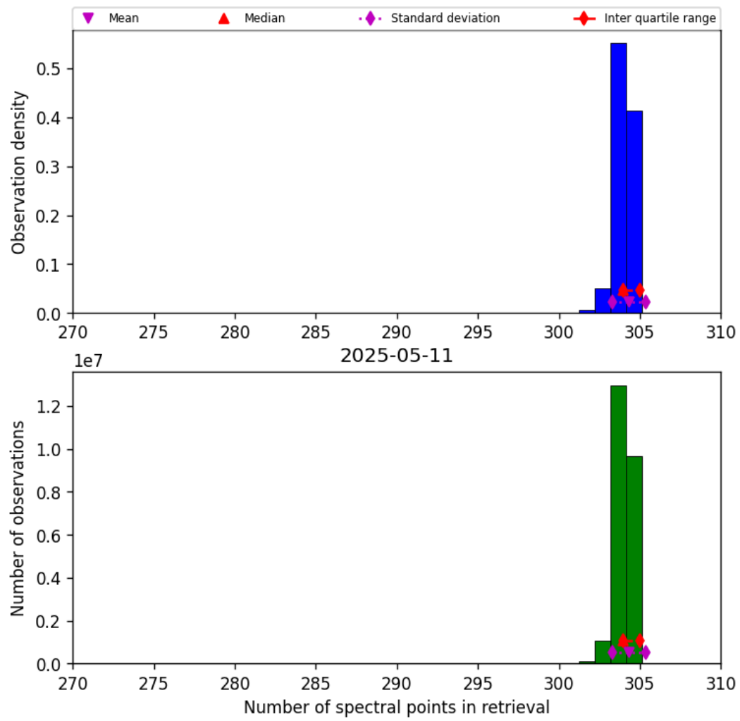
Figure 31: Histogram of “Number of spectral points in retrieval” for 2025-05-11 to 2025-05-12
