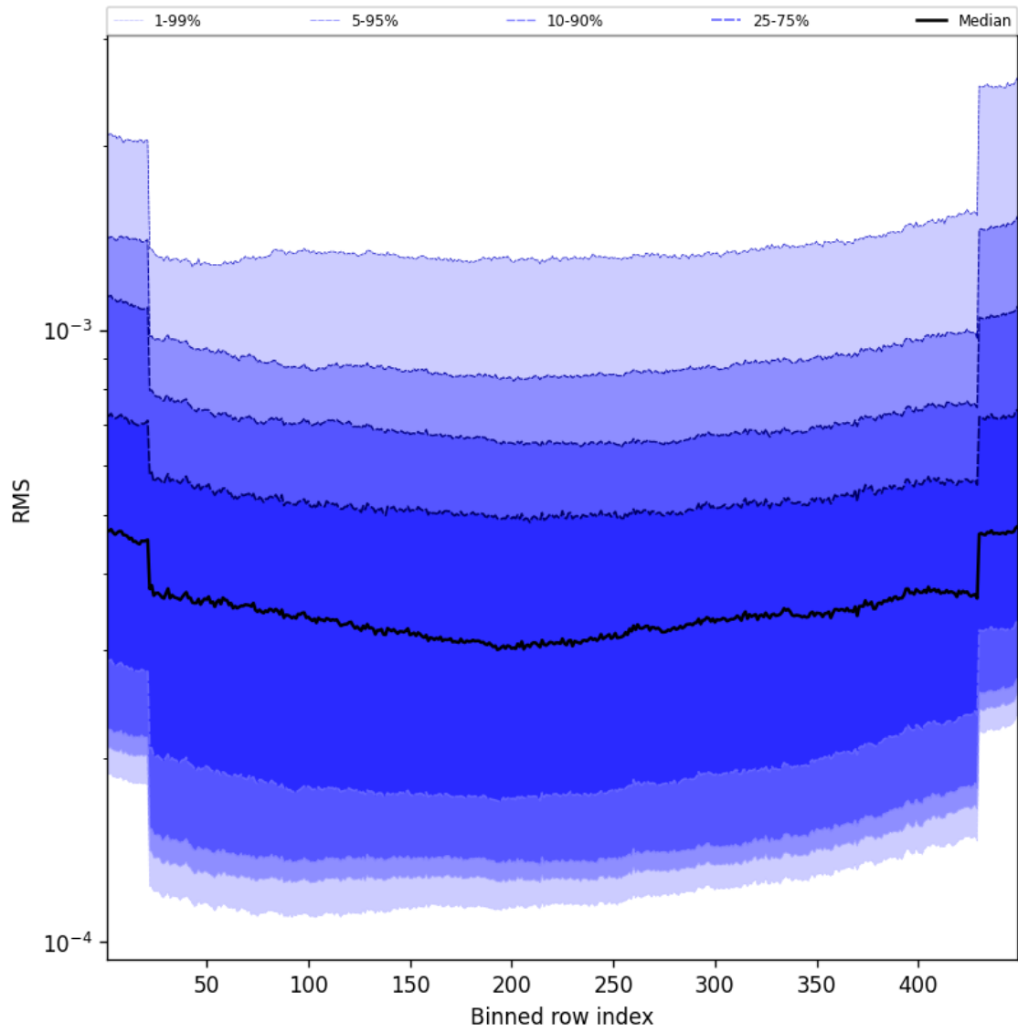
Figure 58: Along track statistics of “RMS” for 2025-05-11 to 2025-05-12
