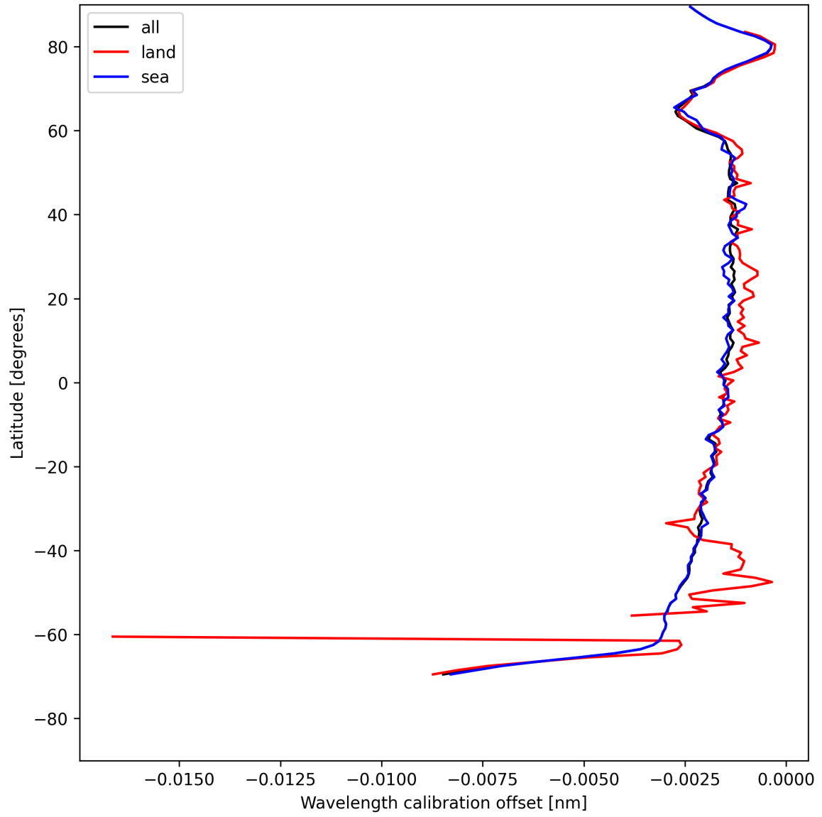
Figure 16: Zonal average of “Wavelength calibration offset” for 2025-05-11 to 2025-05-12.
