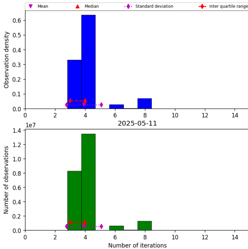
Figure 32: Histogram of “Number of iterations” for 2025-05-11 to 2025-05-12
