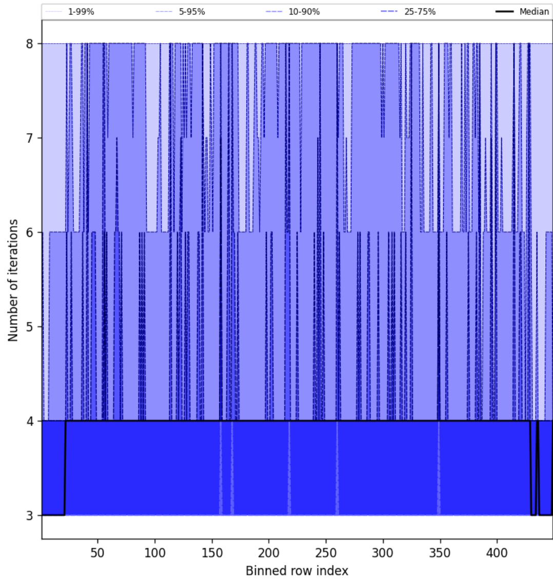
Figure 49: Along track statistics of “Number of iterations” for 2025-05-11 to 2025-05-12
