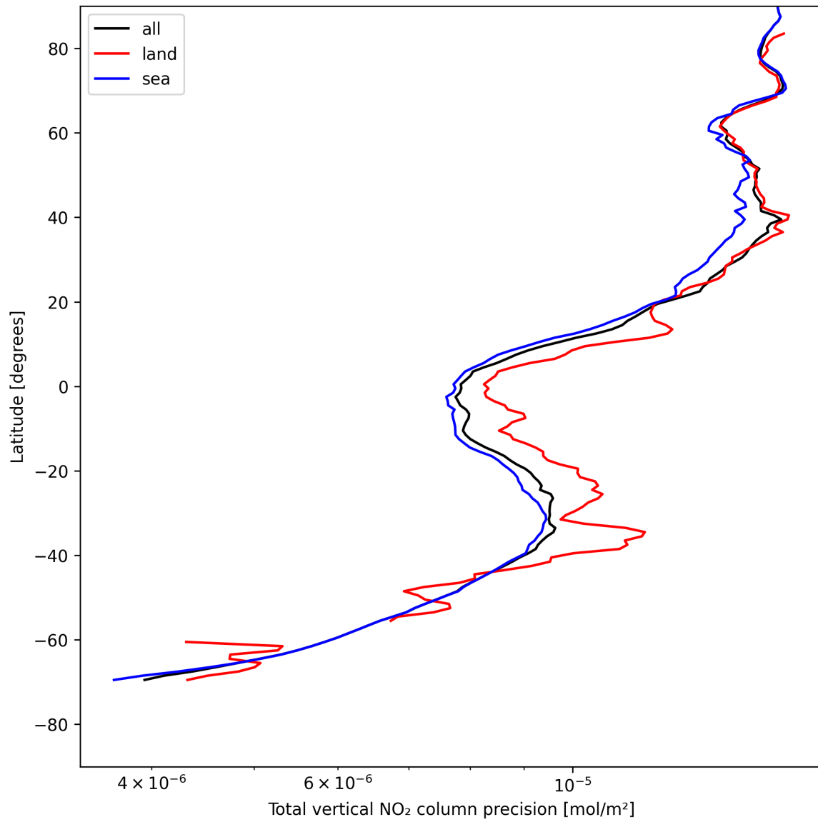
Figure 20: Zonal average of “Total vertical NO 2 column precision” for 2025-05-11 to 2025-05-12.
