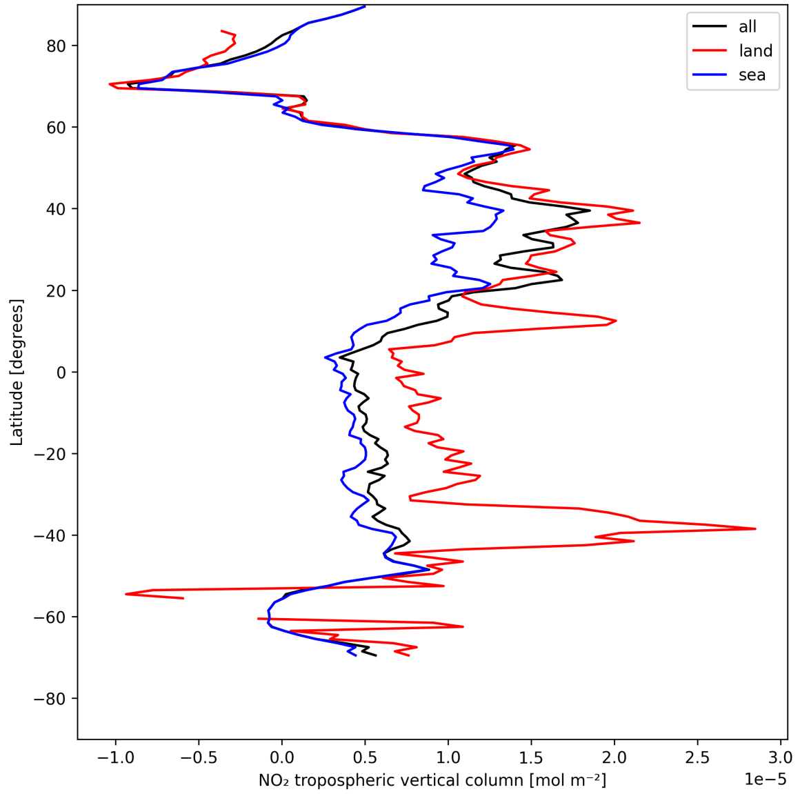
Figure 10: Zonal average of “NO 2 tropospheric vertical column” for 2025-05-11 to 2025-05-12.
