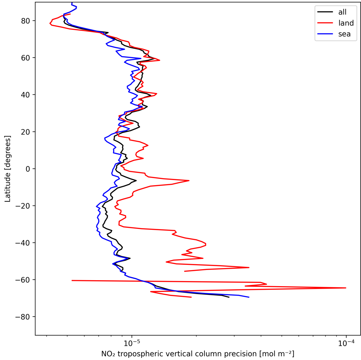
Figure 11: Zonal average of “NO 2 tropospheric vertical column precision” for 2025-05-11 to 2025-05-12.
