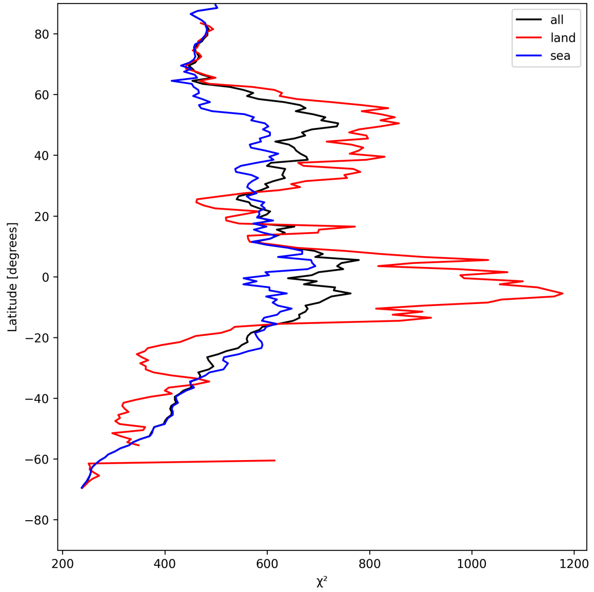
Figure 23: Zonal average of “ \chi^2 ” for 2025-05-11 to 2025-05-12.
