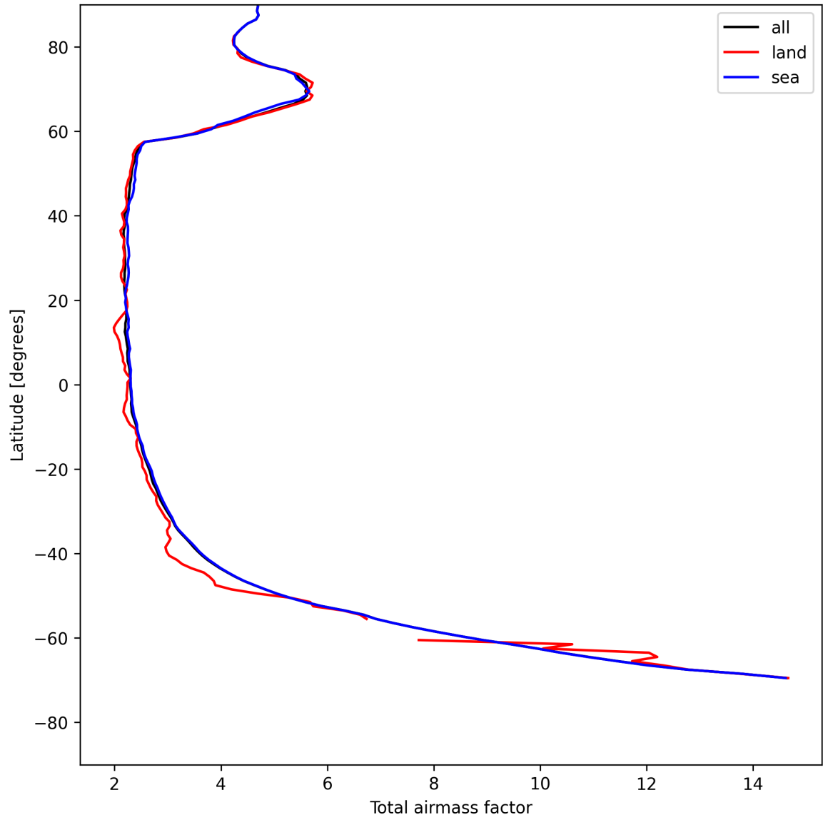
Figure 13: Zonal average of “Total airmass factor” for 2025-05-11 to 2025-05-12.
