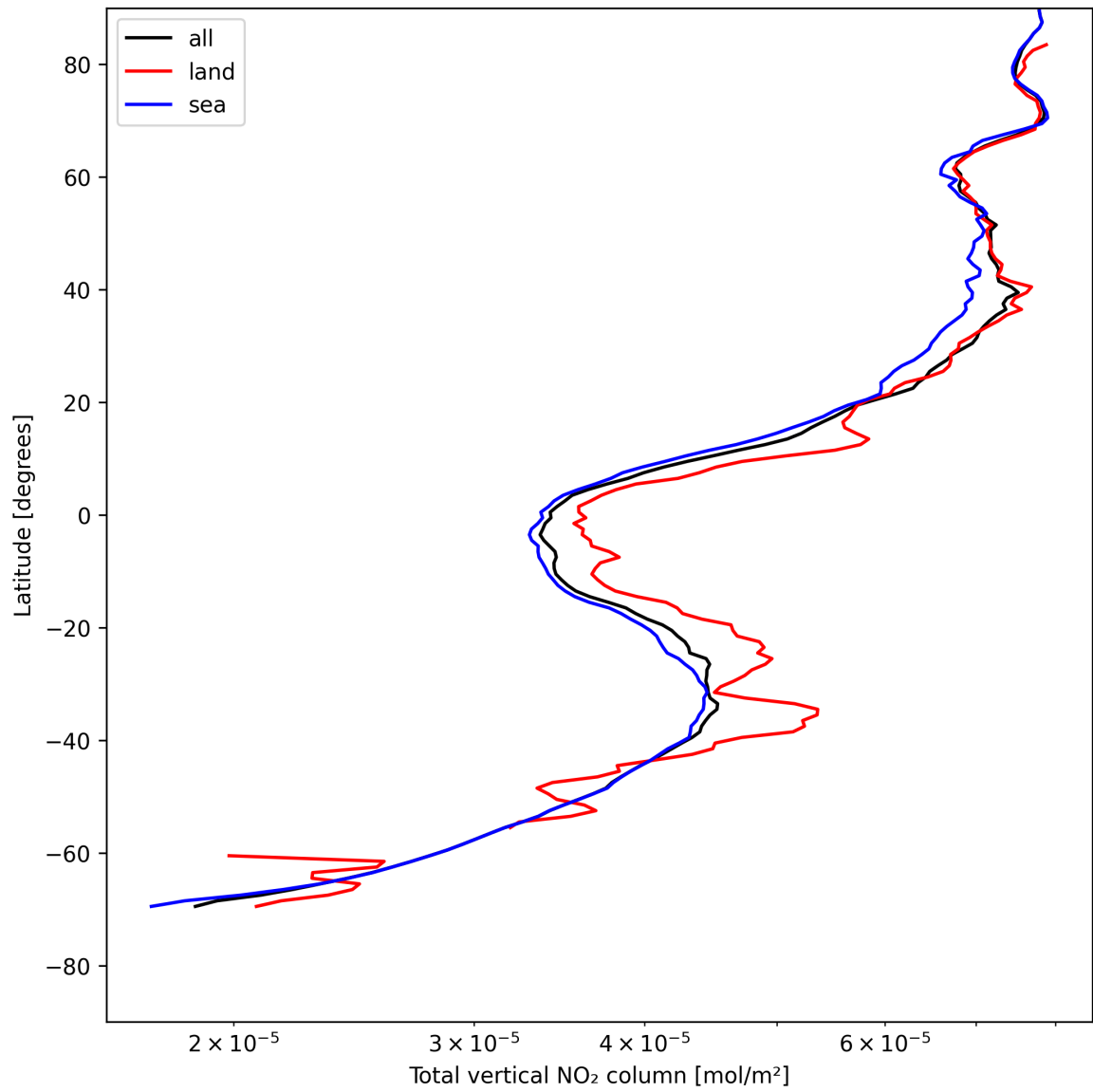
Figure 19: Zonal average of “Total vertical NO 2 column” for 2025-05-11 to 2025-05-12.
