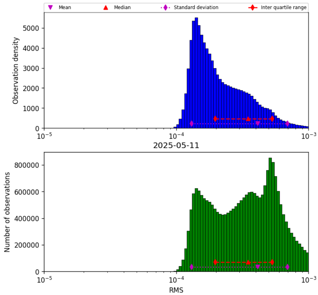
Figure 41: Histogram of “RMS” for 2025-05-11 to 2025-05-12
