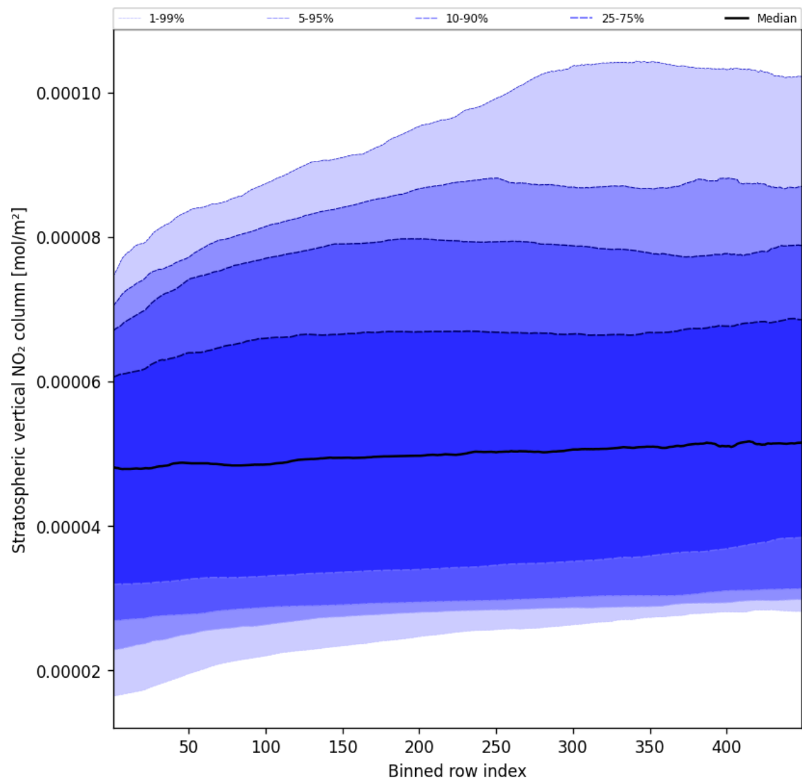
Figure 51: Along track statistics of “Stratospheric vertical NO 2 column” for 2025-05-11 to 2025-05-12
