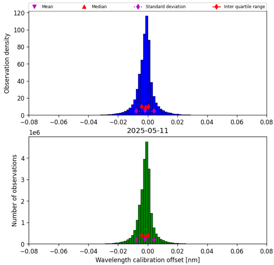
Figure 33: Histogram of “Wavelength calibration offset” for 2025-05-11 to 2025-05-12
