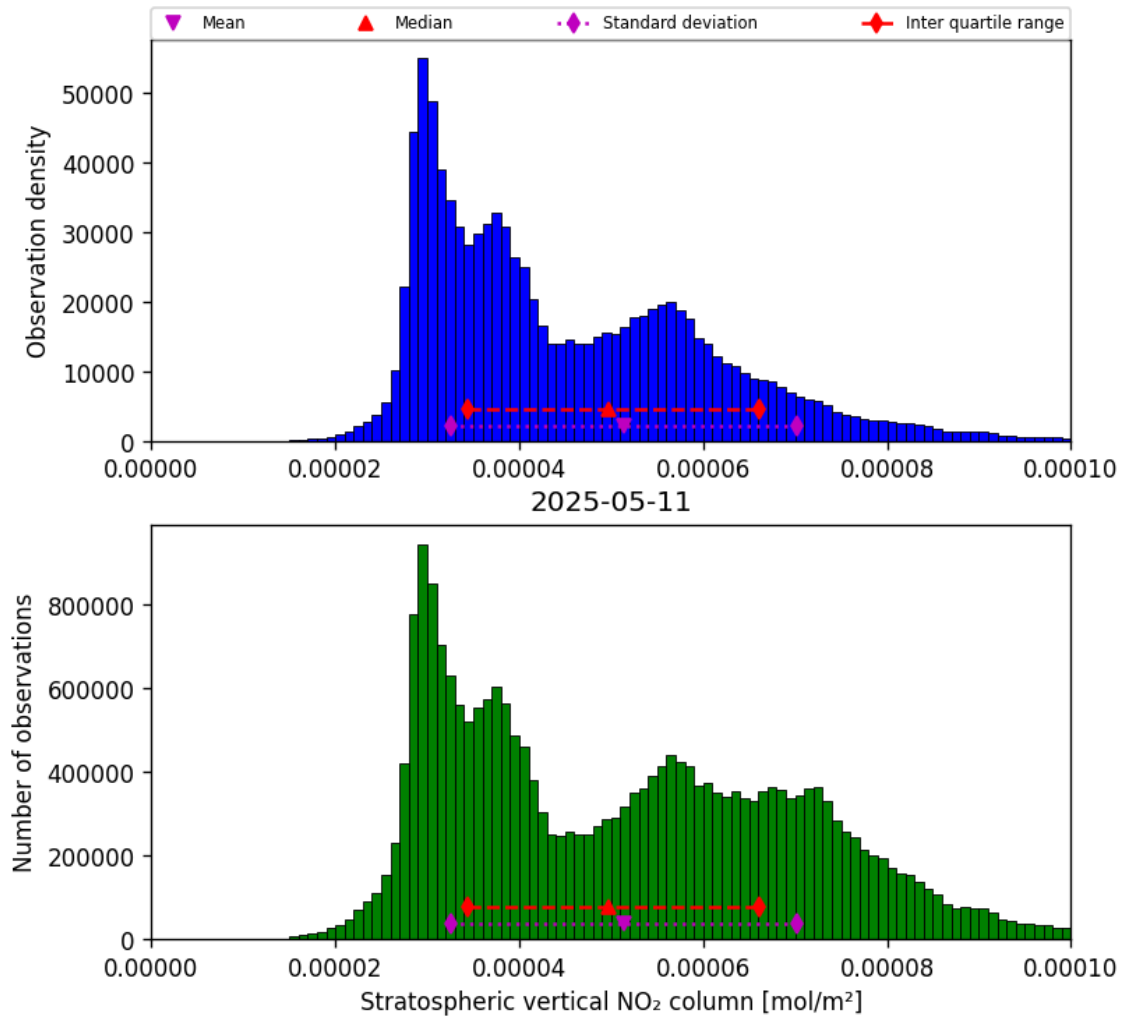
Figure 34: Histogram of “Stratospheric vertical NO 2 column” for 2025-05-11 to 2025-05-12
