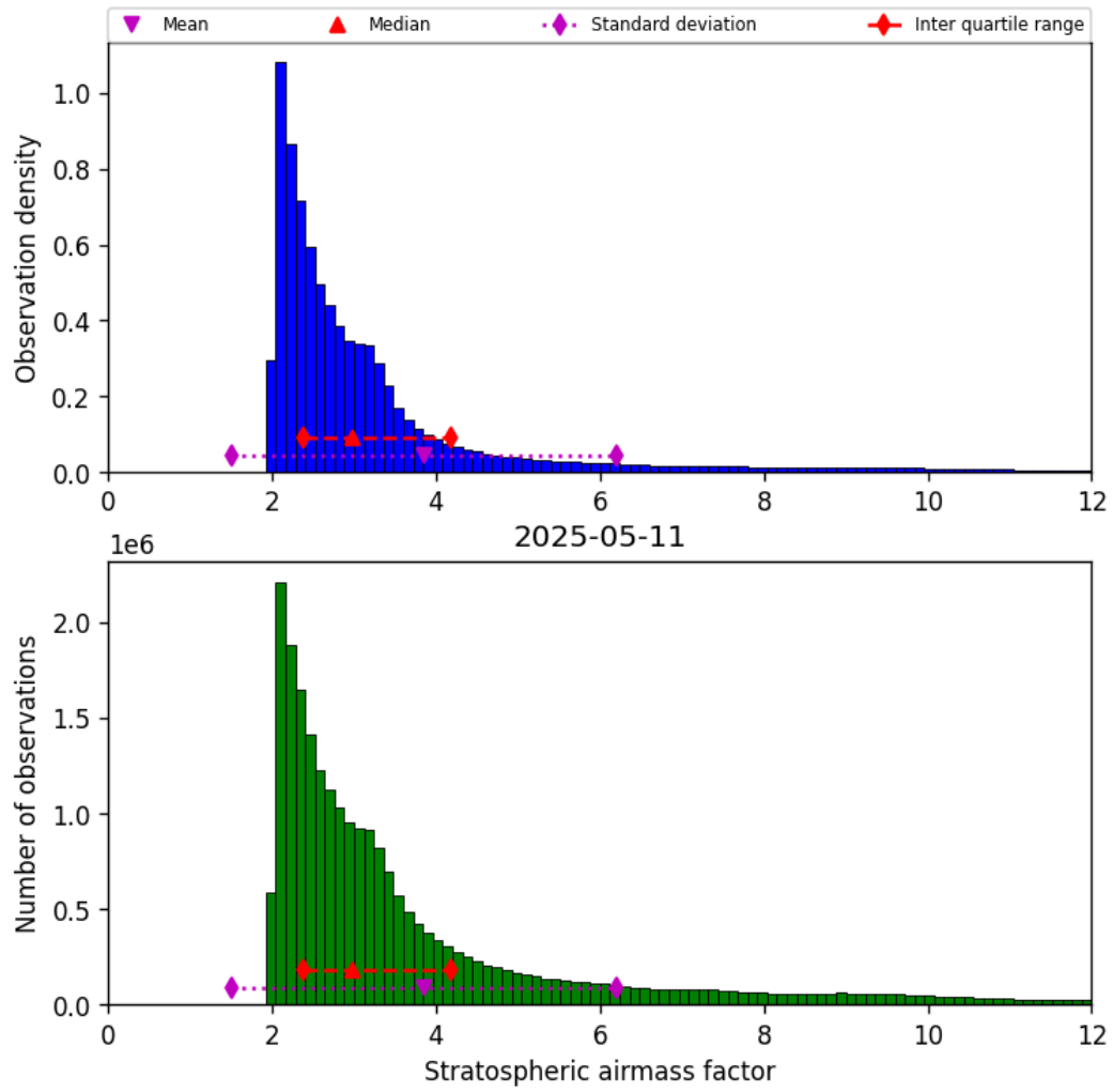
Figure 42: Histogram of “Stratospheric airmass factor” for 2025-05-11 to 2025-05-12
