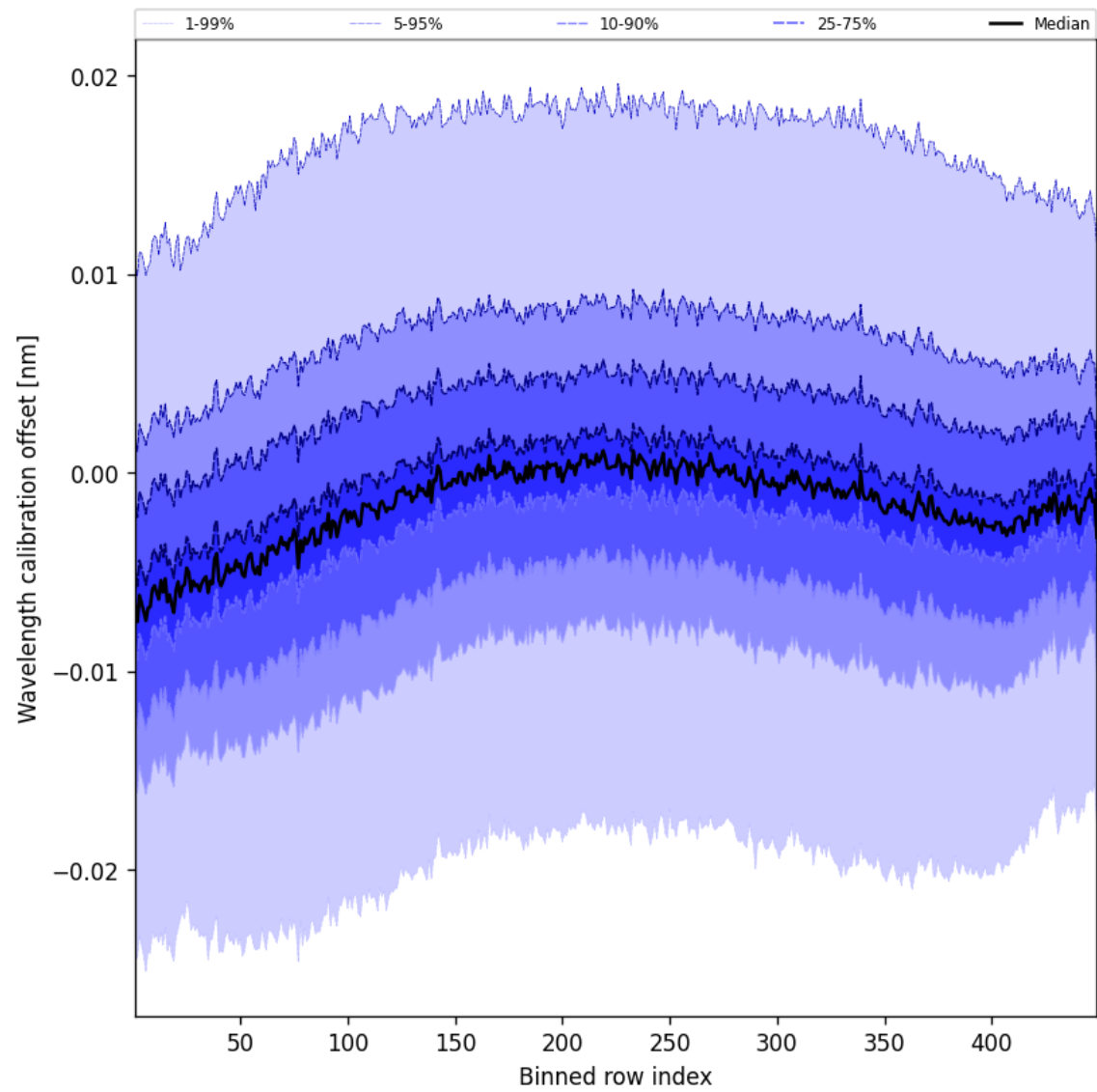
Figure 50: Along track statistics of “Wavelength calibration offset” for 2025-05-11 to 2025-05-12
