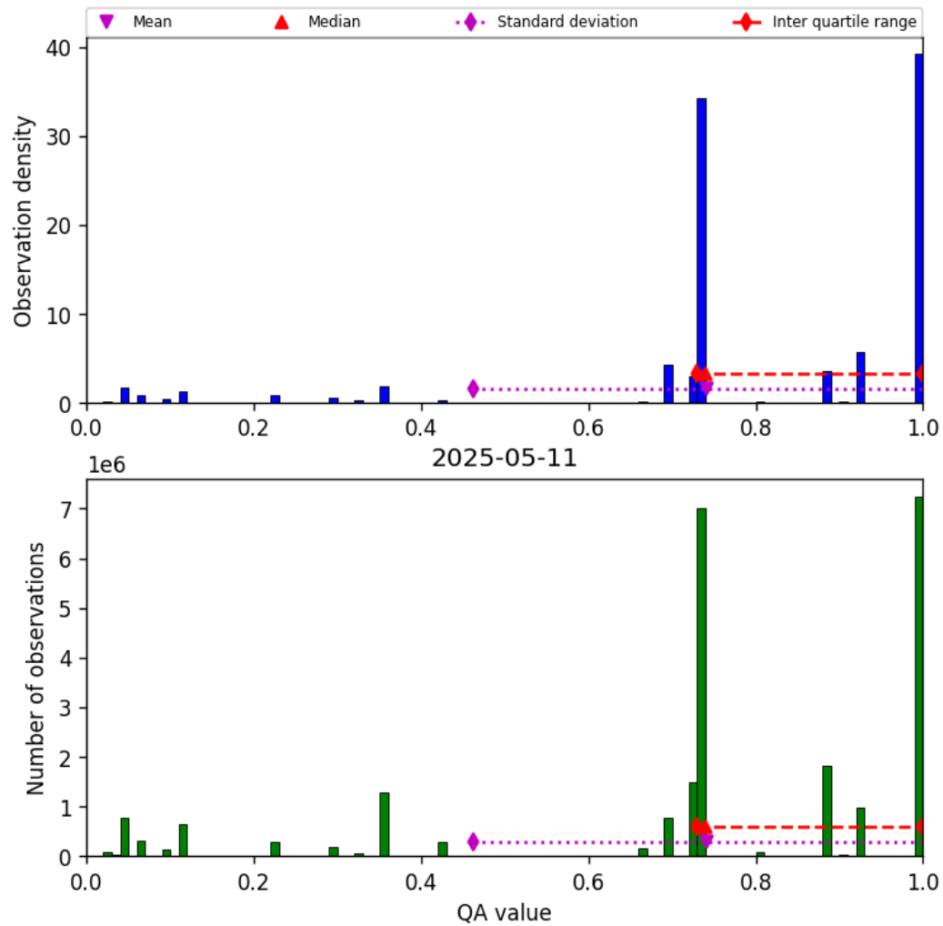
Figure 26: Histogram of “QA value” for 2025-05-11 to 2025-05-12
