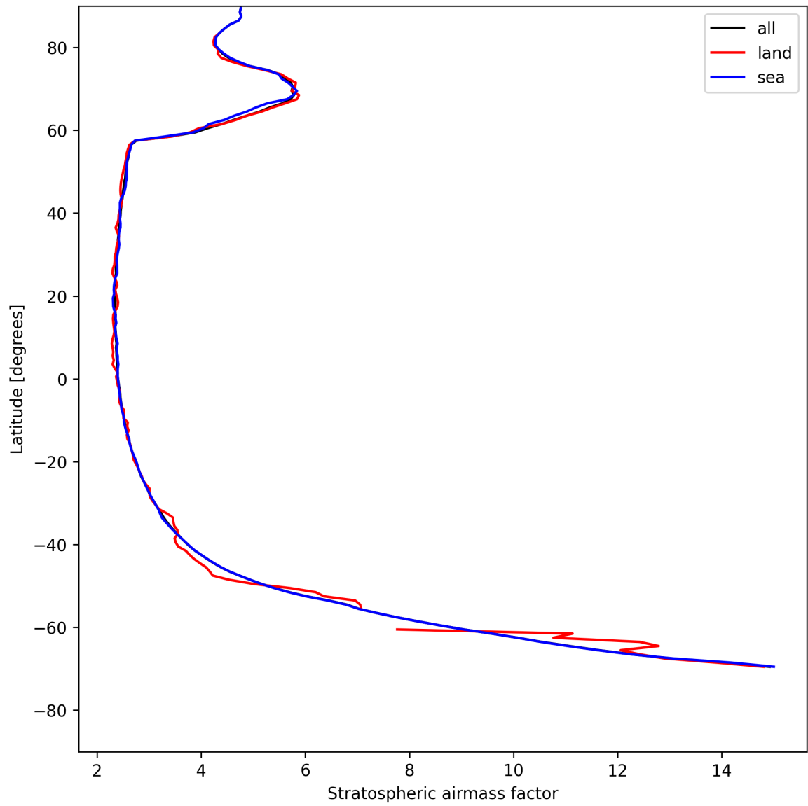
Figure 25: Zonal average of “Stratospheric airmass factor” for 2025-05-11 to 2025-05-12.
