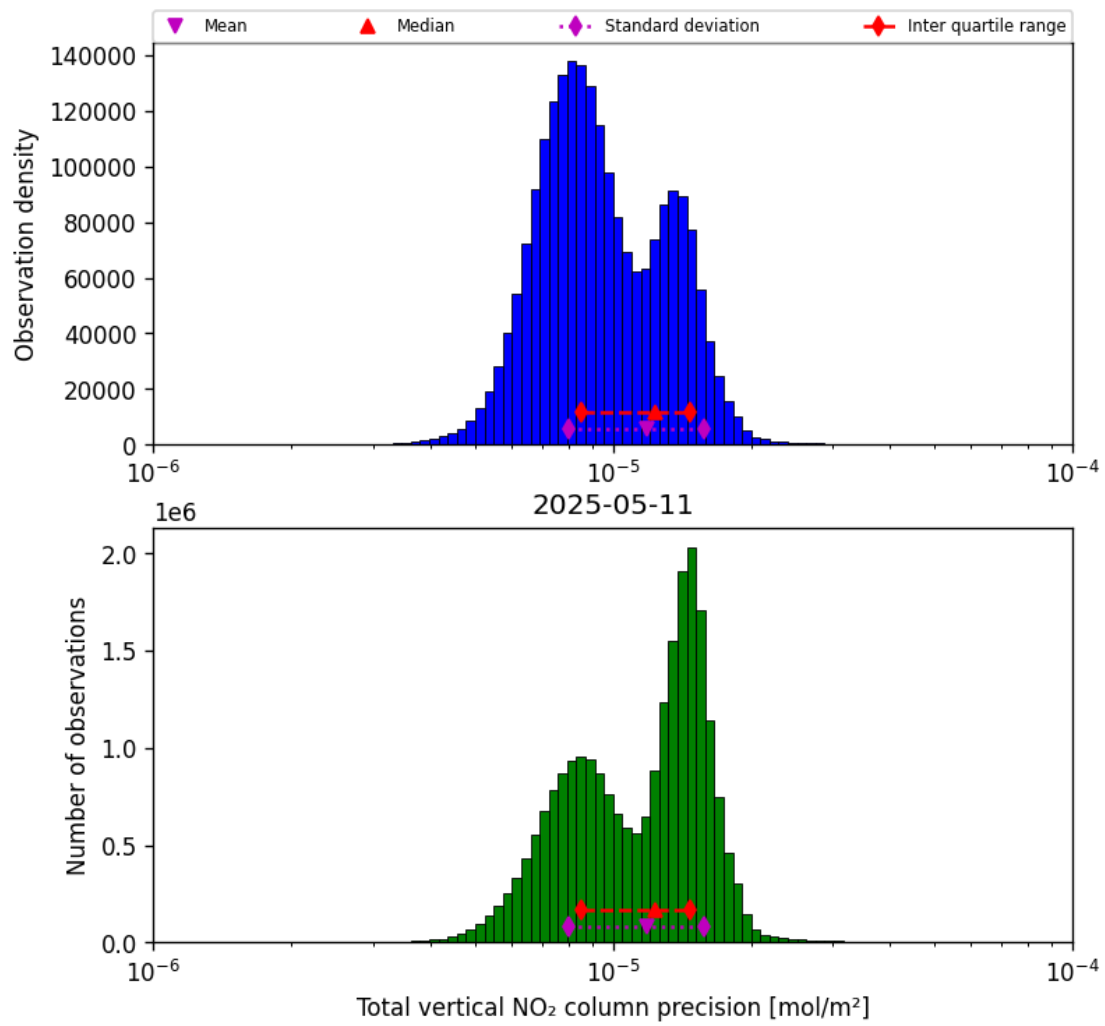
Figure 37: Histogram of “Total vertical NO 2 column precision” for 2025-05-11 to 2025-05-12
