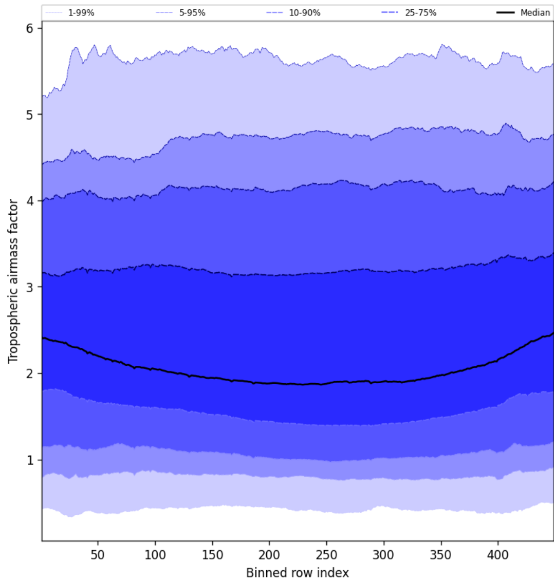
Figure 46: Along track statistics of “Tropospheric airmass factor” for 2025-05-11 to 2025-05-12
