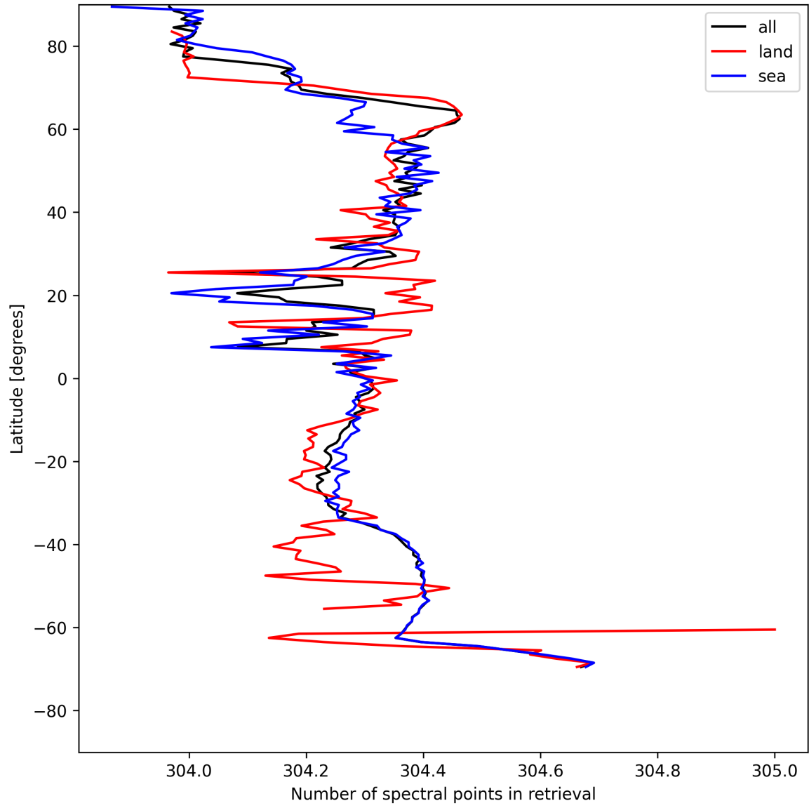
Figure 14: Zonal average of “Number of spectral points in retrieval” for 2025-05-11 to 2025-05-12.
