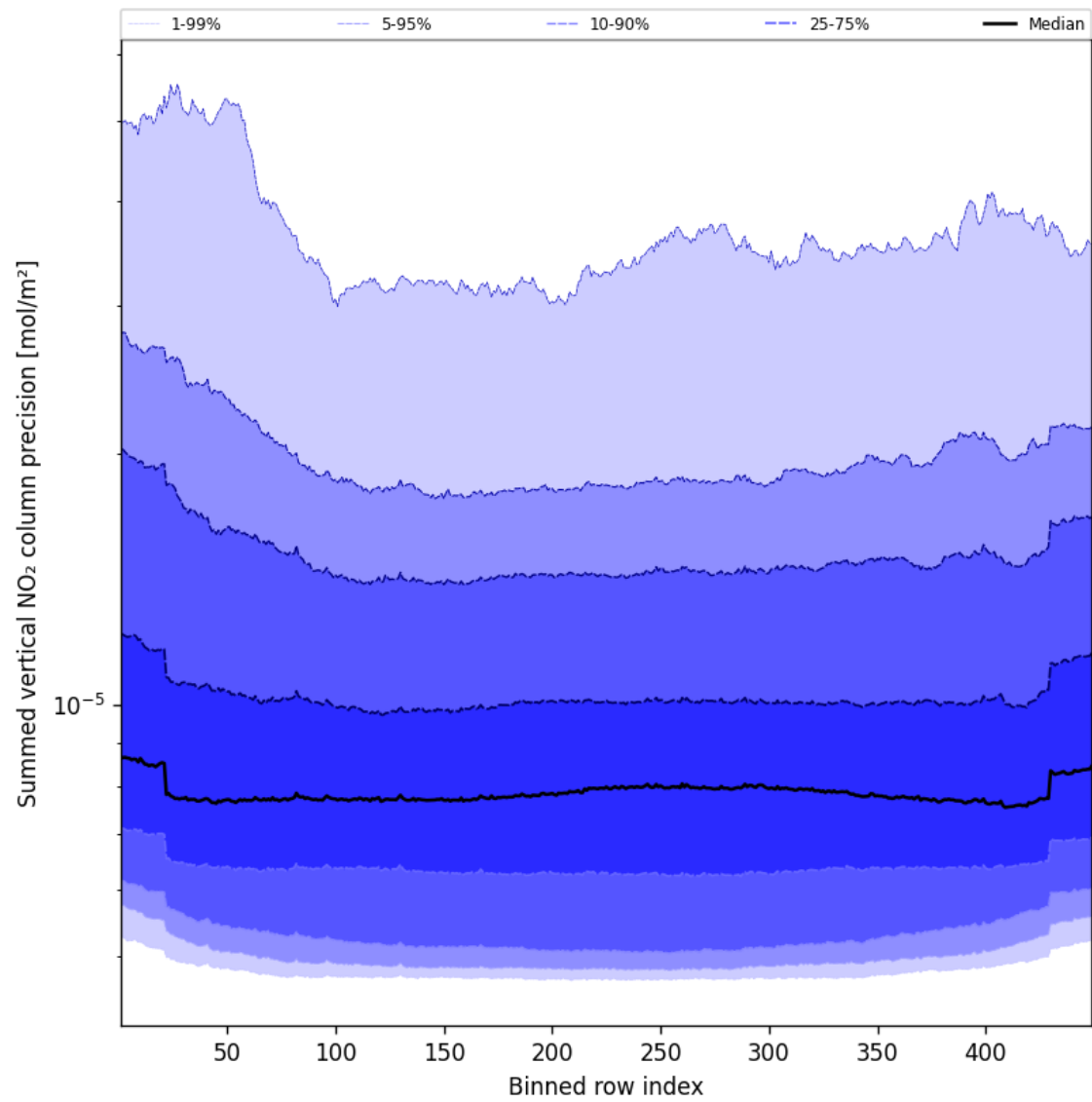
Figure 56: Along track statistics of “Summed vertical NO 2 column precision” for 2025-05-11 to 2025-05-12
