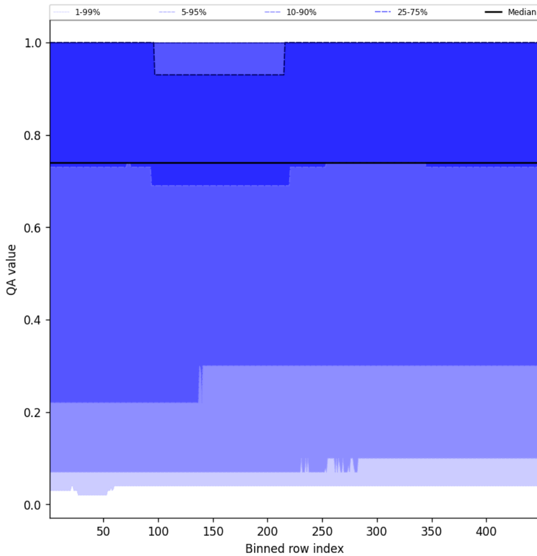
Figure 43: Along track statistics of “QA value” for 2025-05-11 to 2025-05-12
