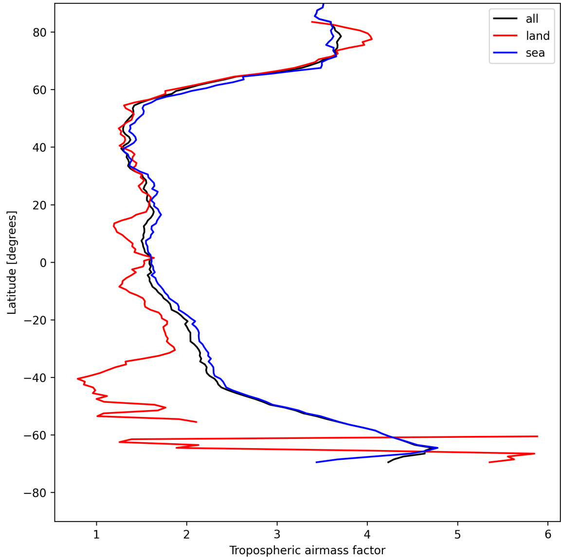
Figure 12: Zonal average of “Tropospheric airmass factor” for 2025-05-11 to 2025-05-12.
