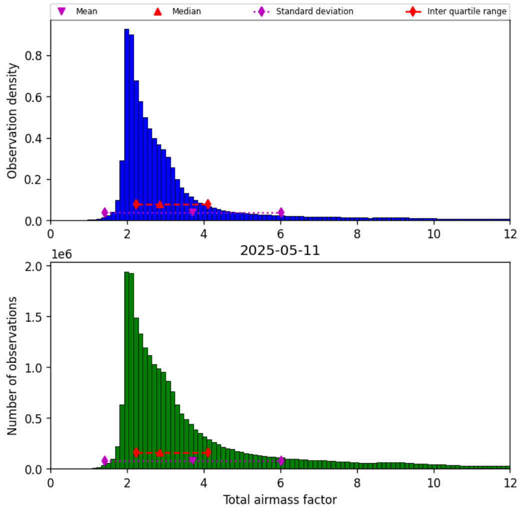
Figure 30: Histogram of “Total airmass factor” for 2025-05-11 to 2025-05-12
