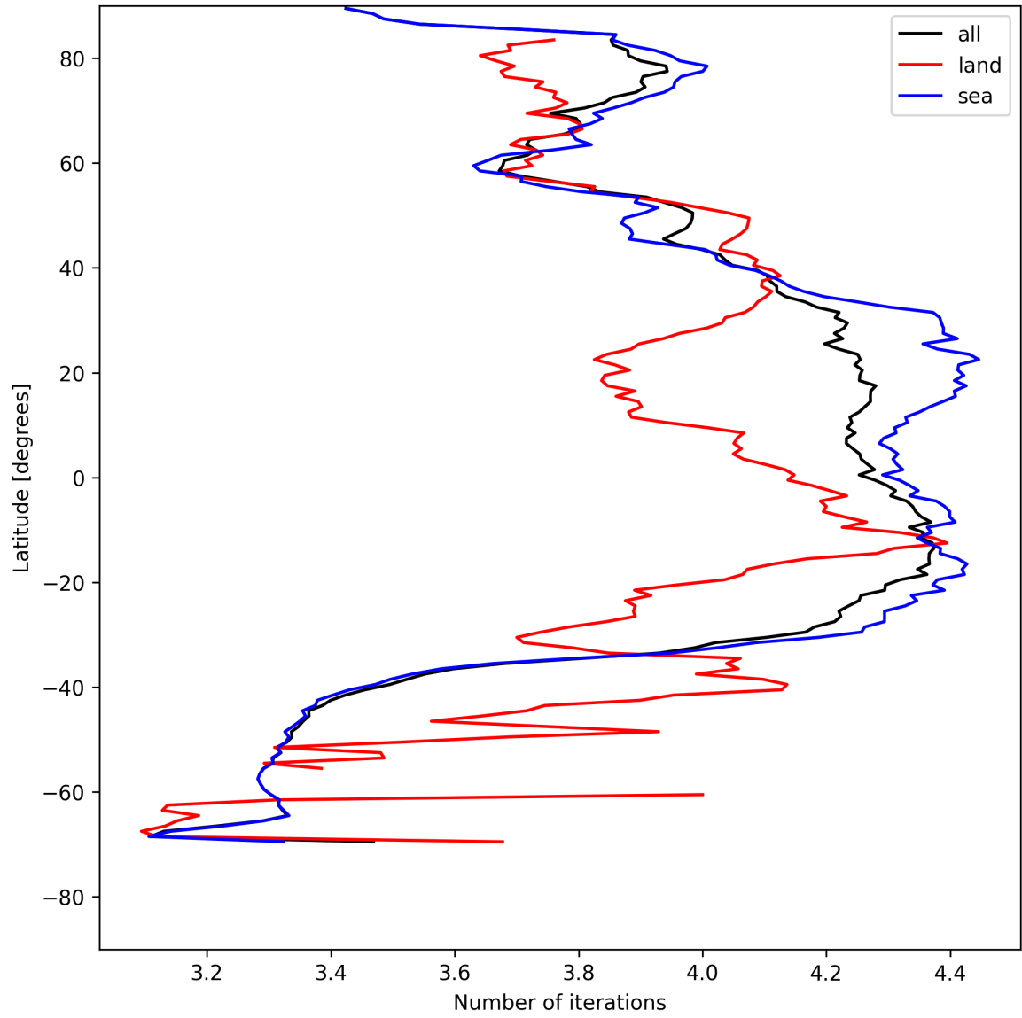
Figure 15: Zonal average of “Number of iterations” for 2025-05-11 to 2025-05-12.
