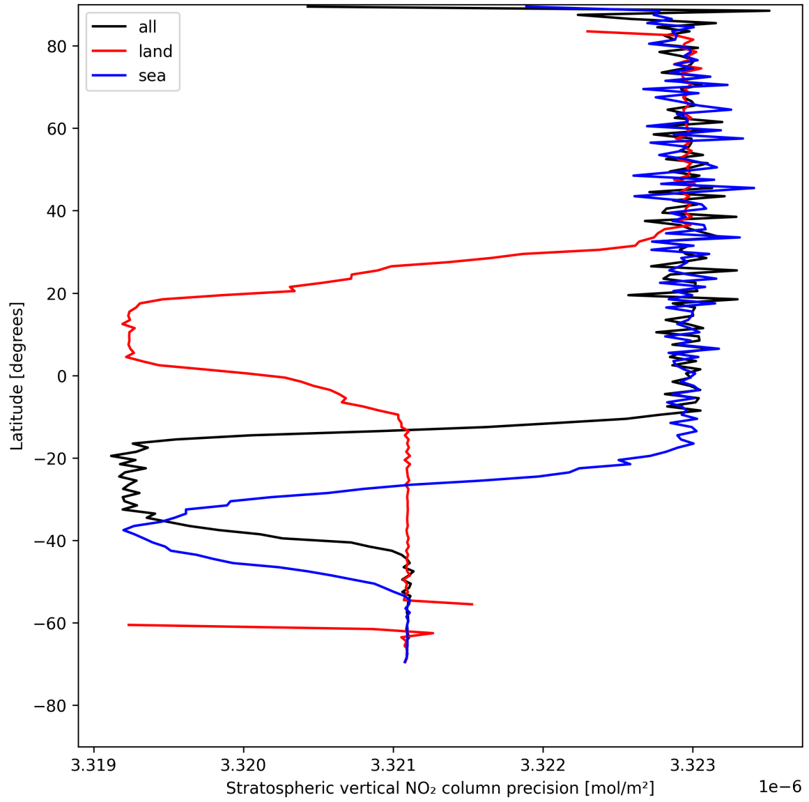
Figure 18: Zonal average of “Stratospheric vertical NO 2 column precision” for 2025-05-11 to 2025-05-12.
