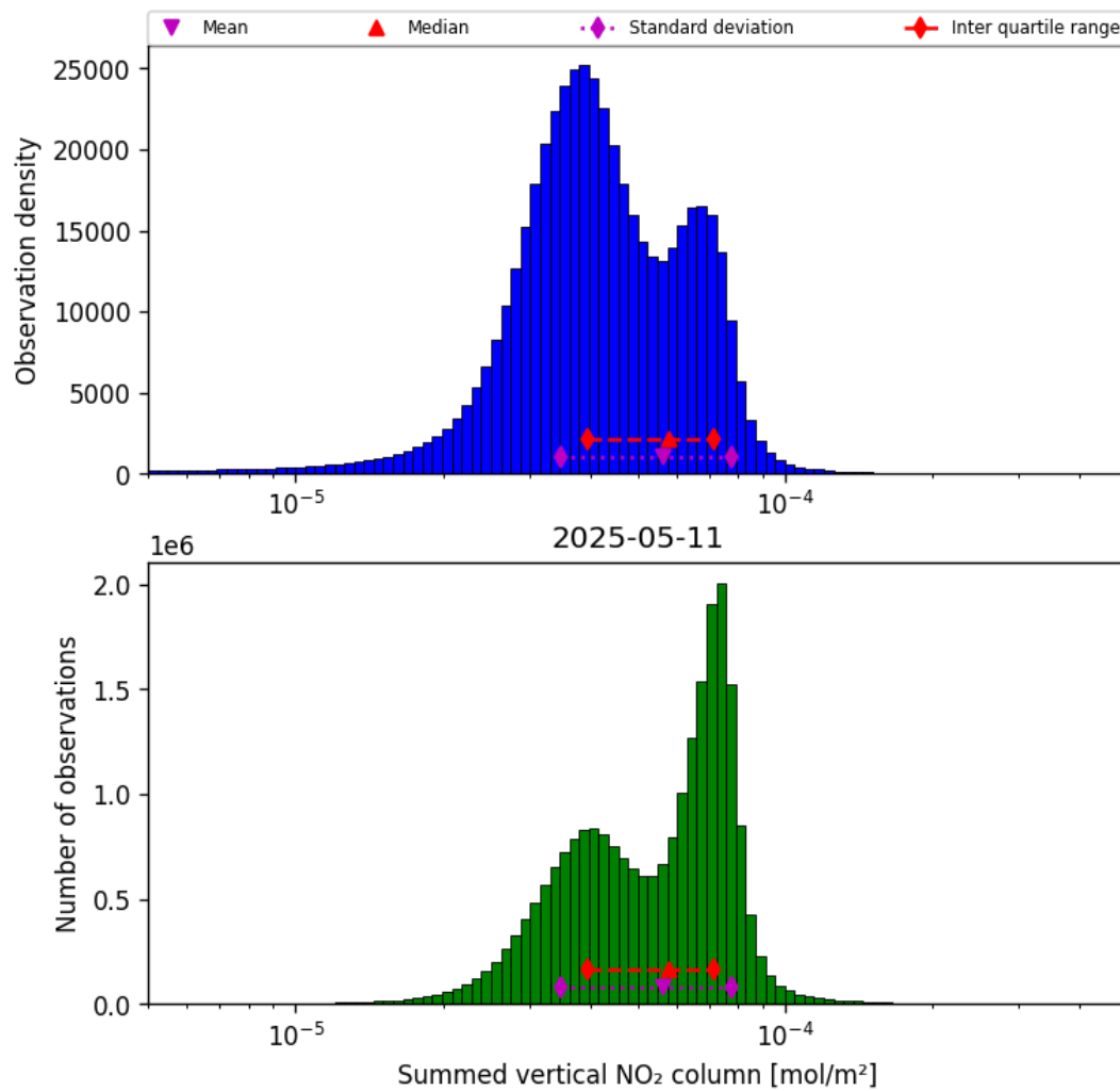
Figure 38: Histogram of "Summed vertical NO 2 column" for 2025-05-11 to 2025-05-12
