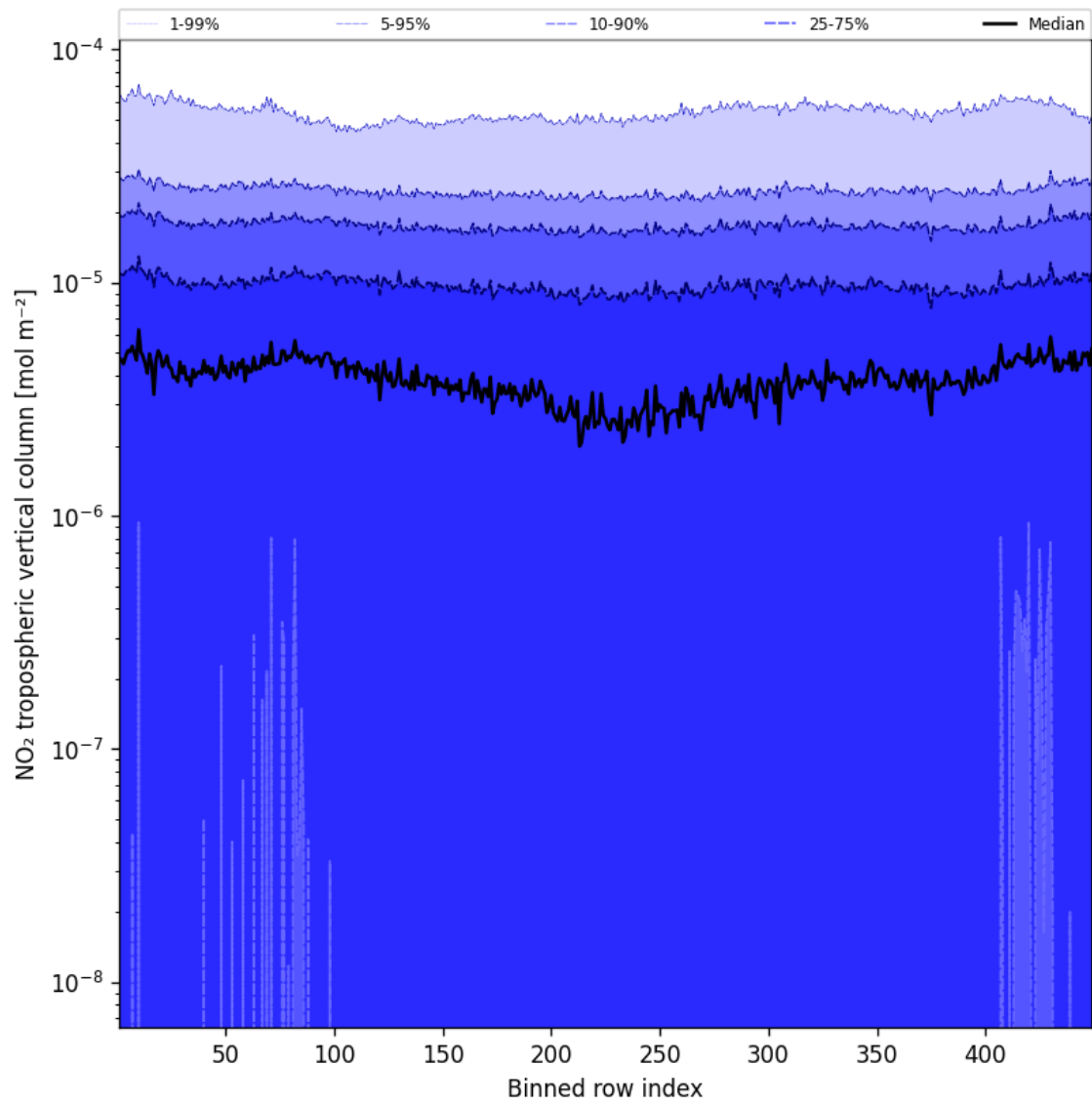
Figure 44: Along track statistics of “NO 2 tropospheric vertical column” for 2025-05-11 to 2025-05-12
