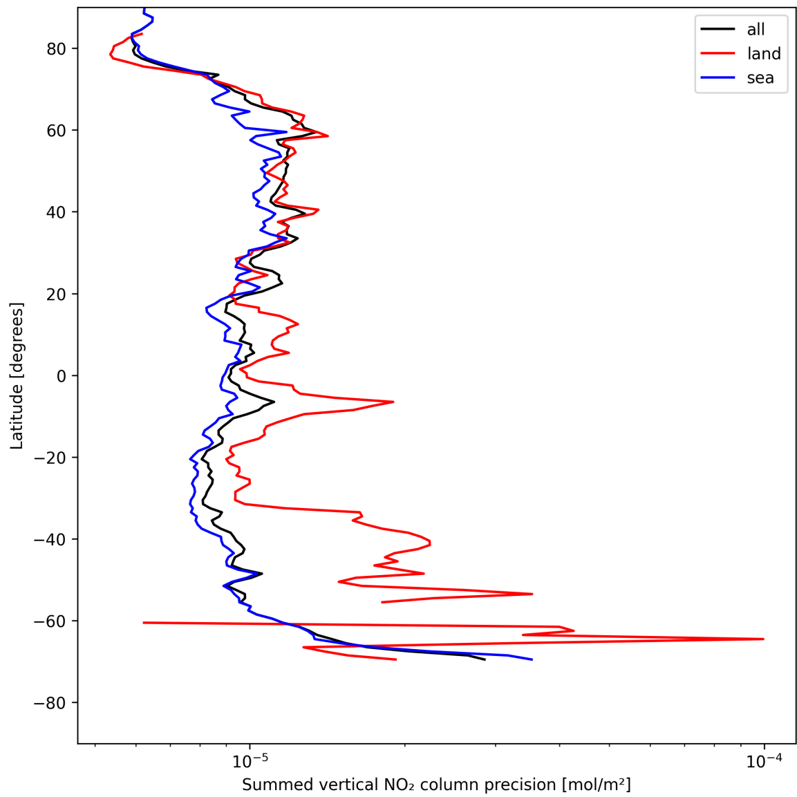
Figure 22: Zonal average of “Summed vertical NO 2 column precision” for 2025-05-11 to 2025-05-12.
