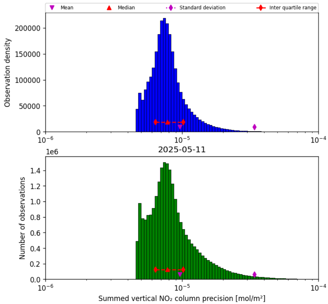
Figure 39: Histogram of “Summed vertical NO 2 column precision” for 2025-05-11 to 2025-05-12
