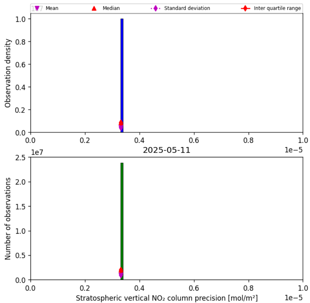
Figure 35: Histogram of “Stratospheric vertical NO 2 column precision” for 2025-05-11 to 2025-05-12
