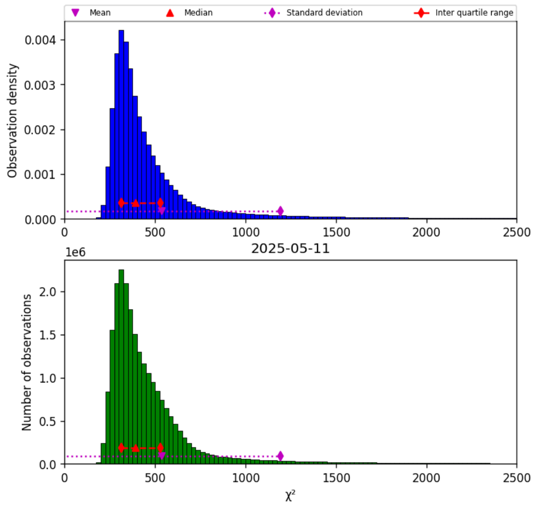
Figure 40: Histogram of “ \chi^2 ” for 2025-05-11 to 2025-05-12
