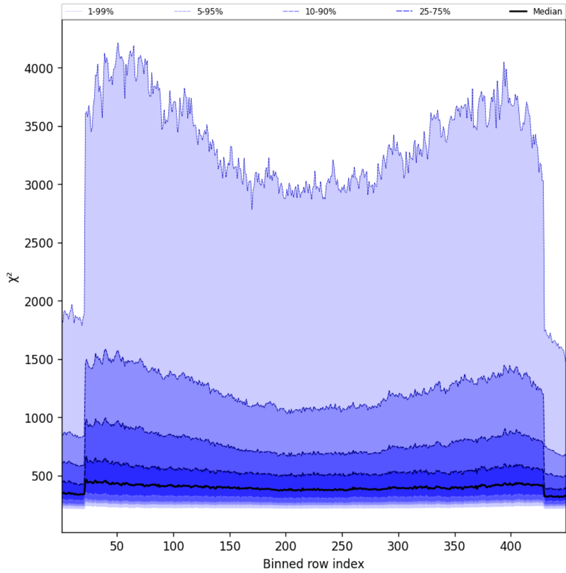
Figure 57: Along track statistics of “ \chi^2 ” for 2025-05-11 to 2025-05-12
