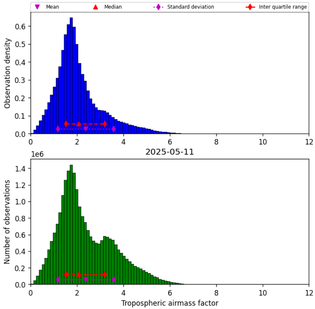
Figure 29: Histogram of “Tropospheric airmass factor” for 2025-05-11 to 2025-05-12
