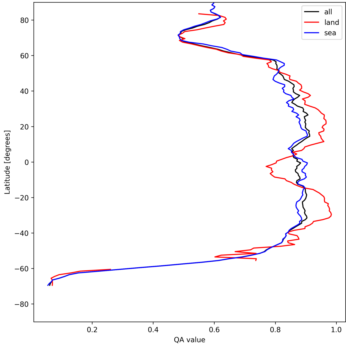
Figure 9: Zonal average of “QA value” for 2025-05-11 to 2025-05-12.
