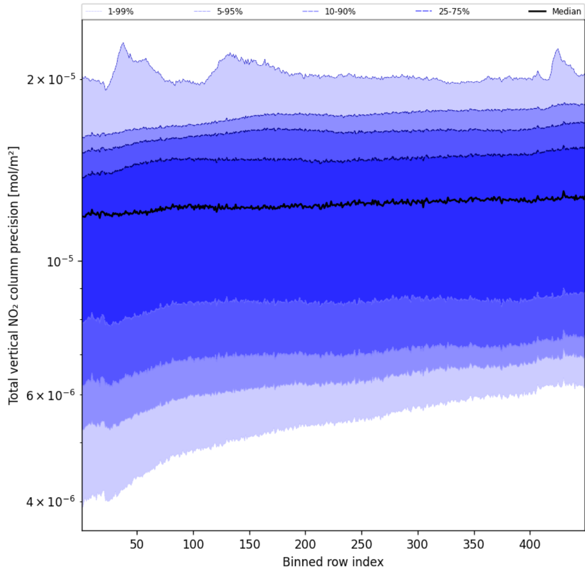
Figure 54: Along track statistics of "Total vertical NO 2 column precision" for 2025-05-11 to 2025-05-12
