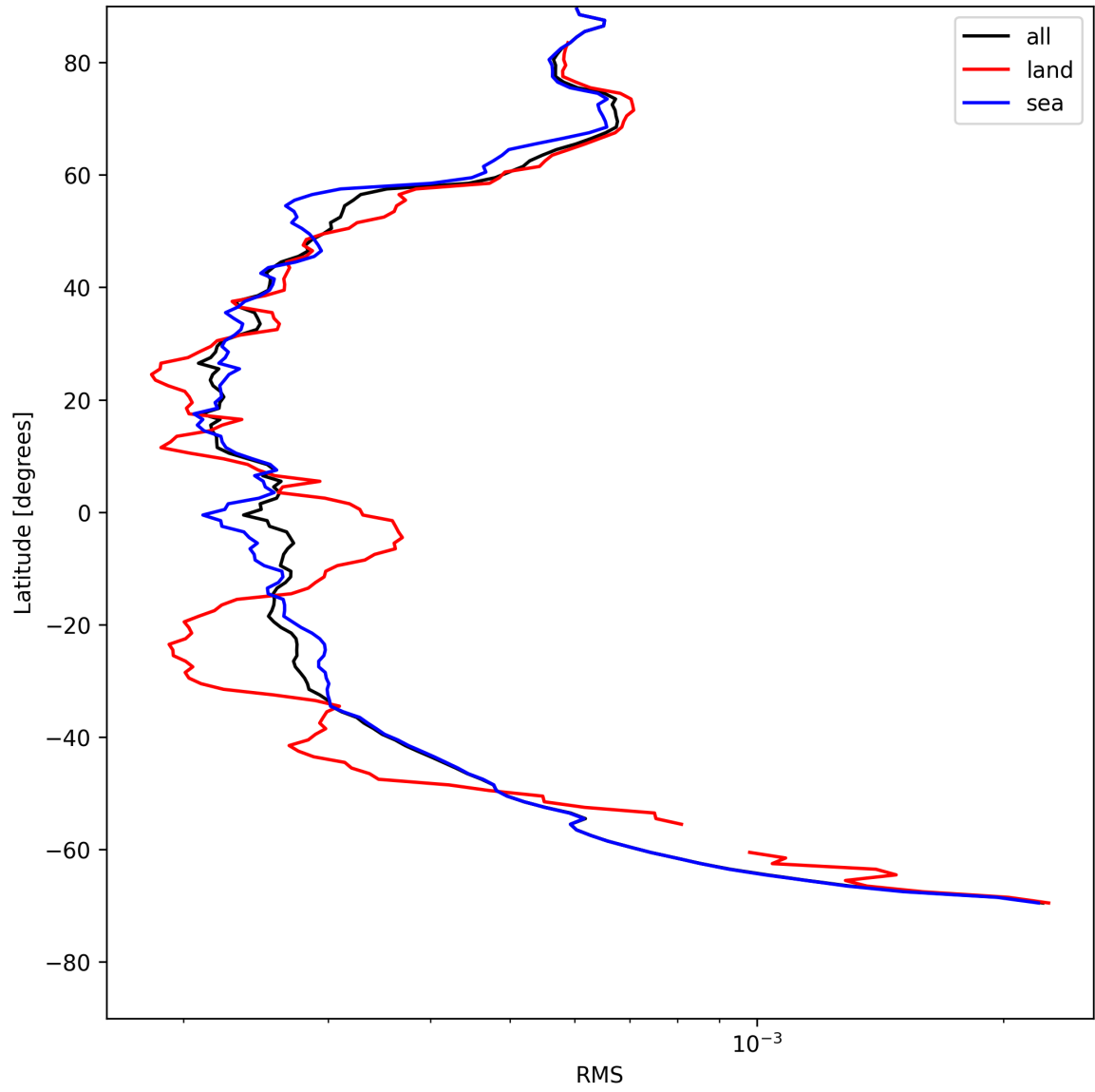
Figure 24: Zonal average of “RMS” for 2025-05-11 to 2025-05-12.
