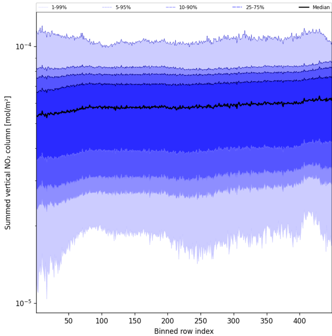
Figure 55: Along track statistics of “Summed vertical NO 2 column” for 2025-05-11 to 2025-05-12
