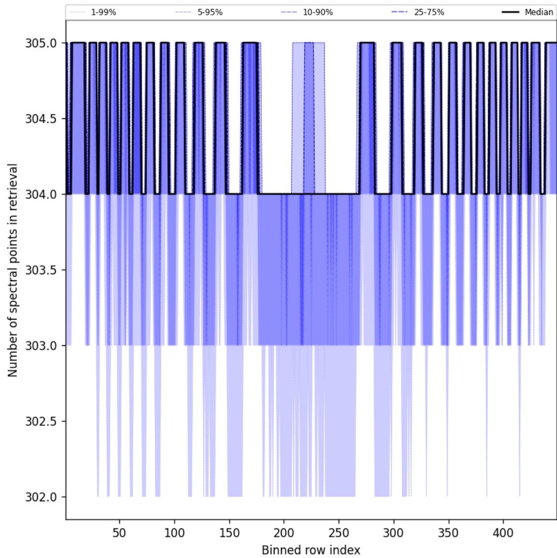
Figure 48: Along track statistics of “Number of spectral points in retrieval” for 2025-05-11 to 2025-05-12
