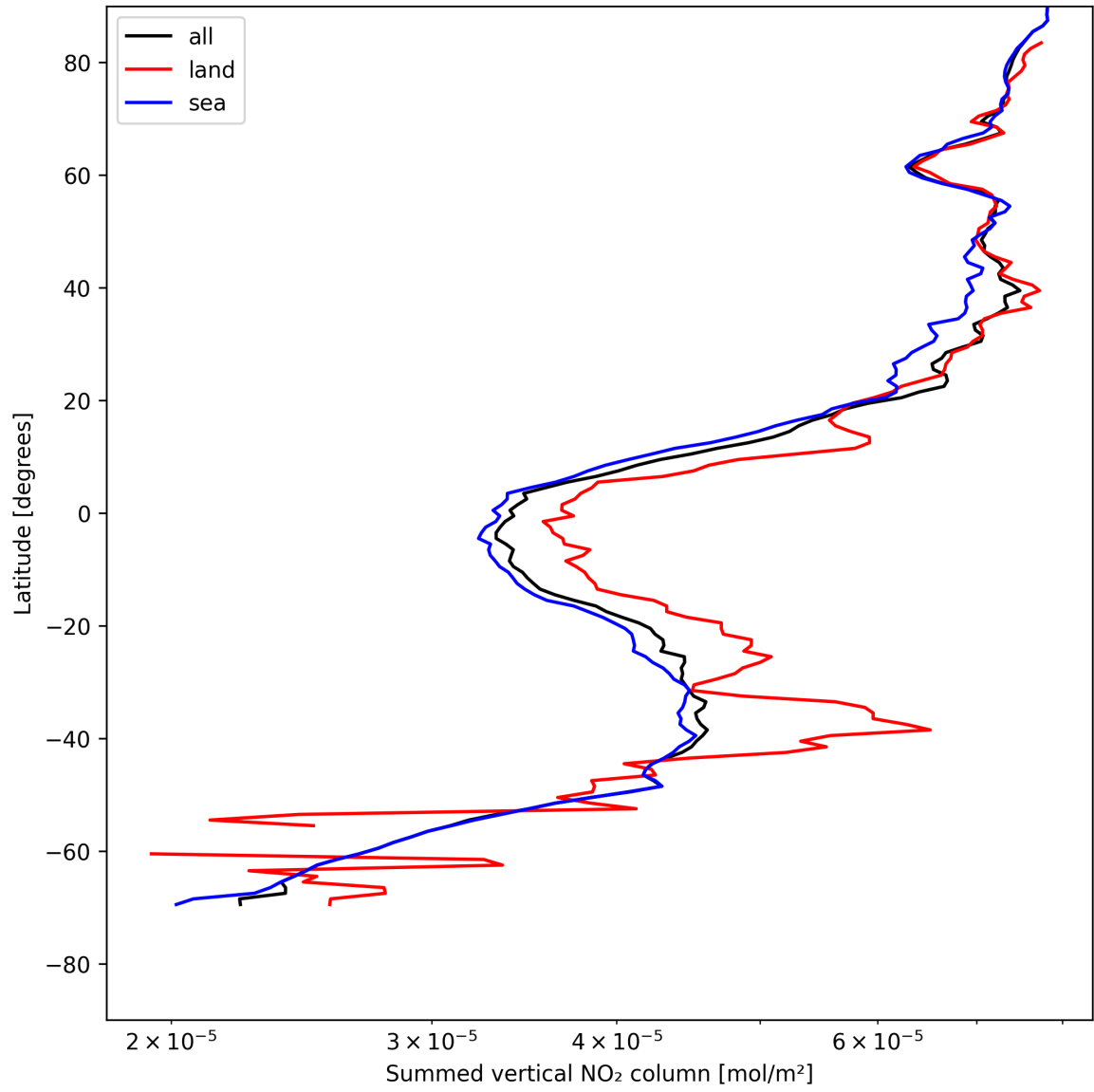
Figure 21: Zonal average of “Summed vertical NO 2 column” for 2025-05-11 to 2025-05-12.
