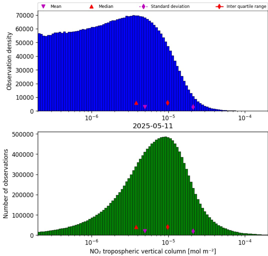
Figure 27: Histogram of “NO 2 tropospheric vertical column” for 2025-05-11 to 2025-05-12
