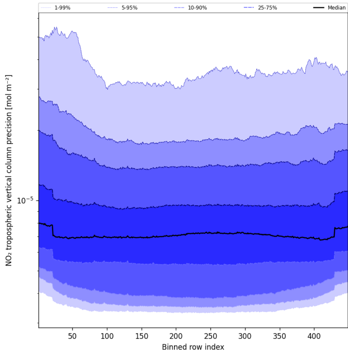
Figure 45: Along track statistics of “NO 2 tropospheric vertical column precision” for 2025-05-11 to 2025-05-12
