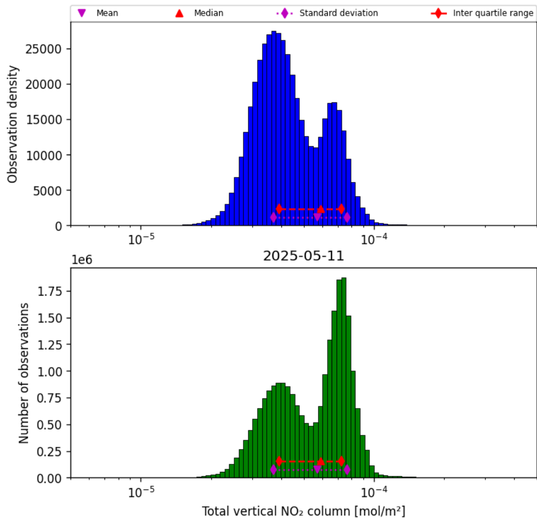
Figure 36: Histogram of “Total vertical NO 2 column” for 2025-05-11 to 2025-05-12
