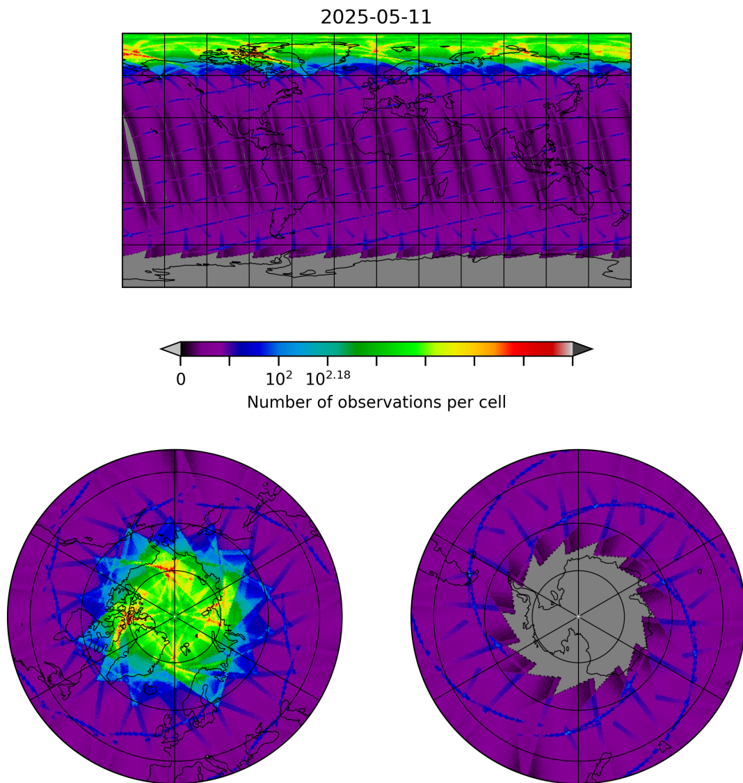
Figure 8: Map of the number of observations for 2025-05-11 to 2025-05-12
