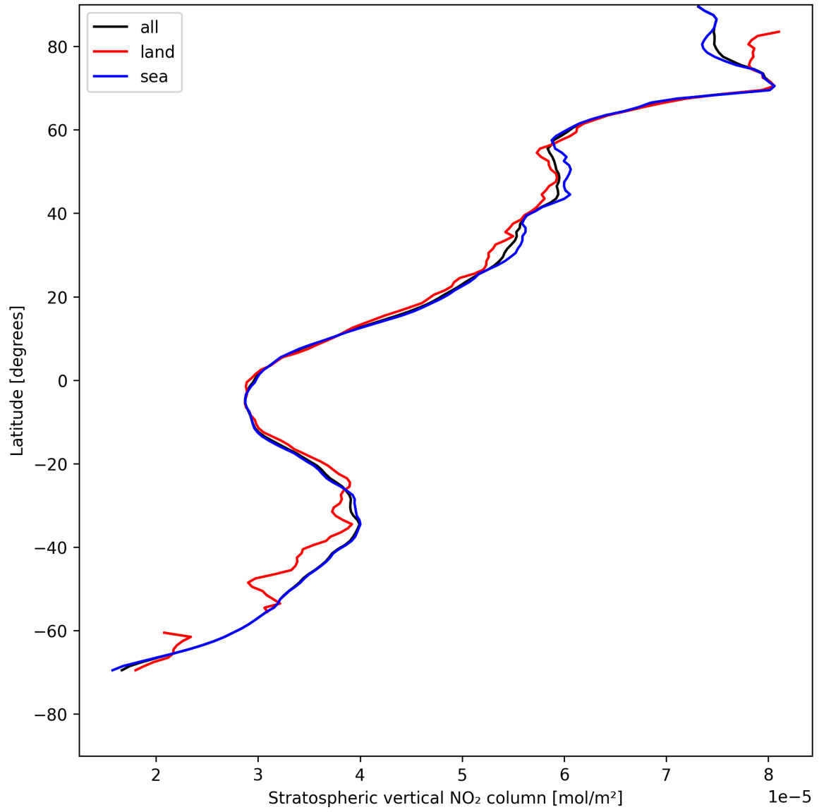
Figure 17: Zonal average of “Stratospheric vertical NO 2 column” for 2025-05-11 to 2025-05-12.
