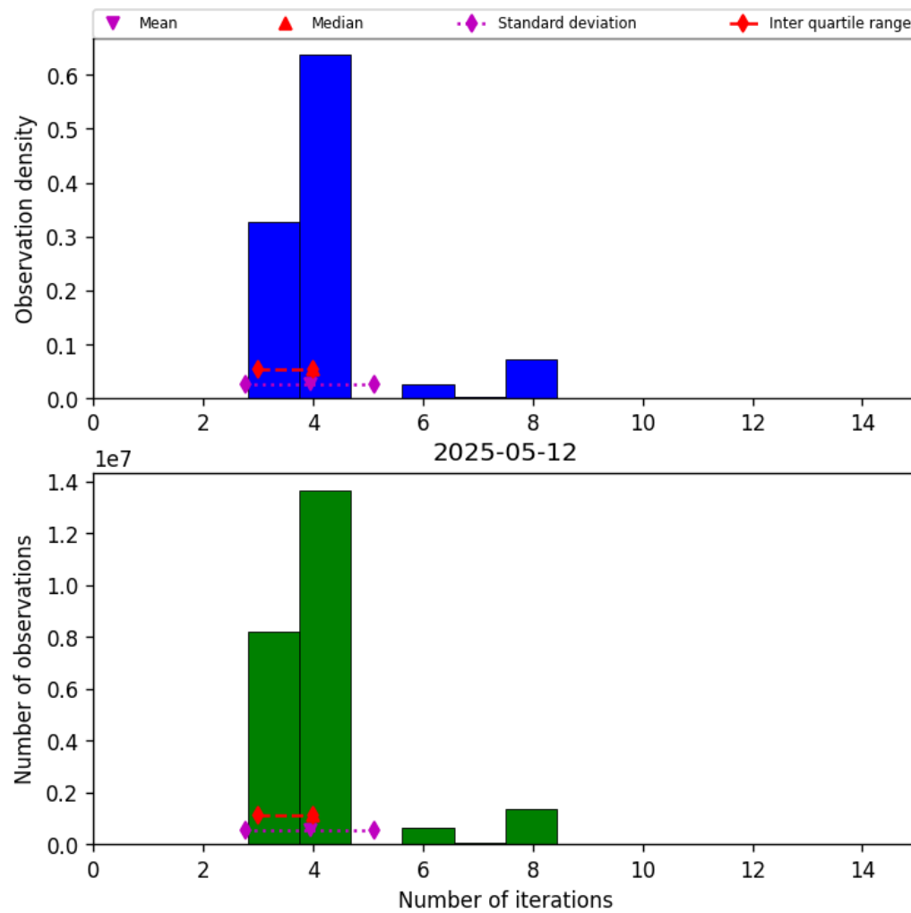
Figure 32: Histogram of “Number of iterations” for 2025-05-12 to 2025-05-13
