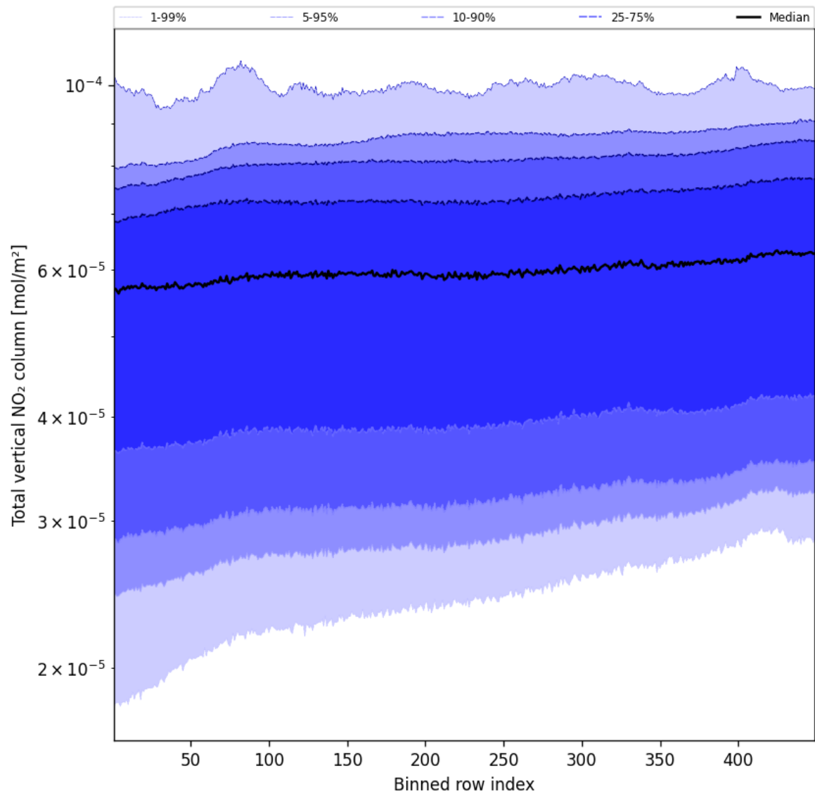
Figure 53: Along track statistics of “Total vertical NO 2 column” for 2025-05-12 to 2025-05-13
