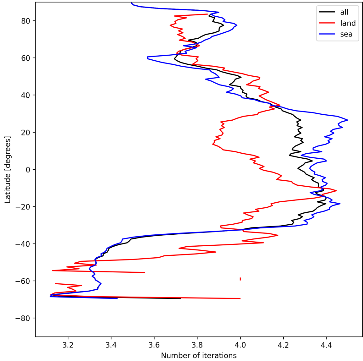
Figure 15: Zonal average of “Number of iterations” for 2025-05-12 to 2025-05-13.
