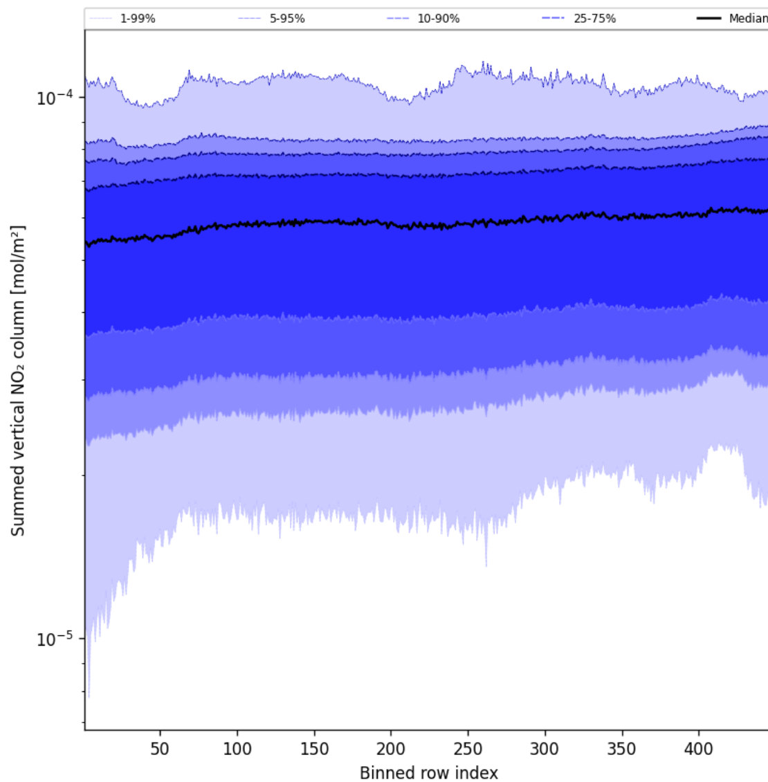
Figure 55: Along track statistics of “Summed vertical NO 2 column” for 2025-05-12 to 2025-05-13
