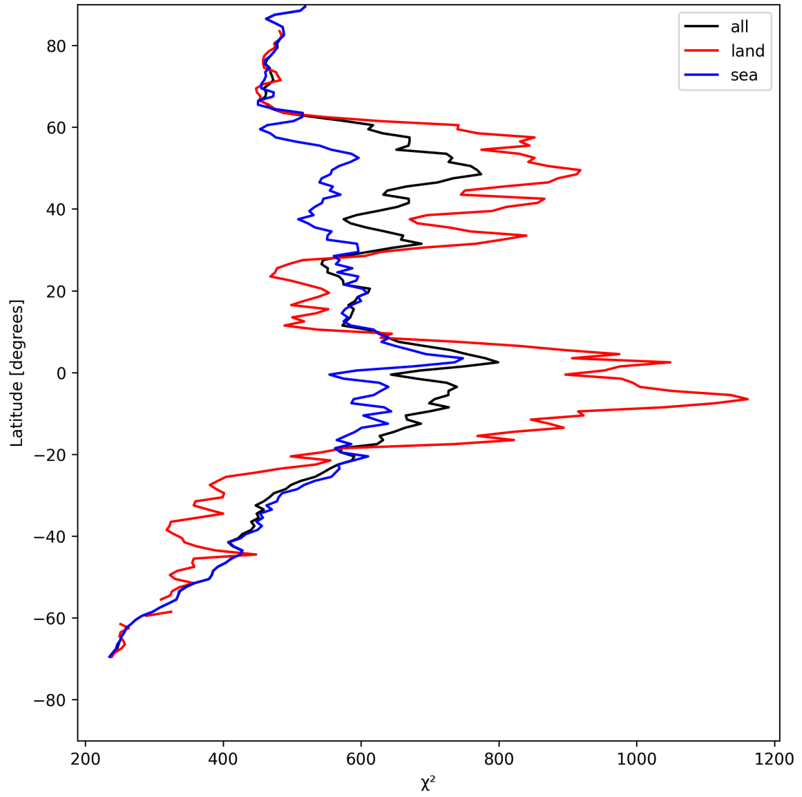
Figure 23: Zonal average of “ \chi^2 ” for 2025-05-12 to 2025-05-13.
