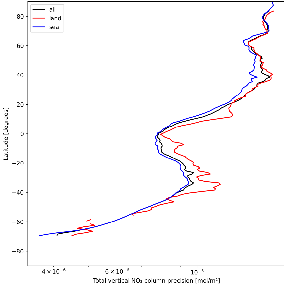
Figure 20: Zonal average of “Total vertical NO 2 column precision” for 2025-05-12 to 2025-05-13.
