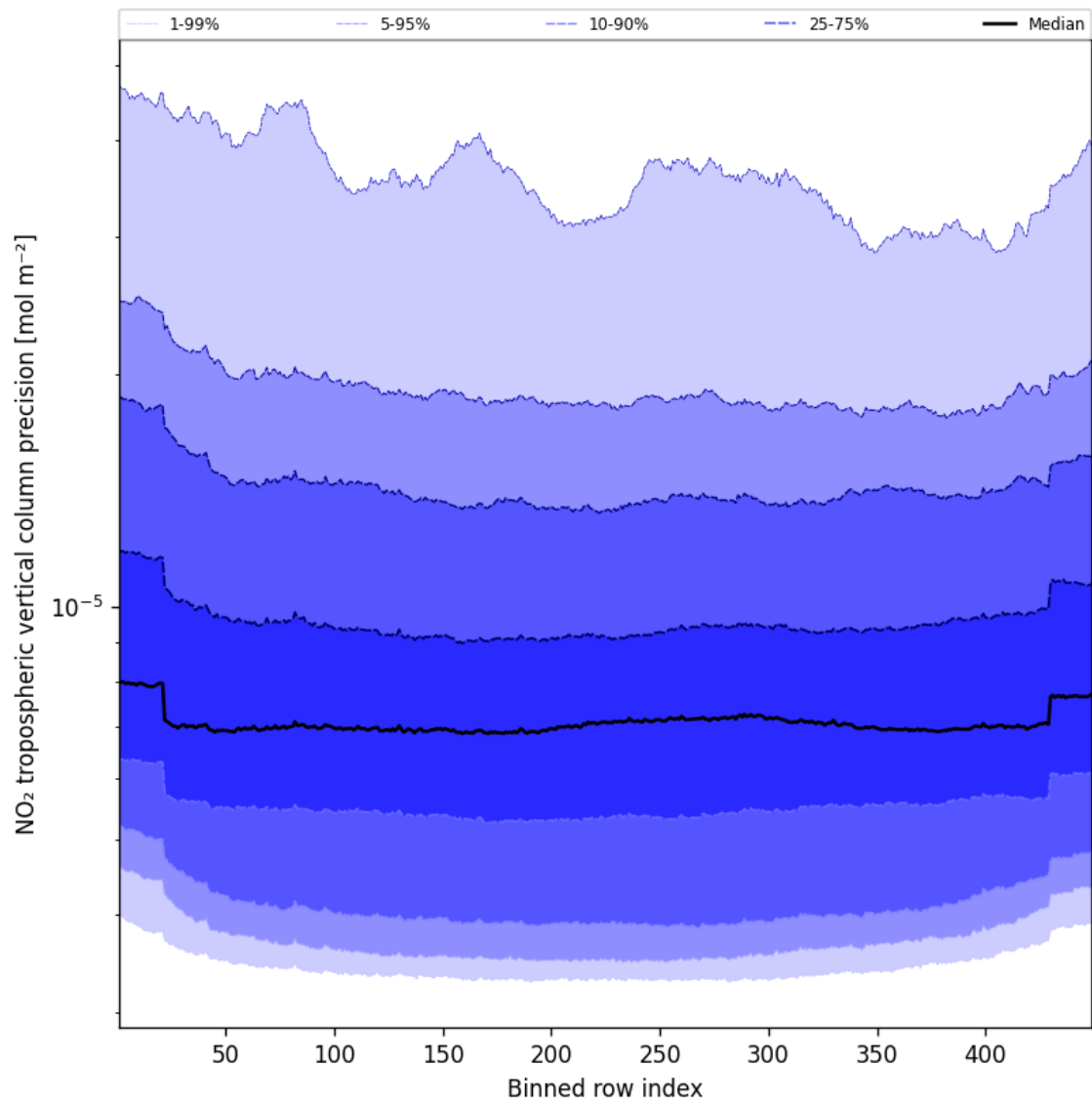
Figure 45: Along track statistics of “NO 2 tropospheric vertical column precision” for 2025-05-12 to 2025-05-13
