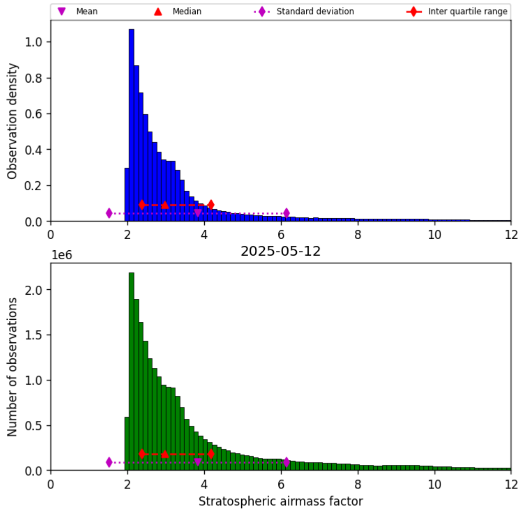
Figure 42: Histogram of “Stratospheric airmass factor” for 2025-05-12 to 2025-05-13
