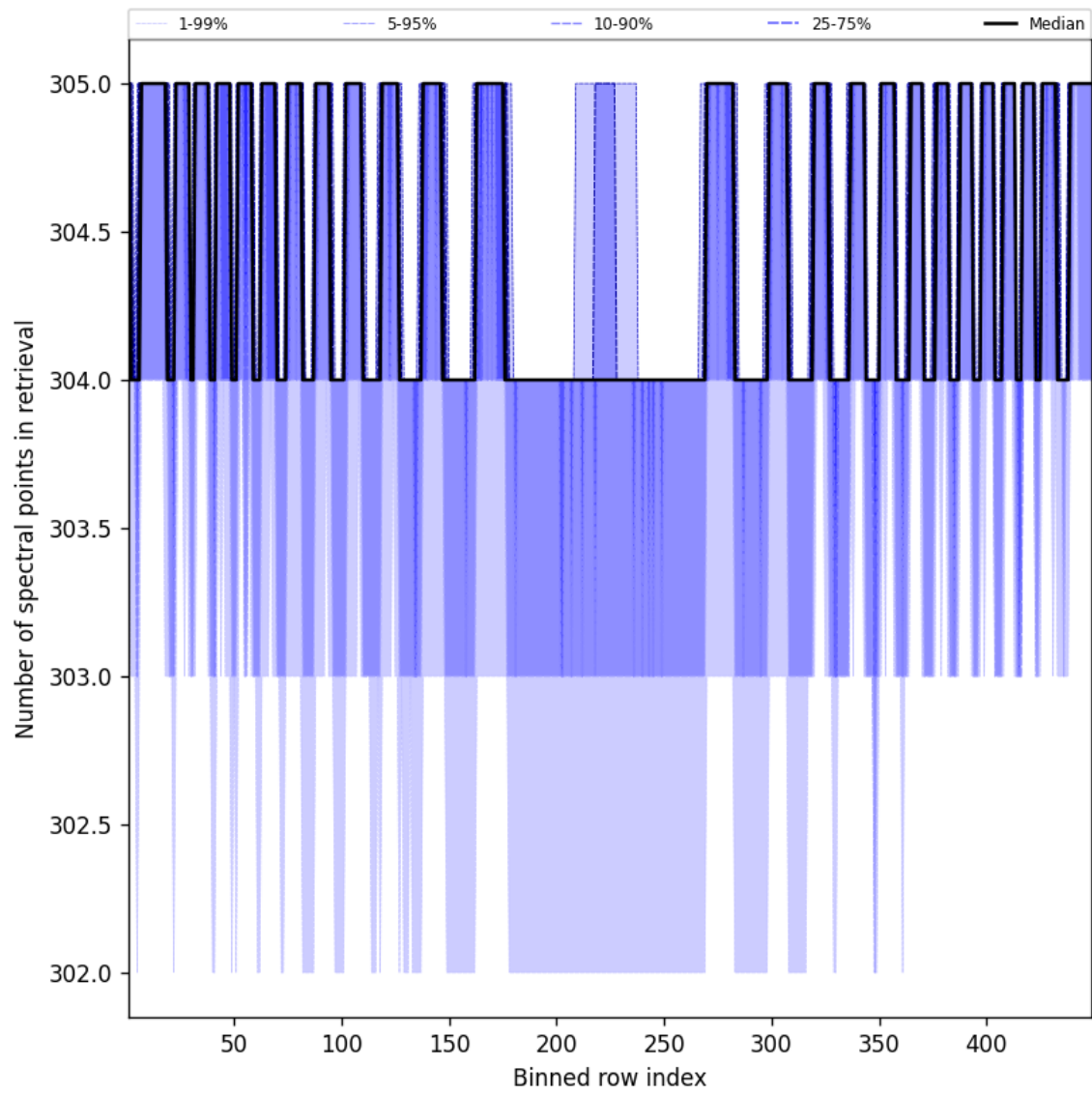
Figure 48: Along track statistics of “Number of spectral points in retrieval” for 2025-05-12 to 2025-05-13
