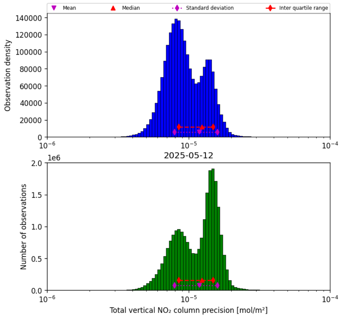
Figure 37: Histogram of “Total vertical NO 2 column precision” for 2025-05-12 to 2025-05-13
