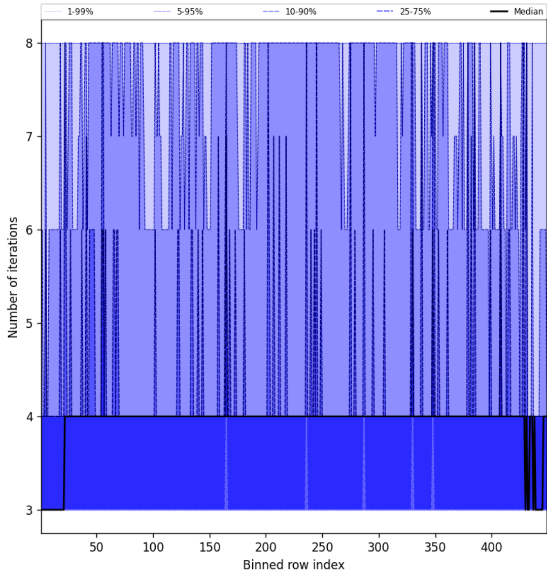
Figure 49: Along track statistics of “Number of iterations” for 2025-05-12 to 2025-05-13
