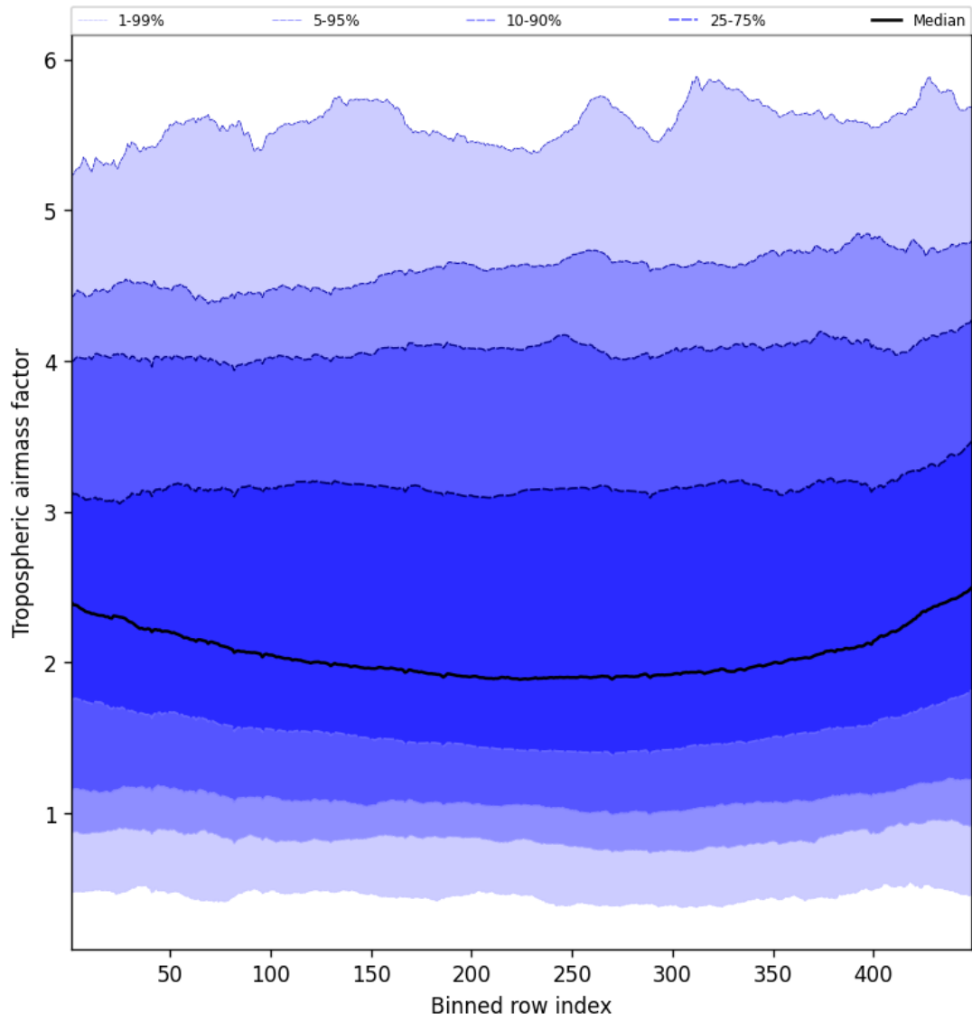
Figure 46: Along track statistics of “Tropospheric airmass factor” for 2025-05-12 to 2025-05-13
