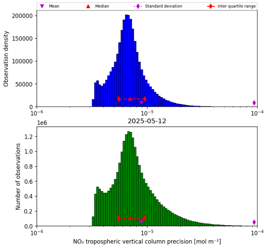
Figure 28: Histogram of “NO 2 tropospheric vertical column precision” for 2025-05-12 to 2025-05-13
