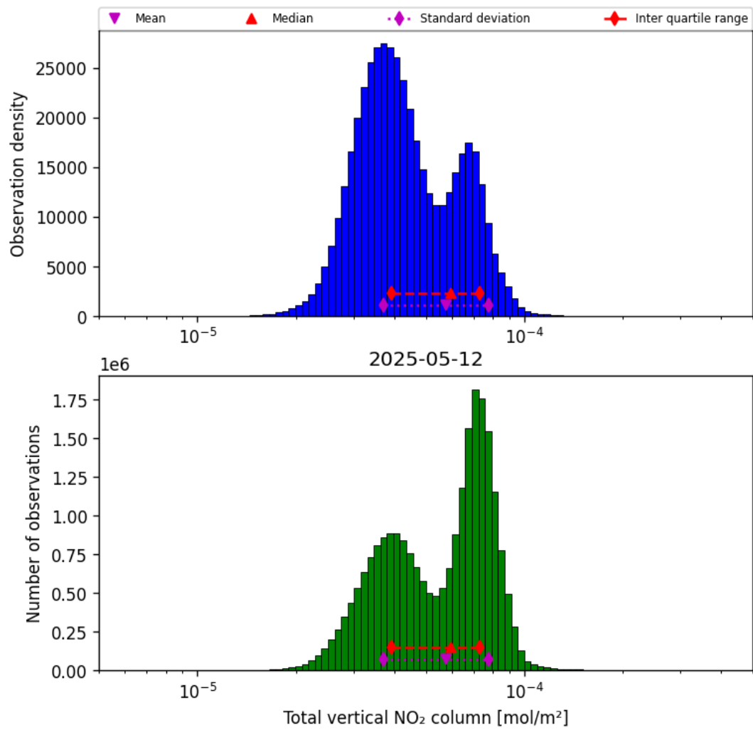
Figure 36: Histogram of “Total vertical NO 2 column” for 2025-05-12 to 2025-05-13
