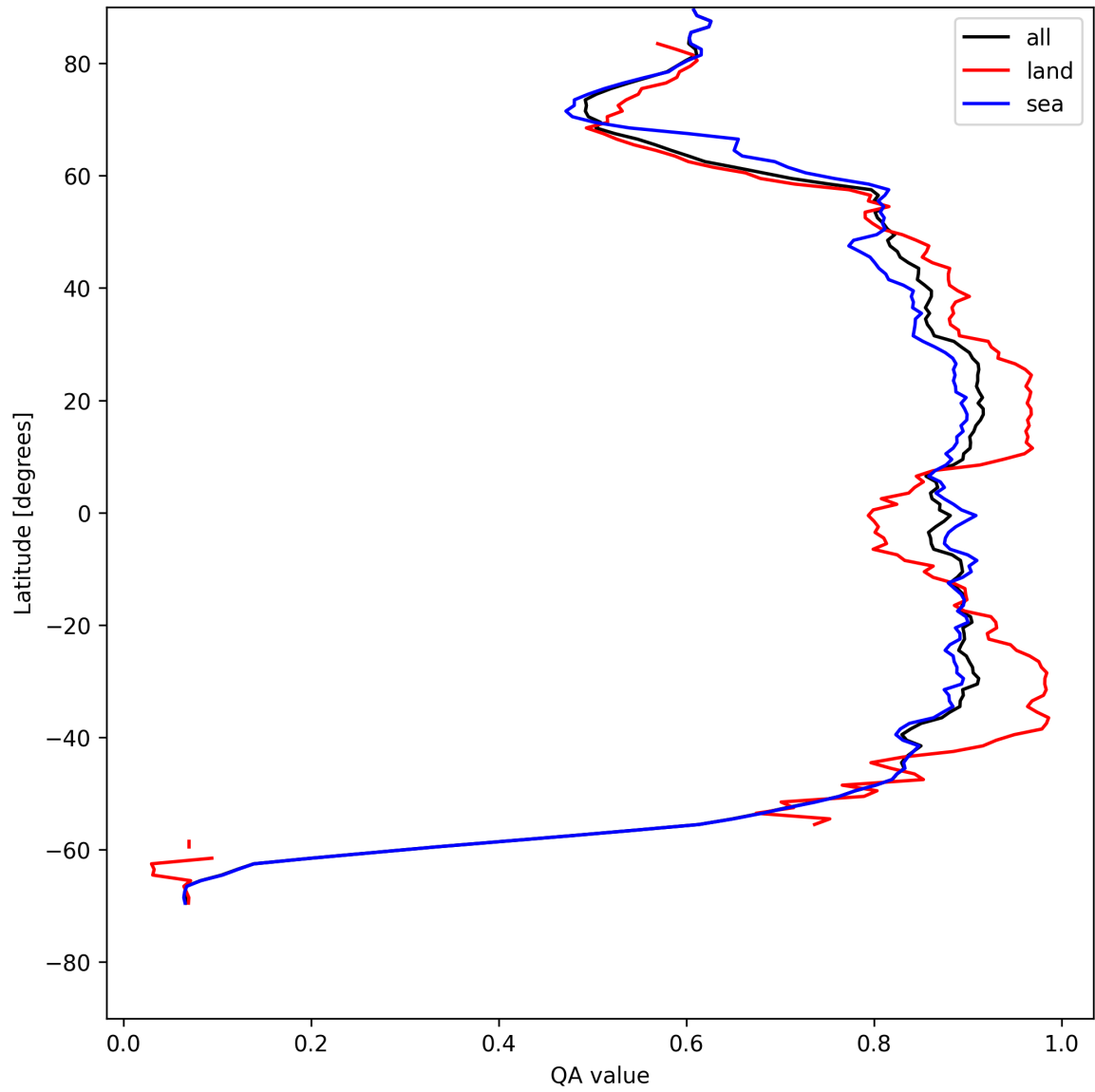
Figure 9: Zonal average of “QA value” for 2025-05-12 to 2025-05-13.
