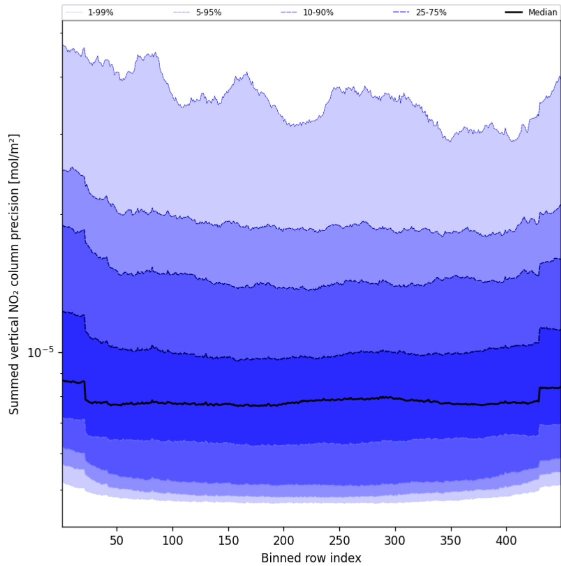
Figure 56: Along track statistics of “Summed vertical NO 2 column precision” for 2025-05-12 to 2025-05-13
