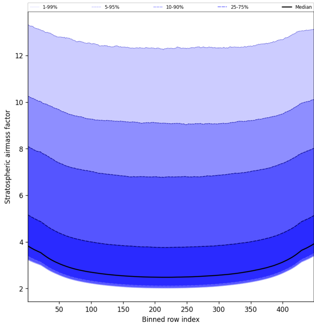
Figure 59: Along track statistics of “Stratospheric airmass factor” for 2025-05-12 to 2025-05-13
