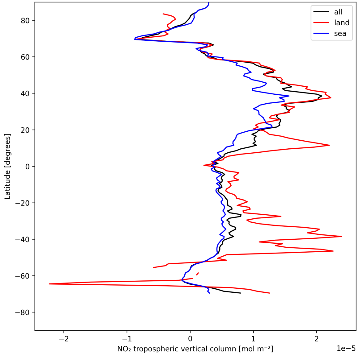
Figure 10: Zonal average of “NO 2 tropospheric vertical column” for 2025-05-12 to 2025-05-13.
