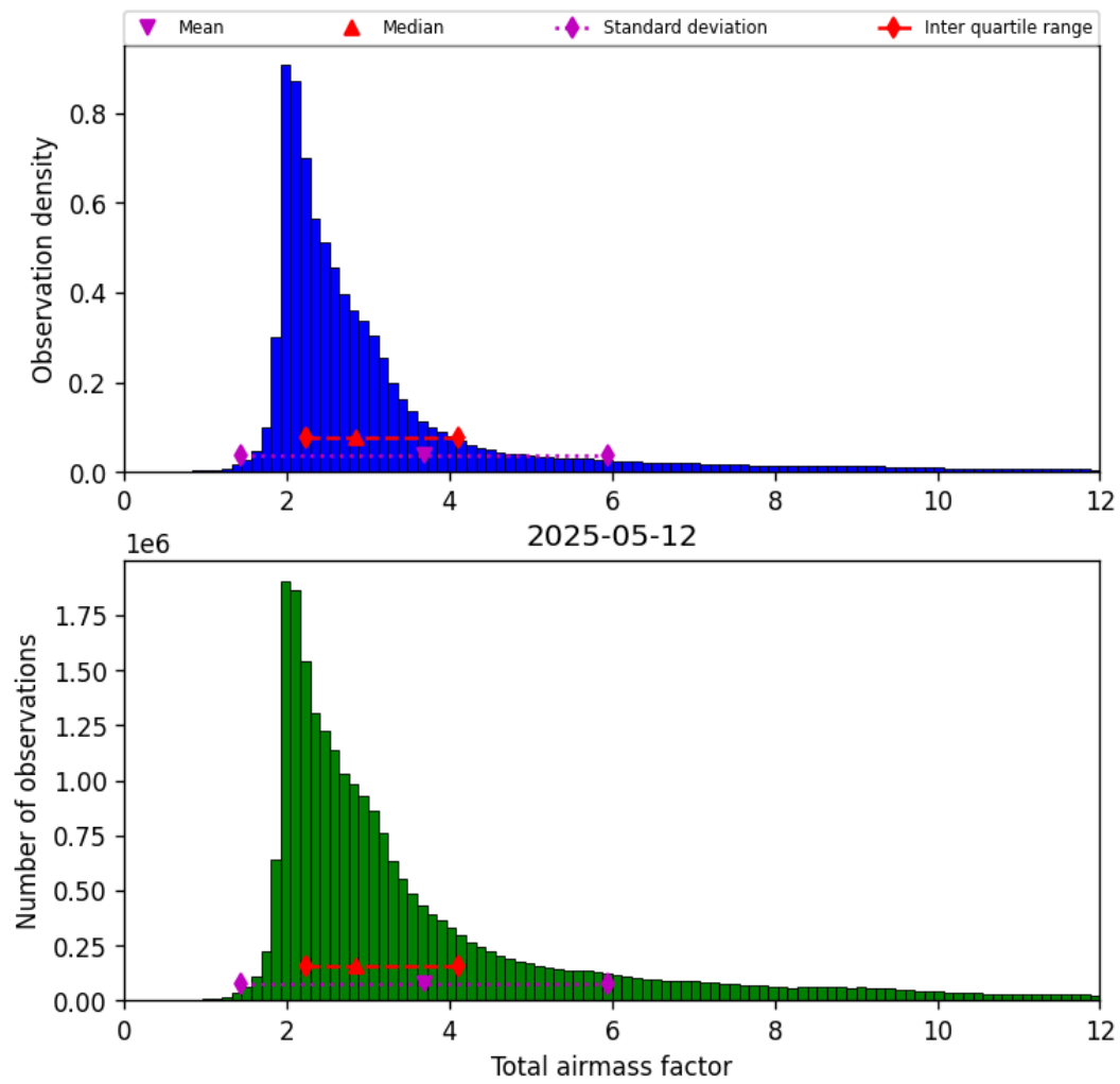
Figure 30: Histogram of “Total airmass factor” for 2025-05-12 to 2025-05-13
