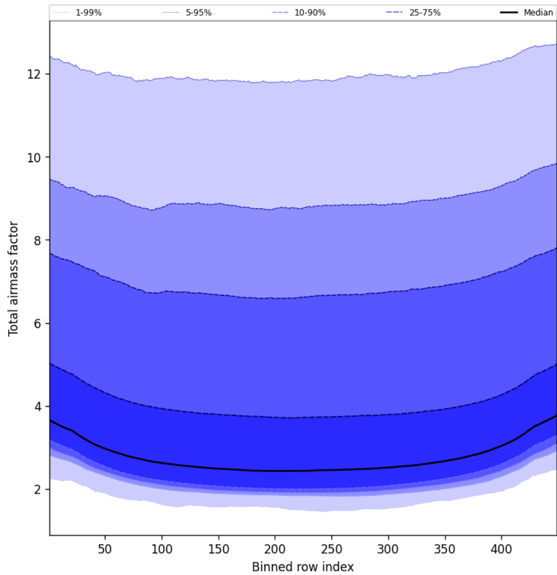
Figure 47: Along track statistics of “Total airmass factor” for 2025-05-12 to 2025-05-13
