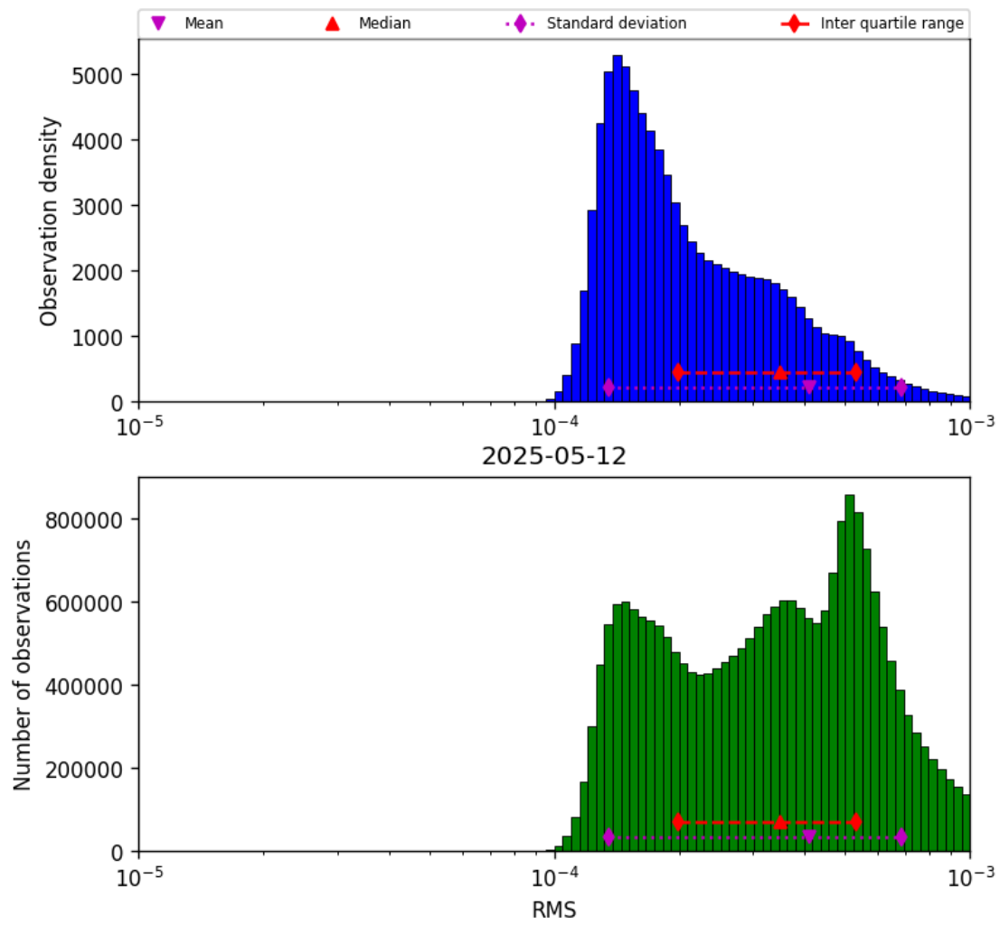
Figure 41: Histogram of “RMS” for 2025-05-12 to 2025-05-13
