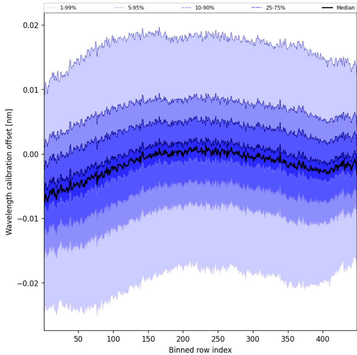
Figure 50: Along track statistics of “Wavelength calibration offset” for 2025-05-12 to 2025-05-13
