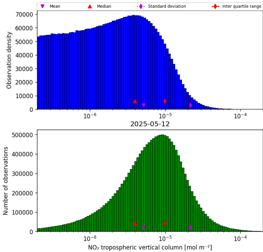
Figure 27: Histogram of “NO 2 tropospheric vertical column” for 2025-05-12 to 2025-05-13
