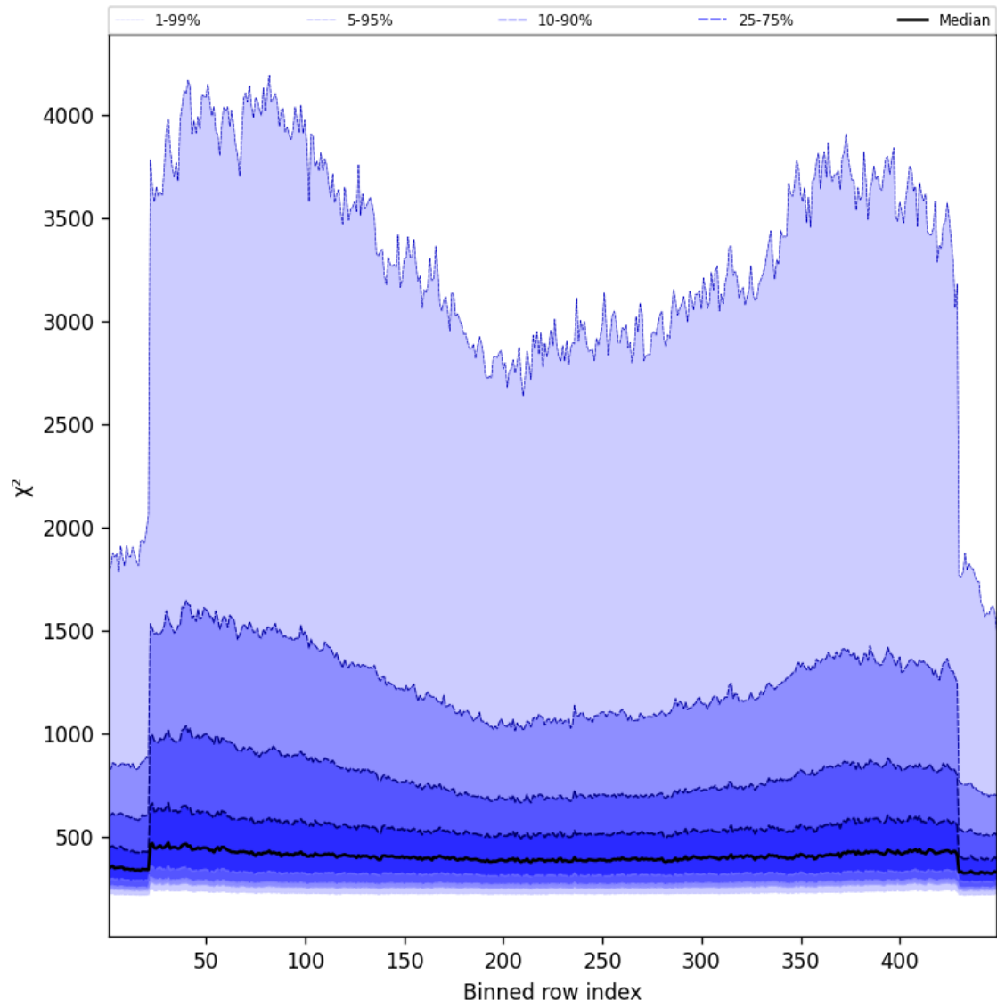
Figure 57: Along track statistics of “ \chi^2 ” for 2025-05-12 to 2025-05-13
