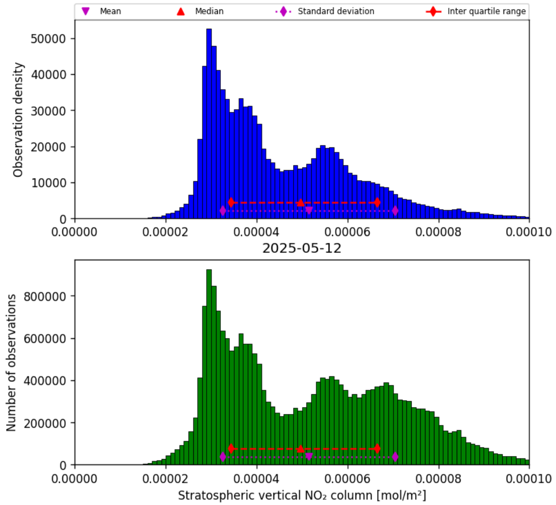
Figure 34: Histogram of “Stratospheric vertical NO 2 column” for 2025-05-12 to 2025-05-13
