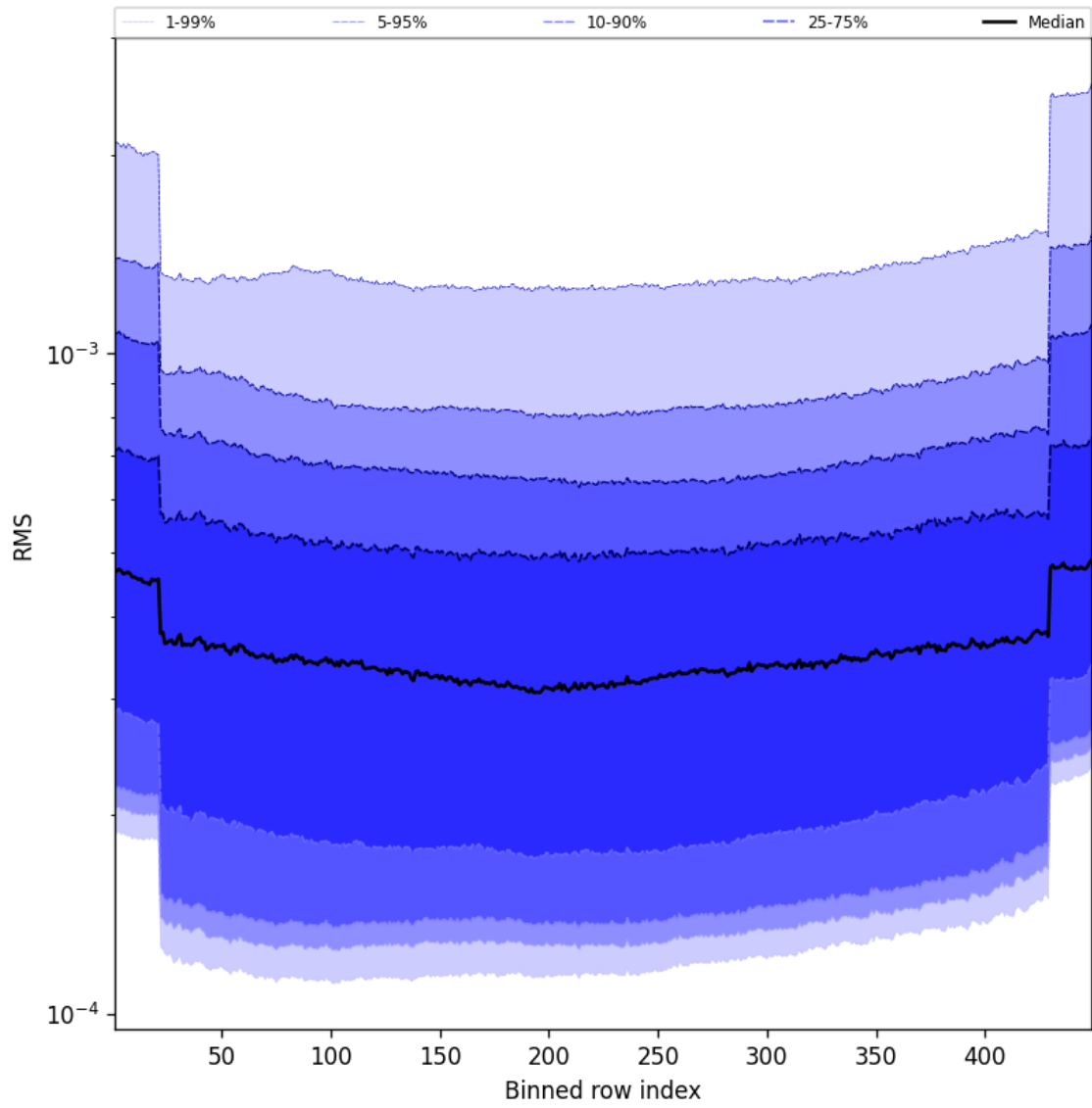
Figure 58: Along track statistics of “RMS” for 2025-05-12 to 2025-05-13
