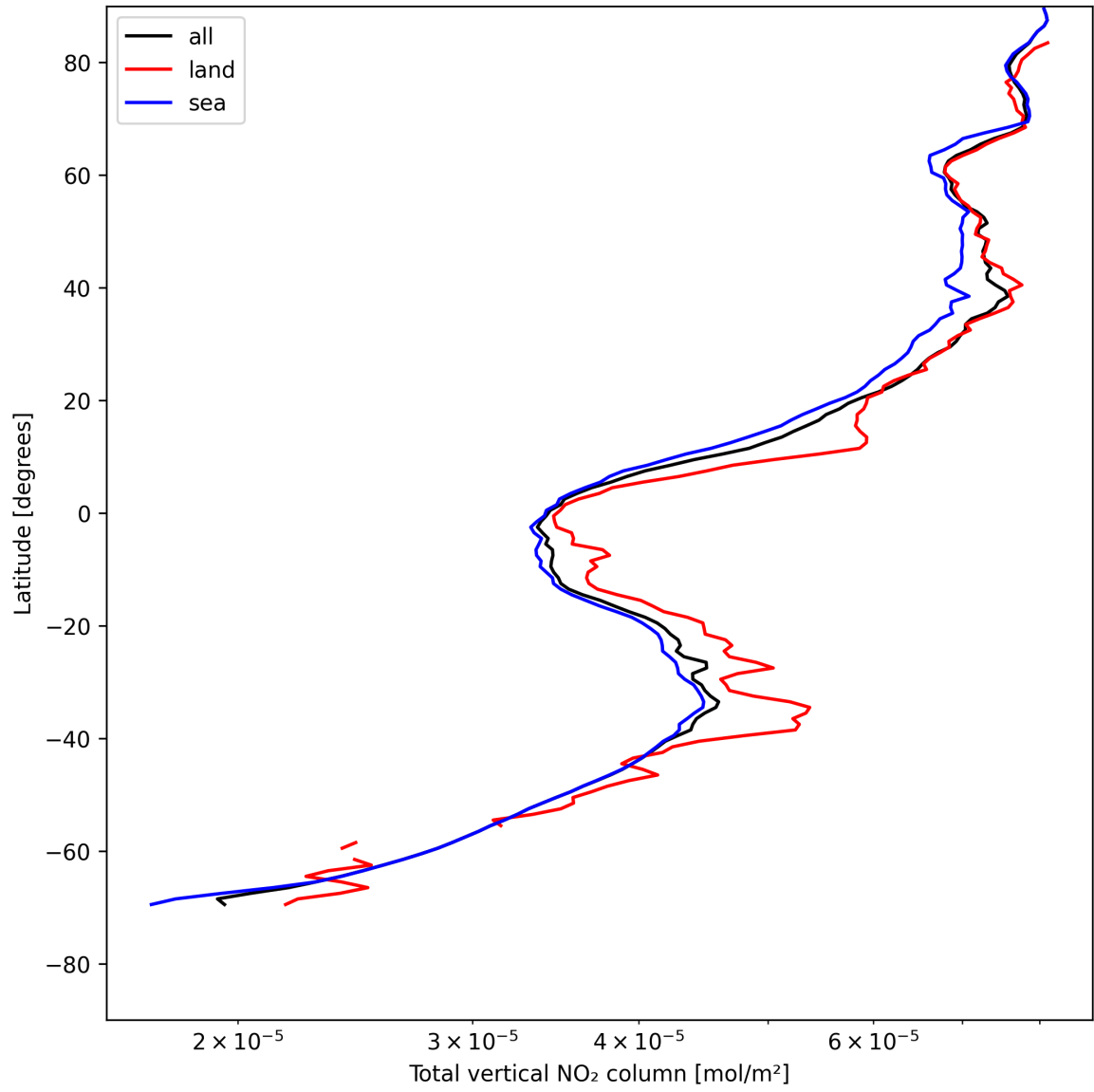
Figure 19: Zonal average of “Total vertical NO 2 column” for 2025-05-12 to 2025-05-13.
