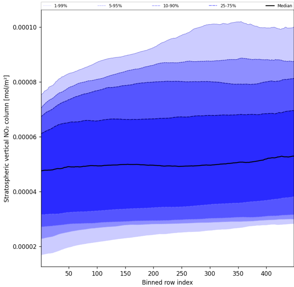
Figure 51: Along track statistics of “Stratospheric vertical NO 2 column” for 2025-05-12 to 2025-05-13
