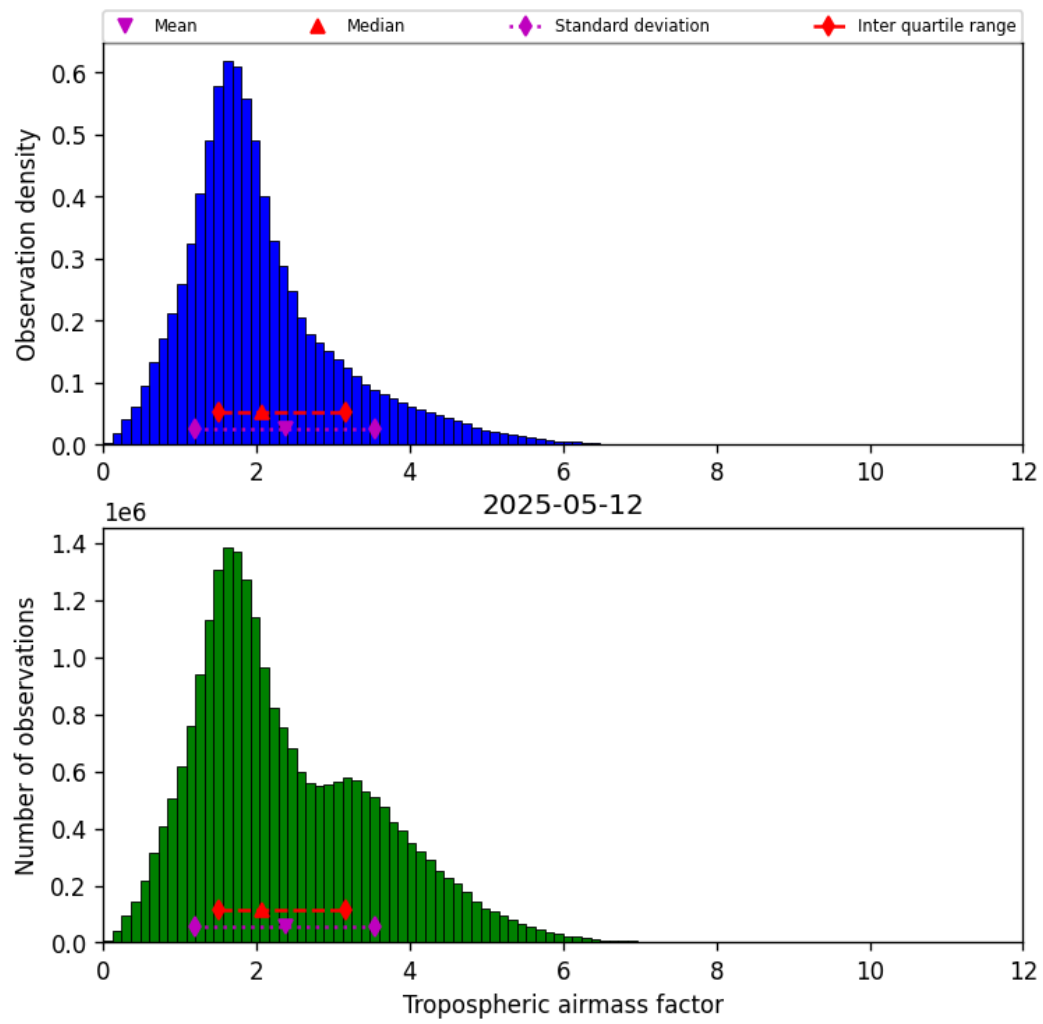
Figure 29: Histogram of “Tropospheric airmass factor” for 2025-05-12 to 2025-05-13
