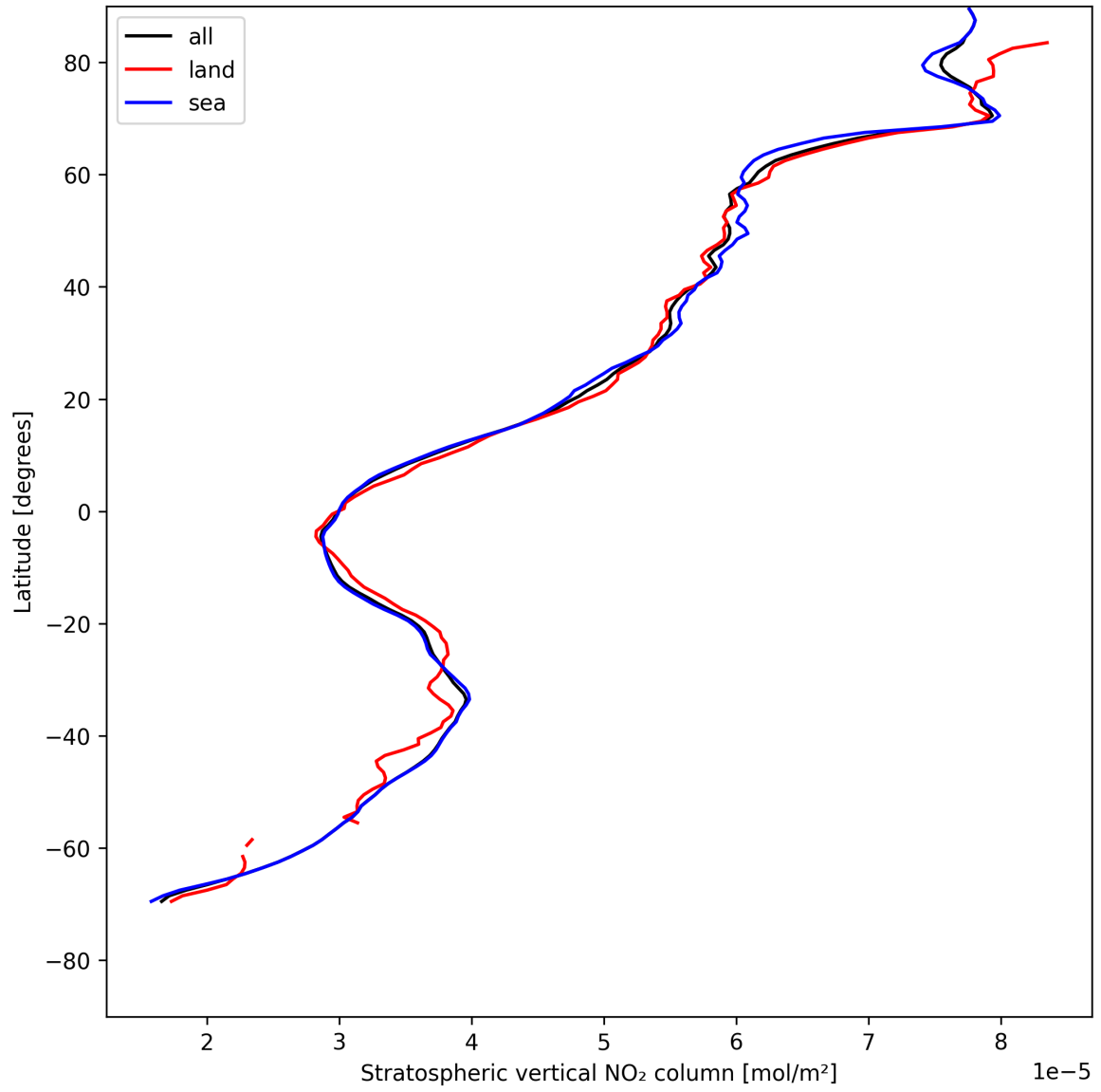
Figure 17: Zonal average of “Stratospheric vertical NO 2 column” for 2025-05-12 to 2025-05-13.
