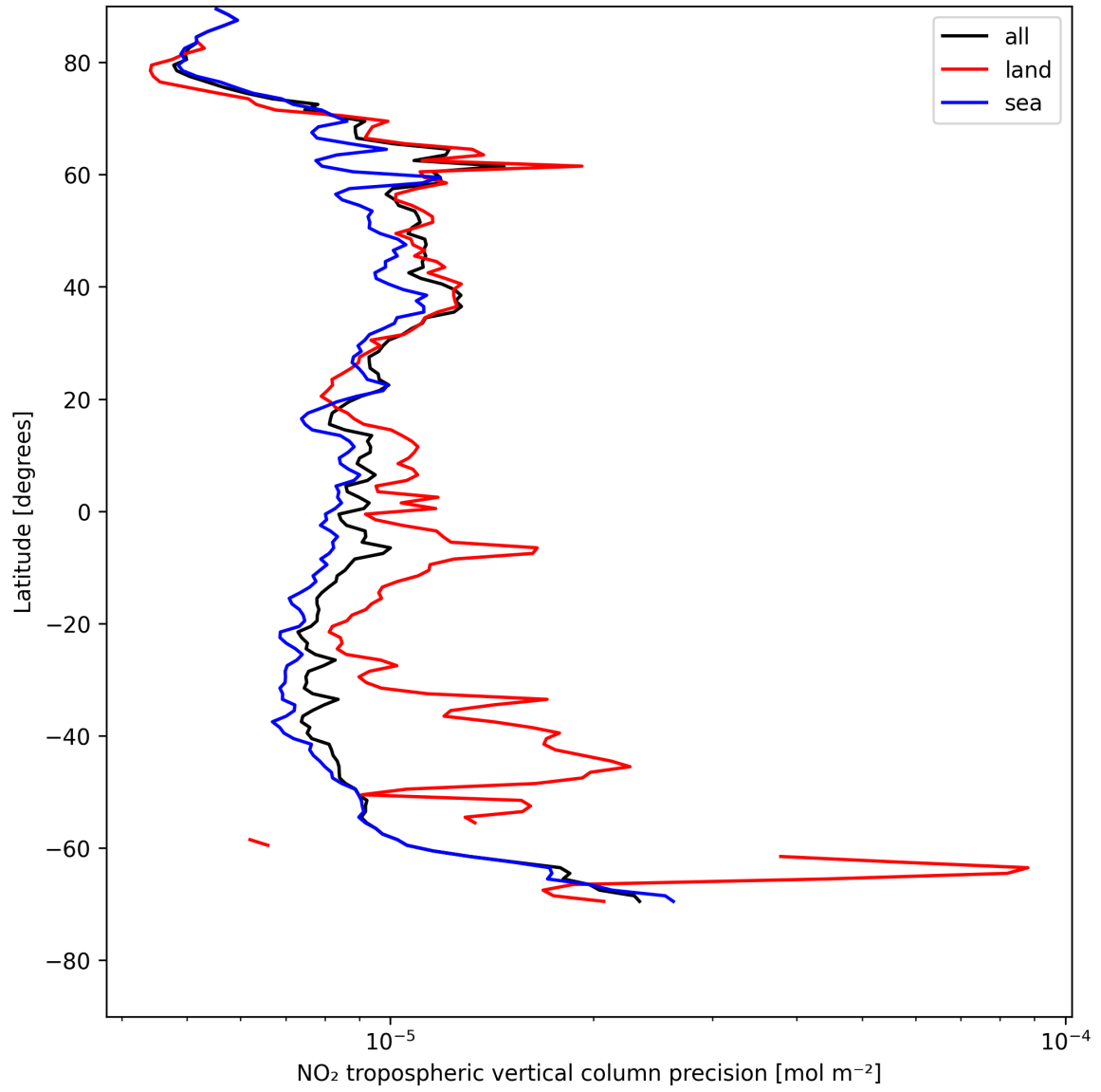
Figure 11: Zonal average of “NO 2 tropospheric vertical column precision” for 2025-05-12 to 2025-05-13.
