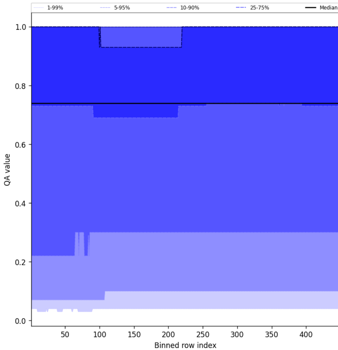
Figure 43: Along track statistics of “QA value” for 2025-05-12 to 2025-05-13
