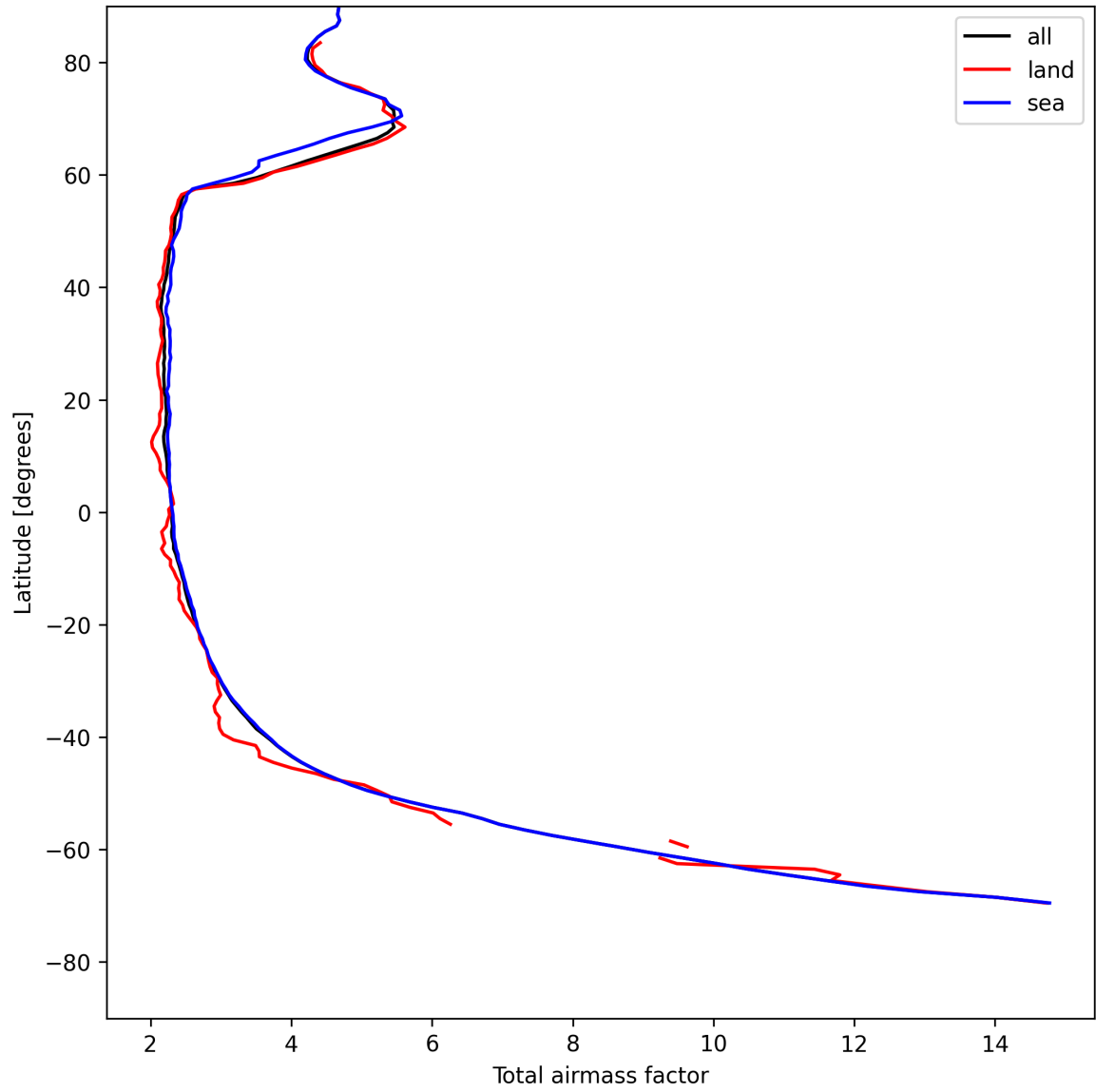
Figure 13: Zonal average of “Total airmass factor” for 2025-05-12 to 2025-05-13.
