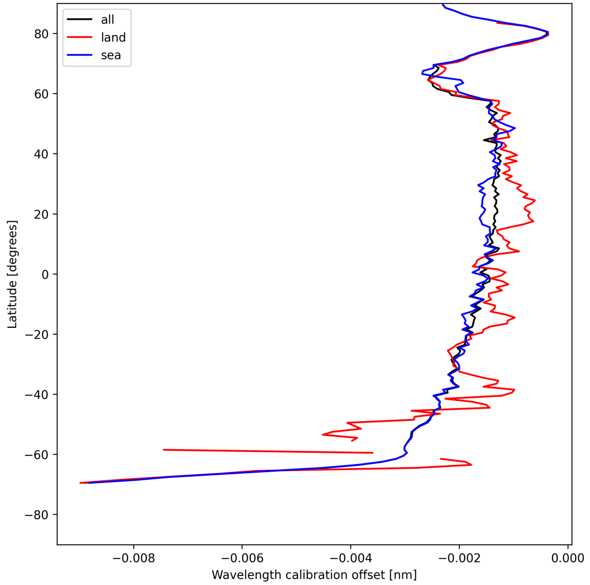
Figure 16: Zonal average of “Wavelength calibration offset” for 2025-05-12 to 2025-05-13.
