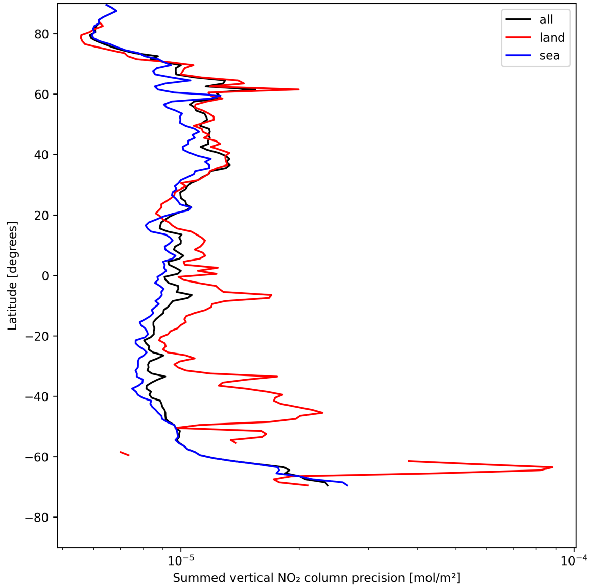
Figure 22: Zonal average of “Summed vertical NO 2 column precision” for 2025-05-12 to 2025-05-13.
