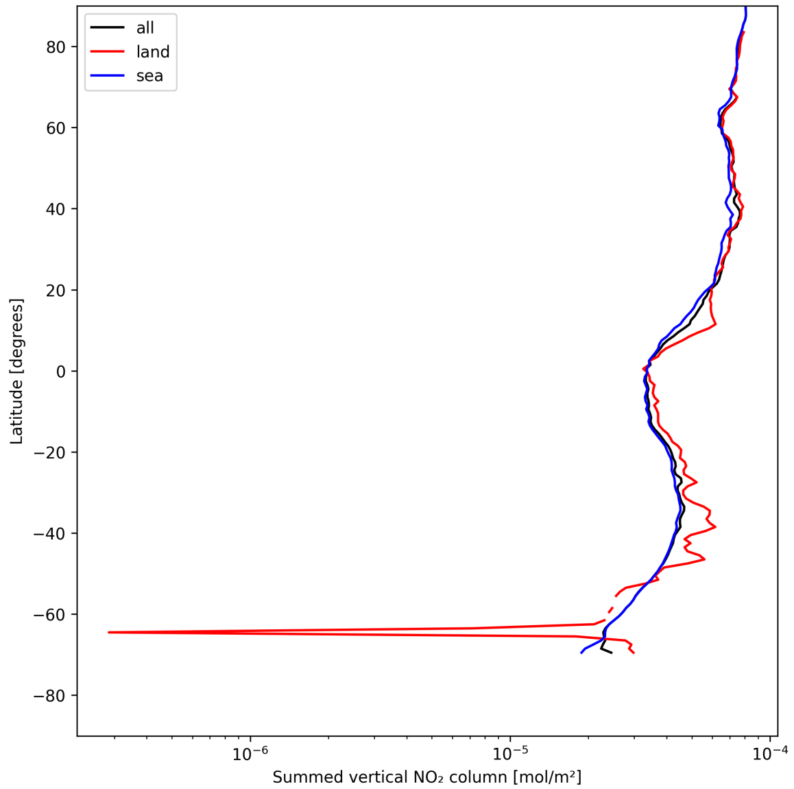
Figure 21: Zonal average of “Summed vertical NO 2 column” for 2025-05-12 to 2025-05-13.
