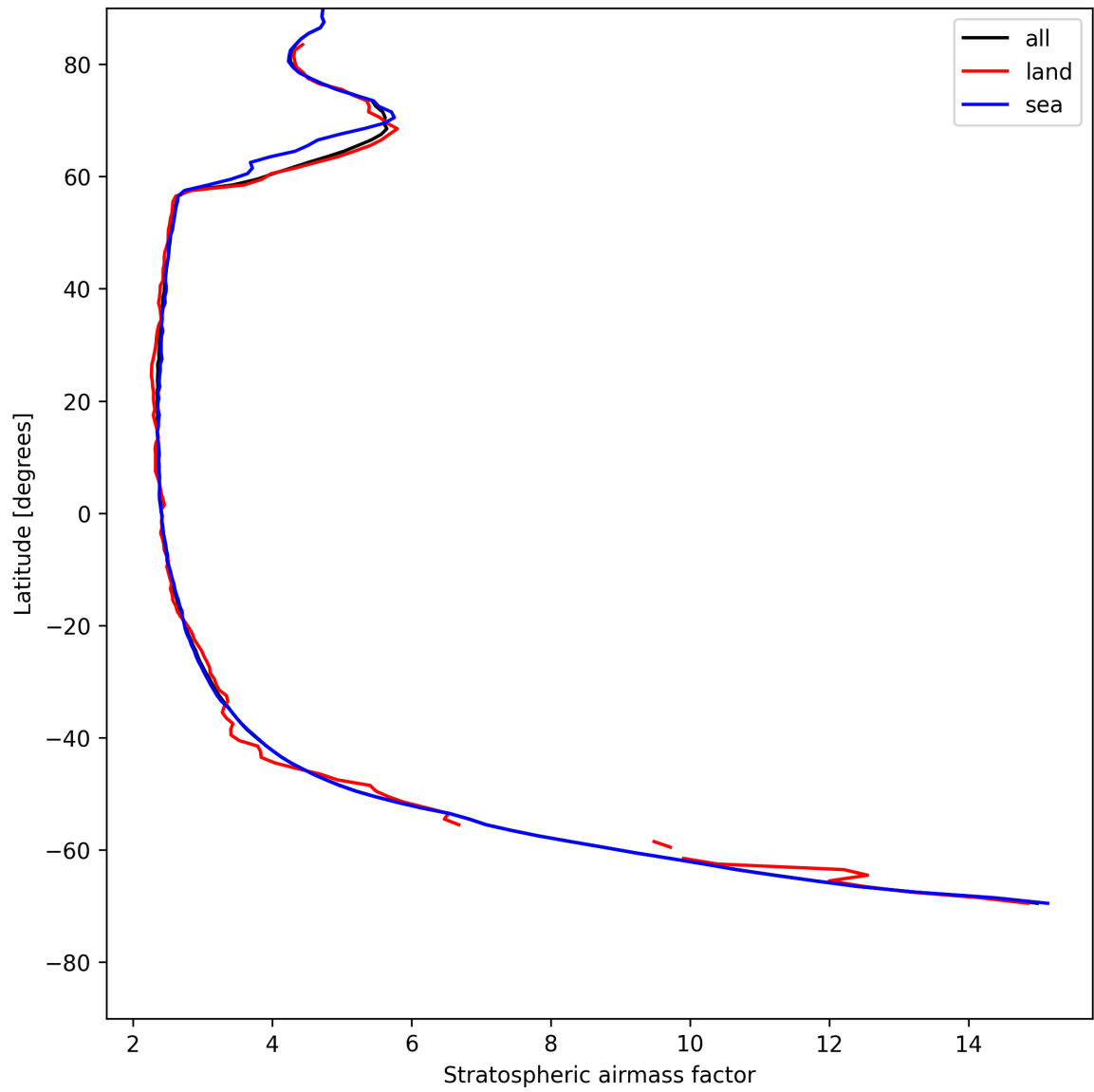
Figure 25: Zonal average of “Stratospheric air mass factor” for 2025-05-12 to 2025-05-13.
