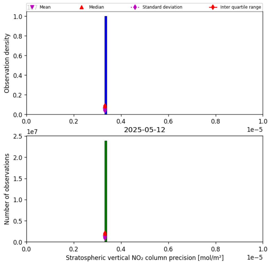
Figure 35: Histogram of “Stratospheric vertical NO 2 column precision” for 2025-05-12 to 2025-05-13
