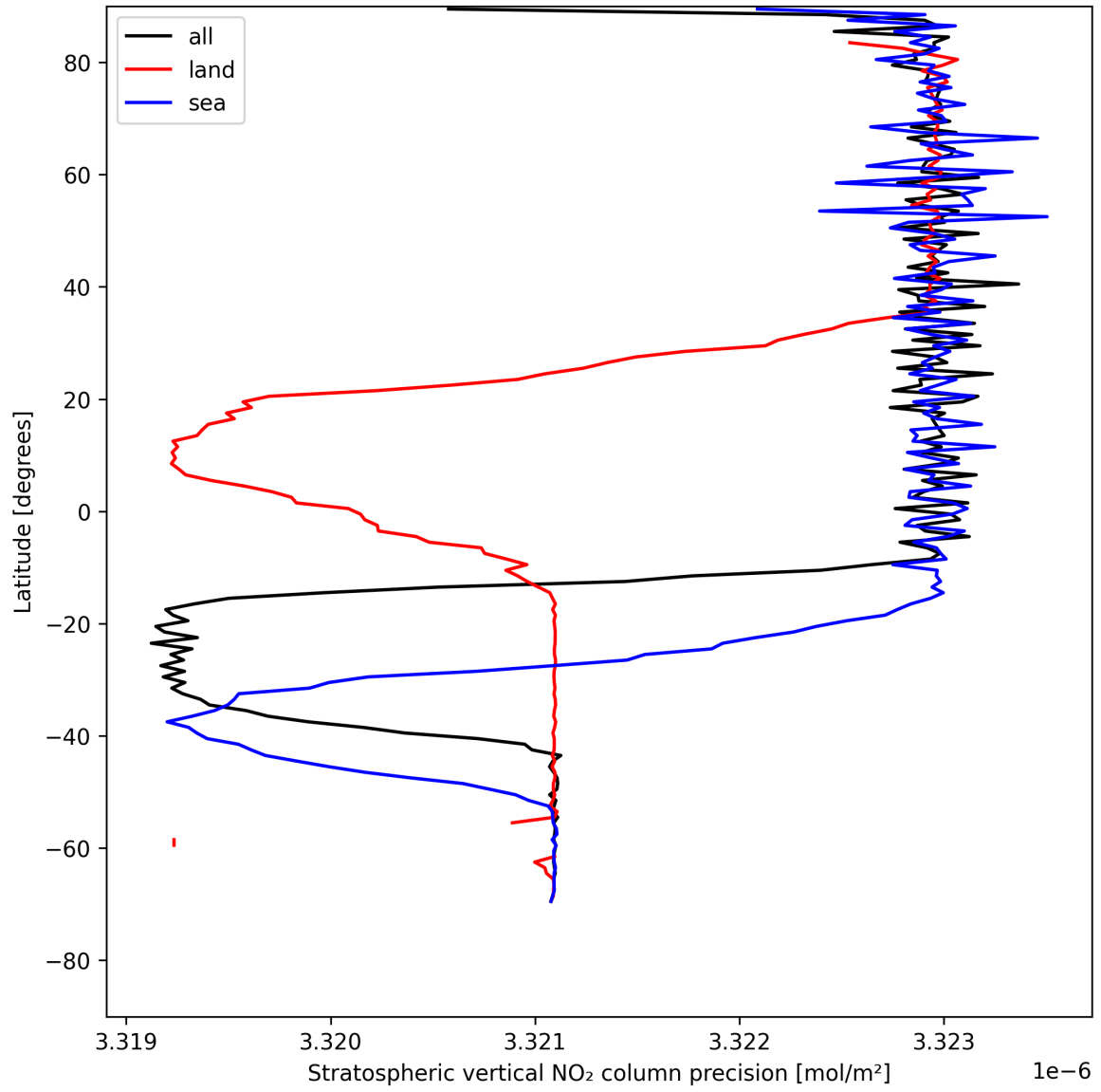
Figure 18: Zonal average of “Stratospheric vertical NO 2 column precision” for 2025-05-12 to 2025-05-13.
