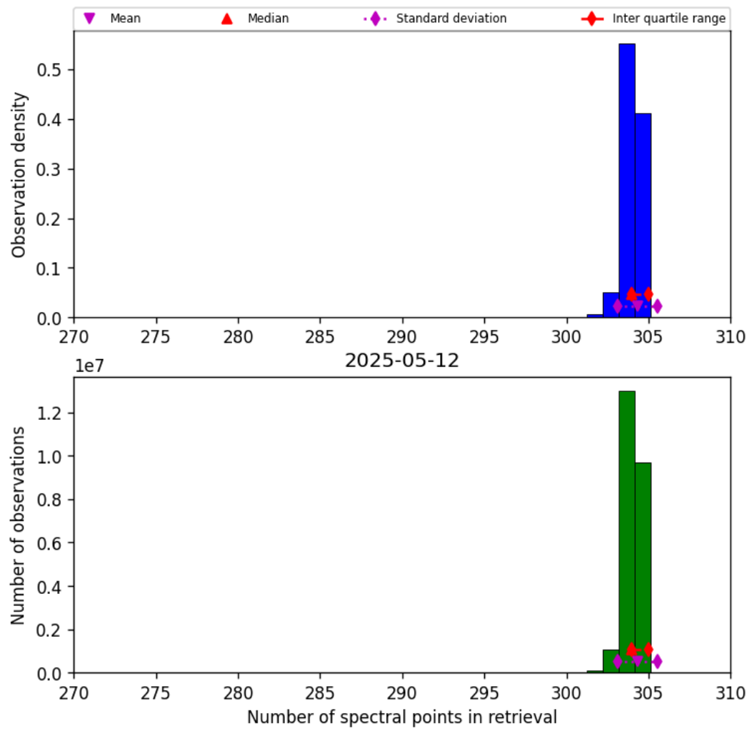
Figure 31: Histogram of “Number of spectral points in retrieval” for 2025-05-12 to 2025-05-13
