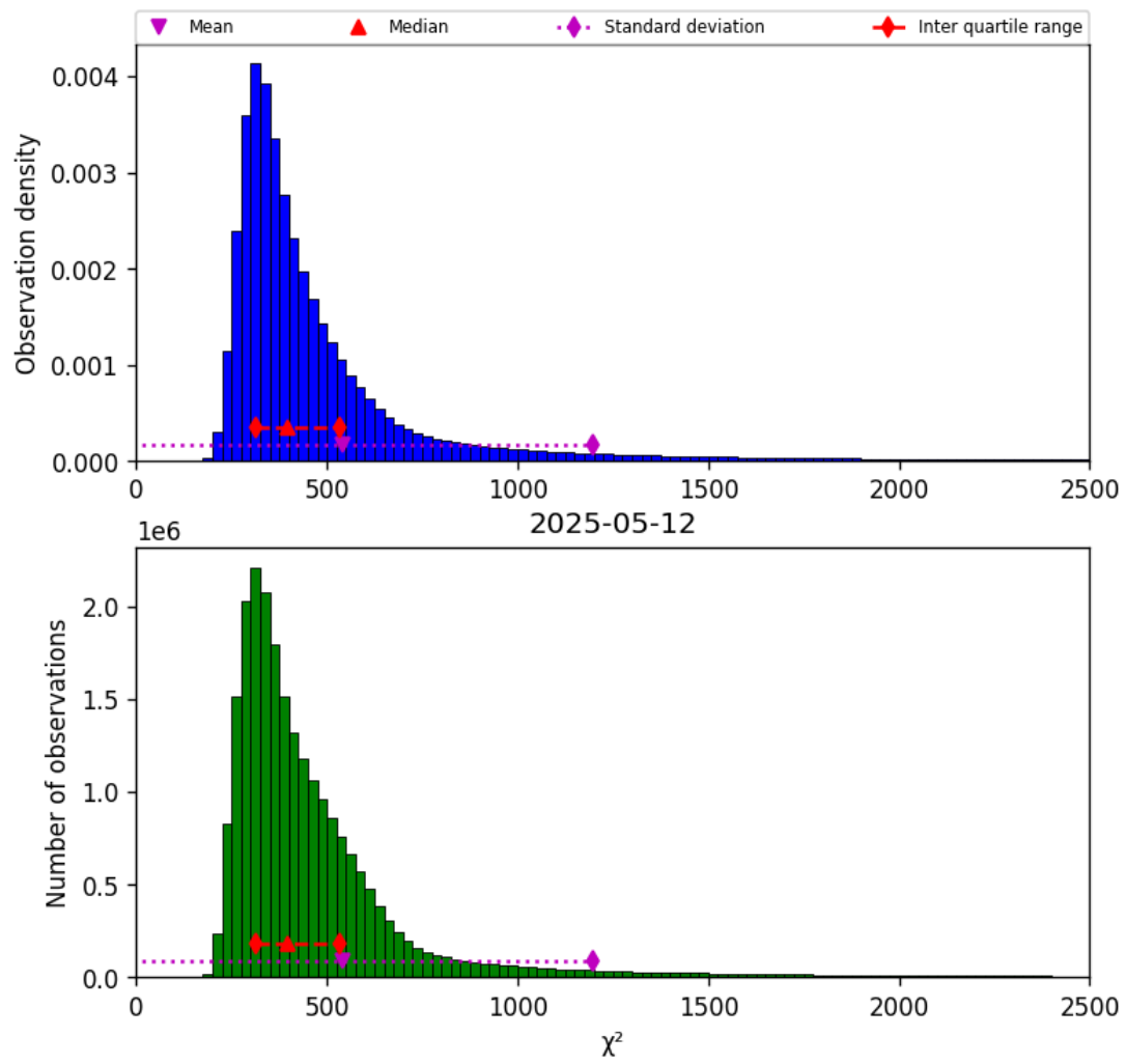
Figure 40: Histogram of “ \chi^2 ” for 2025-05-12 to 2025-05-13
