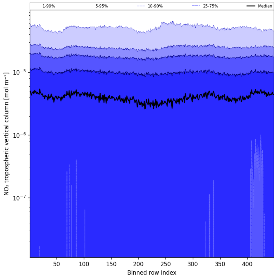
Figure 44: Along track statistics of “NO 2 tropospheric vertical column” for 2025-05-12 to 2025-05-13
