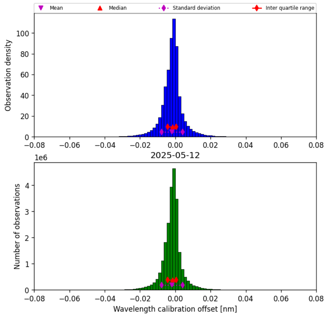
Figure 33: Histogram of “Wavelength calibration offset” for 2025-05-12 to 2025-05-13
