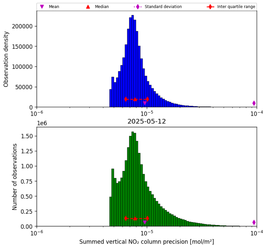
Figure 39: Histogram of “Summed vertical NO 2 column precision” for 2025-05-12 to 2025-05-13
