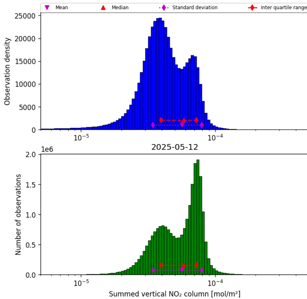
Figure 38: Histogram of “Summed vertical NO 2 column” for 2025-05-12 to 2025-05-13
