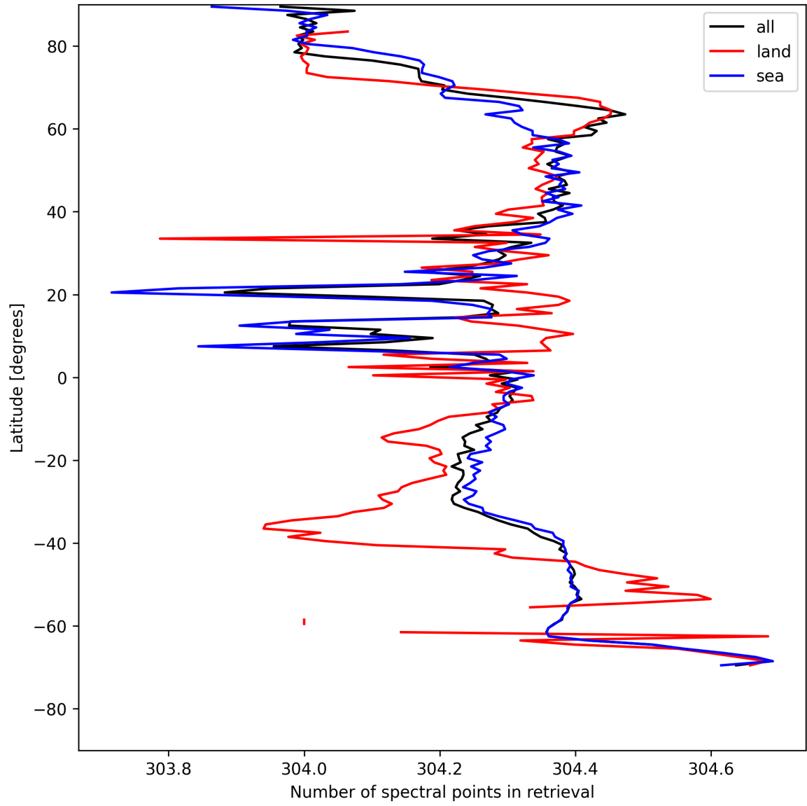
Figure 14: Zonal average of “Number of spectral points in retrieval” for 2025-05-12 to 2025-05-13.
