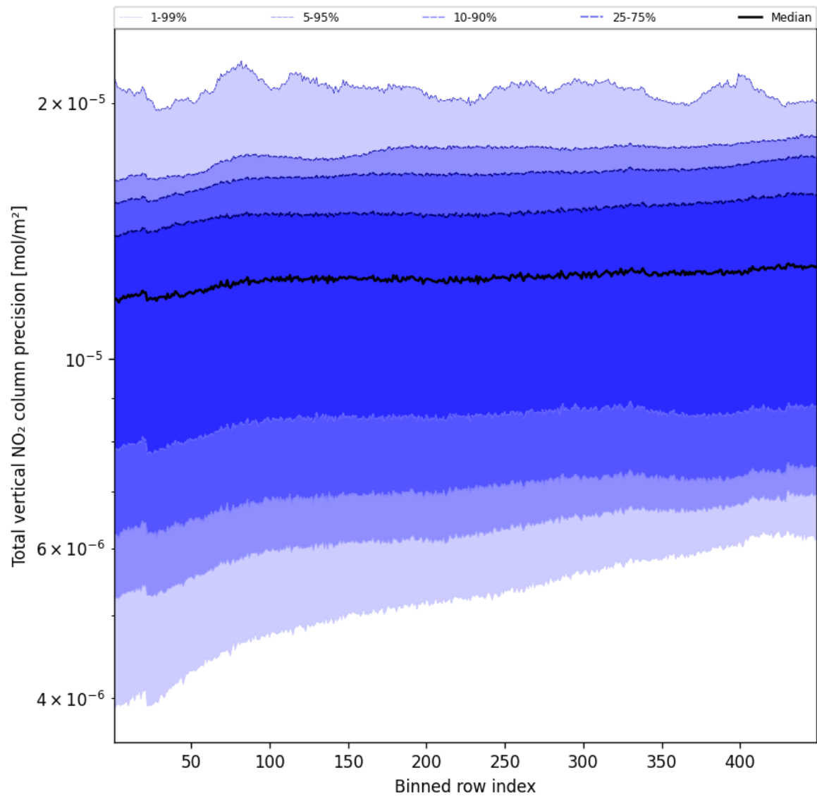
Figure 54: Along track statistics of “Total vertical NO 2 column precision” for 2025-05-12 to 2025-05-13
