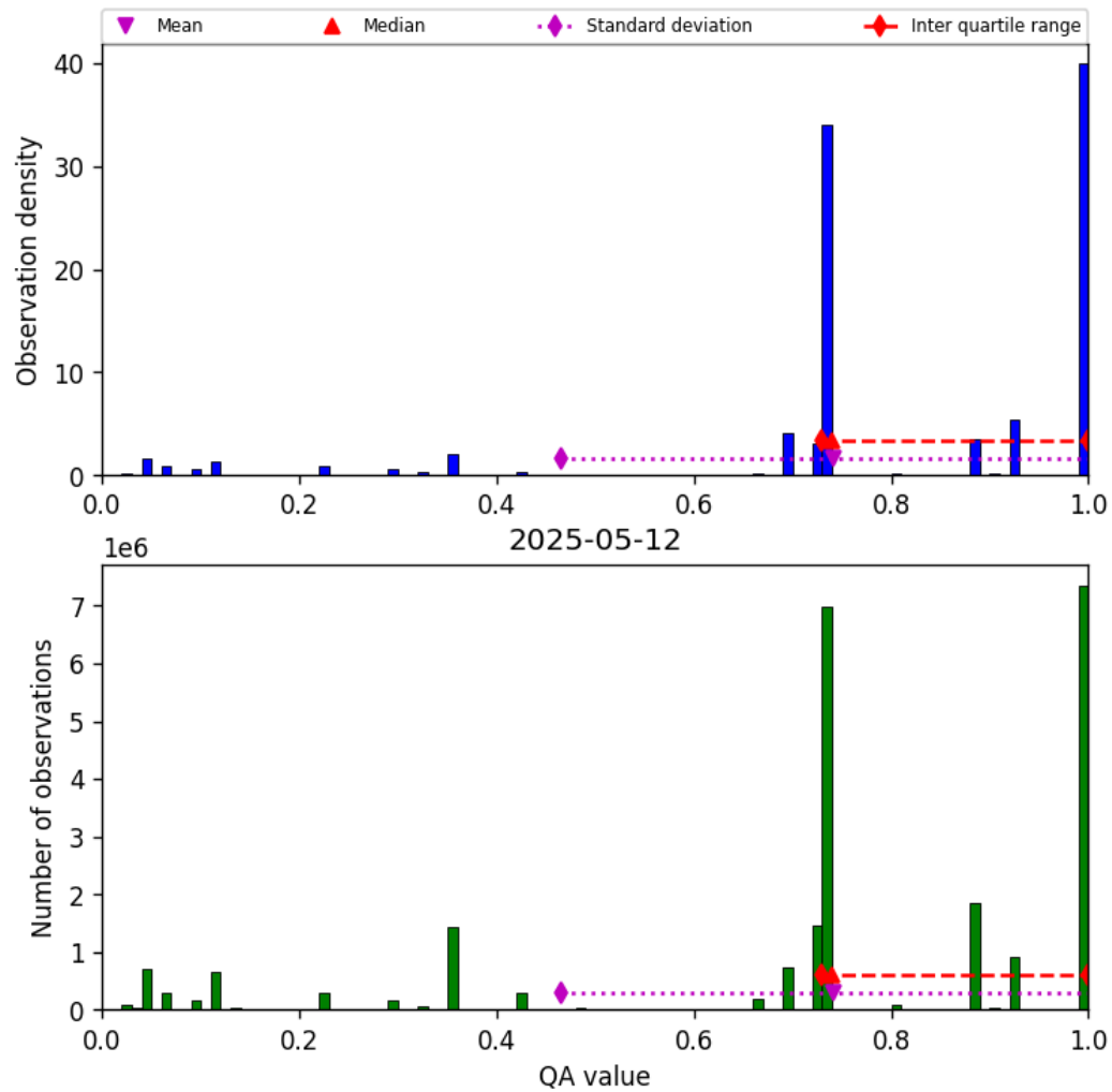
Figure 26: Histogram of “QA value” for 2025-05-12 to 2025-05-13
