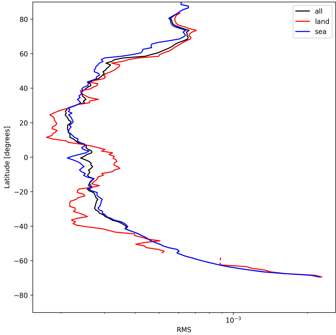
Figure 24: Zonal average of “RMS” for 2025-05-12 to 2025-05-13.
