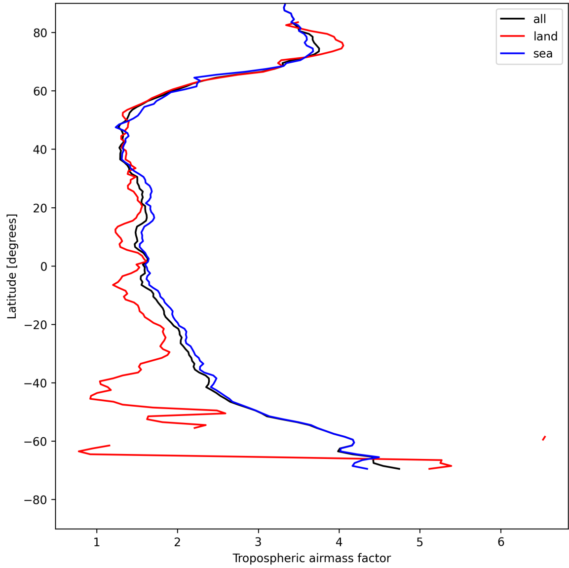
Figure 12: Zonal average of “Tropospheric airmass factor” for 2025-05-12 to 2025-05-13.
