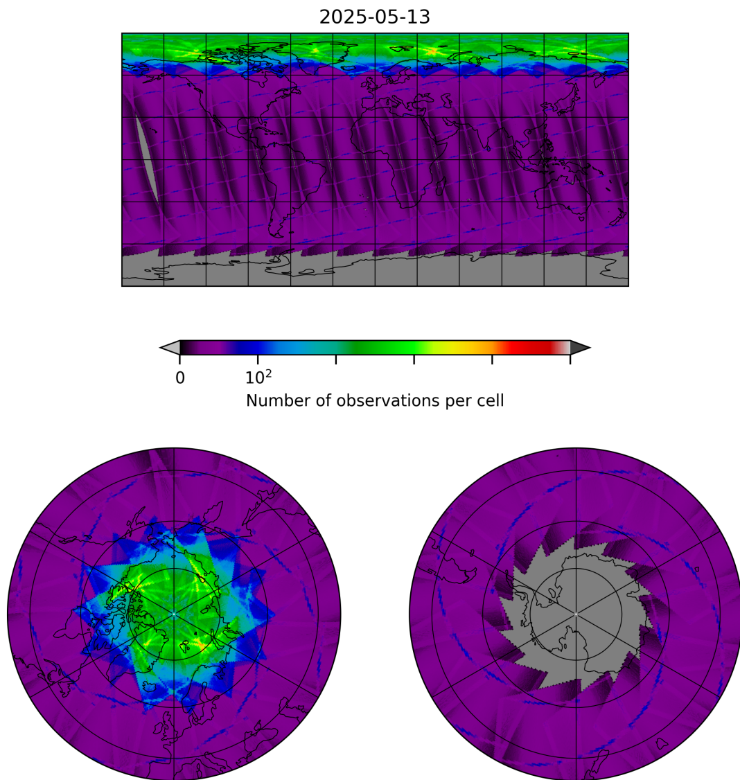
Figure 8: Map of the number of observations for 2025-05-13 to 2025-05-13
