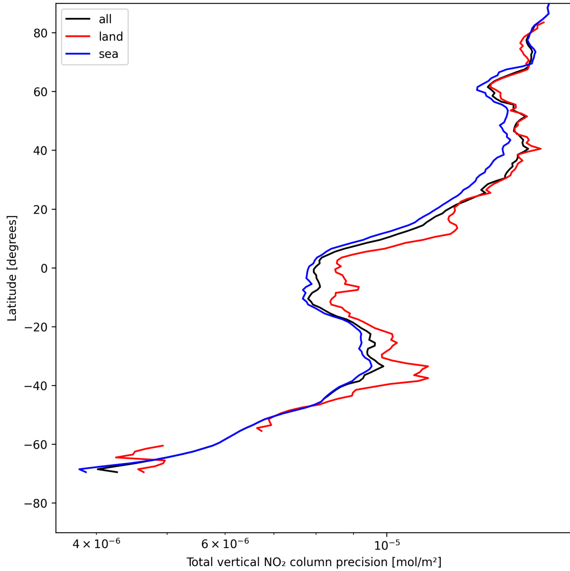
Figure 20: Zonal average of “Total vertical NO 2 column precision” for 2025-05-13 to 2025-05-13.
