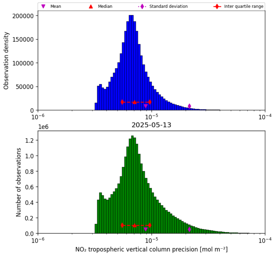
Figure 28: Histogram of “NO 2 tropospheric vertical column precision” for 2025-05-13 to 2025-05-13
