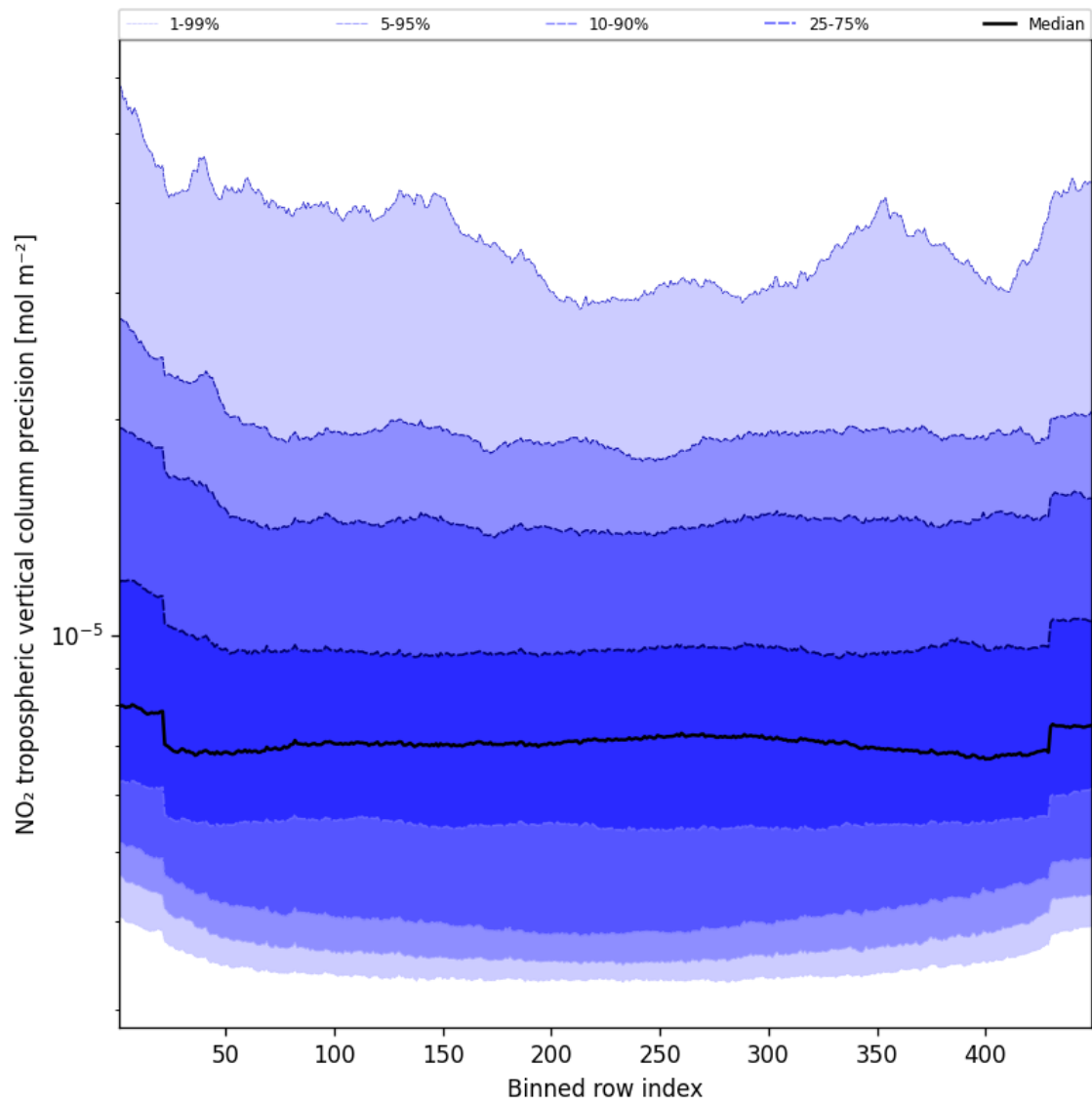
Figure 45: Along track statistics of “NO 2 tropospheric vertical column precision” for 2025-05-13 to 2025-05-13
