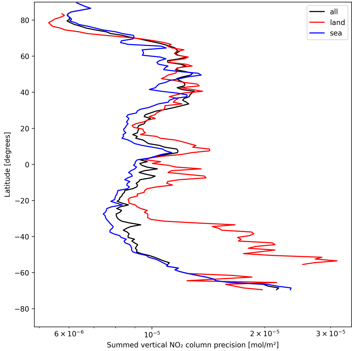
Figure 22: Zonal average of “Summed vertical NO 2 column precision” for 2025-05-13 to 2025-05-13.
