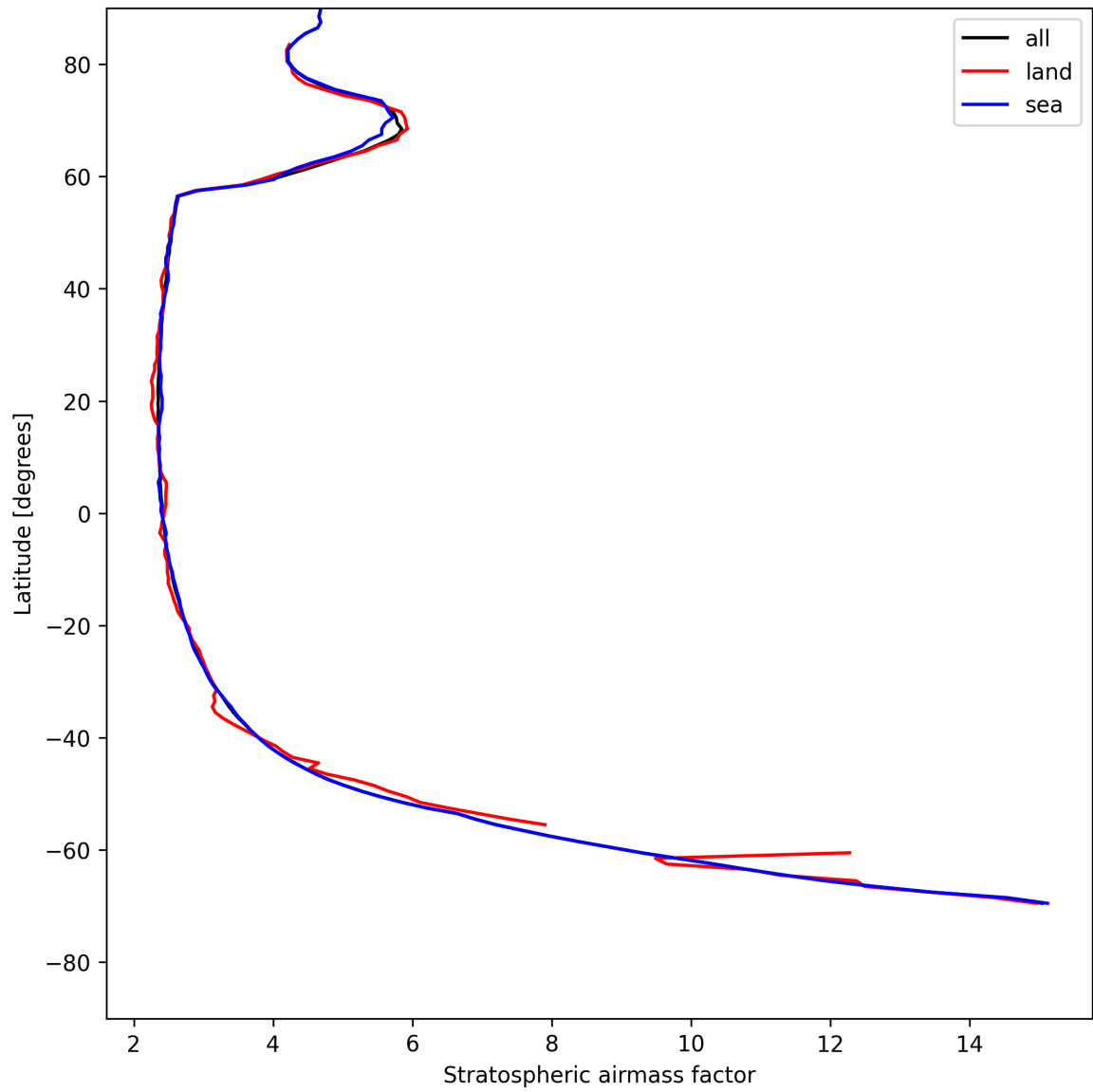
Figure 25: Zonal average of “Stratospheric air mass factor” for 2025-05-13 to 2025-05-13.
