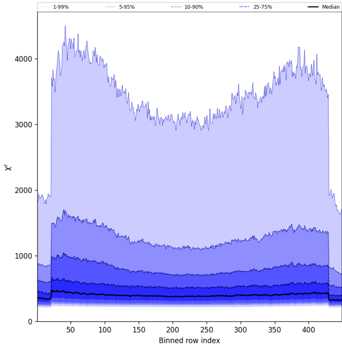
Figure 57: Along track statistics of “ \chi^2 ” for 2025-05-13 to 2025-05-13
