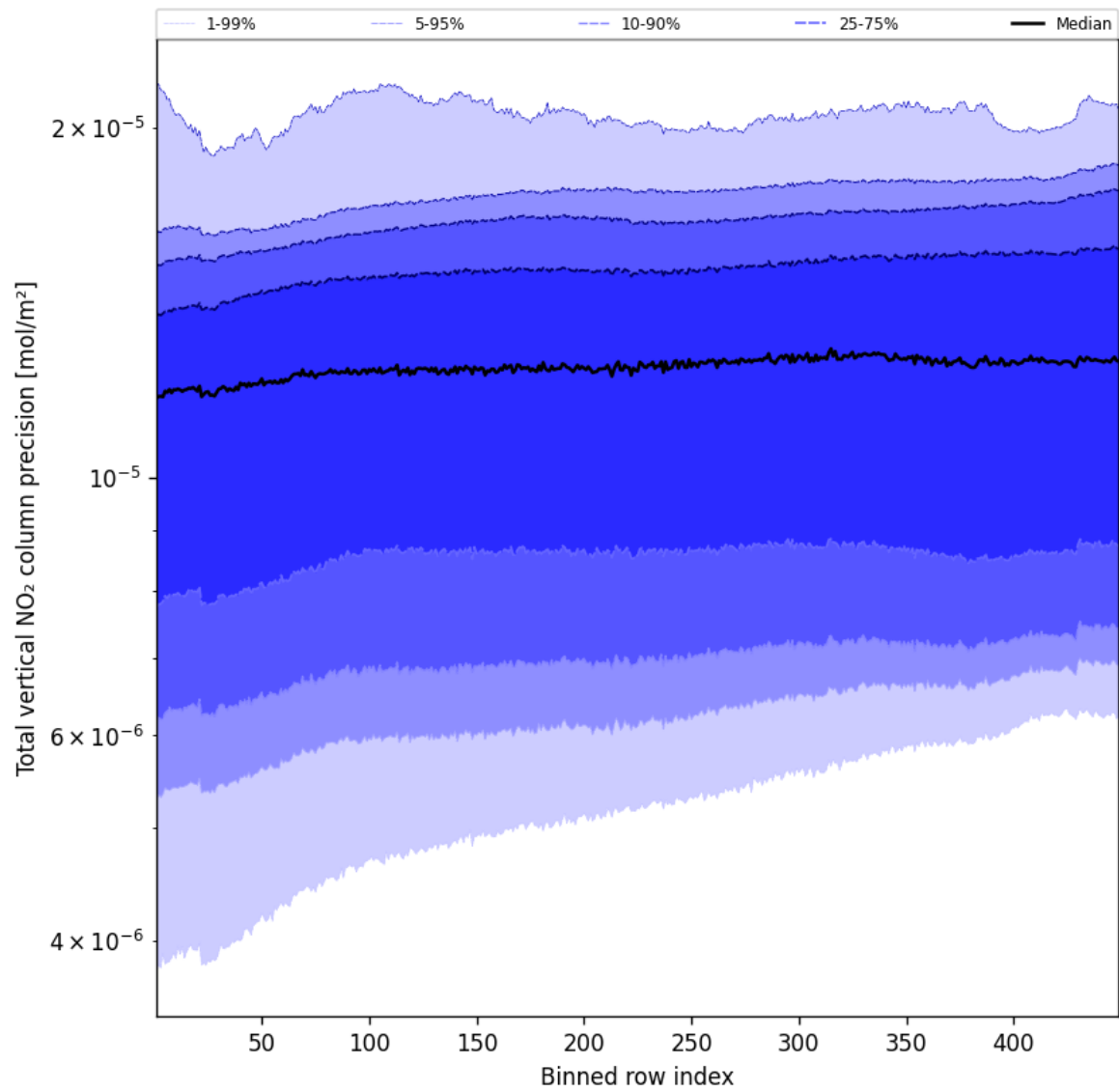
Figure 54: Along track statistics of “Total vertical NO 2 column precision” for 2025-05-13 to 2025-05-13
