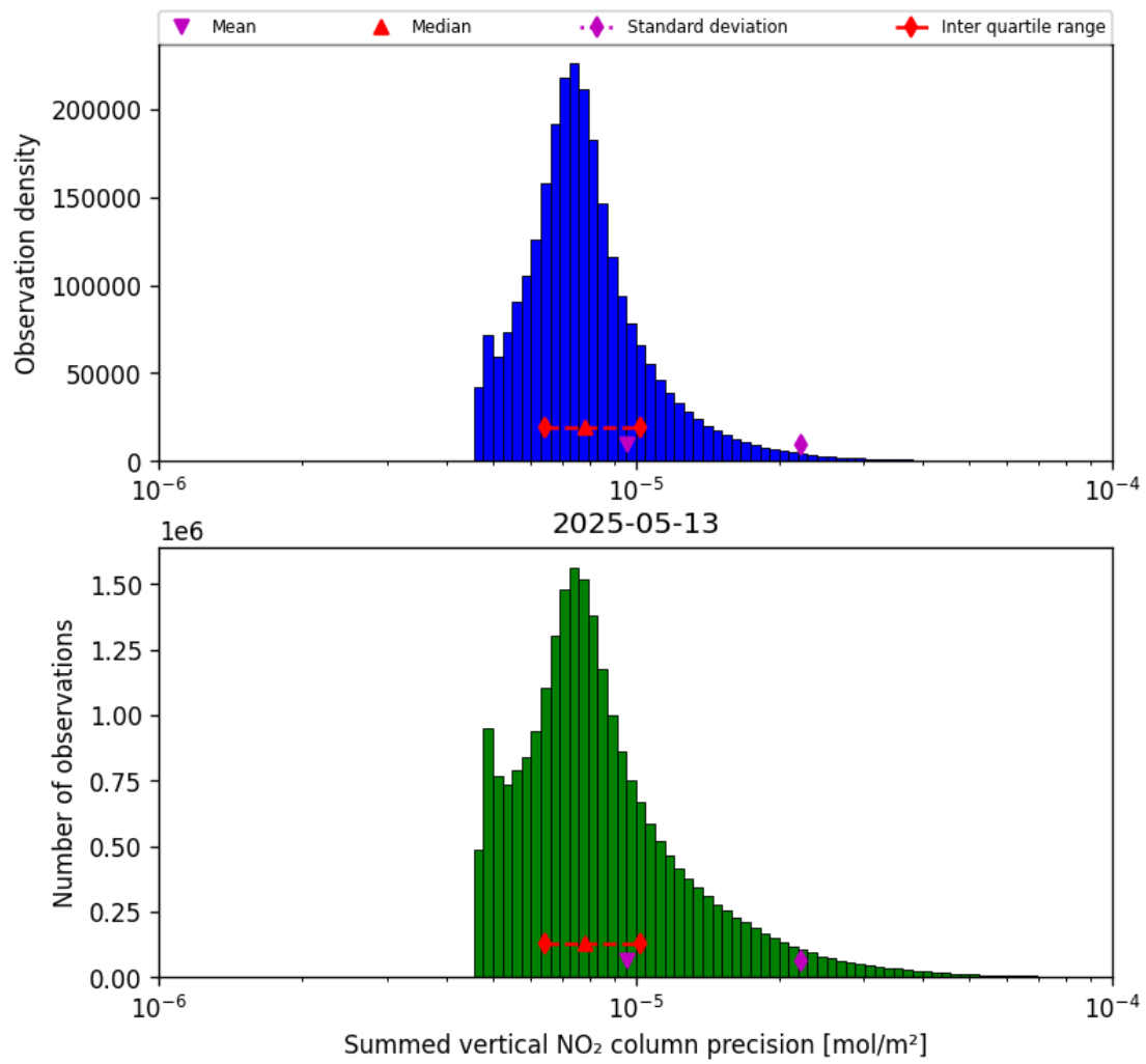
Figure 39: Histogram of "Summed vertical NO 2 column precision" for 2025-05-13 to 2025-05-13
