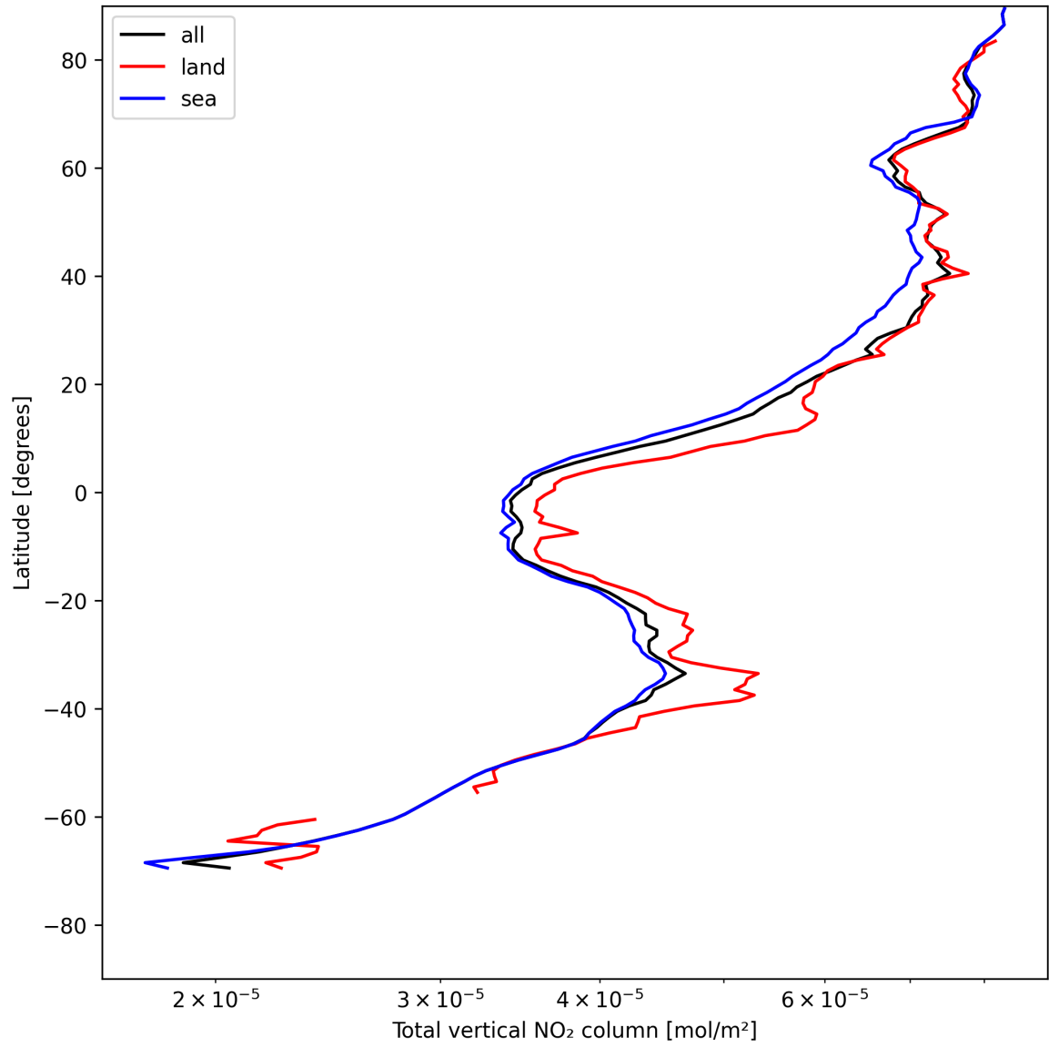
Figure 19: Zonal average of “Total vertical NO 2 column” for 2025-05-13 to 2025-05-13.
