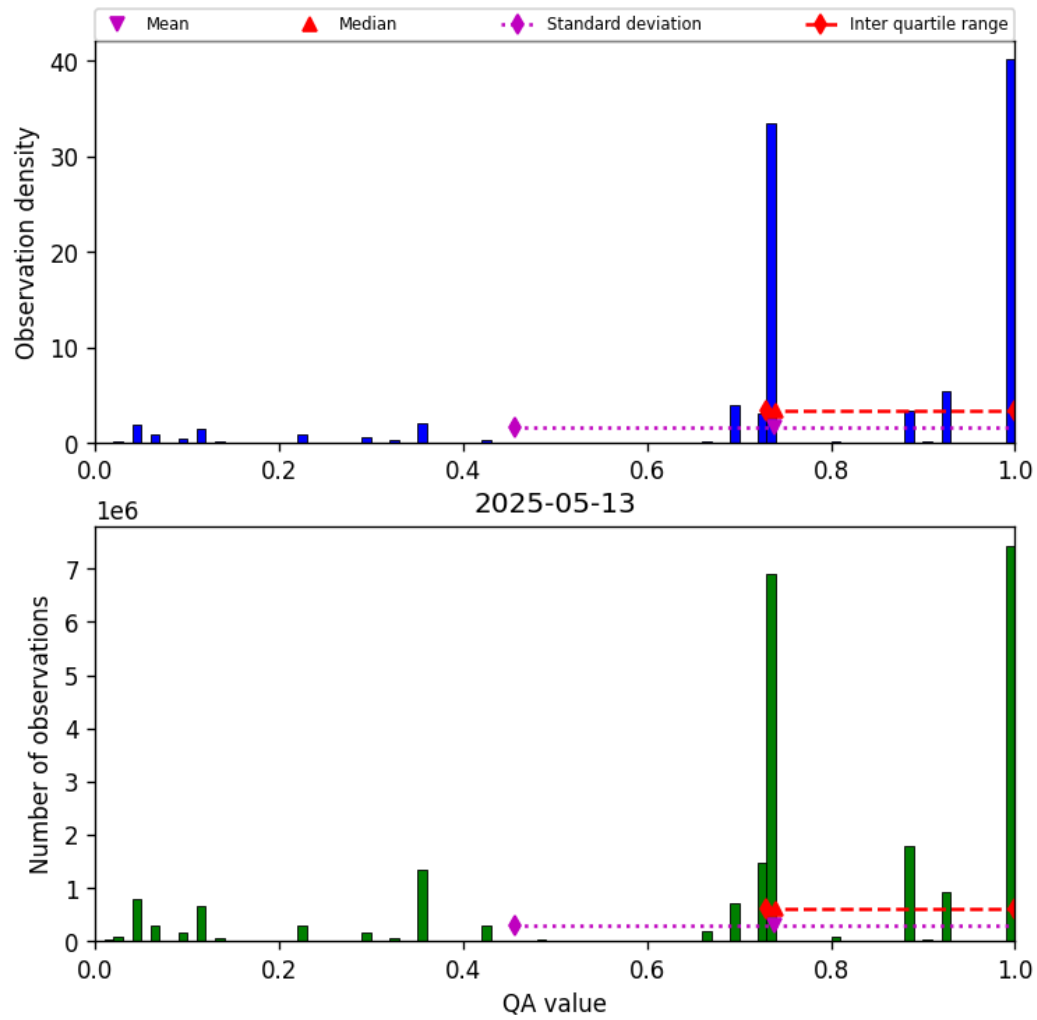
Figure 26: Histogram of “QA value” for 2025-05-13 to 2025-05-13
