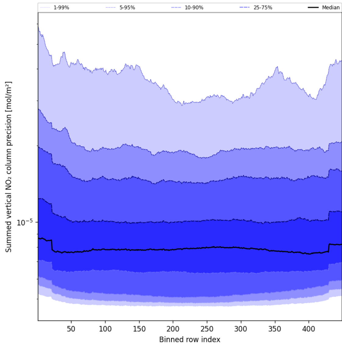
Figure 56: Along track statistics of “Summed vertical NO 2 column precision” for 2025-05-13 to 2025-05-13
