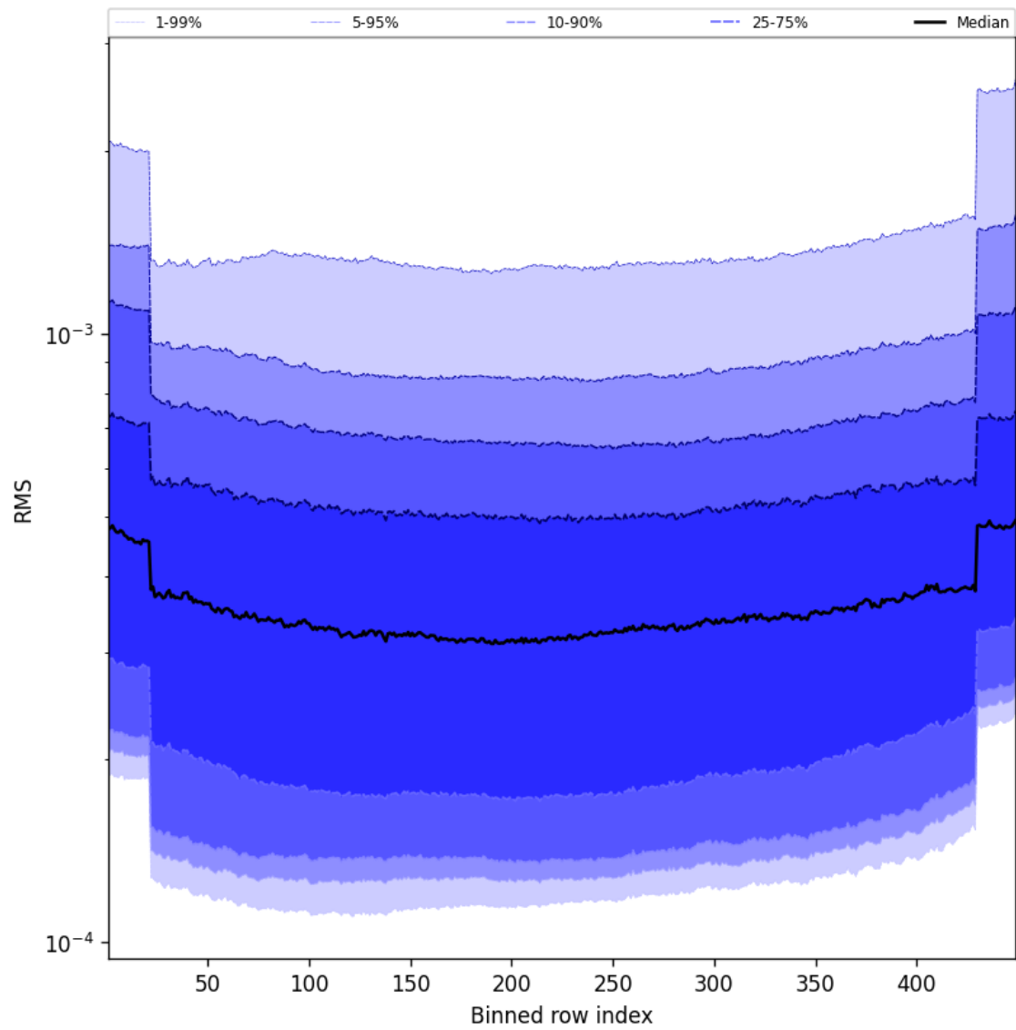
Figure 58: Along track statistics of “RMS” for 2025-05-13 to 2025-05-13
