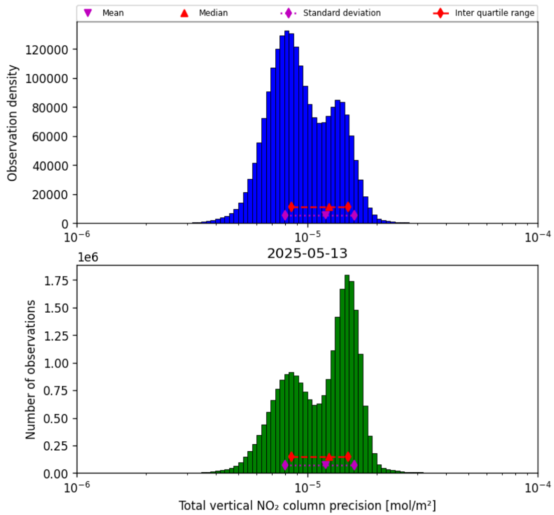
Figure 37: Histogram of “Total vertical NO 2 column precision” for 2025-05-13 to 2025-05-13
