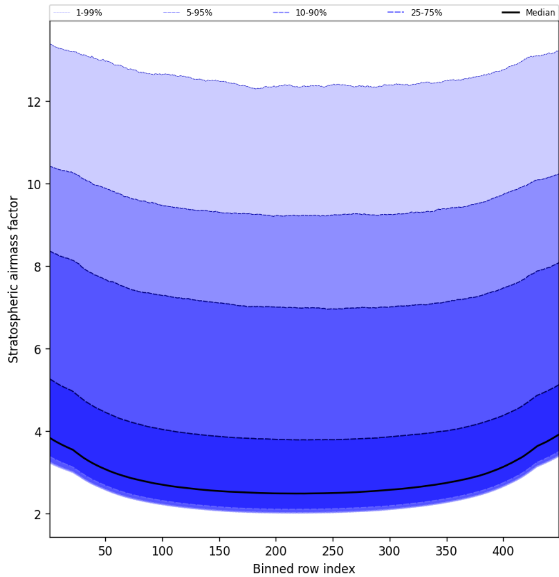
Figure 59: Along track statistics of “Stratospheric airmass factor” for 2025-05-13 to 2025-05-13
