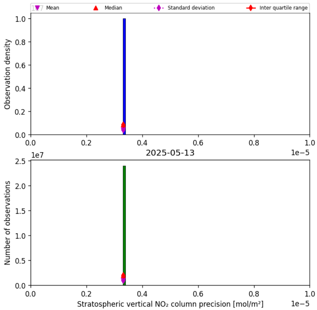
Figure 35: Histogram of “Stratospheric vertical NO 2 column precision” for 2025-05-13 to 2025-05-13
