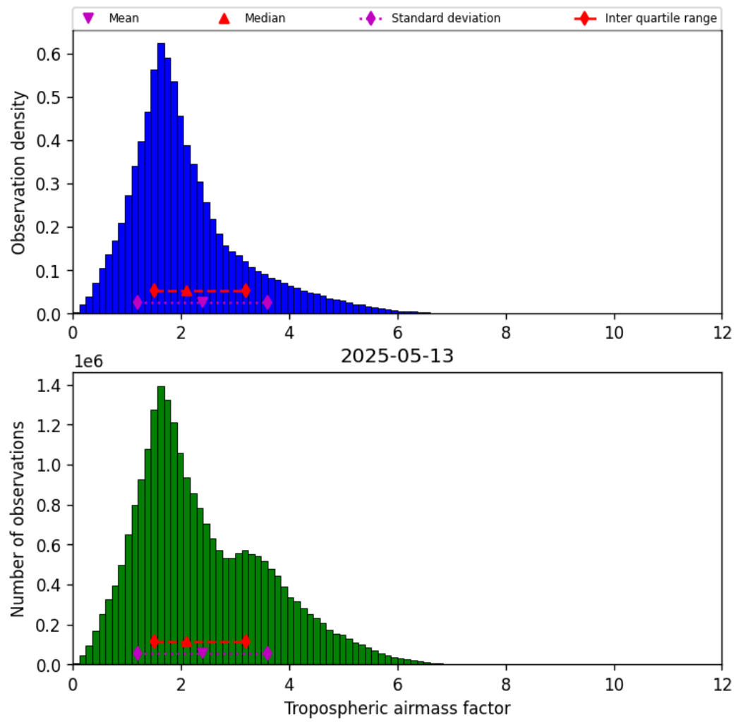
Figure 29: Histogram of “Tropospheric airmass factor” for 2025-05-13 to 2025-05-13
