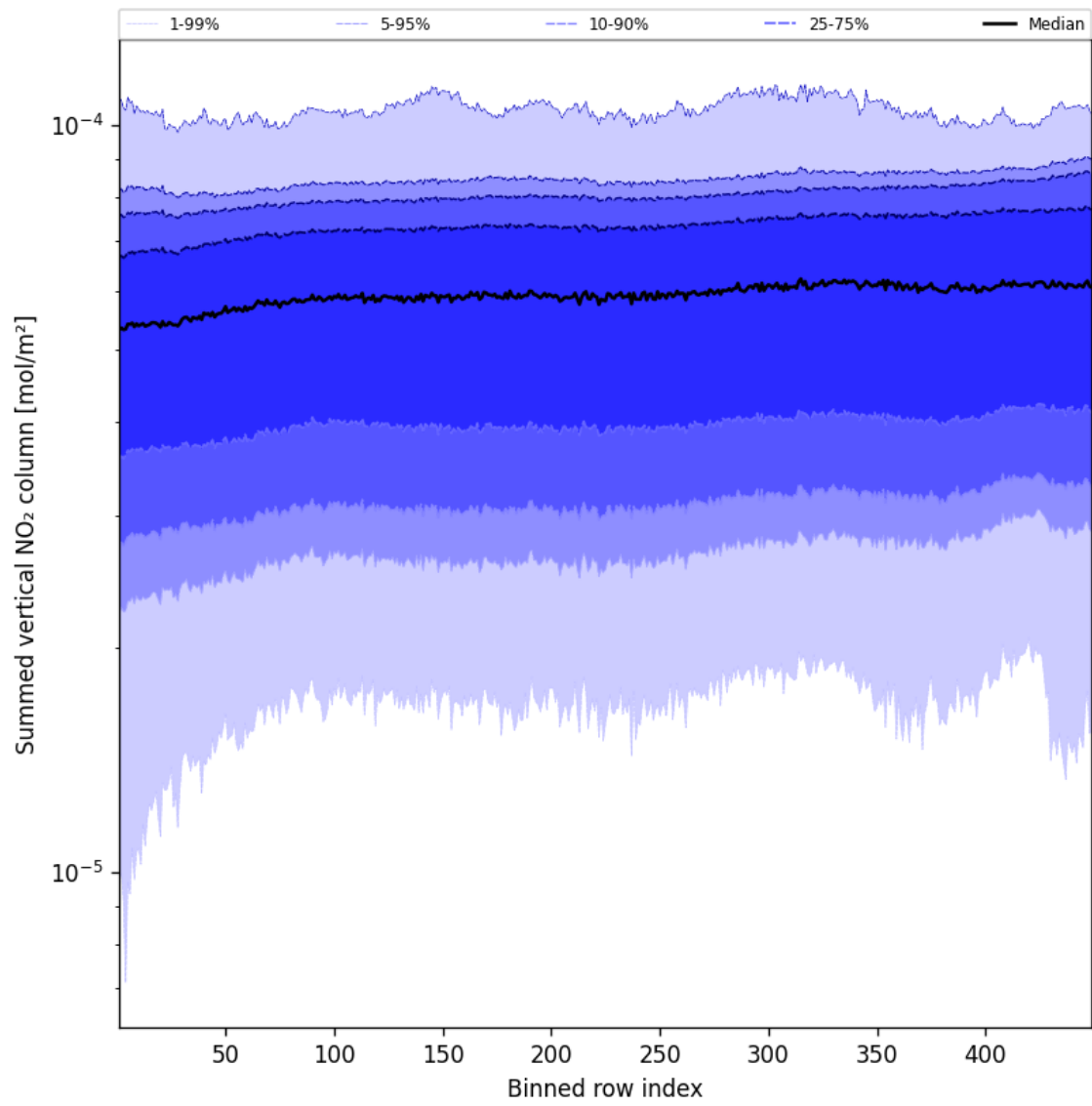
Figure 55: Along track statistics of “Summed vertical NO 2 column” for 2025-05-13 to 2025-05-13
