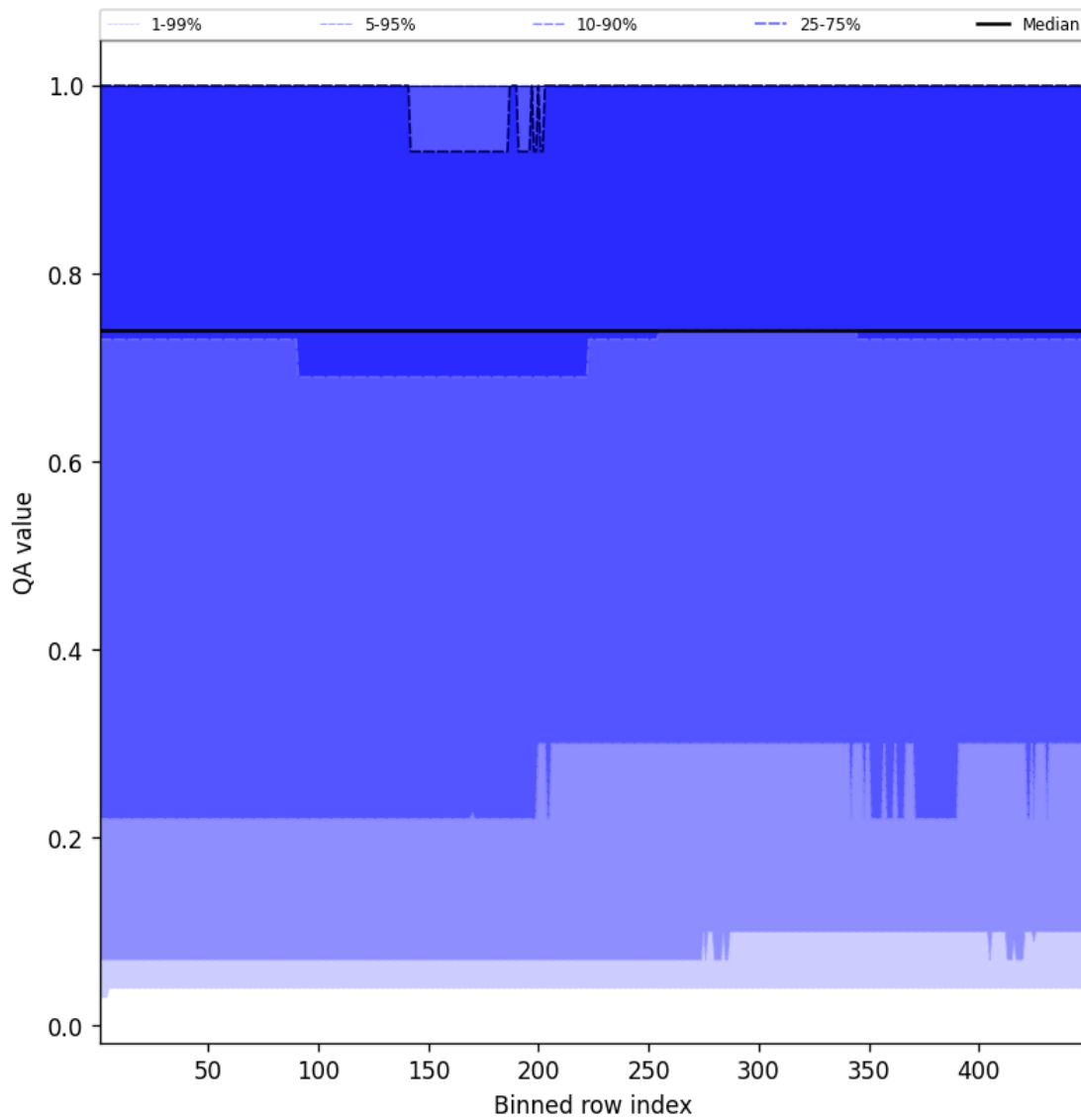
Figure 43: Along track statistics of “QA value” for 2025-05-13 to 2025-05-13
