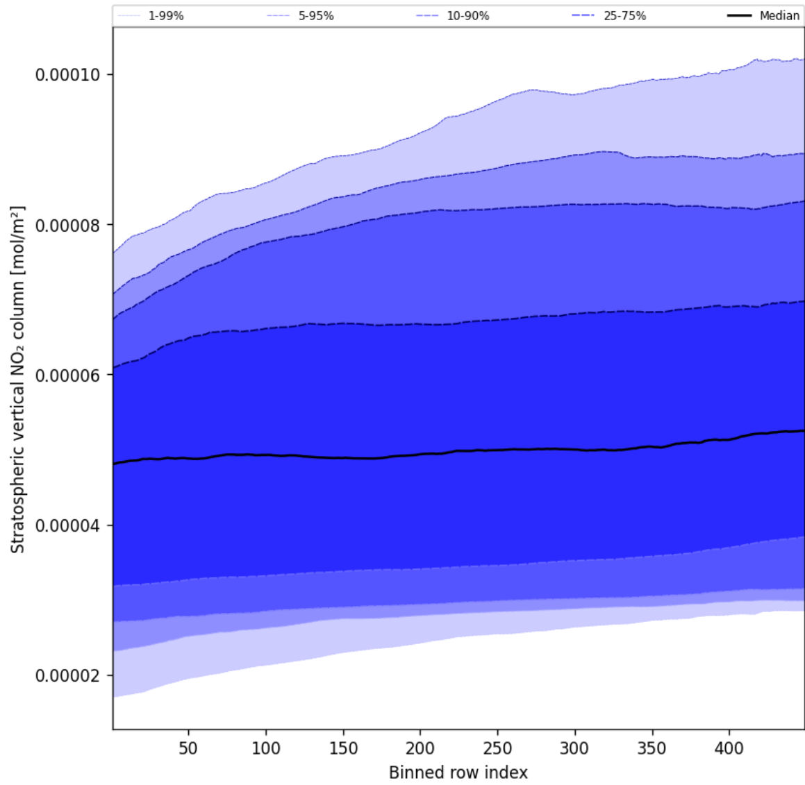
Figure 51: Along track statistics of “Stratospheric vertical NO 2 column” for 2025-05-13 to 2025-05-13
