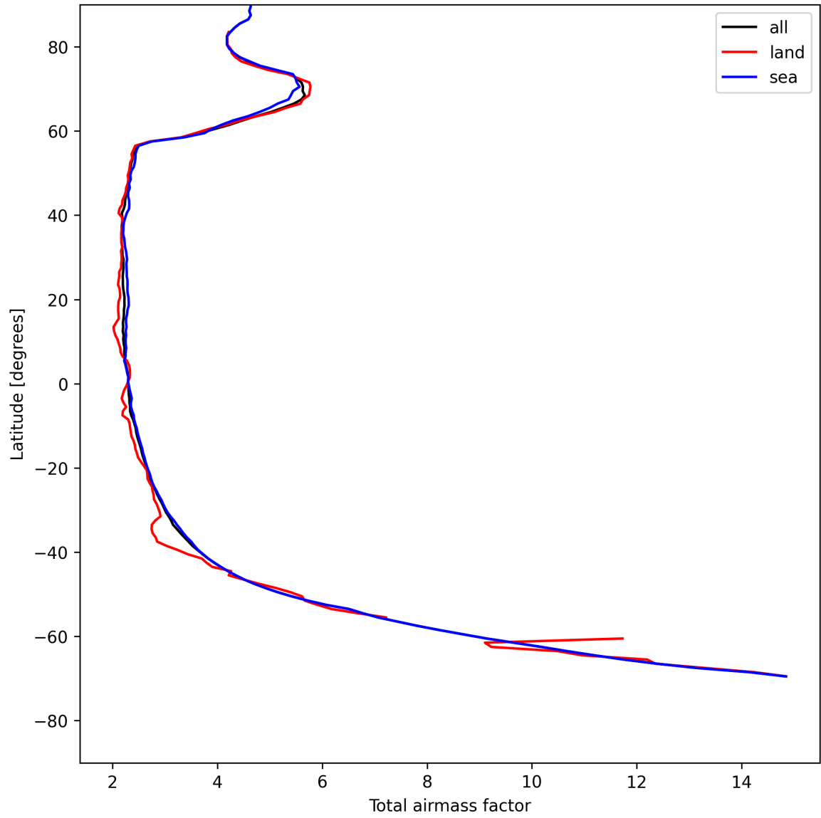
Figure 13: Zonal average of “Total airmass factor” for 2025-05-13 to 2025-05-13.
