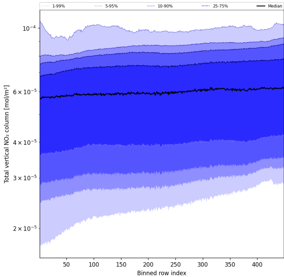
Figure 53: Along track statistics of “Total vertical NO 2 column” for 2025-05-13 to 2025-05-13
