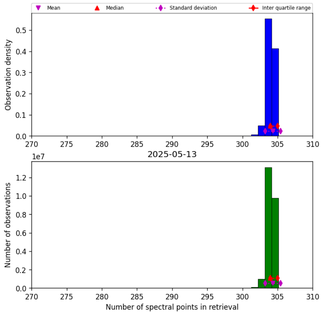
Figure 31: Histogram of “Number of spectral points in retrieval” for 2025-05-13 to 2025-05-13
