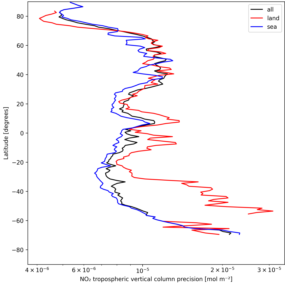
Figure 11: Zonal average of “NO 2 tropospheric vertical column precision” for 2025-05-13 to 2025-05-13.
