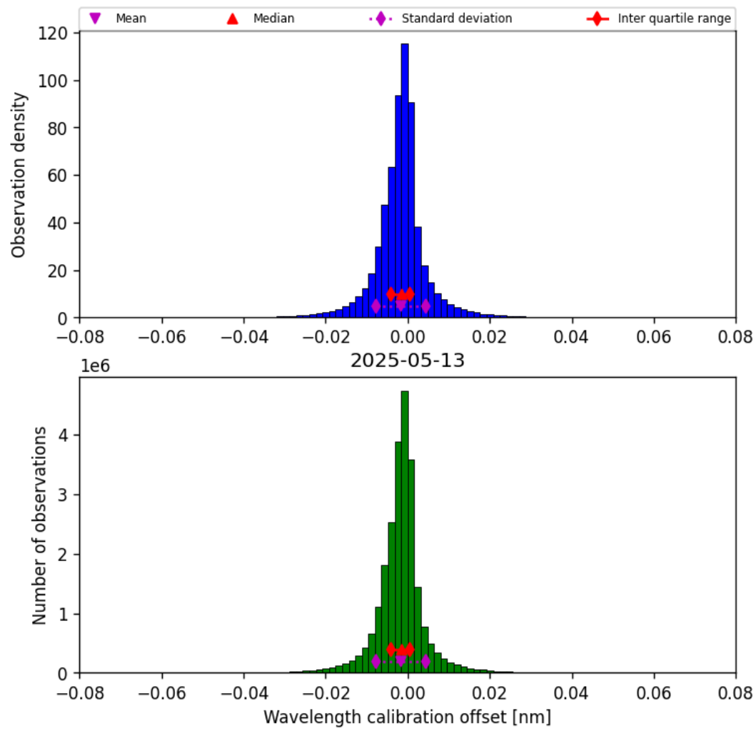
Figure 33: Histogram of “Wavelength calibration offset” for 2025-05-13 to 2025-05-13
