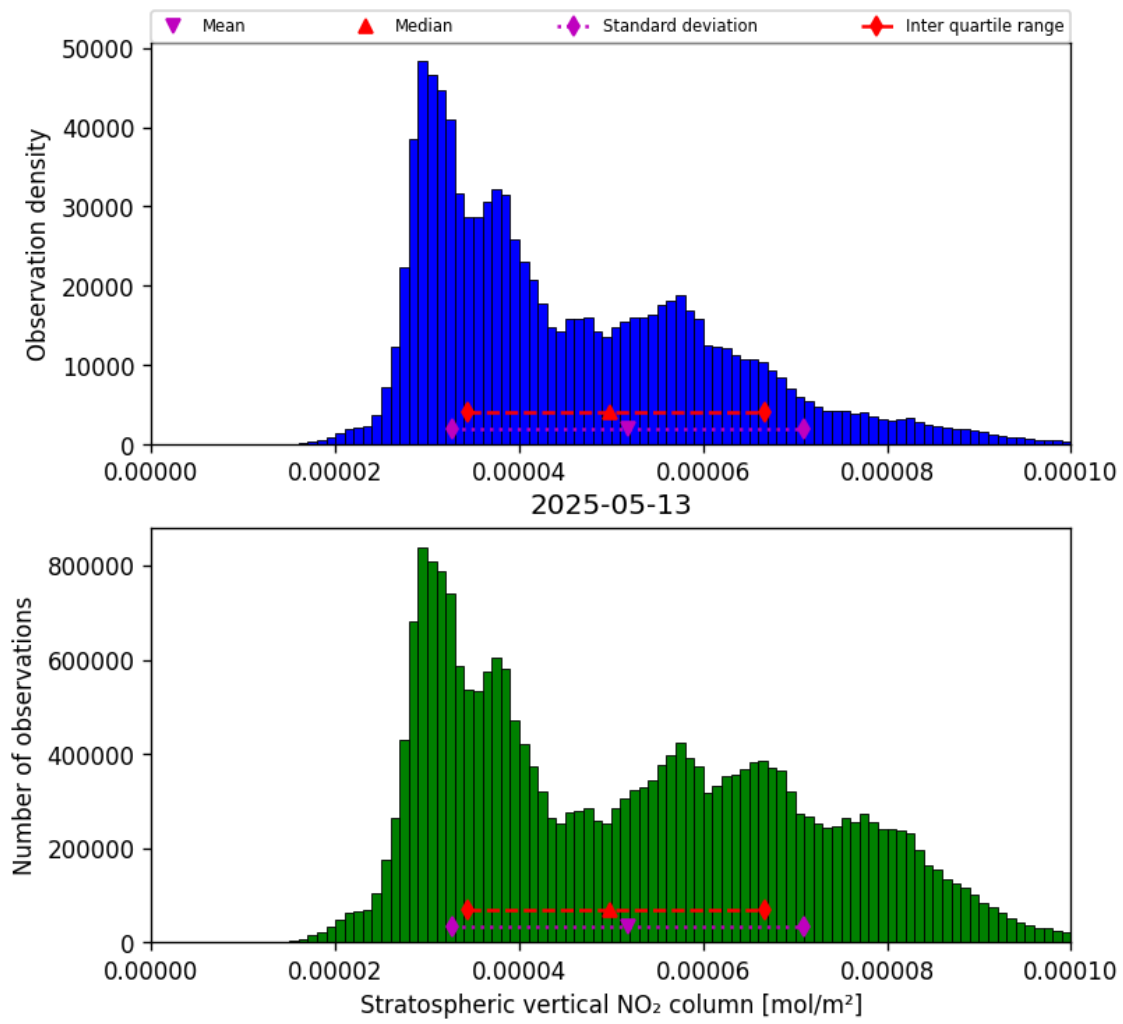
Figure 34: Histogram of “Stratospheric vertical NO 2 column” for 2025-05-13 to 2025-05-13
