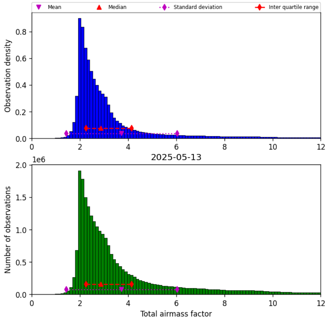
Figure 30: Histogram of “Total airmass factor” for 2025-05-13 to 2025-05-13
