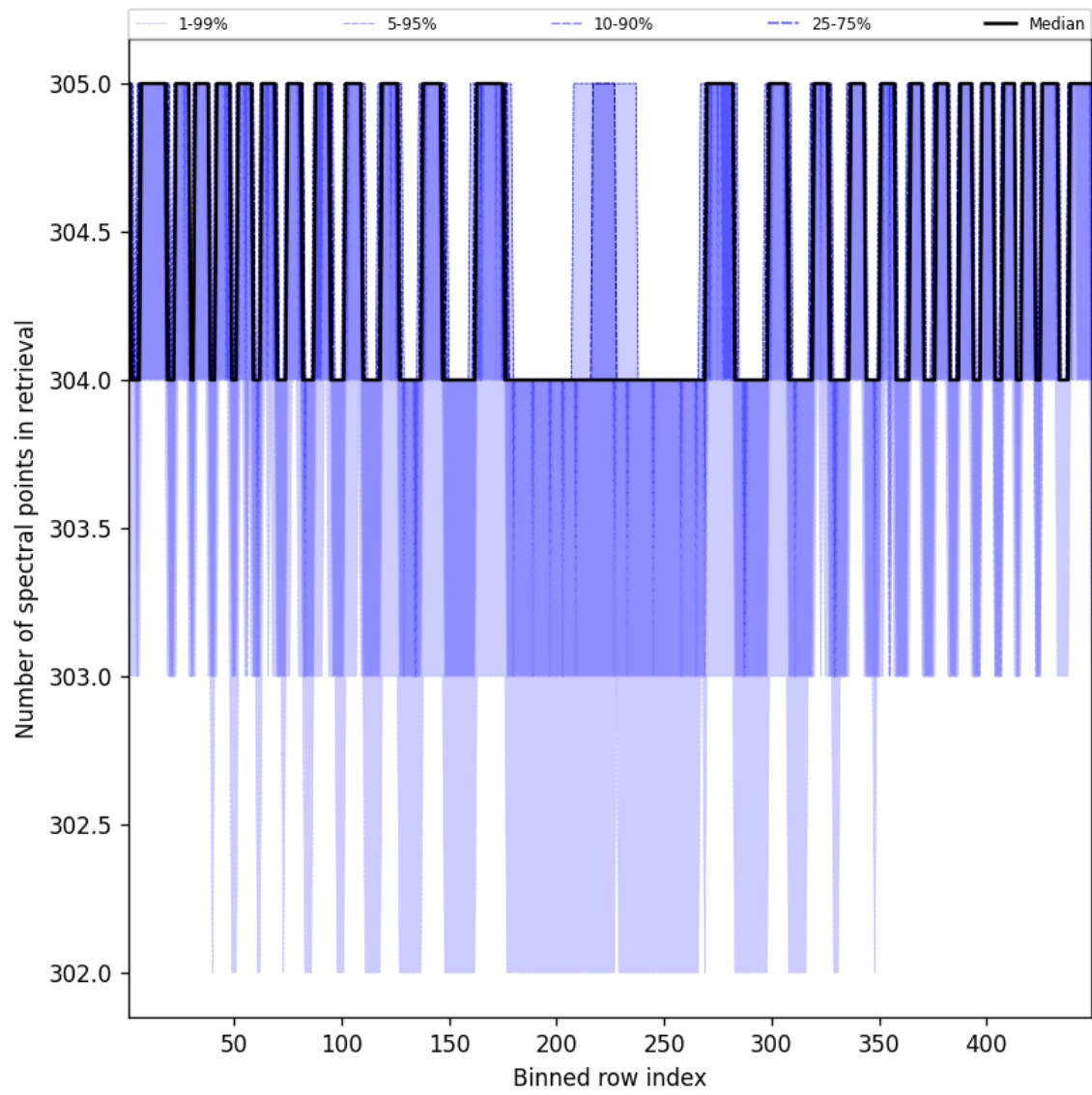
Figure 48: Along track statistics of “Number of spectral points in retrieval” for 2025-05-13 to 2025-05-13
