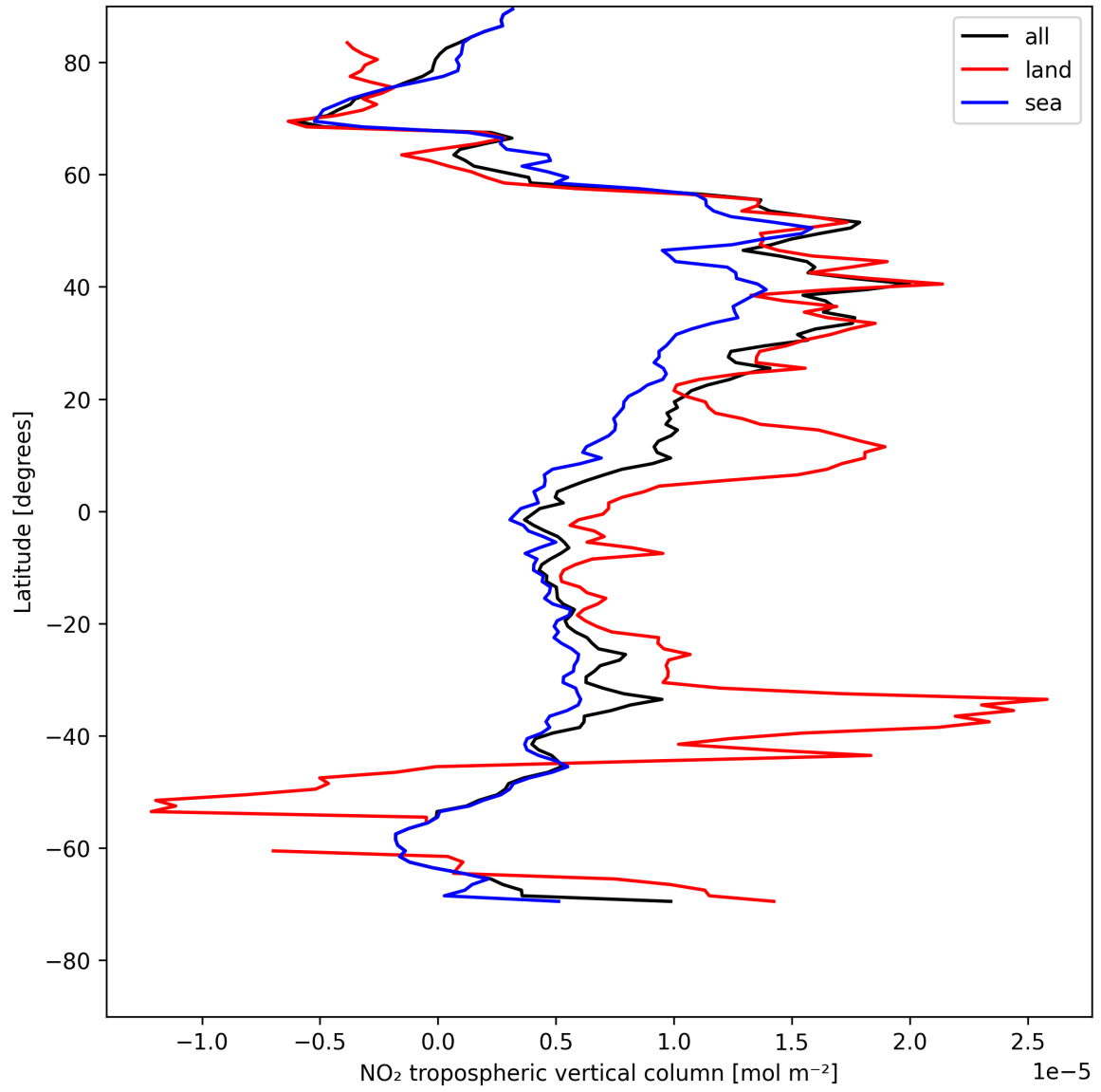
Figure 10: Zonal average of “NO 2 tropospheric vertical column” for 2025-05-13 to 2025-05-13.
