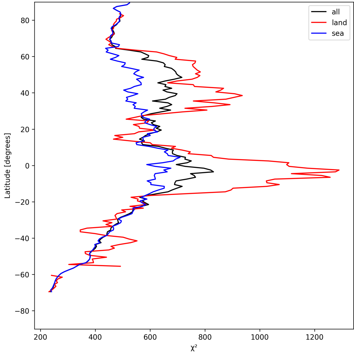
Figure 23: Zonal average of “ \chi^2 ” for 2025-05-13 to 2025-05-13.
