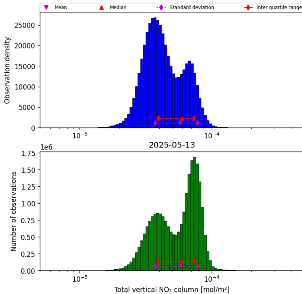
Figure 36: Histogram of "Total vertical NO 2 column" for 2025-05-13 to 2025-05-13
