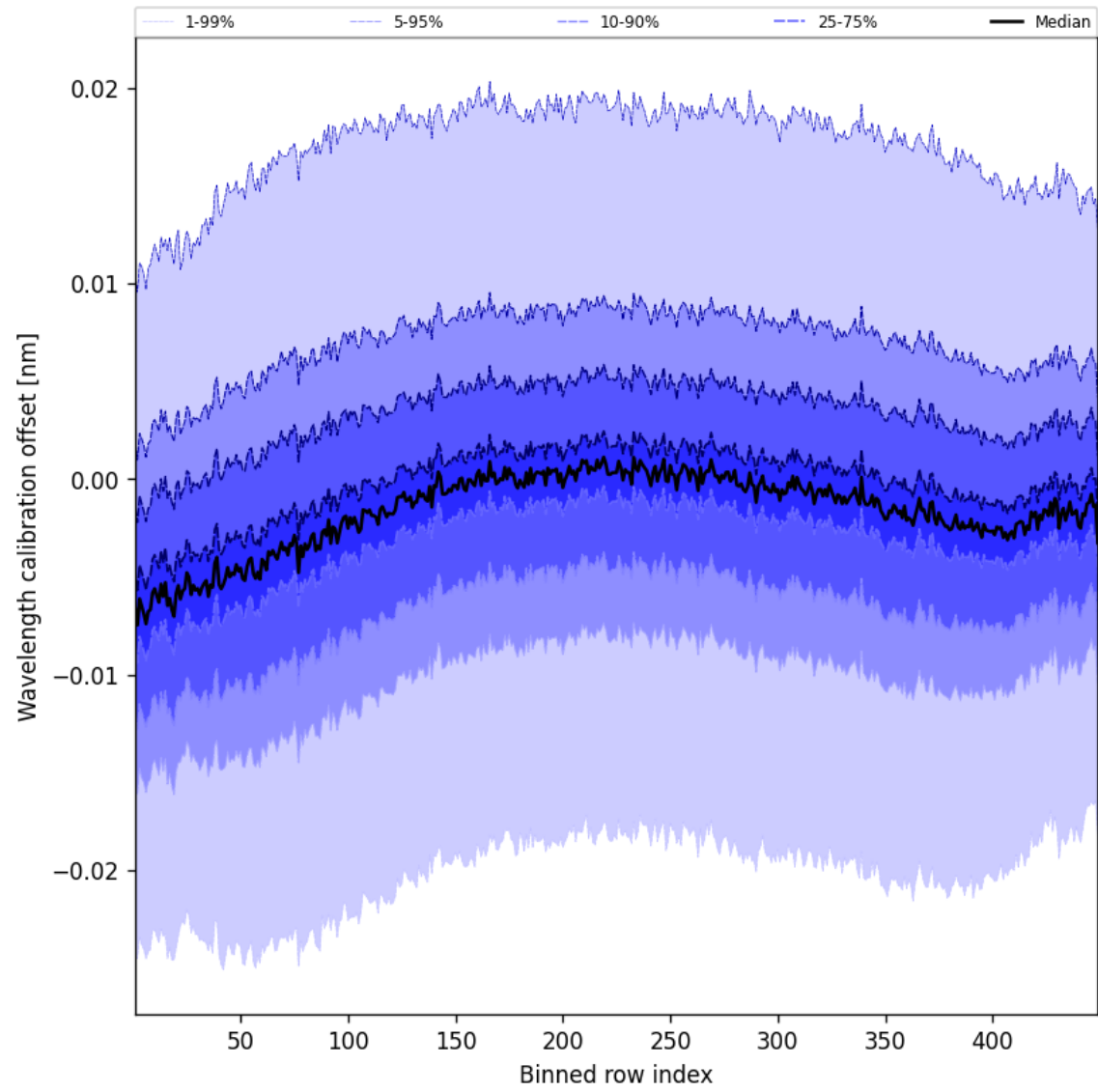
Figure 50: Along track statistics of “Wavelength calibration offset” for 2025-05-13 to 2025-05-13
