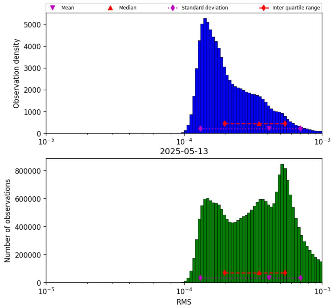
Figure 41: Histogram of “RMS” for 2025-05-13 to 2025-05-13
