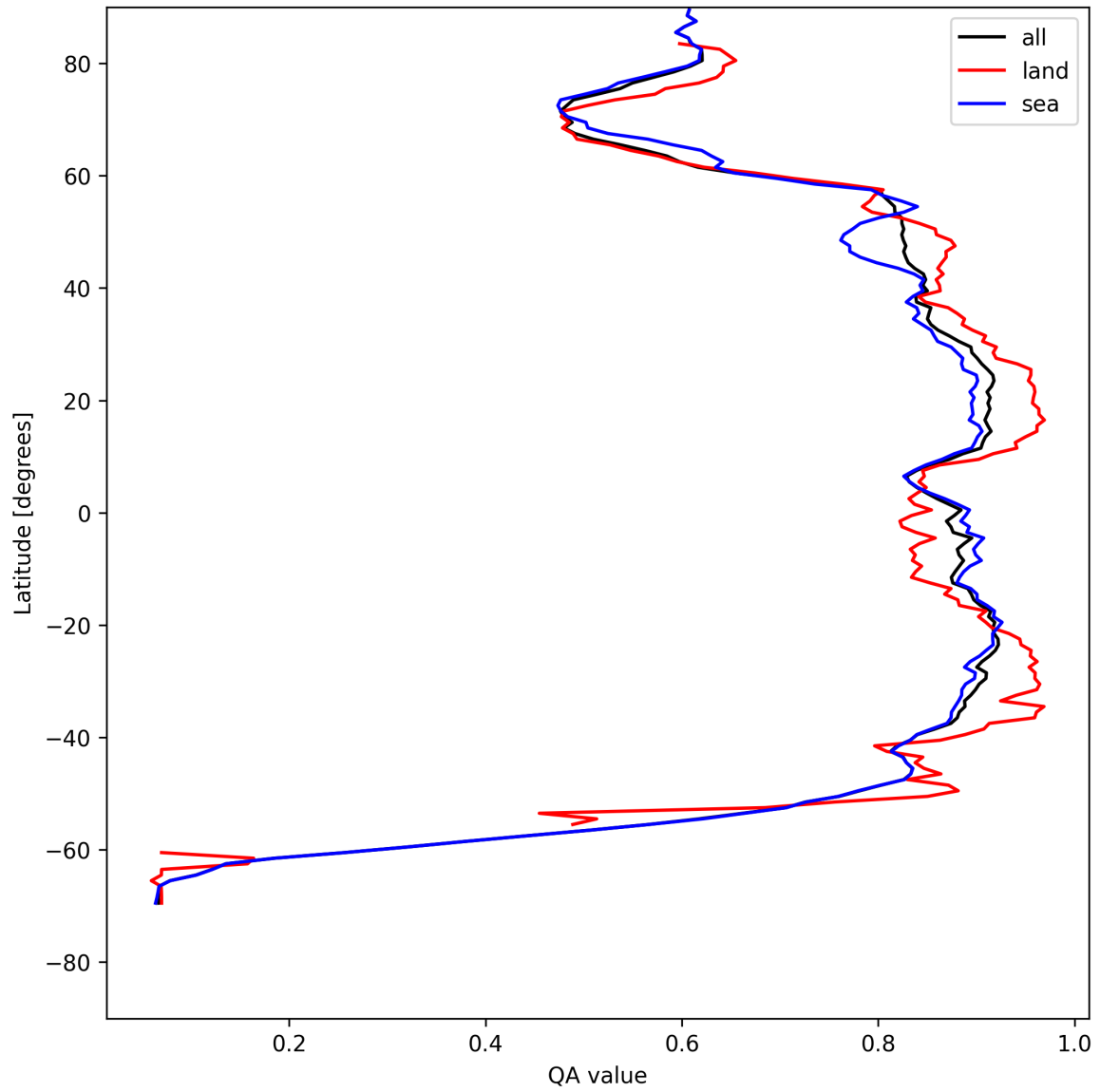
Figure 9: Zonal average of “QA value” for 2025-05-13 to 2025-05-13.
