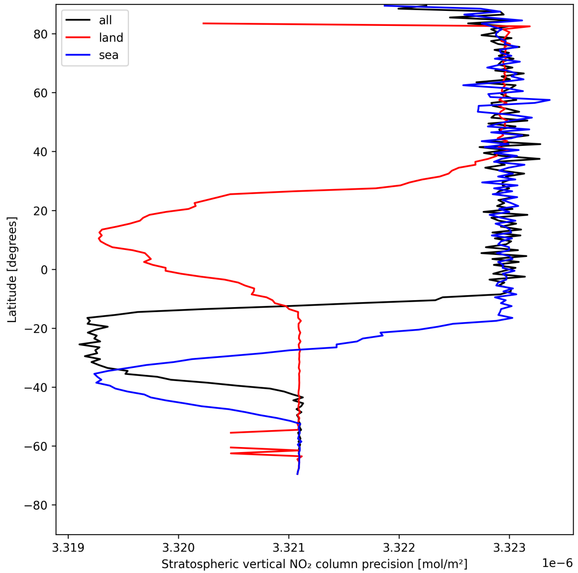
Figure 18: Zonal average of “Stratospheric vertical NO 2 column precision” for 2025-05-13 to 2025-05-13.
