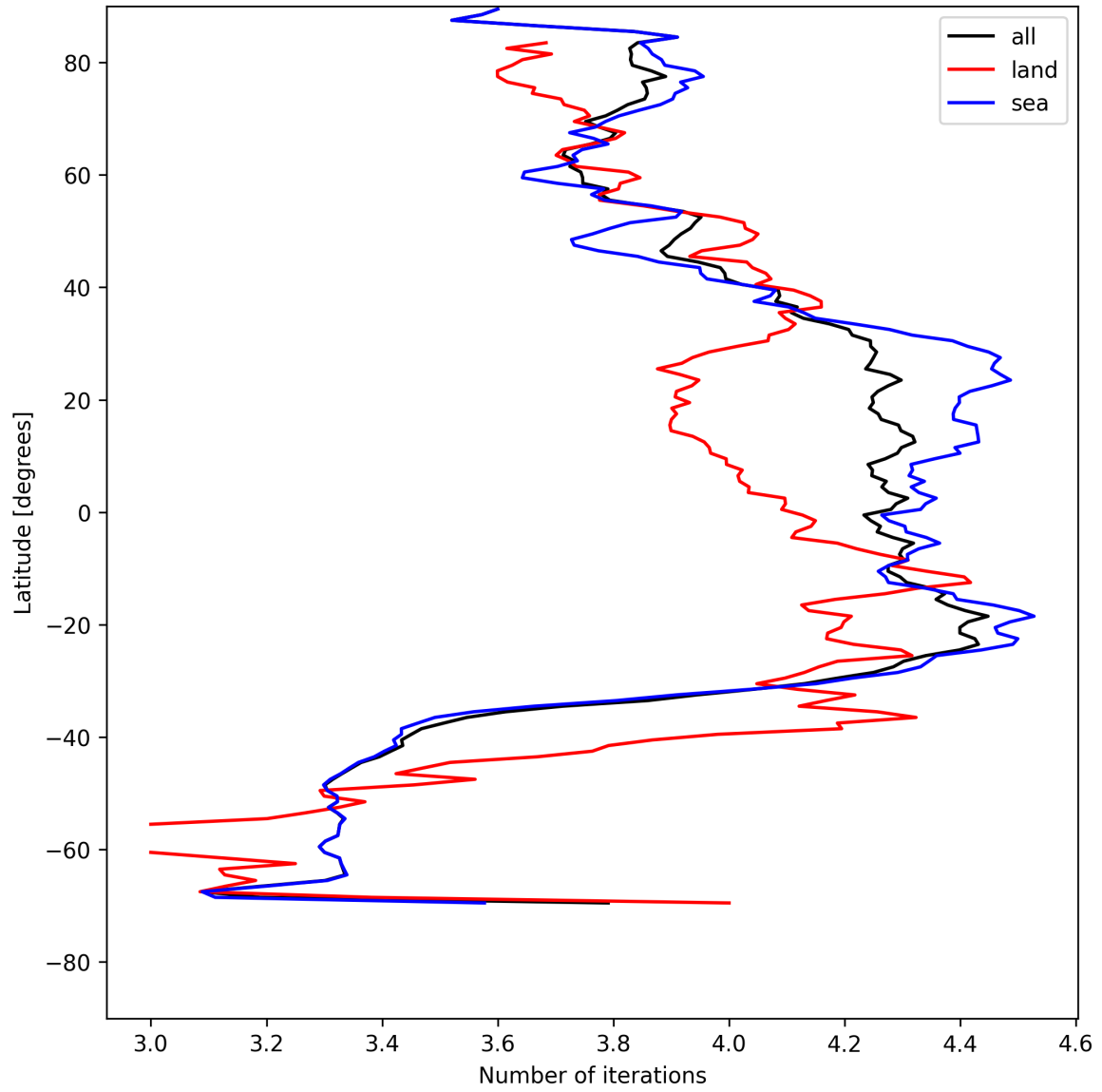
Figure 15: Zonal average of “Number of iterations” for 2025-05-13 to 2025-05-13.
