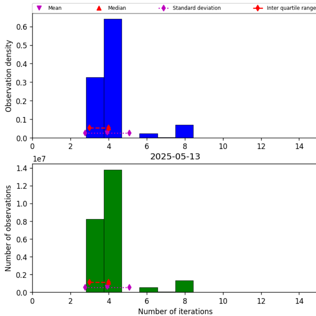
Figure 32: Histogram of “Number of iterations” for 2025-05-13 to 2025-05-13
