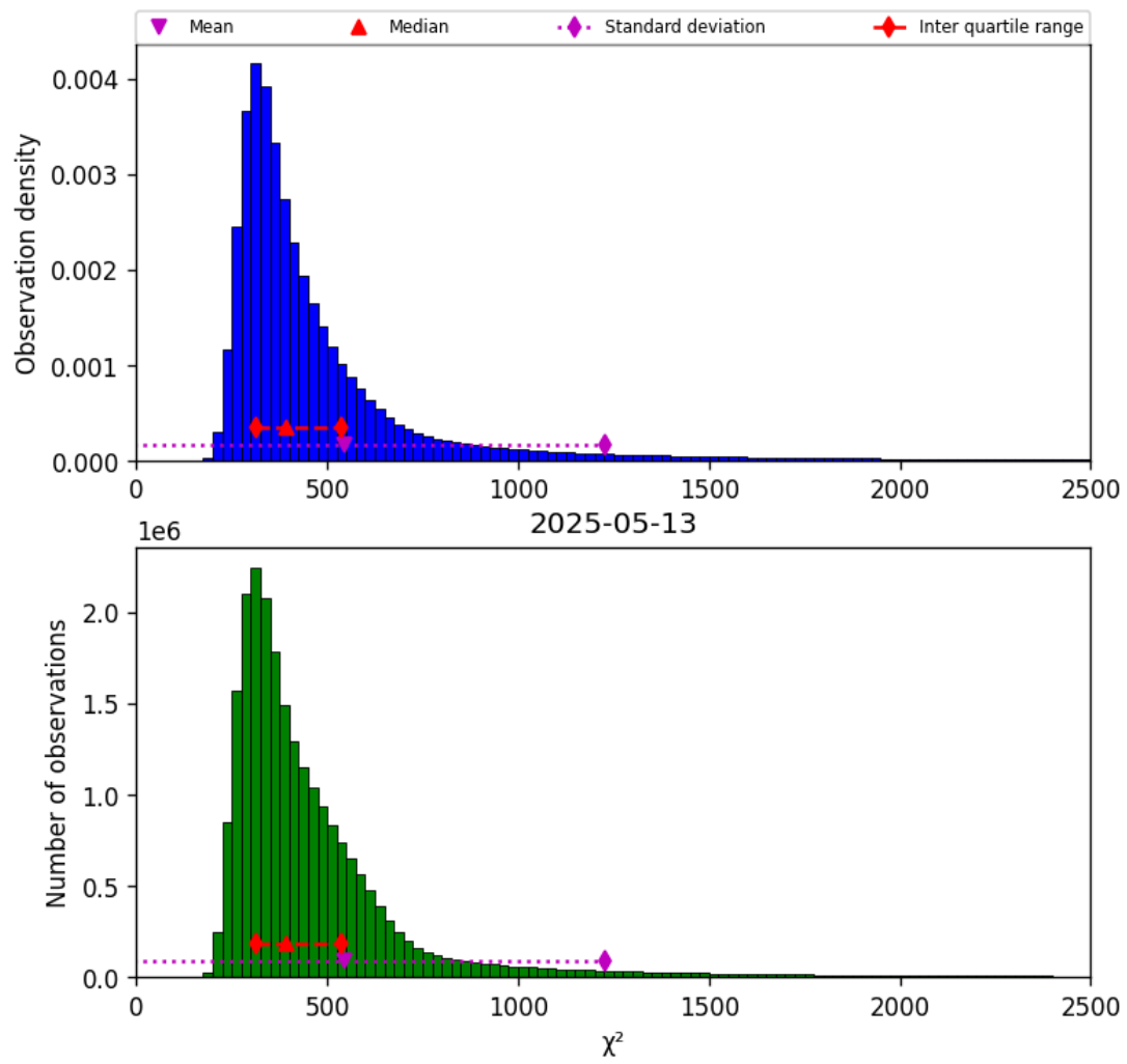
Figure 40: Histogram of “ \chi^2 ” for 2025-05-13 to 2025-05-13
