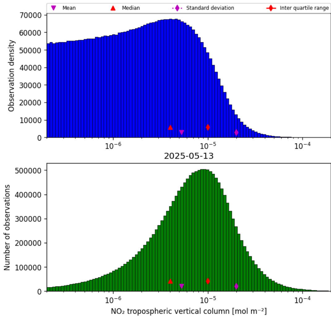
Figure 27: Histogram of “ \text{NO}_2 tropospheric vertical column” for 2025-05-13 to 2025-05-13
