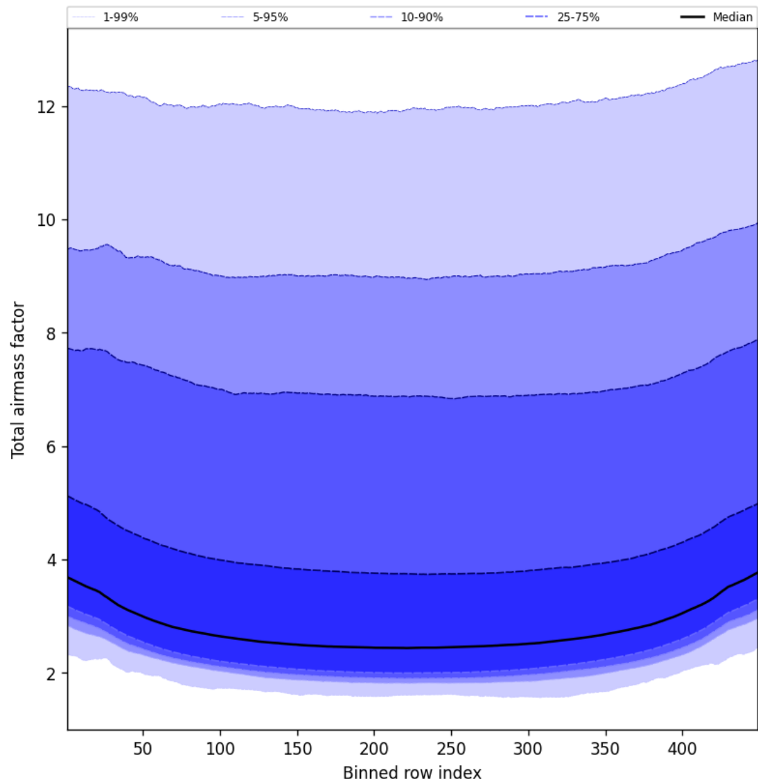
Figure 47: Along track statistics of “Total airmass factor” for 2025-05-13 to 2025-05-13
