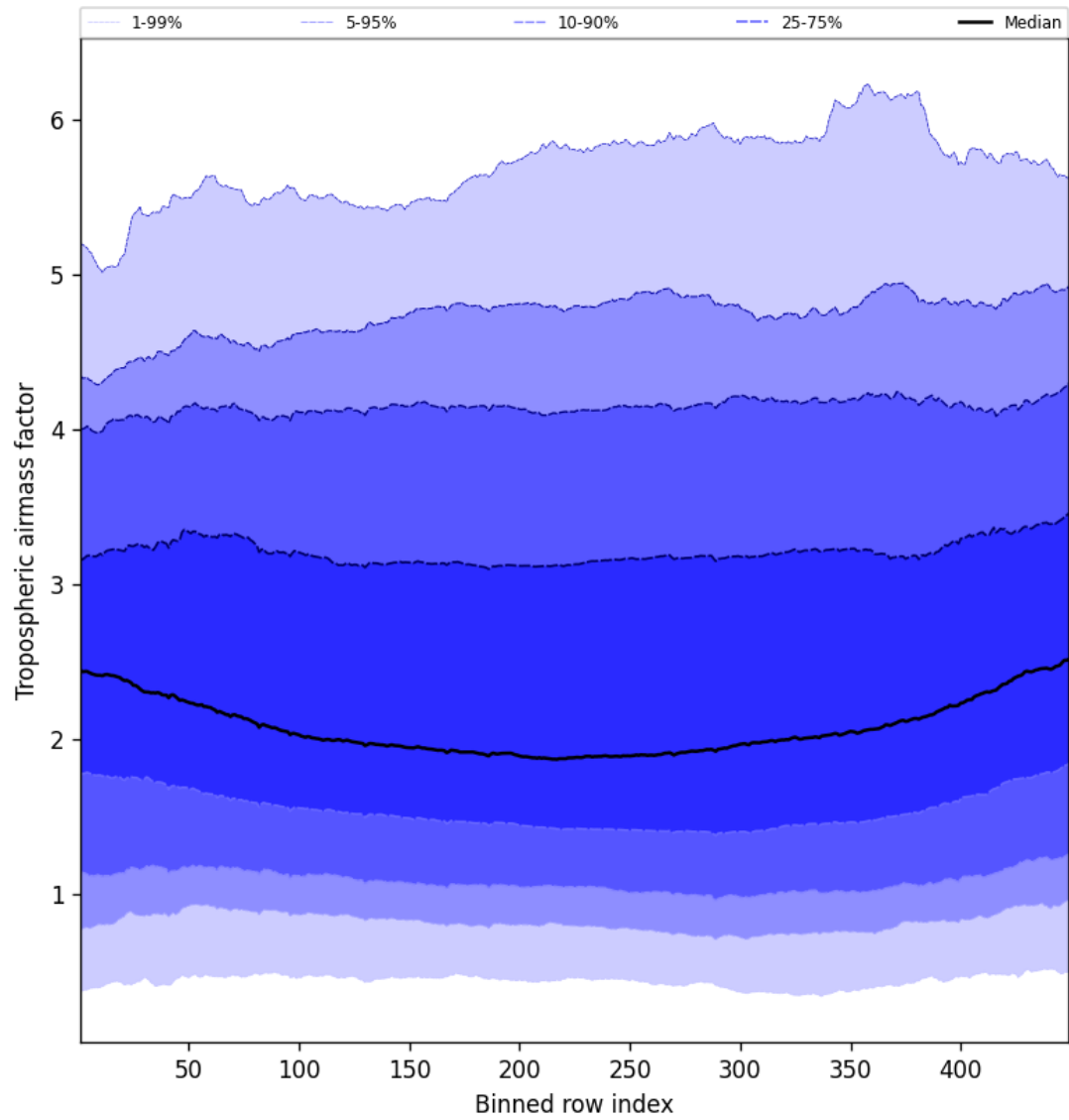
Figure 46: Along track statistics of “Tropospheric airmass factor” for 2025-05-13 to 2025-05-13
