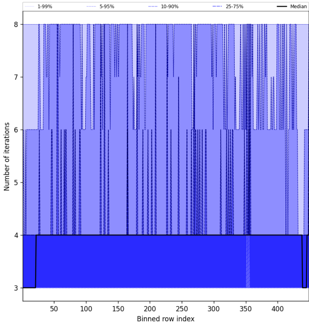
Figure 49: Along track statistics of “Number of iterations” for 2025-05-13 to 2025-05-13
