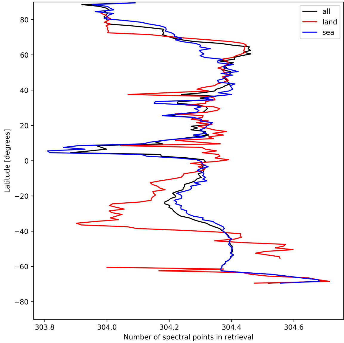
Figure 14: Zonal average of “Number of spectral points in retrieval” for 2025-05-13 to 2025-05-13.
