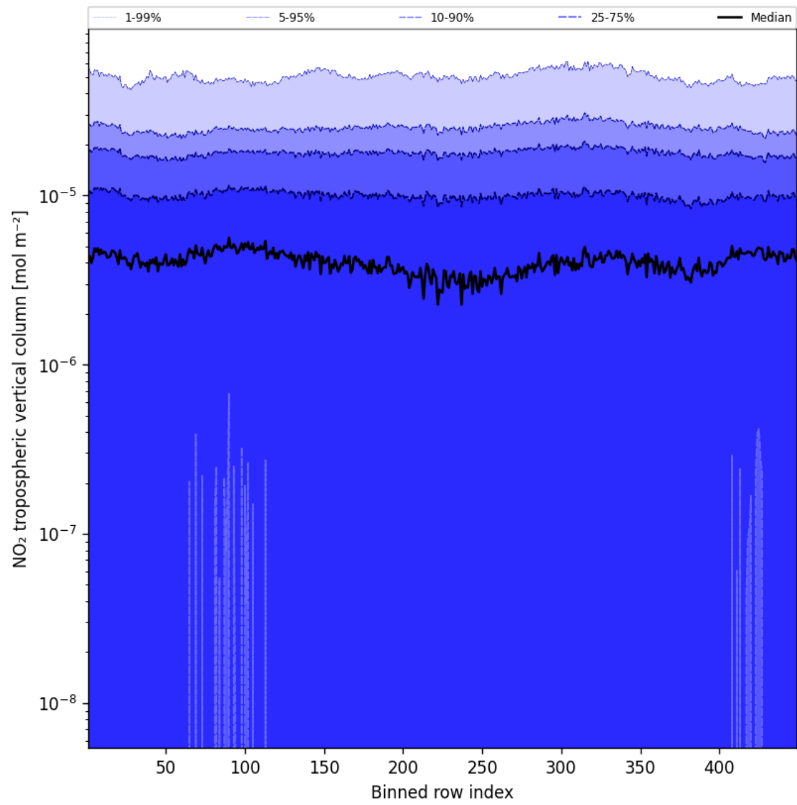
Figure 44: Along track statistics of “NO 2 tropospheric vertical column” for 2025-05-13 to 2025-05-13
