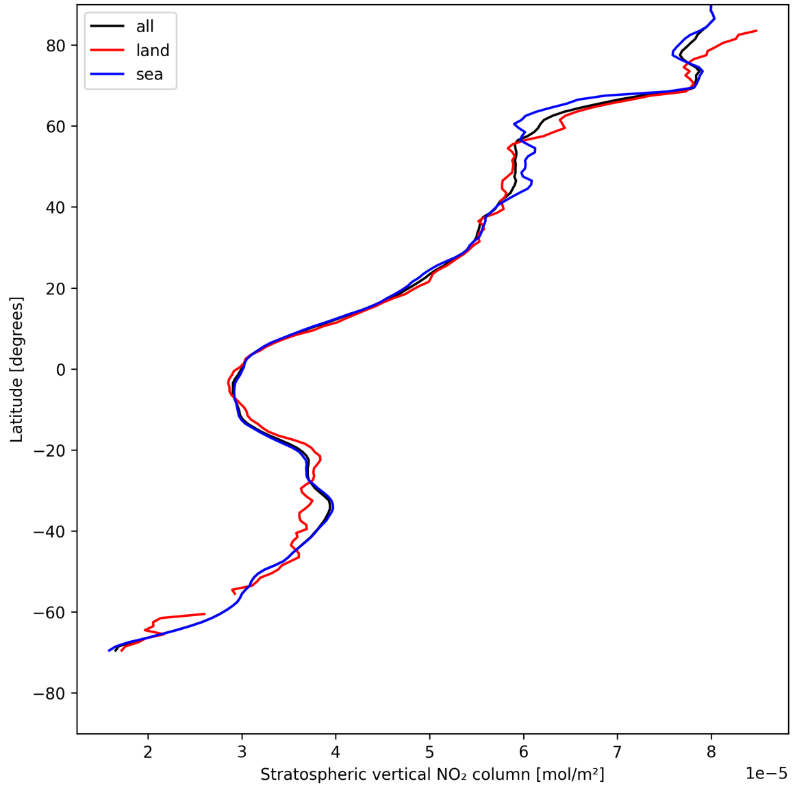
Figure 17: Zonal average of “Stratospheric vertical NO 2 column” for 2025-05-13 to 2025-05-13.
