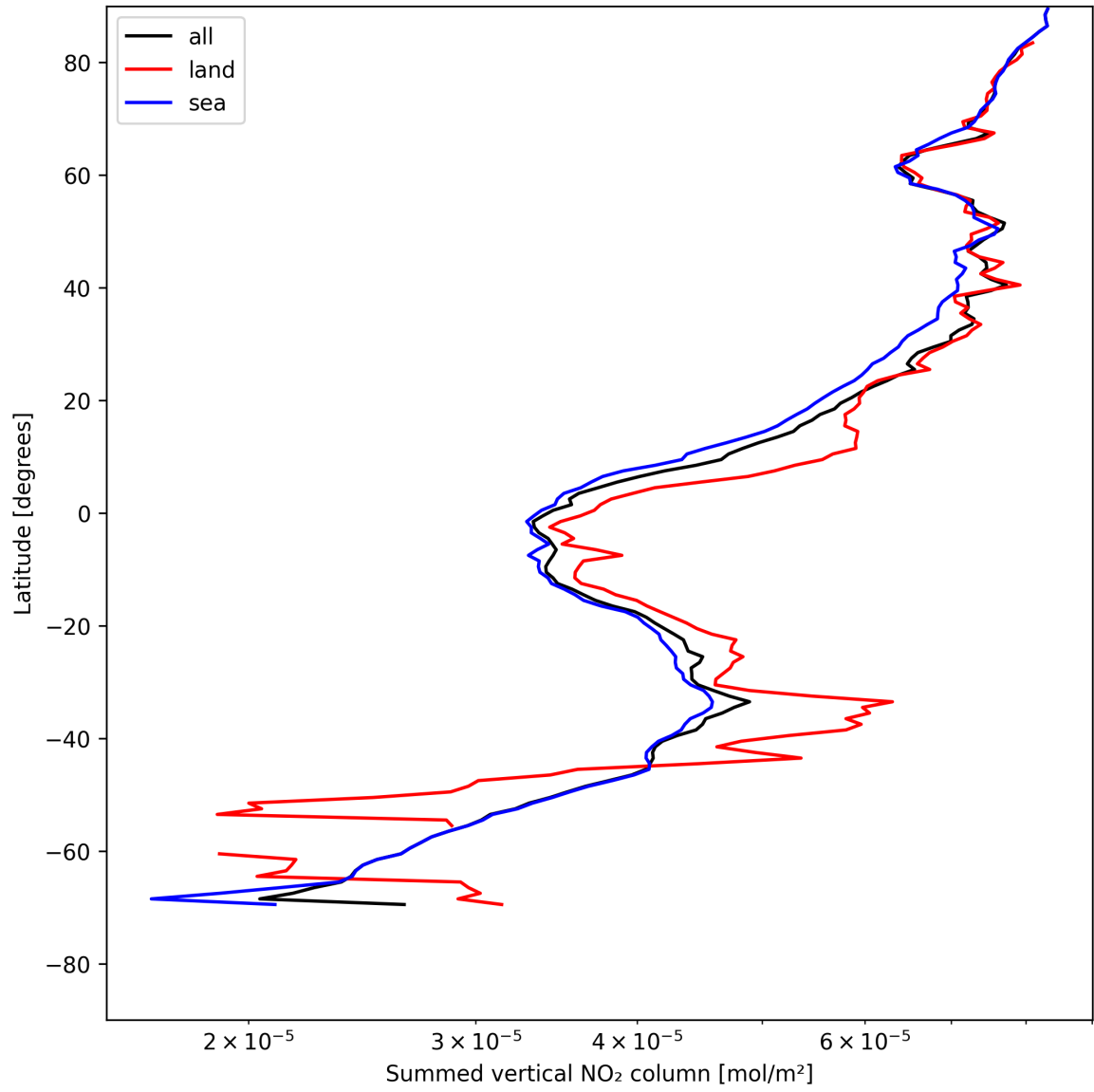
Figure 21: Zonal average of “Summed vertical NO 2 column” for 2025-05-13 to 2025-05-13.
