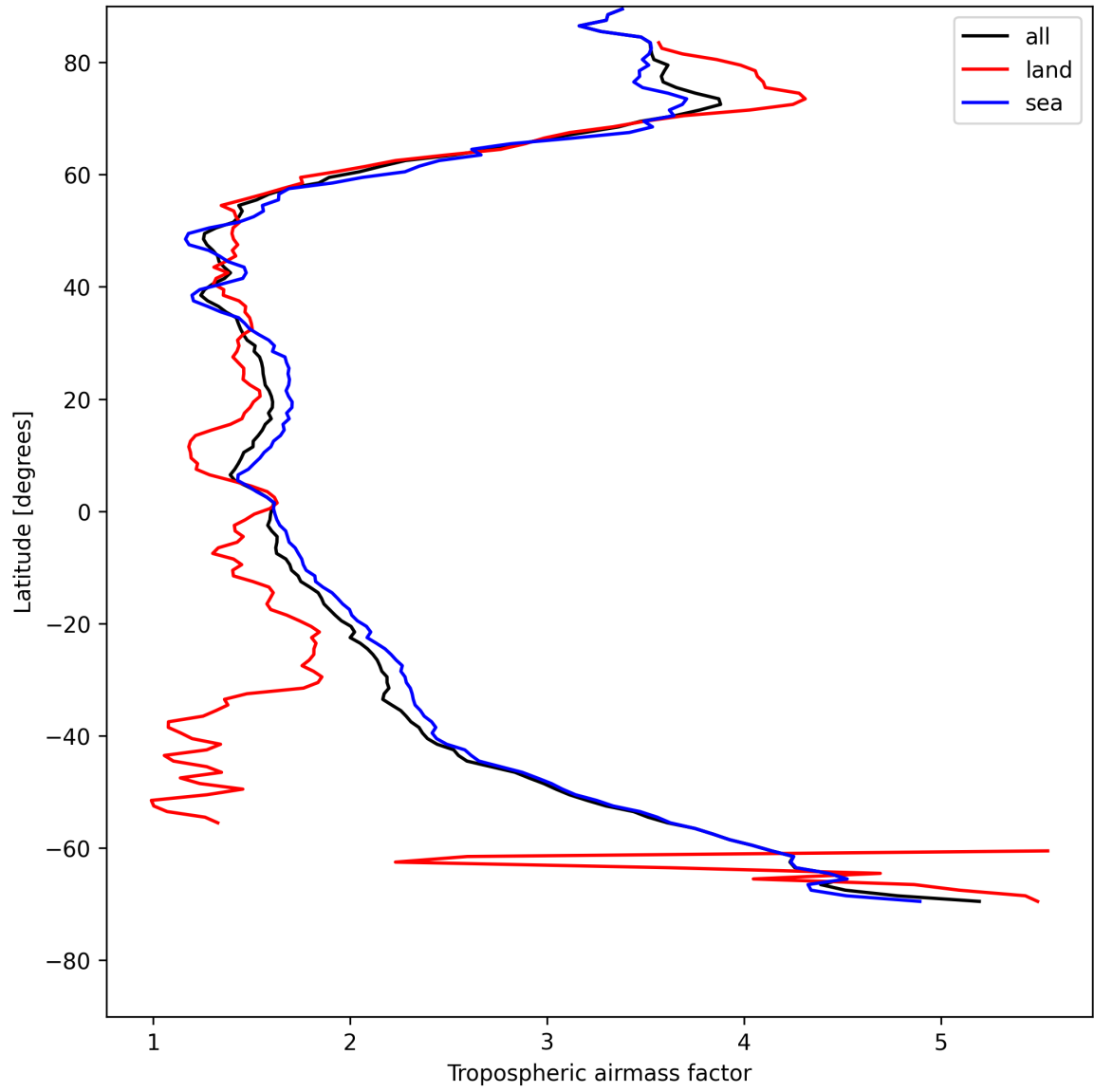
Figure 12: Zonal average of “Tropospheric airmass factor” for 2025-05-13 to 2025-05-13.
