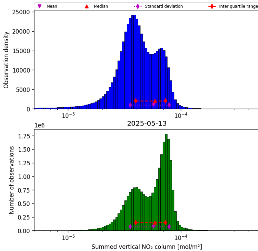
Figure 38: Histogram of “Summed vertical NO 2 column” for 2025-05-13 to 2025-05-13
