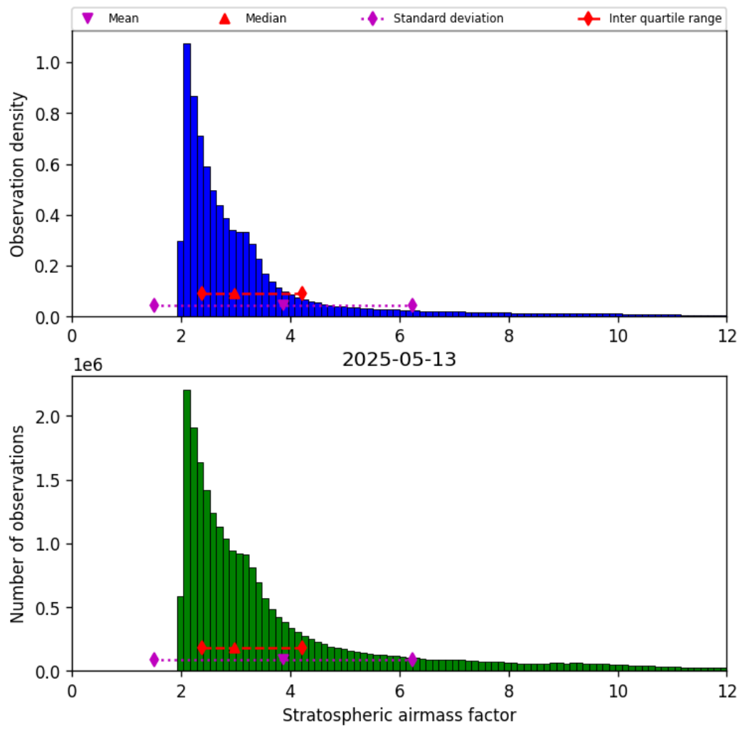
Figure 42: Histogram of “Stratospheric airmass factor” for 2025-05-13 to 2025-05-13
