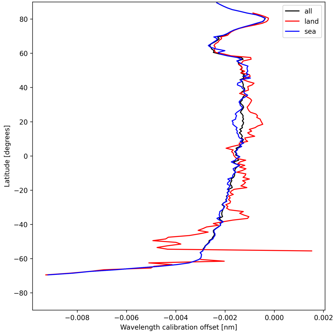
Figure 16: Zonal average of “Wavelength calibration offset” for 2025-05-13 to 2025-05-13.
