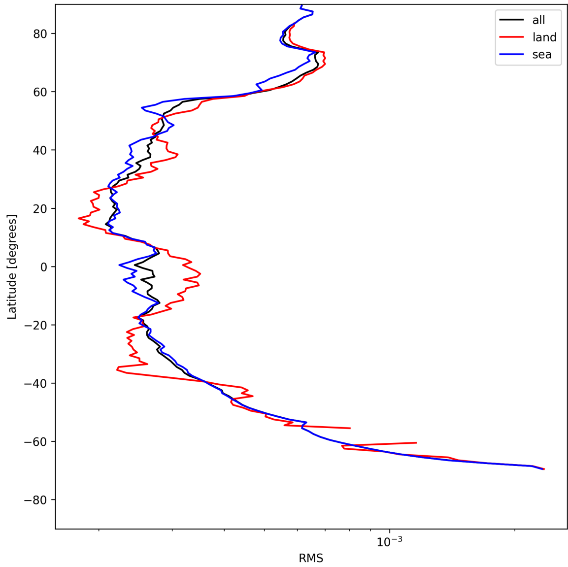
Figure 24: Zonal average of “RMS” for 2025-05-13 to 2025-05-13.
