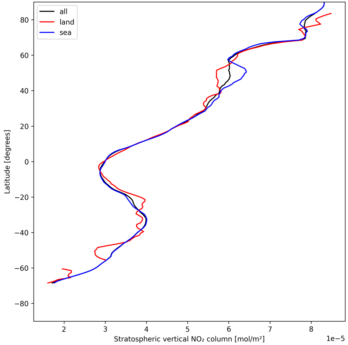
Figure 17: Zonal average of “Stratospheric vertical NO 2 column” for 2025-05-14 to 2025-05-15.
