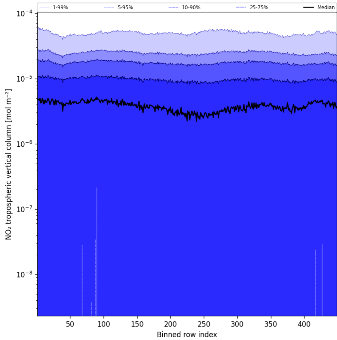
Figure 44: Along track statistics of “NO 2 tropospheric vertical column” for 2025-05-14 to 2025-05-15
