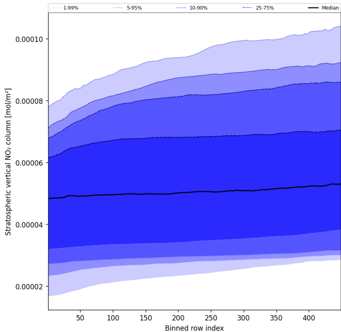
Figure 51: Along track statistics of “Stratospheric vertical NO 2 column” for 2025-05-14 to 2025-05-15
