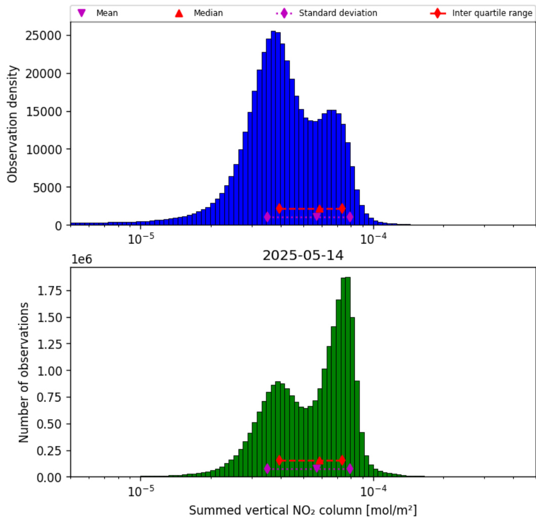
Figure 38: Histogram of “Summed vertical NO 2 column” for 2025-05-14 to 2025-05-15
