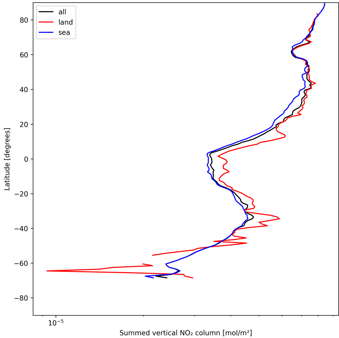
Figure 21: Zonal average of “Summed vertical NO 2 column” for 2025-05-14 to 2025-05-15.
