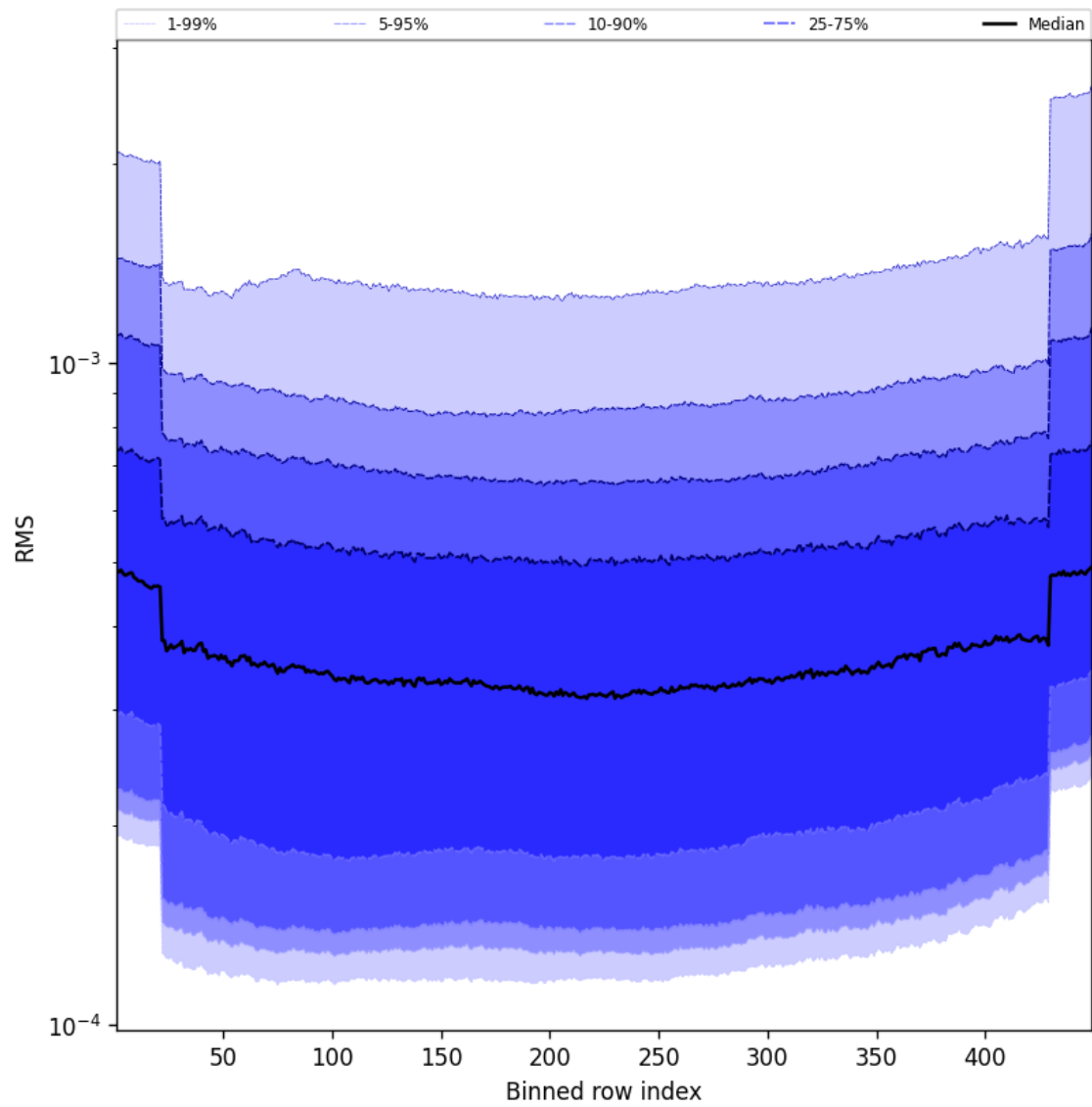
Figure 58: Along track statistics of “RMS” for 2025-05-14 to 2025-05-15
