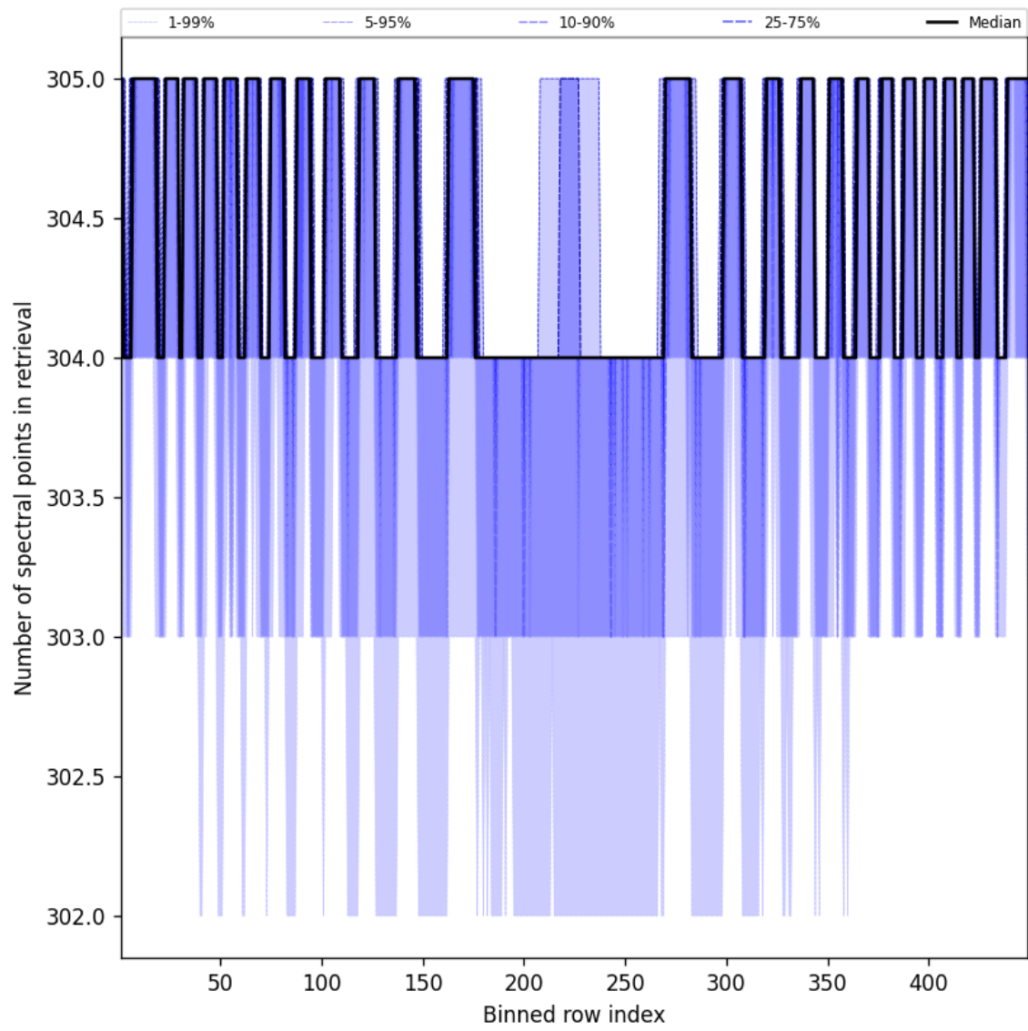
Figure 48: Along track statistics of “Number of spectral points in retrieval” for 2025-05-14 to 2025-05-15
