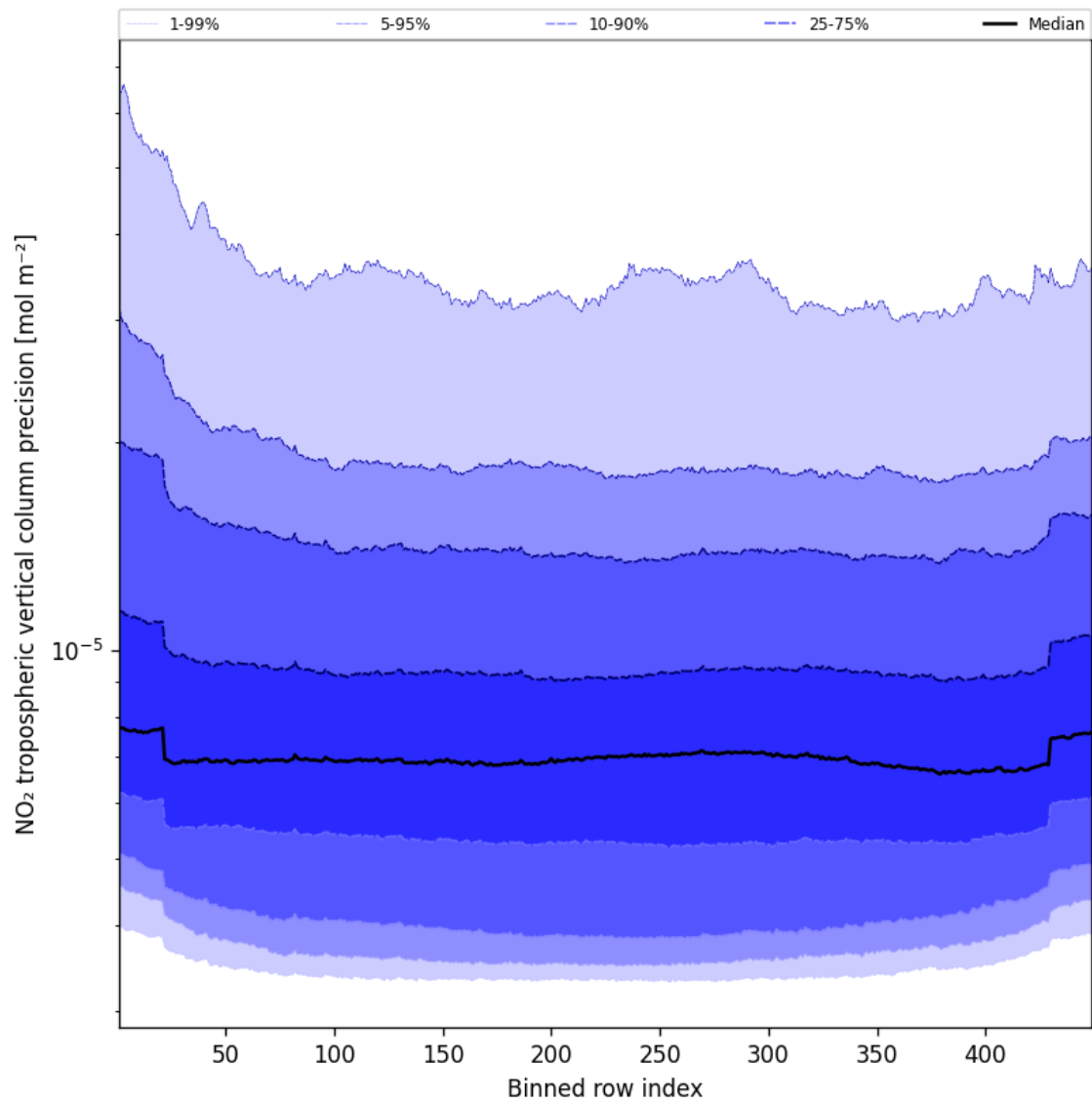
Figure 45: Along track statistics of “NO 2 tropospheric vertical column precision” for 2025-05-14 to 2025-05-15
