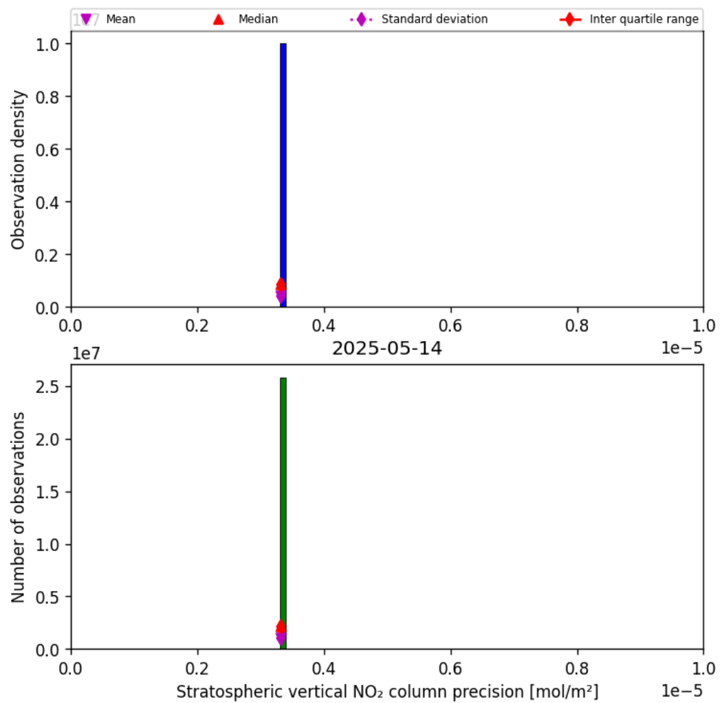
Figure 35: Histogram of “Stratospheric vertical NO 2 column precision” for 2025-05-14 to 2025-05-15
