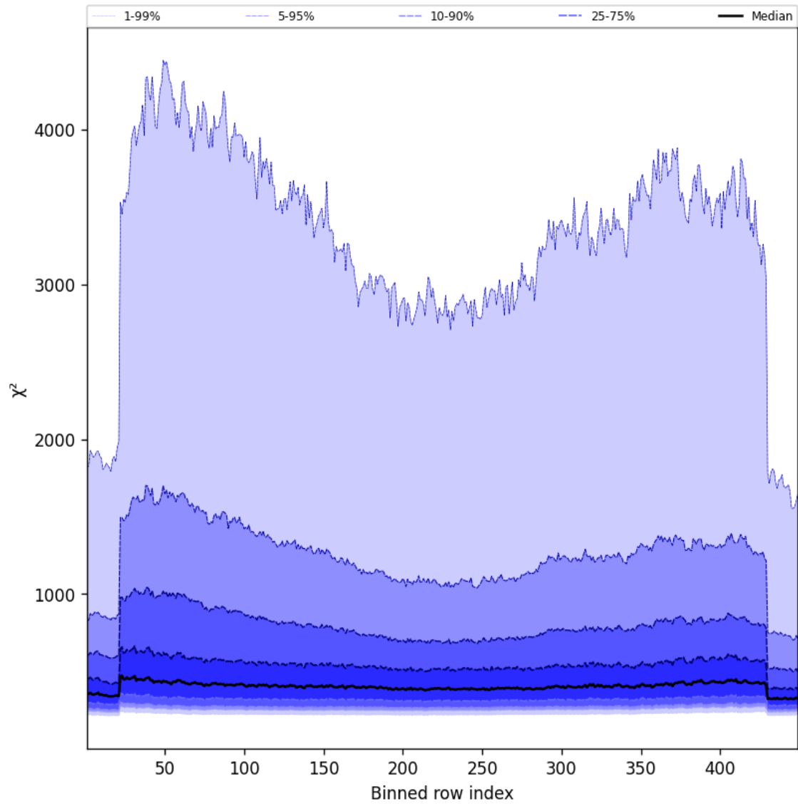
Figure 57: Along track statistics of “ \chi^2 ” for 2025-05-14 to 2025-05-15
