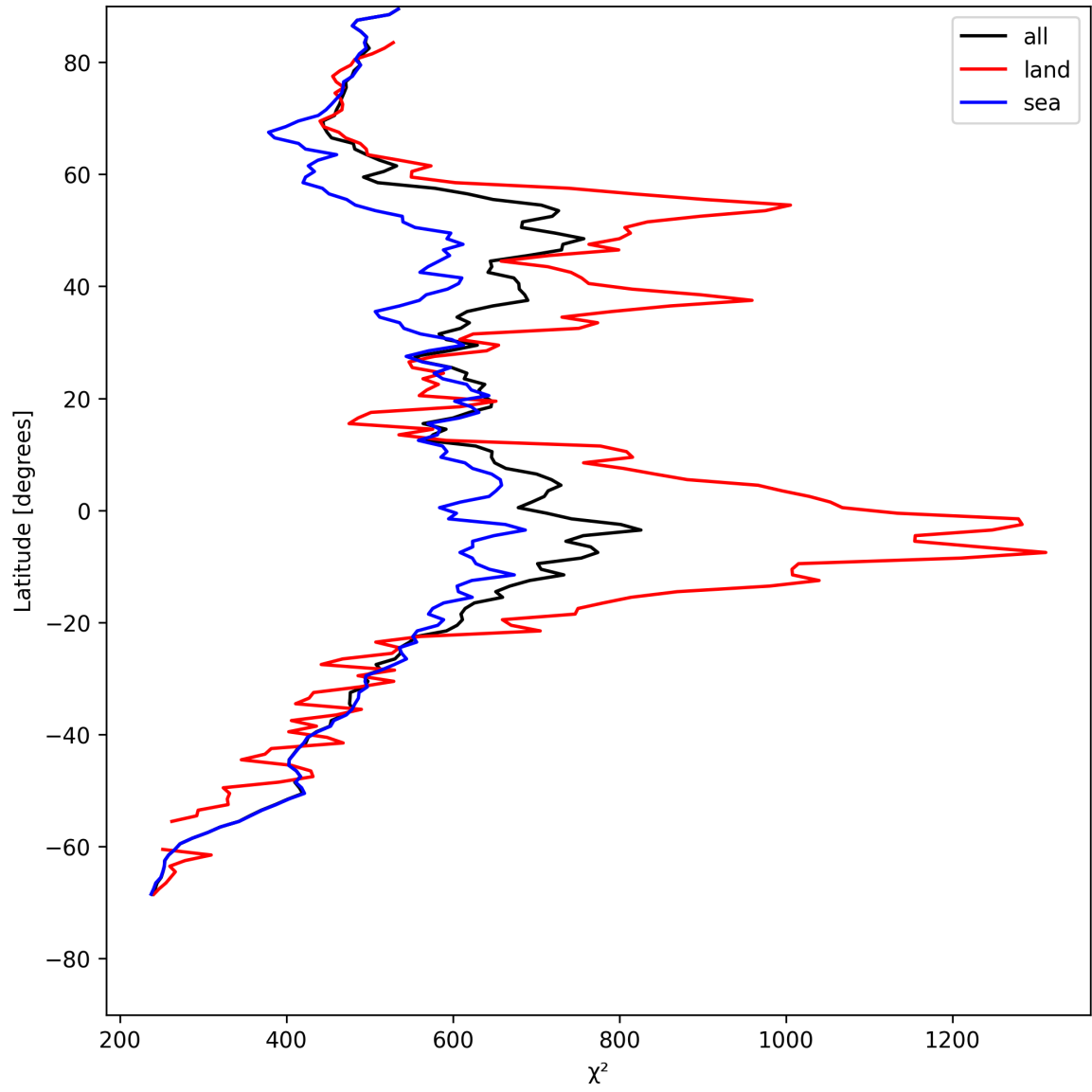
Figure 23: Zonal average of “ \chi^2 ” for 2025-05-14 to 2025-05-15.
