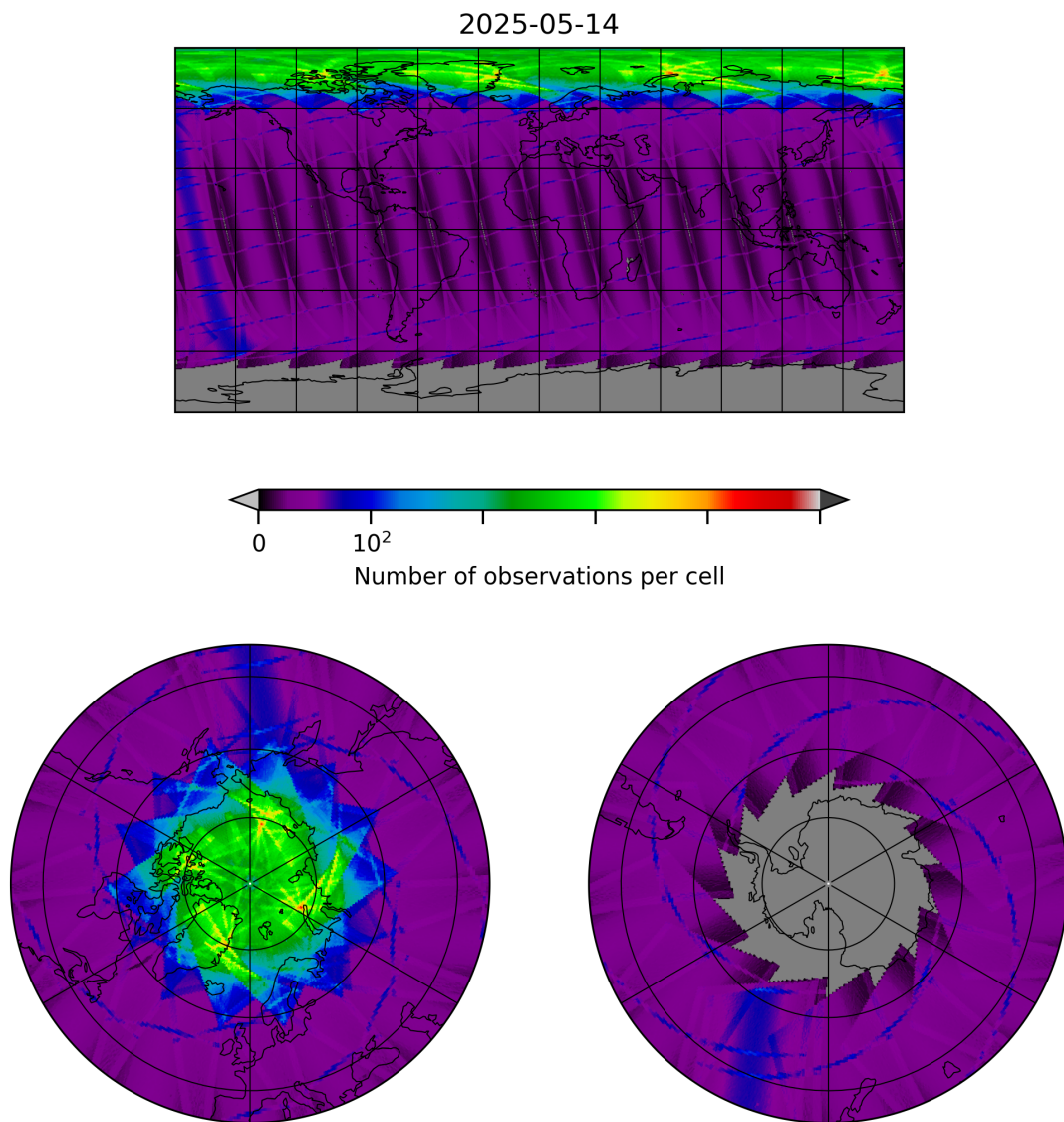
Figure 8: Map of the number of observations for 2025-05-14 to 2025-05-15
