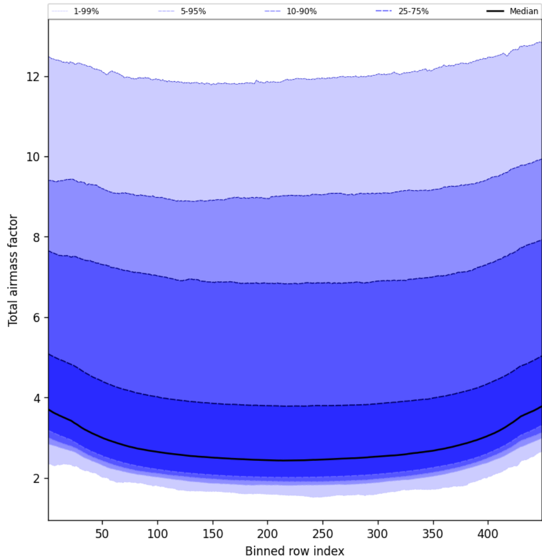
Figure 47: Along track statistics of “Total airmass factor” for 2025-05-14 to 2025-05-15
