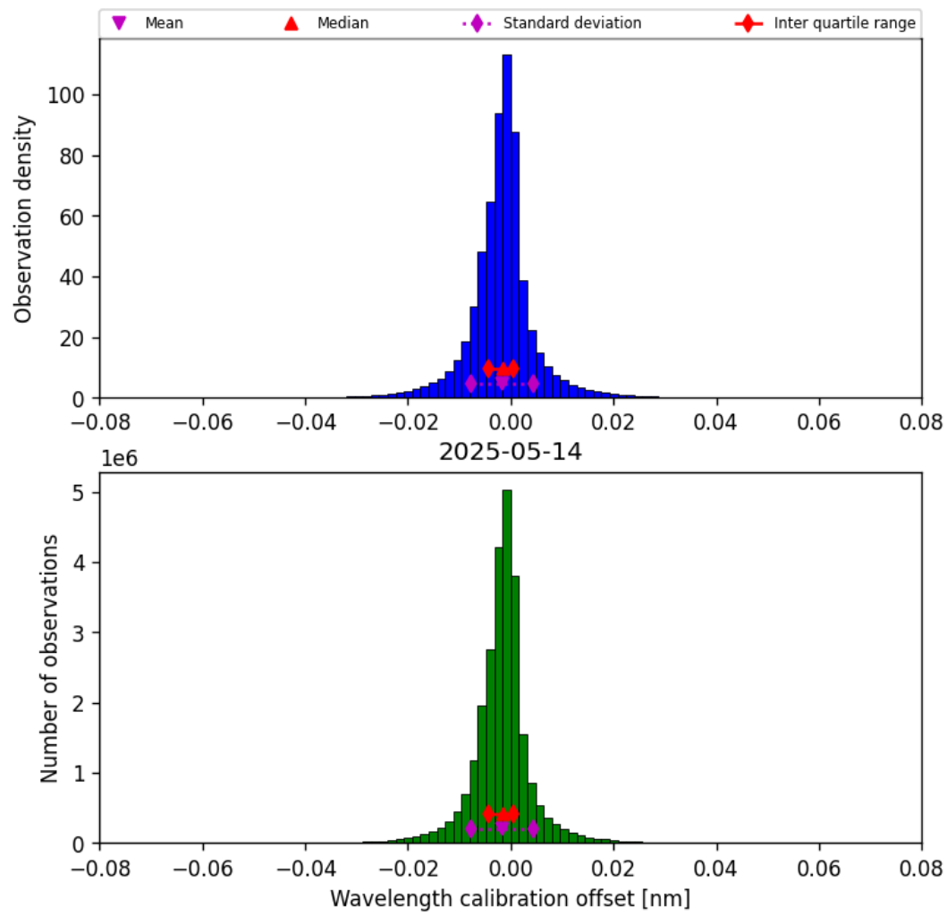
Figure 33: Histogram of “Wavelength calibration offset” for 2025-05-14 to 2025-05-15
