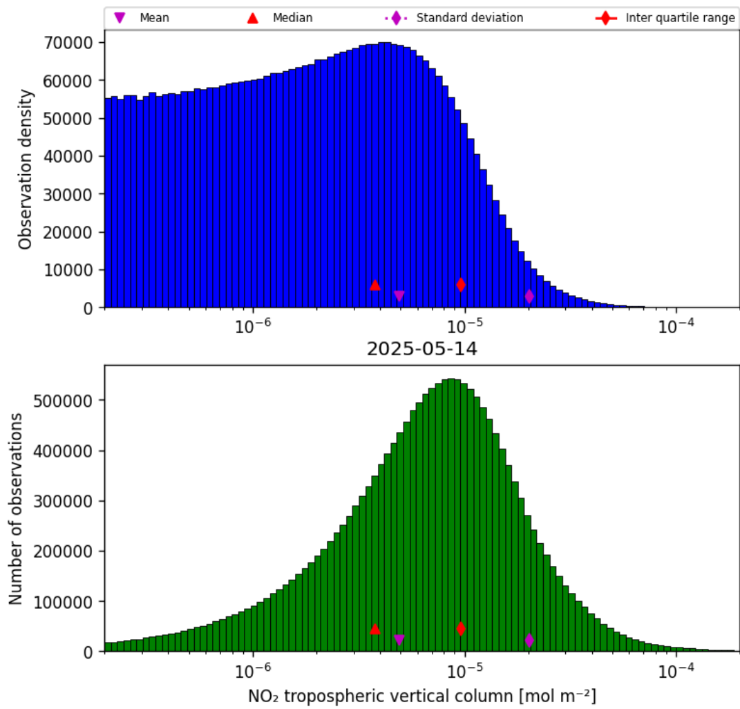
Figure 27: Histogram of “NO 2 tropospheric vertical column” for 2025-05-14 to 2025-05-15
