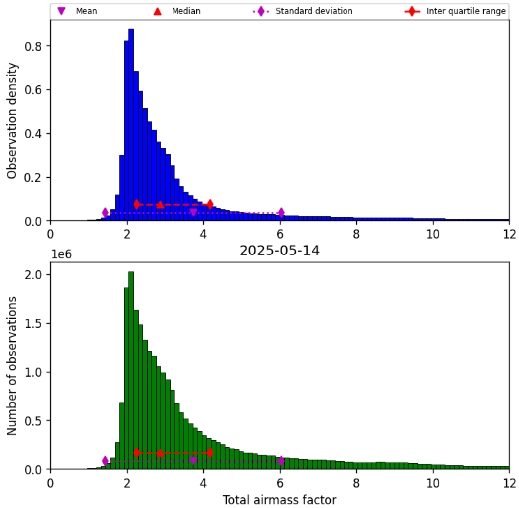
Figure 30: Histogram of “Total airmass factor” for 2025-05-14 to 2025-05-15
