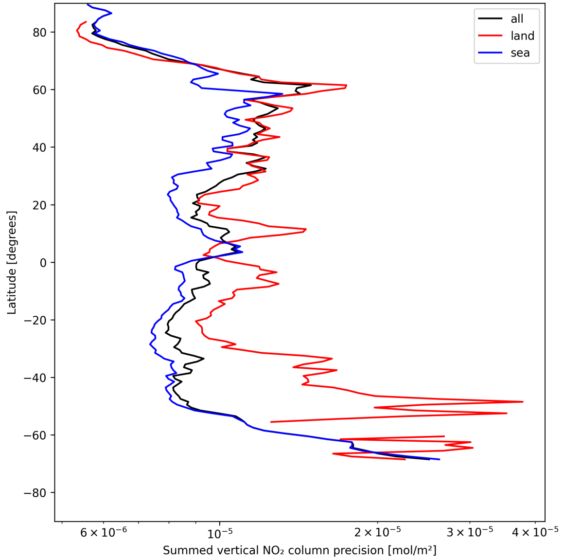
Figure 22: Zonal average of “Summed vertical NO 2 column precision” for 2025-05-14 to 2025-05-15.
