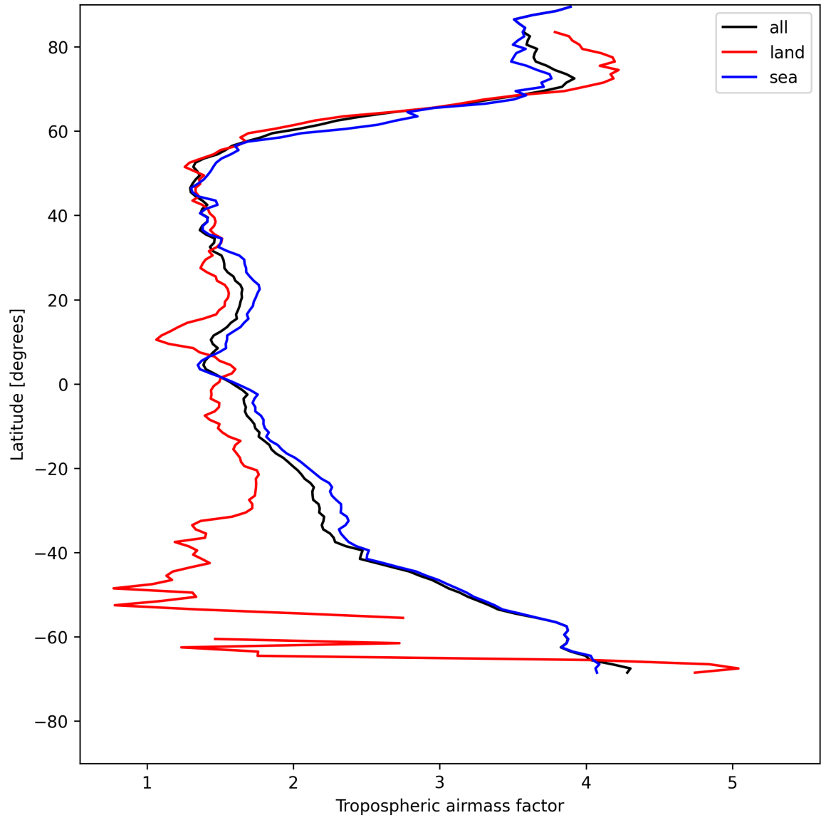
Figure 12: Zonal average of “Tropospheric airmass factor” for 2025-05-14 to 2025-05-15.
