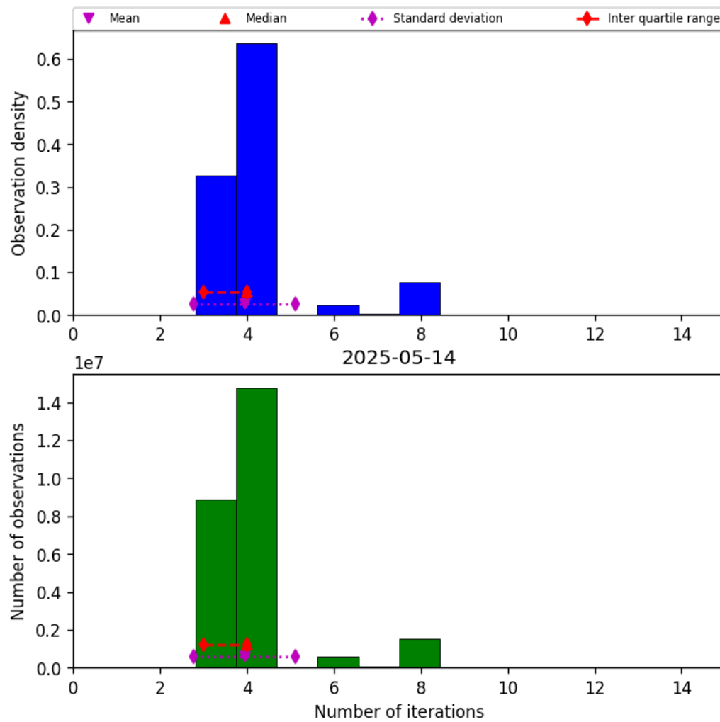
Figure 32: Histogram of “Number of iterations” for 2025-05-14 to 2025-05-15
