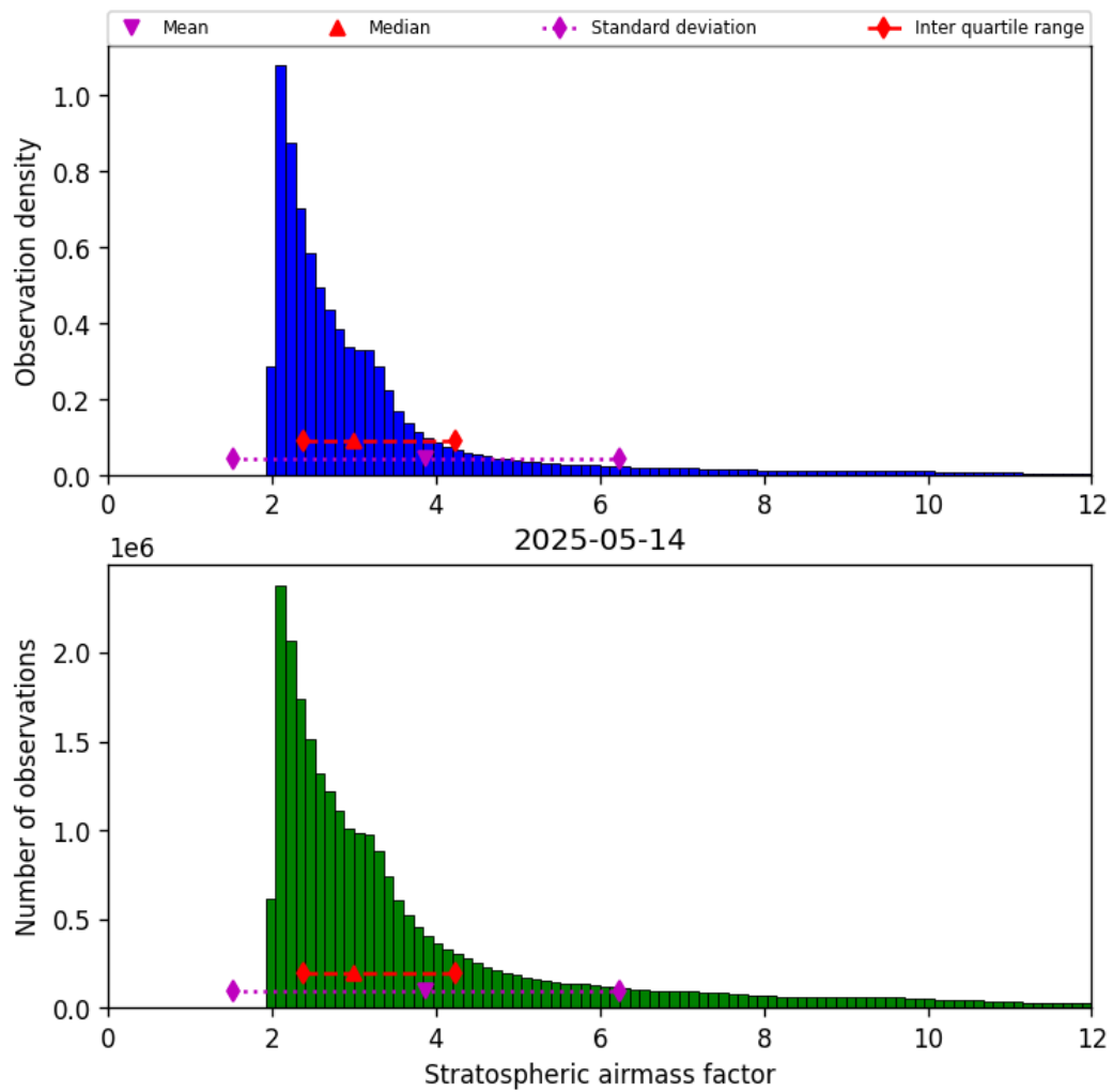
Figure 42: Histogram of “Stratospheric airmass factor” for 2025-05-14 to 2025-05-15
