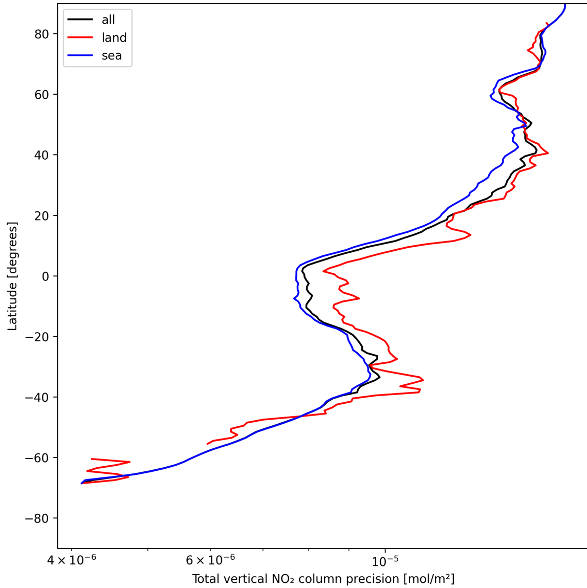
Figure 20: Zonal average of “Total vertical NO 2 column precision” for 2025-05-14 to 2025-05-15.
