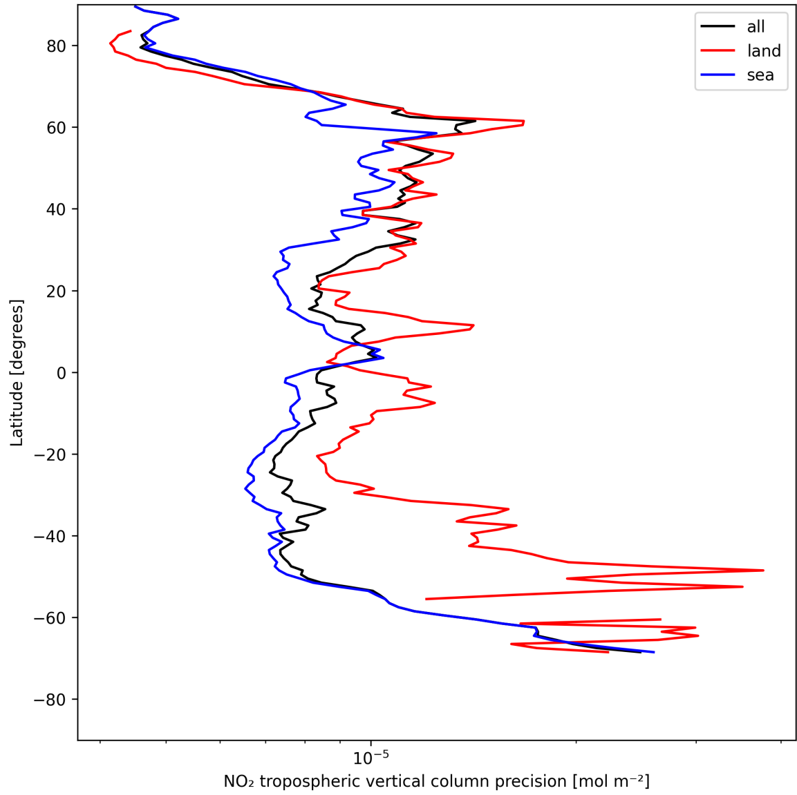
Figure 11: Zonal average of “NO 2 tropospheric vertical column precision” for 2025-05-14 to 2025-05-15.
