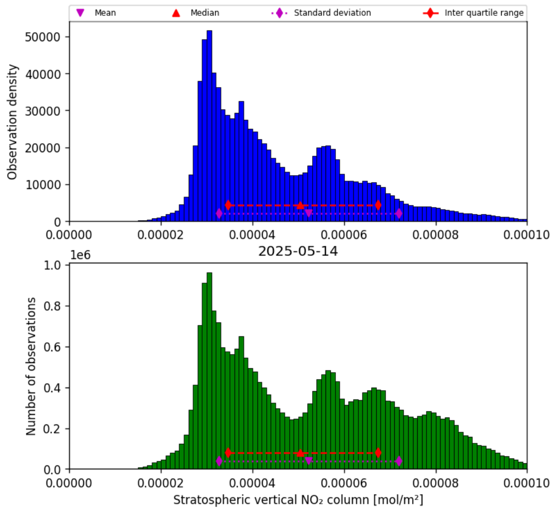
Figure 34: Histogram of “Stratospheric vertical NO 2 column” for 2025-05-14 to 2025-05-15
