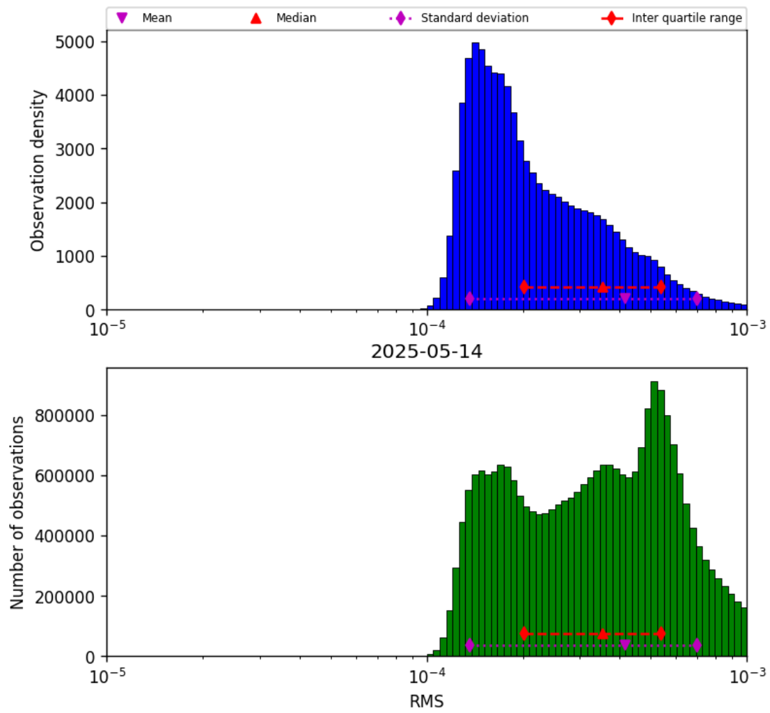
Figure 41: Histogram of “RMS” for 2025-05-14 to 2025-05-15
