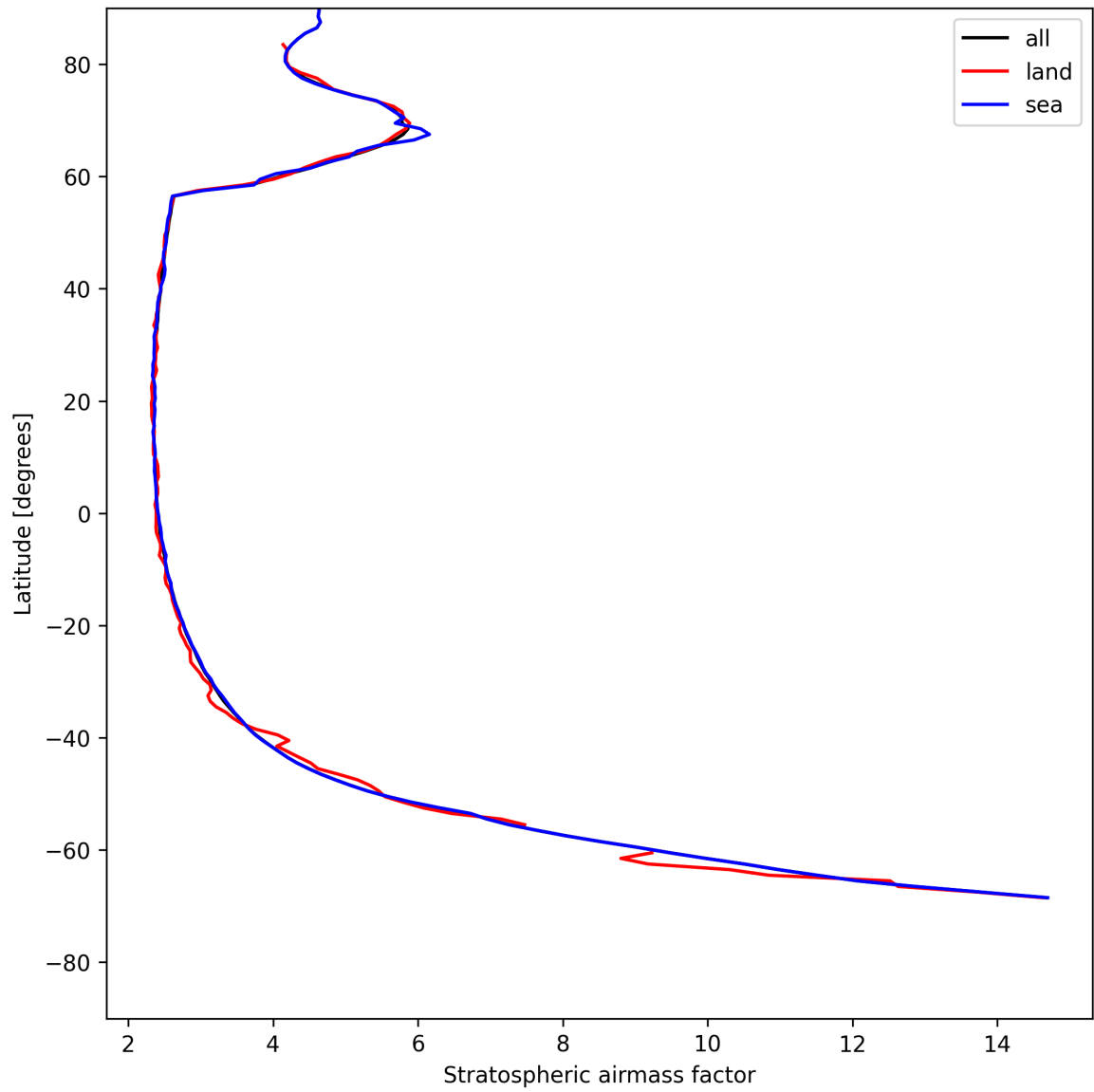
Figure 25: Zonal average of “Stratospheric air mass factor” for 2025-05-14 to 2025-05-15.
