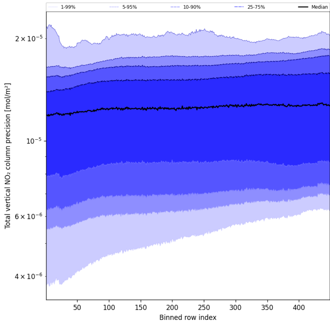
Figure 54: Along track statistics of “Total vertical NO 2 column precision” for 2025-05-14 to 2025-05-15
