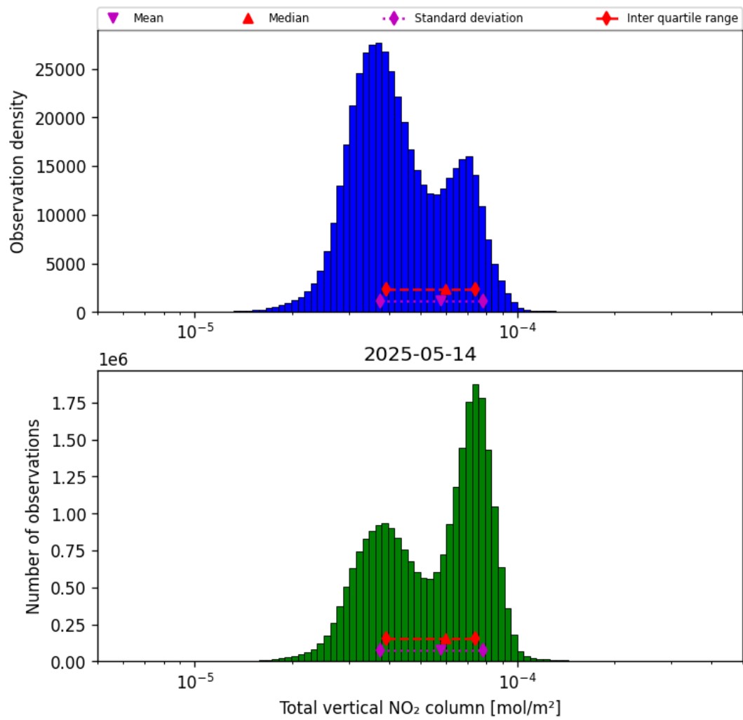
Figure 36: Histogram of “Total vertical NO 2 column” for 2025-05-14 to 2025-05-15
