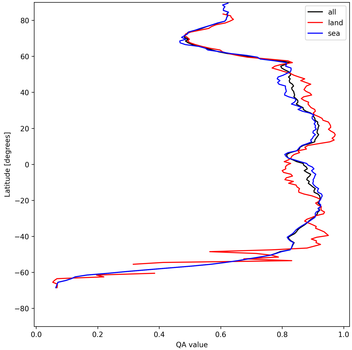
Figure 9: Zonal average of “QA value” for 2025-05-14 to 2025-05-15.
