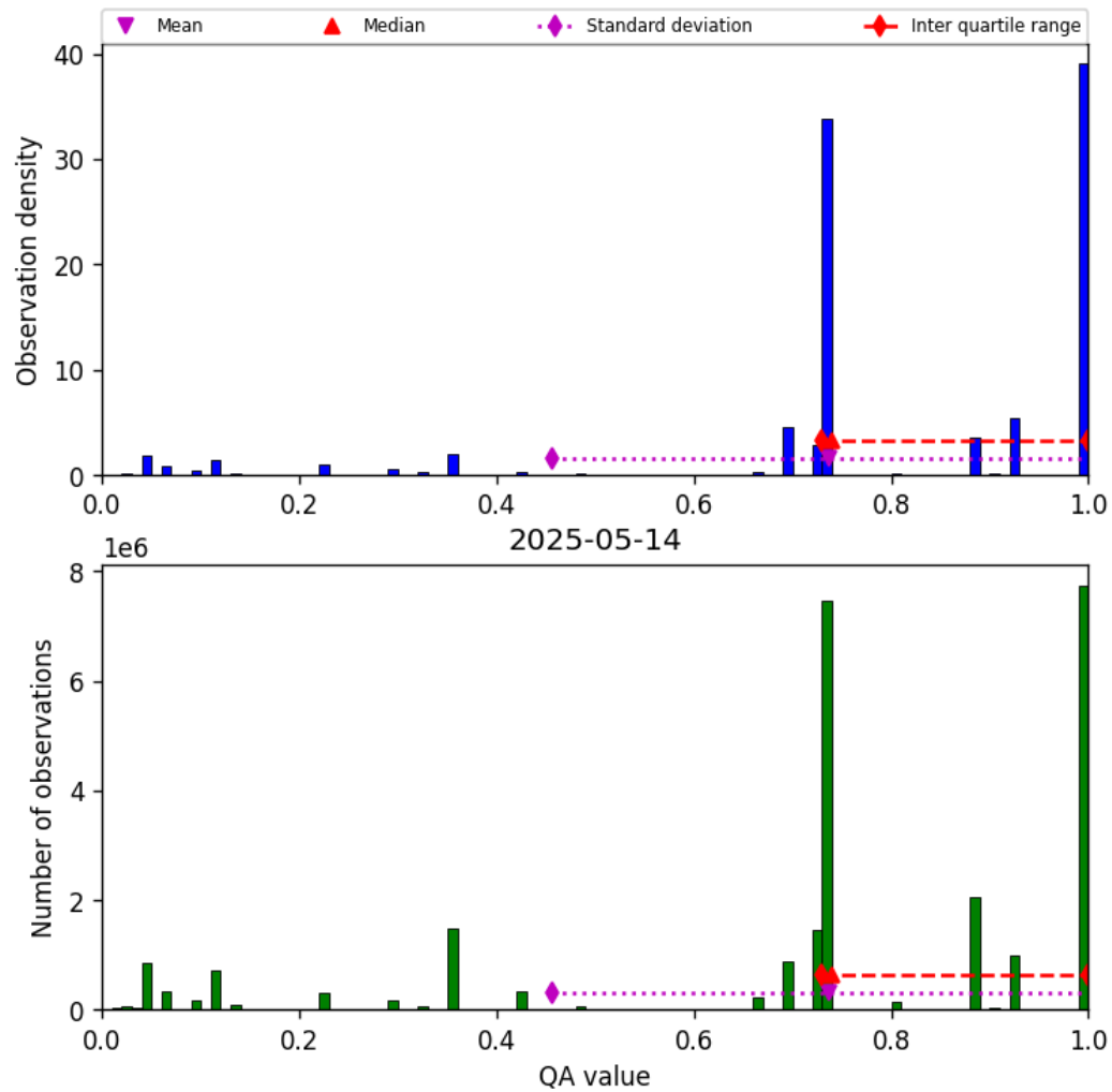
Figure 26: Histogram of “QA value” for 2025-05-14 to 2025-05-15
