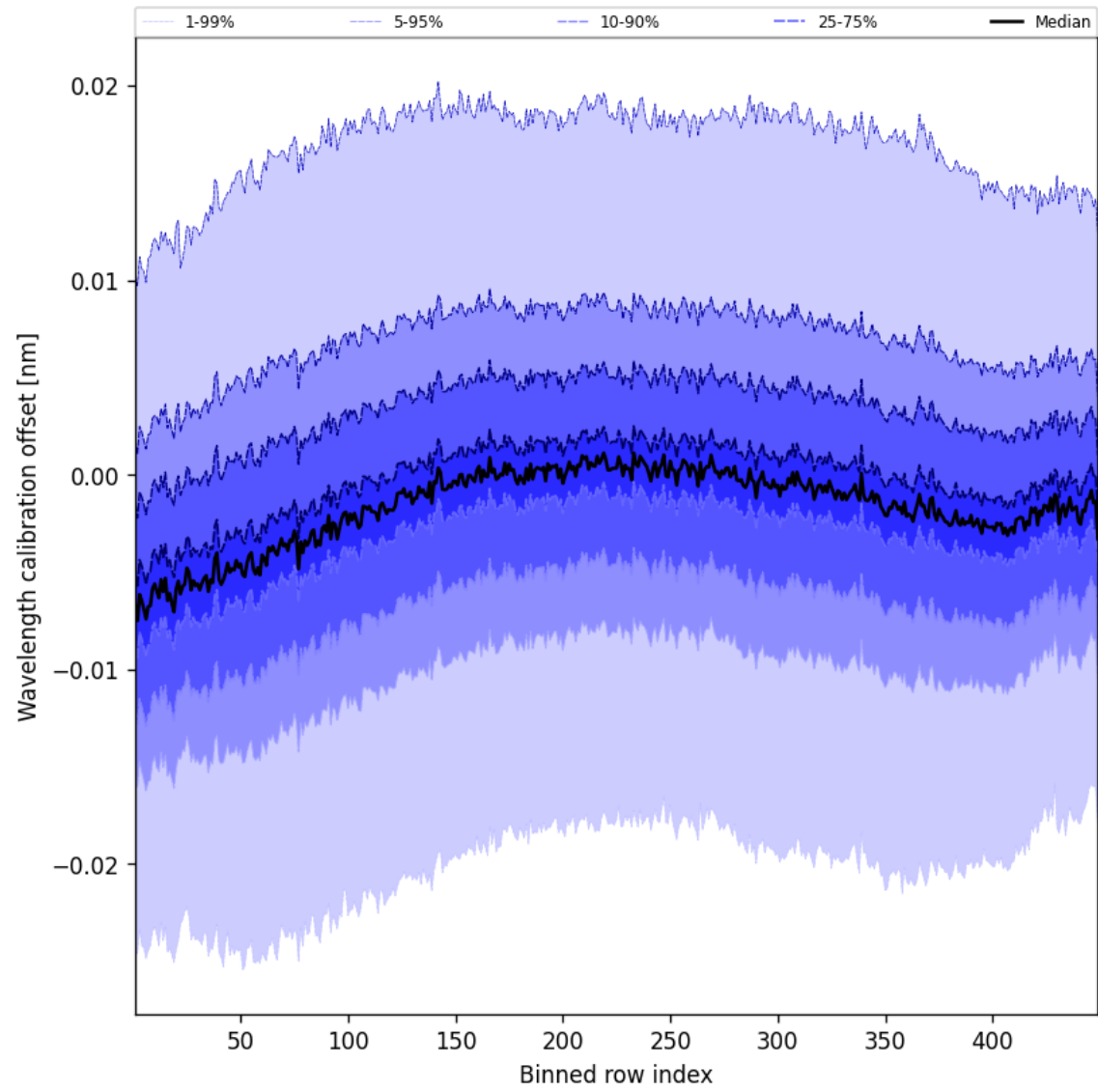
Figure 50: Along track statistics of “Wavelength calibration offset” for 2025-05-14 to 2025-05-15
