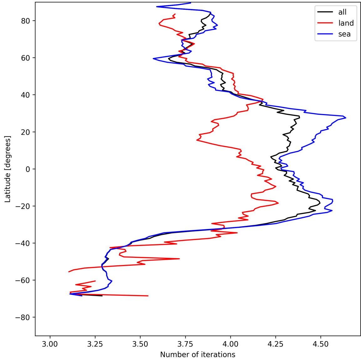
Figure 15: Zonal average of “Number of iterations” for 2025-05-14 to 2025-05-15.
