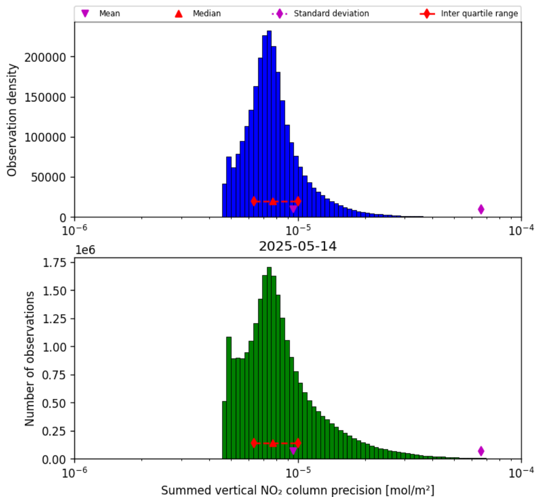
Figure 39: Histogram of “Summed vertical NO 2 column precision” for 2025-05-14 to 2025-05-15
