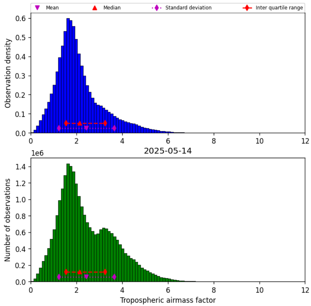
Figure 29: Histogram of “Tropospheric airmass factor” for 2025-05-14 to 2025-05-15
