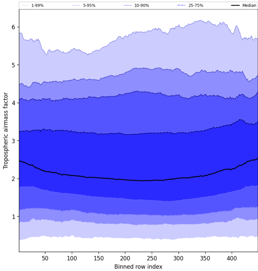
Figure 46: Along track statistics of “Tropospheric airmass factor” for 2025-05-14 to 2025-05-15
