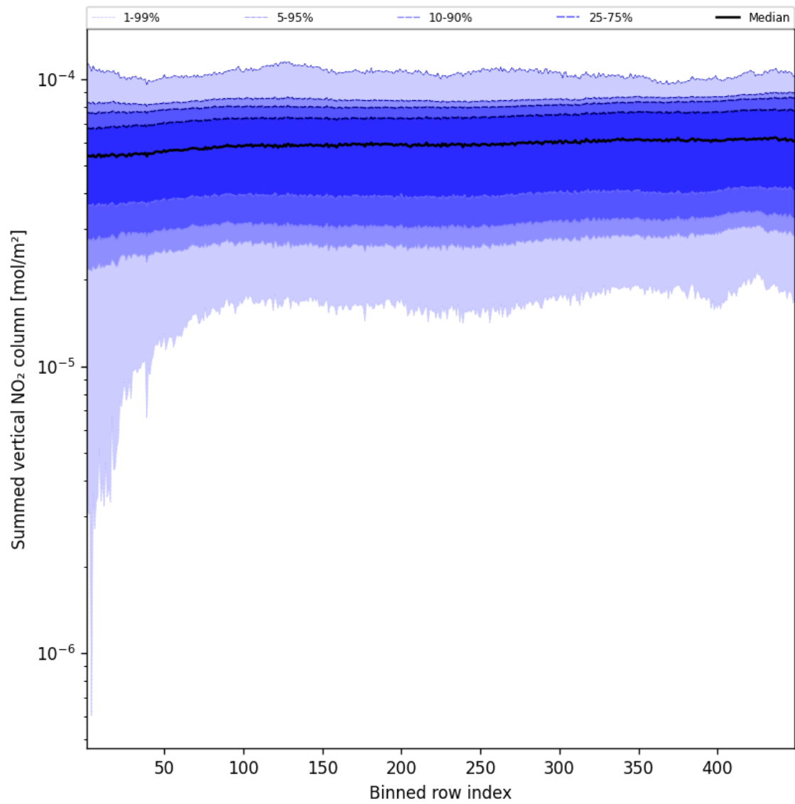
Figure 55: Along track statistics of “Summed vertical NO 2 column” for 2025-05-14 to 2025-05-15
