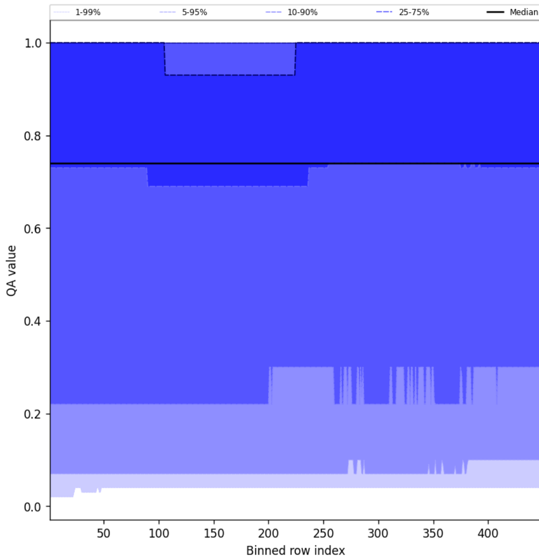
Figure 43: Along track statistics of “QA value” for 2025-05-14 to 2025-05-15
