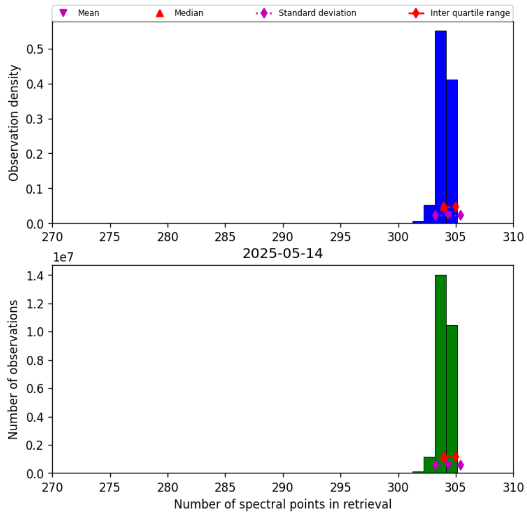
Figure 31: Histogram of “Number of spectral points in retrieval” for 2025-05-14 to 2025-05-15
