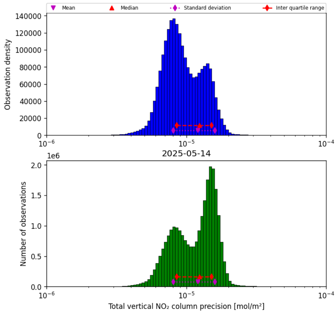
Figure 37: Histogram of “Total vertical NO 2 column precision” for 2025-05-14 to 2025-05-15
