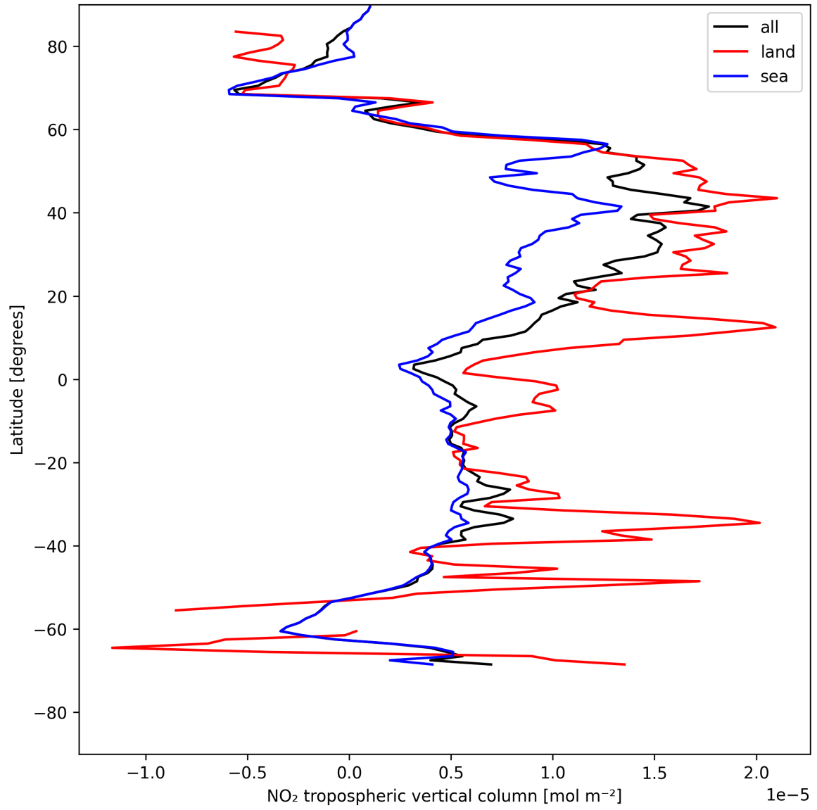
Figure 10: Zonal average of “NO 2 tropospheric vertical column” for 2025-05-14 to 2025-05-15.
