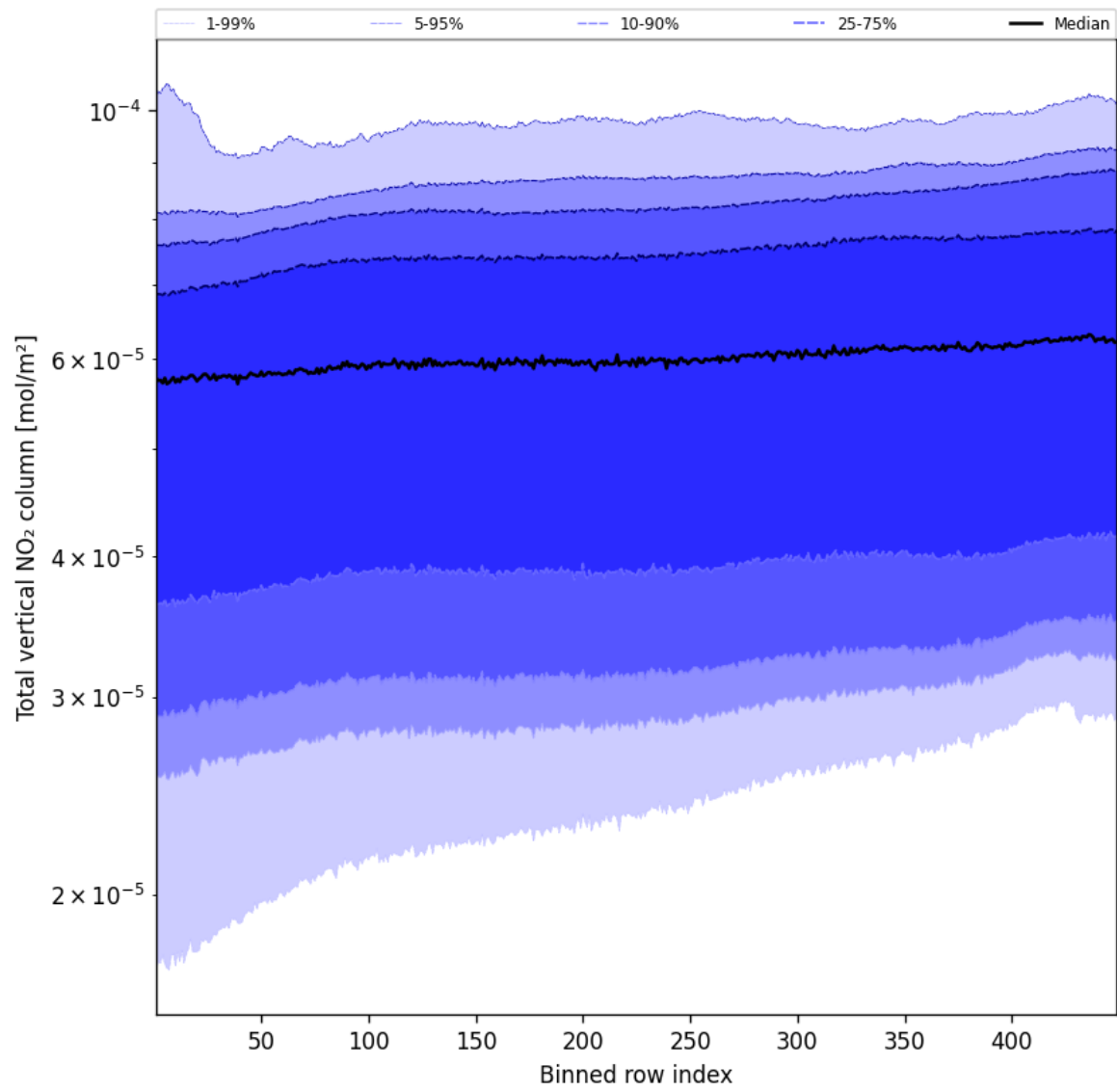
Figure 53: Along track statistics of “Total vertical NO 2 column” for 2025-05-14 to 2025-05-15
