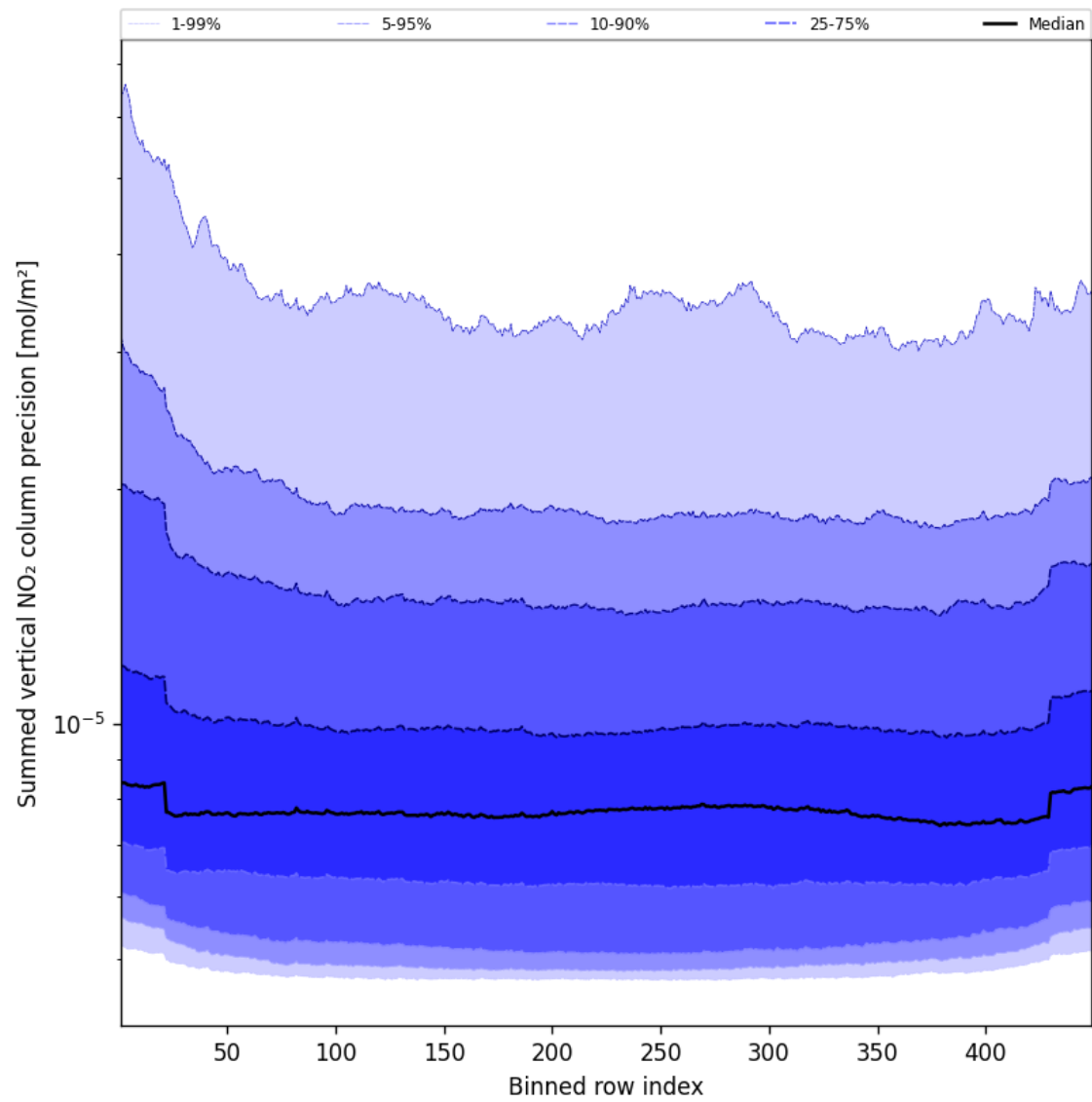
Figure 56: Along track statistics of “Summed vertical NO 2 column precision” for 2025-05-14 to 2025-05-15
