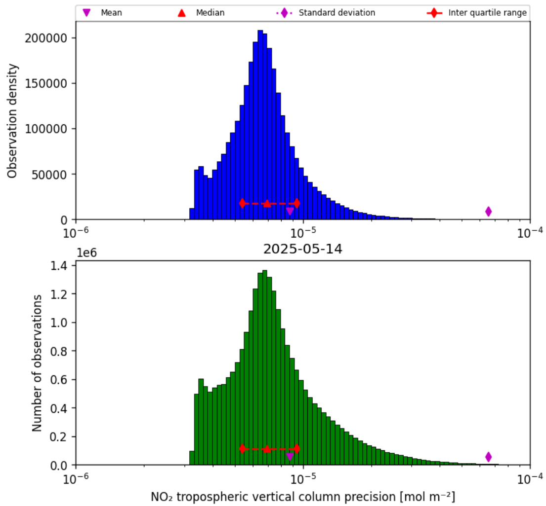
Figure 28: Histogram of “NO 2 tropospheric vertical column precision” for 2025-05-14 to 2025-05-15
