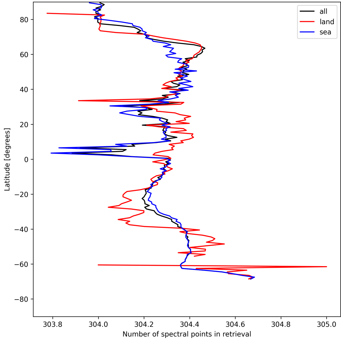
Figure 14: Zonal average of “Number of spectral points in retrieval” for 2025-05-14 to 2025-05-15.
