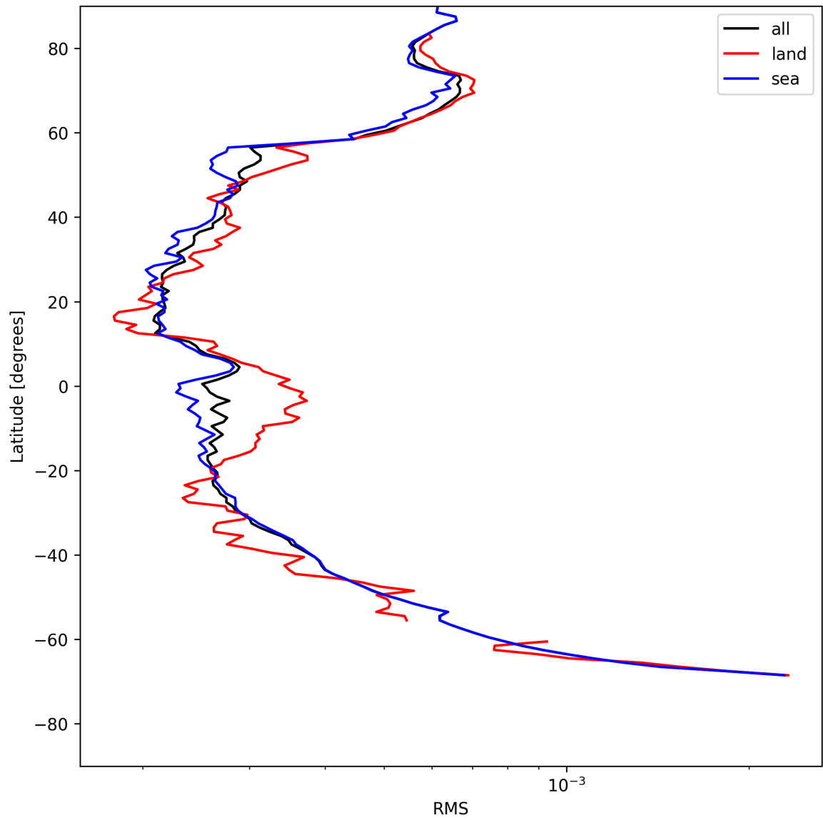
Figure 24: Zonal average of “RMS” for 2025-05-14 to 2025-05-15.
