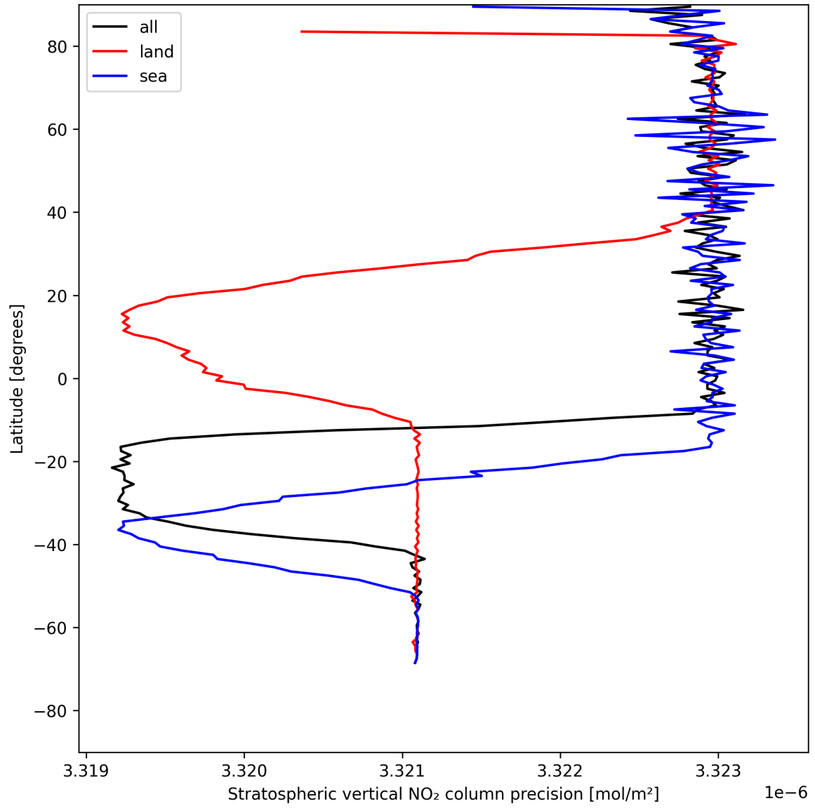
Figure 18: Zonal average of “Stratospheric vertical NO 2 column precision” for 2025-05-14 to 2025-05-15.
