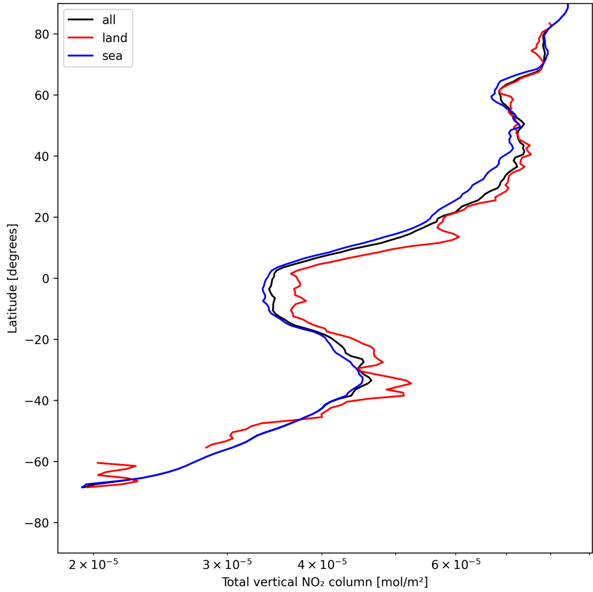
Figure 19: Zonal average of “Total vertical NO 2 column” for 2025-05-14 to 2025-05-15.
