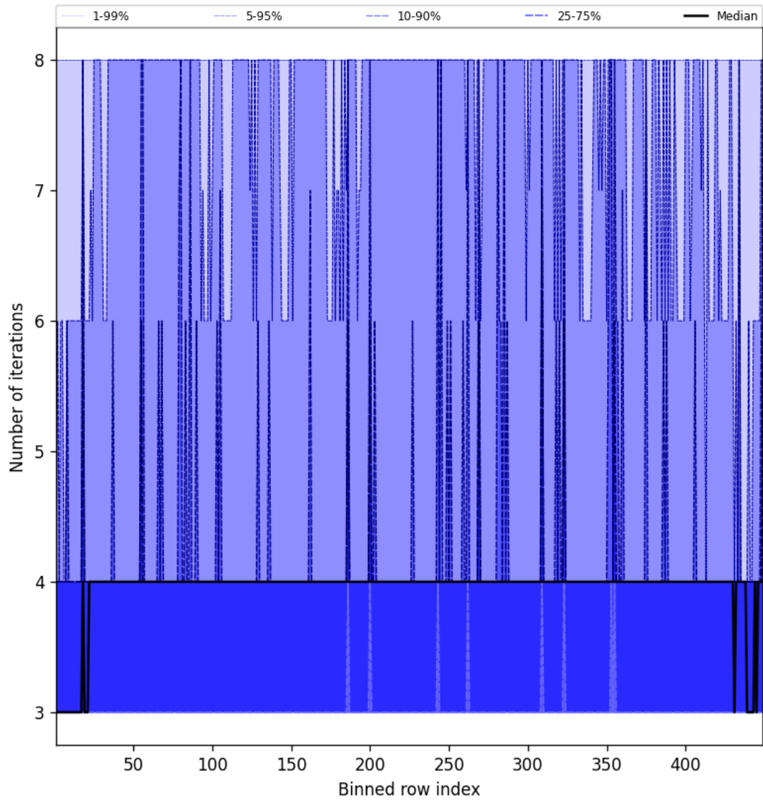
Figure 49: Along track statistics of “Number of iterations” for 2025-05-14 to 2025-05-15
