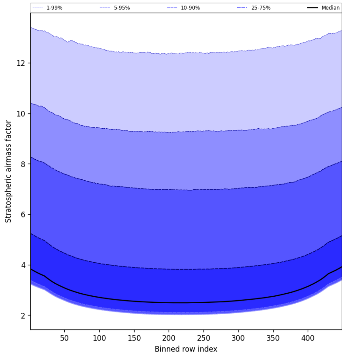
Figure 59: Along track statistics of “Stratospheric airmass factor” for 2025-05-14 to 2025-05-15
