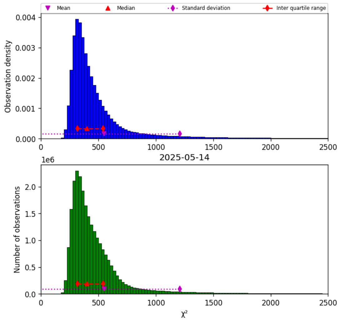
Figure 40: Histogram of “ \chi^2 ” for 2025-05-14 to 2025-05-15
