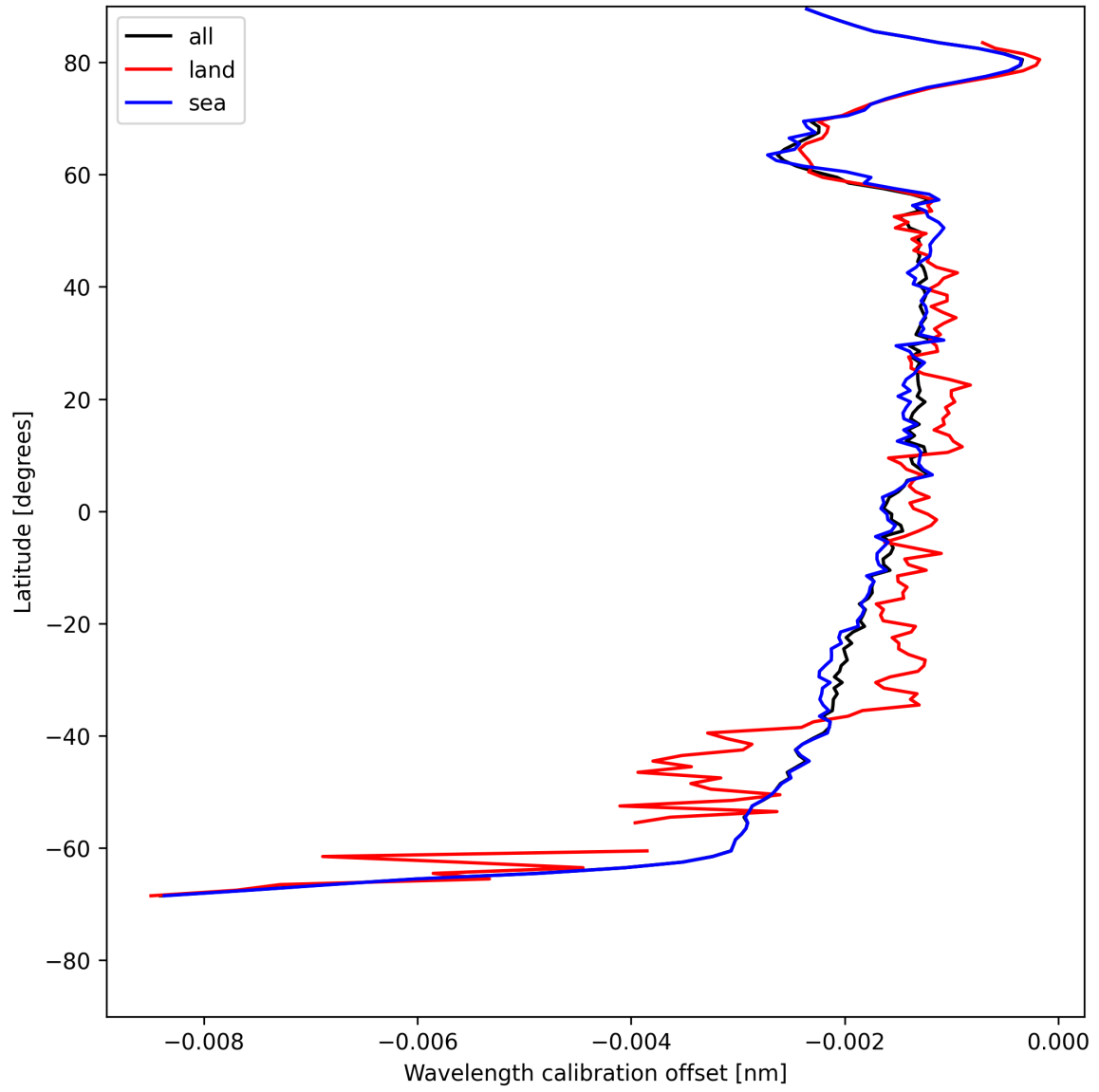
Figure 16: Zonal average of “Wavelength calibration offset” for 2025-05-14 to 2025-05-15.
