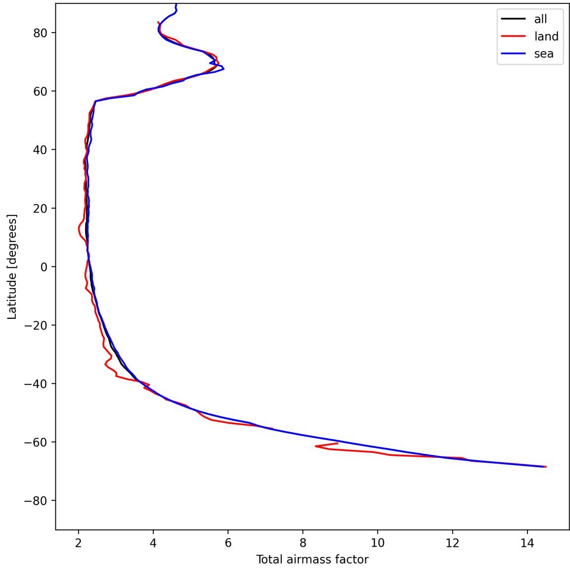
Figure 13: Zonal average of “Total airmass factor” for 2025-05-14 to 2025-05-15.
