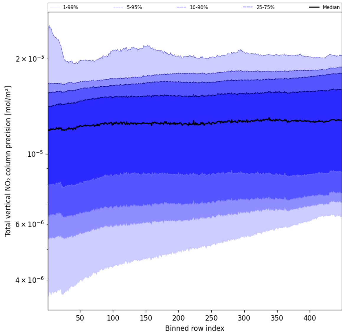
Figure 54: Along track statistics of “Total vertical NO 2 column precision” for 2025-05-15 to 2025-05-16
