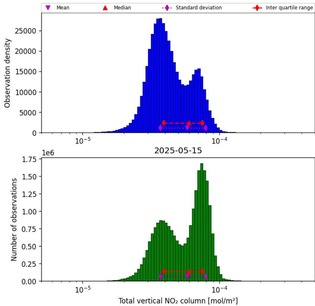
Figure 36: Histogram of “Total vertical NO 2 column” for 2025-05-15 to 2025-05-16
