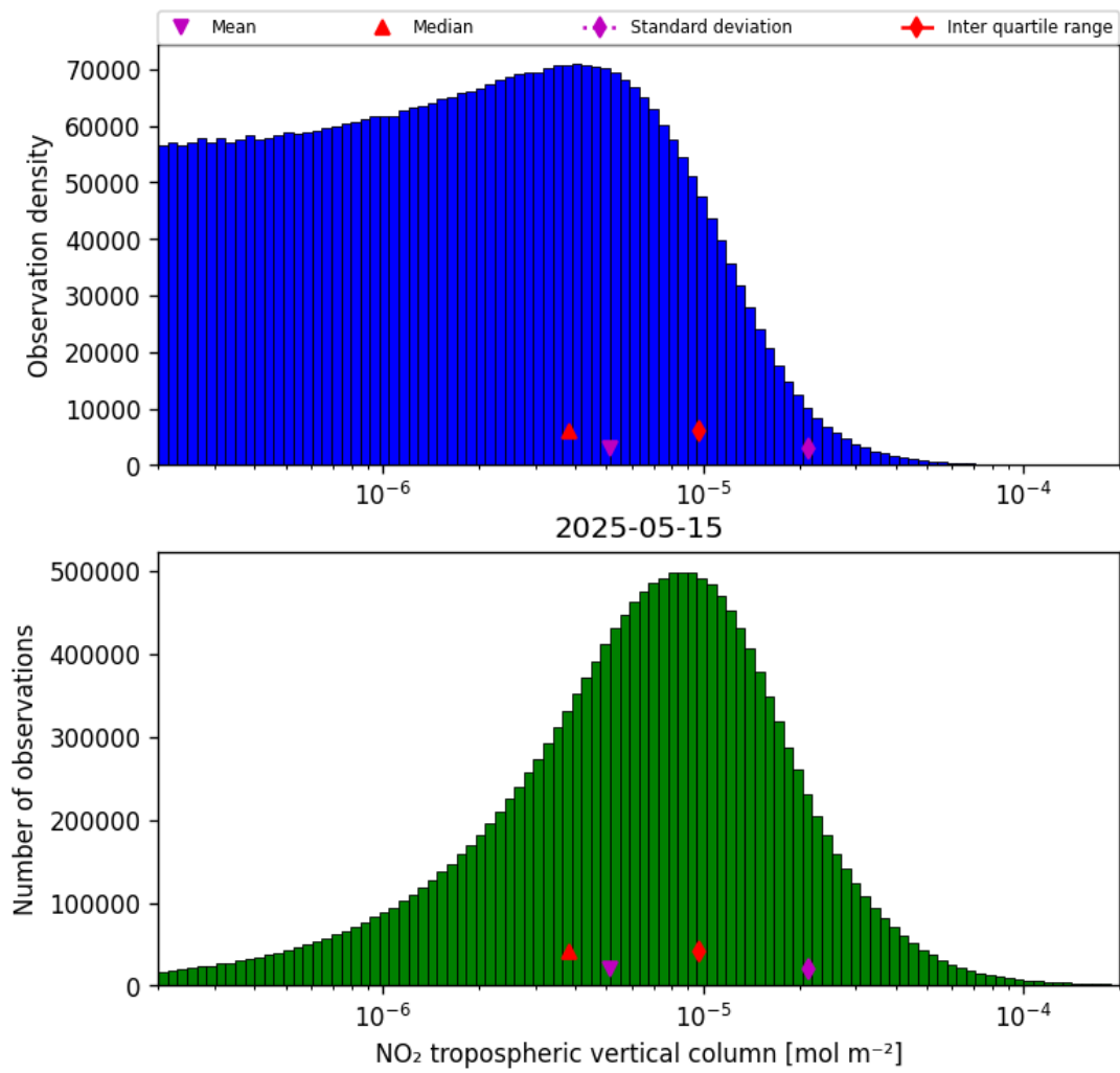
Figure 27: Histogram of “NO 2 tropospheric vertical column” for 2025-05-15 to 2025-05-16
