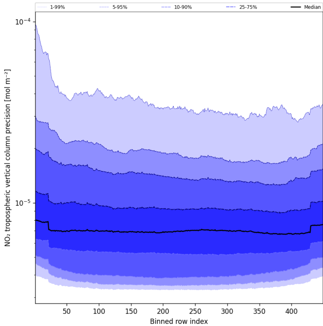
Figure 45: Along track statistics of “NO 2 tropospheric vertical column precision” for 2025-05-15 to 2025-05-16
