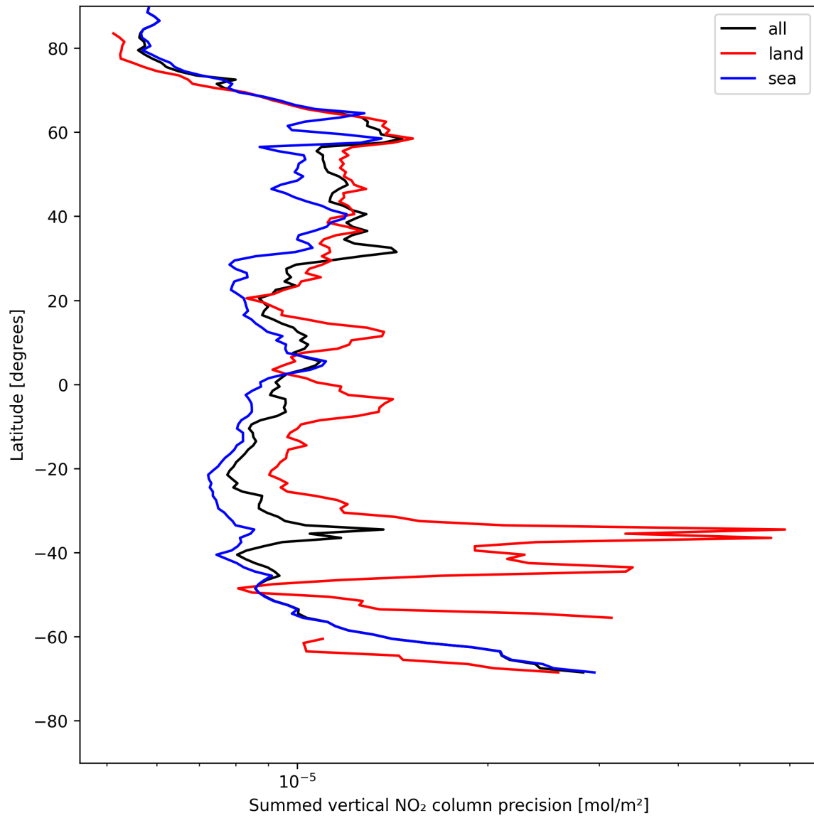
Figure 22: Zonal average of “Summed vertical NO 2 column precision” for 2025-05-15 to 2025-05-16.
