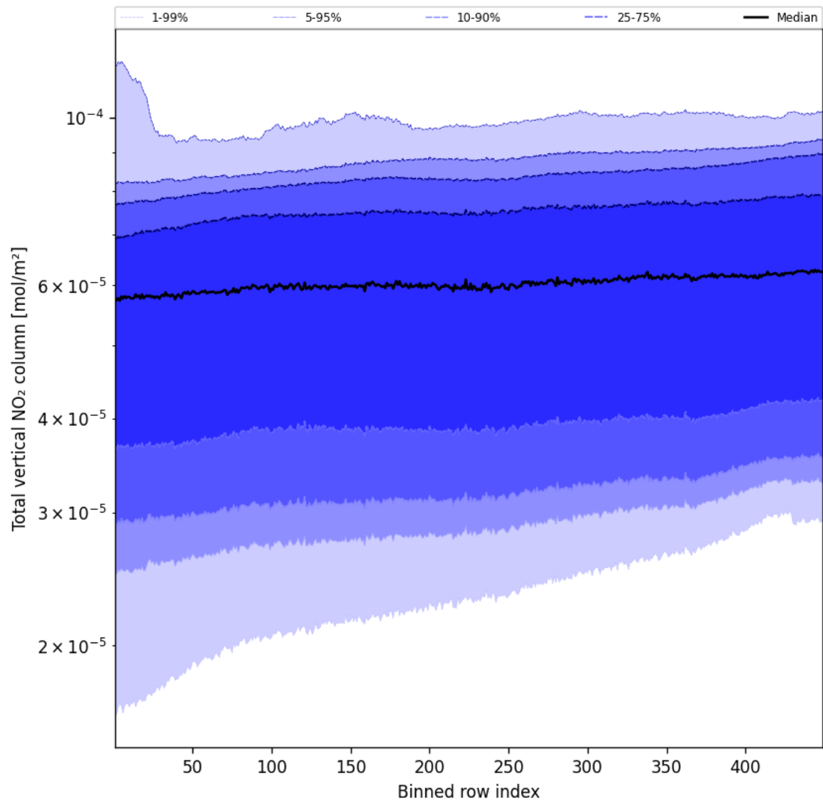
Figure 53: Along track statistics of “Total vertical NO 2 column” for 2025-05-15 to 2025-05-16
