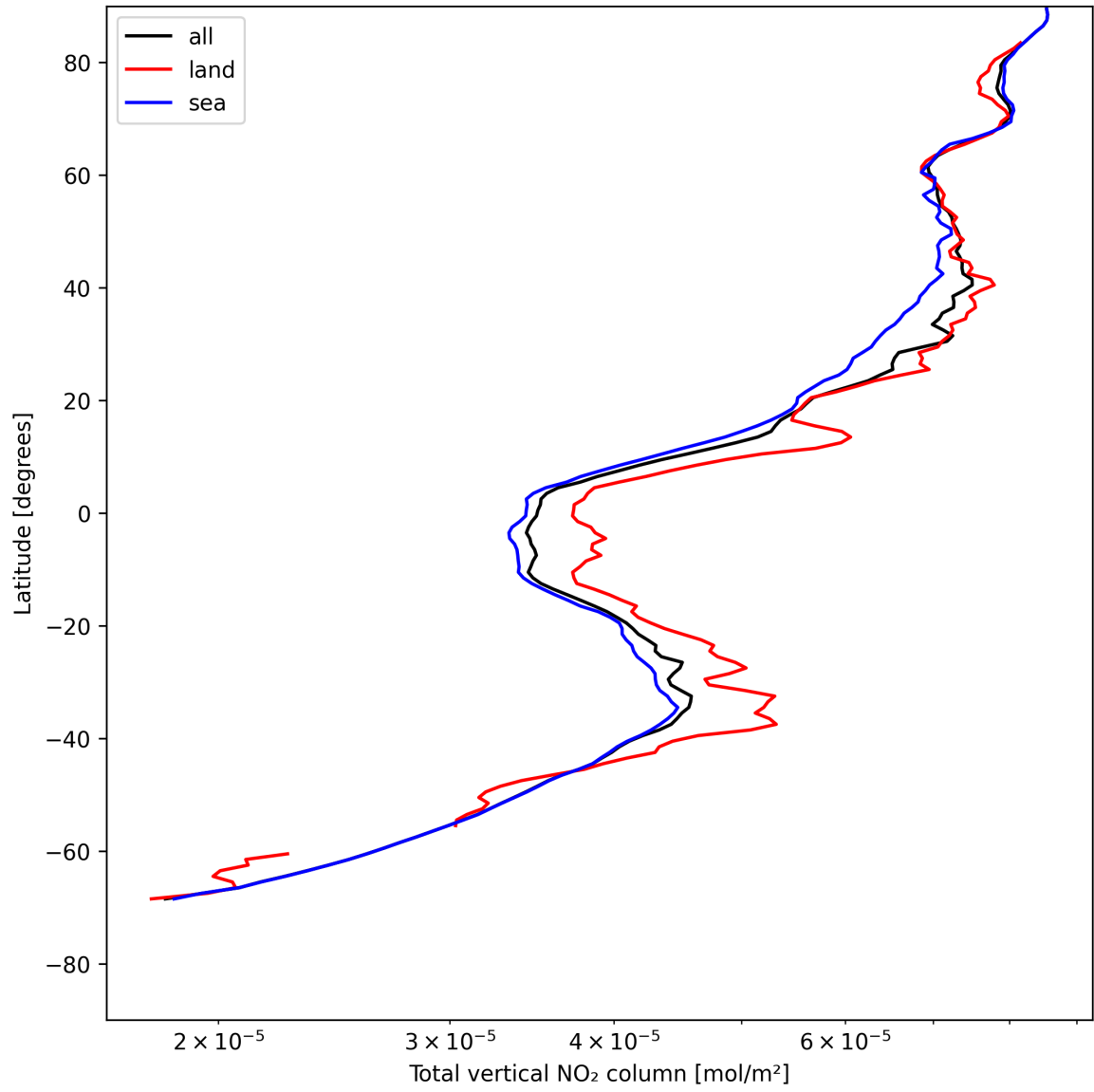
Figure 19: Zonal average of “Total vertical NO 2 column” for 2025-05-15 to 2025-05-16.
