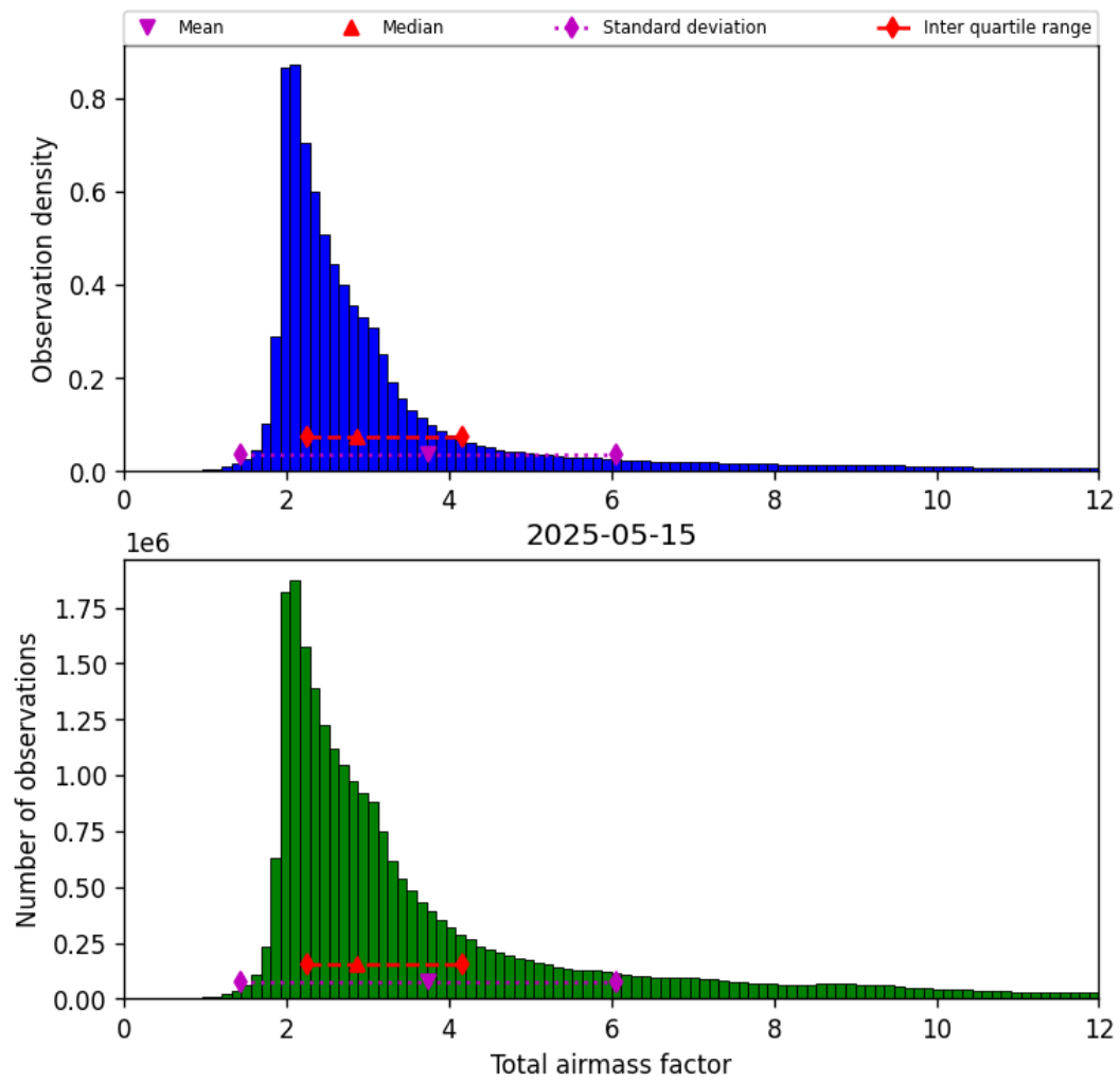
Figure 30: Histogram of “Total airmass factor” for 2025-05-15 to 2025-05-16
