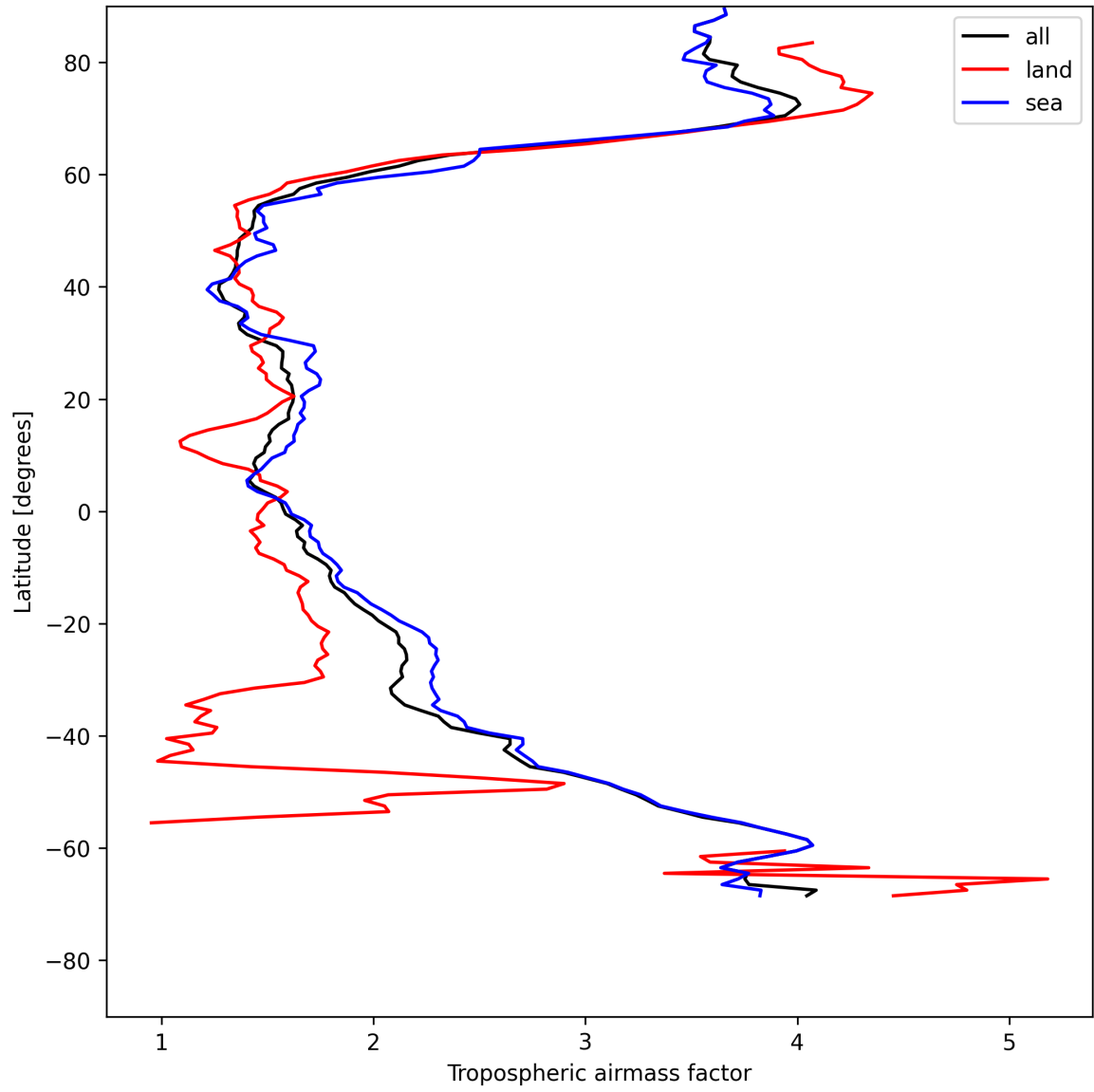
Figure 12: Zonal average of “Tropospheric airmass factor” for 2025-05-15 to 2025-05-16.
