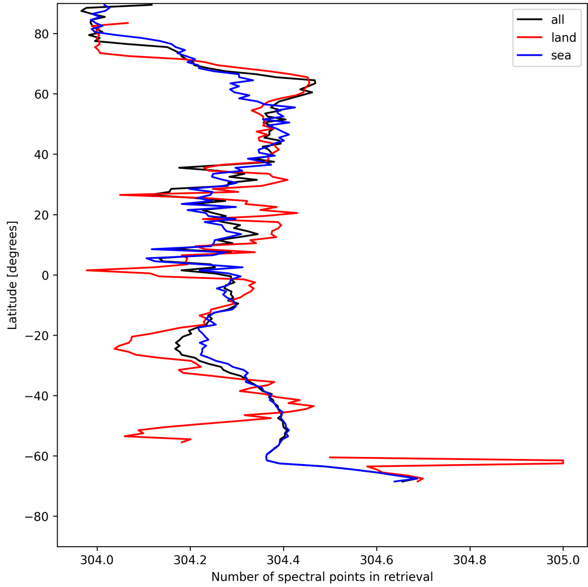
Figure 14: Zonal average of “Number of spectral points in retrieval” for 2025-05-15 to 2025-05-16.
