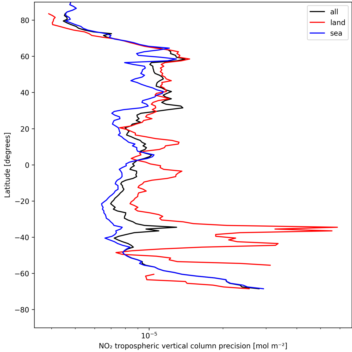
Figure 11: Zonal average of “NO 2 tropospheric vertical column precision” for 2025-05-15 to 2025-05-16.
