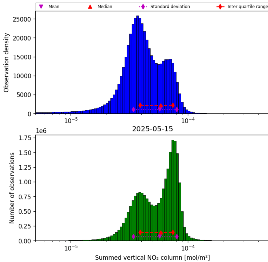
Figure 38: Histogram of “Summed vertical NO 2 column” for 2025-05-15 to 2025-05-16
