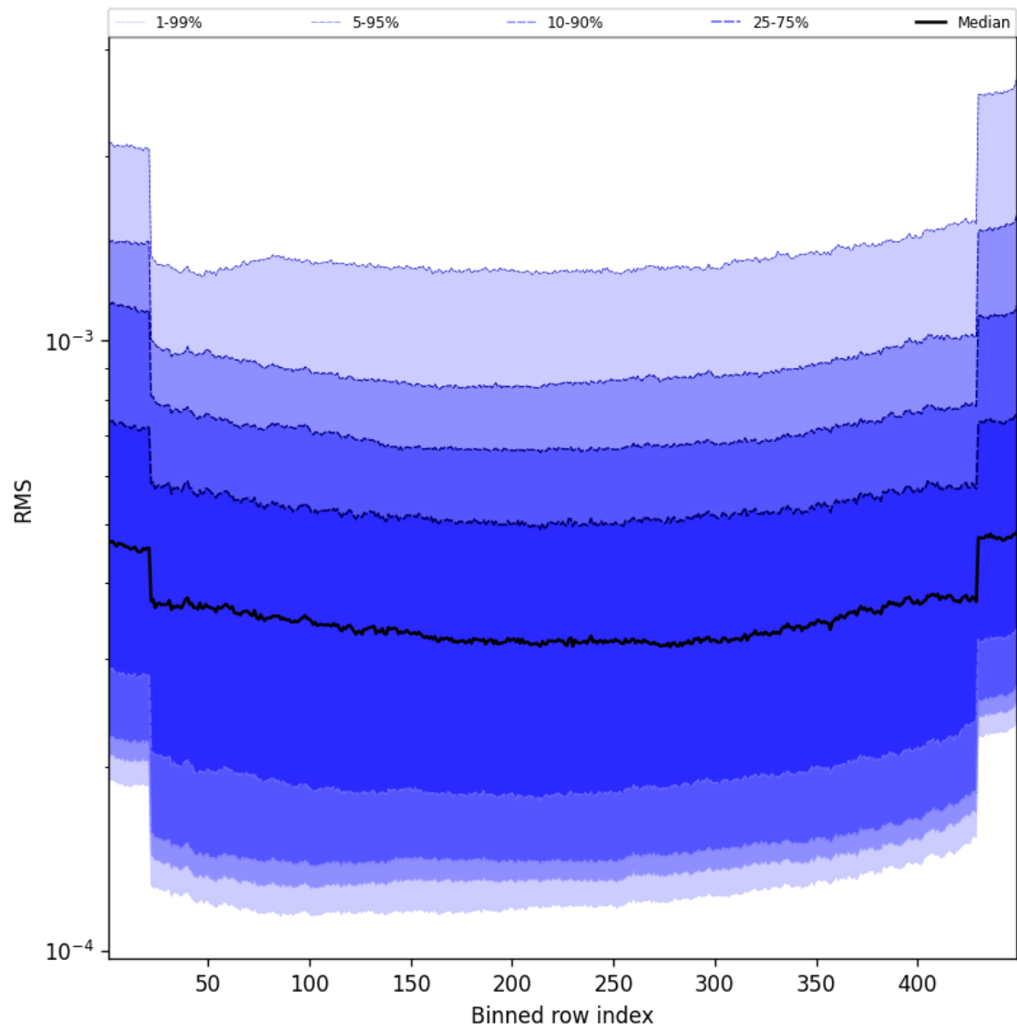
Figure 58: Along track statistics of “RMS” for 2025-05-15 to 2025-05-16
