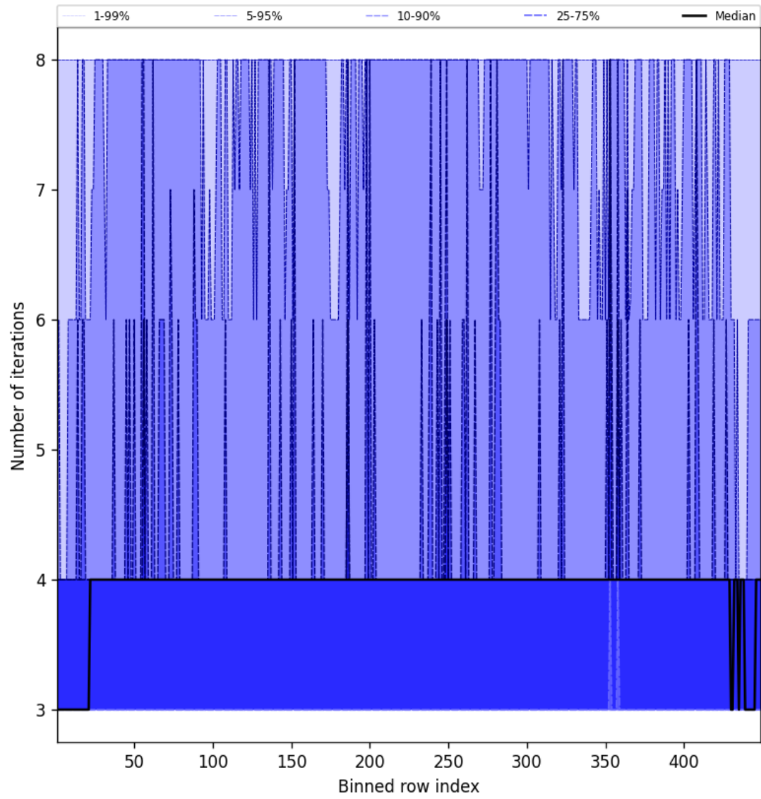
Figure 49: Along track statistics of “Number of iterations” for 2025-05-15 to 2025-05-16
