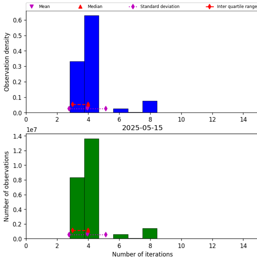
Figure 32: Histogram of “Number of iterations” for 2025-05-15 to 2025-05-16
