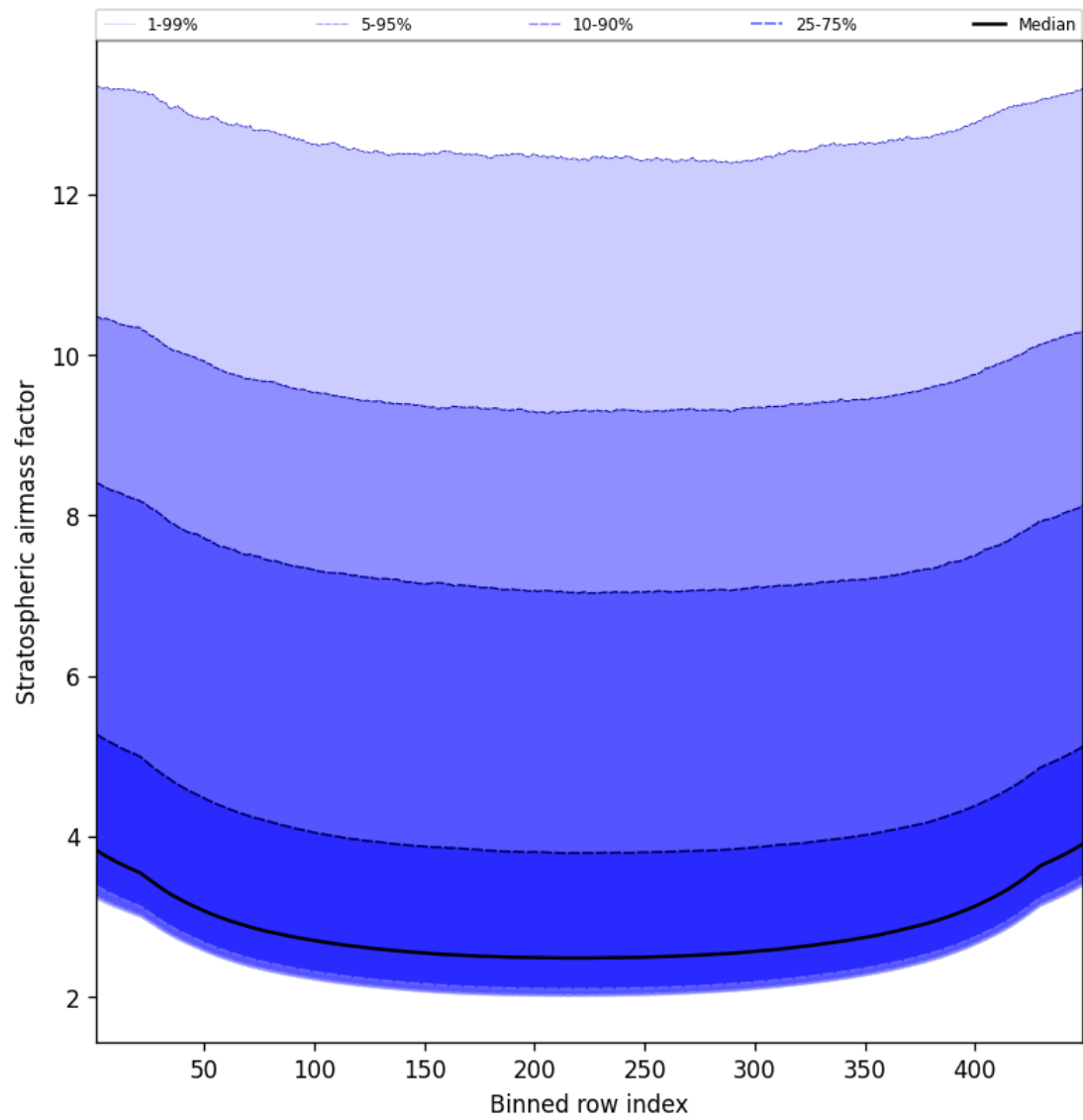
Figure 59: Along track statistics of “Stratospheric airmass factor” for 2025-05-15 to 2025-05-16
