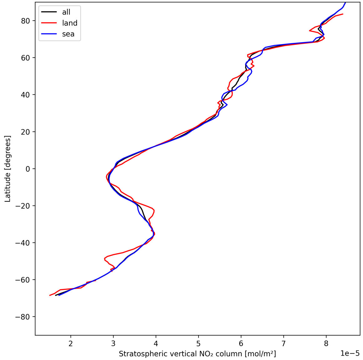
Figure 17: Zonal average of “Stratospheric vertical NO 2 column” for 2025-05-15 to 2025-05-16.
