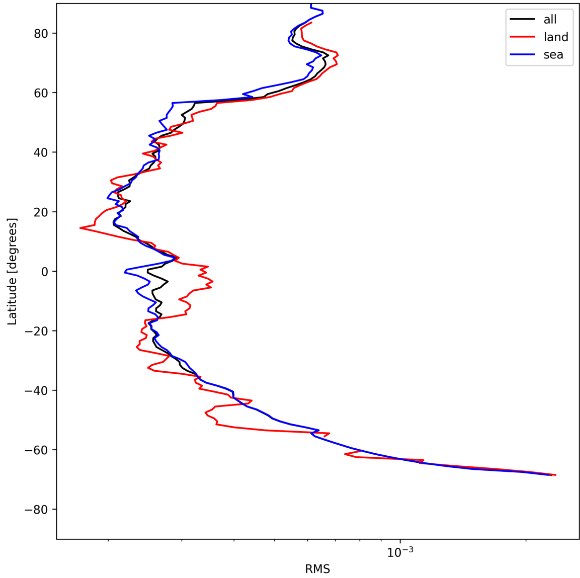
Figure 24: Zonal average of “RMS” for 2025-05-15 to 2025-05-16.
