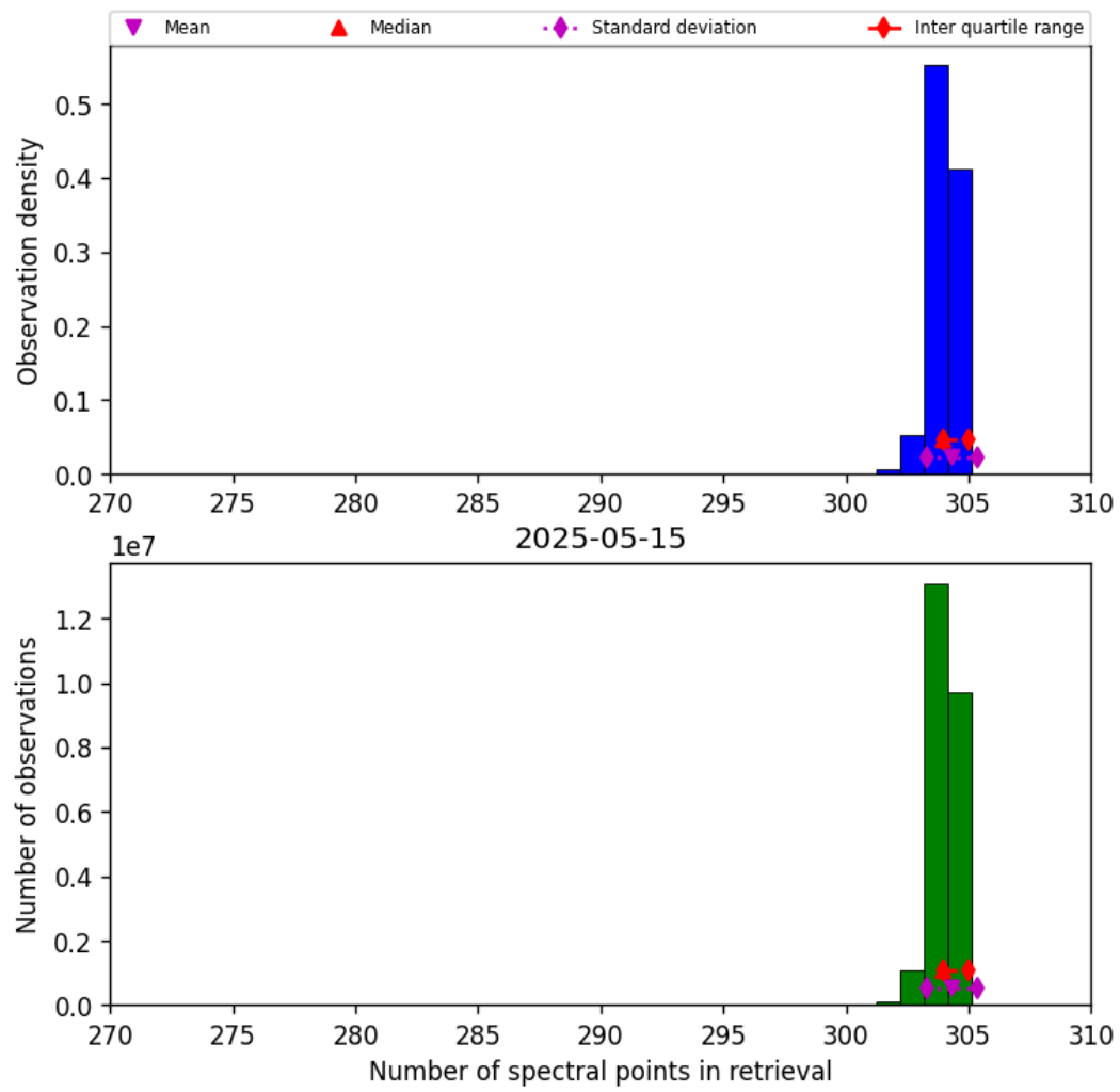
Figure 31: Histogram of “Number of spectral points in retrieval” for 2025-05-15 to 2025-05-16
