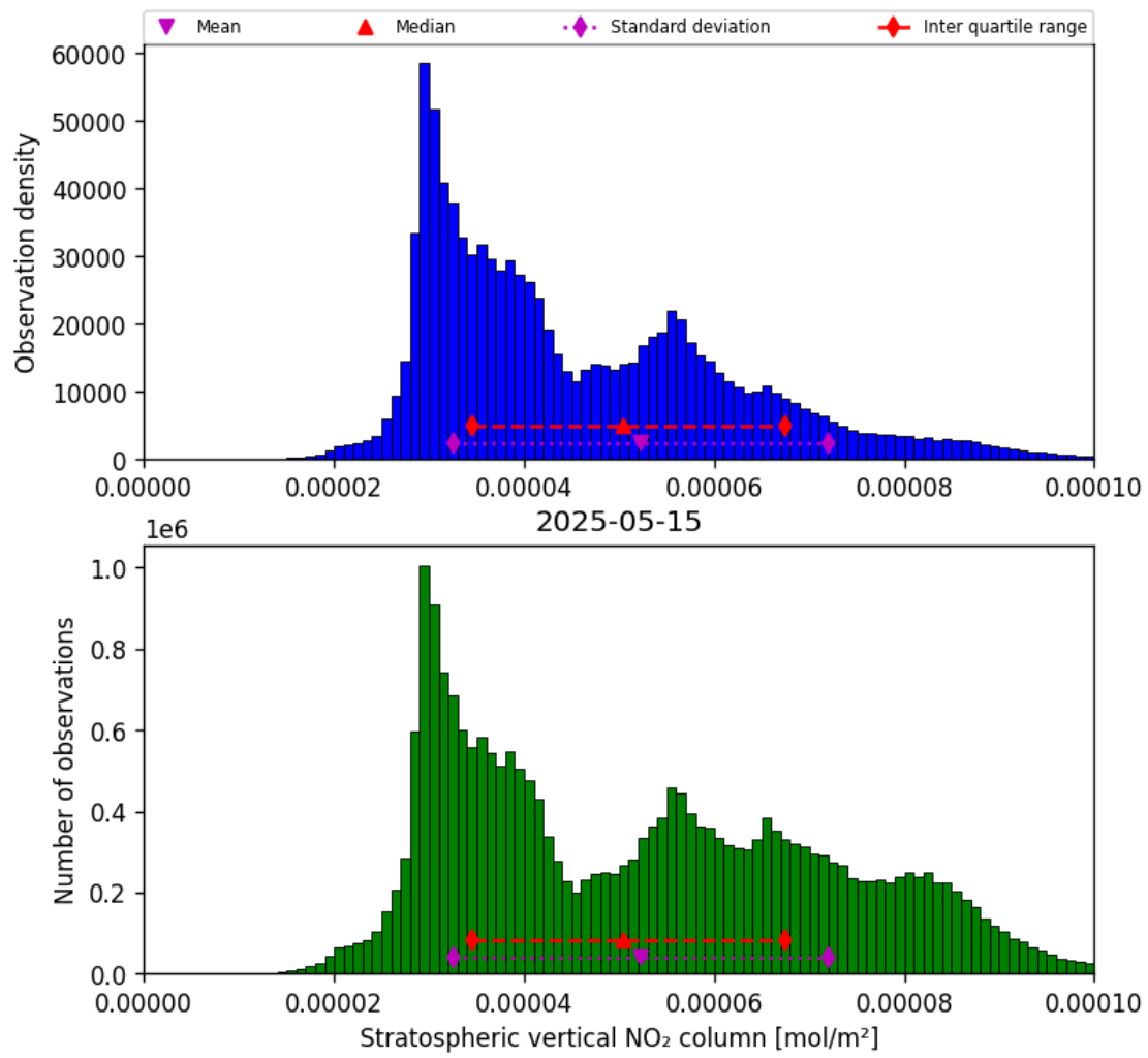
Figure 34: Histogram of “Stratospheric vertical NO 2 column” for 2025-05-15 to 2025-05-16
