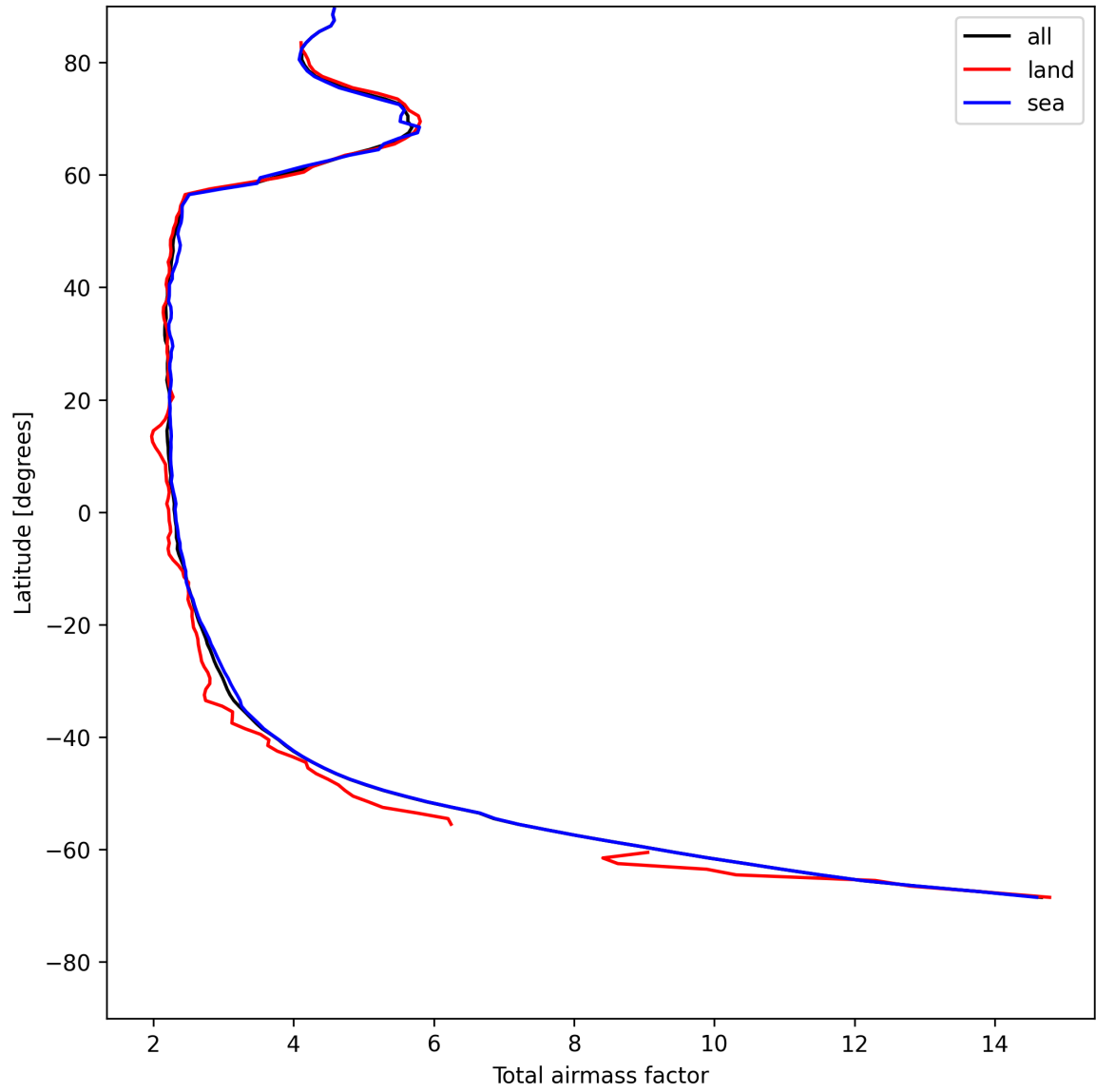
Figure 13: Zonal average of “Total airmass factor” for 2025-05-15 to 2025-05-16.
