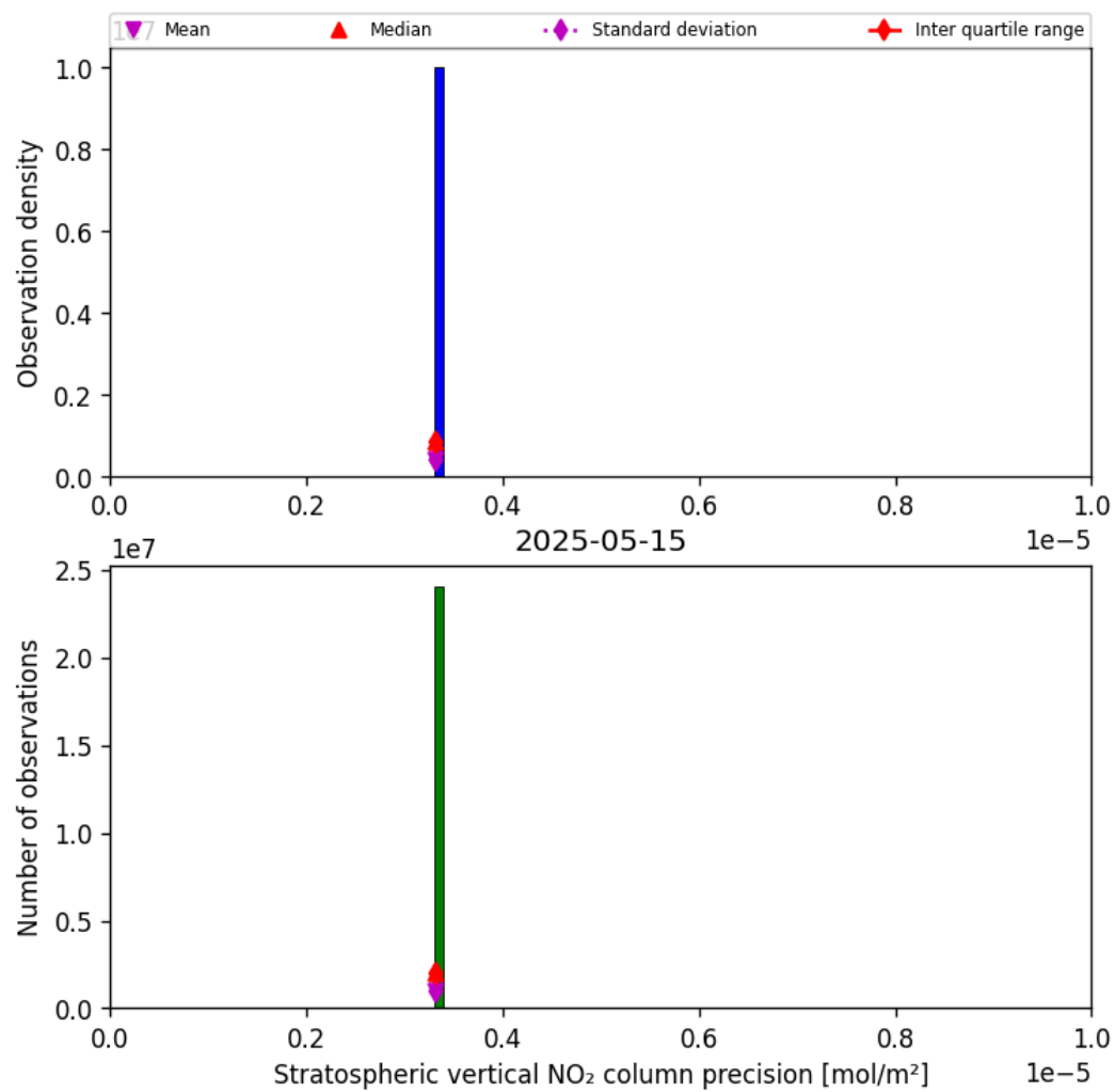
Figure 35: Histogram of “Stratospheric vertical NO 2 column precision” for 2025-05-15 to 2025-05-16
