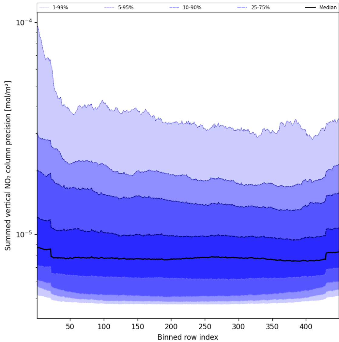
Figure 56: Along track statistics of “Summed vertical NO 2 column precision” for 2025-05-15 to 2025-05-16
