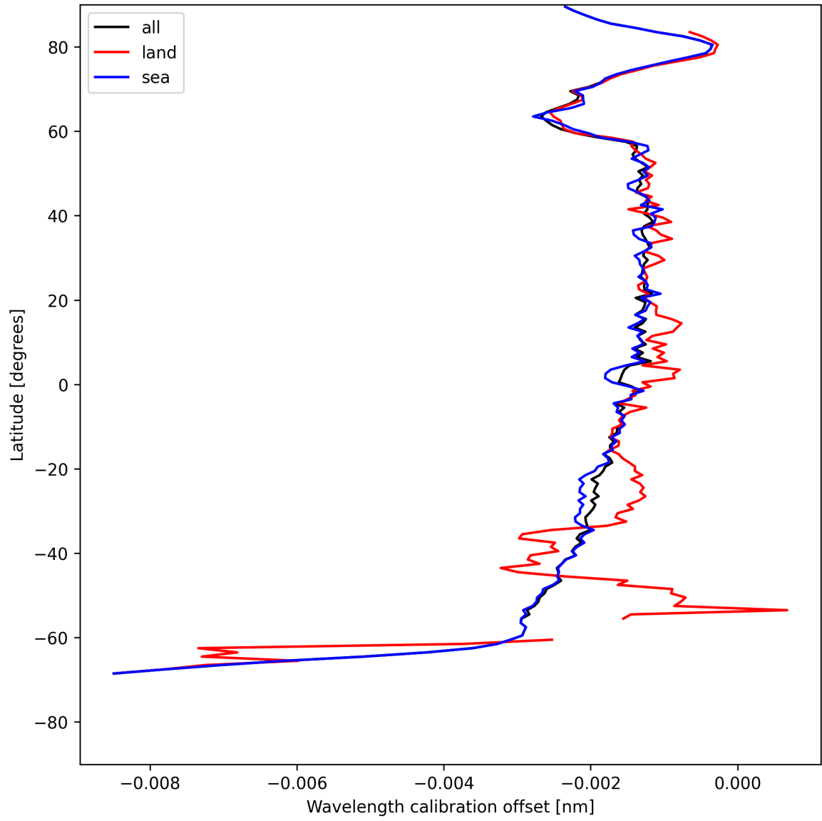
Figure 16: Zonal average of “Wavelength calibration offset” for 2025-05-15 to 2025-05-16.
