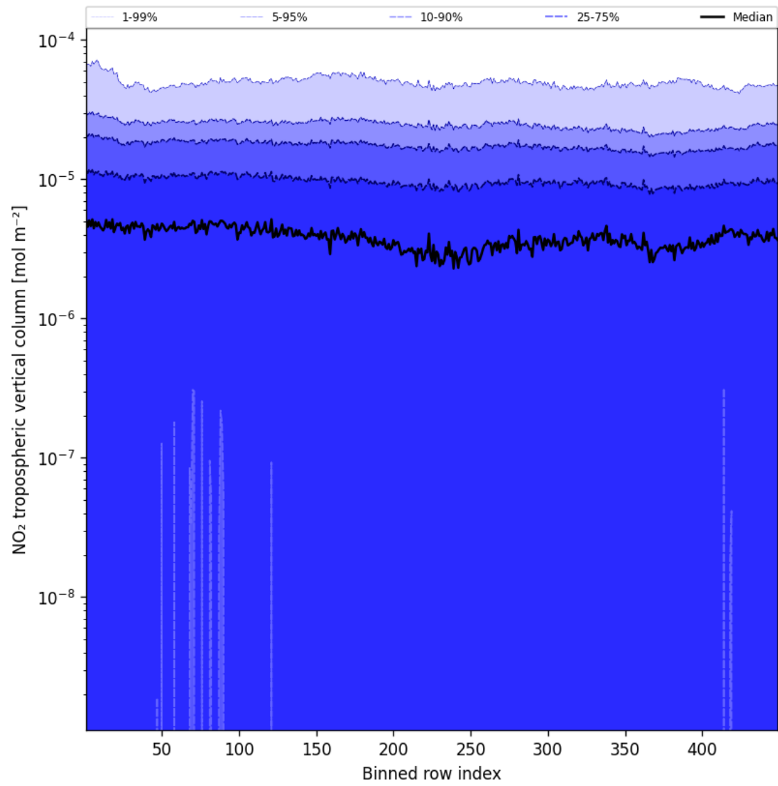
Figure 44: Along track statistics of “NO 2 tropospheric vertical column” for 2025-05-15 to 2025-05-16
