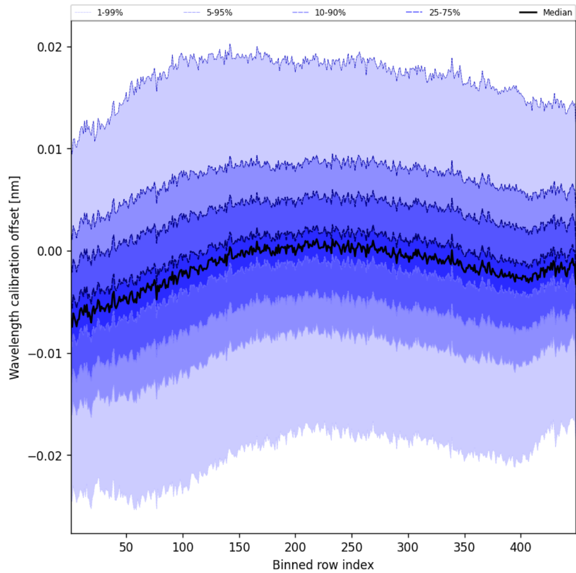
Figure 50: Along track statistics of “Wavelength calibration offset” for 2025-05-15 to 2025-05-16
