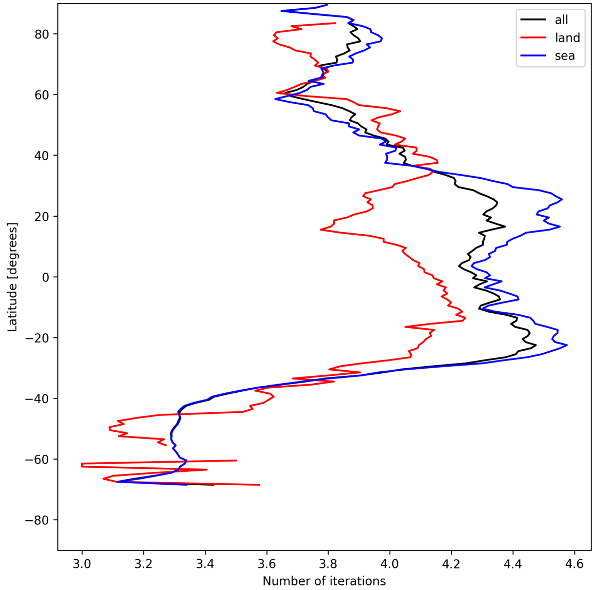
Figure 15: Zonal average of “Number of iterations” for 2025-05-15 to 2025-05-16.
