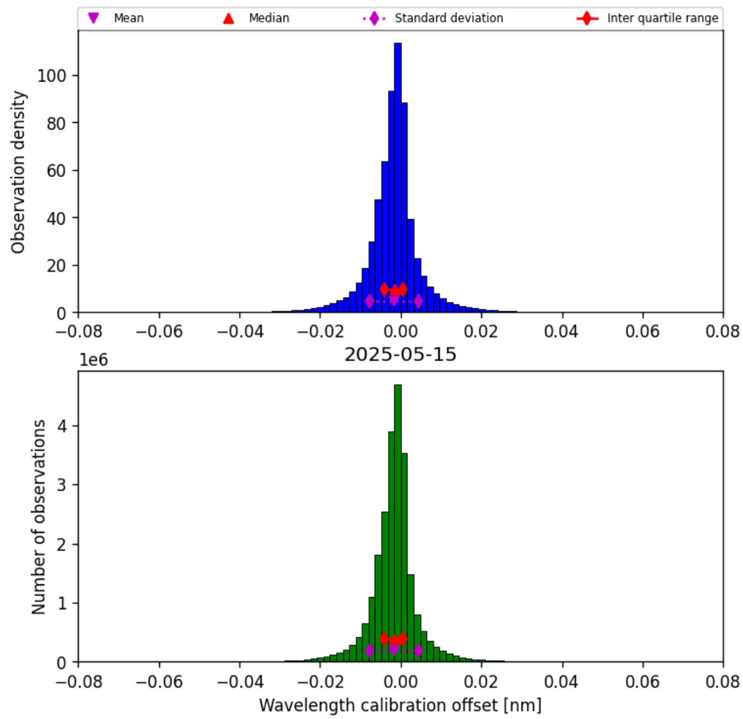
Figure 33: Histogram of “Wavelength calibration offset” for 2025-05-15 to 2025-05-16
