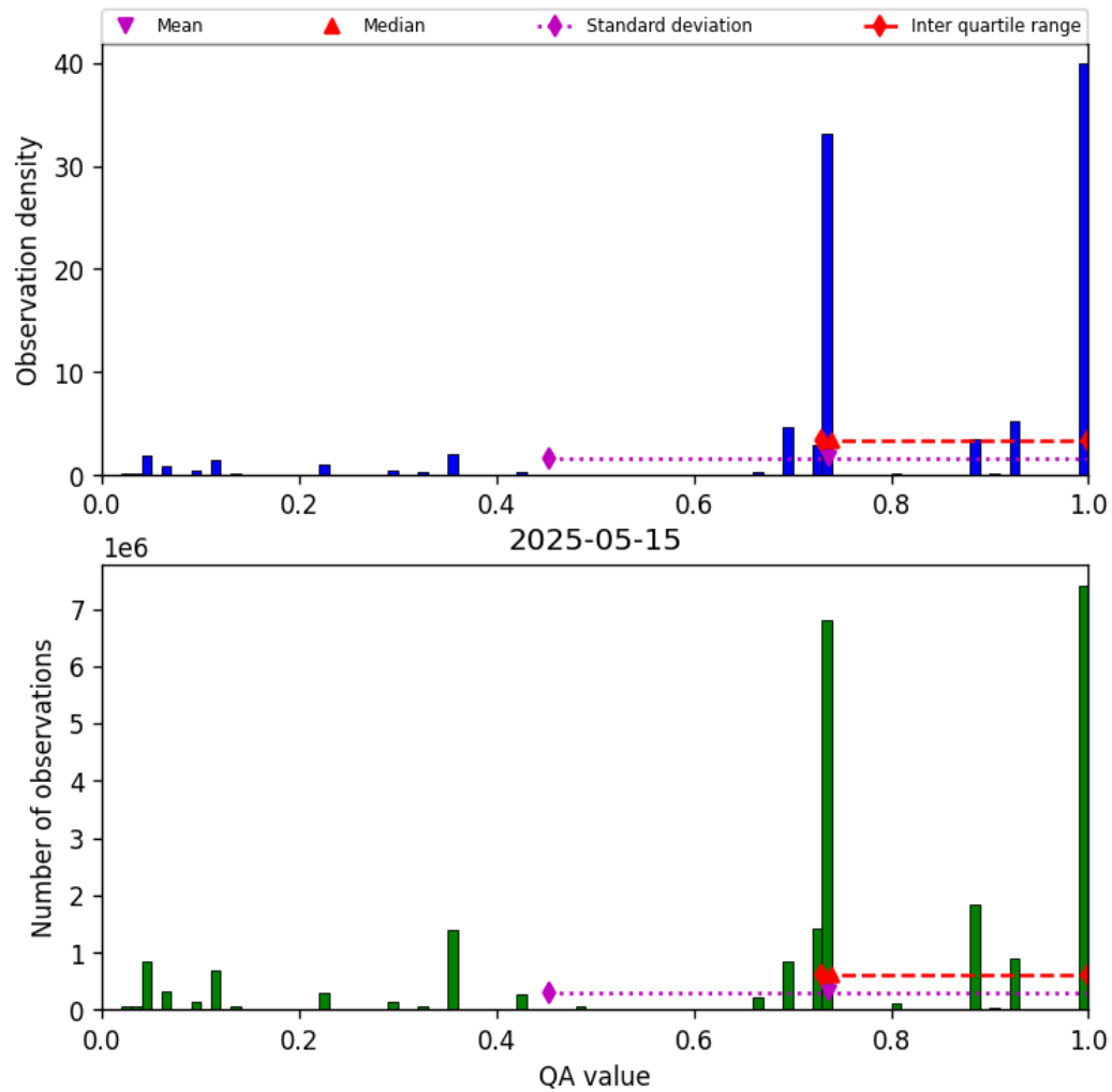
Figure 26: Histogram of “QA value” for 2025-05-15 to 2025-05-16
