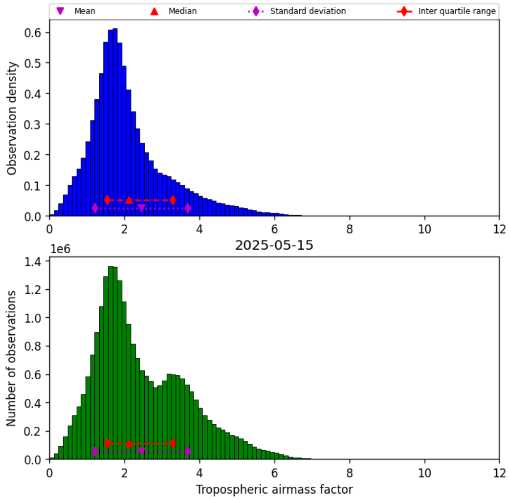
Figure 29: Histogram of “Tropospheric airmass factor” for 2025-05-15 to 2025-05-16
