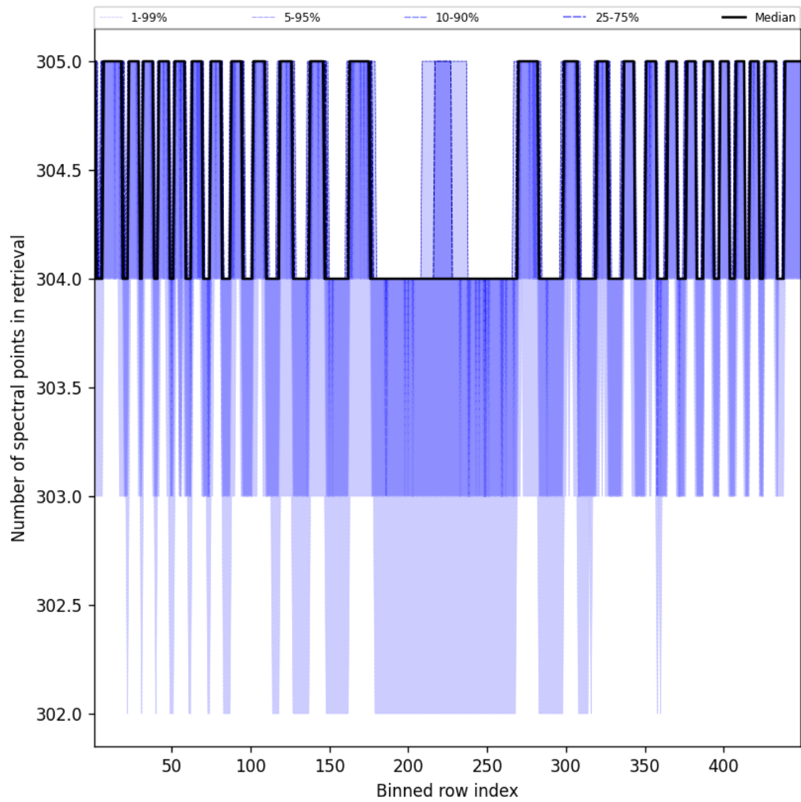
Figure 48: Along track statistics of “Number of spectral points in retrieval” for 2025-05-15 to 2025-05-16
