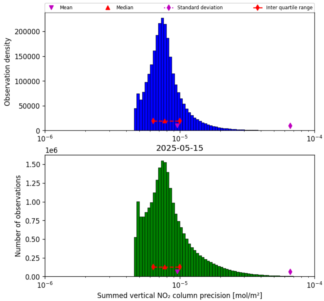
Figure 39: Histogram of "Summed vertical NO 2 column precision" for 2025-05-15 to 2025-05-16
