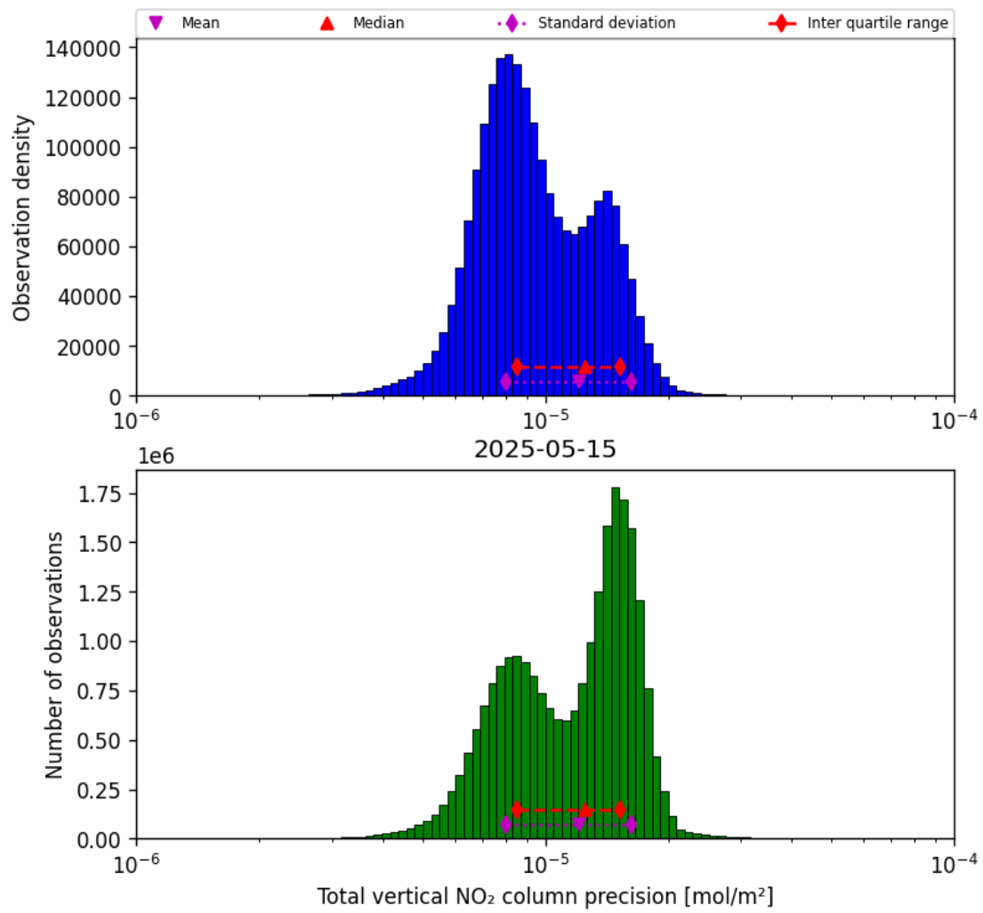
Figure 37: Histogram of “Total vertical NO 2 column precision” for 2025-05-15 to 2025-05-16
