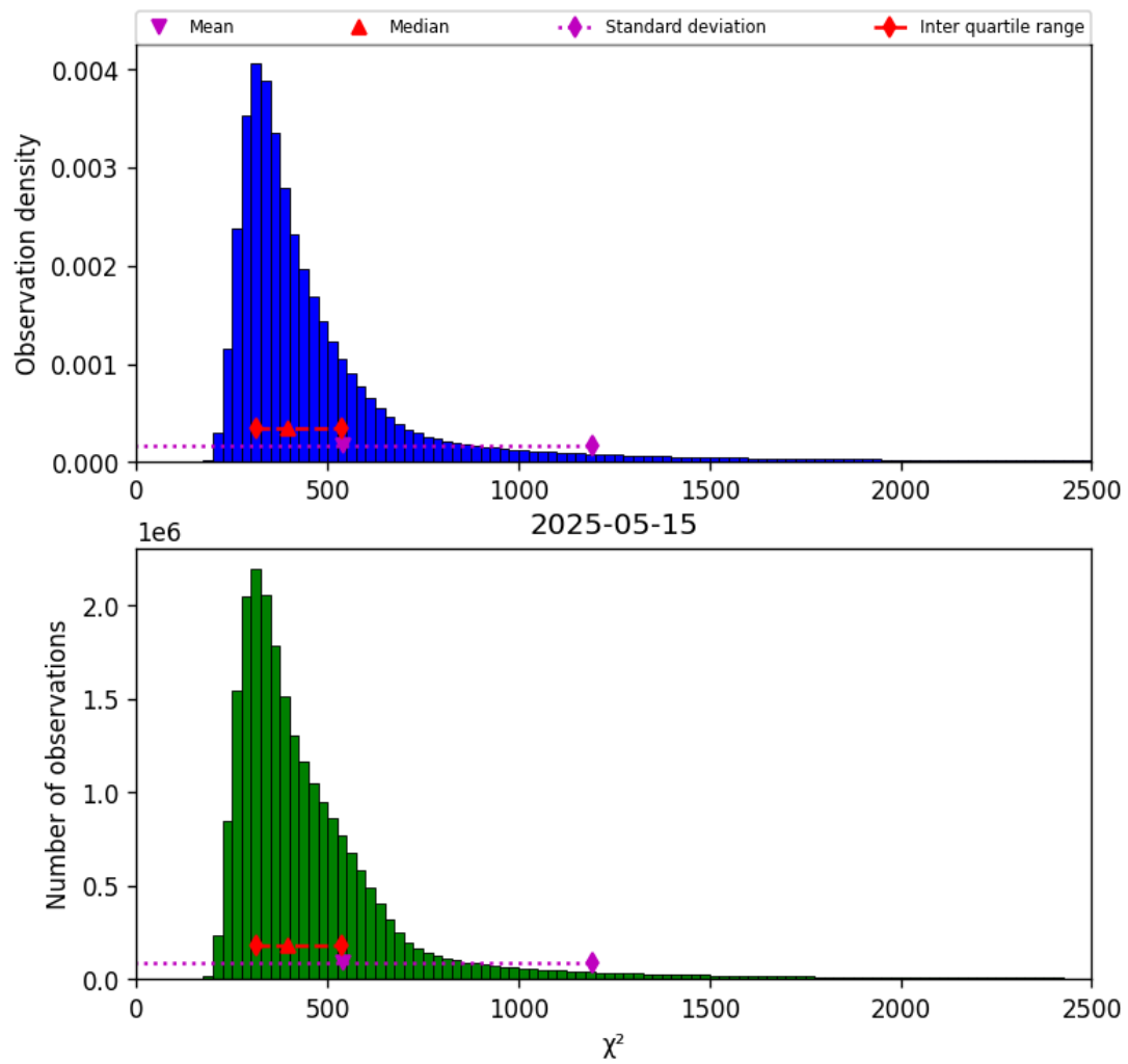
Figure 40: Histogram of “ \chi^2 ” for 2025-05-15 to 2025-05-16
