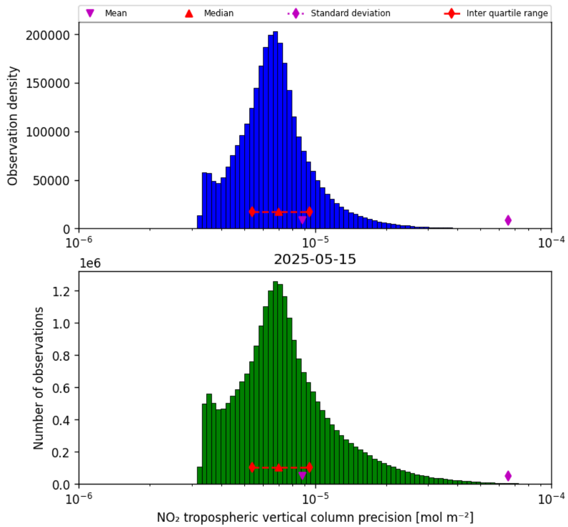
Figure 28: Histogram of “NO 2 tropospheric vertical column precision” for 2025-05-15 to 2025-05-16
