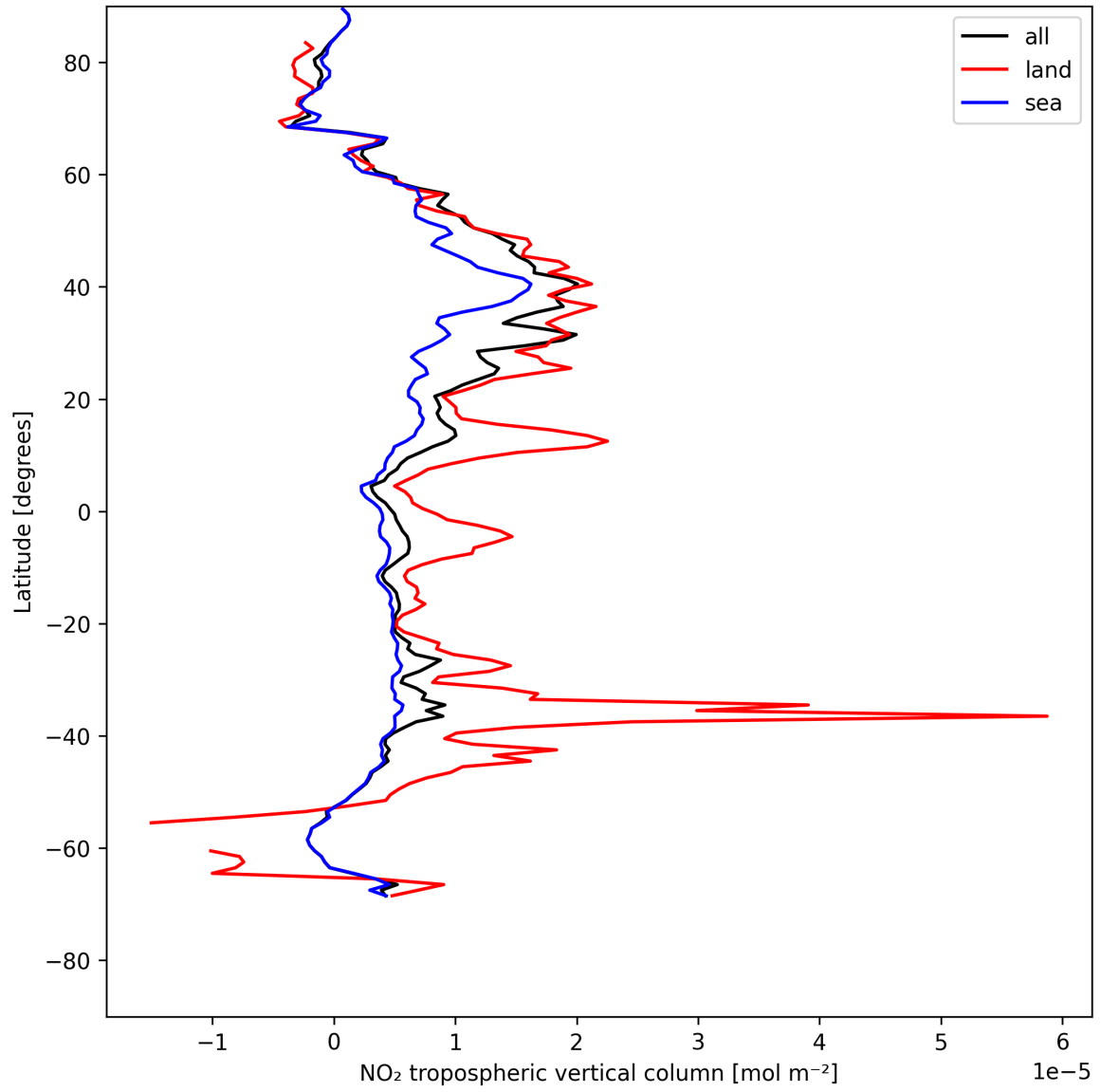
Figure 10: Zonal average of “NO 2 tropospheric vertical column” for 2025-05-15 to 2025-05-16.
