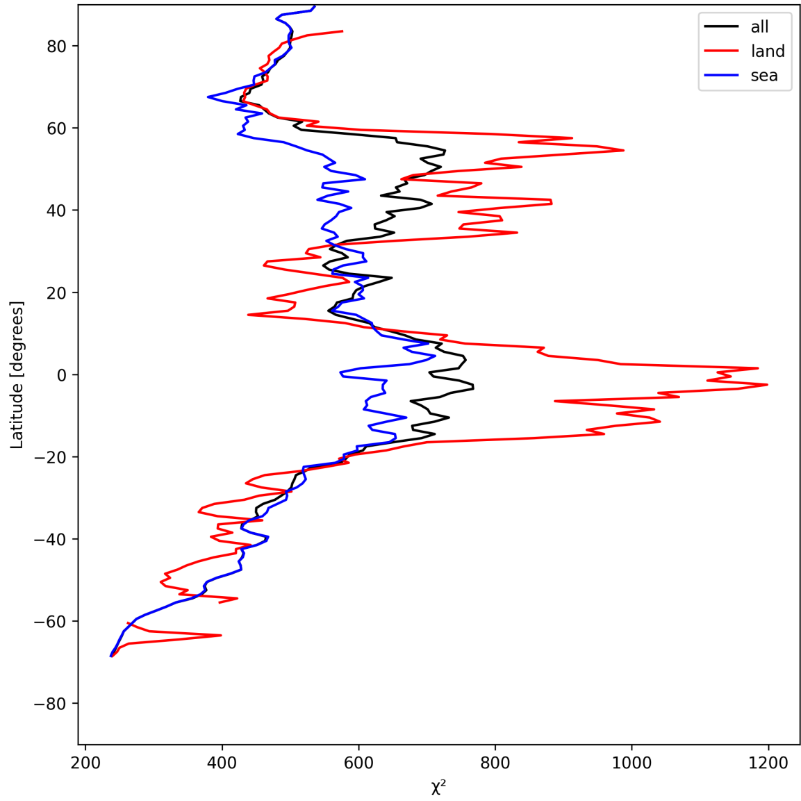
Figure 23: Zonal average of “ \chi^2 ” for 2025-05-15 to 2025-05-16.
