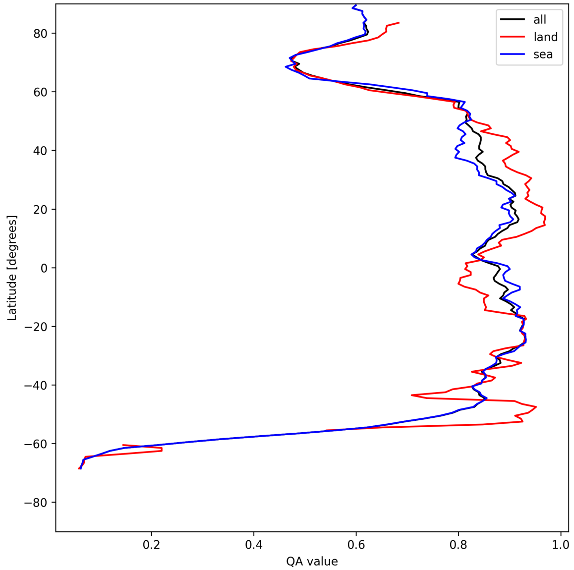
Figure 9: Zonal average of “QA value” for 2025-05-15 to 2025-05-16.
