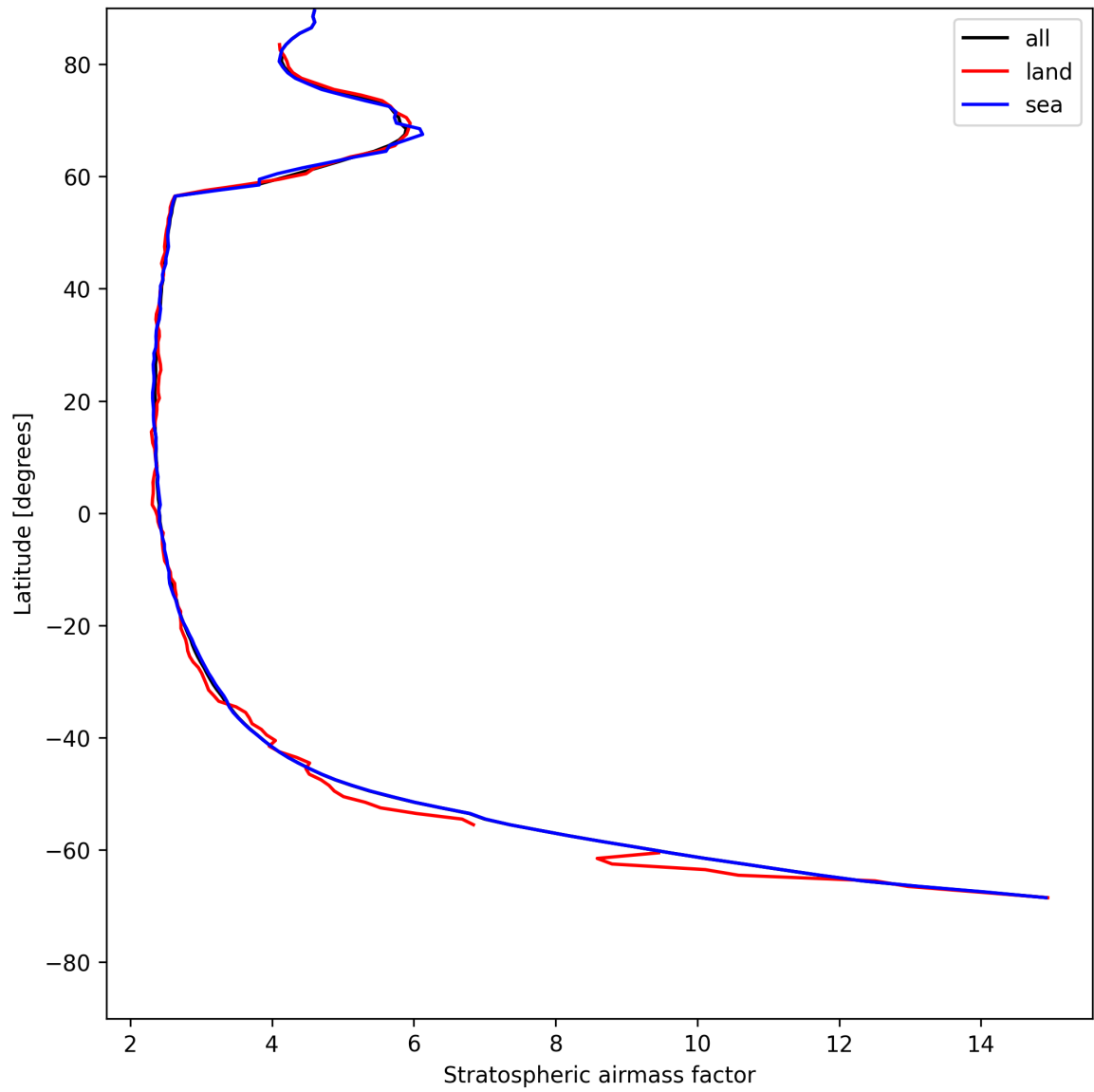
Figure 25: Zonal average of “Stratospheric air mass factor” for 2025-05-15 to 2025-05-16.
