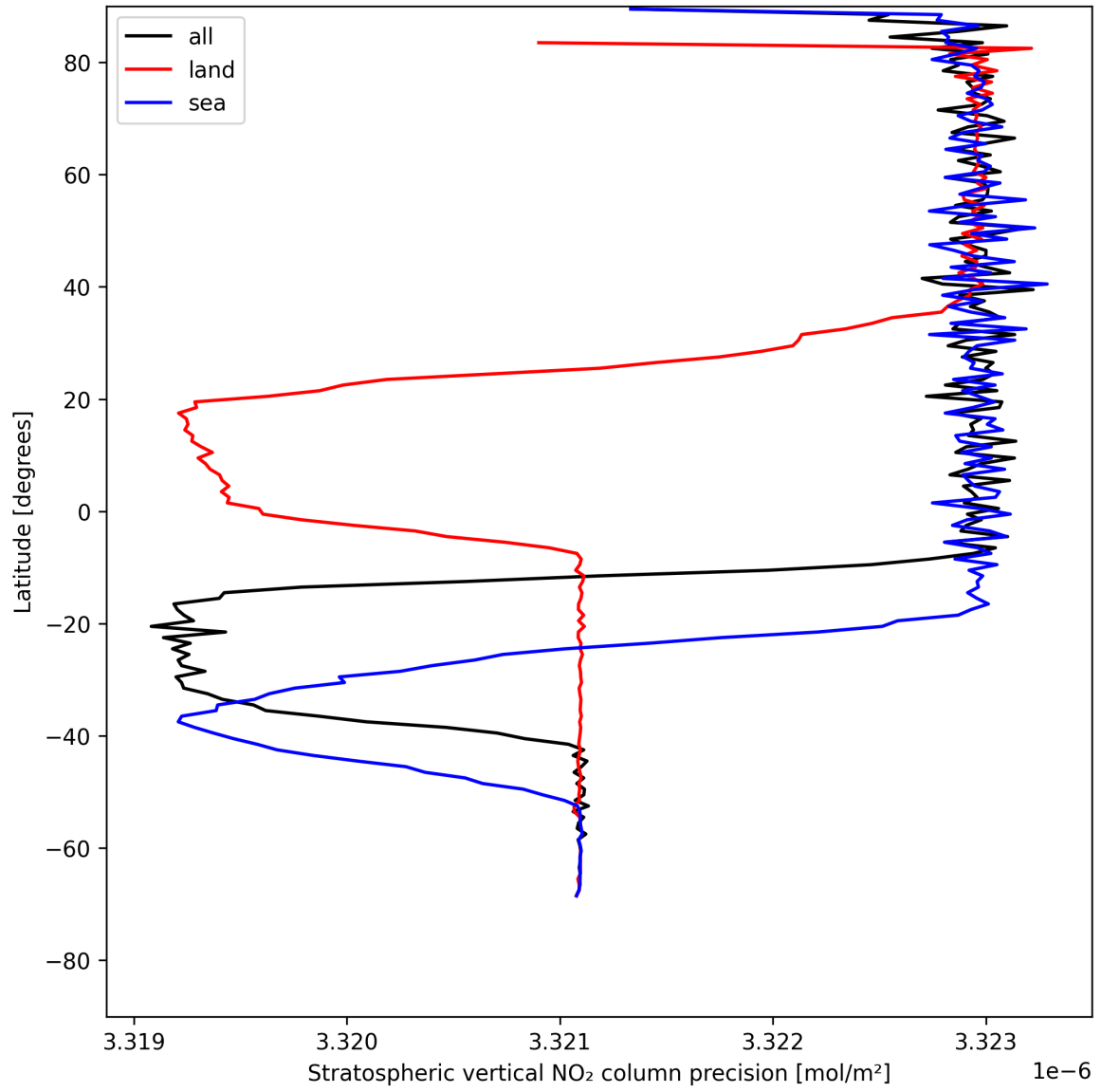
Figure 18: Zonal average of “Stratospheric vertical NO 2 column precision” for 2025-05-15 to 2025-05-16.
