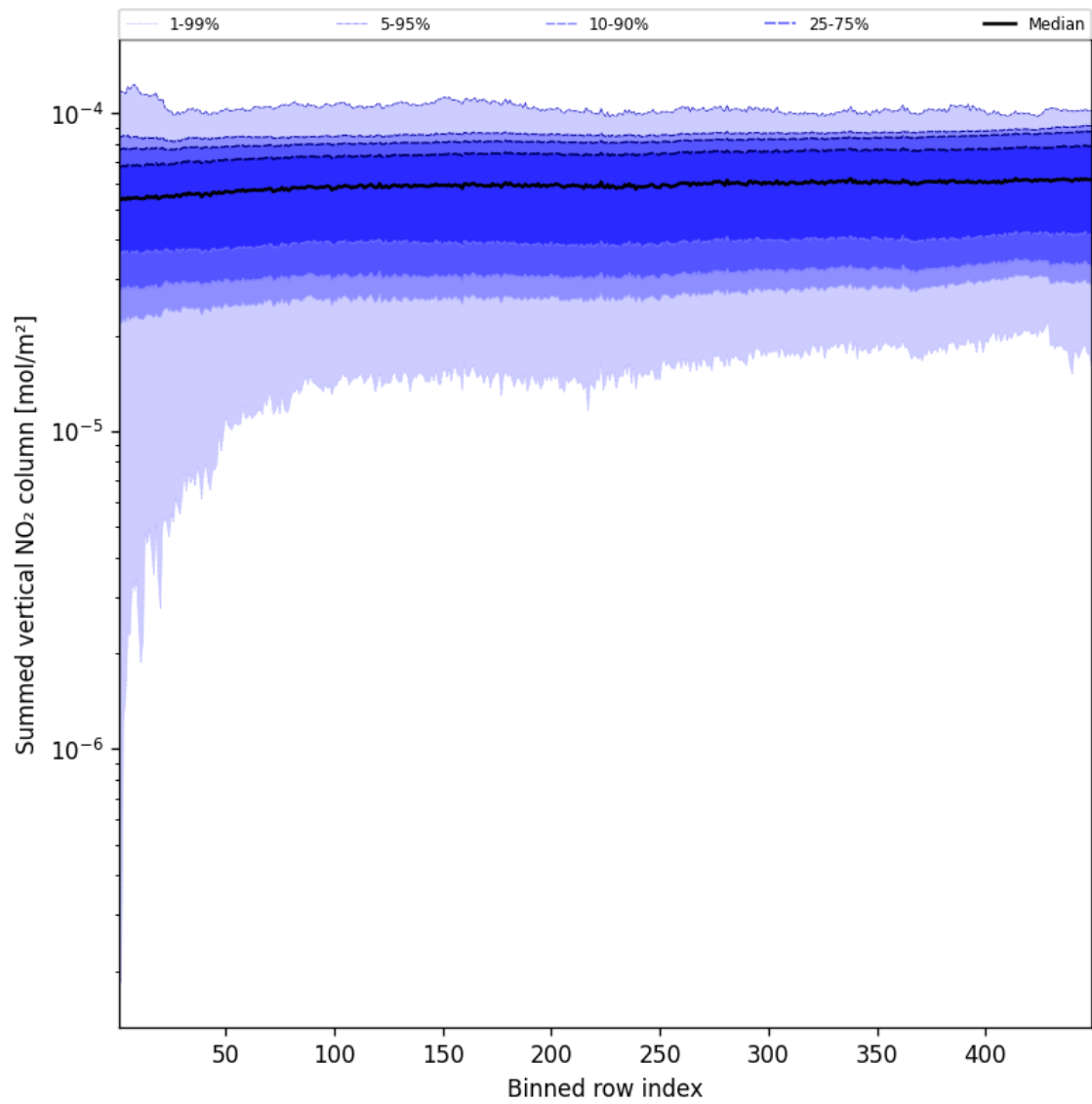
Figure 55: Along track statistics of “Summed vertical NO 2 column” for 2025-05-15 to 2025-05-16
