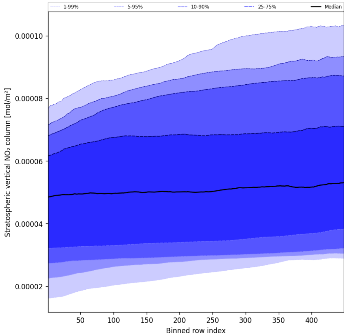
Figure 51: Along track statistics of “Stratospheric vertical NO 2 column” for 2025-05-15 to 2025-05-16
