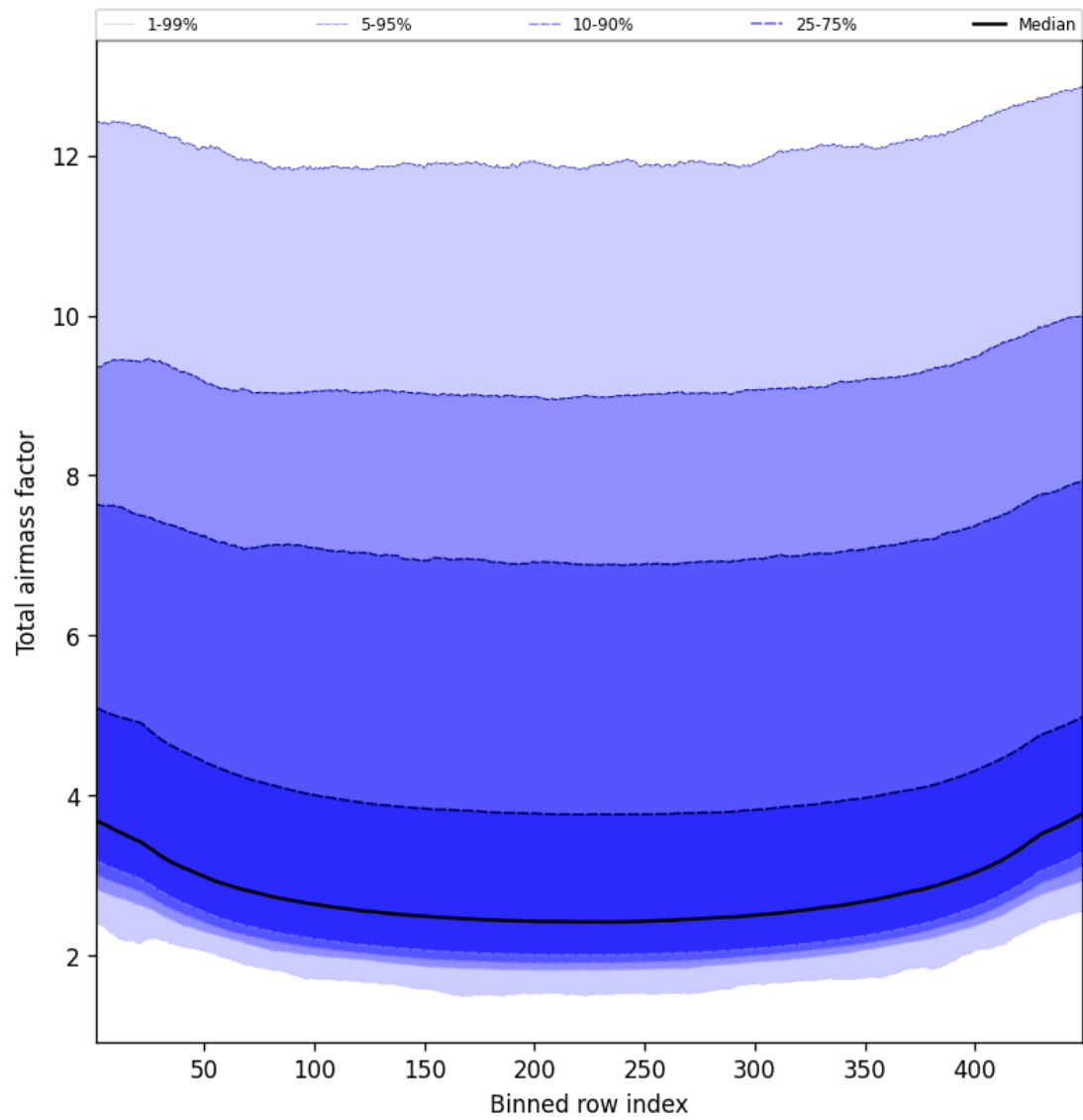
Figure 47: Along track statistics of “Total airmass factor” for 2025-05-15 to 2025-05-16
