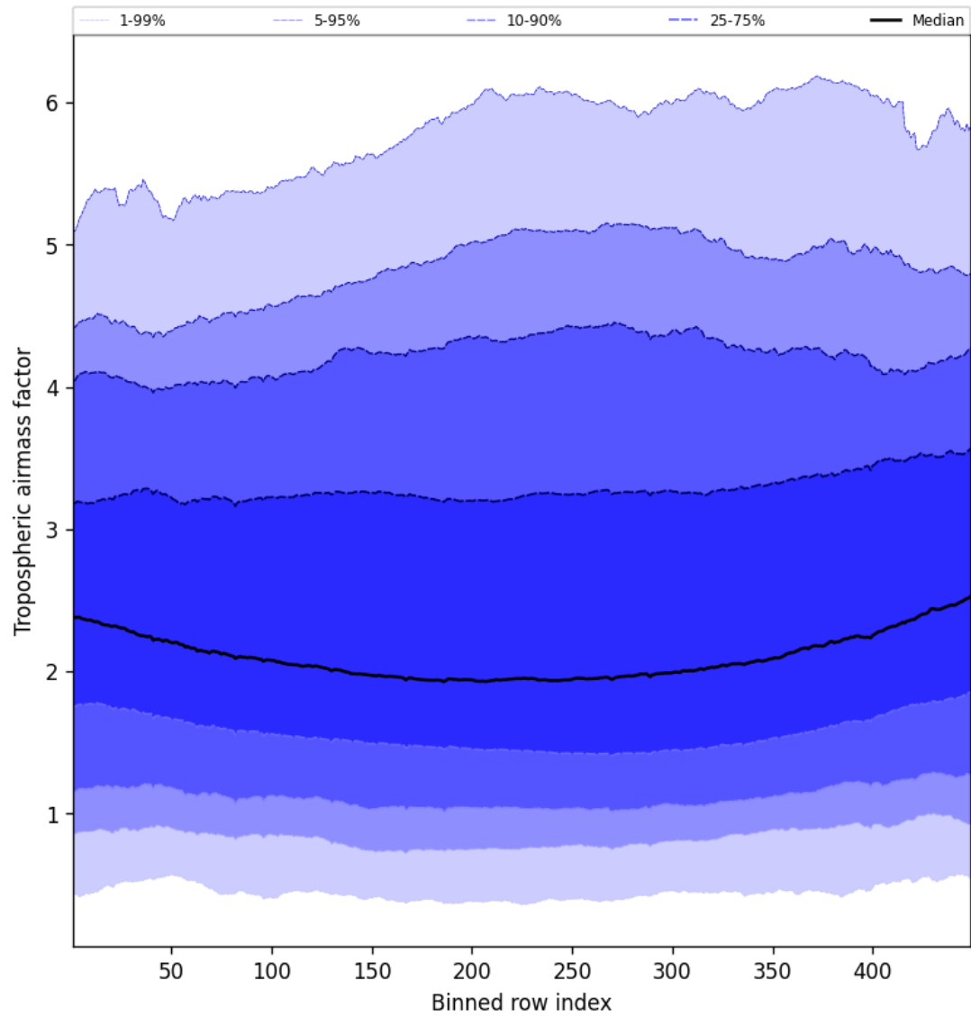
Figure 46: Along track statistics of “Tropospheric airmass factor” for 2025-05-15 to 2025-05-16
