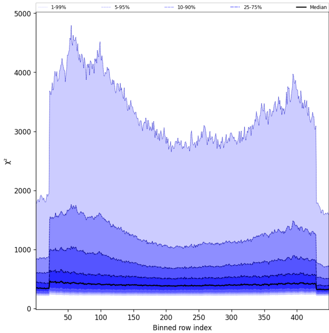
Figure 57: Along track statistics of “ \chi^2 ” for 2025-05-15 to 2025-05-16
