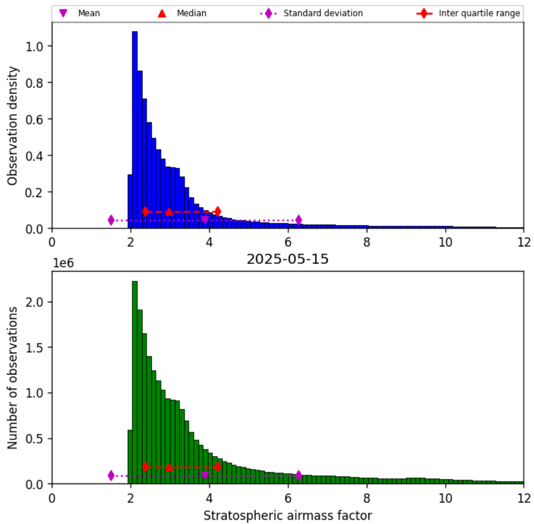
Figure 42: Histogram of “Stratospheric airmass factor” for 2025-05-15 to 2025-05-16
