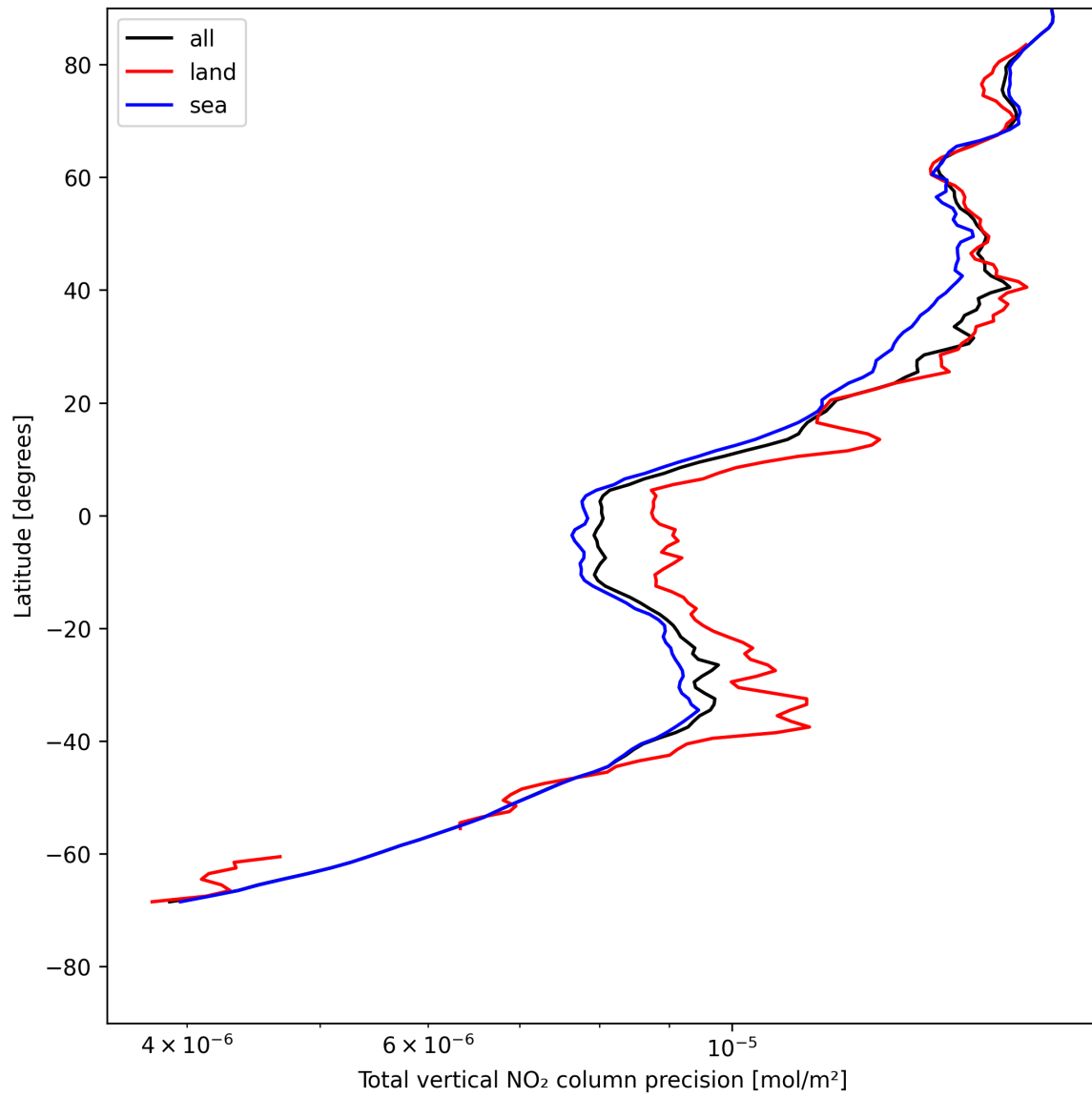
Figure 20: Zonal average of “Total vertical NO 2 column precision” for 2025-05-15 to 2025-05-16.
