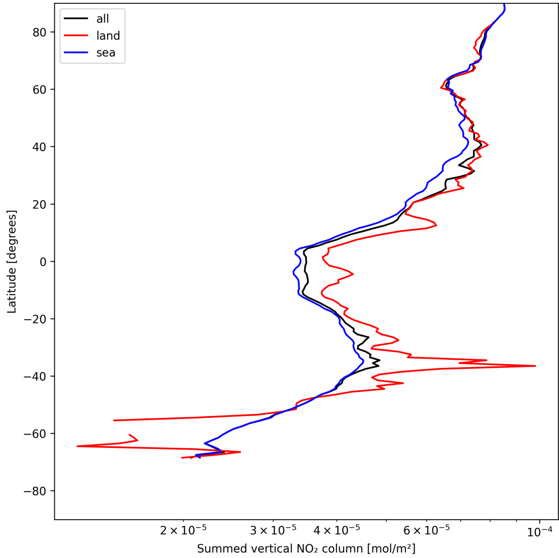
Figure 21: Zonal average of “Summed vertical NO 2 column” for 2025-05-15 to 2025-05-16.
