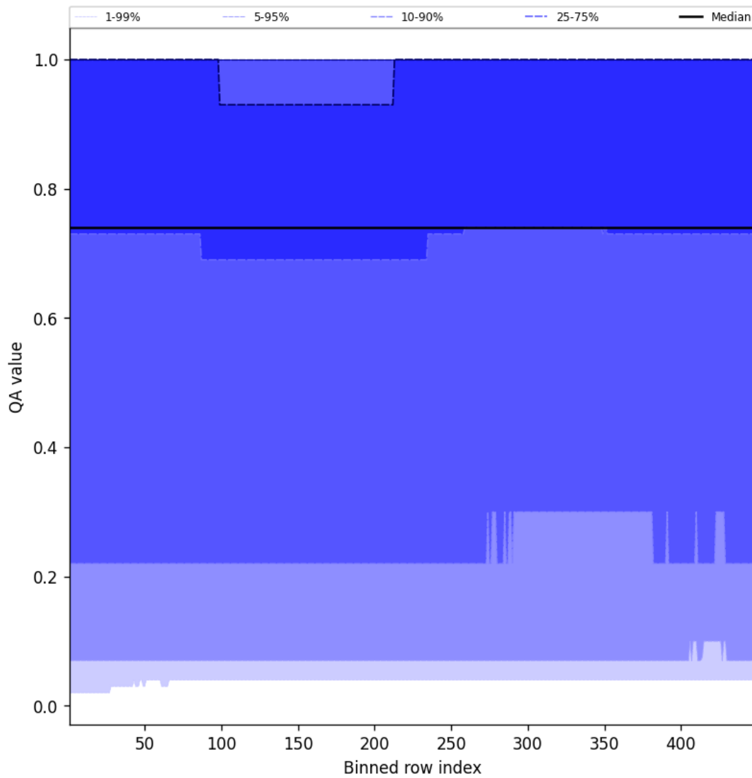
Figure 43: Along track statistics of "QA value" for 2025-05-15 to 2025-05-16
