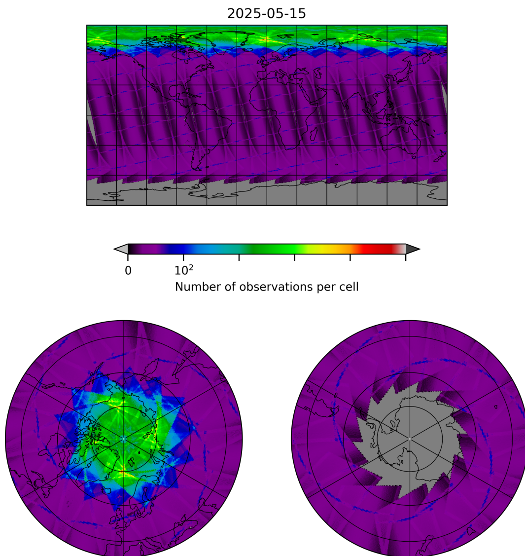
Figure 8: Map of the number of observations for 2025-05-15 to 2025-05-16
