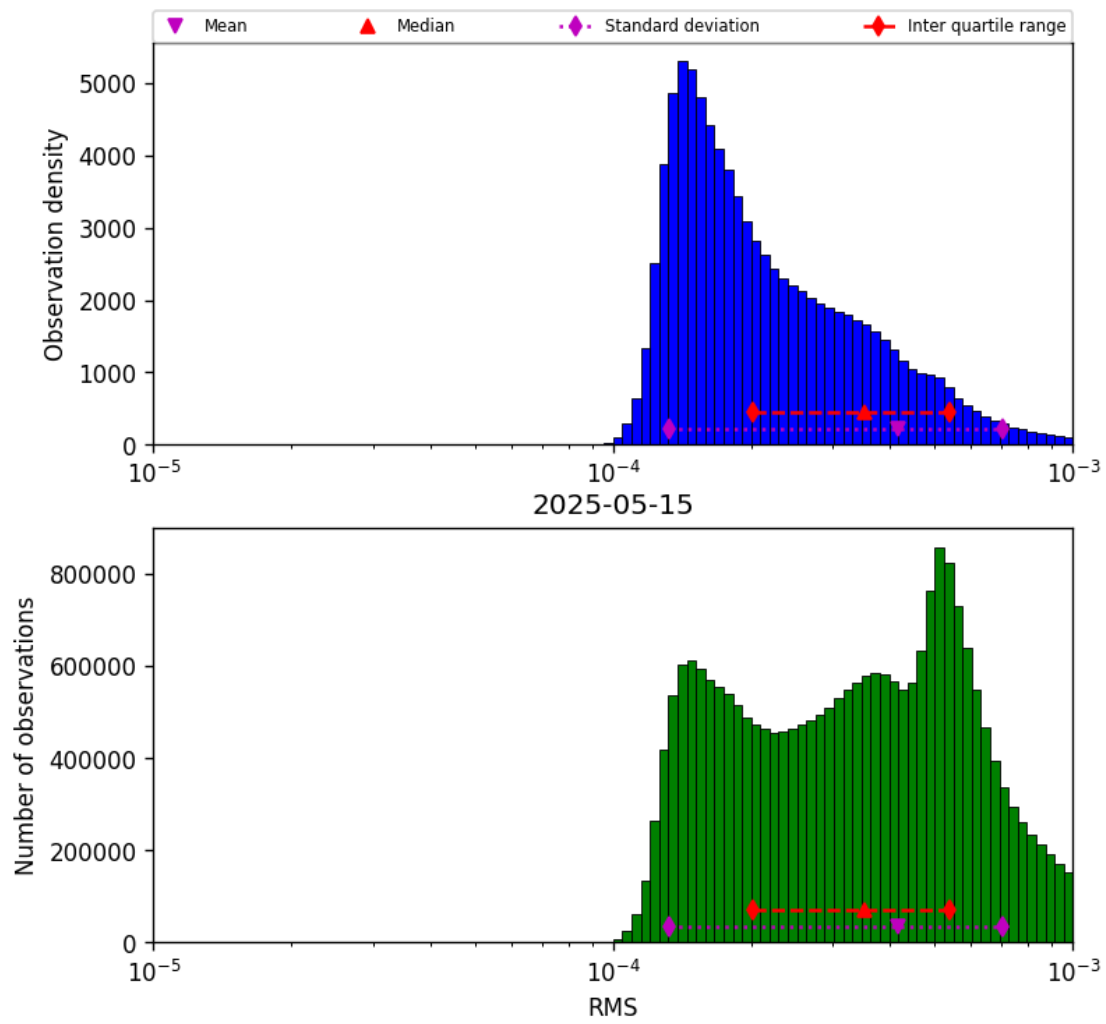
Figure 41: Histogram of “RMS” for 2025-05-15 to 2025-05-16
