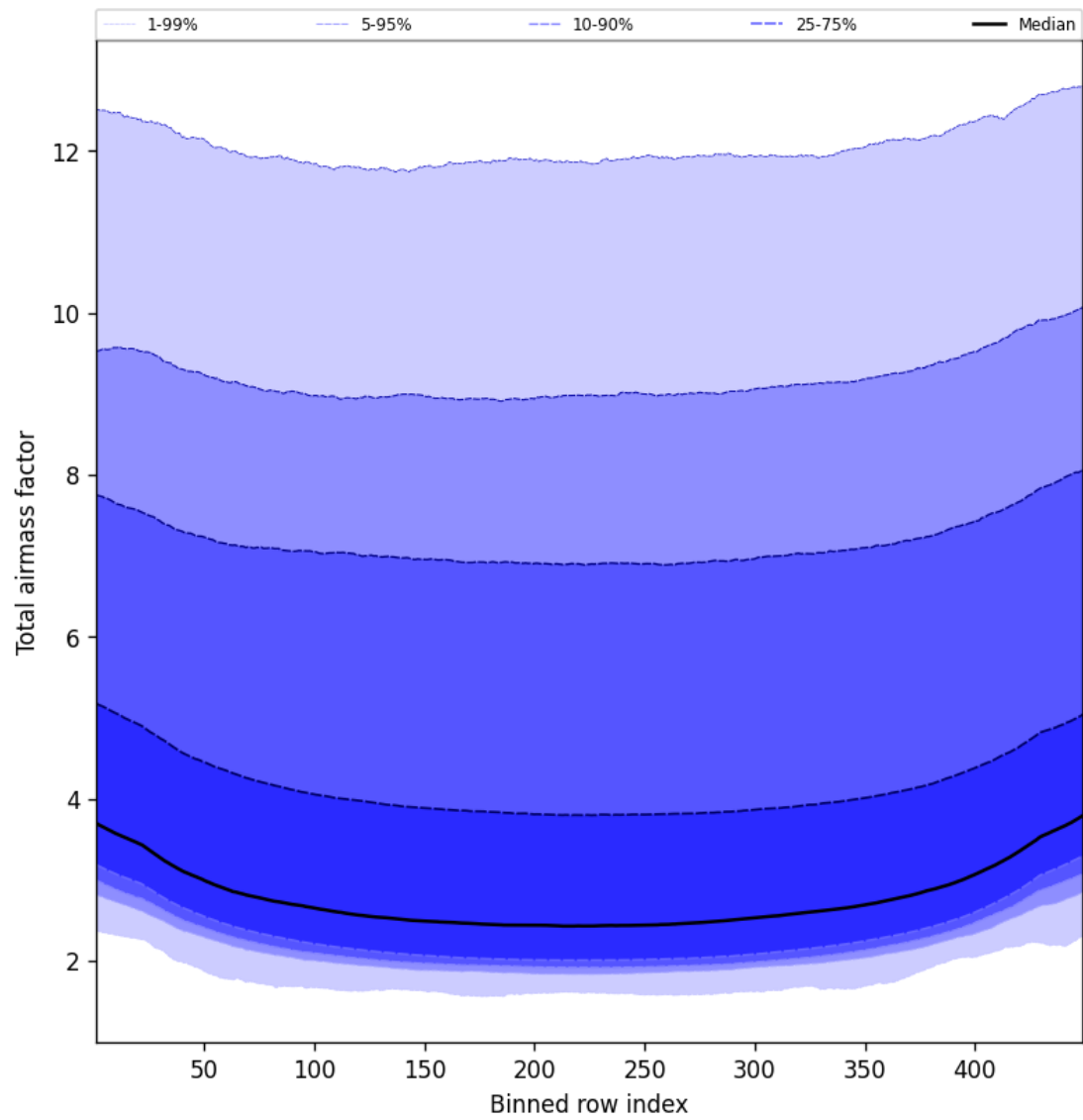
Figure 47: Along track statistics of “Total airmass factor” for 2025-05-16 to 2025-05-17
