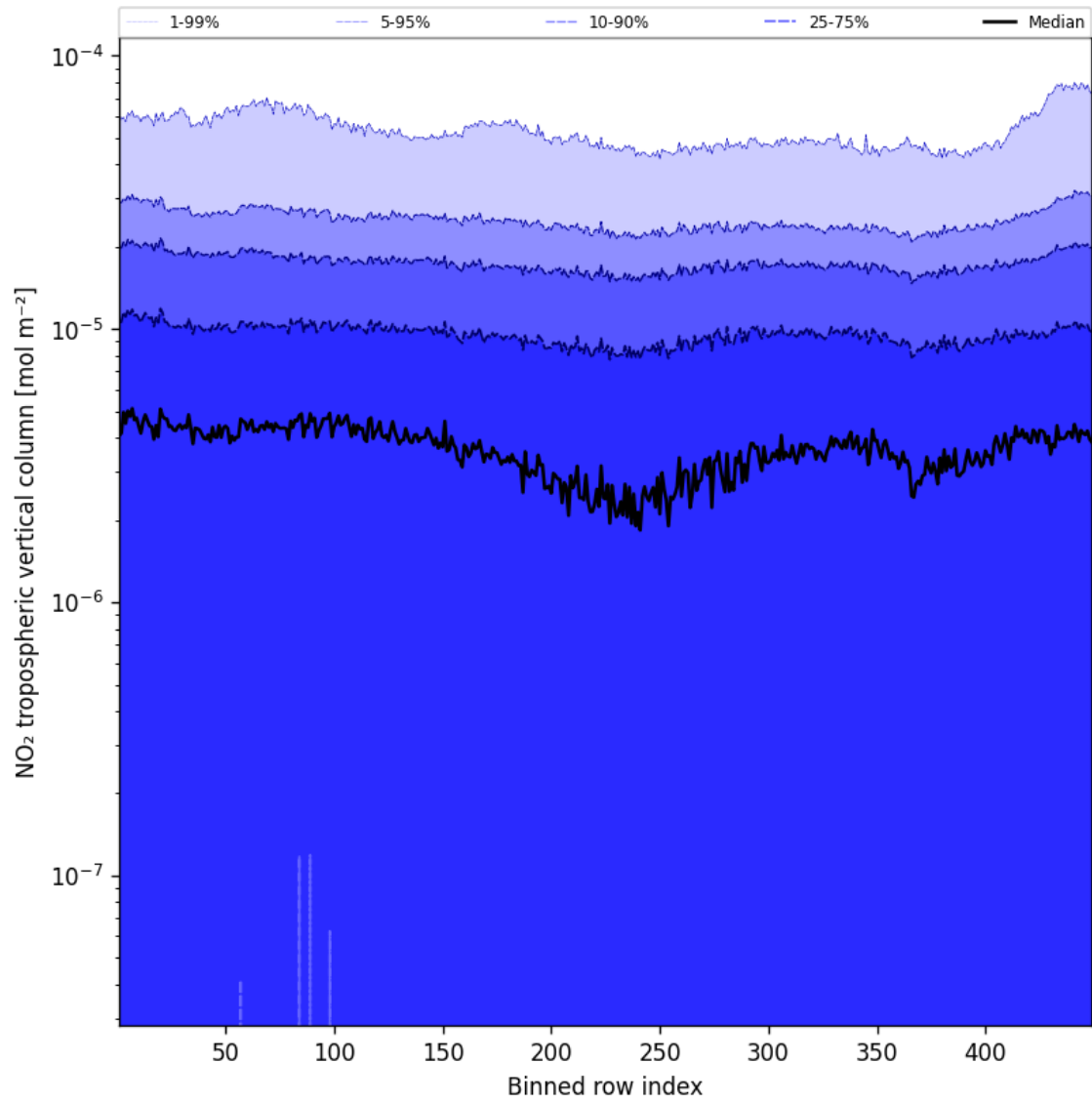
Figure 44: Along track statistics of “NO 2 tropospheric vertical column” for 2025-05-16 to 2025-05-17
