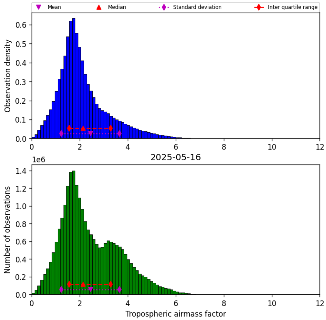
Figure 29: Histogram of “Tropospheric airmass factor” for 2025-05-16 to 2025-05-17
