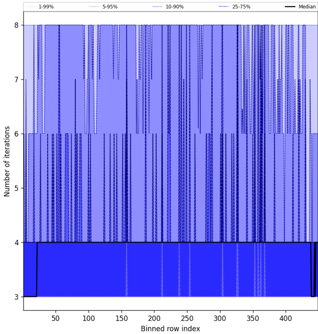
Figure 49: Along track statistics of “Number of iterations” for 2025-05-16 to 2025-05-17
