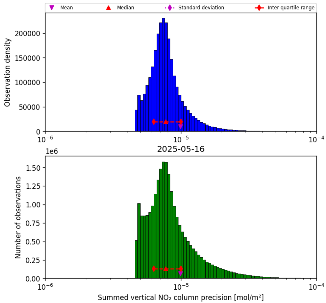
Figure 39: Histogram of “Summed vertical NO 2 column precision” for 2025-05-16 to 2025-05-17
