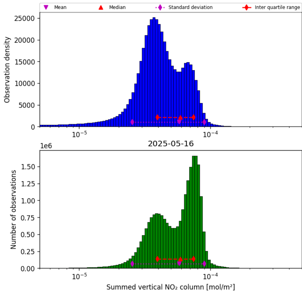
Figure 38: Histogram of “Summed vertical NO 2 column” for 2025-05-16 to 2025-05-17
