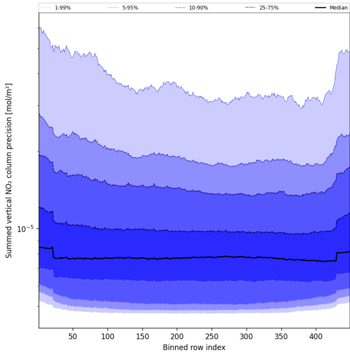
Figure 56: Along track statistics of “Summed vertical NO 2 column precision” for 2025-05-16 to 2025-05-17
