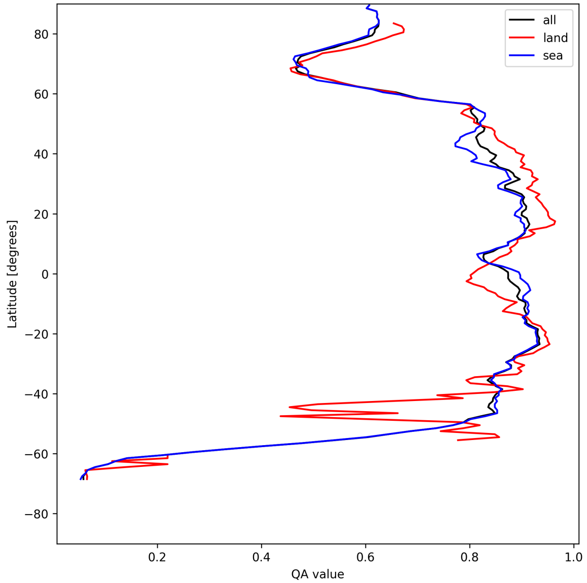
Figure 9: Zonal average of “QA value” for 2025-05-16 to 2025-05-17.
