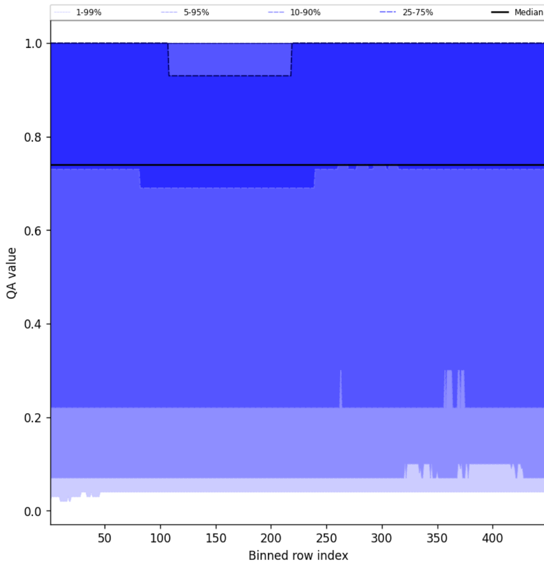
Figure 43: Along track statistics of “QA value” for 2025-05-16 to 2025-05-17
