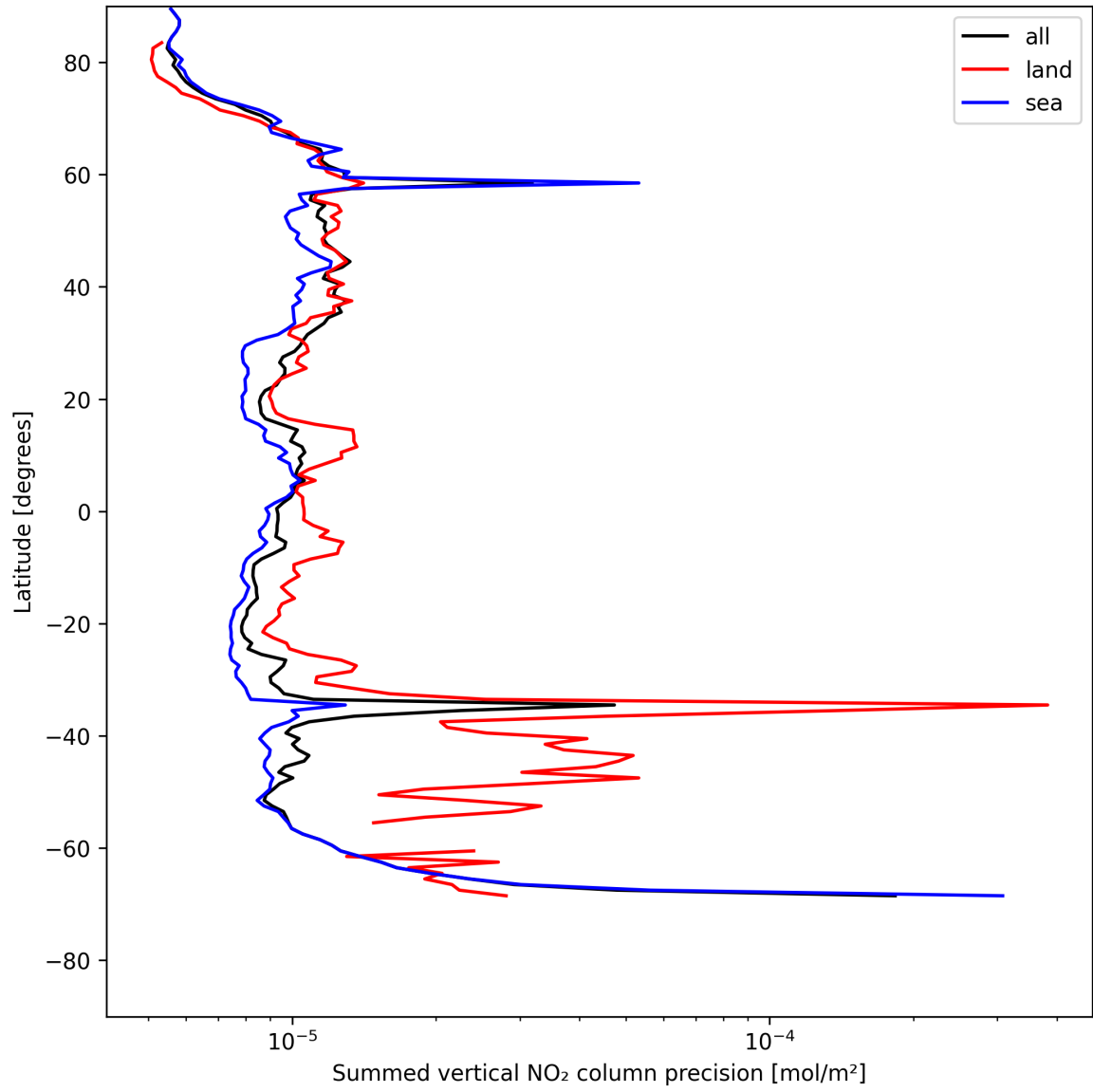
Figure 22: Zonal average of “Summed vertical NO 2 column precision” for 2025-05-16 to 2025-05-17.
