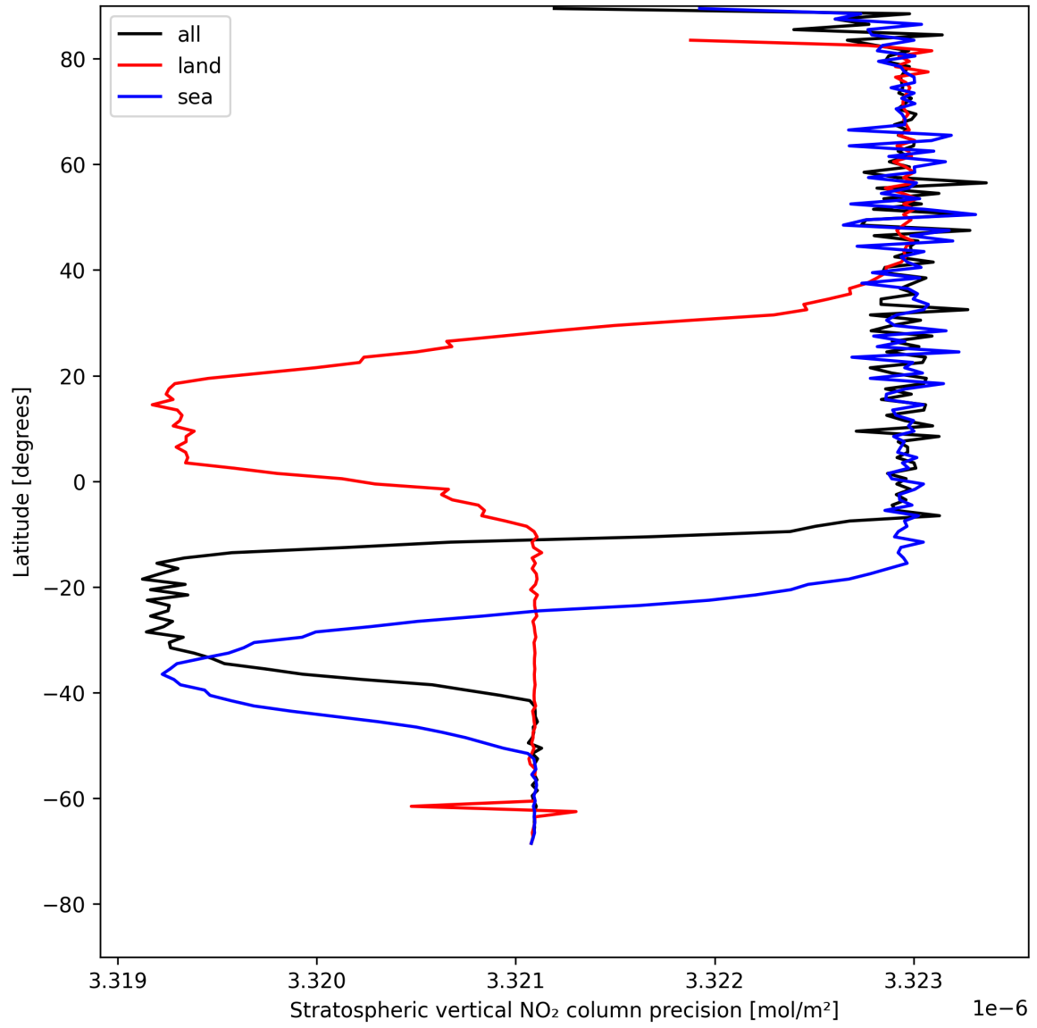
Figure 18: Zonal average of “Stratospheric vertical NO 2 column precision” for 2025-05-16 to 2025-05-17.
