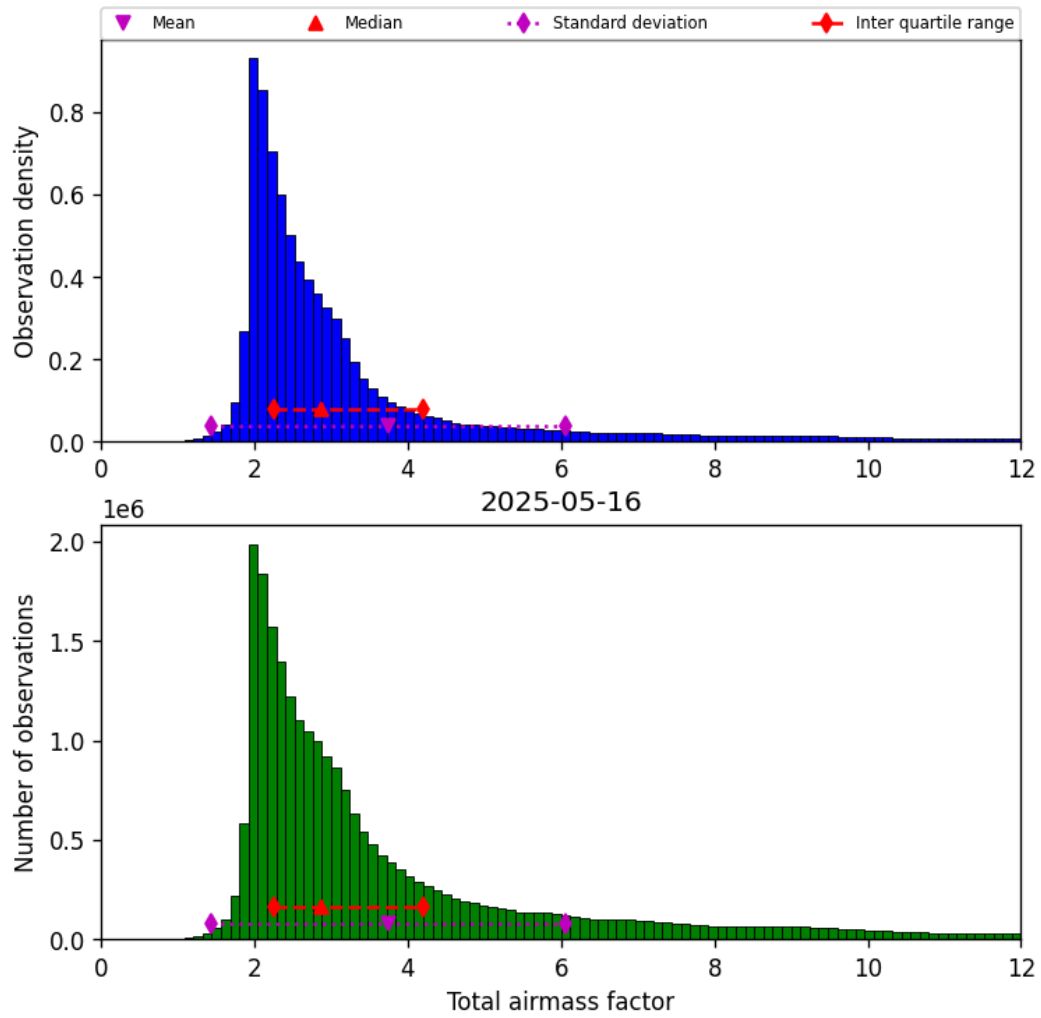
Figure 30: Histogram of “Total airmass factor” for 2025-05-16 to 2025-05-17
