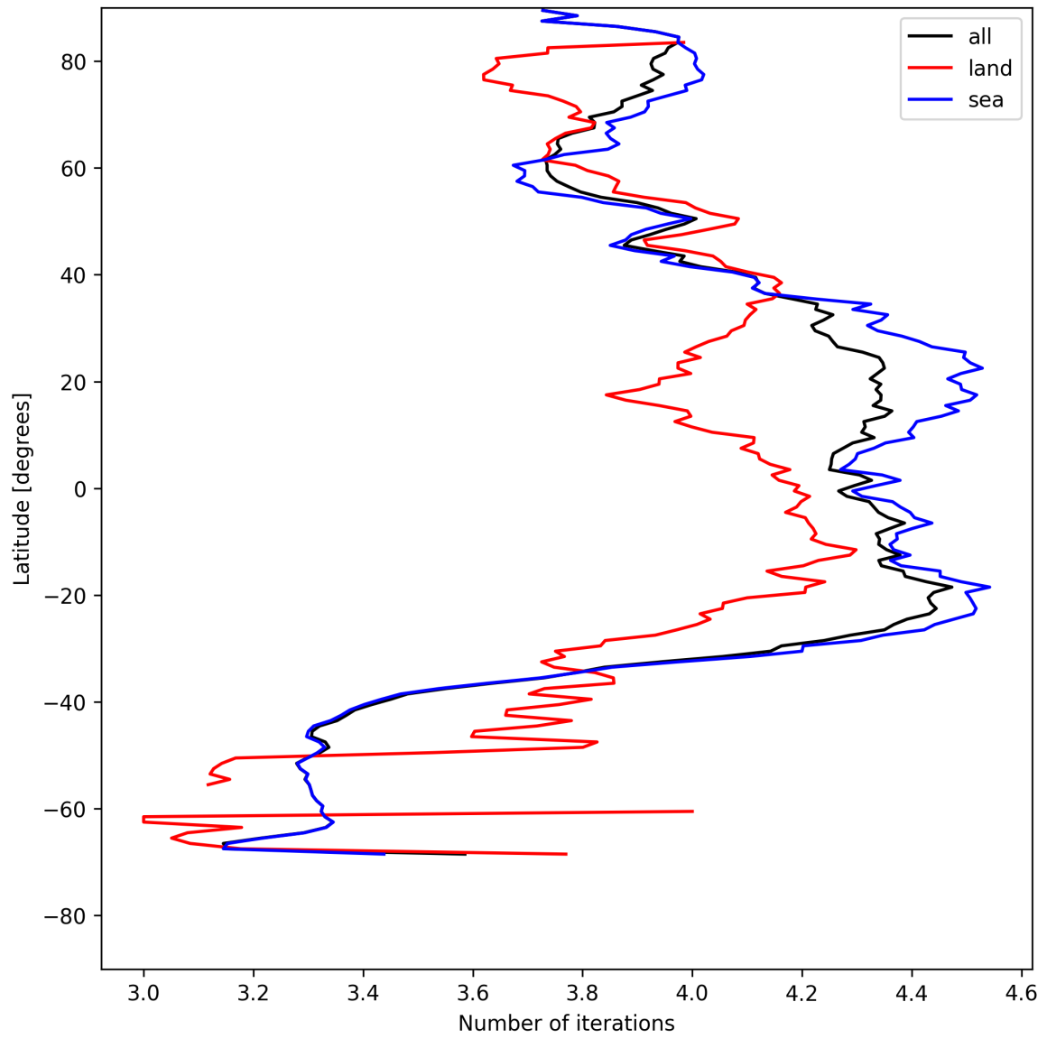
Figure 15: Zonal average of “Number of iterations” for 2025-05-16 to 2025-05-17.
