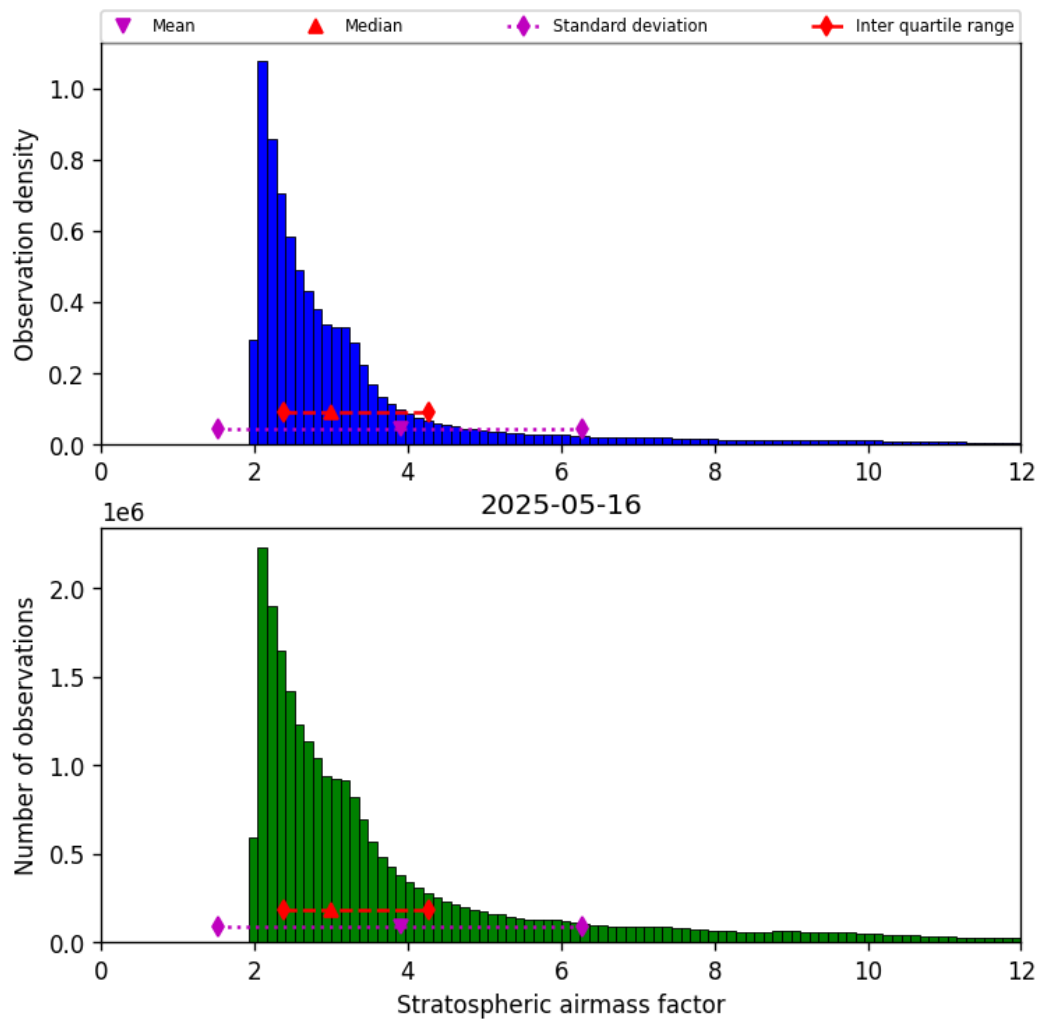
Figure 42: Histogram of “Stratospheric airmass factor” for 2025-05-16 to 2025-05-17
