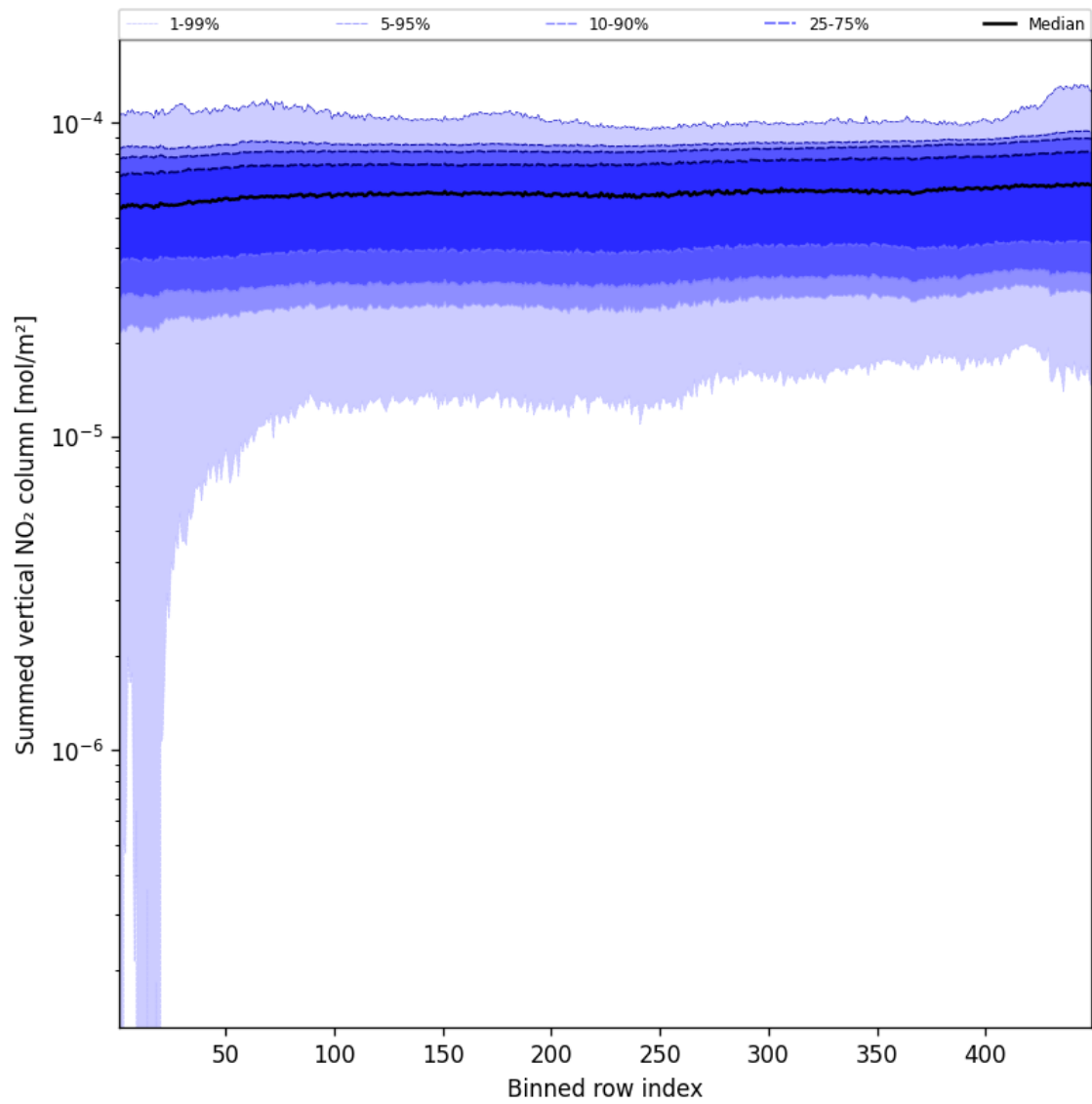
Figure 55: Along track statistics of “Summed vertical NO 2 column” for 2025-05-16 to 2025-05-17
