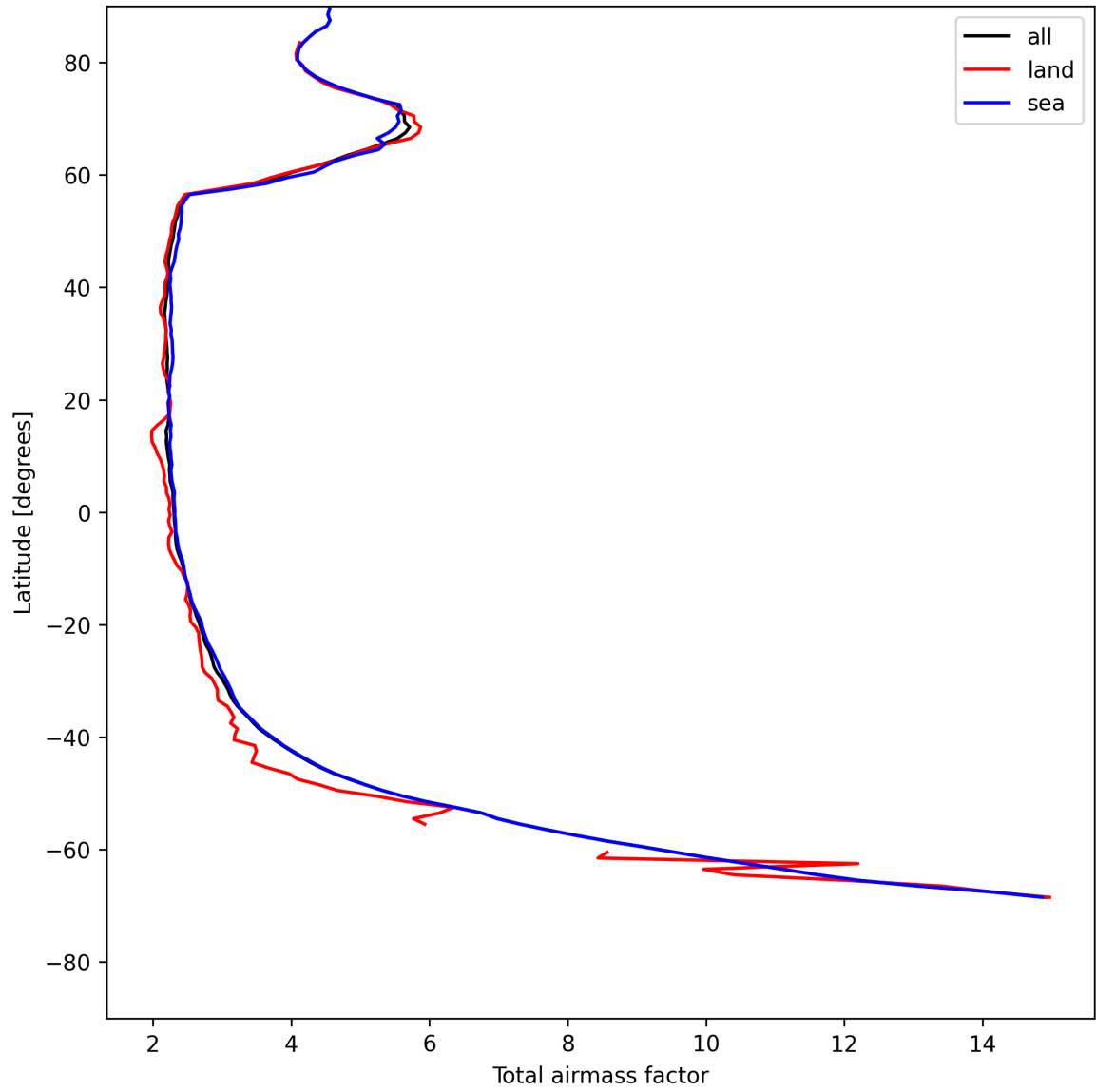
Figure 13: Zonal average of “Total airmass factor” for 2025-05-16 to 2025-05-17.
