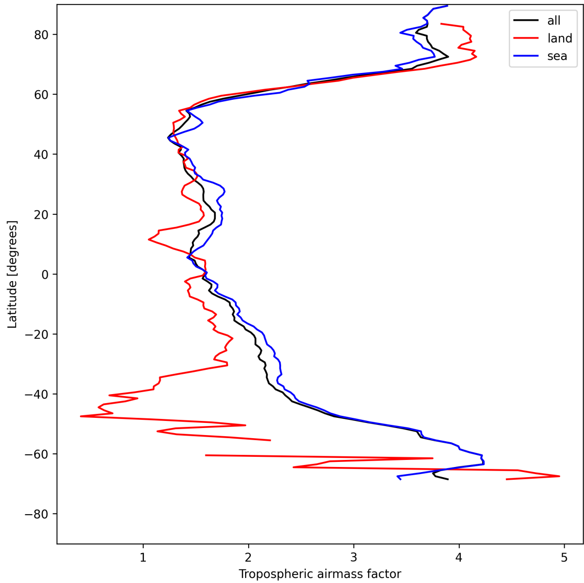
Figure 12: Zonal average of “Tropospheric airmass factor” for 2025-05-16 to 2025-05-17.
