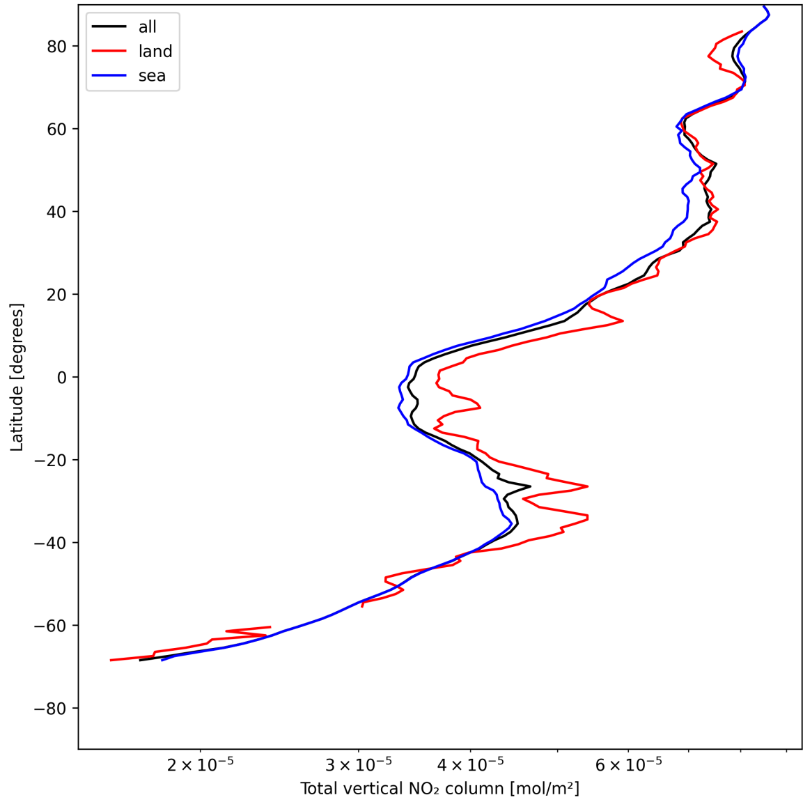
Figure 19: Zonal average of “Total vertical NO 2 column” for 2025-05-16 to 2025-05-17.
