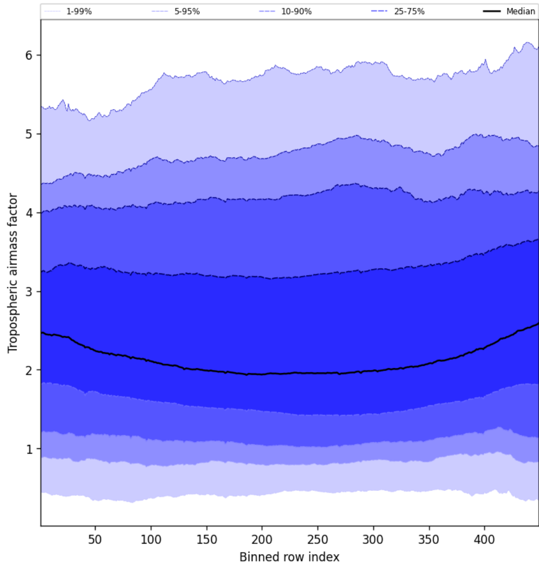
Figure 46: Along track statistics of “Tropospheric airmass factor” for 2025-05-16 to 2025-05-17
