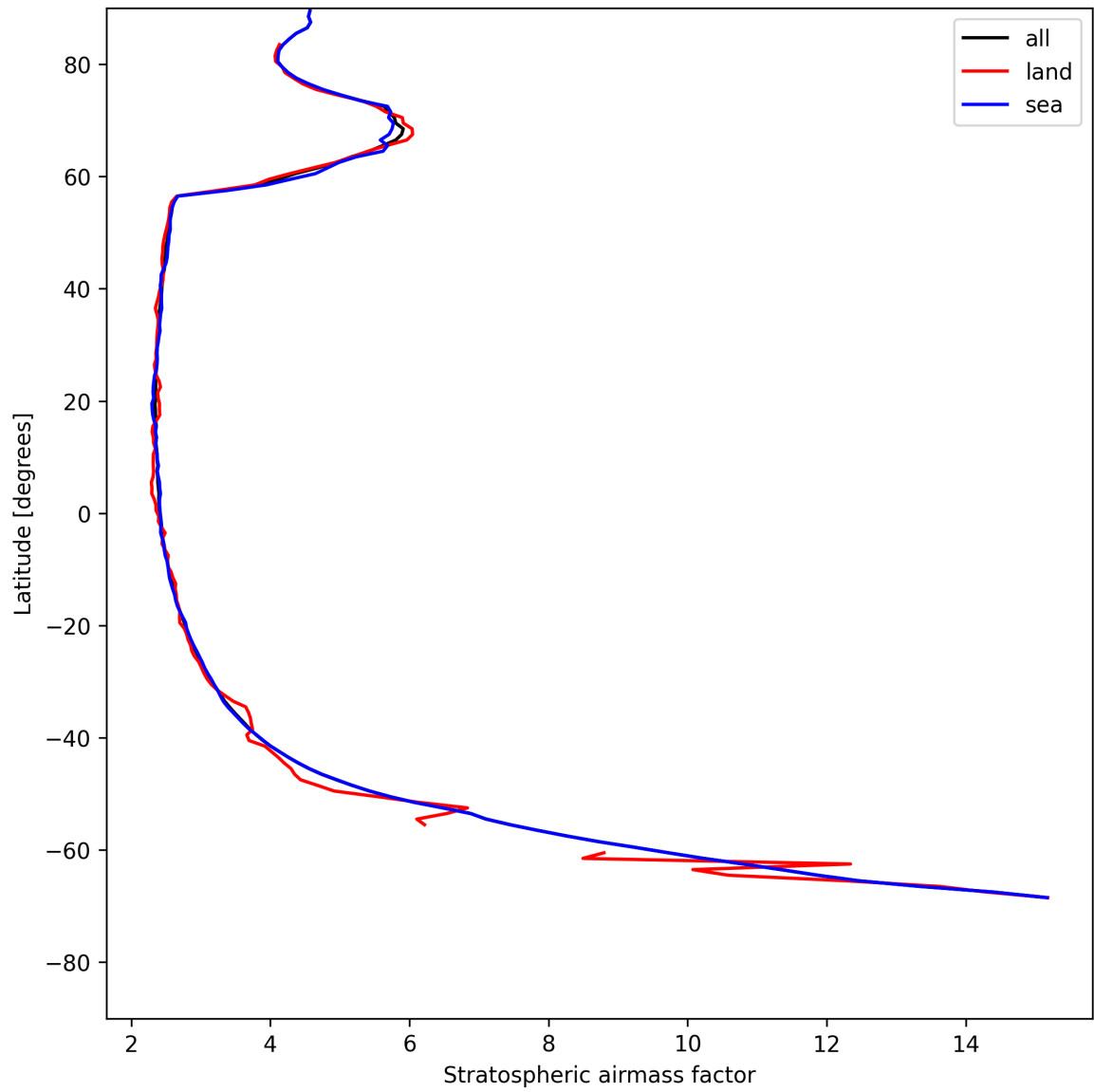
Figure 25: Zonal average of “Stratospheric air mass factor” for 2025-05-16 to 2025-05-17.
