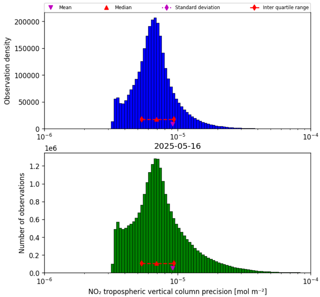
Figure 28: Histogram of “NO 2 tropospheric vertical column precision” for 2025-05-16 to 2025-05-17
