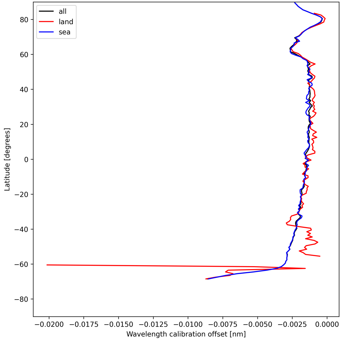
Figure 16: Zonal average of “Wavelength calibration offset” for 2025-05-16 to 2025-05-17.
