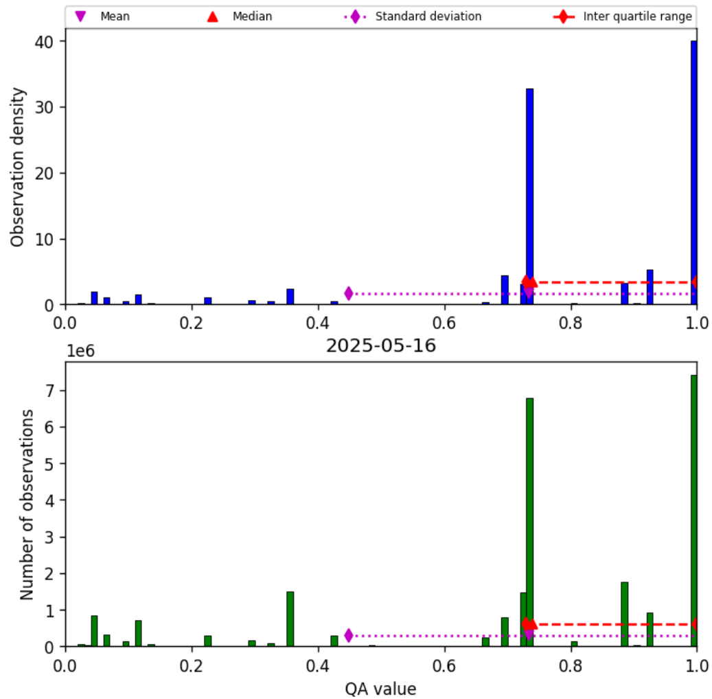
Figure 26: Histogram of “QA value” for 2025-05-16 to 2025-05-17
