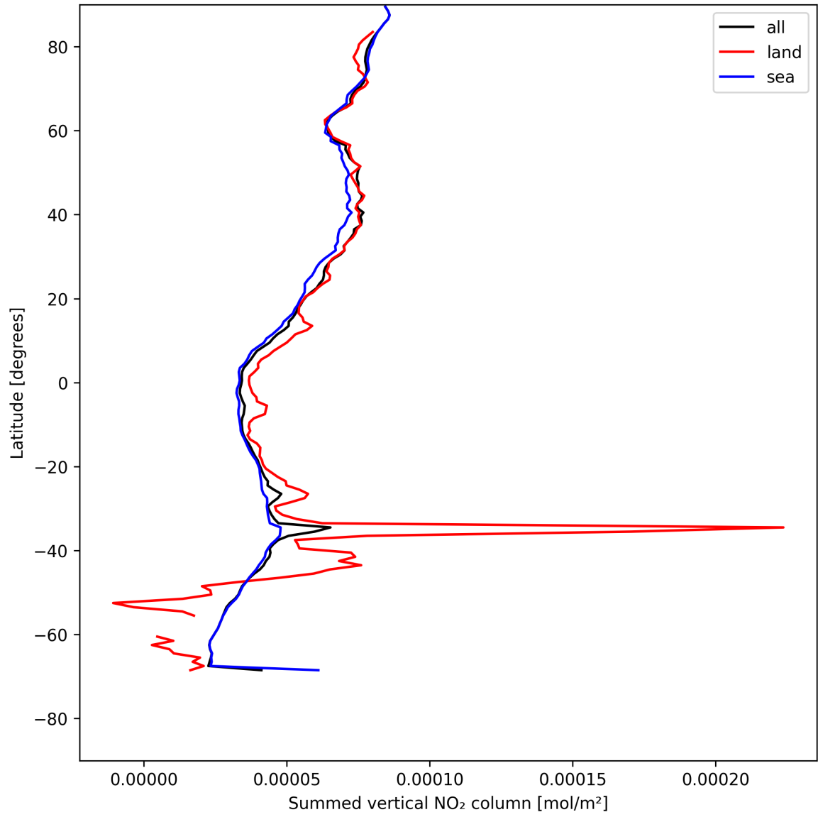
Figure 21: Zonal average of “Summed vertical NO 2 column” for 2025-05-16 to 2025-05-17.
