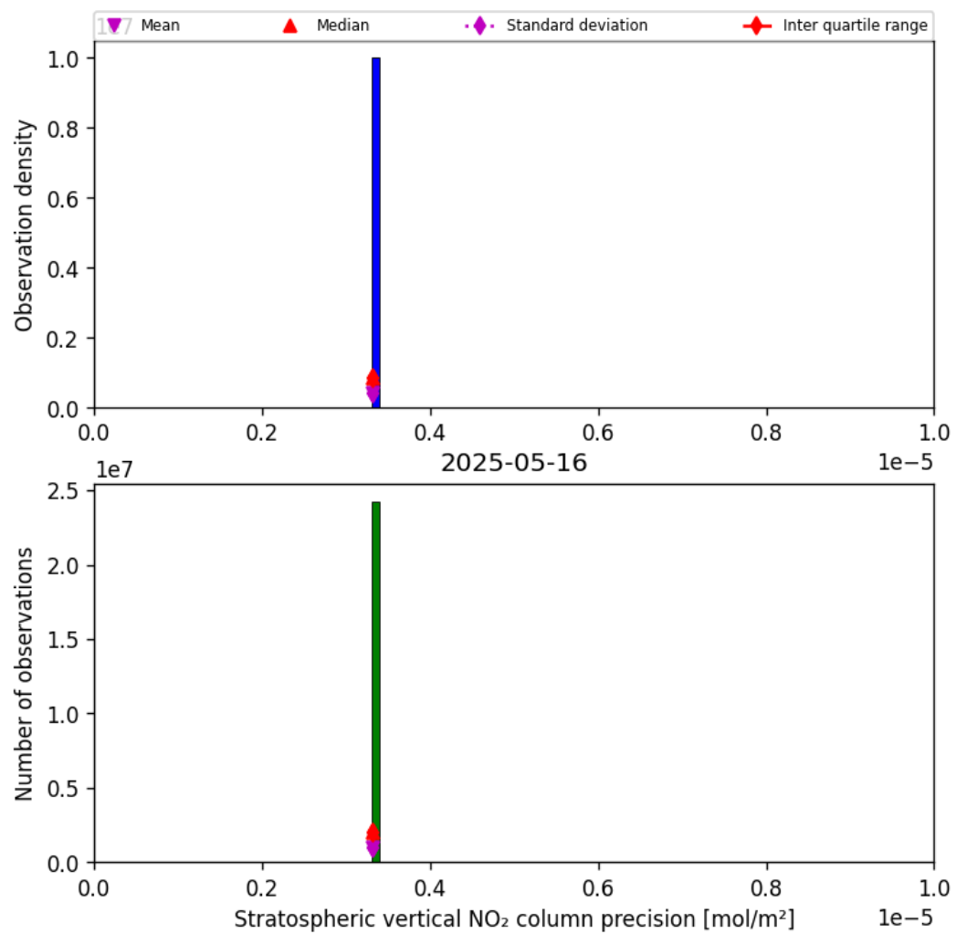
Figure 35: Histogram of “Stratospheric vertical NO 2 column precision” for 2025-05-16 to 2025-05-17
