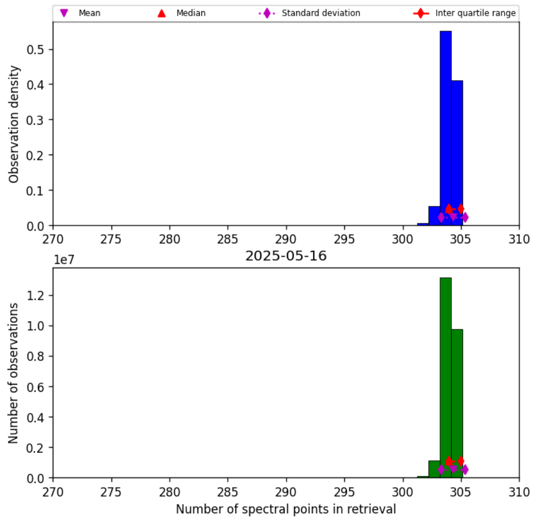
Figure 31: Histogram of “Number of spectral points in retrieval” for 2025-05-16 to 2025-05-17
