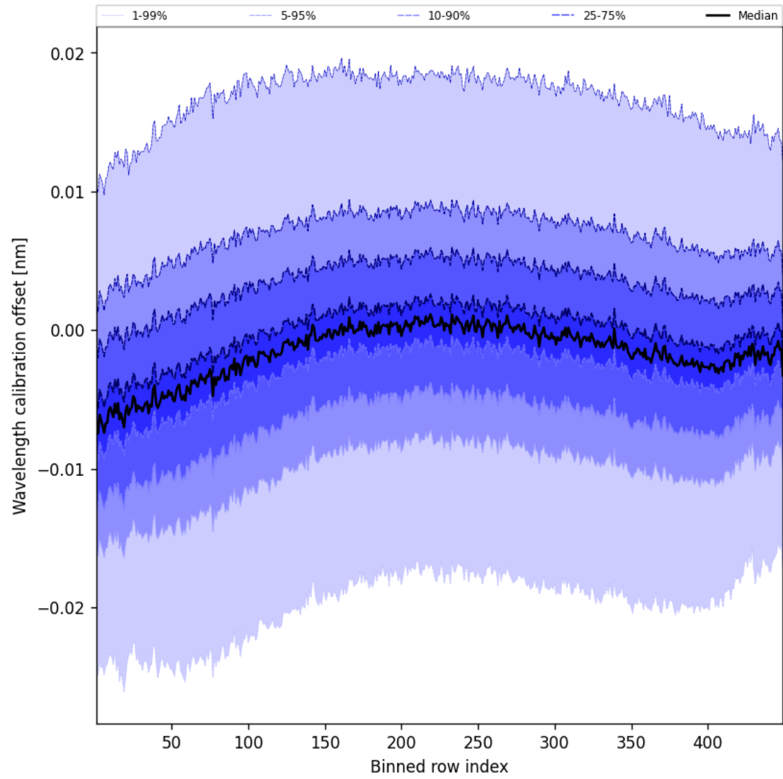
Figure 50: Along track statistics of “Wavelength calibration offset” for 2025-05-16 to 2025-05-17
