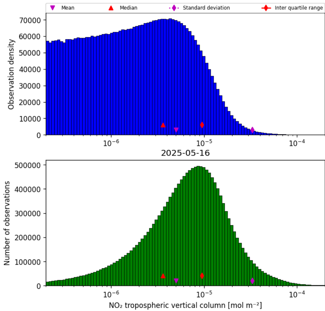
Figure 27: Histogram of “NO 2 tropospheric vertical column” for 2025-05-16 to 2025-05-17
