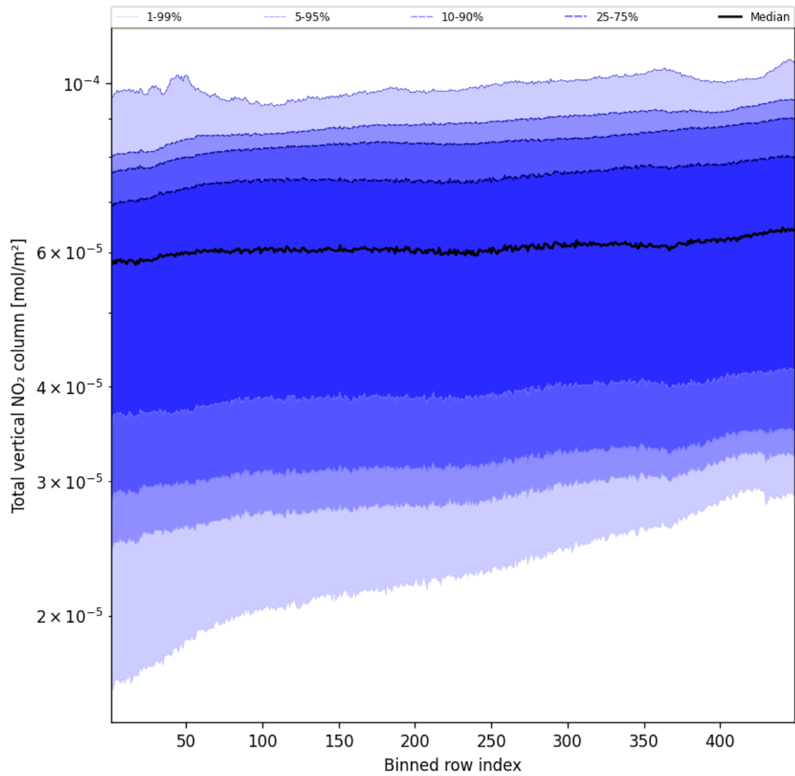
Figure 53: Along track statistics of “Total vertical NO 2 column” for 2025-05-16 to 2025-05-17
