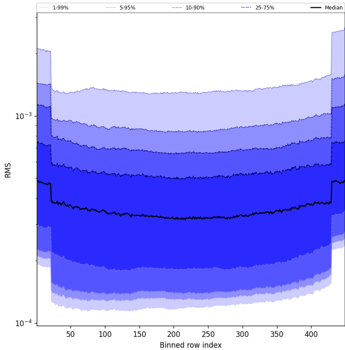
Figure 58: Along track statistics of “RMS” for 2025-05-16 to 2025-05-17
