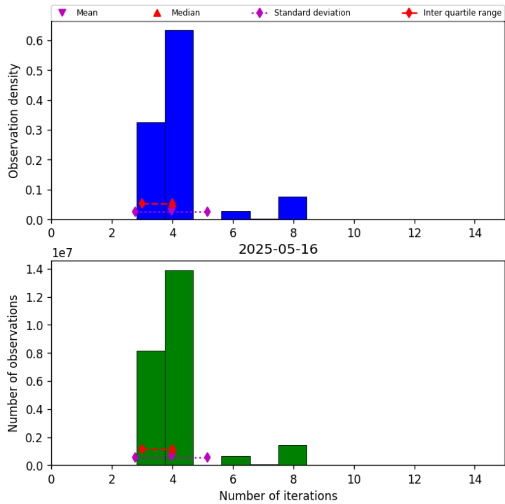
Figure 32: Histogram of “Number of iterations” for 2025-05-16 to 2025-05-17
