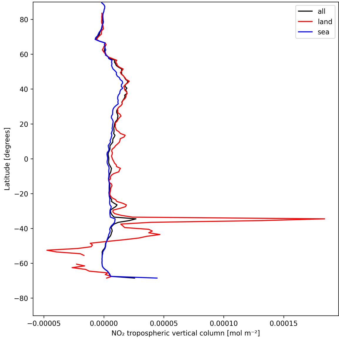
Figure 10: Zonal average of “NO 2 tropospheric vertical column” for 2025-05-16 to 2025-05-17.
