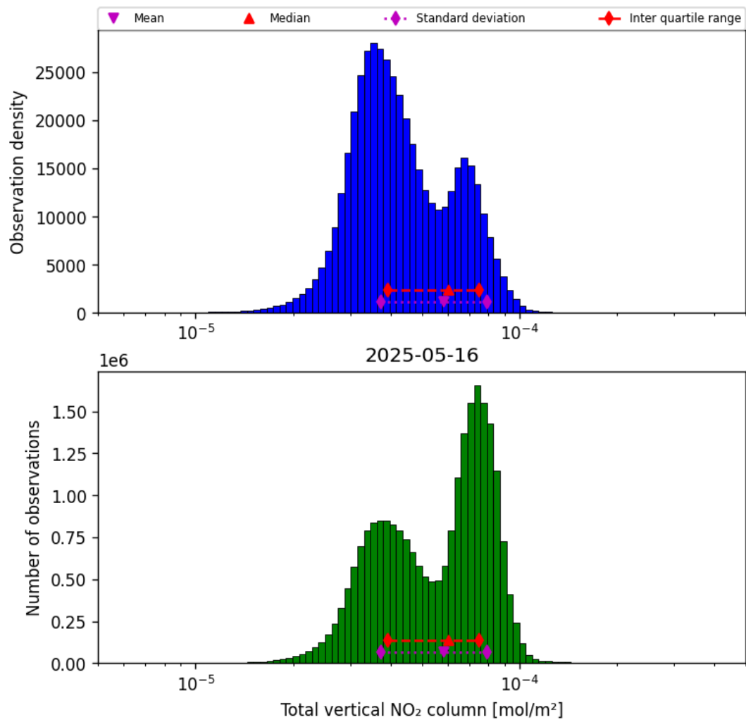
Figure 36: Histogram of "Total vertical NO 2 column" for 2025-05-16 to 2025-05-17
