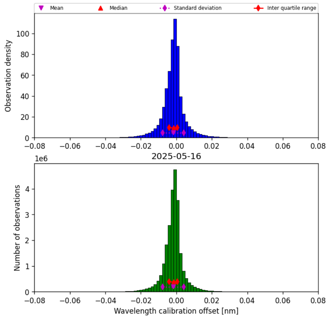
Figure 33: Histogram of “Wavelength calibration offset” for 2025-05-16 to 2025-05-17
