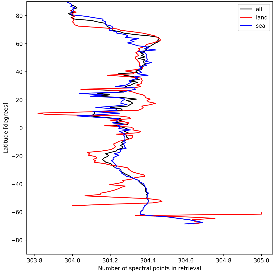
Figure 14: Zonal average of “Number of spectral points in retrieval” for 2025-05-16 to 2025-05-17.
