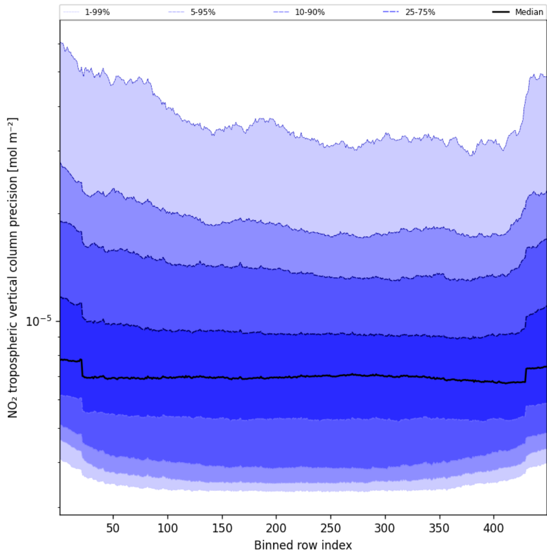
Figure 45: Along track statistics of “NO 2 tropospheric vertical column precision” for 2025-05-16 to 2025-05-17
