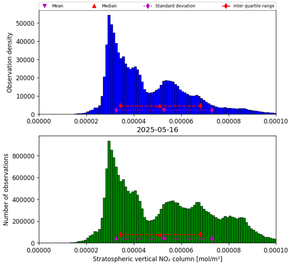
Figure 34: Histogram of “Stratospheric vertical NO 2 column” for 2025-05-16 to 2025-05-17
