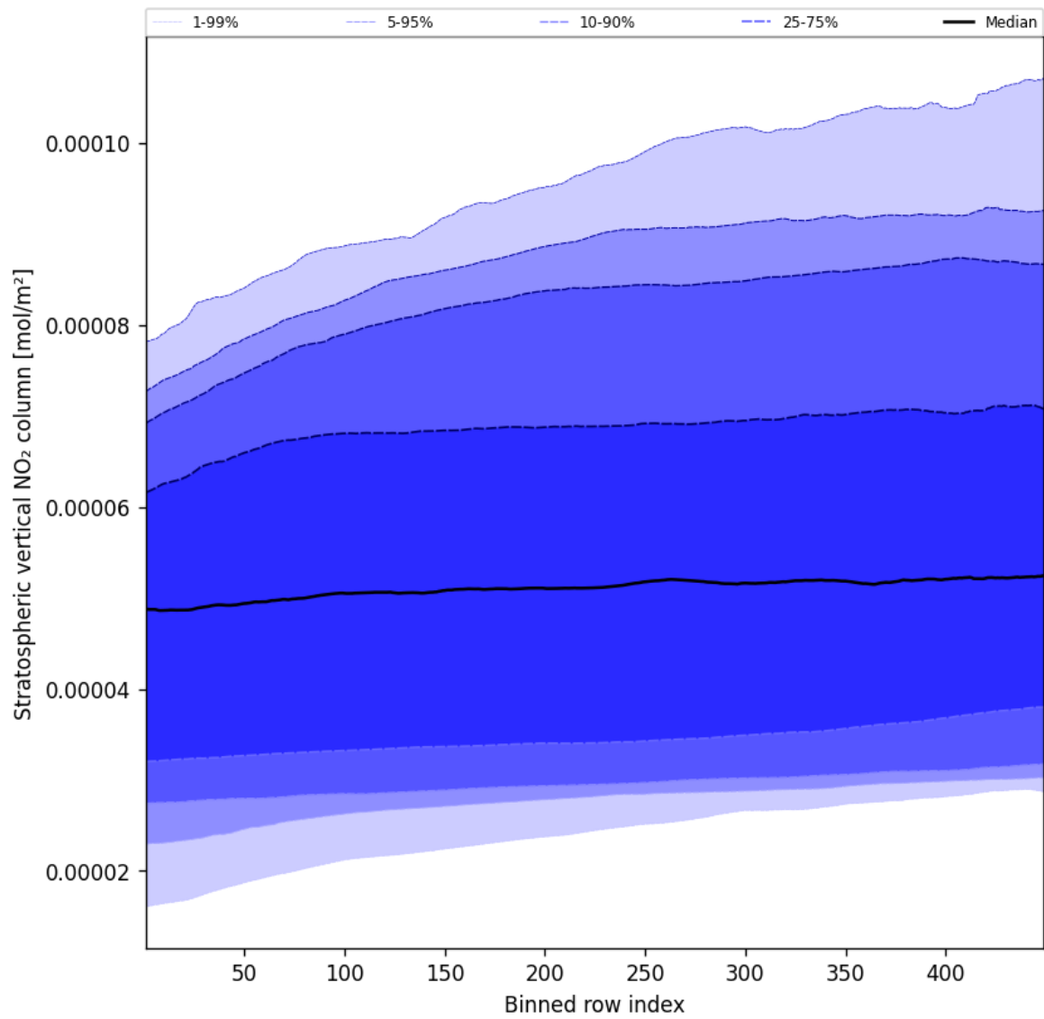
Figure 51: Along track statistics of “Stratospheric vertical NO 2 column” for 2025-05-16 to 2025-05-17
