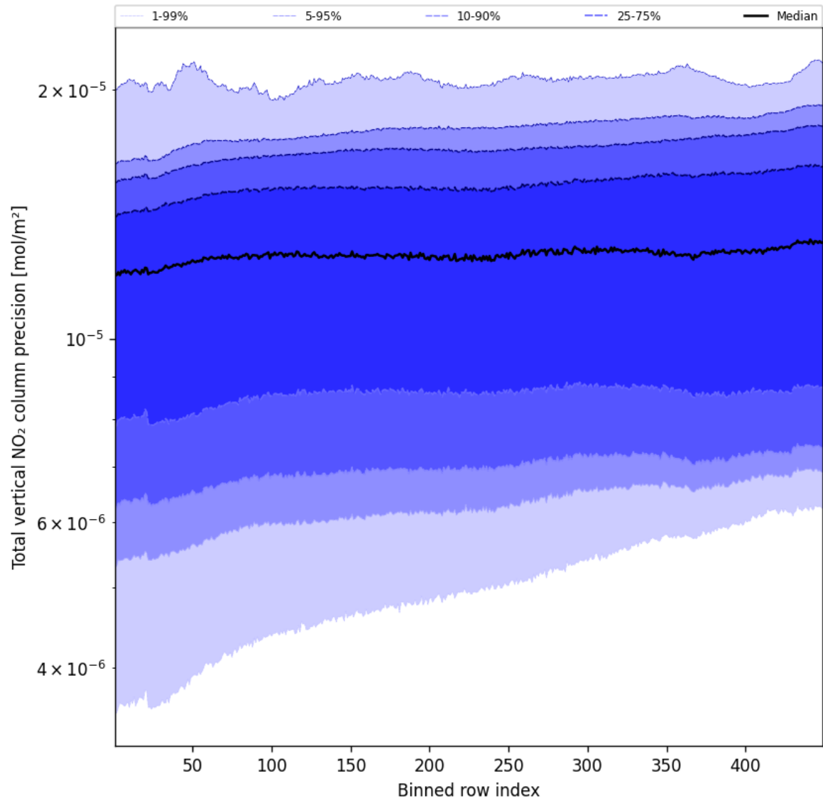
Figure 54: Along track statistics of “Total vertical NO 2 column precision” for 2025-05-16 to 2025-05-17
