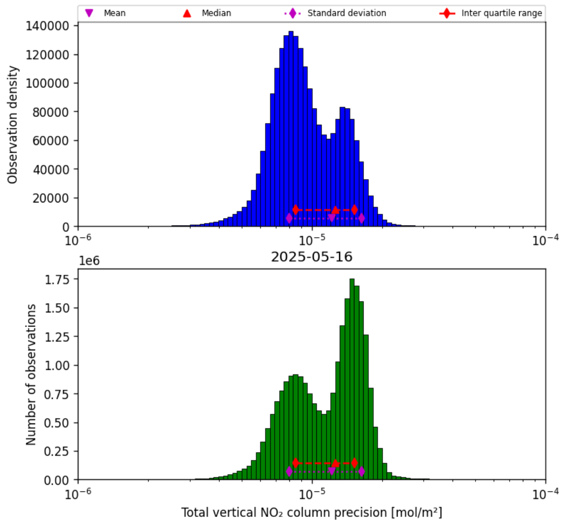
Figure 37: Histogram of “Total vertical NO 2 column precision” for 2025-05-16 to 2025-05-17
