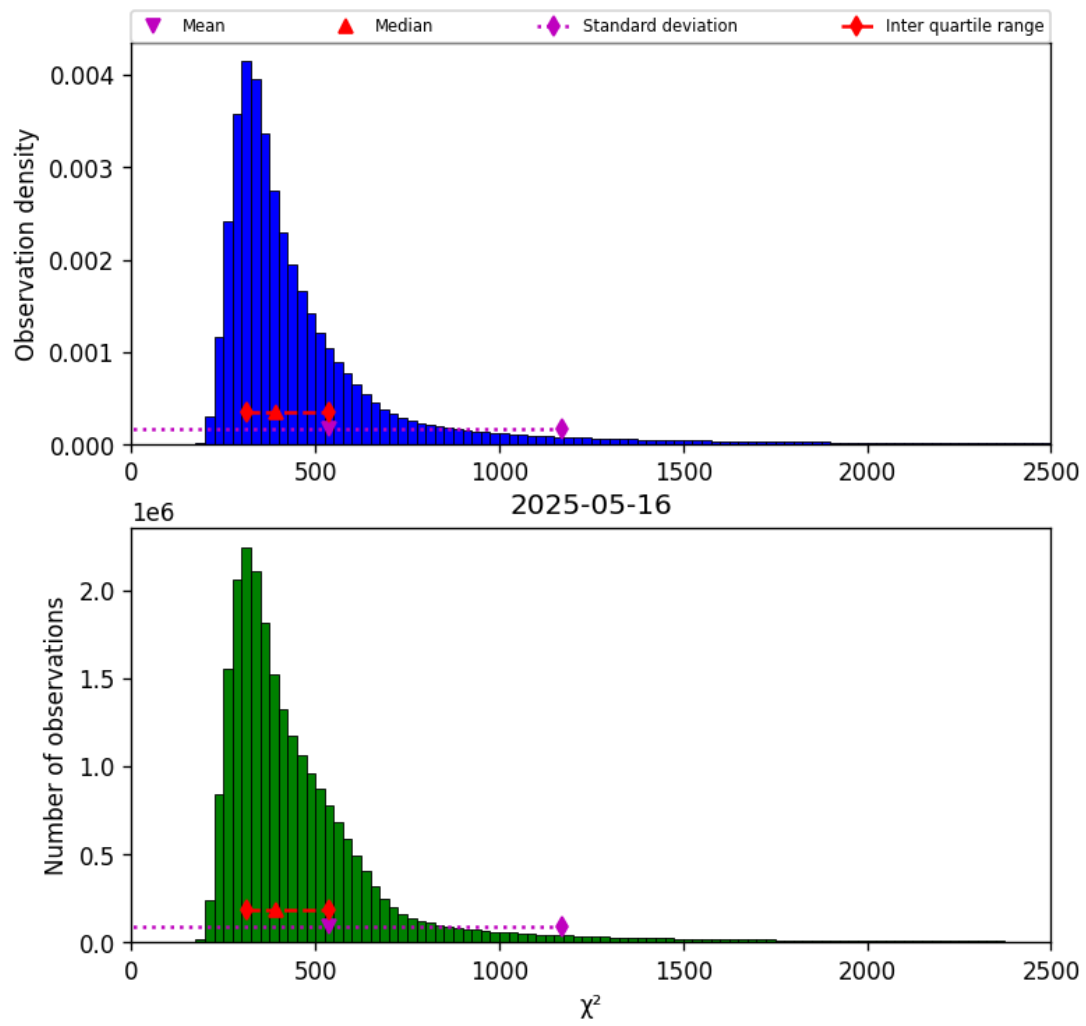
Figure 40: Histogram of “ \chi^2 ” for 2025-05-16 to 2025-05-17
