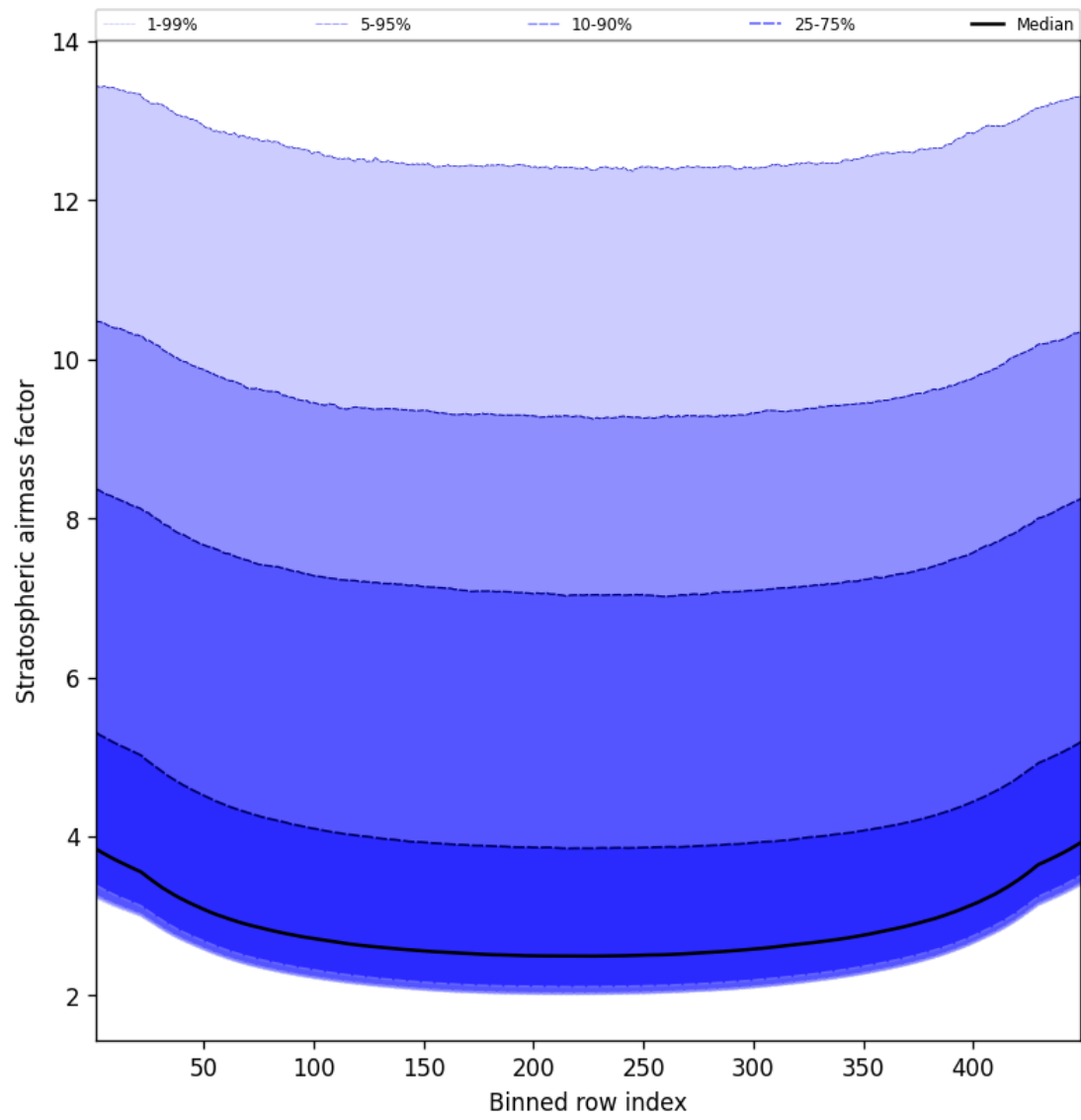
Figure 59: Along track statistics of “Stratospheric airmass factor” for 2025-05-16 to 2025-05-17
