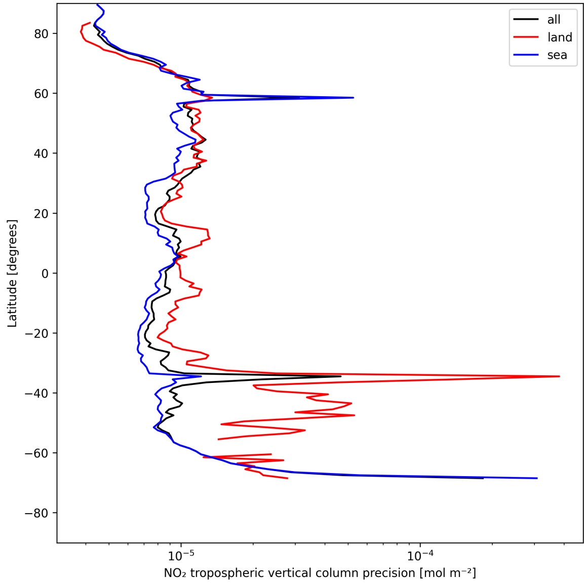
Figure 11: Zonal average of “NO 2 tropospheric vertical column precision” for 2025-05-16 to 2025-05-17.
