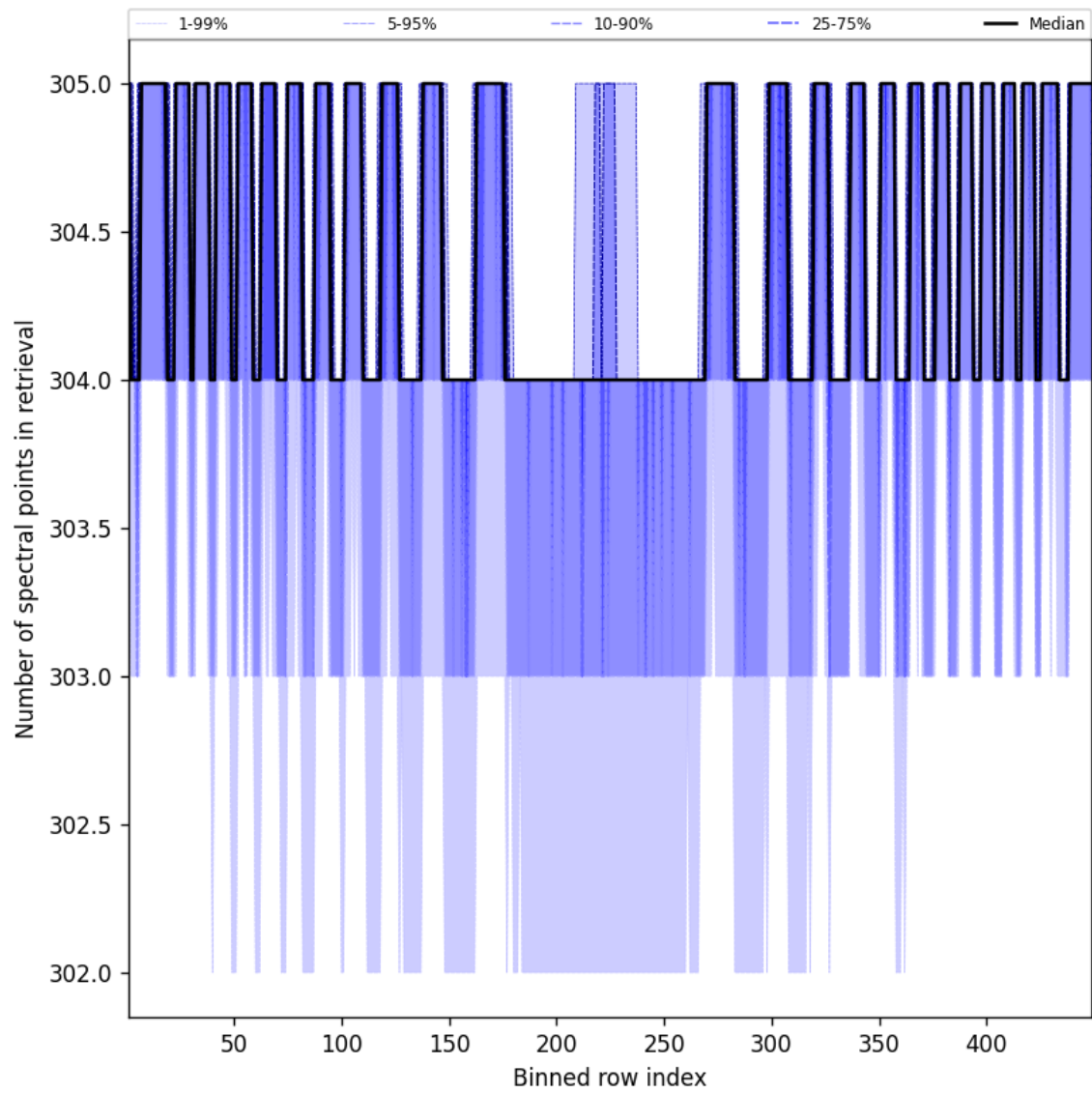
Figure 48: Along track statistics of “Number of spectral points in retrieval” for 2025-05-16 to 2025-05-17
