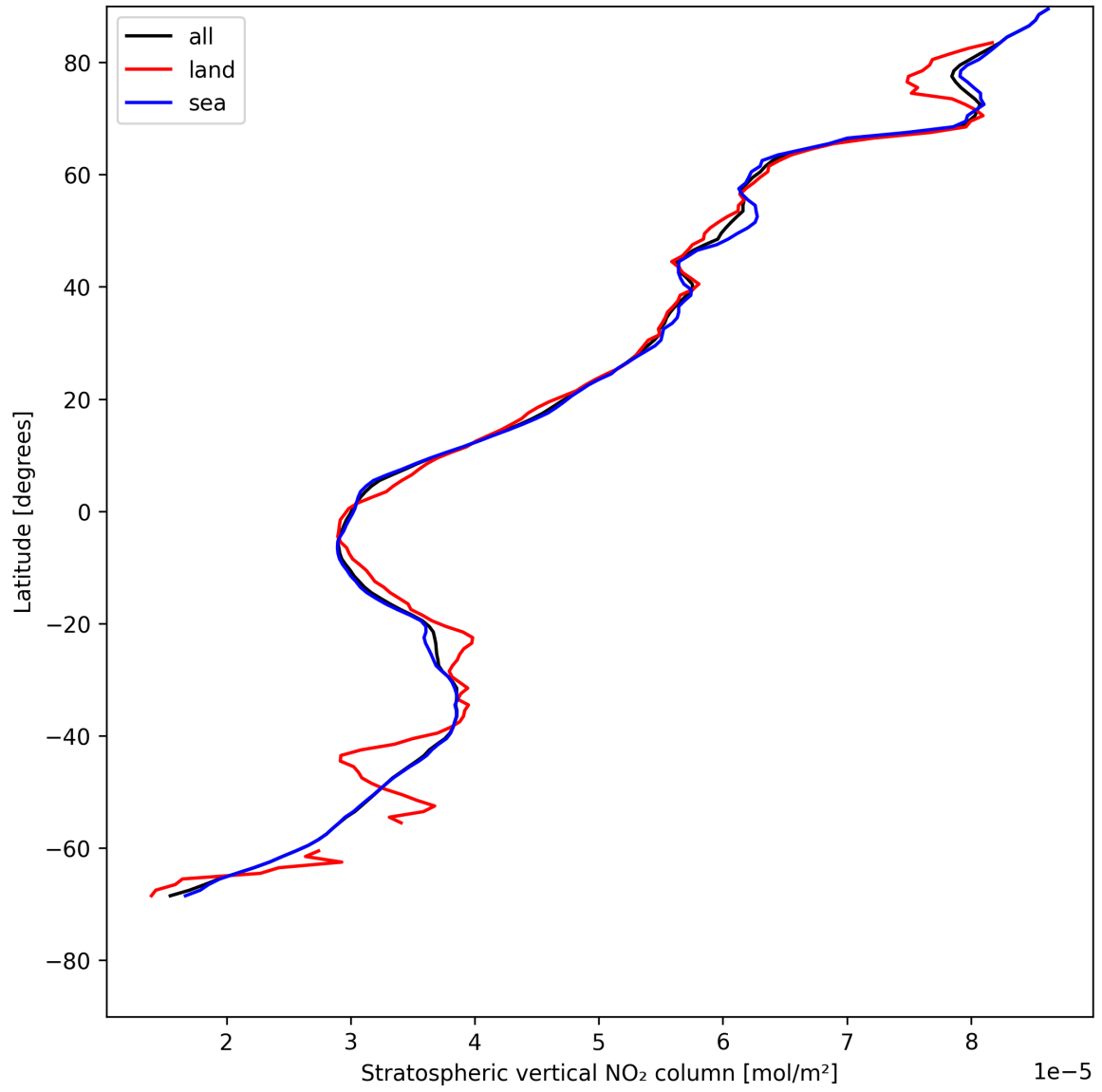
Figure 17: Zonal average of “Stratospheric vertical NO 2 column” for 2025-05-16 to 2025-05-17.
