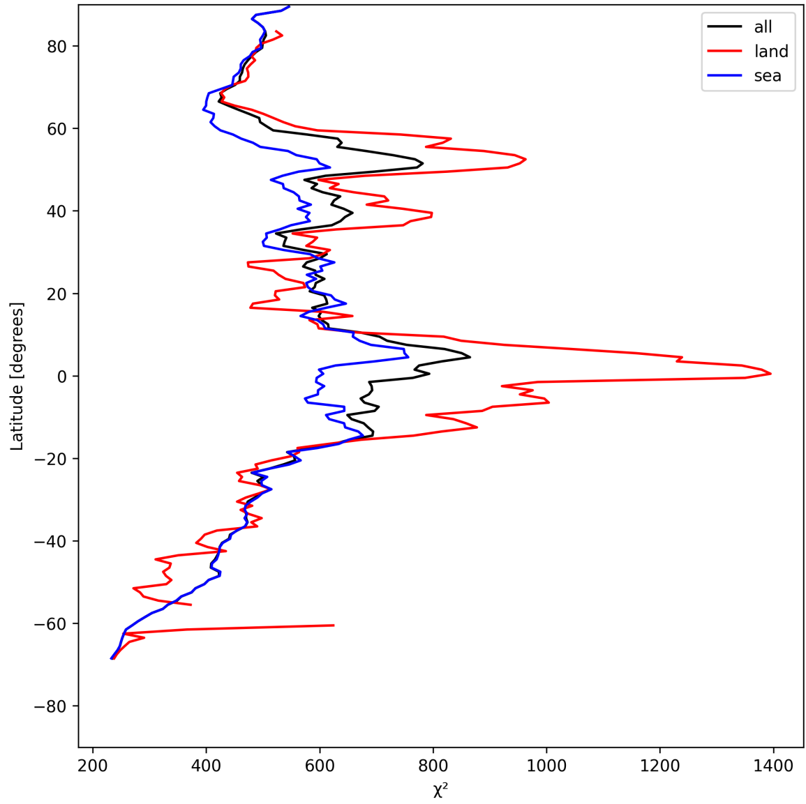
Figure 23: Zonal average of “ \chi^2 ” for 2025-05-16 to 2025-05-17.
