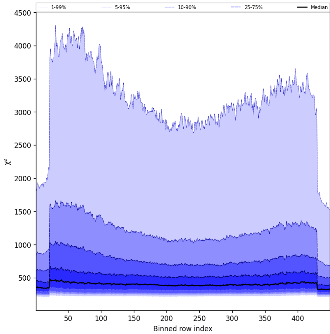
Figure 57: Along track statistics of “ \chi^2 ” for 2025-05-16 to 2025-05-17
