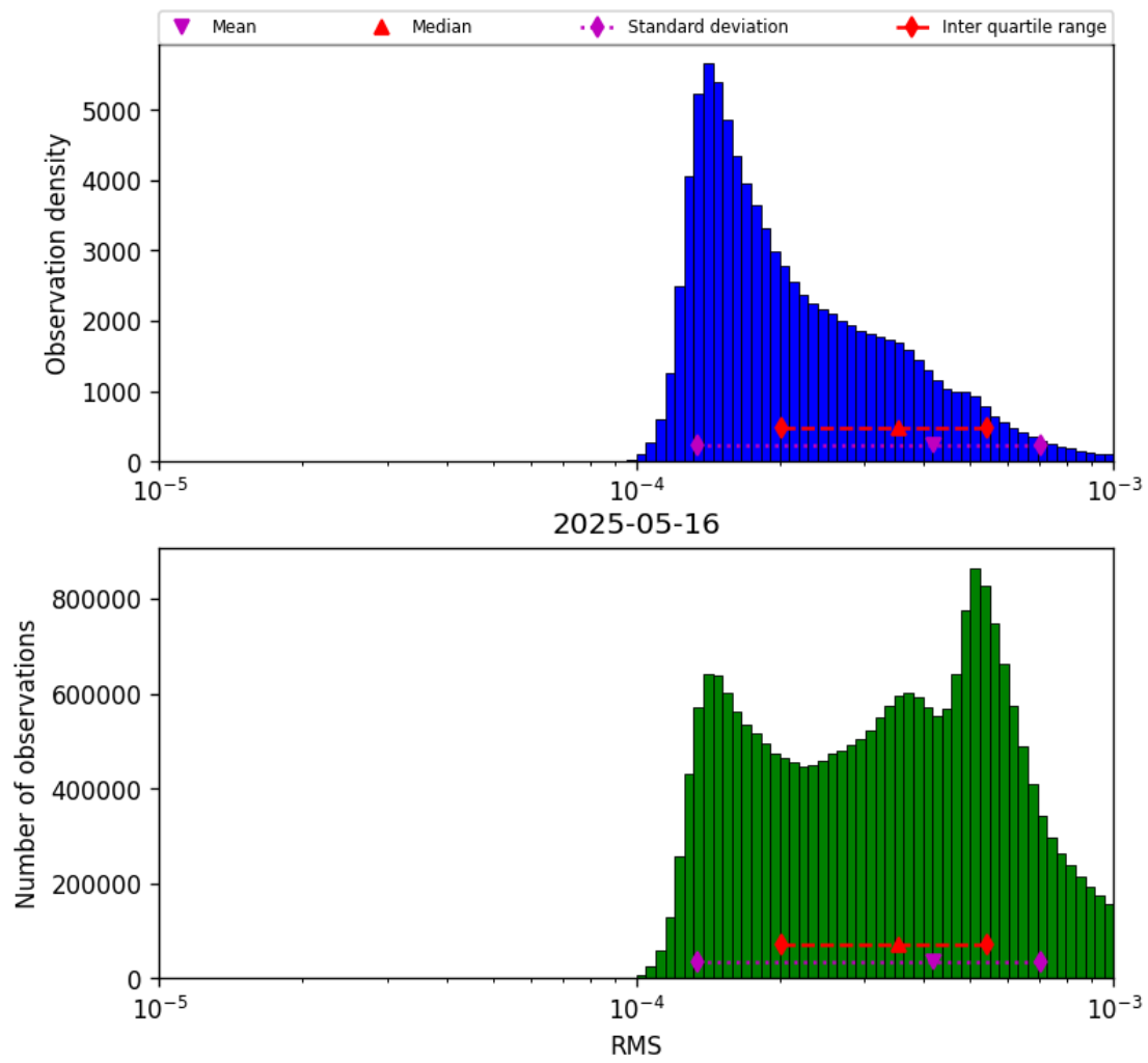
Figure 41: Histogram of “RMS” for 2025-05-16 to 2025-05-17
