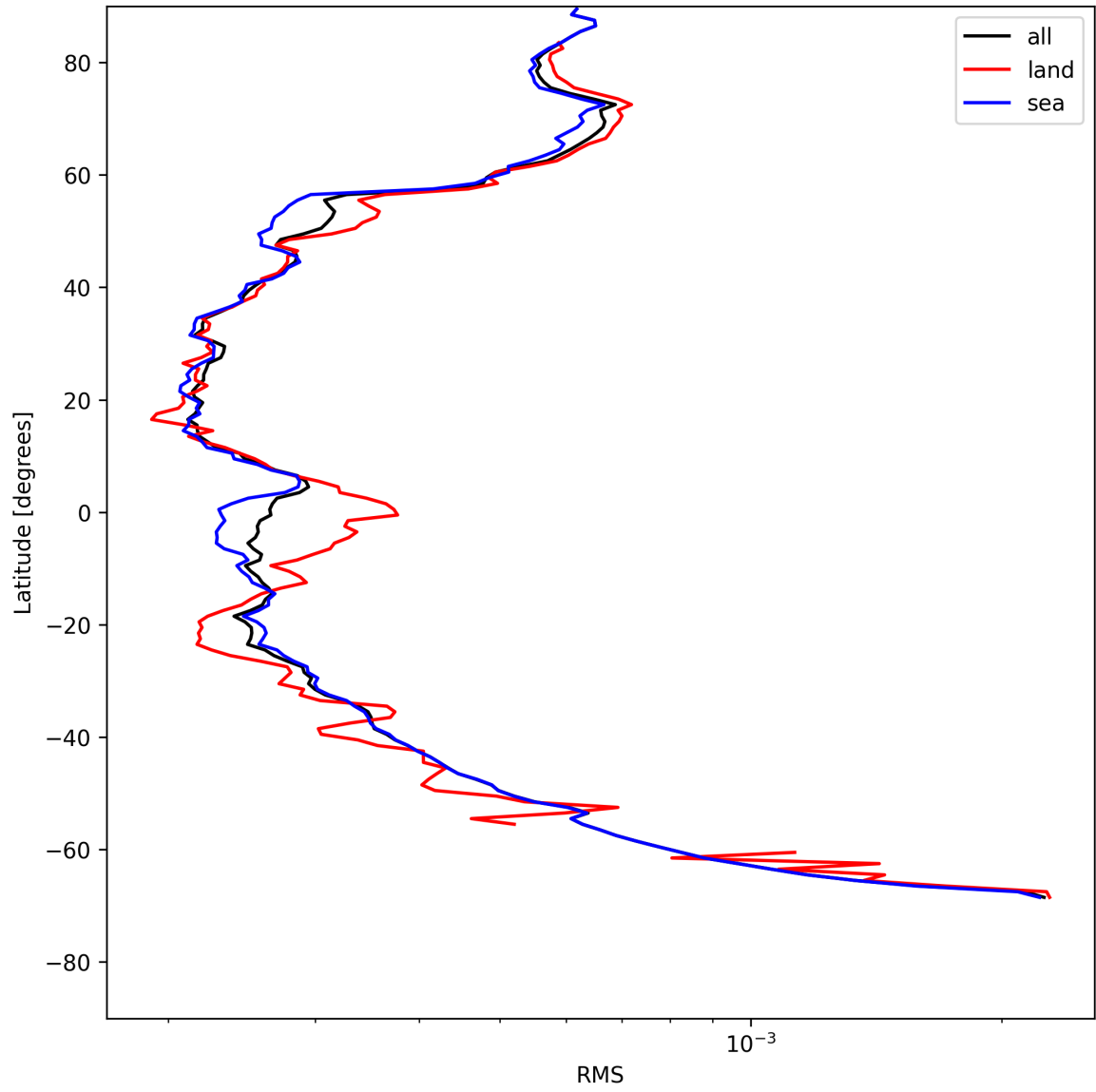
Figure 24: Zonal average of “RMS” for 2025-05-16 to 2025-05-17.
