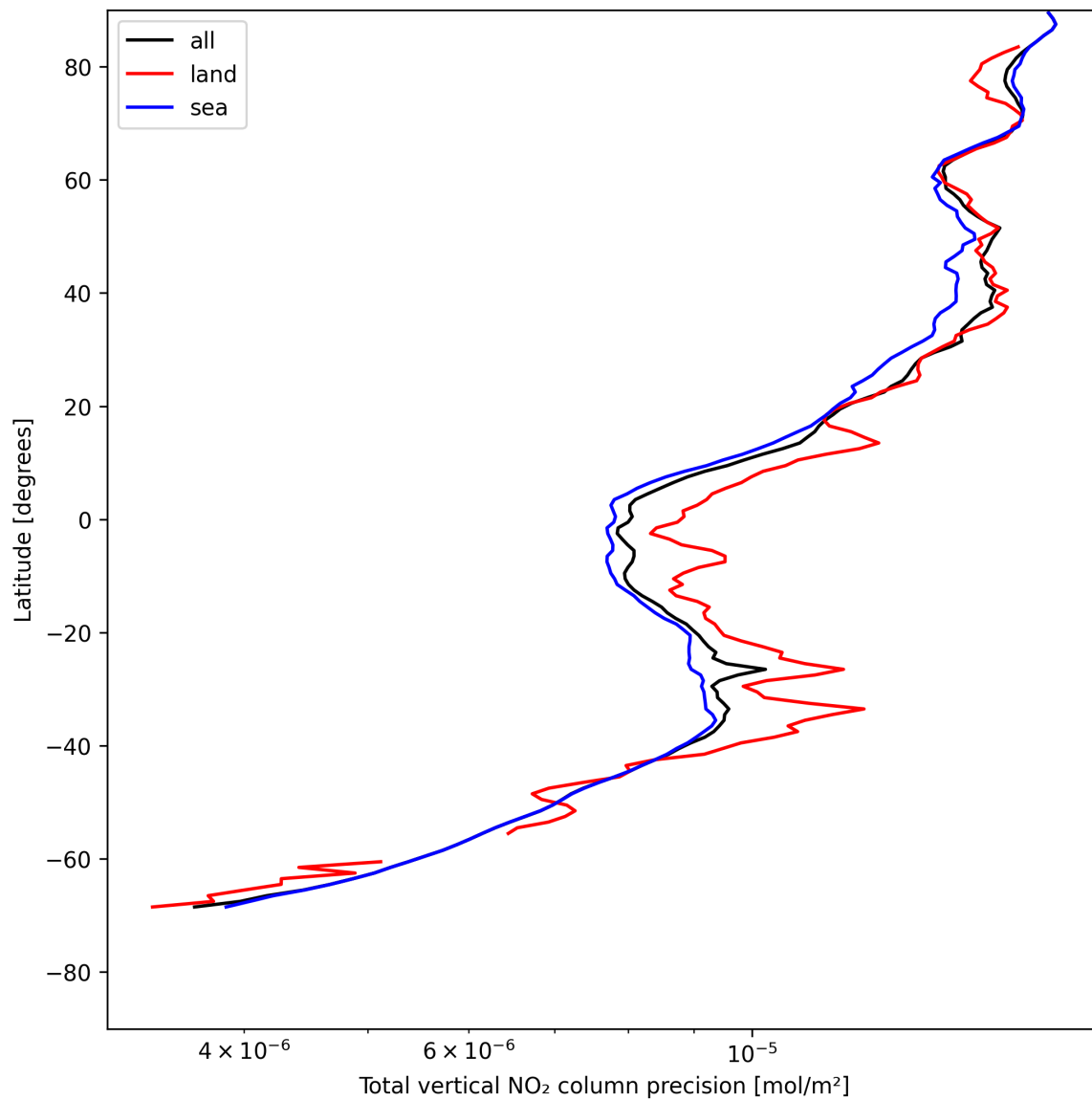
Figure 20: Zonal average of “Total vertical NO 2 column precision” for 2025-05-16 to 2025-05-17.
