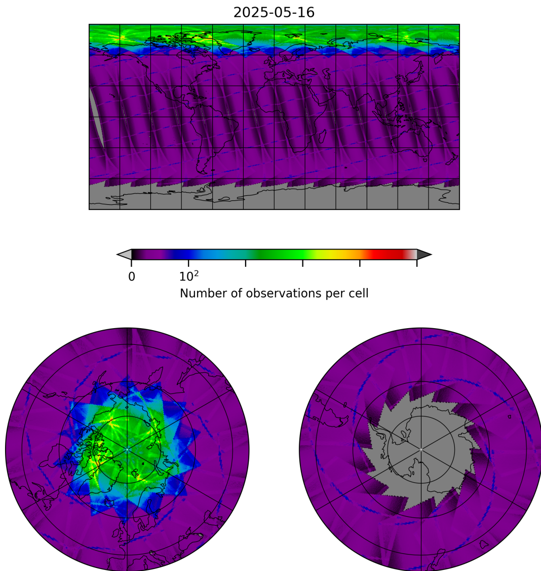
Figure 8: Map of the number of observations for 2025-05-16 to 2025-05-17
