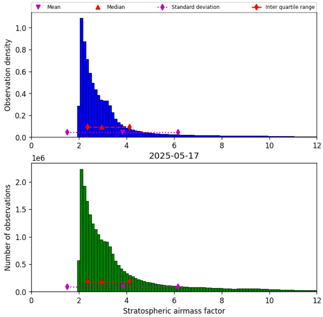
Figure 42: Histogram of “Stratospheric airmass factor” for 2025-05-17 to 2025-05-18
