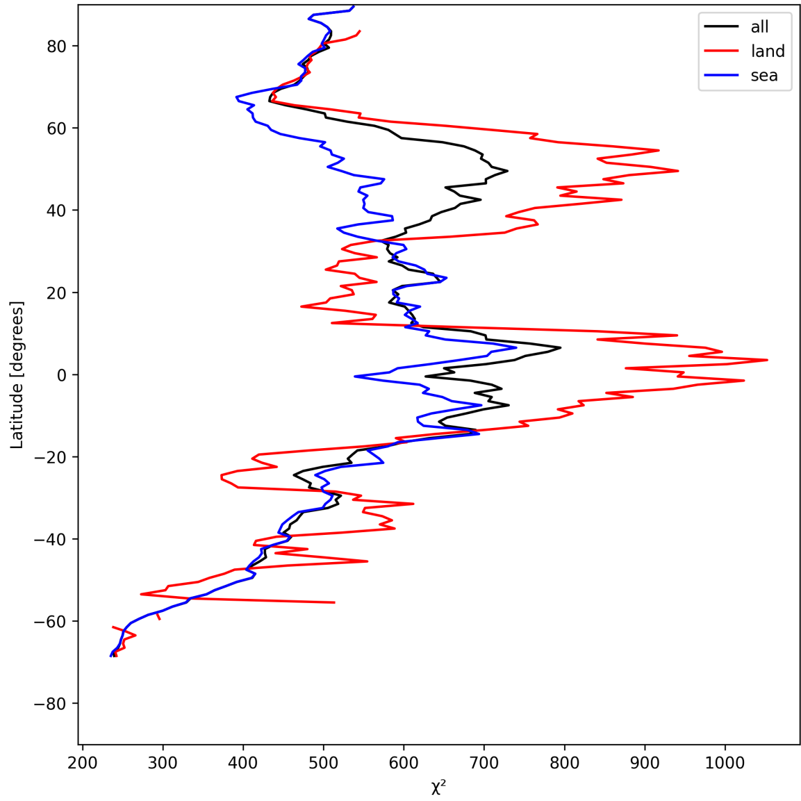
Figure 23: Zonal average of “ \chi^2 ” for 2025-05-17 to 2025-05-18.
