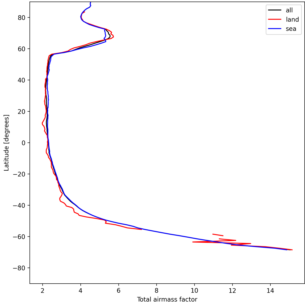
Figure 13: Zonal average of “Total airmass factor” for 2025-05-17 to 2025-05-18.
