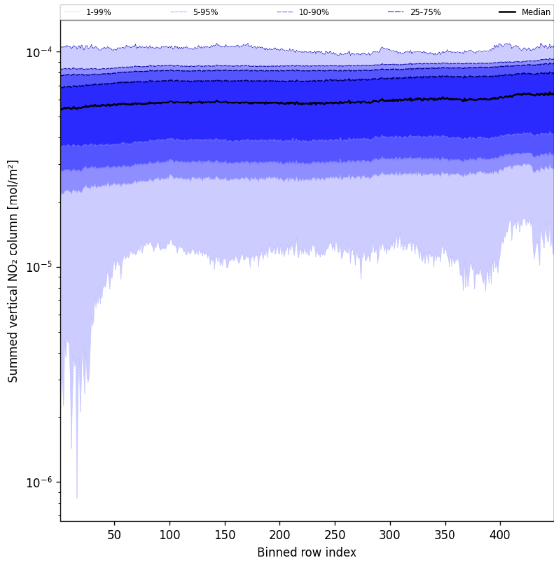
Figure 55: Along track statistics of “Summed vertical NO 2 column” for 2025-05-17 to 2025-05-18
