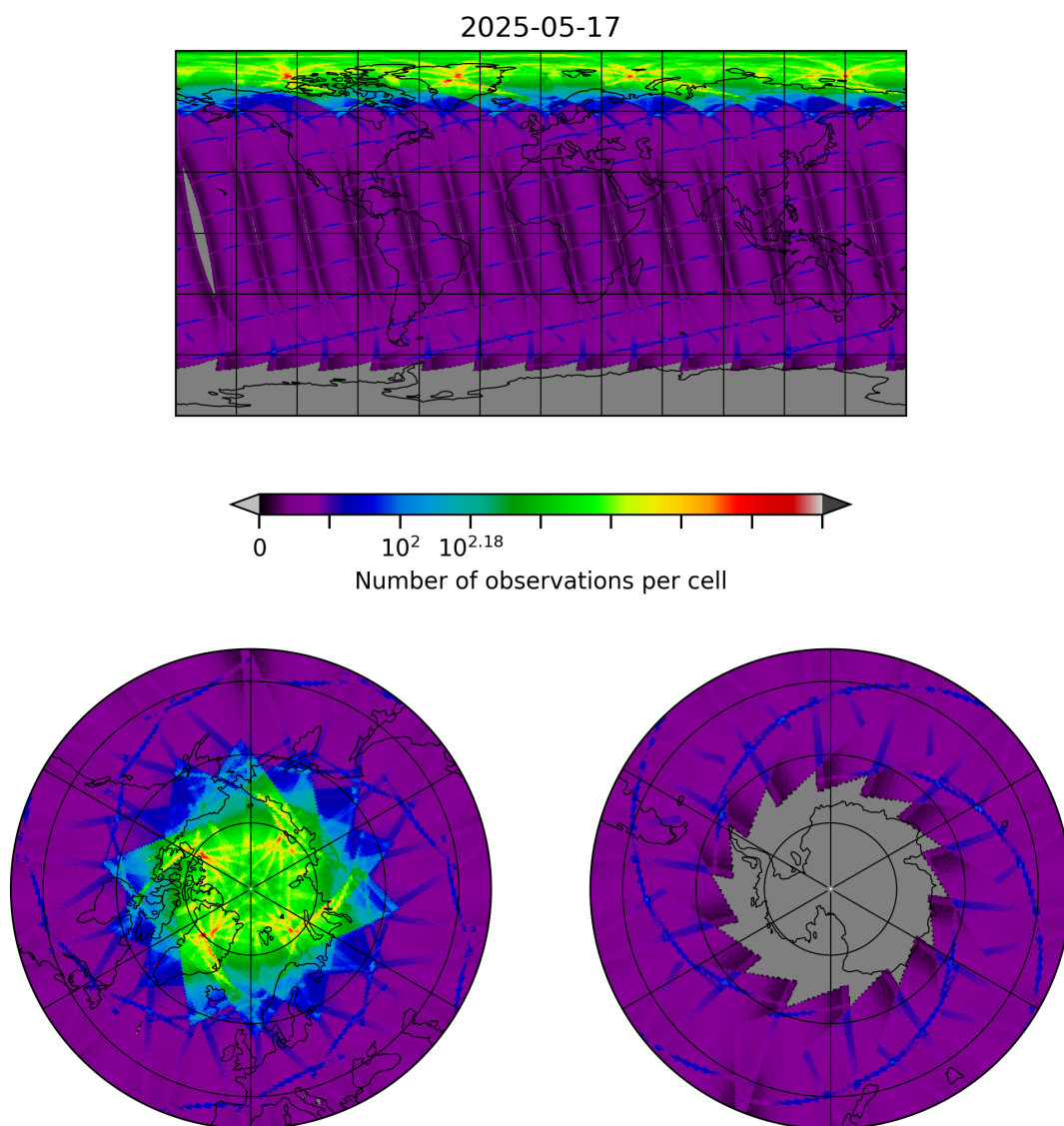
Figure 8: Map of the number of observations for 2025-05-17 to 2025-05-18
