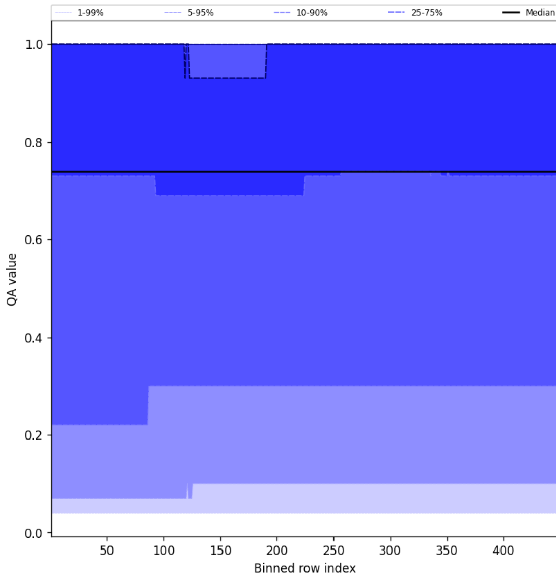
Figure 43: Along track statistics of “QA value” for 2025-05-17 to 2025-05-18
