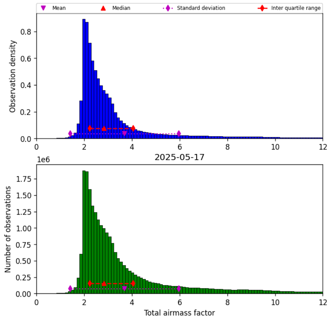
Figure 30: Histogram of “Total airmass factor” for 2025-05-17 to 2025-05-18
