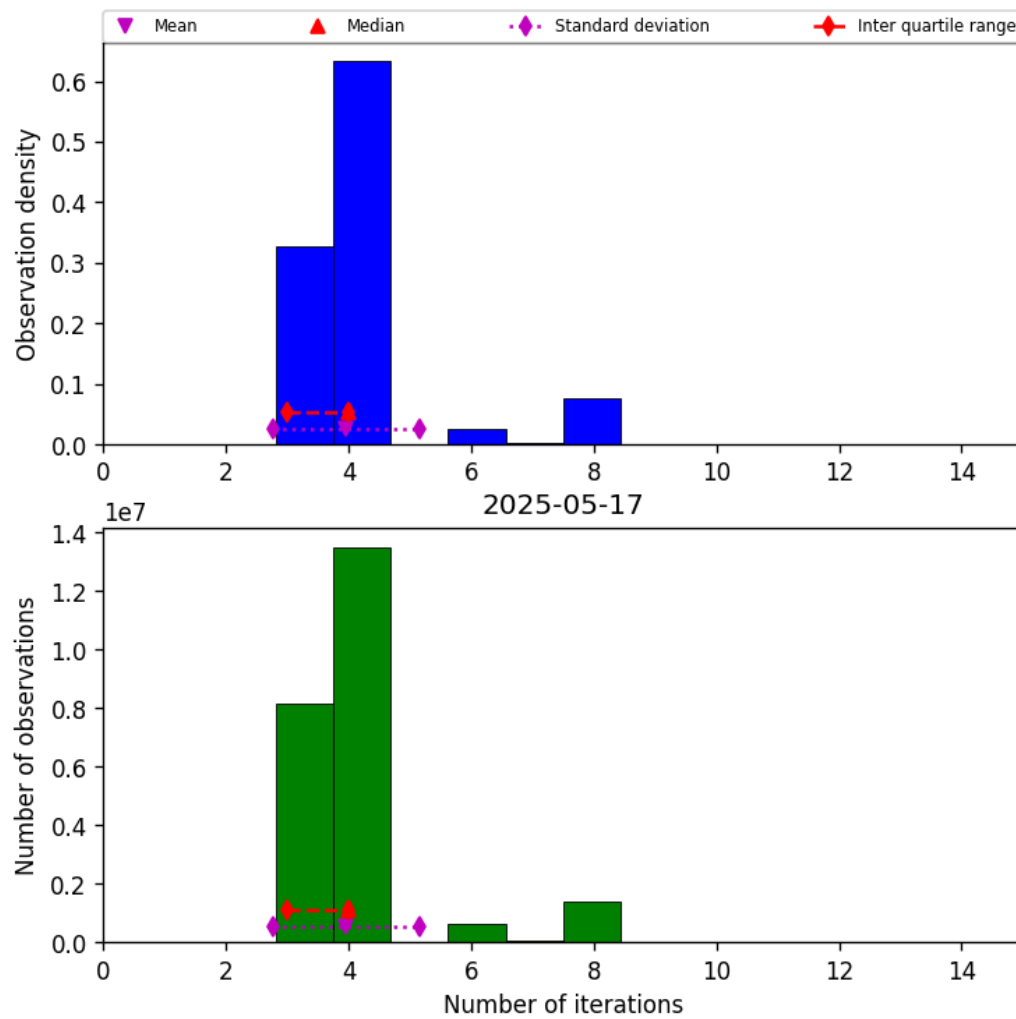
Figure 32: Histogram of “Number of iterations” for 2025-05-17 to 2025-05-18
