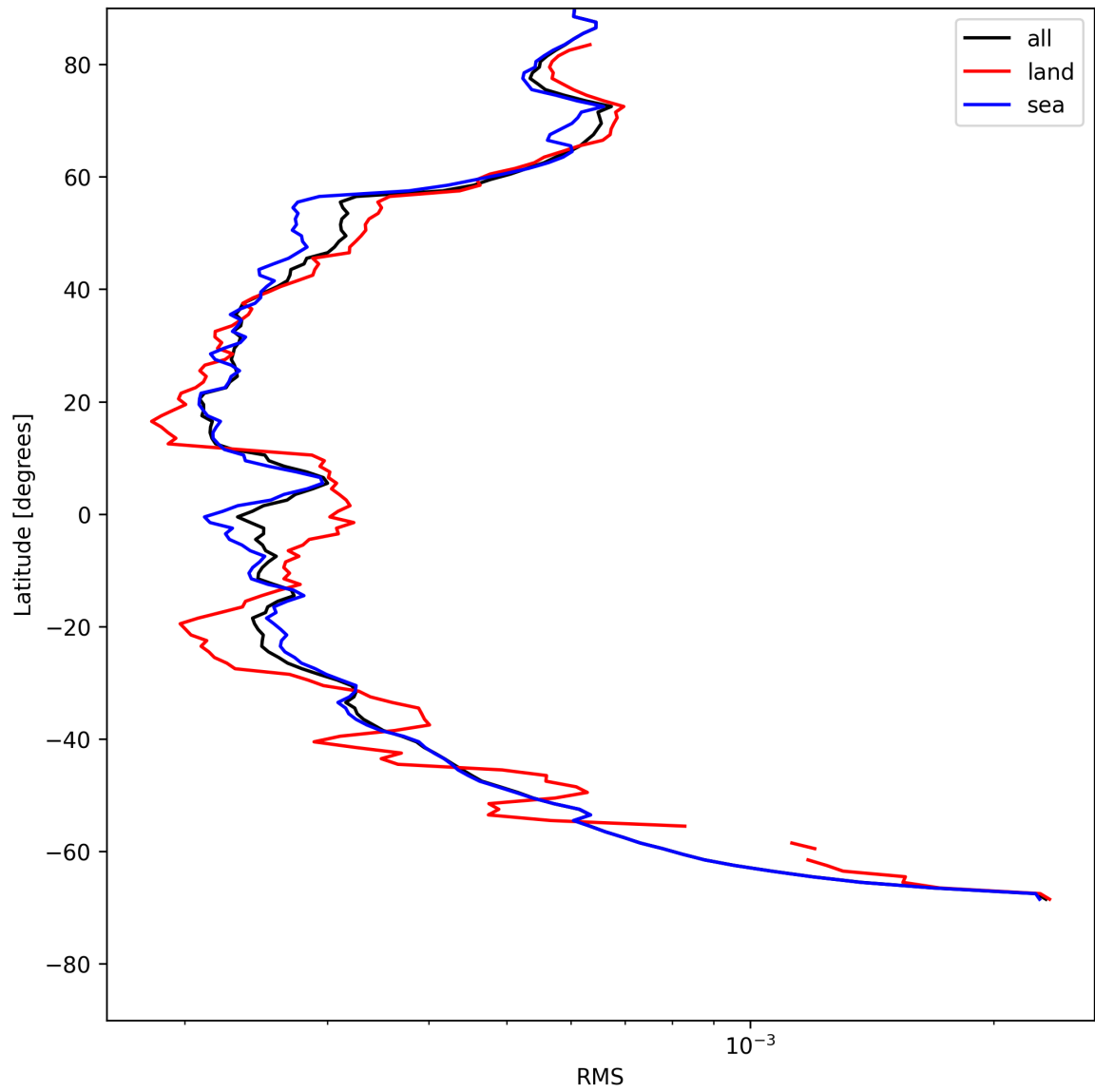
Figure 24: Zonal average of “RMS” for 2025-05-17 to 2025-05-18.
