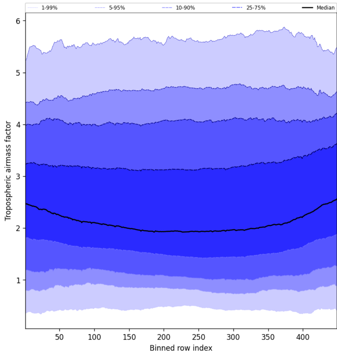
Figure 46: Along track statistics of “Tropospheric airmass factor” for 2025-05-17 to 2025-05-18
