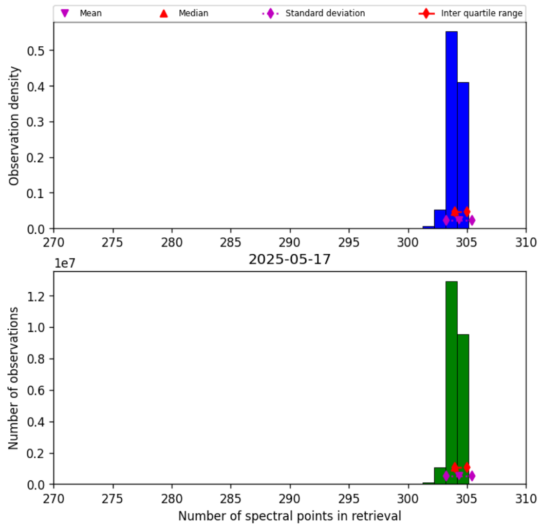
Figure 31: Histogram of “Number of spectral points in retrieval” for 2025-05-17 to 2025-05-18
