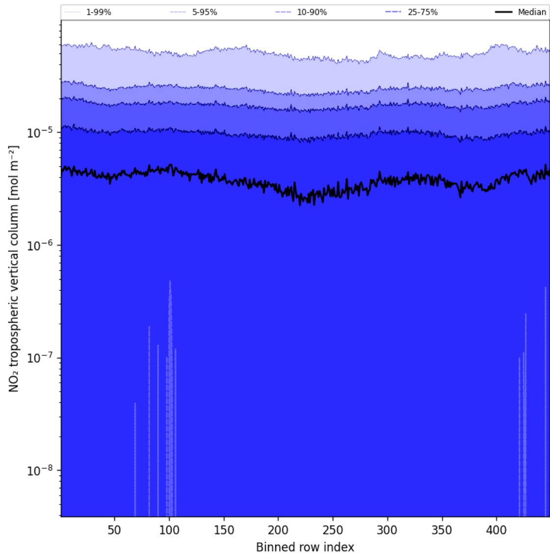
Figure 44: Along track statistics of “NO 2 tropospheric vertical column” for 2025-05-17 to 2025-05-18
