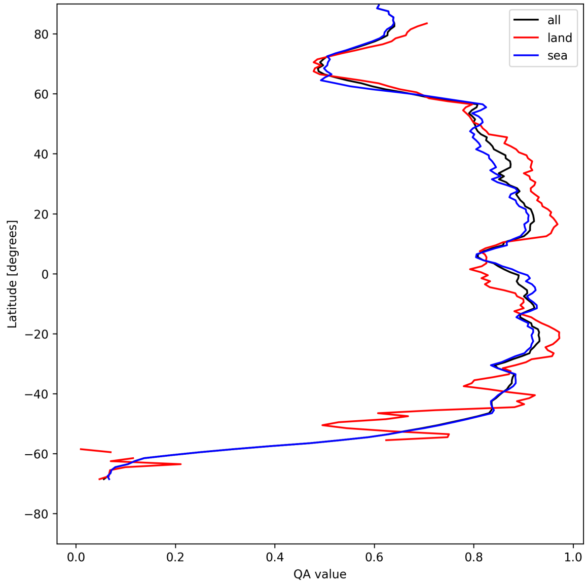
Figure 9: Zonal average of “QA value” for 2025-05-17 to 2025-05-18.
