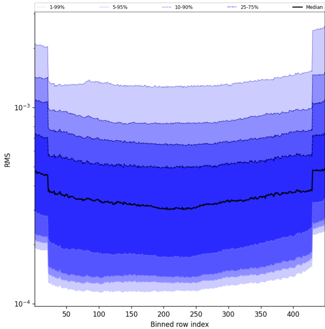
Figure 58: Along track statistics of “RMS” for 2025-05-17 to 2025-05-18
