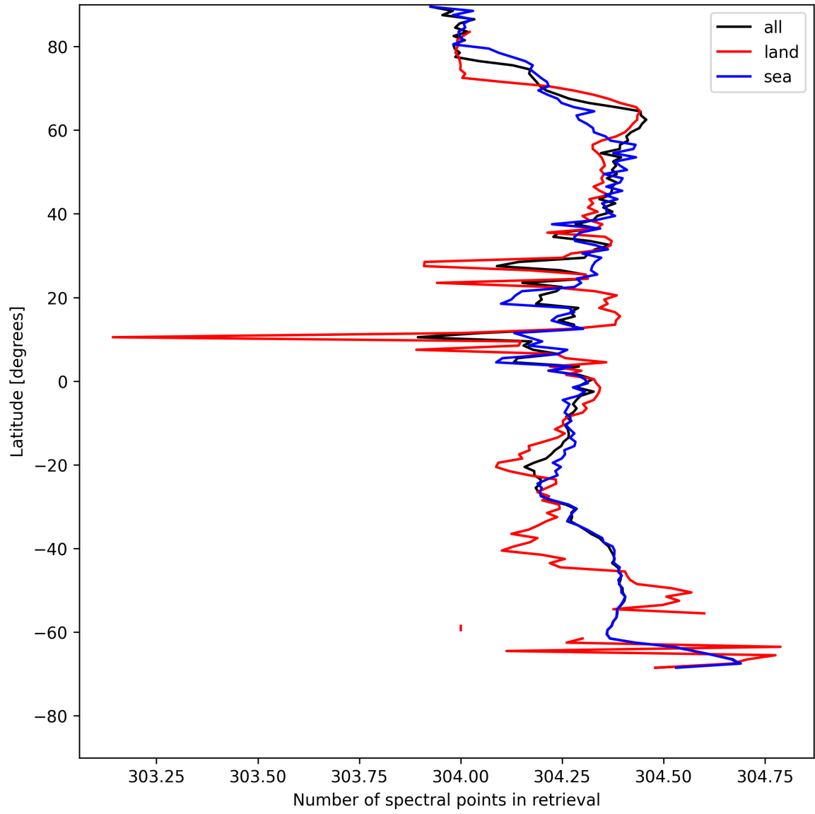
Figure 14: Zonal average of “Number of spectral points in retrieval” for 2025-05-17 to 2025-05-18.
