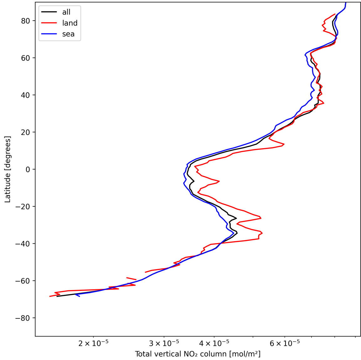
Figure 19: Zonal average of “Total vertical NO 2 column” for 2025-05-17 to 2025-05-18.
