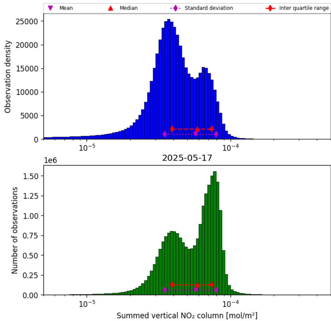
Figure 38: Histogram of “Summed vertical NO 2 column” for 2025-05-17 to 2025-05-18
