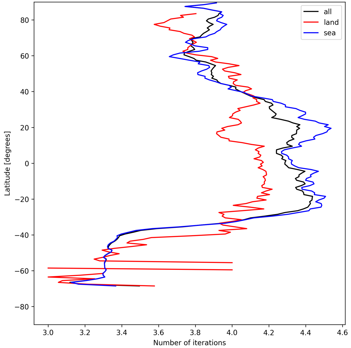
Figure 15: Zonal average of “Number of iterations” for 2025-05-17 to 2025-05-18.
