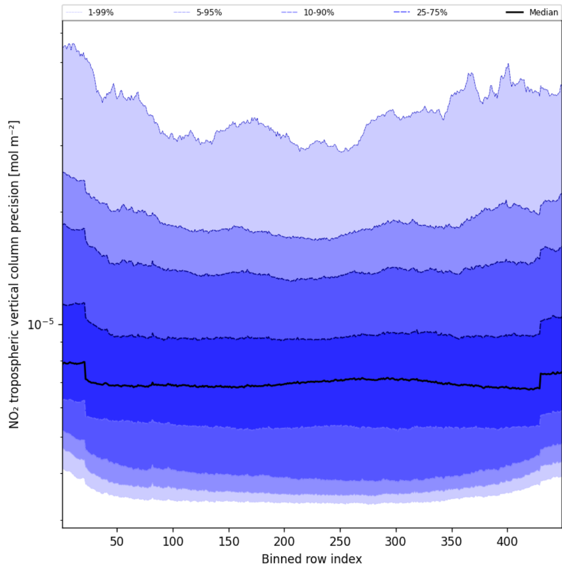
Figure 45: Along track statistics of “NO 2 tropospheric vertical column precision” for 2025-05-17 to 2025-05-18
