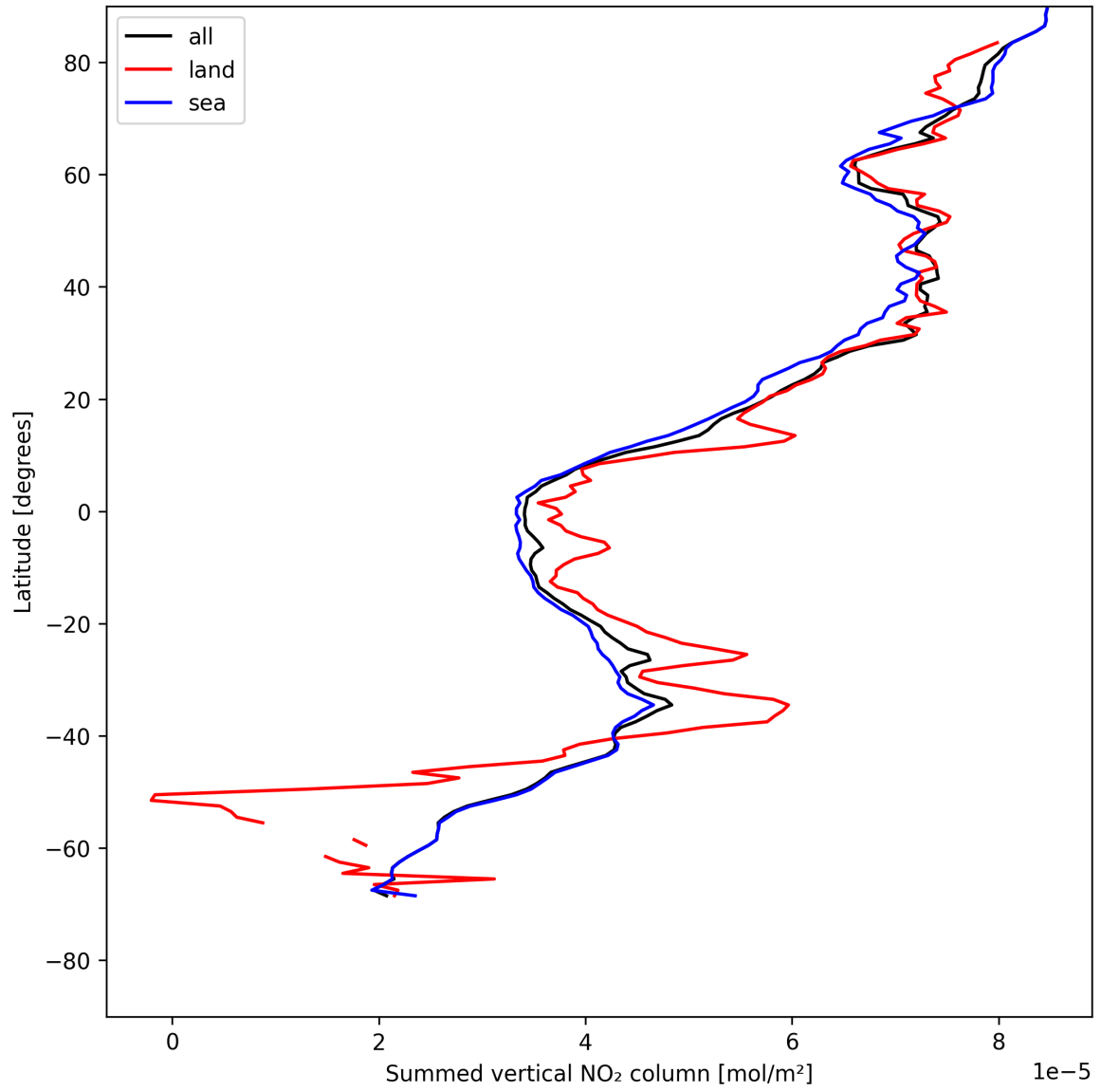
Figure 21: Zonal average of “Summed vertical NO 2 column” for 2025-05-17 to 2025-05-18.
