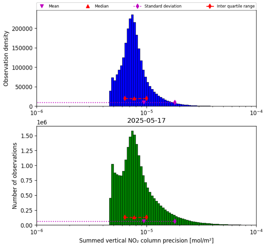
Figure 39: Histogram of “Summed vertical NO 2 column precision” for 2025-05-17 to 2025-05-18
