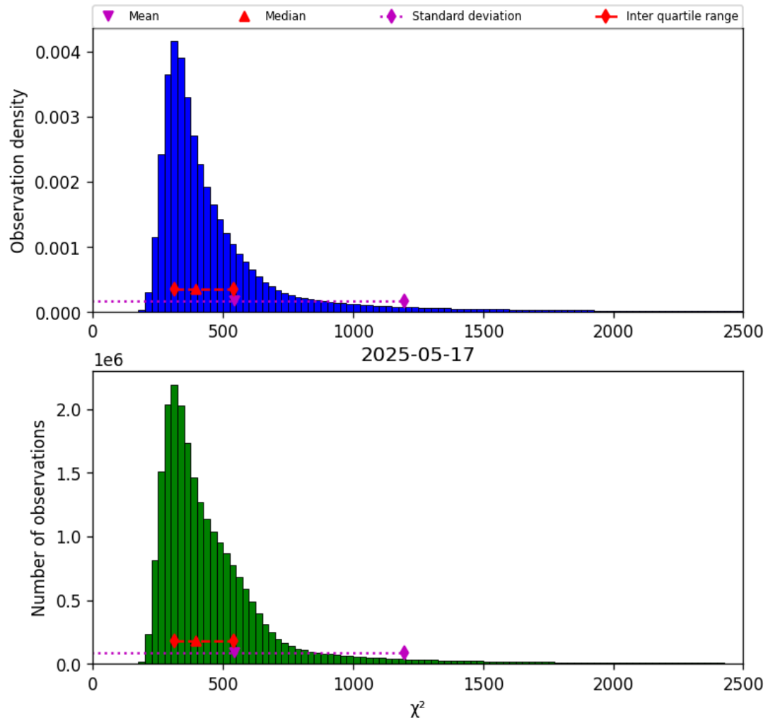
Figure 40: Histogram of “ \chi^2 ” for 2025-05-17 to 2025-05-18
