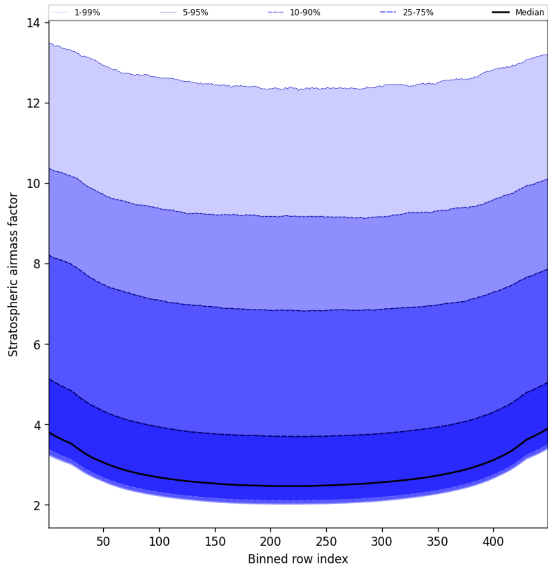
Figure 59: Along track statistics of “Stratospheric airmass factor” for 2025-05-17 to 2025-05-18
