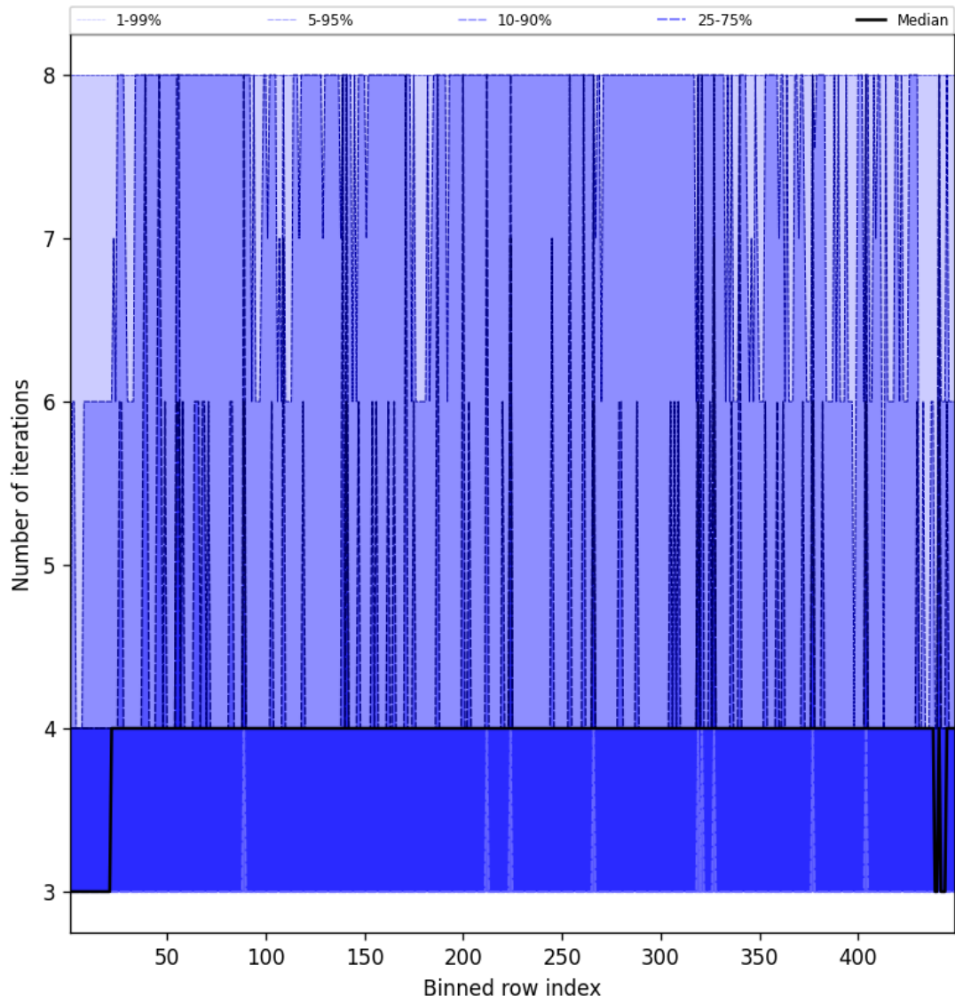
Figure 49: Along track statistics of “Number of iterations” for 2025-05-17 to 2025-05-18
