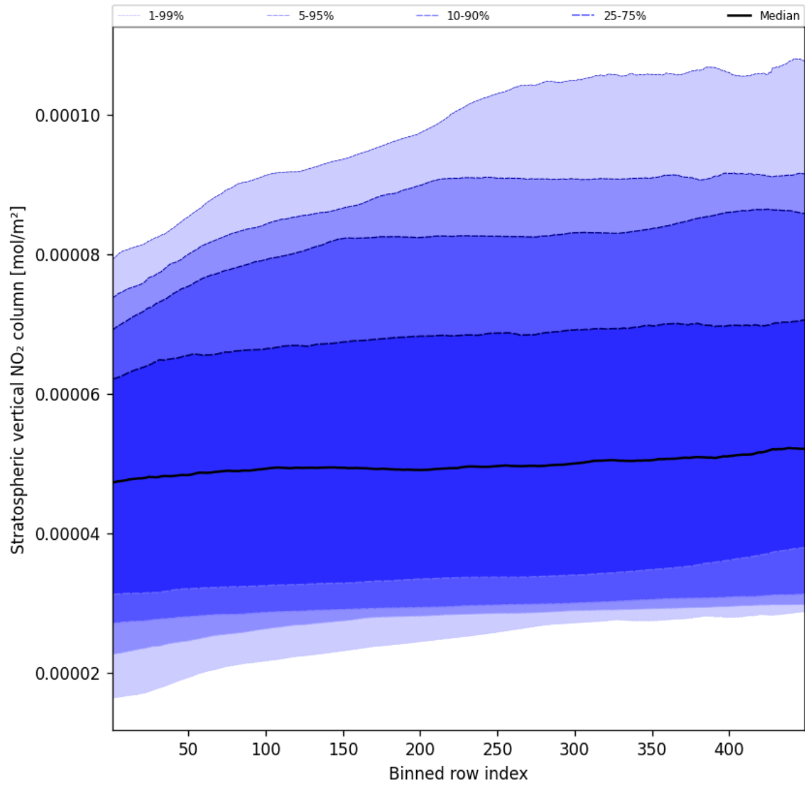
Figure 51: Along track statistics of “Stratospheric vertical NO 2 column” for 2025-05-17 to 2025-05-18
