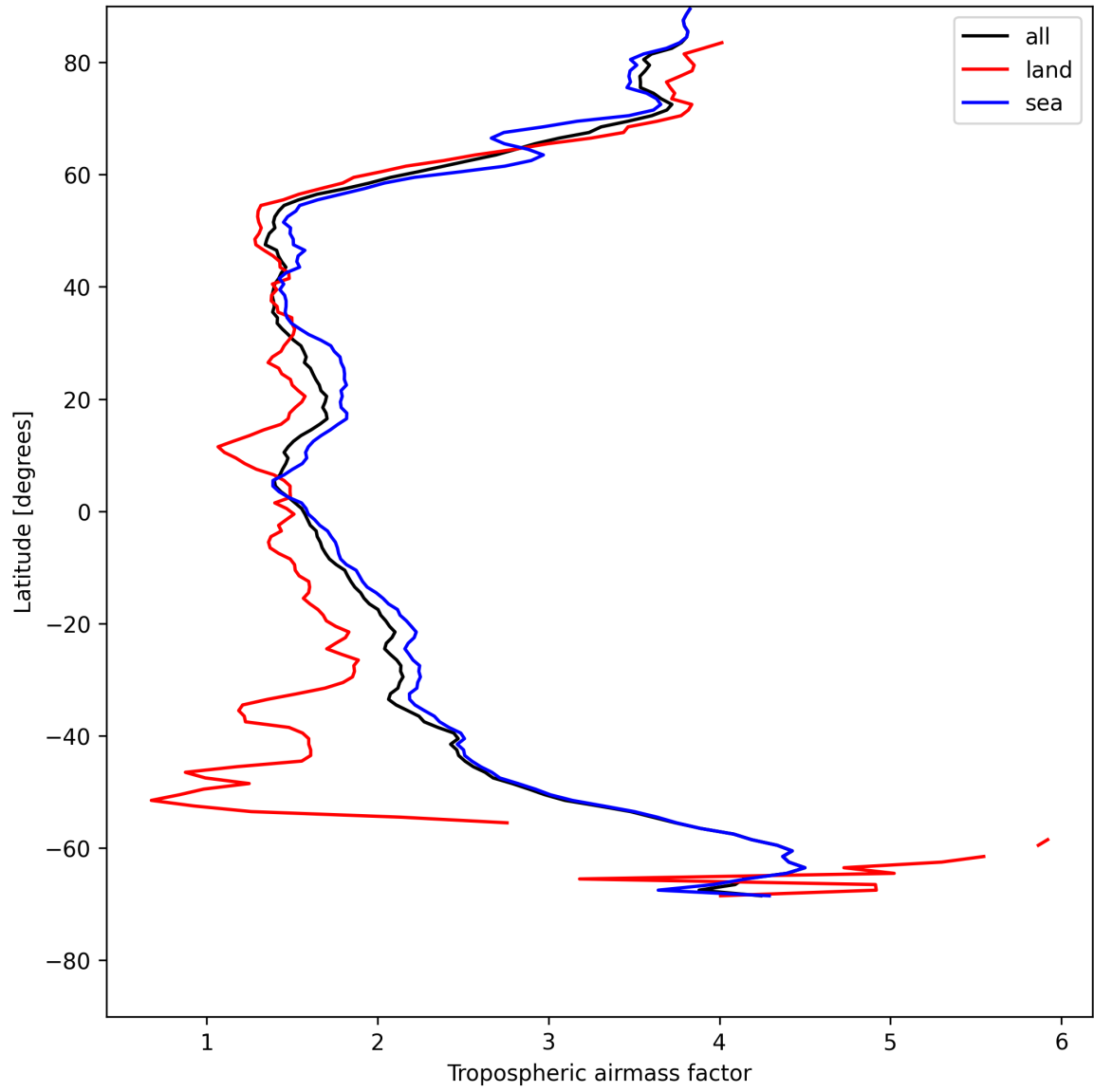
Figure 12: Zonal average of “Tropospheric air mass factor” for 2025-05-17 to 2025-05-18.
