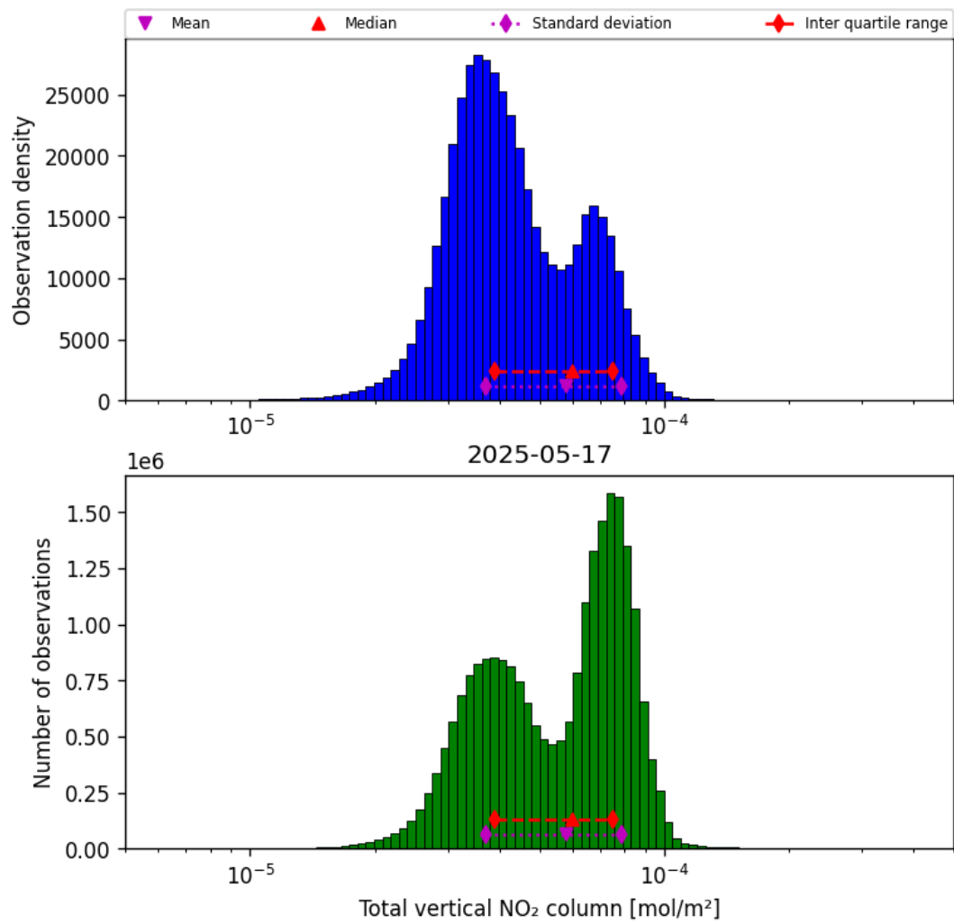
Figure 36: Histogram of “Total vertical NO 2 column” for 2025-05-17 to 2025-05-18
