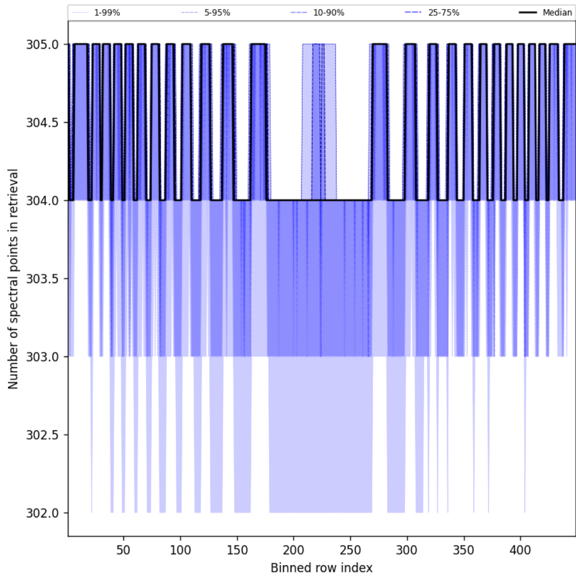
Figure 48: Along track statistics of “Number of spectral points in retrieval” for 2025-05-17 to 2025-05-18
