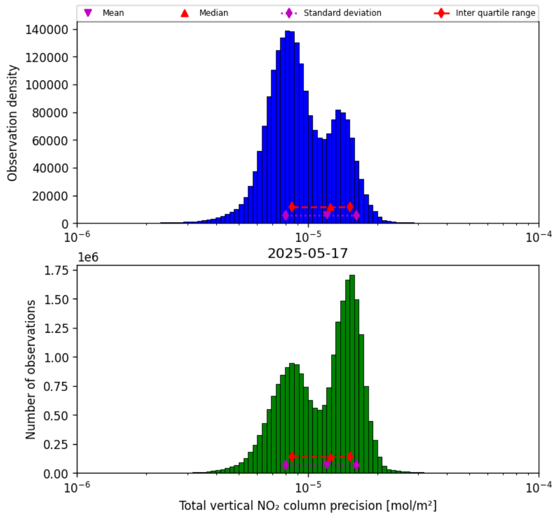
Figure 37: Histogram of “Total vertical NO 2 column precision” for 2025-05-17 to 2025-05-18
