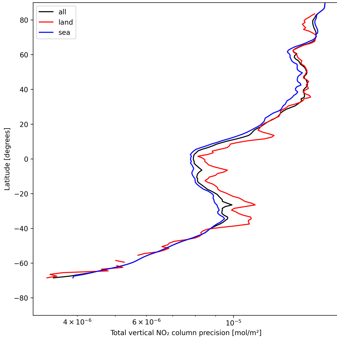
Figure 20: Zonal average of “Total vertical NO 2 column precision” for 2025-05-17 to 2025-05-18.
