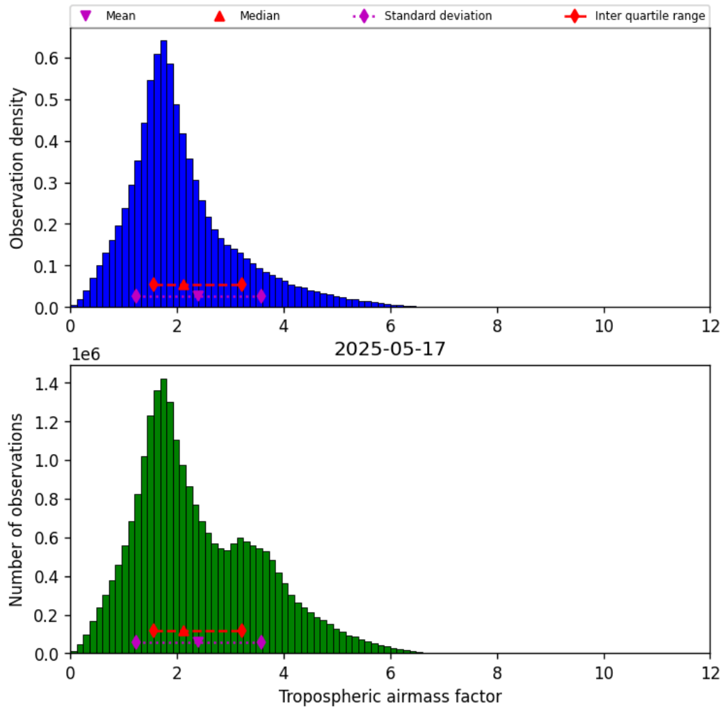
Figure 29: Histogram of “Tropospheric airmass factor” for 2025-05-17 to 2025-05-18
