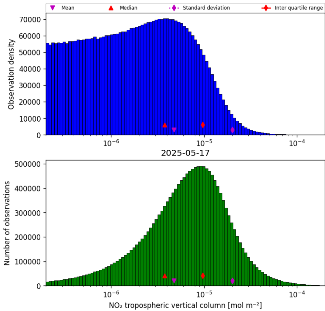
Figure 27: Histogram of “NO 2 tropospheric vertical column” for 2025-05-17 to 2025-05-18
