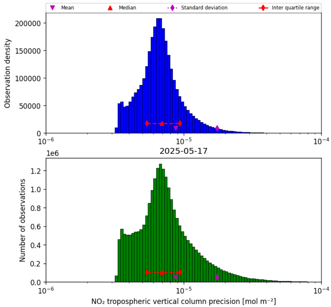
Figure 28: Histogram of “NO 2 tropospheric vertical column precision” for 2025-05-17 to 2025-05-18
