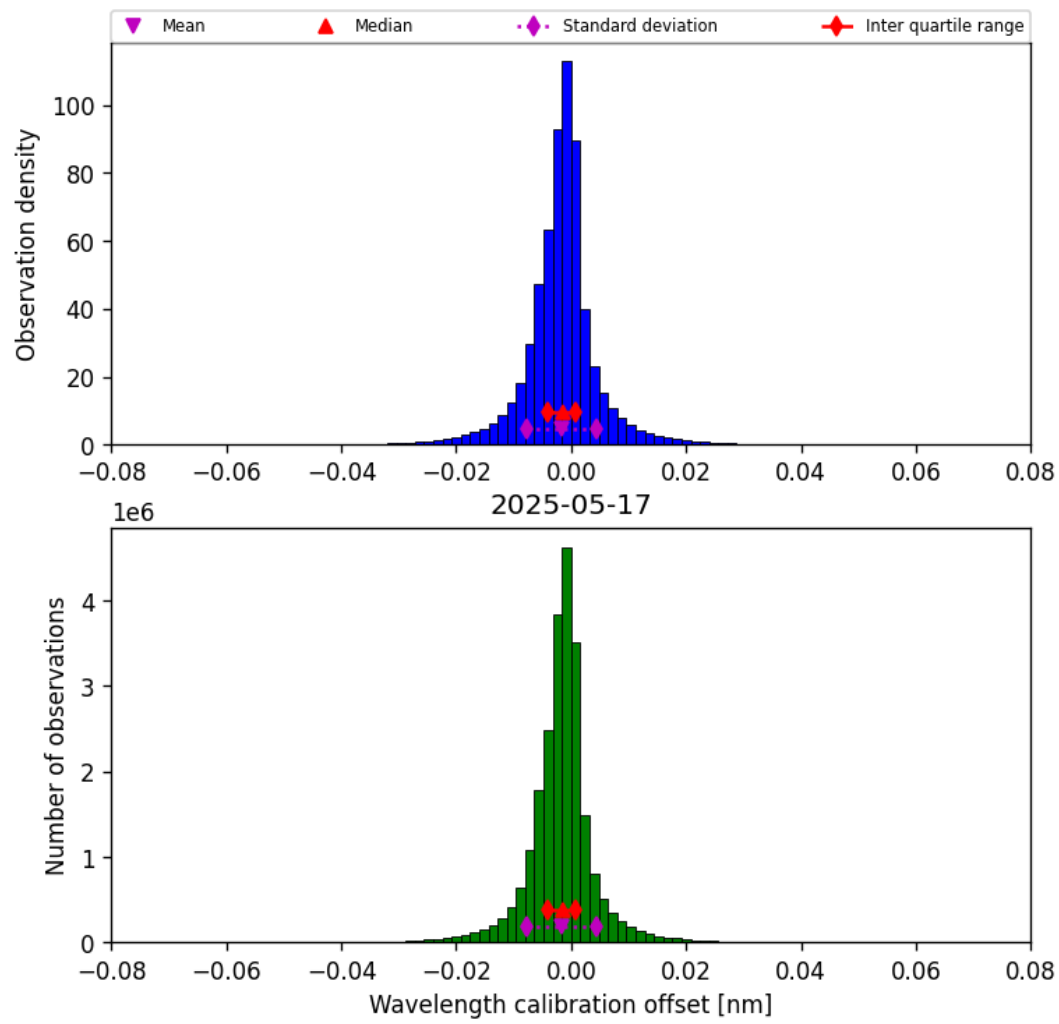
Figure 33: Histogram of “Wavelength calibration offset” for 2025-05-17 to 2025-05-18
