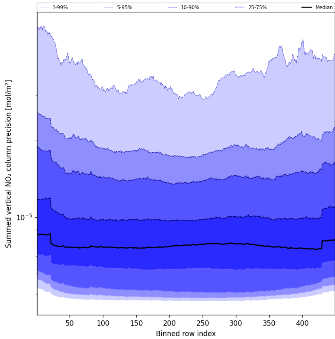
Figure 56: Along track statistics of “Summed vertical NO 2 column precision” for 2025-05-17 to 2025-05-18
