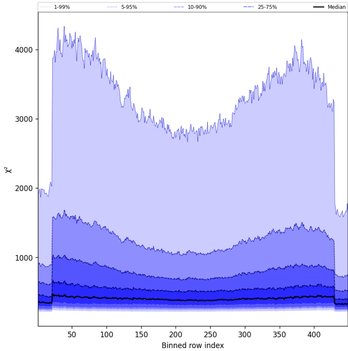
Figure 57: Along track statistics of “ \chi^2 ” for 2025-05-17 to 2025-05-18
