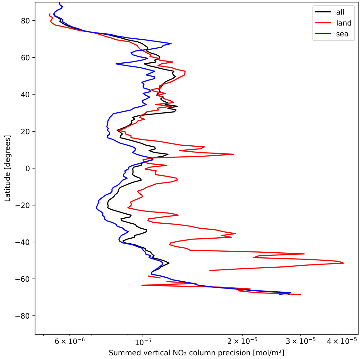
Figure 22: Zonal average of “Summed vertical NO 2 column precision” for 2025-05-17 to 2025-05-18.
