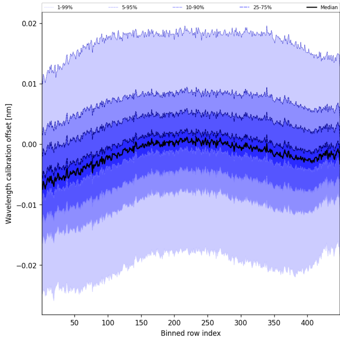
Figure 50: Along track statistics of “Wavelength calibration offset” for 2025-05-17 to 2025-05-18
