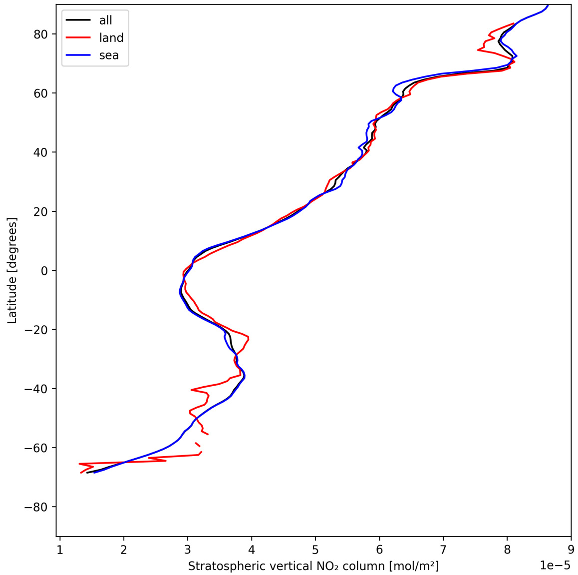
Figure 17: Zonal average of “Stratospheric vertical NO 2 column” for 2025-05-17 to 2025-05-18.
