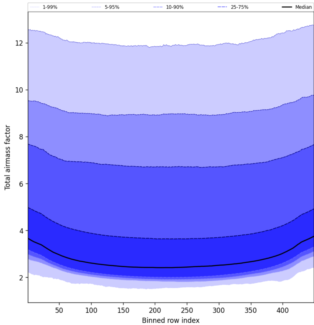
Figure 47: Along track statistics of “Total airmass factor” for 2025-05-17 to 2025-05-18
