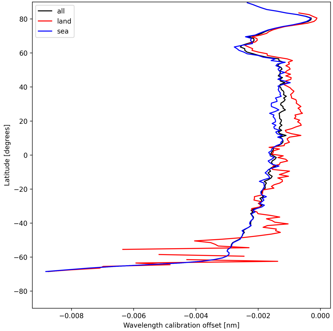
Figure 16: Zonal average of “Wavelength calibration offset” for 2025-05-17 to 2025-05-18.
