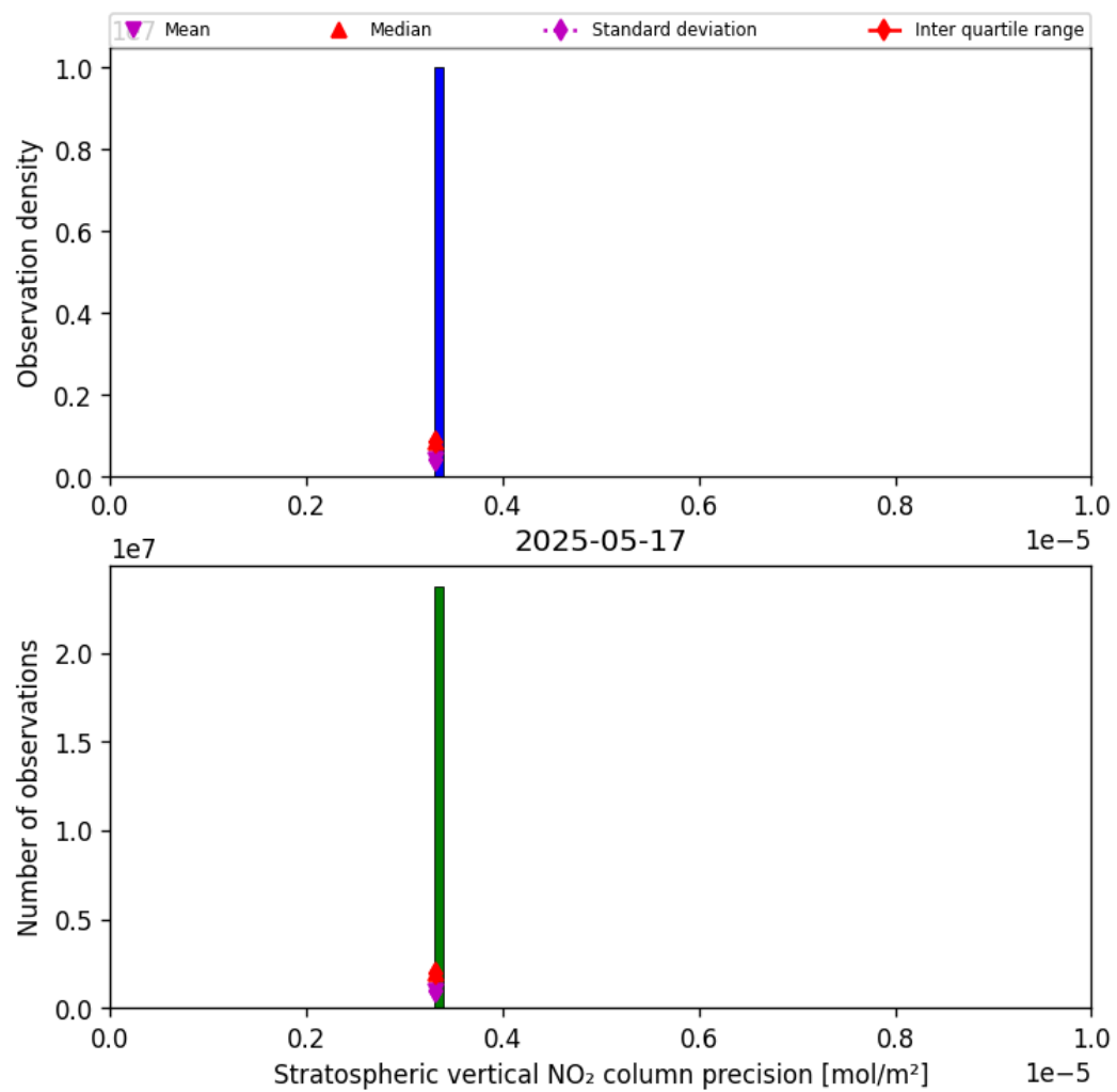
Figure 35: Histogram of “Stratospheric vertical NO 2 column precision” for 2025-05-17 to 2025-05-18
