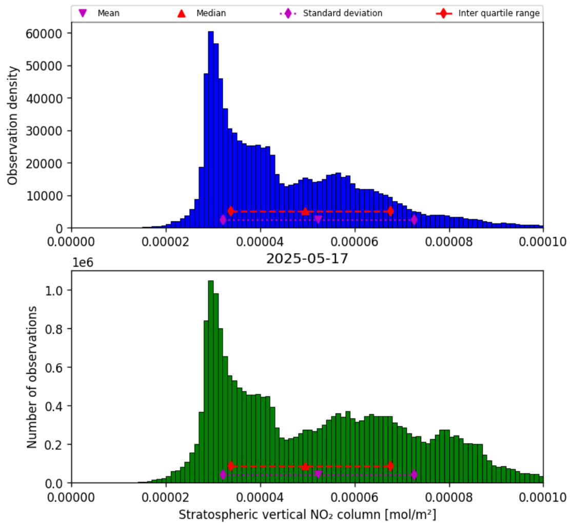
Figure 34: Histogram of “Stratospheric vertical NO 2 column” for 2025-05-17 to 2025-05-18
