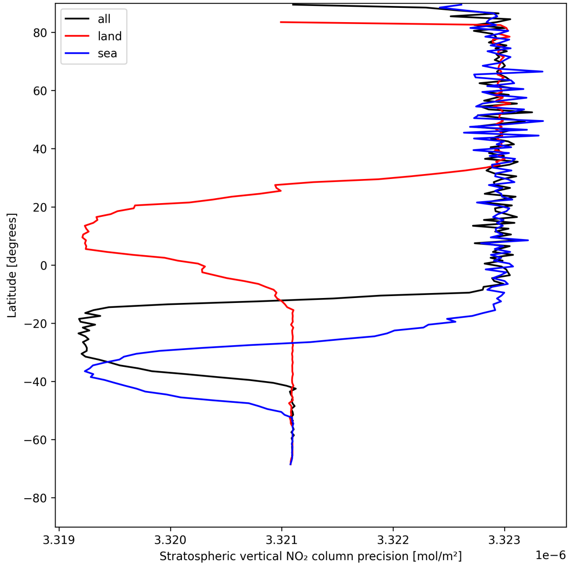
Figure 18: Zonal average of “Stratospheric vertical NO 2 column precision” for 2025-05-17 to 2025-05-18.
