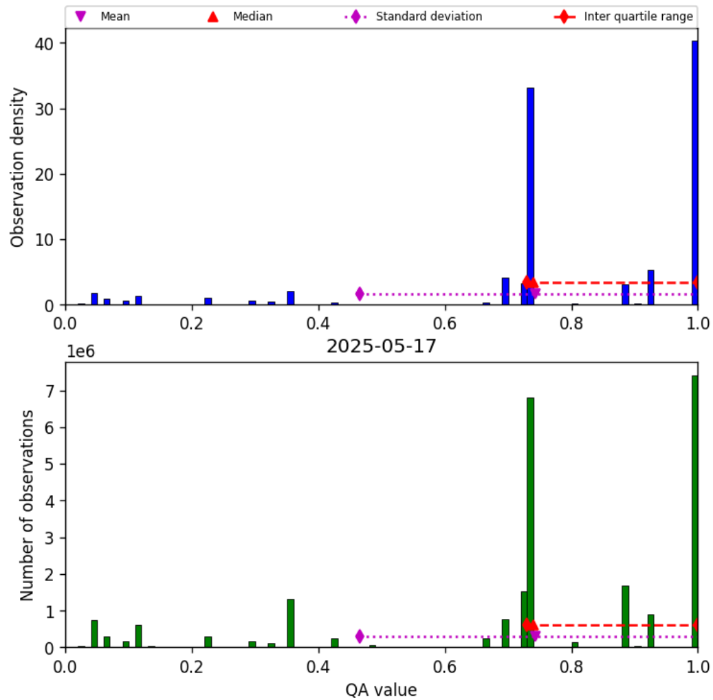
Figure 26: Histogram of “QA value” for 2025-05-17 to 2025-05-18
