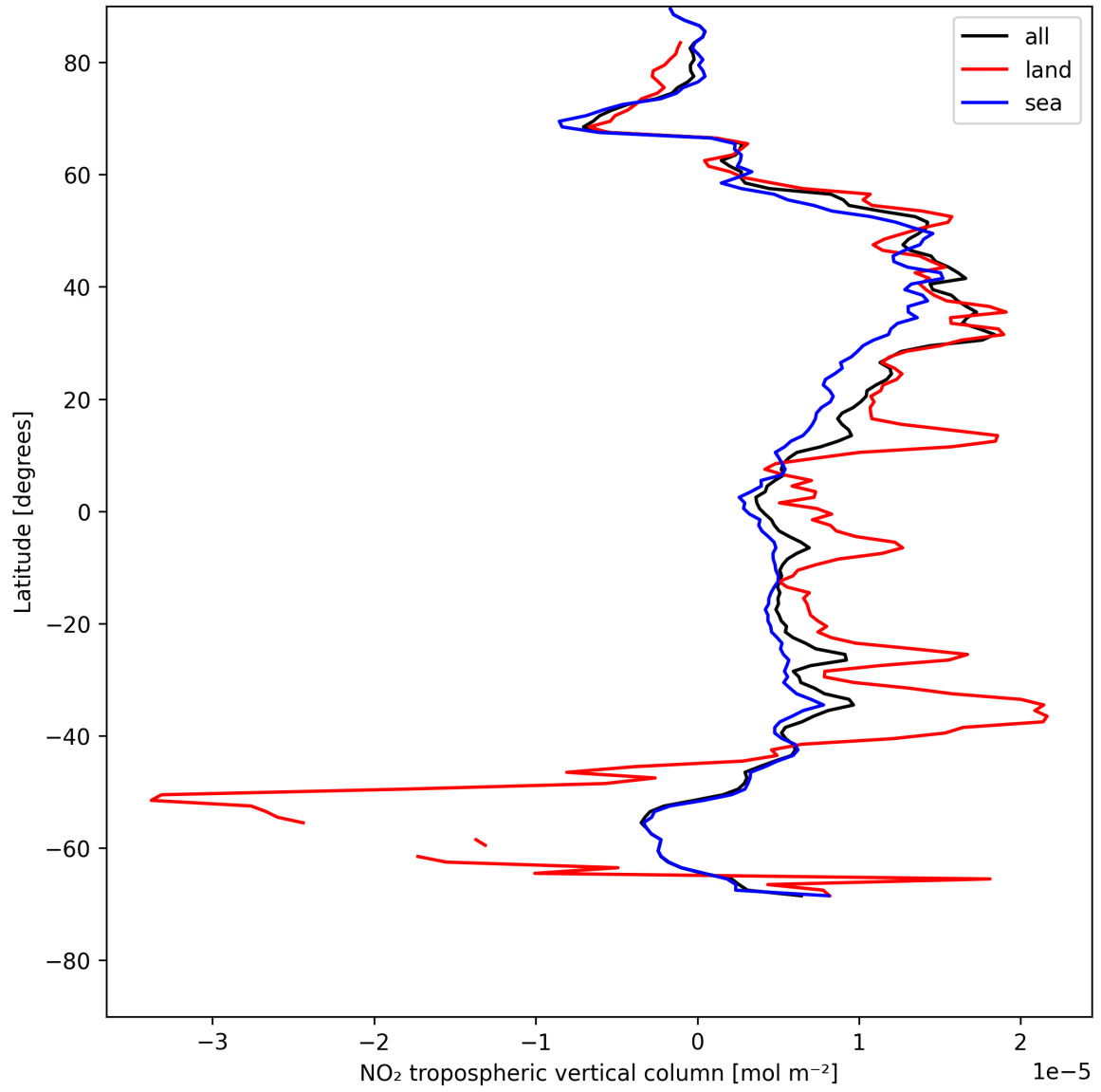
Figure 10: Zonal average of “NO 2 tropospheric vertical column” for 2025-05-17 to 2025-05-18.
