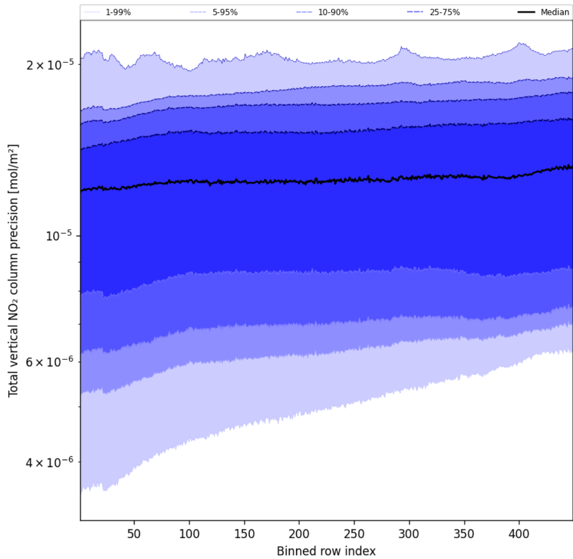
Figure 54: Along track statistics of "Total vertical NO 2 column precision" for 2025-05-17 to 2025-05-18
