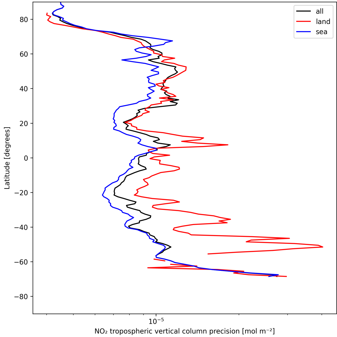
Figure 11: Zonal average of “NO 2 tropospheric vertical column precision” for 2025-05-17 to 2025-05-18.
