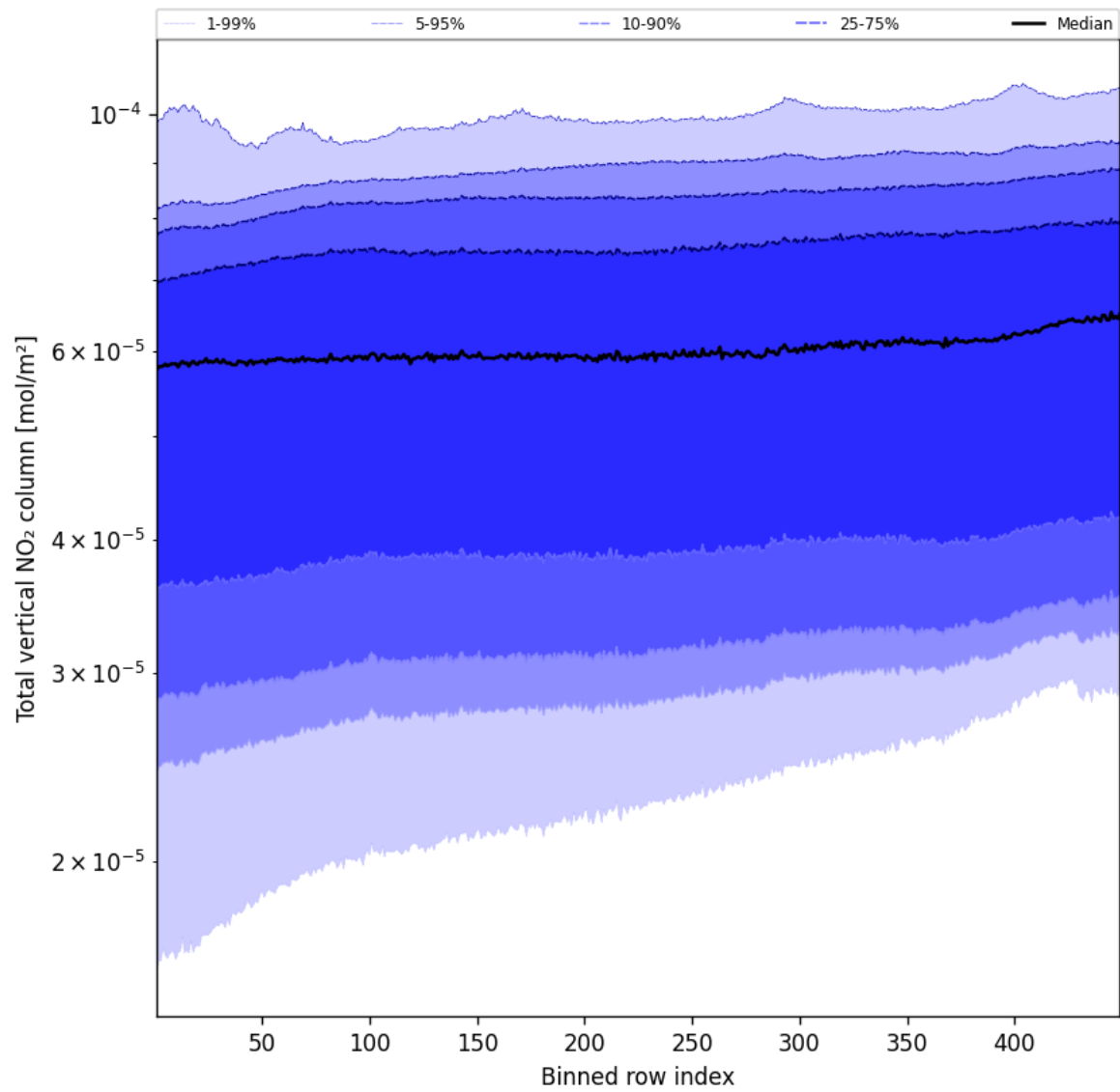
Figure 53: Along track statistics of “Total vertical NO 2 column” for 2025-05-17 to 2025-05-18
