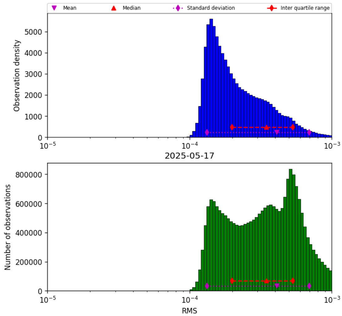
Figure 41: Histogram of “RMS” for 2025-05-17 to 2025-05-18
