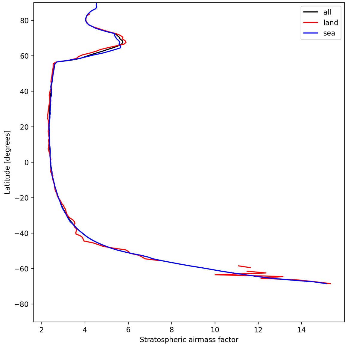
Figure 25: Zonal average of “Stratospheric airmass factor” for 2025-05-17 to 2025-05-18.
