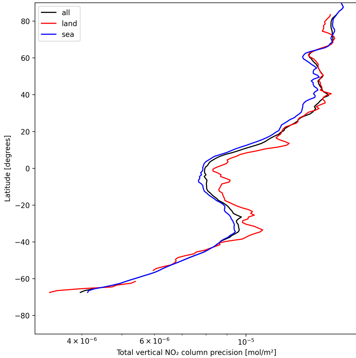
Figure 20: Zonal average of “Total vertical NO 2 column precision” for 2025-05-18 to 2025-05-19.
