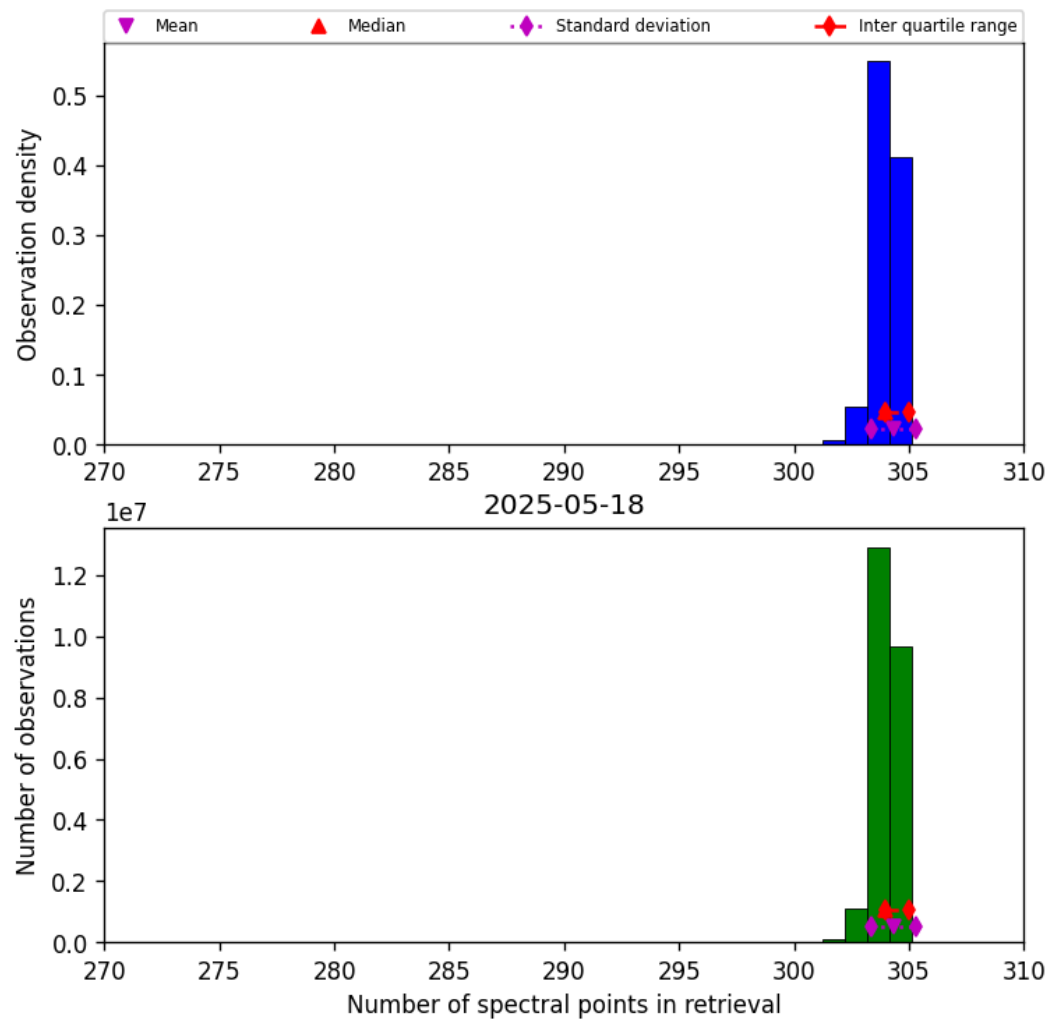
Figure 31: Histogram of “Number of spectral points in retrieval” for 2025-05-18 to 2025-05-19
