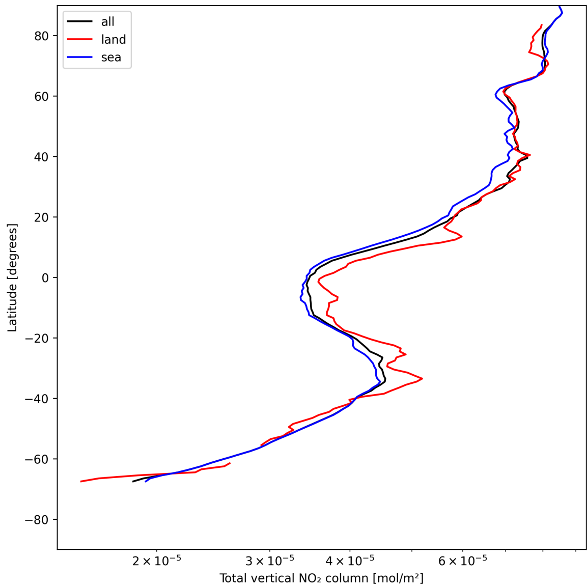
Figure 19: Zonal average of “Total vertical NO 2 column” for 2025-05-18 to 2025-05-19.
