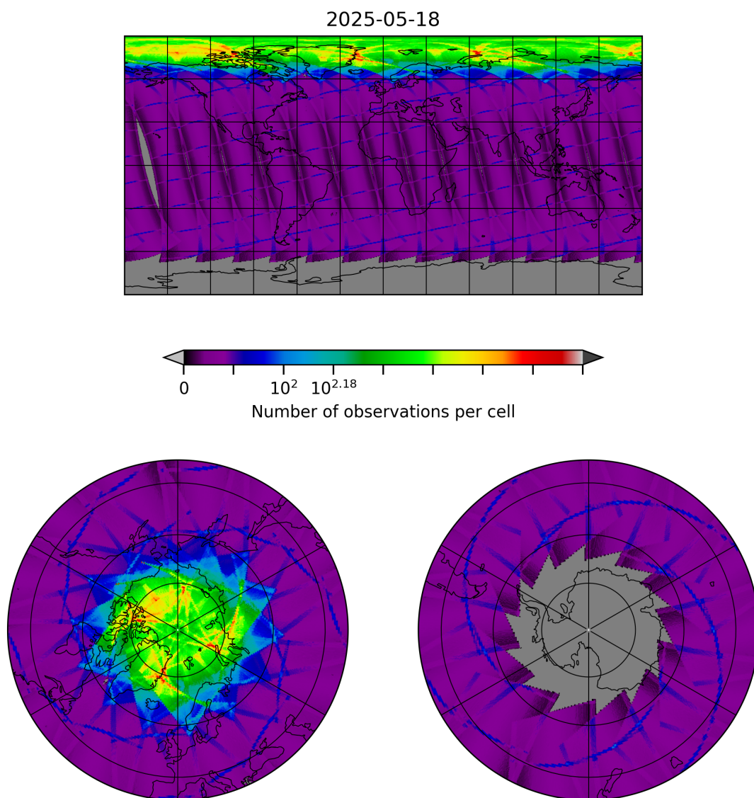
Figure 8: Map of the number of observations for 2025-05-18 to 2025-05-19
