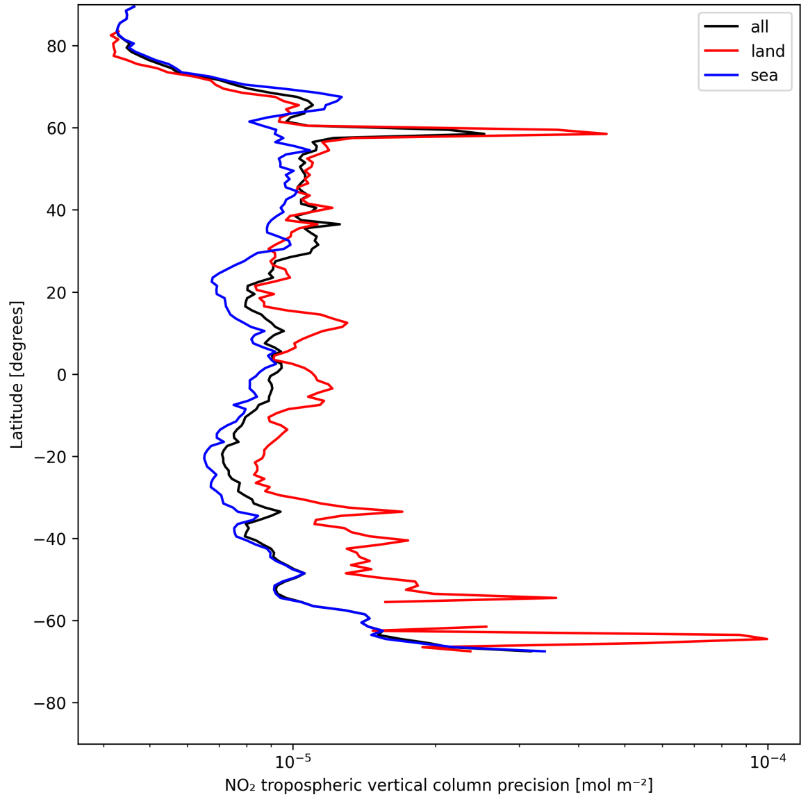
Figure 11: Zonal average of “NO 2 tropospheric vertical column precision” for 2025-05-18 to 2025-05-19.
