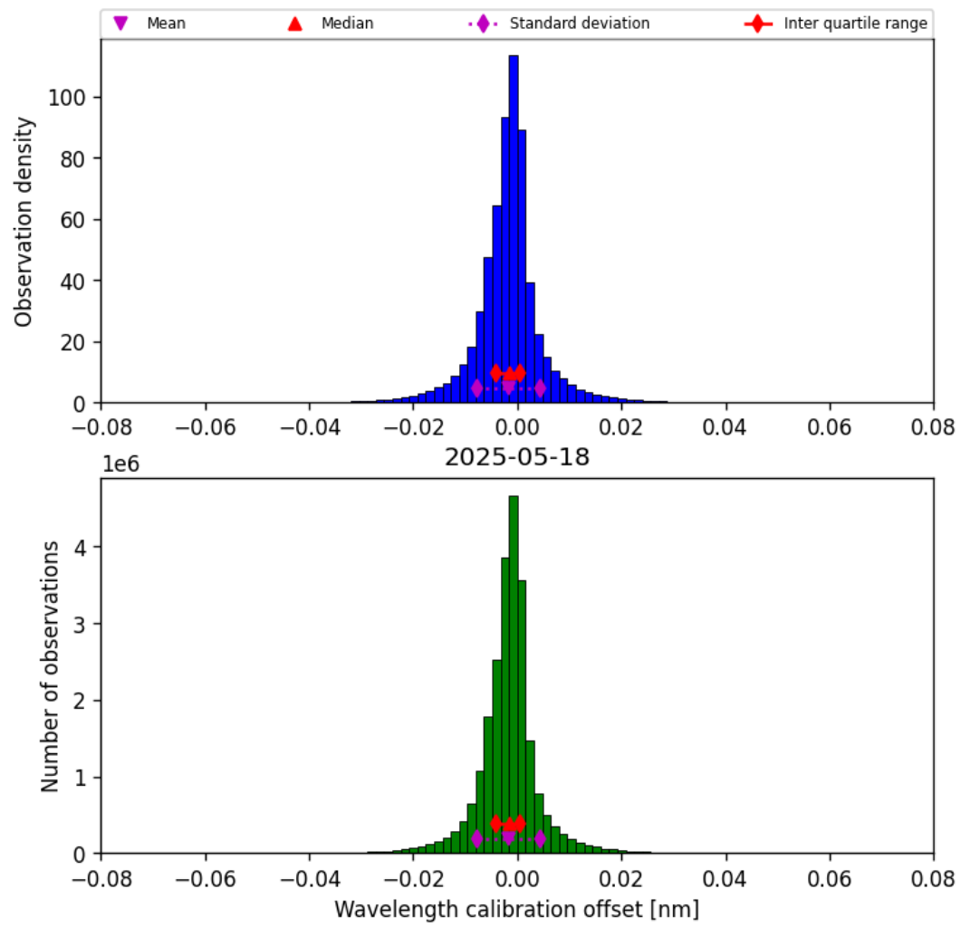
Figure 33: Histogram of “Wavelength calibration offset” for 2025-05-18 to 2025-05-19
