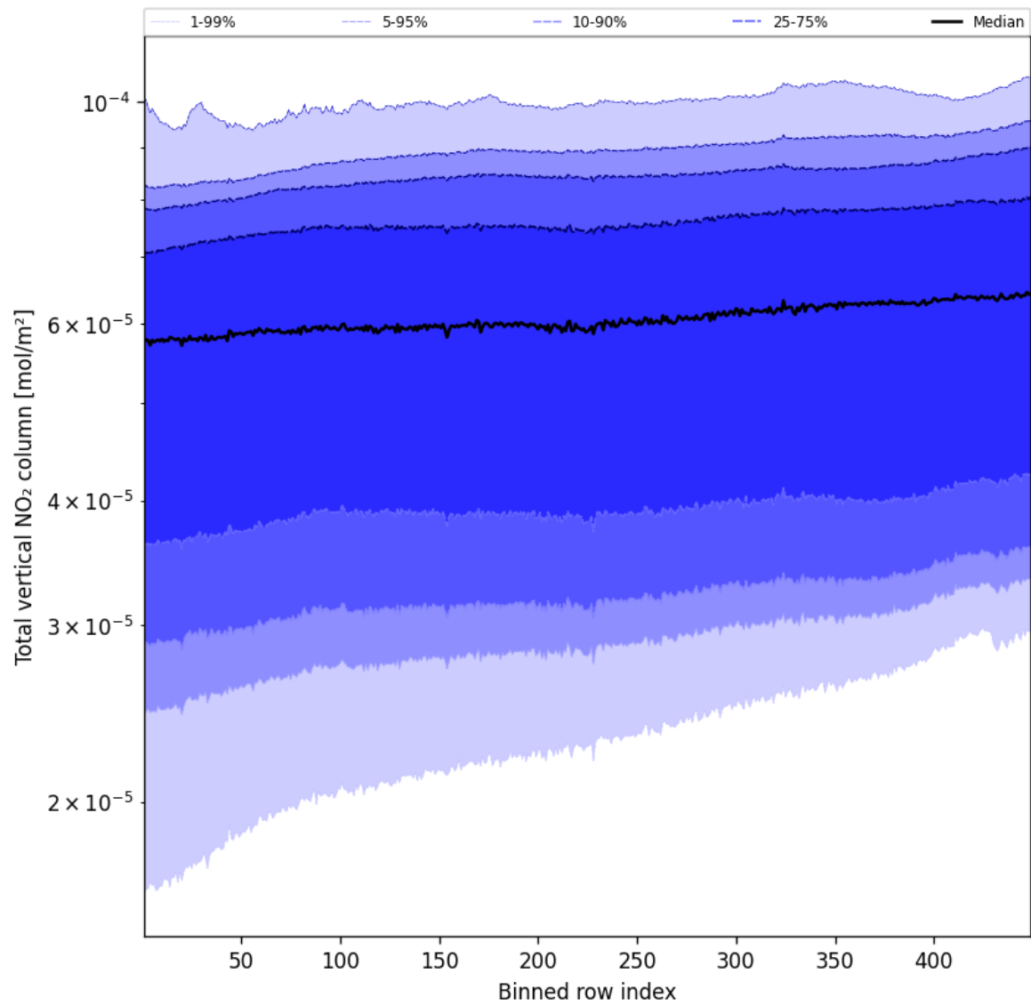
Figure 53: Along track statistics of “Total vertical NO 2 column” for 2025-05-18 to 2025-05-19
