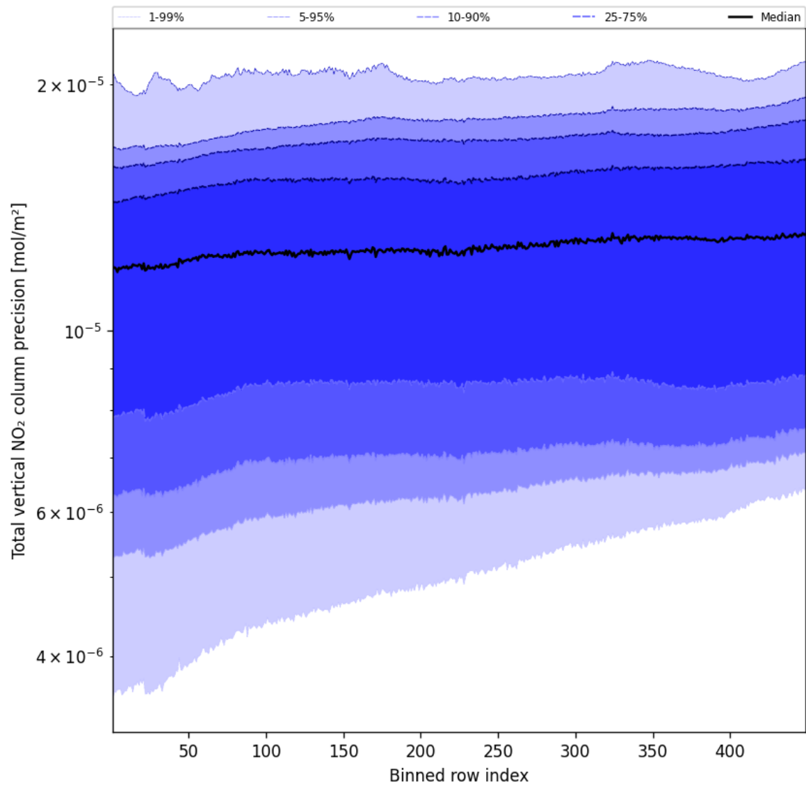
Figure 54: Along track statistics of "Total vertical NO 2 column precision" for 2025-05-18 to 2025-05-19
