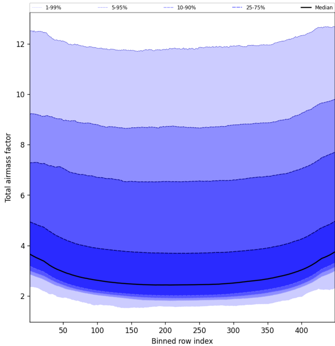
Figure 47: Along track statistics of “Total airmass factor” for 2025-05-18 to 2025-05-19
