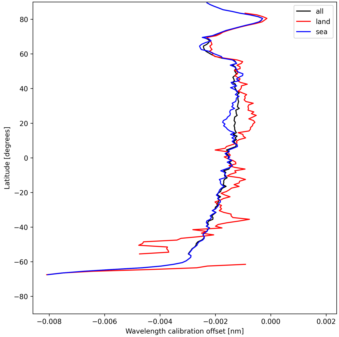
Figure 16: Zonal average of “Wavelength calibration offset” for 2025-05-18 to 2025-05-19.
