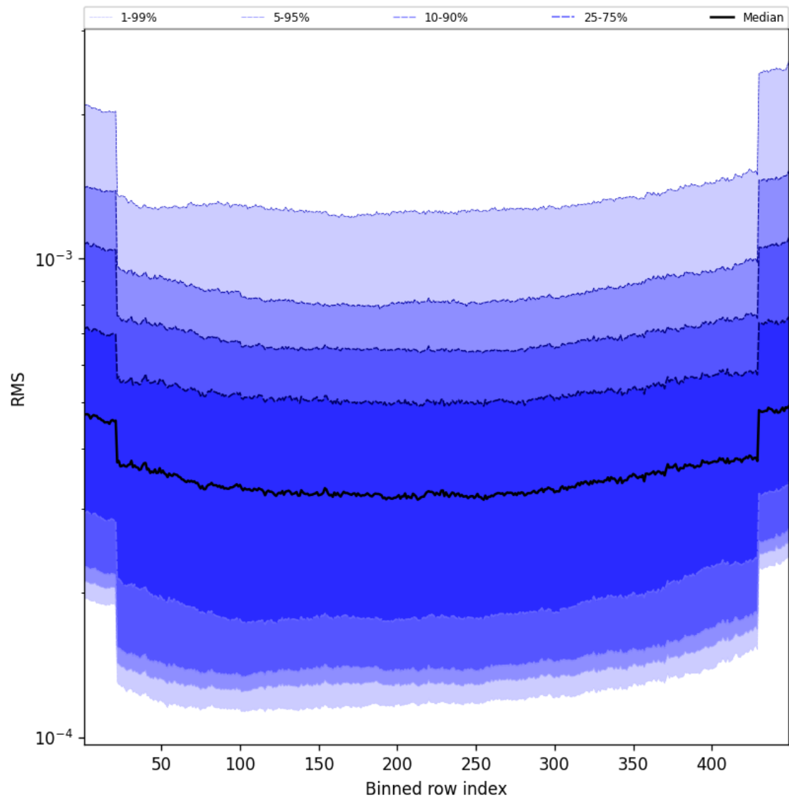
Figure 58: Along track statistics of “RMS” for 2025-05-18 to 2025-05-19
