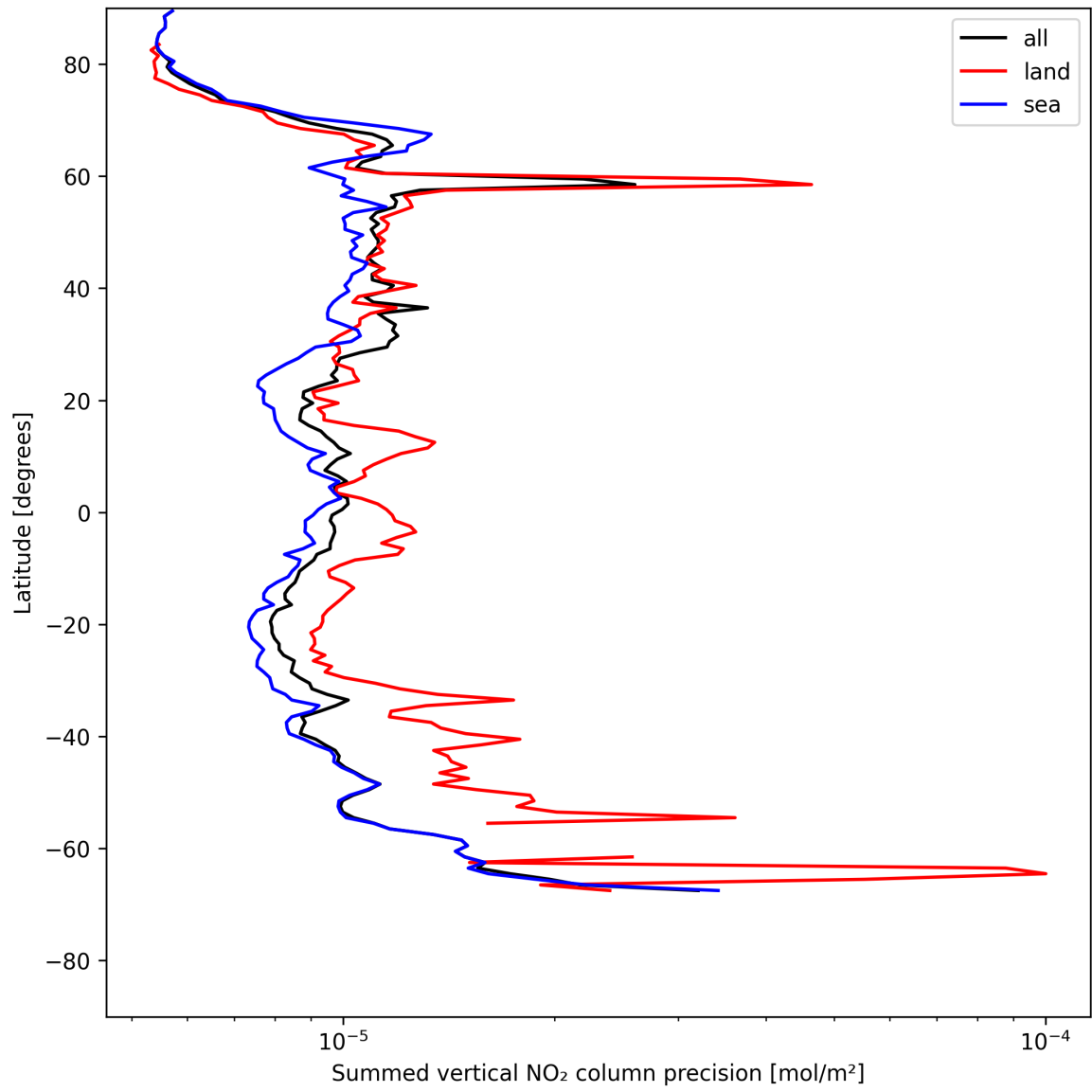
Figure 22: Zonal average of “Summed vertical NO 2 column precision” for 2025-05-18 to 2025-05-19.
