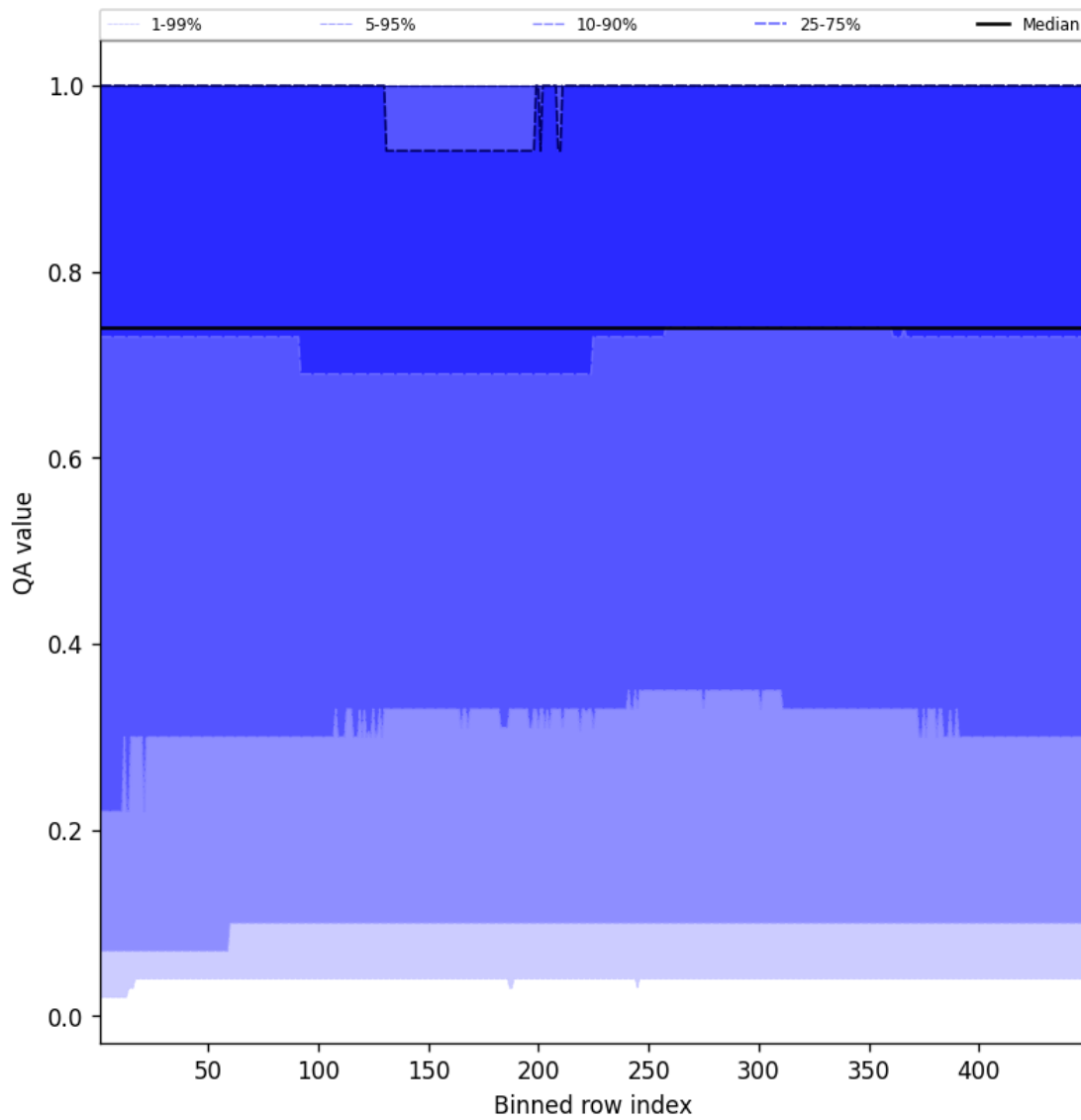
Figure 43: Along track statistics of “QA value” for 2025-05-18 to 2025-05-19
