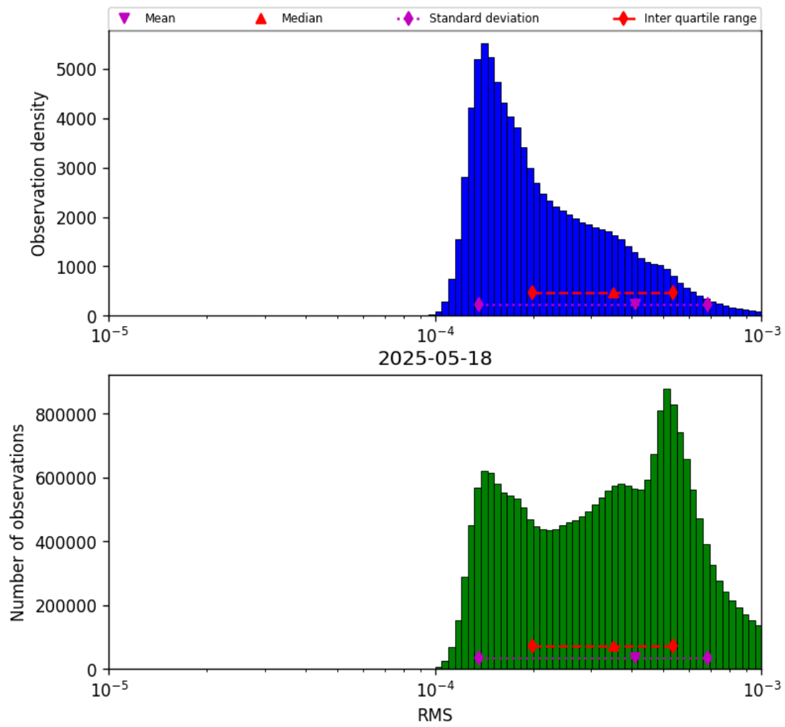
Figure 41: Histogram of “RMS” for 2025-05-18 to 2025-05-19
