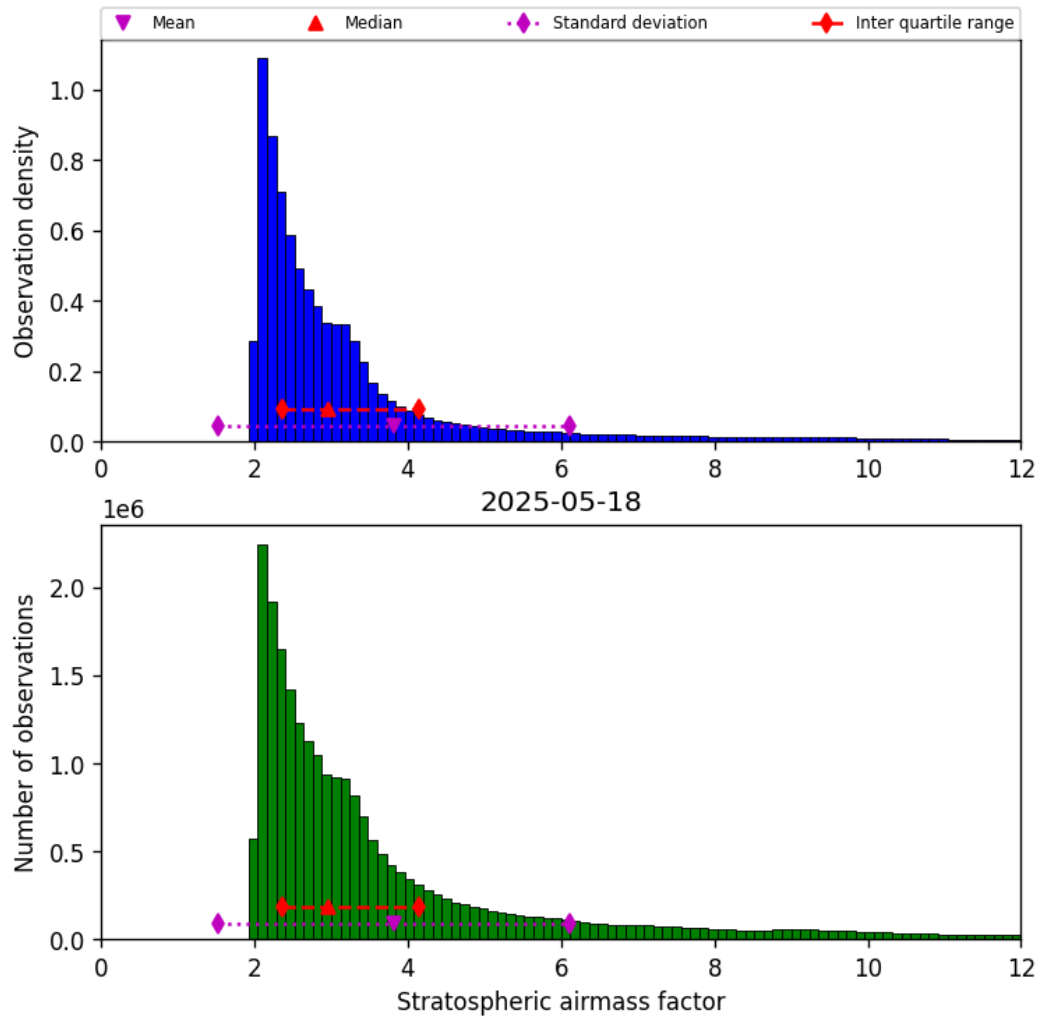
Figure 42: Histogram of “Stratospheric airmass factor” for 2025-05-18 to 2025-05-19
