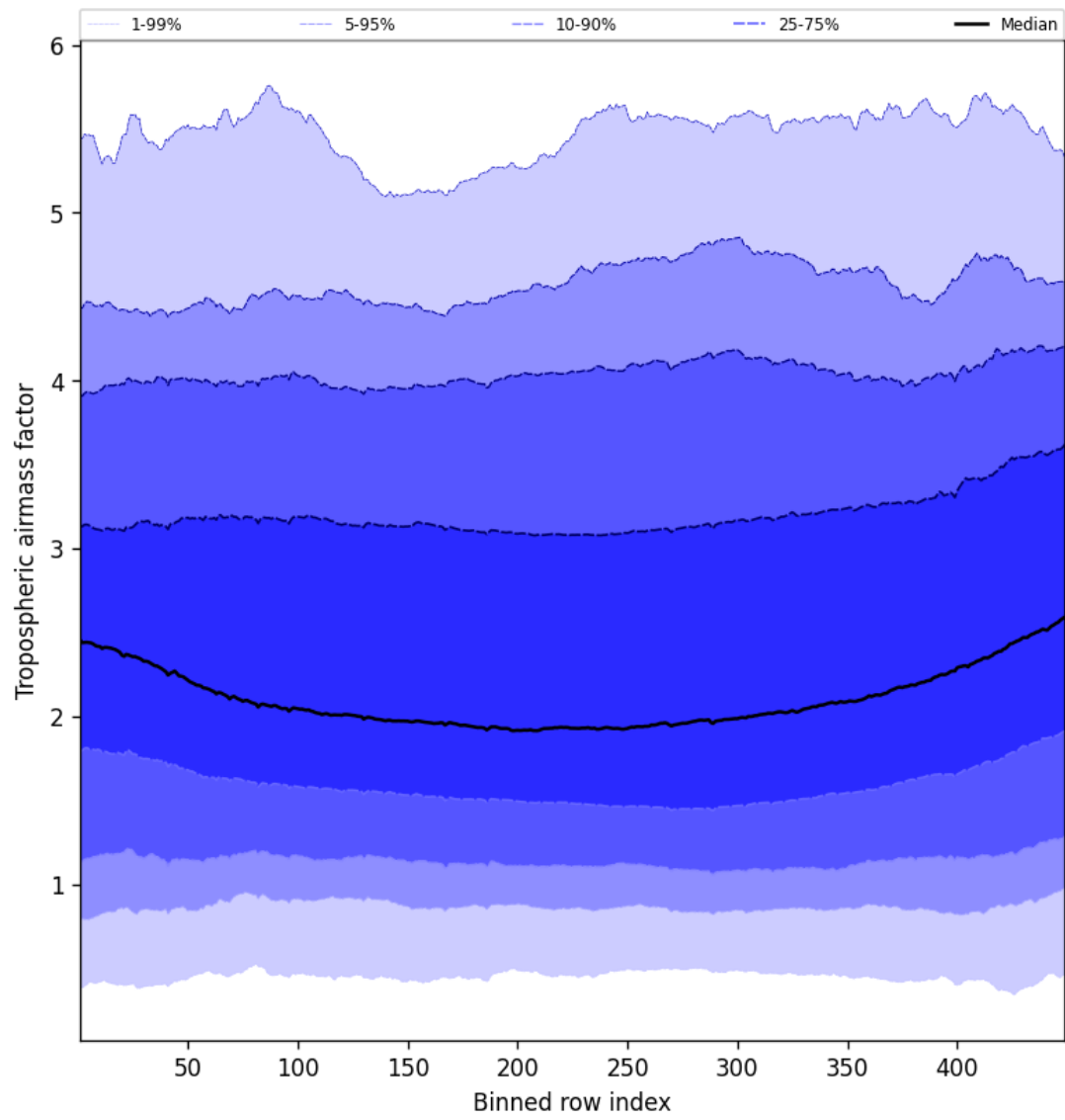
Figure 46: Along track statistics of “Tropospheric airmass factor” for 2025-05-18 to 2025-05-19
