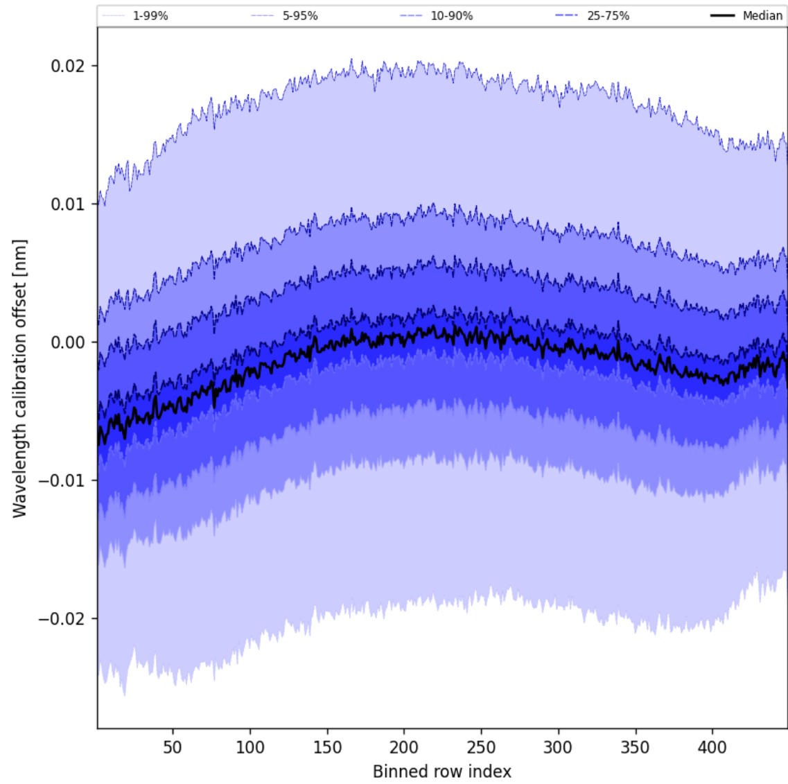
Figure 50: Along track statistics of “Wavelength calibration offset” for 2025-05-18 to 2025-05-19
