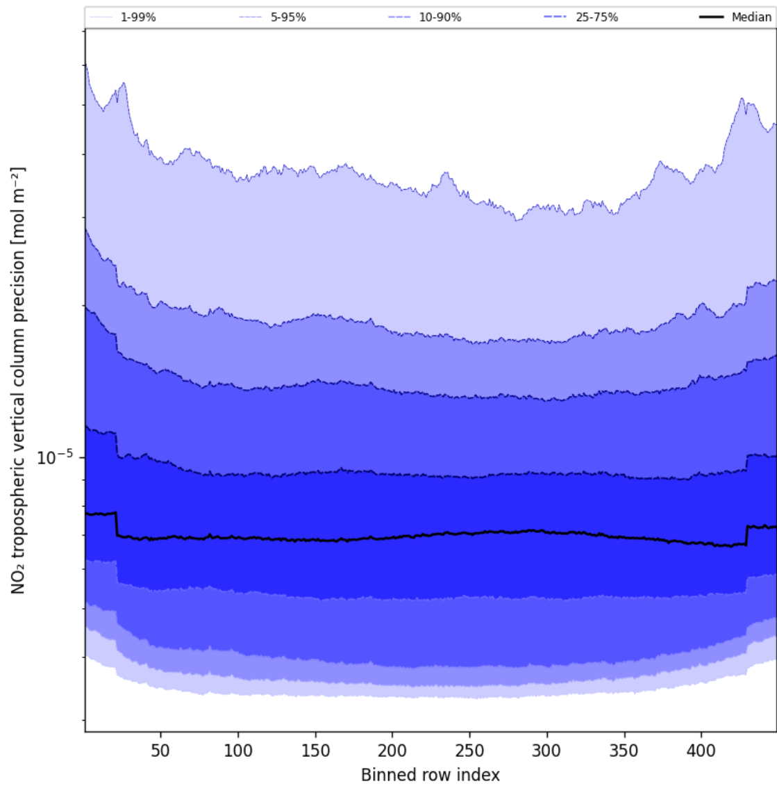
Figure 45: Along track statistics of “NO 2 tropospheric vertical column precision” for 2025-05-18 to 2025-05-19
