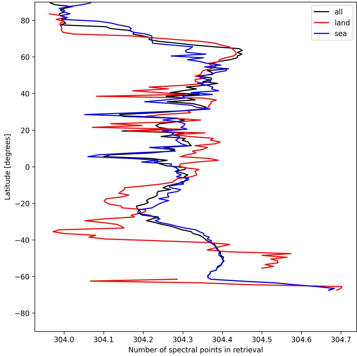
Figure 14: Zonal average of “Number of spectral points in retrieval” for 2025-05-18 to 2025-05-19.
