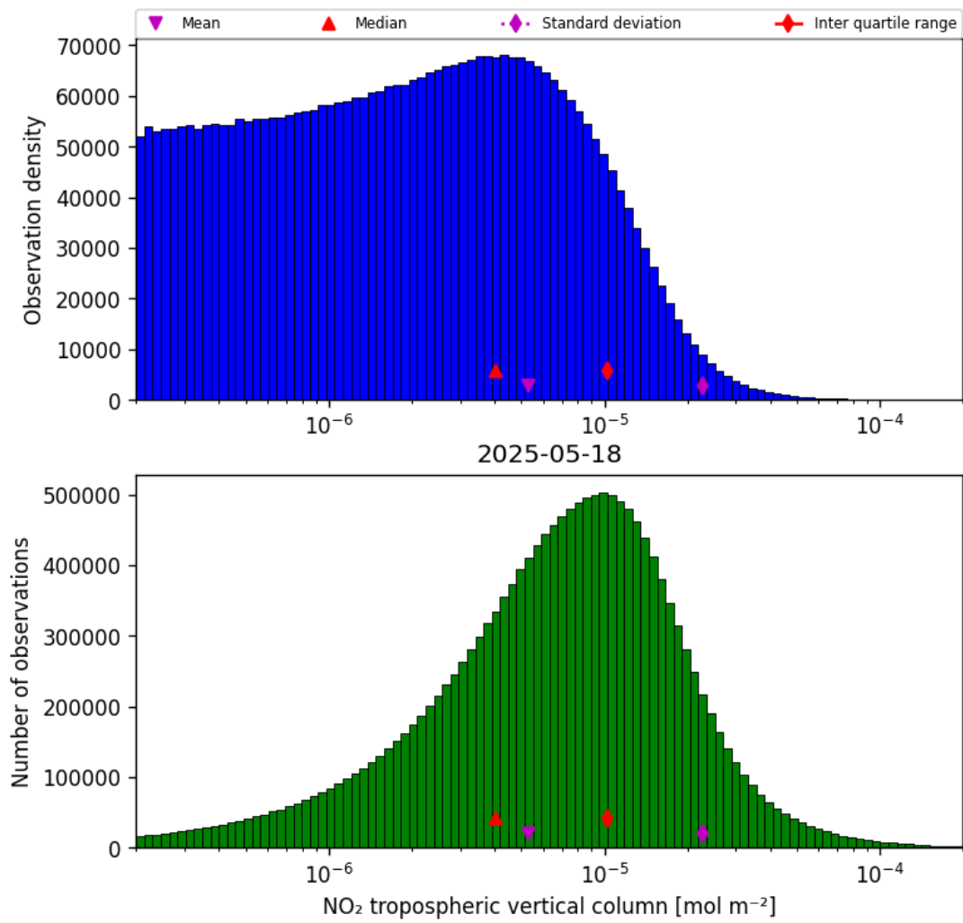
Figure 27: Histogram of “NO 2 tropospheric vertical column” for 2025-05-18 to 2025-05-19
