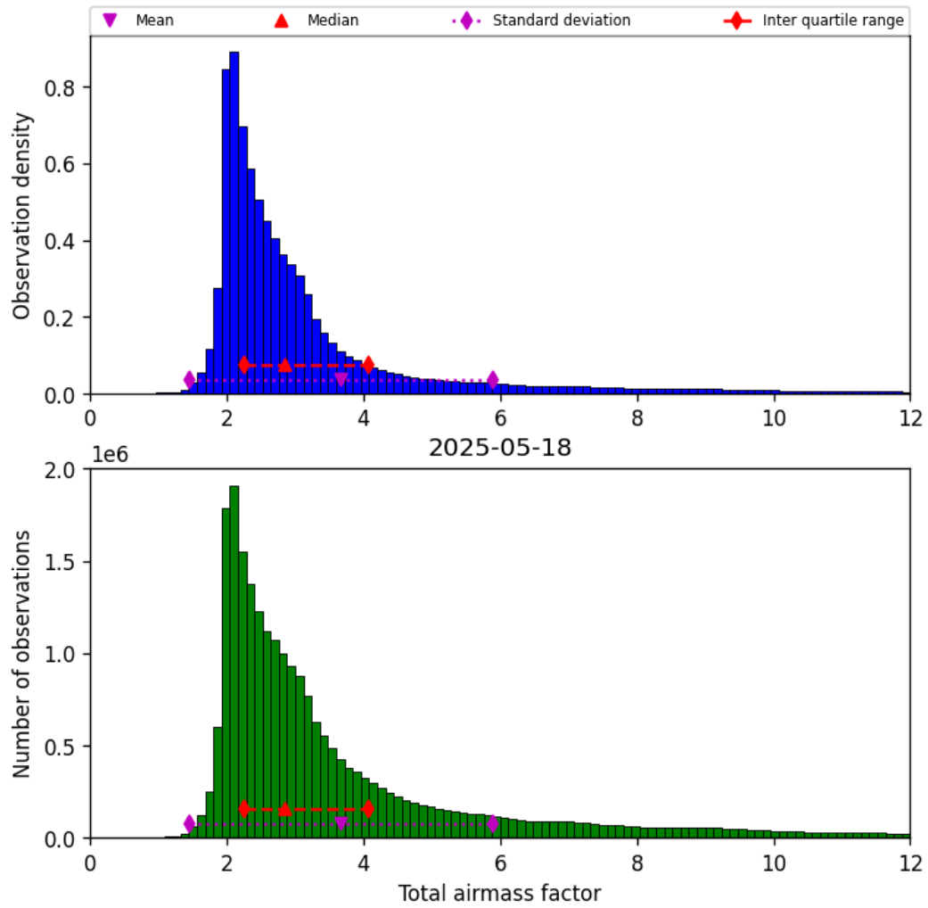
Figure 30: Histogram of “Total airmass factor” for 2025-05-18 to 2025-05-19
