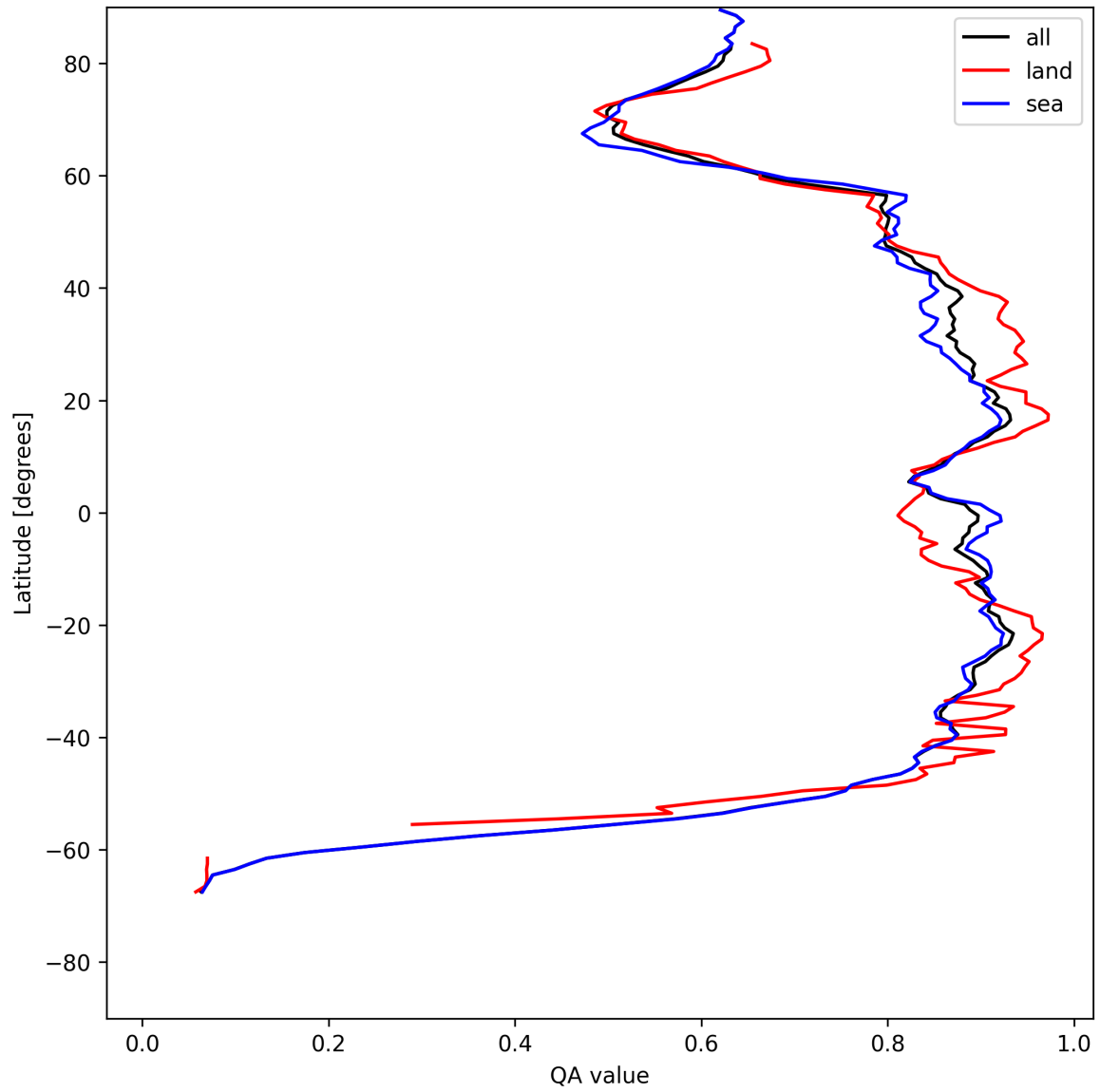
Figure 9: Zonal average of “QA value” for 2025-05-18 to 2025-05-19.
