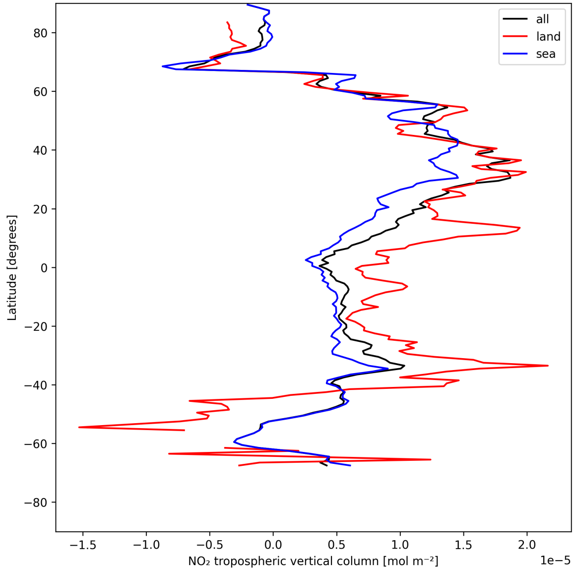
Figure 10: Zonal average of “NO 2 tropospheric vertical column” for 2025-05-18 to 2025-05-19.
