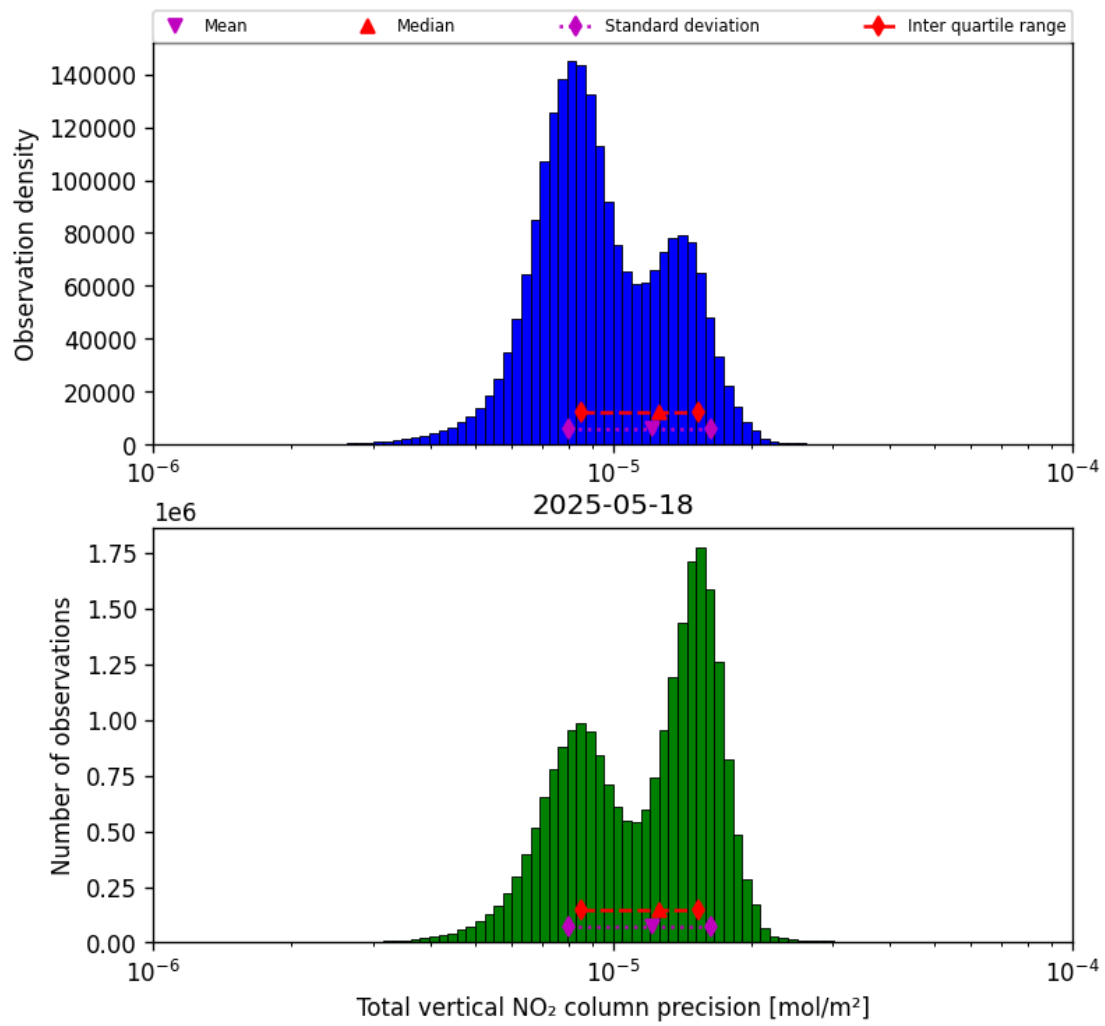
Figure 37: Histogram of “Total vertical NO 2 column precision” for 2025-05-18 to 2025-05-19
