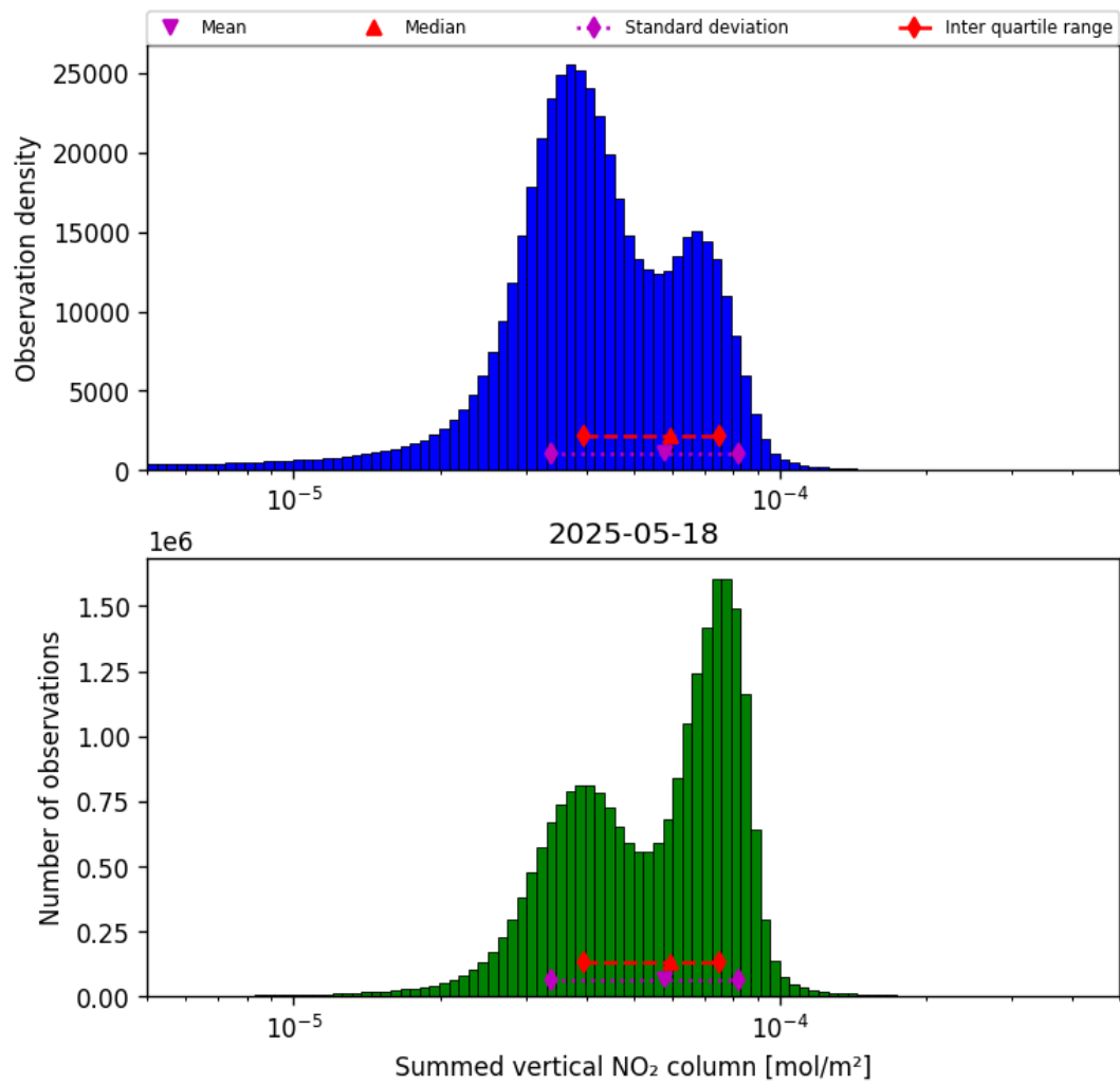
Figure 38: Histogram of “Summed vertical NO 2 column” for 2025-05-18 to 2025-05-19
