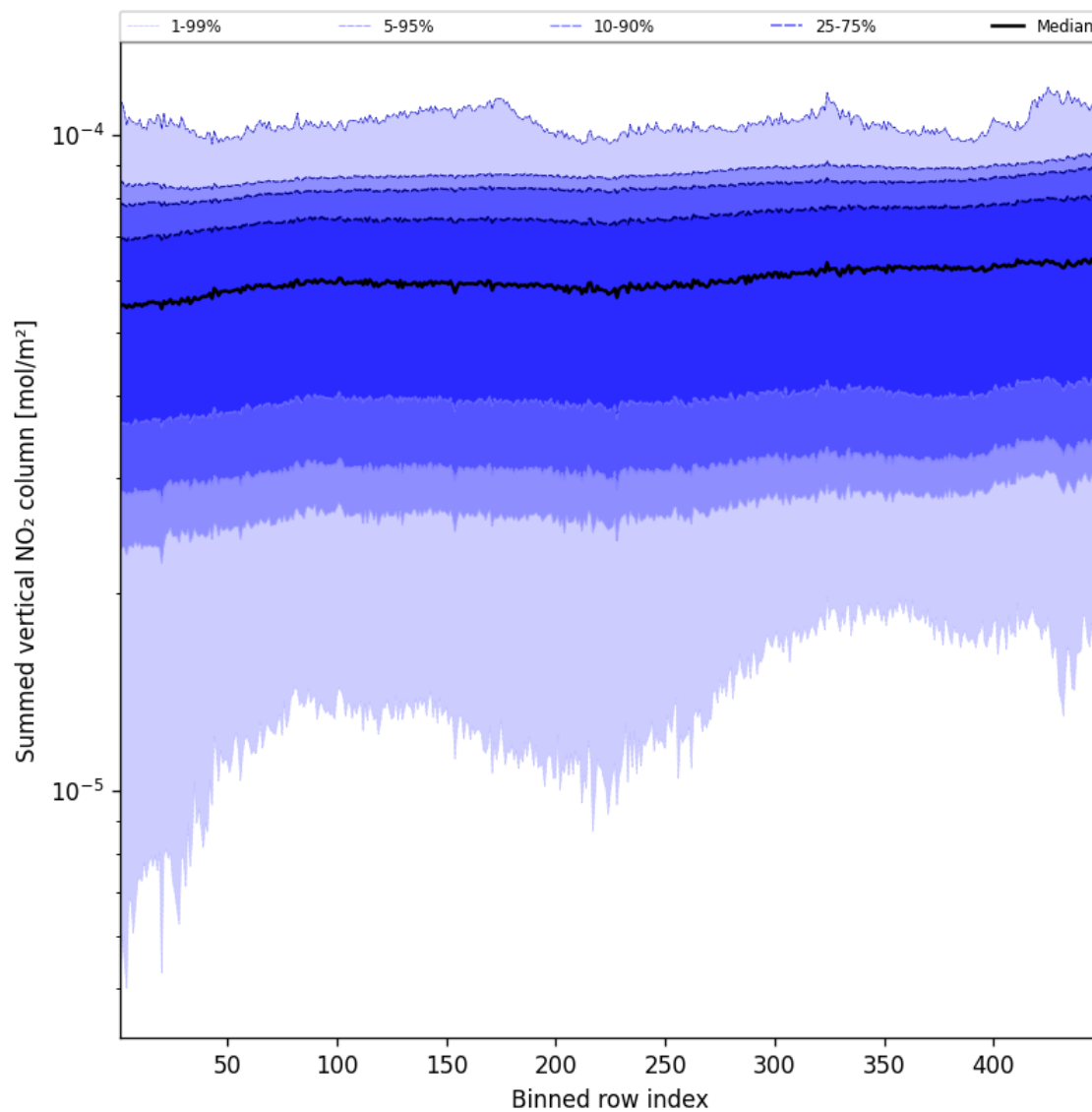
Figure 55: Along track statistics of “Summed vertical NO 2 column” for 2025-05-18 to 2025-05-19
