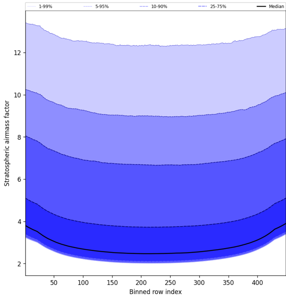
Figure 59: Along track statistics of “Stratospheric airmass factor” for 2025-05-18 to 2025-05-19
