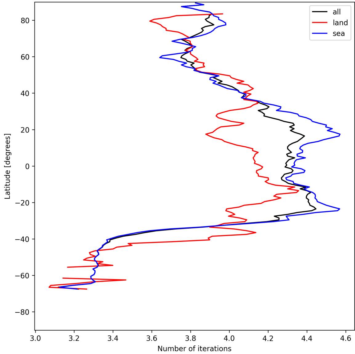
Figure 15: Zonal average of “Number of iterations” for 2025-05-18 to 2025-05-19.
