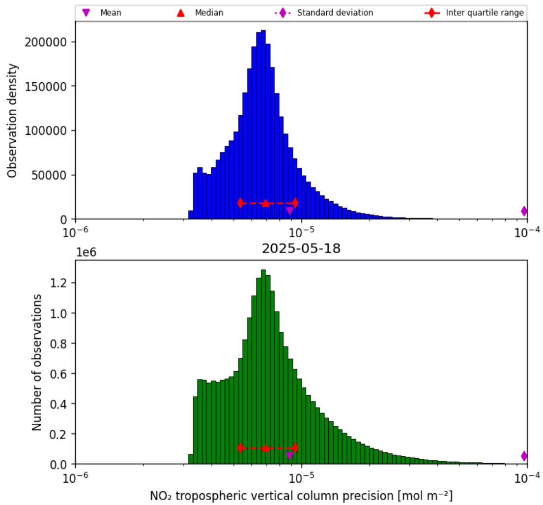
Figure 28: Histogram of “NO 2 tropospheric vertical column precision” for 2025-05-18 to 2025-05-19
