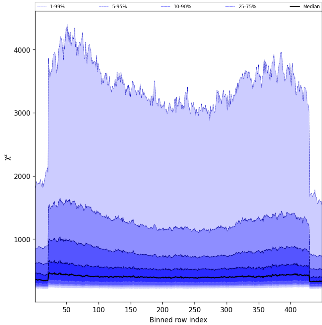
Figure 57: Along track statistics of “ \chi^2 ” for 2025-05-18 to 2025-05-19
