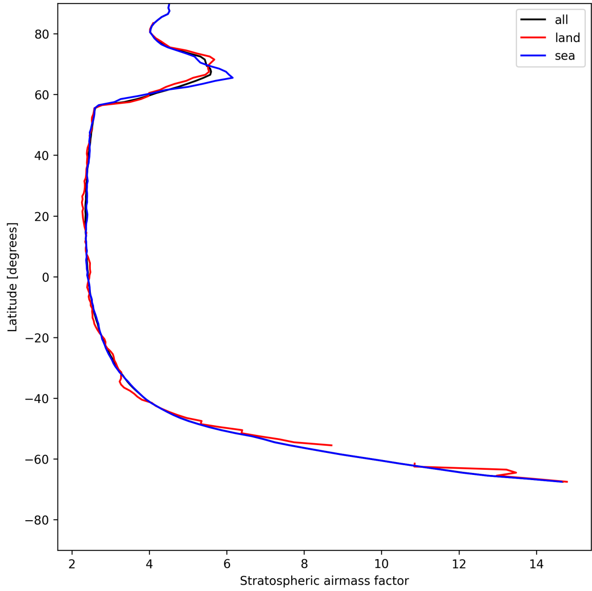
Figure 25: Zonal average of “Stratospheric air mass factor” for 2025-05-18 to 2025-05-19.
