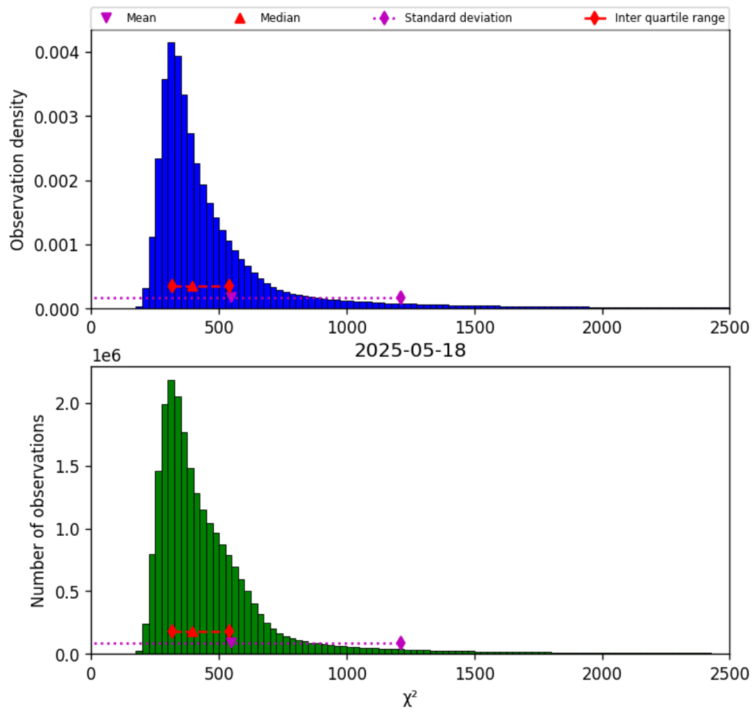
Figure 40: Histogram of “ \chi^2 ” for 2025-05-18 to 2025-05-19
