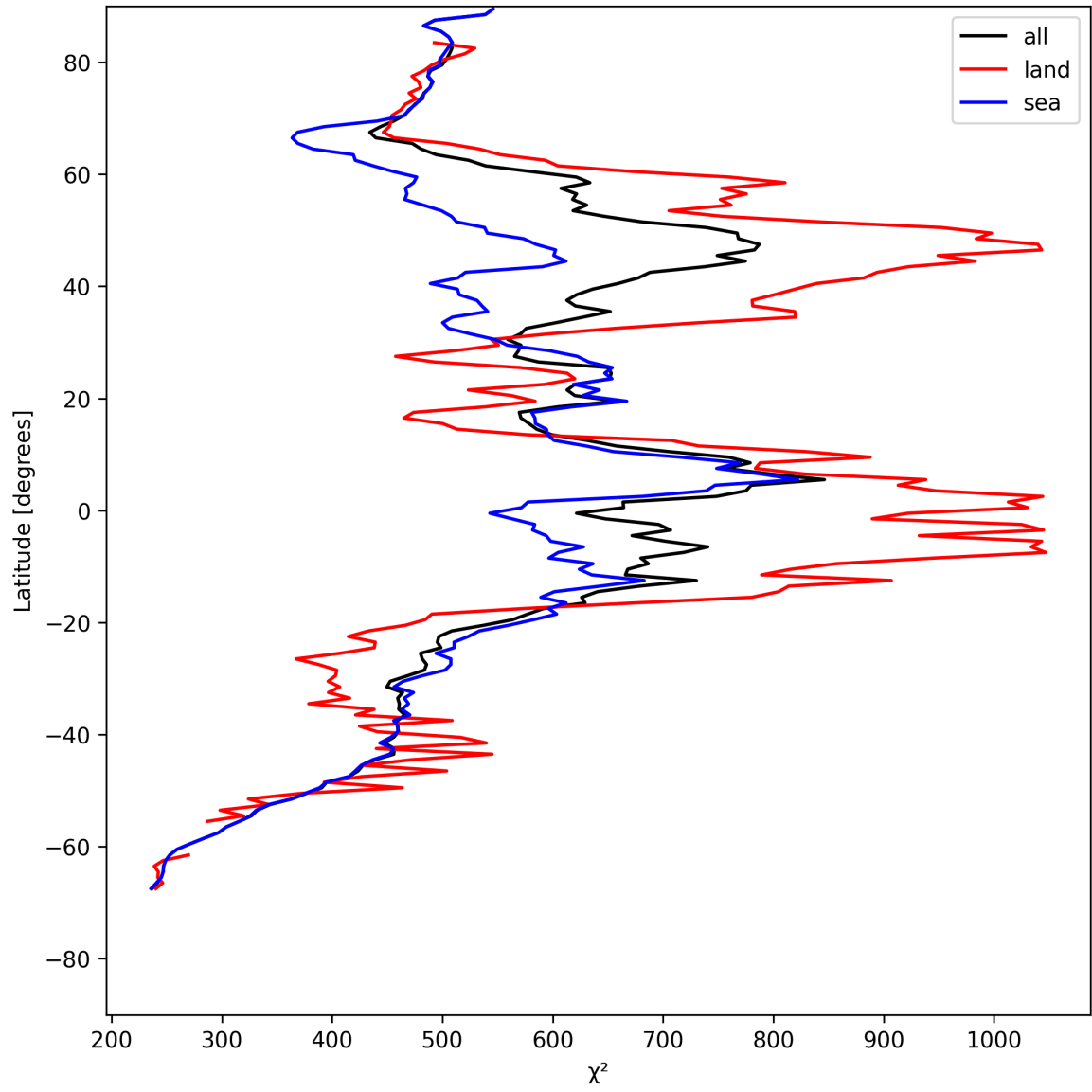
Figure 23: Zonal average of “ \chi^2 ” for 2025-05-18 to 2025-05-19.
