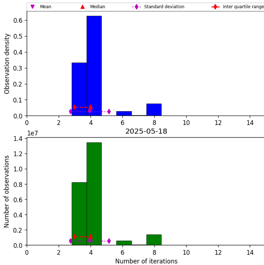
Figure 32: Histogram of “Number of iterations” for 2025-05-18 to 2025-05-19
