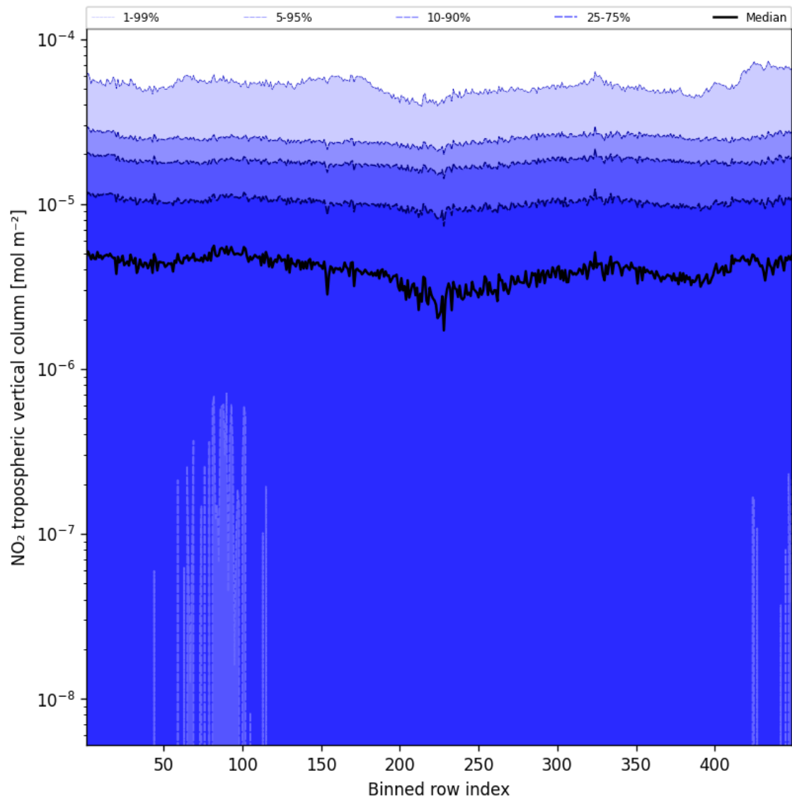
Figure 44: Along track statistics of “NO 2 tropospheric vertical column” for 2025-05-18 to 2025-05-19
