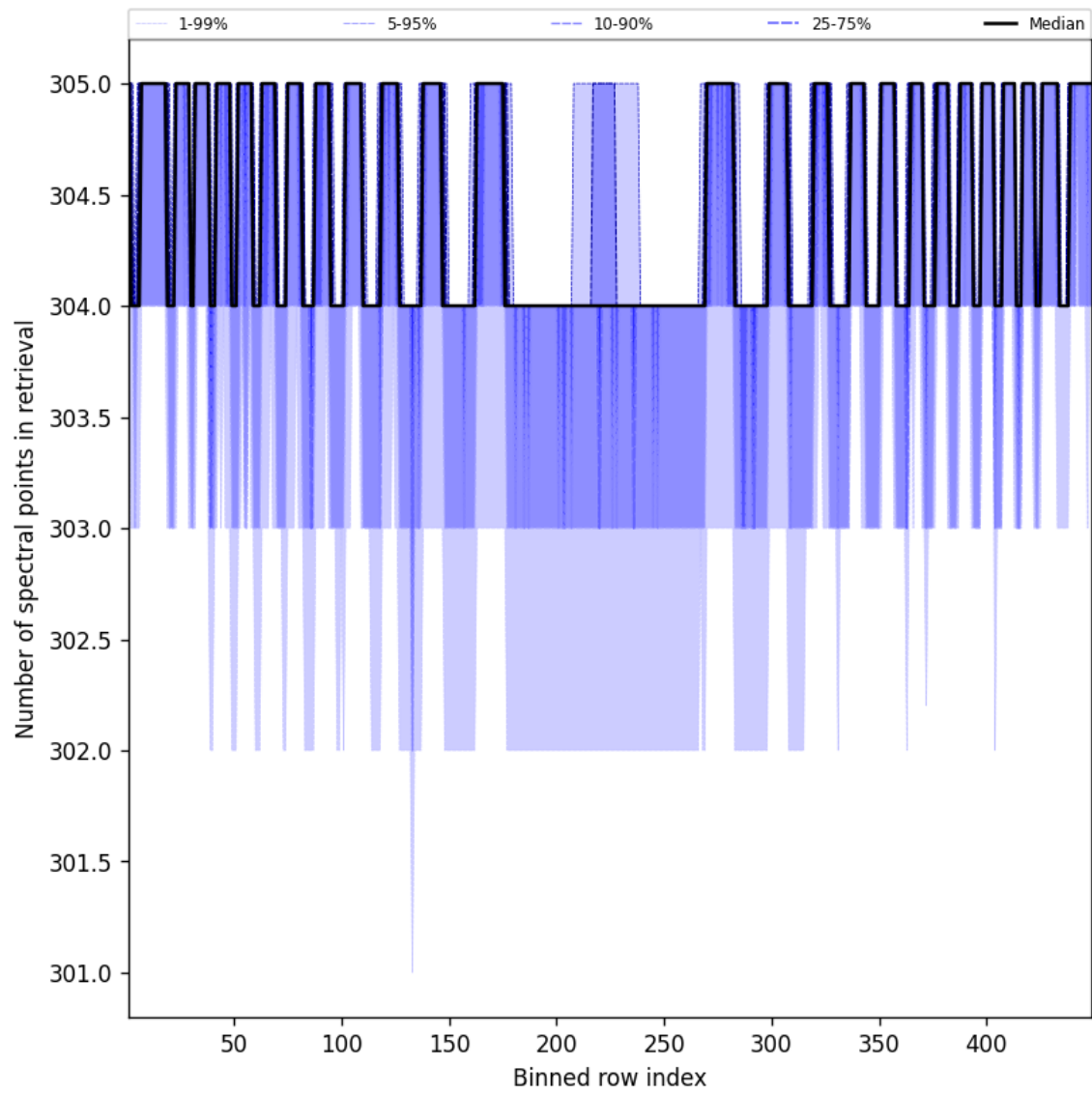
Figure 48: Along track statistics of “Number of spectral points in retrieval” for 2025-05-18 to 2025-05-19
