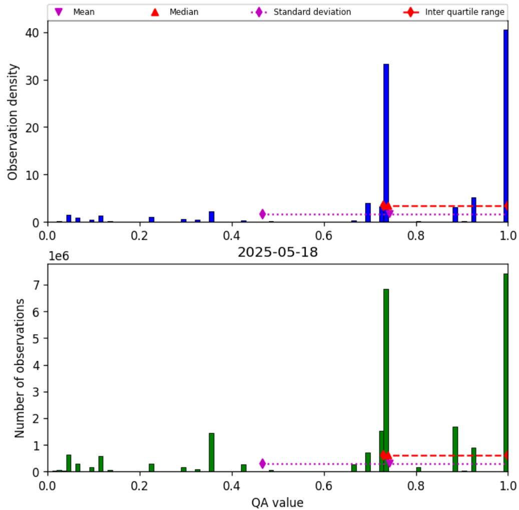
Figure 26: Histogram of “QA value” for 2025-05-18 to 2025-05-19
