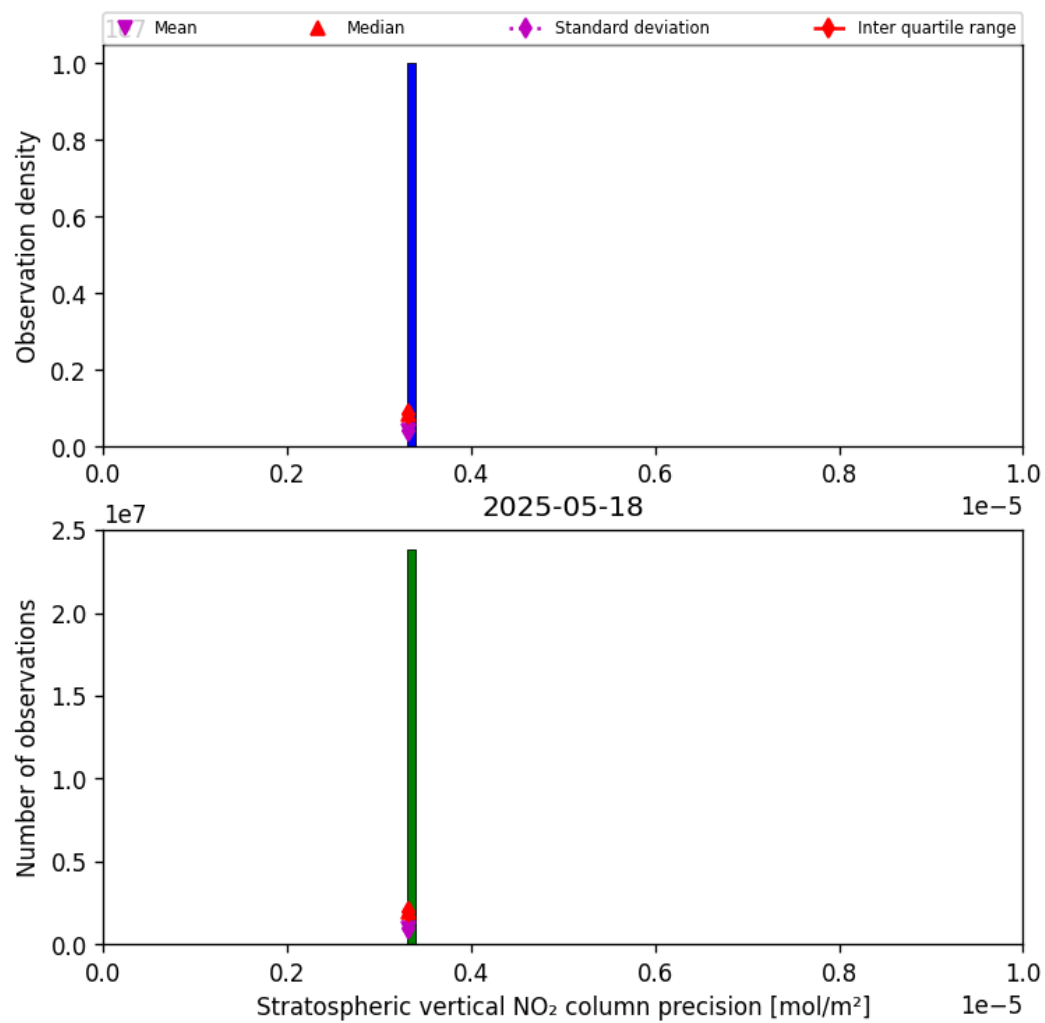
Figure 35: Histogram of “Stratospheric vertical NO 2 column precision” for 2025-05-18 to 2025-05-19
