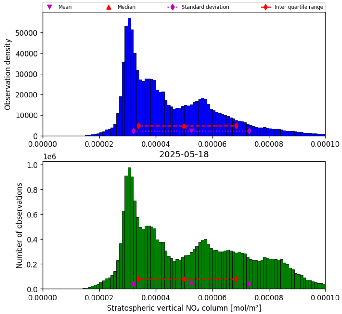
Figure 34: Histogram of “Stratospheric vertical NO 2 column” for 2025-05-18 to 2025-05-19
