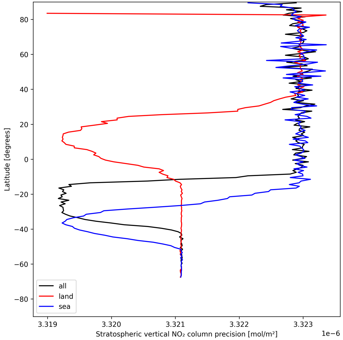
Figure 18: Zonal average of “Stratospheric vertical NO 2 column precision” for 2025-05-18 to 2025-05-19.
