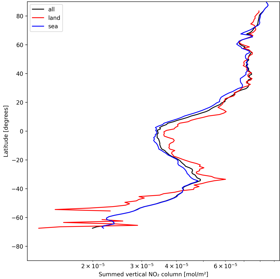
Figure 21: Zonal average of “Summed vertical NO 2 column” for 2025-05-18 to 2025-05-19.
