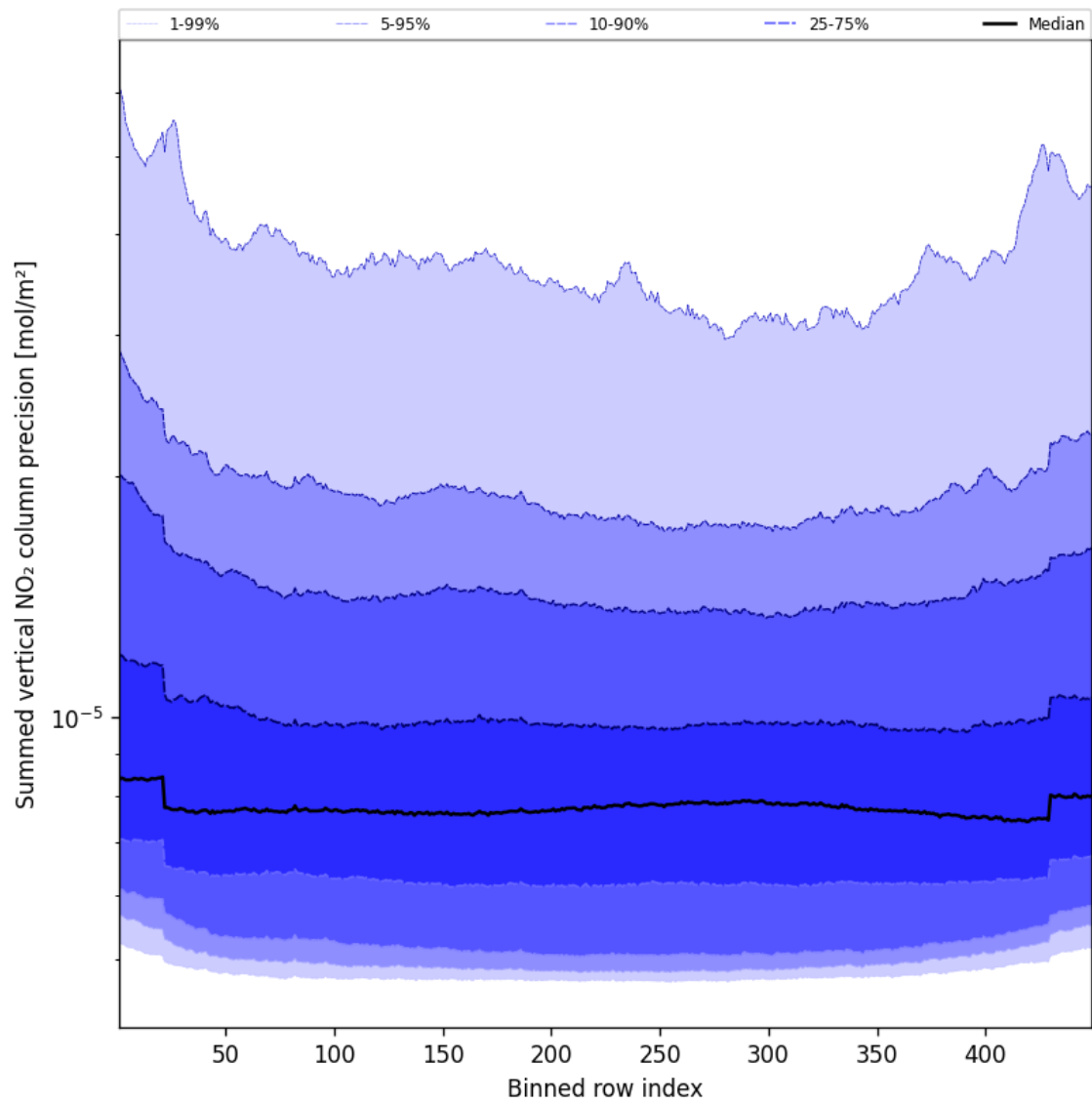
Figure 56: Along track statistics of “Summed vertical NO 2 column precision” for 2025-05-18 to 2025-05-19
