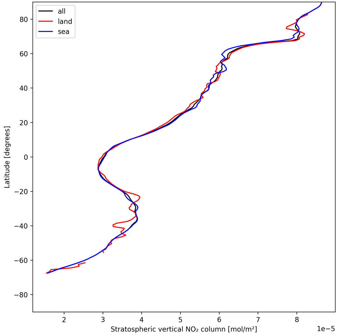
Figure 17: Zonal average of “Stratospheric vertical NO 2 column” for 2025-05-18 to 2025-05-19.
