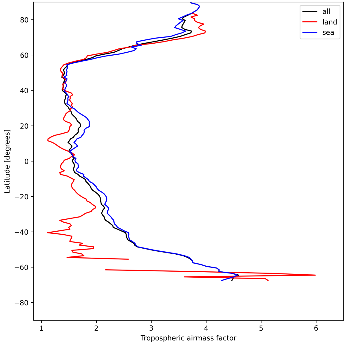
Figure 12: Zonal average of “Tropospheric airmass factor” for 2025-05-18 to 2025-05-19.
