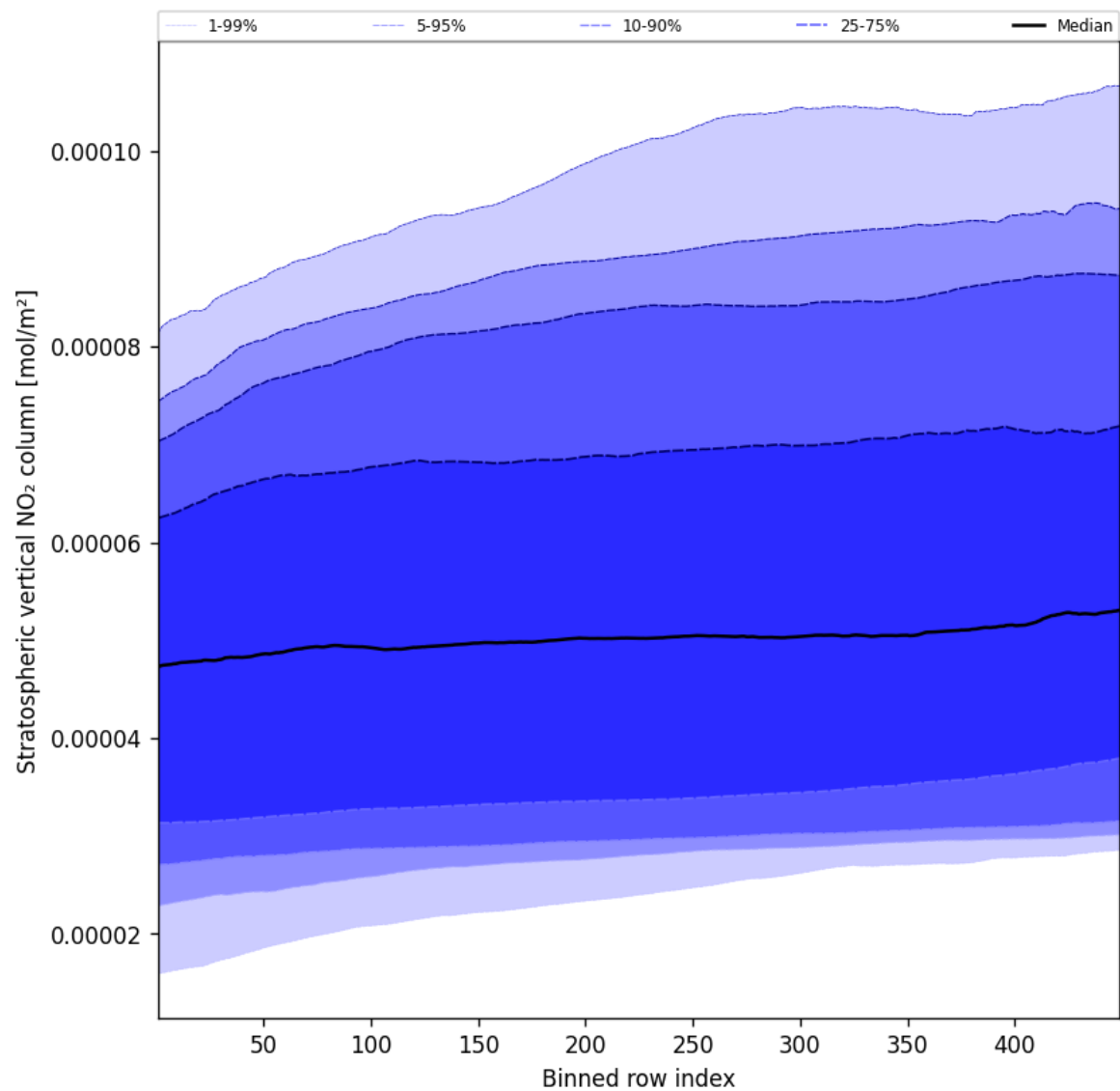
Figure 51: Along track statistics of “Stratospheric vertical NO 2 column” for 2025-05-18 to 2025-05-19
