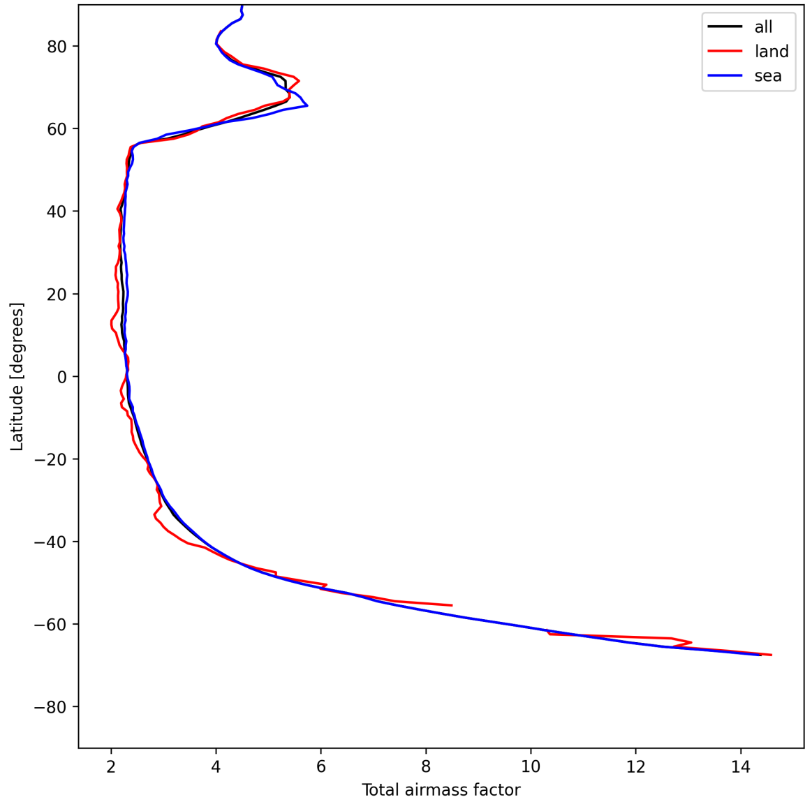
Figure 13: Zonal average of “Total airmass factor” for 2025-05-18 to 2025-05-19.
