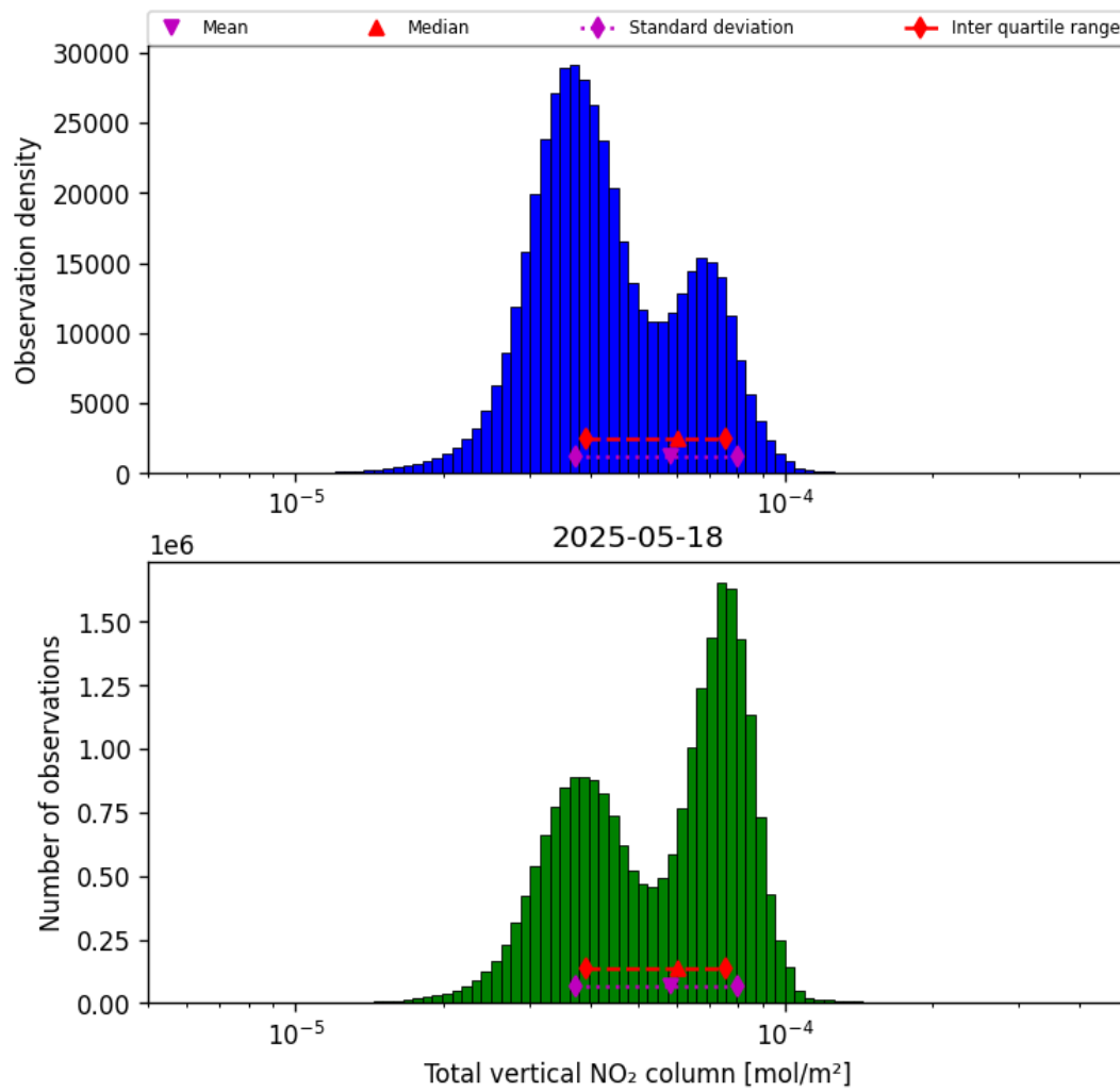
Figure 36: Histogram of “Total vertical NO 2 column” for 2025-05-18 to 2025-05-19
