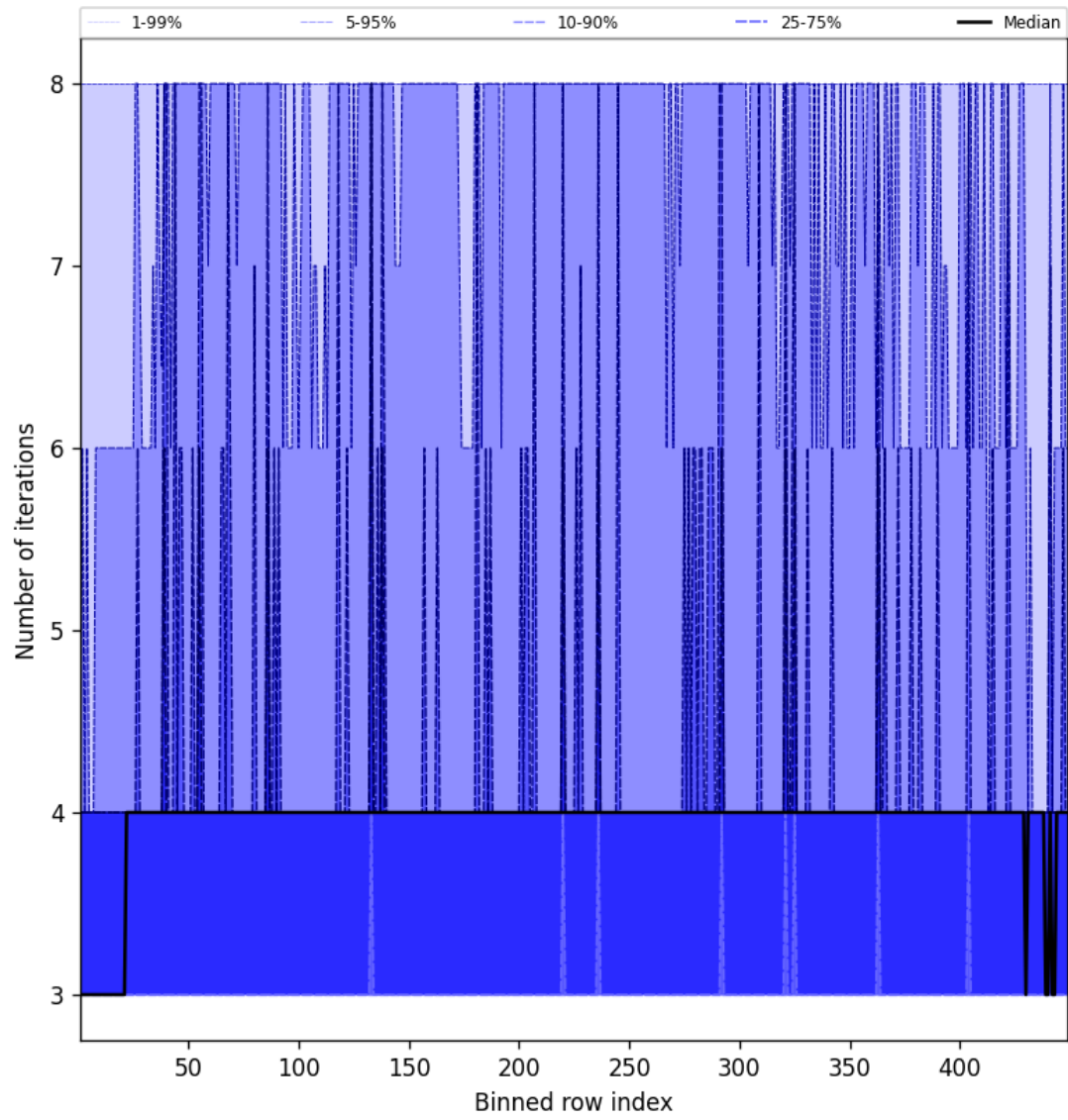
Figure 49: Along track statistics of “Number of iterations” for 2025-05-18 to 2025-05-19
