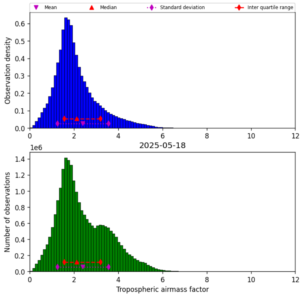
Figure 29: Histogram of “Tropospheric airmass factor” for 2025-05-18 to 2025-05-19
