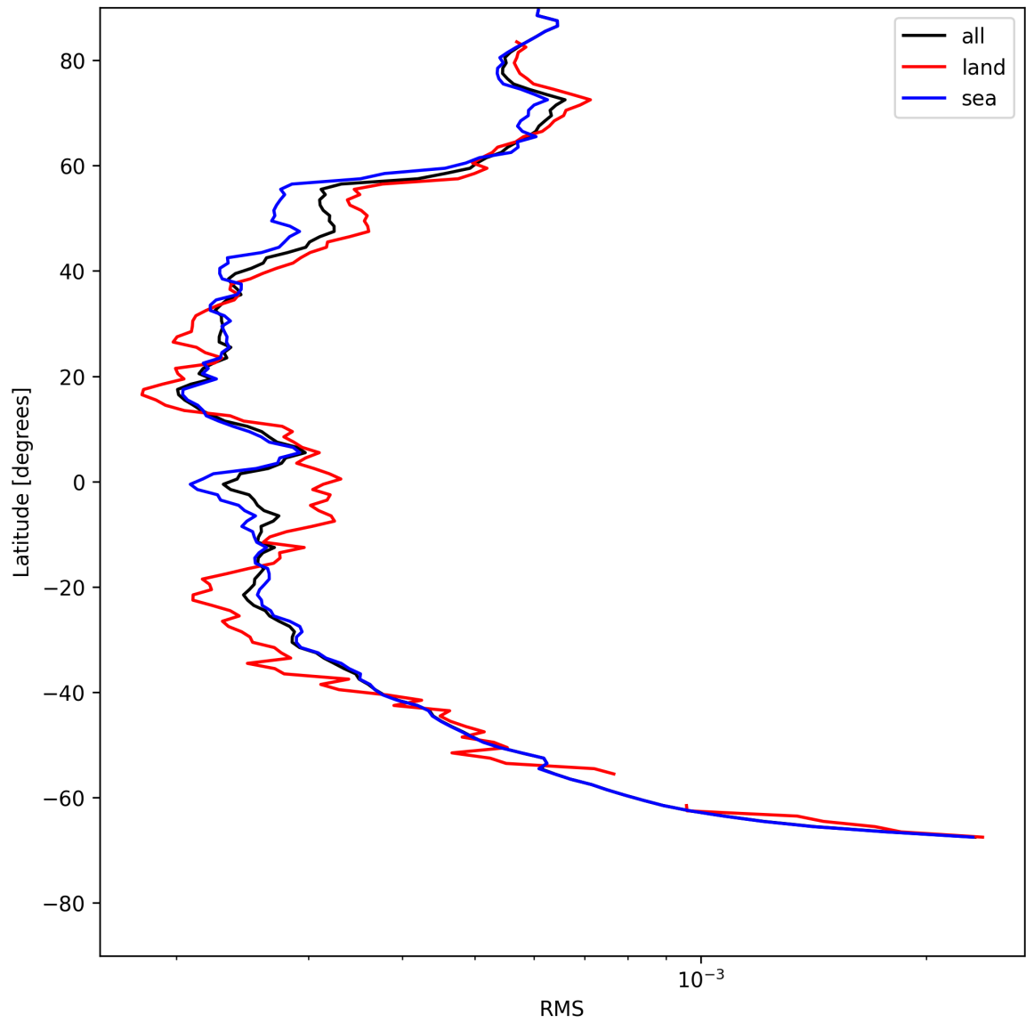
Figure 24: Zonal average of “RMS” for 2025-05-18 to 2025-05-19.
