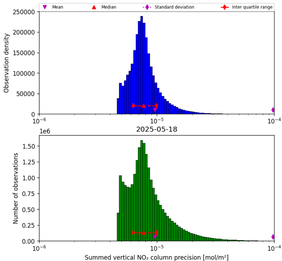
Figure 39: Histogram of "Summed vertical NO 2 column precision" for 2025-05-18 to 2025-05-19
