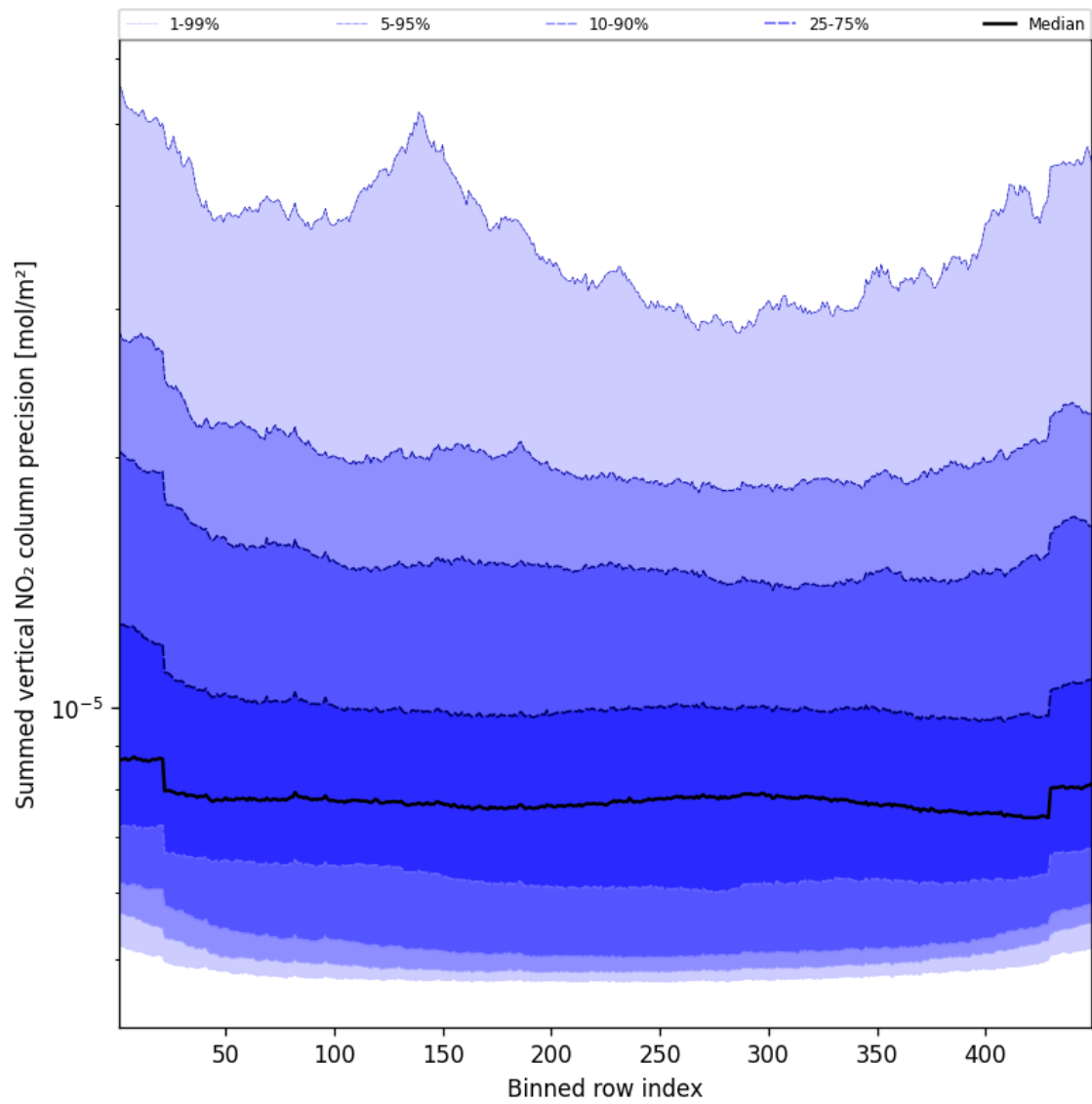
Figure 56: Along track statistics of “Summed vertical NO 2 column precision” for 2025-05-19 to 2025-05-19
