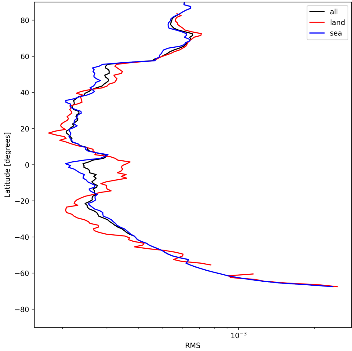
Figure 24: Zonal average of “RMS” for 2025-05-19 to 2025-05-19.
