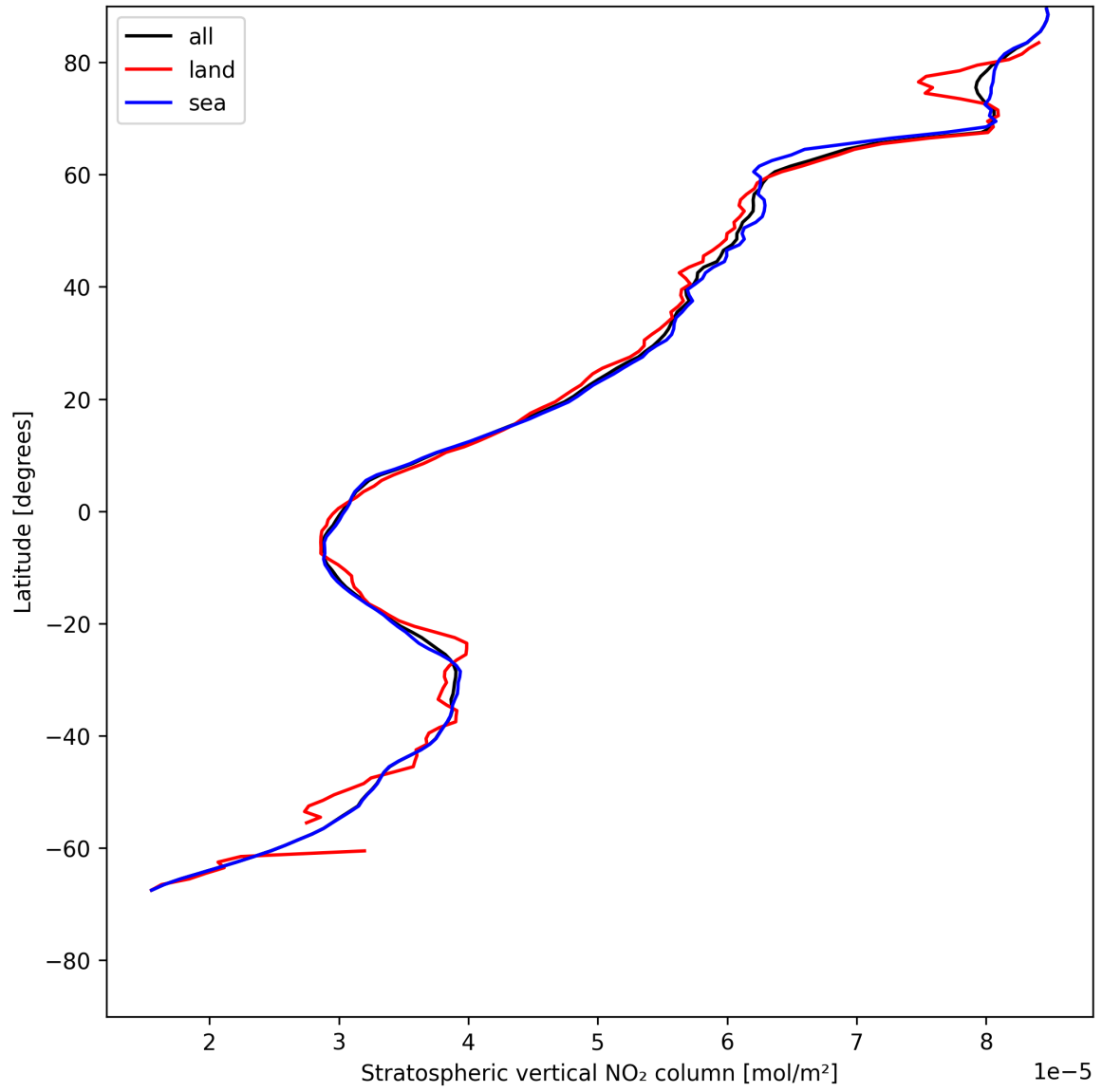
Figure 17: Zonal average of “Stratospheric vertical NO 2 column” for 2025-05-19 to 2025-05-19.
