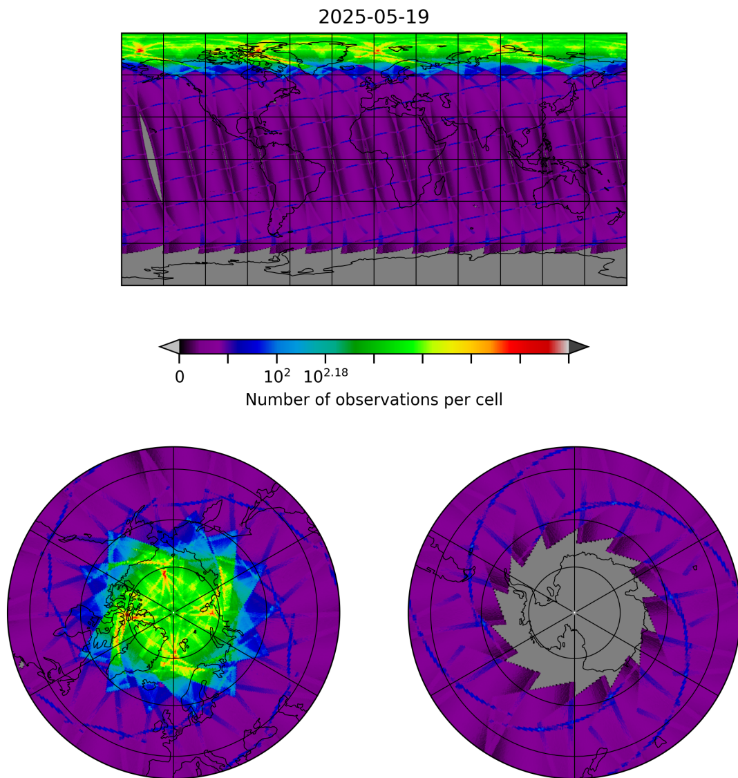
Figure 8: Map of the number of observations for 2025-05-19 to 2025-05-19
