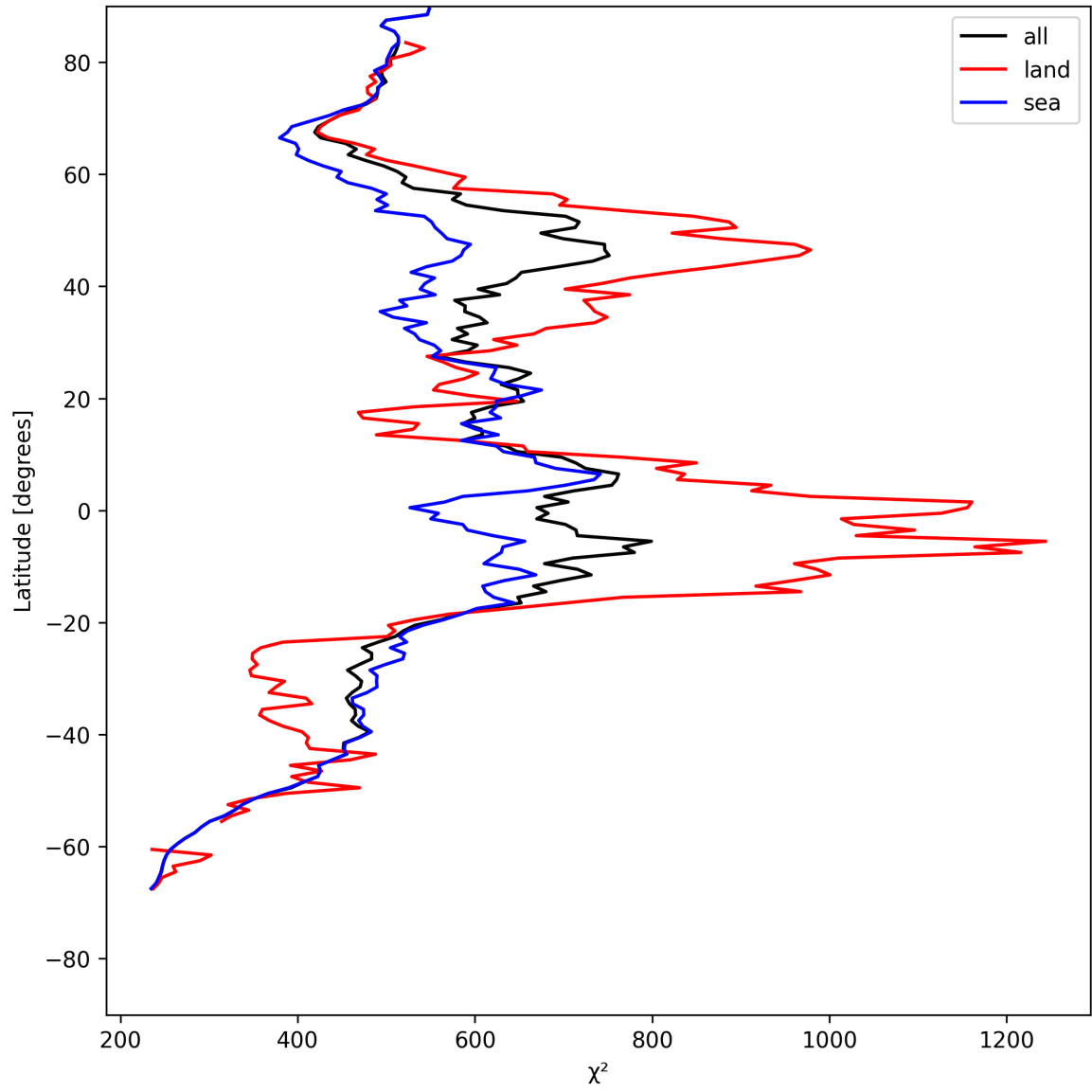
Figure 23: Zonal average of “ \chi^2 ” for 2025-05-19 to 2025-05-19.
