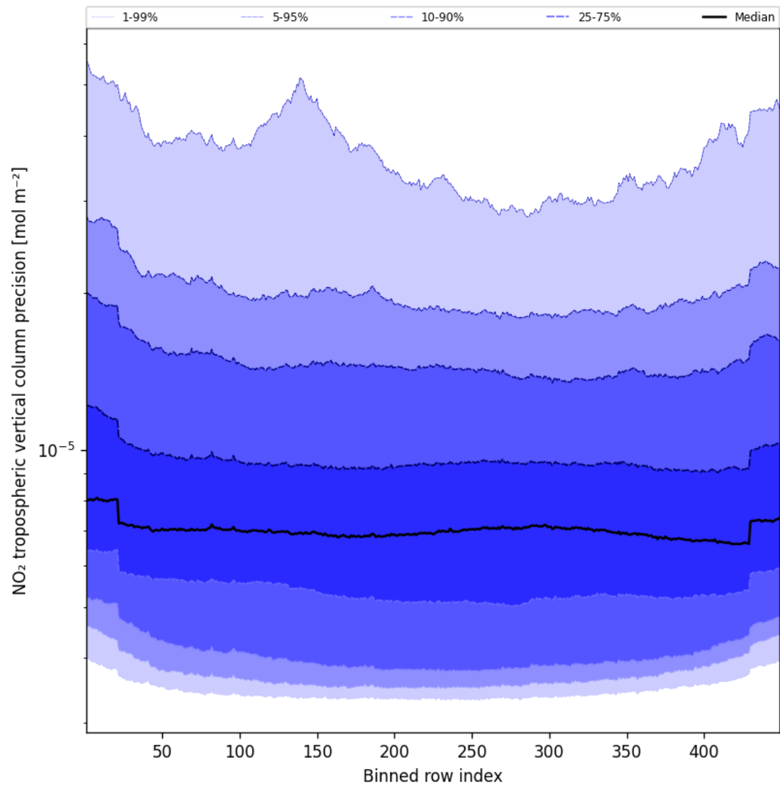
Figure 45: Along track statistics of “NO 2 tropospheric vertical column precision” for 2025-05-19 to 2025-05-19
