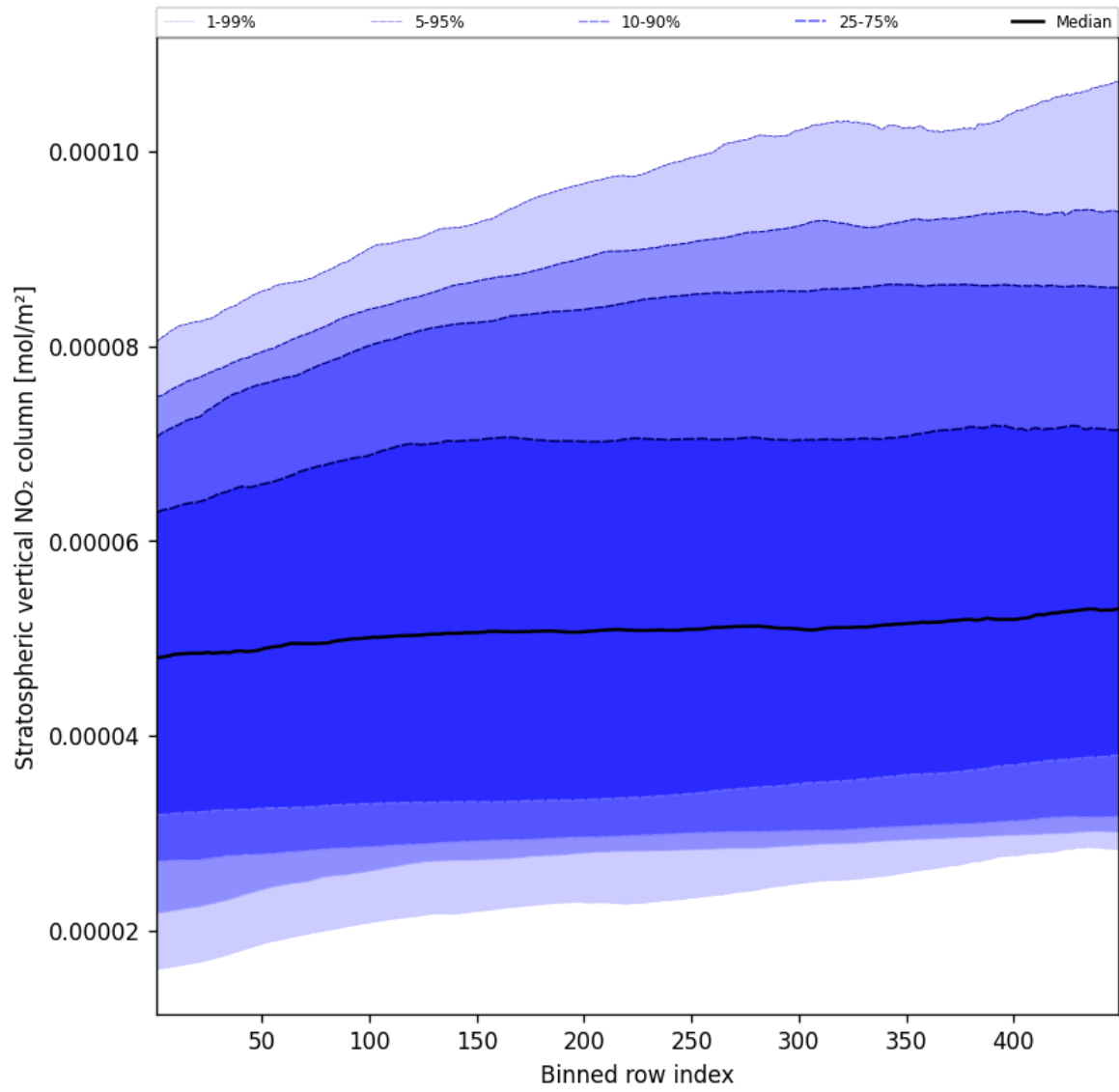
Figure 51: Along track statistics of “Stratospheric vertical NO 2 column” for 2025-05-19 to 2025-05-19
