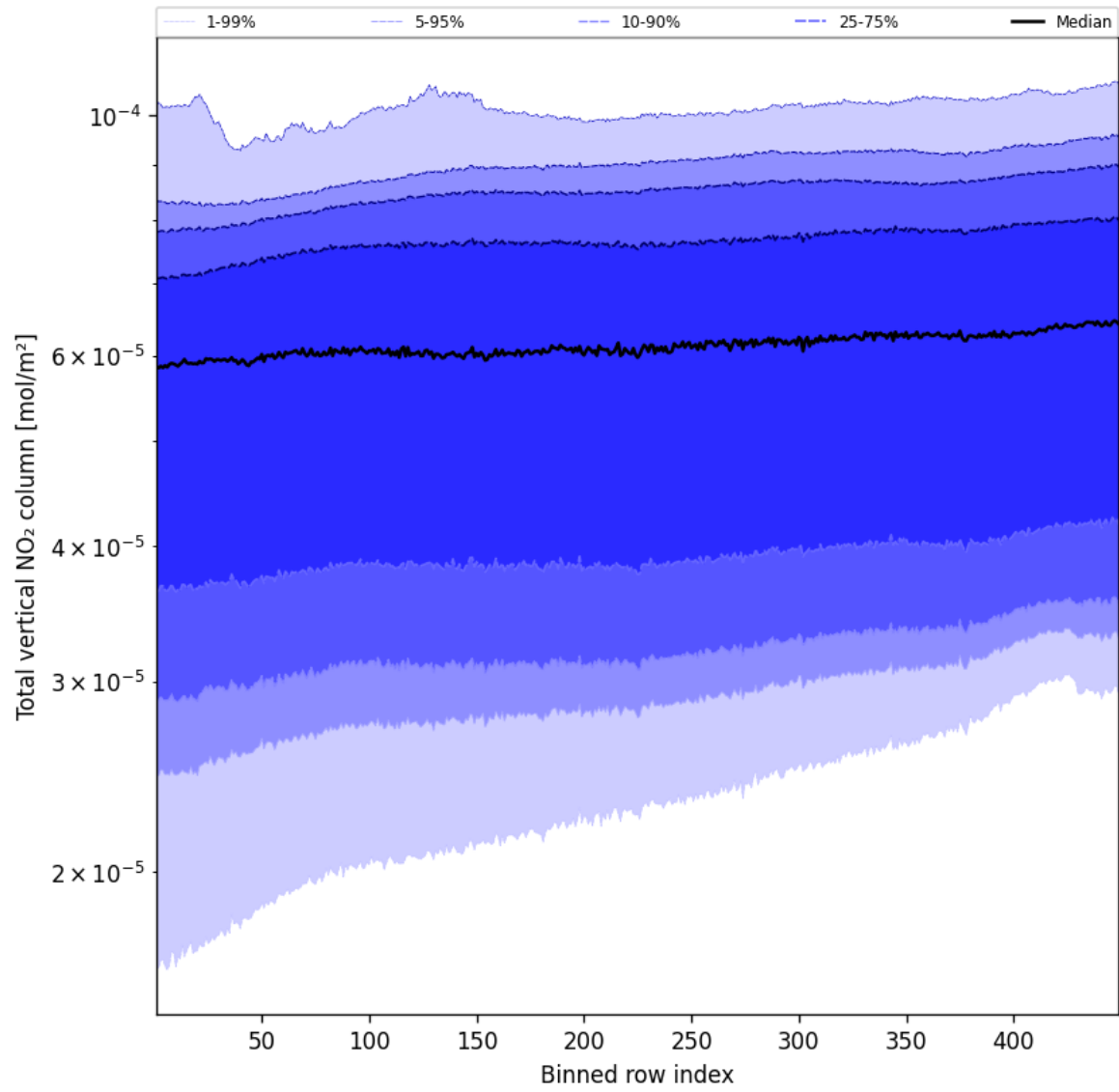
Figure 53: Along track statistics of “Total vertical NO 2 column” for 2025-05-19 to 2025-05-19
