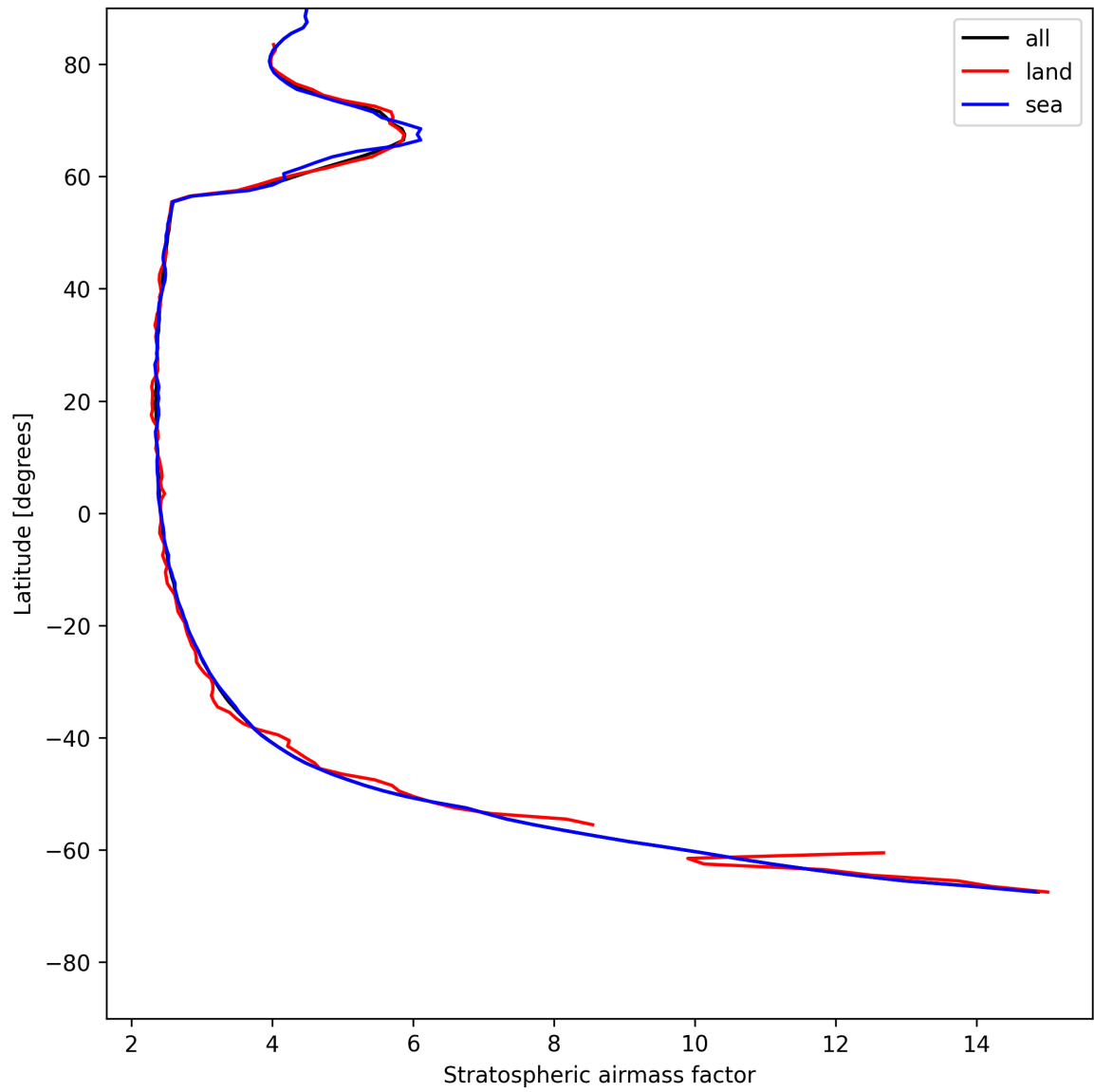
Figure 25: Zonal average of “Stratospheric air mass factor” for 2025-05-19 to 2025-05-19.
