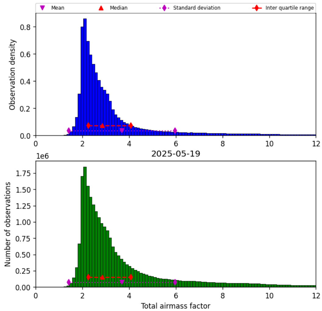
Figure 30: Histogram of “Total airmass factor” for 2025-05-19 to 2025-05-19
