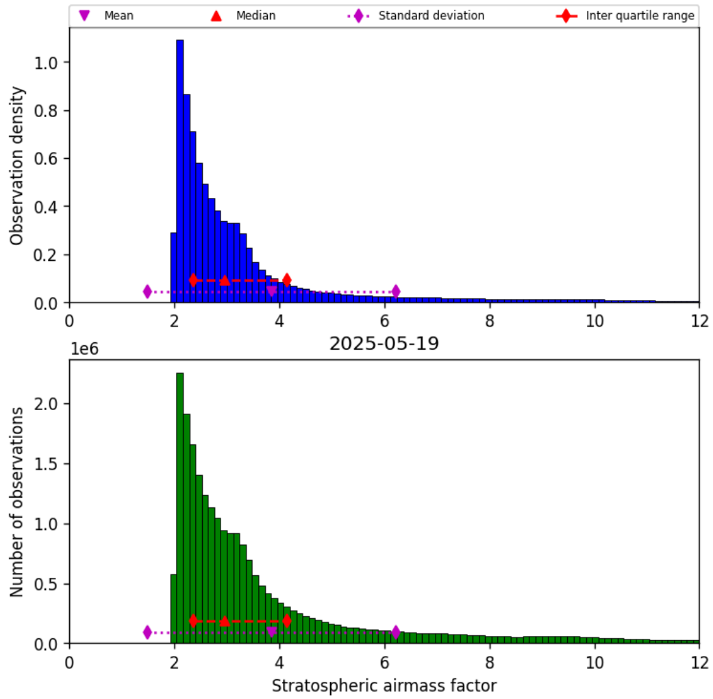
Figure 42: Histogram of “Stratospheric airmass factor” for 2025-05-19 to 2025-05-19
