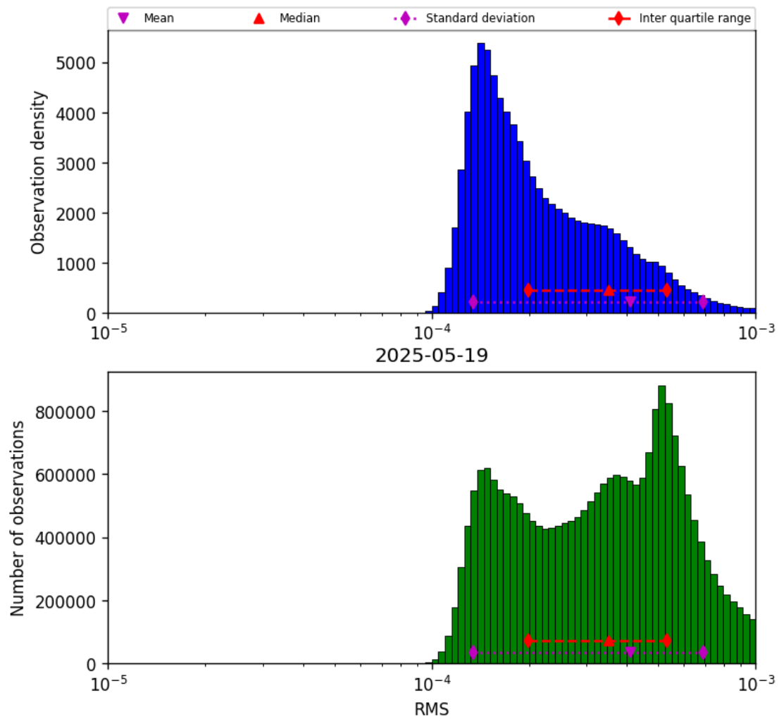
Figure 41: Histogram of “RMS” for 2025-05-19 to 2025-05-19
