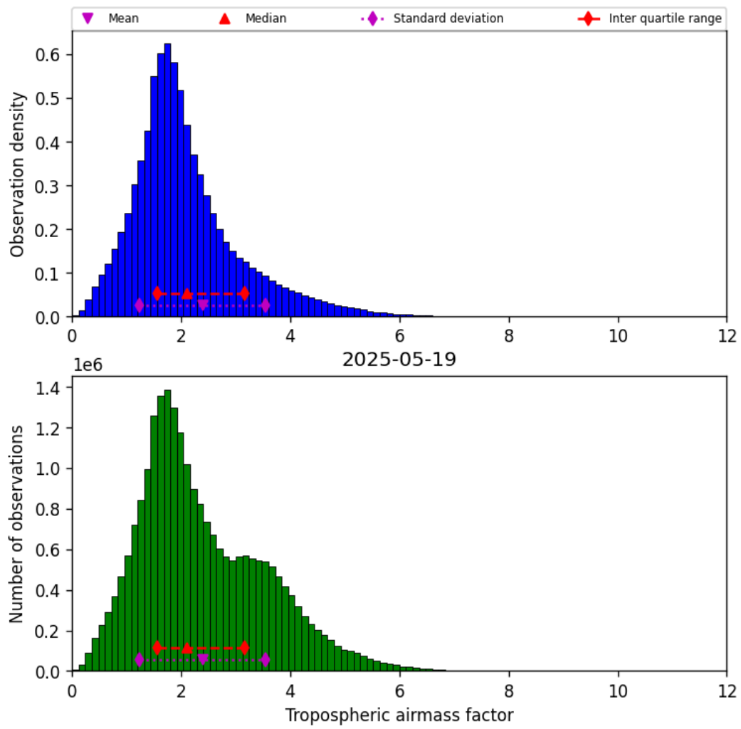
Figure 29: Histogram of “Tropospheric airmass factor” for 2025-05-19 to 2025-05-19
