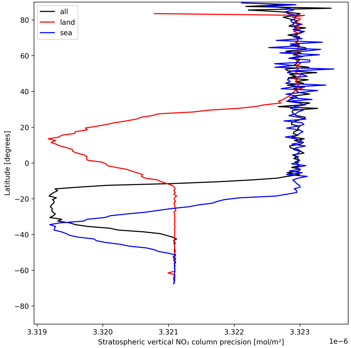
Figure 18: Zonal average of “Stratospheric vertical NO 2 column precision” for 2025-05-19 to 2025-05-19.
