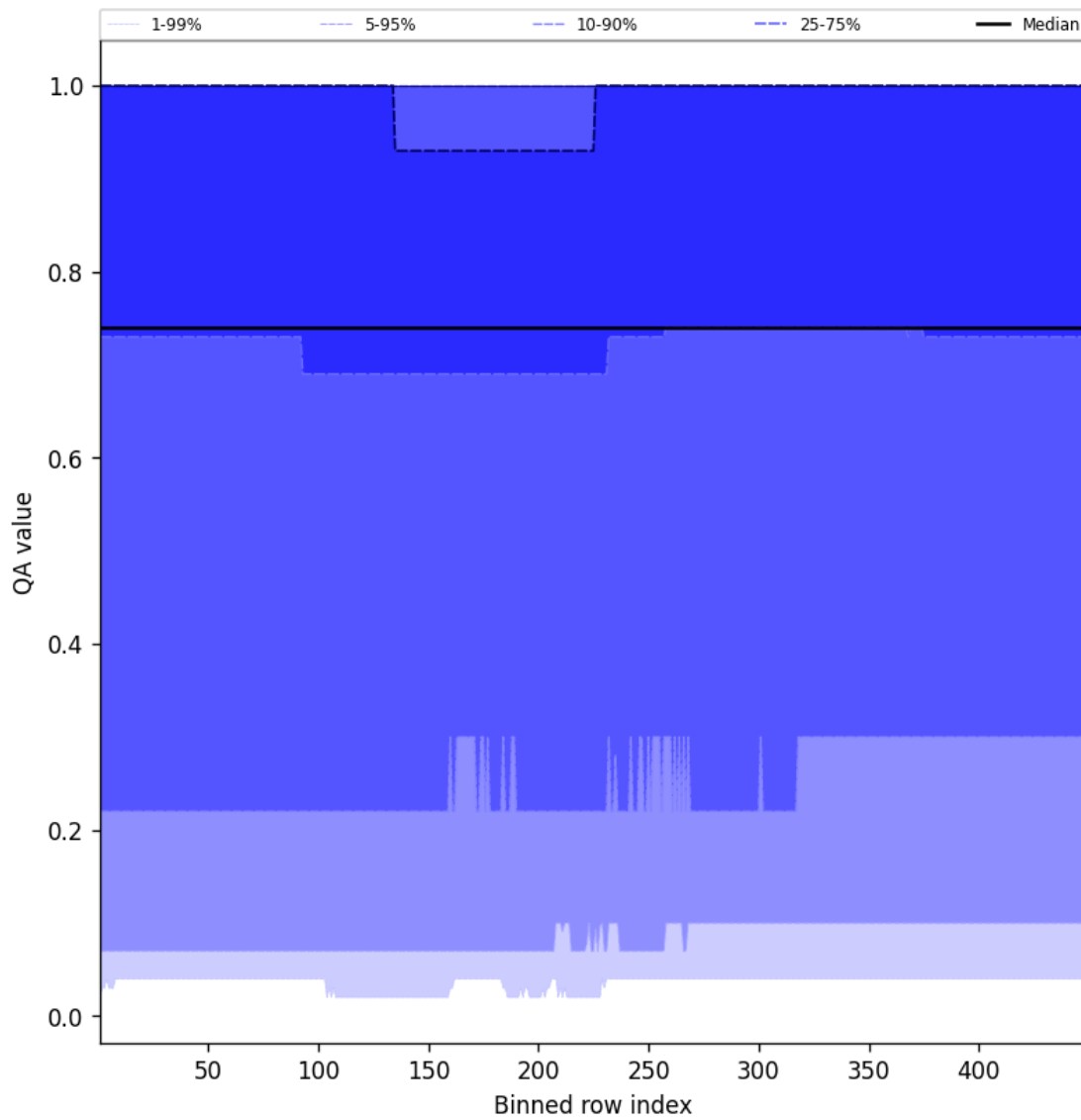
Figure 43: Along track statistics of "QA value" for 2025-05-19 to 2025-05-19
