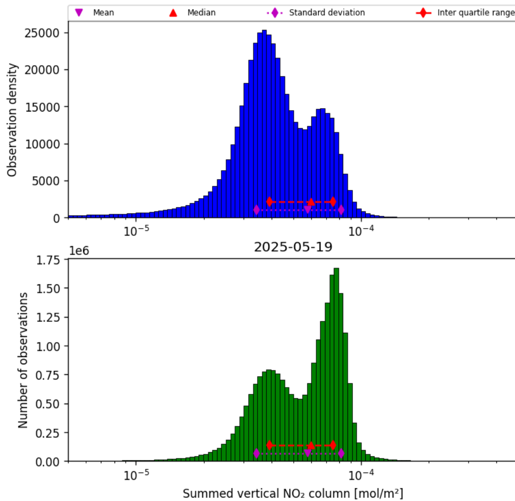
Figure 38: Histogram of “Summed vertical NO 2 column” for 2025-05-19 to 2025-05-19
