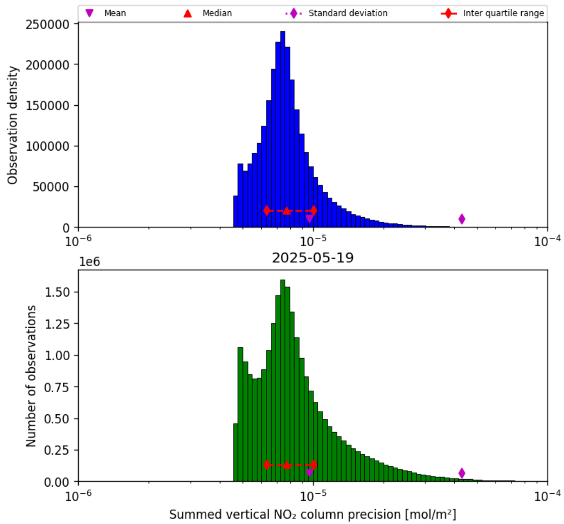
Figure 39: Histogram of "Summed vertical NO 2 column precision" for 2025-05-19 to 2025-05-19
