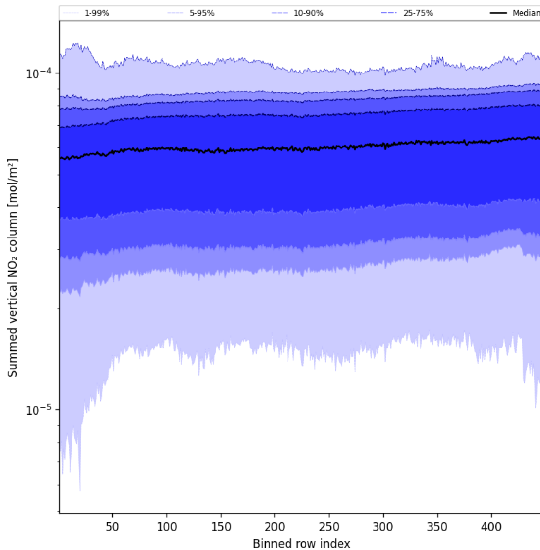
Figure 55: Along track statistics of “Summed vertical NO 2 column” for 2025-05-19 to 2025-05-19
