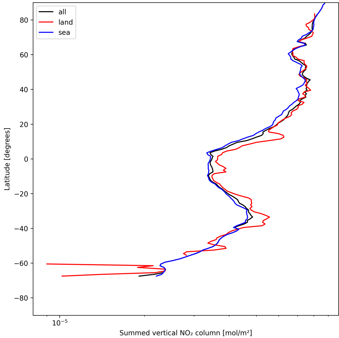
Figure 21: Zonal average of “Summed vertical NO 2 column” for 2025-05-19 to 2025-05-19.
