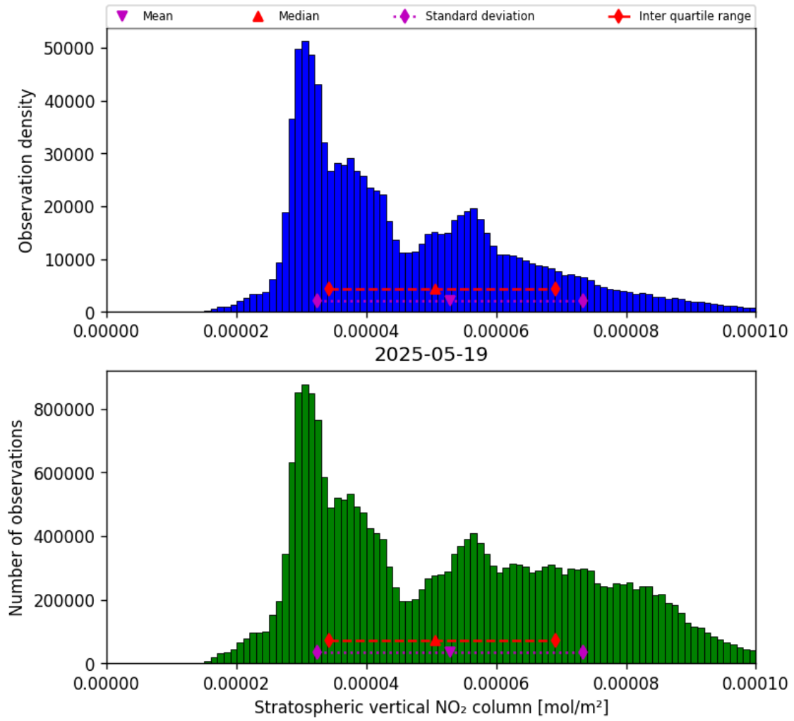
Figure 34: Histogram of “Stratospheric vertical NO 2 column” for 2025-05-19 to 2025-05-19
