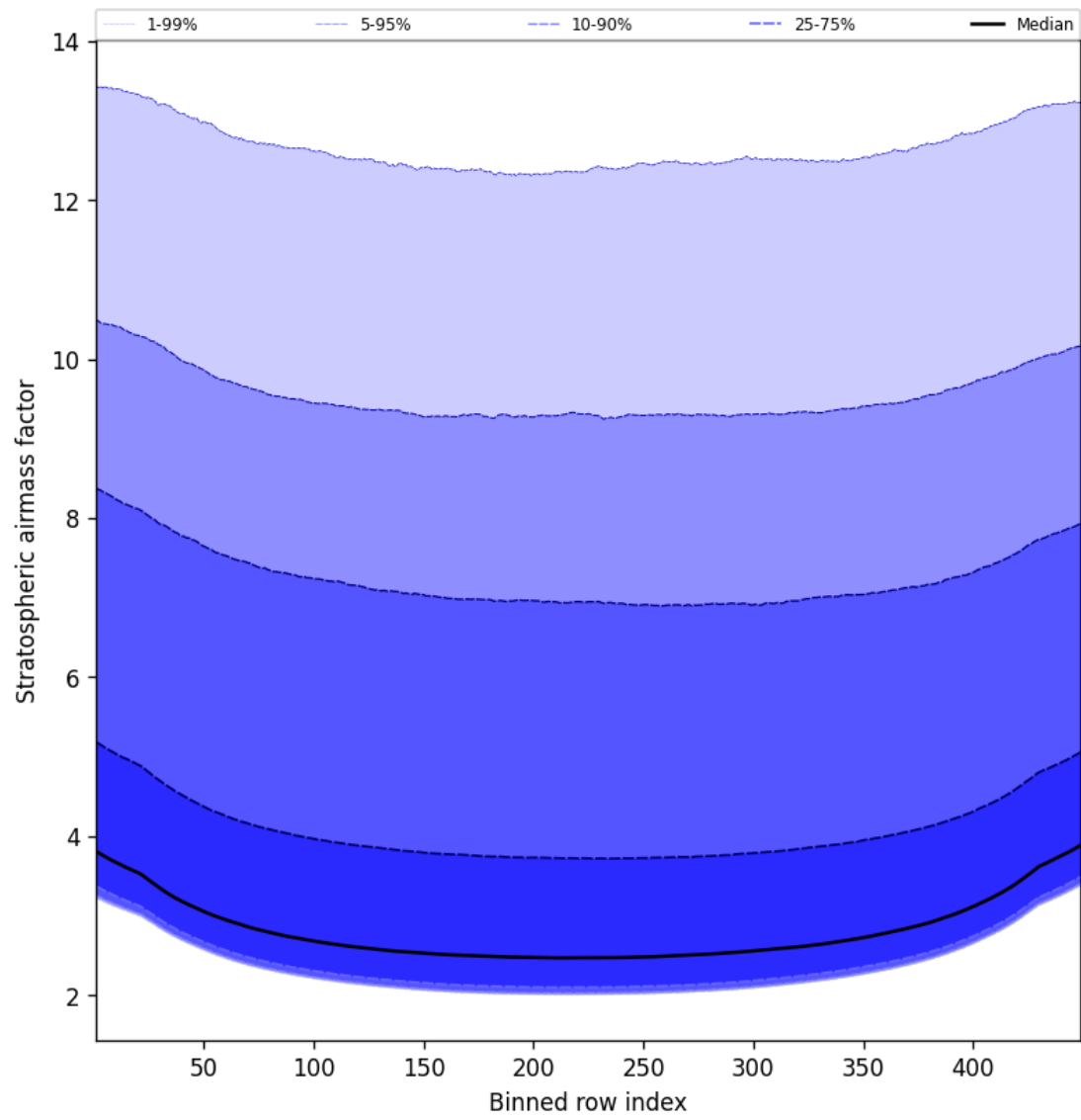
Figure 59: Along track statistics of “Stratospheric airmass factor” for 2025-05-19 to 2025-05-19
