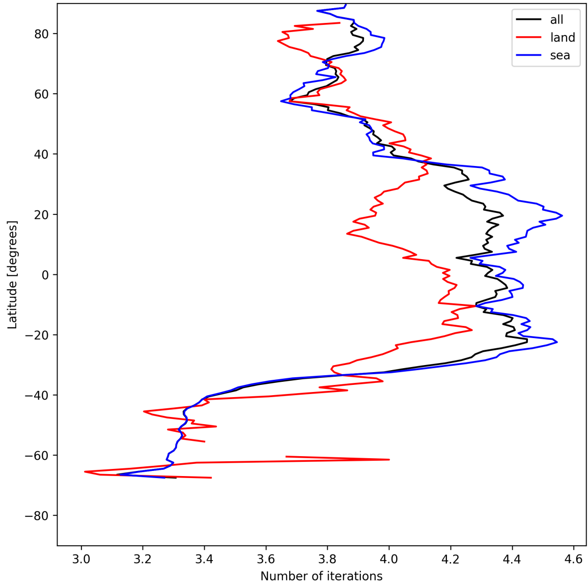
Figure 15: Zonal average of “Number of iterations” for 2025-05-19 to 2025-05-19.
