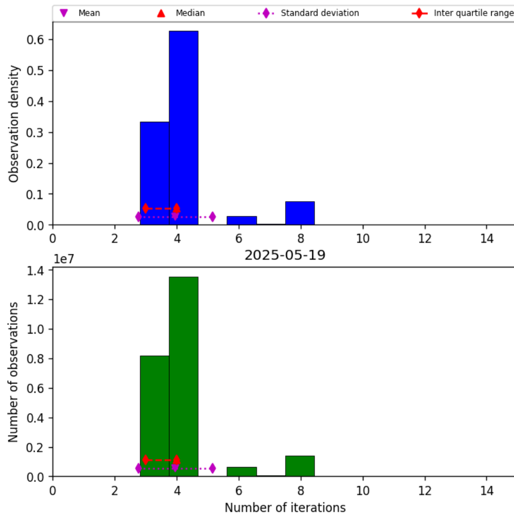
Figure 32: Histogram of “Number of iterations” for 2025-05-19 to 2025-05-19
