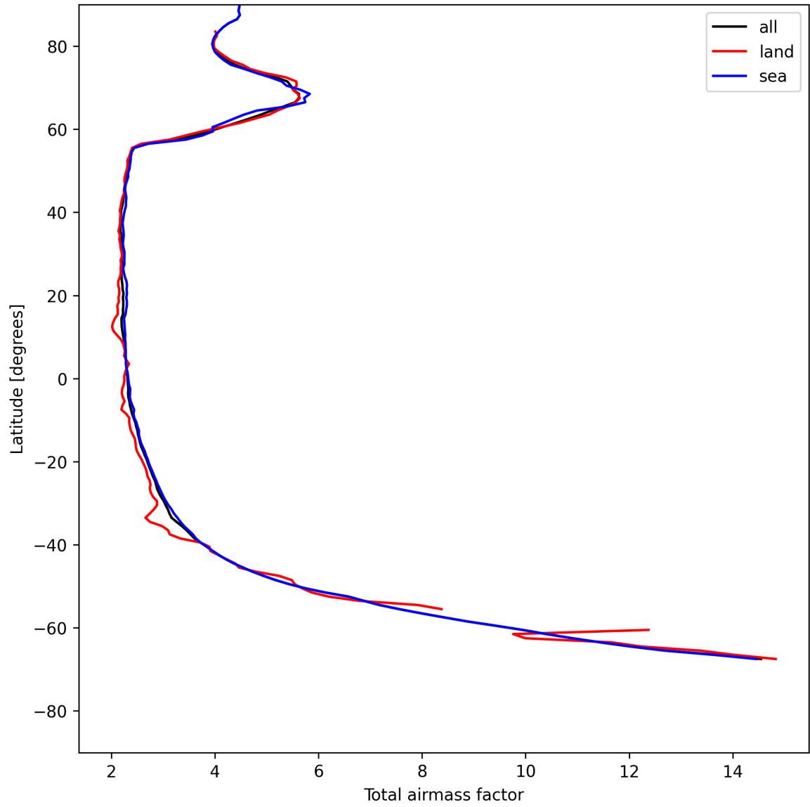
Figure 13: Zonal average of “Total airmass factor” for 2025-05-19 to 2025-05-19.
