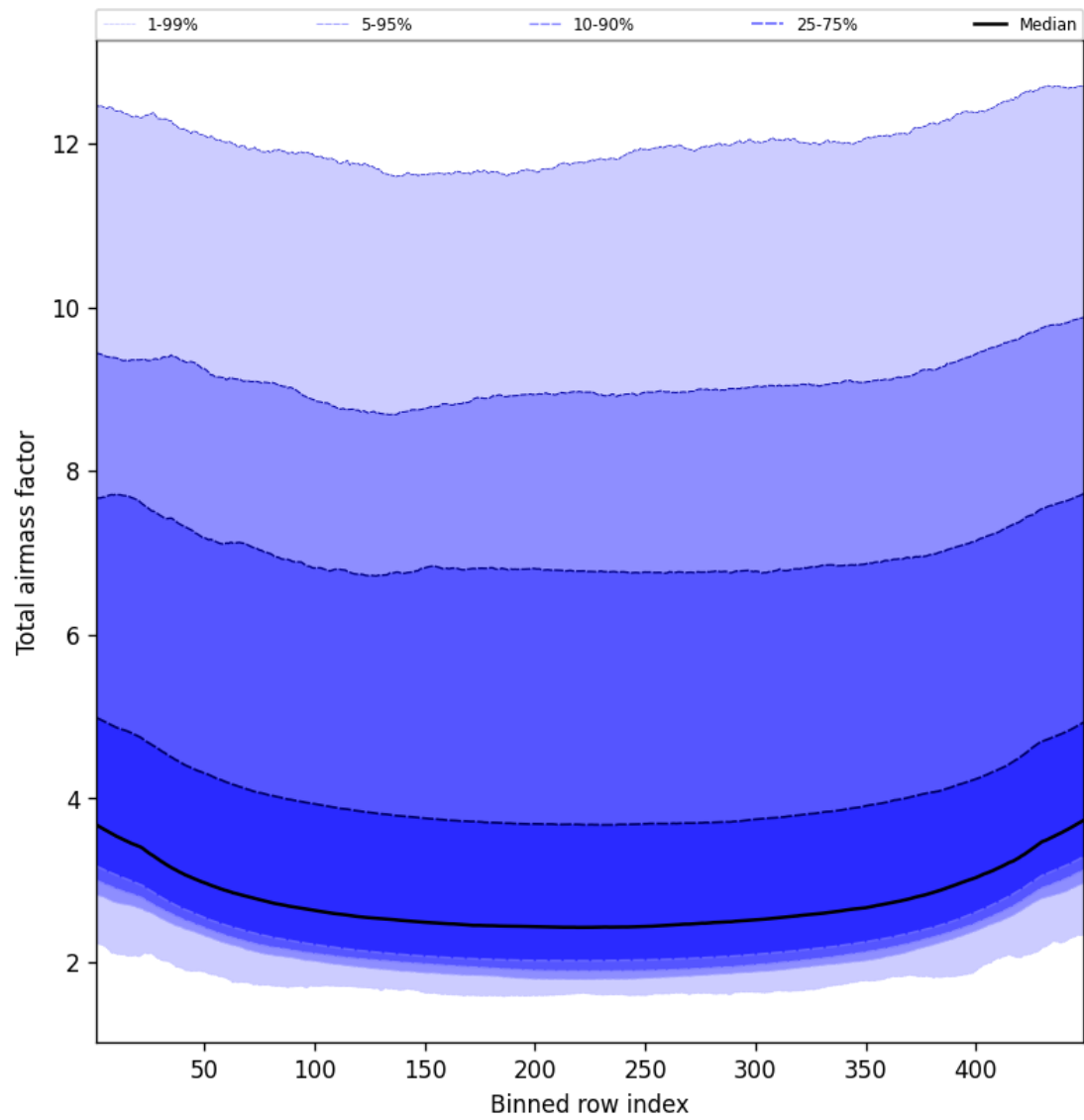
Figure 47: Along track statistics of “Total airmass factor” for 2025-05-19 to 2025-05-19
