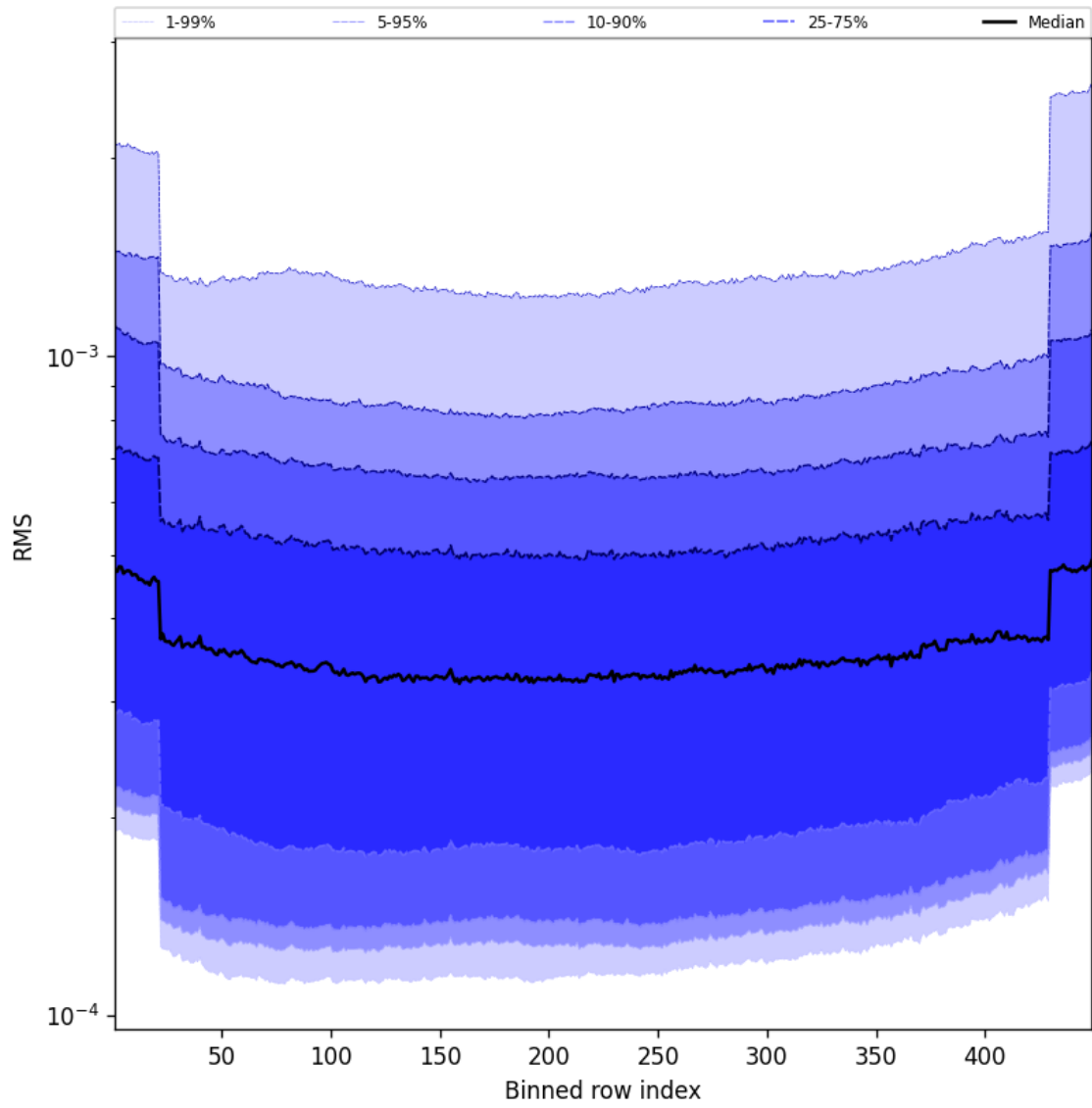
Figure 58: Along track statistics of “RMS” for 2025-05-19 to 2025-05-19
