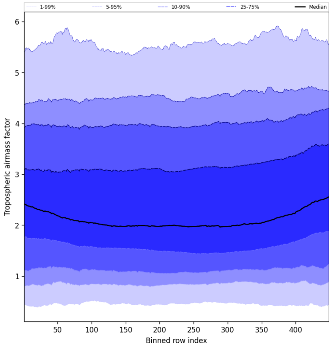
Figure 46: Along track statistics of “Tropospheric airmass factor” for 2025-05-19 to 2025-05-19
