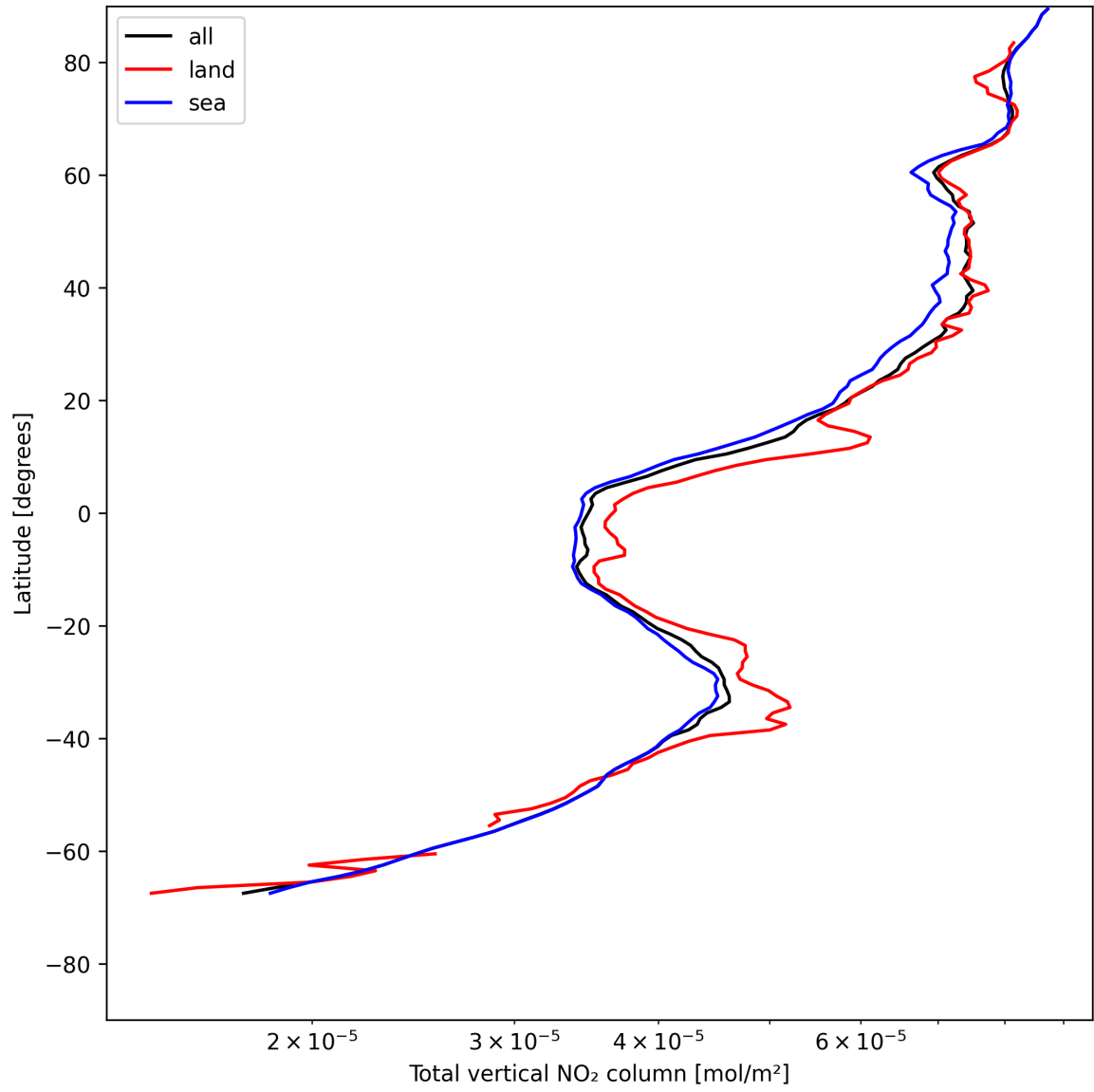
Figure 19: Zonal average of “Total vertical NO 2 column” for 2025-05-19 to 2025-05-19.
