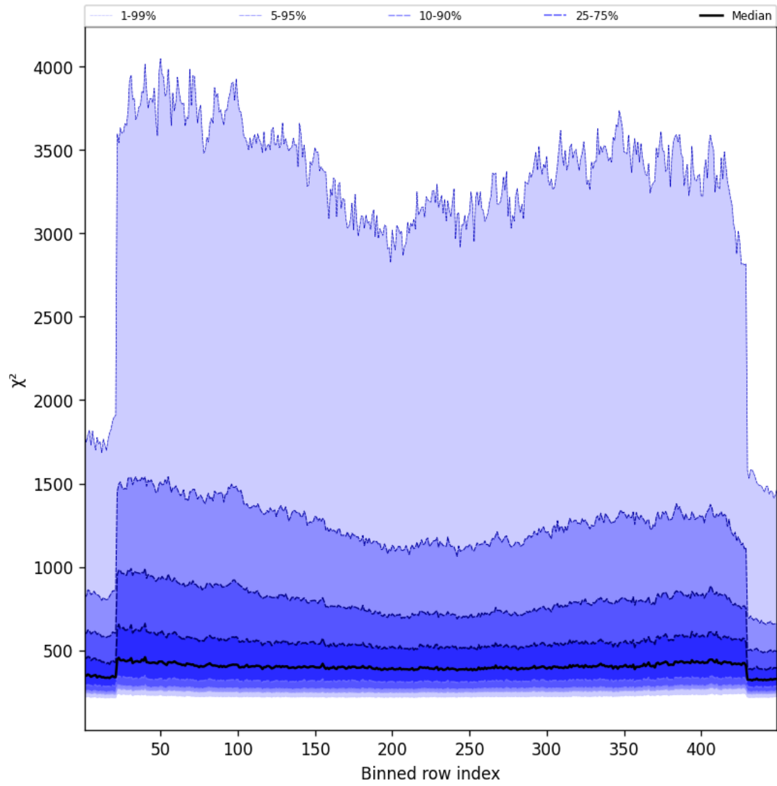
Figure 57: Along track statistics of “ \chi^2 ” for 2025-05-19 to 2025-05-19
