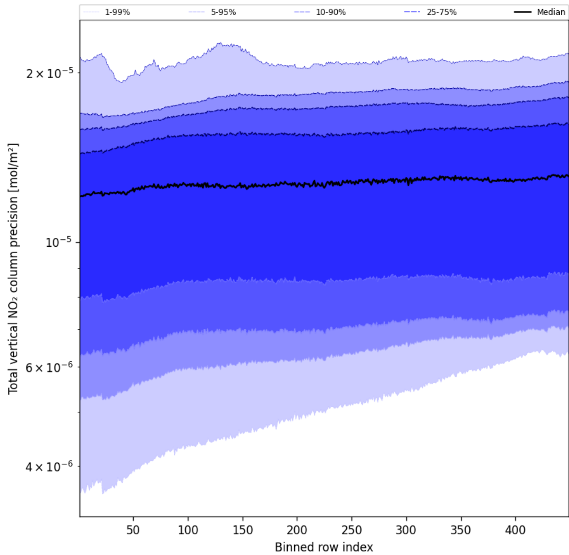
Figure 54: Along track statistics of “Total vertical NO 2 column precision” for 2025-05-19 to 2025-05-19
