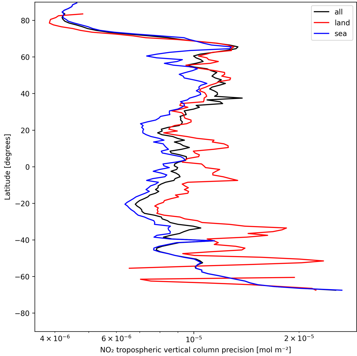
Figure 11: Zonal average of “NO 2 tropospheric vertical column precision” for 2025-05-19 to 2025-05-19.
