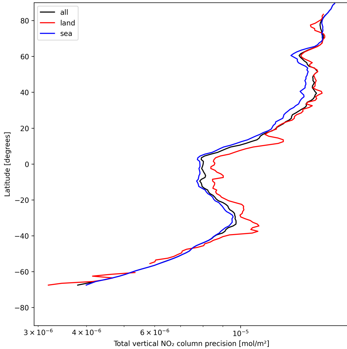
Figure 20: Zonal average of “Total vertical NO 2 column precision” for 2025-05-19 to 2025-05-19.
