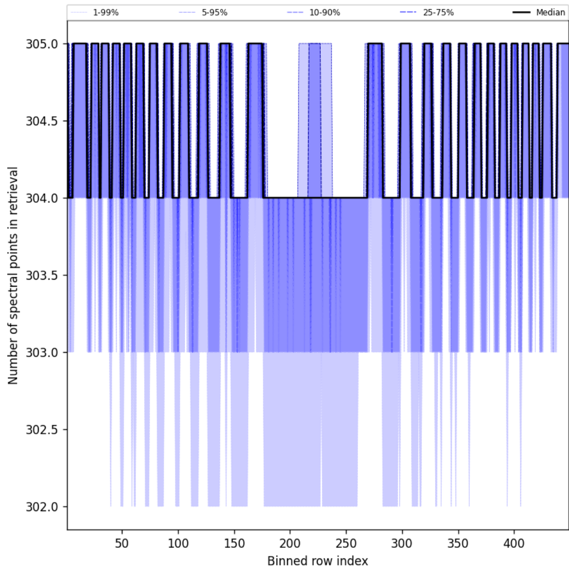
Figure 48: Along track statistics of “Number of spectral points in retrieval” for 2025-05-19 to 2025-05-19
