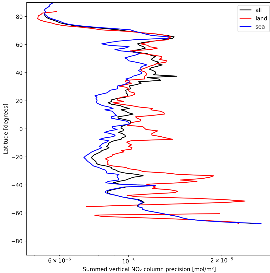
Figure 22: Zonal average of “Summed vertical NO 2 column precision” for 2025-05-19 to 2025-05-19.
