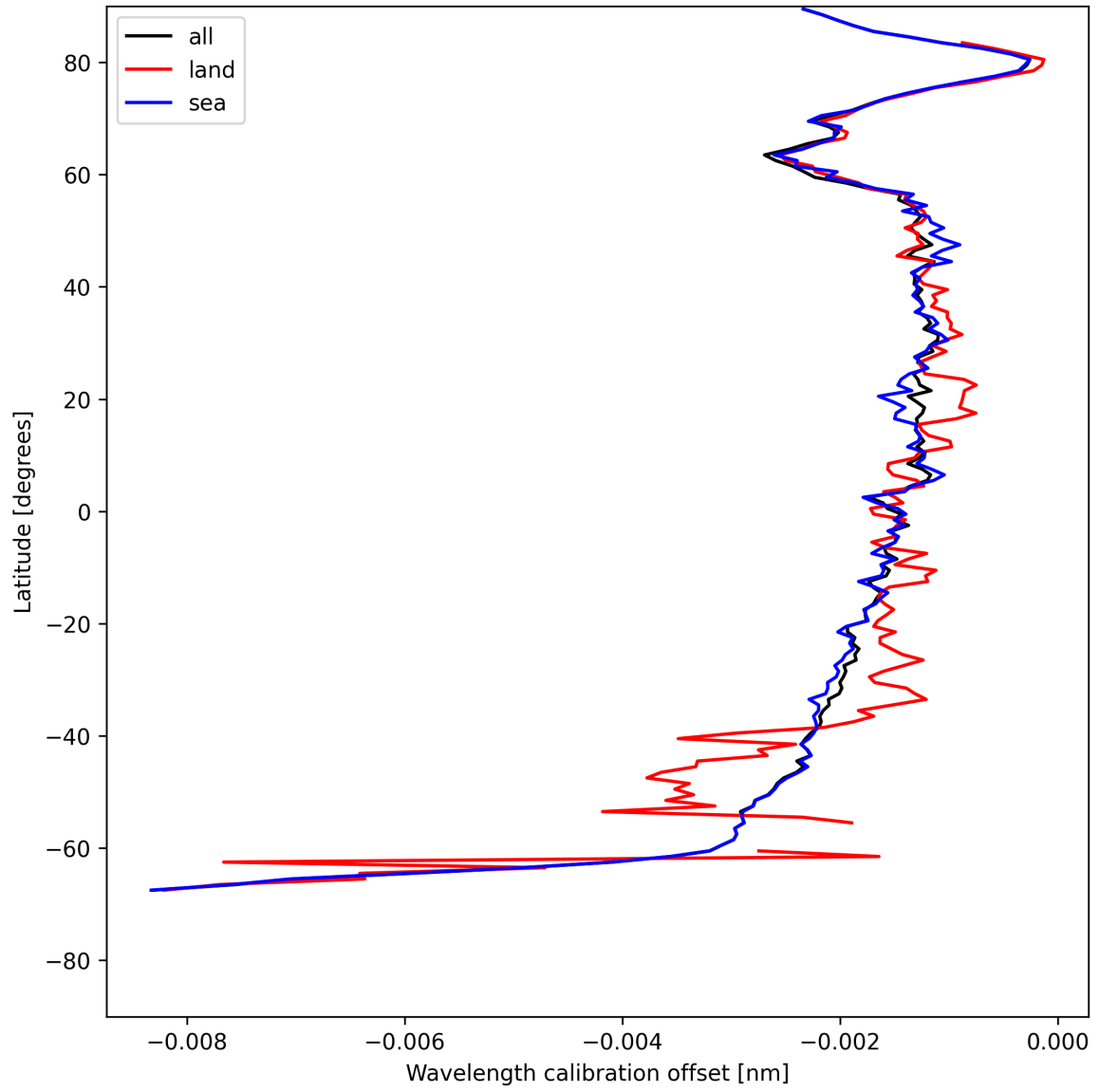
Figure 16: Zonal average of “Wavelength calibration offset” for 2025-05-19 to 2025-05-19.
