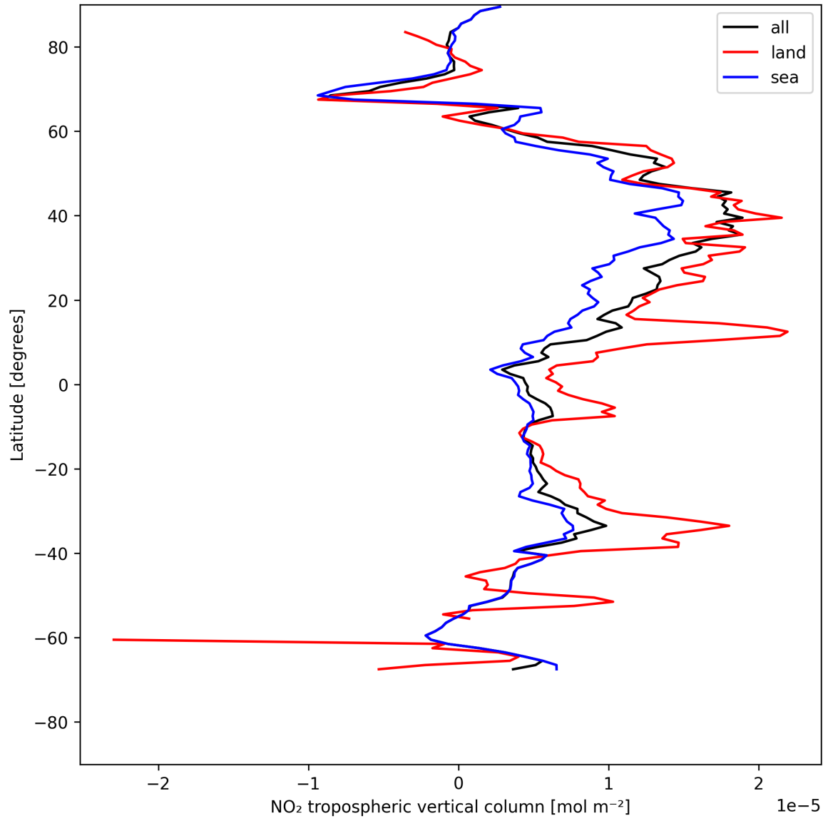
Figure 10: Zonal average of “NO 2 tropospheric vertical column” for 2025-05-19 to 2025-05-19.
