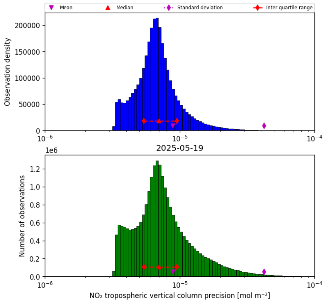
Figure 28: Histogram of “NO 2 tropospheric vertical column precision” for 2025-05-19 to 2025-05-19
