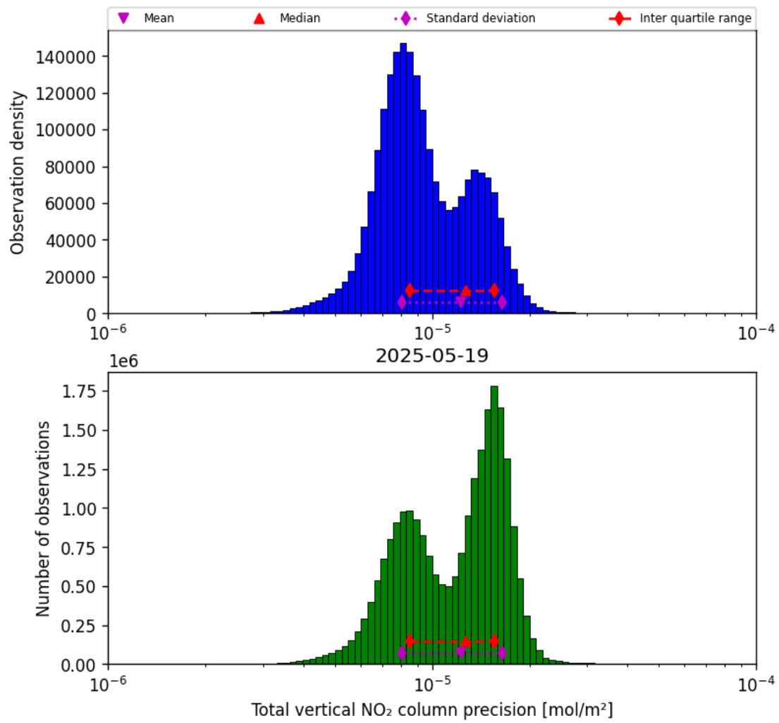
Figure 37: Histogram of "Total vertical NO 2 column precision" for 2025-05-19 to 2025-05-19
