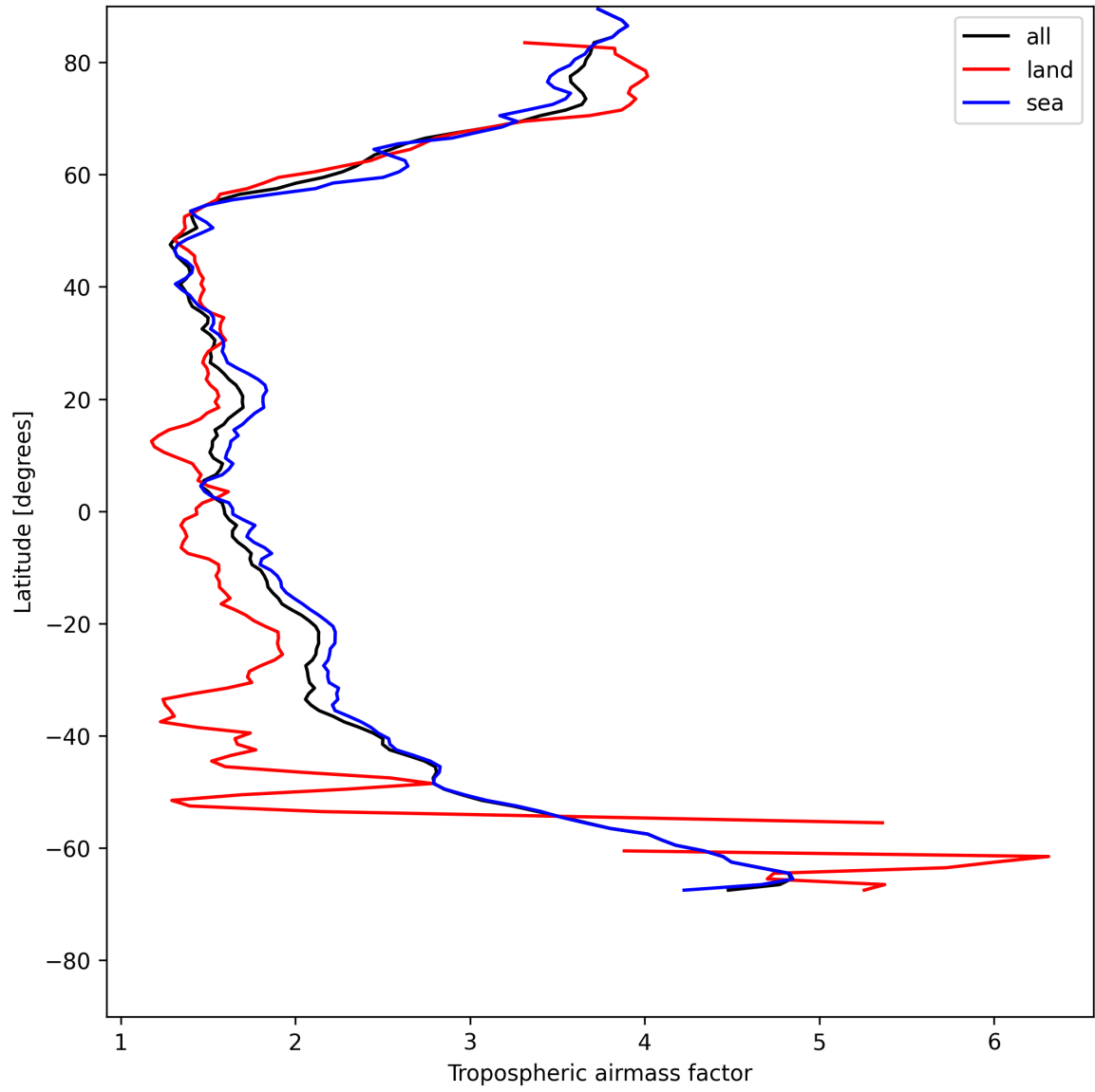
Figure 12: Zonal average of “Tropospheric air mass factor” for 2025-05-19 to 2025-05-19.
