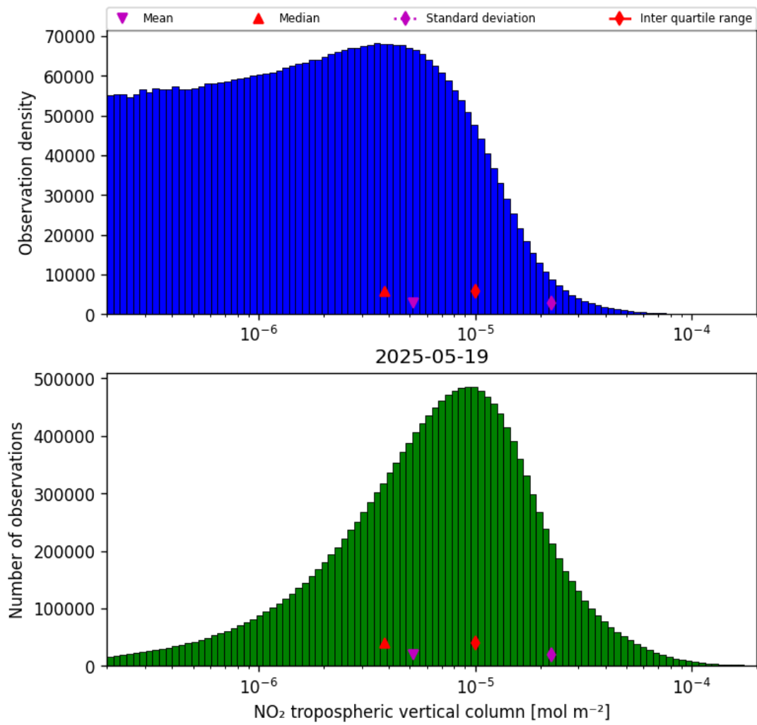
Figure 27: Histogram of “NO 2 tropospheric vertical column” for 2025-05-19 to 2025-05-19
