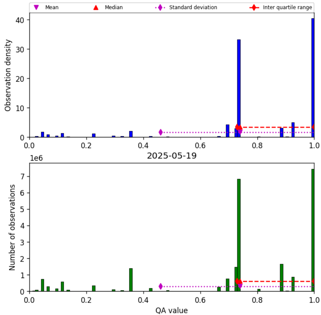
Figure 26: Histogram of “QA value” for 2025-05-19 to 2025-05-19
