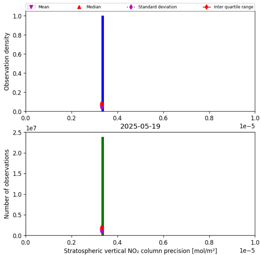
Figure 35: Histogram of “Stratospheric vertical NO 2 column precision” for 2025-05-19 to 2025-05-19
