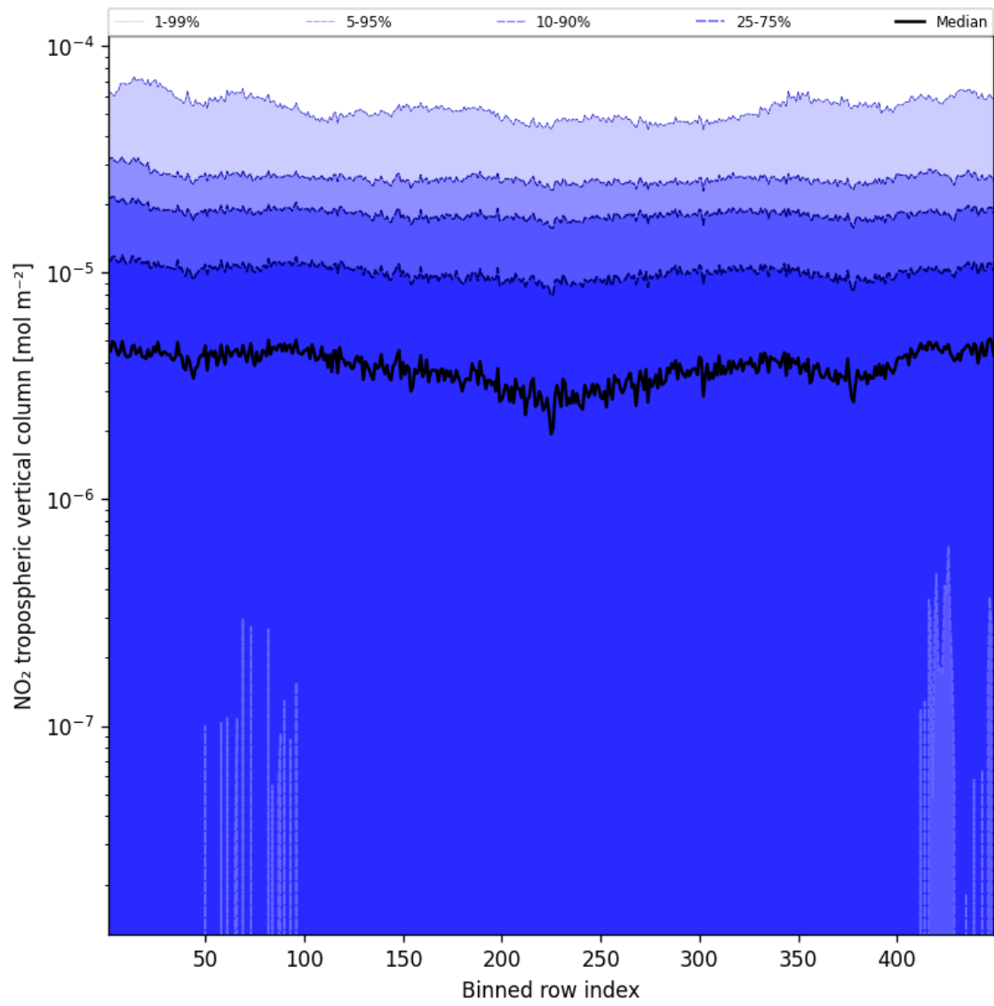
Figure 44: Along track statistics of "NO 2 tropospheric vertical column" for 2025-05-19 to 2025-05-19
