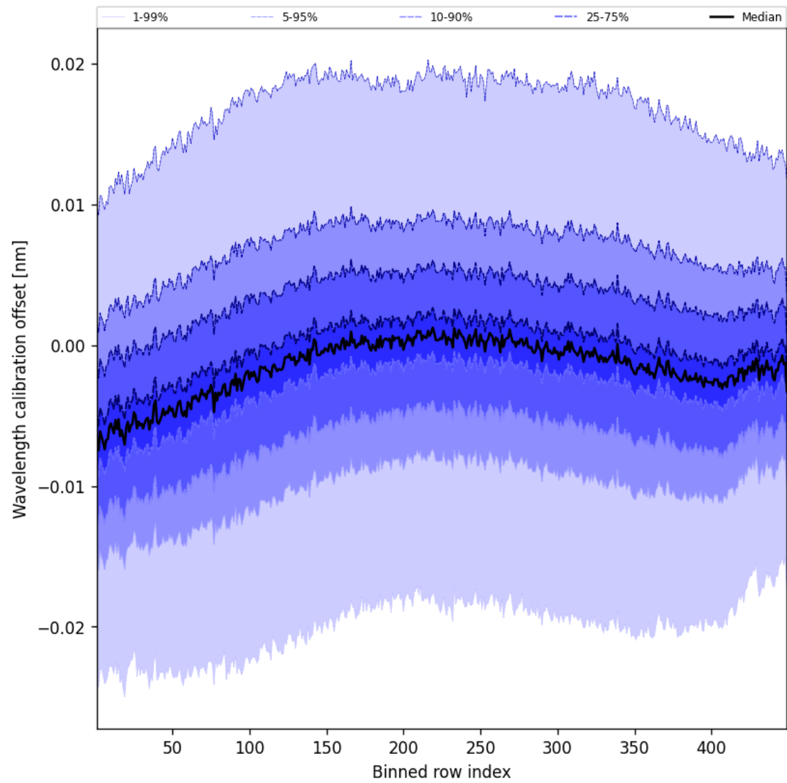
Figure 50: Along track statistics of “Wavelength calibration offset” for 2025-05-19 to 2025-05-19
