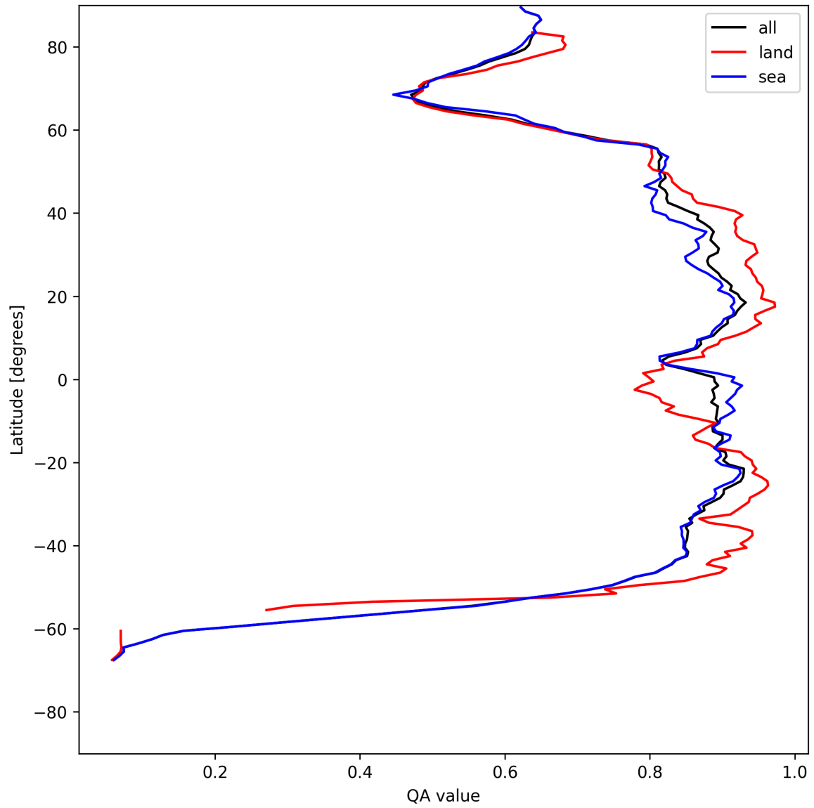
Figure 9: Zonal average of “QA value” for 2025-05-19 to 2025-05-19.
