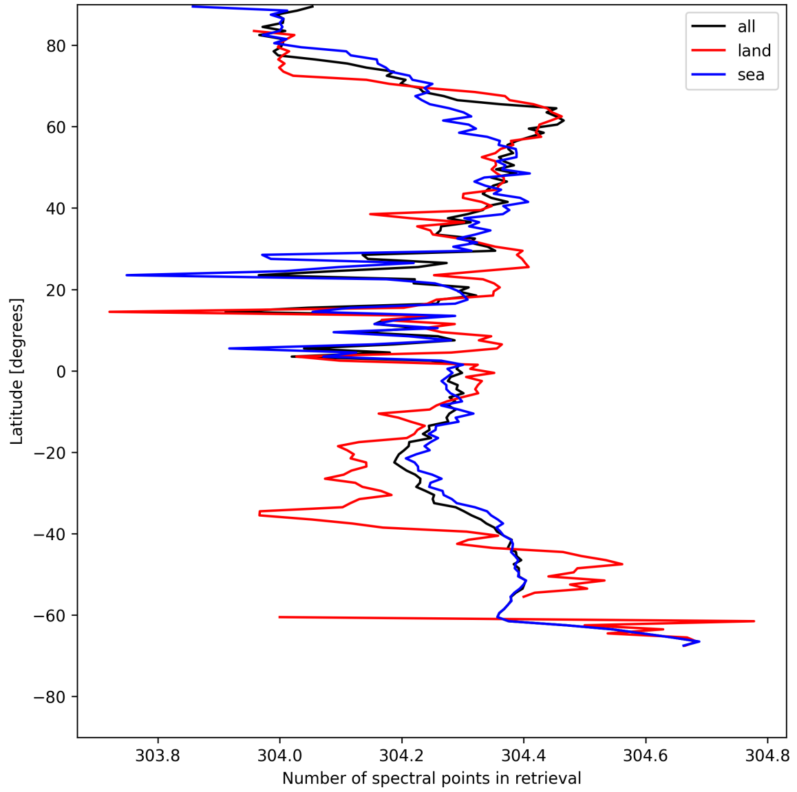
Figure 14: Zonal average of “Number of spectral points in retrieval” for 2025-05-19 to 2025-05-19.
