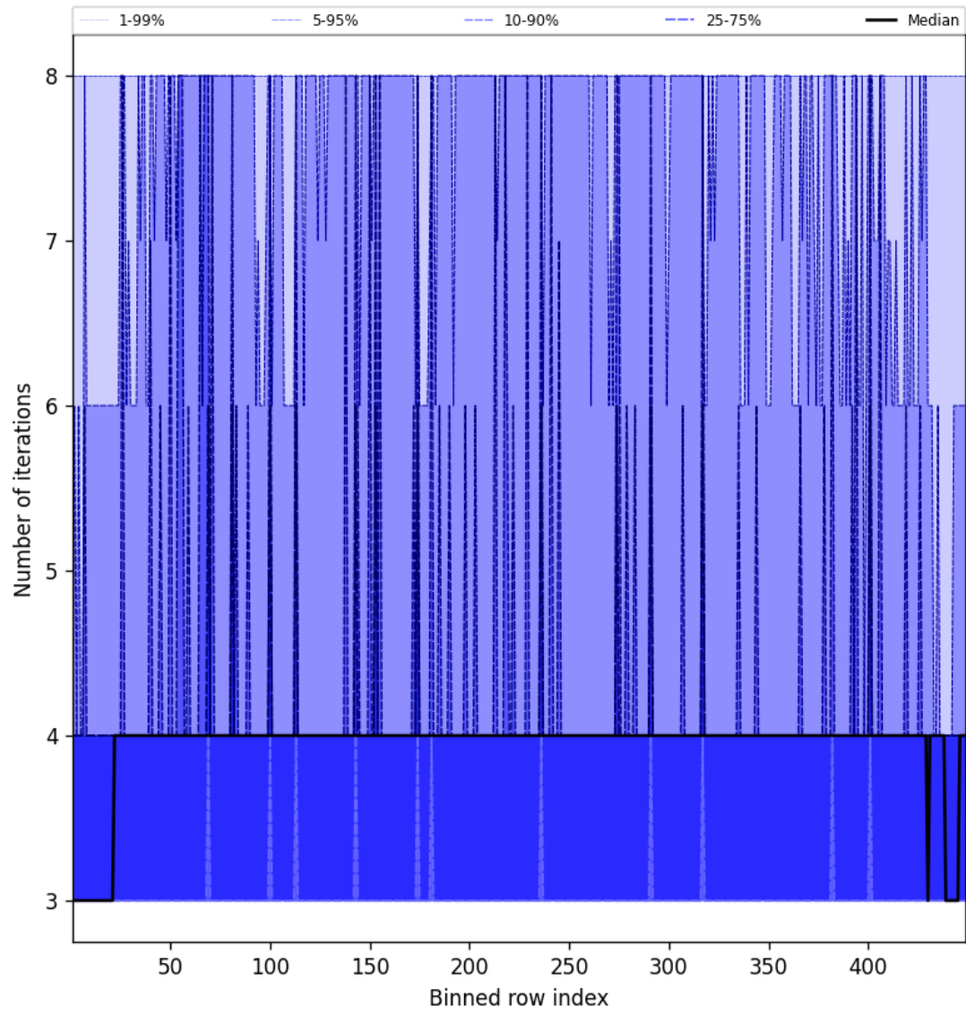
Figure 49: Along track statistics of “Number of iterations” for 2025-05-19 to 2025-05-19
