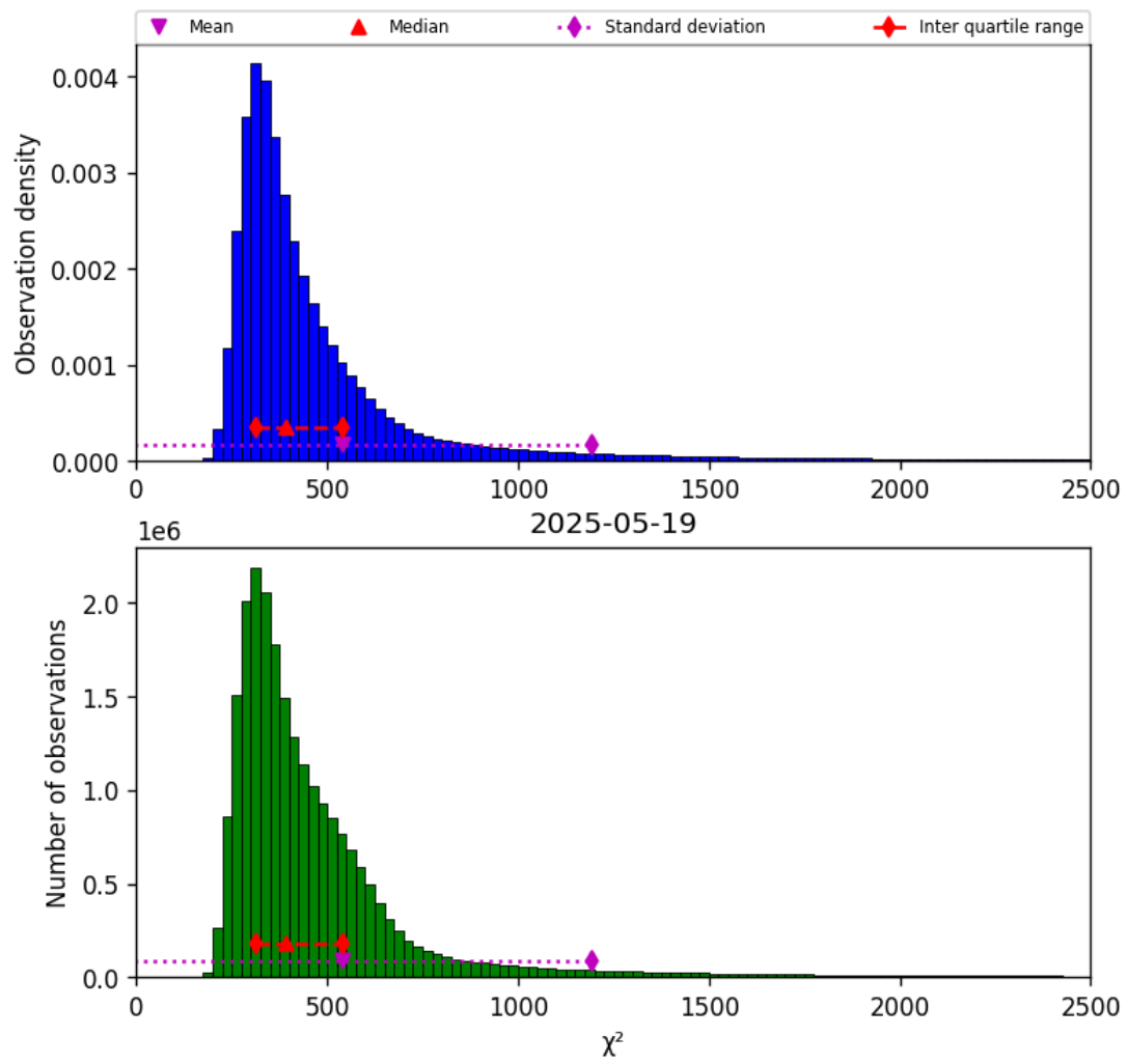
Figure 40: Histogram of " \chi^2 " for 2025-05-19 to 2025-05-19
