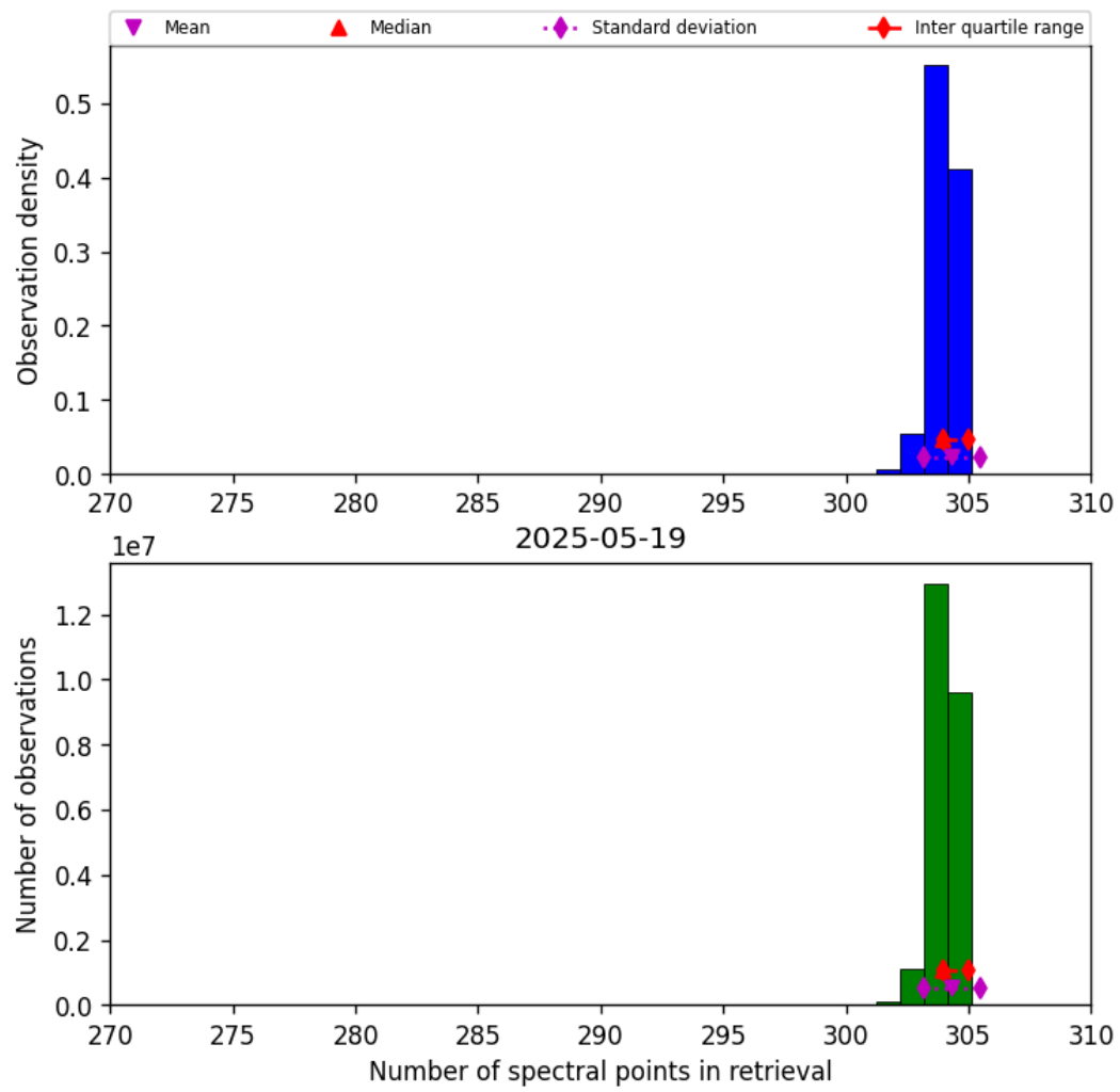
Figure 31: Histogram of “Number of spectral points in retrieval” for 2025-05-19 to 2025-05-19
