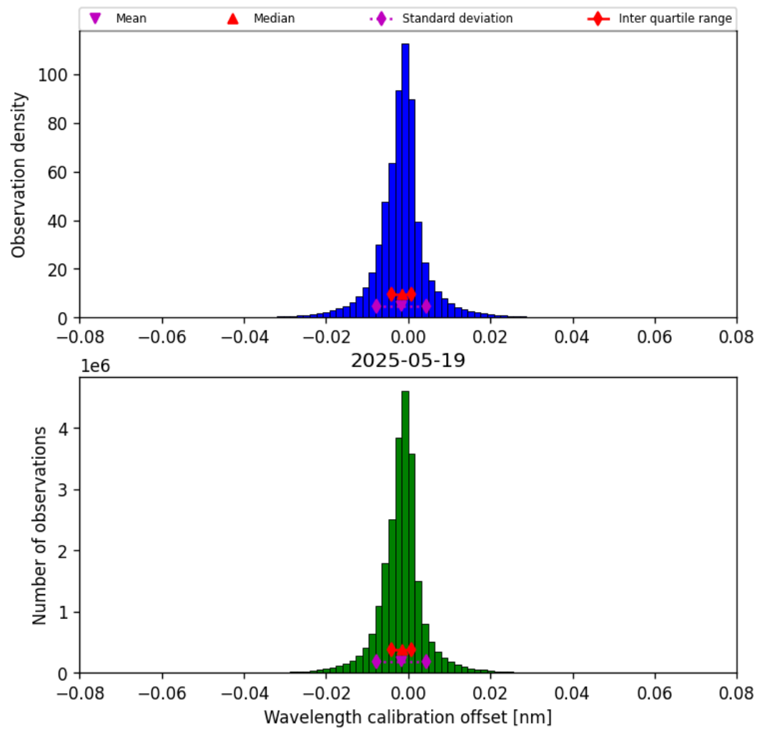
Figure 33: Histogram of “Wavelength calibration offset” for 2025-05-19 to 2025-05-19
