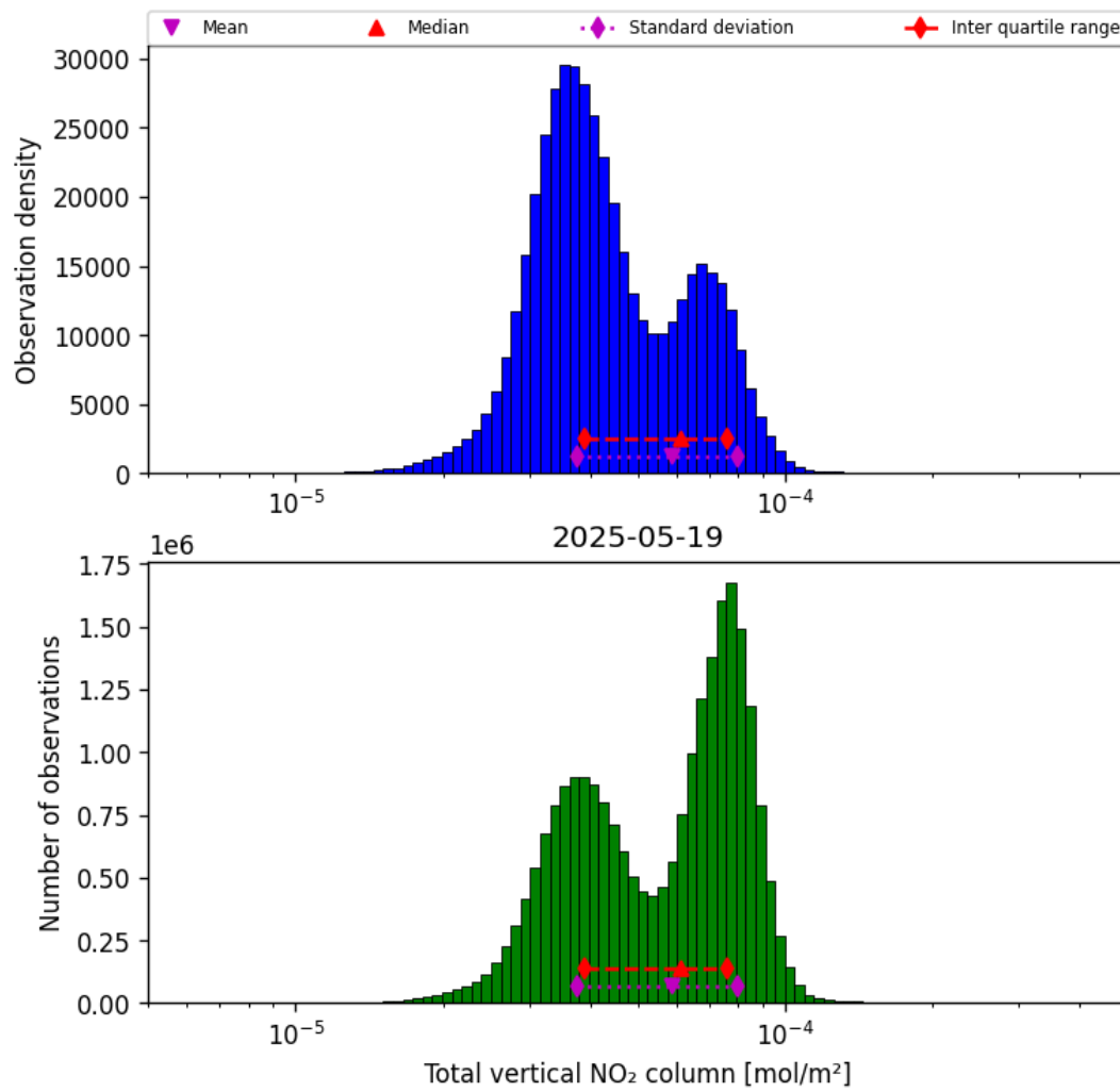
Figure 36: Histogram of “Total vertical NO 2 column” for 2025-05-19 to 2025-05-19
