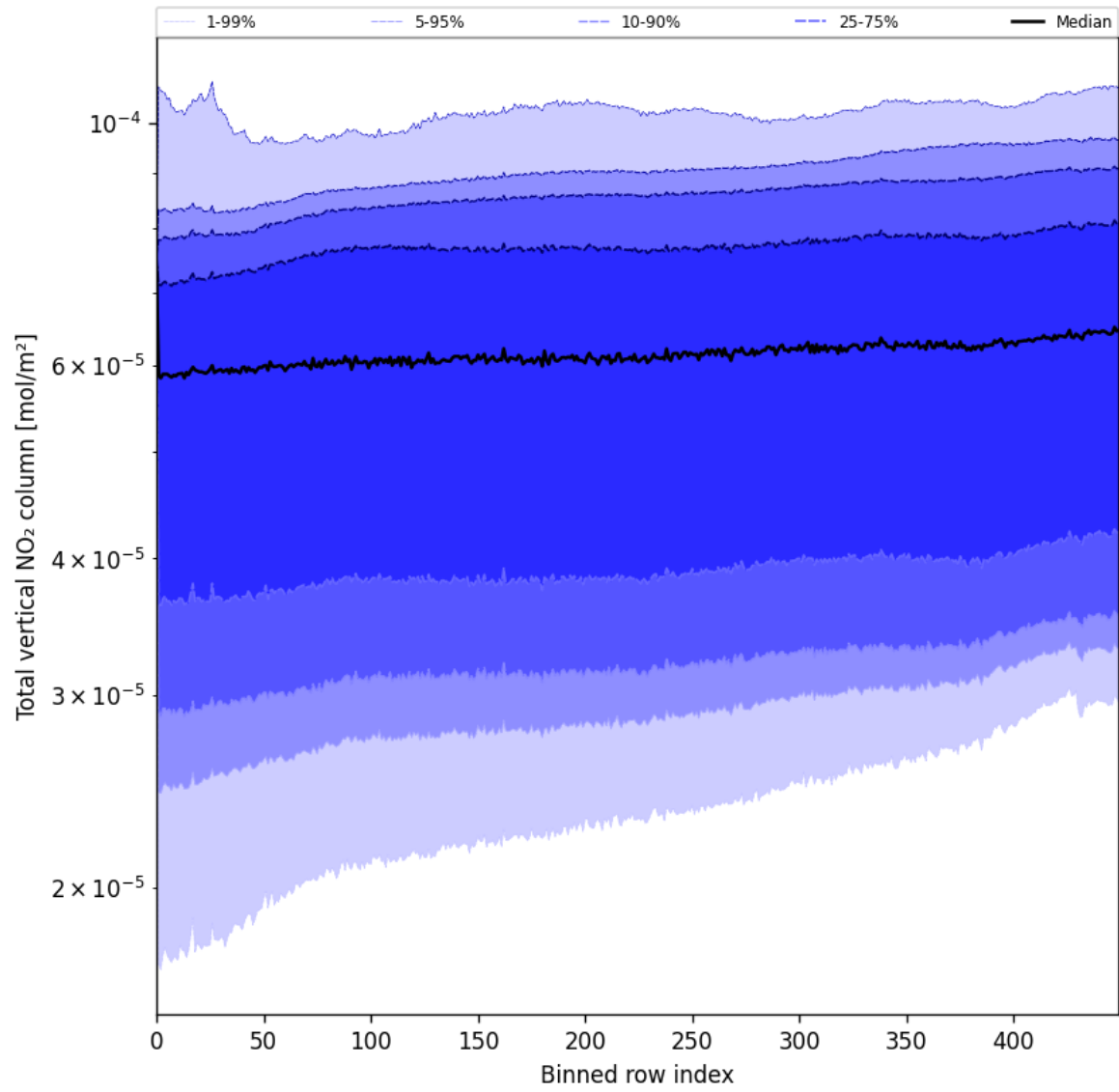
Figure 53: Along track statistics of “Total vertical NO 2 column” for 2025-05-20 to 2025-05-21
