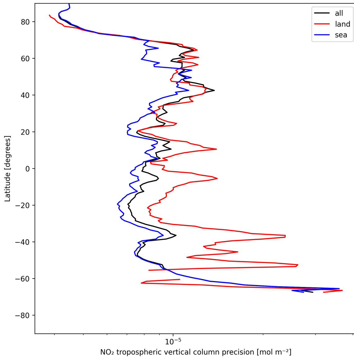
Figure 11: Zonal average of “NO 2 tropospheric vertical column precision” for 2025-05-20 to 2025-05-21.
