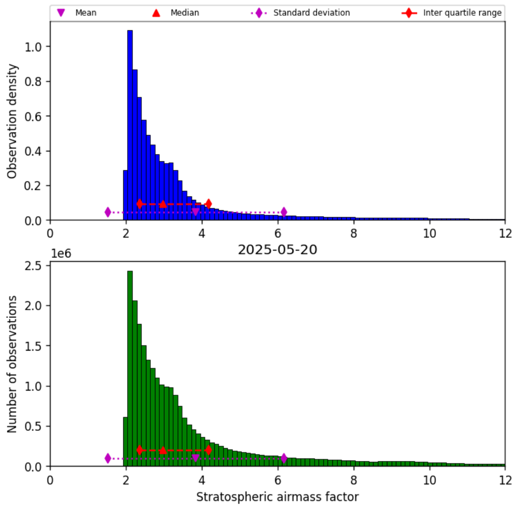
Figure 42: Histogram of “Stratospheric airmass factor” for 2025-05-20 to 2025-05-21
