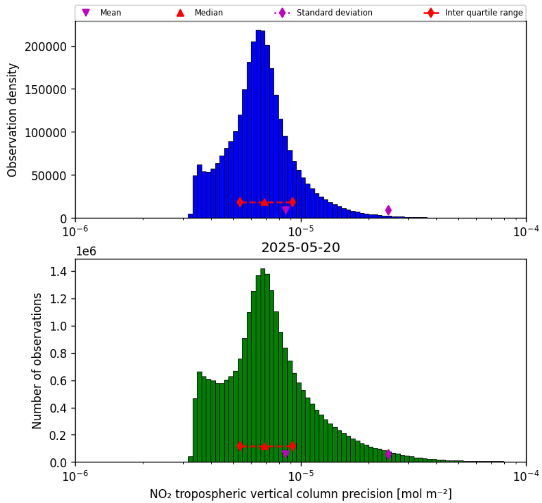
Figure 28: Histogram of “NO 2 tropospheric vertical column precision” for 2025-05-20 to 2025-05-21
