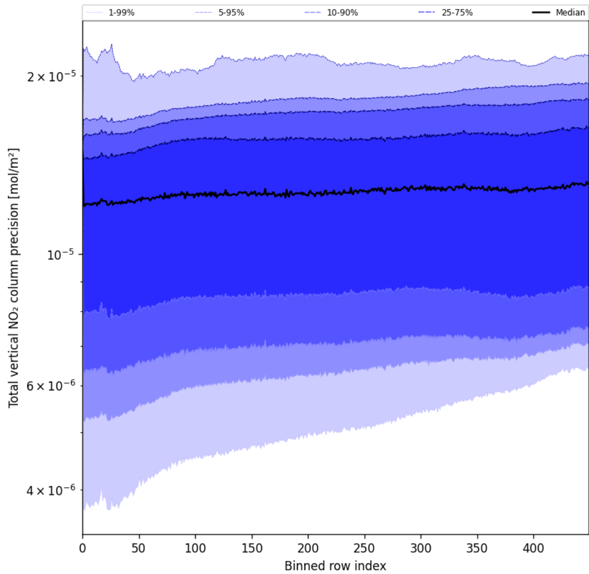
Figure 54: Along track statistics of “Total vertical NO 2 column precision” for 2025-05-20 to 2025-05-21
