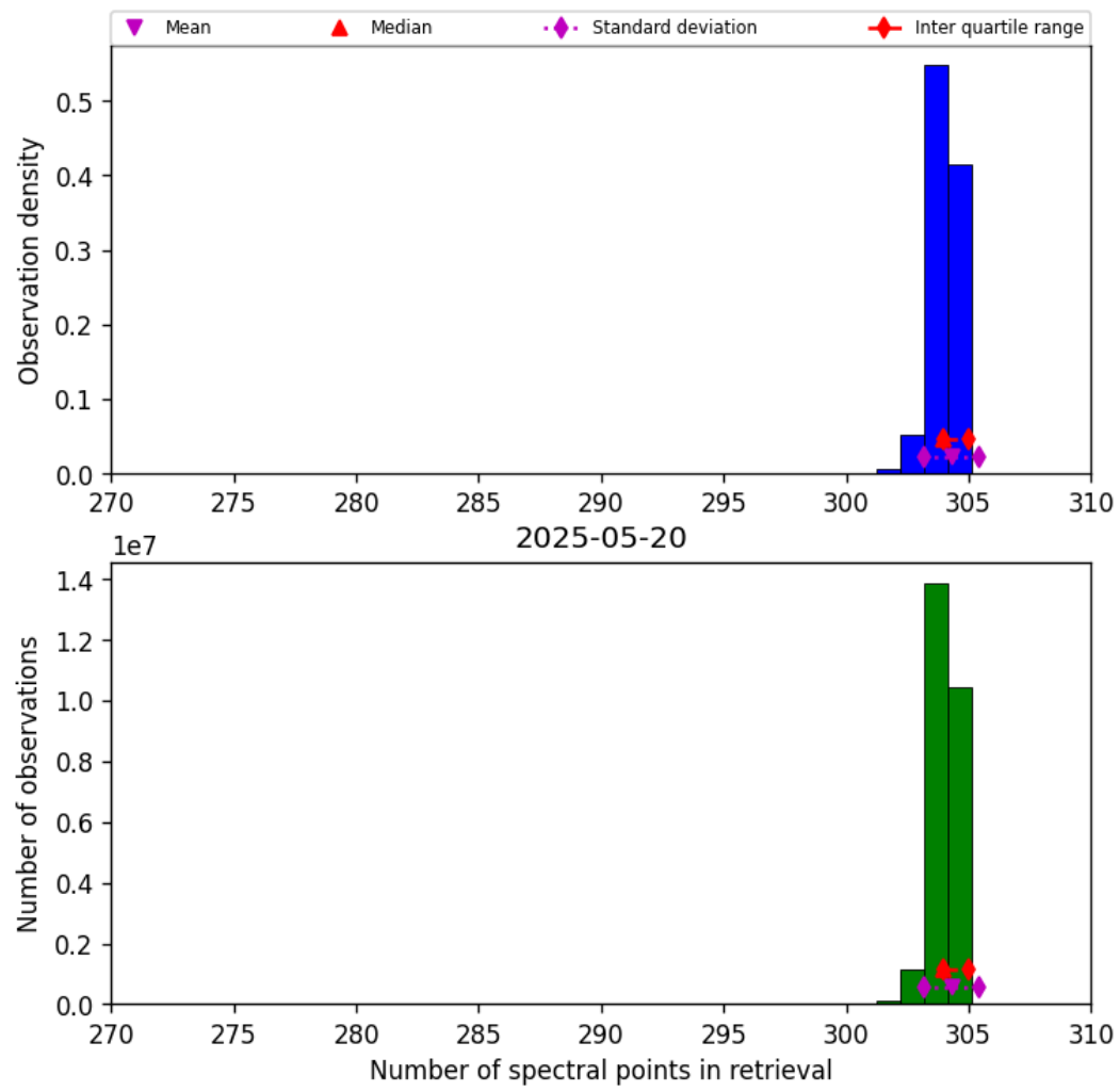
Figure 31: Histogram of “Number of spectral points in retrieval” for 2025-05-20 to 2025-05-21
