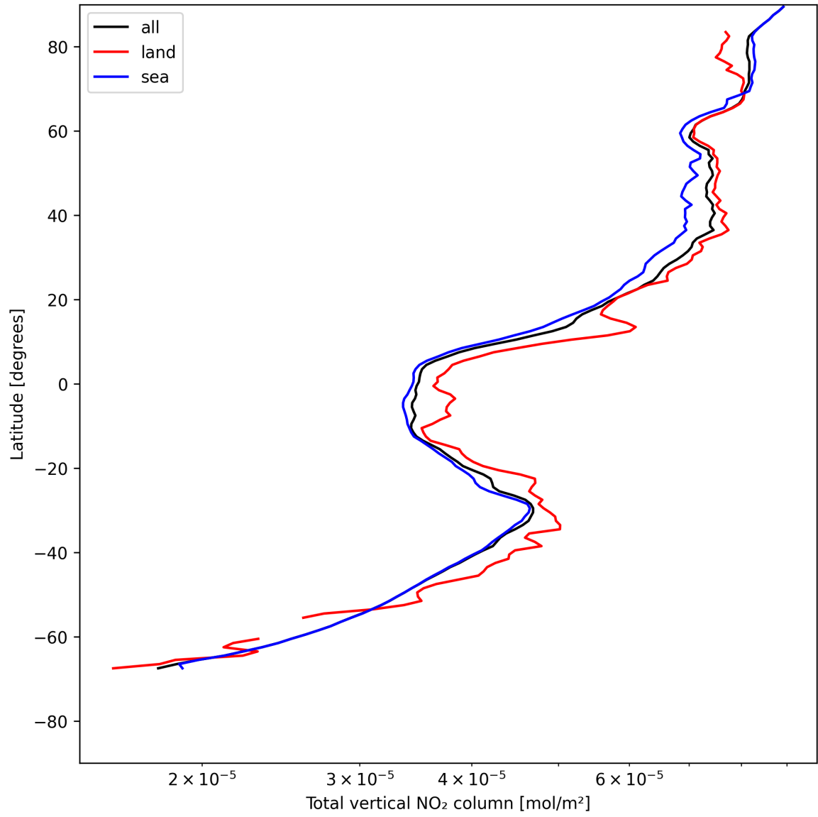
Figure 19: Zonal average of “Total vertical NO 2 column” for 2025-05-20 to 2025-05-21.
