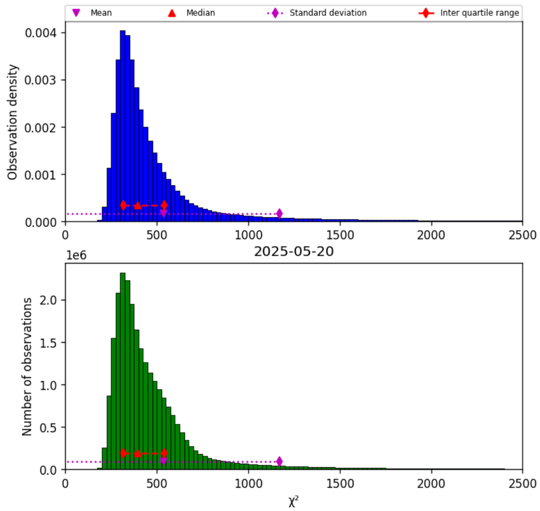
Figure 40: Histogram of “ \chi^2 ” for 2025-05-20 to 2025-05-21
