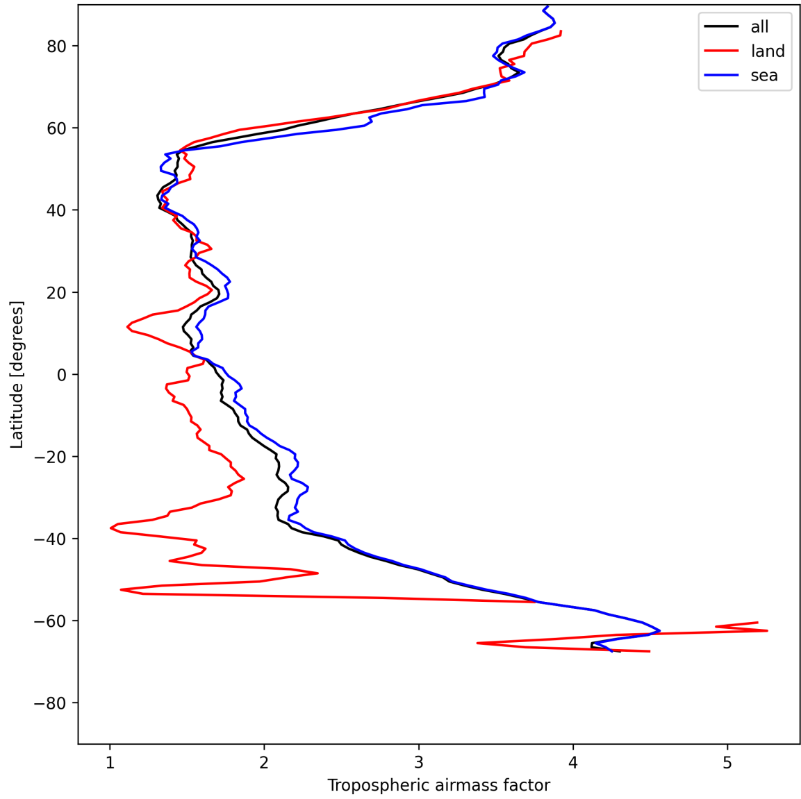
Figure 12: Zonal average of “Tropospheric airmass factor” for 2025-05-20 to 2025-05-21.
