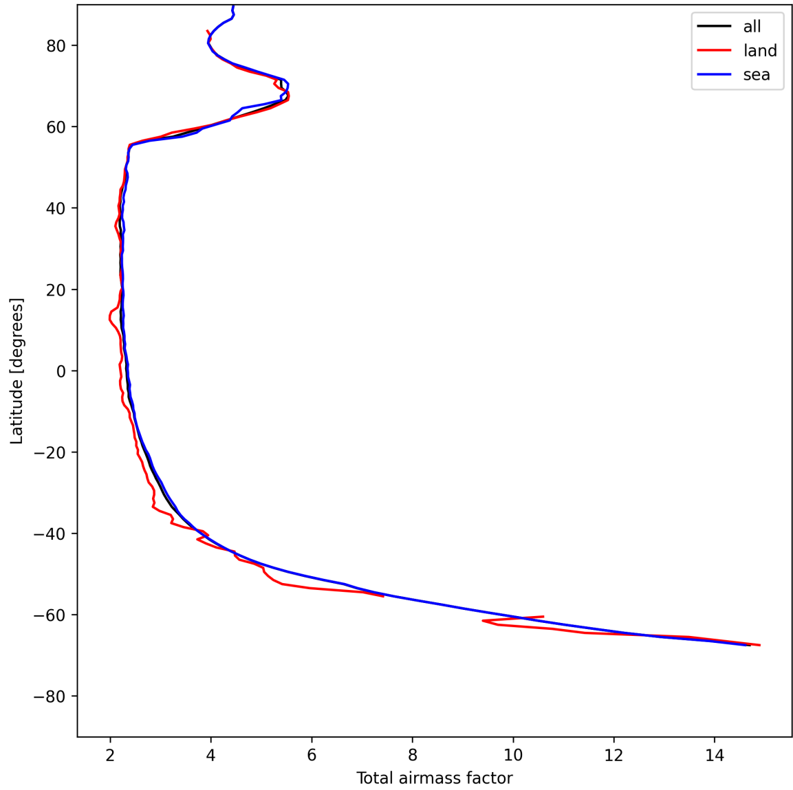
Figure 13: Zonal average of “Total airmass factor” for 2025-05-20 to 2025-05-21.
