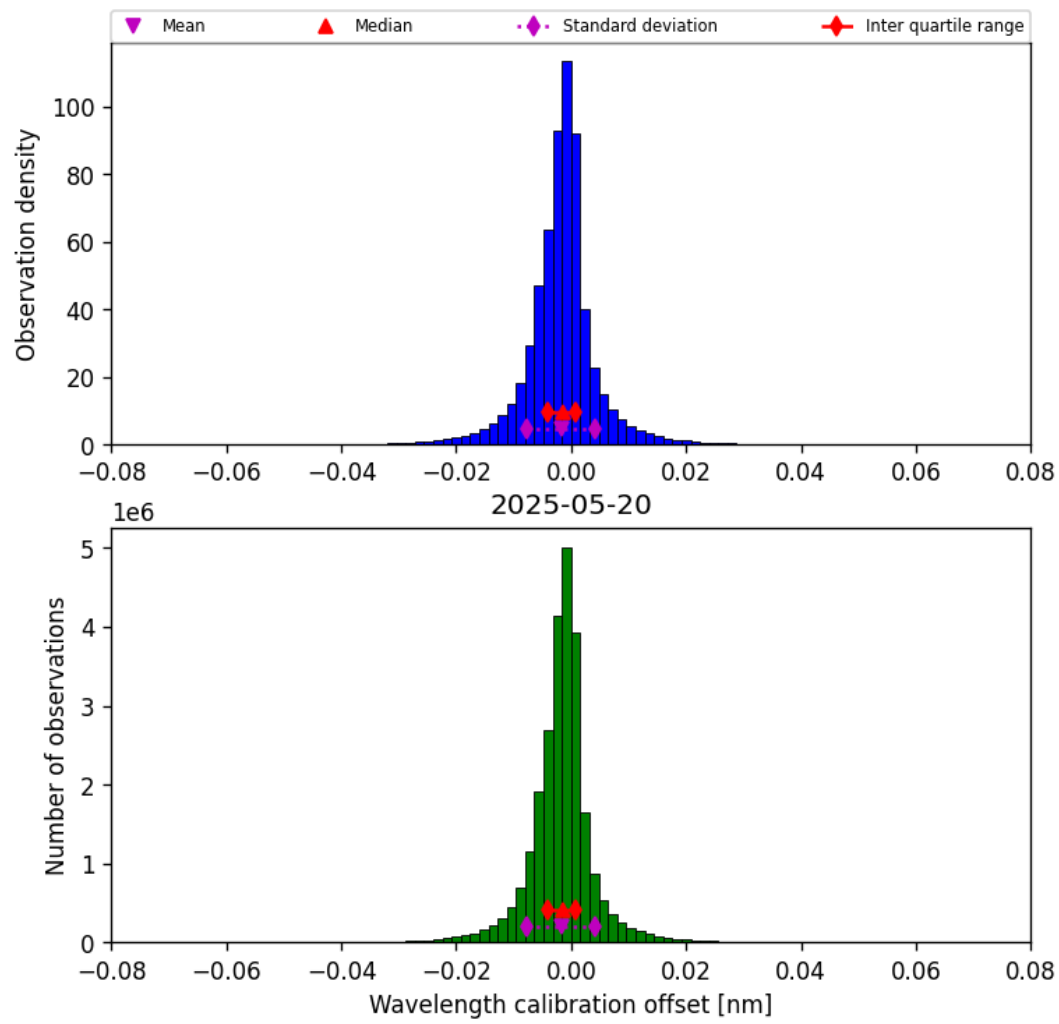
Figure 33: Histogram of “Wavelength calibration offset” for 2025-05-20 to 2025-05-21
