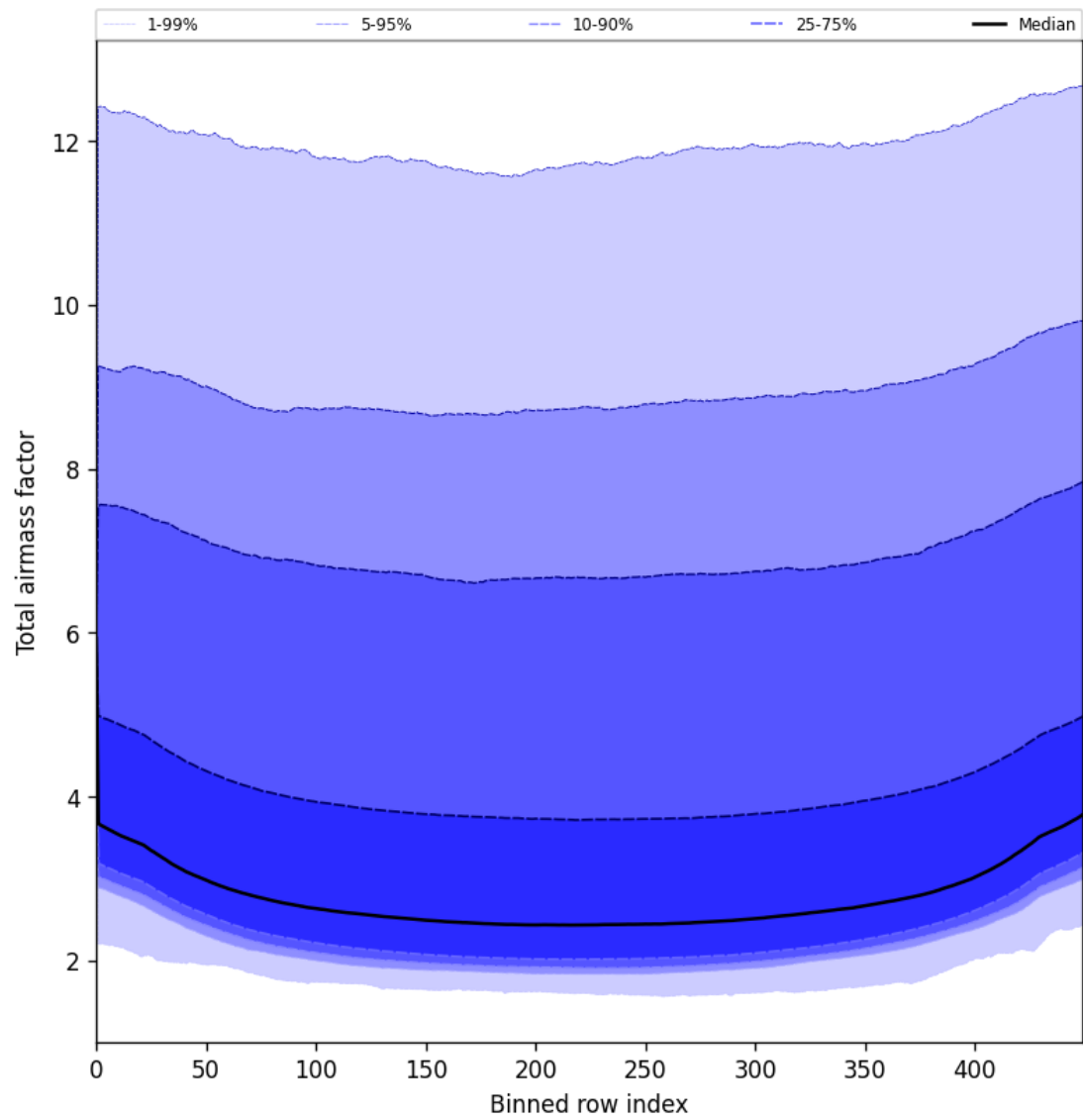
Figure 47: Along track statistics of “Total airmass factor” for 2025-05-20 to 2025-05-21
