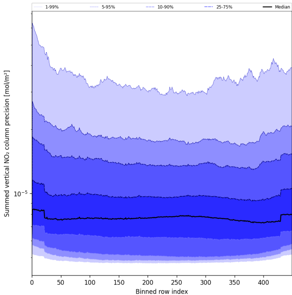
Figure 56: Along track statistics of “Summed vertical NO 2 column precision” for 2025-05-20 to 2025-05-21
