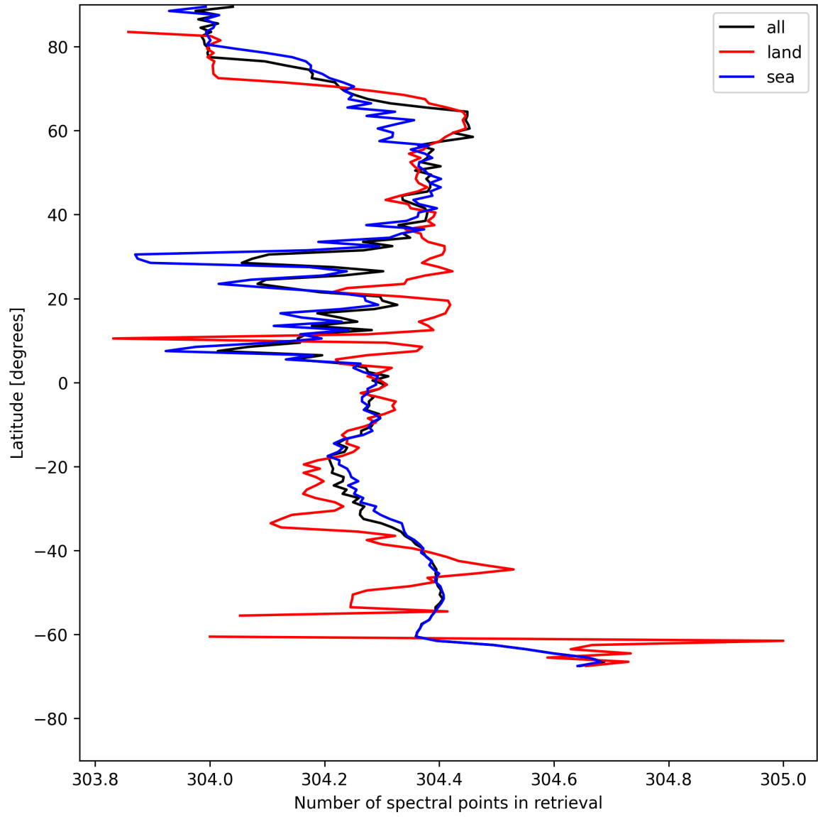
Figure 14: Zonal average of “Number of spectral points in retrieval” for 2025-05-20 to 2025-05-21.
