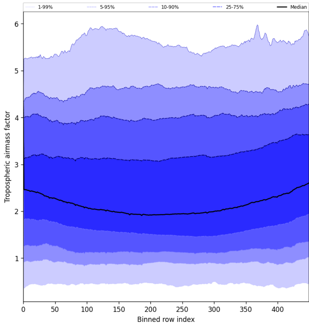
Figure 46: Along track statistics of “Tropospheric airmass factor” for 2025-05-20 to 2025-05-21
