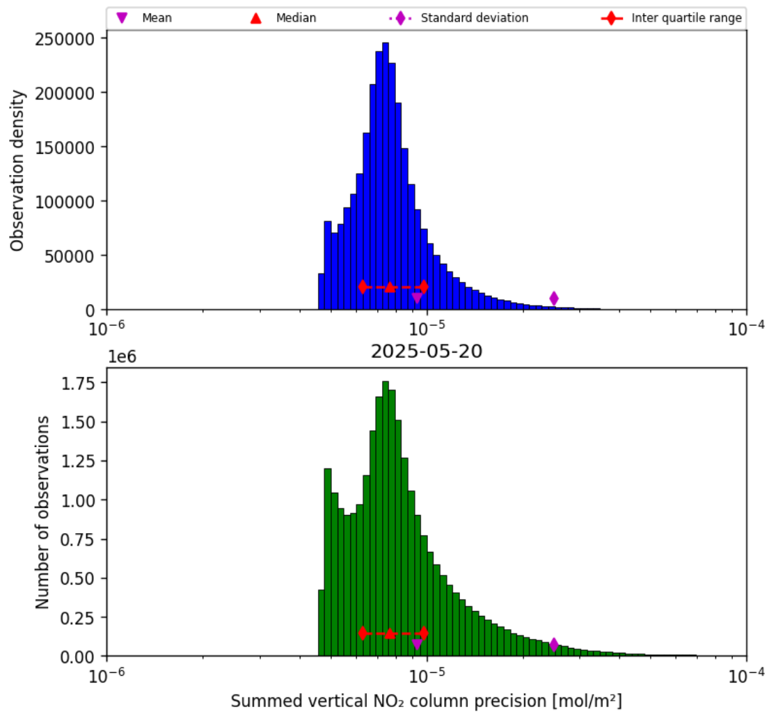
Figure 39: Histogram of “Summed vertical NO 2 column precision” for 2025-05-20 to 2025-05-21
