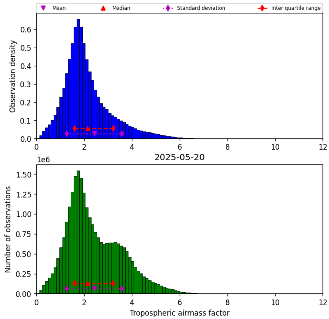
Figure 29: Histogram of “Tropospheric airmass factor” for 2025-05-20 to 2025-05-21
