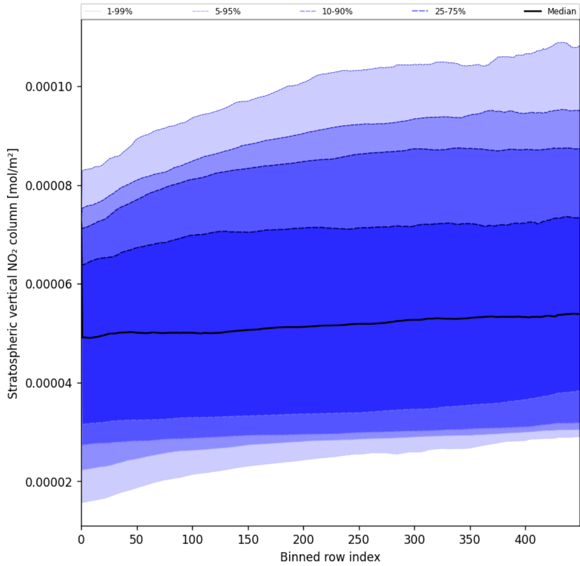
Figure 51: Along track statistics of “Stratospheric vertical NO 2 column” for 2025-05-20 to 2025-05-21
