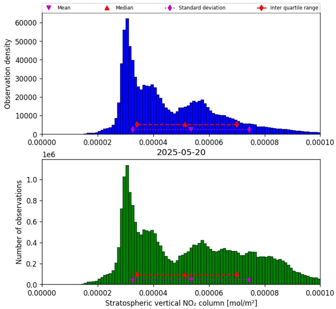
Figure 34: Histogram of “Stratospheric vertical NO 2 column” for 2025-05-20 to 2025-05-21
