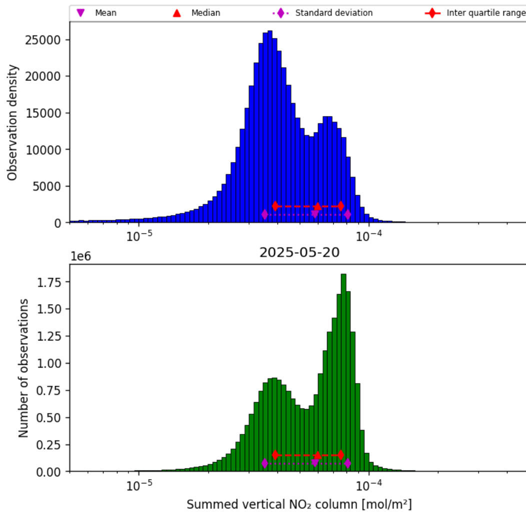
Figure 38: Histogram of “Summed vertical NO 2 column” for 2025-05-20 to 2025-05-21
