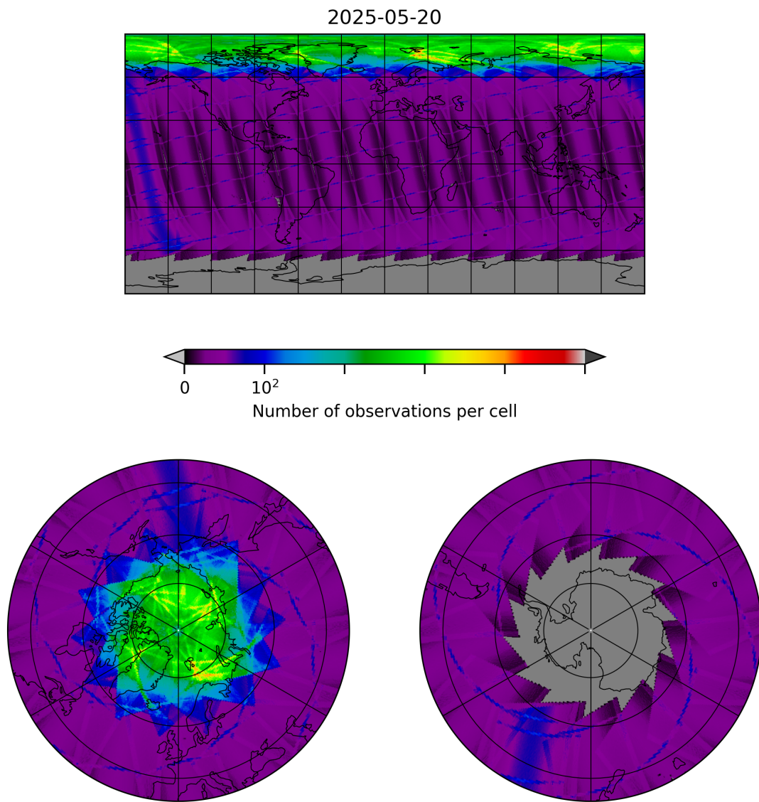
Figure 8: Map of the number of observations for 2025-05-20 to 2025-05-21
