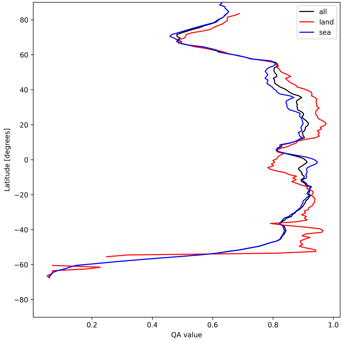
Figure 9: Zonal average of “QA value” for 2025-05-20 to 2025-05-21.
