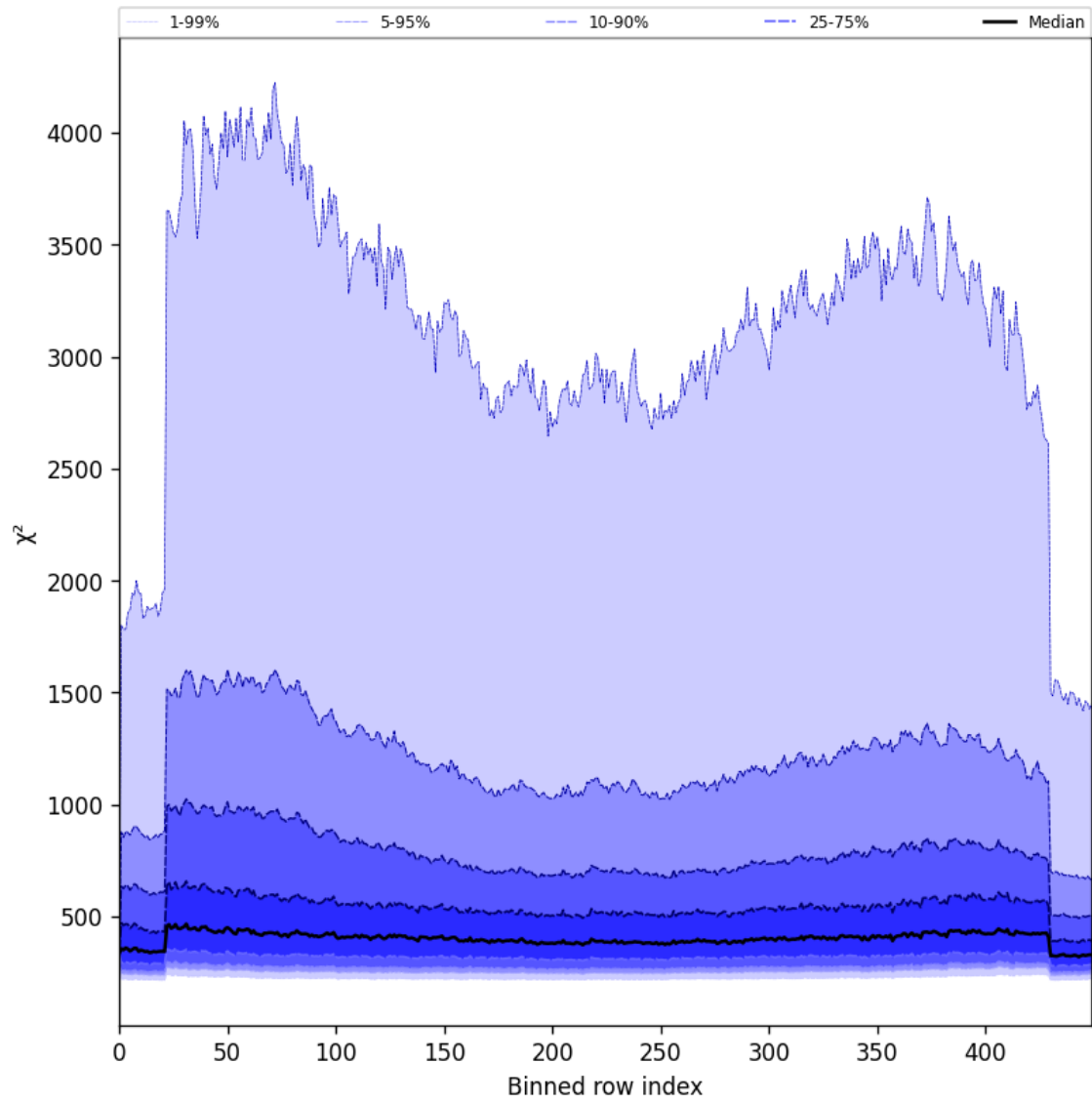
Figure 57: Along track statistics of “ \chi^2 ” for 2025-05-20 to 2025-05-21
