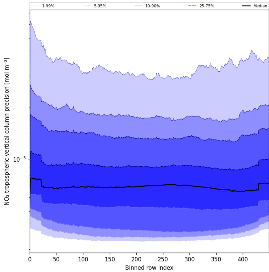
Figure 45: Along track statistics of “NO 2 tropospheric vertical column precision” for 2025-05-20 to 2025-05-21
