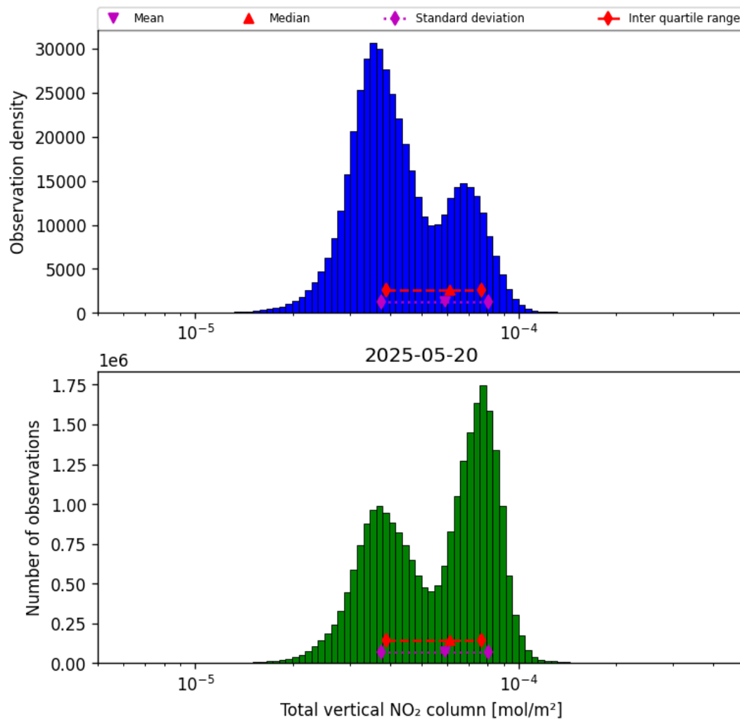
Figure 36: Histogram of "Total vertical NO 2 column" for 2025-05-20 to 2025-05-21
