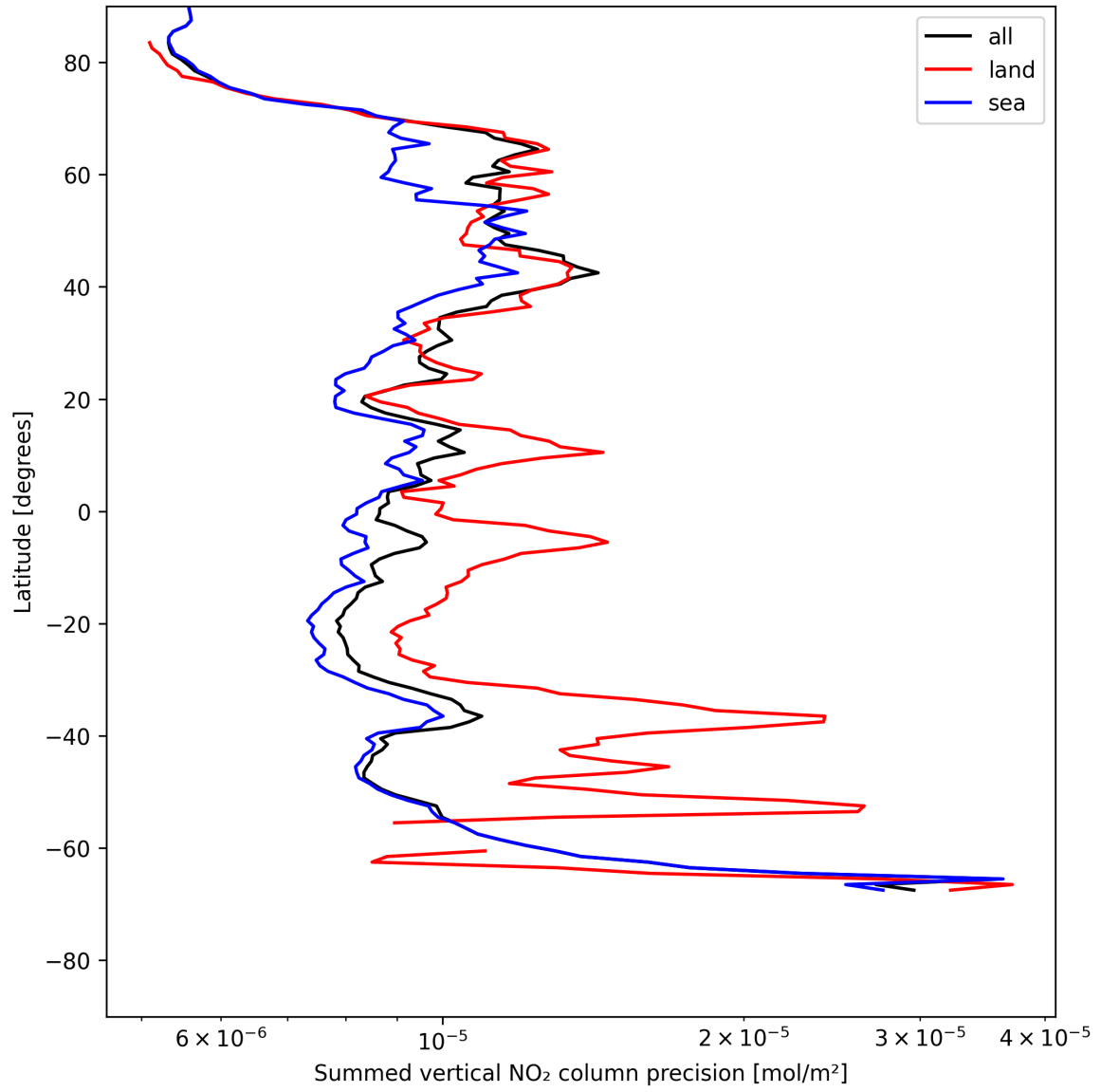
Figure 22: Zonal average of “Summed vertical NO 2 column precision” for 2025-05-20 to 2025-05-21.
