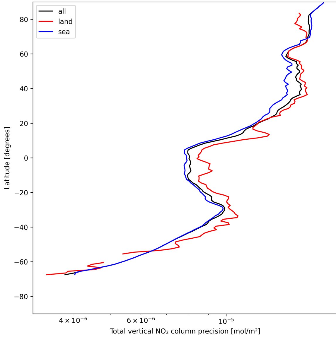
Figure 20: Zonal average of “Total vertical NO 2 column precision” for 2025-05-20 to 2025-05-21.
