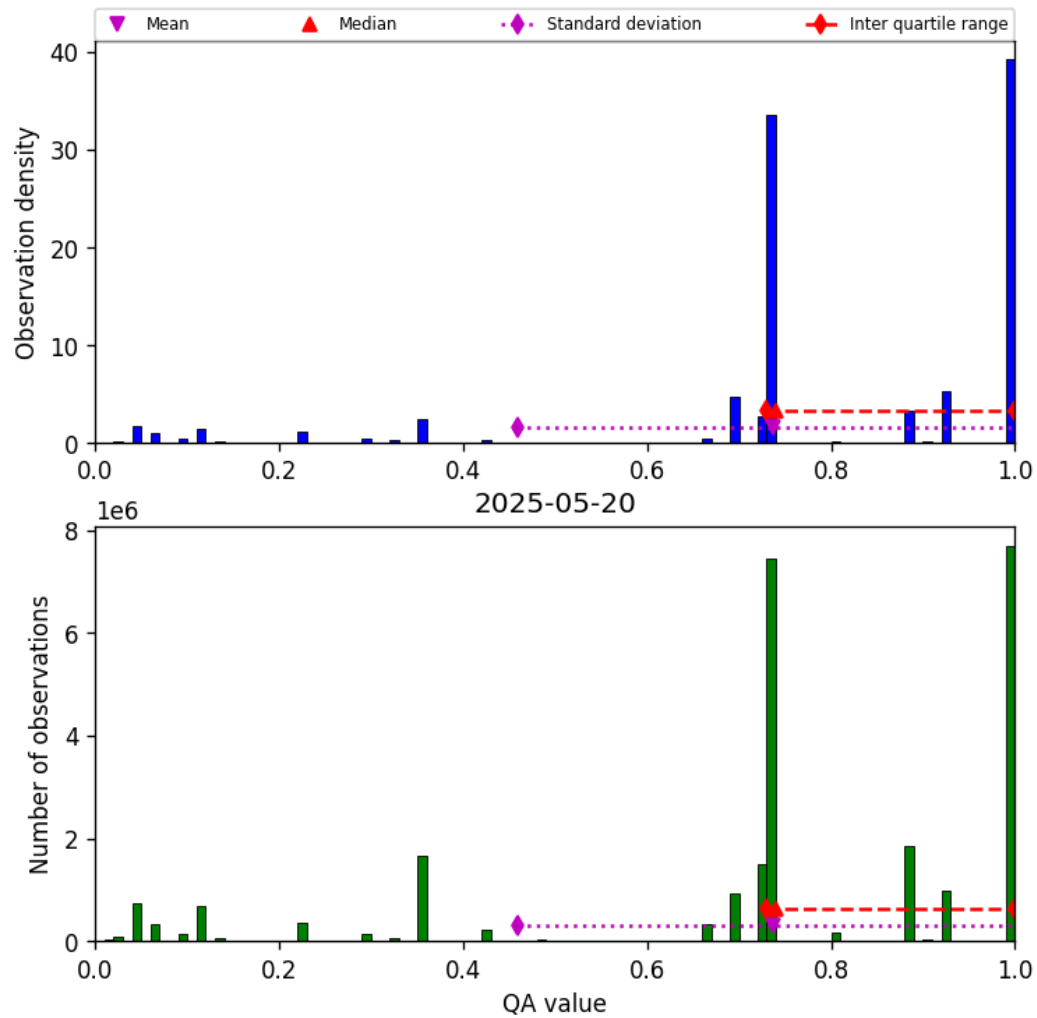
Figure 26: Histogram of “QA value” for 2025-05-20 to 2025-05-21
