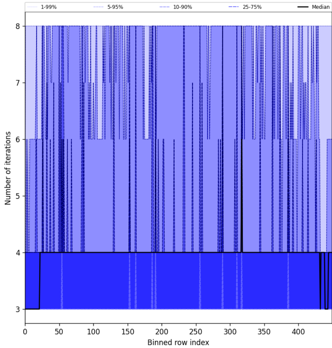
Figure 49: Along track statistics of “Number of iterations” for 2025-05-20 to 2025-05-21
