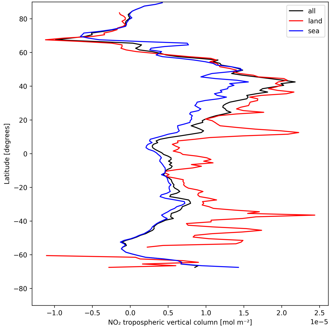
Figure 10: Zonal average of “NO 2 tropospheric vertical column” for 2025-05-20 to 2025-05-21.
