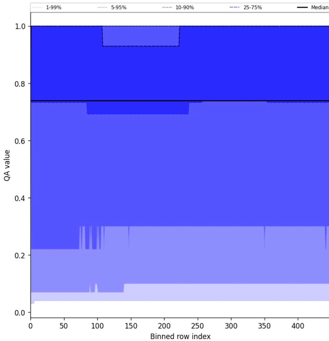
Figure 43: Along track statistics of “QA value” for 2025-05-20 to 2025-05-21
