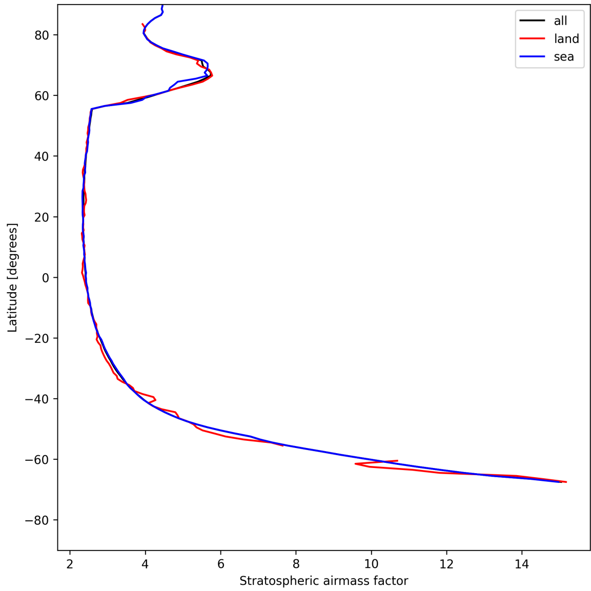
Figure 25: Zonal average of “Stratospheric airmass factor” for 2025-05-20 to 2025-05-21.
