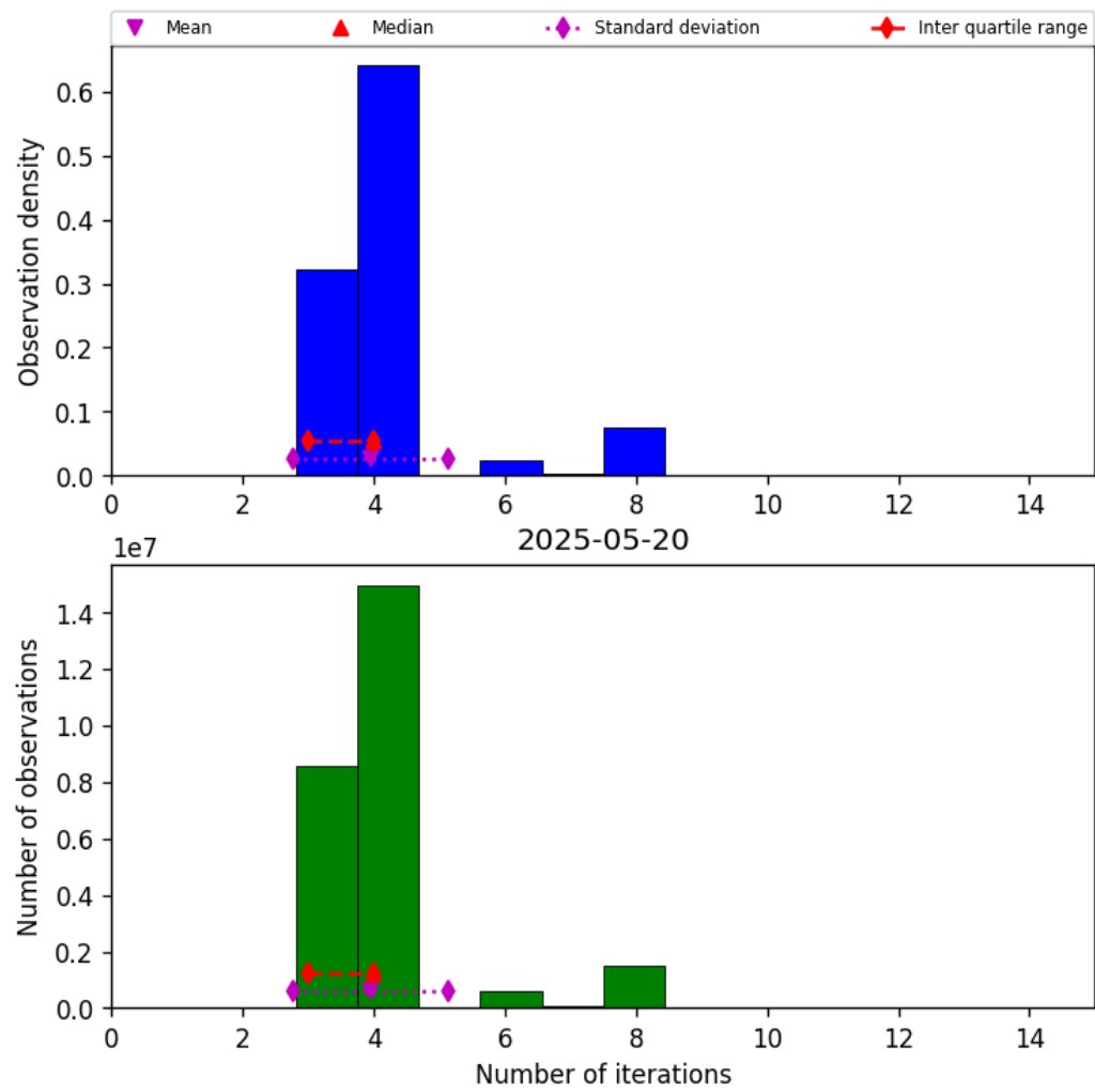
Figure 32: Histogram of “Number of iterations” for 2025-05-20 to 2025-05-21
