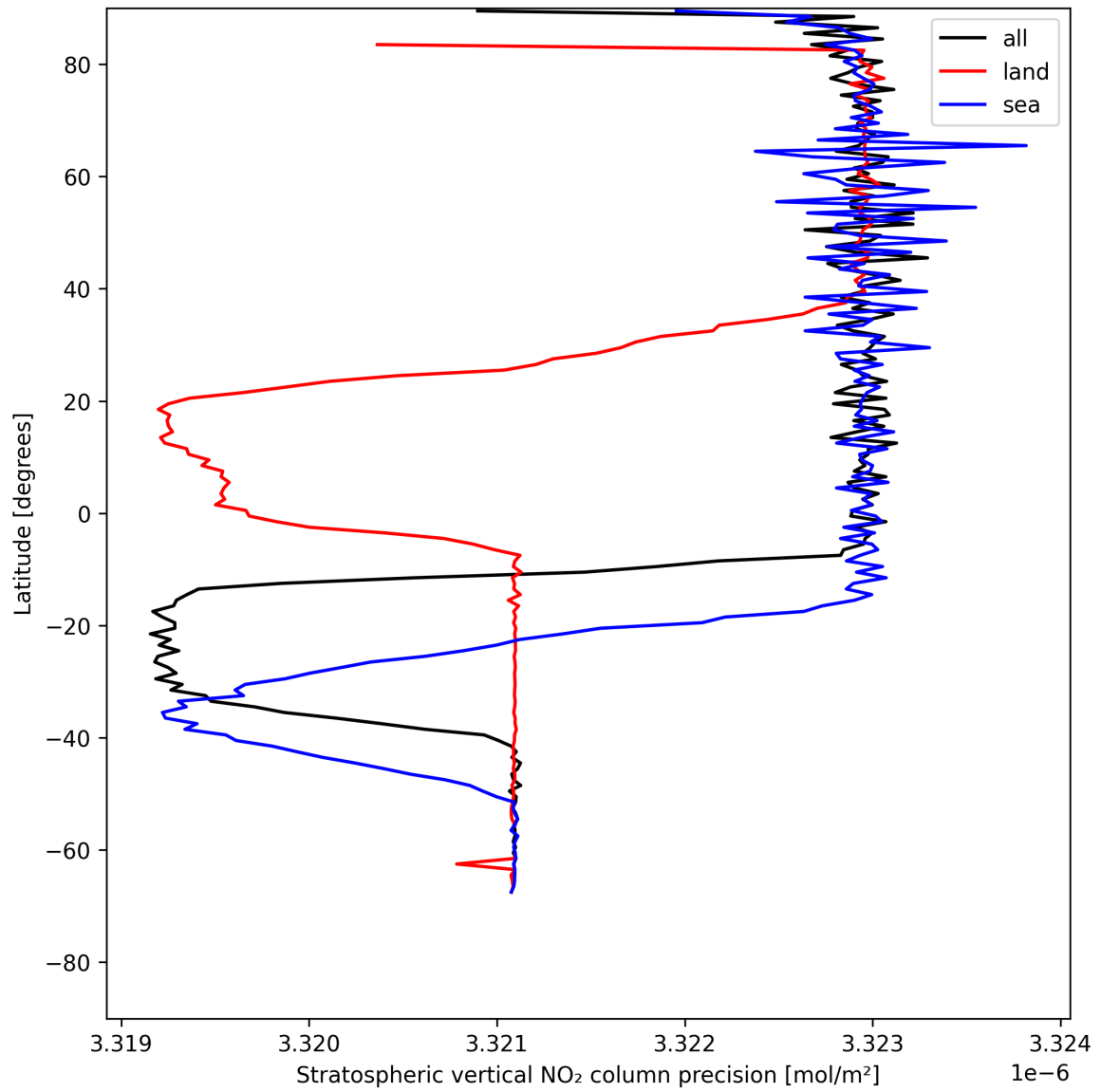
Figure 18: Zonal average of “Stratospheric vertical NO 2 column precision” for 2025-05-20 to 2025-05-21.
