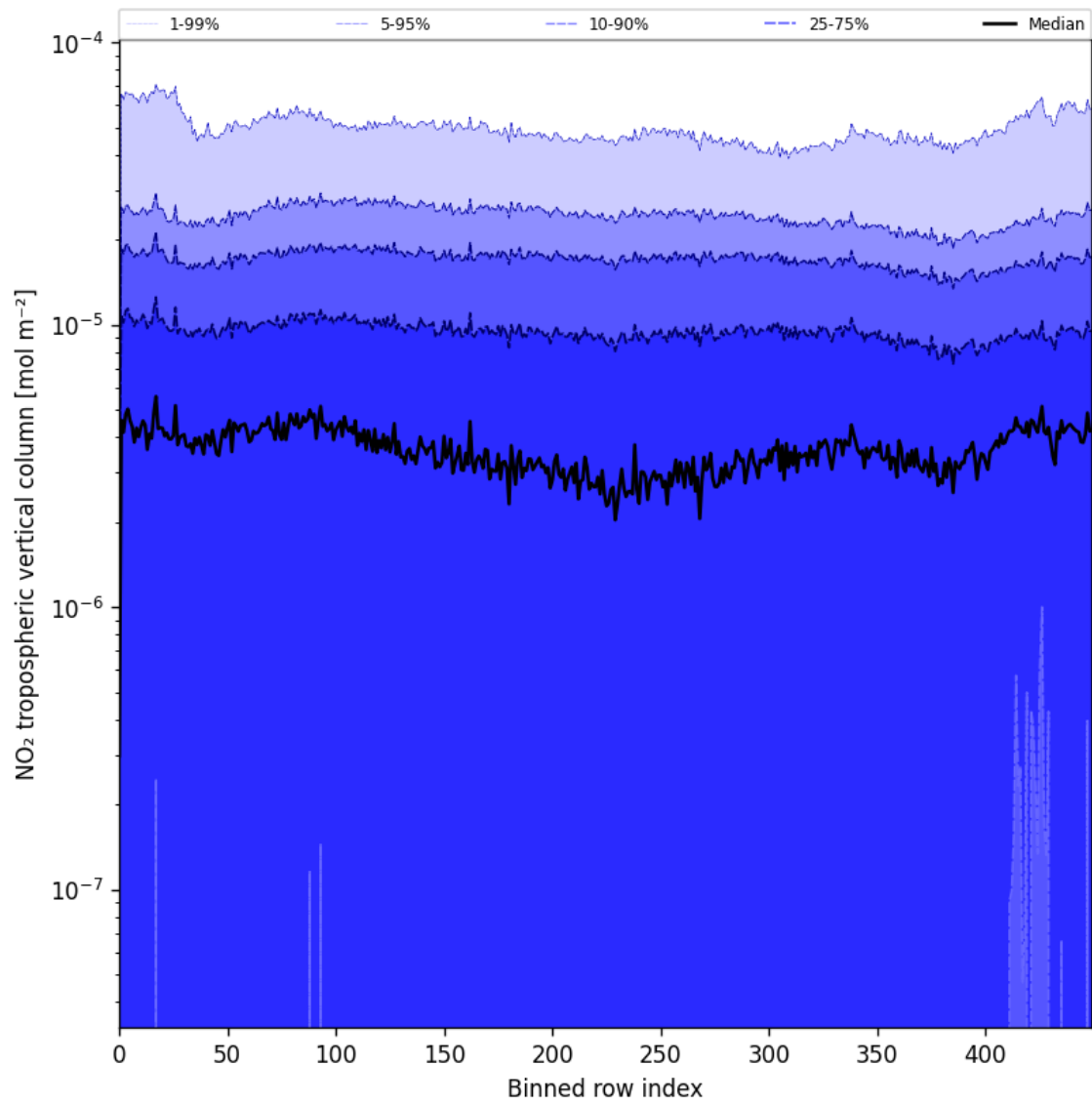
Figure 44: Along track statistics of “NO 2 tropospheric vertical column” for 2025-05-20 to 2025-05-21
