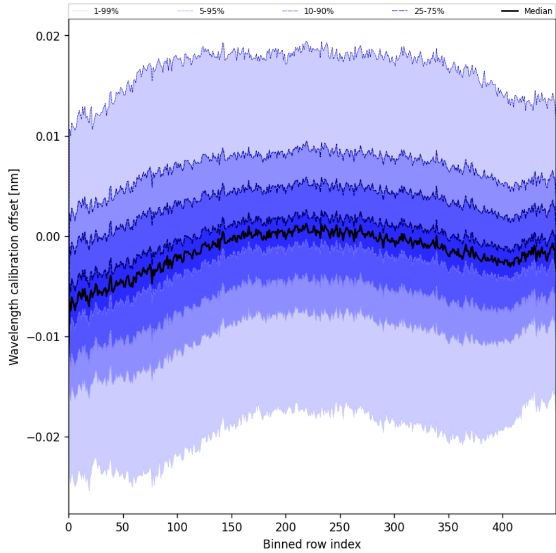
Figure 50: Along track statistics of “Wavelength calibration offset” for 2025-05-20 to 2025-05-21
