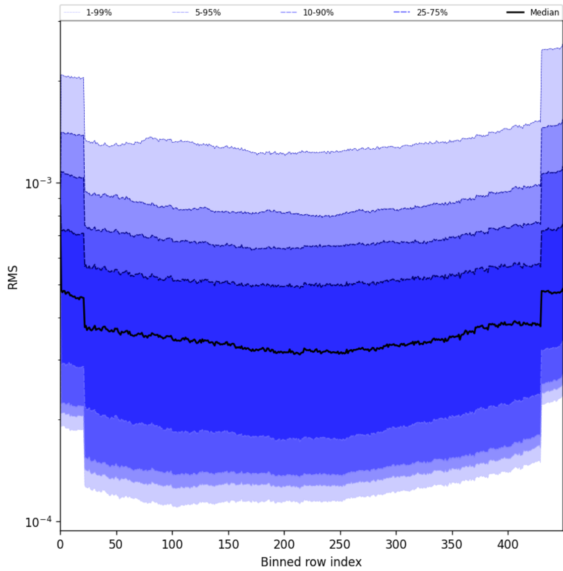
Figure 58: Along track statistics of “RMS” for 2025-05-20 to 2025-05-21
