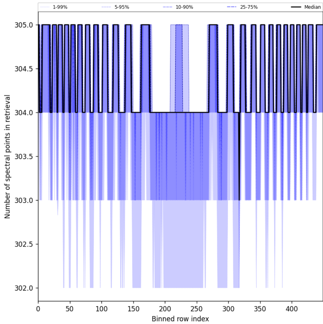
Figure 48: Along track statistics of “Number of spectral points in retrieval” for 2025-05-20 to 2025-05-21
