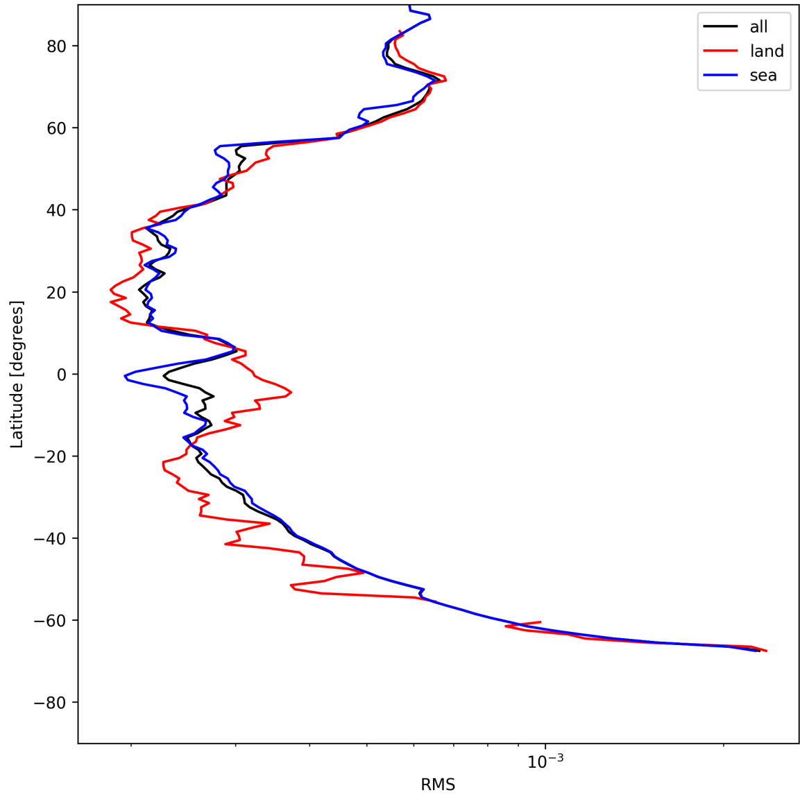
Figure 24: Zonal average of “RMS” for 2025-05-20 to 2025-05-21.
