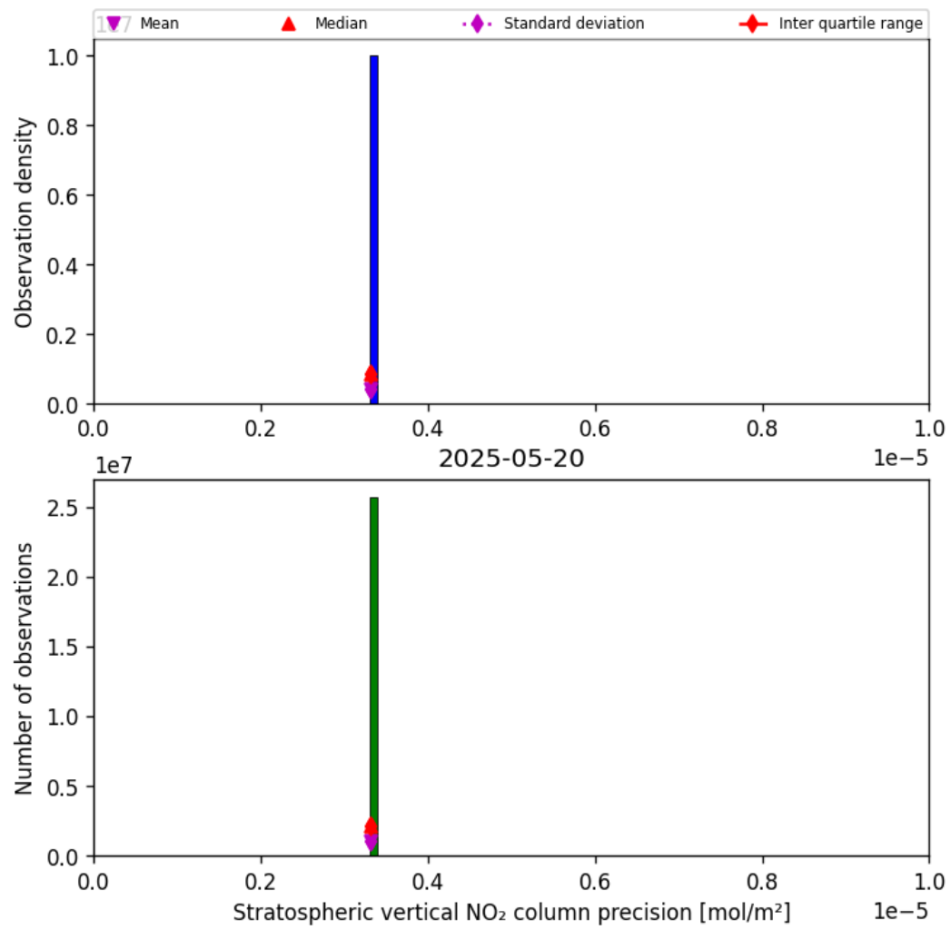
Figure 35: Histogram of “Stratospheric vertical NO 2 column precision” for 2025-05-20 to 2025-05-21
