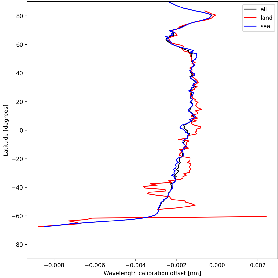
Figure 16: Zonal average of “Wavelength calibration offset” for 2025-05-20 to 2025-05-21.
