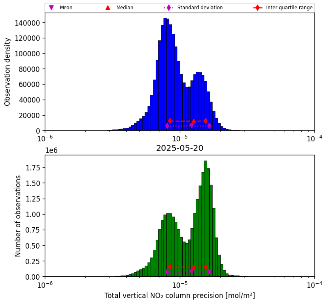
Figure 37: Histogram of “Total vertical NO 2 column precision” for 2025-05-20 to 2025-05-21
