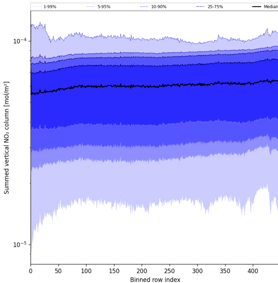
Figure 55: Along track statistics of “Summed vertical NO 2 column” for 2025-05-20 to 2025-05-21
