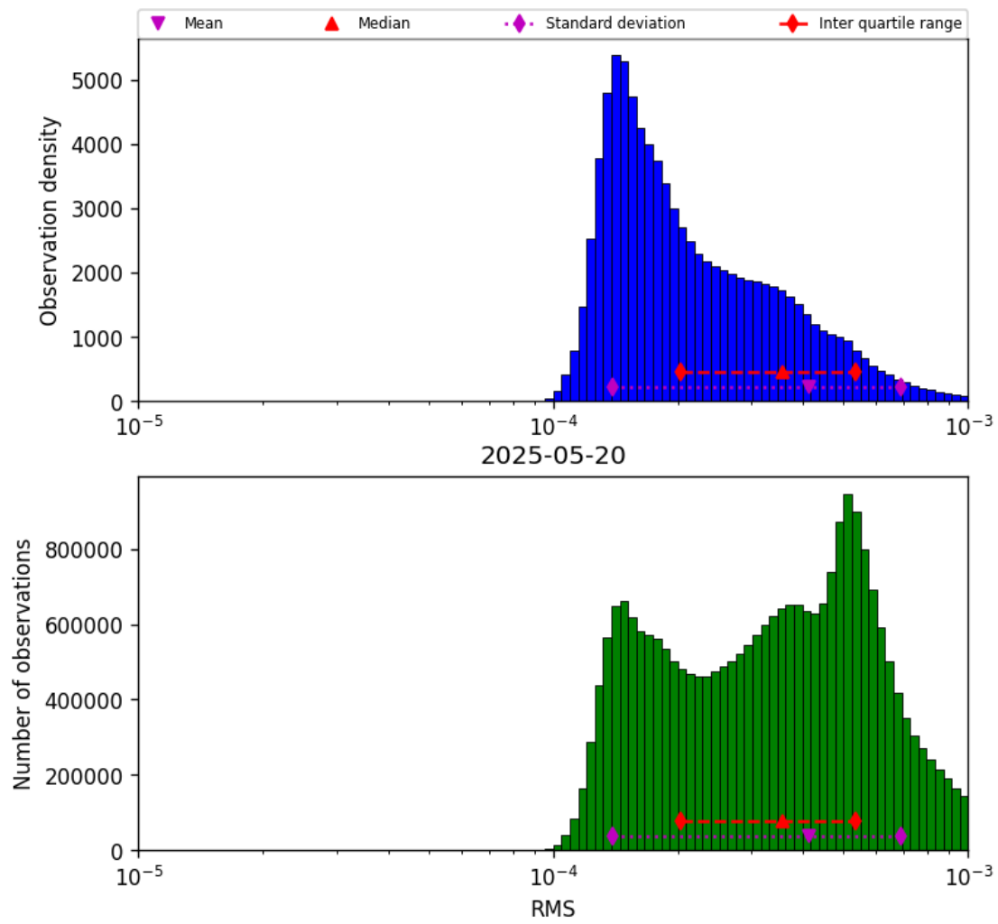
Figure 41: Histogram of “RMS” for 2025-05-20 to 2025-05-21
