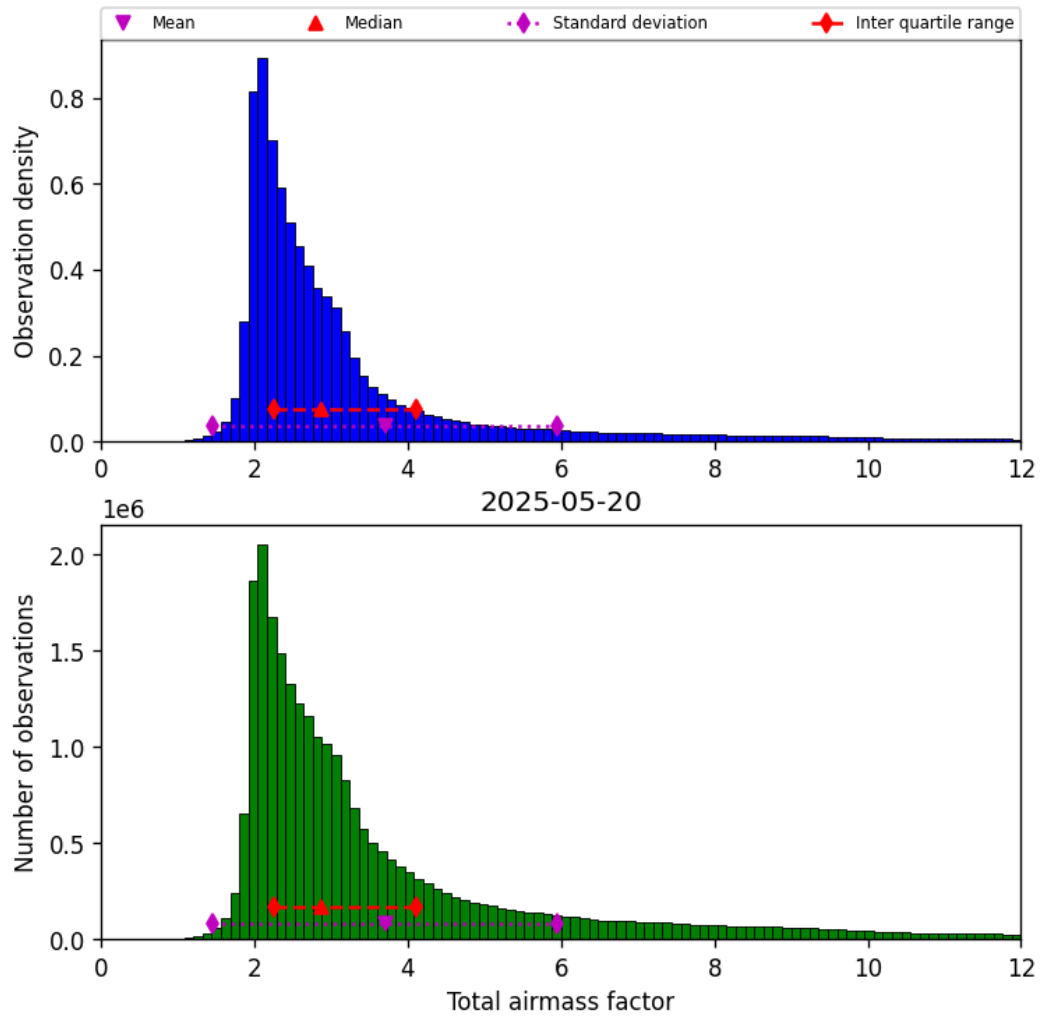
Figure 30: Histogram of “Total airmass factor” for 2025-05-20 to 2025-05-21
