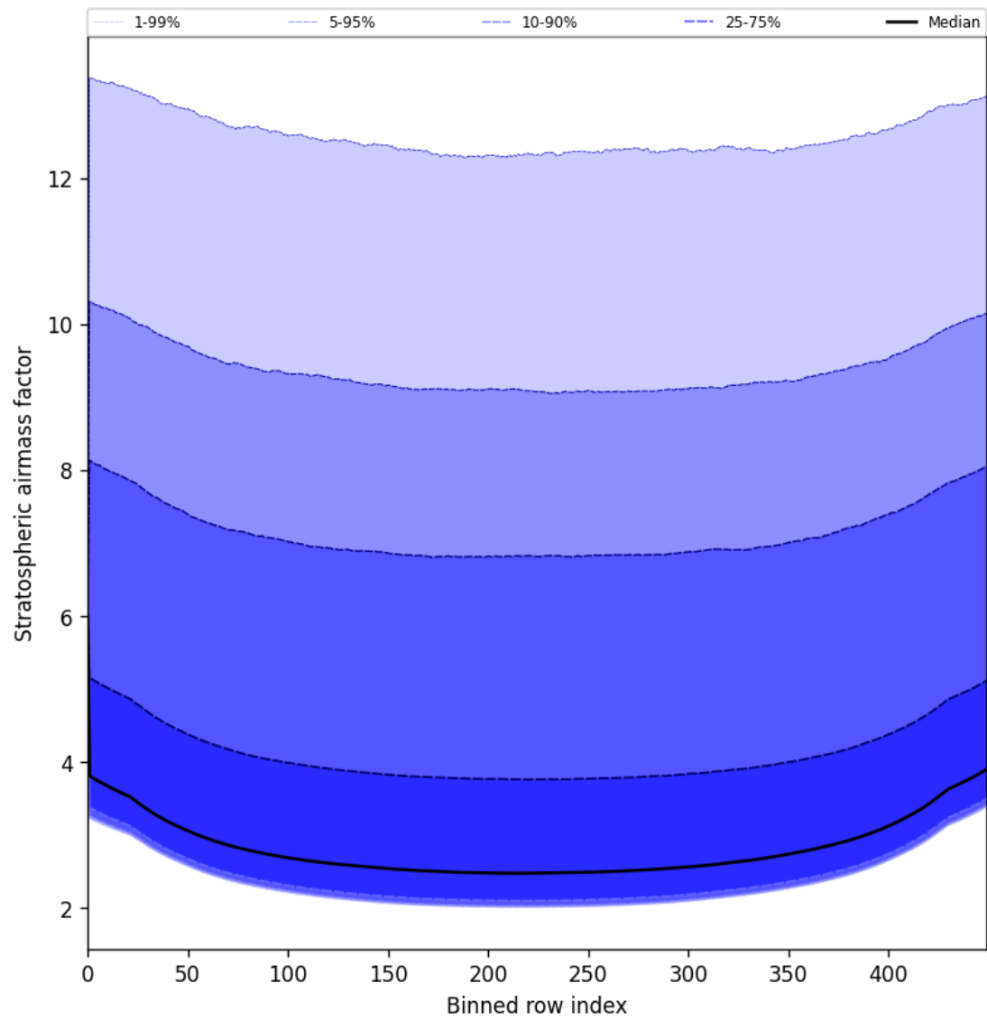
Figure 59: Along track statistics of “Stratospheric air mass factor” for 2025-05-20 to 2025-05-21
