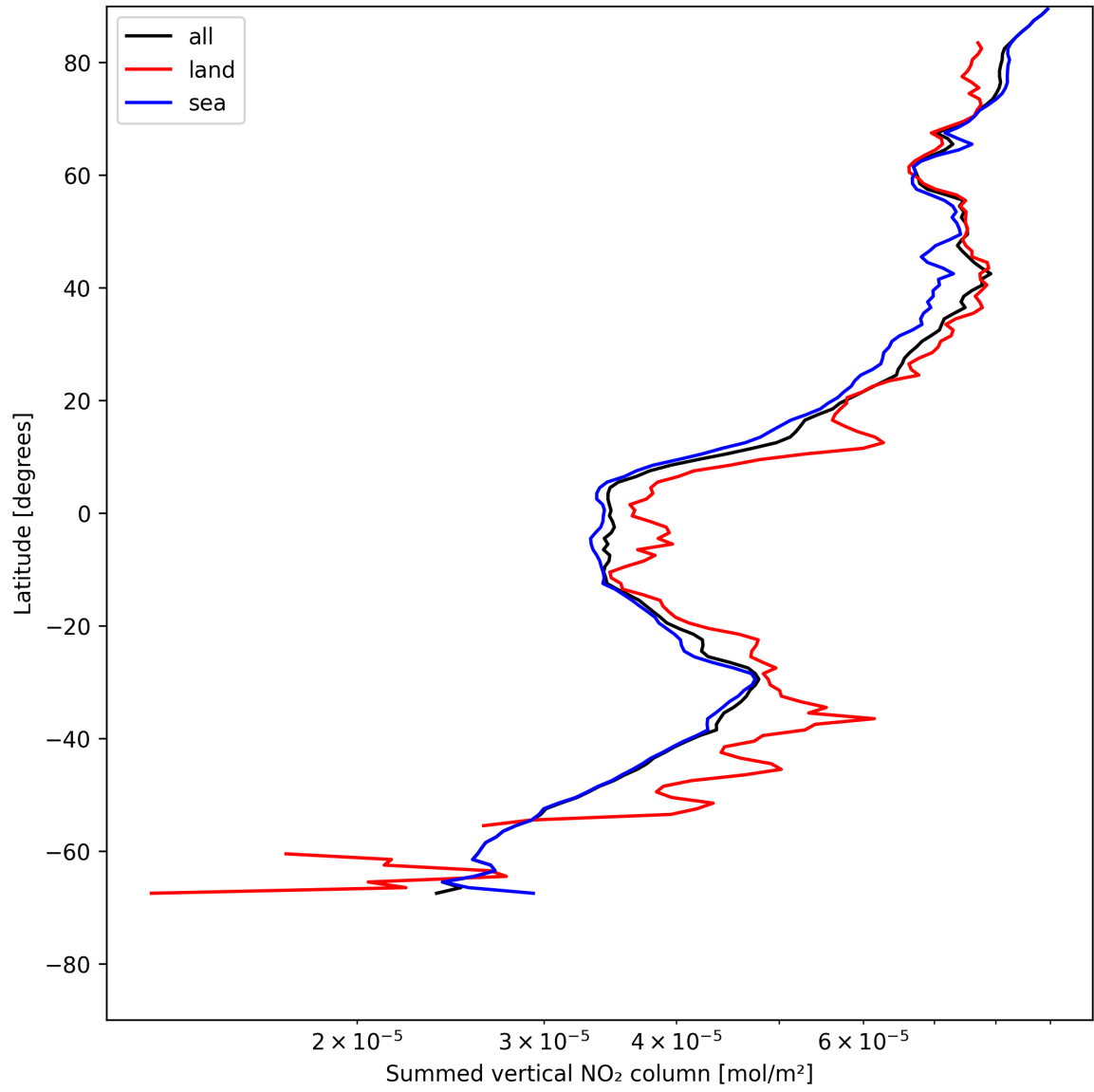
Figure 21: Zonal average of “Summed vertical NO 2 column” for 2025-05-20 to 2025-05-21.
