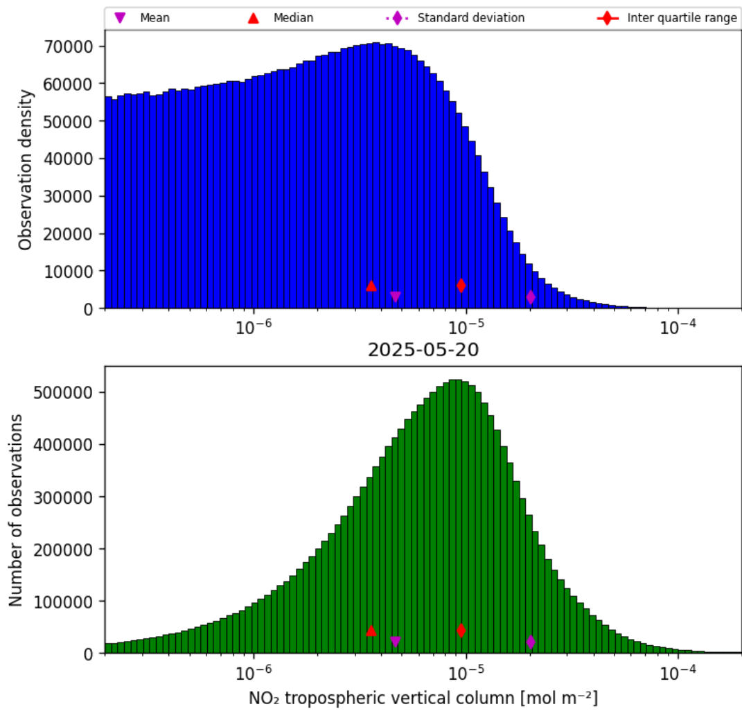
Figure 27: Histogram of “NO 2 tropospheric vertical column” for 2025-05-20 to 2025-05-21
