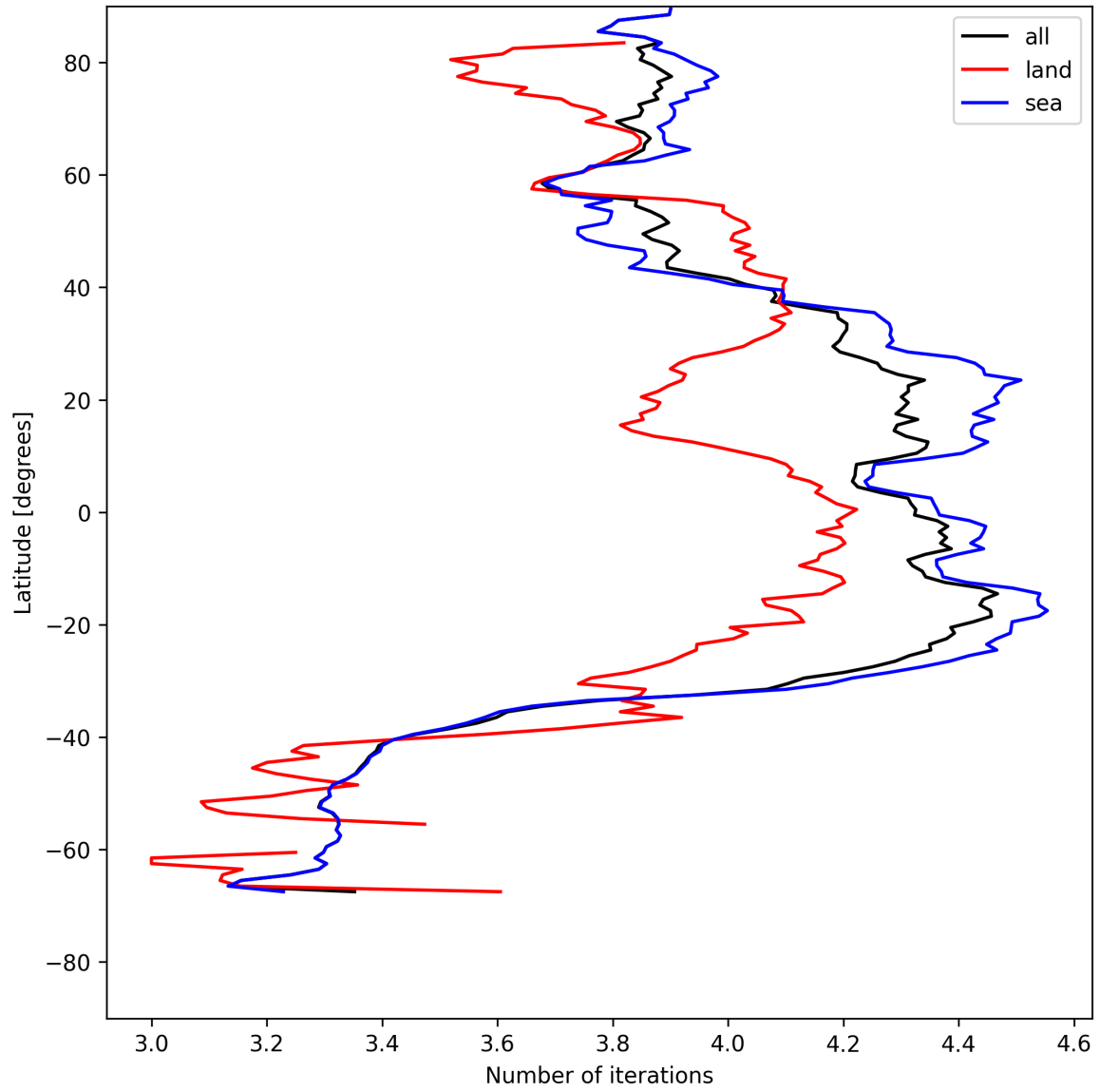
Figure 15: Zonal average of “Number of iterations” for 2025-05-20 to 2025-05-21.
