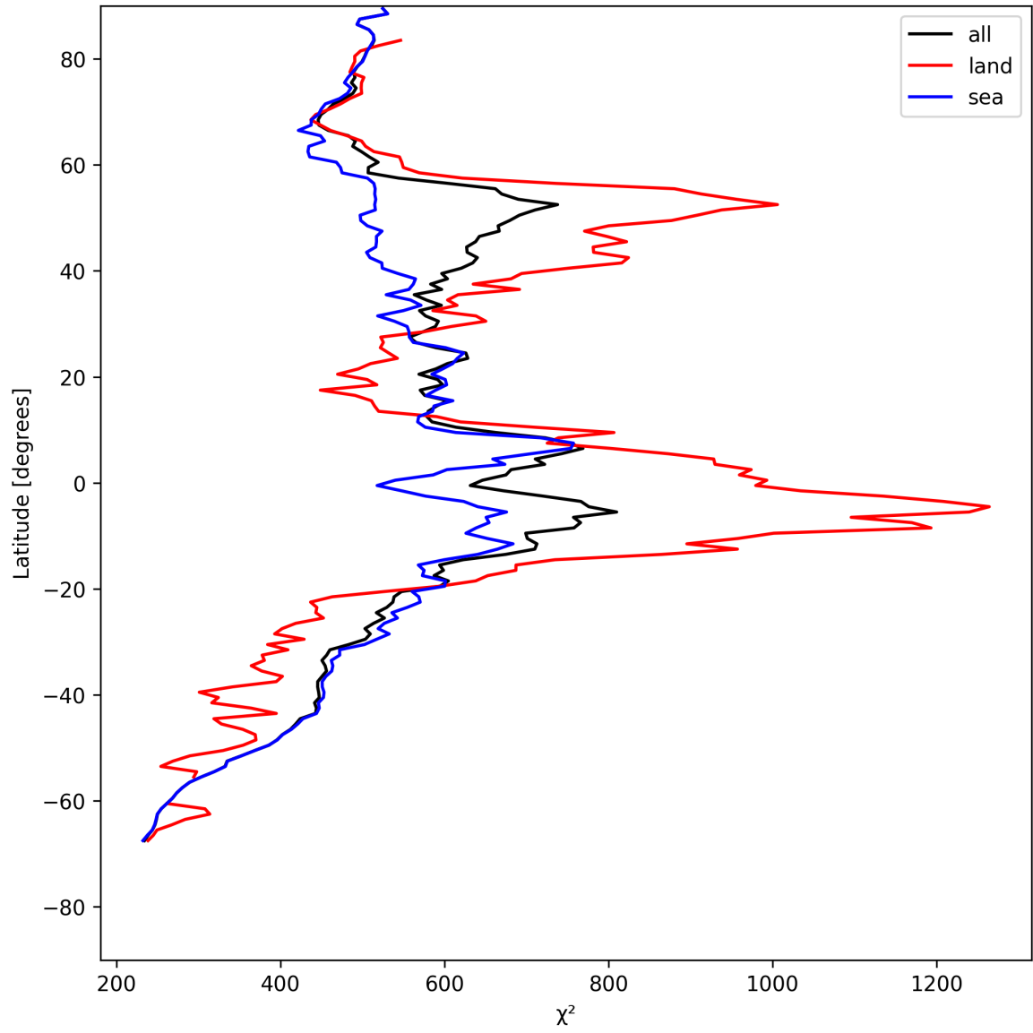
Figure 23: Zonal average of “ \chi^2 ” for 2025-05-20 to 2025-05-21.
