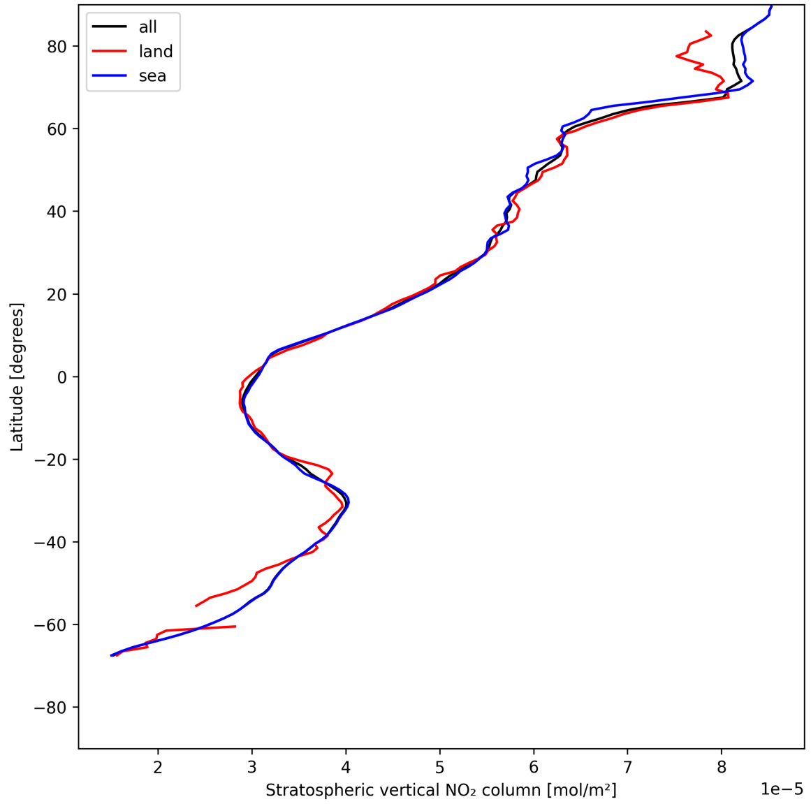
Figure 17: Zonal average of “Stratospheric vertical NO 2 column” for 2025-05-20 to 2025-05-21.
