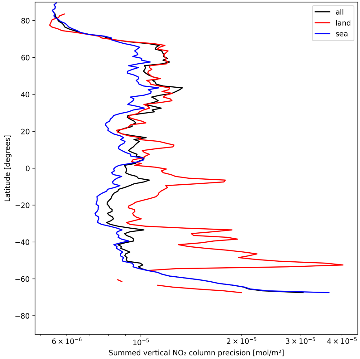
Figure 22: Zonal average of “Summed vertical NO 2 column precision” for 2025-05-21 to 2025-05-22.
