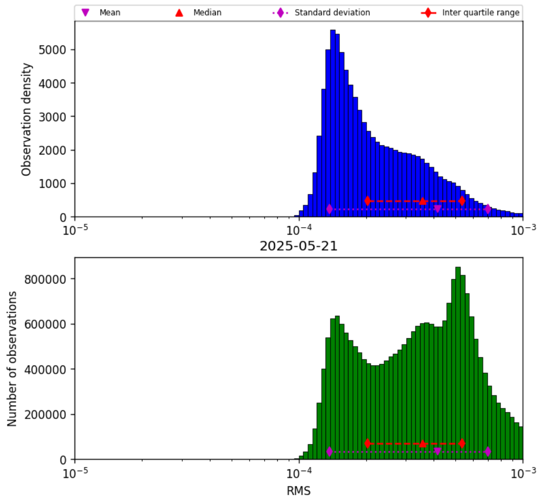
Figure 41: Histogram of “RMS” for 2025-05-21 to 2025-05-22
