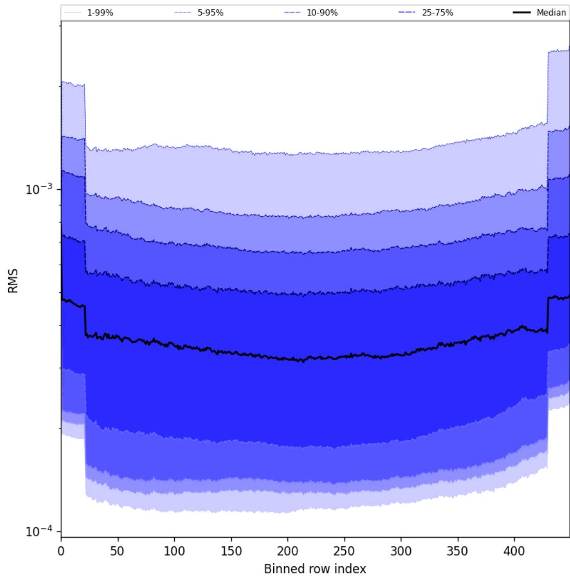
Figure 58: Along track statistics of “RMS” for 2025-05-21 to 2025-05-22
