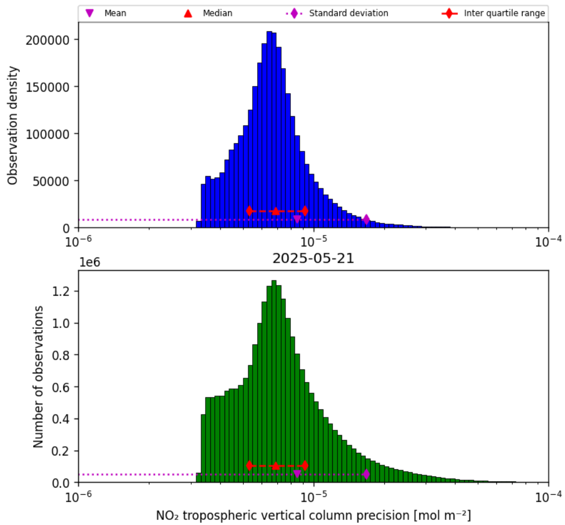
Figure 28: Histogram of “NO 2 tropospheric vertical column precision” for 2025-05-21 to 2025-05-22
