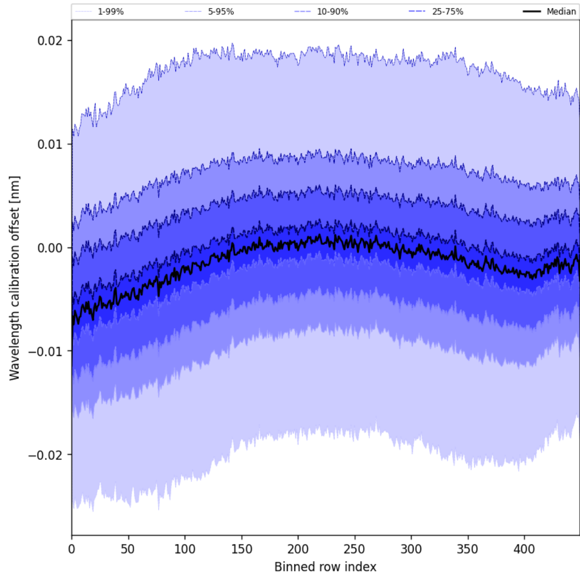
Figure 50: Along track statistics of “Wavelength calibration offset” for 2025-05-21 to 2025-05-22
