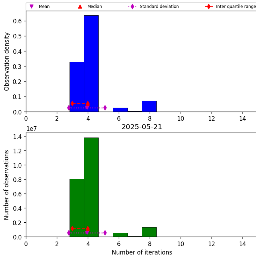
Figure 32: Histogram of “Number of iterations” for 2025-05-21 to 2025-05-22
