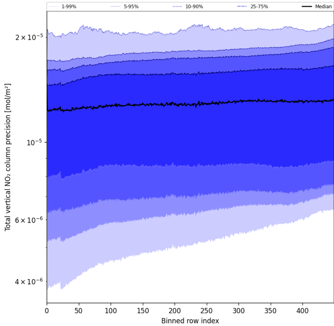
Figure 54: Along track statistics of “Total vertical NO 2 column precision” for 2025-05-21 to 2025-05-22
