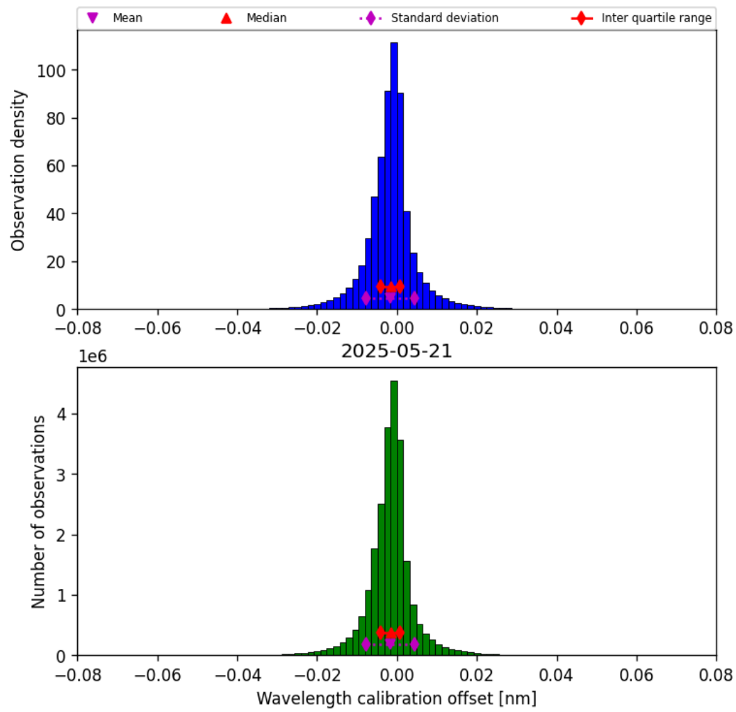
Figure 33: Histogram of “Wavelength calibration offset” for 2025-05-21 to 2025-05-22
