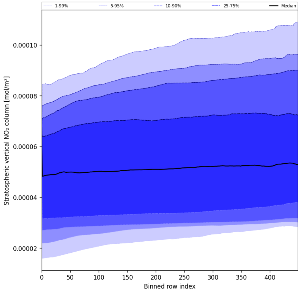
Figure 51: Along track statistics of “Stratospheric vertical NO 2 column” for 2025-05-21 to 2025-05-22
