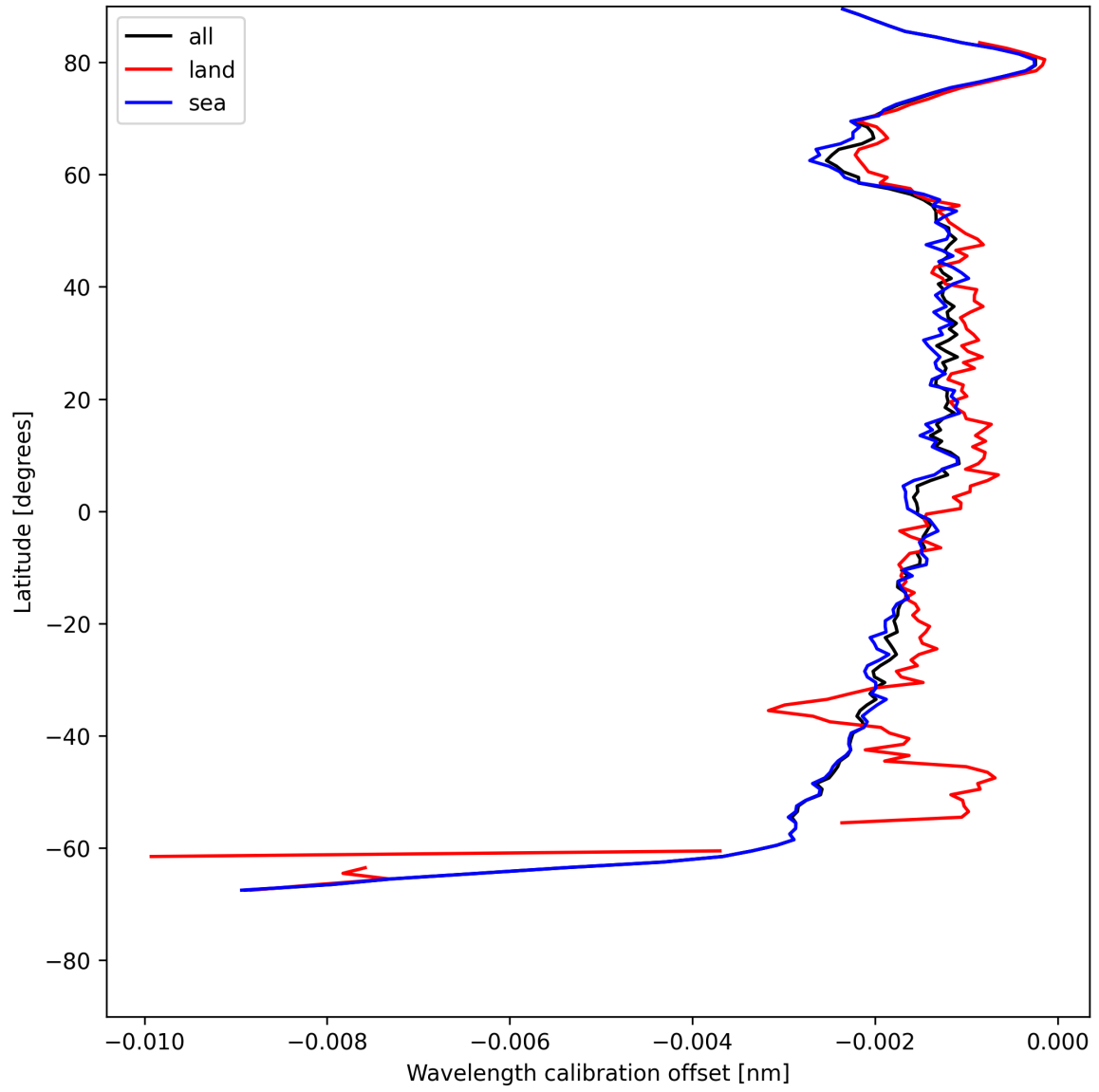
Figure 16: Zonal average of “Wavelength calibration offset” for 2025-05-21 to 2025-05-22.
