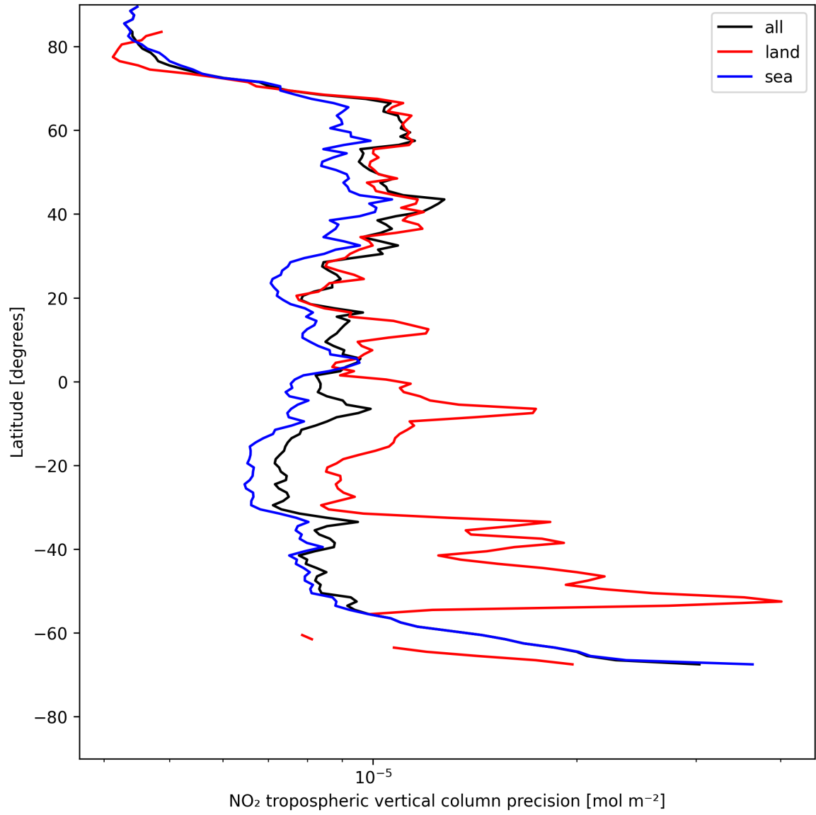
Figure 11: Zonal average of “NO 2 tropospheric vertical column precision” for 2025-05-21 to 2025-05-22.
