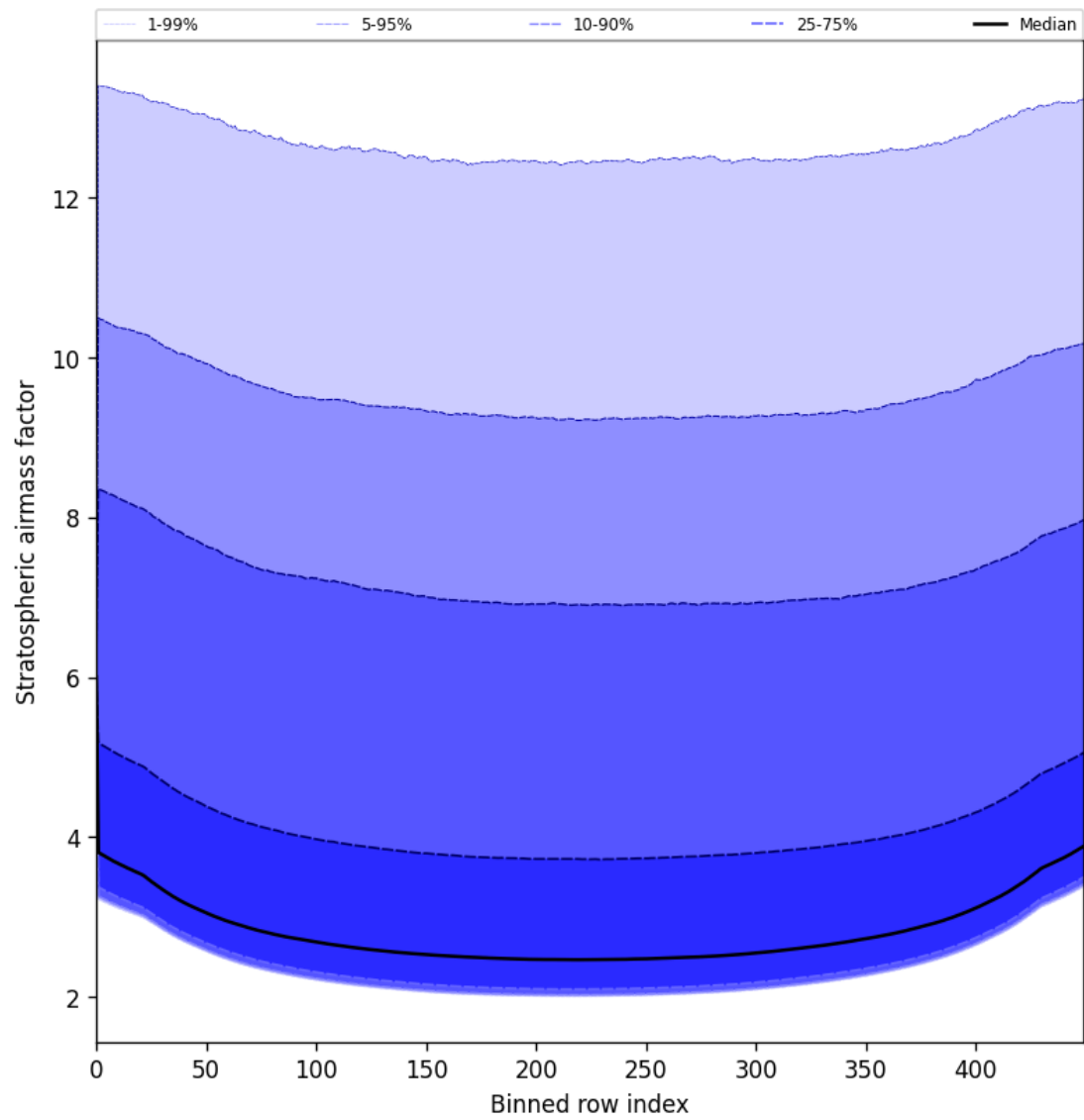
Figure 59: Along track statistics of “Stratospheric airmass factor” for 2025-05-21 to 2025-05-22
