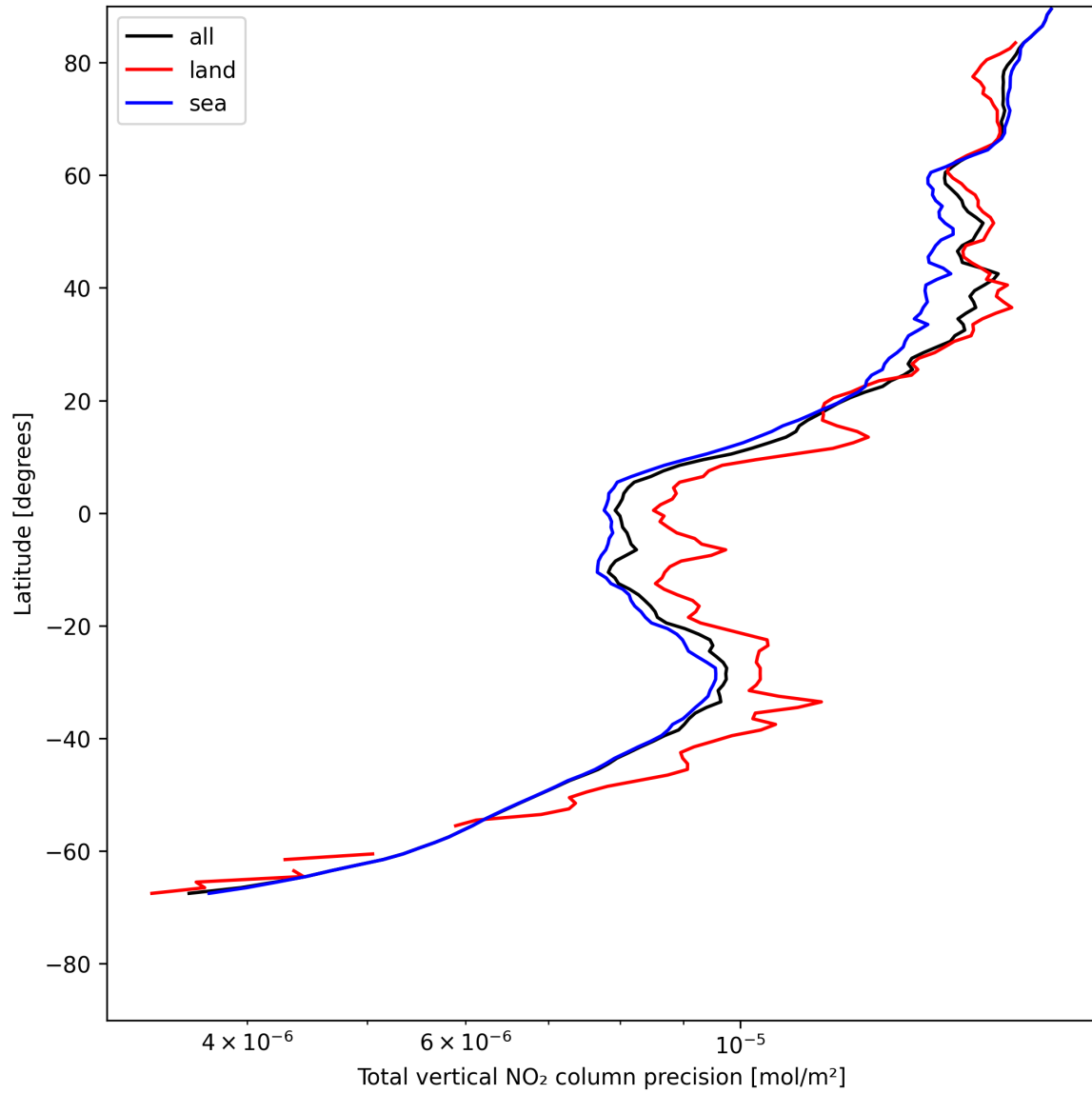
Figure 20: Zonal average of “Total vertical NO 2 column precision” for 2025-05-21 to 2025-05-22.
