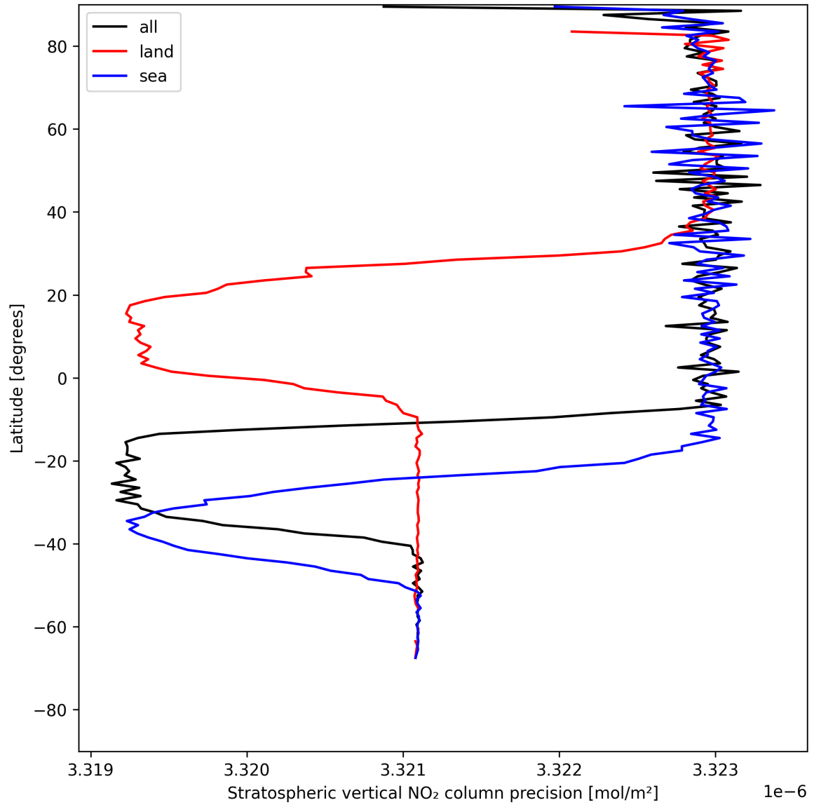
Figure 18: Zonal average of “Stratospheric vertical NO 2 column precision” for 2025-05-21 to 2025-05-22.
