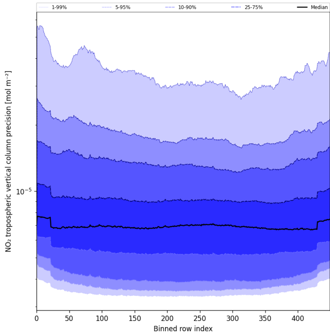
Figure 45: Along track statistics of “NO 2 tropospheric vertical column precision” for 2025-05-21 to 2025-05-22
