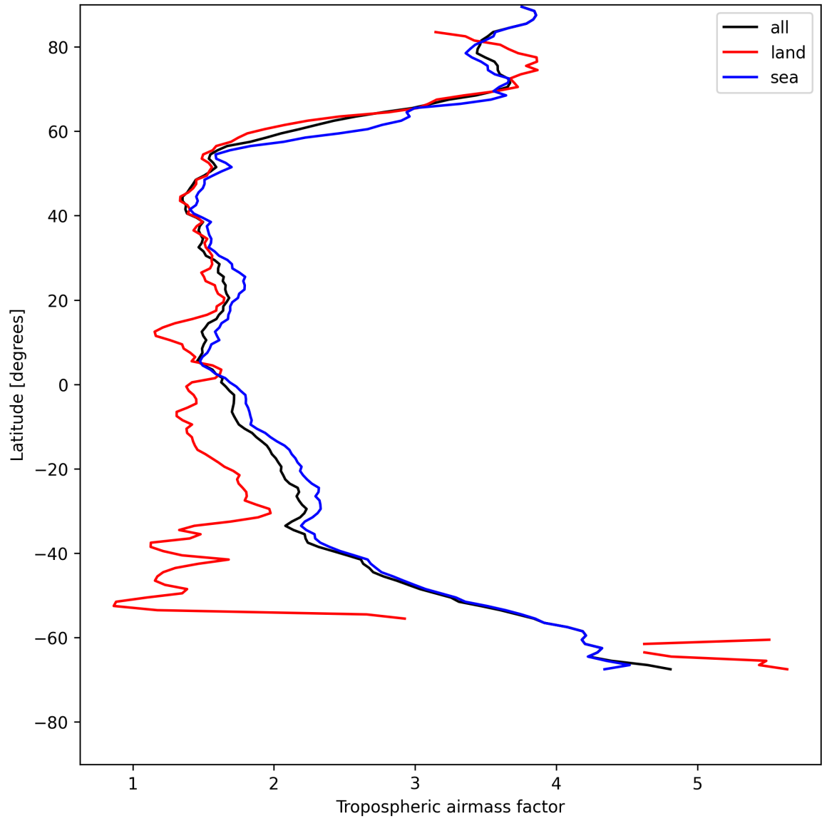
Figure 12: Zonal average of “Tropospheric air mass factor” for 2025-05-21 to 2025-05-22.
