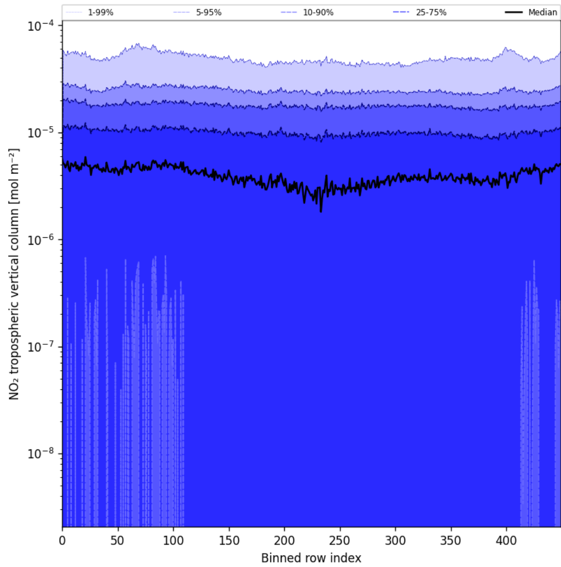
Figure 44: Along track statistics of “NO 2 tropospheric vertical column” for 2025-05-21 to 2025-05-22
