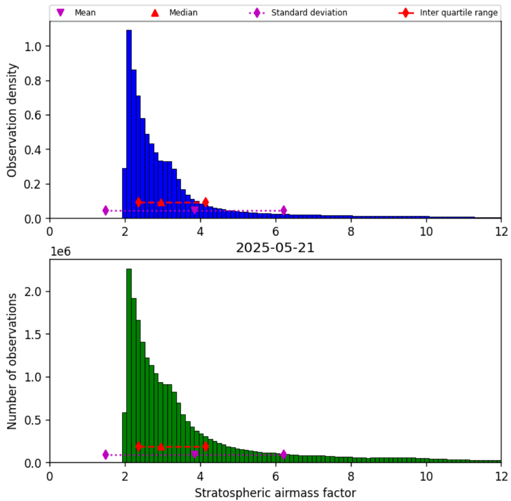
Figure 42: Histogram of “Stratospheric airmass factor” for 2025-05-21 to 2025-05-22
