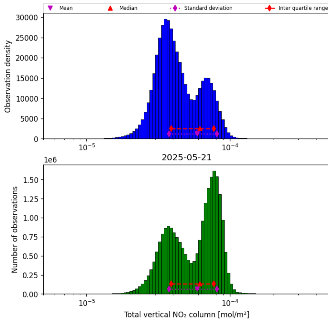
Figure 36: Histogram of “Total vertical NO 2 column” for 2025-05-21 to 2025-05-22
