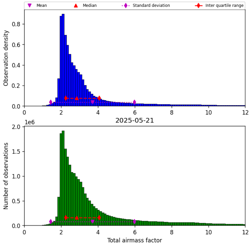
Figure 30: Histogram of “Total airmass factor” for 2025-05-21 to 2025-05-22
