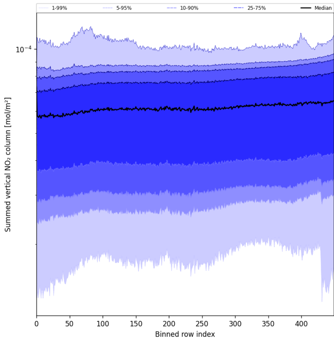
Figure 55: Along track statistics of “Summed vertical NO 2 column” for 2025-05-21 to 2025-05-22
