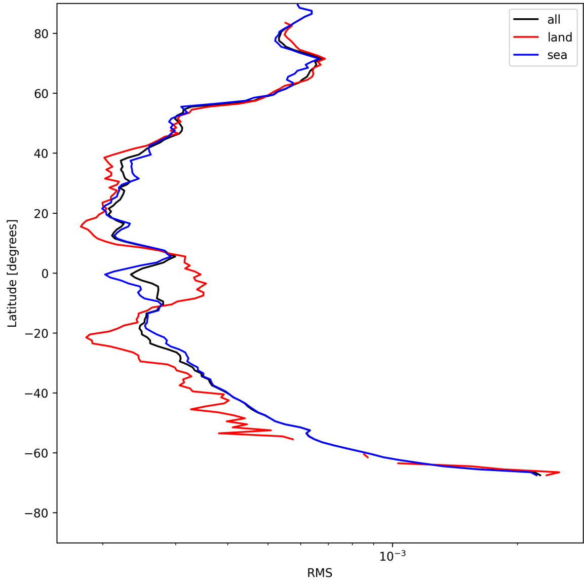
Figure 24: Zonal average of “RMS” for 2025-05-21 to 2025-05-22.
