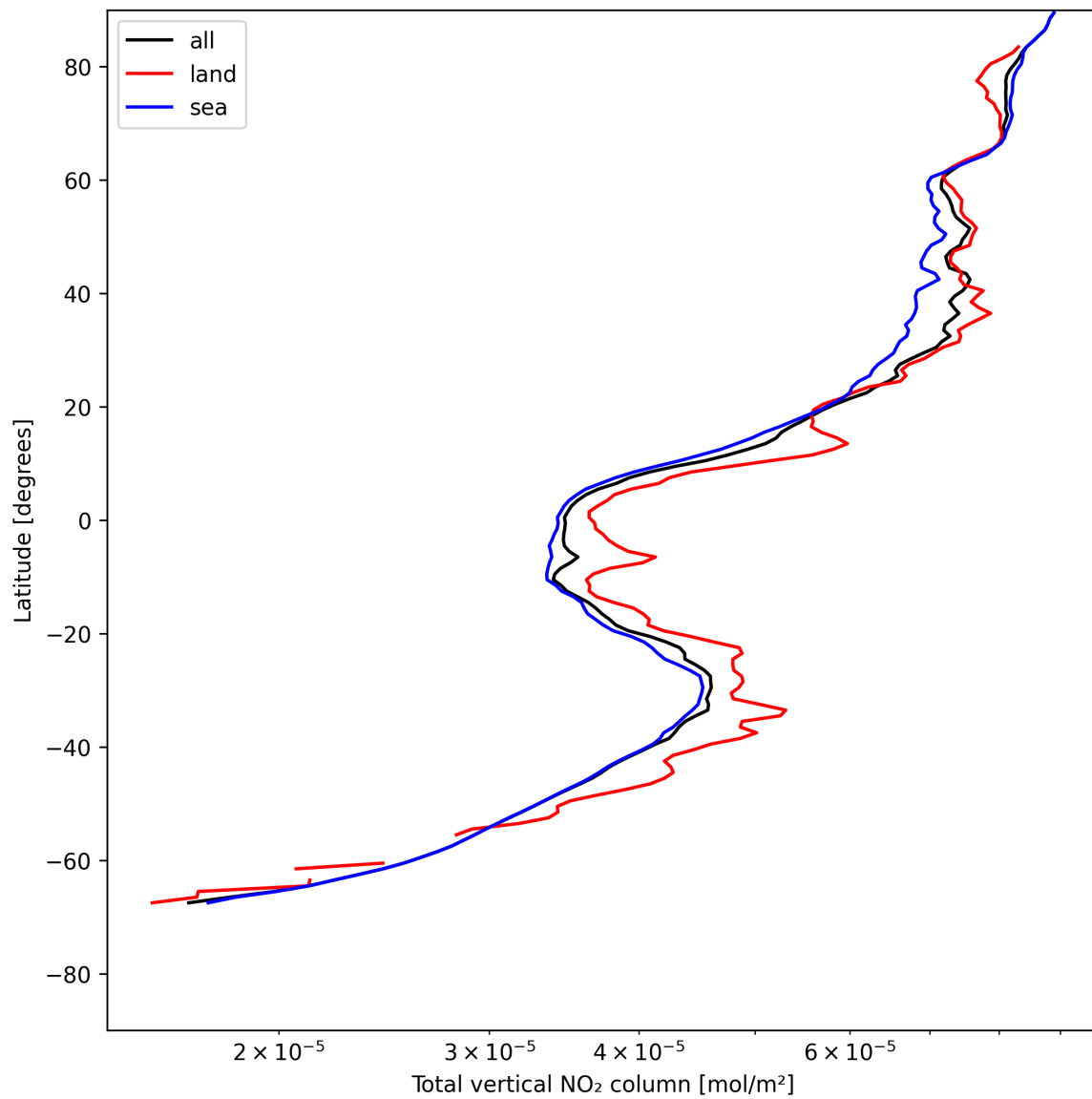
Figure 19: Zonal average of “Total vertical NO 2 column” for 2025-05-21 to 2025-05-22.
