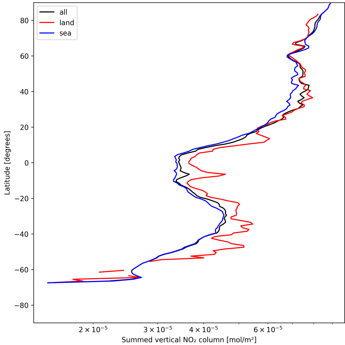
Figure 21: Zonal average of “Summed vertical NO 2 column” for 2025-05-21 to 2025-05-22.
