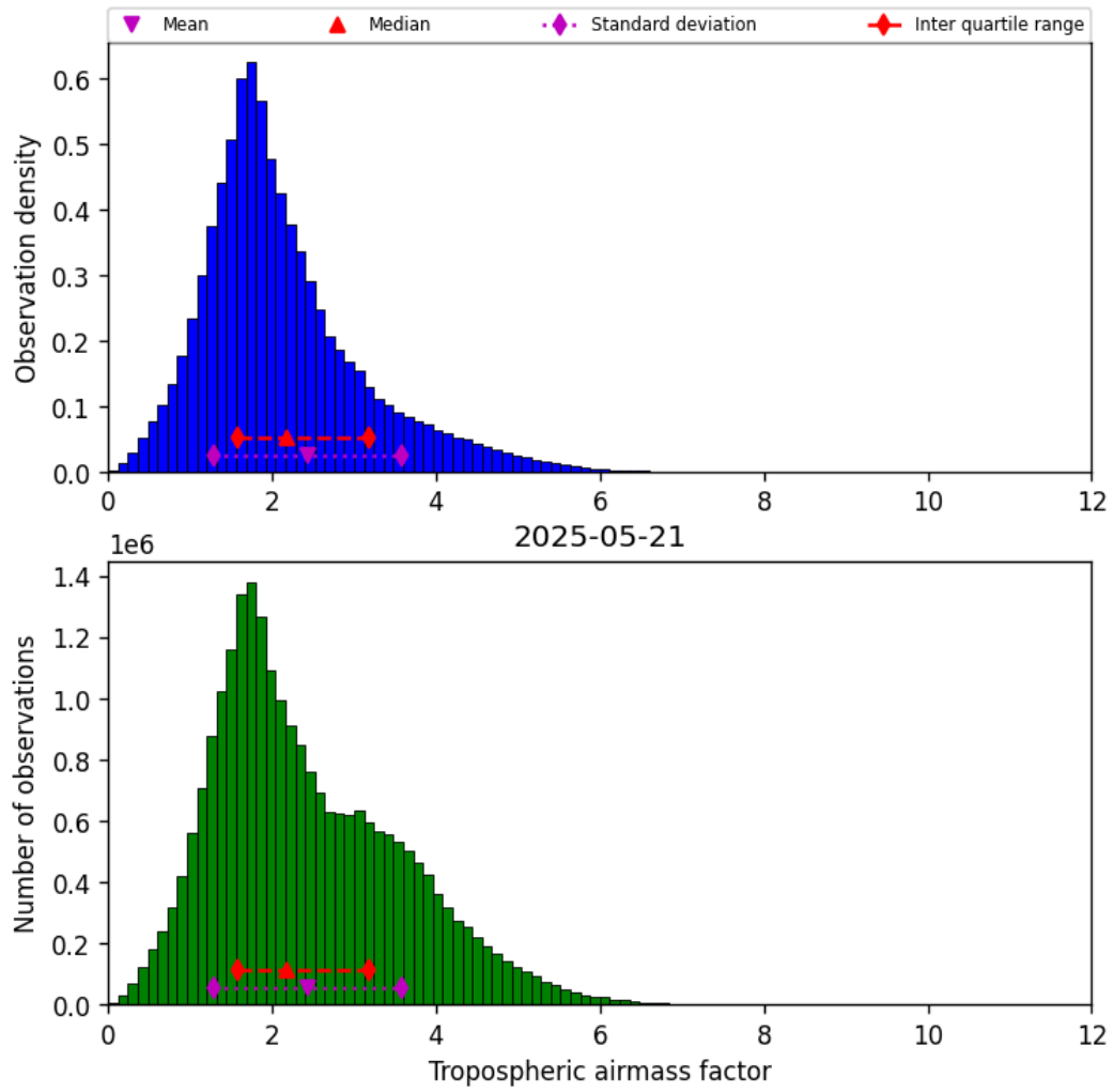
Figure 29: Histogram of “Tropospheric airmass factor” for 2025-05-21 to 2025-05-22
