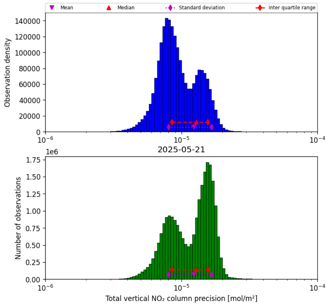
Figure 37: Histogram of “Total vertical NO 2 column precision” for 2025-05-21 to 2025-05-22
