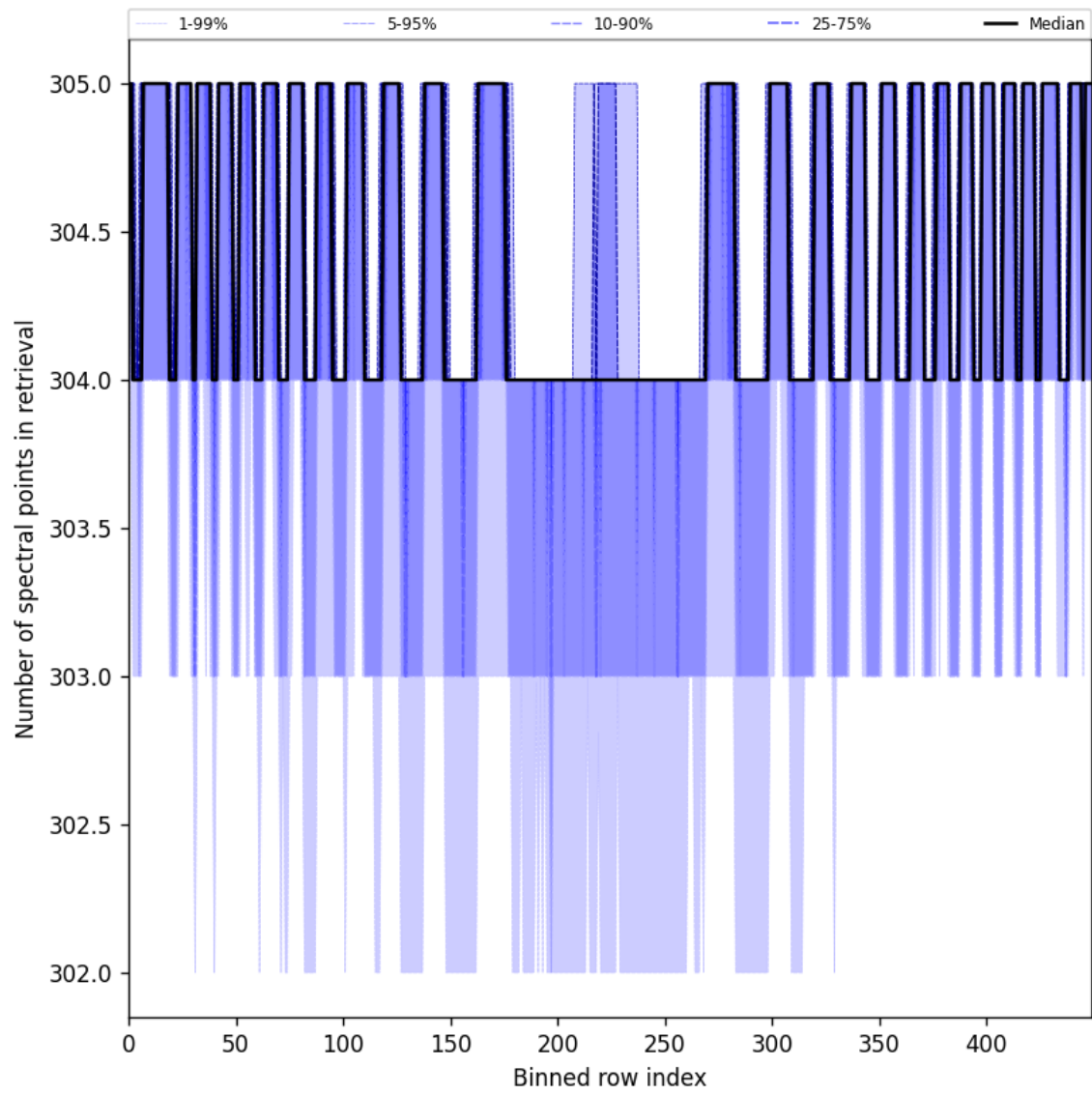
Figure 48: Along track statistics of “Number of spectral points in retrieval” for 2025-05-21 to 2025-05-22
