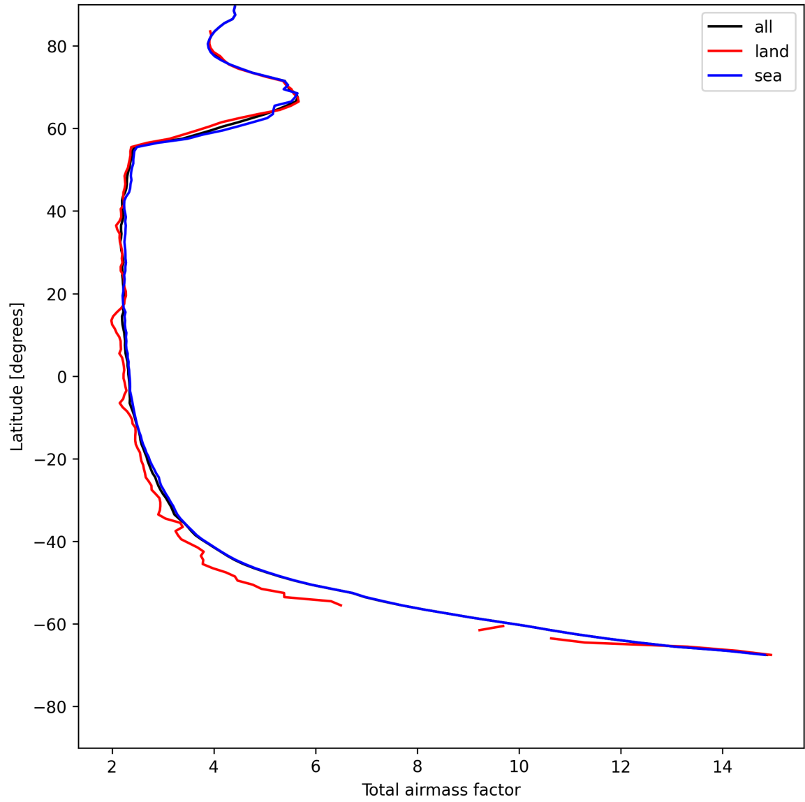
Figure 13: Zonal average of “Total airmass factor” for 2025-05-21 to 2025-05-22.
