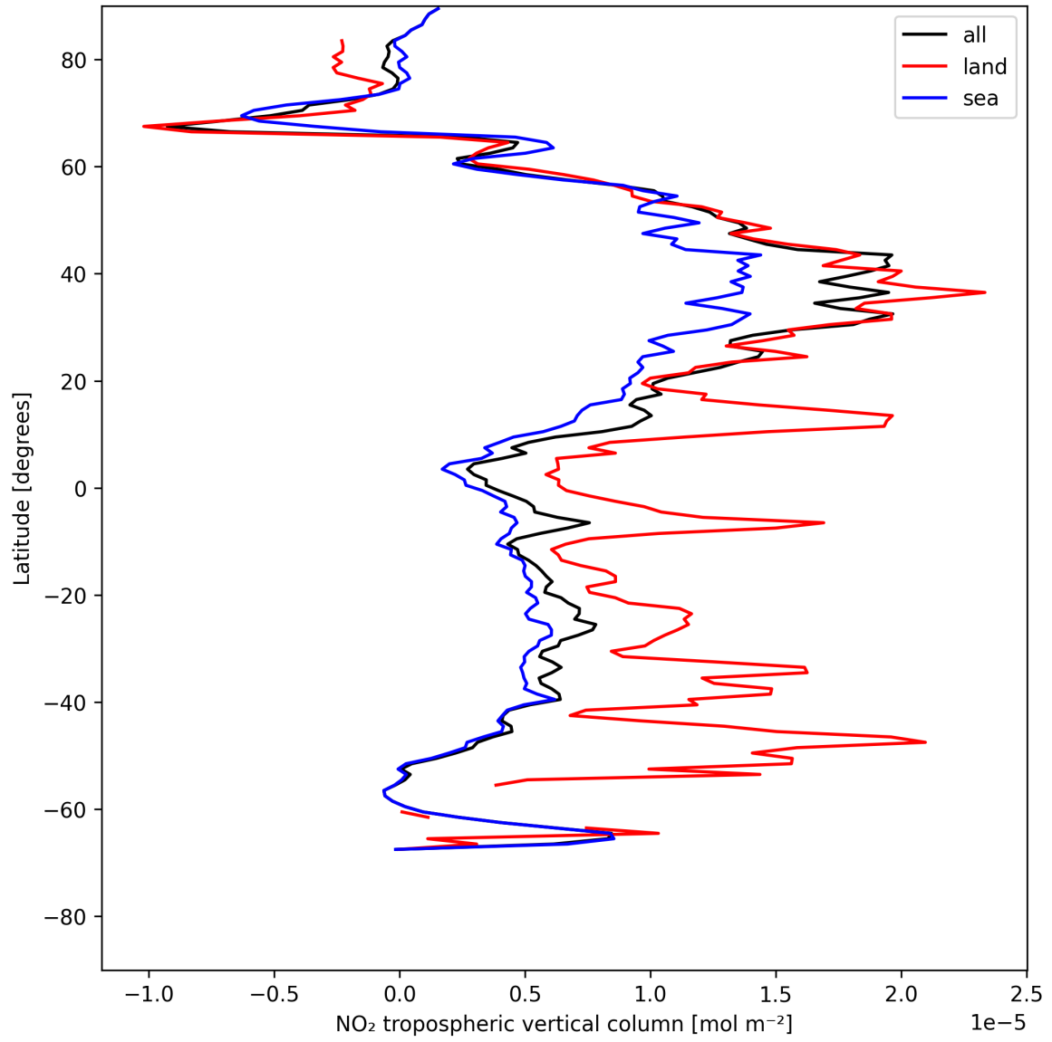
Figure 10: Zonal average of “NO 2 tropospheric vertical column” for 2025-05-21 to 2025-05-22.
