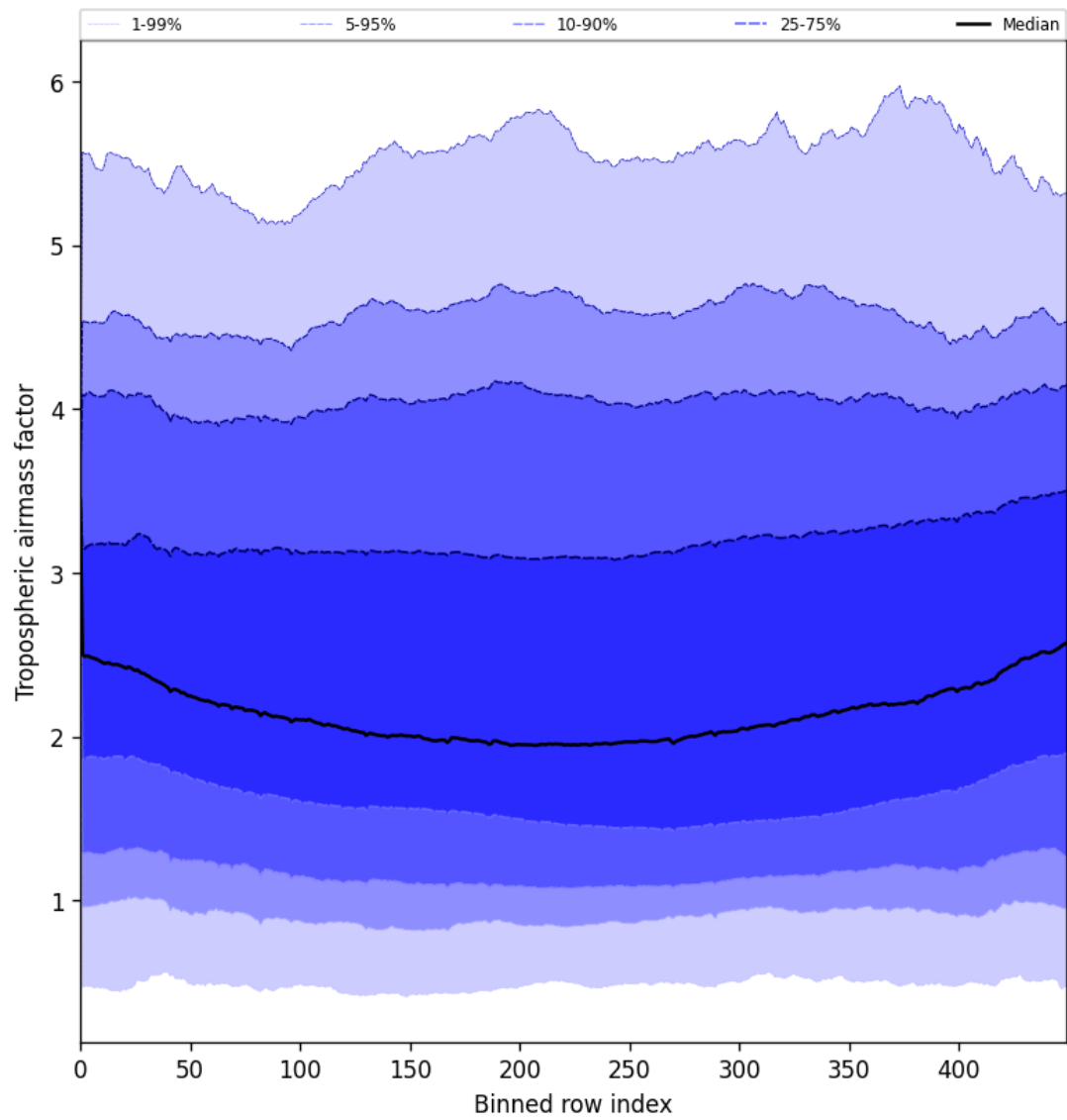
Figure 46: Along track statistics of “Tropospheric airmass factor” for 2025-05-21 to 2025-05-22
