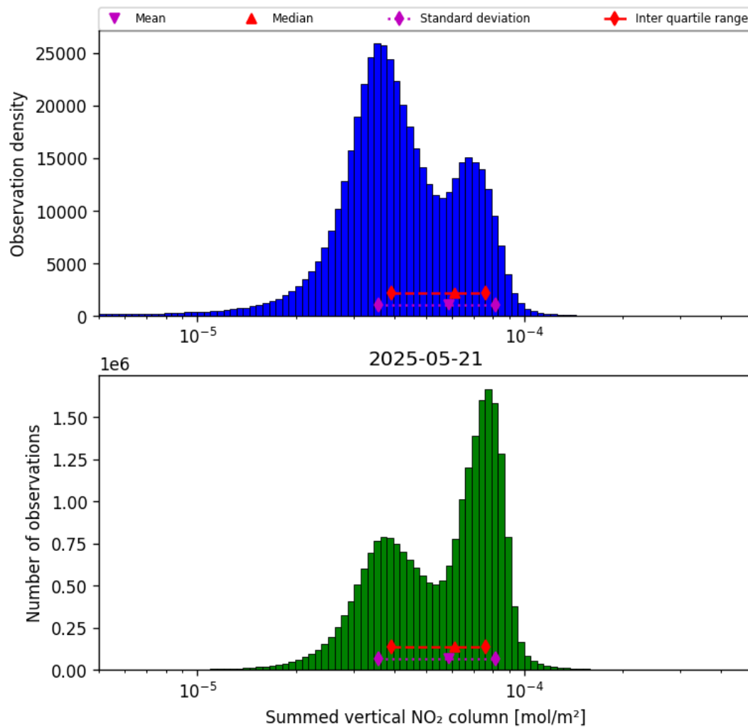
Figure 38: Histogram of “Summed vertical NO 2 column” for 2025-05-21 to 2025-05-22
