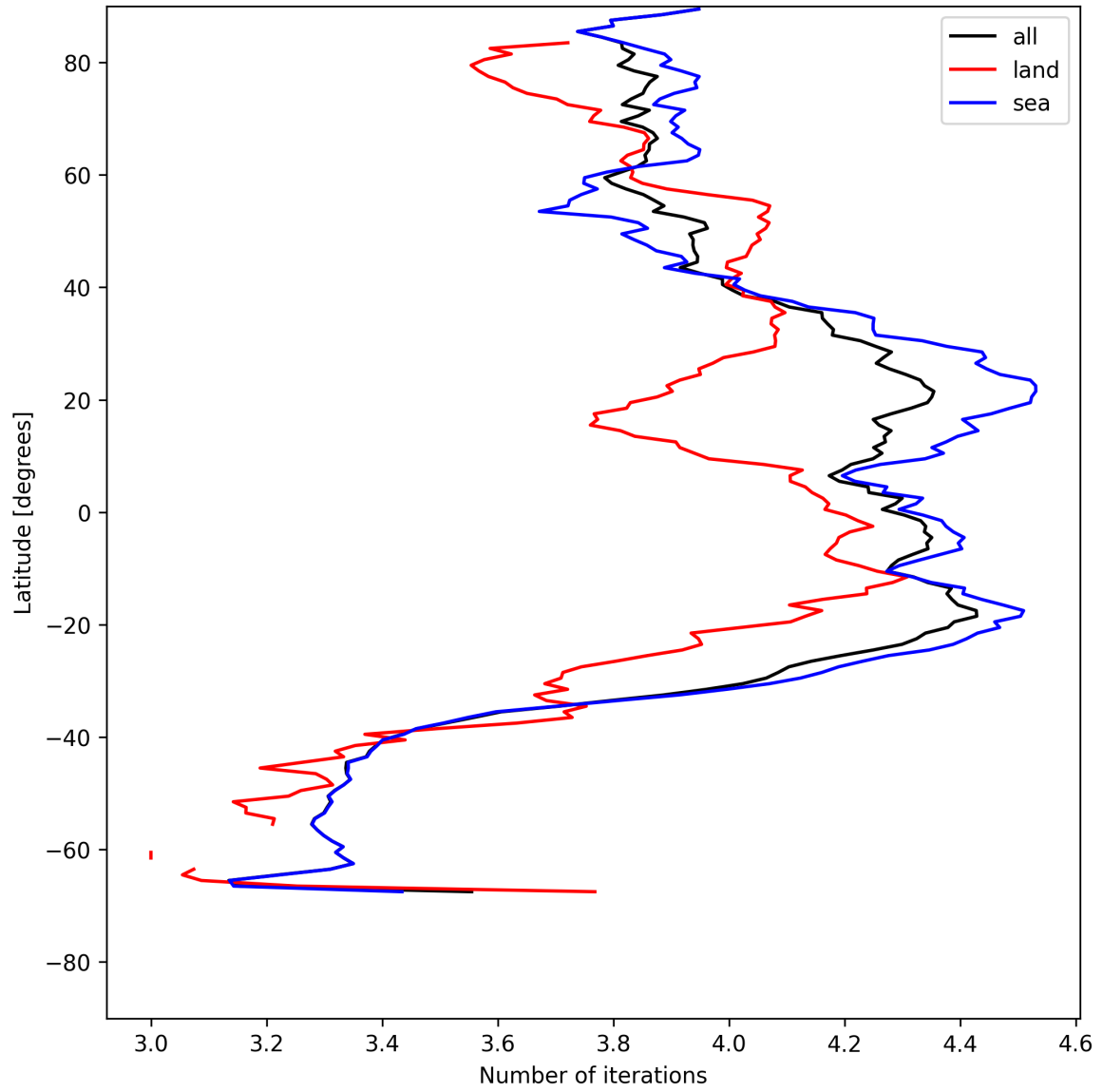
Figure 15: Zonal average of “Number of iterations” for 2025-05-21 to 2025-05-22.
