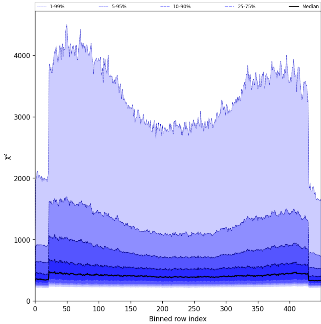
Figure 57: Along track statistics of “ \chi^2 ” for 2025-05-21 to 2025-05-22
