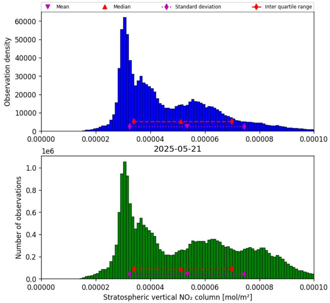
Figure 34: Histogram of “Stratospheric vertical NO 2 column” for 2025-05-21 to 2025-05-22
