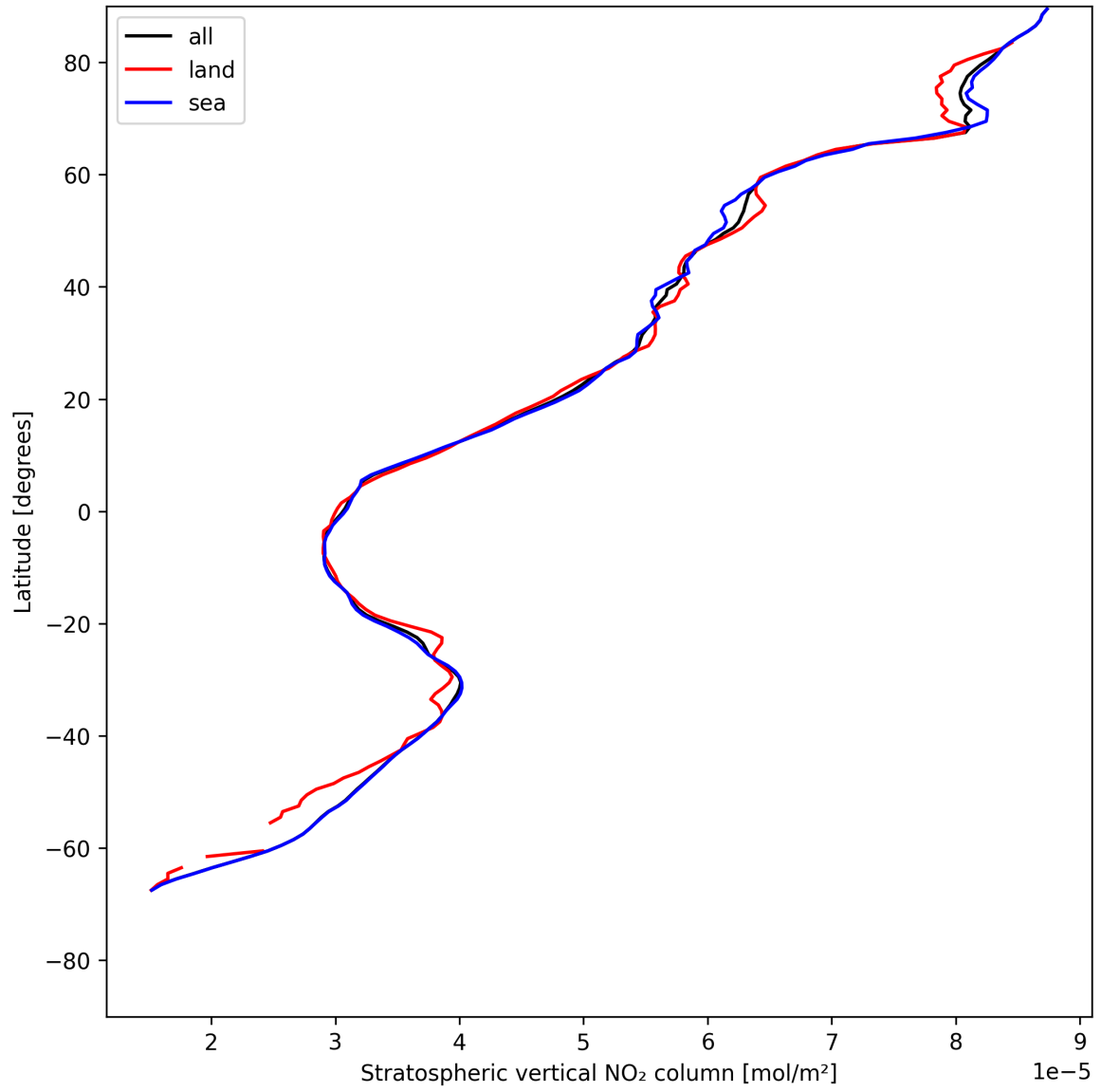
Figure 17: Zonal average of “Stratospheric vertical NO 2 column” for 2025-05-21 to 2025-05-22.
