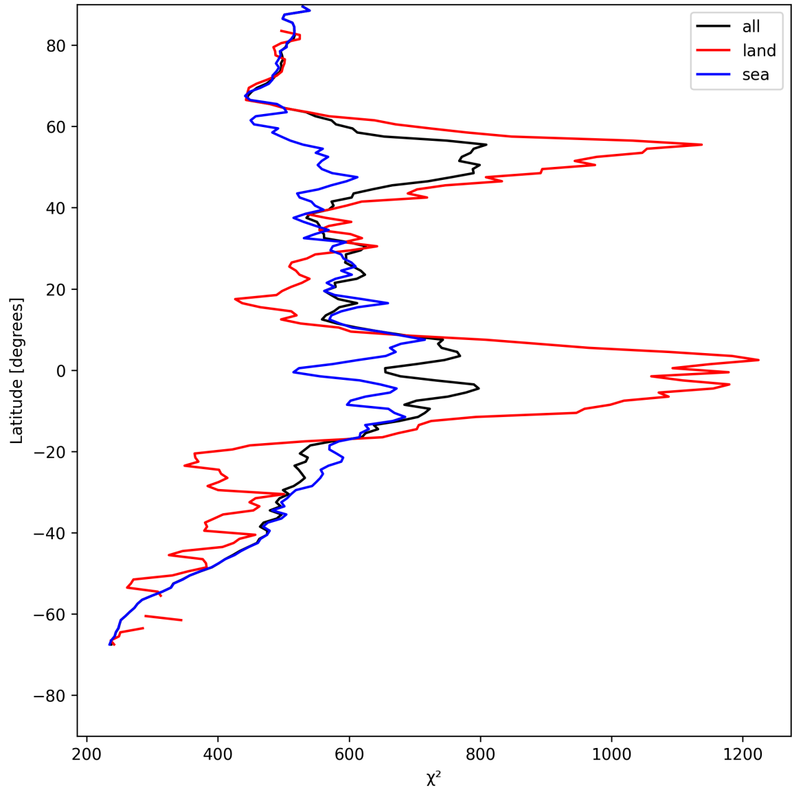
Figure 23: Zonal average of “ \chi^2 ” for 2025-05-21 to 2025-05-22.
