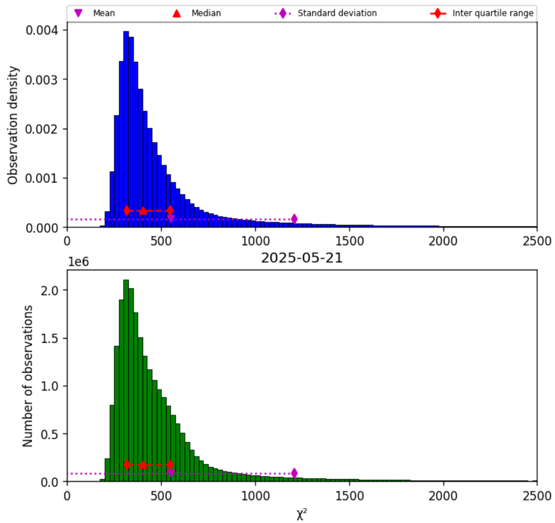
Figure 40: Histogram of “ \chi^2 ” for 2025-05-21 to 2025-05-22
