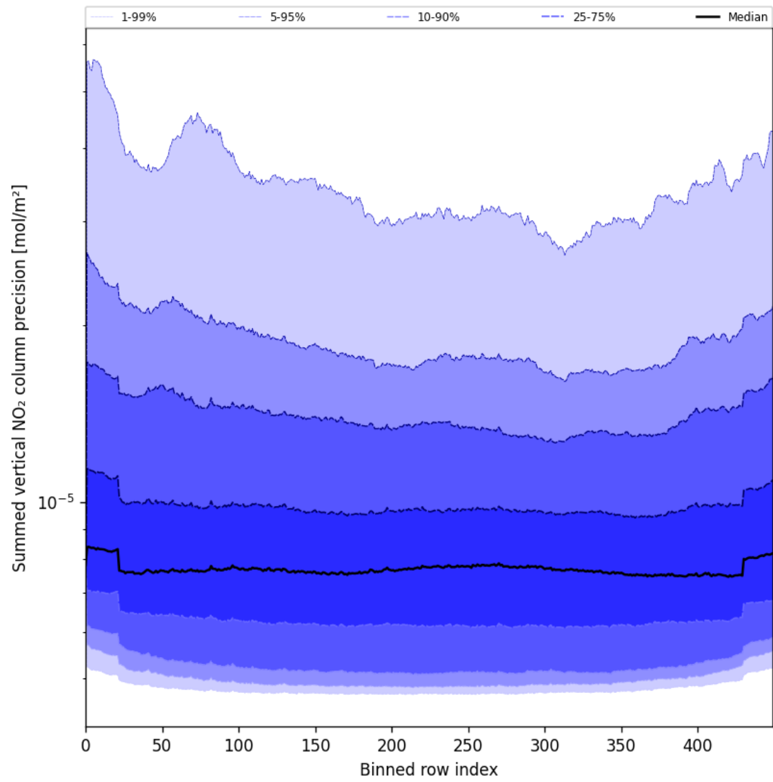
Figure 56: Along track statistics of “Summed vertical NO 2 column precision” for 2025-05-21 to 2025-05-22
