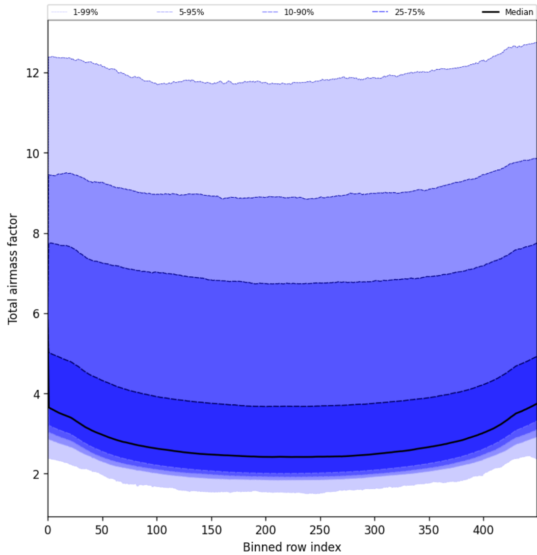
Figure 47: Along track statistics of “Total airmass factor” for 2025-05-21 to 2025-05-22
