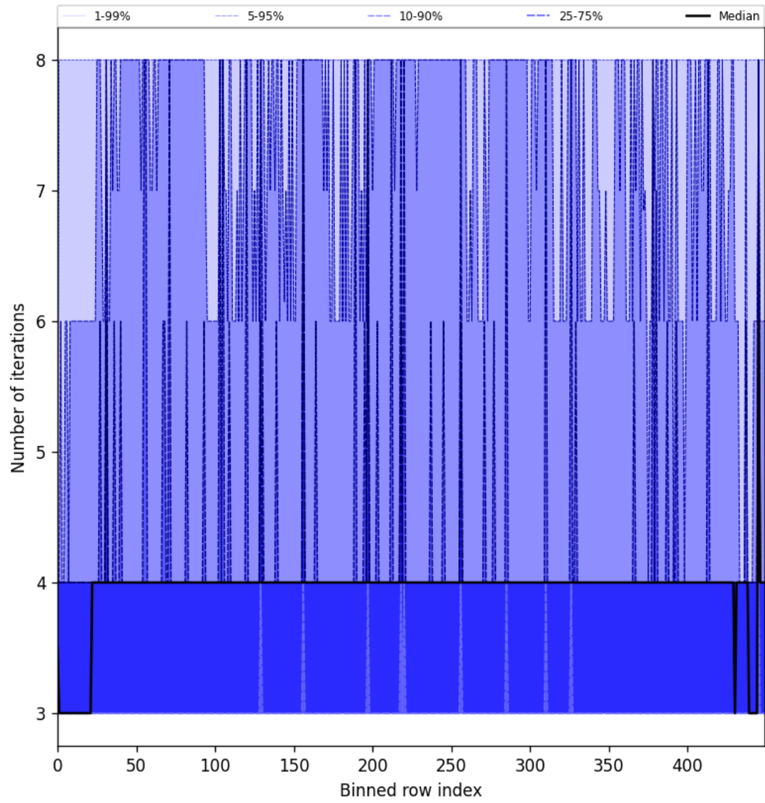
Figure 49: Along track statistics of “Number of iterations” for 2025-05-21 to 2025-05-22
