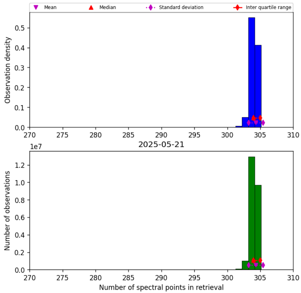
Figure 31: Histogram of “Number of spectral points in retrieval” for 2025-05-21 to 2025-05-22
