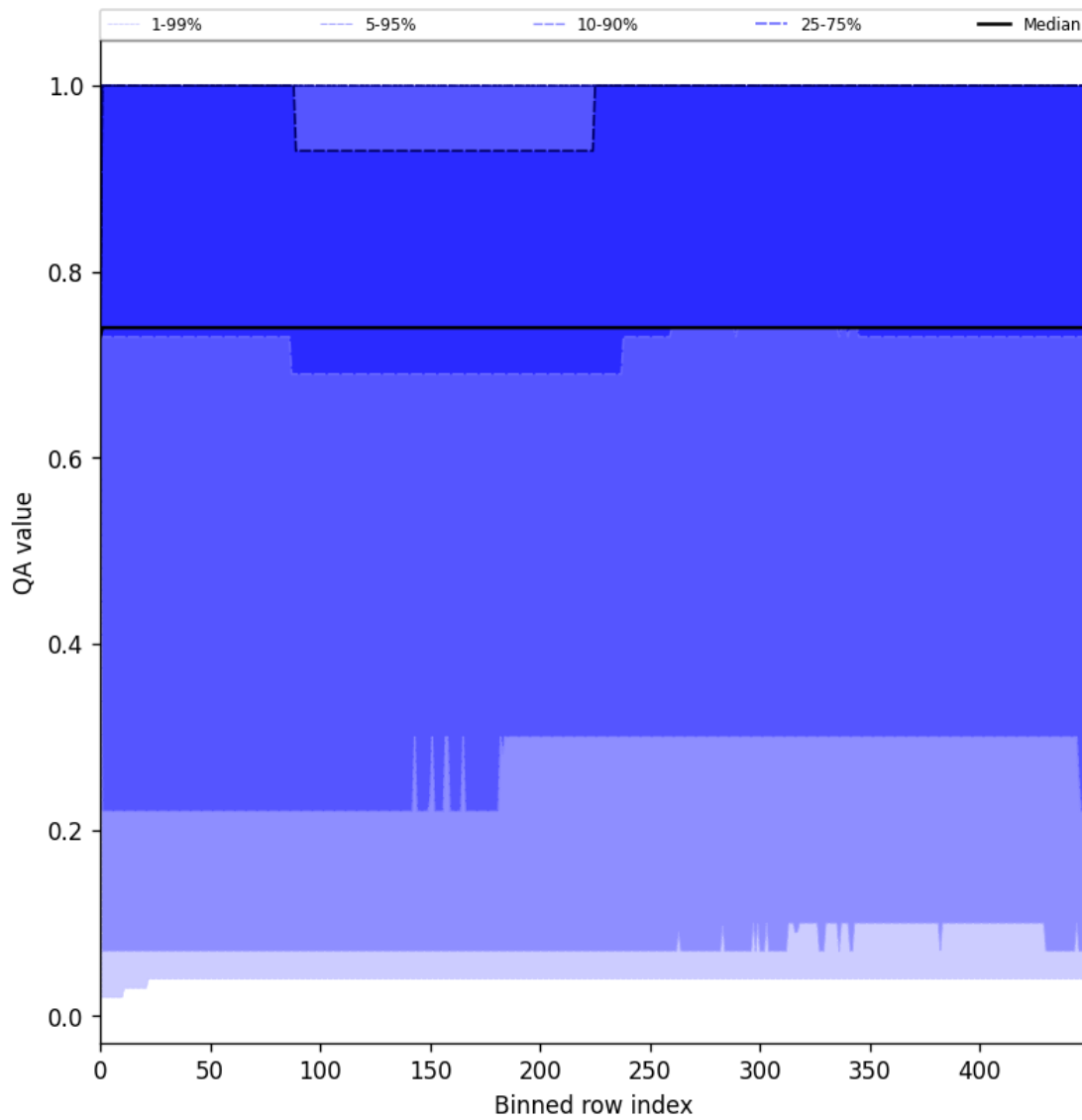
Figure 43: Along track statistics of “QA value” for 2025-05-21 to 2025-05-22
