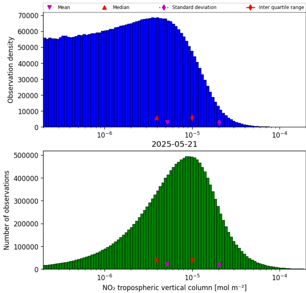
Figure 27: Histogram of “NO 2 tropospheric vertical column” for 2025-05-21 to 2025-05-22
