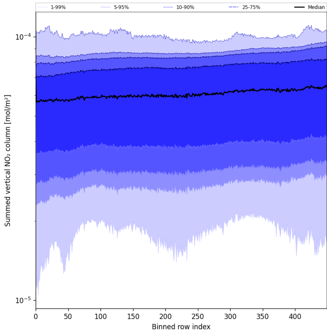
Figure 55: Along track statistics of “Summed vertical NO 2 column” for 2025-05-22 to 2025-05-23
