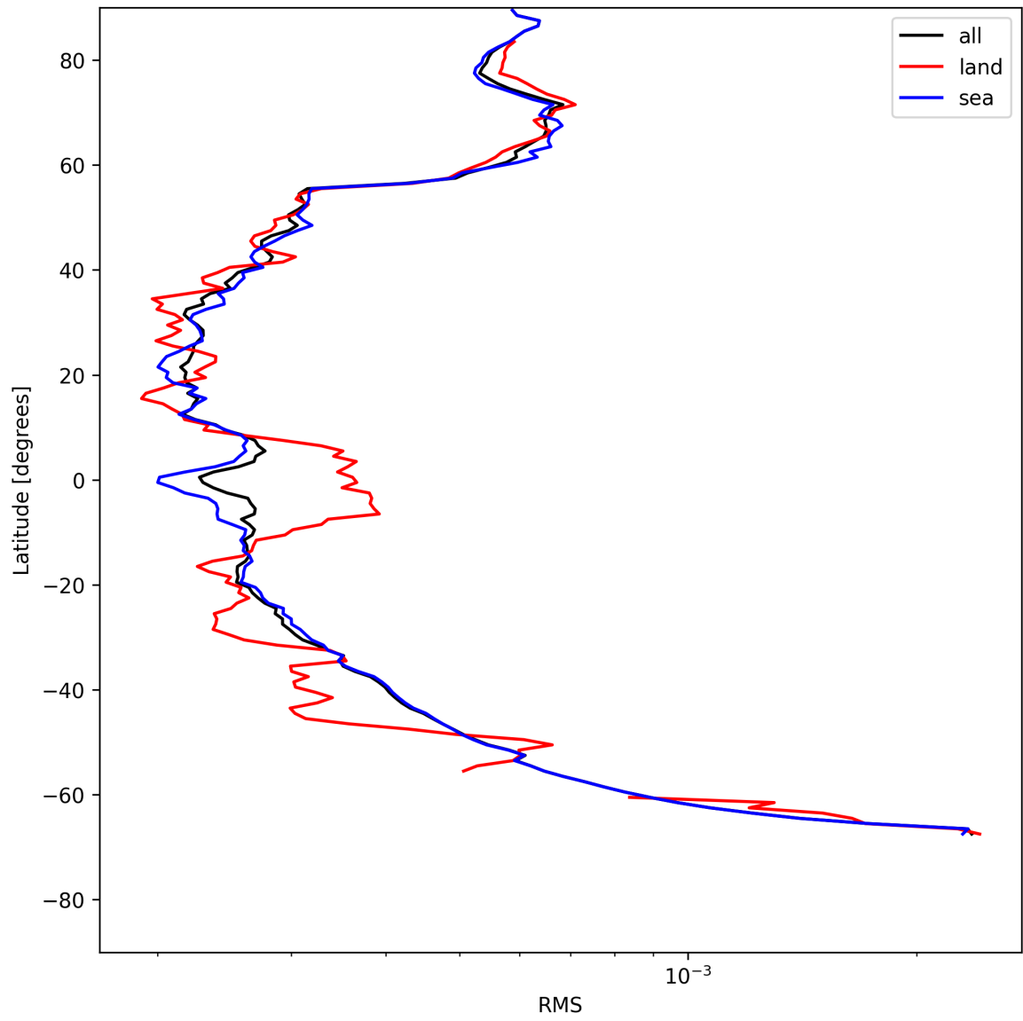
Figure 24: Zonal average of “RMS” for 2025-05-22 to 2025-05-23.
