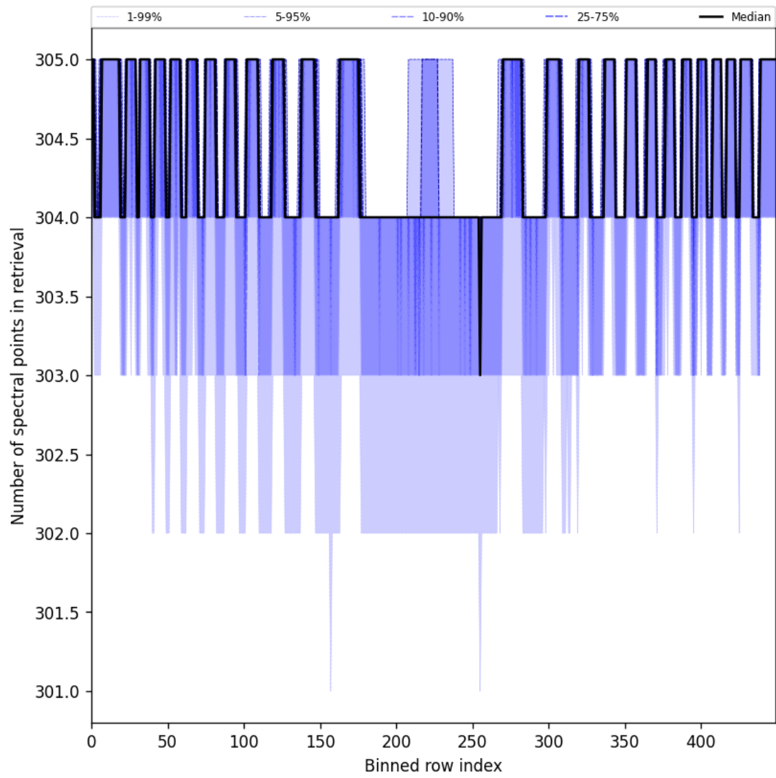
Figure 48: Along track statistics of “Number of spectral points in retrieval” for 2025-05-22 to 2025-05-23
