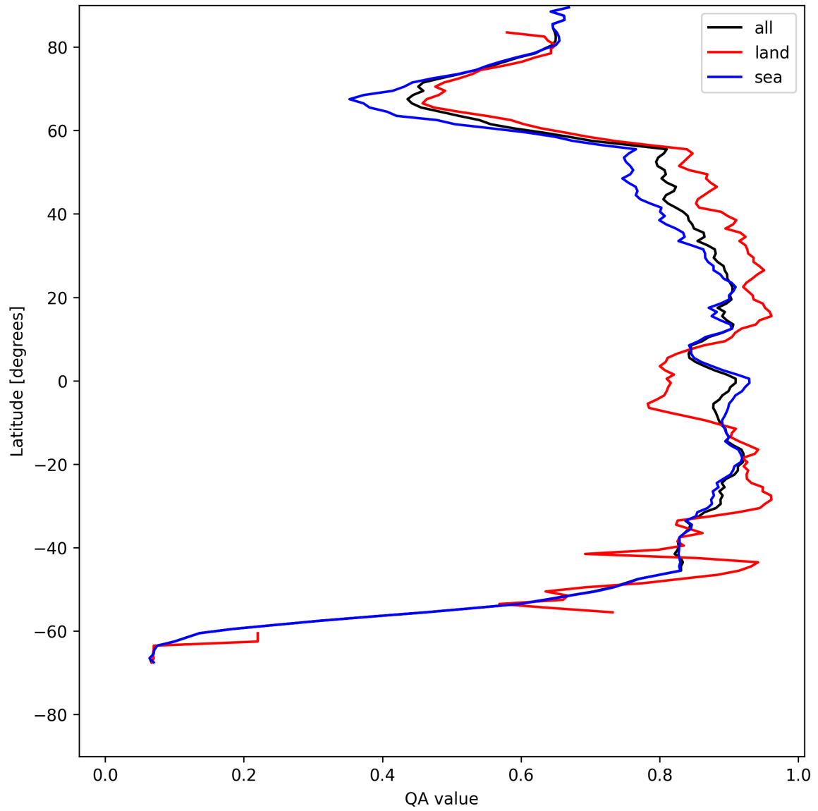
Figure 9: Zonal average of “QA value” for 2025-05-22 to 2025-05-23.
