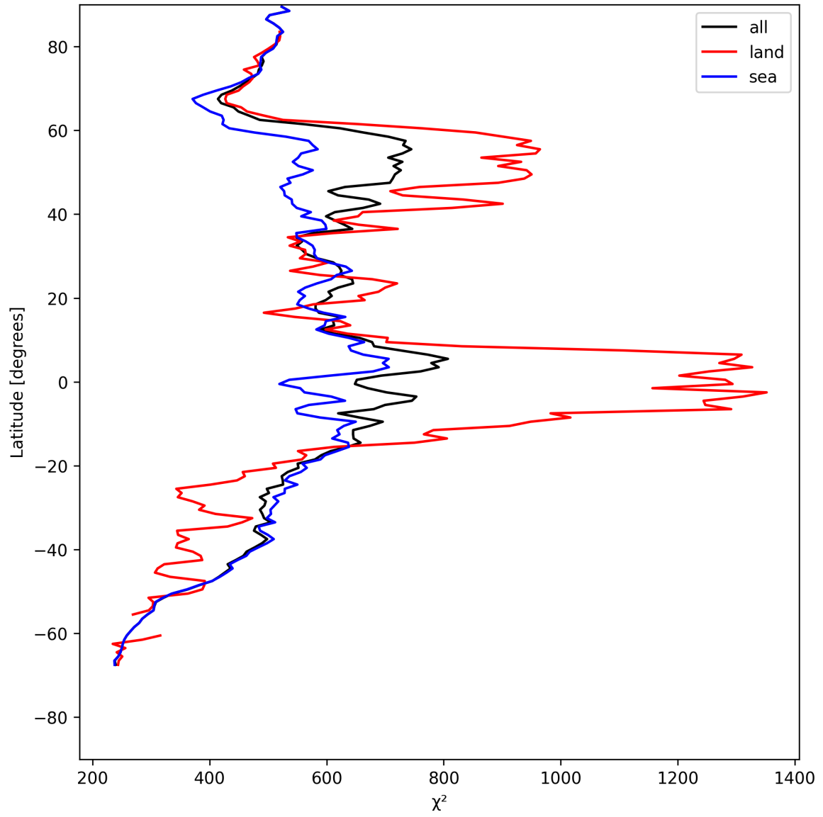
Figure 23: Zonal average of “ \chi^2 ” for 2025-05-22 to 2025-05-23.
