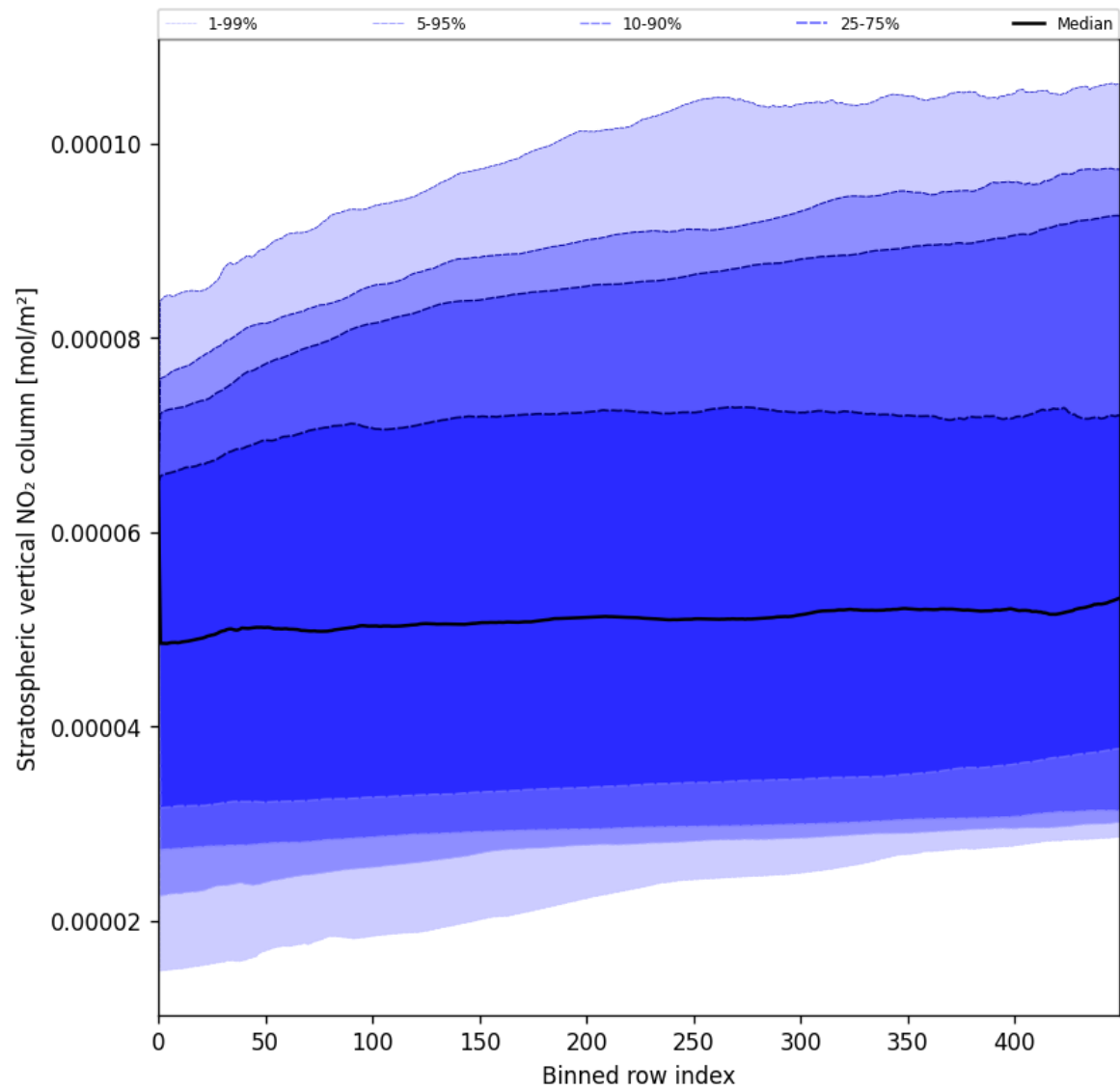
Figure 51: Along track statistics of “Stratospheric vertical NO 2 column” for 2025-05-22 to 2025-05-23
