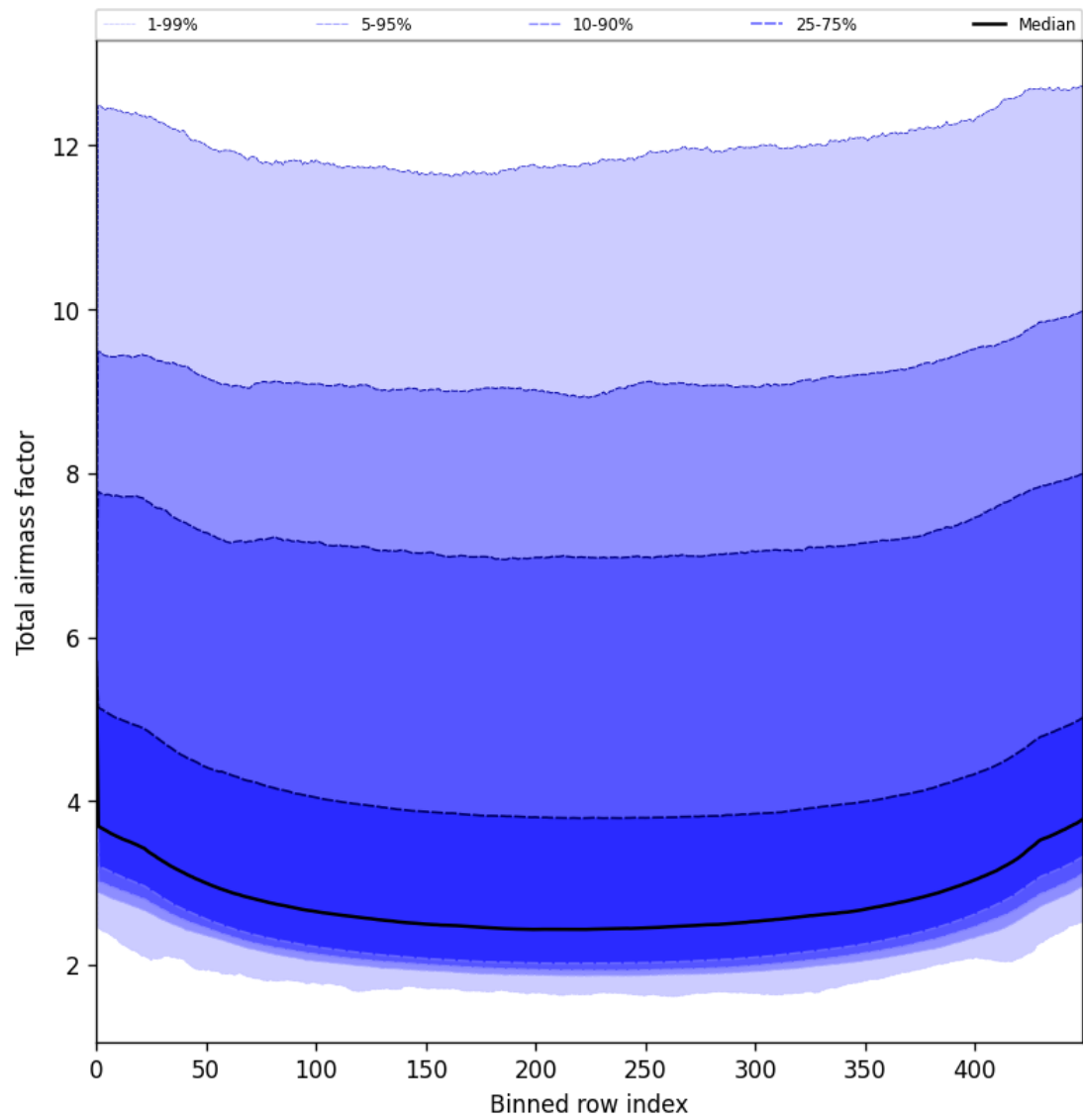
Figure 47: Along track statistics of “Total airmass factor” for 2025-05-22 to 2025-05-23
