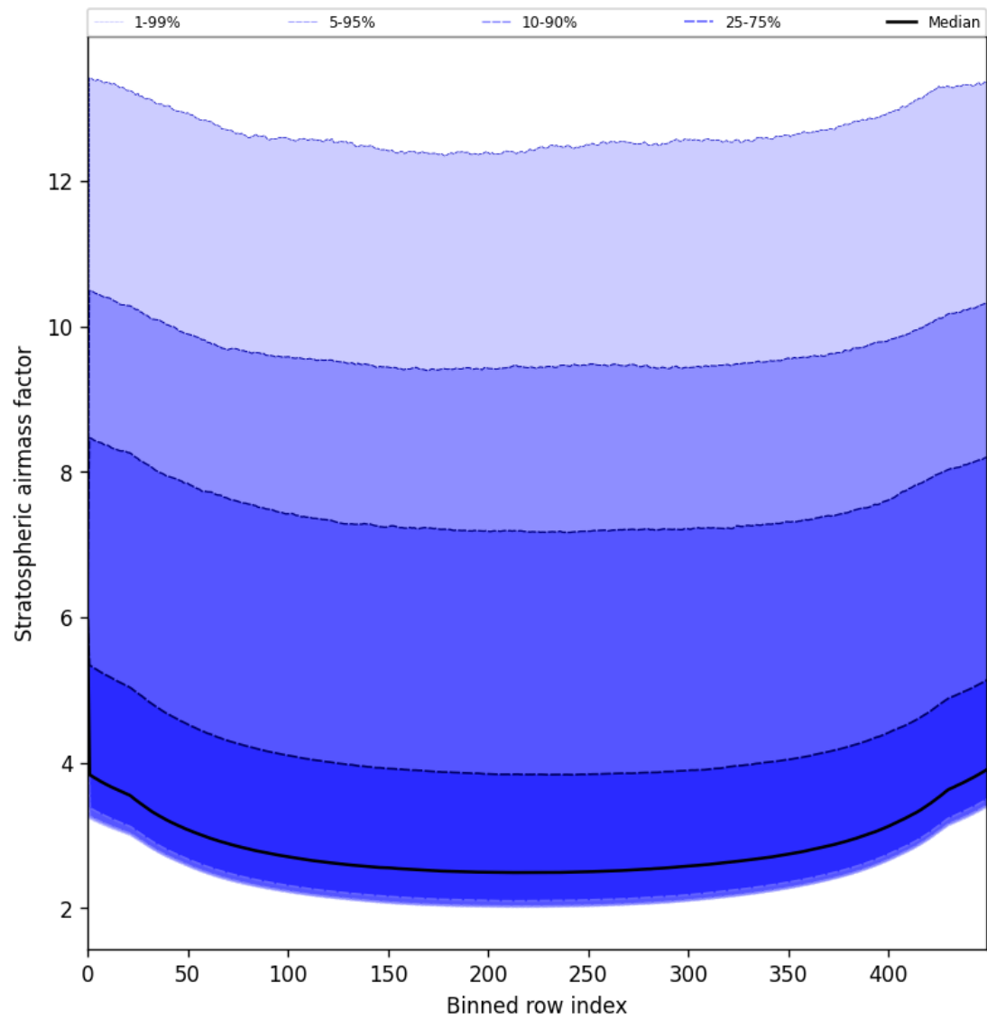
Figure 59: Along track statistics of “Stratospheric airmass factor” for 2025-05-22 to 2025-05-23
