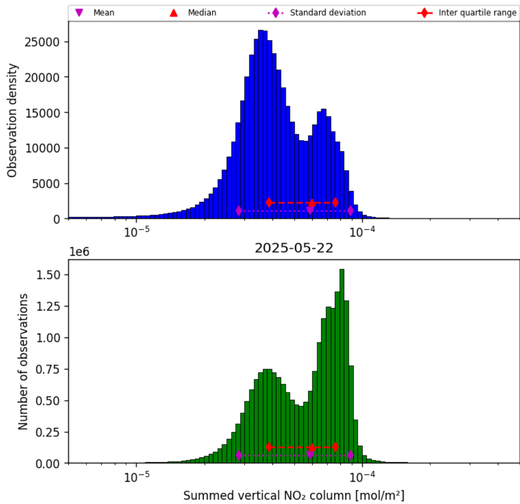
Figure 38: Histogram of "Summed vertical NO 2 column" for 2025-05-22 to 2025-05-23
