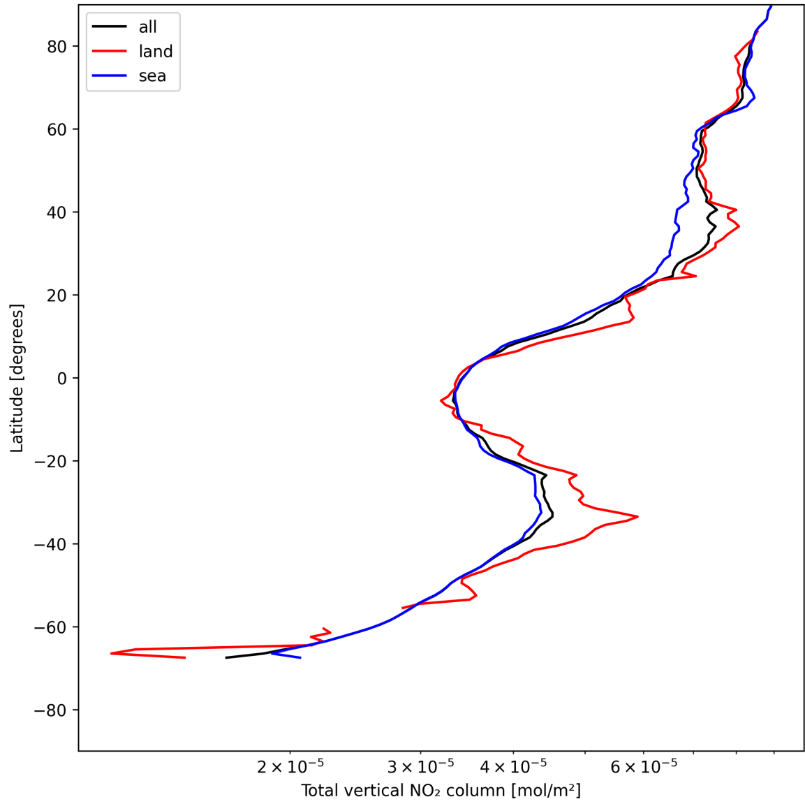
Figure 19: Zonal average of “Total vertical NO 2 column” for 2025-05-22 to 2025-05-23.
