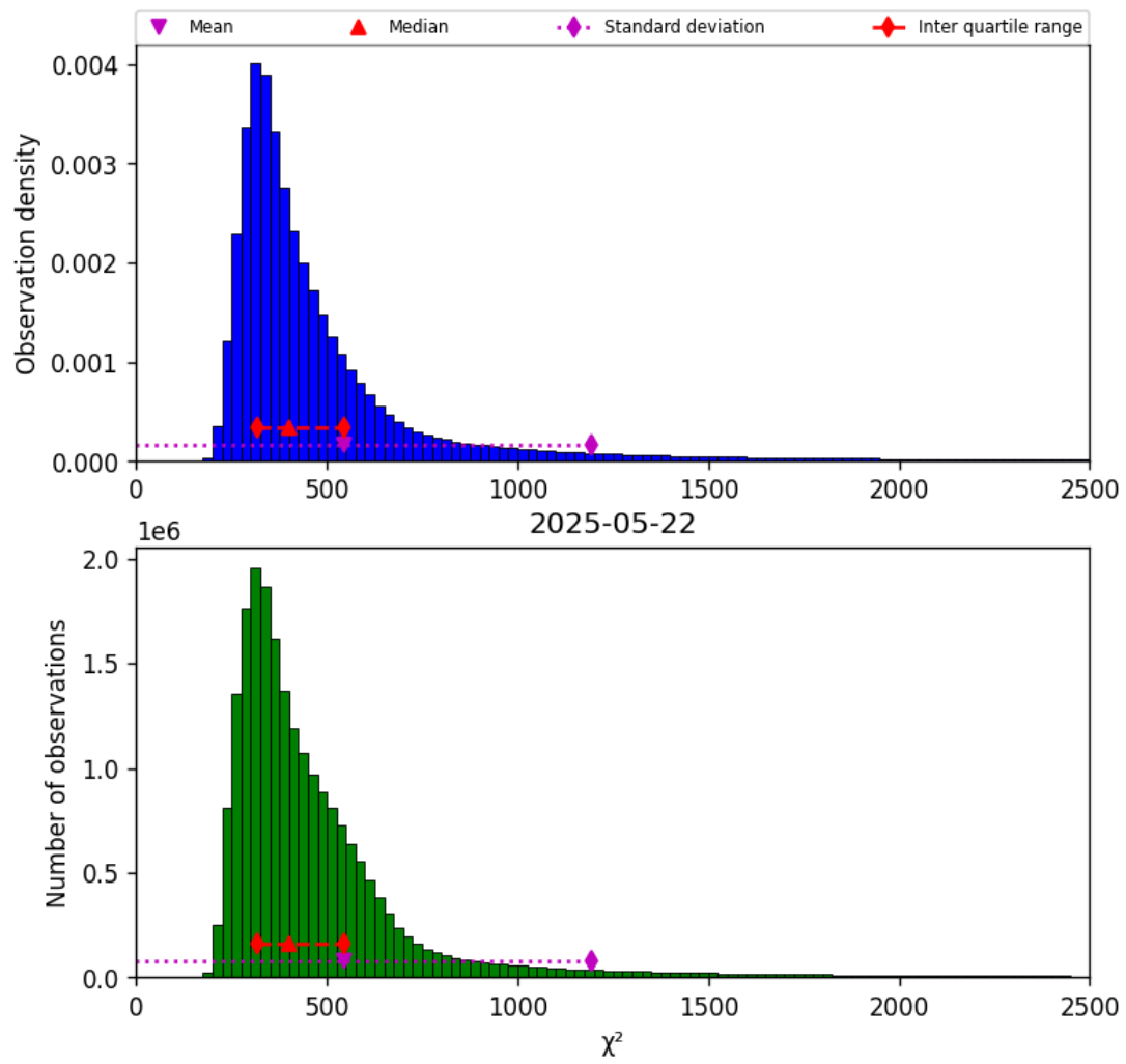
Figure 40: Histogram of " \chi^2 " for 2025-05-22 to 2025-05-23
