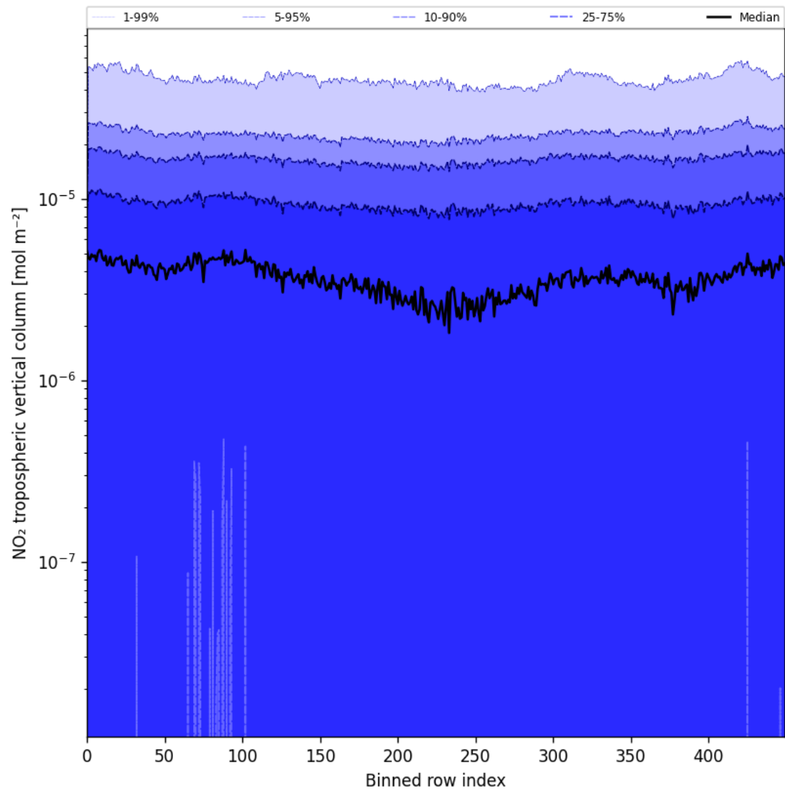
Figure 44: Along track statistics of “NO 2 tropospheric vertical column” for 2025-05-22 to 2025-05-23
