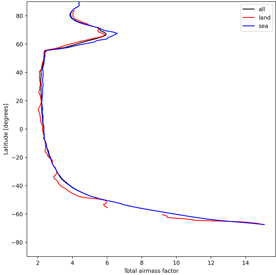
Figure 13: Zonal average of “Total airmass factor” for 2025-05-22 to 2025-05-23.
