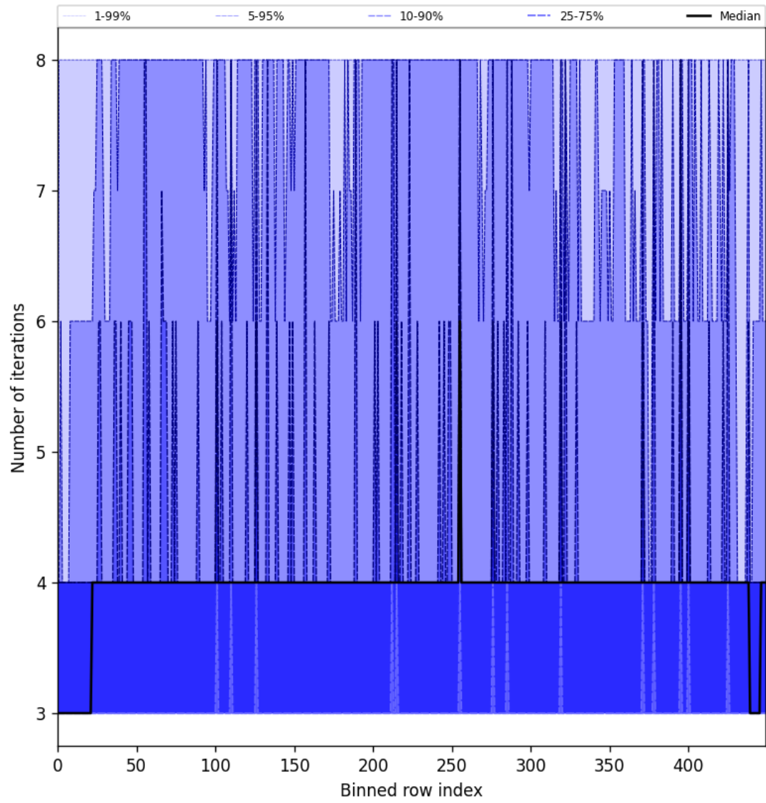
Figure 49: Along track statistics of “Number of iterations” for 2025-05-22 to 2025-05-23
