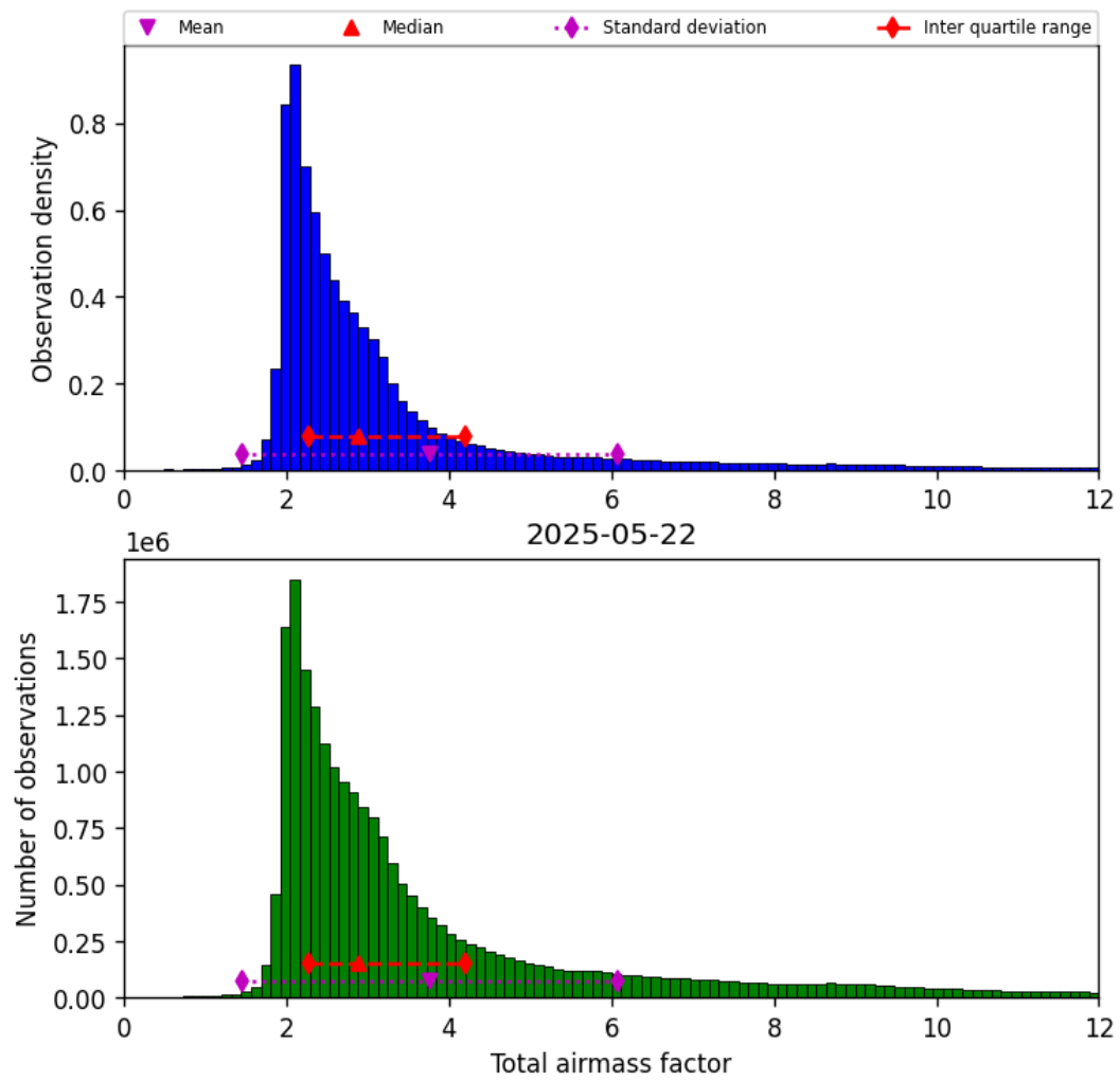
Figure 30: Histogram of “Total airmass factor” for 2025-05-22 to 2025-05-23
