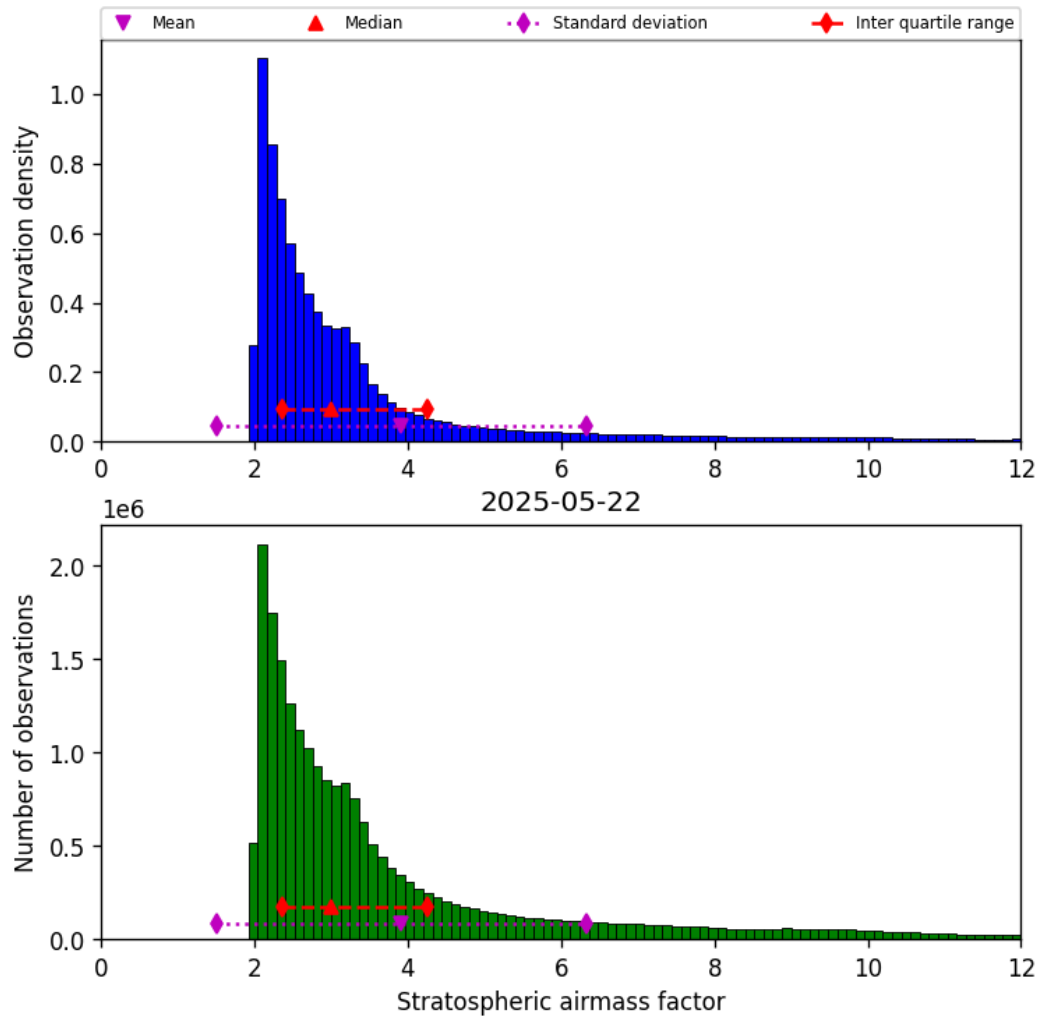
Figure 42: Histogram of “Stratospheric airmass factor” for 2025-05-22 to 2025-05-23
