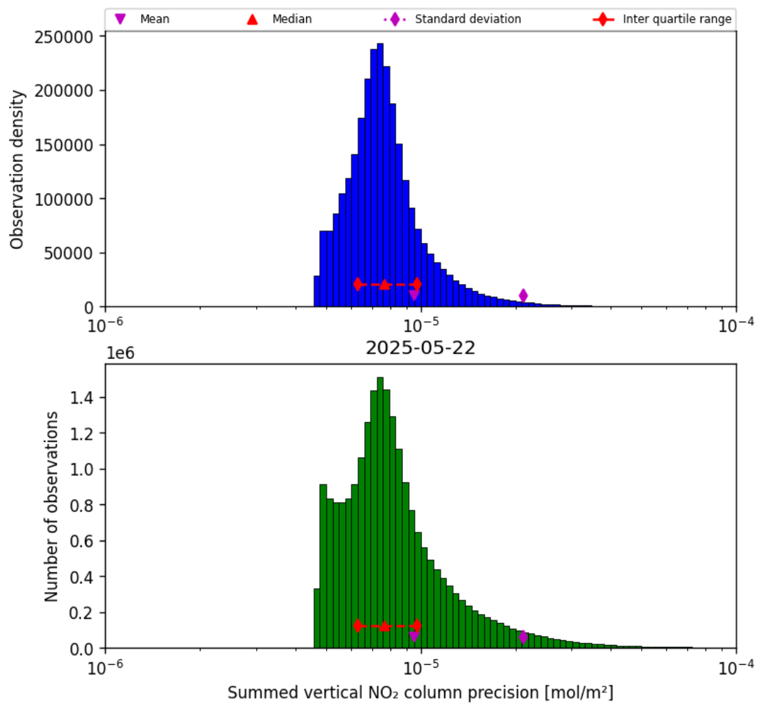
Figure 39: Histogram of “Summed vertical NO 2 column precision” for 2025-05-22 to 2025-05-23
