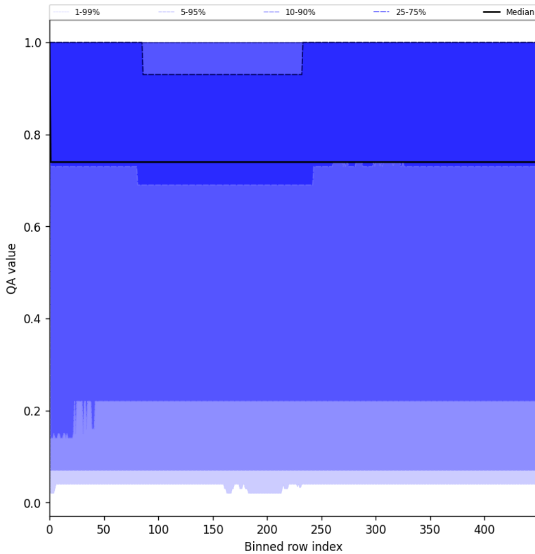
Figure 43: Along track statistics of “QA value” for 2025-05-22 to 2025-05-23
