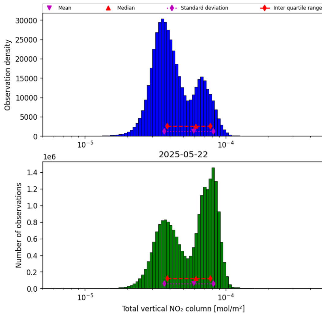
Figure 36: Histogram of “Total vertical NO 2 column” for 2025-05-22 to 2025-05-23
