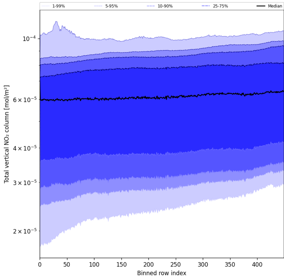
Figure 53: Along track statistics of “Total vertical NO 2 column” for 2025-05-22 to 2025-05-23
