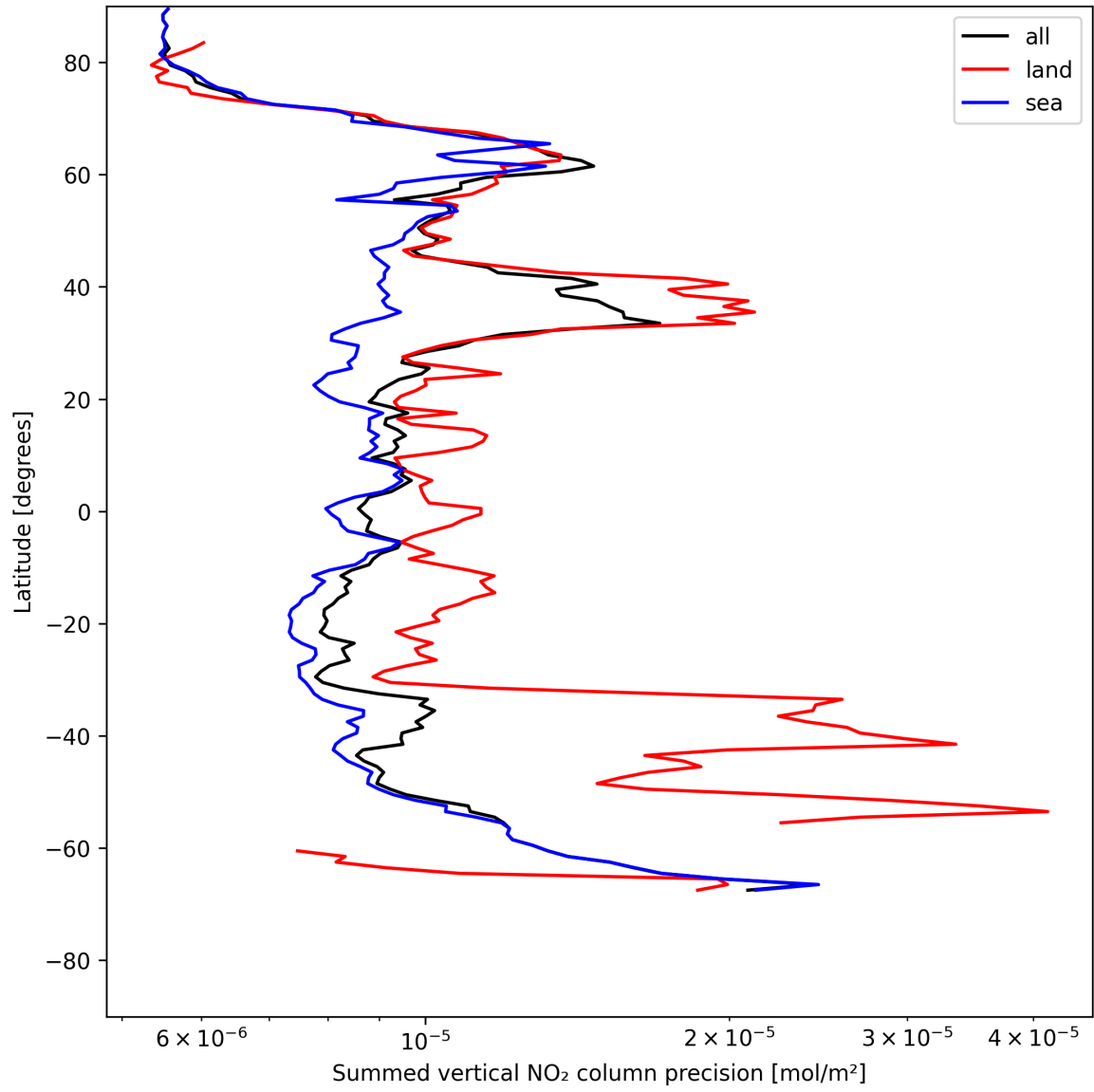
Figure 22: Zonal average of “Summed vertical NO 2 column precision” for 2025-05-22 to 2025-05-23.
