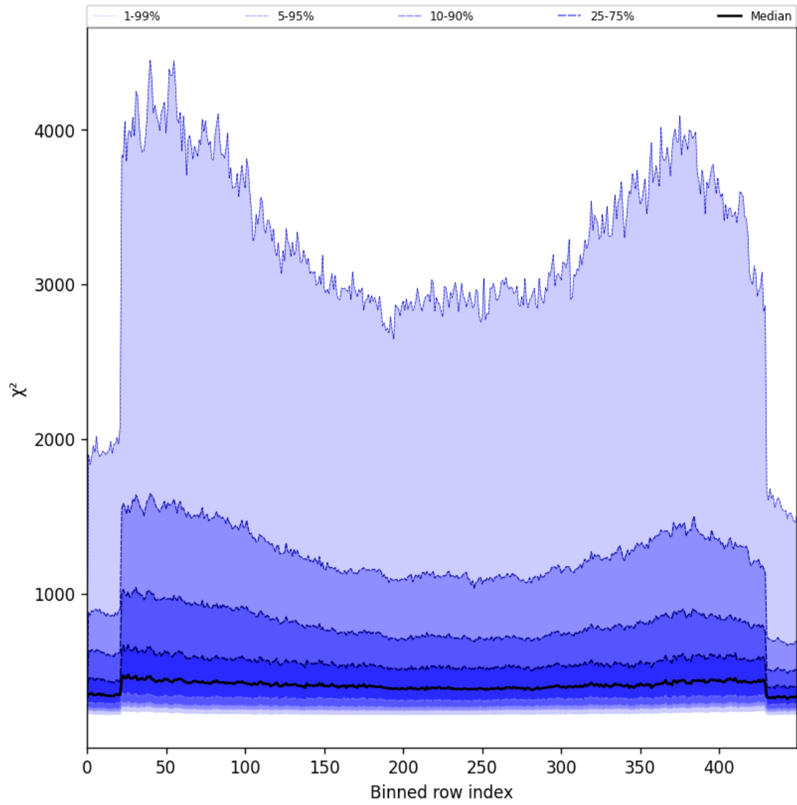
Figure 57: Along track statistics of “ \chi^2 ” for 2025-05-22 to 2025-05-23
