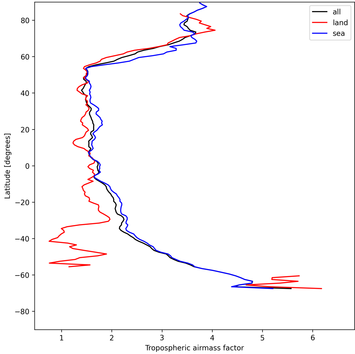
Figure 12: Zonal average of “Tropospheric airmass factor” for 2025-05-22 to 2025-05-23.
