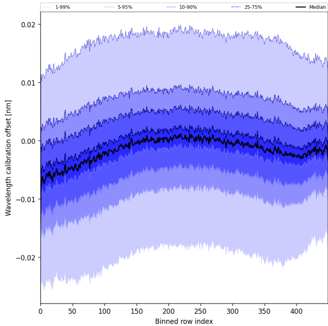
Figure 50: Along track statistics of “Wavelength calibration offset” for 2025-05-22 to 2025-05-23
