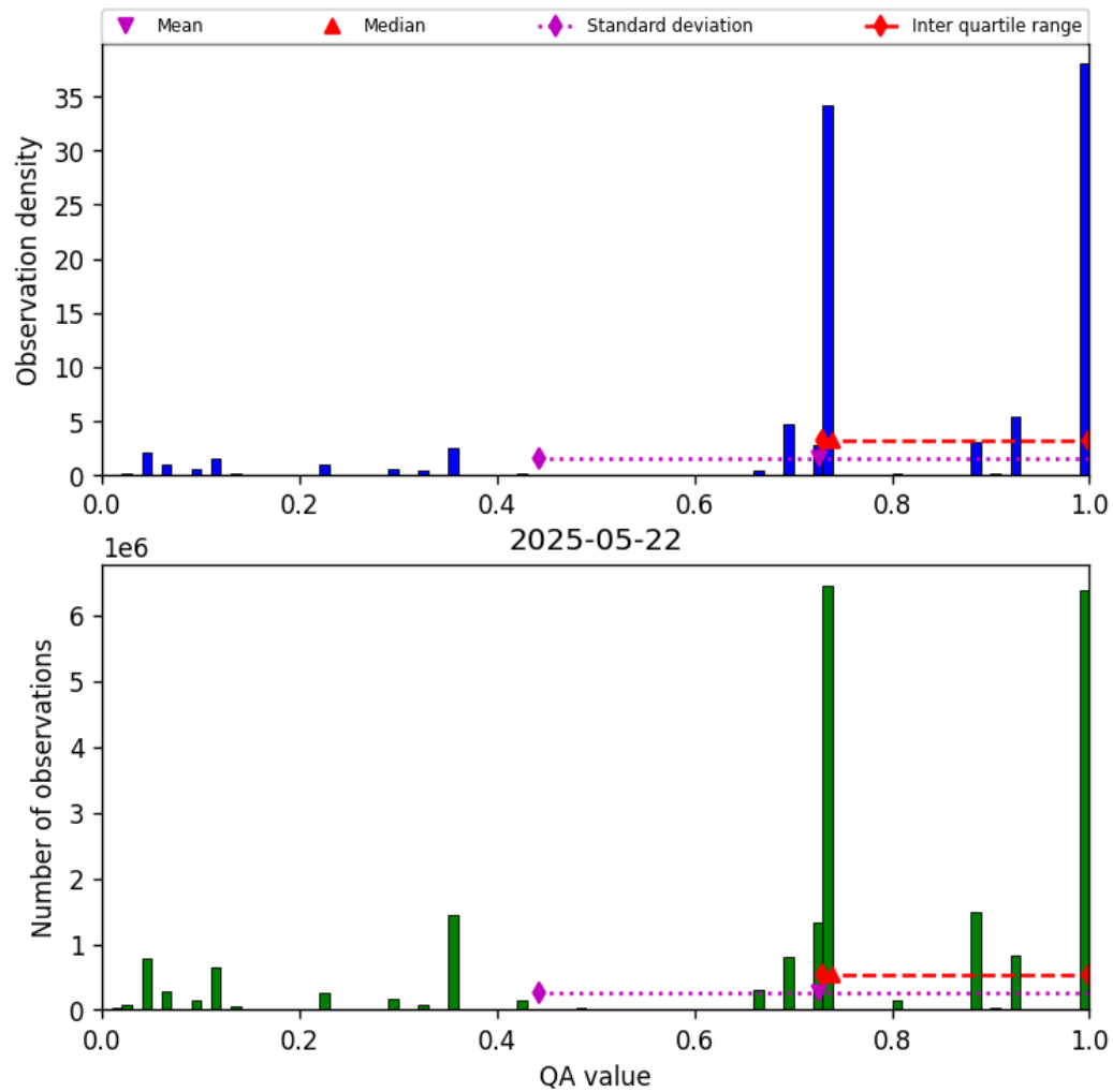
Figure 26: Histogram of “QA value” for 2025-05-22 to 2025-05-23
