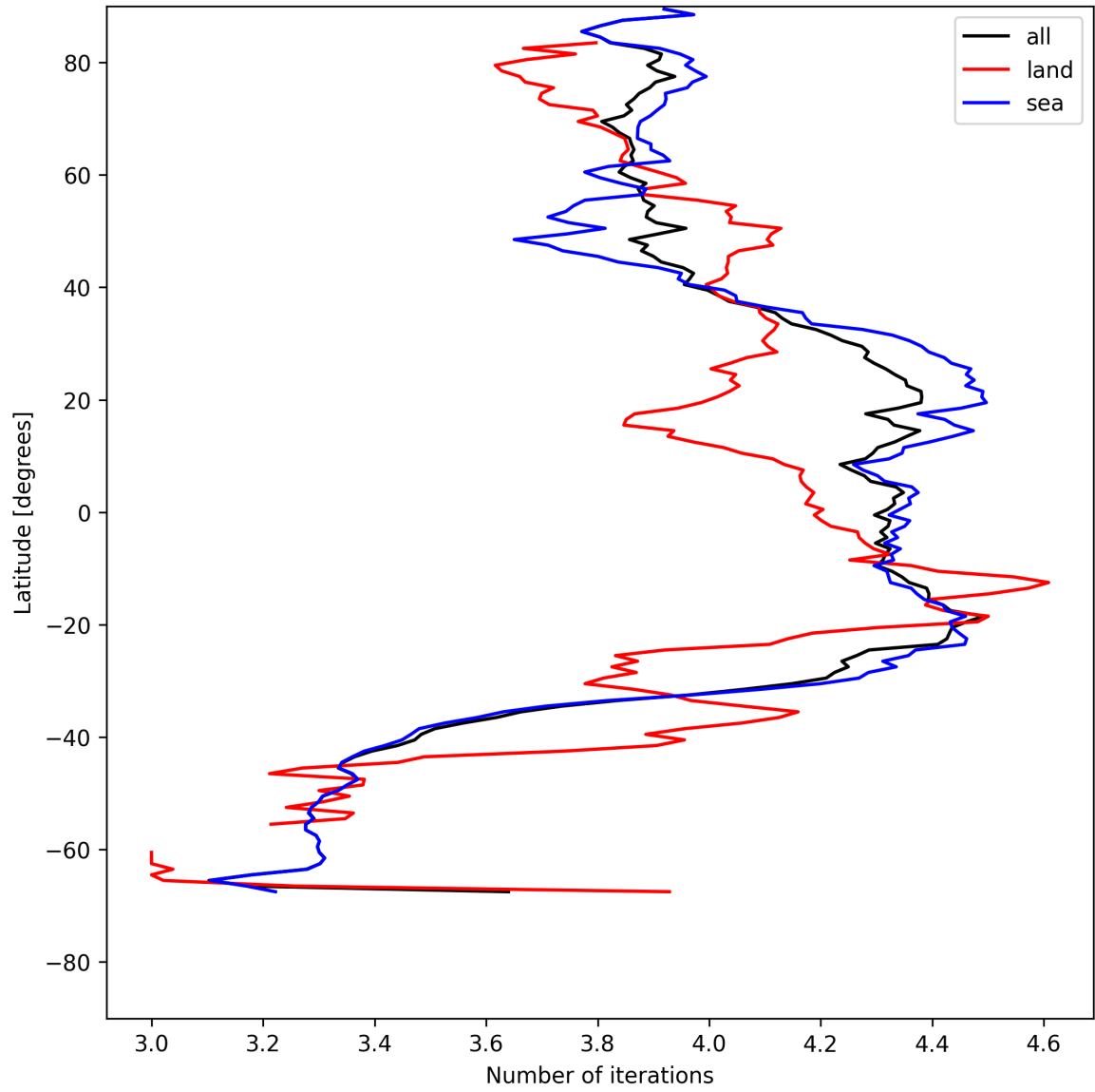
Figure 15: Zonal average of “Number of iterations” for 2025-05-22 to 2025-05-23.
