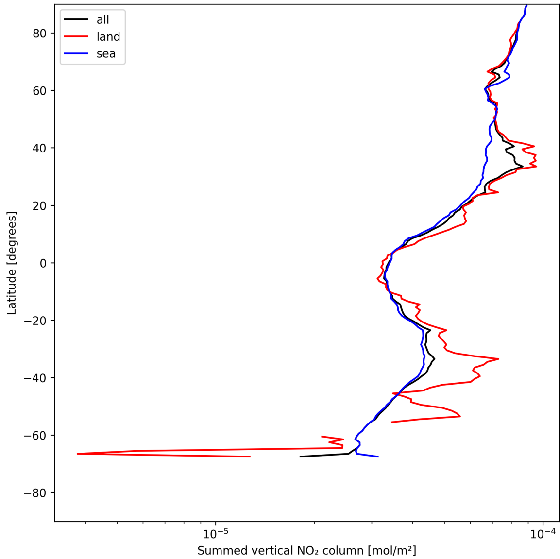
Figure 21: Zonal average of “Summed vertical NO 2 column” for 2025-05-22 to 2025-05-23.
