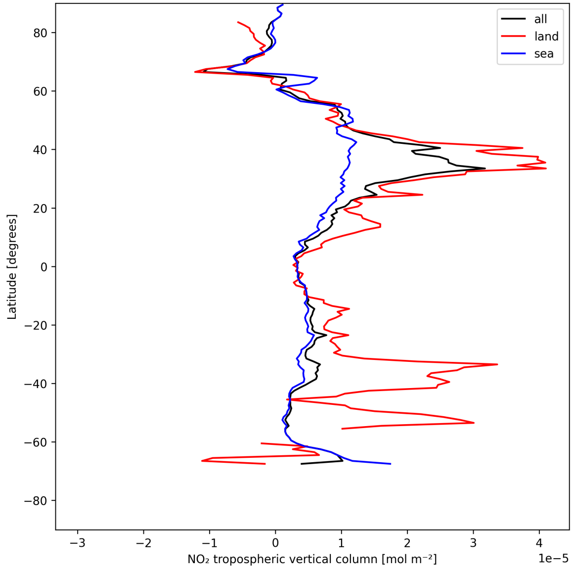
Figure 10: Zonal average of “NO 2 tropospheric vertical column” for 2025-05-22 to 2025-05-23.
