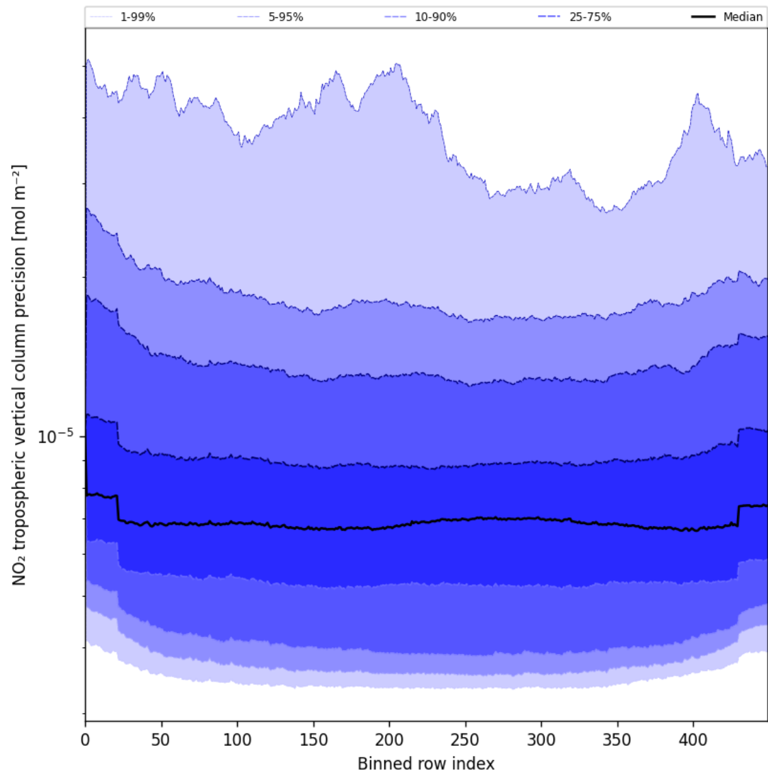
Figure 45: Along track statistics of “NO 2 tropospheric vertical column precision” for 2025-05-22 to 2025-05-23
