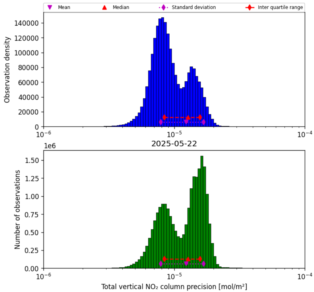
Figure 37: Histogram of “Total vertical NO 2 column precision” for 2025-05-22 to 2025-05-23
