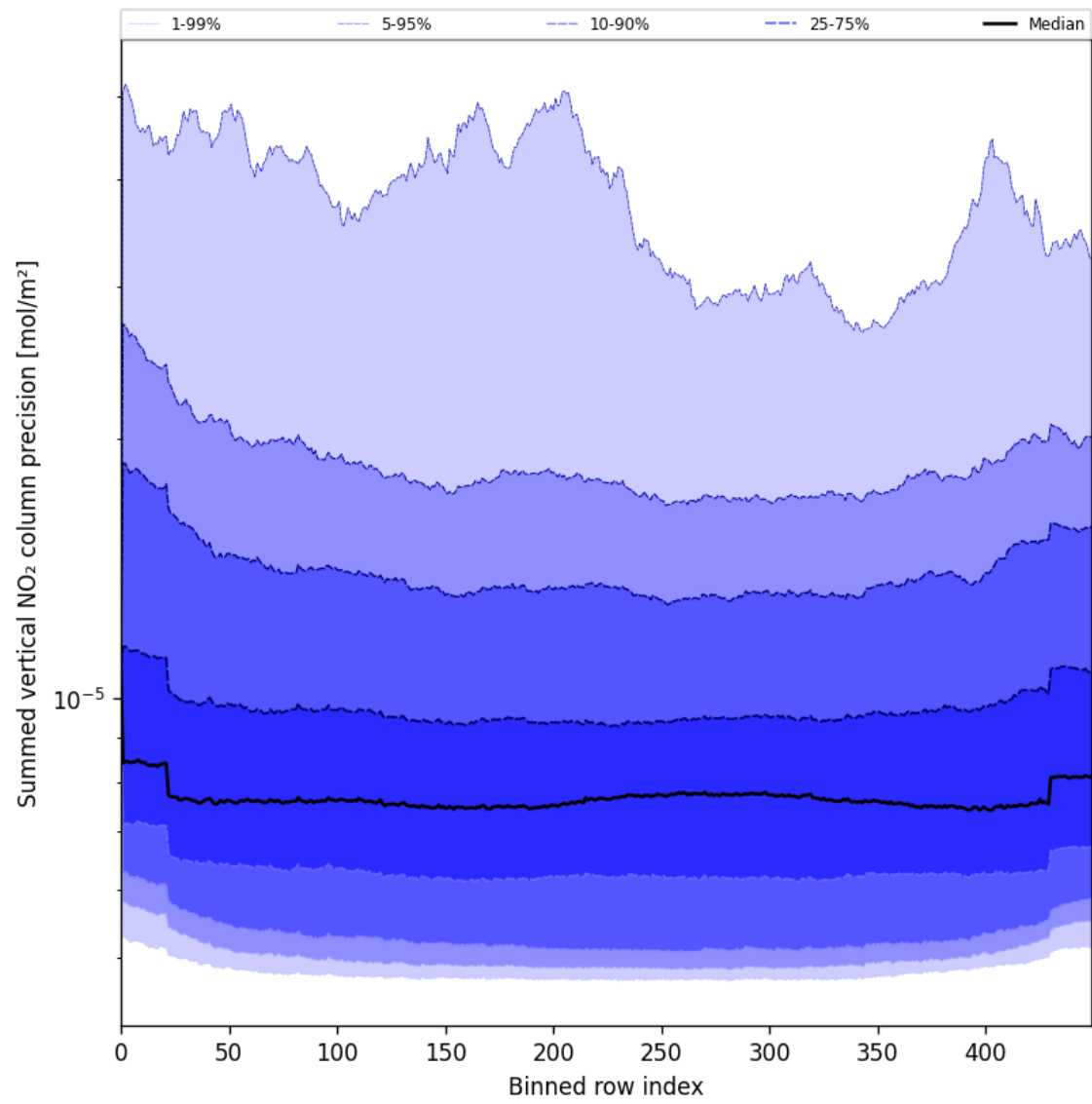
Figure 56: Along track statistics of “Summed vertical NO 2 column precision” for 2025-05-22 to 2025-05-23
