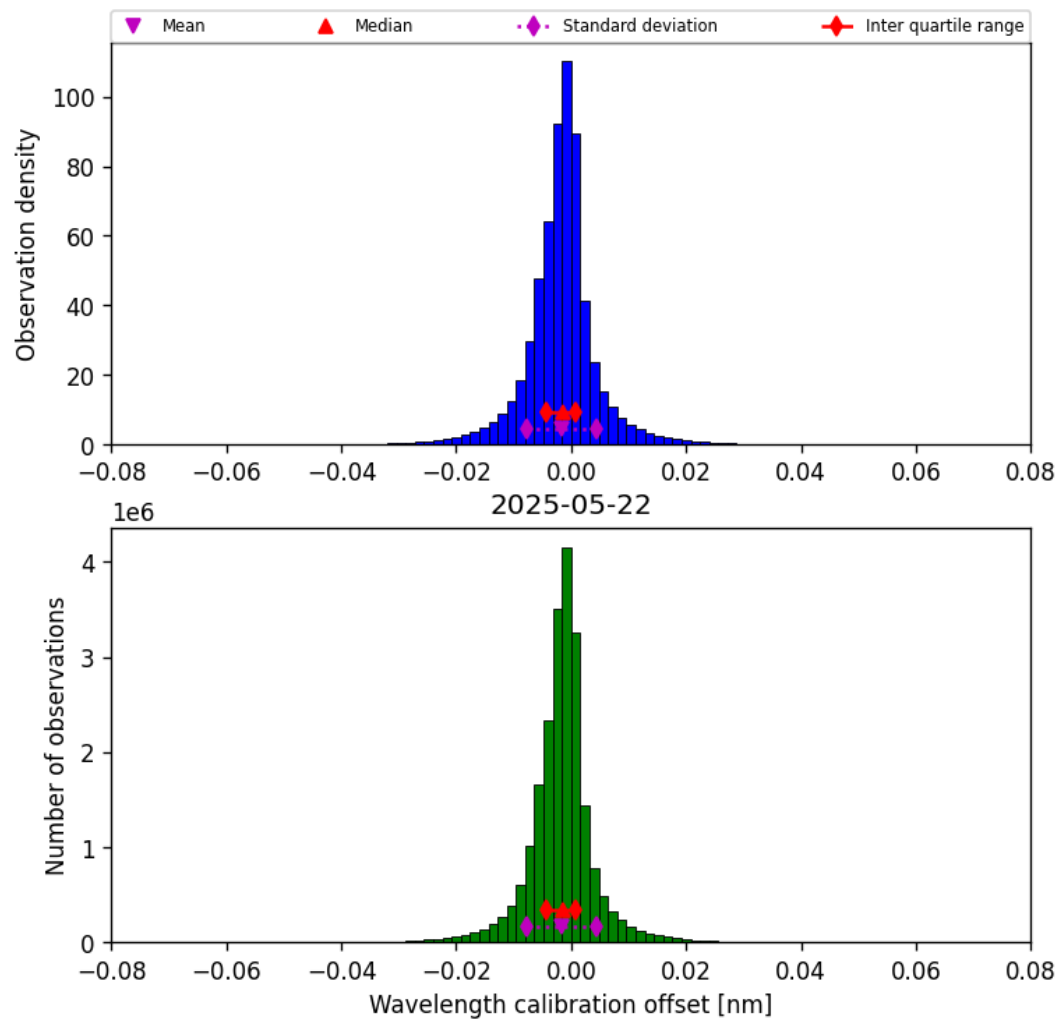
Figure 33: Histogram of “Wavelength calibration offset” for 2025-05-22 to 2025-05-23
