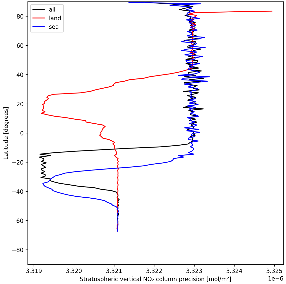
Figure 18: Zonal average of “Stratospheric vertical NO 2 column precision” for 2025-05-22 to 2025-05-23.
