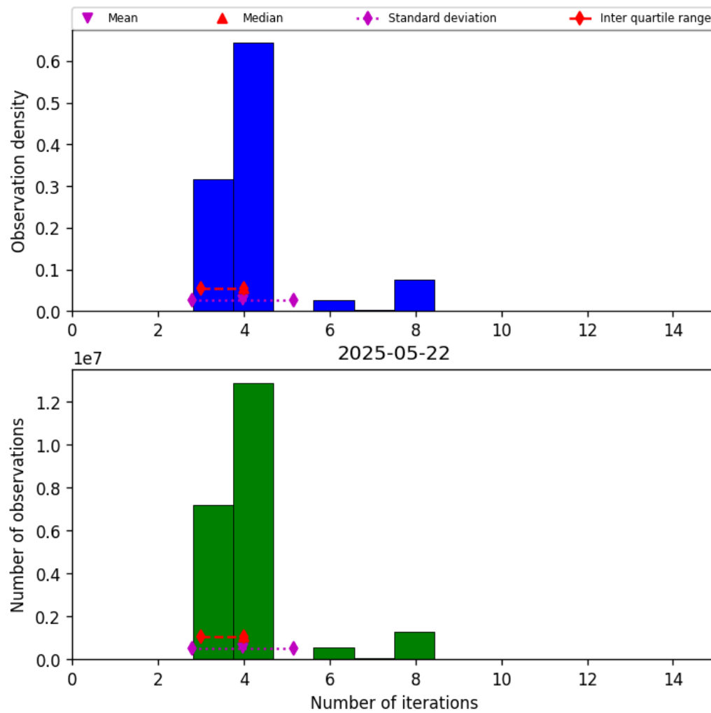
Figure 32: Histogram of “Number of iterations” for 2025-05-22 to 2025-05-23
