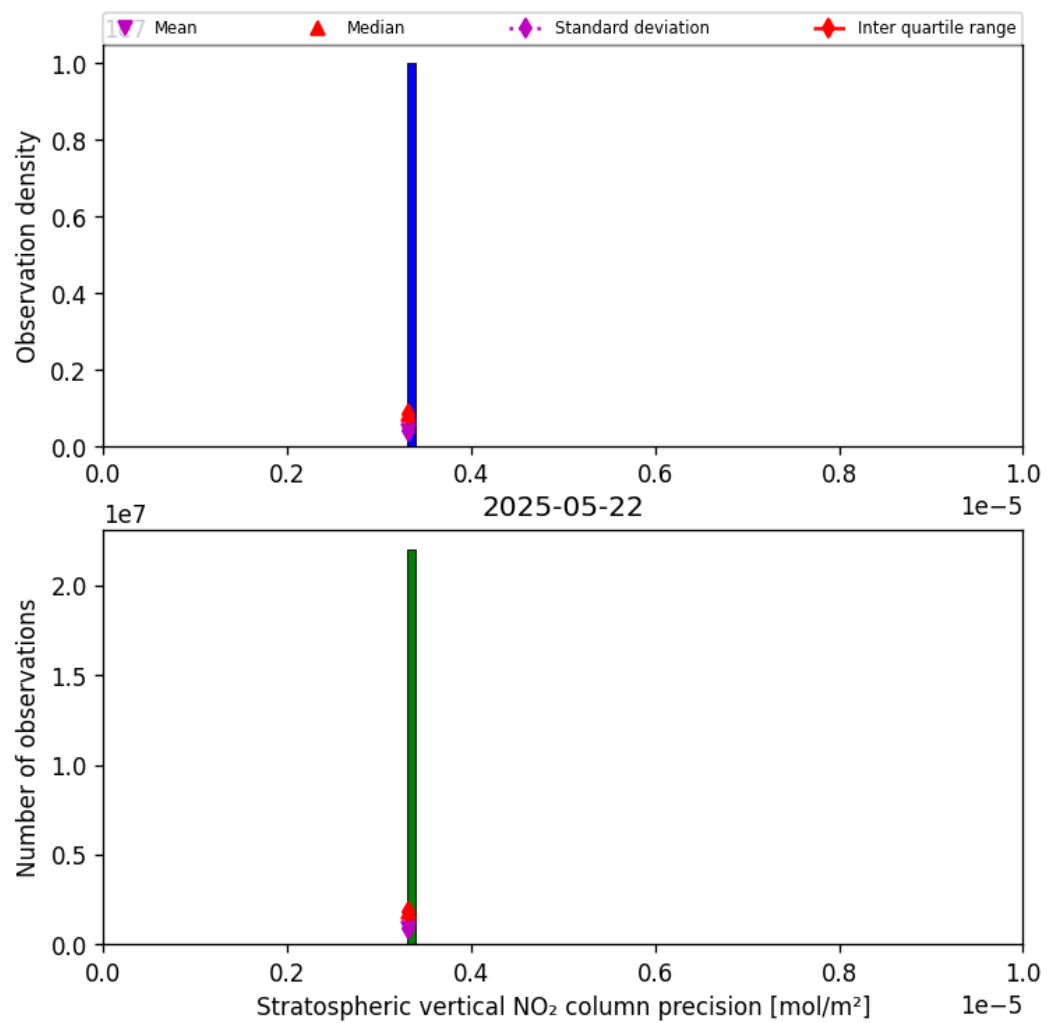
Figure 35: Histogram of “Stratospheric vertical NO 2 column precision” for 2025-05-22 to 2025-05-23
