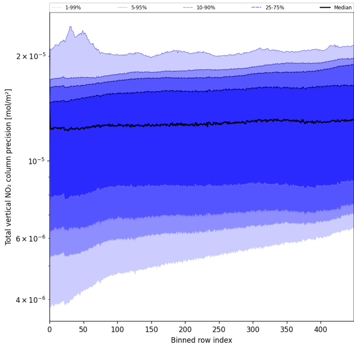
Figure 54: Along track statistics of "Total vertical NO 2 column precision" for 2025-05-22 to 2025-05-23
