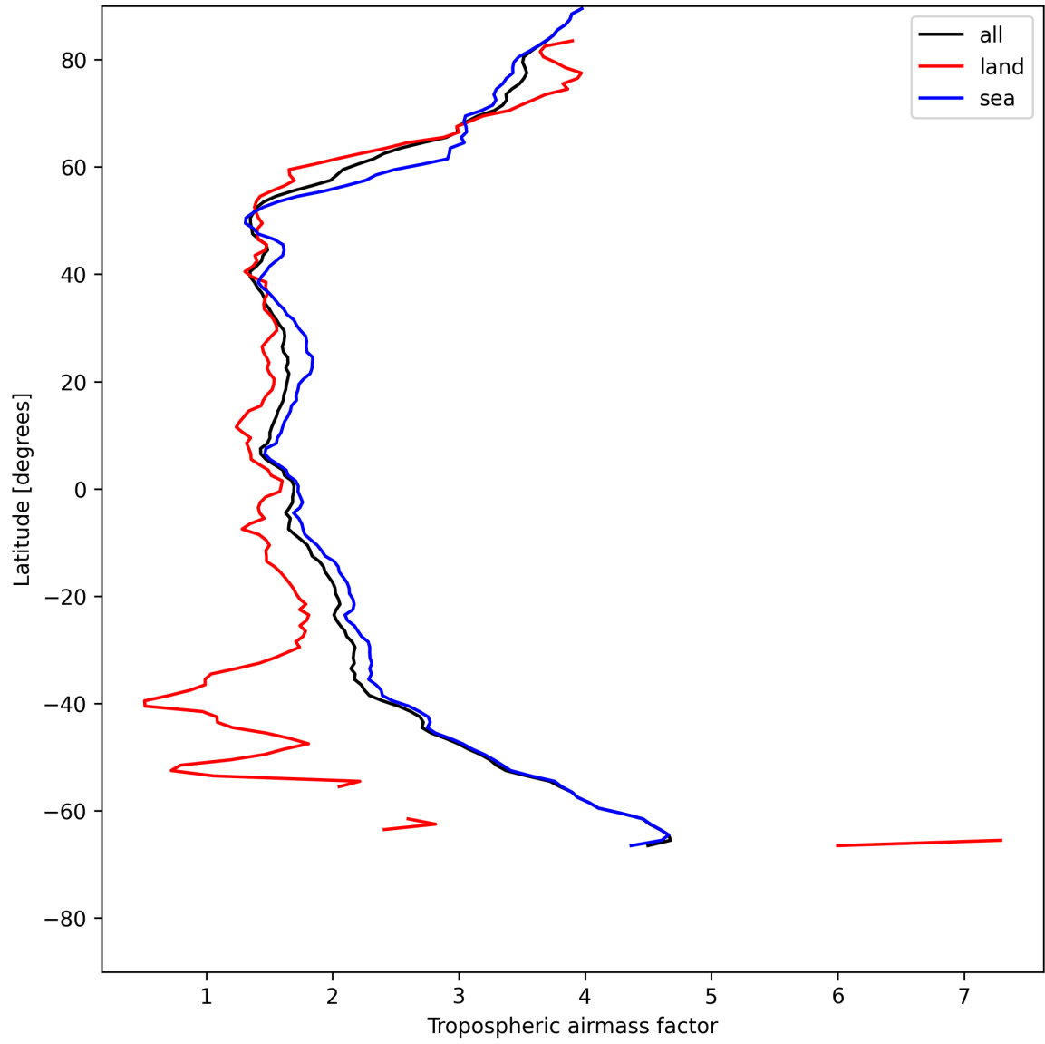
Figure 12: Zonal average of “Tropospheric airmass factor” for 2025-05-23 to 2025-05-24.
