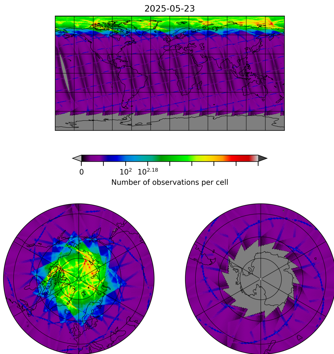
Figure 8: Map of the number of observations for 2025-05-23 to 2025-05-24
