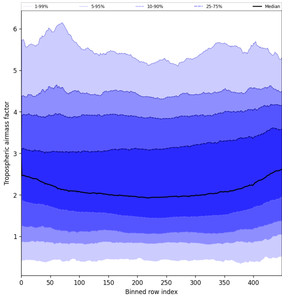
Figure 46: Along track statistics of “Tropospheric airmass factor” for 2025-05-23 to 2025-05-24
