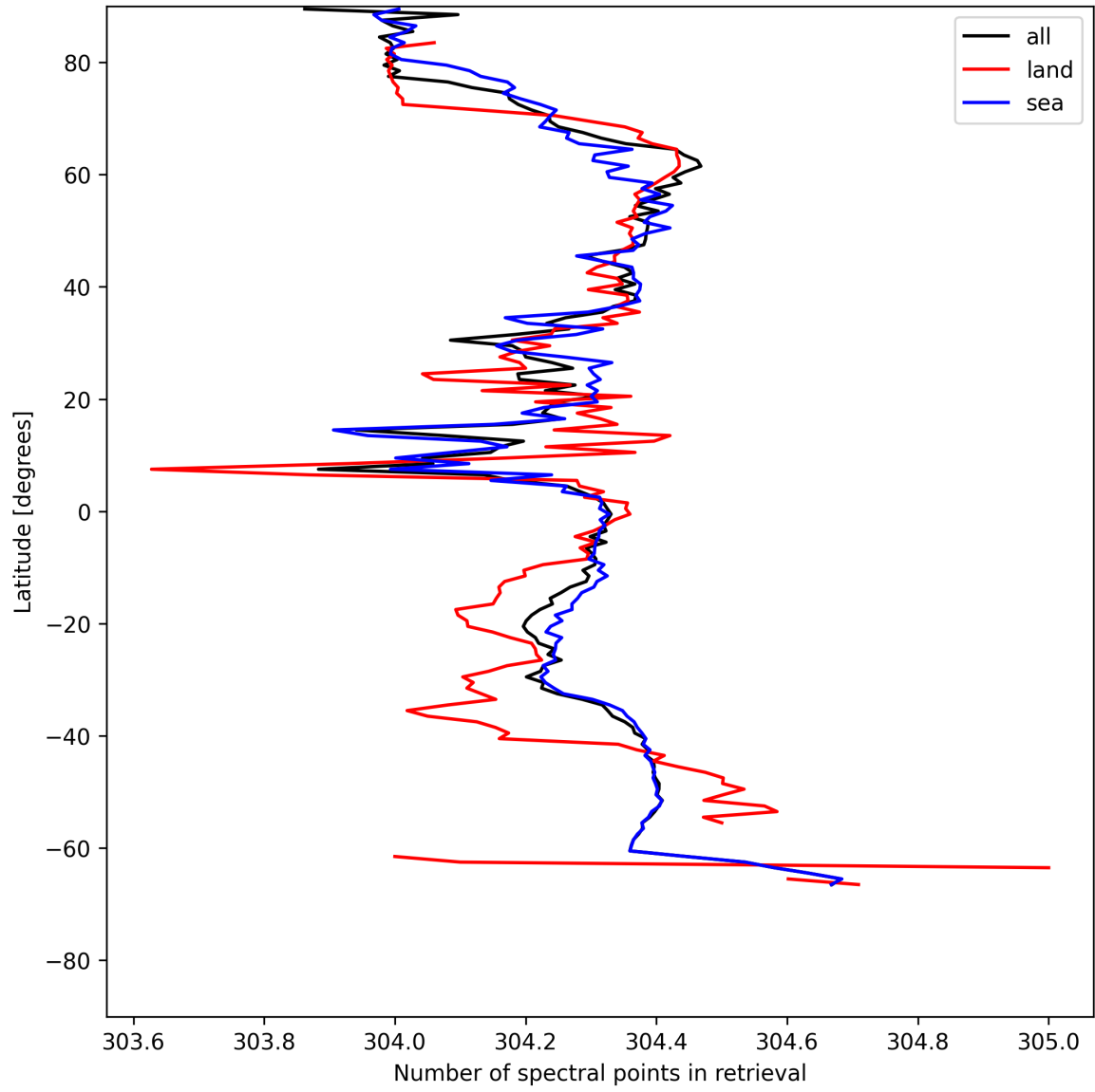
Figure 14: Zonal average of “Number of spectral points in retrieval” for 2025-05-23 to 2025-05-24.
