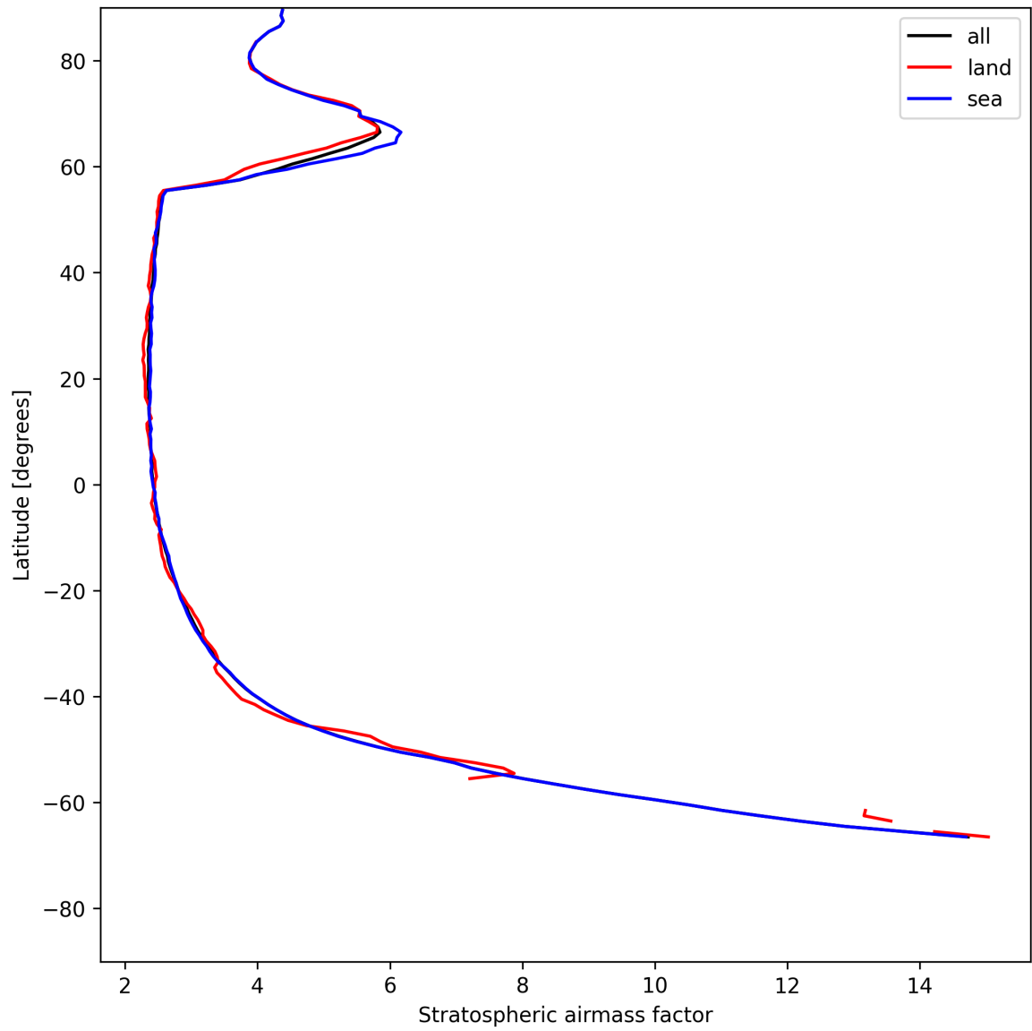
Figure 25: Zonal average of “Stratospheric air mass factor” for 2025-05-23 to 2025-05-24.
