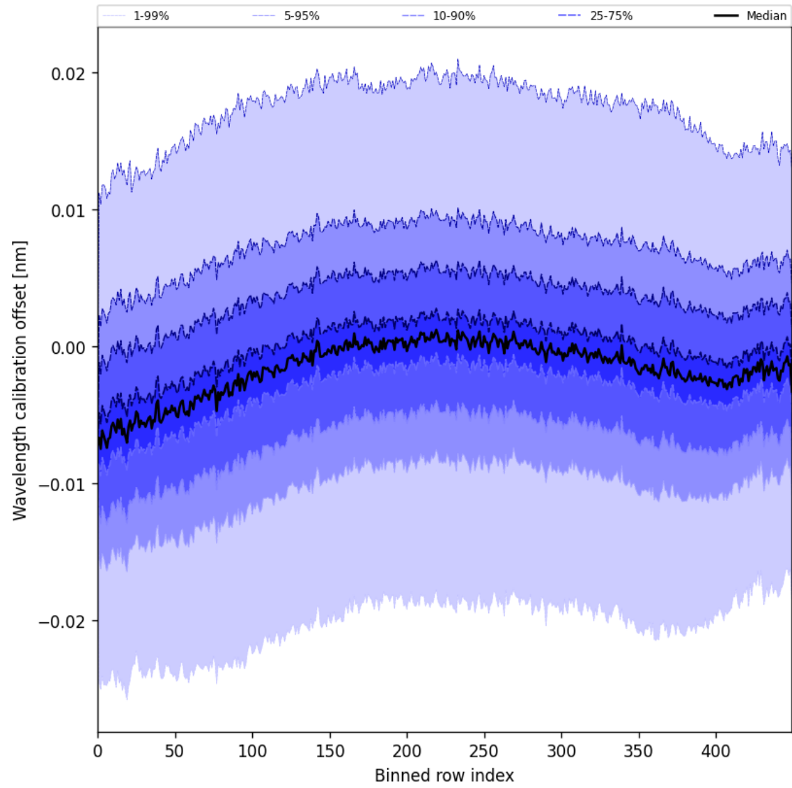
Figure 50: Along track statistics of “Wavelength calibration offset” for 2025-05-23 to 2025-05-24
