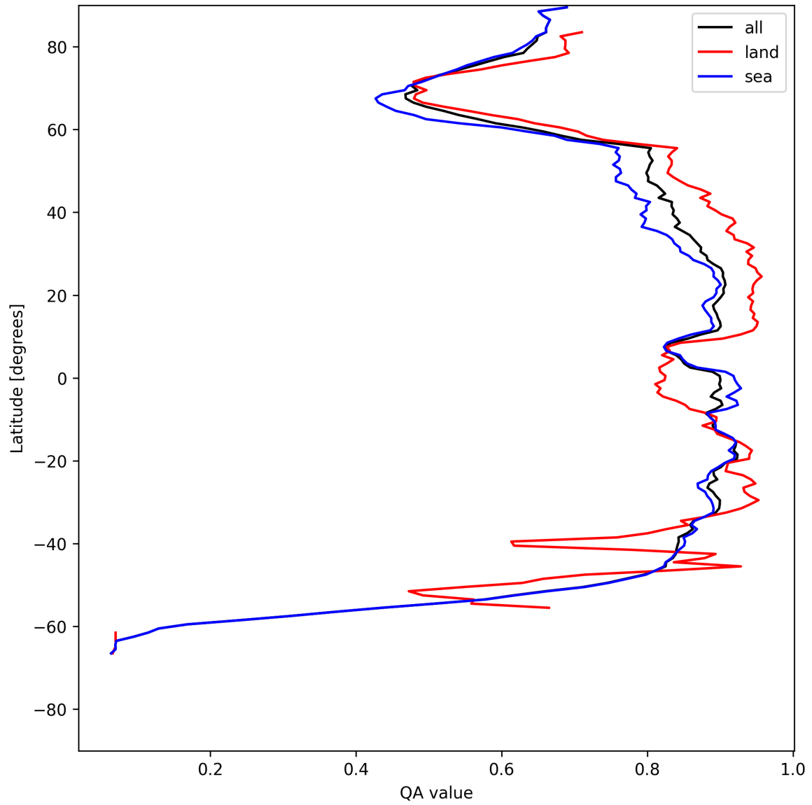
Figure 9: Zonal average of “QA value” for 2025-05-23 to 2025-05-24.
