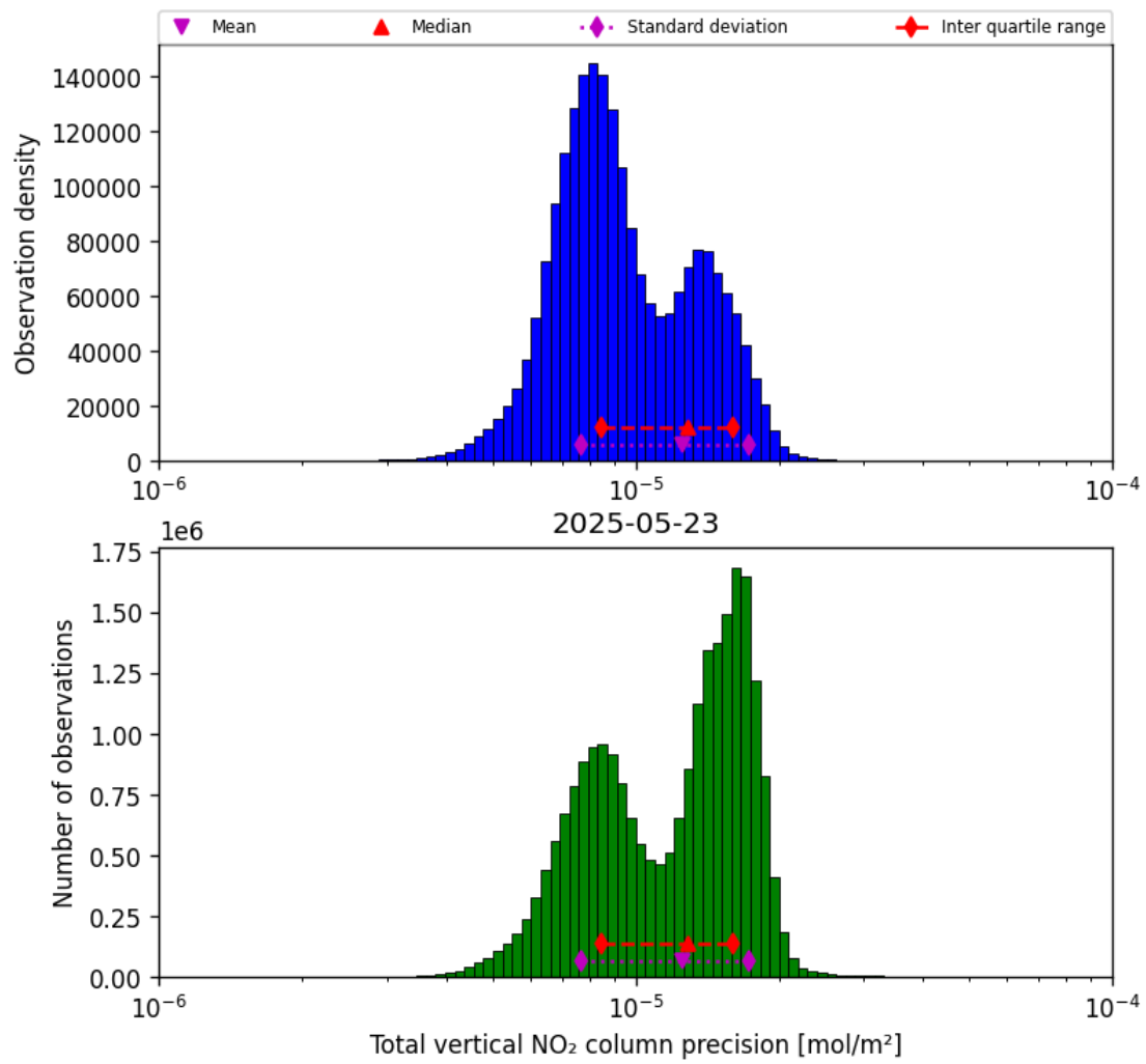
Figure 37: Histogram of “Total vertical NO 2 column precision” for 2025-05-23 to 2025-05-24
