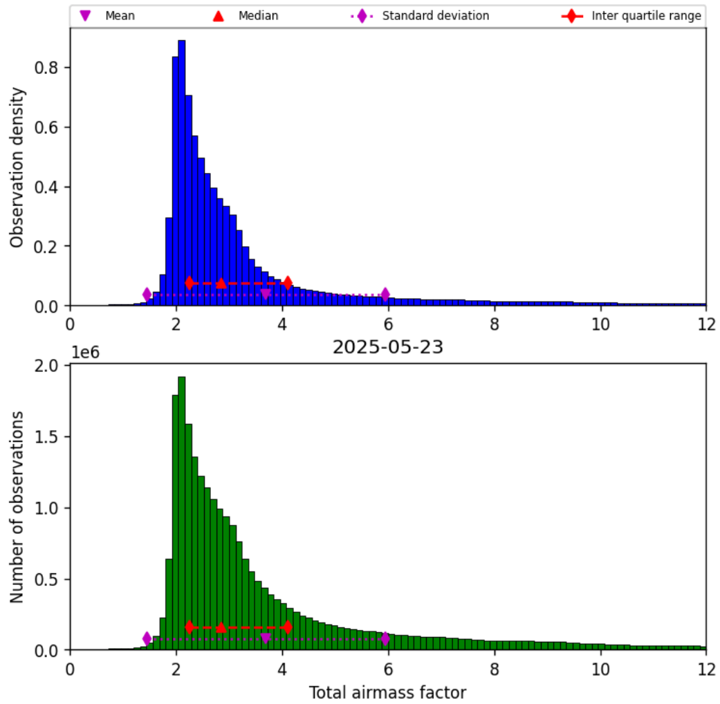
Figure 30: Histogram of “Total airmass factor” for 2025-05-23 to 2025-05-24
