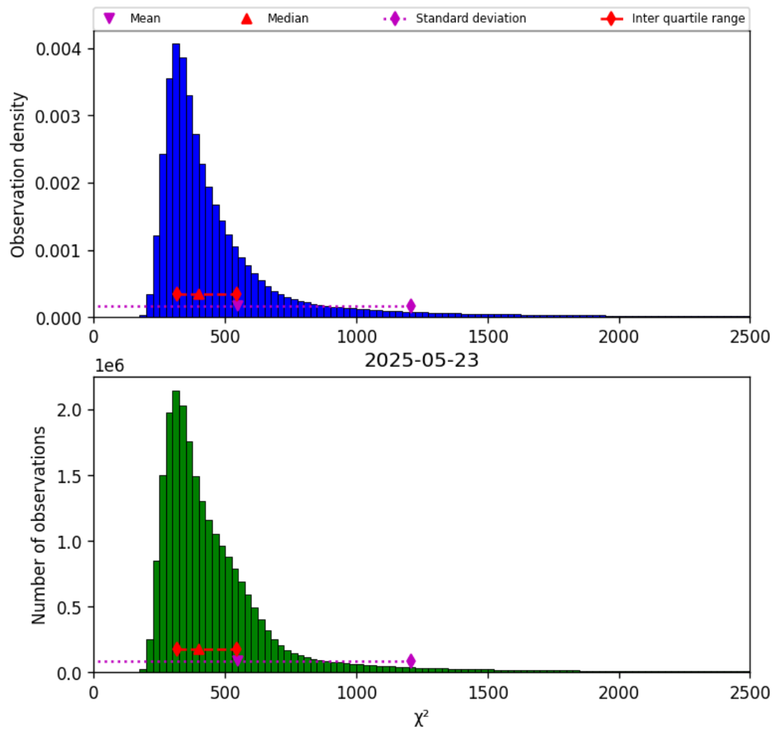
Figure 40: Histogram of “ \chi^2 ” for 2025-05-23 to 2025-05-24
