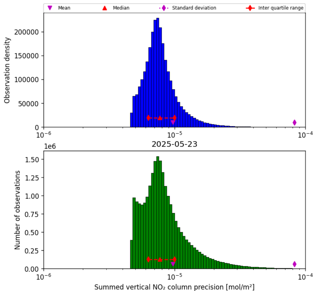
Figure 39: Histogram of “Summed vertical NO 2 column precision” for 2025-05-23 to 2025-05-24
