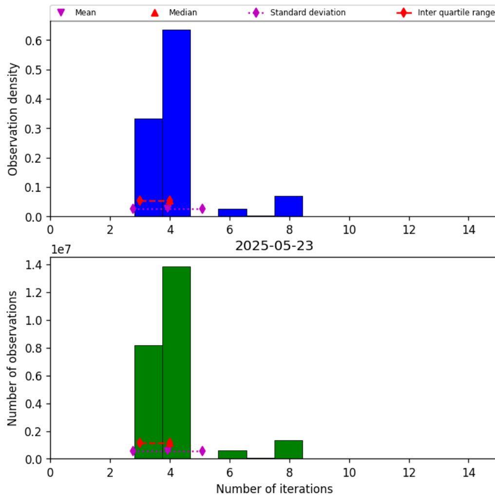
Figure 32: Histogram of “Number of iterations” for 2025-05-23 to 2025-05-24
