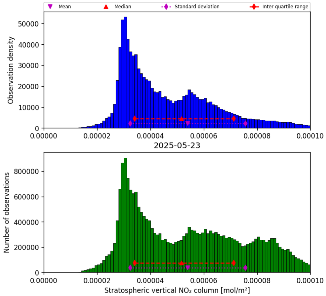
Figure 34: Histogram of “Stratospheric vertical NO 2 column” for 2025-05-23 to 2025-05-24
