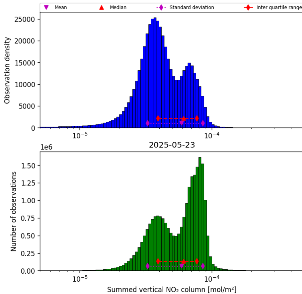
Figure 38: Histogram of “Summed vertical NO 2 column” for 2025-05-23 to 2025-05-24
