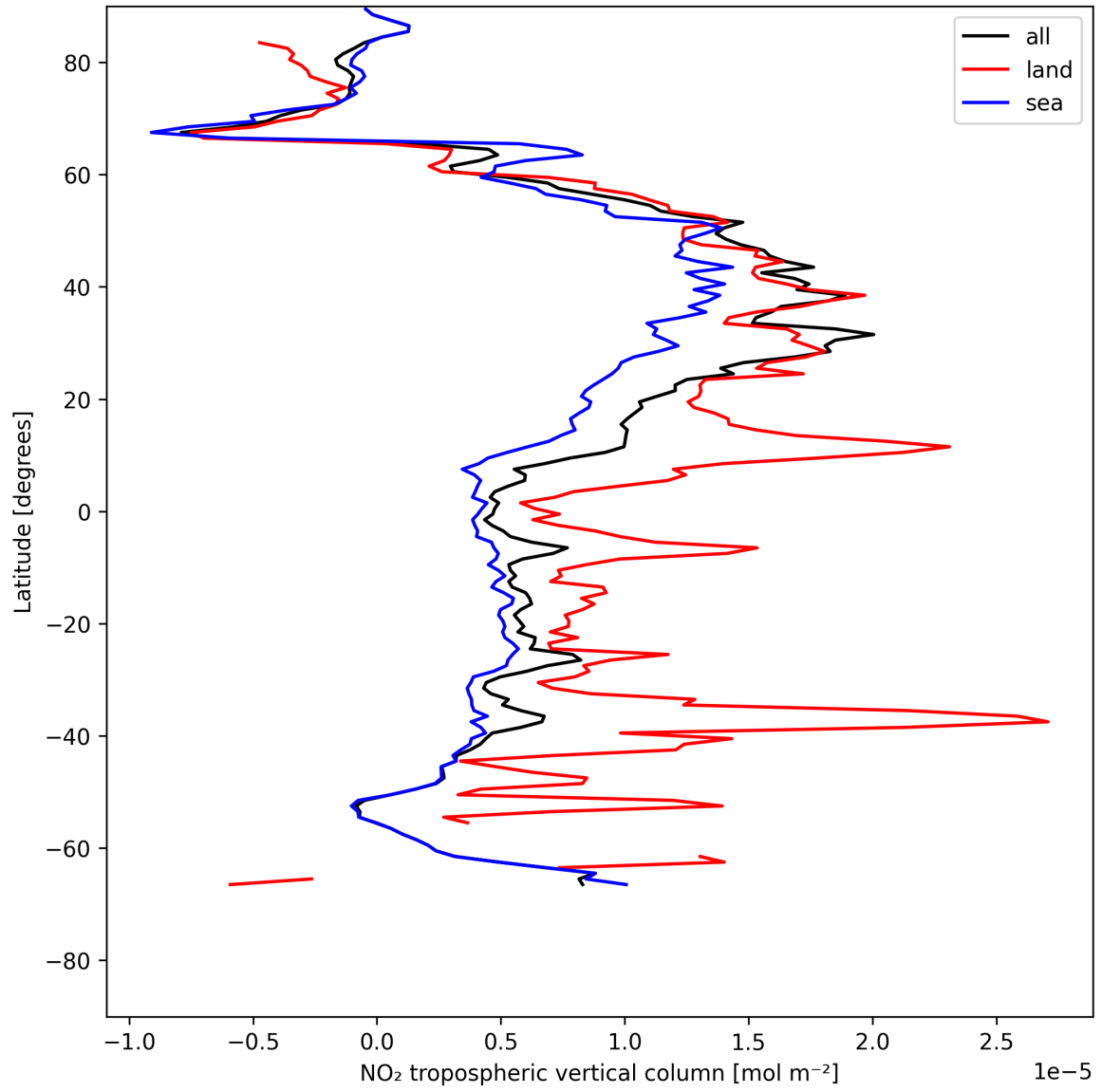
Figure 10: Zonal average of “NO 2 tropospheric vertical column” for 2025-05-23 to 2025-05-24.
