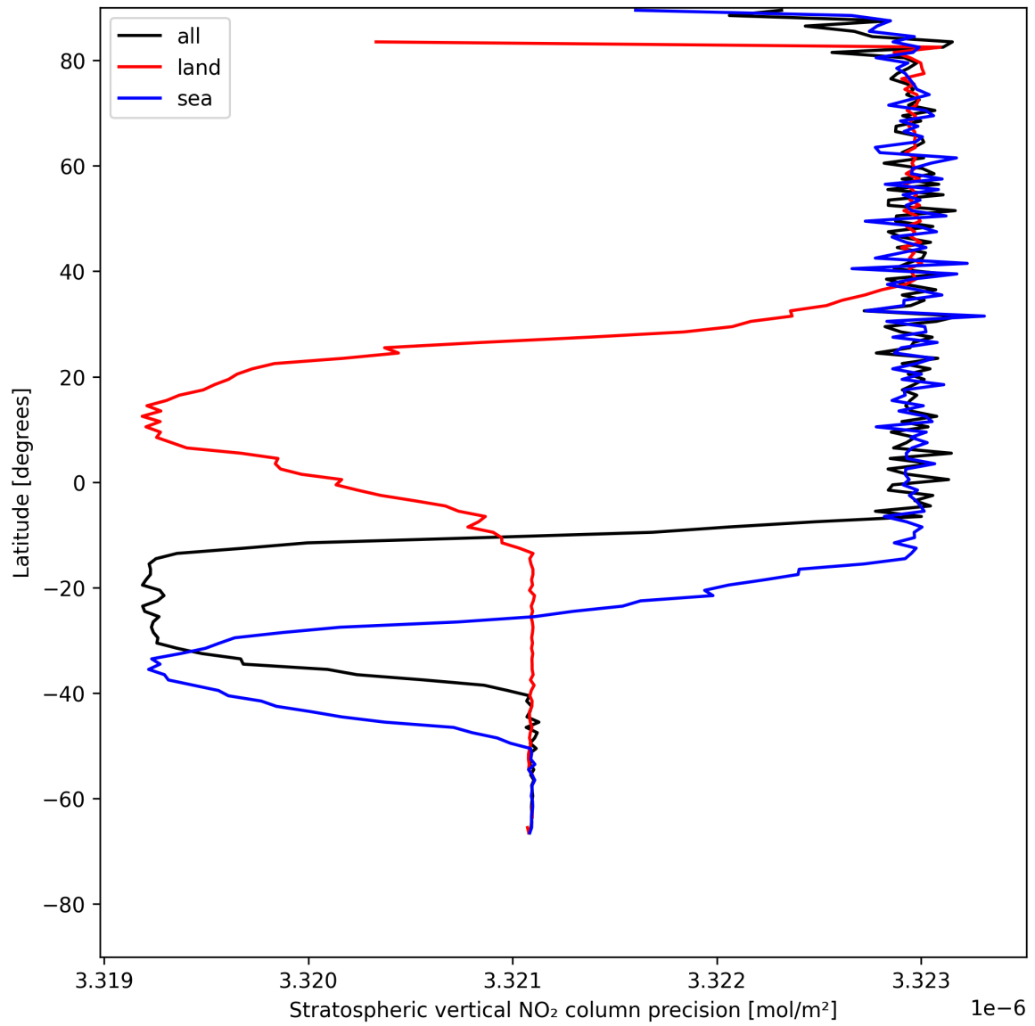
Figure 18: Zonal average of “Stratospheric vertical NO 2 column precision” for 2025-05-23 to 2025-05-24.
