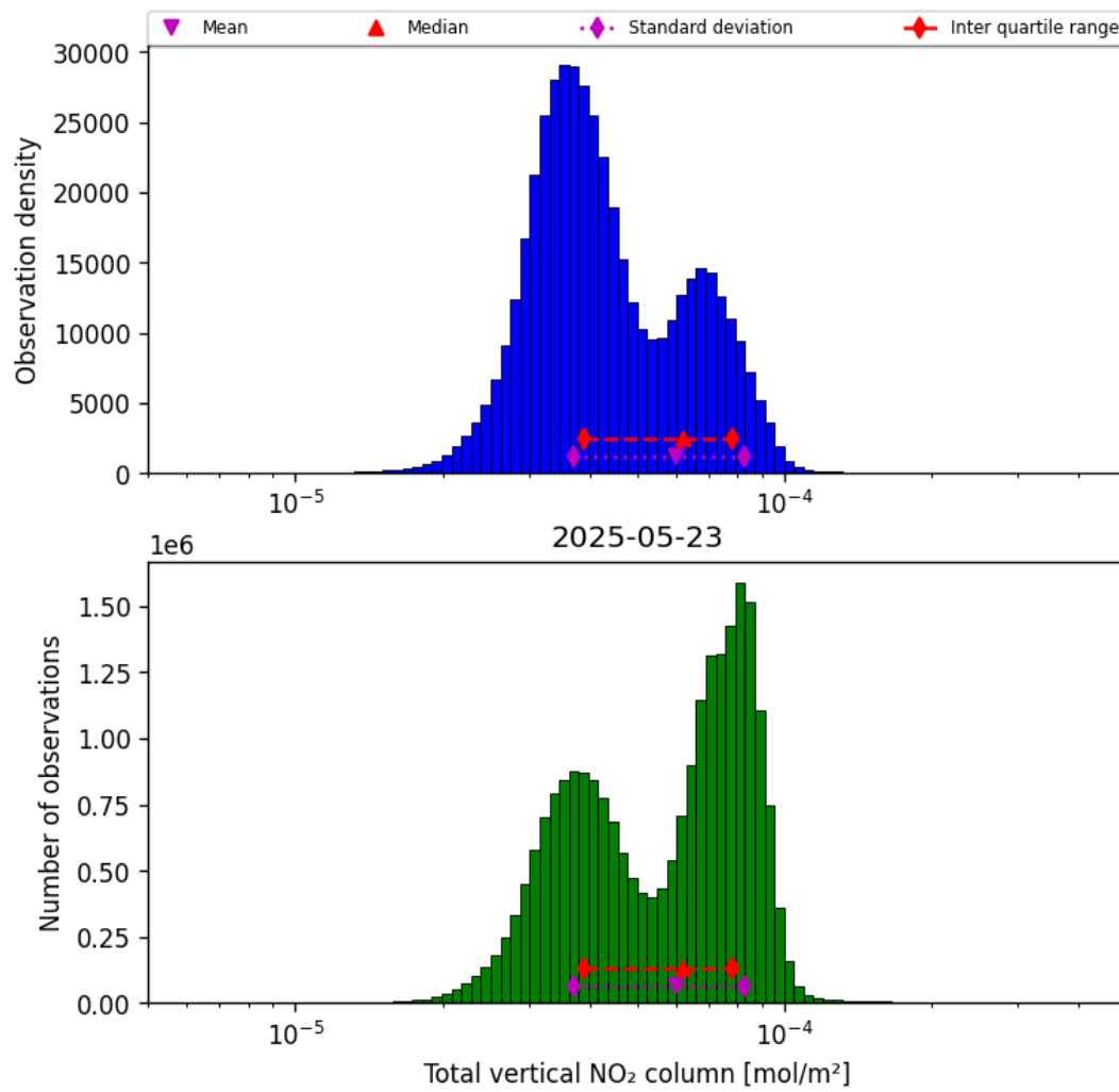
Figure 36: Histogram of “Total vertical NO 2 column” for 2025-05-23 to 2025-05-24
