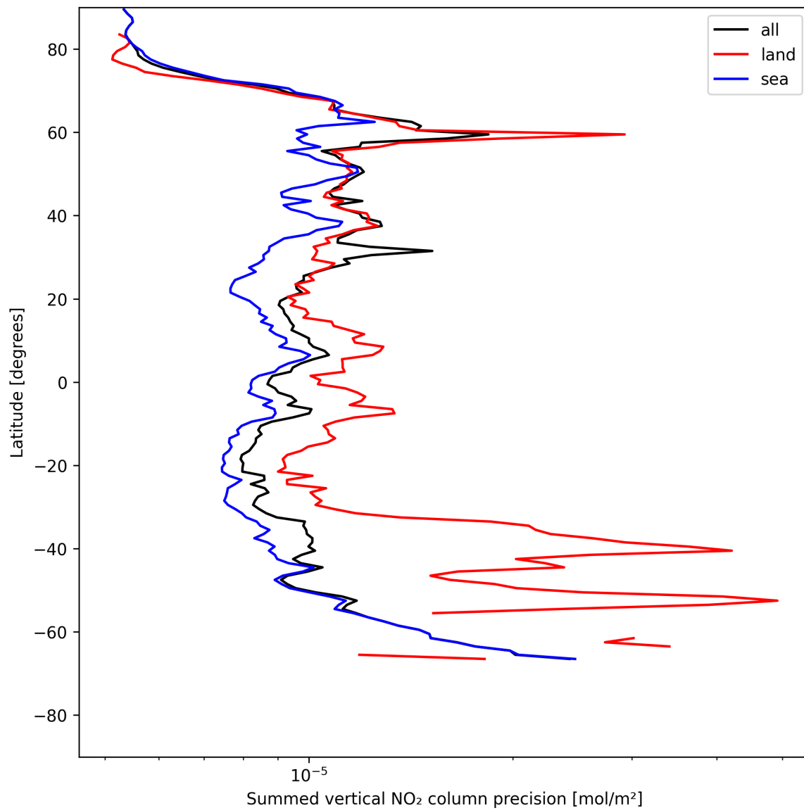
Figure 22: Zonal average of “Summed vertical NO 2 column precision” for 2025-05-23 to 2025-05-24.
