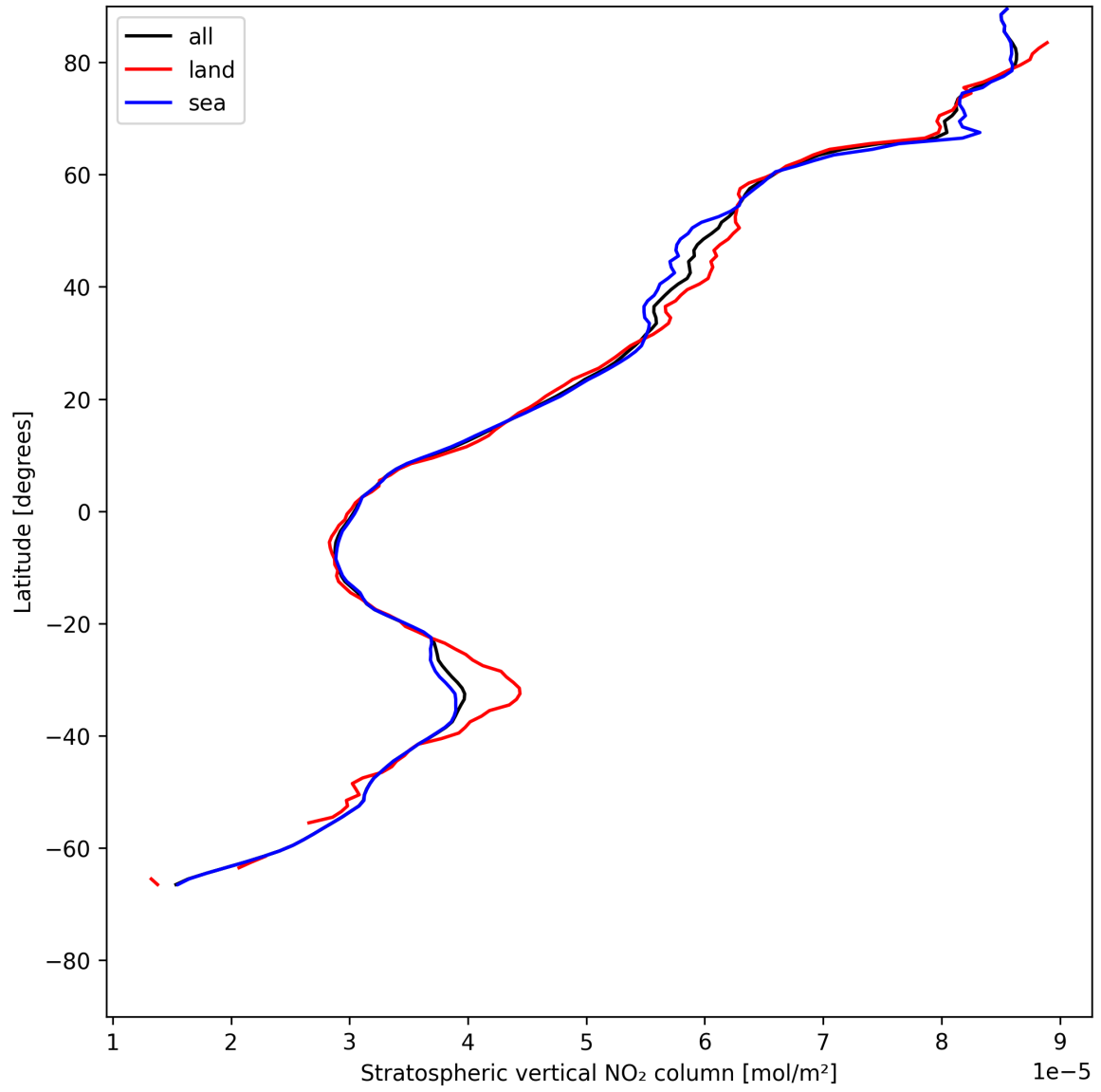
Figure 17: Zonal average of “Stratospheric vertical NO 2 column” for 2025-05-23 to 2025-05-24.
