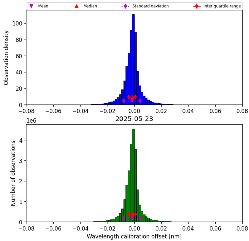
Figure 33: Histogram of “Wavelength calibration offset” for 2025-05-23 to 2025-05-24
