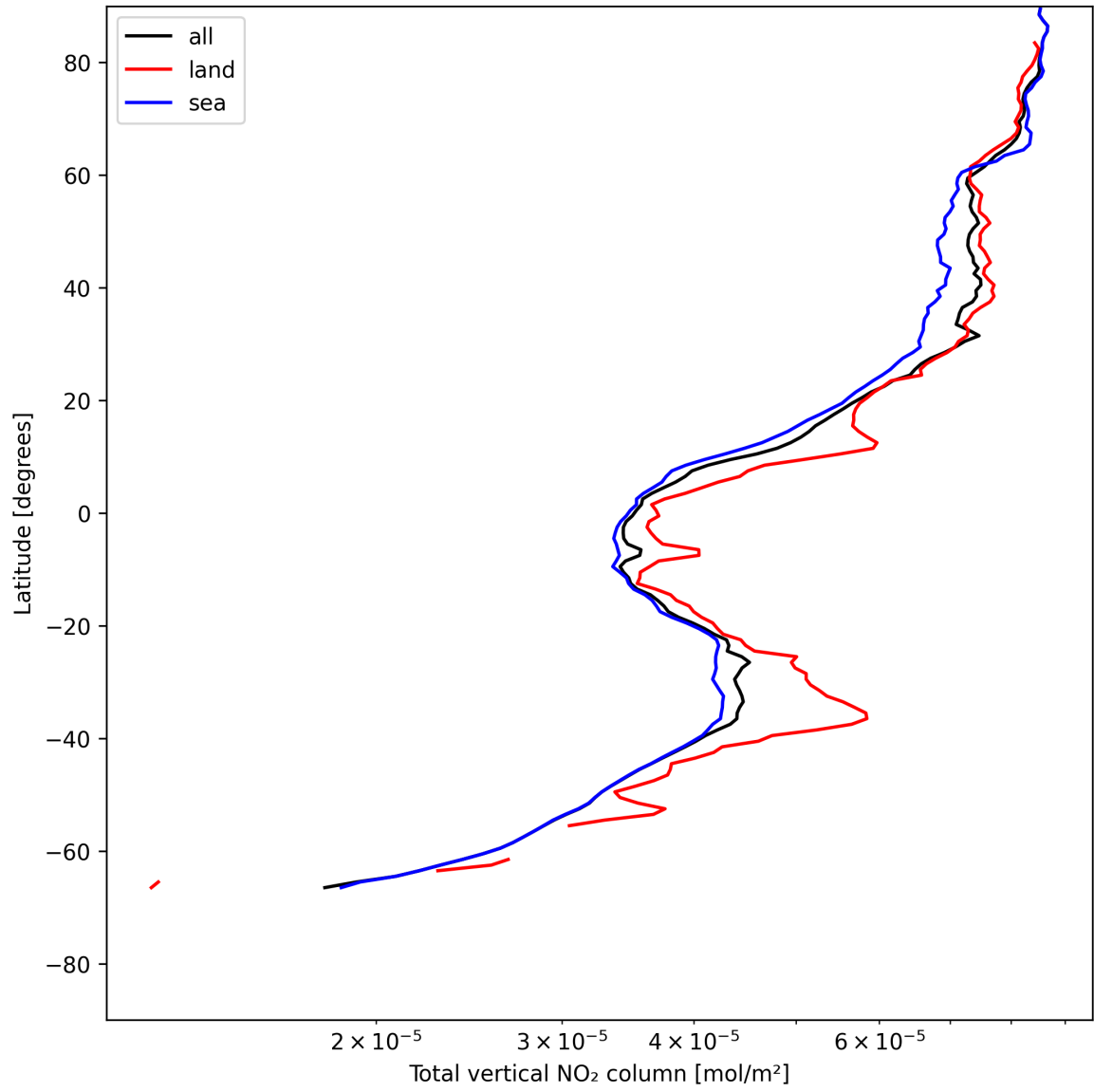
Figure 19: Zonal average of “Total vertical NO 2 column” for 2025-05-23 to 2025-05-24.
