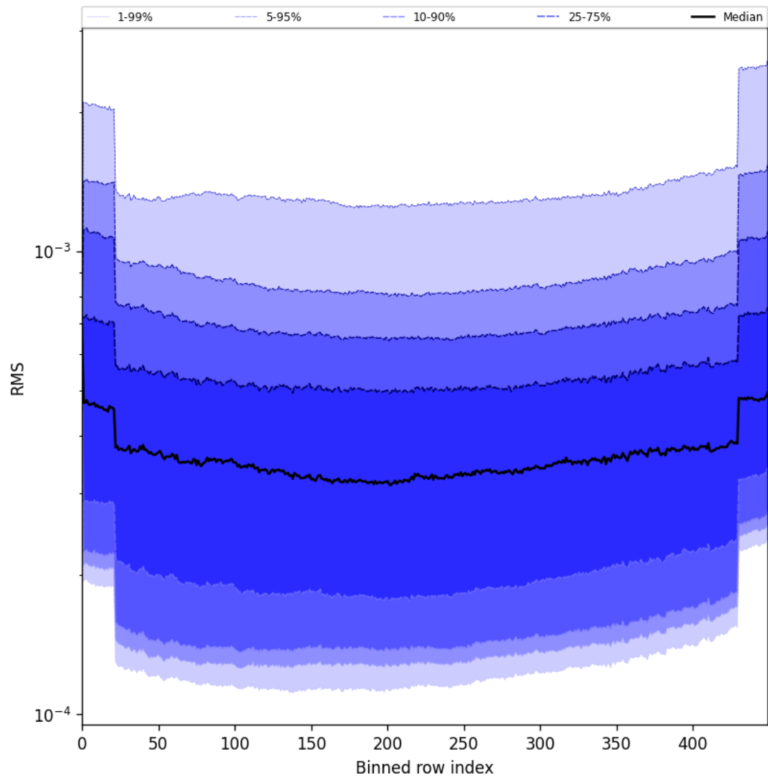
Figure 58: Along track statistics of “RMS” for 2025-05-23 to 2025-05-24
