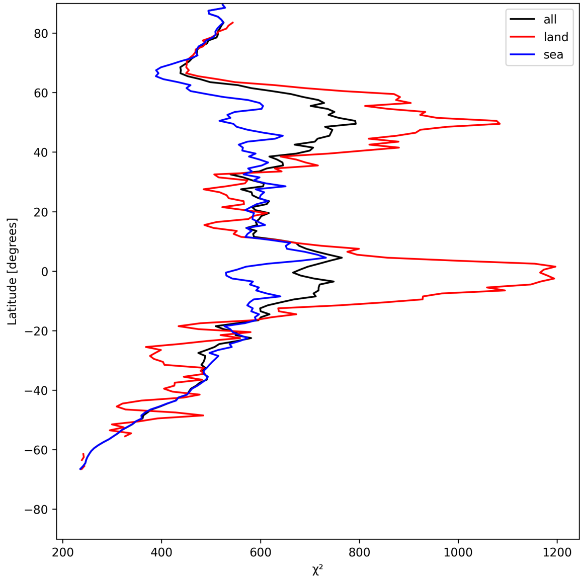
Figure 23: Zonal average of “ \chi^2 ” for 2025-05-23 to 2025-05-24.
