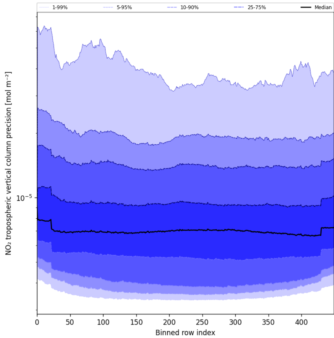
Figure 45: Along track statistics of “NO 2 tropospheric vertical column precision” for 2025-05-23 to 2025-05-24
