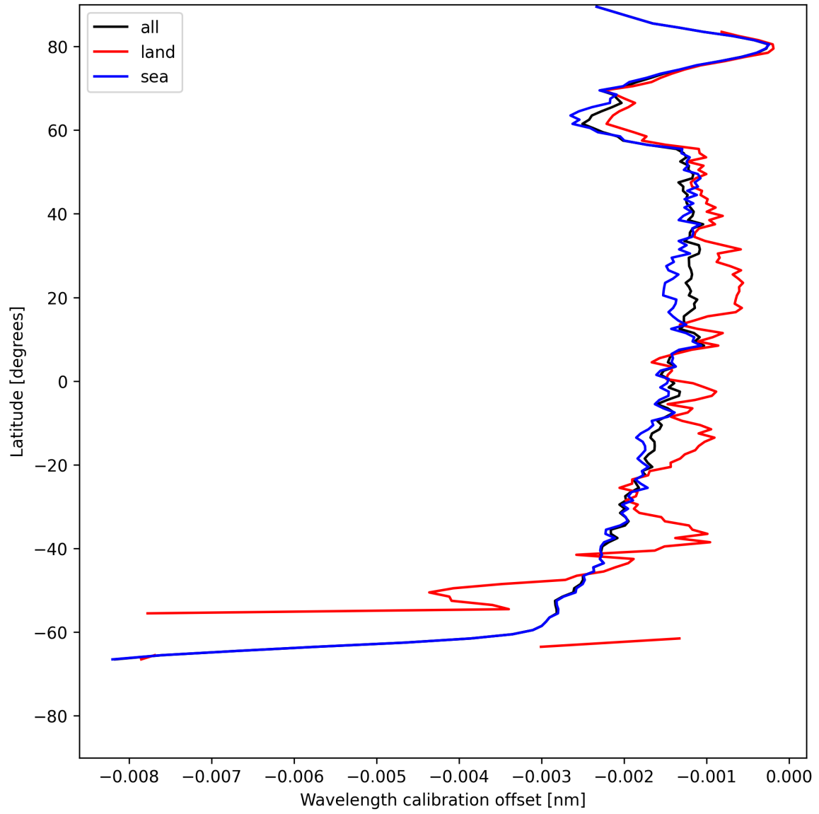
Figure 16: Zonal average of “Wavelength calibration offset” for 2025-05-23 to 2025-05-24.
