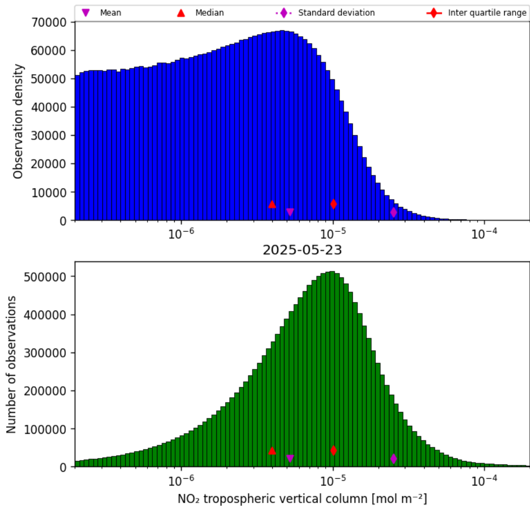
Figure 27: Histogram of “NO 2 tropospheric vertical column” for 2025-05-23 to 2025-05-24
