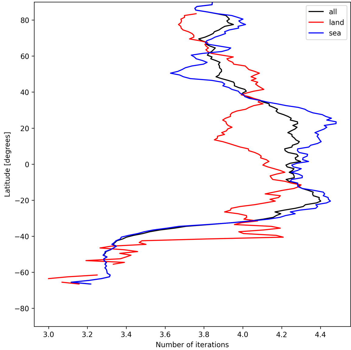
Figure 15: Zonal average of “Number of iterations” for 2025-05-23 to 2025-05-24.
