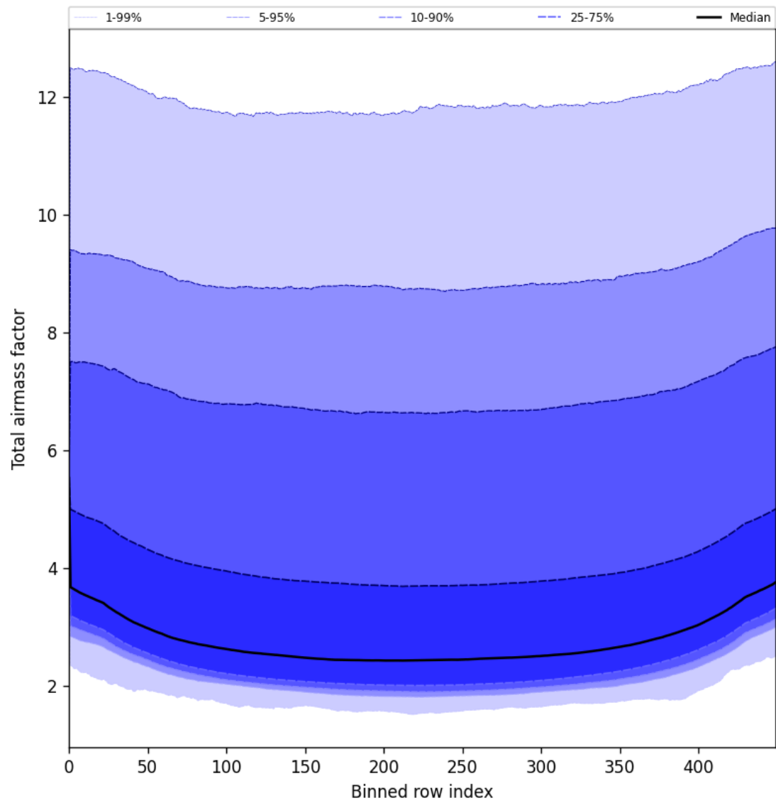
Figure 47: Along track statistics of “Total airmass factor” for 2025-05-23 to 2025-05-24
