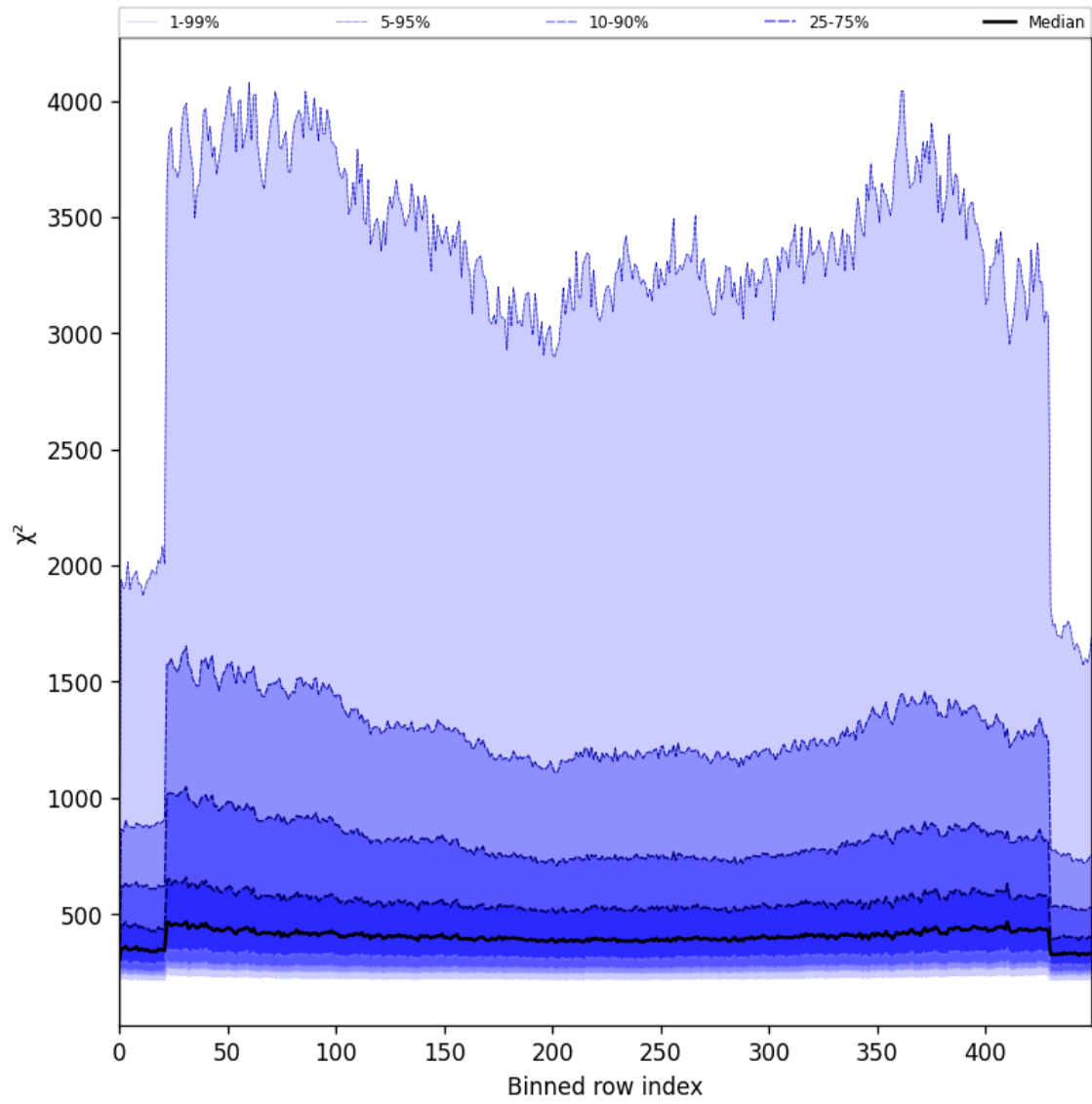
Figure 57: Along track statistics of “ \chi^2 ” for 2025-05-23 to 2025-05-24
