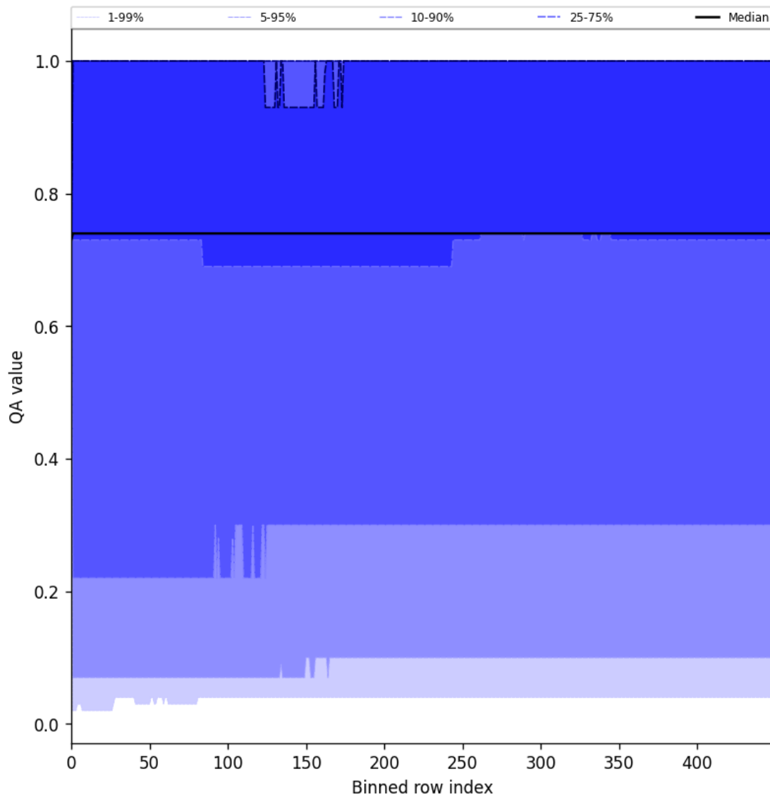
Figure 43: Along track statistics of “QA value” for 2025-05-23 to 2025-05-24
