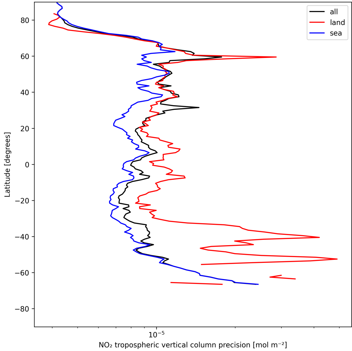
Figure 11: Zonal average of “NO 2 tropospheric vertical column precision” for 2025-05-23 to 2025-05-24.
