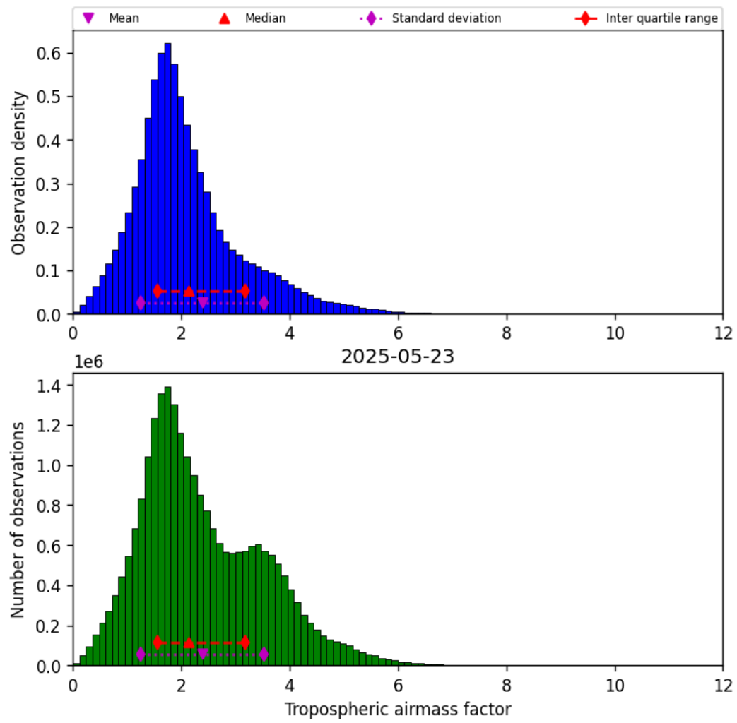
Figure 29: Histogram of “Tropospheric airmass factor” for 2025-05-23 to 2025-05-24
