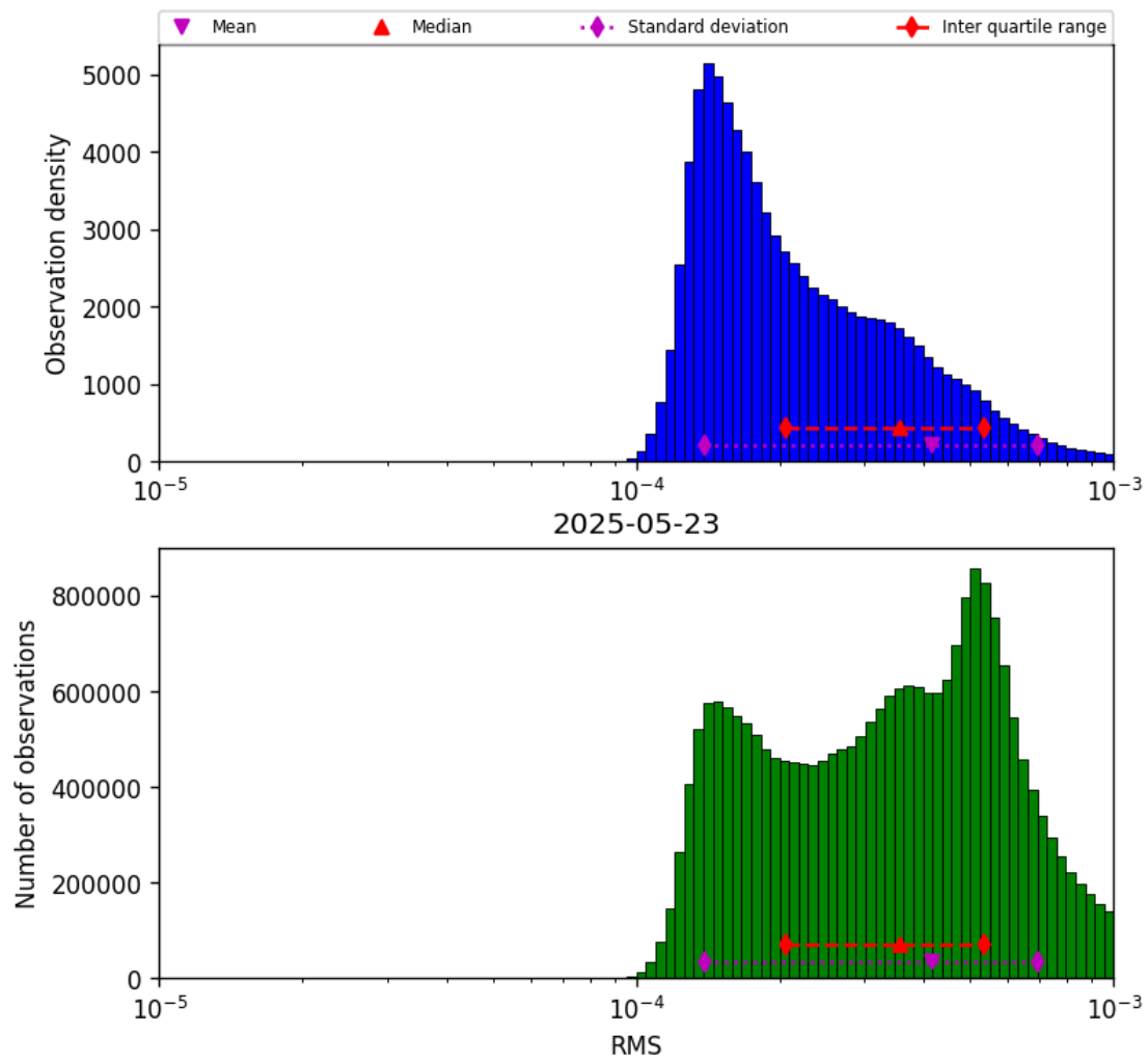
Figure 41: Histogram of “RMS” for 2025-05-23 to 2025-05-24
