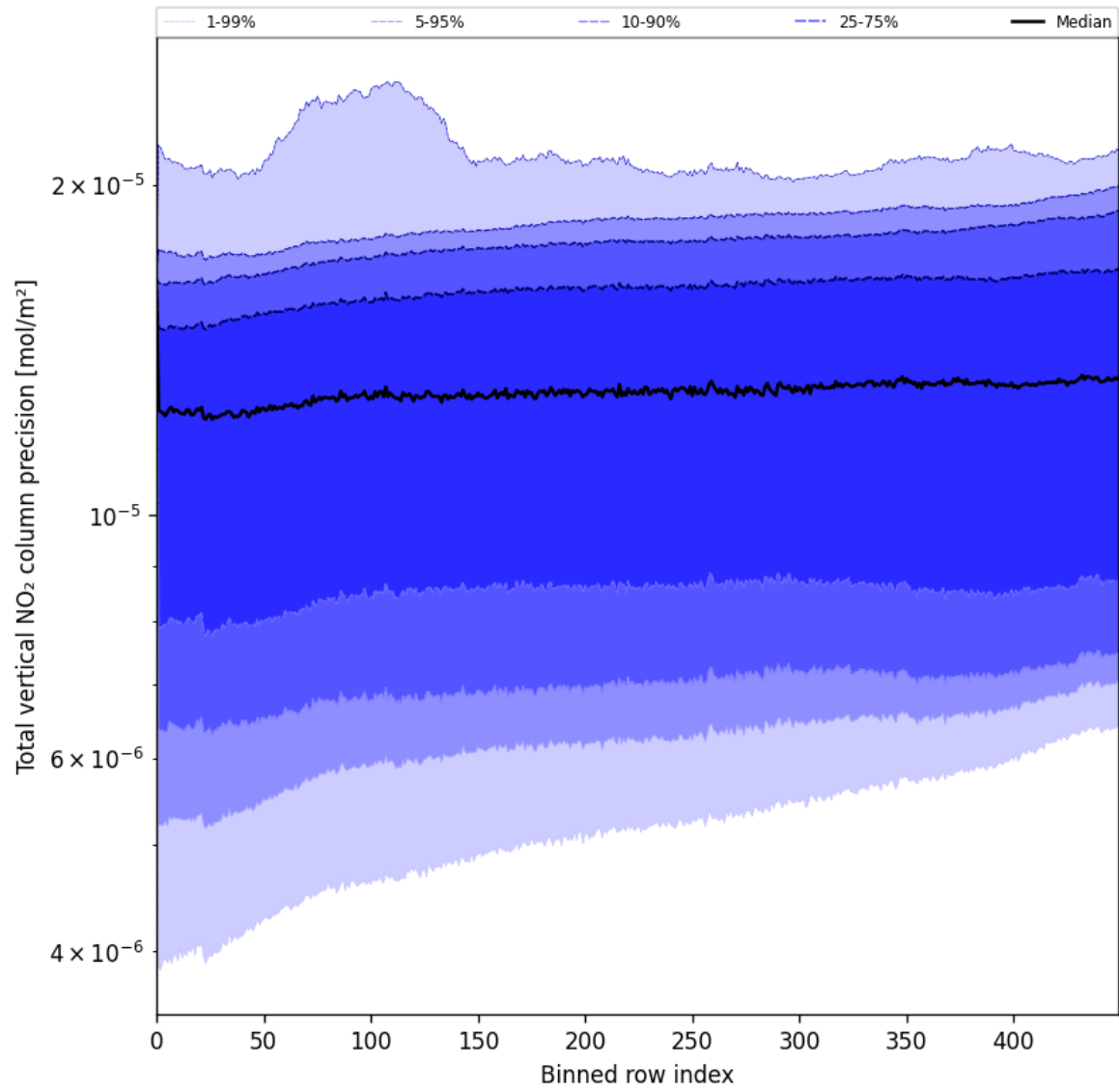
Figure 54: Along track statistics of “Total vertical NO 2 column precision” for 2025-05-23 to 2025-05-24
