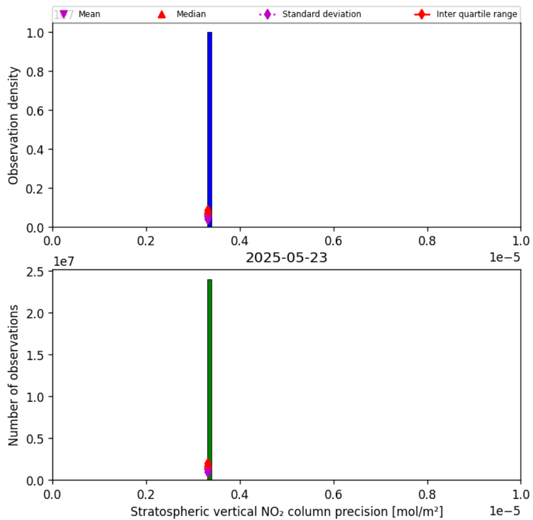
Figure 35: Histogram of “Stratospheric vertical NO 2 column precision” for 2025-05-23 to 2025-05-24
