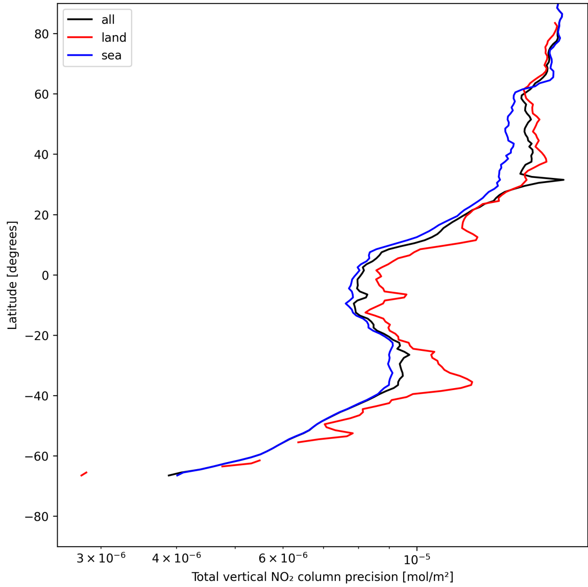
Figure 20: Zonal average of “Total vertical NO 2 column precision” for 2025-05-23 to 2025-05-24.
