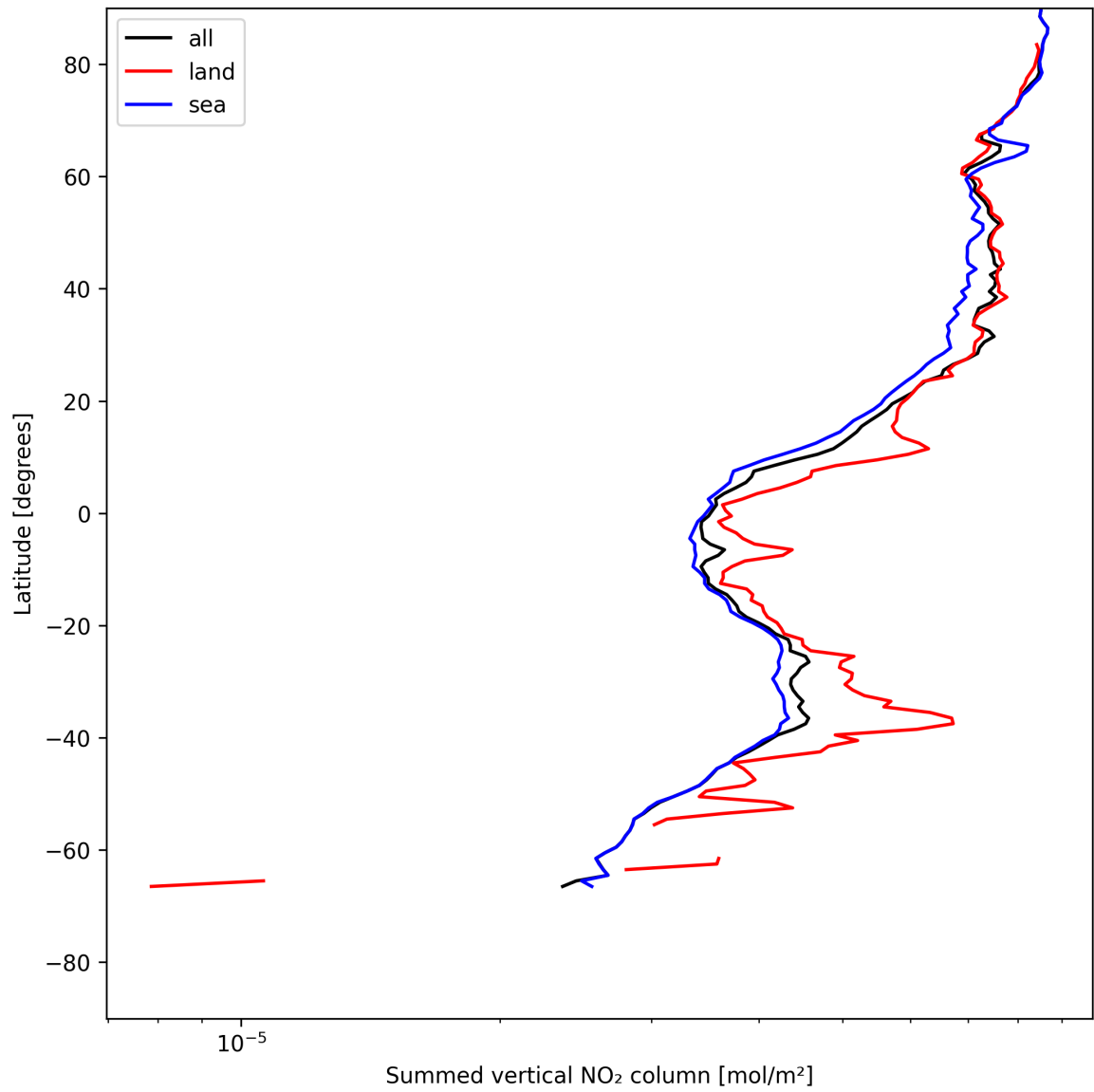
Figure 21: Zonal average of “Summed vertical NO 2 column” for 2025-05-23 to 2025-05-24.
