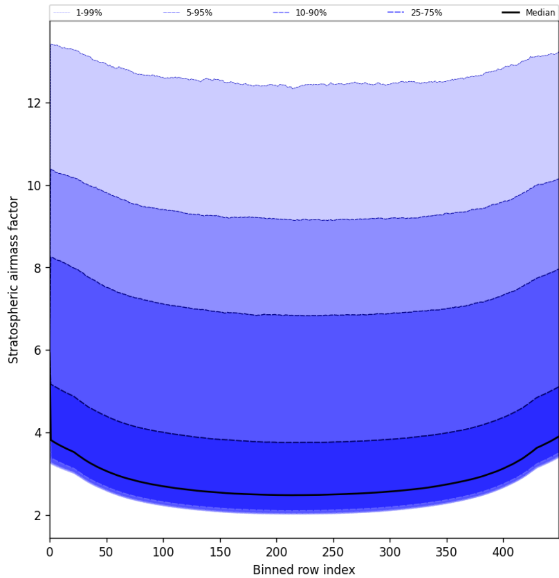
Figure 59: Along track statistics of “Stratospheric airmass factor” for 2025-05-23 to 2025-05-24
