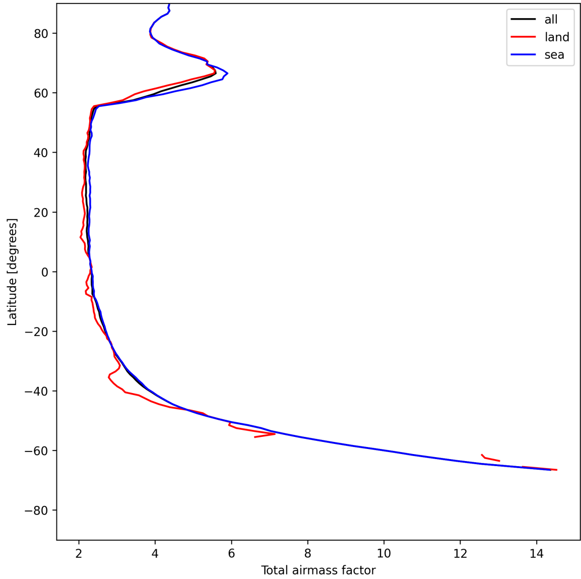
Figure 13: Zonal average of “Total airmass factor” for 2025-05-23 to 2025-05-24.
