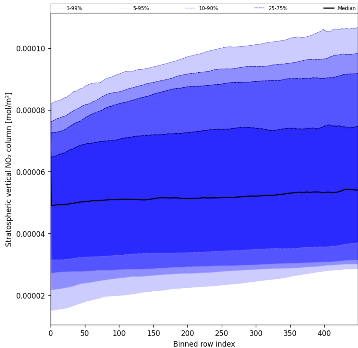
Figure 51: Along track statistics of “Stratospheric vertical NO 2 column” for 2025-05-23 to 2025-05-24
