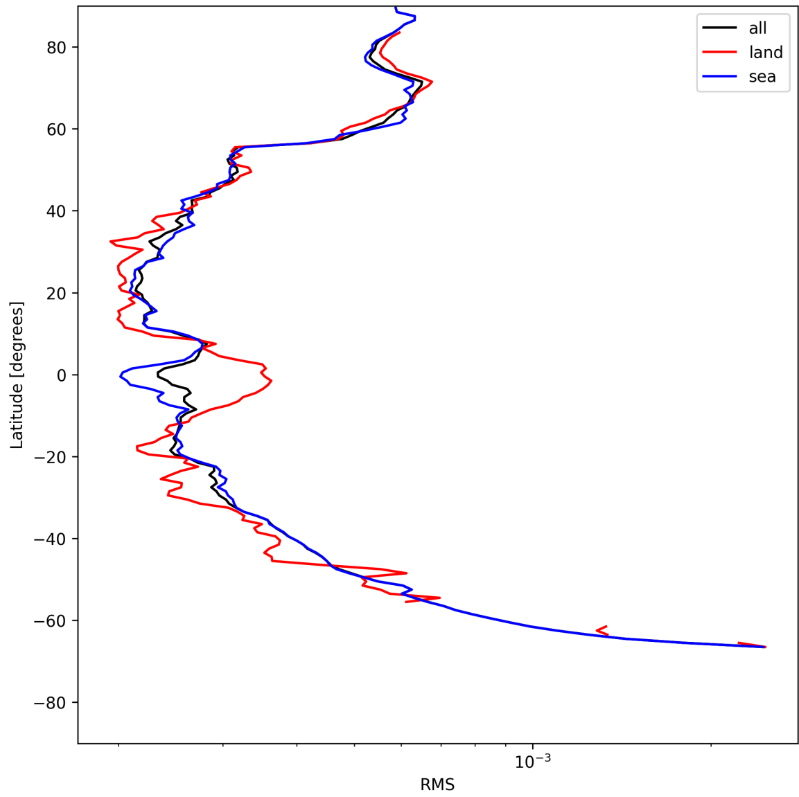
Figure 24: Zonal average of “RMS” for 2025-05-23 to 2025-05-24.
