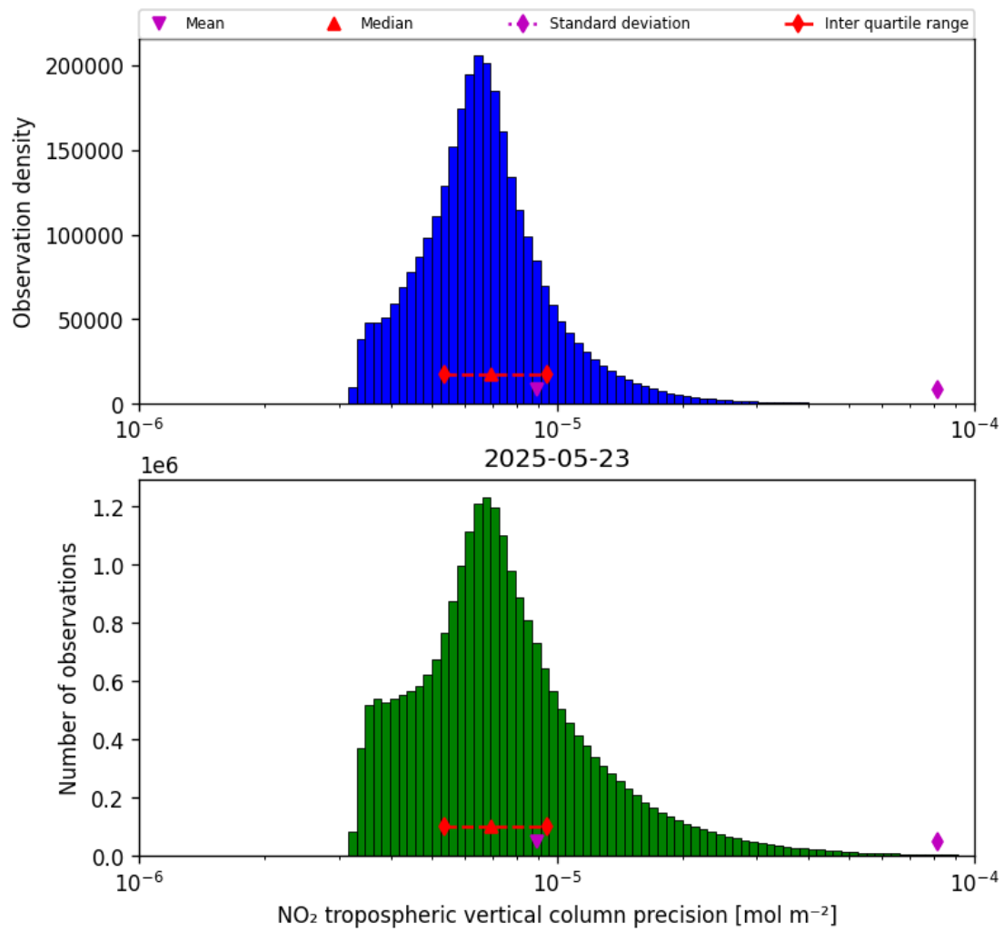
Figure 28: Histogram of “NO 2 tropospheric vertical column precision” for 2025-05-23 to 2025-05-24
