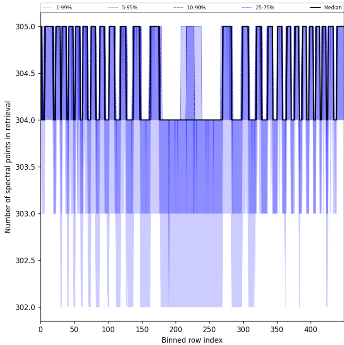
Figure 48: Along track statistics of “Number of spectral points in retrieval” for 2025-05-23 to 2025-05-24
