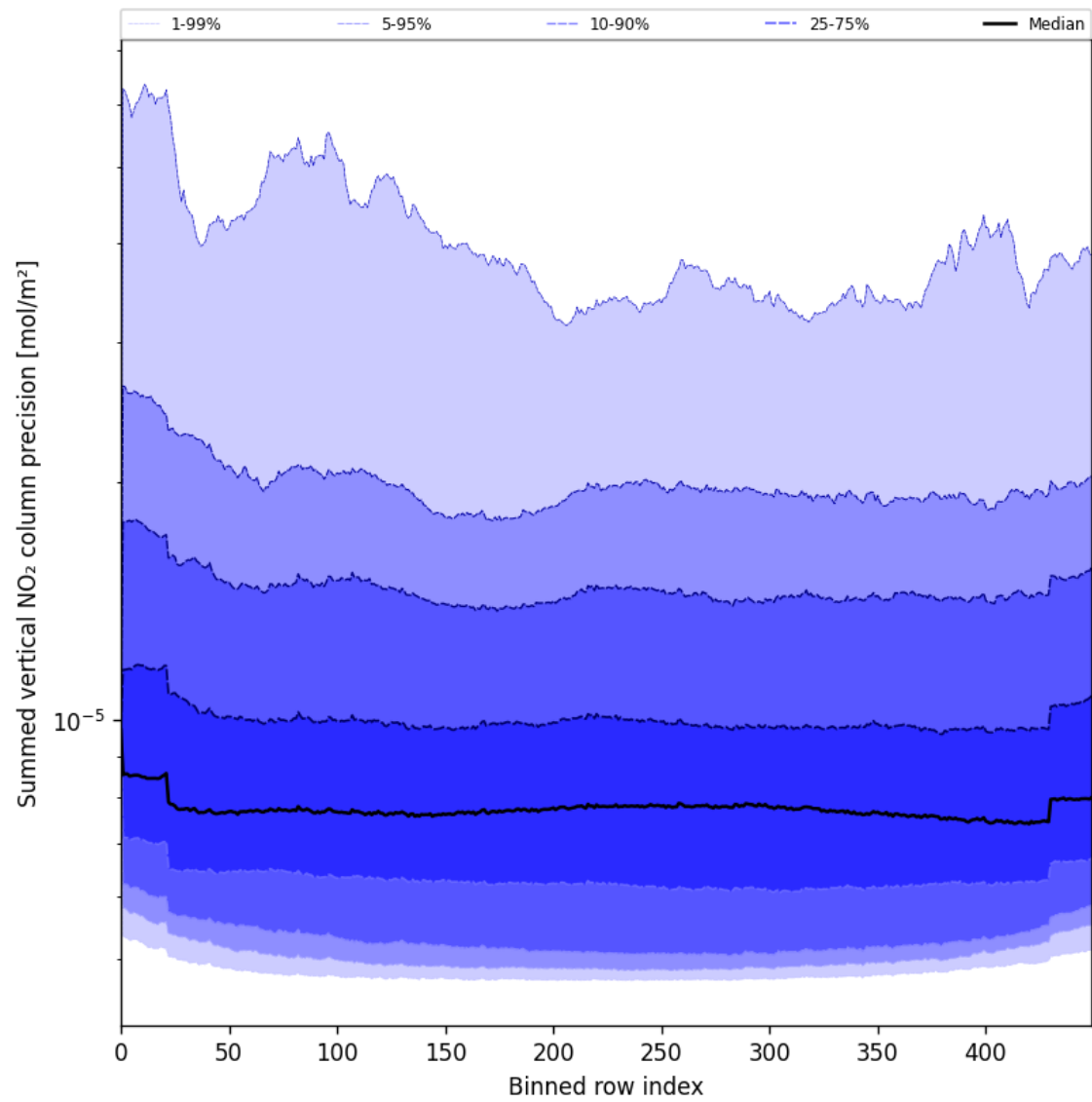
Figure 56: Along track statistics of “Summed vertical NO 2 column precision” for 2025-05-23 to 2025-05-24
