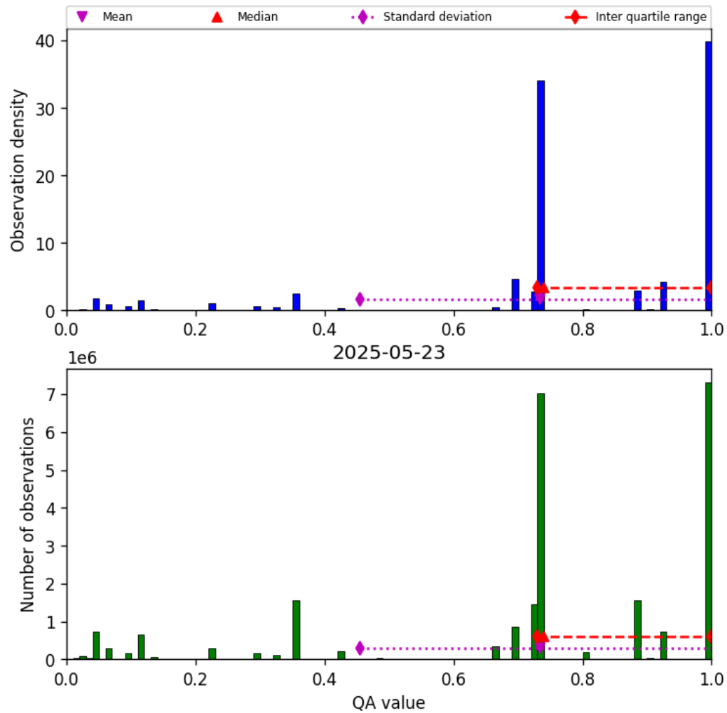
Figure 26: Histogram of “QA value” for 2025-05-23 to 2025-05-24
