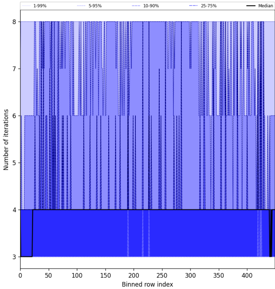
Figure 49: Along track statistics of “Number of iterations” for 2025-05-23 to 2025-05-24
