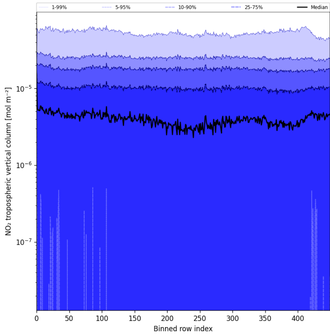
Figure 44: Along track statistics of “NO 2 tropospheric vertical column” for 2025-05-23 to 2025-05-24
