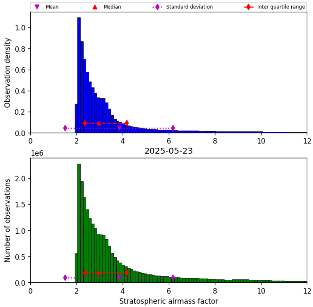
Figure 42: Histogram of “Stratospheric airmass factor” for 2025-05-23 to 2025-05-24
