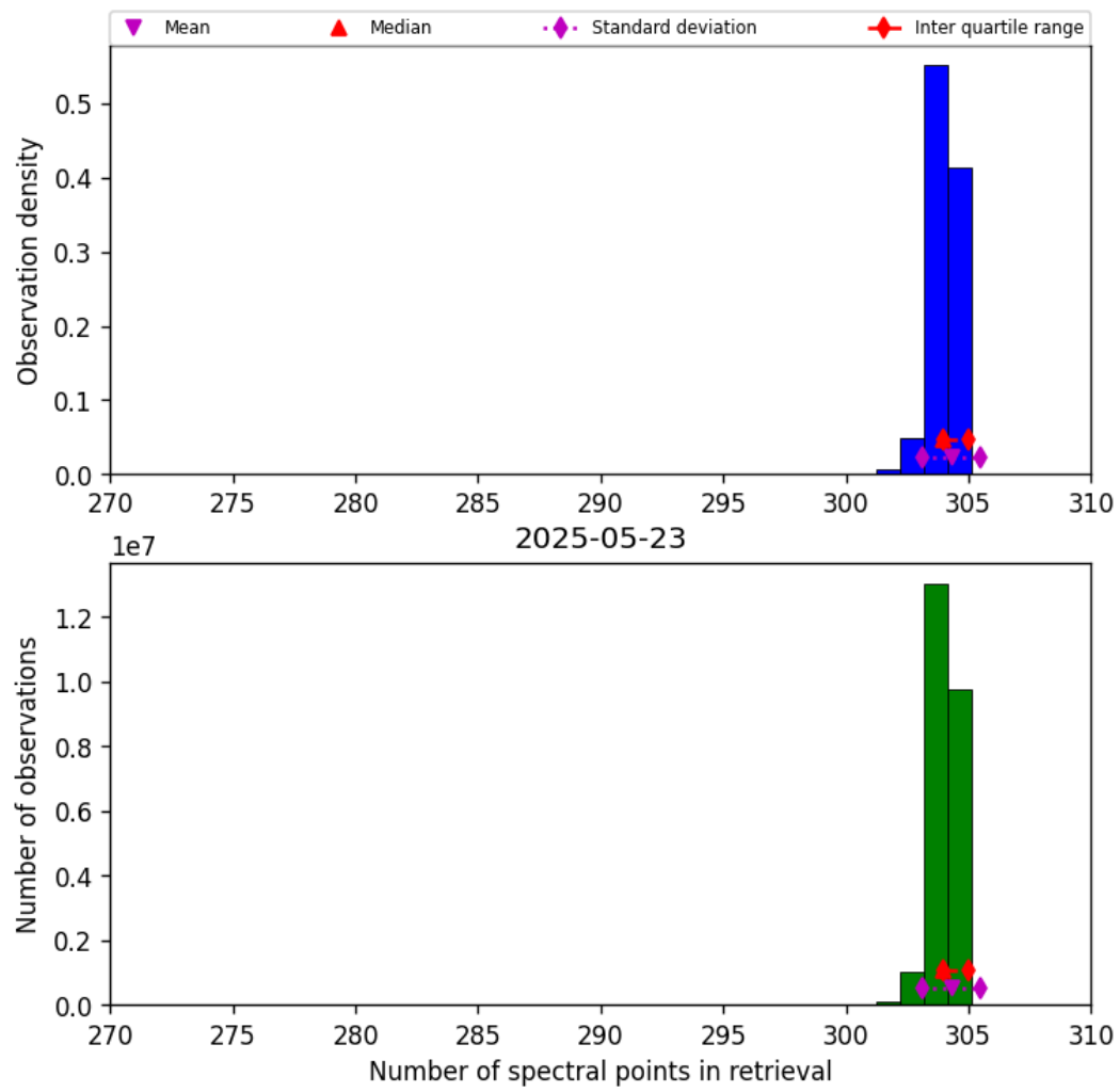
Figure 31: Histogram of “Number of spectral points in retrieval” for 2025-05-23 to 2025-05-24
