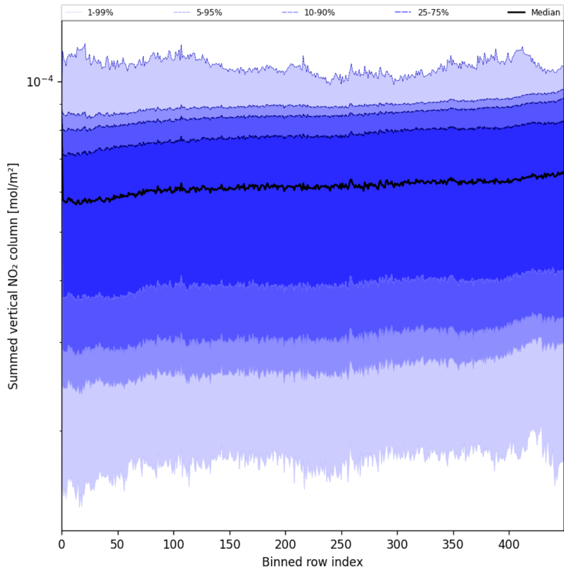
Figure 55: Along track statistics of “Summed vertical NO 2 column” for 2025-05-23 to 2025-05-24
