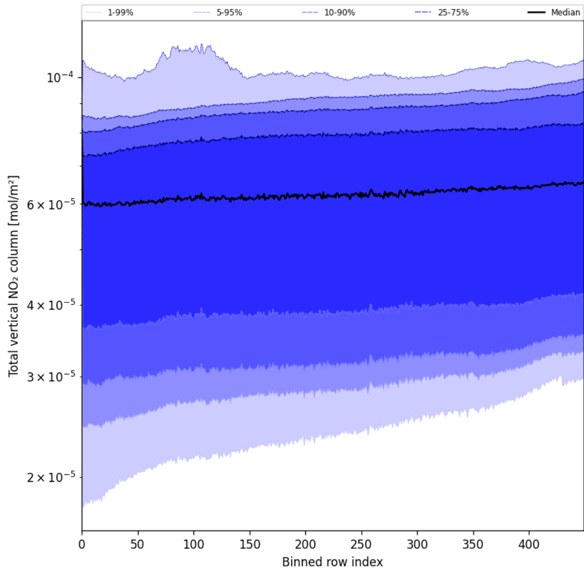
Figure 53: Along track statistics of “Total vertical NO 2 column” for 2025-05-23 to 2025-05-24
