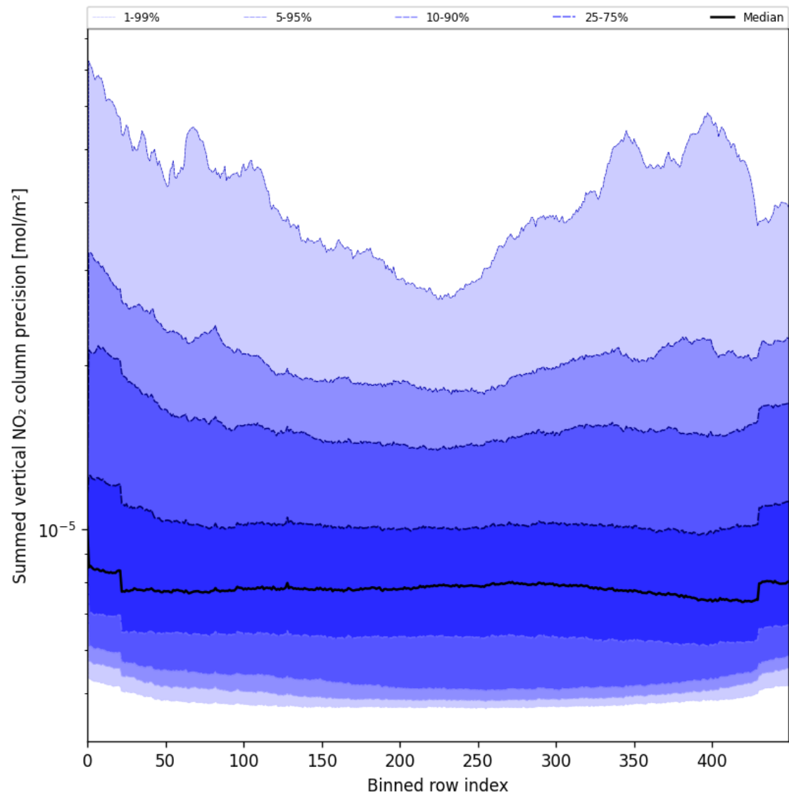
Figure 56: Along track statistics of “Summed vertical NO 2 column precision” for 2025-05-24 to 2025-05-24
