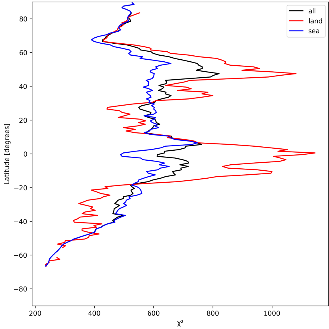
Figure 23: Zonal average of “ \chi^2 ” for 2025-05-24 to 2025-05-24.
