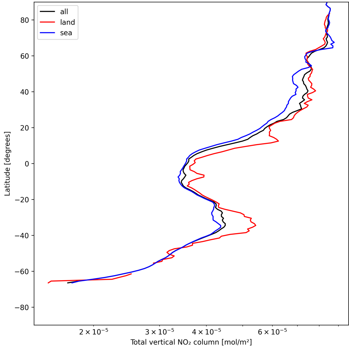
Figure 19: Zonal average of “Total vertical NO 2 column” for 2025-05-24 to 2025-05-24.
