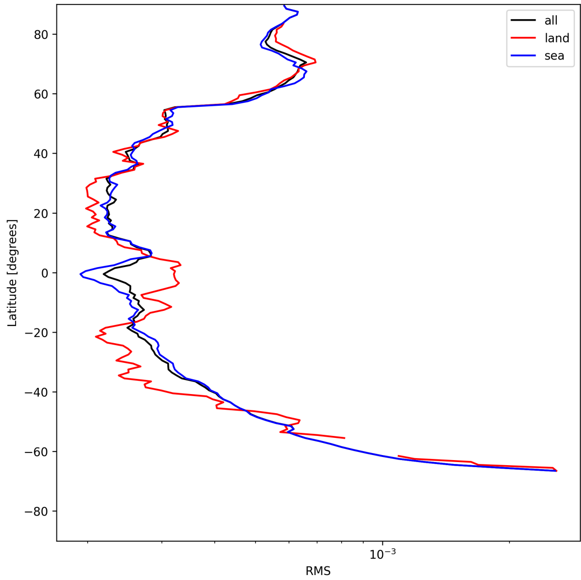
Figure 24: Zonal average of “RMS” for 2025-05-24 to 2025-05-24.
