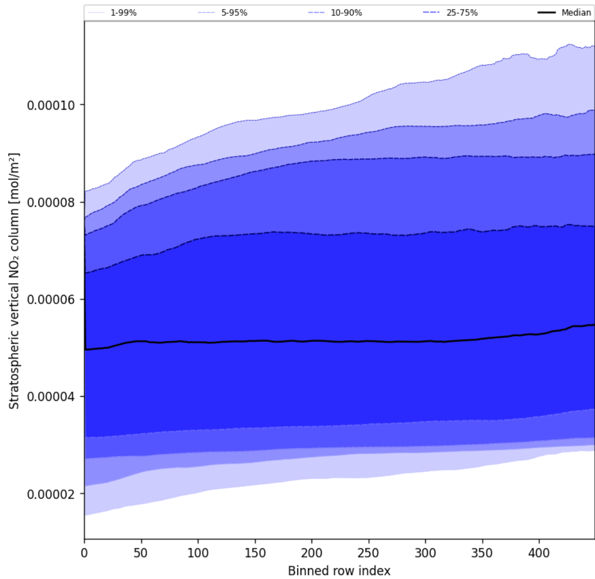
Figure 51: Along track statistics of “Stratospheric vertical NO 2 column” for 2025-05-24 to 2025-05-24
