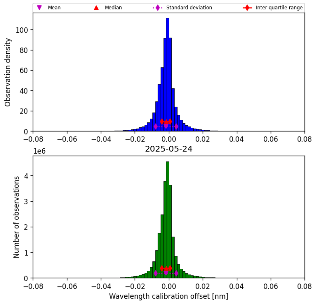
Figure 33: Histogram of “Wavelength calibration offset” for 2025-05-24 to 2025-05-24
