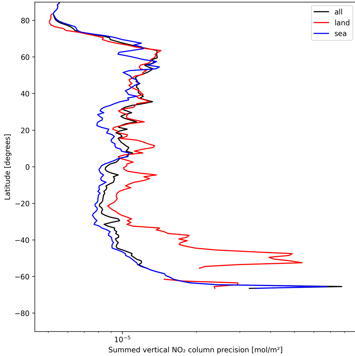
Figure 22: Zonal average of “Summed vertical NO 2 column precision” for 2025-05-24 to 2025-05-24.
