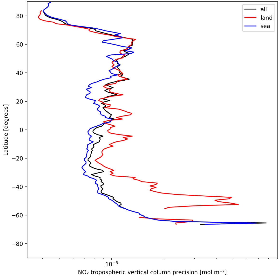
Figure 11: Zonal average of “NO 2 tropospheric vertical column precision” for 2025-05-24 to 2025-05-24.
