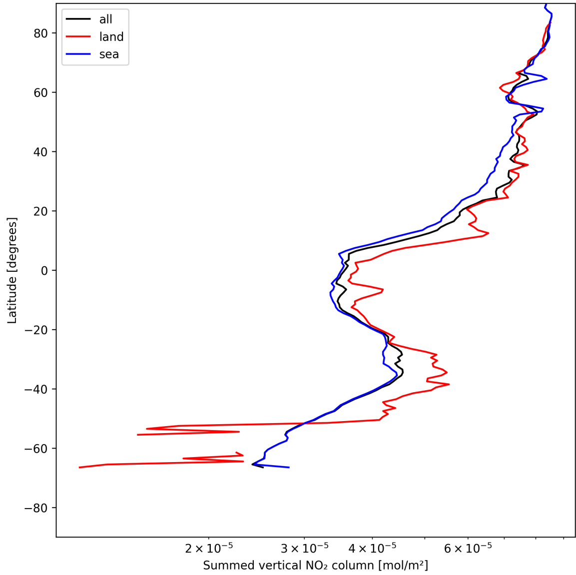
Figure 21: Zonal average of “Summed vertical NO 2 column” for 2025-05-24 to 2025-05-24.
