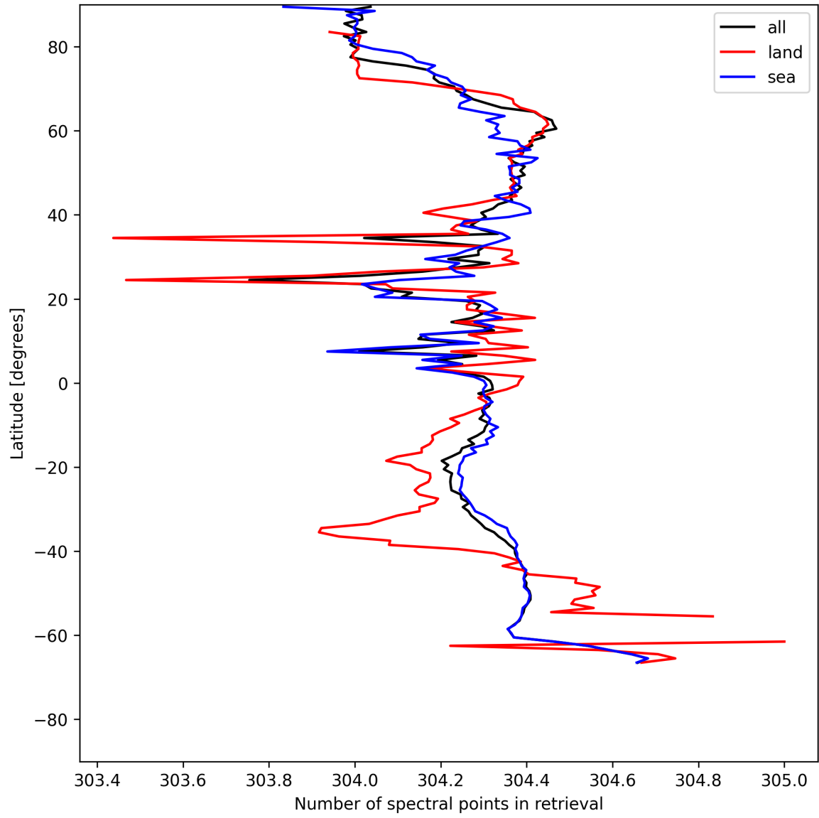
Figure 14: Zonal average of “Number of spectral points in retrieval” for 2025-05-24 to 2025-05-24.
