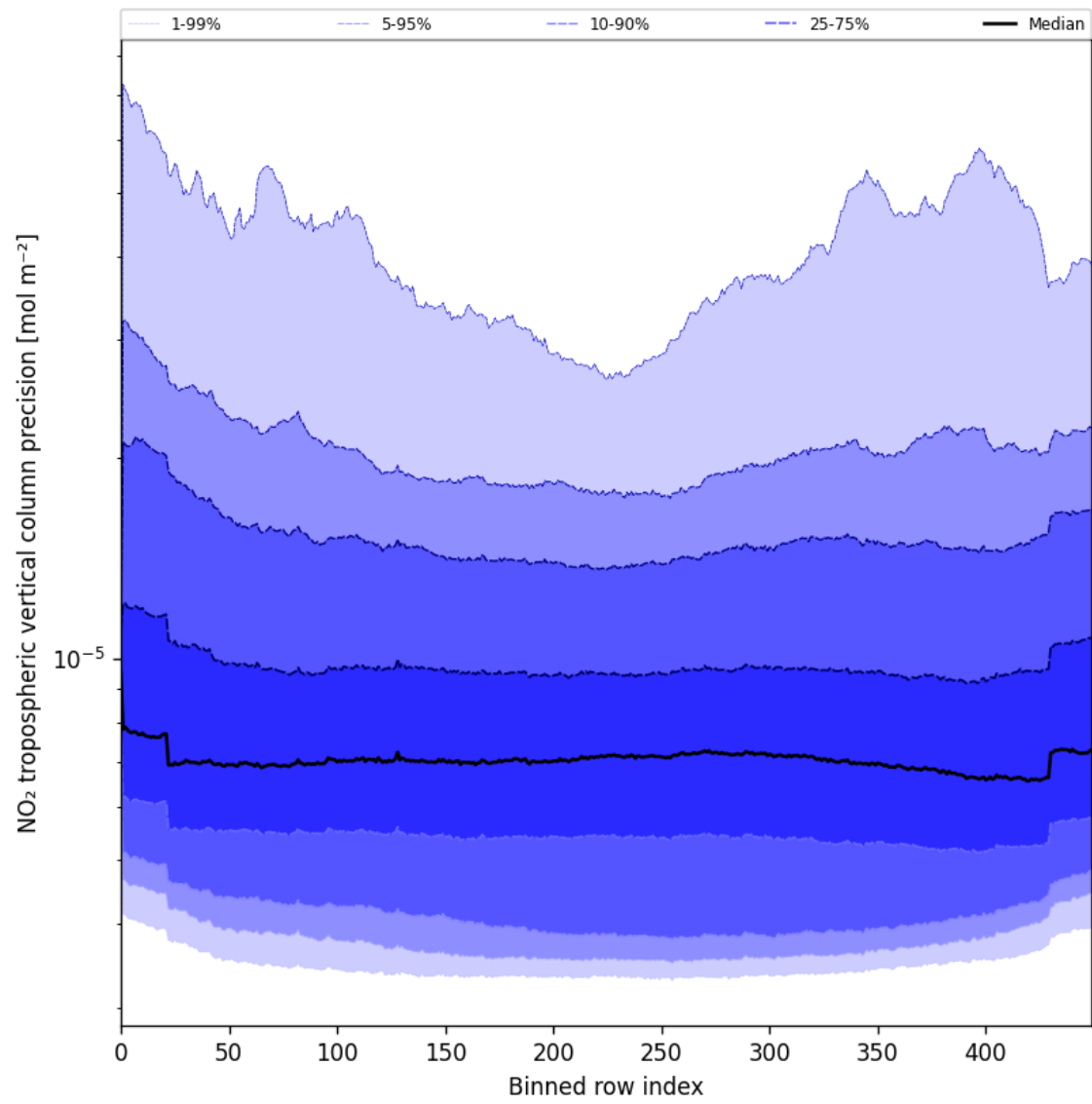
Figure 45: Along track statistics of “NO 2 tropospheric vertical column precision” for 2025-05-24 to 2025-05-24
