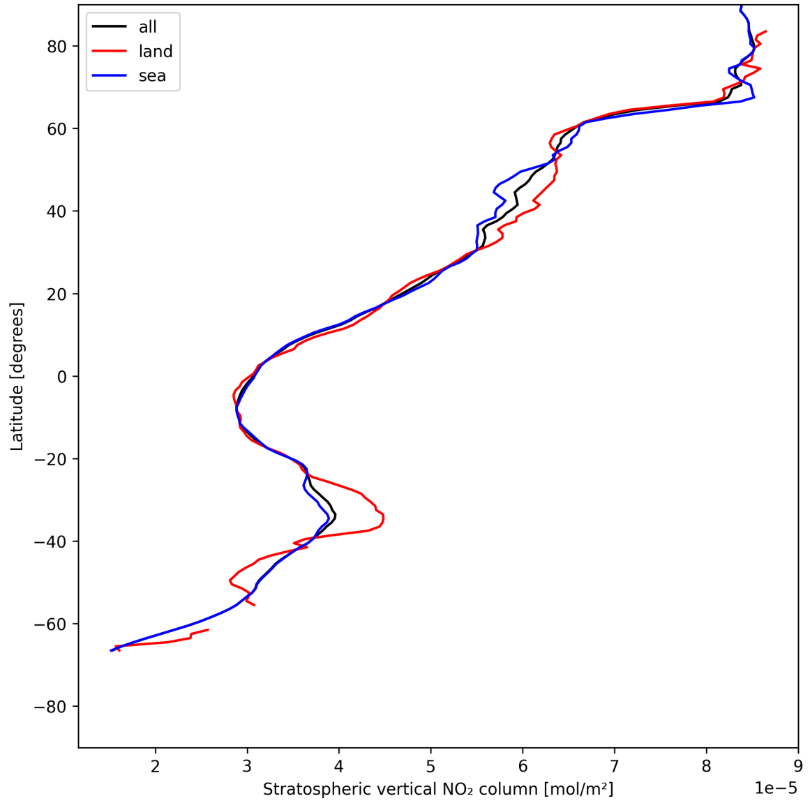
Figure 17: Zonal average of “Stratospheric vertical NO 2 column” for 2025-05-24 to 2025-05-24.
