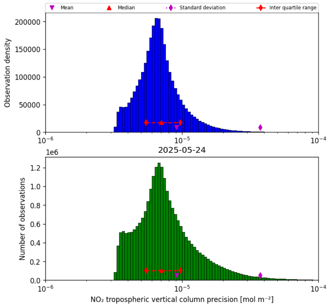
Figure 28: Histogram of “NO 2 tropospheric vertical column precision” for 2025-05-24 to 2025-05-24
