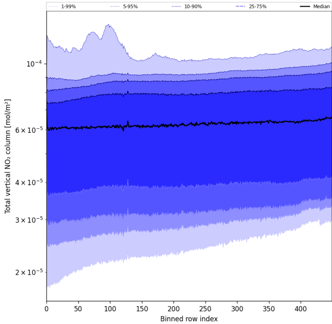
Figure 53: Along track statistics of “Total vertical NO 2 column” for 2025-05-24 to 2025-05-24
