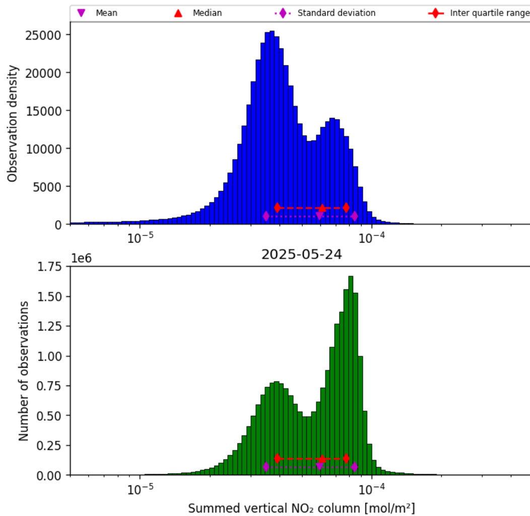
Figure 38: Histogram of “Summed vertical NO 2 column” for 2025-05-24 to 2025-05-24
