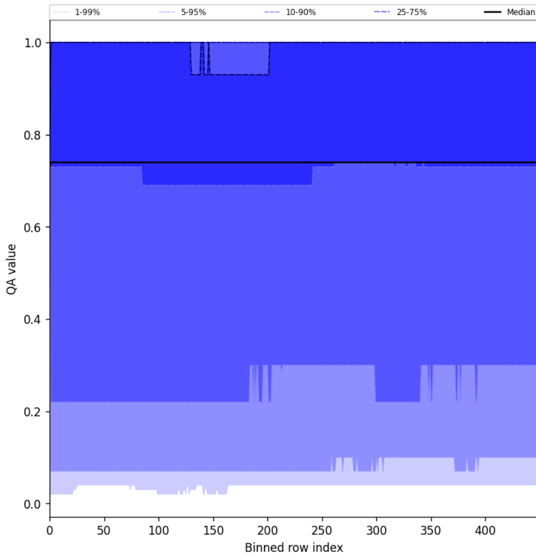
Figure 43: Along track statistics of “QA value” for 2025-05-24 to 2025-05-24
