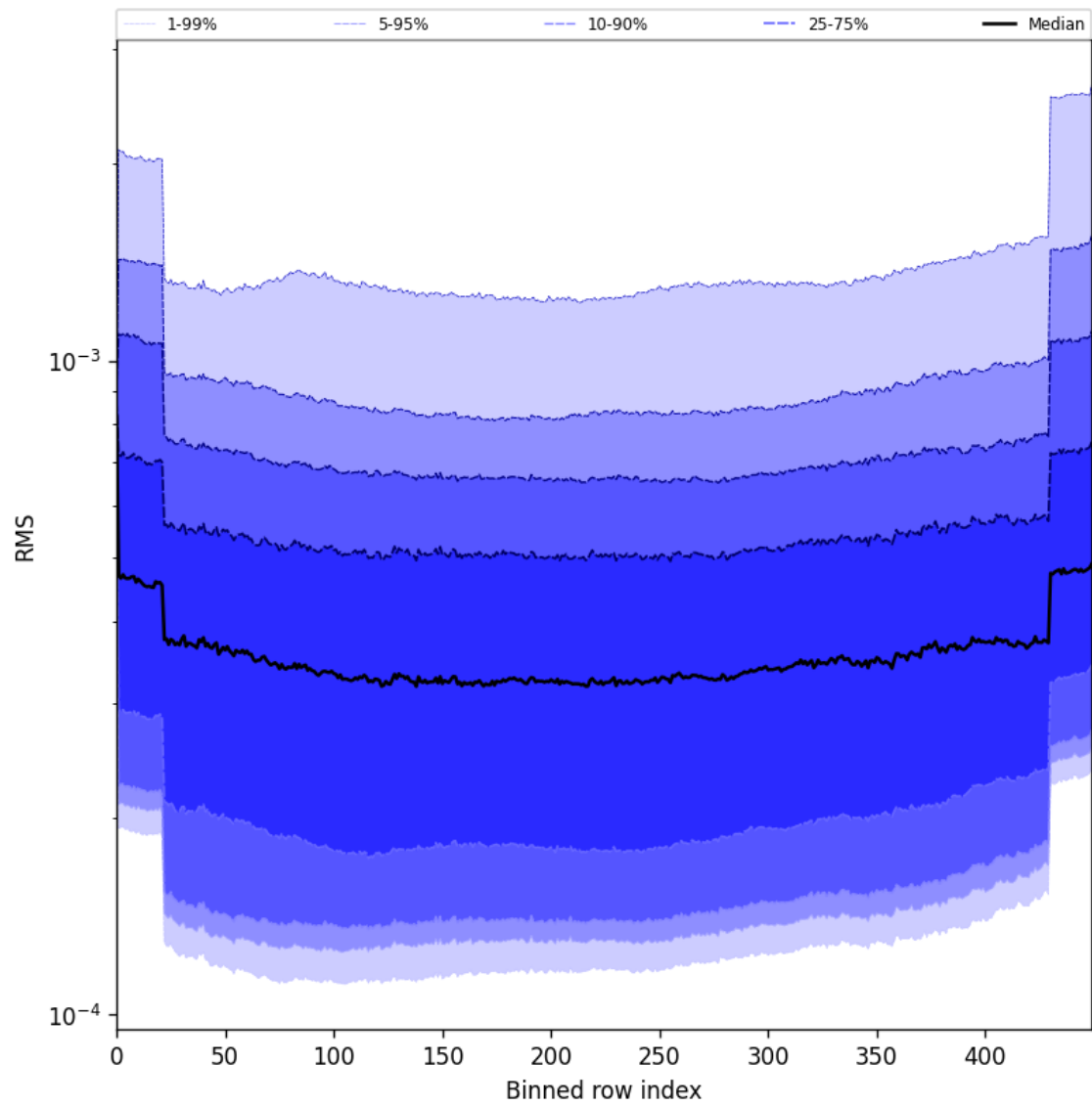
Figure 58: Along track statistics of “RMS” for 2025-05-24 to 2025-05-24
