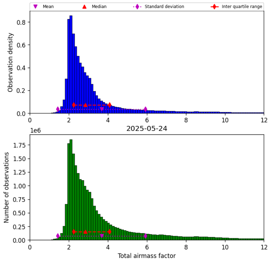
Figure 30: Histogram of “Total airmass factor” for 2025-05-24 to 2025-05-24
