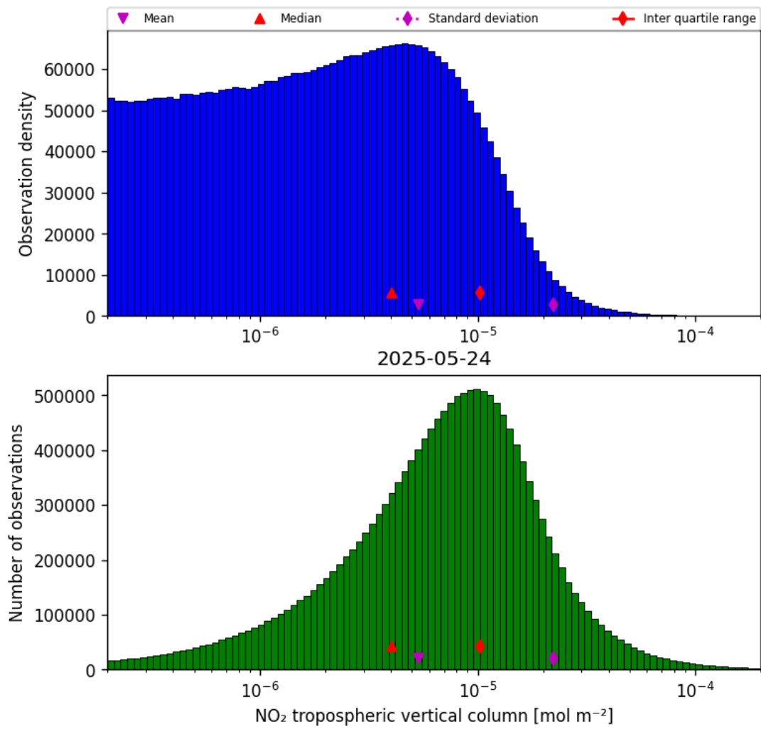
Figure 27: Histogram of “ \text{NO}_2 tropospheric vertical column” for 2025-05-24 to 2025-05-24
