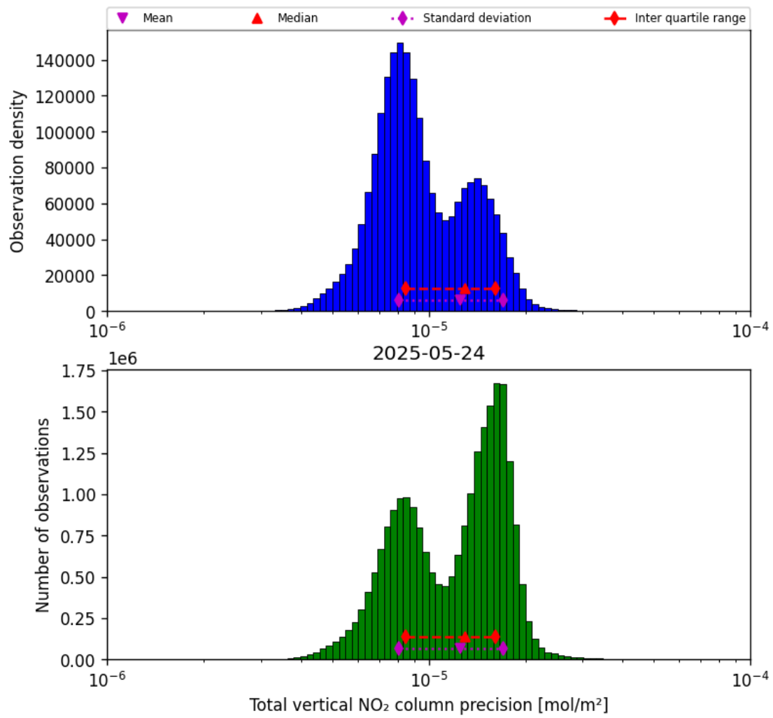
Figure 37: Histogram of “Total vertical NO 2 column precision” for 2025-05-24 to 2025-05-24
