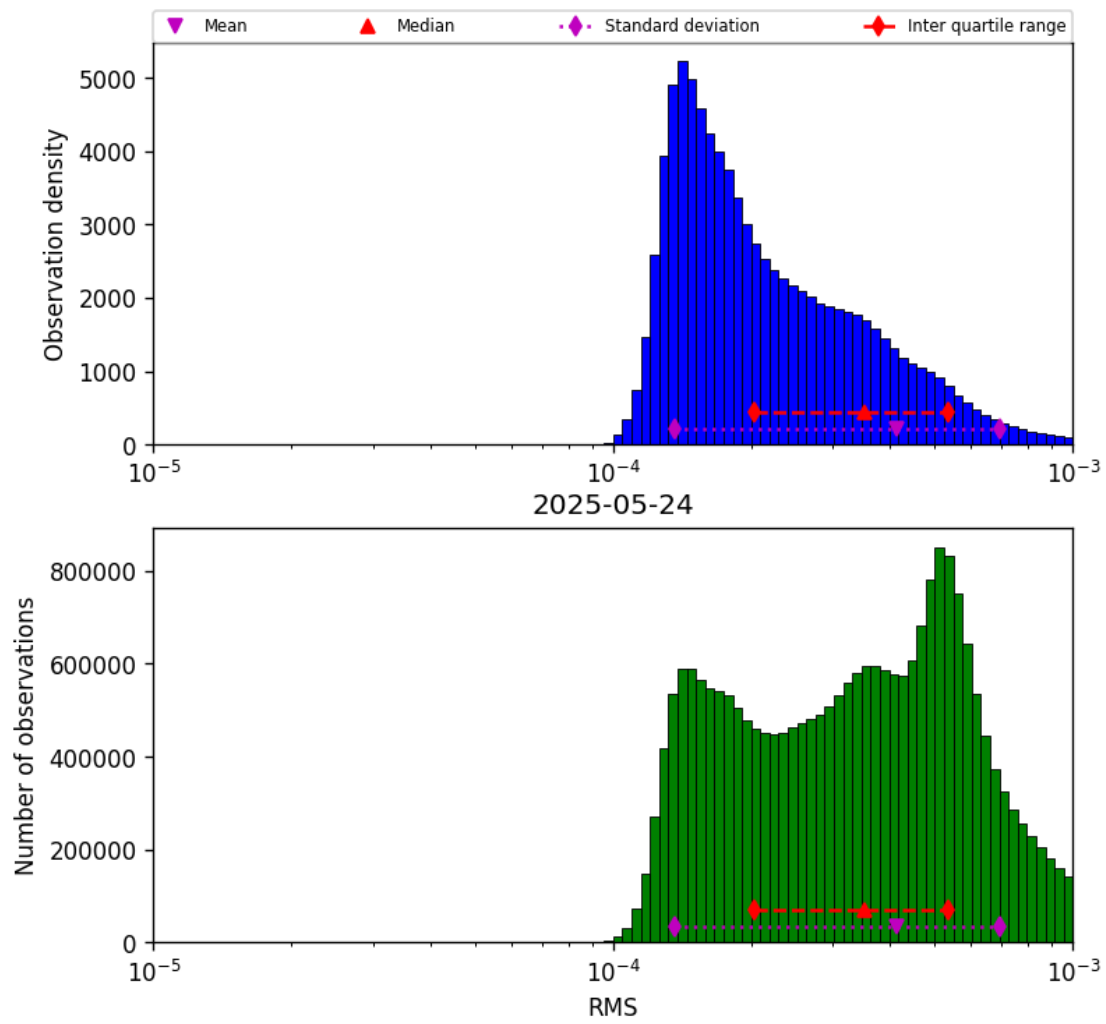
Figure 41: Histogram of “RMS” for 2025-05-24 to 2025-05-24
