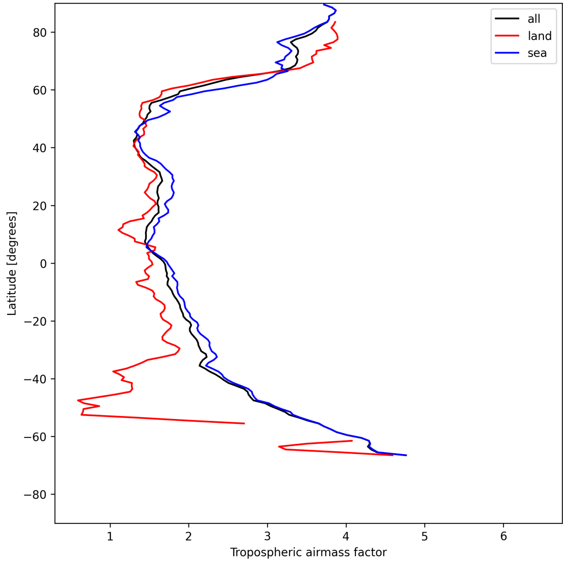
Figure 12: Zonal average of “Tropospheric airmass factor” for 2025-05-24 to 2025-05-24.
