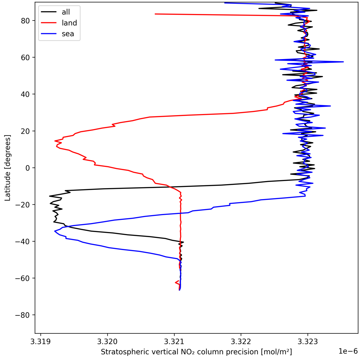
Figure 18: Zonal average of “Stratospheric vertical NO 2 column precision” for 2025-05-24 to 2025-05-24.
