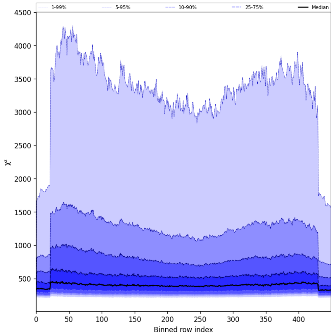
Figure 57: Along track statistics of “ \chi^2 ” for 2025-05-24 to 2025-05-24
