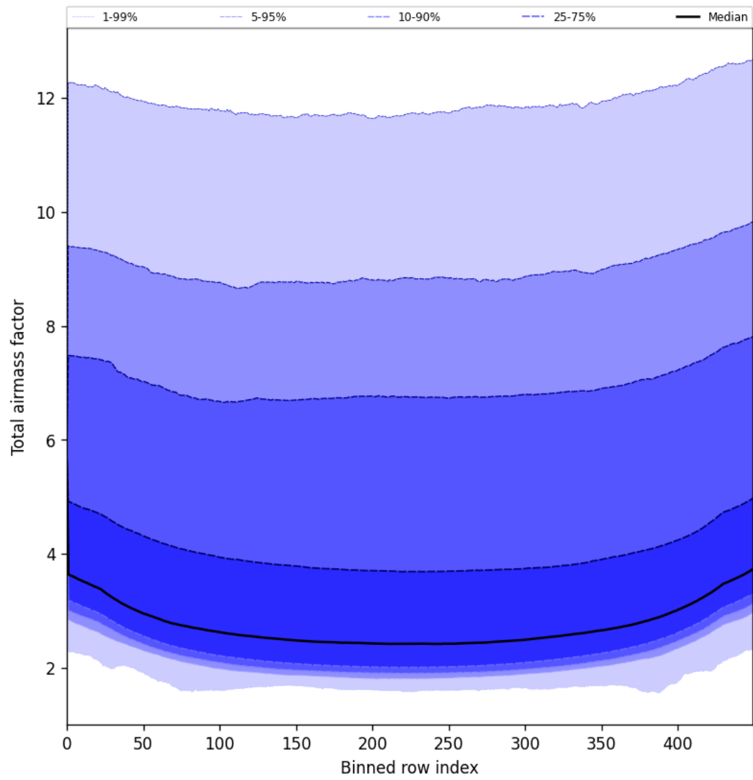
Figure 47: Along track statistics of “Total airmass factor” for 2025-05-24 to 2025-05-24
