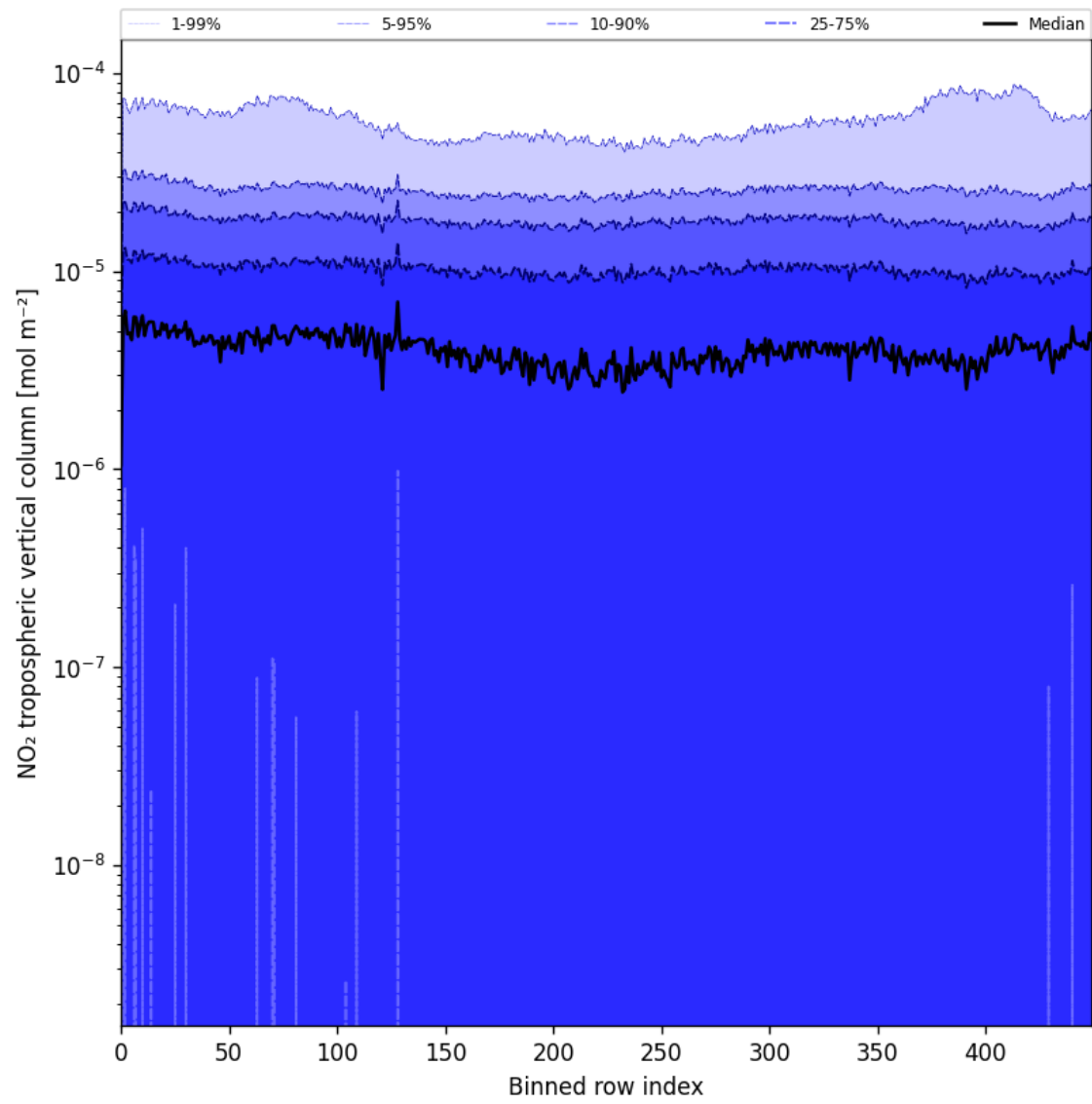
Figure 44: Along track statistics of “NO 2 tropospheric vertical column” for 2025-05-24 to 2025-05-24
