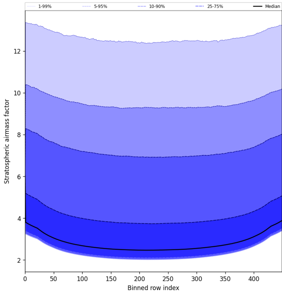
Figure 59: Along track statistics of “Stratospheric airmass factor” for 2025-05-24 to 2025-05-24
