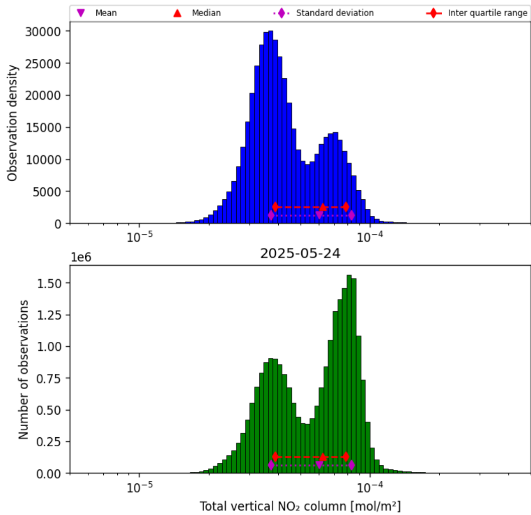
Figure 36: Histogram of "Total vertical NO 2 column" for 2025-05-24 to 2025-05-24
