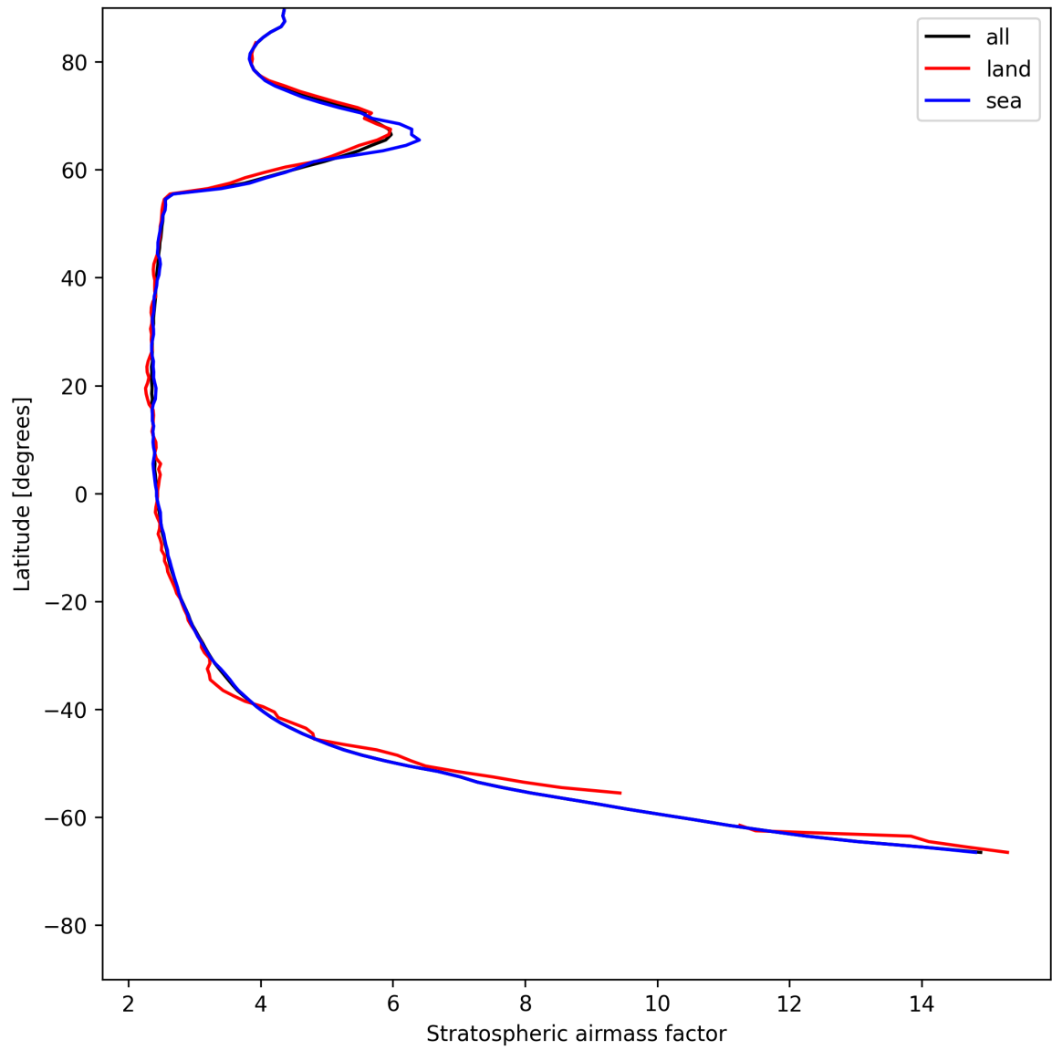
Figure 25: Zonal average of “Stratospheric airmass factor” for 2025-05-24 to 2025-05-24.
