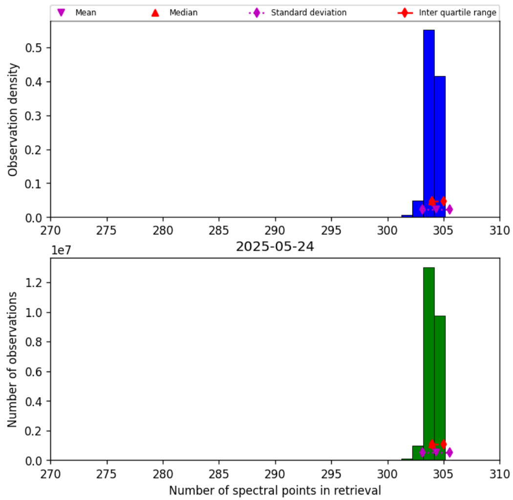
Figure 31: Histogram of “Number of spectral points in retrieval” for 2025-05-24 to 2025-05-24
