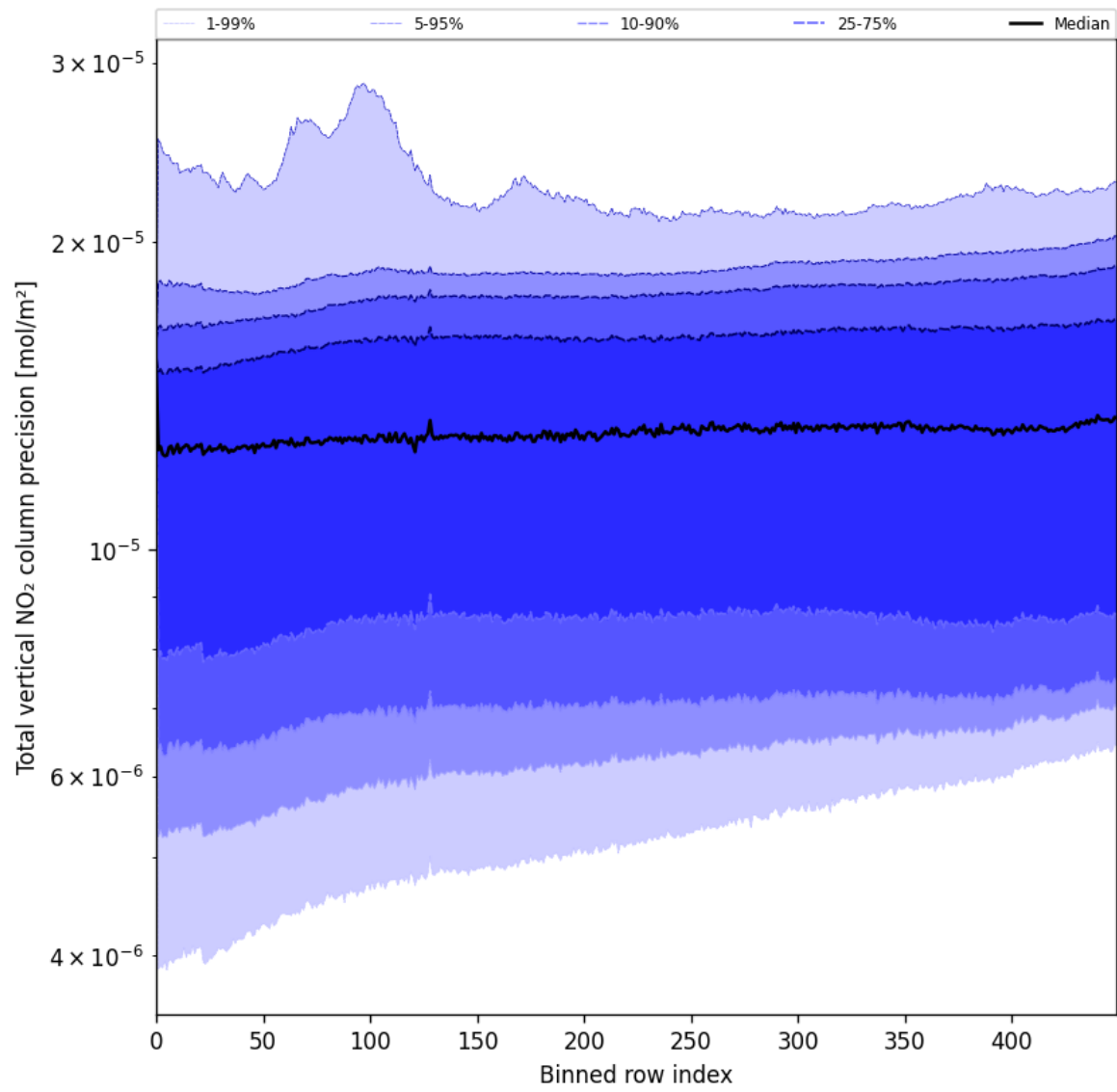
Figure 54: Along track statistics of "Total vertical NO 2 column precision" for 2025-05-24 to 2025-05-24
