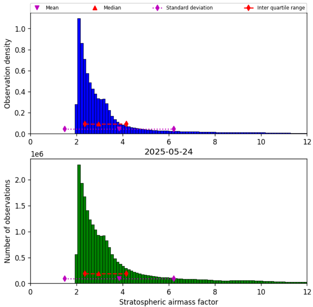
Figure 42: Histogram of “Stratospheric airmass factor” for 2025-05-24 to 2025-05-24
