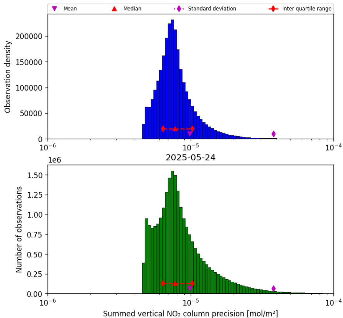
Figure 39: Histogram of "Summed vertical NO 2 column precision" for 2025-05-24 to 2025-05-24
