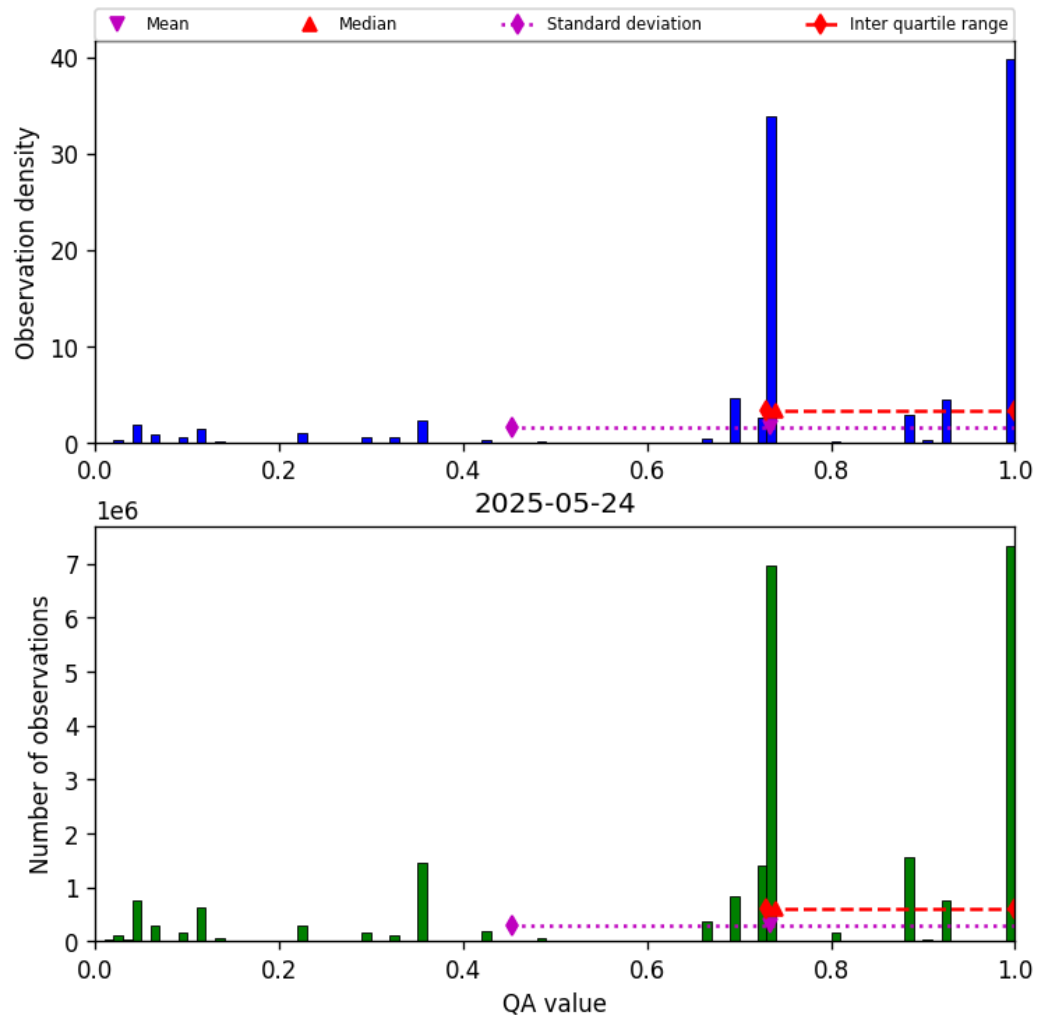
Figure 26: Histogram of “QA value” for 2025-05-24 to 2025-05-24
