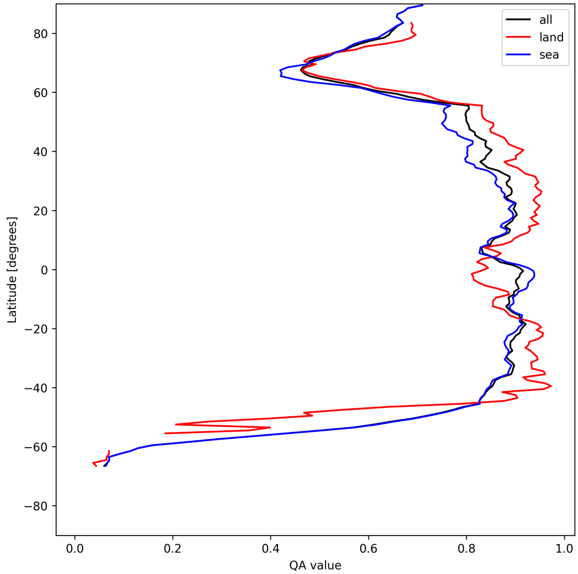
Figure 9: Zonal average of “QA value” for 2025-05-24 to 2025-05-24.
