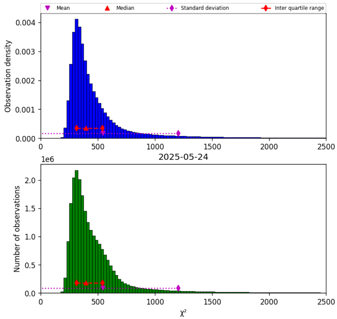
Figure 40: Histogram of “ \chi^2 ” for 2025-05-24 to 2025-05-24
