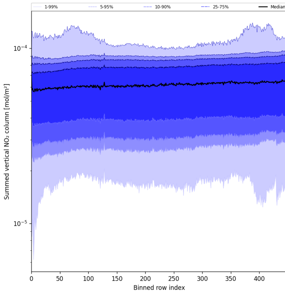
Figure 55: Along track statistics of “Summed vertical NO 2 column” for 2025-05-24 to 2025-05-24
