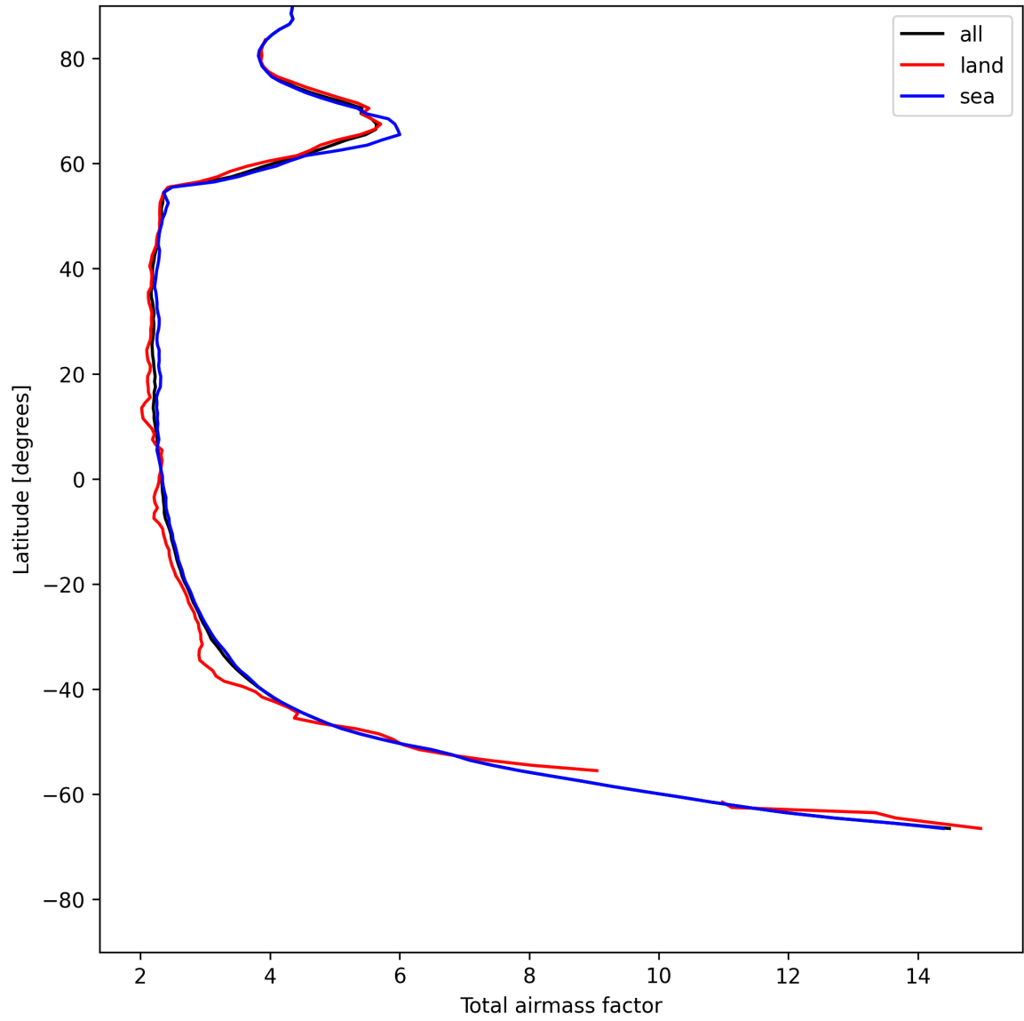
Figure 13: Zonal average of “Total airmass factor” for 2025-05-24 to 2025-05-24.
