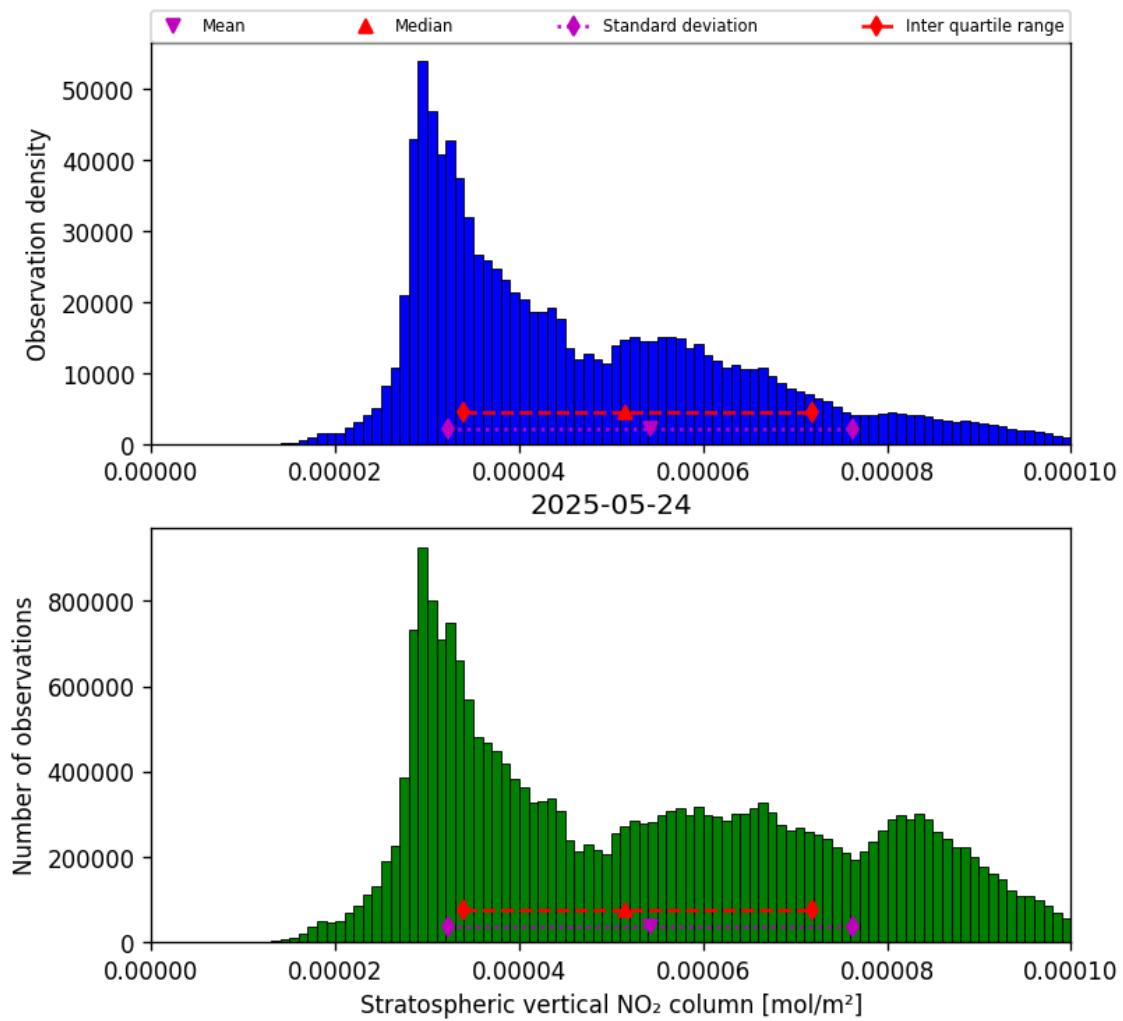
Figure 34: Histogram of “Stratospheric vertical NO 2 column” for 2025-05-24 to 2025-05-24
