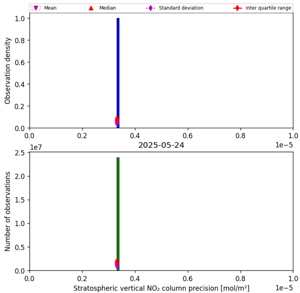
Figure 35: Histogram of “Stratospheric vertical NO 2 column precision” for 2025-05-24 to 2025-05-24
