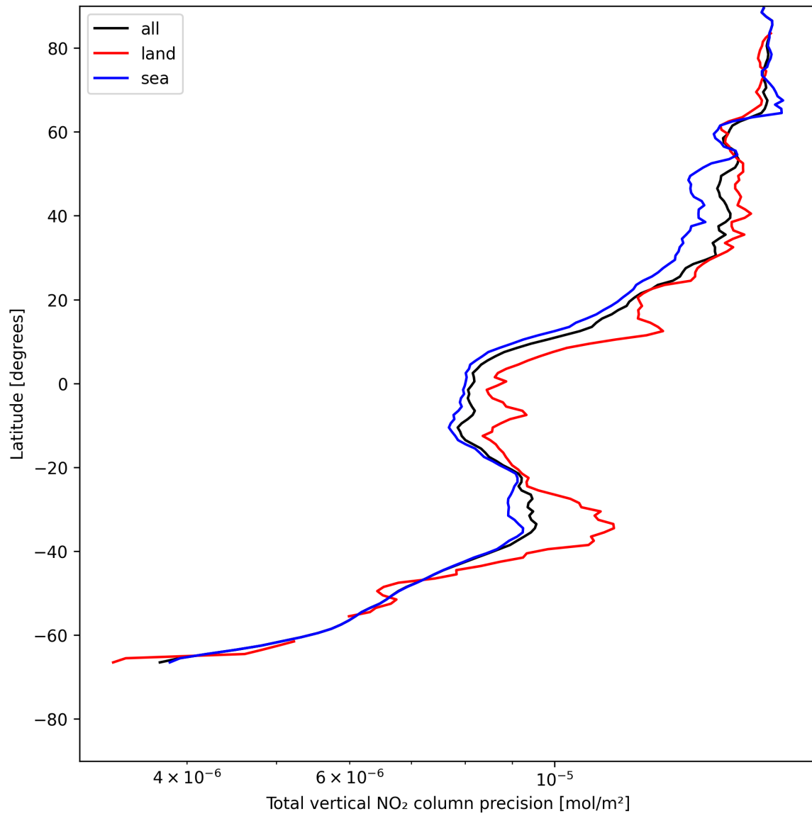
Figure 20: Zonal average of “Total vertical NO 2 column precision” for 2025-05-24 to 2025-05-24.
