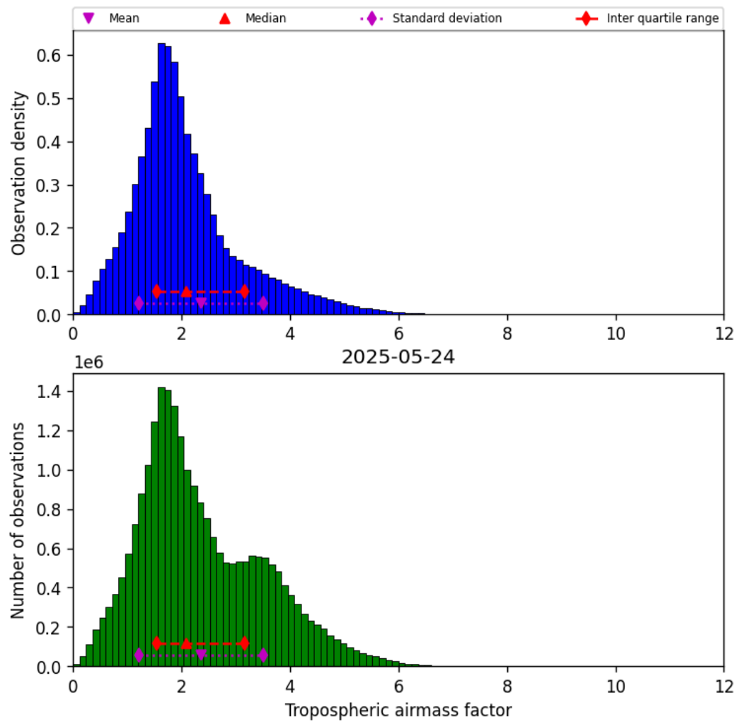
Figure 29: Histogram of “Tropospheric airmass factor” for 2025-05-24 to 2025-05-24
