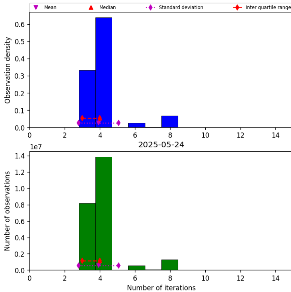
Figure 32: Histogram of “Number of iterations” for 2025-05-24 to 2025-05-24
