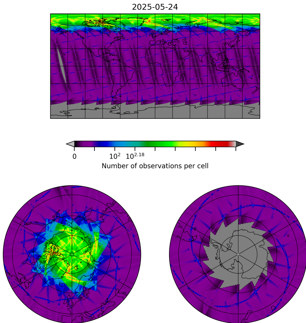
Figure 8: Map of the number of observations for 2025-05-24 to 2025-05-24
