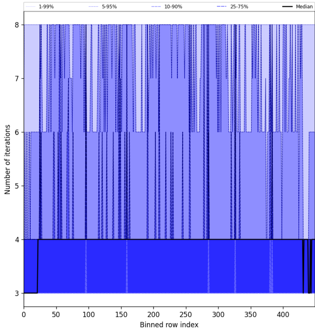
Figure 49: Along track statistics of “Number of iterations” for 2025-05-24 to 2025-05-24
