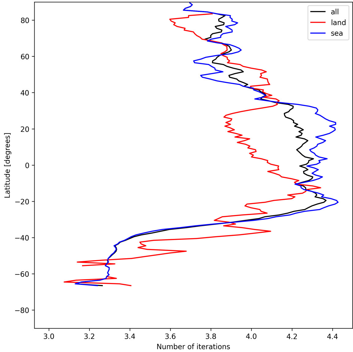
Figure 15: Zonal average of “Number of iterations” for 2025-05-24 to 2025-05-24.
