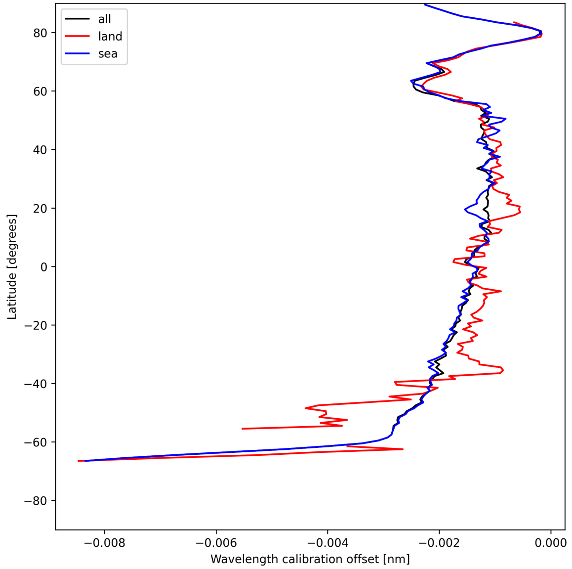
Figure 16: Zonal average of “Wavelength calibration offset” for 2025-05-24 to 2025-05-24.
