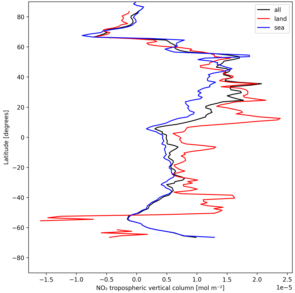
Figure 10: Zonal average of “NO 2 tropospheric vertical column” for 2025-05-24 to 2025-05-24.
