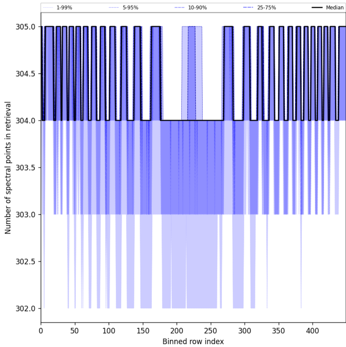
Figure 48: Along track statistics of “Number of spectral points in retrieval” for 2025-05-24 to 2025-05-24
