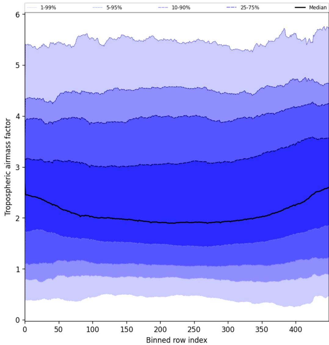
Figure 46: Along track statistics of “Tropospheric airmass factor” for 2025-05-24 to 2025-05-24
