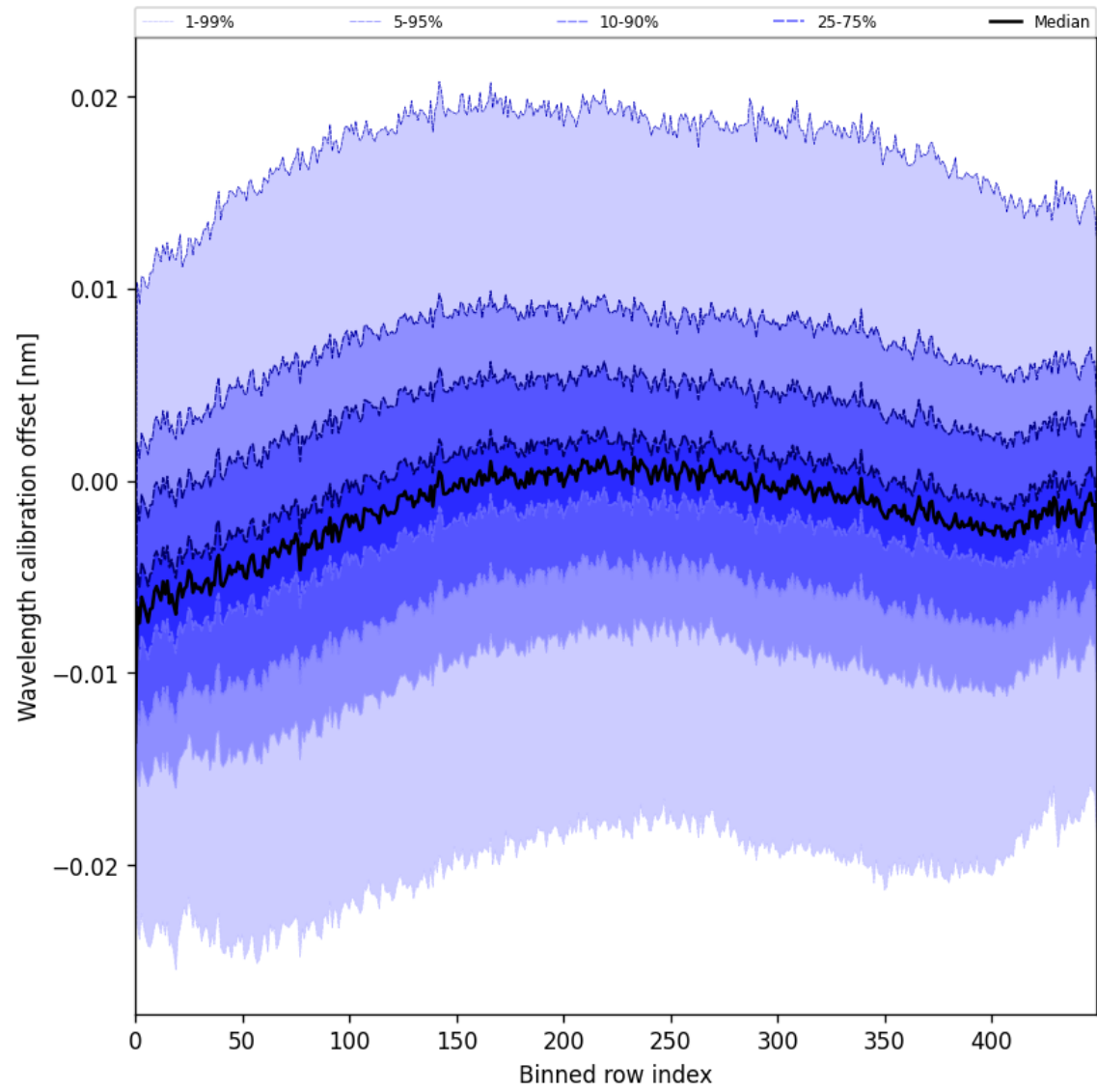
Figure 50: Along track statistics of “Wavelength calibration offset” for 2025-05-24 to 2025-05-24
