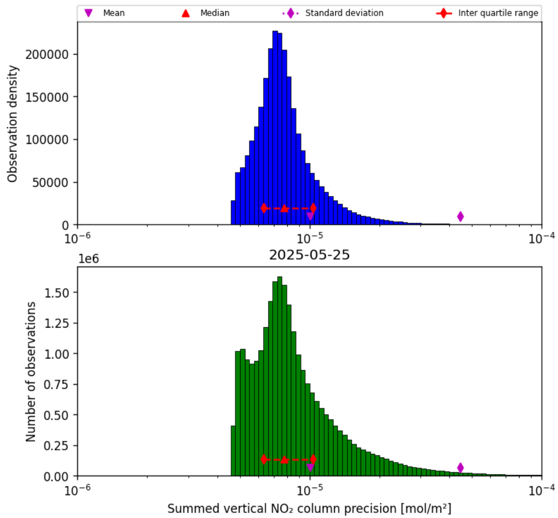
Figure 39: Histogram of “Summed vertical NO 2 column precision” for 2025-05-25 to 2025-05-26
