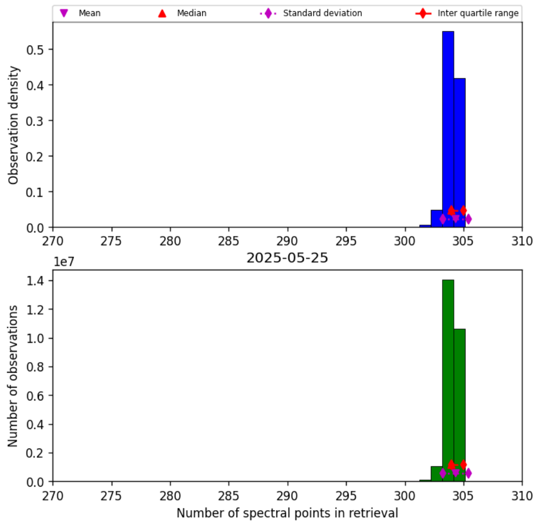
Figure 31: Histogram of “Number of spectral points in retrieval” for 2025-05-25 to 2025-05-26
