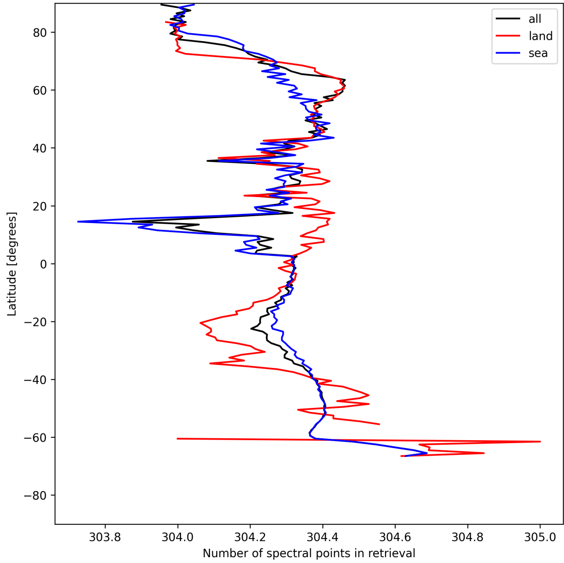
Figure 14: Zonal average of “Number of spectral points in retrieval” for 2025-05-25 to 2025-05-26.
