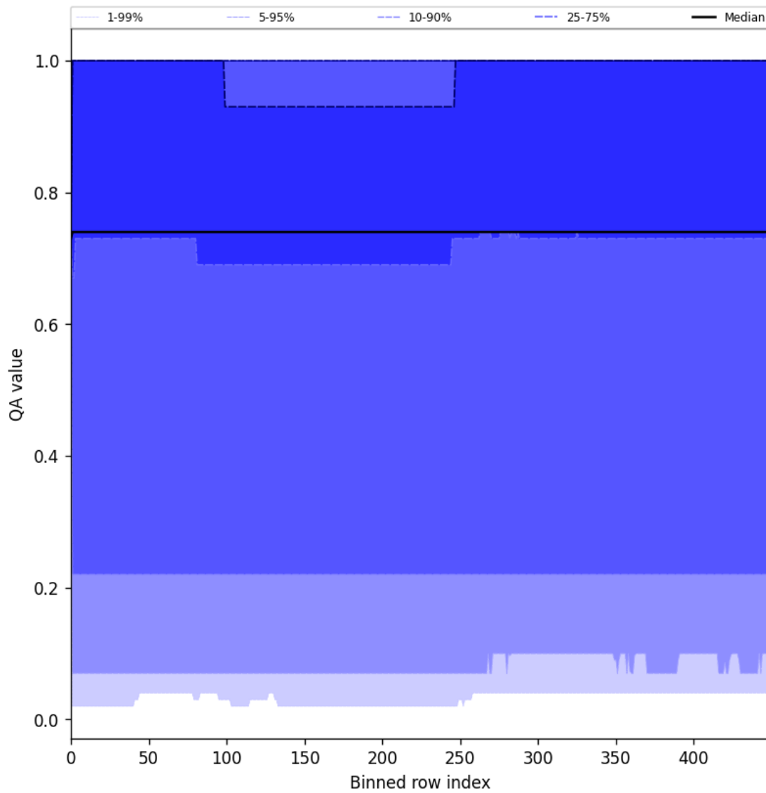
Figure 43: Along track statistics of "QA value" for 2025-05-25 to 2025-05-26
