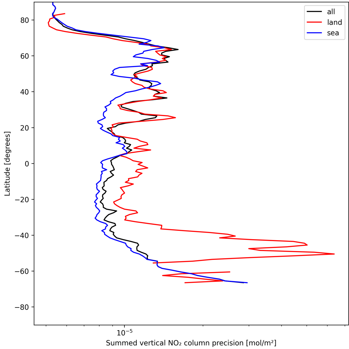
Figure 22: Zonal average of “Summed vertical NO 2 column precision” for 2025-05-25 to 2025-05-26.
