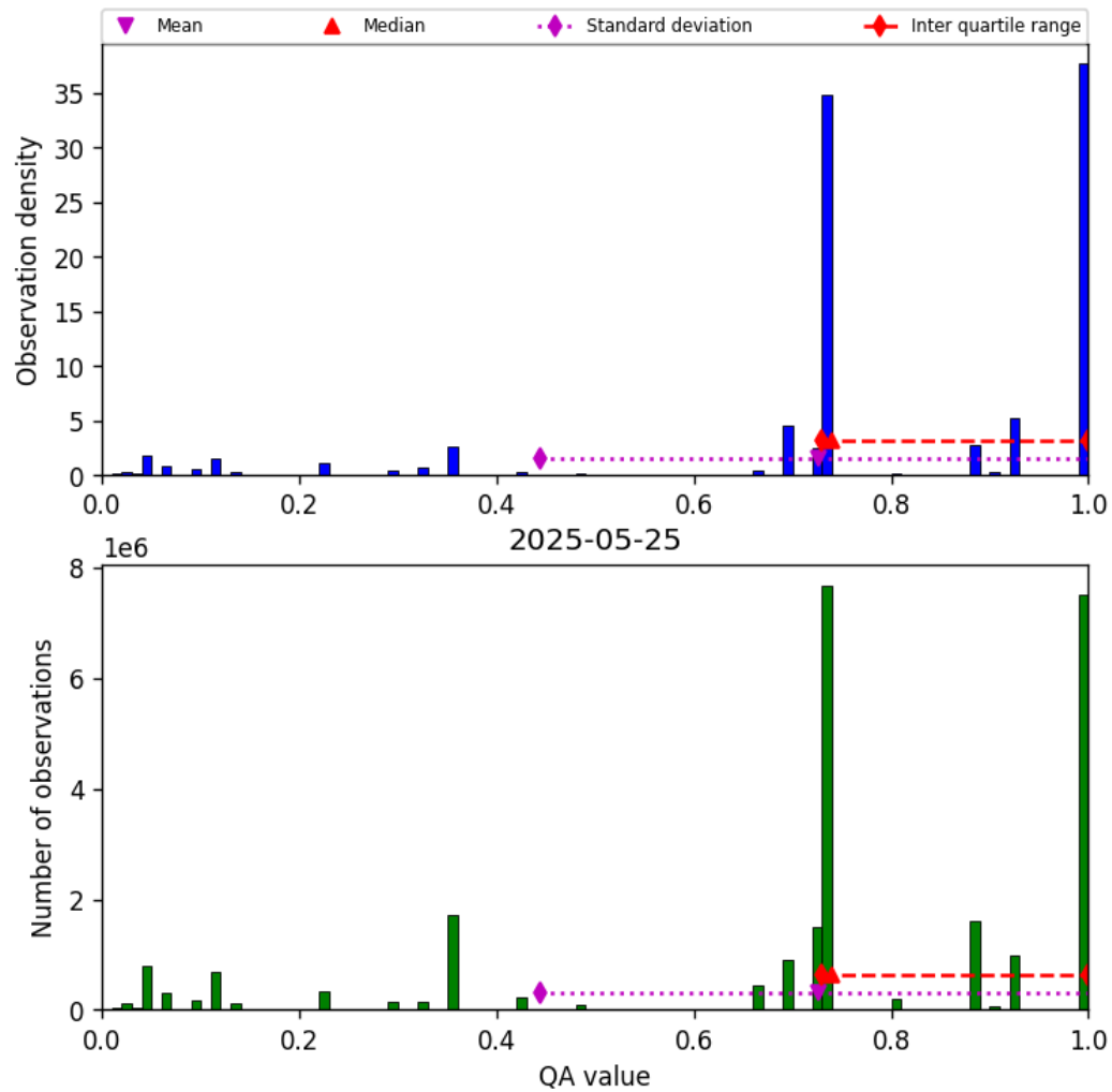
Figure 26: Histogram of “QA value” for 2025-05-25 to 2025-05-26
