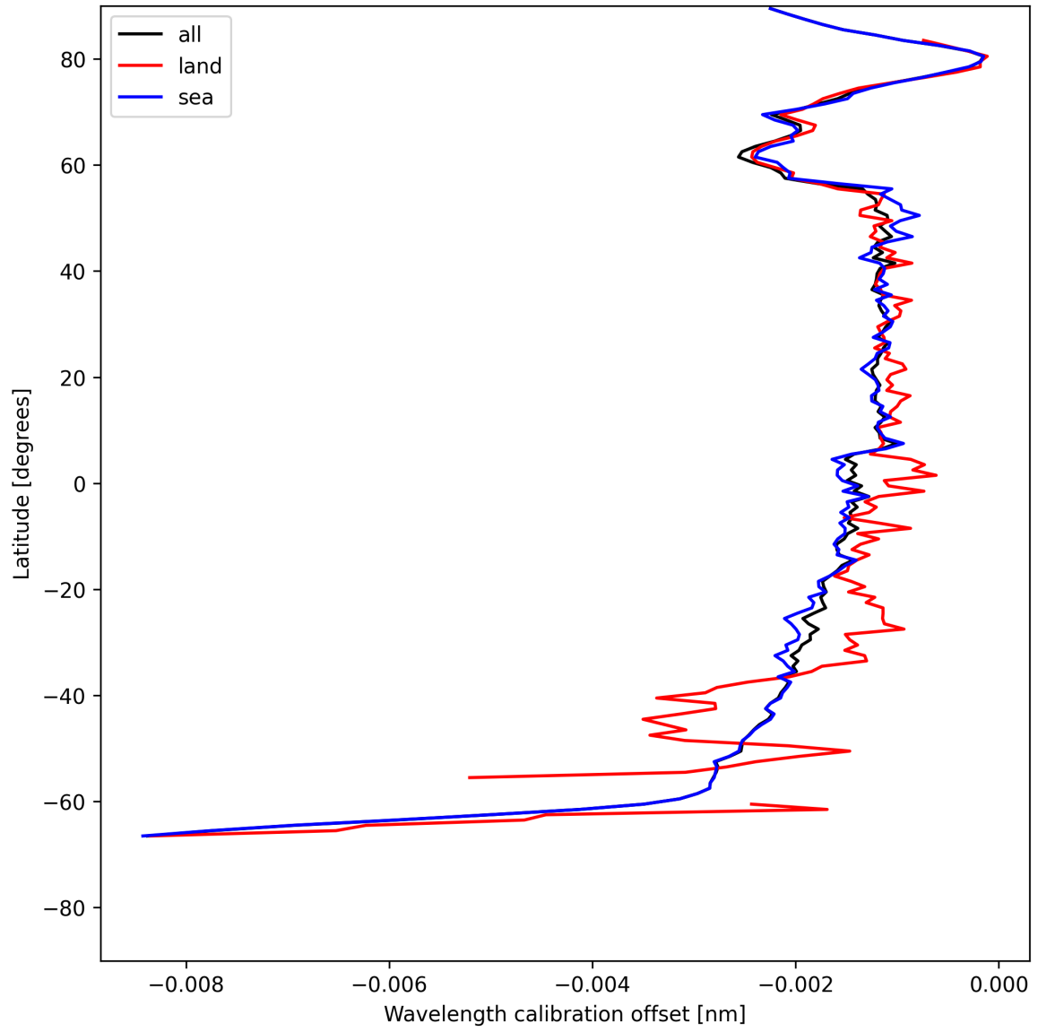
Figure 16: Zonal average of “Wavelength calibration offset” for 2025-05-25 to 2025-05-26.
