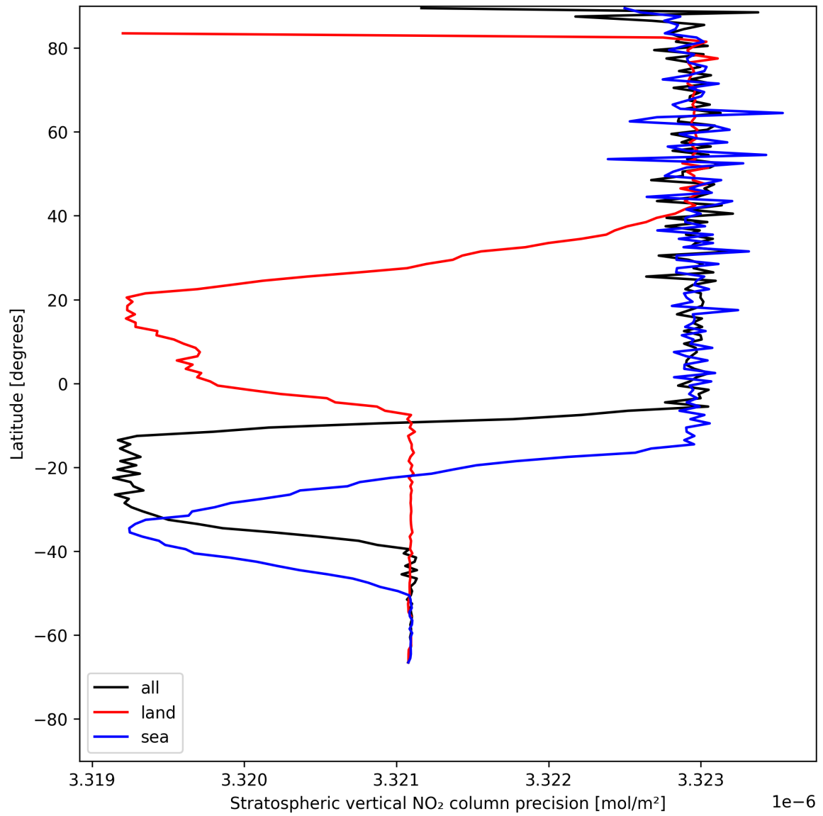
Figure 18: Zonal average of “Stratospheric vertical NO 2 column precision” for 2025-05-25 to 2025-05-26.
