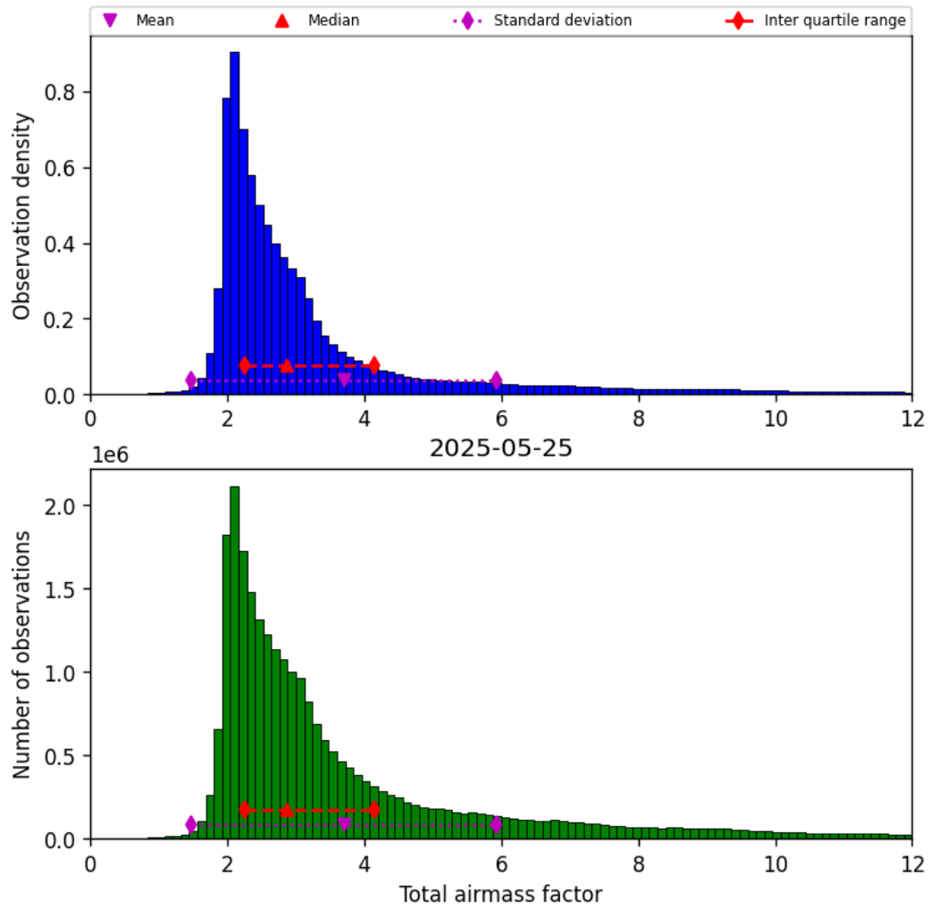
Figure 30: Histogram of “Total airmass factor” for 2025-05-25 to 2025-05-26
