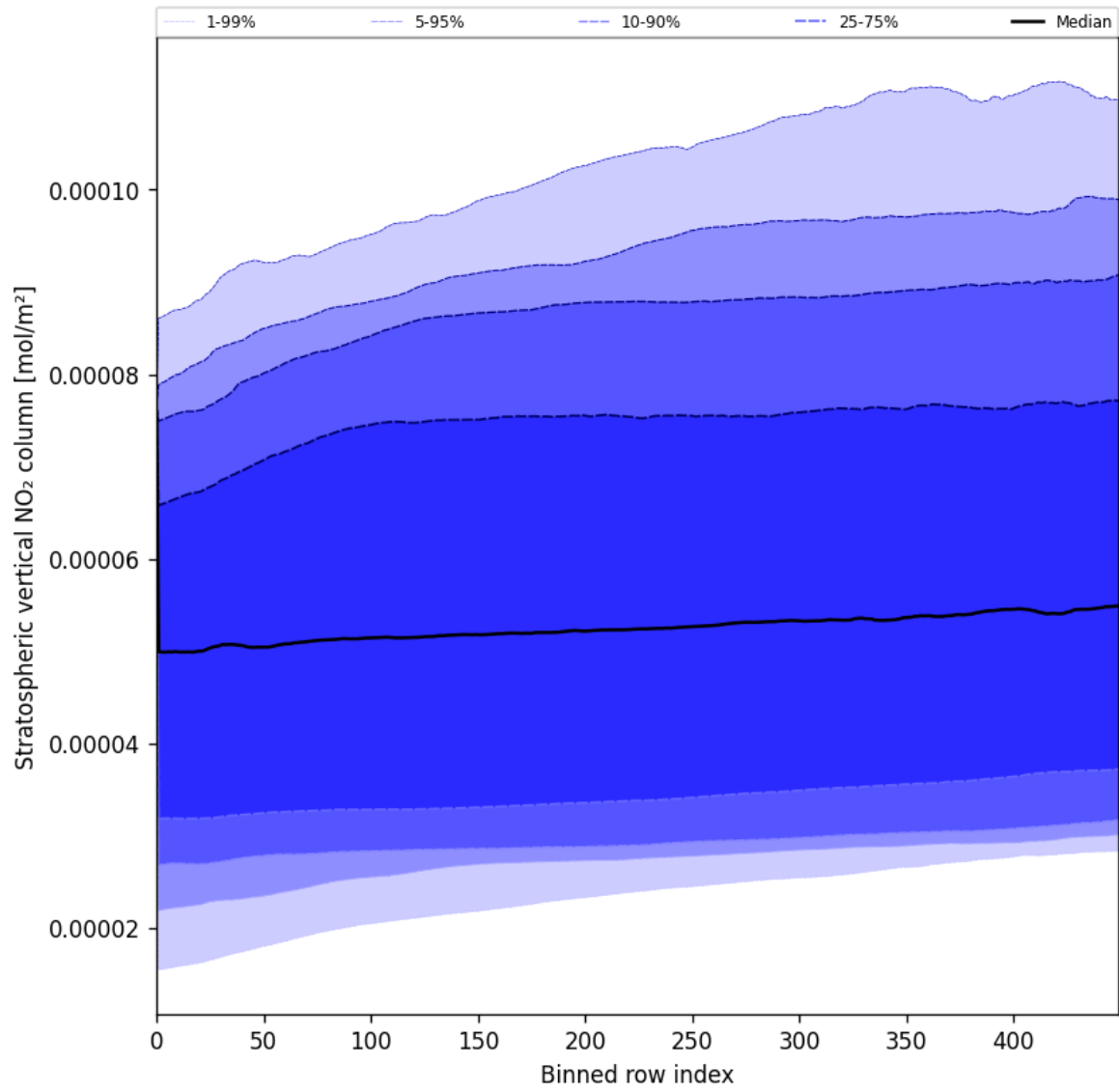
Figure 51: Along track statistics of “Stratospheric vertical NO 2 column” for 2025-05-25 to 2025-05-26
