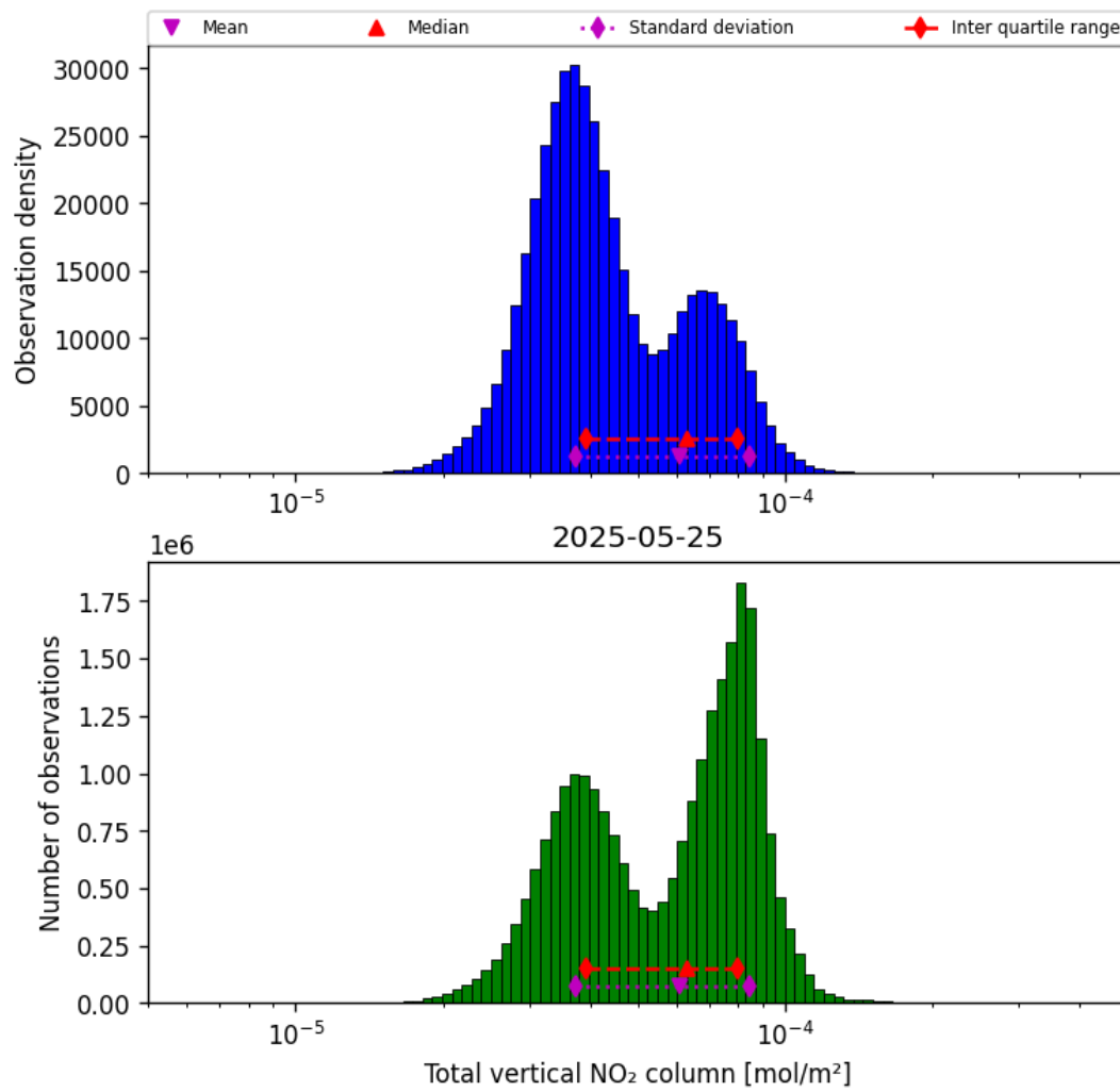
Figure 36: Histogram of “Total vertical NO 2 column” for 2025-05-25 to 2025-05-26
