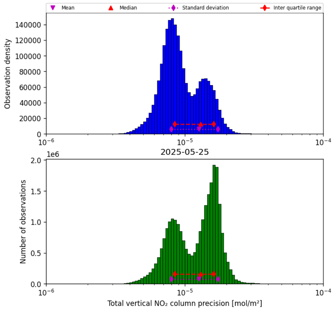
Figure 37: Histogram of "Total vertical NO 2 column precision" for 2025-05-25 to 2025-05-26
