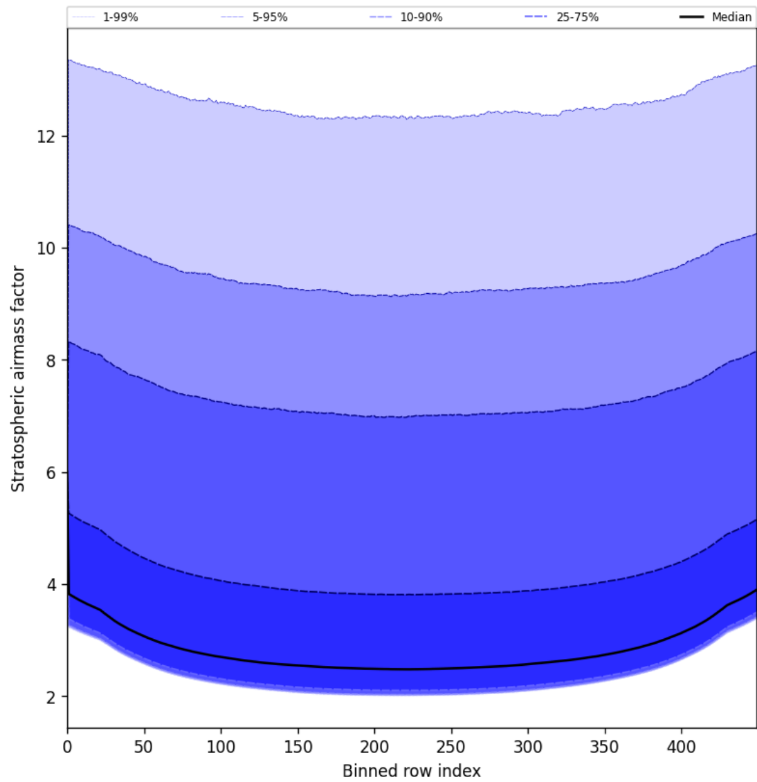
Figure 59: Along track statistics of “Stratospheric airmass factor” for 2025-05-25 to 2025-05-26
