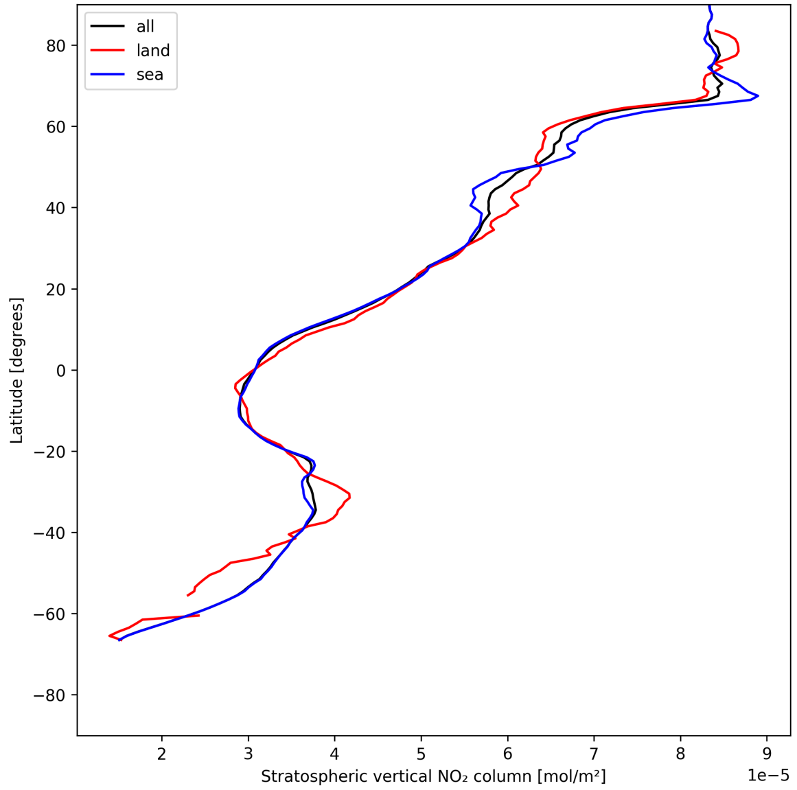
Figure 17: Zonal average of “Stratospheric vertical NO 2 column” for 2025-05-25 to 2025-05-26.
