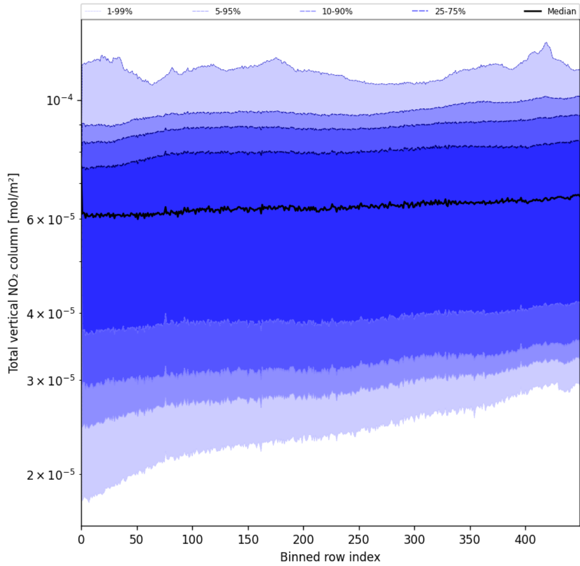
Figure 53: Along track statistics of “Total vertical NO 2 column” for 2025-05-25 to 2025-05-26
