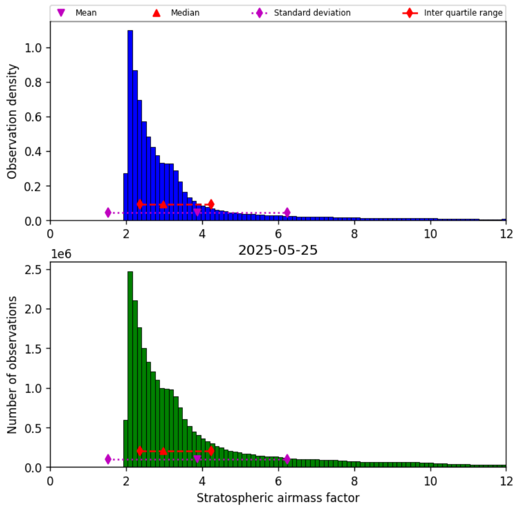
Figure 42: Histogram of “Stratospheric airmass factor” for 2025-05-25 to 2025-05-26
