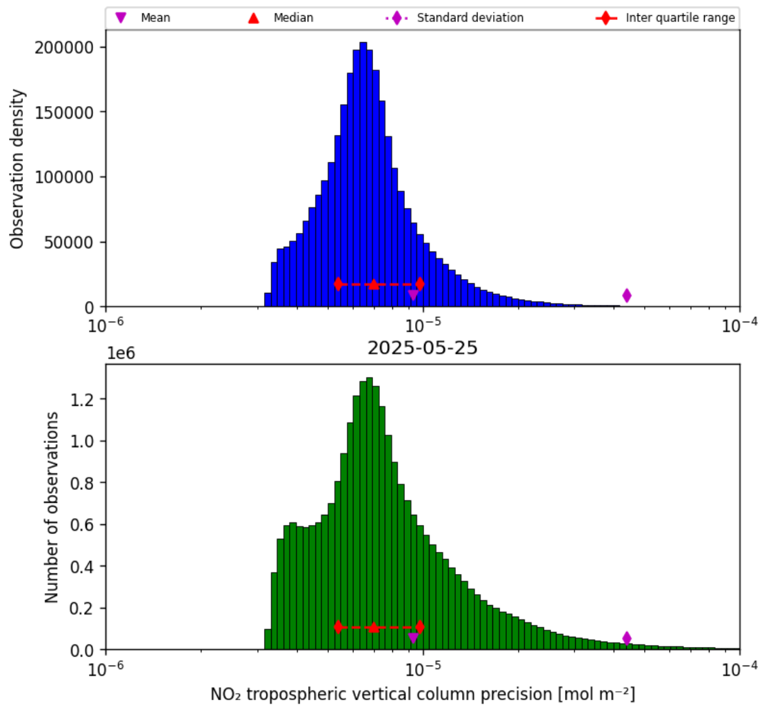
Figure 28: Histogram of “NO 2 tropospheric vertical column precision” for 2025-05-25 to 2025-05-26
