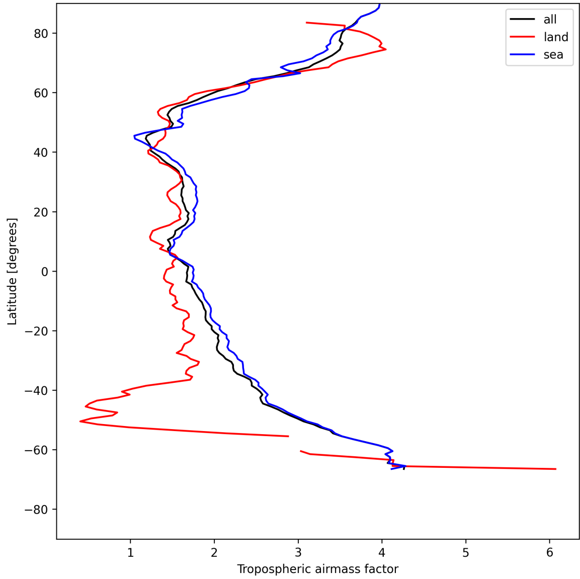
Figure 12: Zonal average of “Tropospheric airmass factor” for 2025-05-25 to 2025-05-26.
