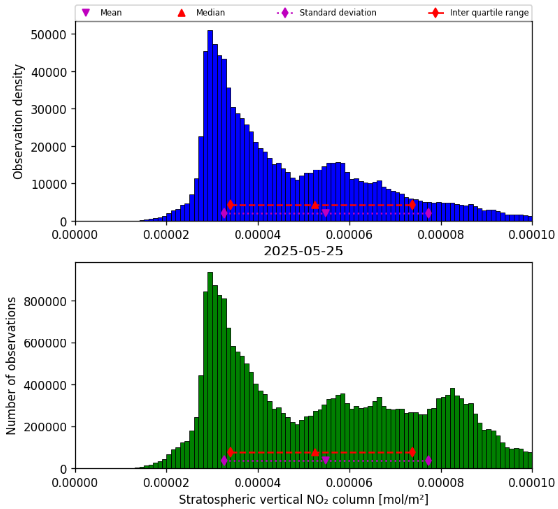
Figure 34: Histogram of “Stratospheric vertical NO 2 column” for 2025-05-25 to 2025-05-26
