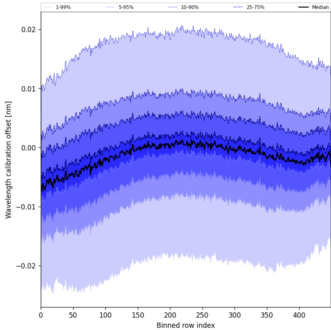
Figure 50: Along track statistics of “Wavelength calibration offset” for 2025-05-25 to 2025-05-26
