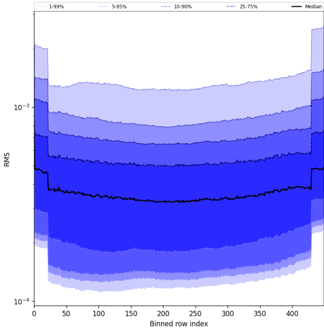
Figure 58: Along track statistics of “RMS” for 2025-05-25 to 2025-05-26
