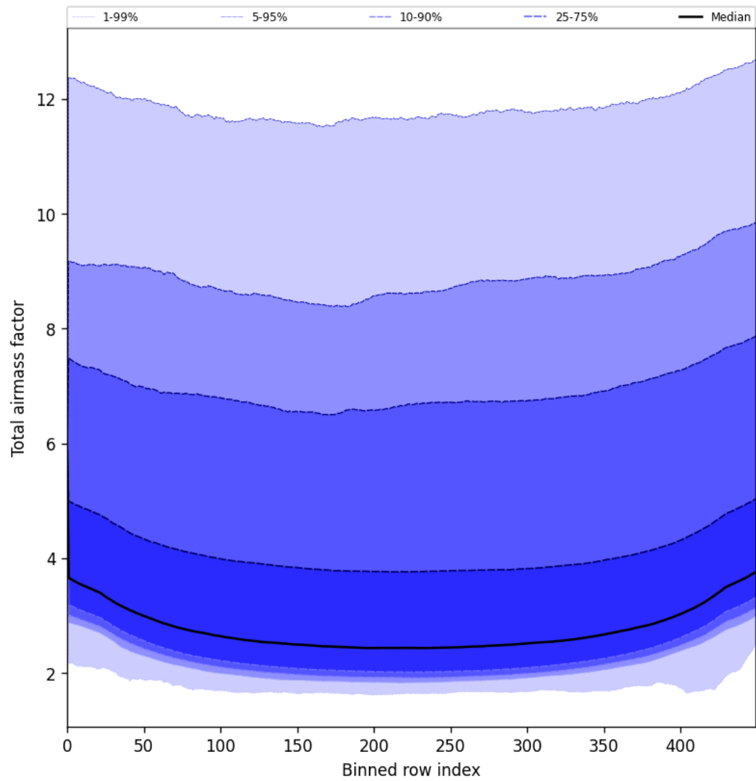
Figure 47: Along track statistics of “Total airmass factor” for 2025-05-25 to 2025-05-26
