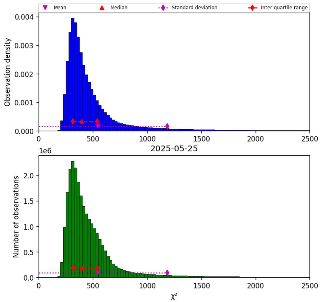
Figure 40: Histogram of “ \chi^2 ” for 2025-05-25 to 2025-05-26
