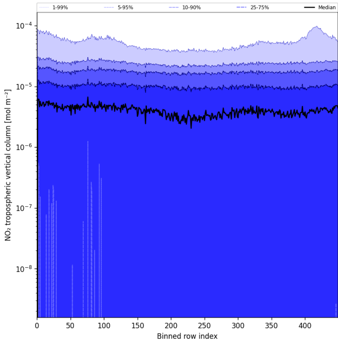
Figure 44: Along track statistics of “NO 2 tropospheric vertical column” for 2025-05-25 to 2025-05-26
