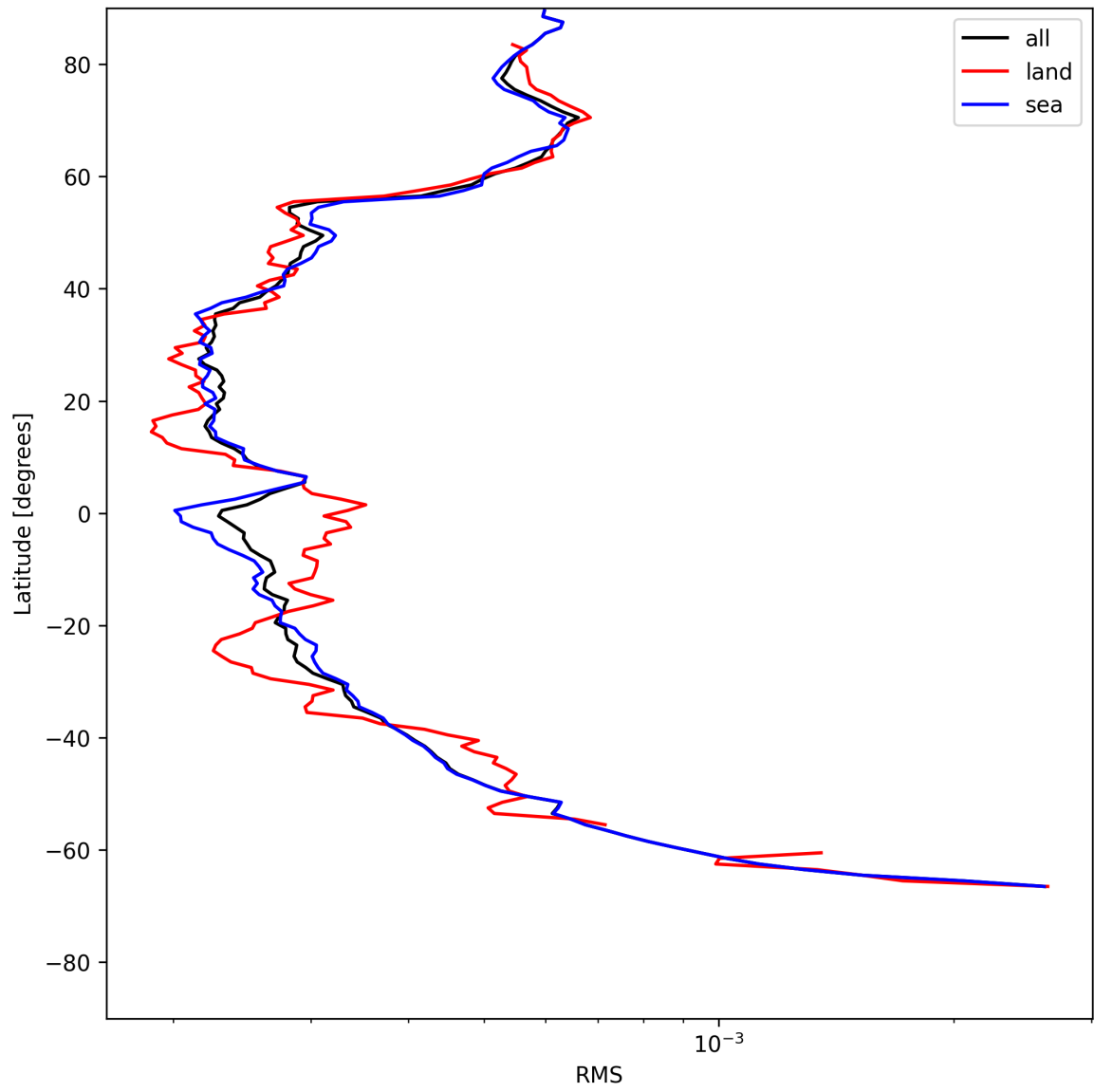
Figure 24: Zonal average of “RMS” for 2025-05-25 to 2025-05-26.
