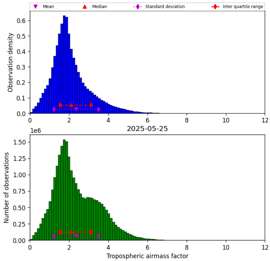
Figure 29: Histogram of “Tropospheric airmass factor” for 2025-05-25 to 2025-05-26
