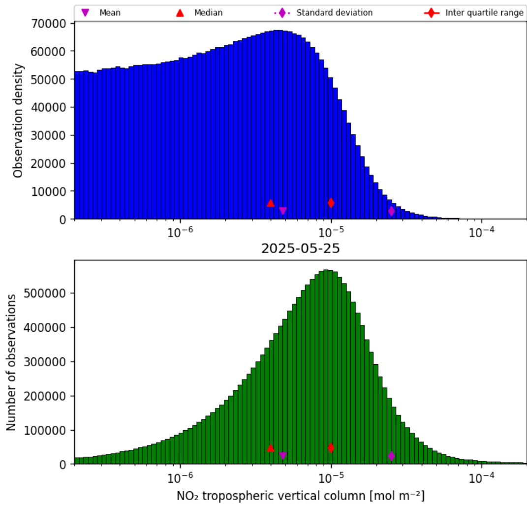
Figure 27: Histogram of “NO 2 tropospheric vertical column” for 2025-05-25 to 2025-05-26
