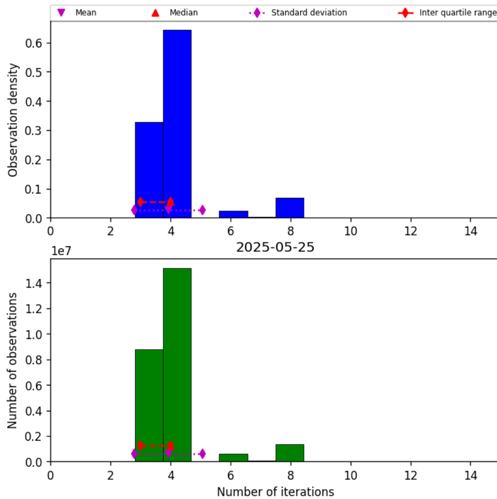
Figure 32: Histogram of “Number of iterations” for 2025-05-25 to 2025-05-26
