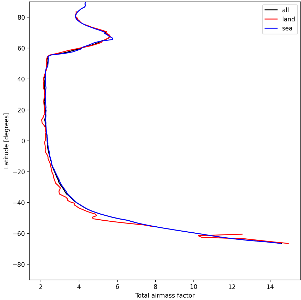
Figure 13: Zonal average of “Total airmass factor” for 2025-05-25 to 2025-05-26.
