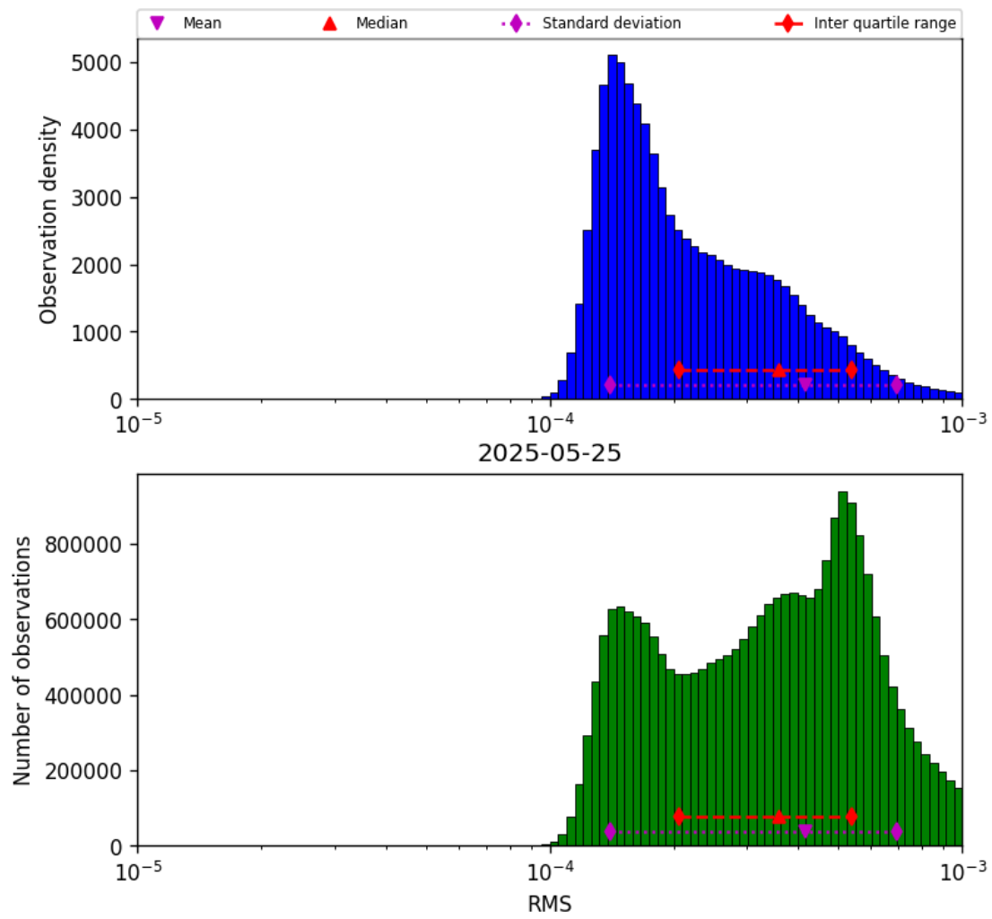
Figure 41: Histogram of “RMS” for 2025-05-25 to 2025-05-26
