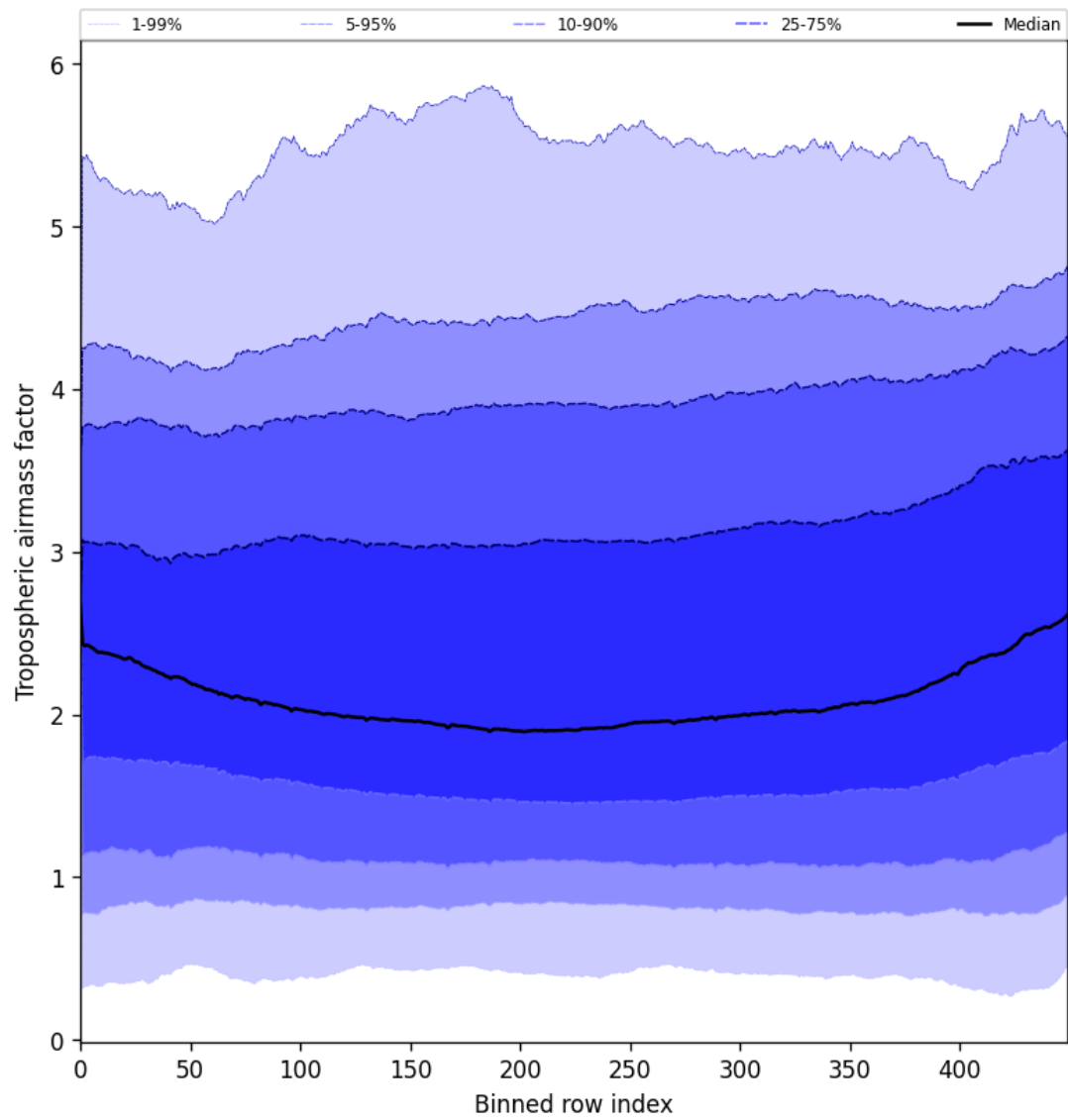
Figure 46: Along track statistics of “Tropospheric airmass factor” for 2025-05-25 to 2025-05-26
