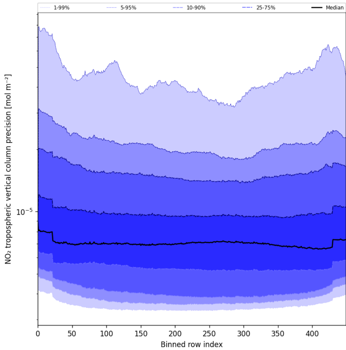
Figure 45: Along track statistics of “NO 2 tropospheric vertical column precision” for 2025-05-25 to 2025-05-26
