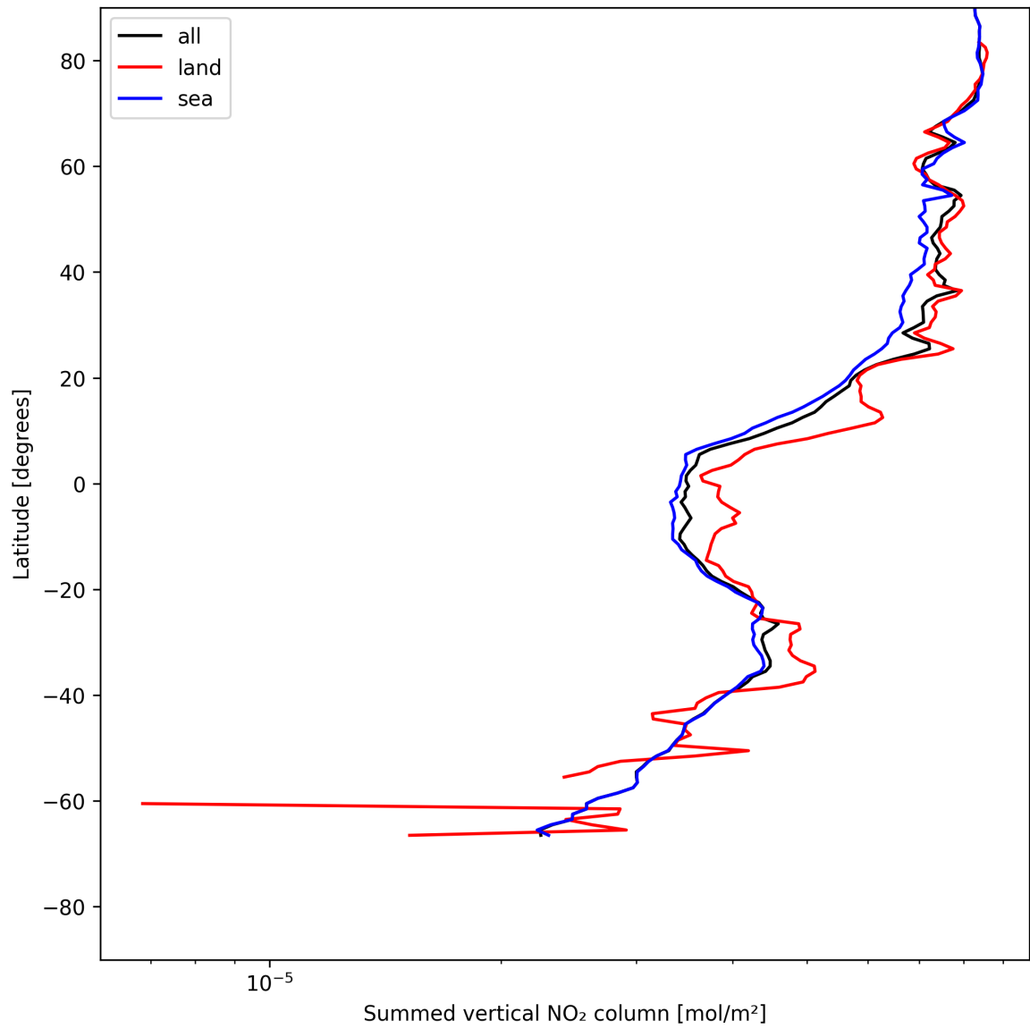
Figure 21: Zonal average of “Summed vertical NO 2 column” for 2025-05-25 to 2025-05-26.
