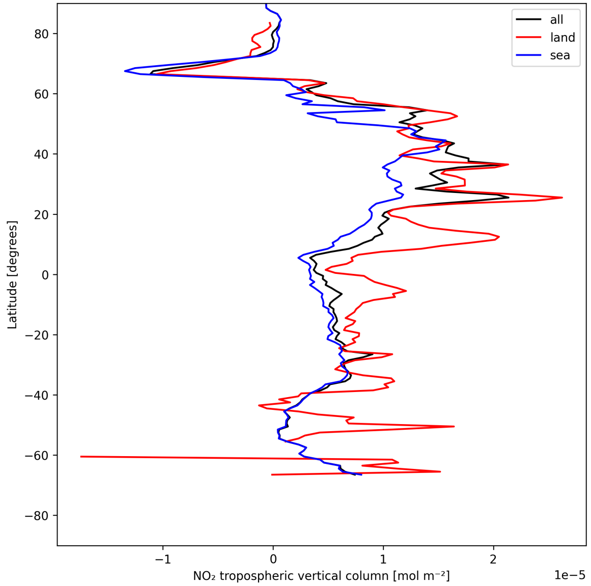
Figure 10: Zonal average of “NO 2 tropospheric vertical column” for 2025-05-25 to 2025-05-26.
