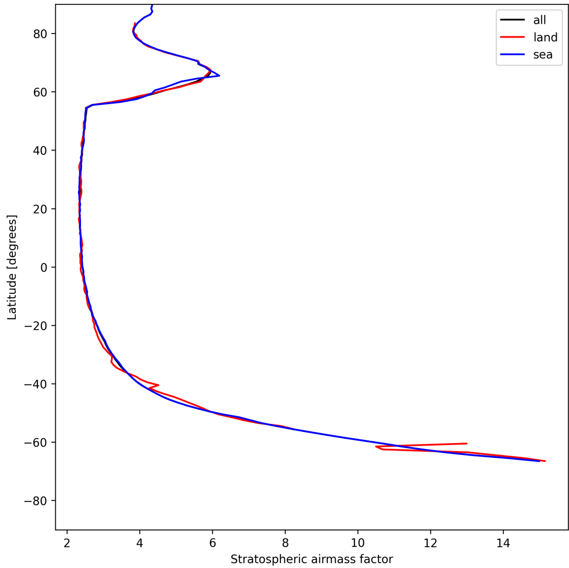
Figure 25: Zonal average of “Stratospheric airmass factor” for 2025-05-25 to 2025-05-26.
