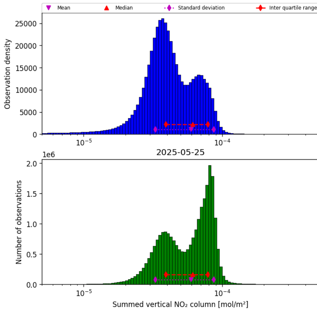
Figure 38: Histogram of “Summed vertical NO 2 column” for 2025-05-25 to 2025-05-26
