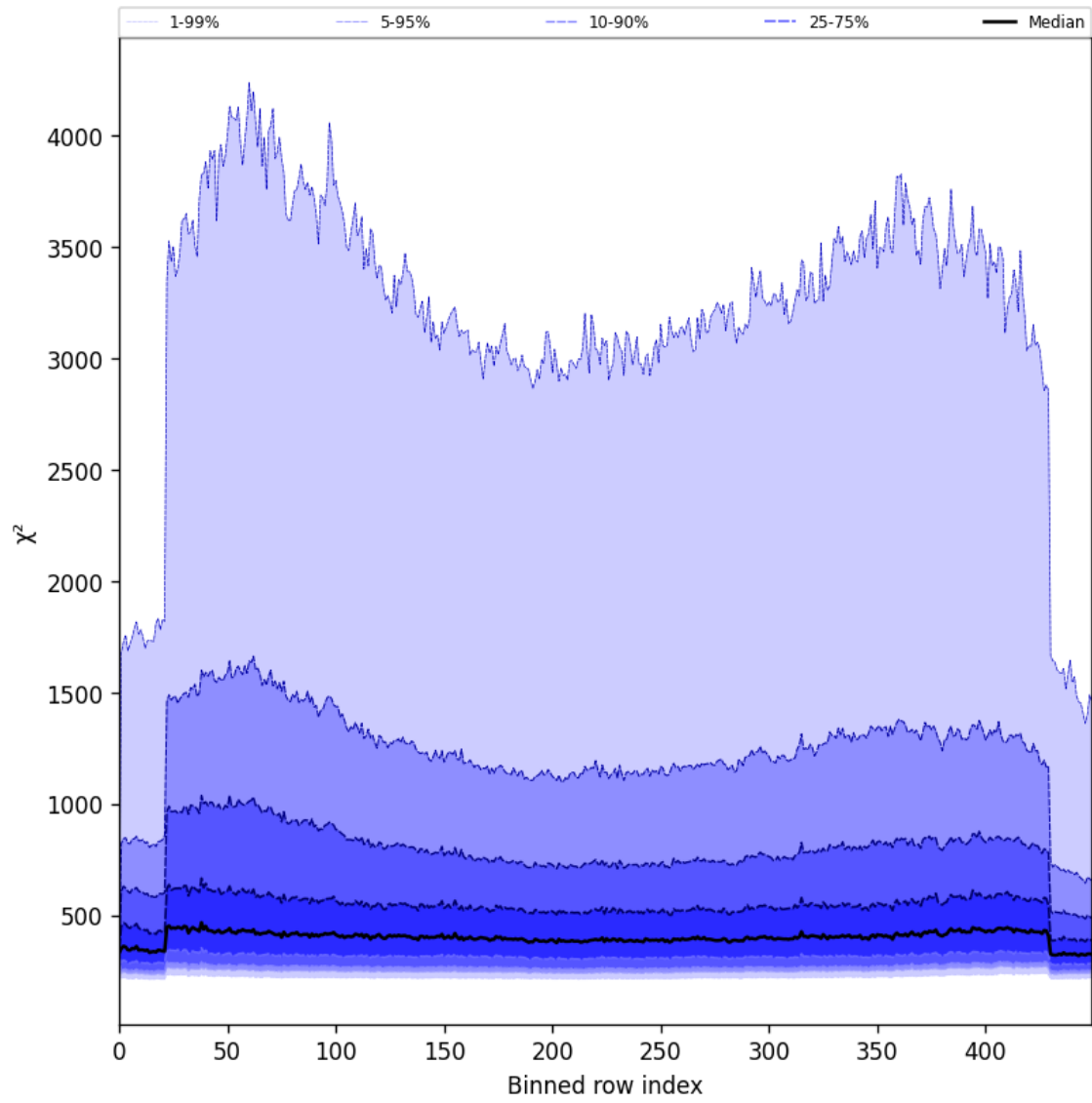
Figure 57: Along track statistics of “ \chi^2 ” for 2025-05-25 to 2025-05-26
