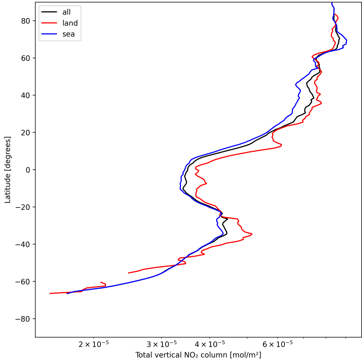
Figure 19: Zonal average of “Total vertical NO 2 column” for 2025-05-25 to 2025-05-26.
