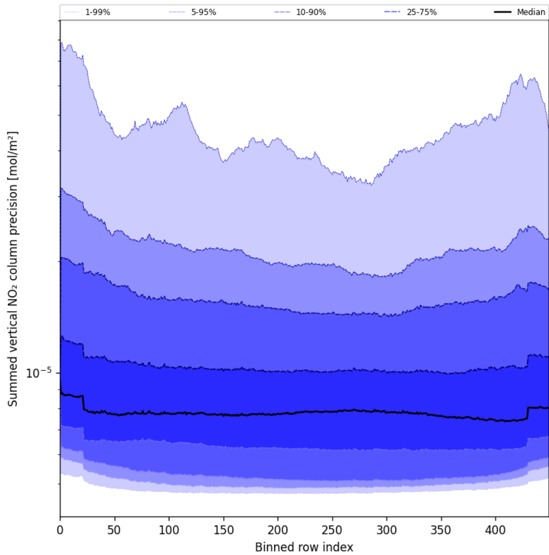
Figure 56: Along track statistics of “Summed vertical NO 2 column precision” for 2025-05-25 to 2025-05-26
