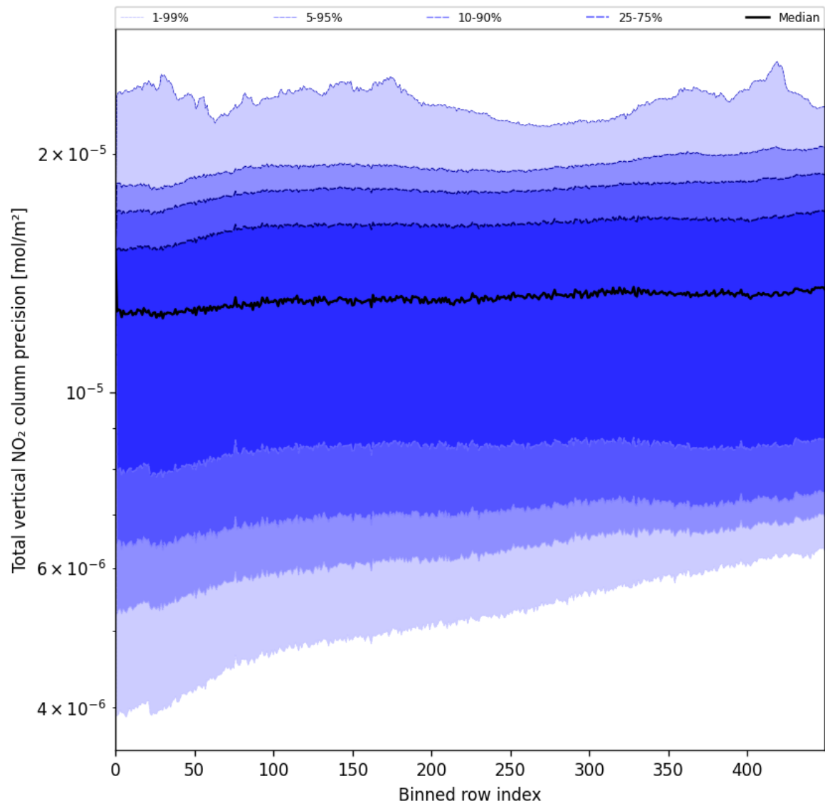
Figure 54: Along track statistics of “Total vertical NO 2 column precision” for 2025-05-25 to 2025-05-26
