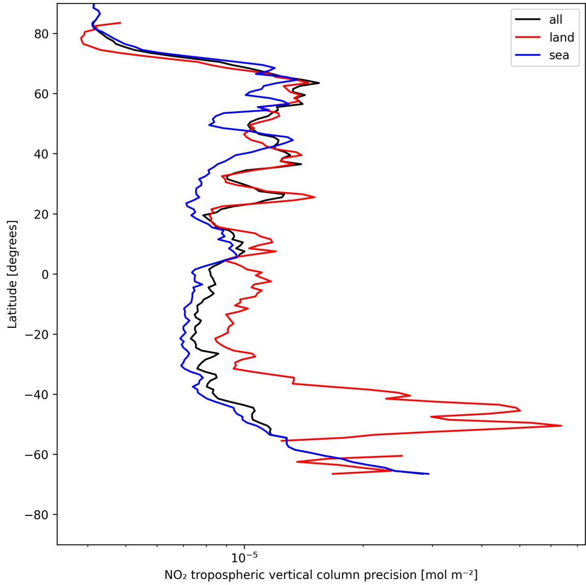
Figure 11: Zonal average of “NO 2 tropospheric vertical column precision” for 2025-05-25 to 2025-05-26.
