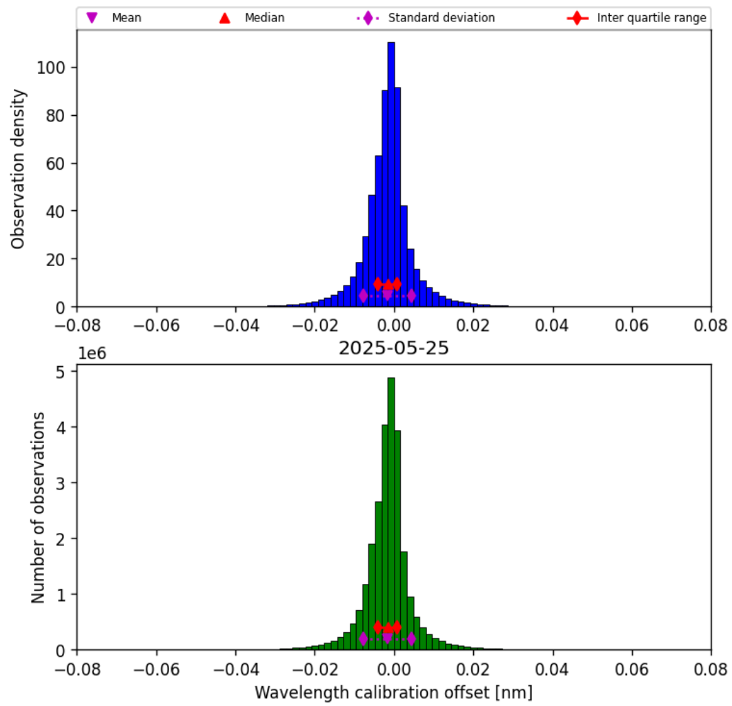
Figure 33: Histogram of “Wavelength calibration offset” for 2025-05-25 to 2025-05-26
