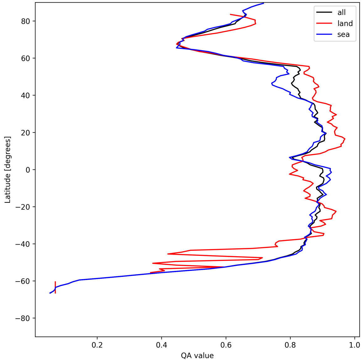
Figure 9: Zonal average of “QA value” for 2025-05-25 to 2025-05-26.
