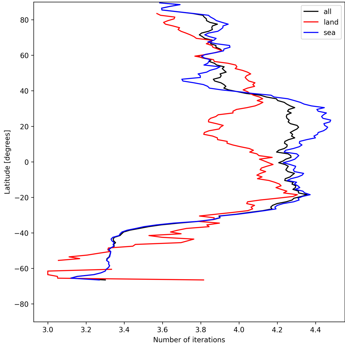
Figure 15: Zonal average of “Number of iterations” for 2025-05-25 to 2025-05-26.
