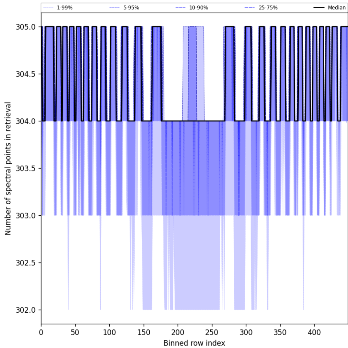
Figure 48: Along track statistics of “Number of spectral points in retrieval” for 2025-05-25 to 2025-05-26
