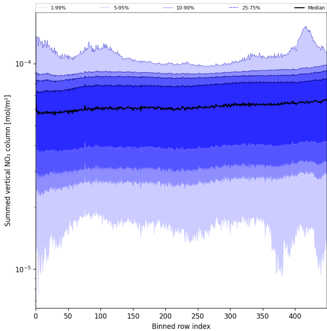
Figure 55: Along track statistics of “Summed vertical NO 2 column” for 2025-05-25 to 2025-05-26
