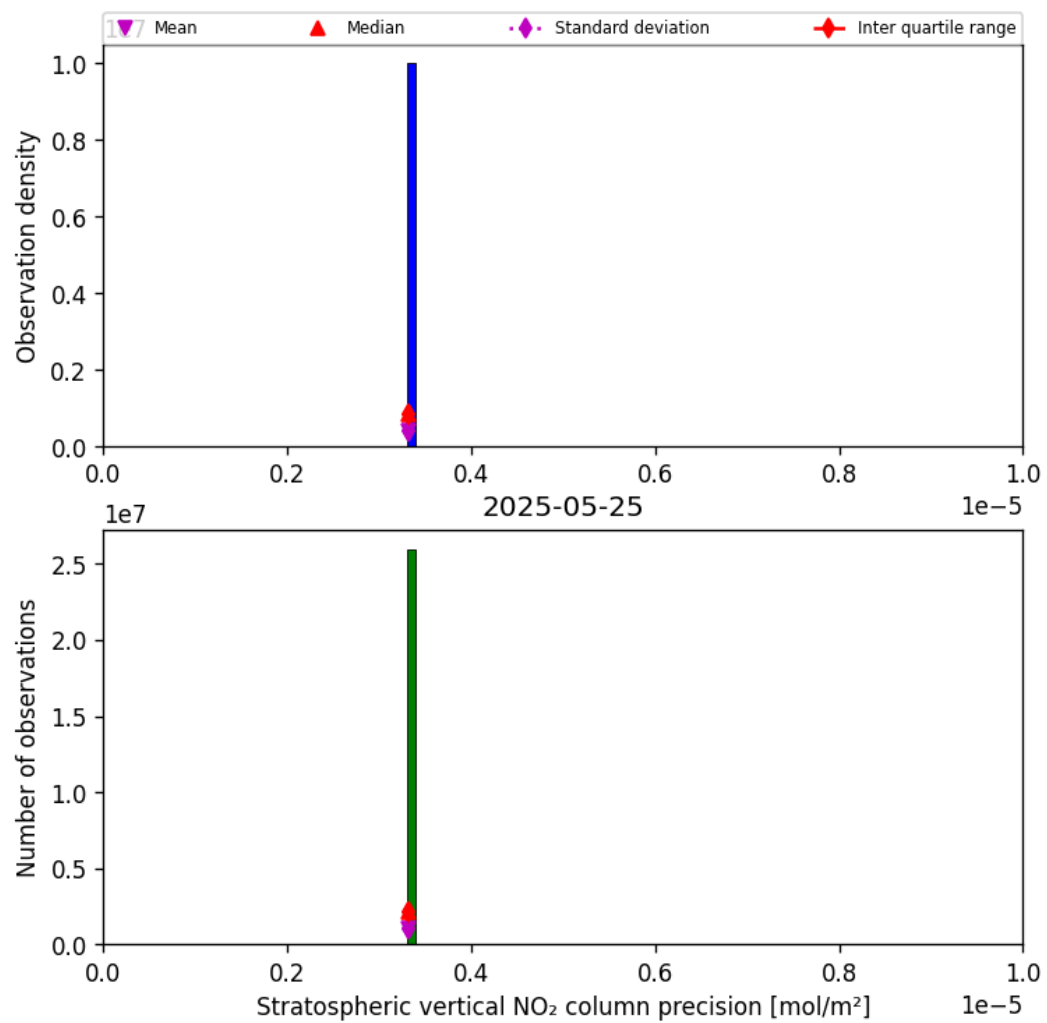
Figure 35: Histogram of “Stratospheric vertical NO 2 column precision” for 2025-05-25 to 2025-05-26
