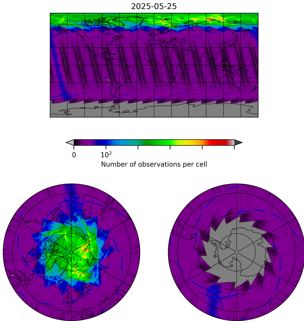
Figure 8: Map of the number of observations for 2025-05-25 to 2025-05-26
