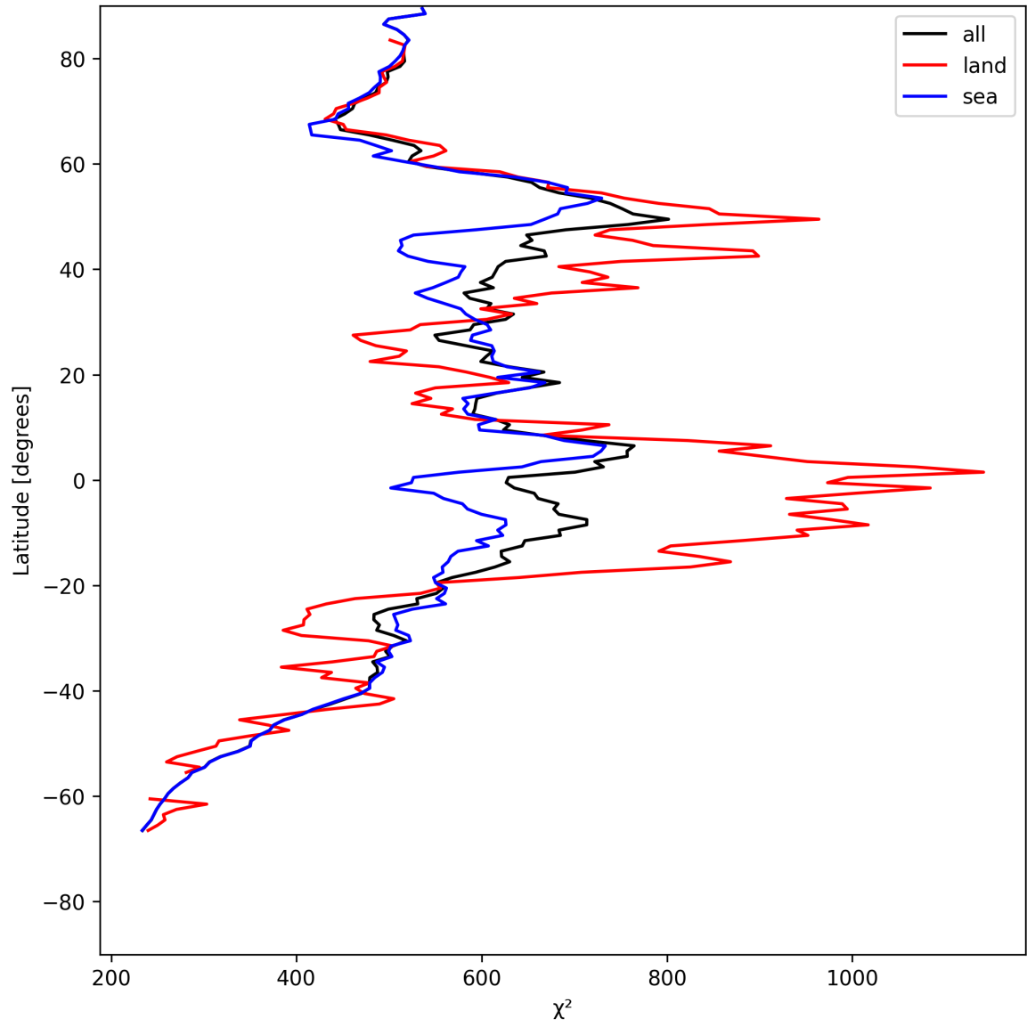
Figure 23: Zonal average of “ \chi^2 ” for 2025-05-25 to 2025-05-26.
