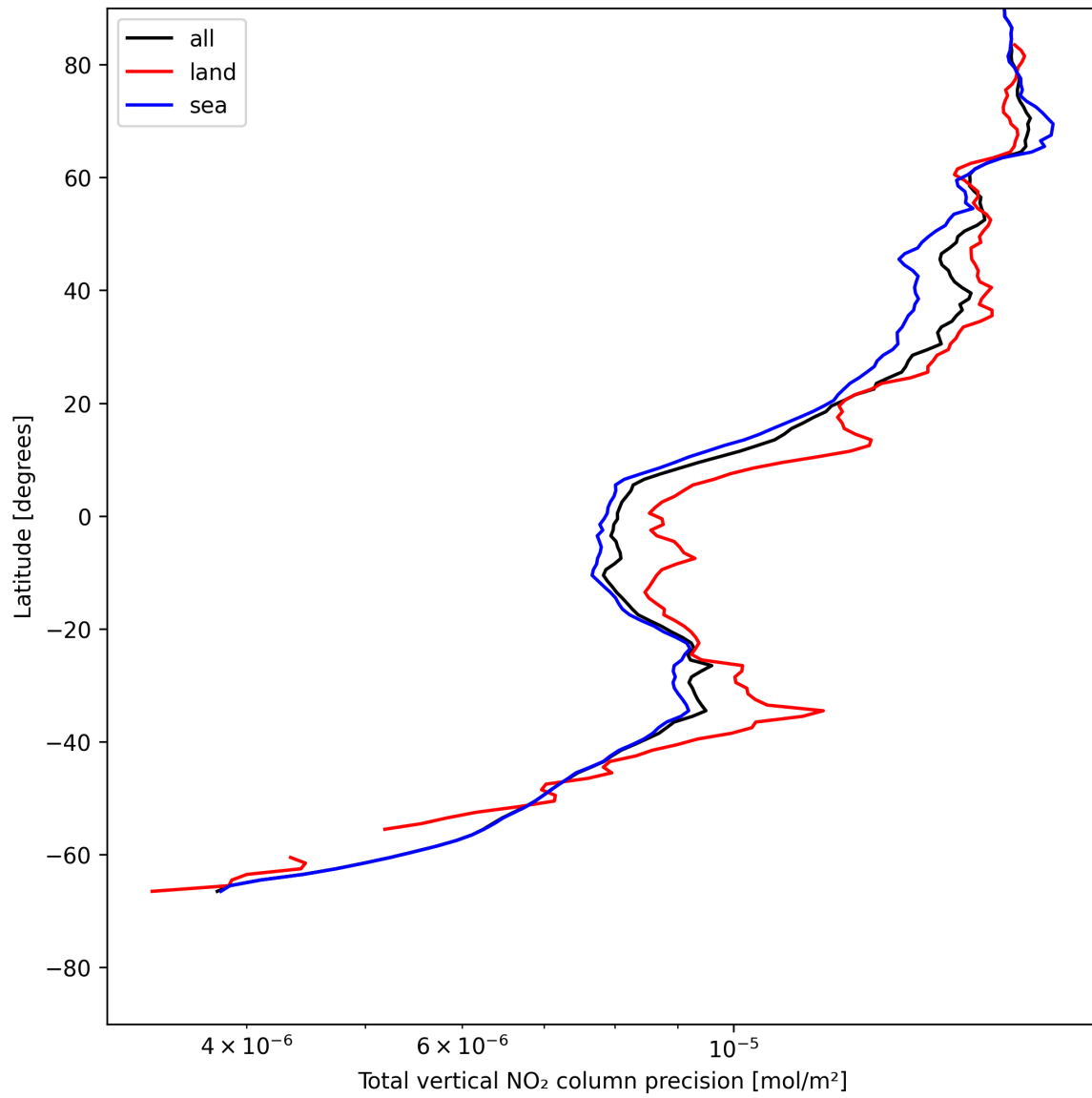
Figure 20: Zonal average of “Total vertical NO 2 column precision” for 2025-05-25 to 2025-05-26.
