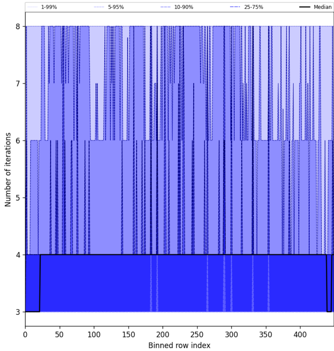
Figure 49: Along track statistics of “Number of iterations” for 2025-05-25 to 2025-05-26
