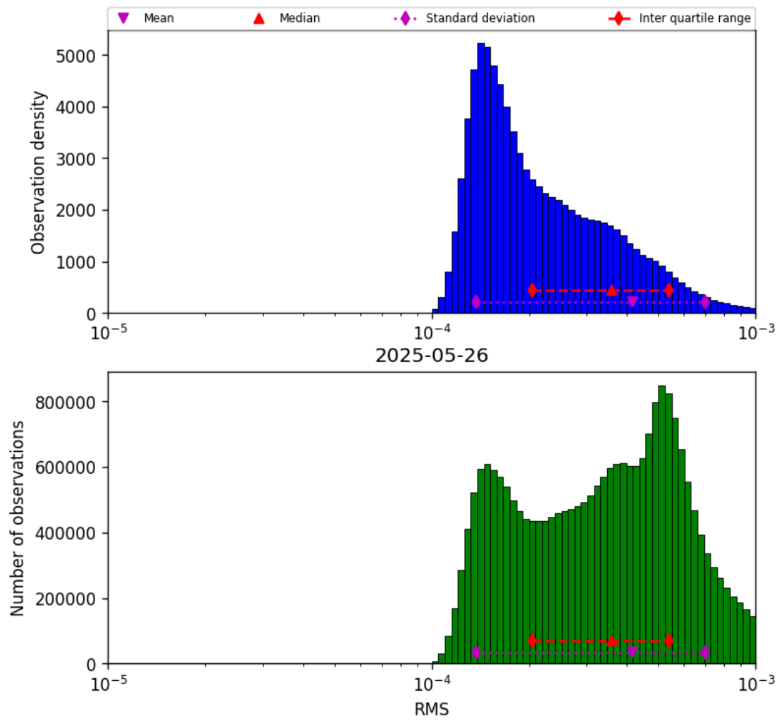
Figure 41: Histogram of “RMS” for 2025-05-26 to 2025-05-27
