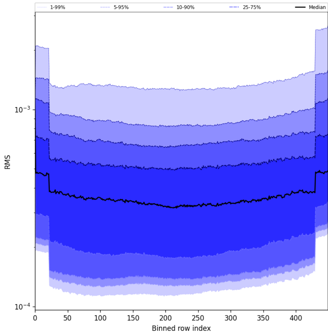
Figure 58: Along track statistics of “RMS” for 2025-05-26 to 2025-05-27
