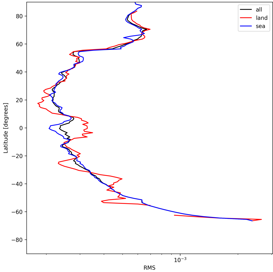
Figure 24: Zonal average of “RMS” for 2025-05-26 to 2025-05-27.
