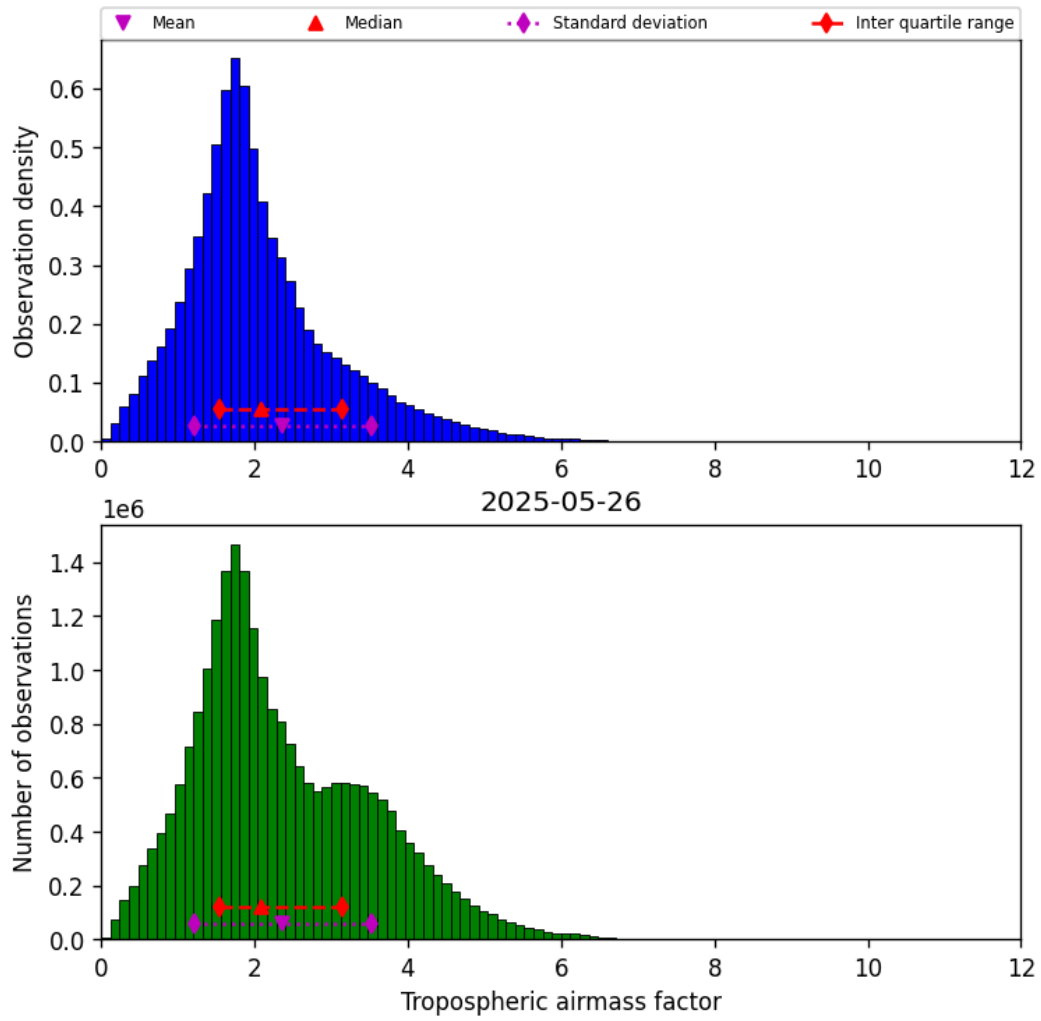
Figure 29: Histogram of “Tropospheric airmass factor” for 2025-05-26 to 2025-05-27
