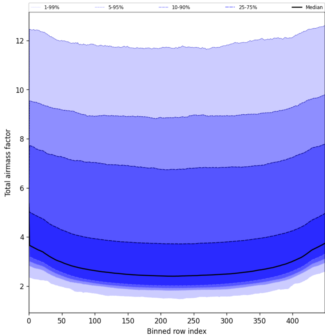
Figure 47: Along track statistics of “Total airmass factor” for 2025-05-26 to 2025-05-27
