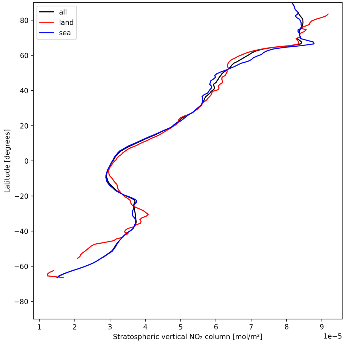
Figure 17: Zonal average of “Stratospheric vertical NO 2 column” for 2025-05-26 to 2025-05-27.
