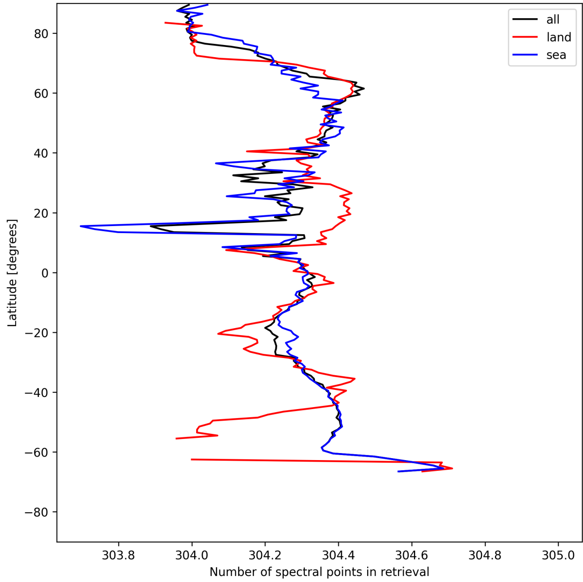
Figure 14: Zonal average of “Number of spectral points in retrieval” for 2025-05-26 to 2025-05-27.
