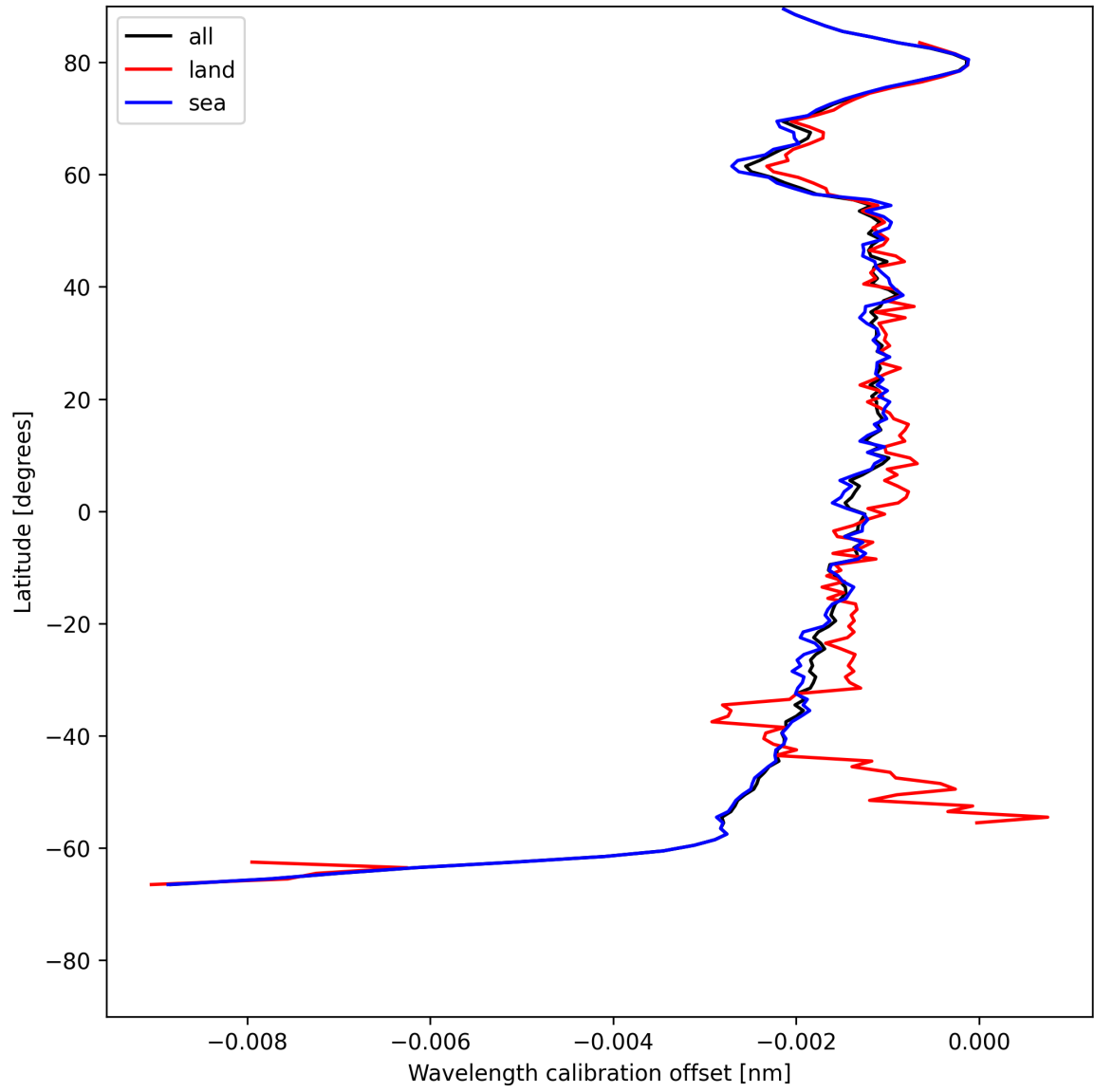
Figure 16: Zonal average of “Wavelength calibration offset” for 2025-05-26 to 2025-05-27.
