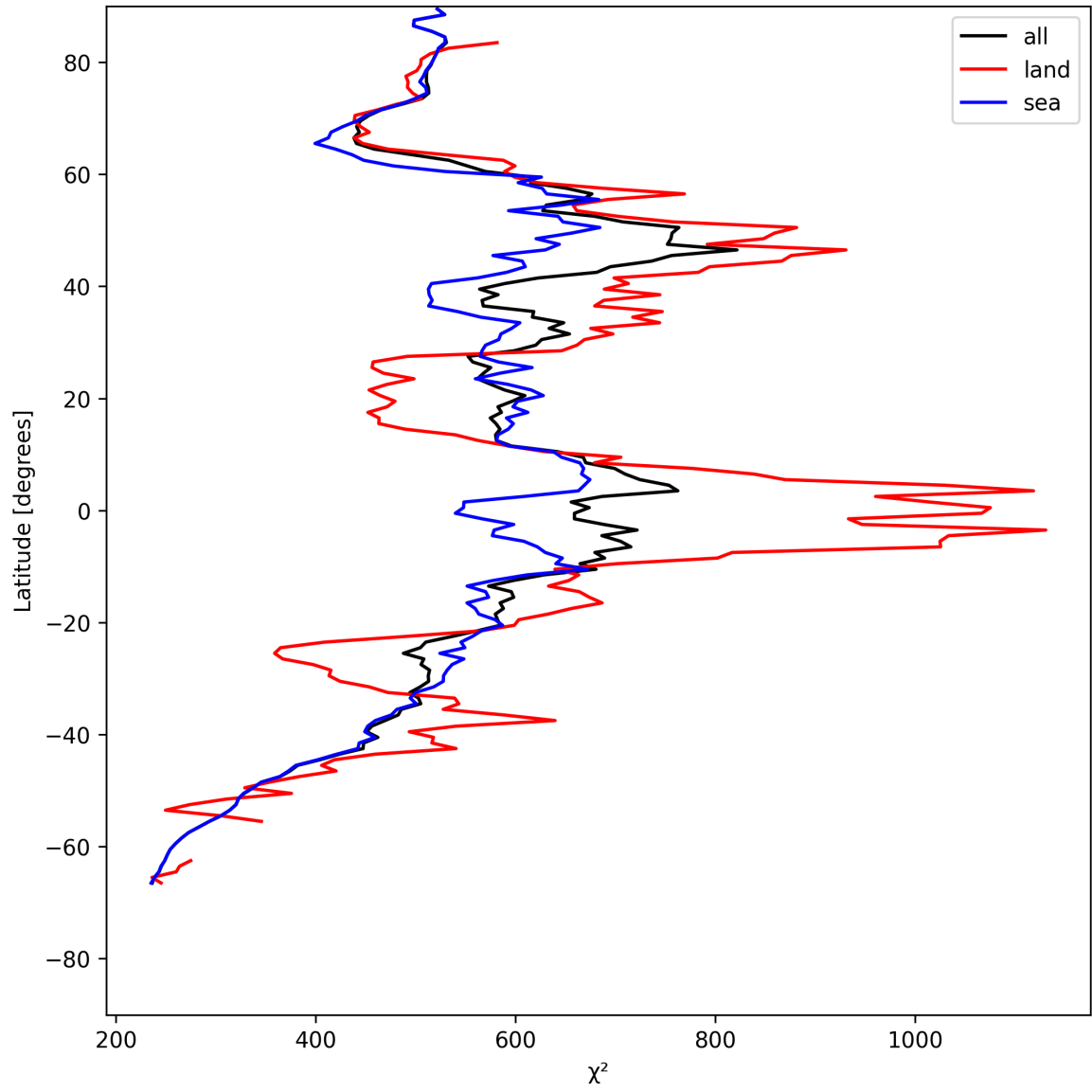
Figure 23: Zonal average of “ \chi^2 ” for 2025-05-26 to 2025-05-27.
