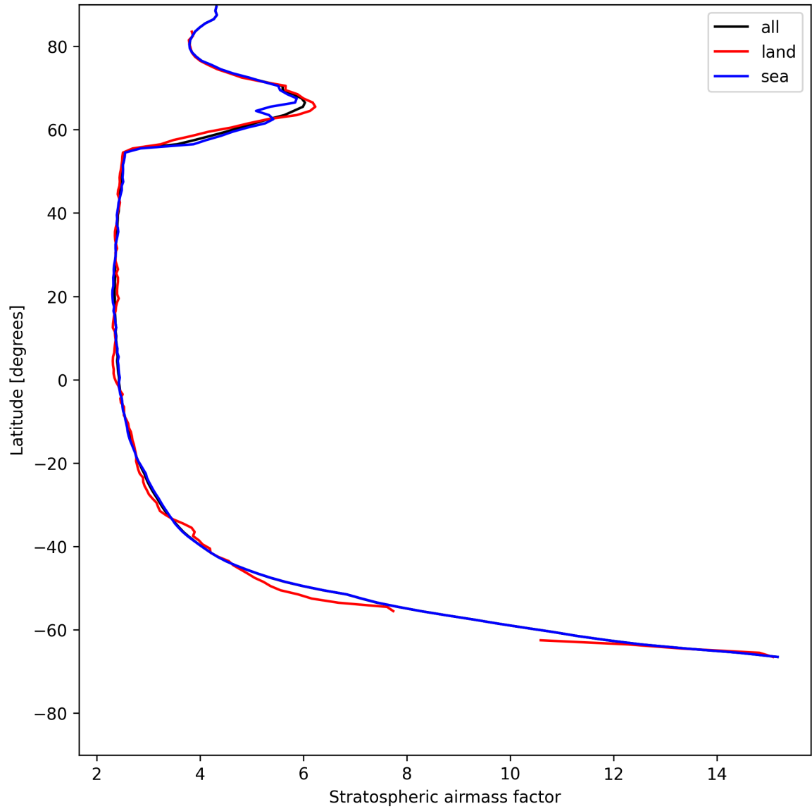
Figure 25: Zonal average of “Stratospheric air mass factor” for 2025-05-26 to 2025-05-27.
