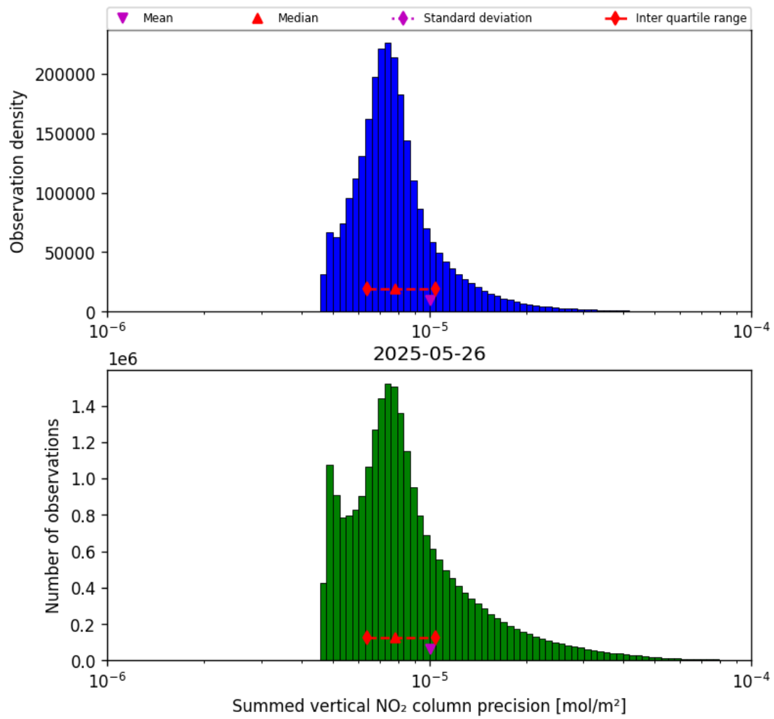
Figure 39: Histogram of “Summed vertical NO 2 column precision” for 2025-05-26 to 2025-05-27
