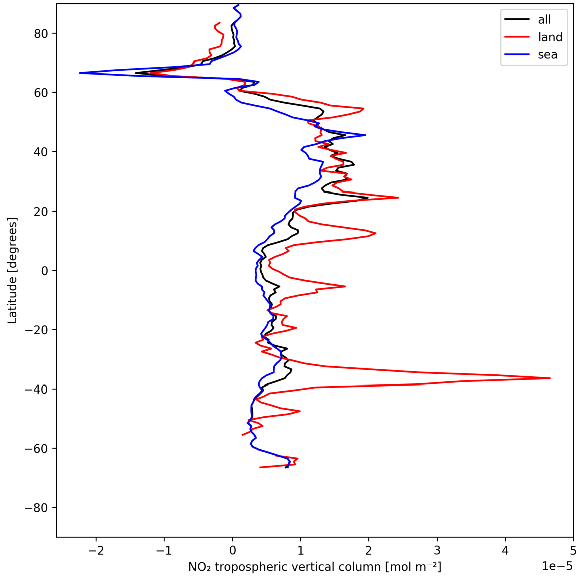
Figure 10: Zonal average of “NO 2 tropospheric vertical column” for 2025-05-26 to 2025-05-27.
