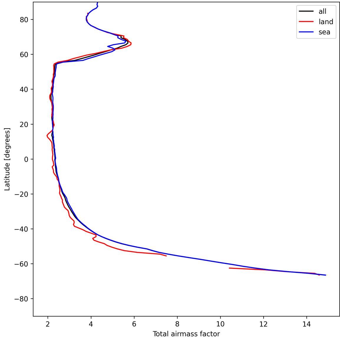
Figure 13: Zonal average of “Total airmass factor” for 2025-05-26 to 2025-05-27.
