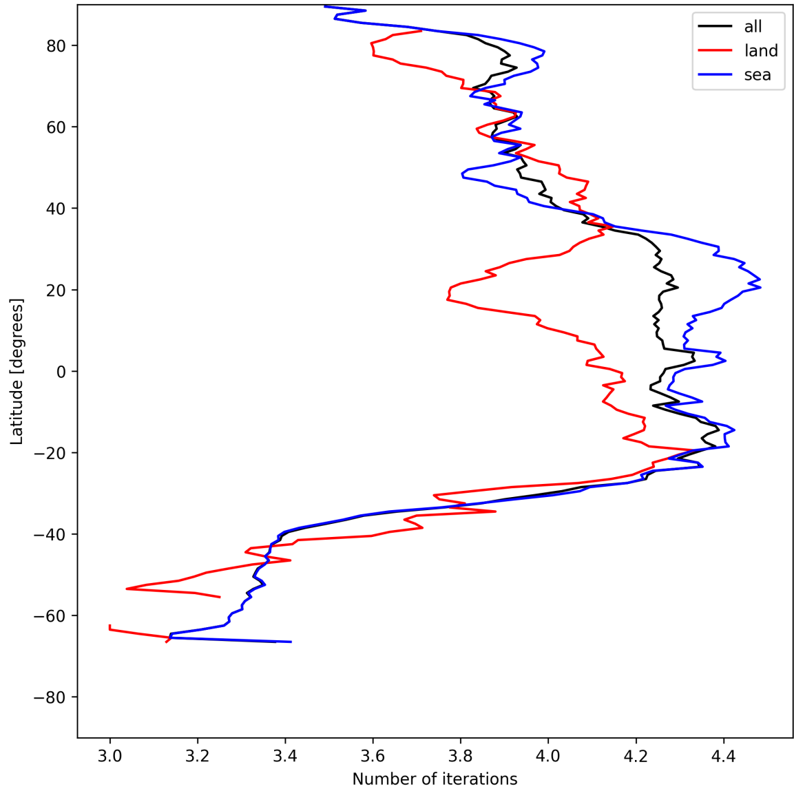
Figure 15: Zonal average of “Number of iterations” for 2025-05-26 to 2025-05-27.
