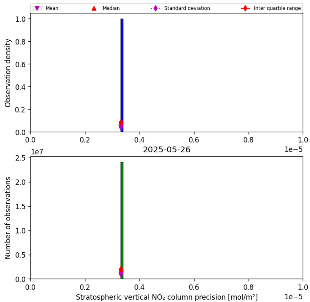
Figure 35: Histogram of “Stratospheric vertical NO 2 column precision” for 2025-05-26 to 2025-05-27
