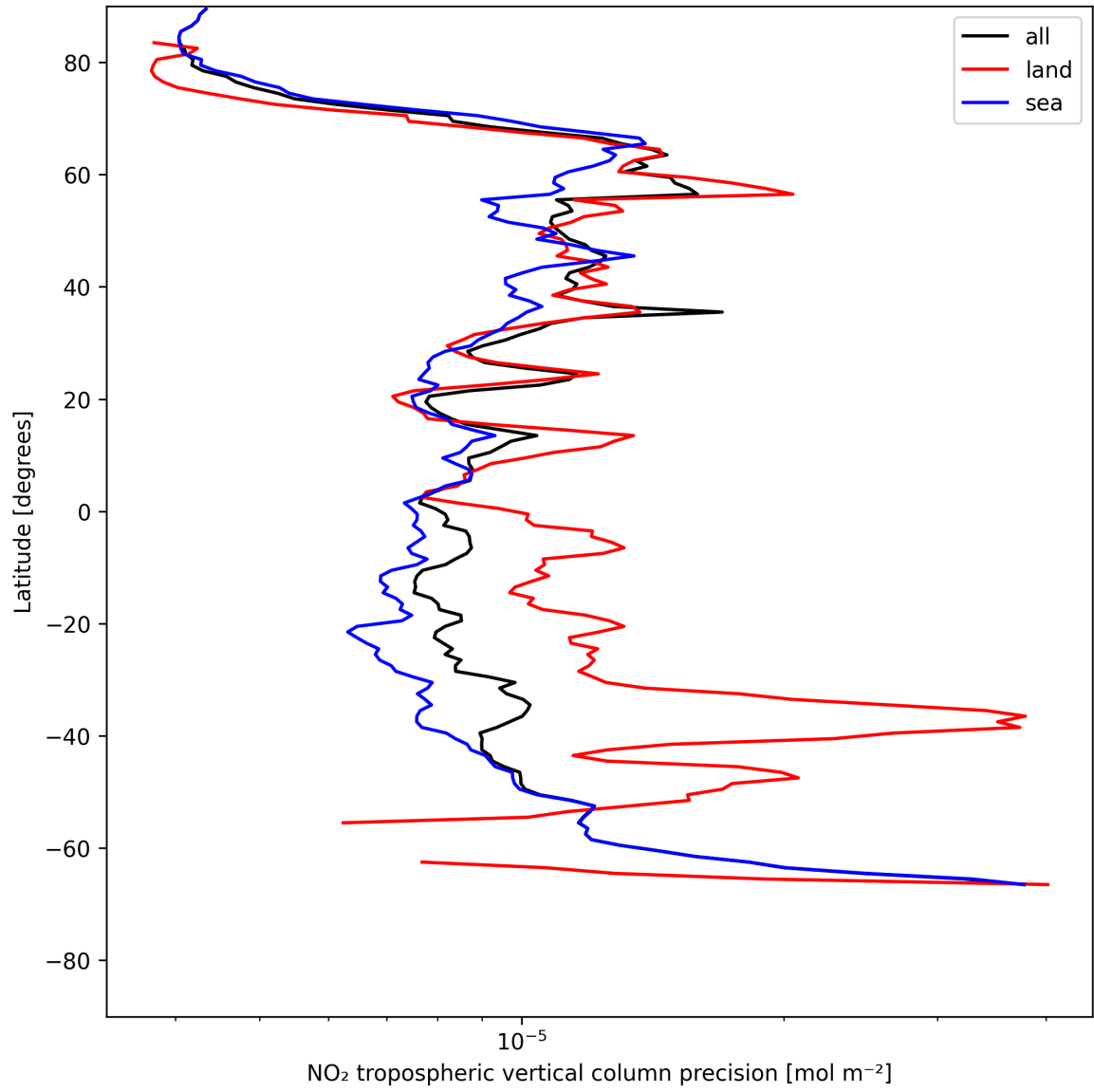
Figure 11: Zonal average of “NO 2 tropospheric vertical column precision” for 2025-05-26 to 2025-05-27.
