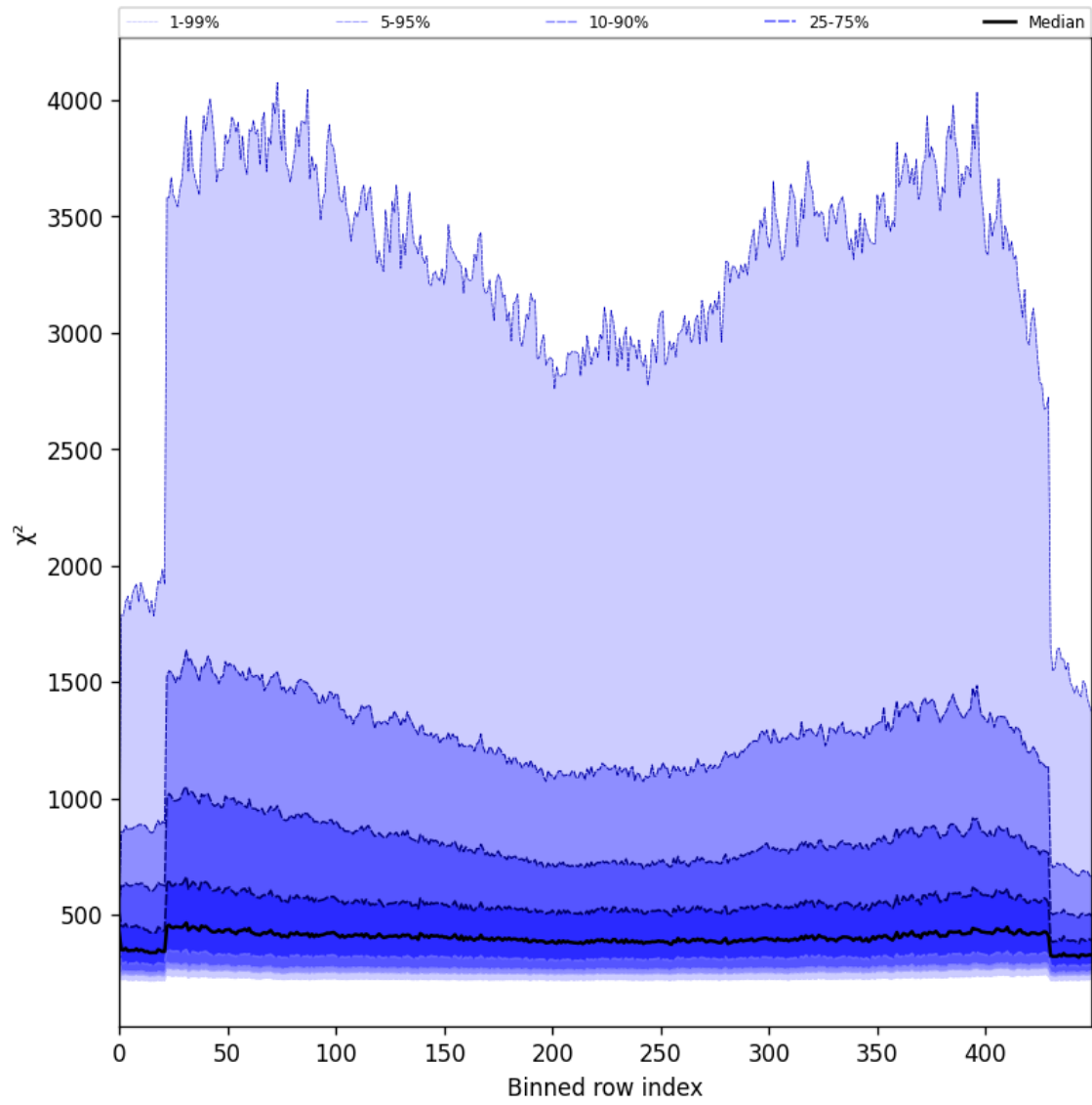
Figure 57: Along track statistics of “ \chi^2 ” for 2025-05-26 to 2025-05-27
