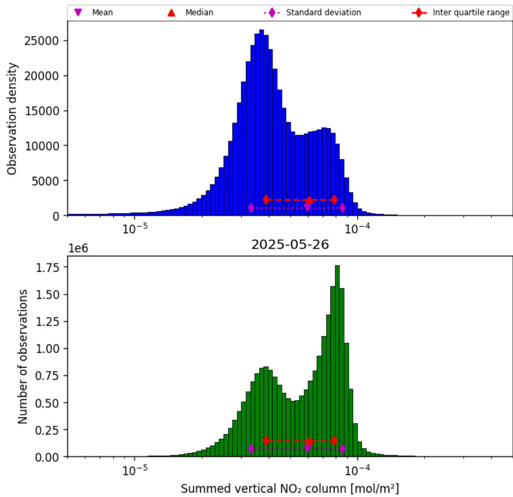
Figure 38: Histogram of “Summed vertical NO 2 column” for 2025-05-26 to 2025-05-27
