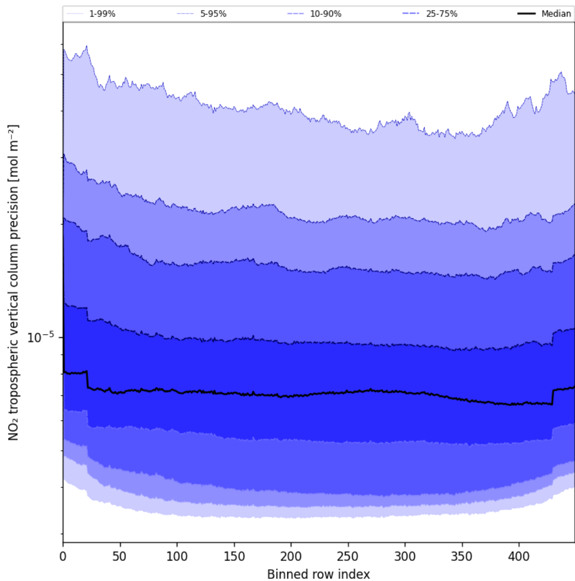
Figure 45: Along track statistics of “NO 2 tropospheric vertical column precision” for 2025-05-26 to 2025-05-27
