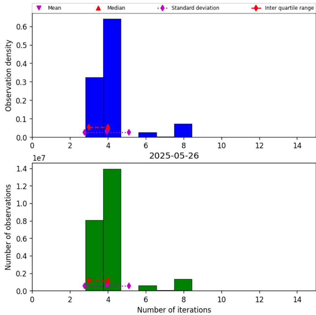
Figure 32: Histogram of “Number of iterations” for 2025-05-26 to 2025-05-27
