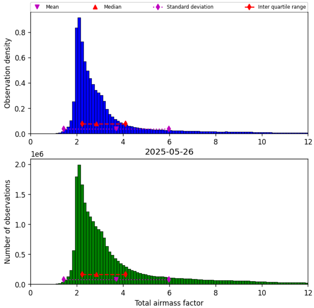
Figure 30: Histogram of “Total airmass factor” for 2025-05-26 to 2025-05-27
