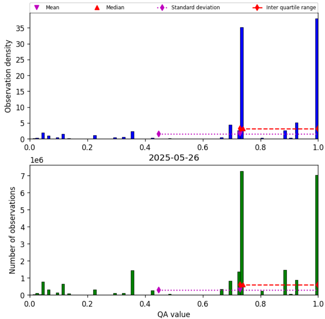
Figure 26: Histogram of “QA value” for 2025-05-26 to 2025-05-27
