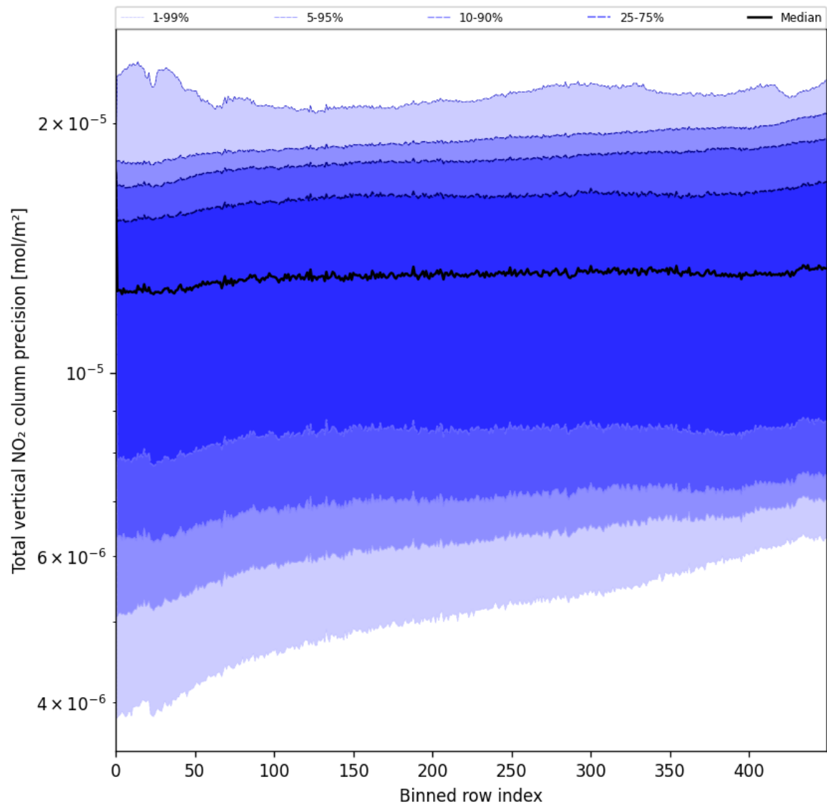
Figure 54: Along track statistics of “Total vertical NO 2 column precision” for 2025-05-26 to 2025-05-27
