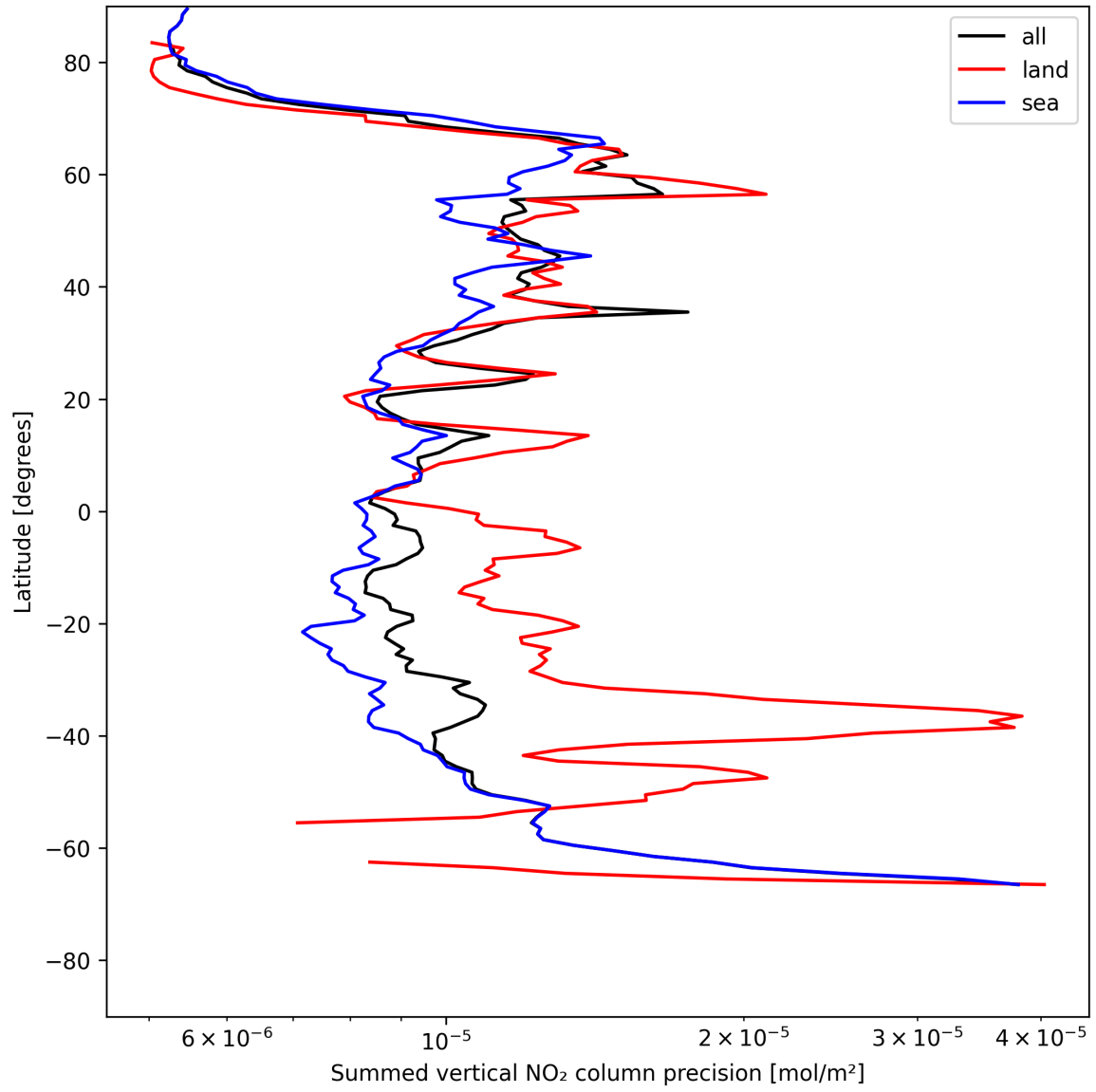
Figure 22: Zonal average of “Summed vertical NO 2 column precision” for 2025-05-26 to 2025-05-27.
