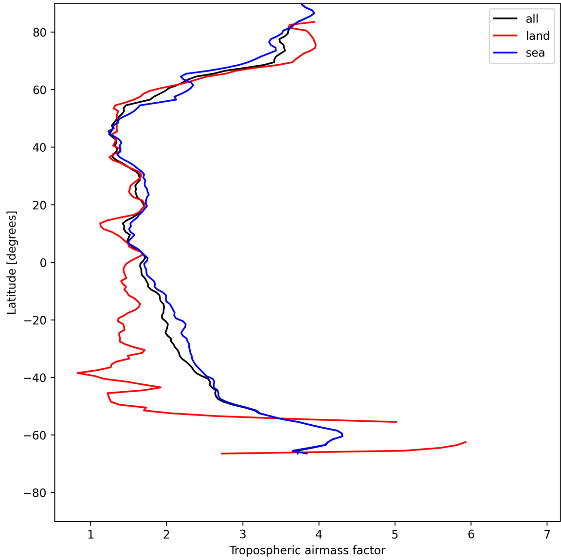
Figure 12: Zonal average of “Tropospheric air mass factor” for 2025-05-26 to 2025-05-27.
