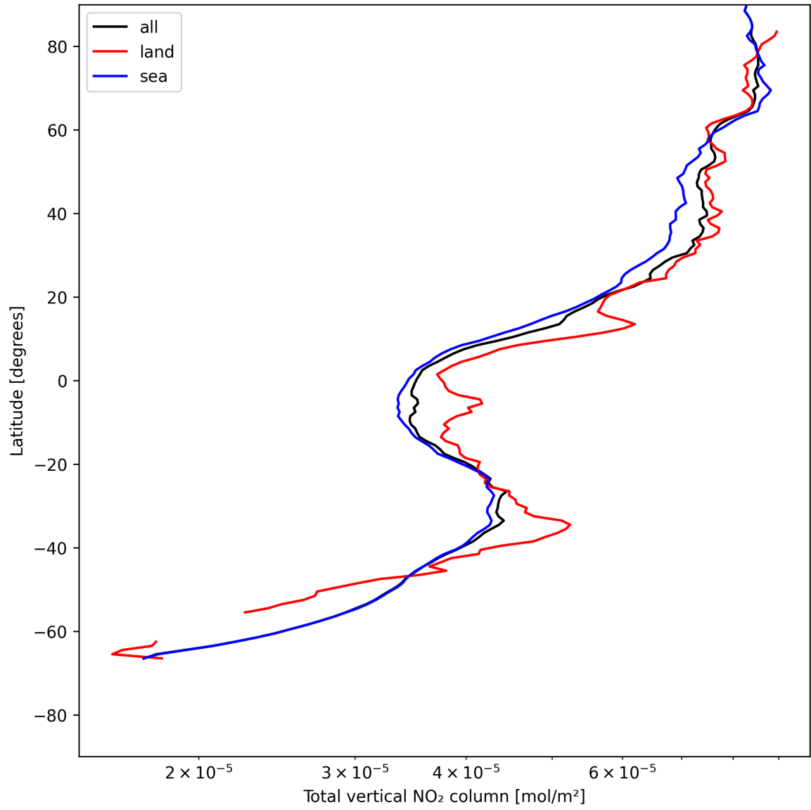
Figure 19: Zonal average of “Total vertical NO 2 column” for 2025-05-26 to 2025-05-27.
