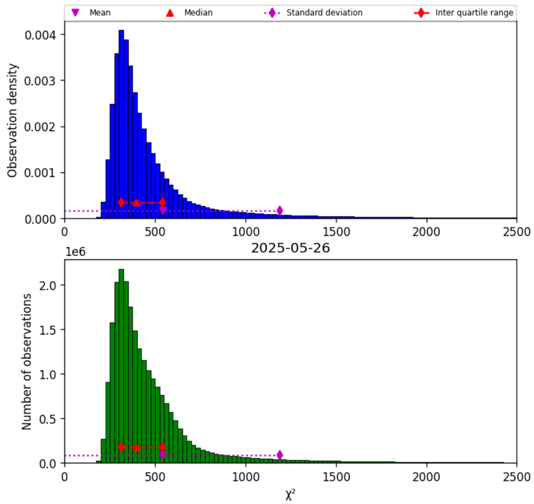
Figure 40: Histogram of “ \chi^2 ” for 2025-05-26 to 2025-05-27
