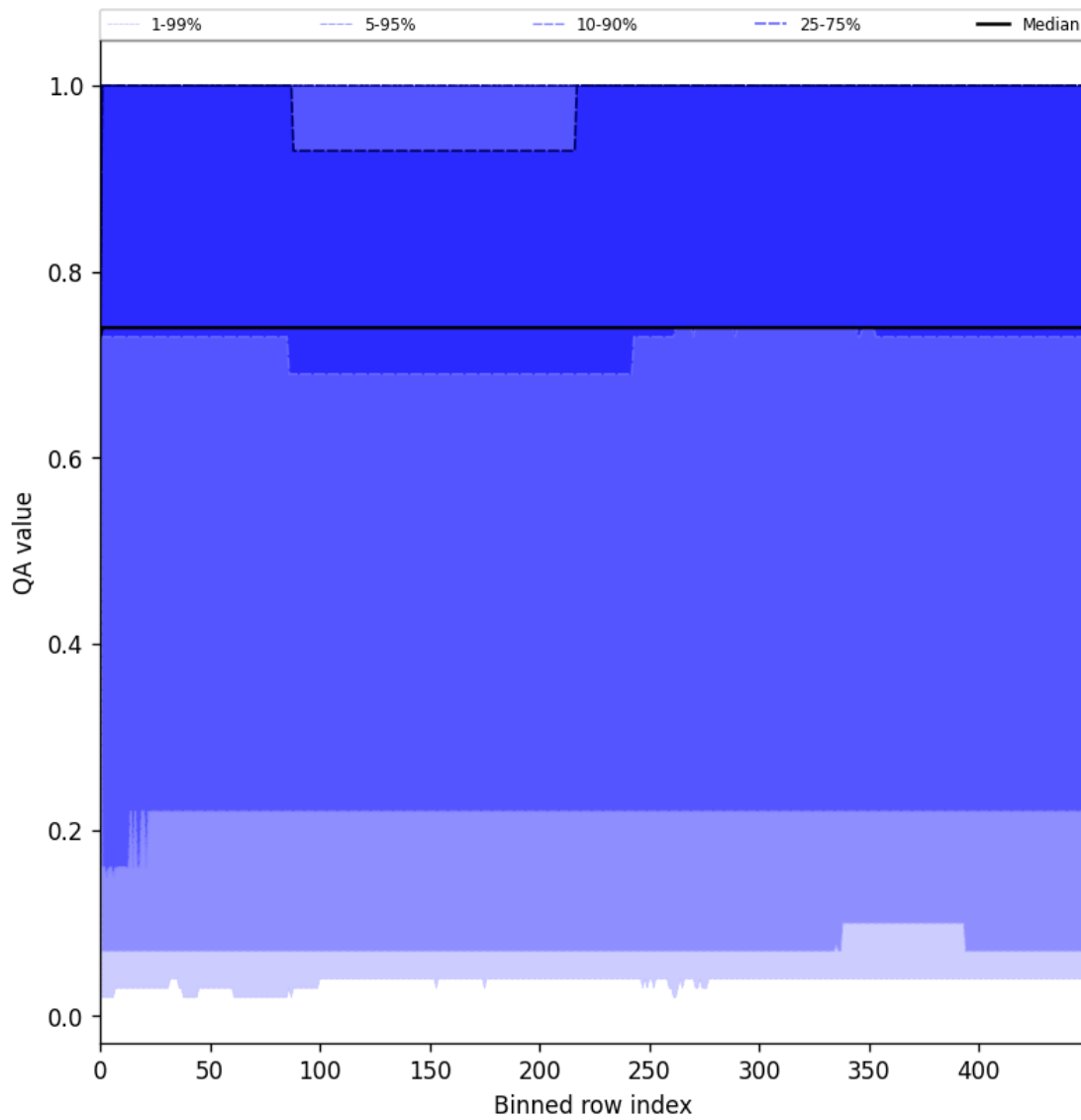
Figure 43: Along track statistics of “QA value” for 2025-05-26 to 2025-05-27
