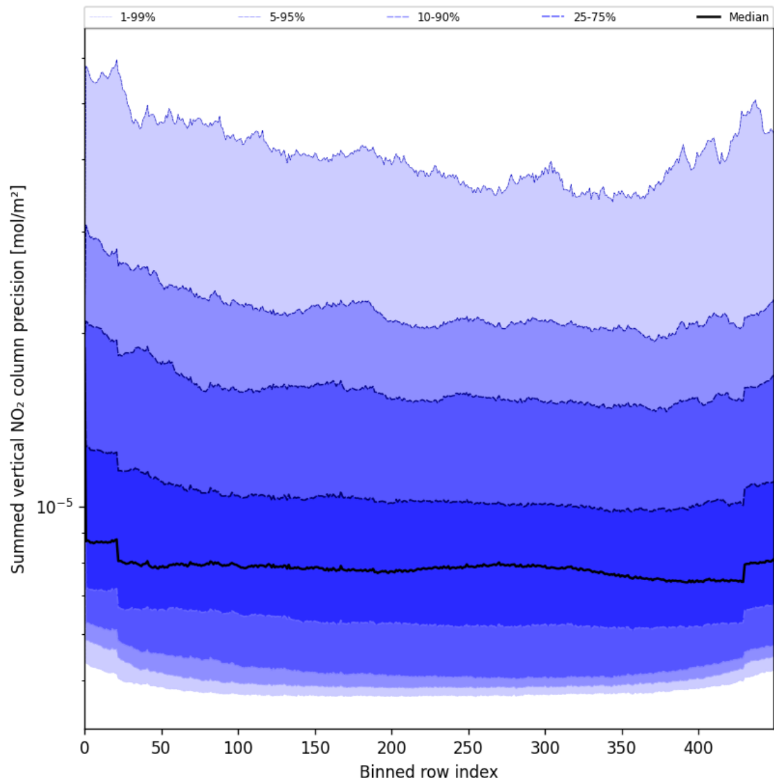
Figure 56: Along track statistics of “Summed vertical NO 2 column precision” for 2025-05-26 to 2025-05-27
