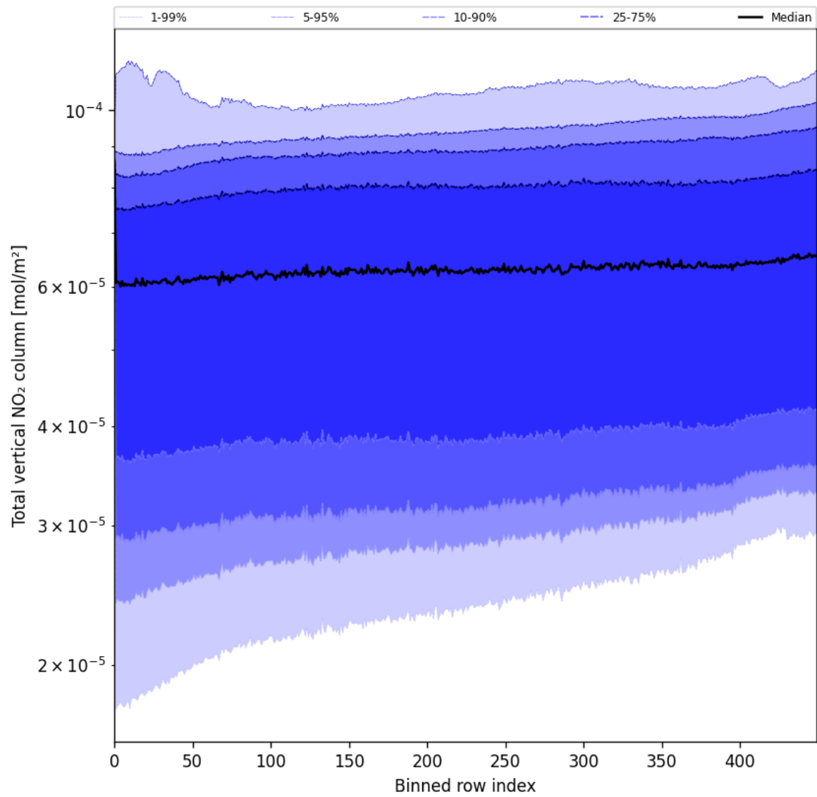
Figure 53: Along track statistics of “Total vertical NO 2 column” for 2025-05-26 to 2025-05-27
