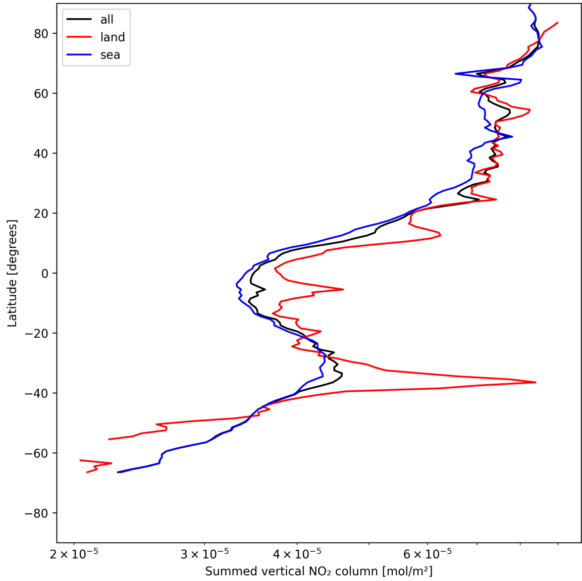
Figure 21: Zonal average of “Summed vertical NO 2 column” for 2025-05-26 to 2025-05-27.
