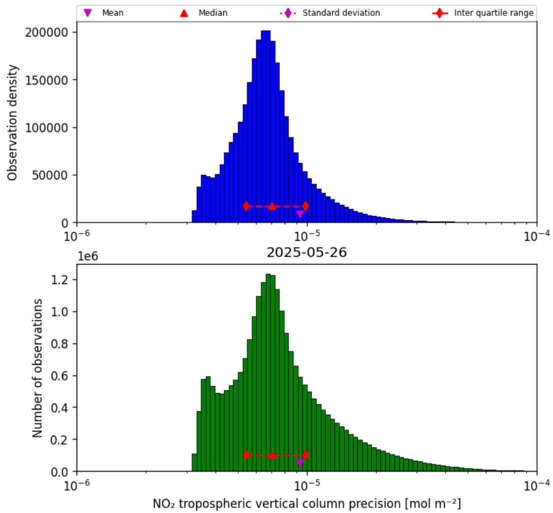
Figure 28: Histogram of “NO 2 tropospheric vertical column precision” for 2025-05-26 to 2025-05-27
