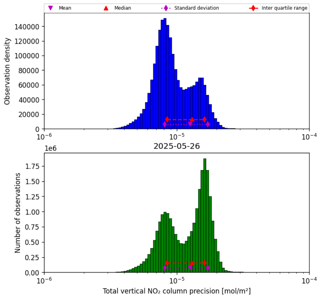
Figure 37: Histogram of “Total vertical NO 2 column precision” for 2025-05-26 to 2025-05-27
