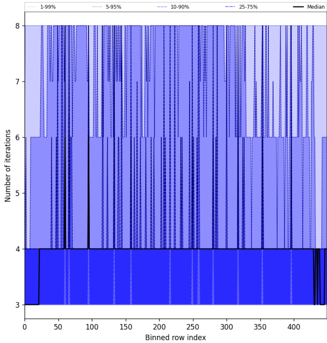
Figure 49: Along track statistics of “Number of iterations” for 2025-05-26 to 2025-05-27
