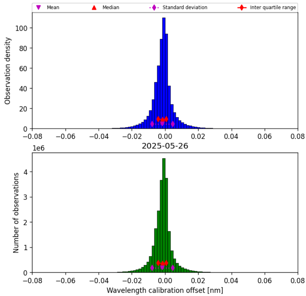
Figure 33: Histogram of “Wavelength calibration offset” for 2025-05-26 to 2025-05-27
