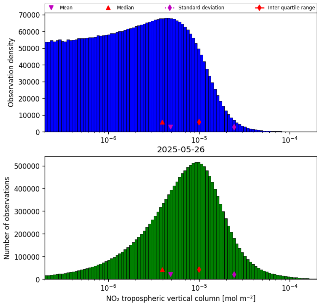
Figure 27: Histogram of “NO 2 tropospheric vertical column” for 2025-05-26 to 2025-05-27
