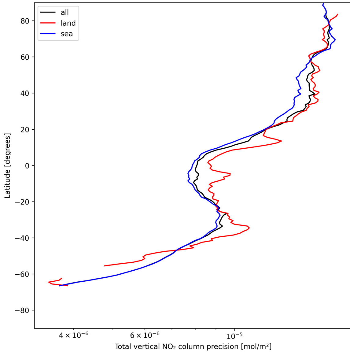
Figure 20: Zonal average of “Total vertical NO 2 column precision” for 2025-05-26 to 2025-05-27.
