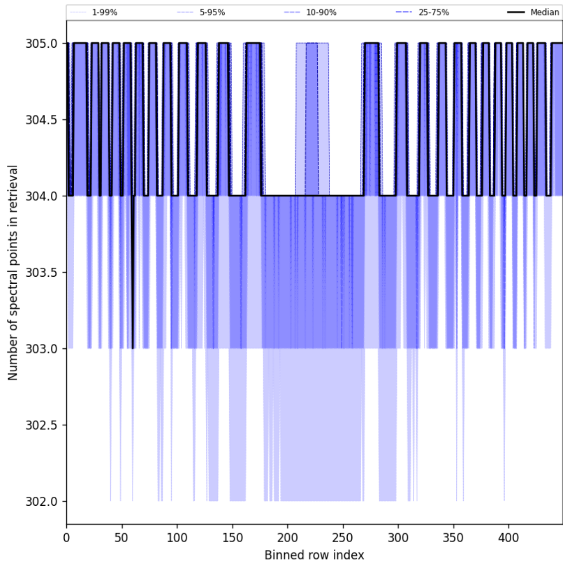
Figure 48: Along track statistics of “Number of spectral points in retrieval” for 2025-05-26 to 2025-05-27
