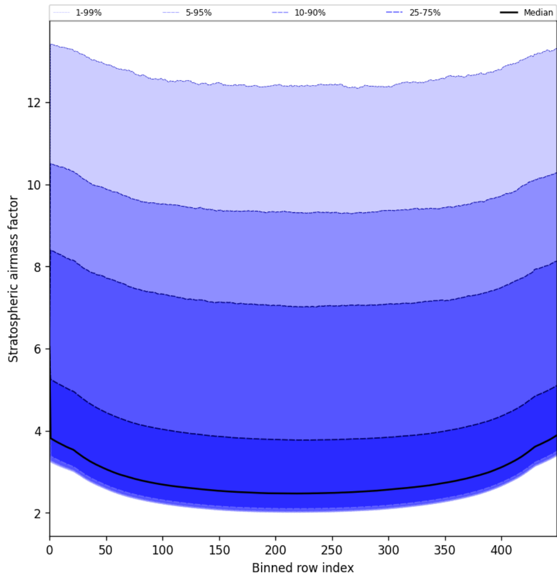
Figure 59: Along track statistics of “Stratospheric airmass factor” for 2025-05-26 to 2025-05-27
