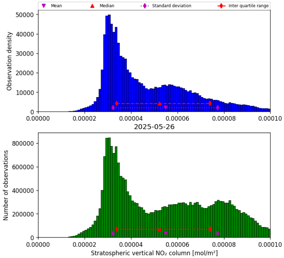
Figure 34: Histogram of “Stratospheric vertical NO 2 column” for 2025-05-26 to 2025-05-27
