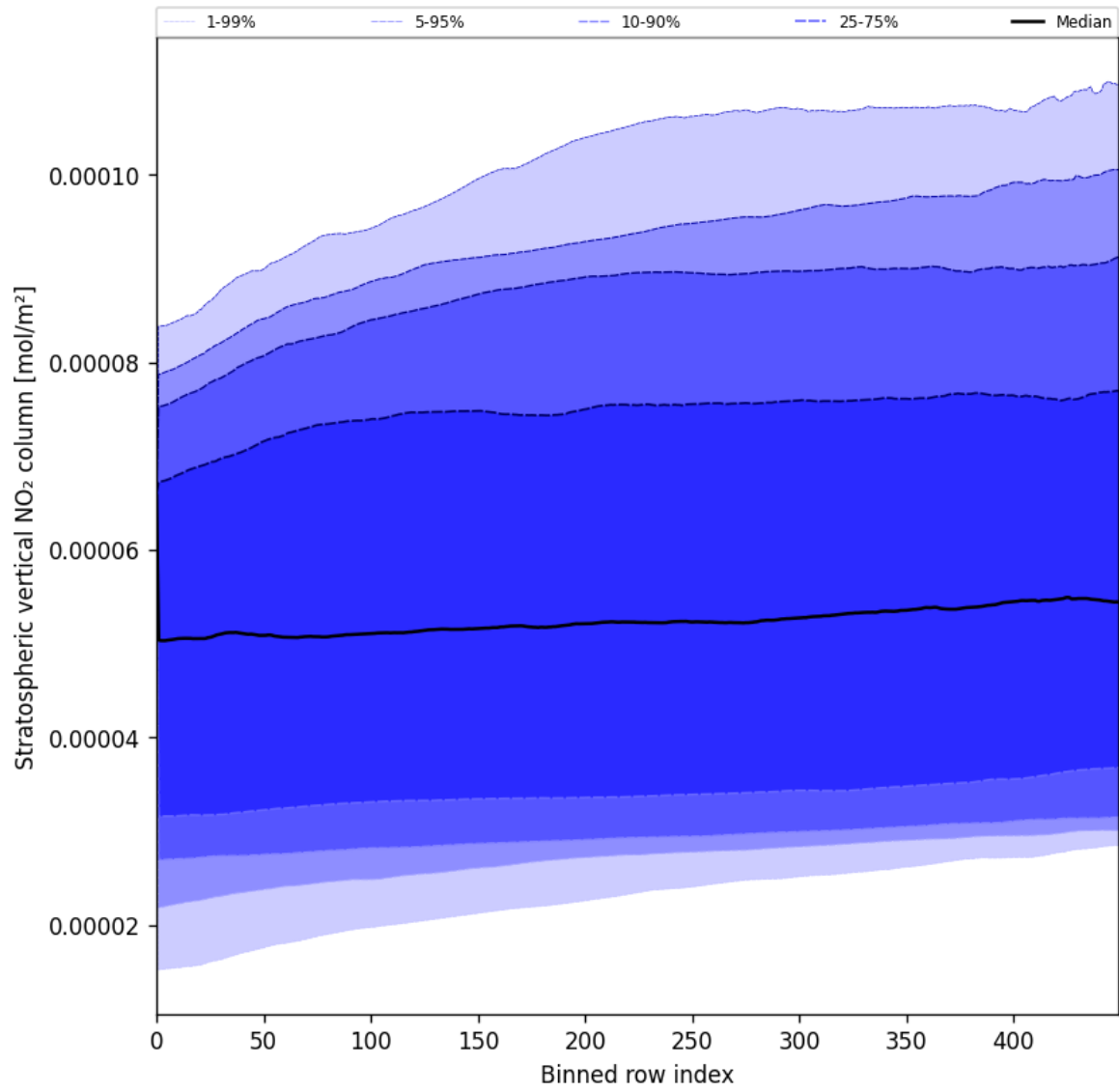
Figure 51: Along track statistics of “Stratospheric vertical NO 2 column” for 2025-05-26 to 2025-05-27
