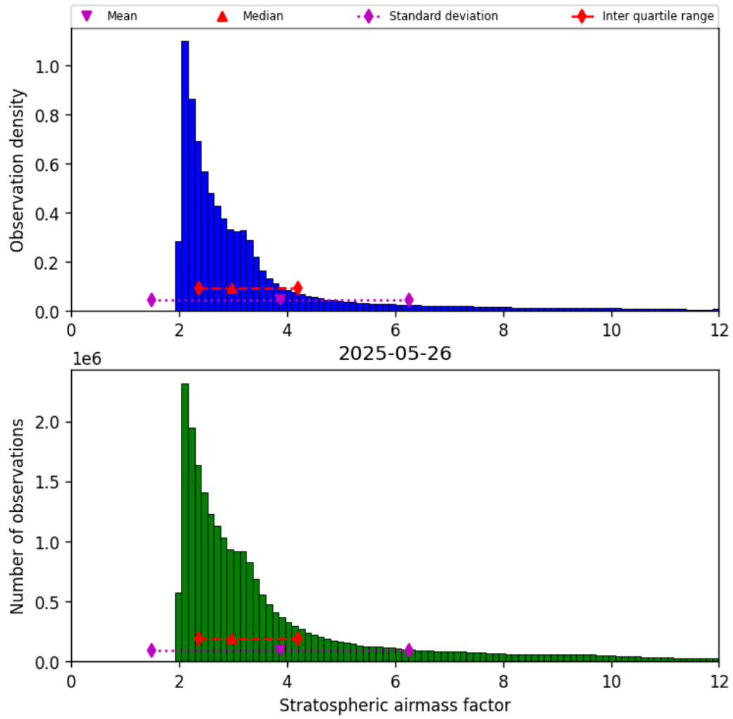
Figure 42: Histogram of “Stratospheric airmass factor” for 2025-05-26 to 2025-05-27
