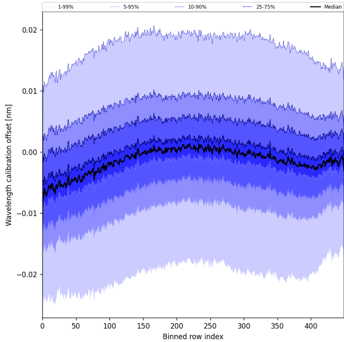
Figure 50: Along track statistics of “Wavelength calibration offset” for 2025-05-26 to 2025-05-27
