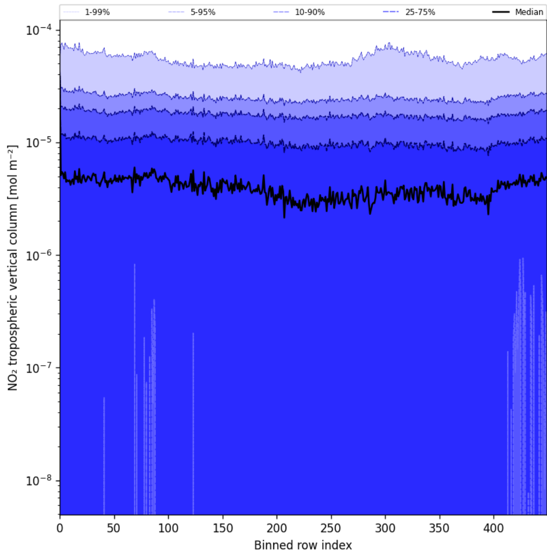
Figure 44: Along track statistics of “NO 2 tropospheric vertical column” for 2025-05-26 to 2025-05-27
