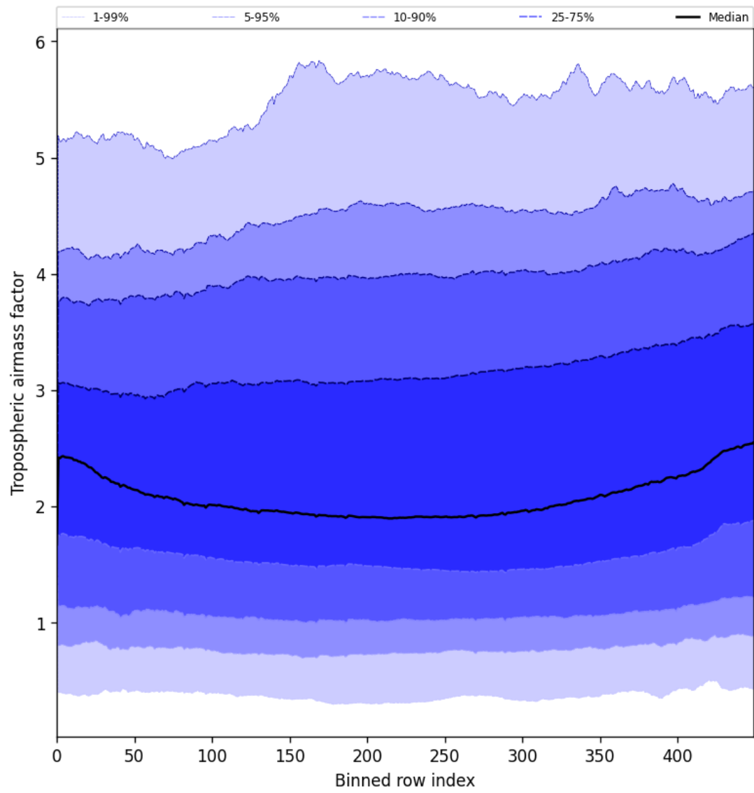
Figure 46: Along track statistics of “Tropospheric airmass factor” for 2025-05-26 to 2025-05-27
