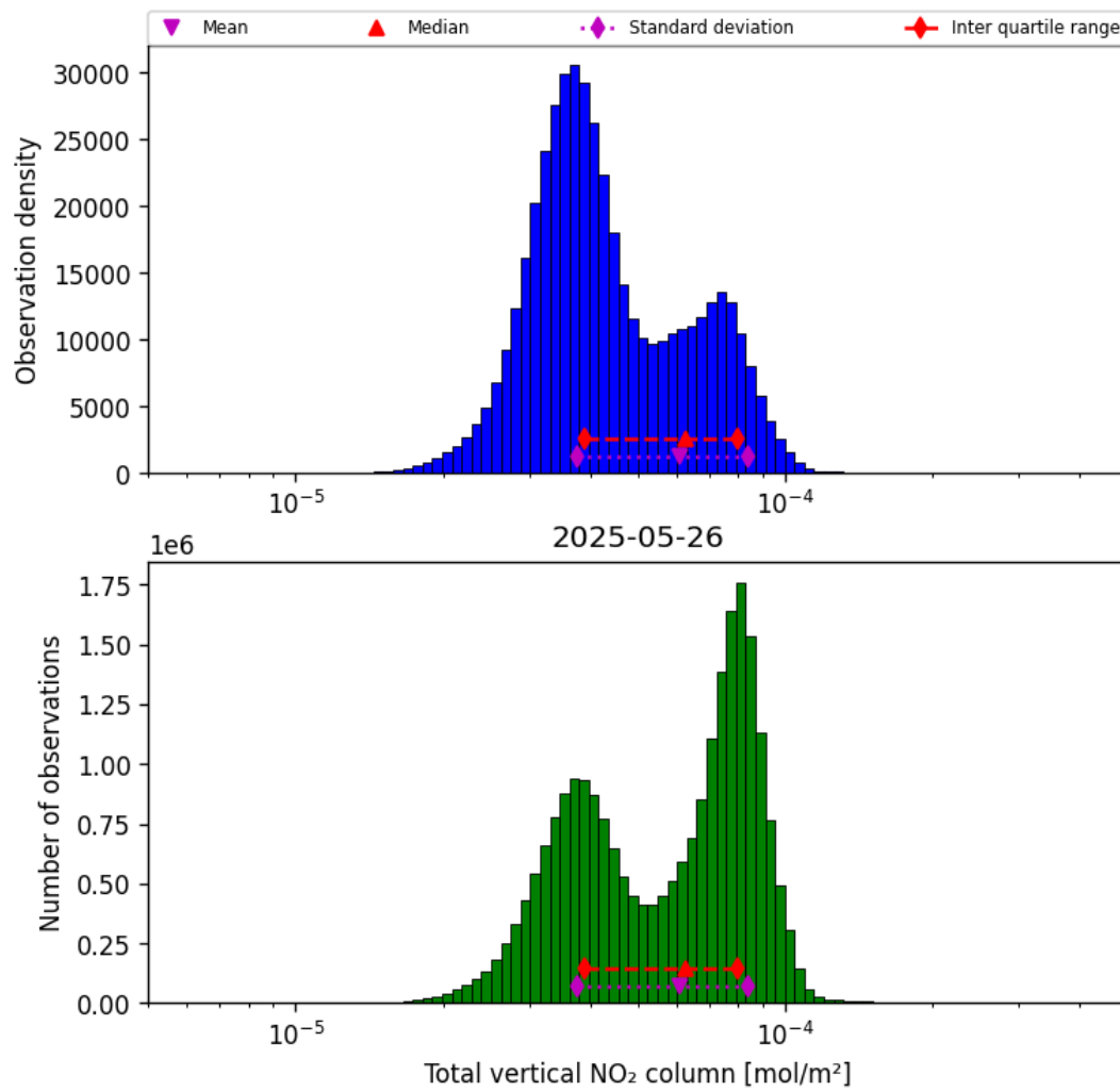
Figure 36: Histogram of "Total vertical NO 2 column" for 2025-05-26 to 2025-05-27
