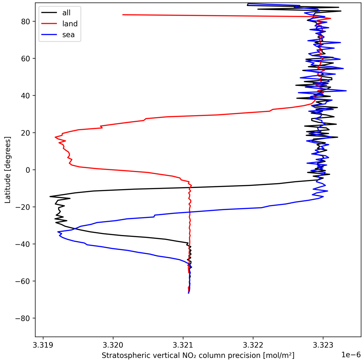
Figure 18: Zonal average of “Stratospheric vertical NO 2 column precision” for 2025-05-26 to 2025-05-27.
