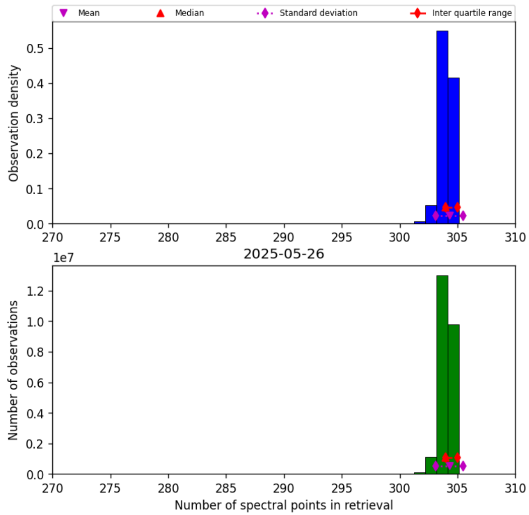
Figure 31: Histogram of “Number of spectral points in retrieval” for 2025-05-26 to 2025-05-27
