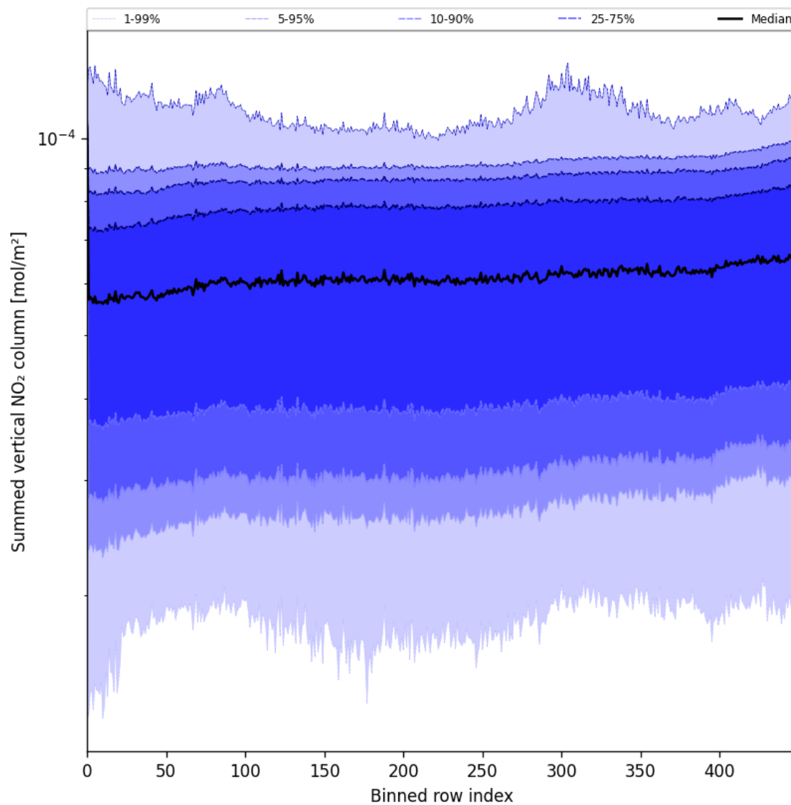
Figure 55: Along track statistics of “Summed vertical NO 2 column” for 2025-05-26 to 2025-05-27
