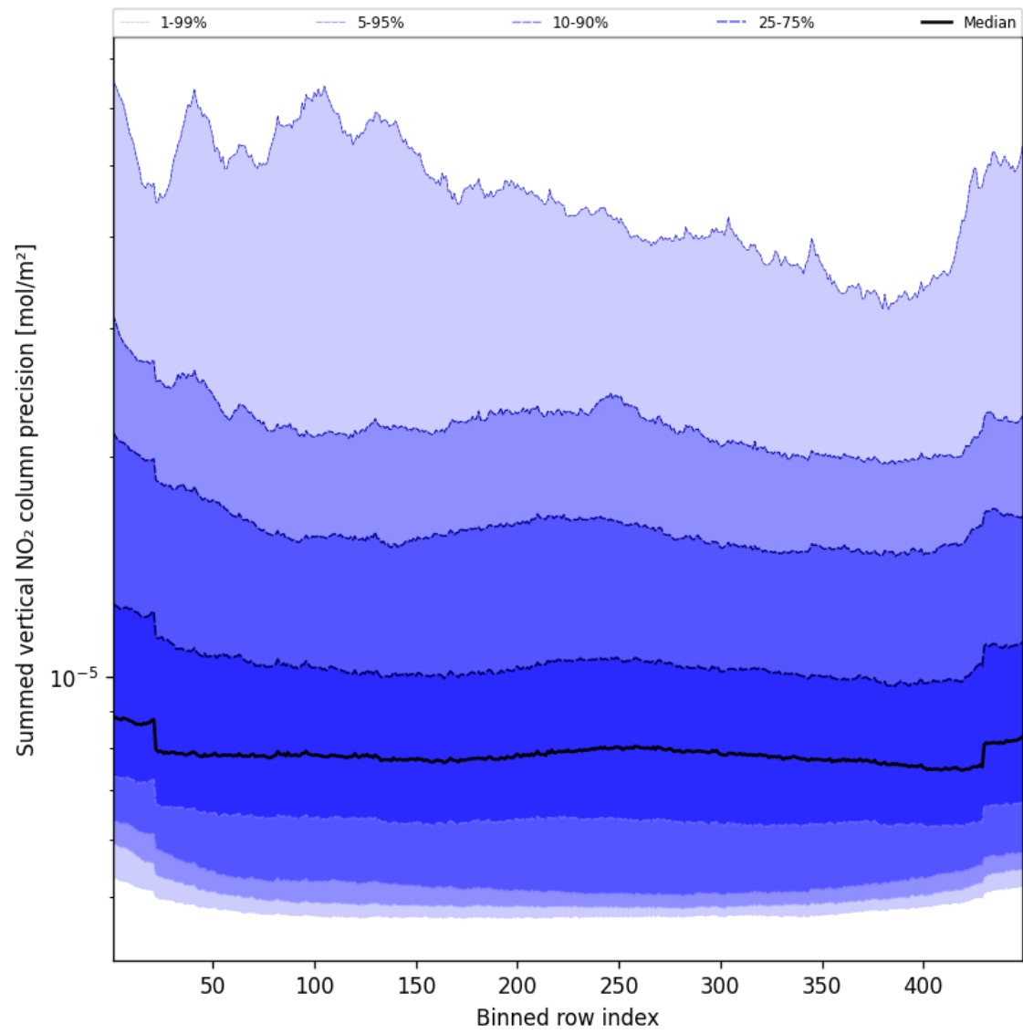
Figure 56: Along track statistics of “Summed vertical NO 2 column precision” for 2025-05-27 to 2025-05-28
