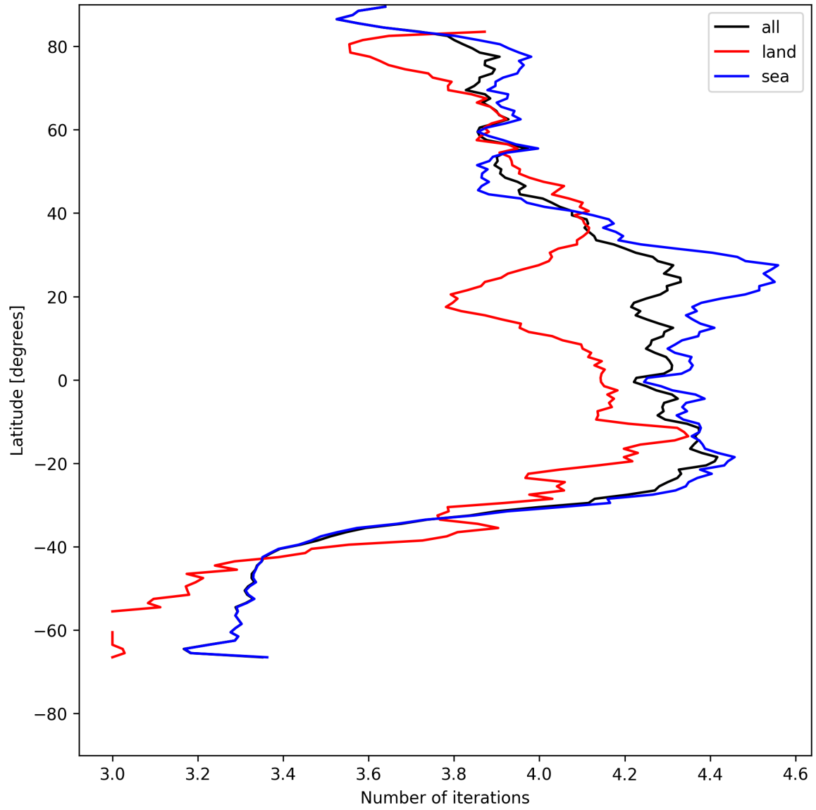
Figure 15: Zonal average of “Number of iterations” for 2025-05-27 to 2025-05-28.
