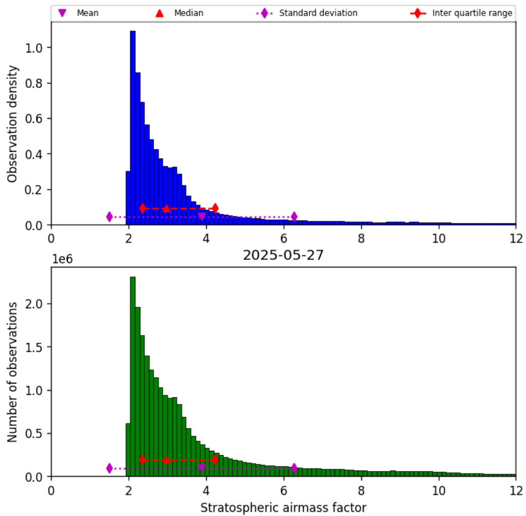
Figure 42: Histogram of “Stratospheric airmass factor” for 2025-05-27 to 2025-05-28
