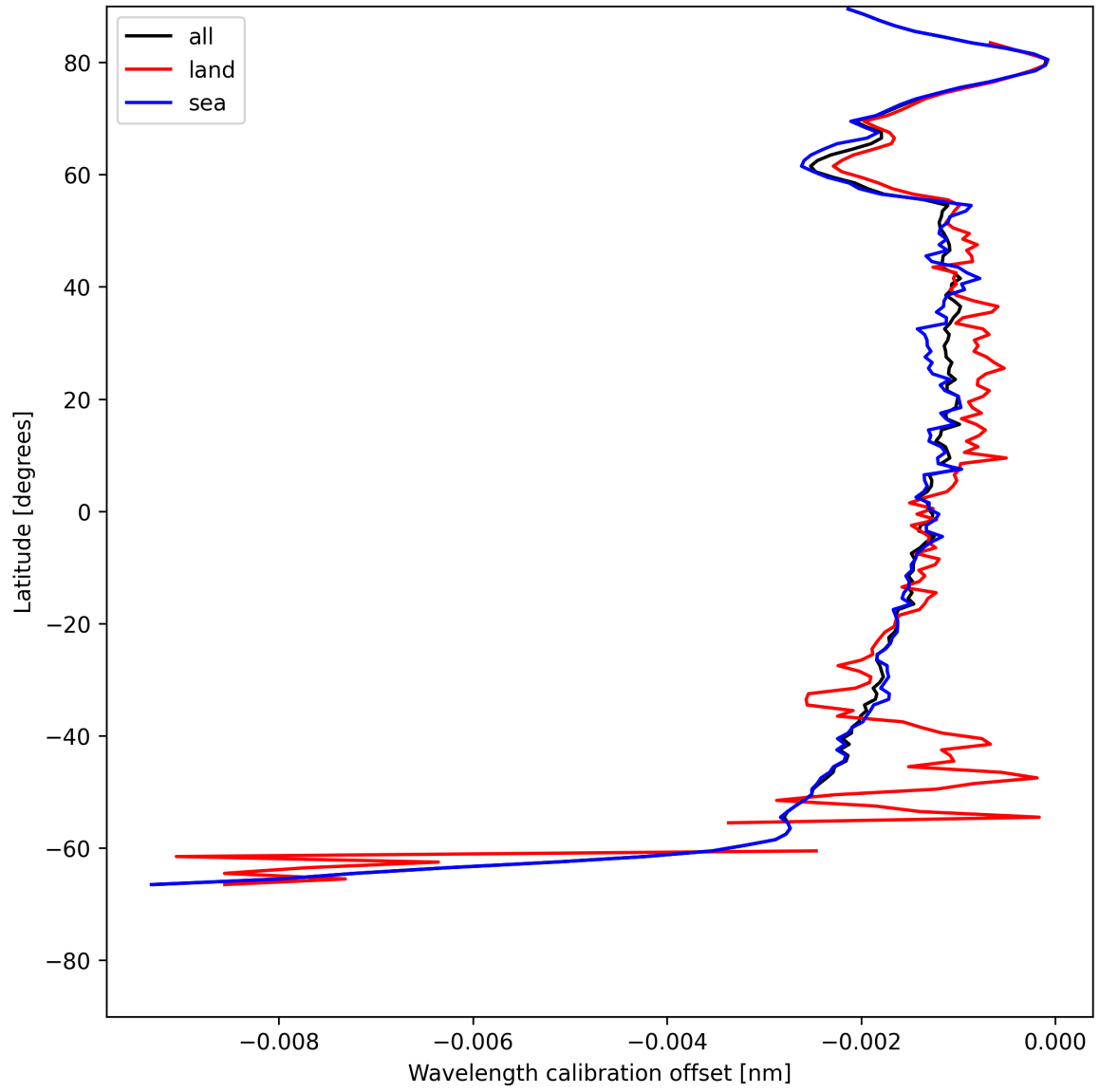
Figure 16: Zonal average of “Wavelength calibration offset” for 2025-05-27 to 2025-05-28.
