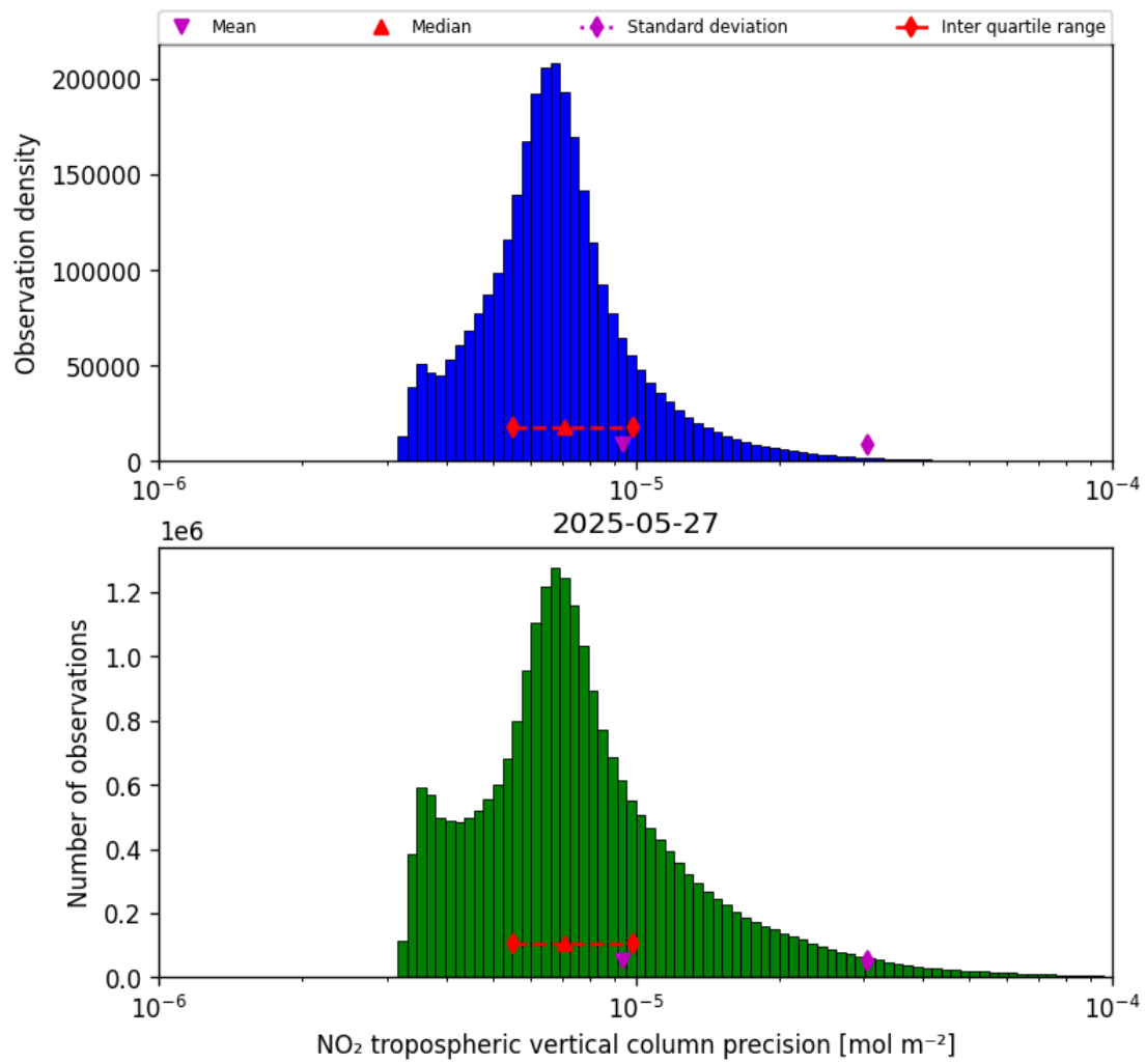
Figure 28: Histogram of “NO 2 tropospheric vertical column precision” for 2025-05-27 to 2025-05-28
