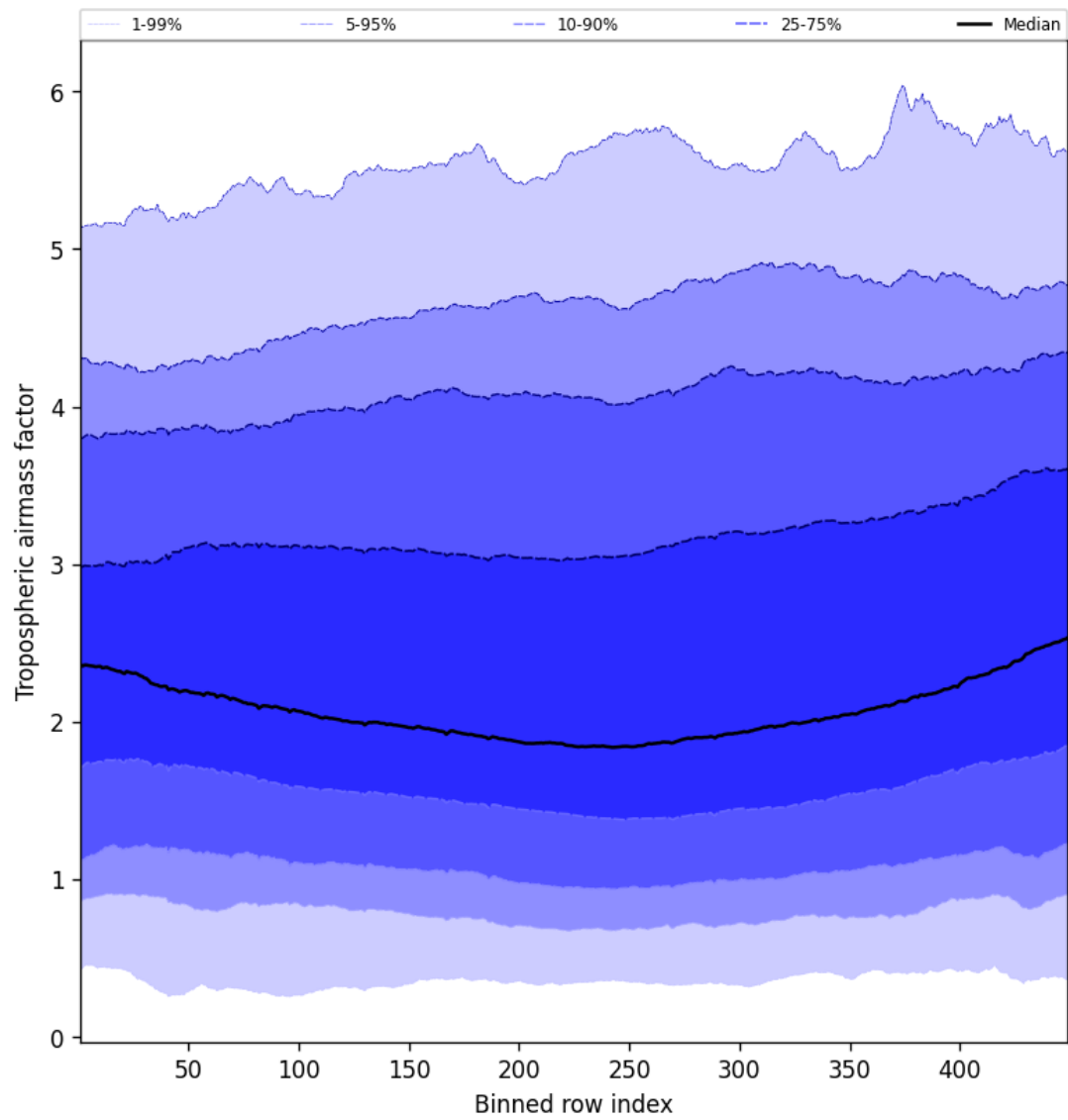
Figure 46: Along track statistics of “Tropospheric airmass factor” for 2025-05-27 to 2025-05-28
