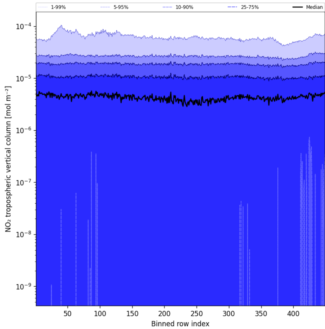
Figure 44: Along track statistics of “NO 2 tropospheric vertical column” for 2025-05-27 to 2025-05-28
