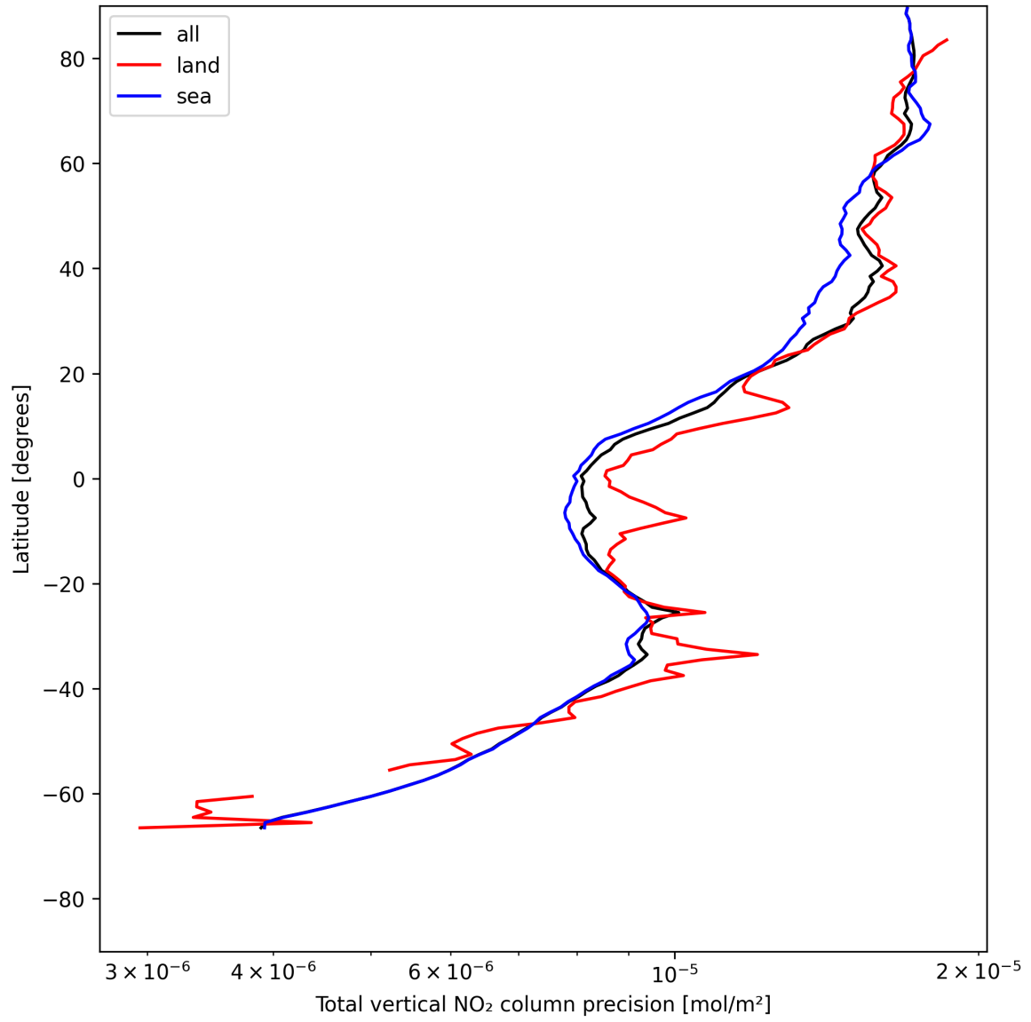
Figure 20: Zonal average of “Total vertical NO 2 column precision” for 2025-05-27 to 2025-05-28.
