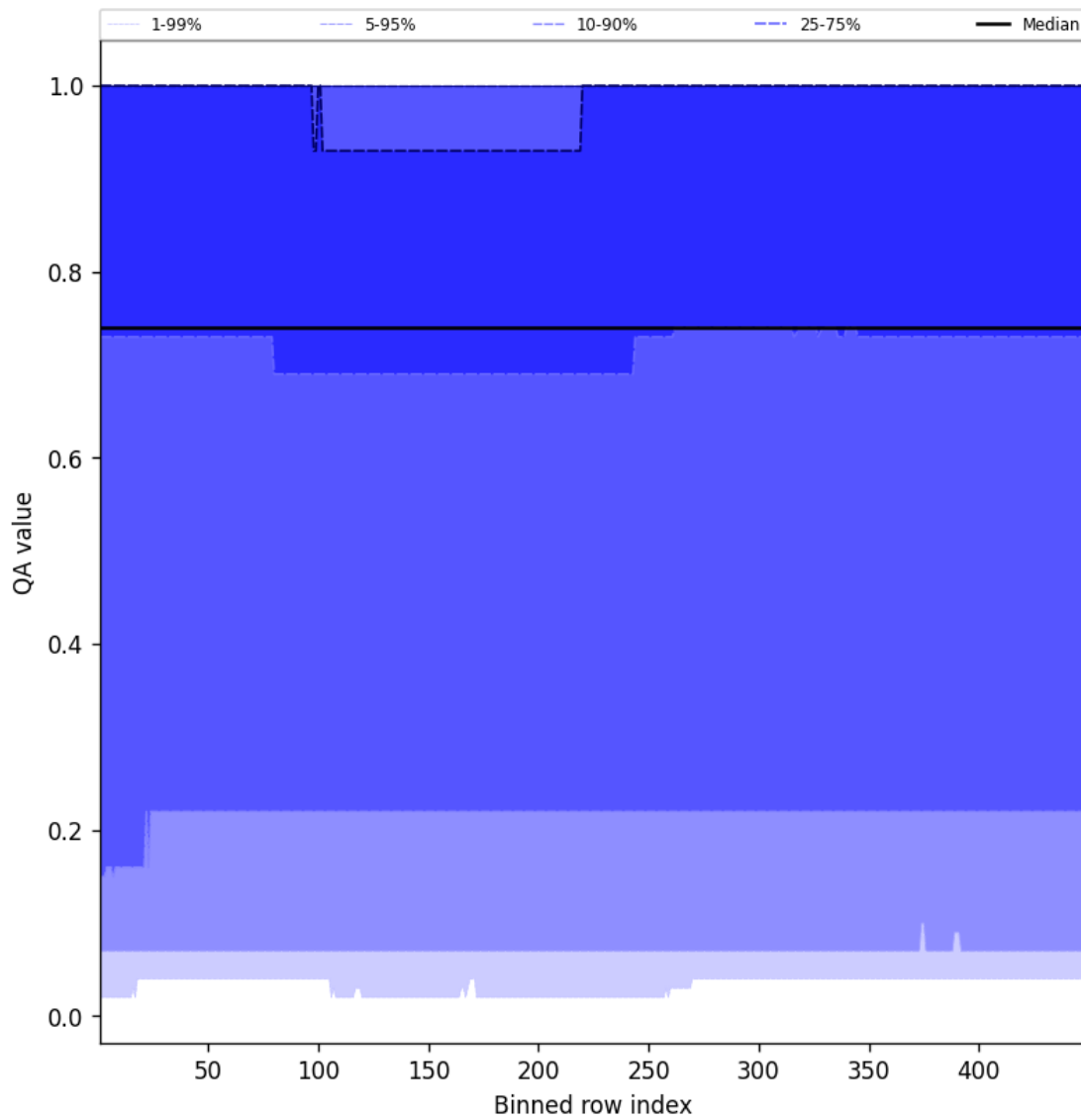
Figure 43: Along track statistics of “QA value” for 2025-05-27 to 2025-05-28
