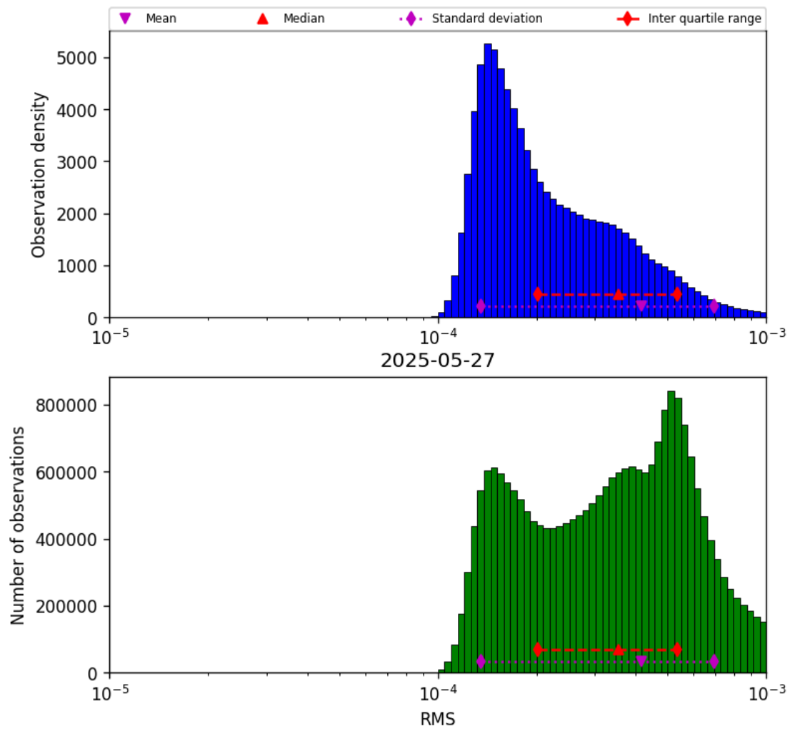
Figure 41: Histogram of “RMS” for 2025-05-27 to 2025-05-28
