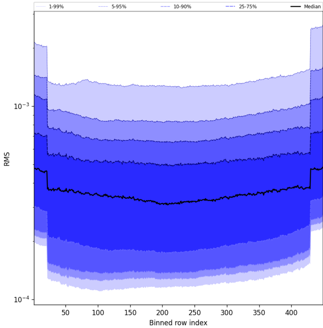
Figure 58: Along track statistics of “RMS” for 2025-05-27 to 2025-05-28
