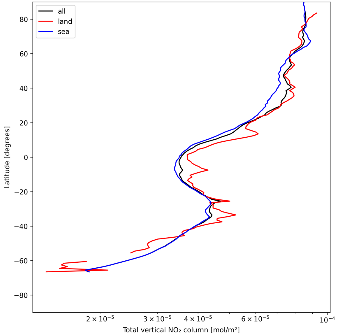
Figure 19: Zonal average of “Total vertical NO 2 column” for 2025-05-27 to 2025-05-28.
