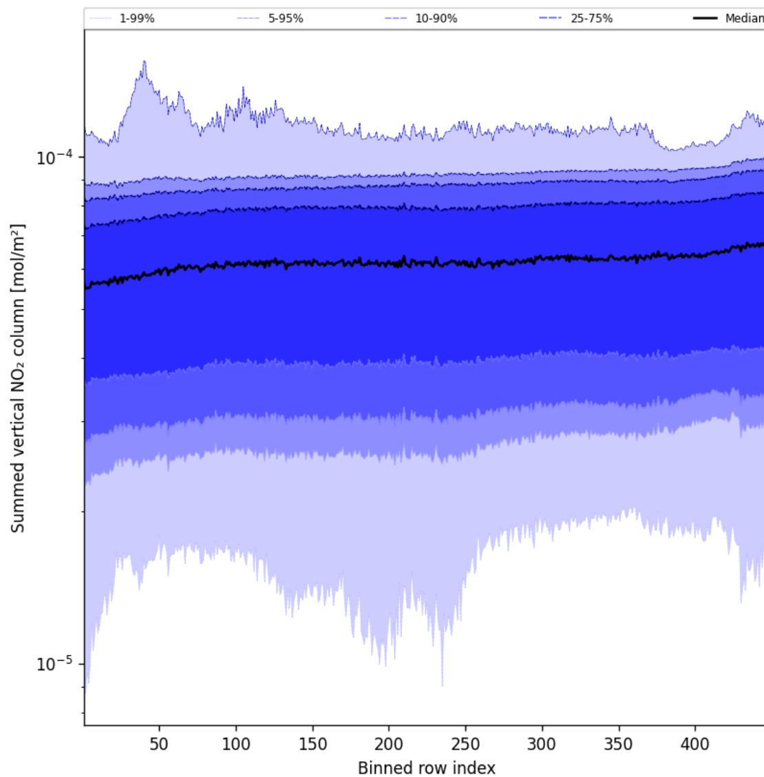
Figure 55: Along track statistics of “Summed vertical NO 2 column” for 2025-05-27 to 2025-05-28
