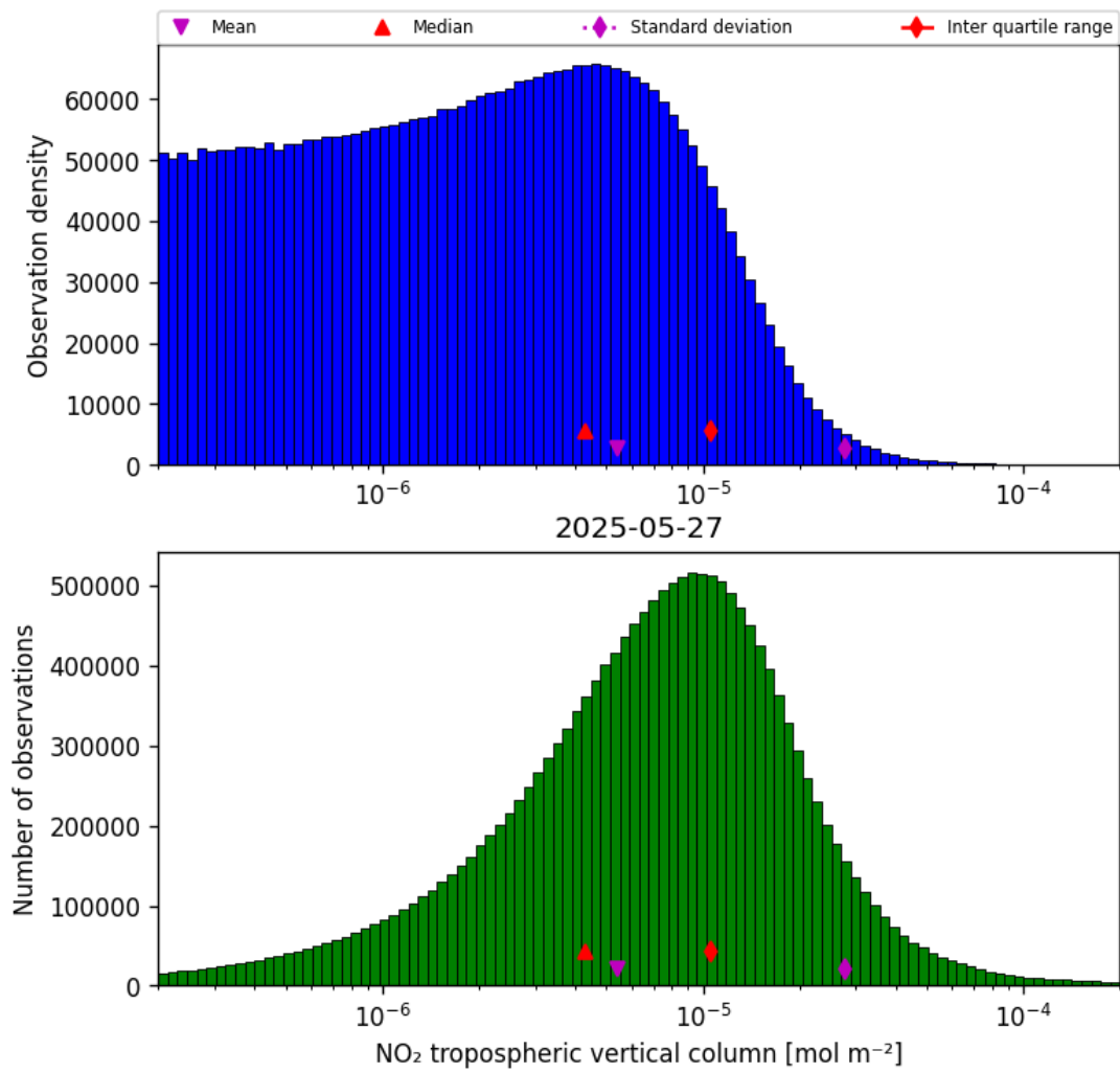
Figure 27: Histogram of “NO 2 tropospheric vertical column” for 2025-05-27 to 2025-05-28
