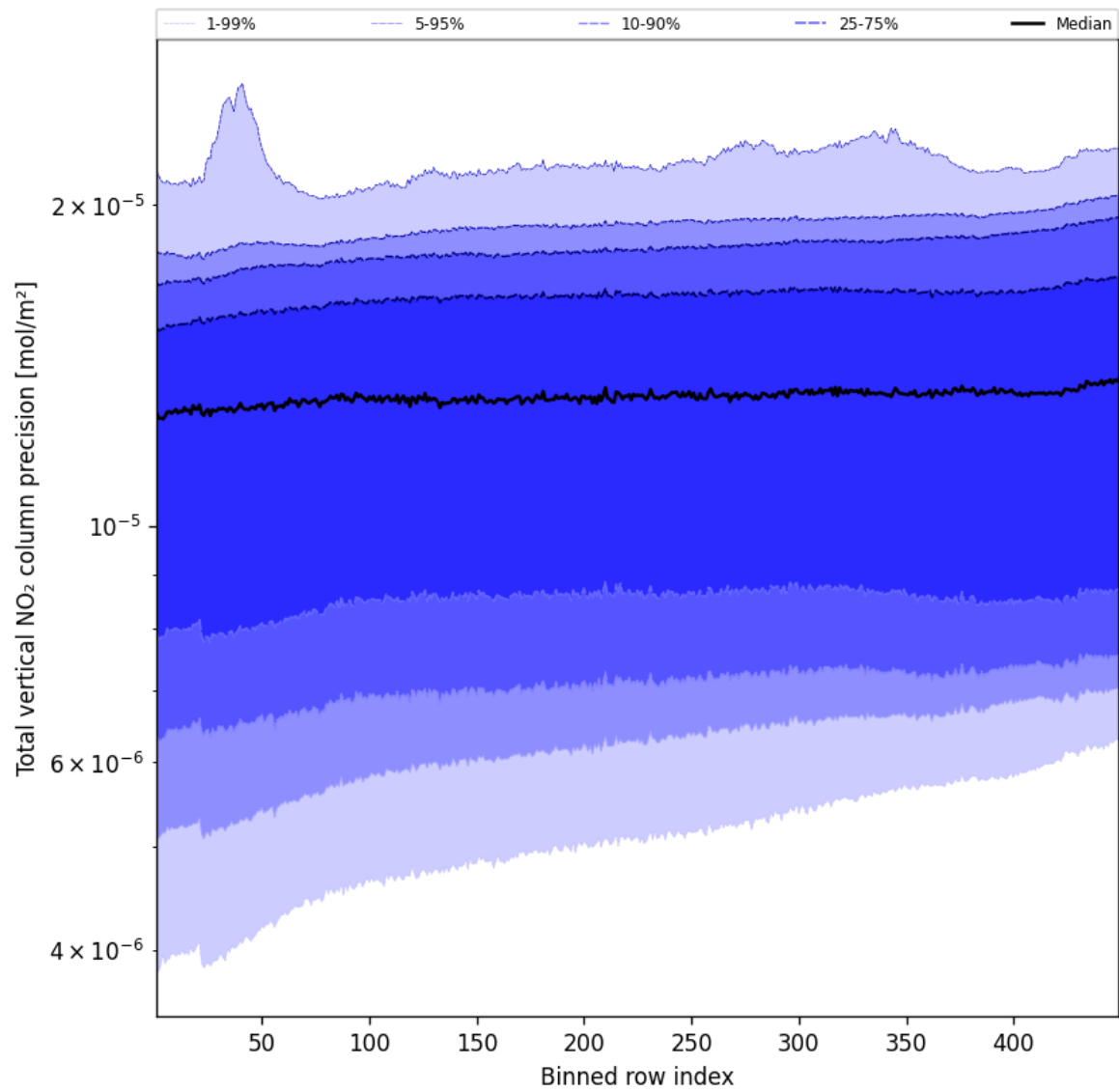
Figure 54: Along track statistics of “Total vertical NO 2 column precision” for 2025-05-27 to 2025-05-28
