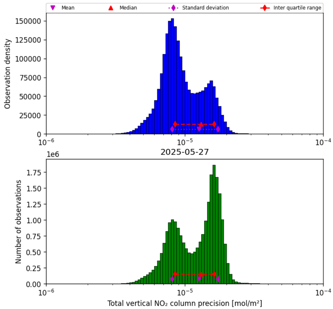
Figure 37: Histogram of “Total vertical NO 2 column precision” for 2025-05-27 to 2025-05-28
