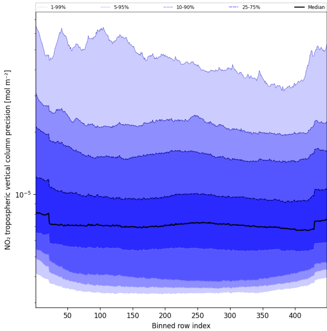
Figure 45: Along track statistics of “NO 2 tropospheric vertical column precision” for 2025-05-27 to 2025-05-28
