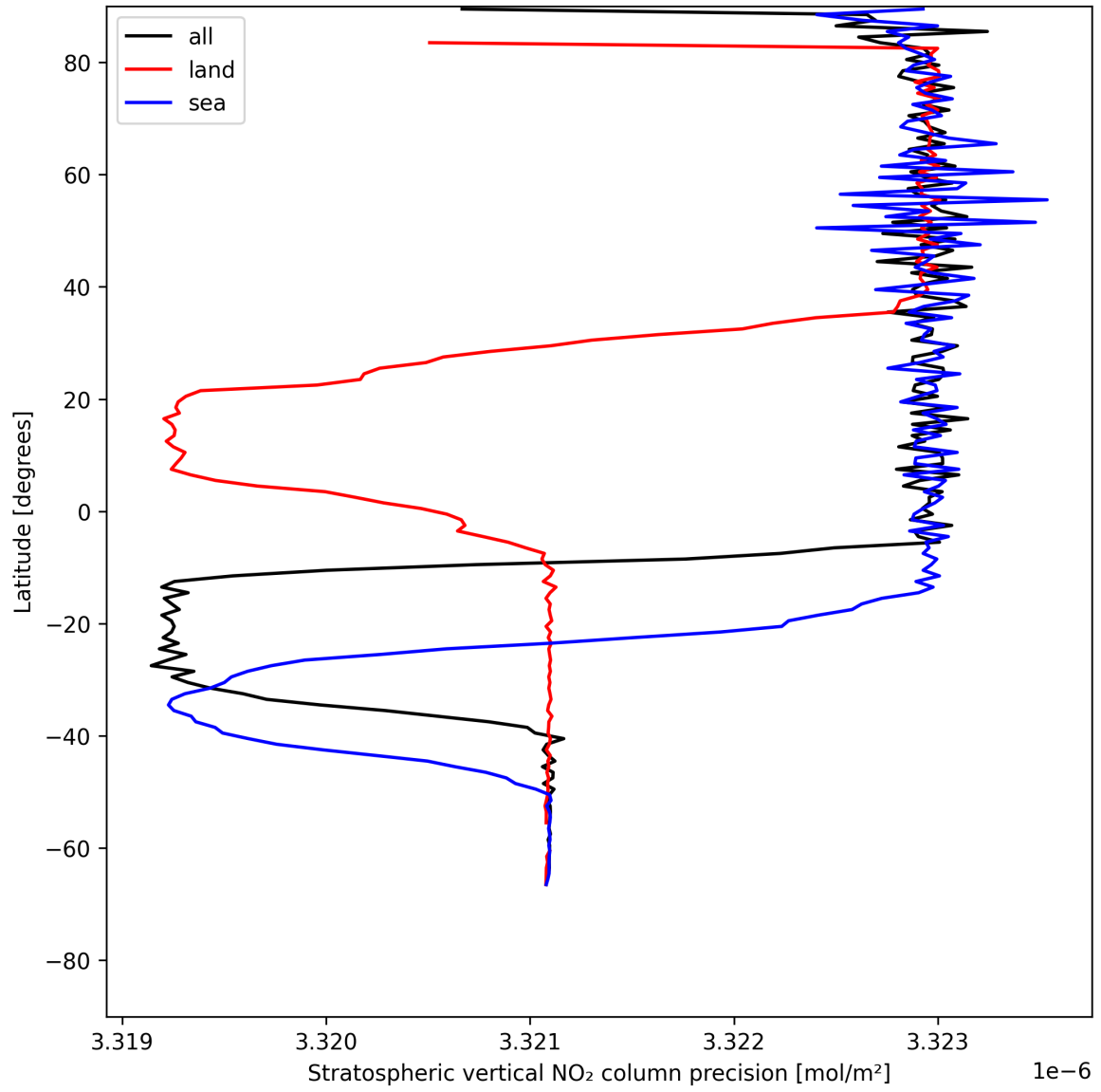
Figure 18: Zonal average of “Stratospheric vertical NO 2 column precision” for 2025-05-27 to 2025-05-28.
