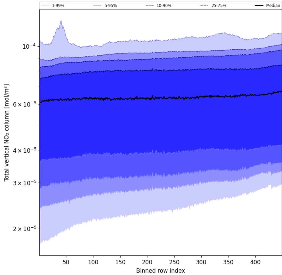
Figure 53: Along track statistics of “Total vertical NO 2 column” for 2025-05-27 to 2025-05-28
