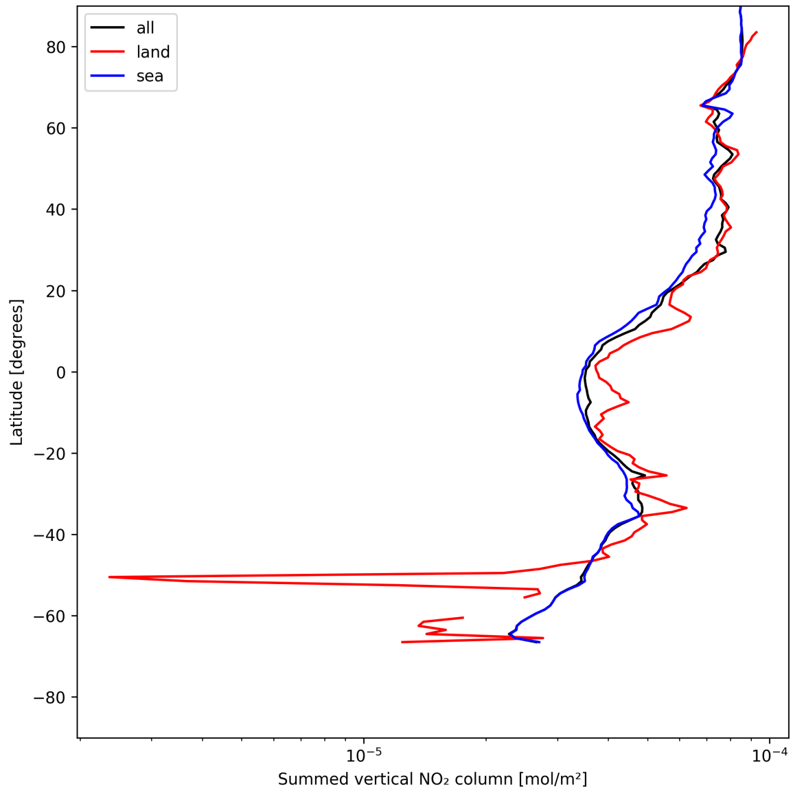
Figure 21: Zonal average of “Summed vertical NO 2 column” for 2025-05-27 to 2025-05-28.
