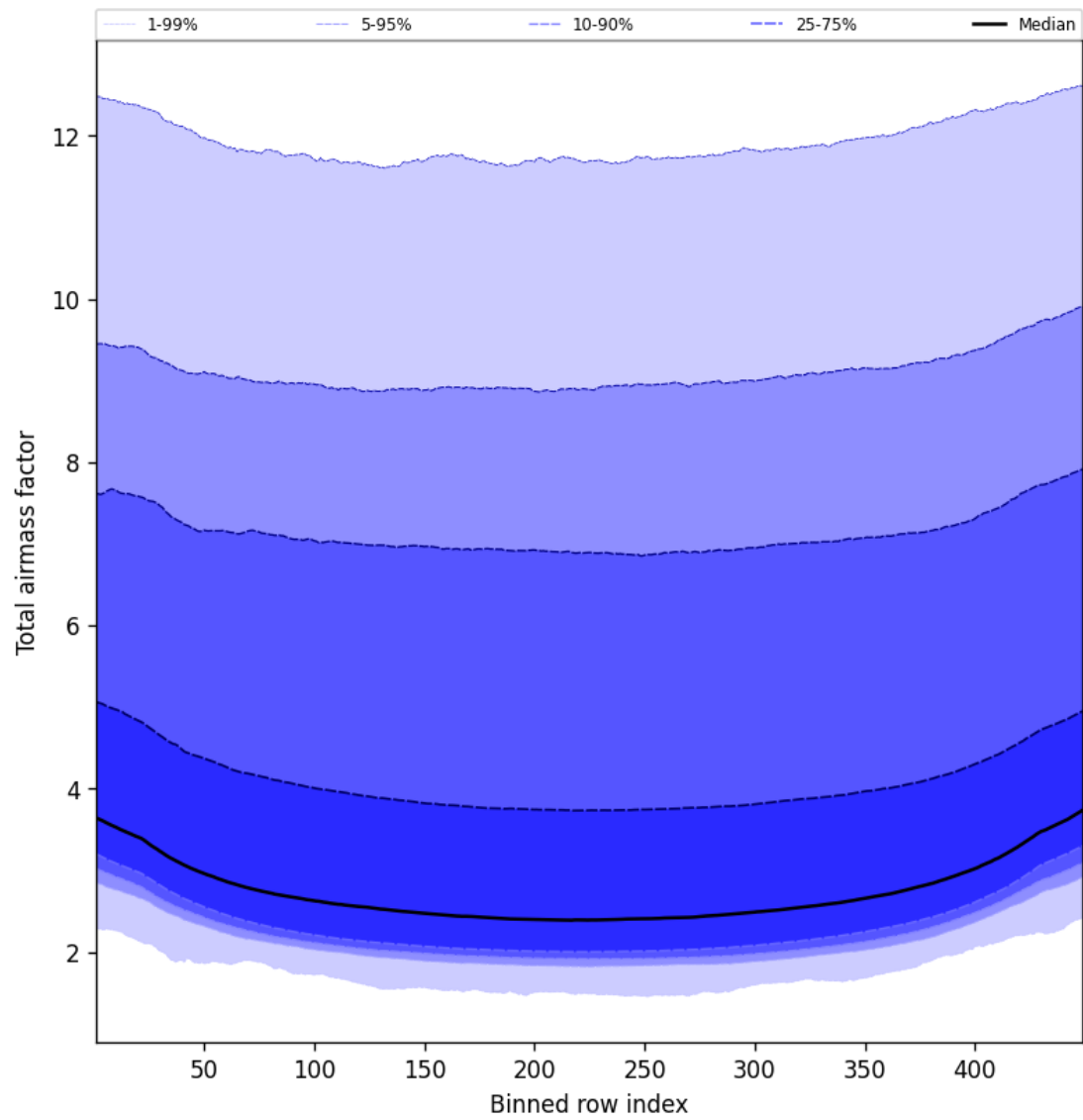
Figure 47: Along track statistics of “Total airmass factor” for 2025-05-27 to 2025-05-28
