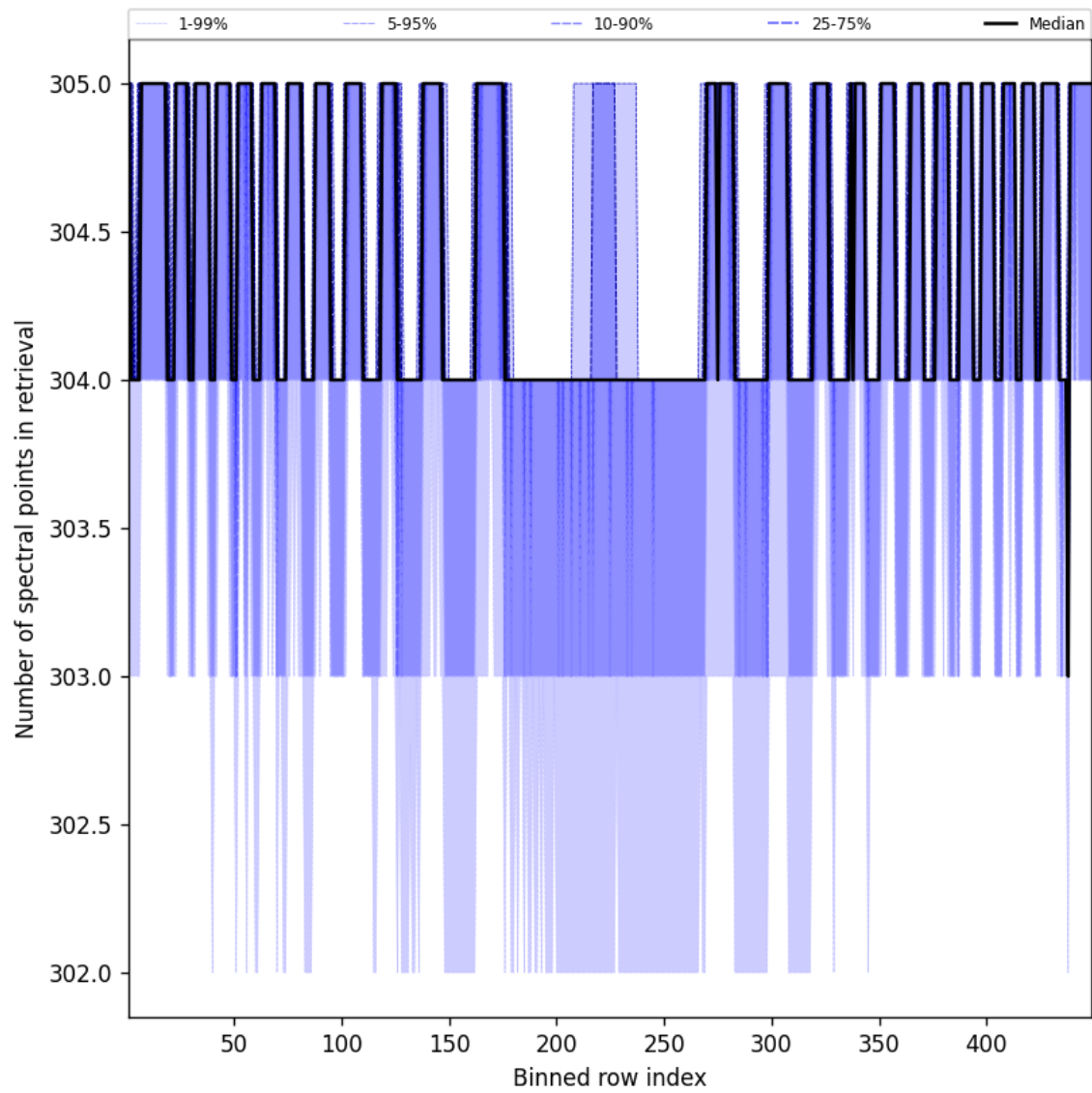
Figure 48: Along track statistics of “Number of spectral points in retrieval” for 2025-05-27 to 2025-05-28
