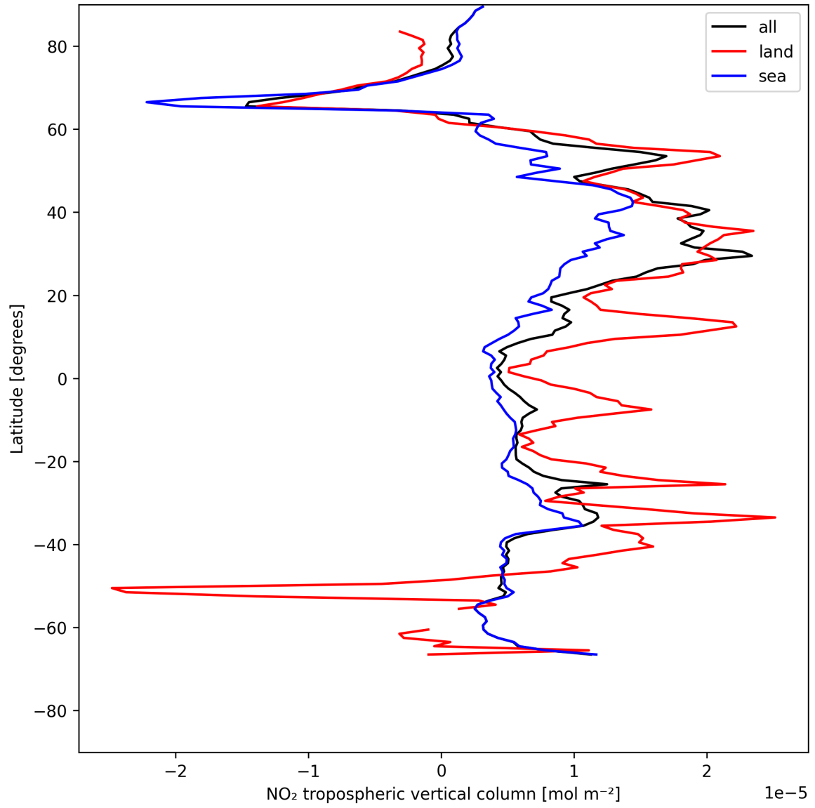
Figure 10: Zonal average of “NO 2 tropospheric vertical column” for 2025-05-27 to 2025-05-28.
