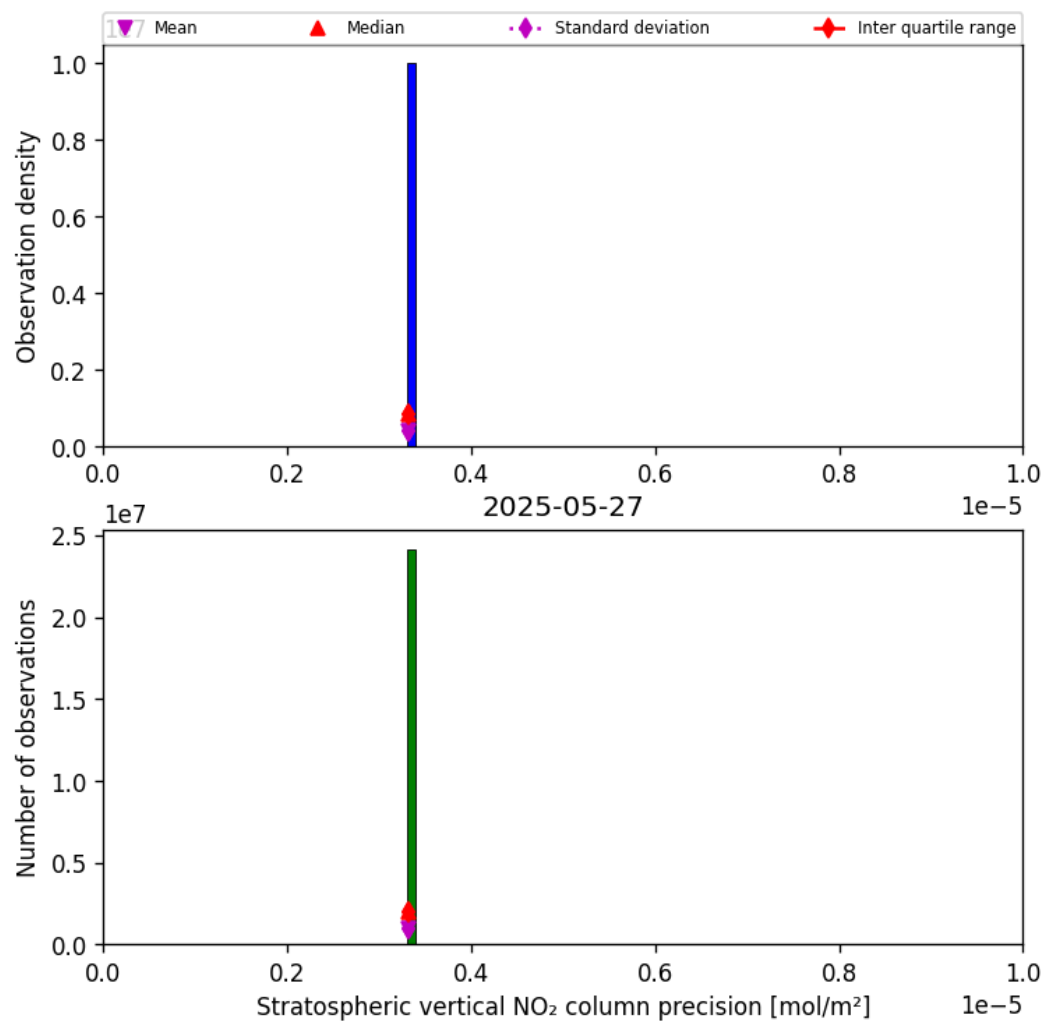
Figure 35: Histogram of “Stratospheric vertical NO 2 column precision” for 2025-05-27 to 2025-05-28
