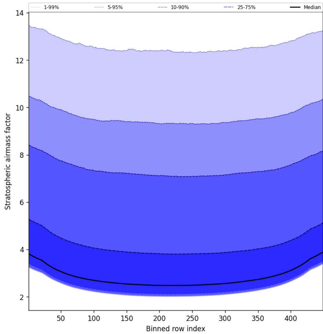
Figure 59: Along track statistics of “Stratospheric airmass factor” for 2025-05-27 to 2025-05-28
