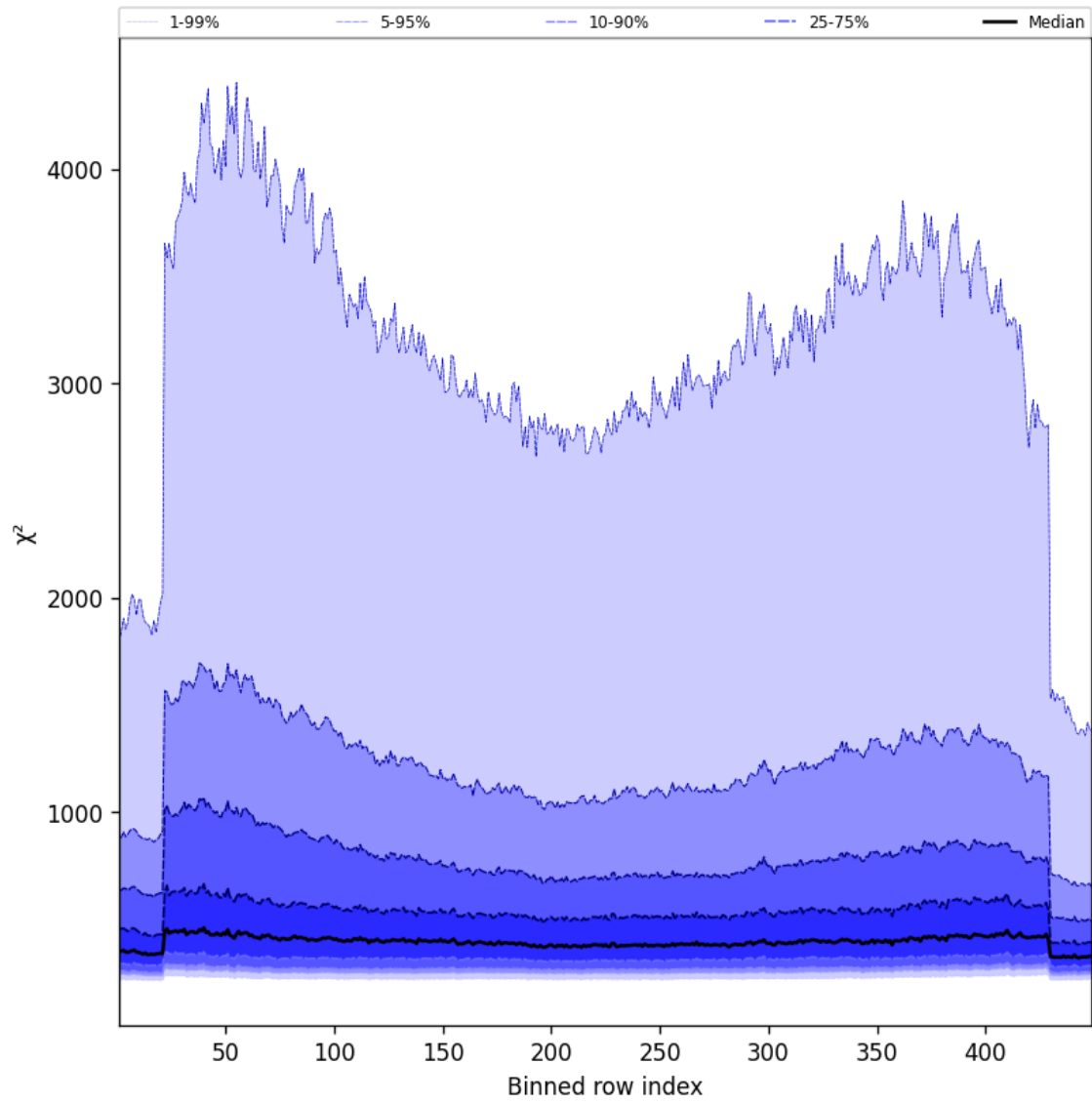
Figure 57: Along track statistics of “ \chi^2 ” for 2025-05-27 to 2025-05-28
