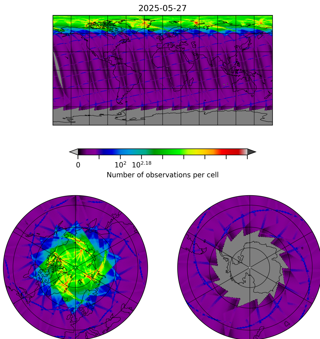
Figure 8: Map of the number of observations for 2025-05-27 to 2025-05-28
