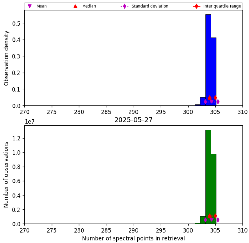
Figure 31: Histogram of “Number of spectral points in retrieval” for 2025-05-27 to 2025-05-28
