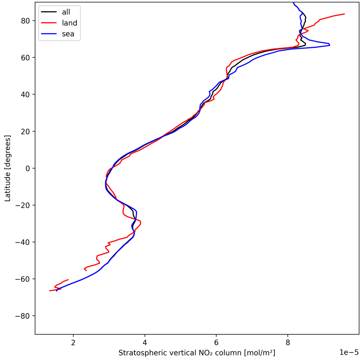
Figure 17: Zonal average of “Stratospheric vertical NO 2 column” for 2025-05-27 to 2025-05-28.
