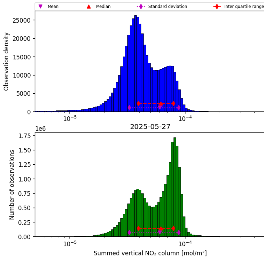
Figure 38: Histogram of “Summed vertical NO 2 column” for 2025-05-27 to 2025-05-28
