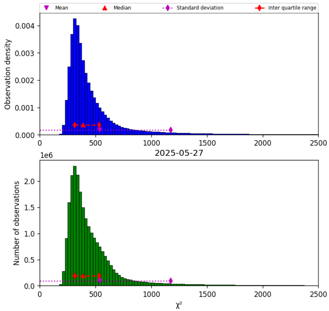
Figure 40: Histogram of “ \chi^2 ” for 2025-05-27 to 2025-05-28
