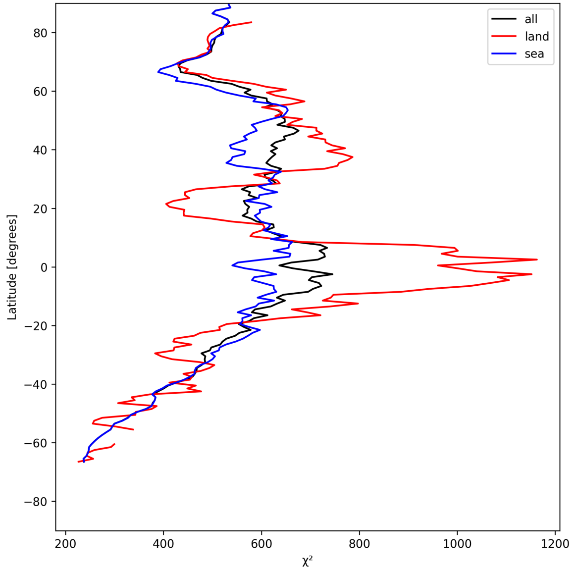
Figure 23: Zonal average of “ \chi^2 ” for 2025-05-27 to 2025-05-28.
