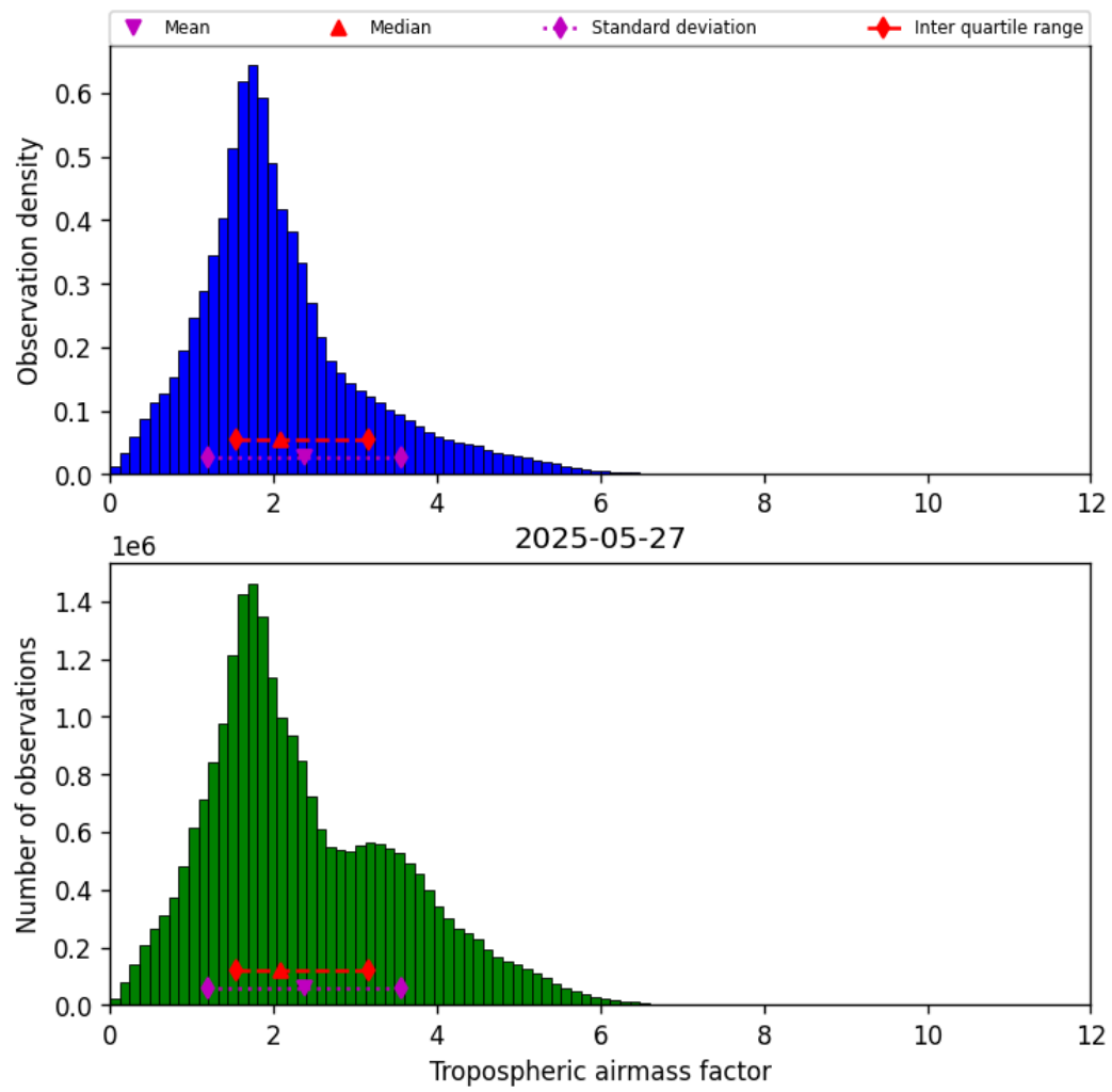
Figure 29: Histogram of “Tropospheric airmass factor” for 2025-05-27 to 2025-05-28
