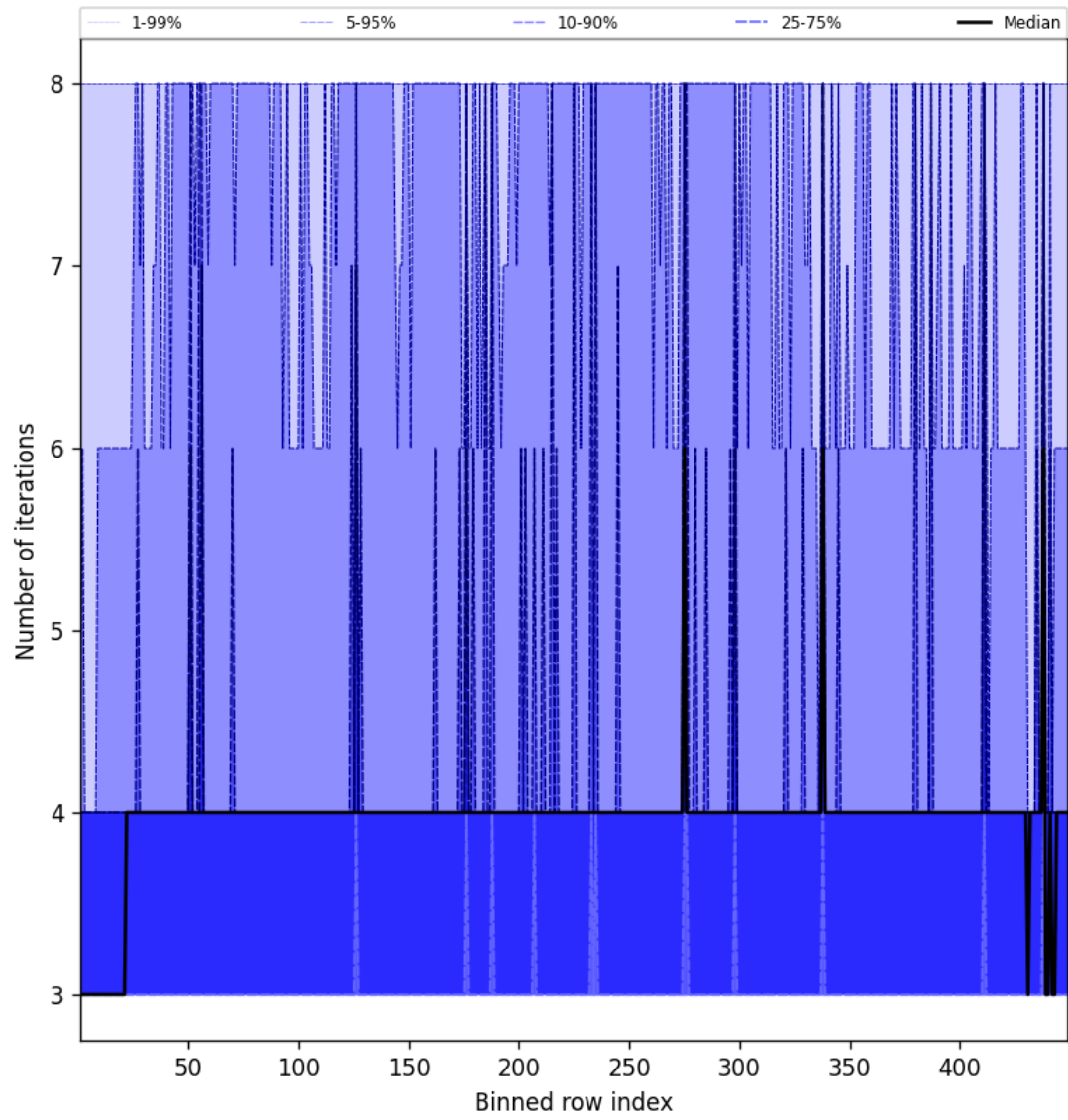
Figure 49: Along track statistics of “Number of iterations” for 2025-05-27 to 2025-05-28
