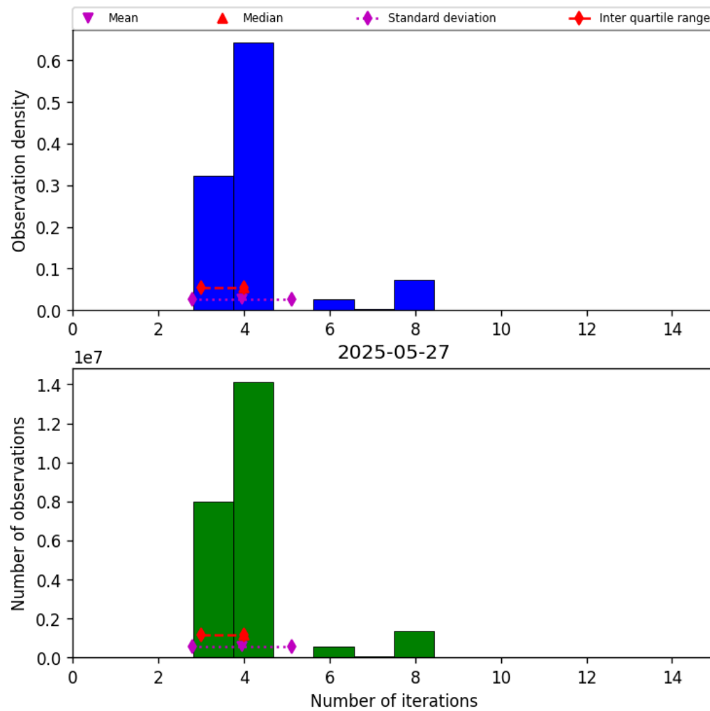
Figure 32: Histogram of “Number of iterations” for 2025-05-27 to 2025-05-28
