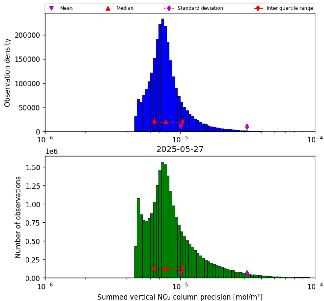
Figure 39: Histogram of “Summed vertical NO 2 column precision” for 2025-05-27 to 2025-05-28
