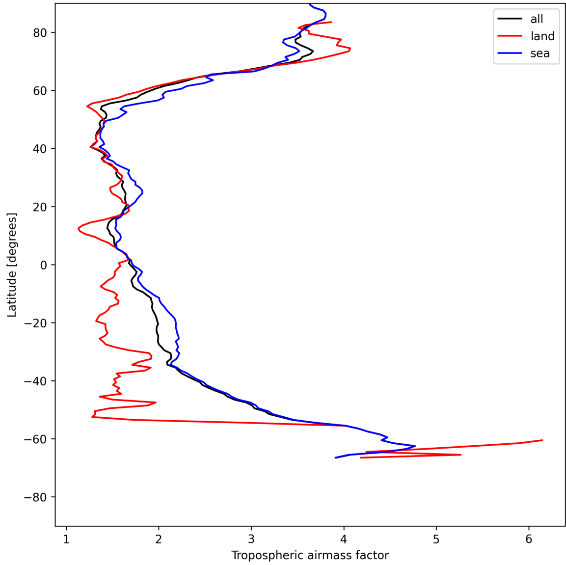
Figure 12: Zonal average of “Tropospheric airmass factor” for 2025-05-27 to 2025-05-28.
