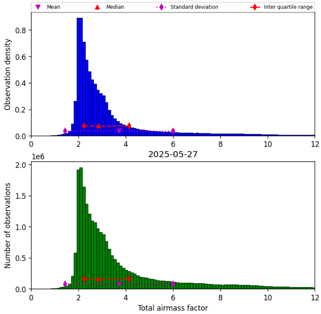
Figure 30: Histogram of “Total airmass factor” for 2025-05-27 to 2025-05-28
