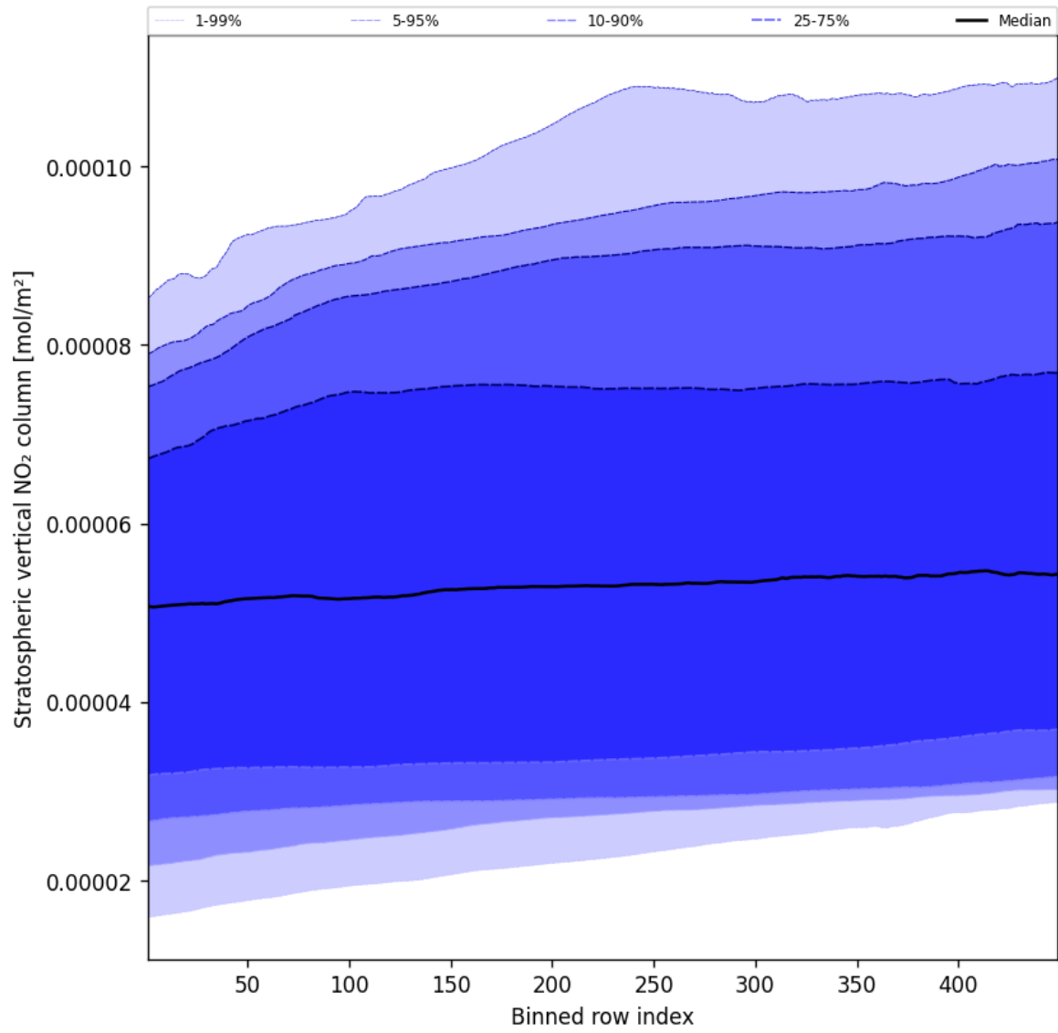
Figure 51: Along track statistics of “Stratospheric vertical NO 2 column” for 2025-05-27 to 2025-05-28
