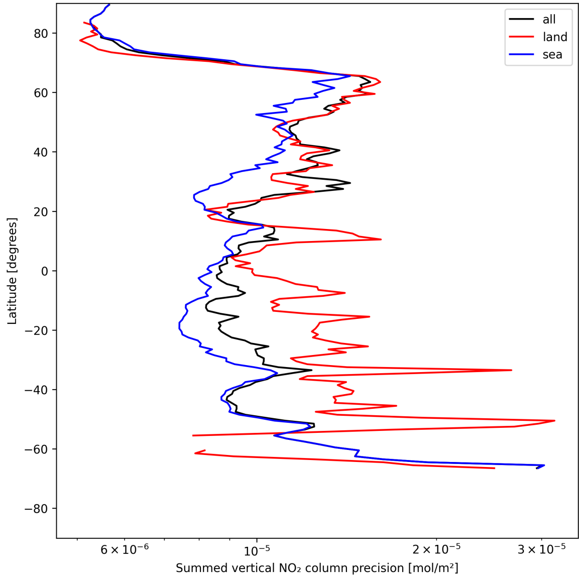
Figure 22: Zonal average of “Summed vertical NO 2 column precision” for 2025-05-27 to 2025-05-28.
