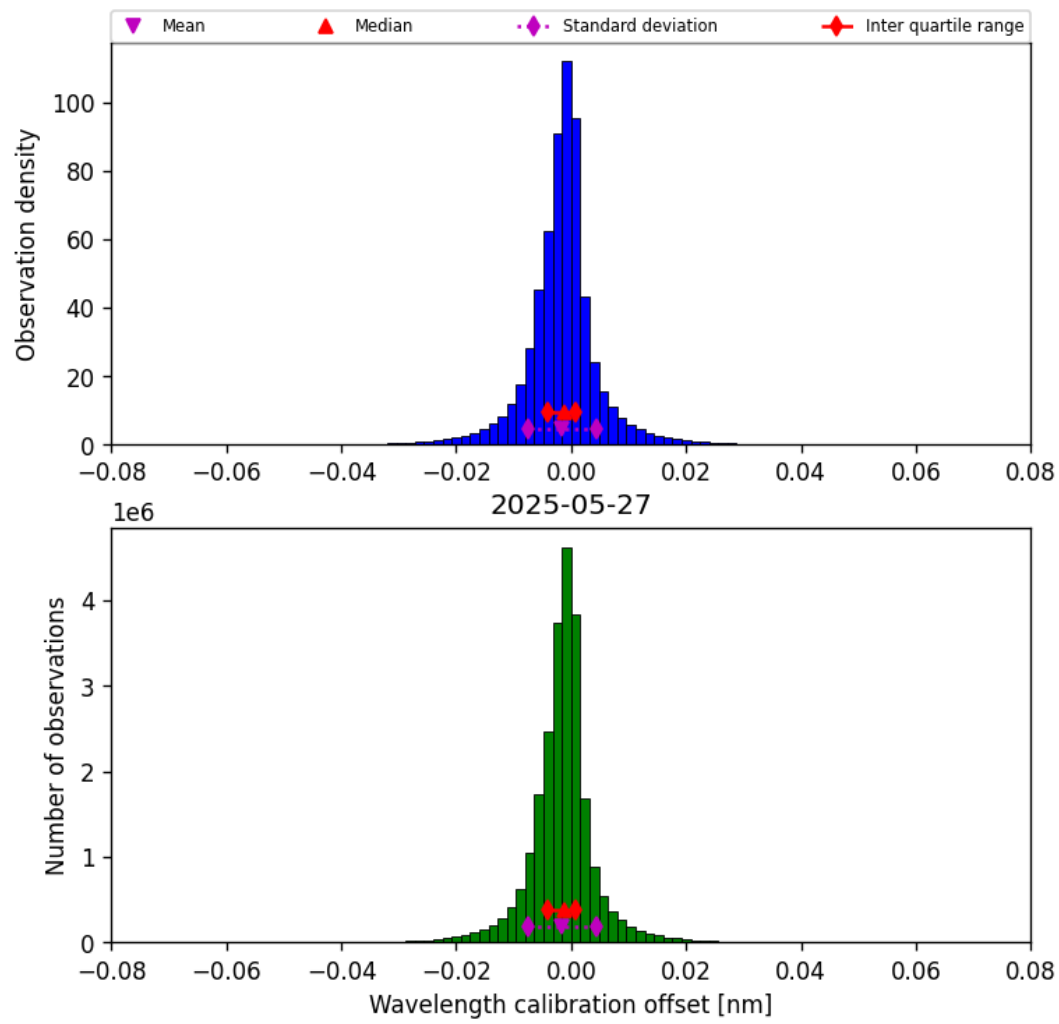
Figure 33: Histogram of “Wavelength calibration offset” for 2025-05-27 to 2025-05-28
