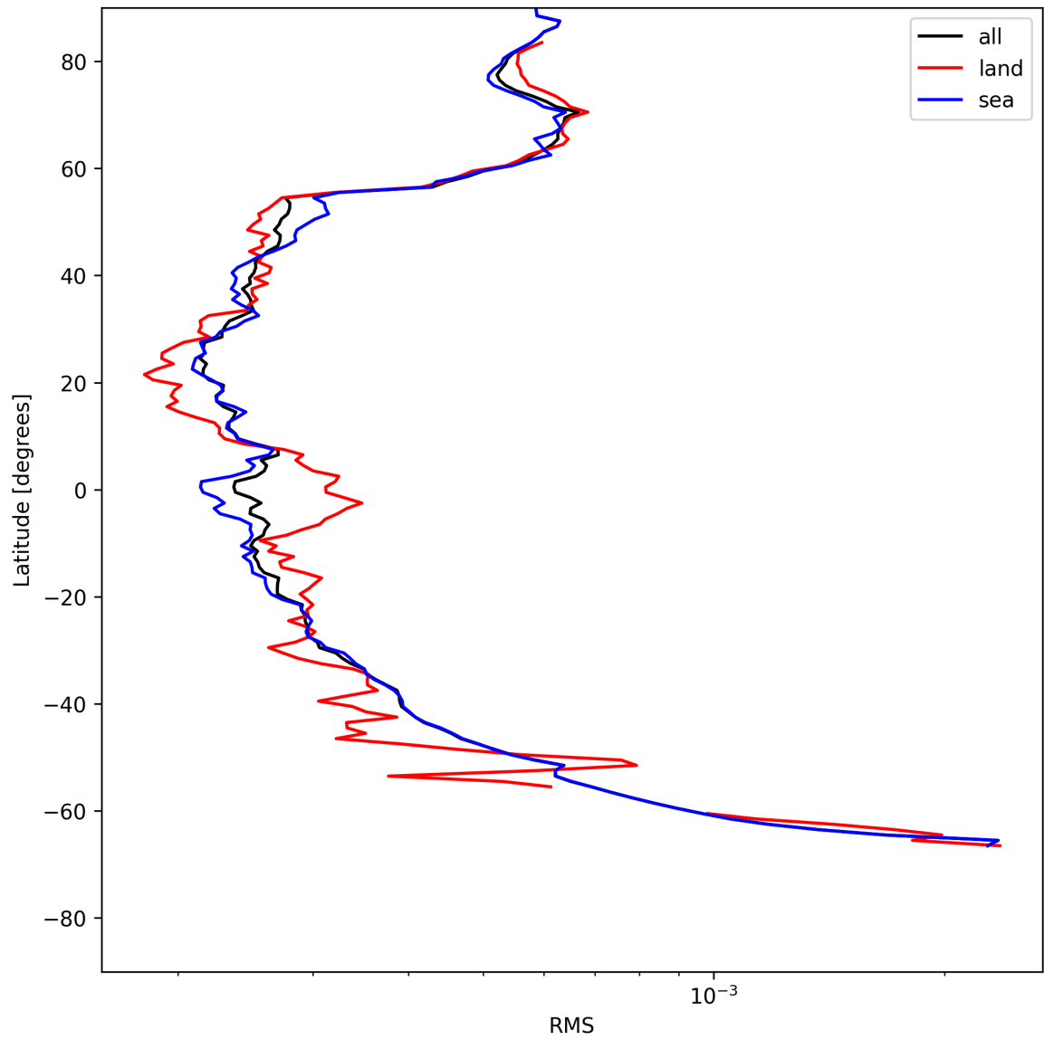
Figure 24: Zonal average of “RMS” for 2025-05-27 to 2025-05-28.
