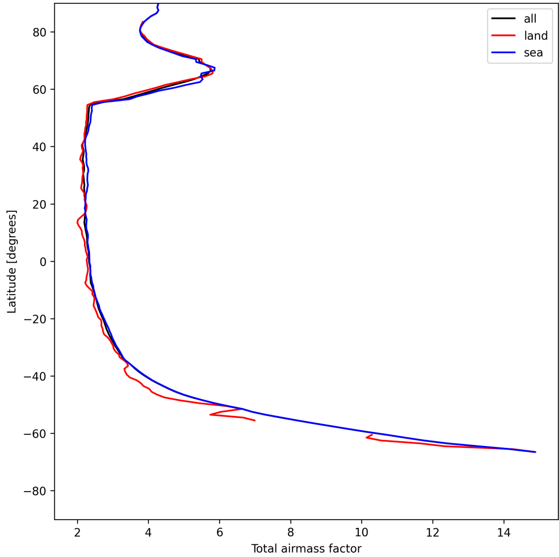
Figure 13: Zonal average of “Total airmass factor” for 2025-05-27 to 2025-05-28.
