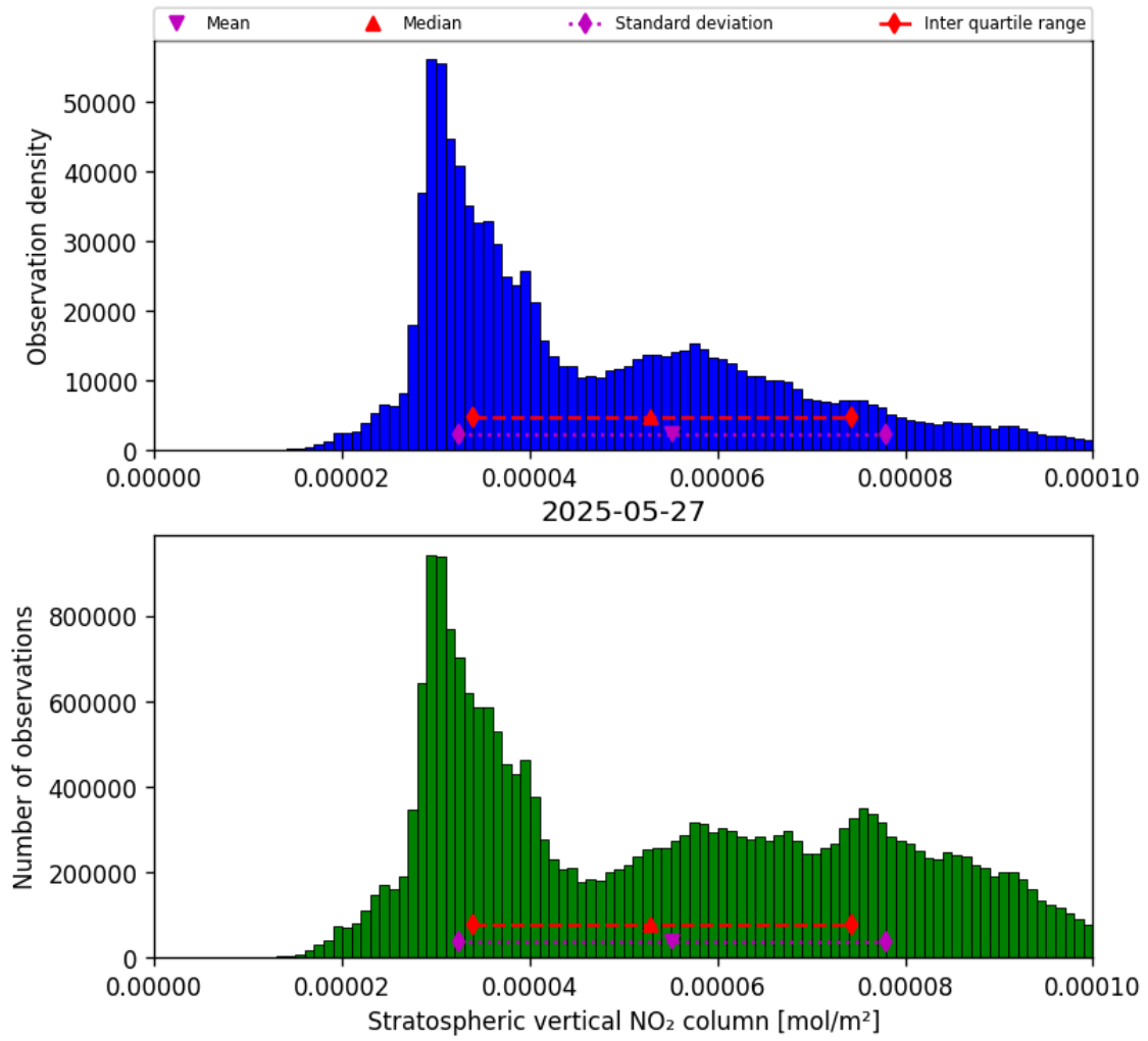
Figure 34: Histogram of “Stratospheric vertical NO 2 column” for 2025-05-27 to 2025-05-28
