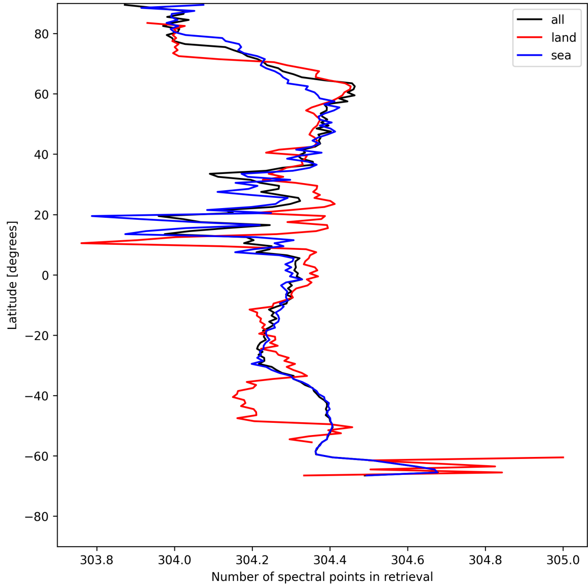
Figure 14: Zonal average of “Number of spectral points in retrieval” for 2025-05-27 to 2025-05-28.
