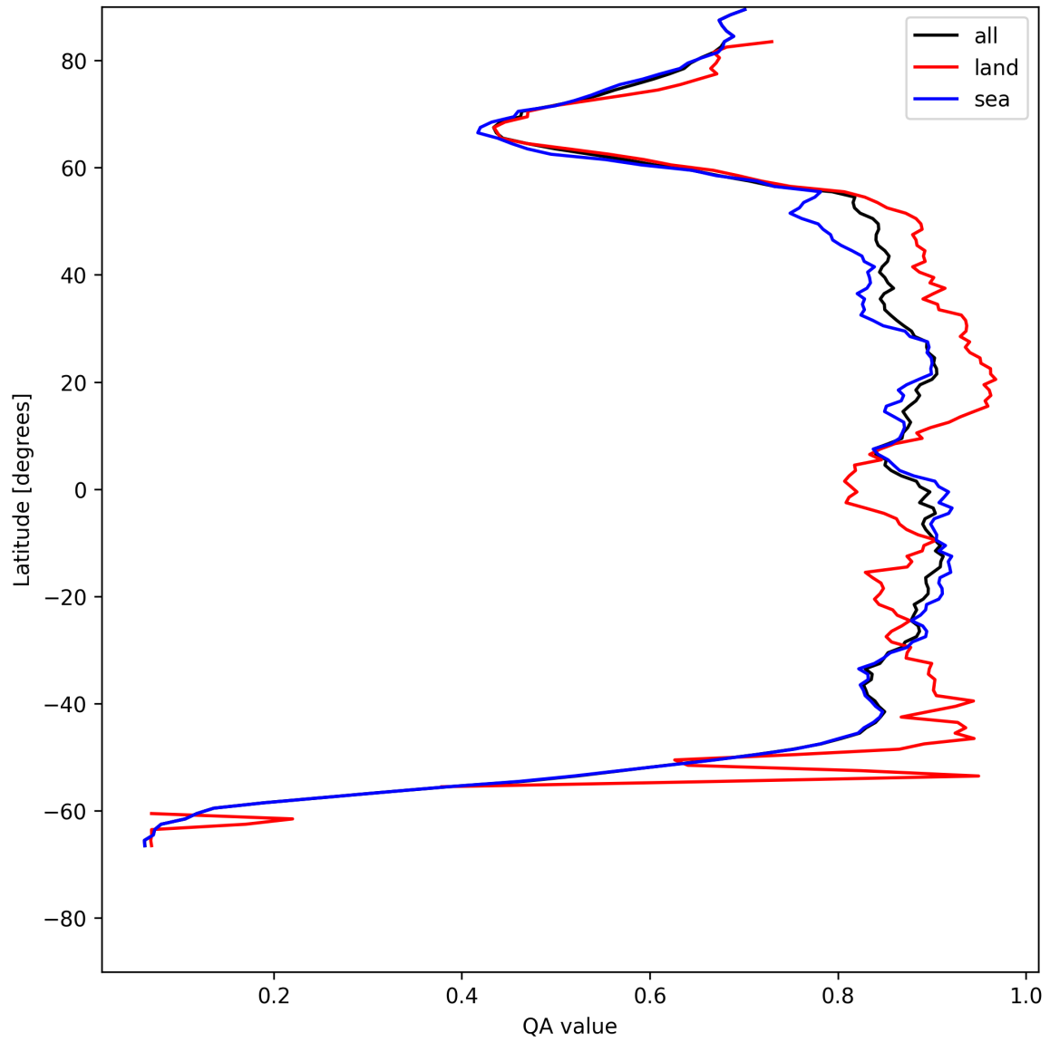
Figure 9: Zonal average of “QA value” for 2025-05-27 to 2025-05-28.
