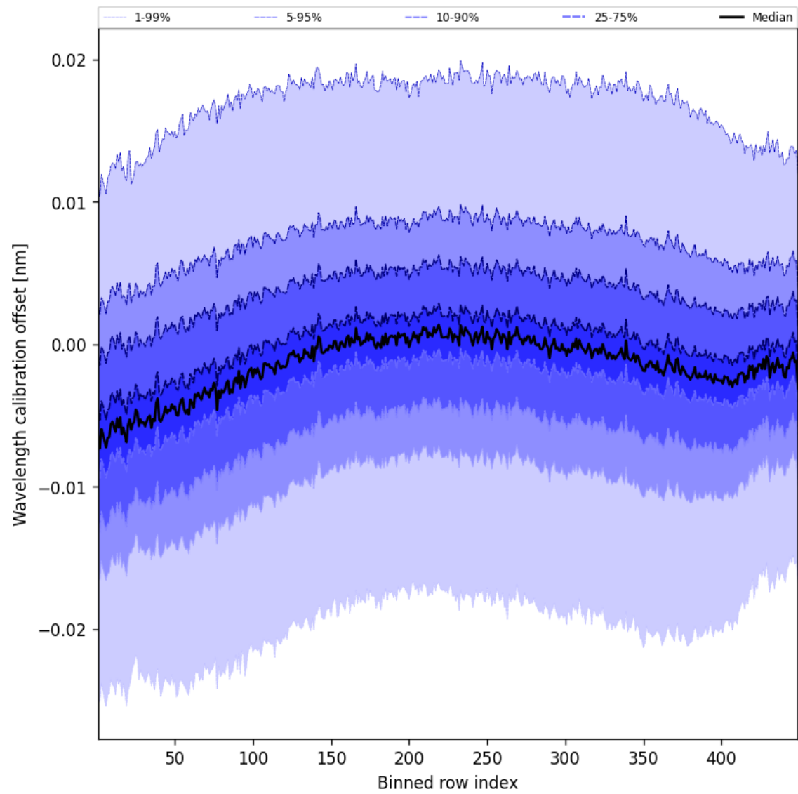
Figure 50: Along track statistics of “Wavelength calibration offset” for 2025-05-27 to 2025-05-28
