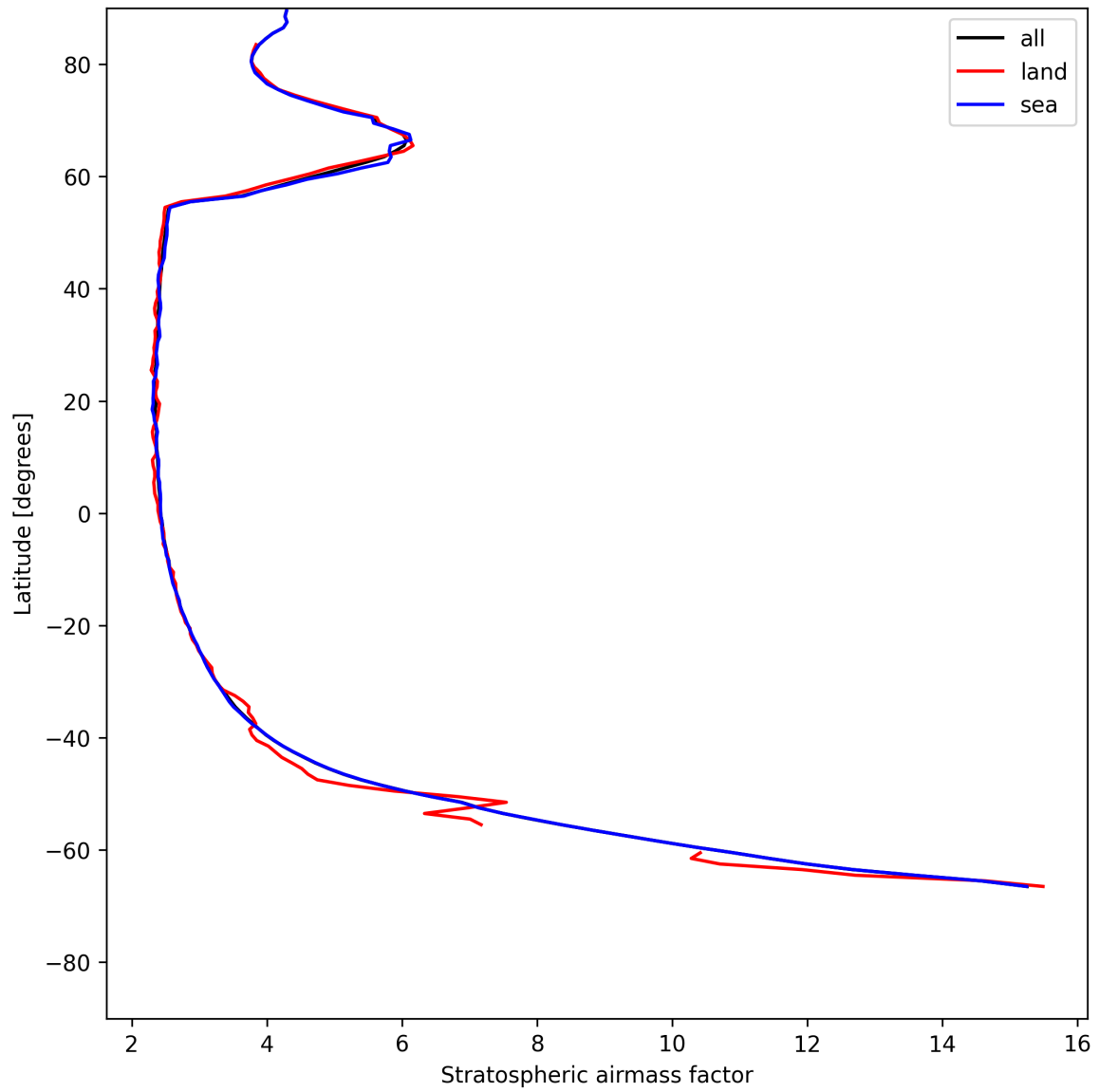
Figure 25: Zonal average of “Stratospheric airmass factor” for 2025-05-27 to 2025-05-28.
