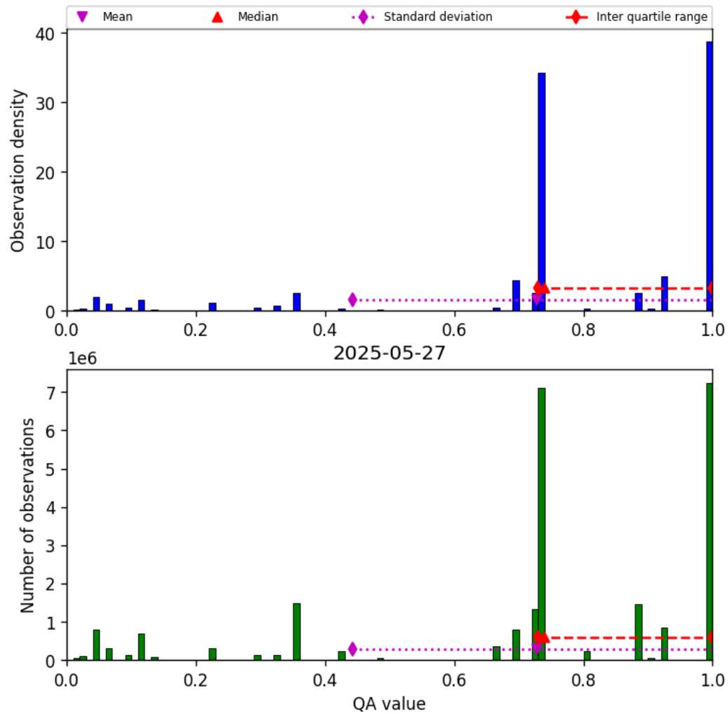
Figure 26: Histogram of “QA value” for 2025-05-27 to 2025-05-28
