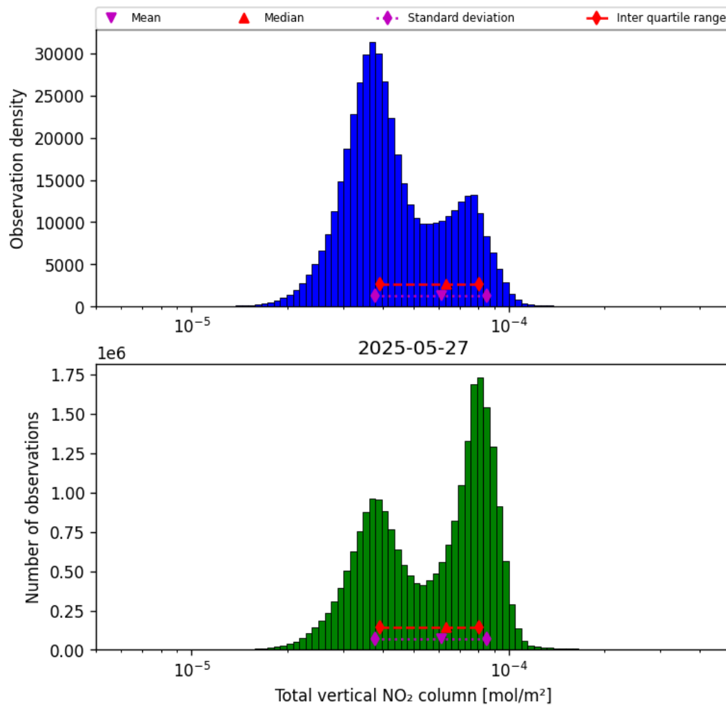
Figure 36: Histogram of “Total vertical NO 2 column” for 2025-05-27 to 2025-05-28
