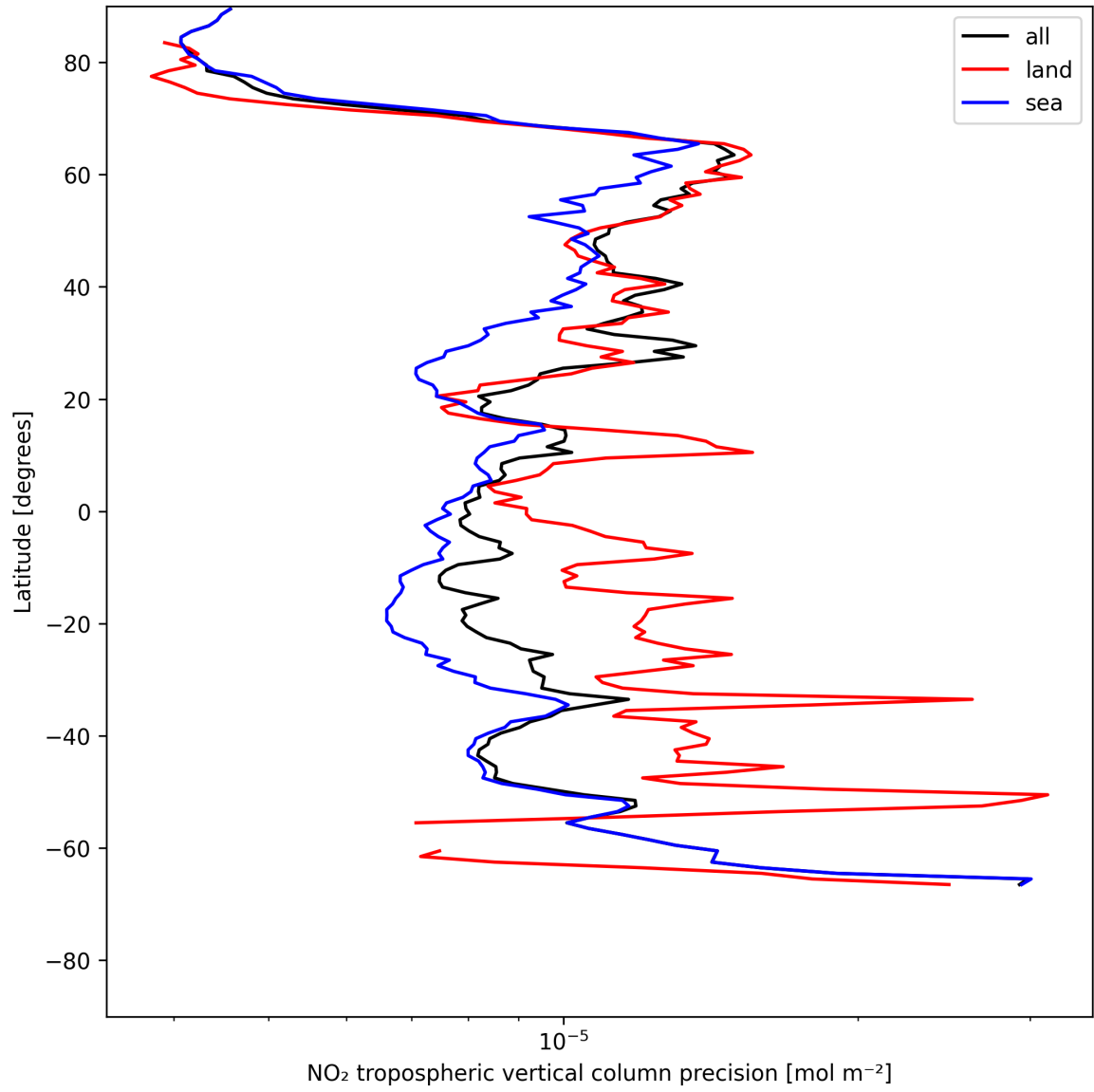
Figure 11: Zonal average of “NO 2 tropospheric vertical column precision” for 2025-05-27 to 2025-05-28.
