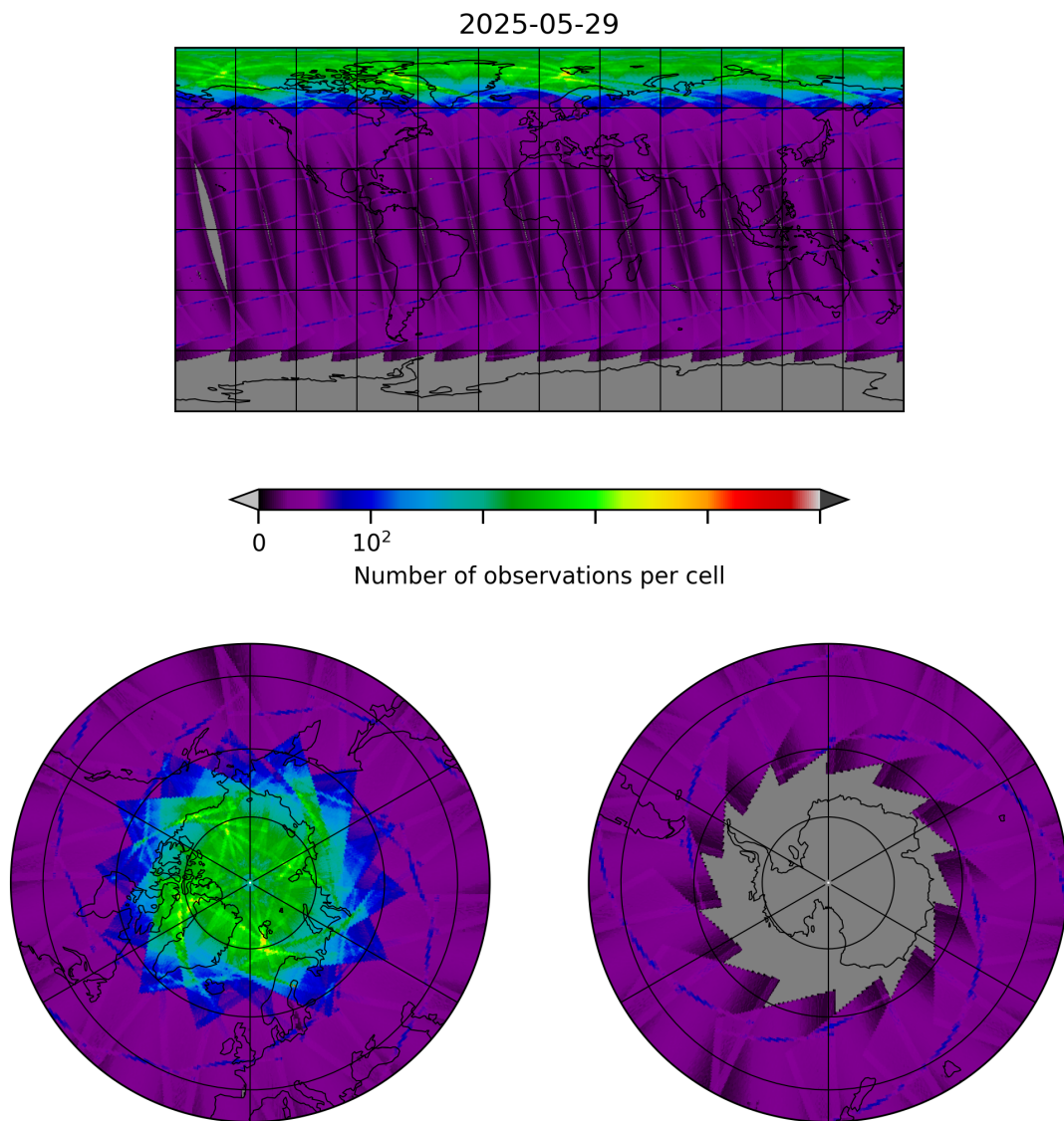
Figure 8: Map of the number of observations for 2025-05-29 to 2025-05-29
