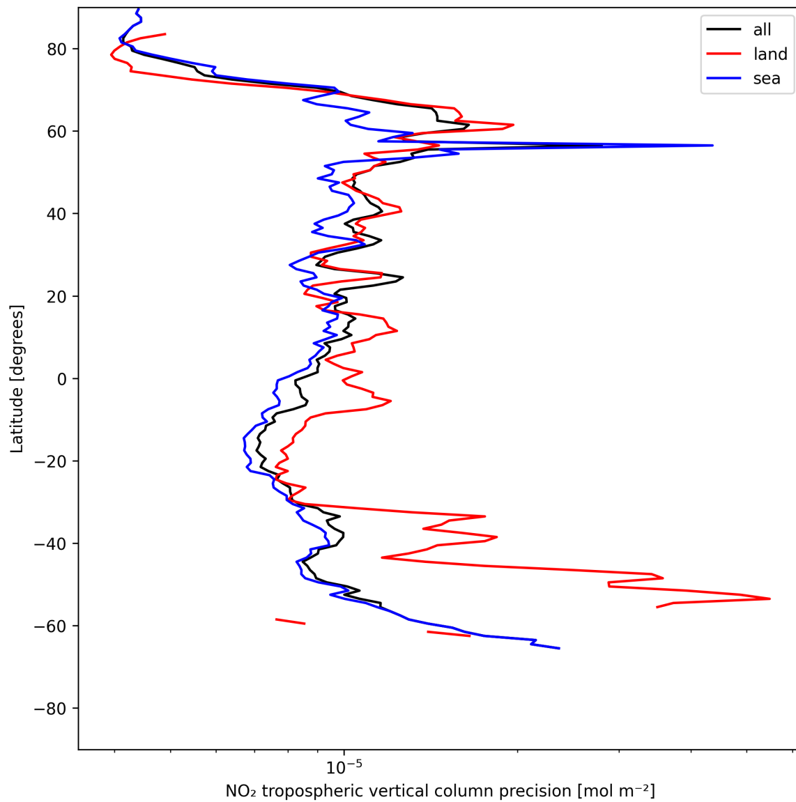
Figure 11: Zonal average of “NO 2 tropospheric vertical column precision” for 2025-05-29 to 2025-05-29.
