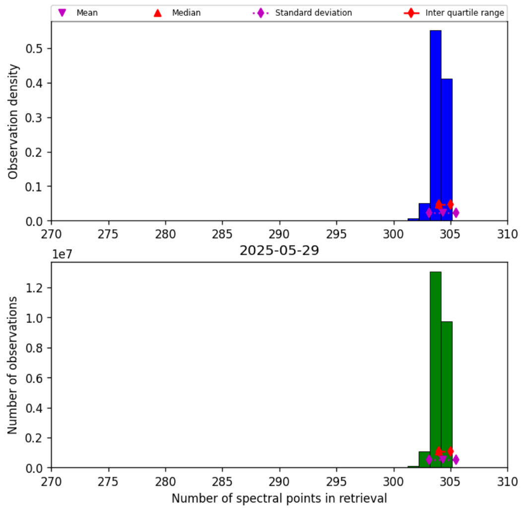
Figure 31: Histogram of “Number of spectral points in retrieval” for 2025-05-29 to 2025-05-29
