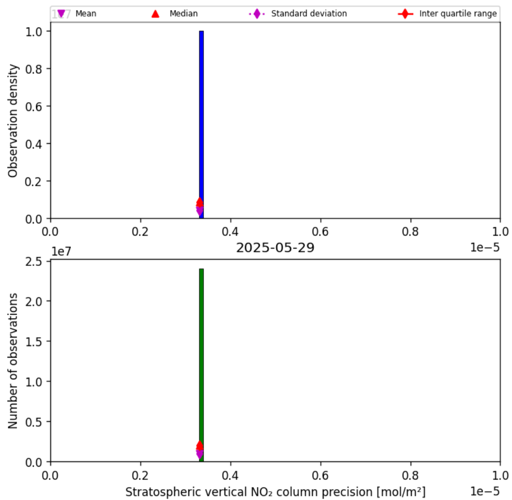
Figure 35: Histogram of “Stratospheric vertical NO 2 column precision” for 2025-05-29 to 2025-05-29
