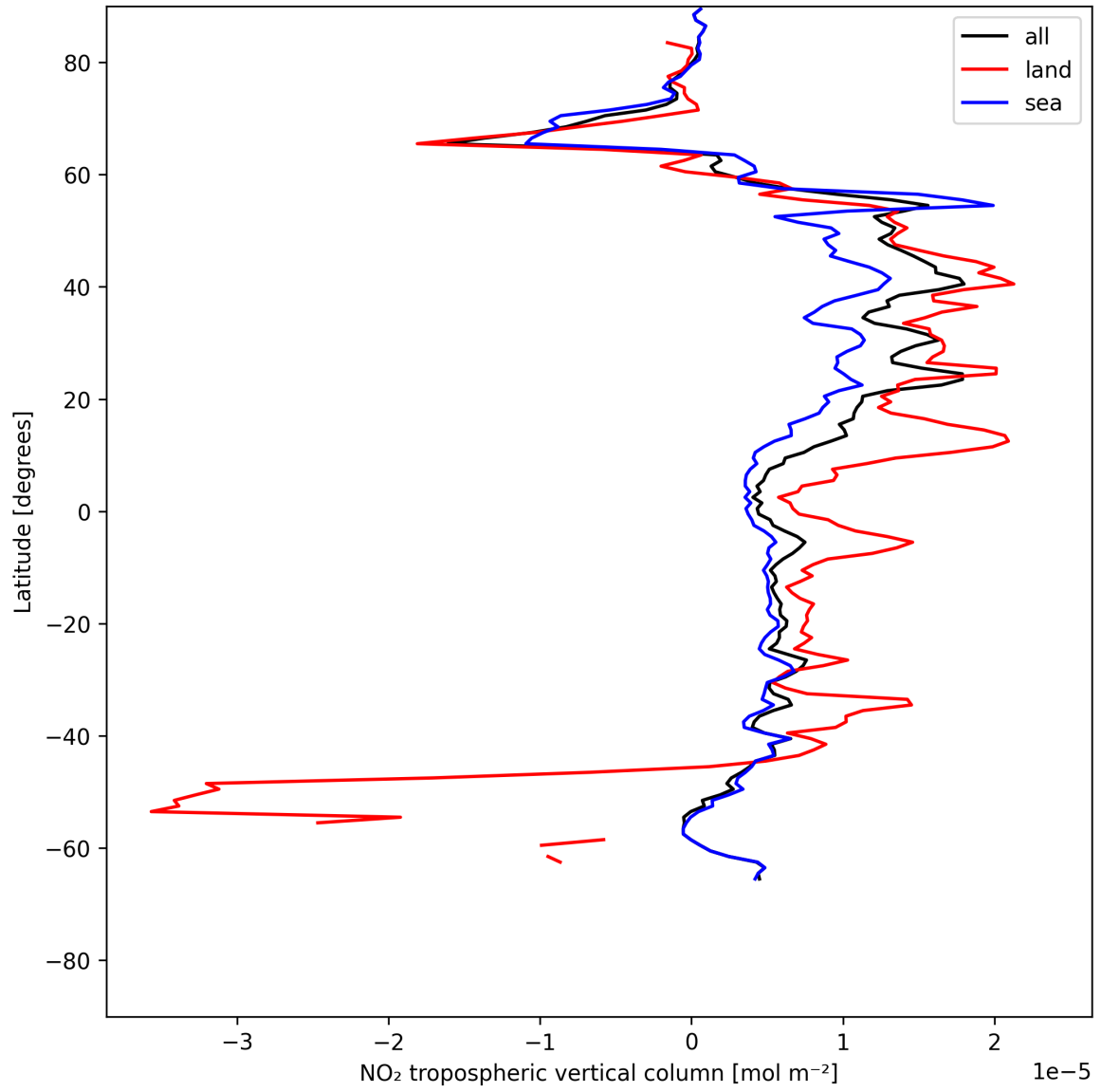
Figure 10: Zonal average of “NO 2 tropospheric vertical column” for 2025-05-29 to 2025-05-29.
