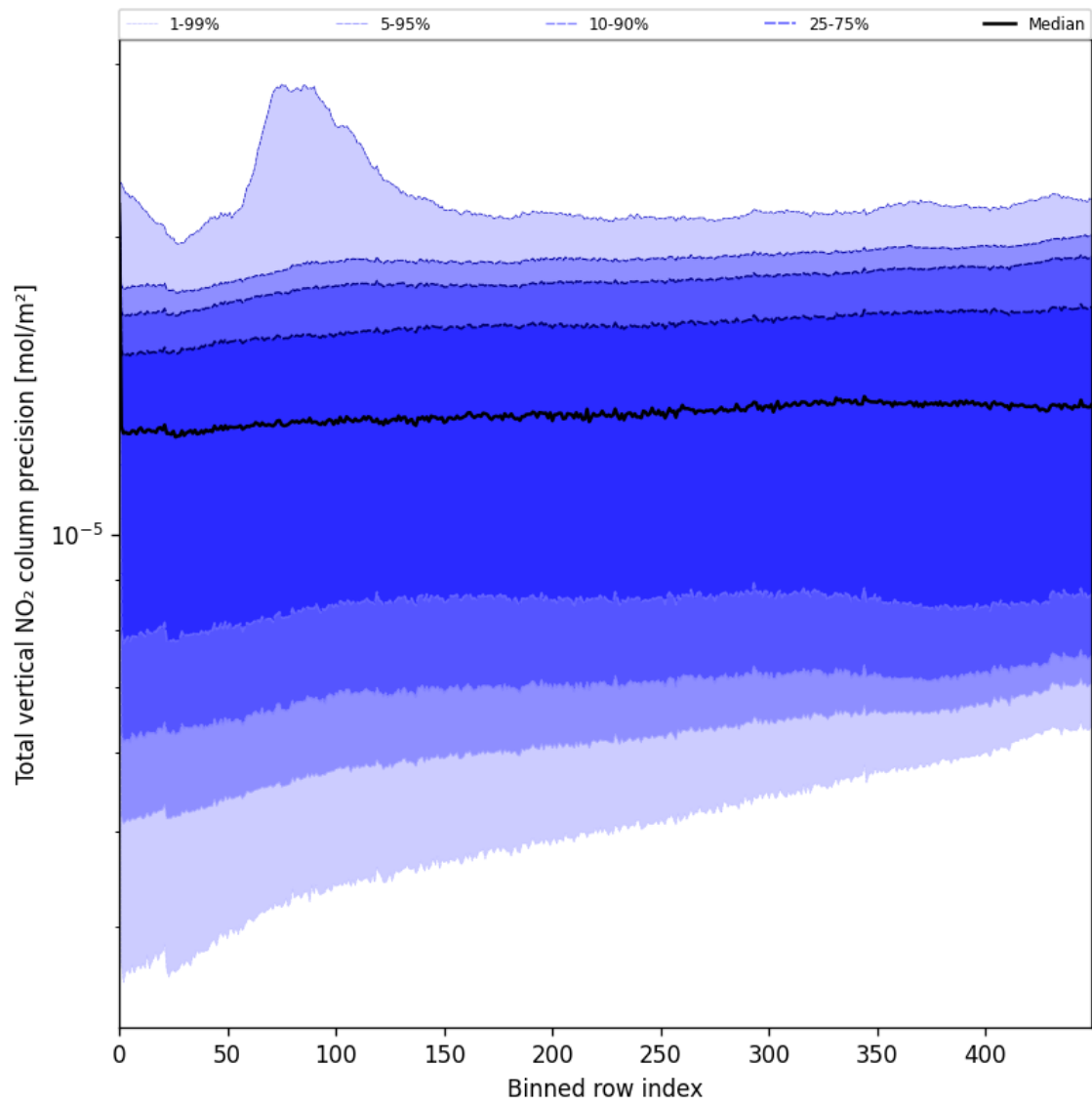
Figure 54: Along track statistics of “Total vertical NO 2 column precision” for 2025-05-29 to 2025-05-29
