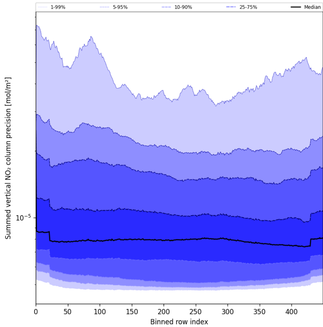
Figure 56: Along track statistics of “Summed vertical NO 2 column precision” for 2025-05-29 to 2025-05-29
