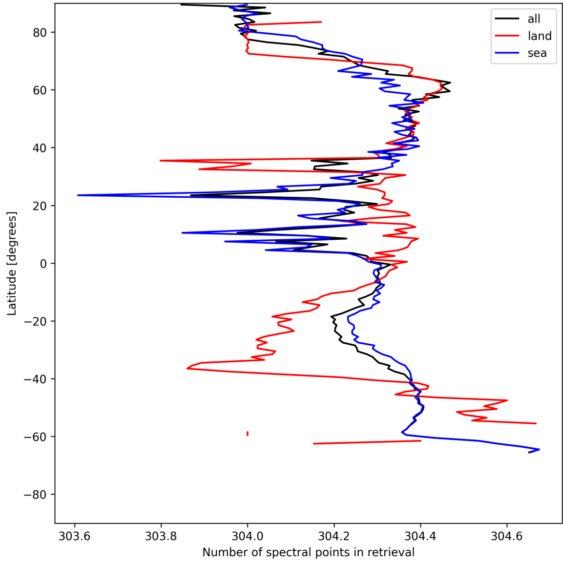
Figure 14: Zonal average of “Number of spectral points in retrieval” for 2025-05-29 to 2025-05-29.
