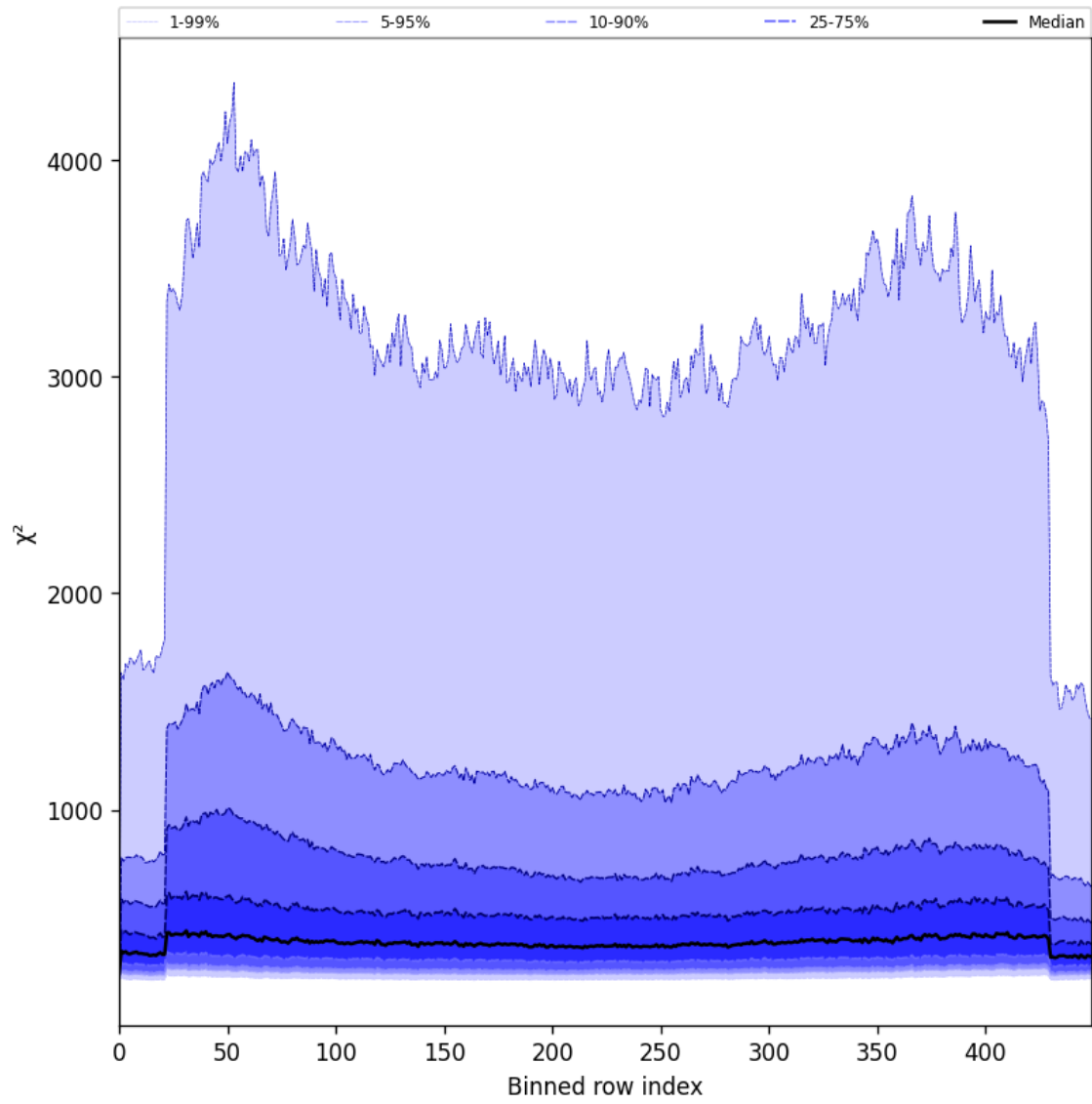
Figure 57: Along track statistics of “ \chi^2 ” for 2025-05-29 to 2025-05-29
