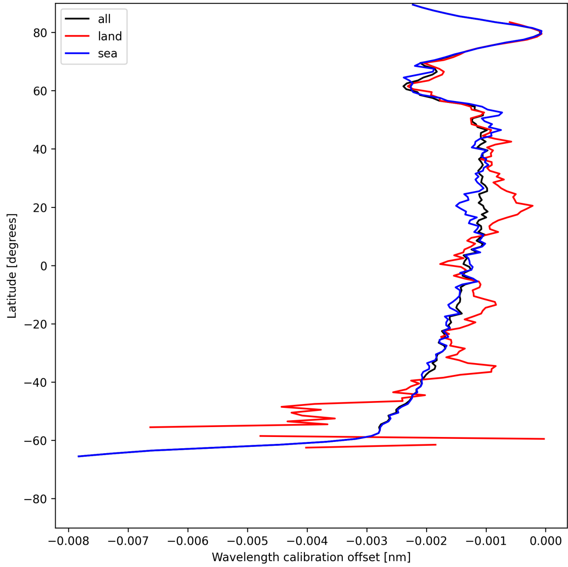
Figure 16: Zonal average of “Wavelength calibration offset” for 2025-05-29 to 2025-05-29.
