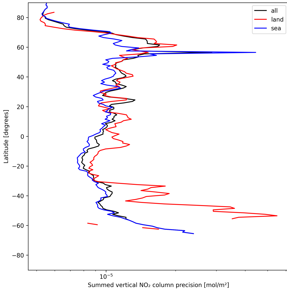
Figure 22: Zonal average of “Summed vertical NO 2 column precision” for 2025-05-29 to 2025-05-29.
