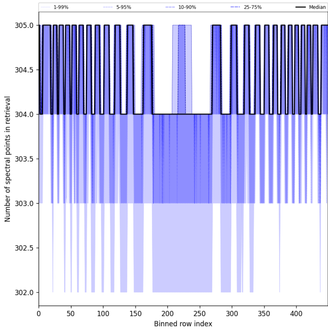
Figure 48: Along track statistics of “Number of spectral points in retrieval” for 2025-05-29 to 2025-05-29
