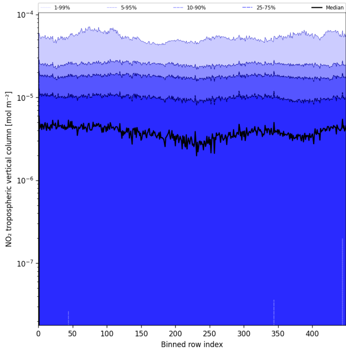
Figure 44: Along track statistics of “NO 2 tropospheric vertical column” for 2025-05-29 to 2025-05-29
