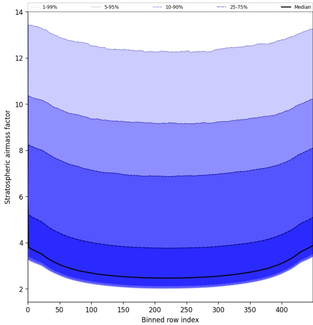
Figure 59: Along track statistics of “Stratospheric airmass factor” for 2025-05-29 to 2025-05-29
