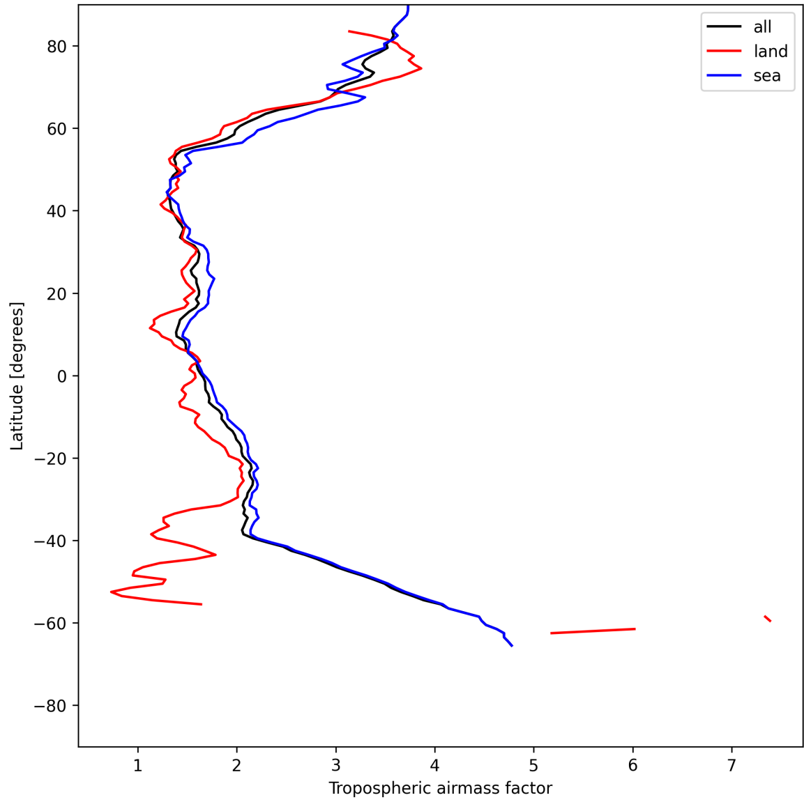
Figure 12: Zonal average of “Tropospheric airmass factor” for 2025-05-29 to 2025-05-29.
