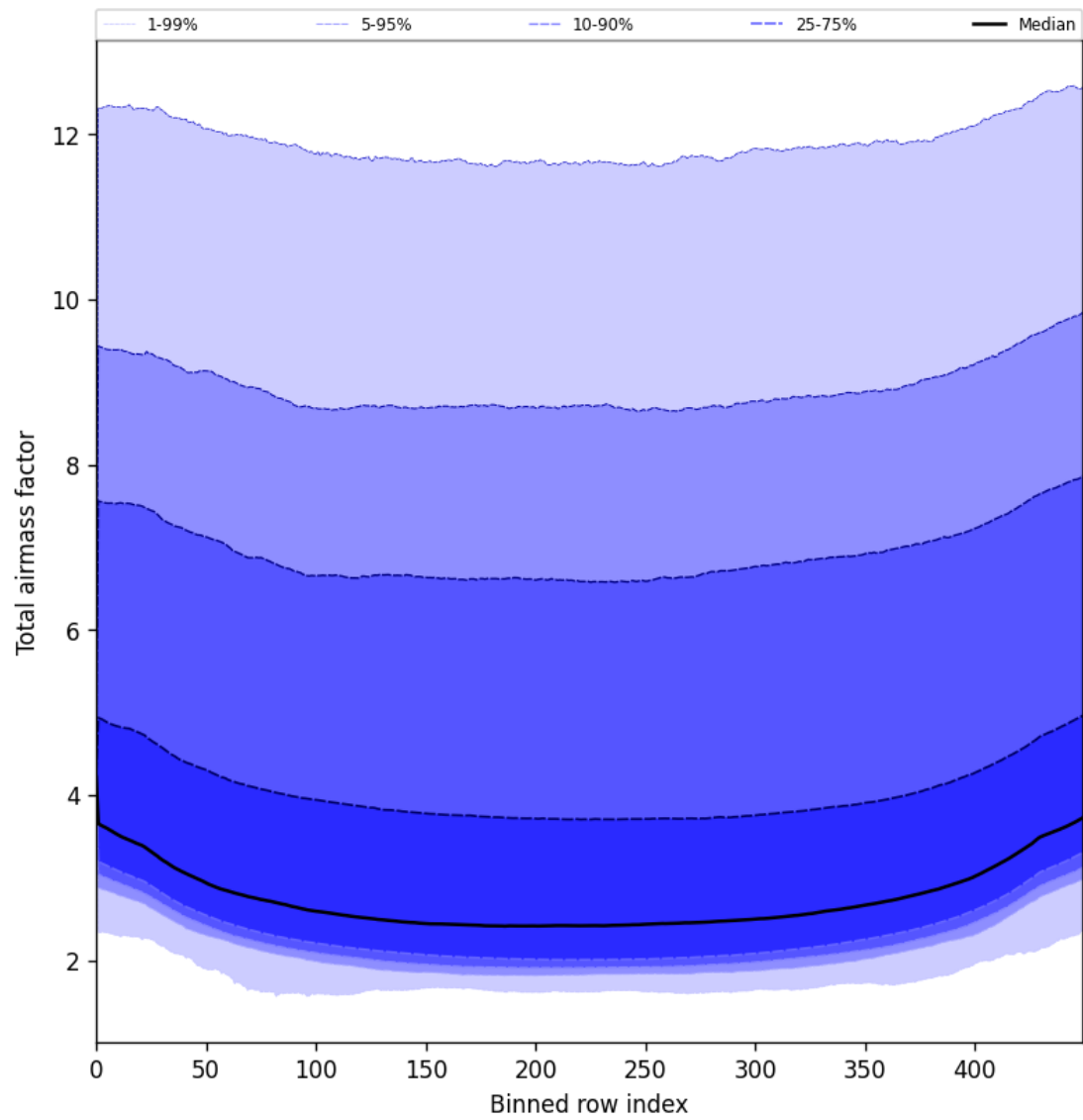
Figure 47: Along track statistics of “Total airmass factor” for 2025-05-29 to 2025-05-29
