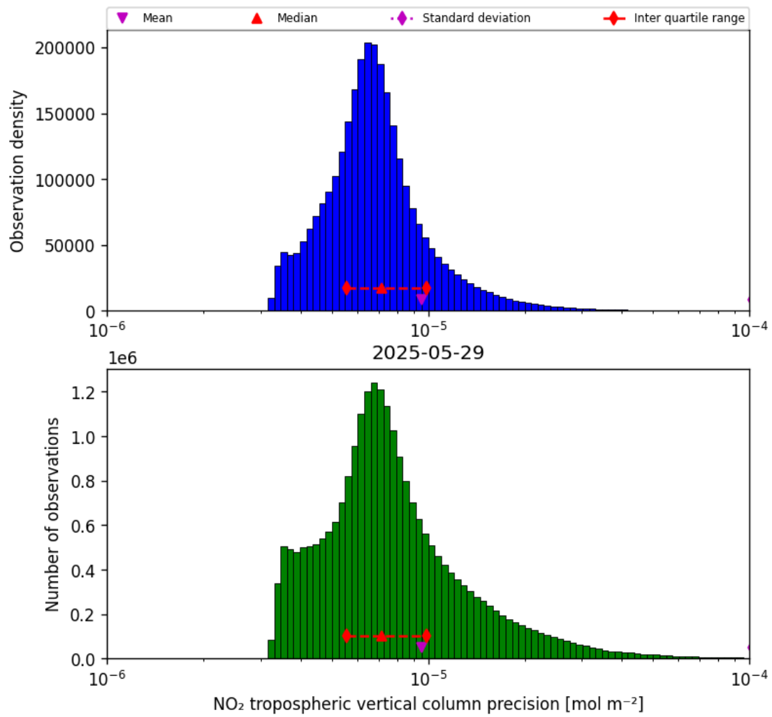
Figure 28: Histogram of “NO 2 tropospheric vertical column precision” for 2025-05-29 to 2025-05-29
