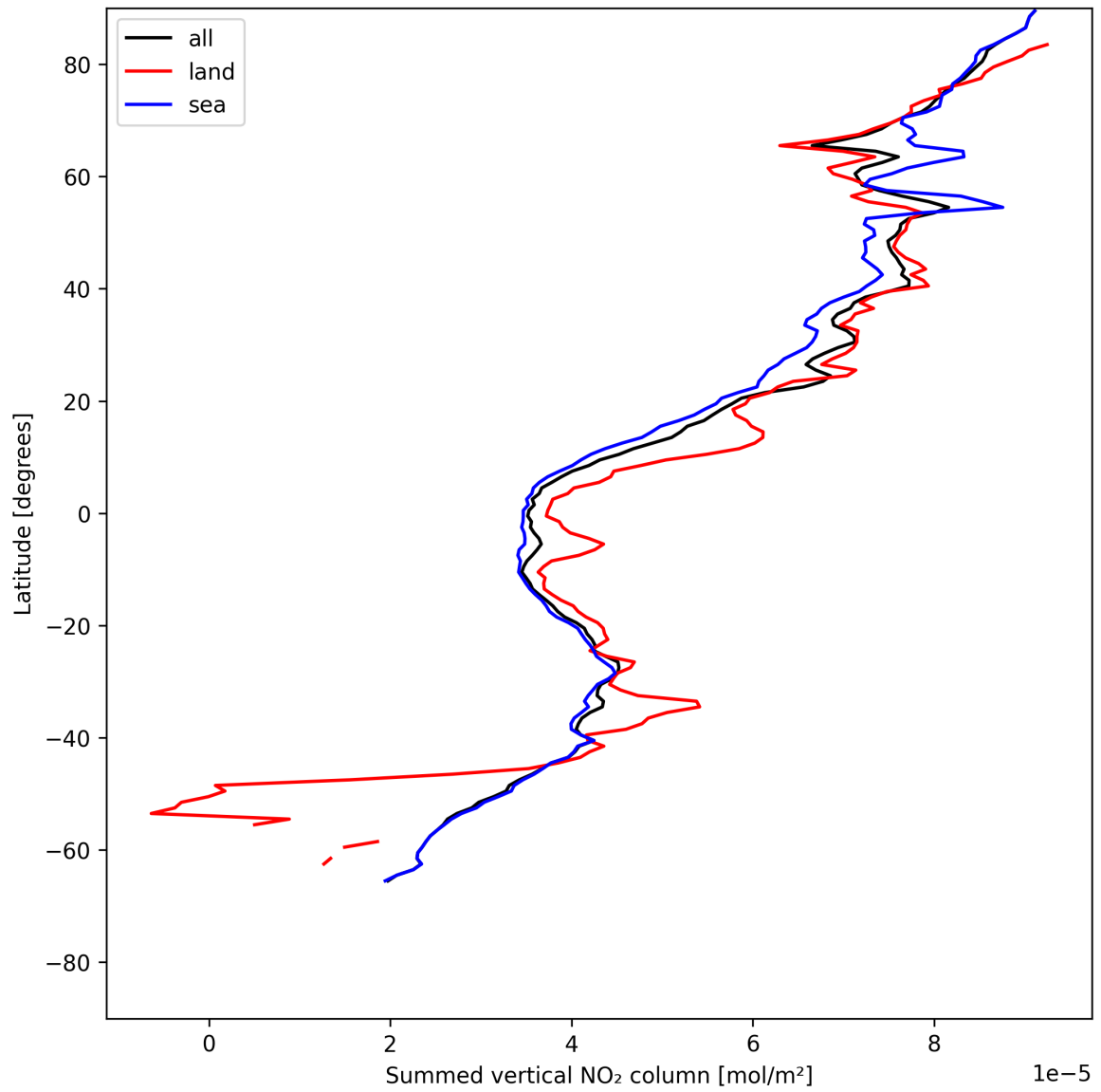
Figure 21: Zonal average of “Summed vertical NO 2 column” for 2025-05-29 to 2025-05-29.
