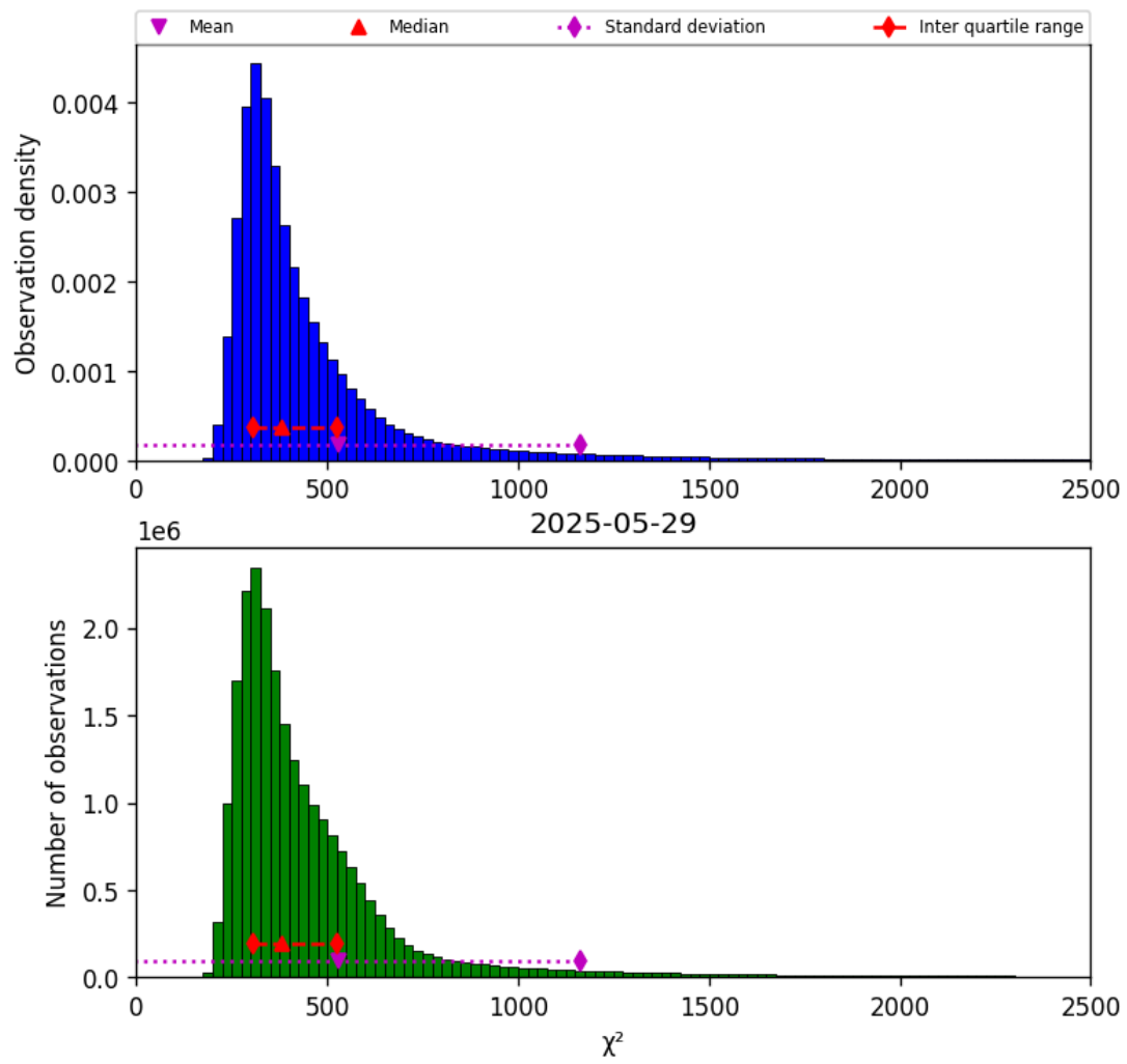
Figure 40: Histogram of “ \chi^2 ” for 2025-05-29 to 2025-05-29
