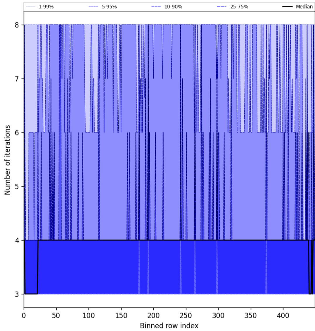
Figure 49: Along track statistics of “Number of iterations” for 2025-05-29 to 2025-05-29
