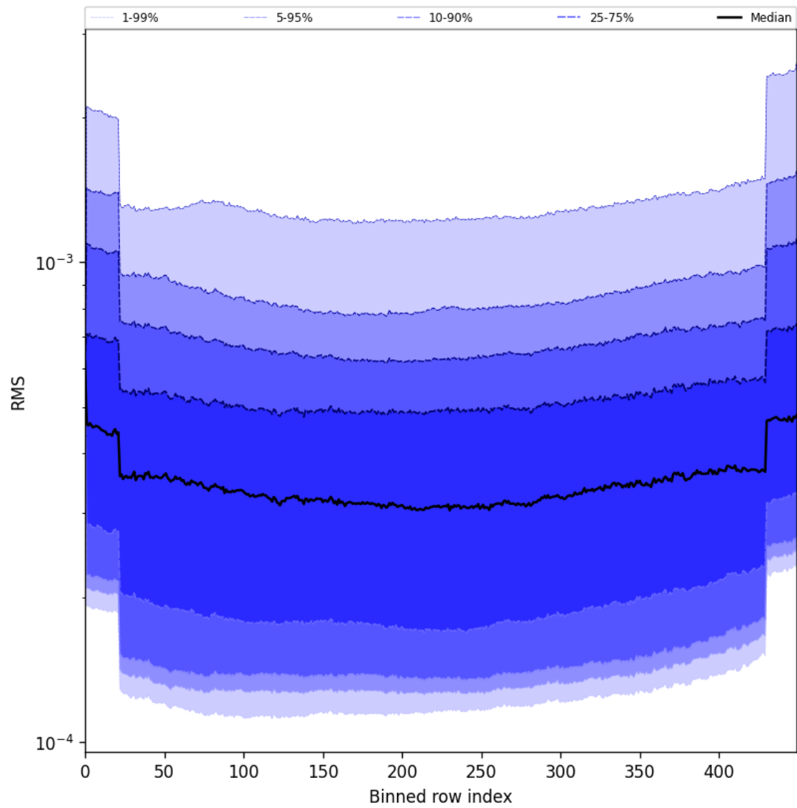
Figure 58: Along track statistics of “RMS” for 2025-05-29 to 2025-05-29
