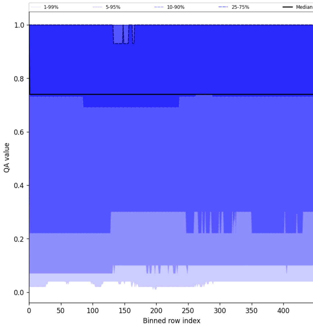
Figure 43: Along track statistics of “QA value” for 2025-05-29 to 2025-05-29
