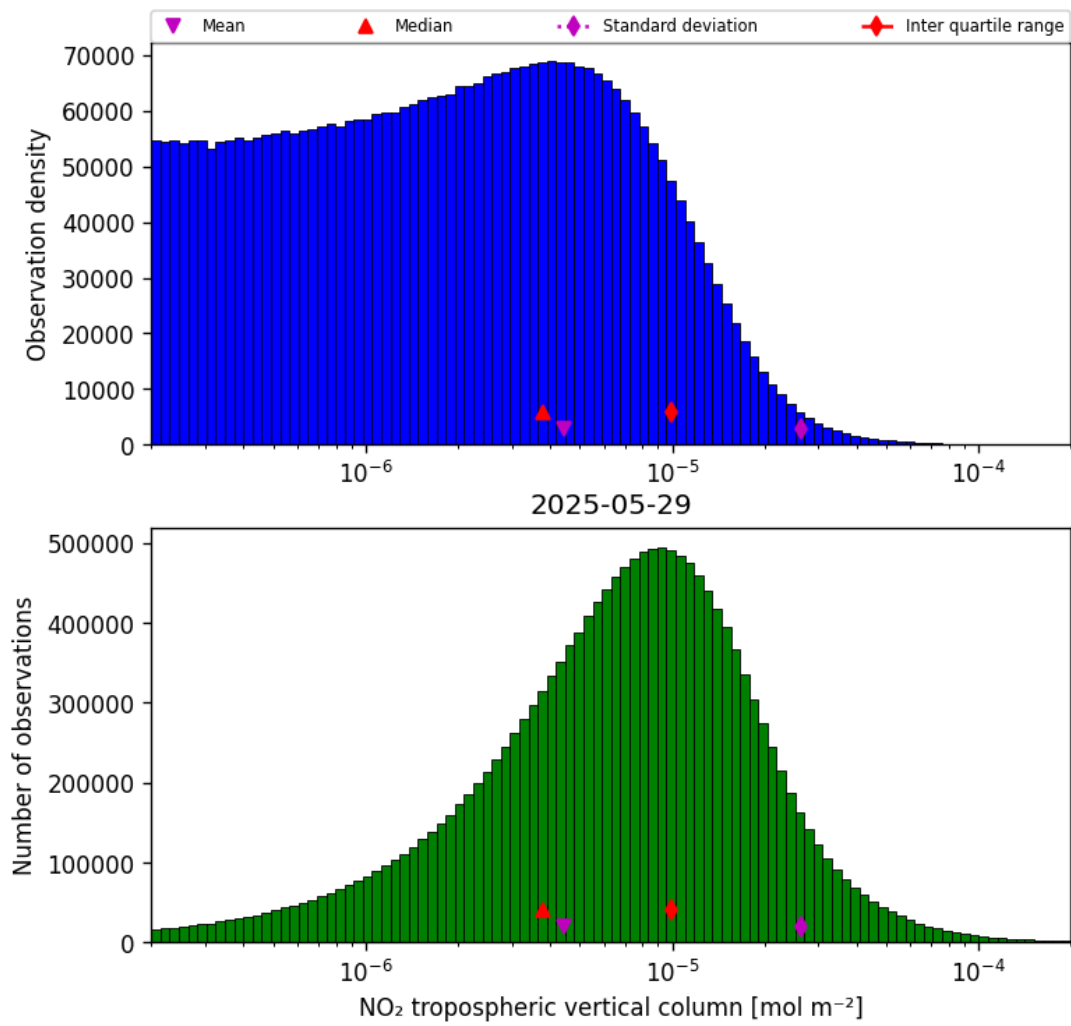
Figure 27: Histogram of “ \text{NO}_2 tropospheric vertical column” for 2025-05-29 to 2025-05-29
