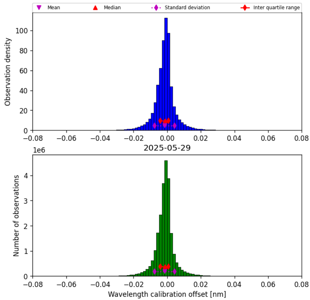
Figure 33: Histogram of “Wavelength calibration offset” for 2025-05-29 to 2025-05-29
