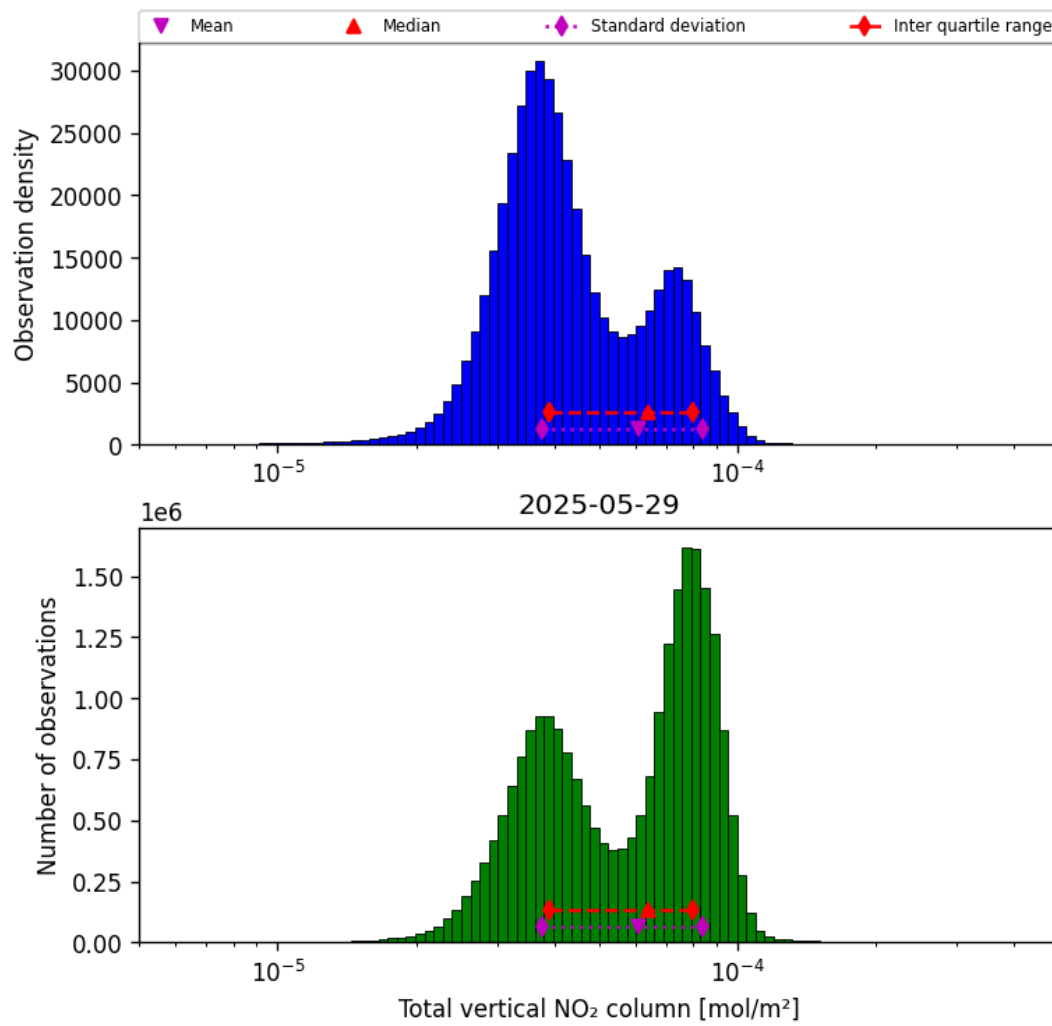
Figure 36: Histogram of "Total vertical NO 2 column" for 2025-05-29 to 2025-05-29
