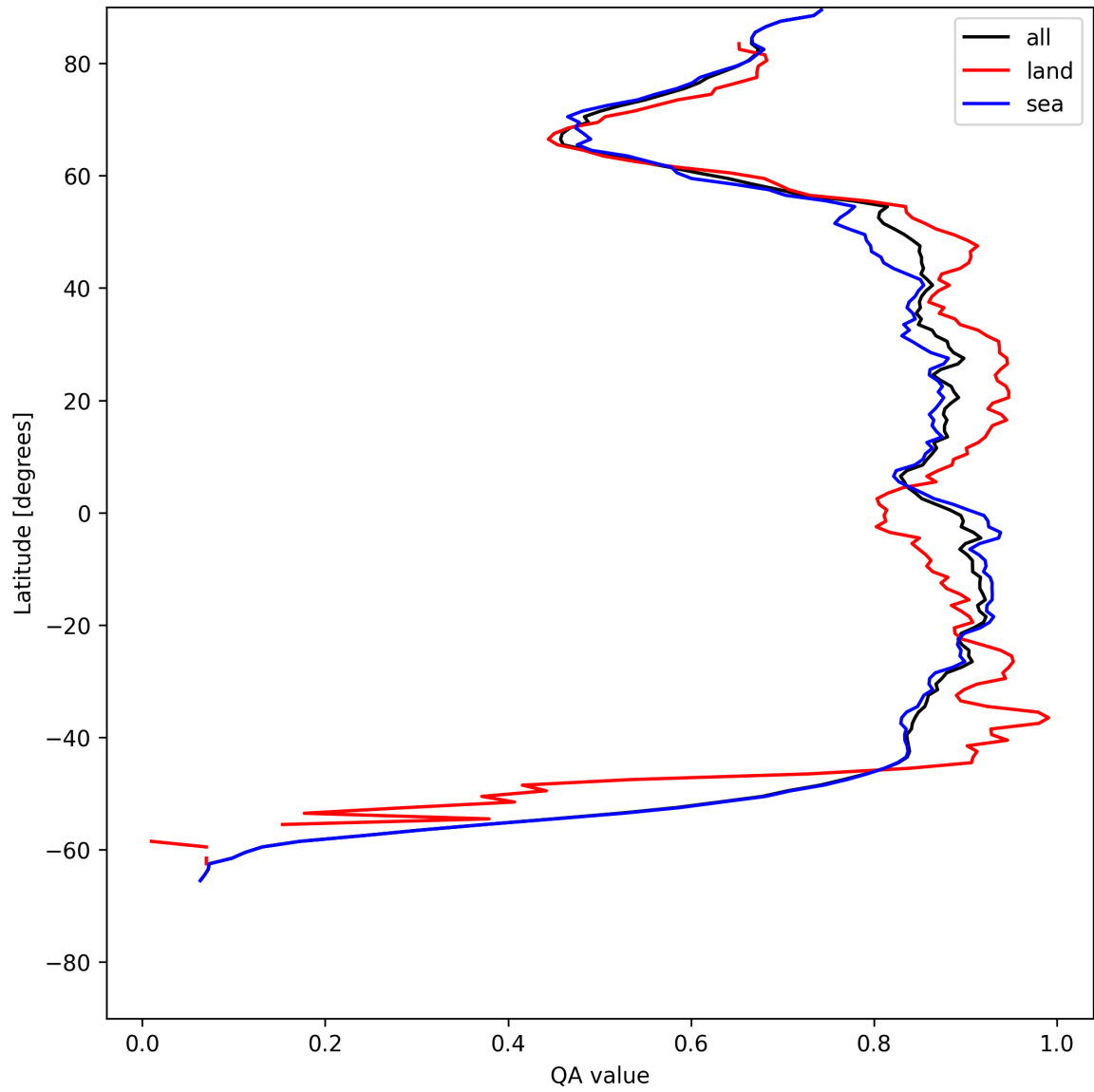
Figure 9: Zonal average of “QA value” for 2025-05-29 to 2025-05-29.
