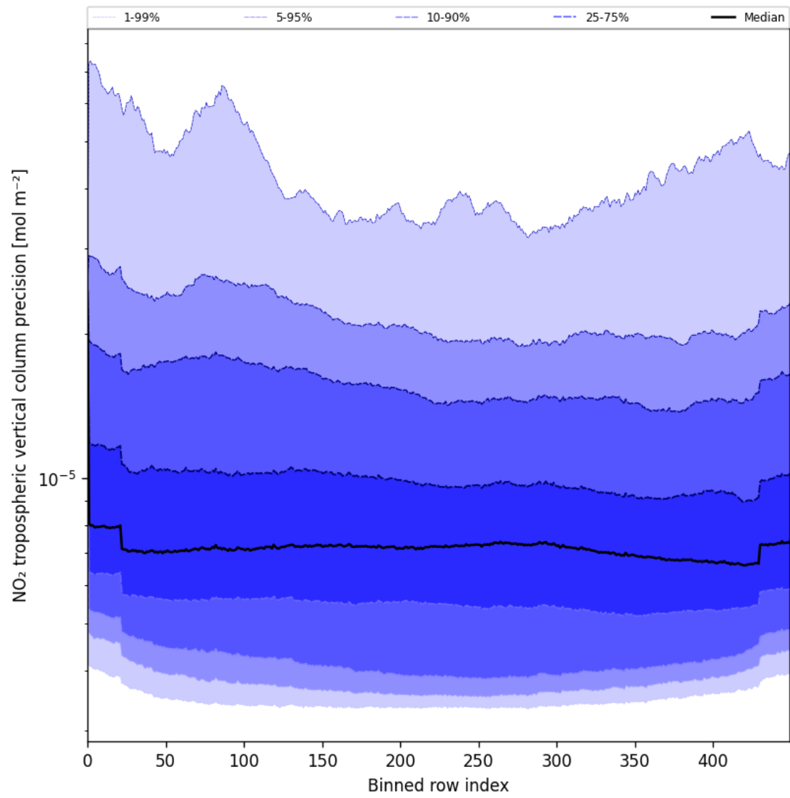
Figure 45: Along track statistics of “NO 2 tropospheric vertical column precision” for 2025-05-29 to 2025-05-29
