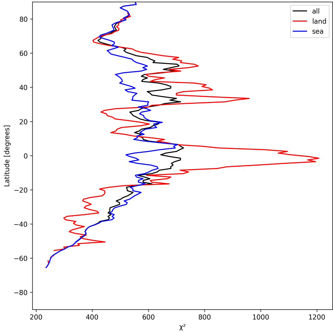
Figure 23: Zonal average of “ \chi^2 ” for 2025-05-29 to 2025-05-29.
