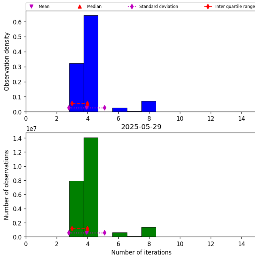
Figure 32: Histogram of “Number of iterations” for 2025-05-29 to 2025-05-29
