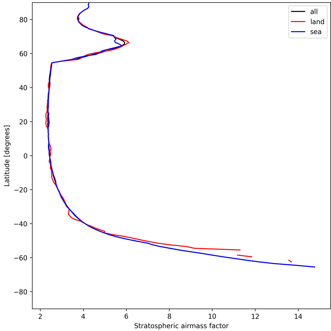
Figure 25: Zonal average of “Stratospheric air mass factor” for 2025-05-29 to 2025-05-29.
