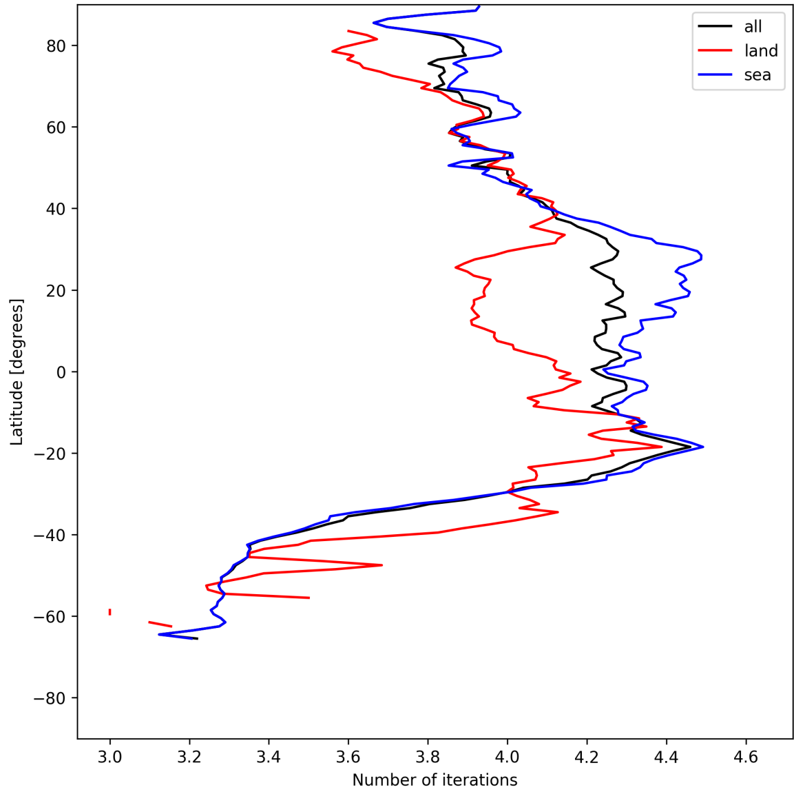
Figure 15: Zonal average of “Number of iterations” for 2025-05-29 to 2025-05-29.
