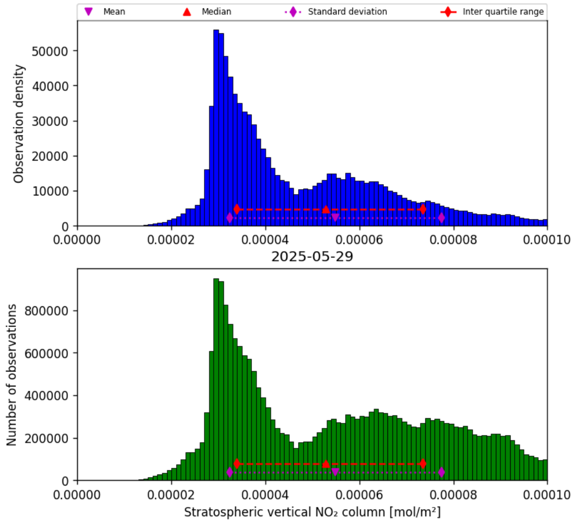
Figure 34: Histogram of “Stratospheric vertical NO 2 column” for 2025-05-29 to 2025-05-29
