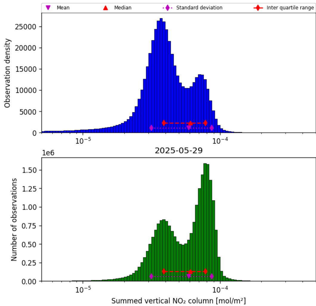
Figure 38: Histogram of “Summed vertical NO 2 column” for 2025-05-29 to 2025-05-29
