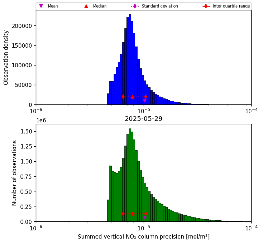
Figure 39: Histogram of "Summed vertical NO 2 column precision" for 2025-05-29 to 2025-05-29
