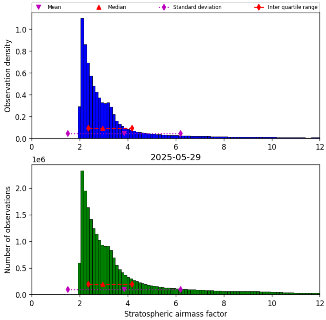
Figure 42: Histogram of “Stratospheric airmass factor” for 2025-05-29 to 2025-05-29
