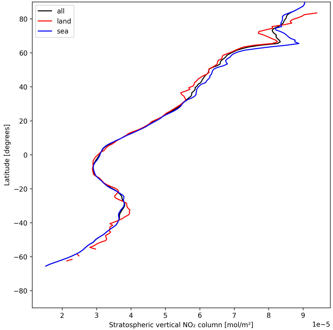
Figure 17: Zonal average of “Stratospheric vertical NO 2 column” for 2025-05-29 to 2025-05-29.
