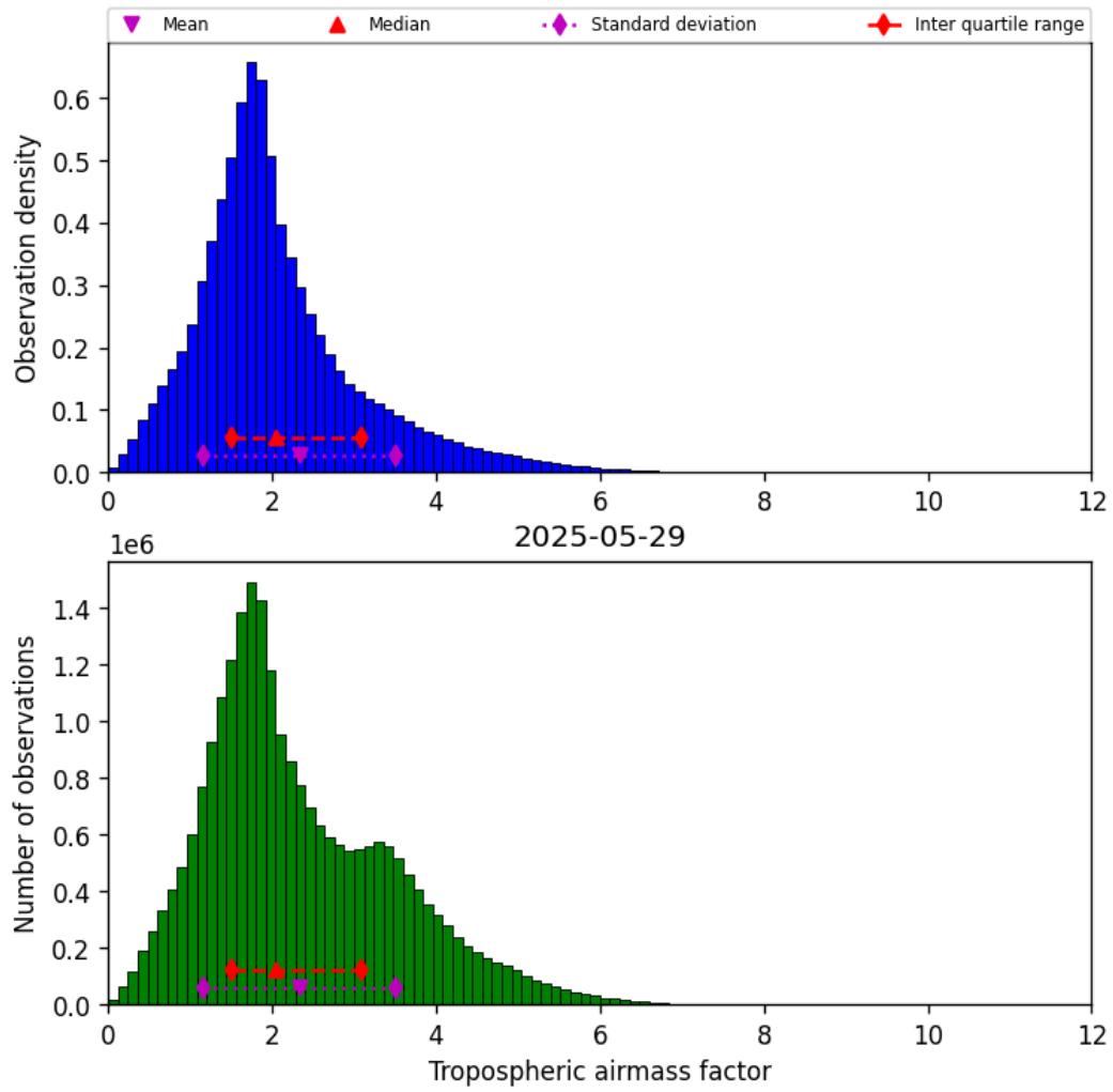
Figure 29: Histogram of “Tropospheric airmass factor” for 2025-05-29 to 2025-05-29
