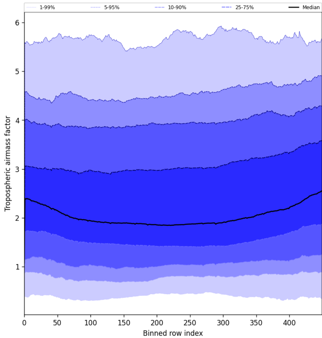
Figure 46: Along track statistics of “Tropospheric airmass factor” for 2025-05-29 to 2025-05-29
