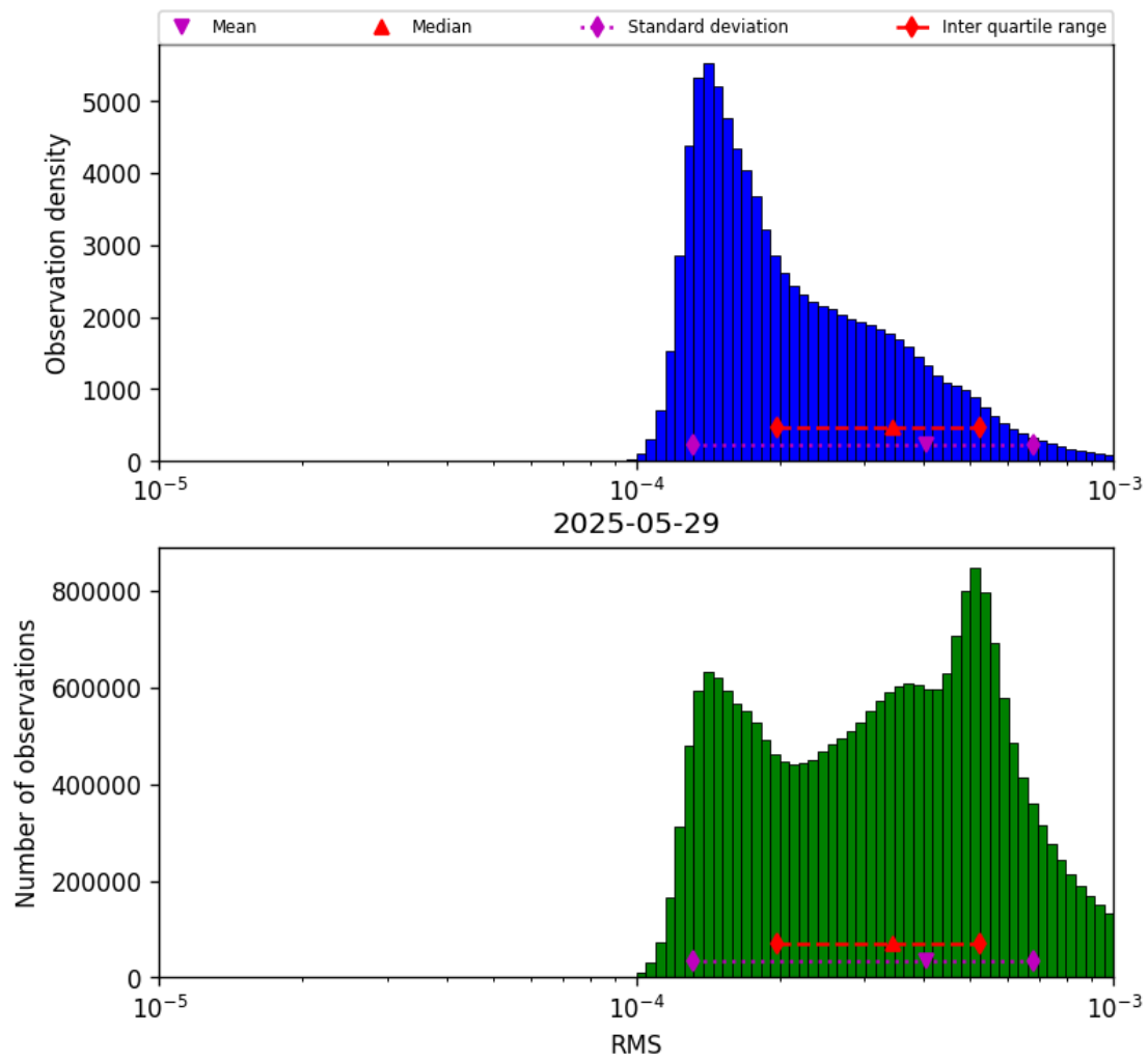
Figure 41: Histogram of “RMS” for 2025-05-29 to 2025-05-29
