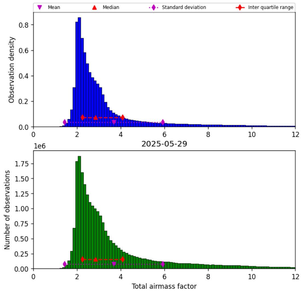
Figure 30: Histogram of “Total airmass factor” for 2025-05-29 to 2025-05-29
