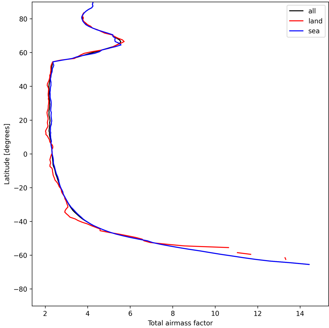
Figure 13: Zonal average of “Total airmass factor” for 2025-05-29 to 2025-05-29.
