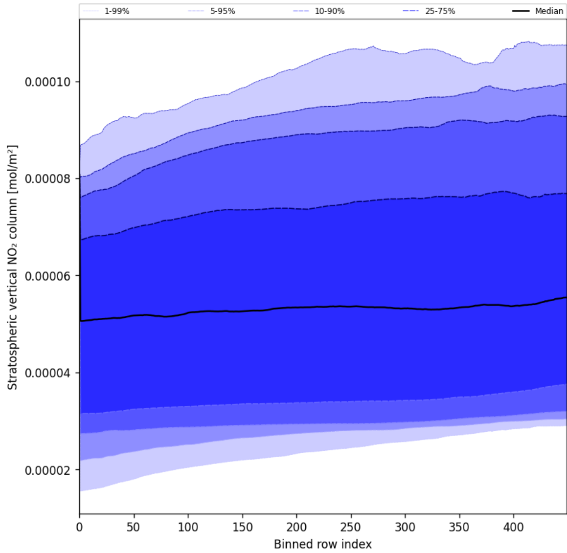
Figure 51: Along track statistics of “Stratospheric vertical NO 2 column” for 2025-05-29 to 2025-05-29
