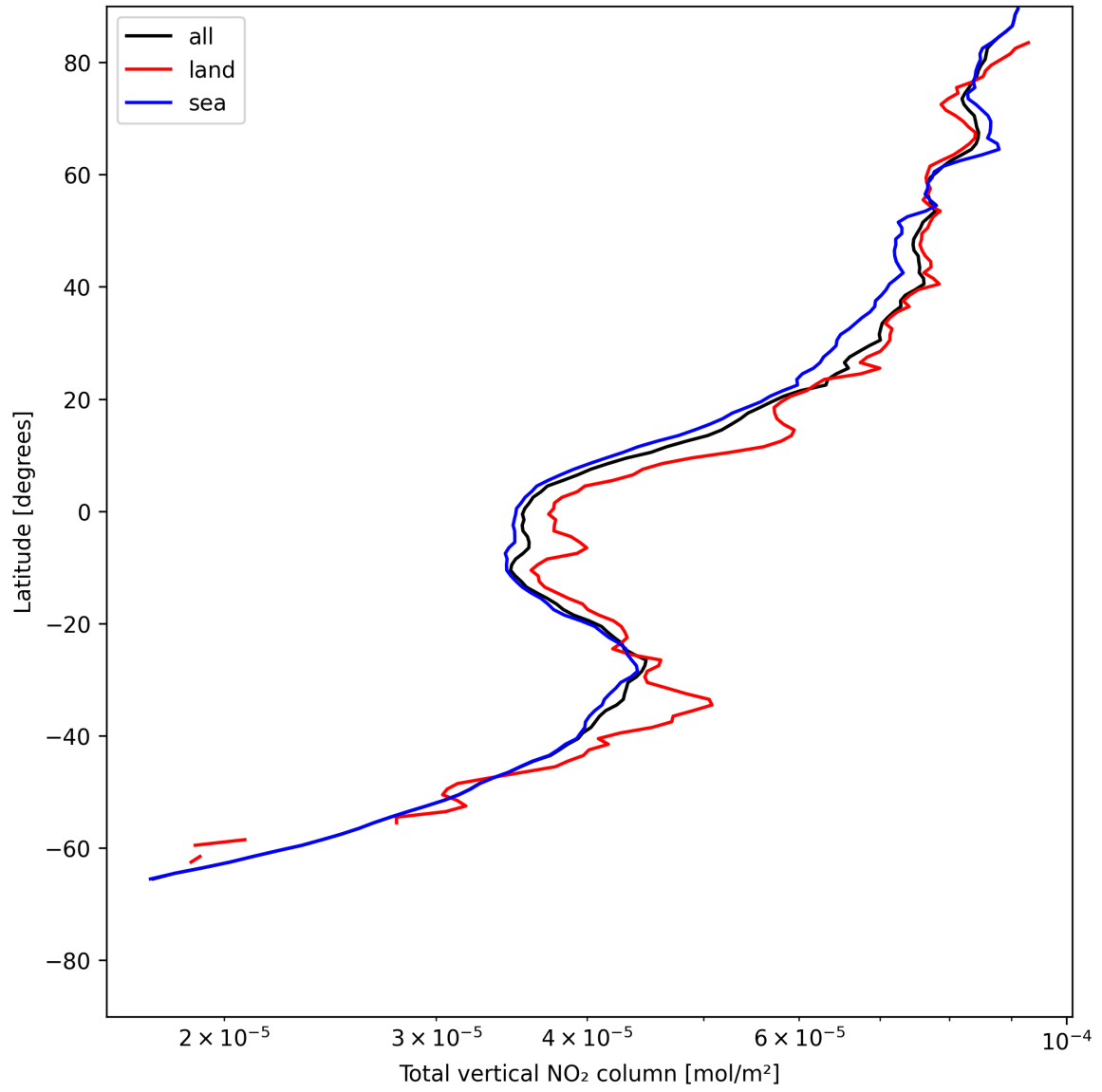
Figure 19: Zonal average of “Total vertical NO 2 column” for 2025-05-29 to 2025-05-29.
