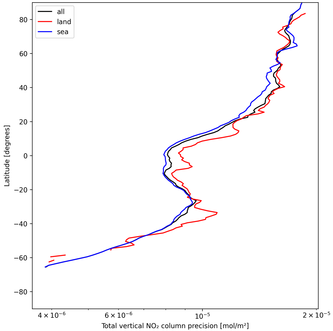
Figure 20: Zonal average of “Total vertical NO 2 column precision” for 2025-05-29 to 2025-05-29.
