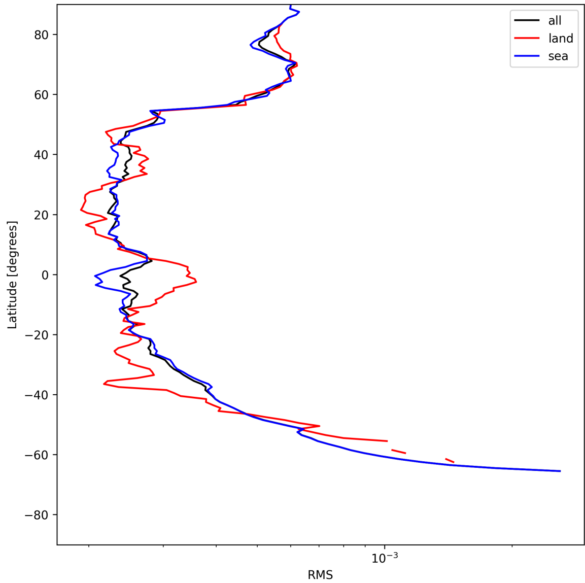
Figure 24: Zonal average of “RMS” for 2025-05-29 to 2025-05-29.
