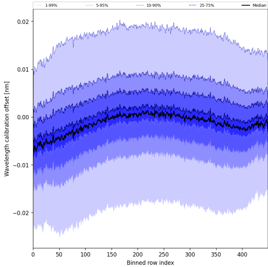
Figure 50: Along track statistics of “Wavelength calibration offset” for 2025-05-29 to 2025-05-29
