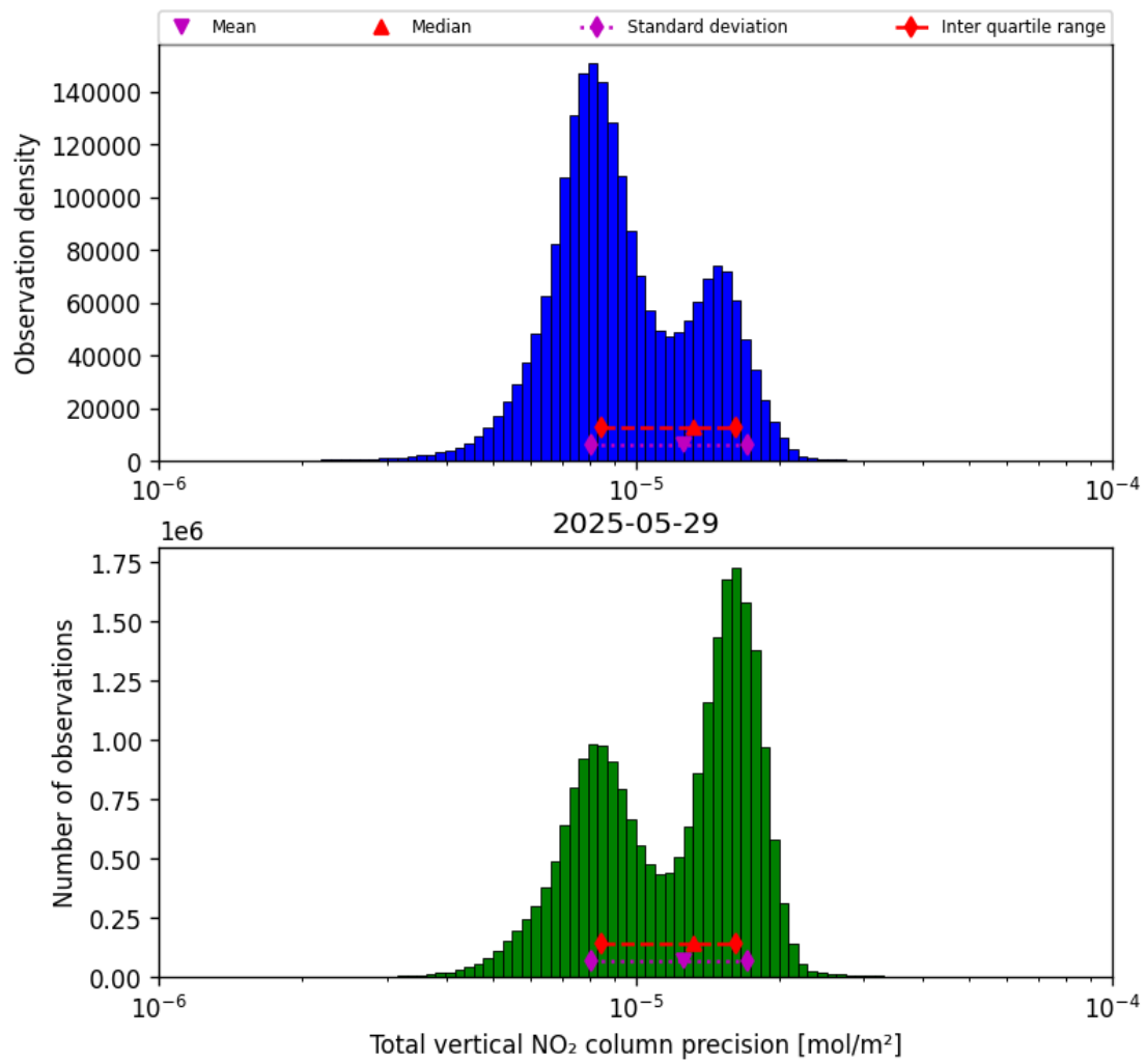
Figure 37: Histogram of “Total vertical NO 2 column precision” for 2025-05-29 to 2025-05-29
