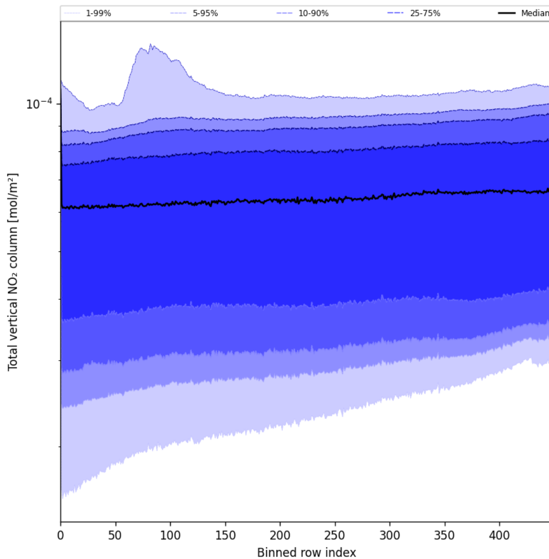
Figure 53: Along track statistics of “Total vertical NO 2 column” for 2025-05-29 to 2025-05-29
