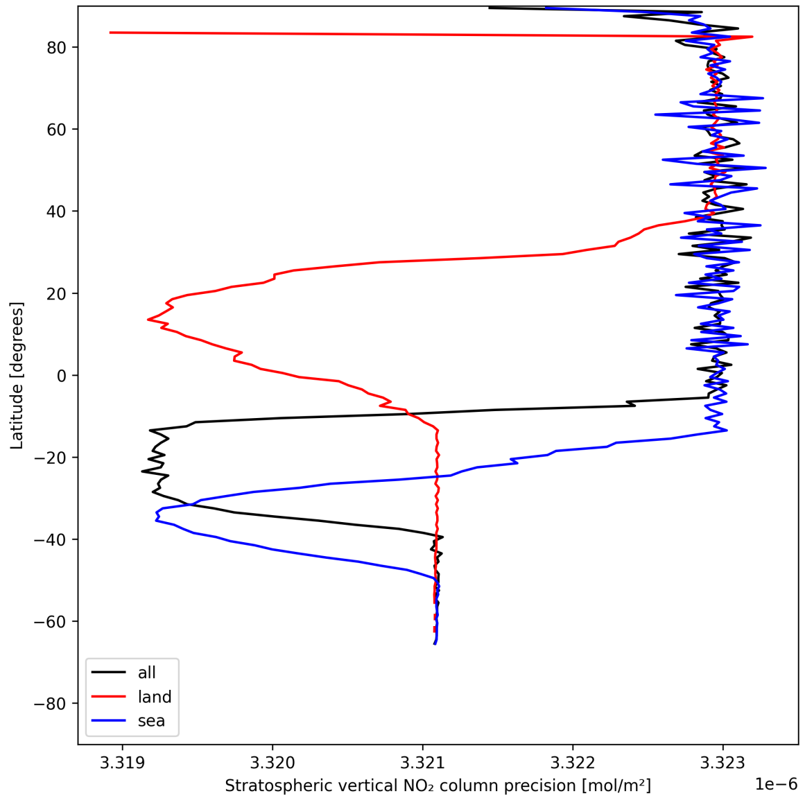
Figure 18: Zonal average of “Stratospheric vertical NO 2 column precision” for 2025-05-29 to 2025-05-29.
