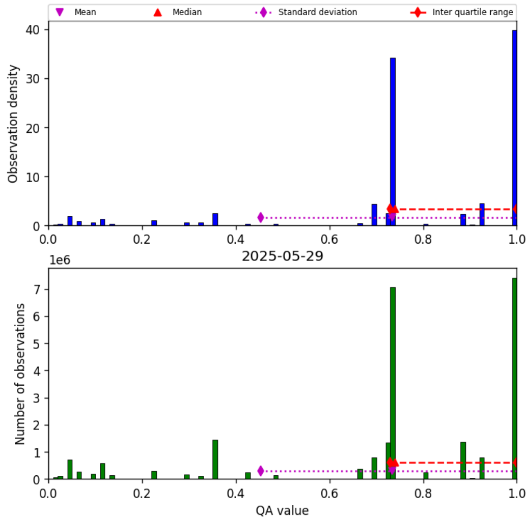
Figure 26: Histogram of “QA value” for 2025-05-29 to 2025-05-29
