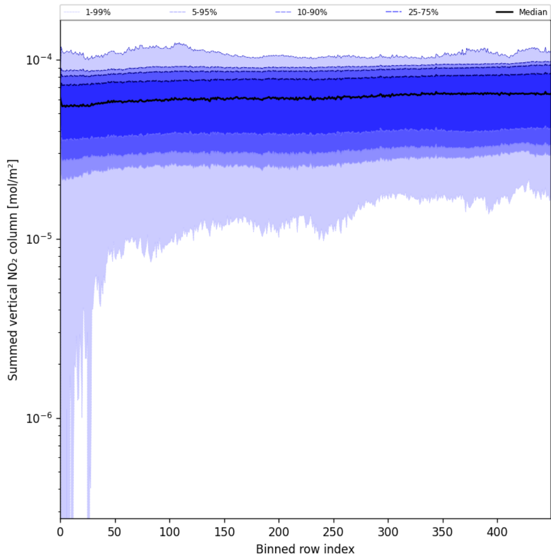
Figure 55: Along track statistics of “Summed vertical NO 2 column” for 2025-05-29 to 2025-05-29
