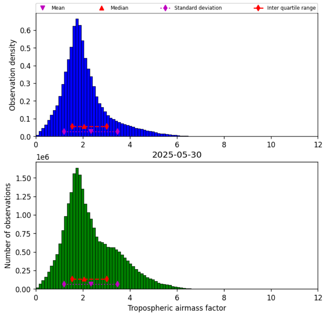
Figure 29: Histogram of “Tropospheric airmass factor” for 2025-05-30 to 2025-05-31
