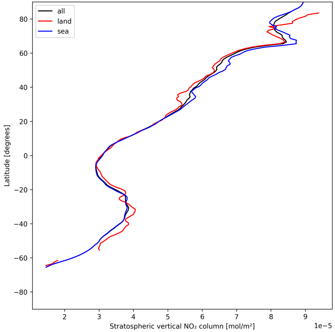
Figure 17: Zonal average of “Stratospheric vertical NO 2 column” for 2025-05-30 to 2025-05-31.
