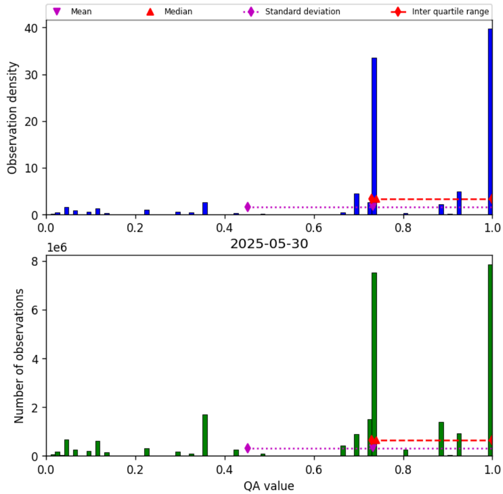
Figure 26: Histogram of “QA value” for 2025-05-30 to 2025-05-31
