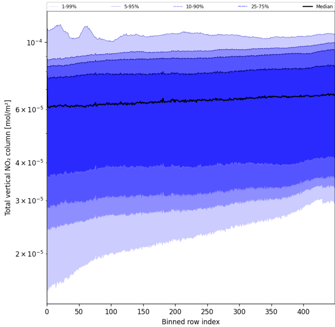
Figure 53: Along track statistics of “Total vertical NO 2 column” for 2025-05-30 to 2025-05-31
