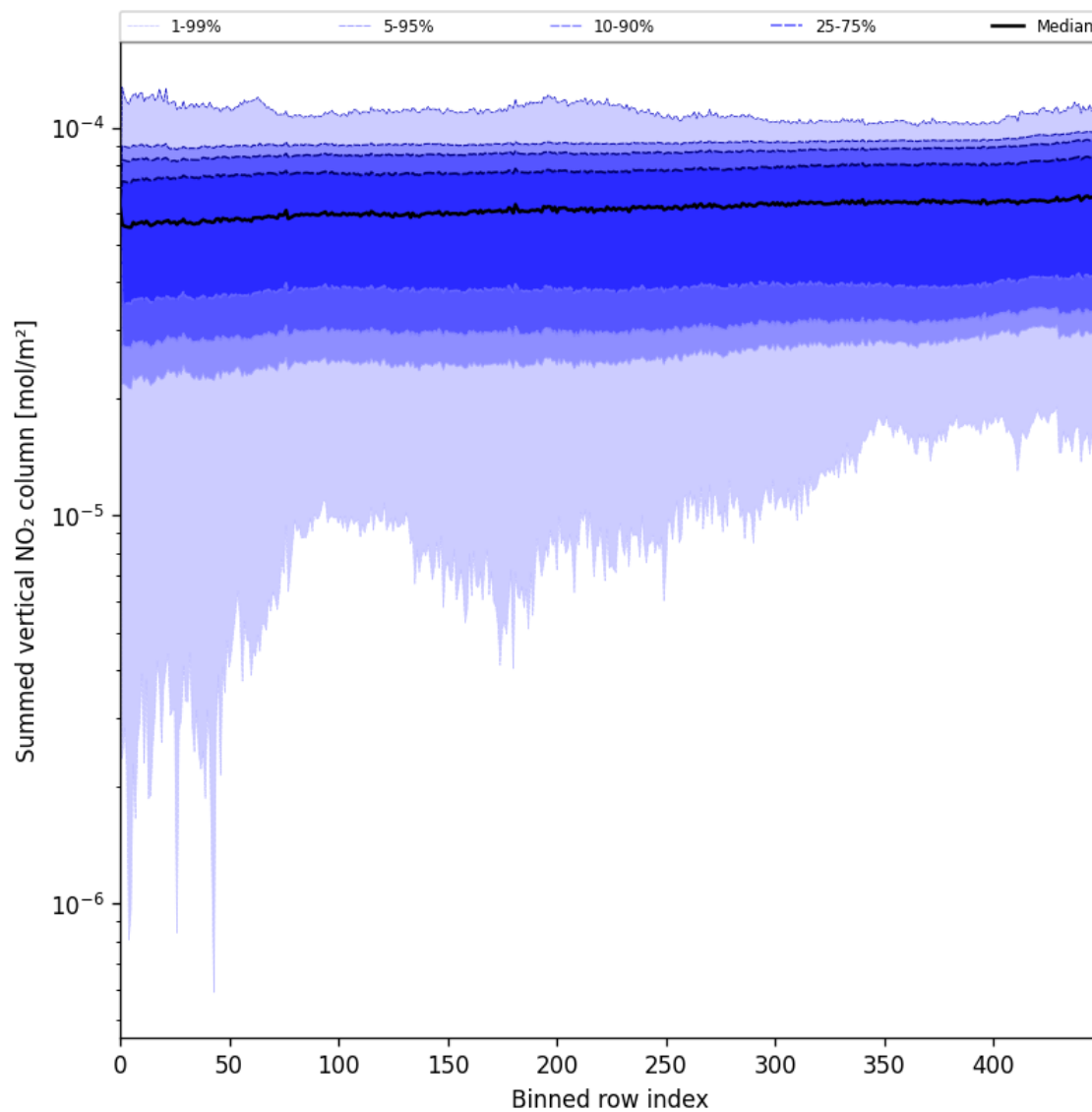
Figure 55: Along track statistics of “Summed vertical NO 2 column” for 2025-05-30 to 2025-05-31
