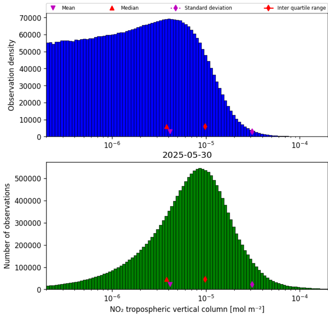
Figure 27: Histogram of “NO 2 tropospheric vertical column” for 2025-05-30 to 2025-05-31
