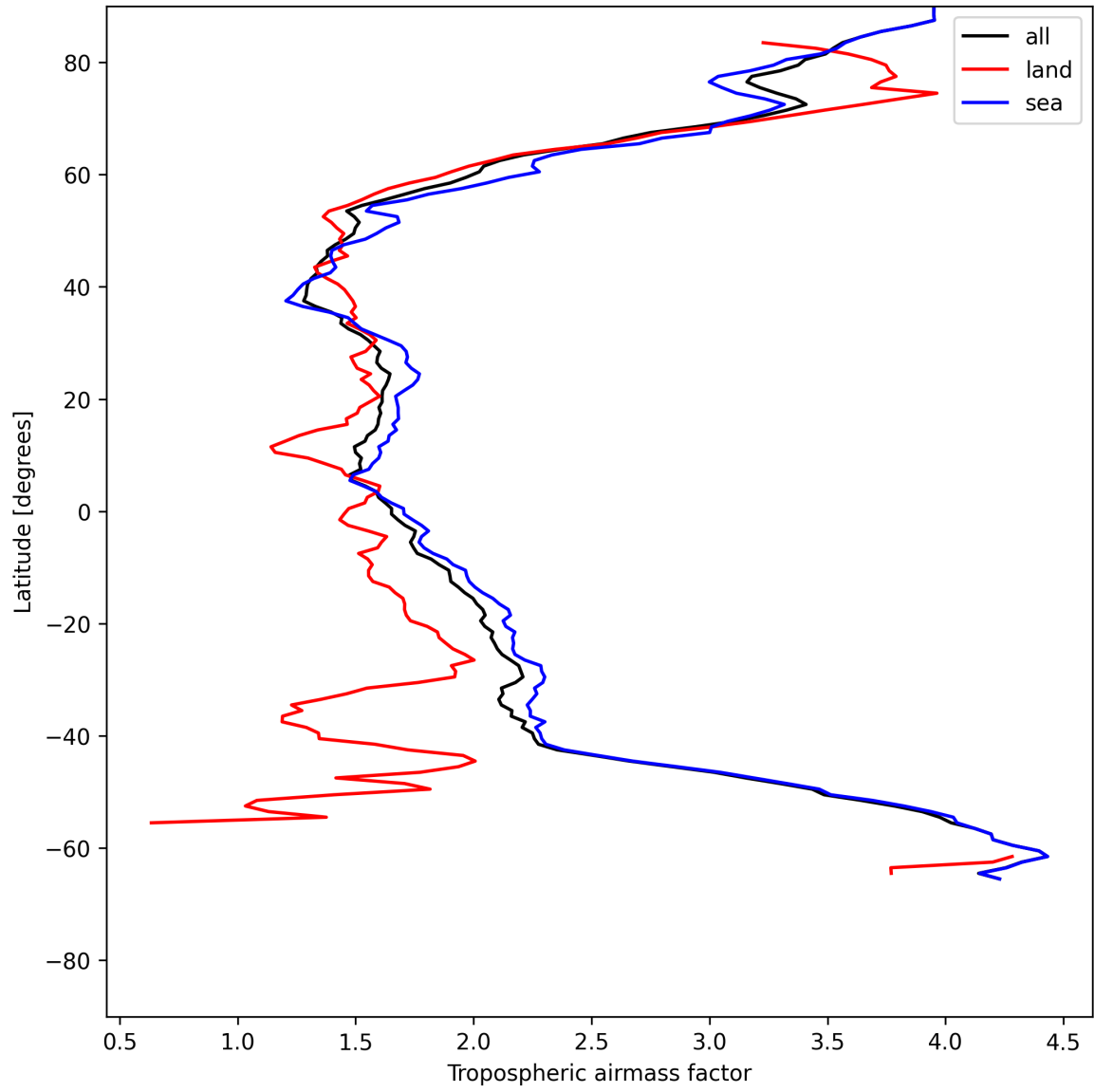
Figure 12: Zonal average of “Tropospheric airmass factor” for 2025-05-30 to 2025-05-31.
