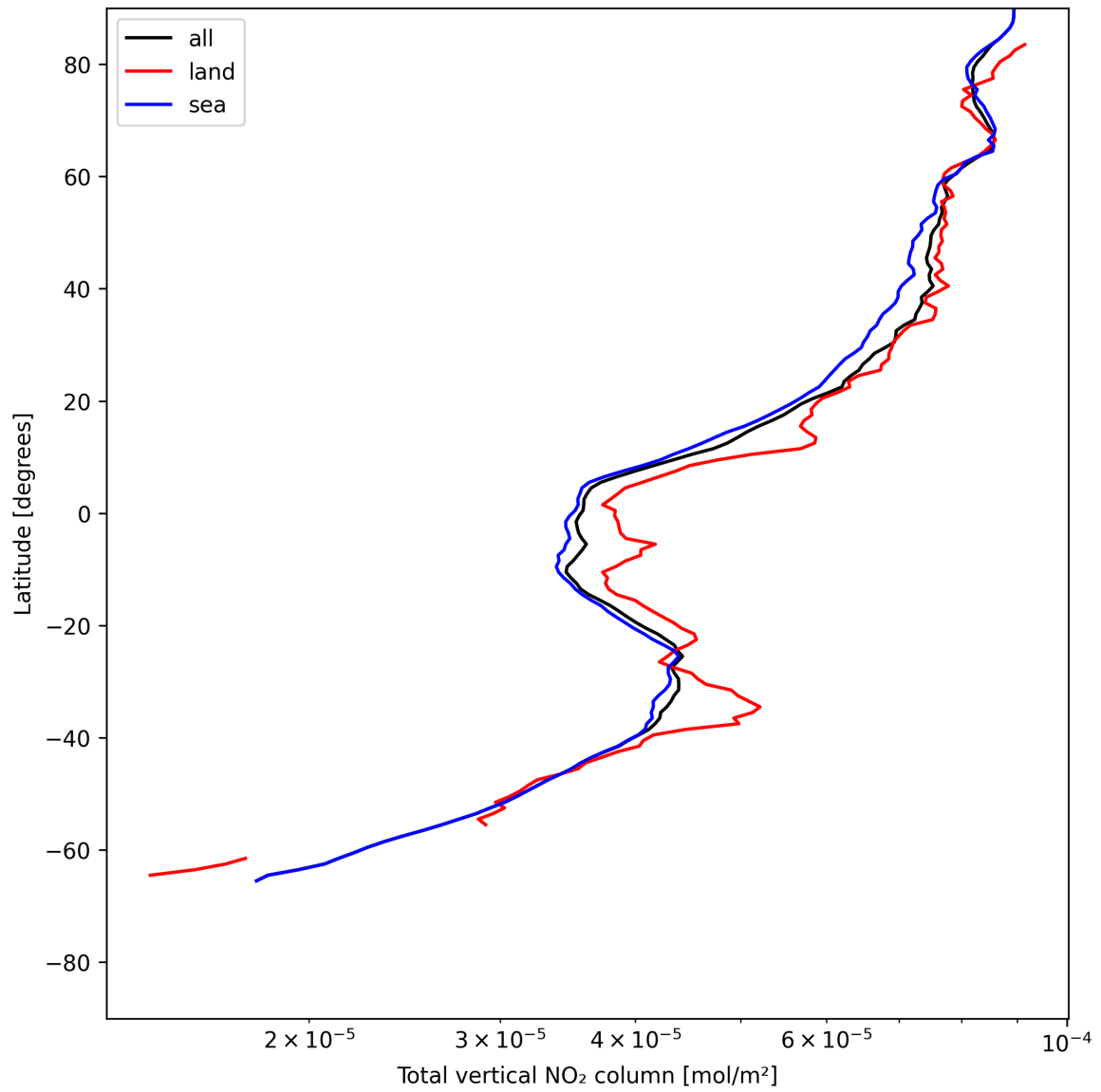
Figure 19: Zonal average of “Total vertical NO 2 column” for 2025-05-30 to 2025-05-31.
