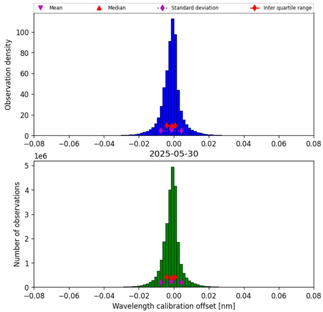
Figure 33: Histogram of “Wavelength calibration offset” for 2025-05-30 to 2025-05-31
