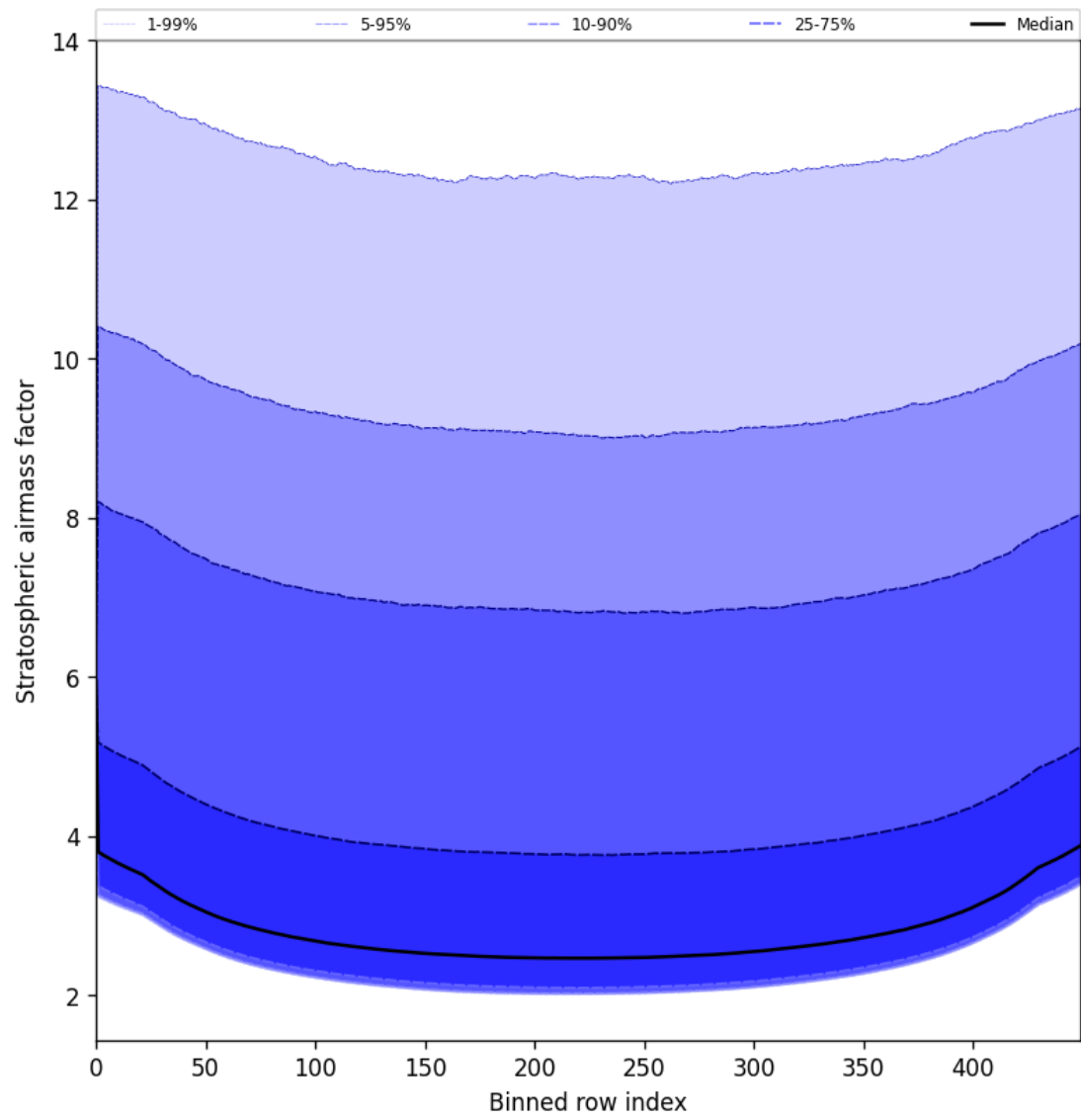
Figure 59: Along track statistics of “Stratospheric airmass factor” for 2025-05-30 to 2025-05-31
