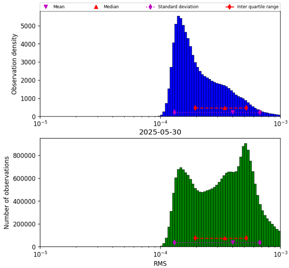
Figure 41: Histogram of “RMS” for 2025-05-30 to 2025-05-31
