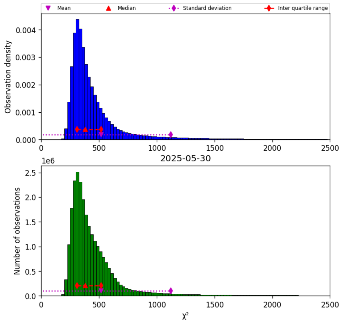
Figure 40: Histogram of “ \chi^2 ” for 2025-05-30 to 2025-05-31
