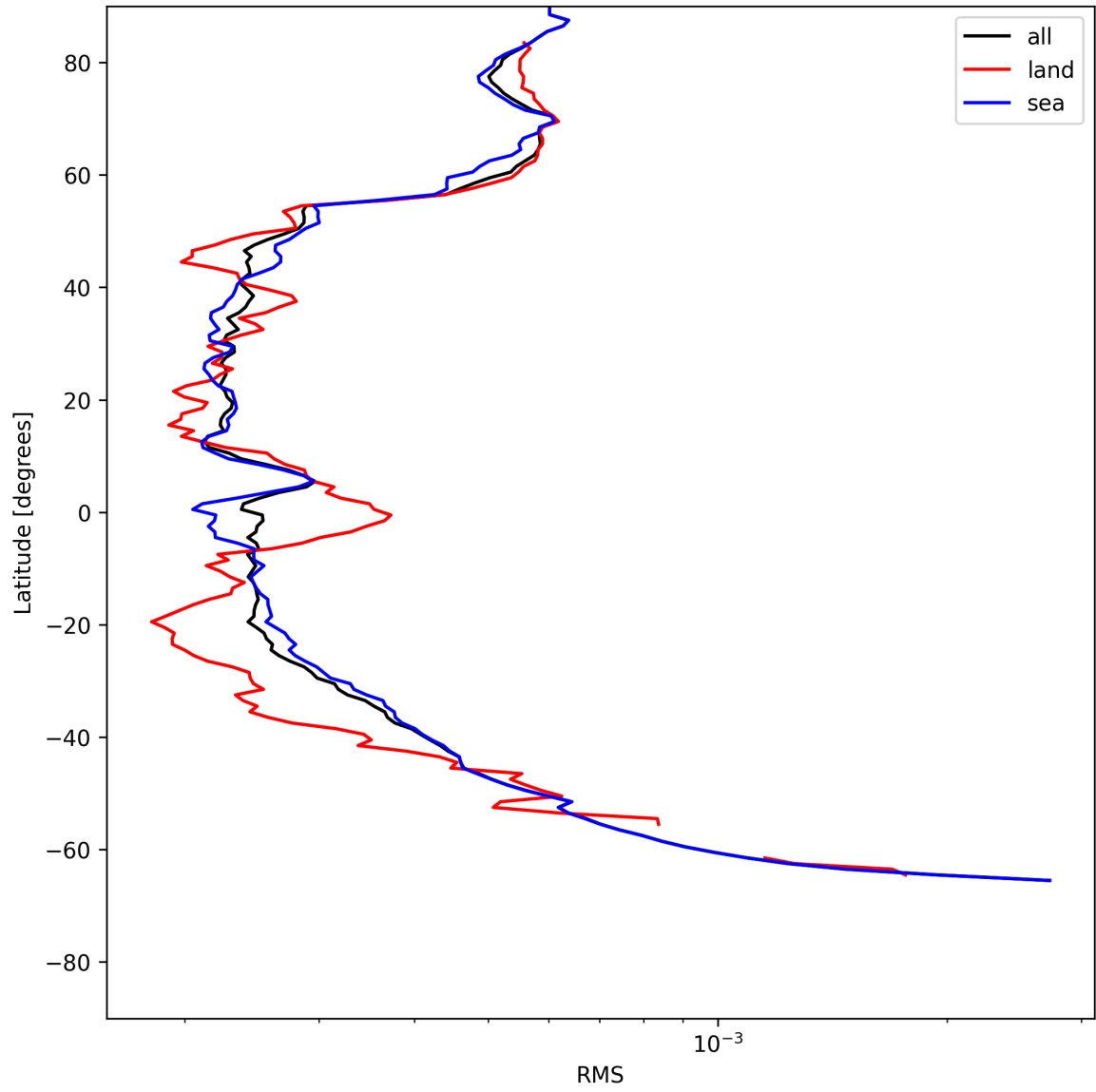
Figure 24: Zonal average of “RMS” for 2025-05-30 to 2025-05-31.
