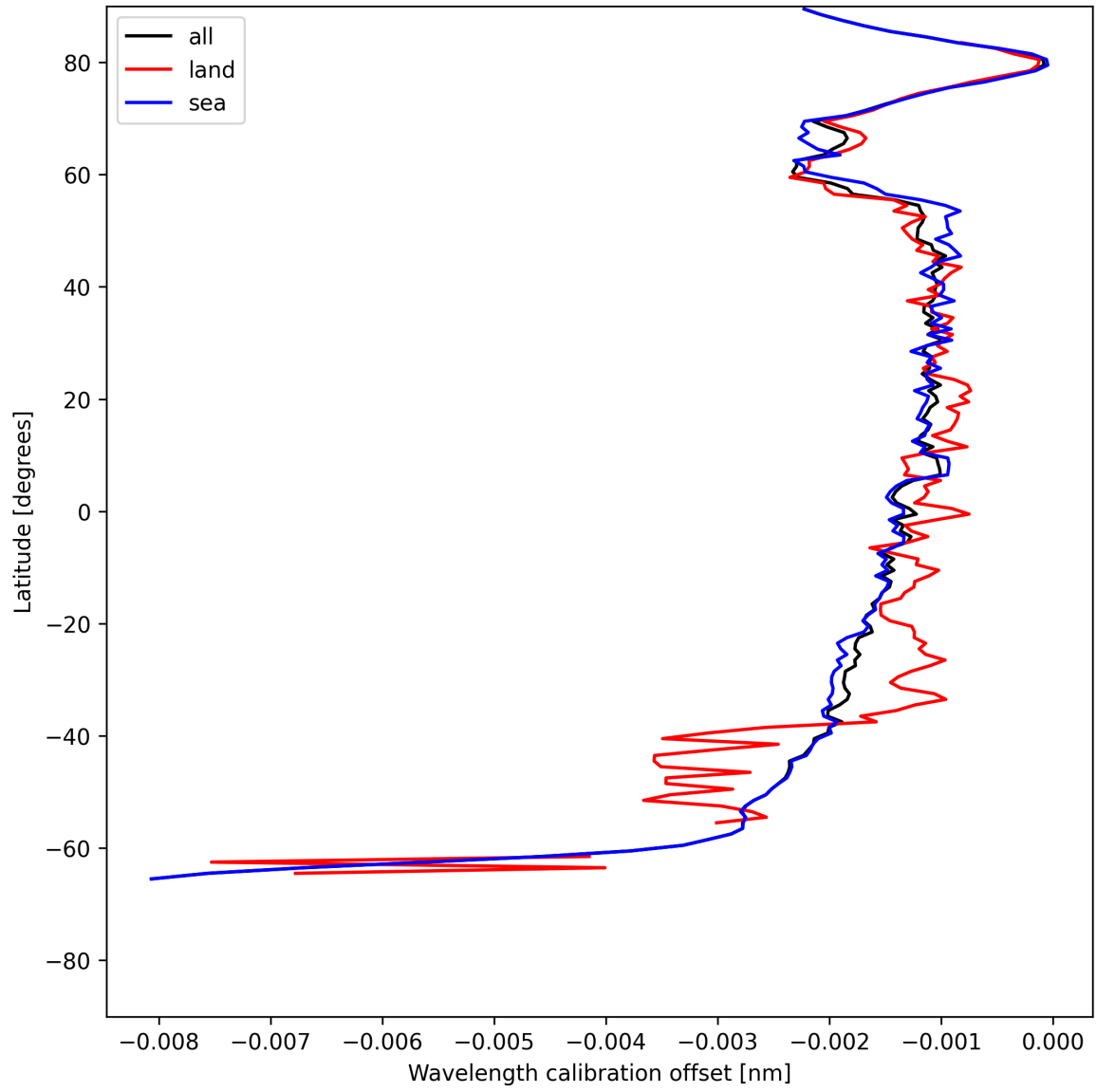
Figure 16: Zonal average of “Wavelength calibration offset” for 2025-05-30 to 2025-05-31.
