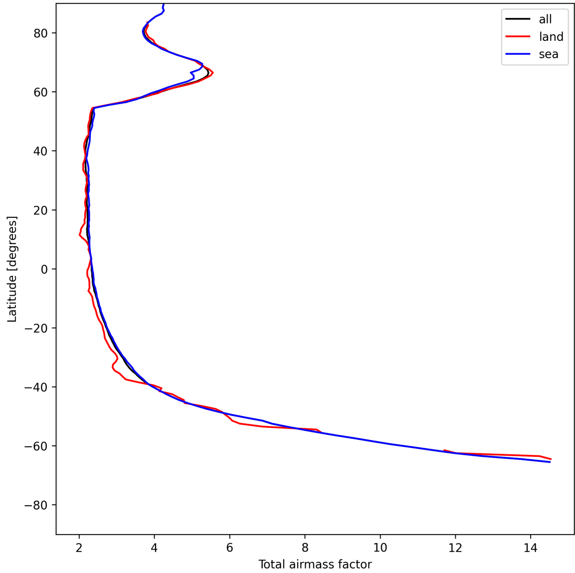
Figure 13: Zonal average of “Total airmass factor” for 2025-05-30 to 2025-05-31.
