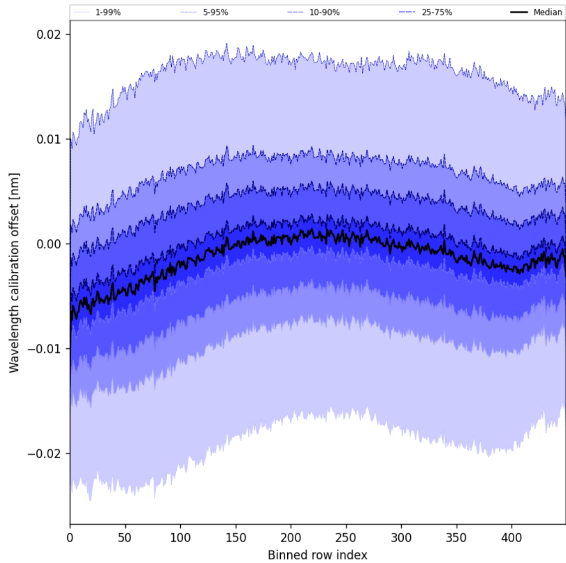
Figure 50: Along track statistics of “Wavelength calibration offset” for 2025-05-30 to 2025-05-31
