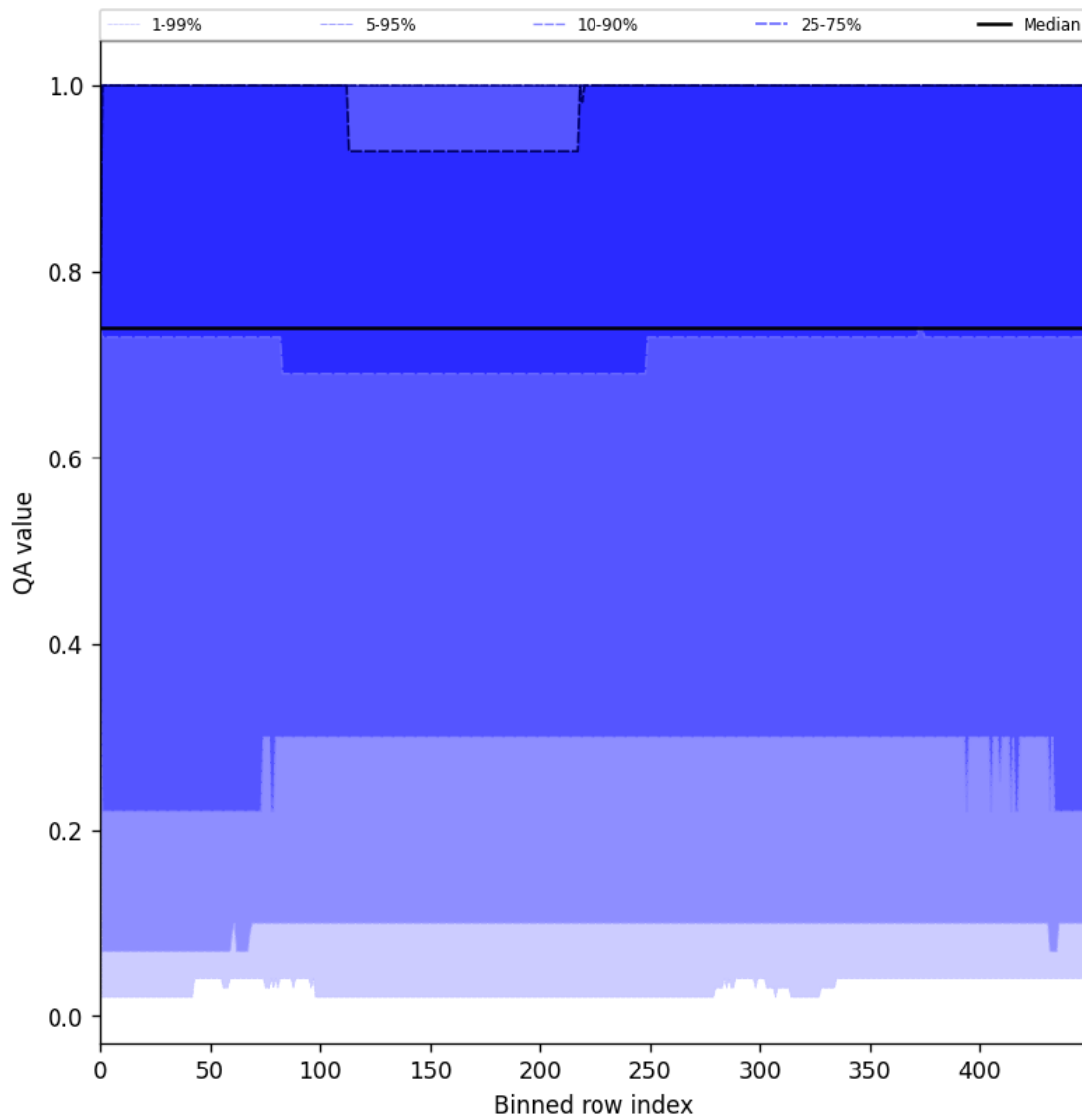
Figure 43: Along track statistics of “QA value” for 2025-05-30 to 2025-05-31
