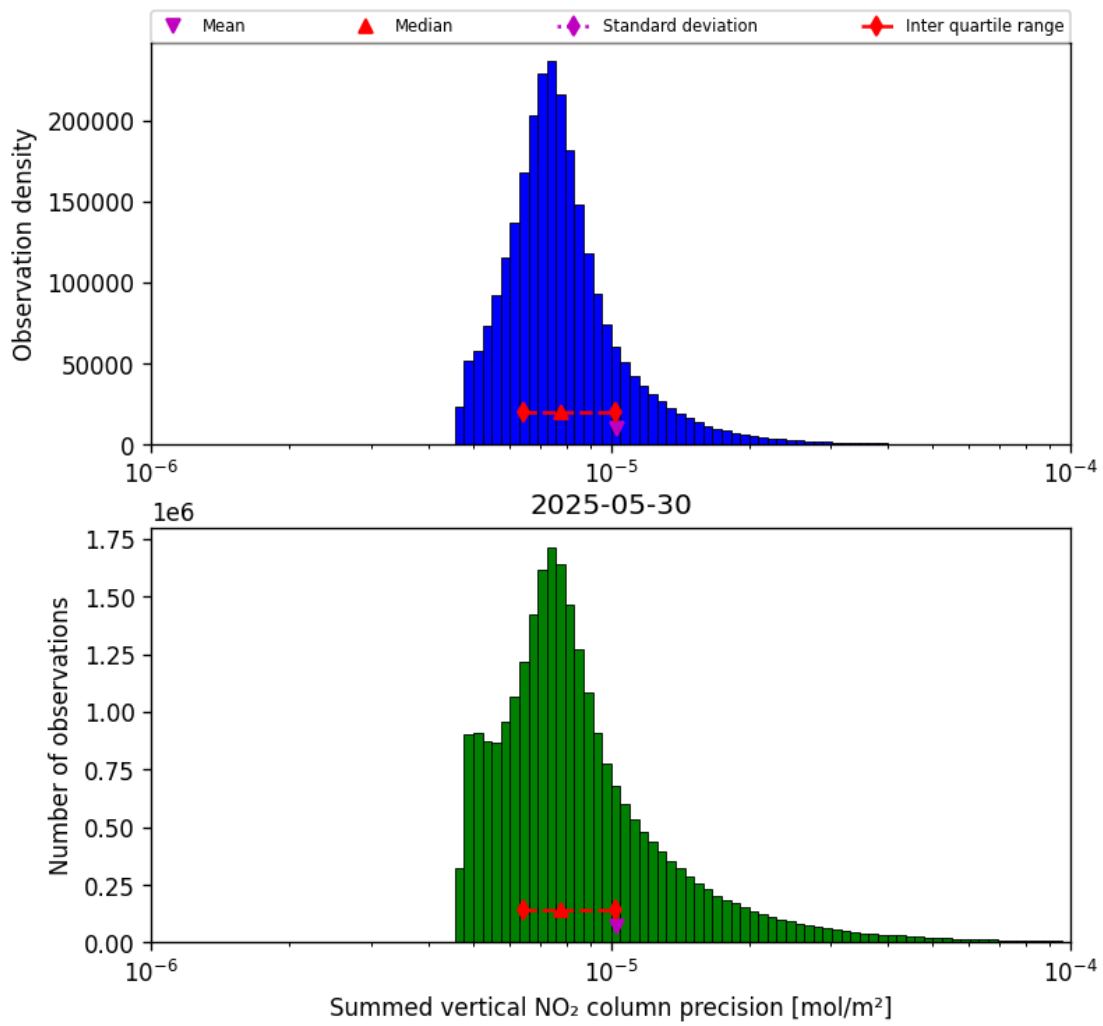
Figure 39: Histogram of “Summed vertical NO 2 column precision” for 2025-05-30 to 2025-05-31
