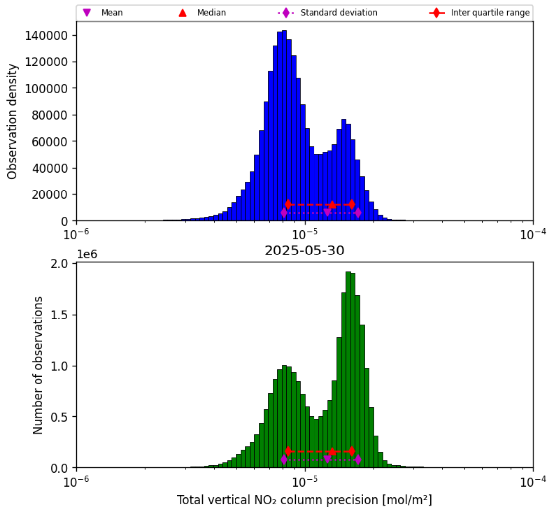
Figure 37: Histogram of “Total vertical NO 2 column precision” for 2025-05-30 to 2025-05-31
