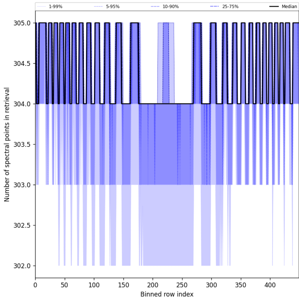
Figure 48: Along track statistics of “Number of spectral points in retrieval” for 2025-05-30 to 2025-05-31
