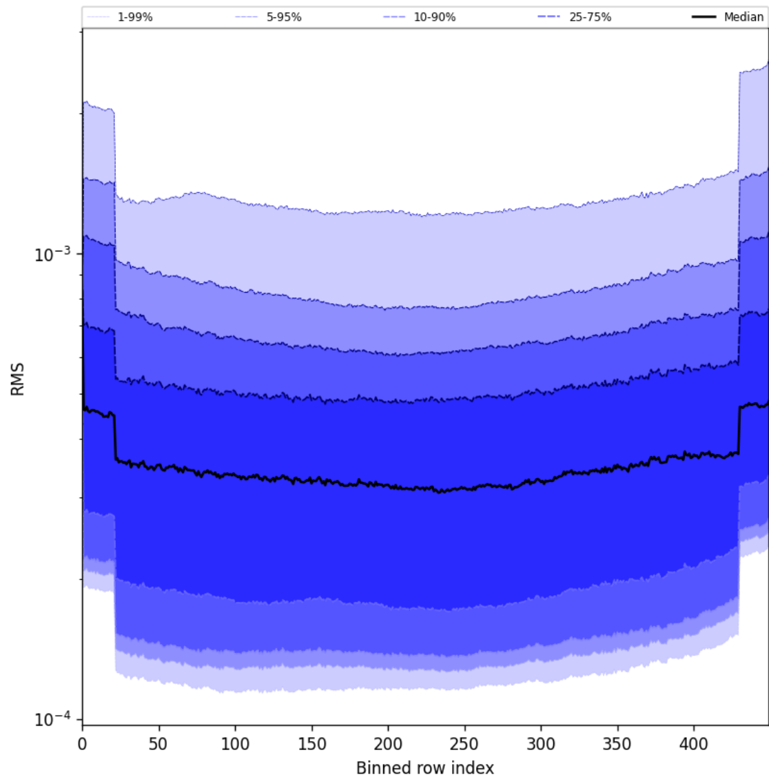
Figure 58: Along track statistics of “RMS” for 2025-05-30 to 2025-05-31
