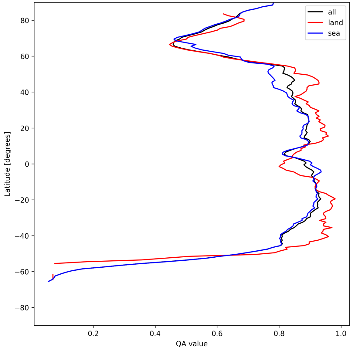
Figure 9: Zonal average of “QA value” for 2025-05-30 to 2025-05-31.
