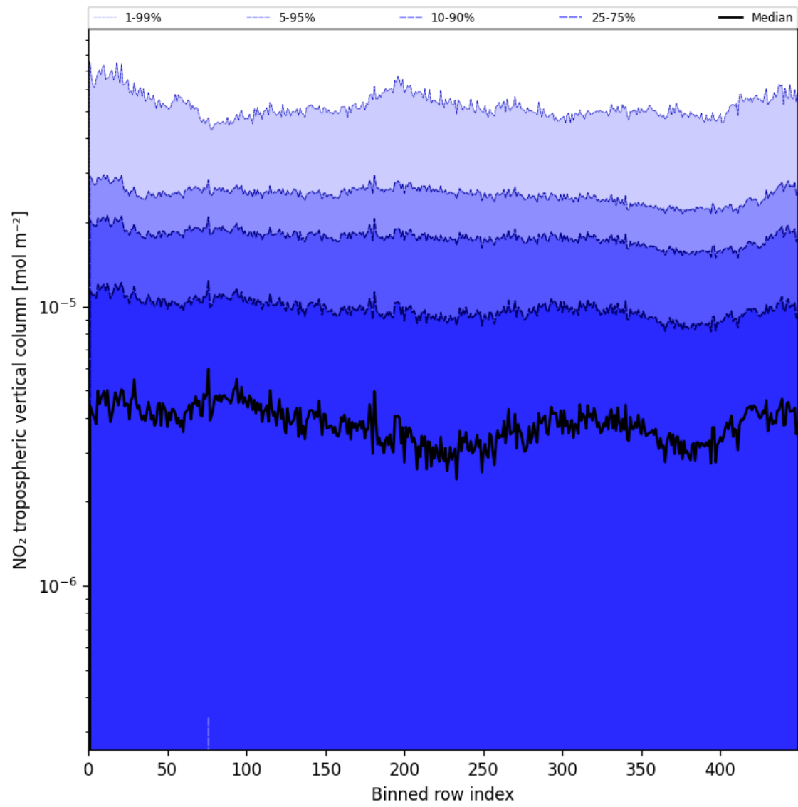
Figure 44: Along track statistics of “NO 2 tropospheric vertical column” for 2025-05-30 to 2025-05-31
