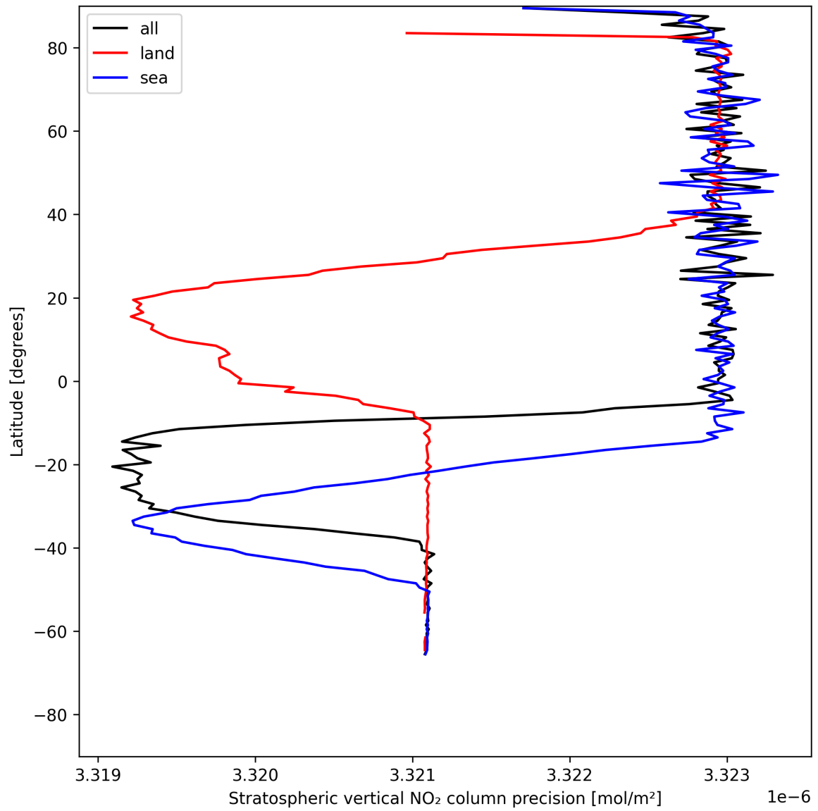
Figure 18: Zonal average of “Stratospheric vertical NO 2 column precision” for 2025-05-30 to 2025-05-31.
