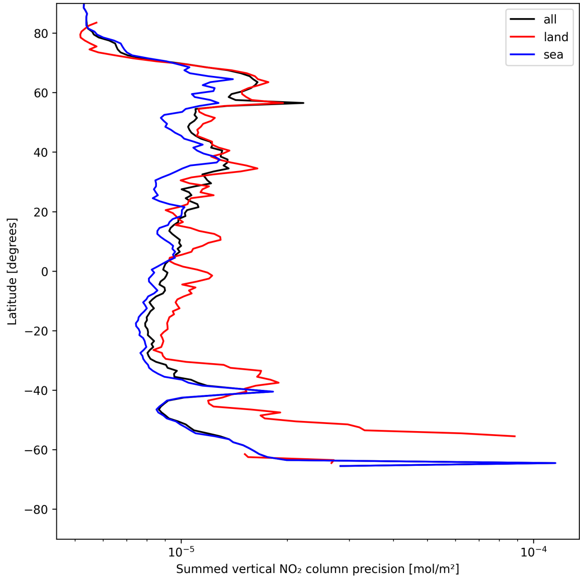
Figure 22: Zonal average of “Summed vertical NO 2 column precision” for 2025-05-30 to 2025-05-31.
