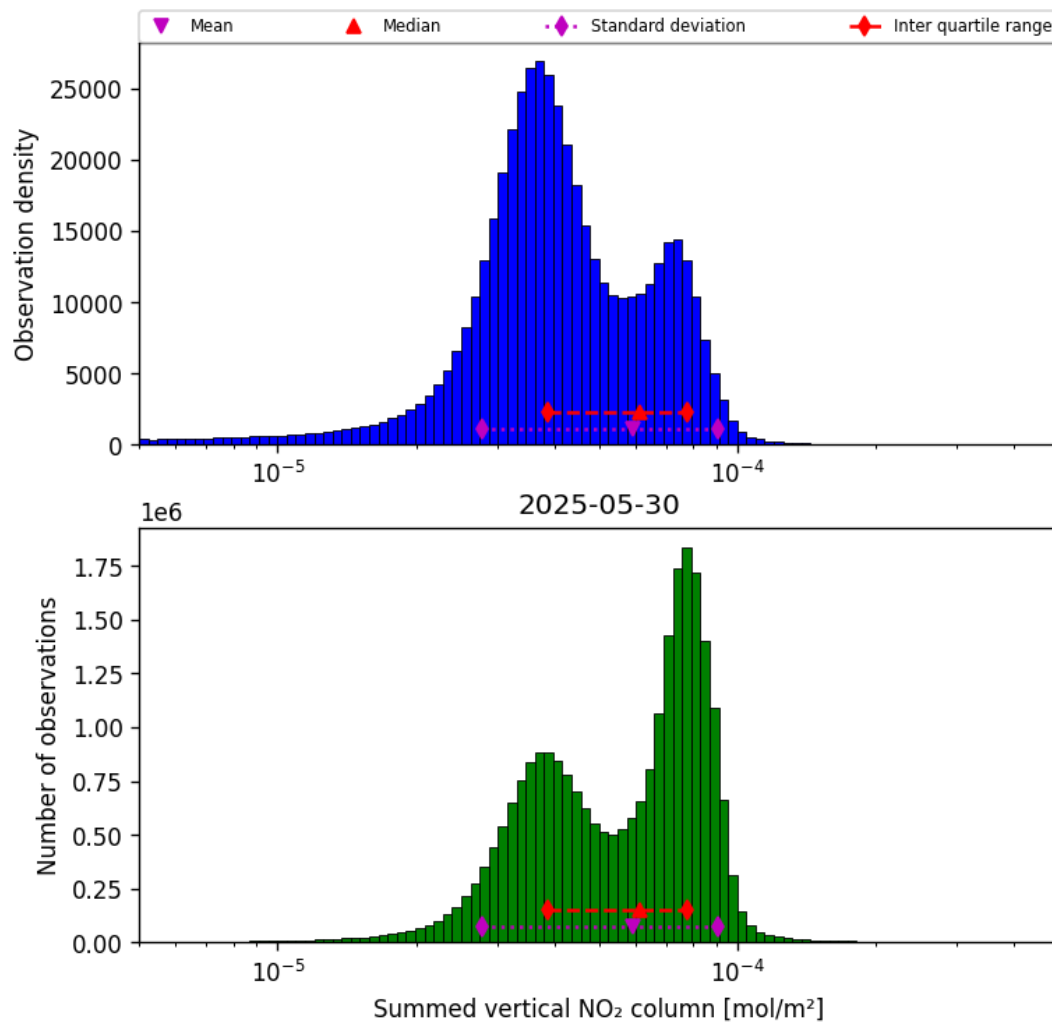
Figure 38: Histogram of “Summed vertical NO 2 column” for 2025-05-30 to 2025-05-31
