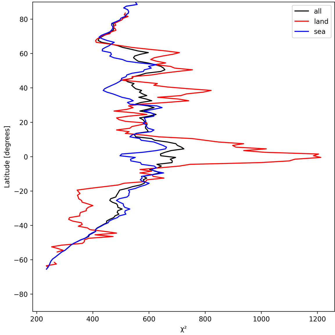
Figure 23: Zonal average of “ \chi^2 ” for 2025-05-30 to 2025-05-31.
