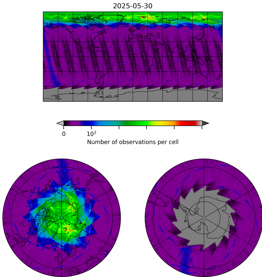
Figure 8: Map of the number of observations for 2025-05-30 to 2025-05-31
