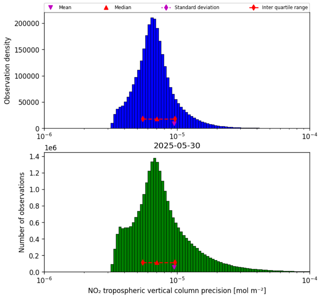
Figure 28: Histogram of “NO 2 tropospheric vertical column precision” for 2025-05-30 to 2025-05-31
