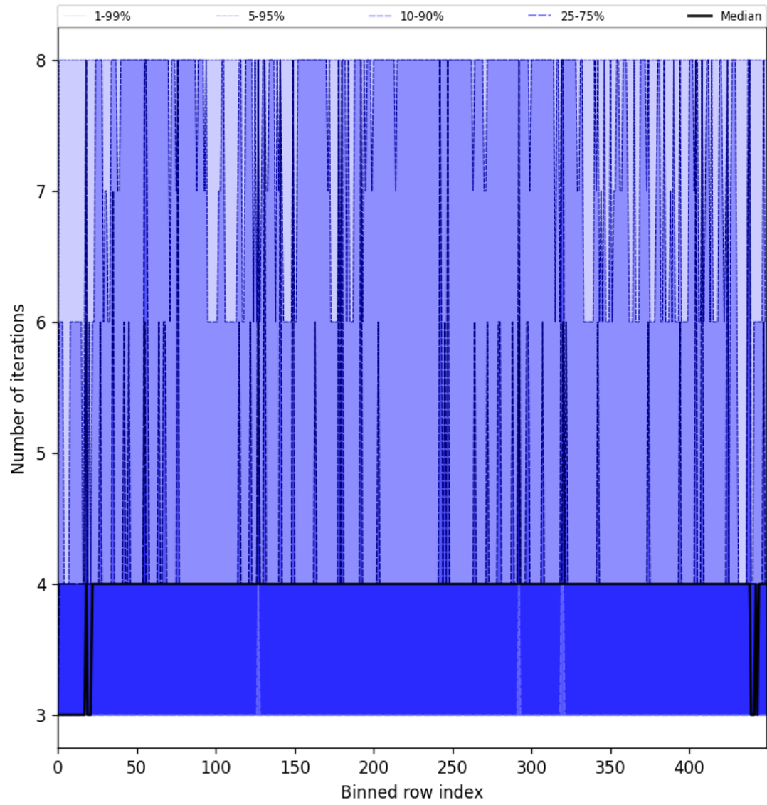
Figure 49: Along track statistics of “Number of iterations” for 2025-05-30 to 2025-05-31
