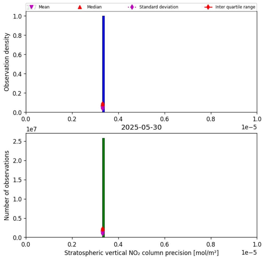
Figure 35: Histogram of “Stratospheric vertical NO 2 column precision” for 2025-05-30 to 2025-05-31
