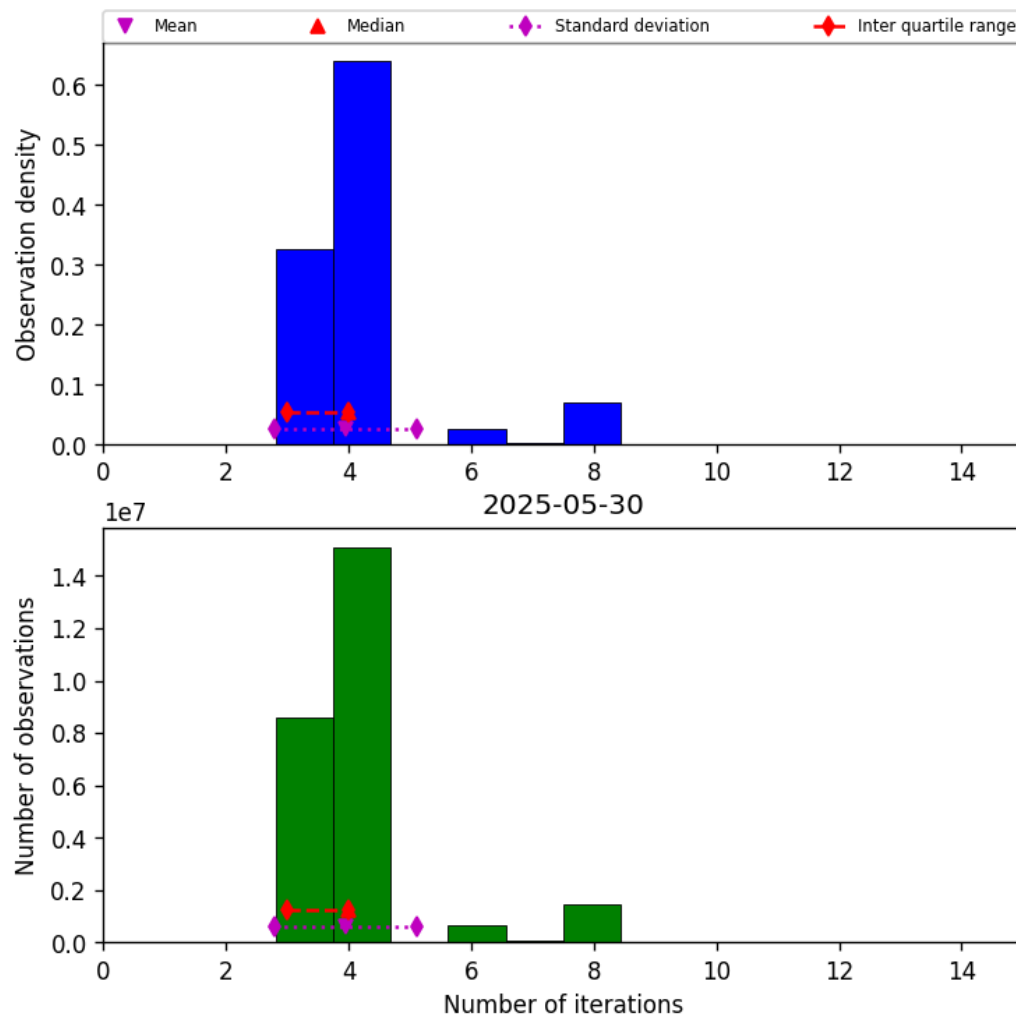
Figure 32: Histogram of “Number of iterations” for 2025-05-30 to 2025-05-31
