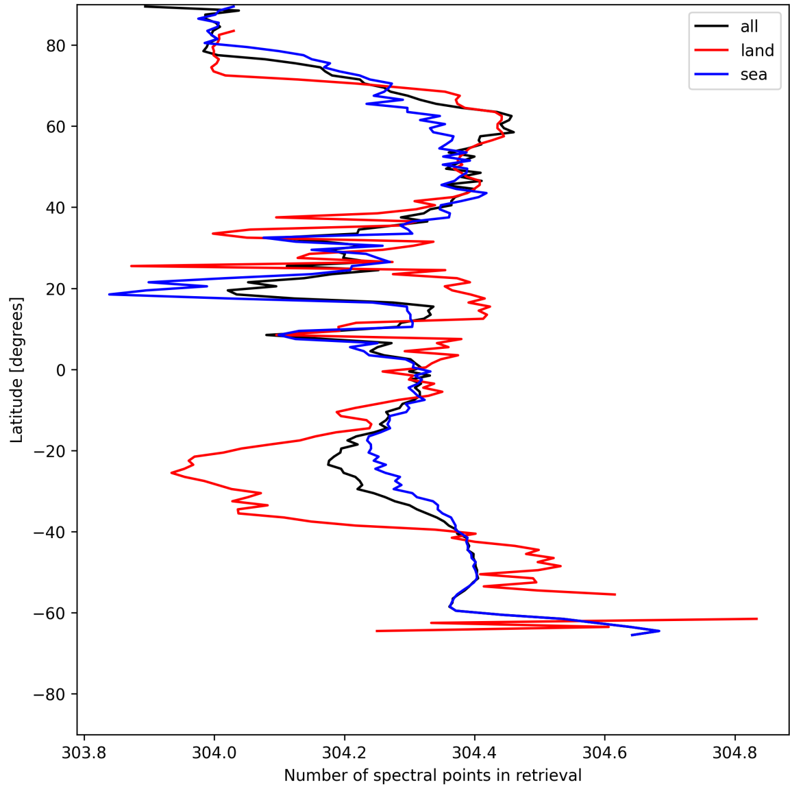
Figure 14: Zonal average of “Number of spectral points in retrieval” for 2025-05-30 to 2025-05-31.
