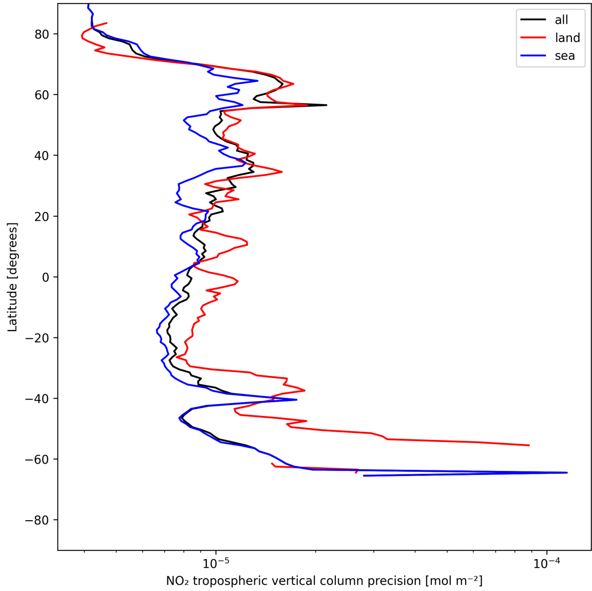
Figure 11: Zonal average of “NO 2 tropospheric vertical column precision” for 2025-05-30 to 2025-05-31.
