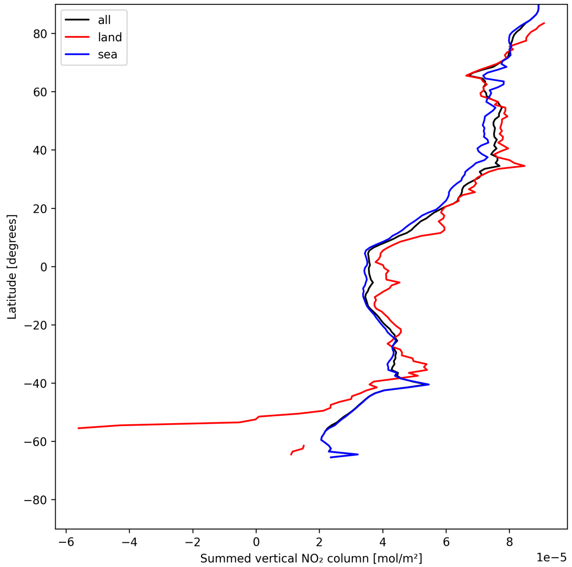
Figure 21: Zonal average of “Summed vertical NO 2 column” for 2025-05-30 to 2025-05-31.
