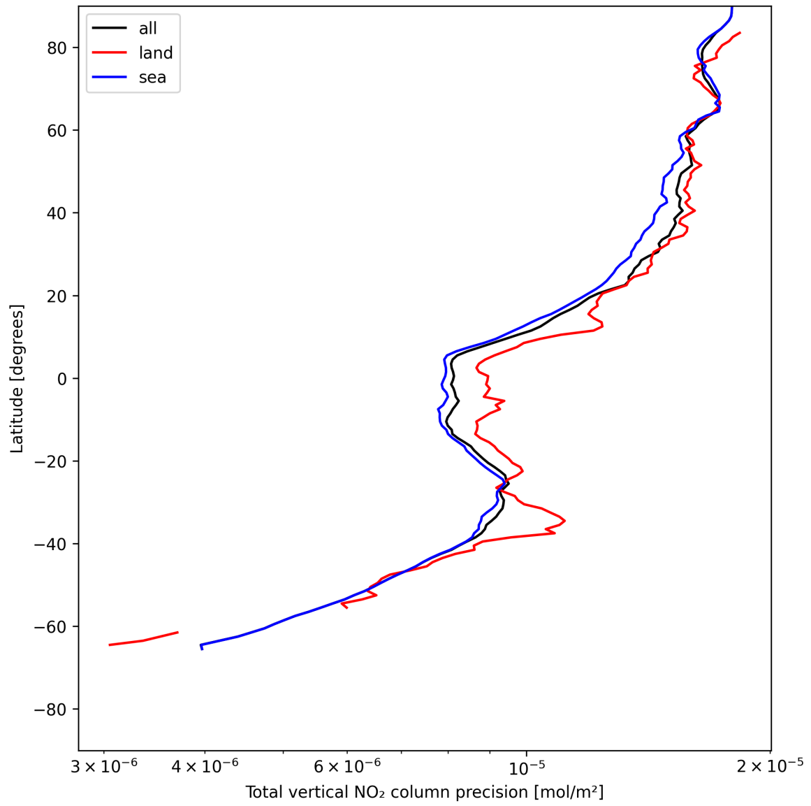
Figure 20: Zonal average of “Total vertical NO 2 column precision” for 2025-05-30 to 2025-05-31.
