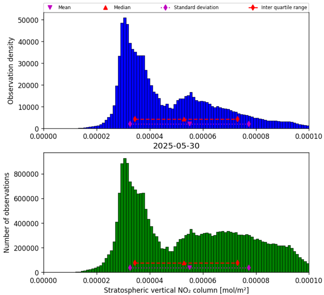
Figure 34: Histogram of “Stratospheric vertical NO 2 column” for 2025-05-30 to 2025-05-31
