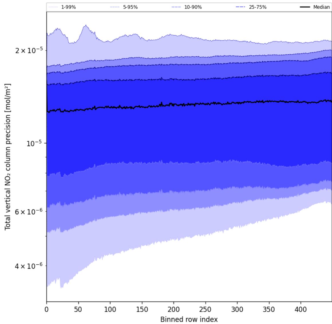
Figure 54: Along track statistics of “Total vertical NO 2 column precision” for 2025-05-30 to 2025-05-31
