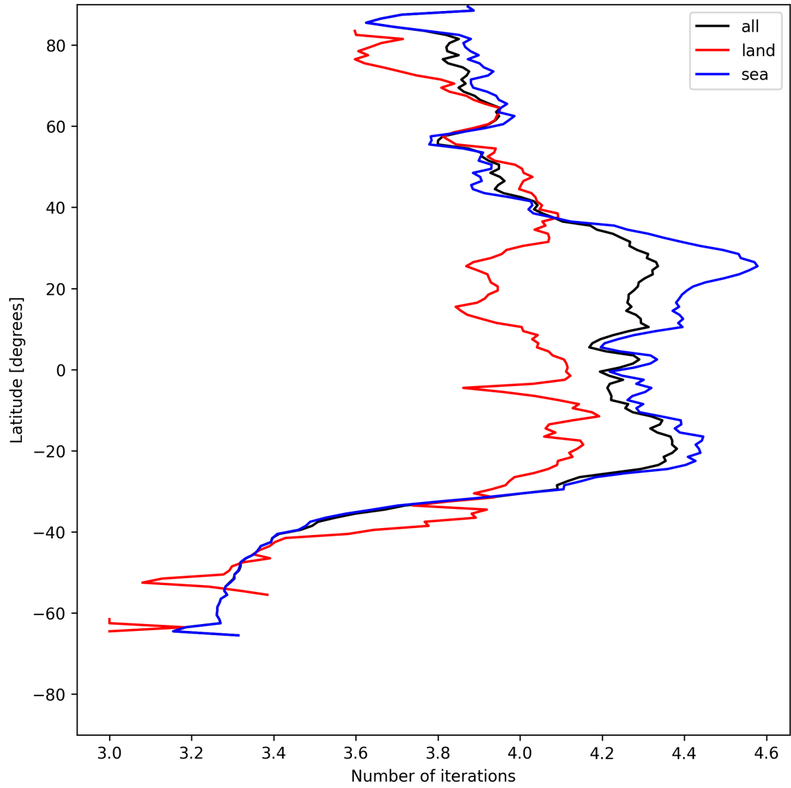
Figure 15: Zonal average of “Number of iterations” for 2025-05-30 to 2025-05-31.
