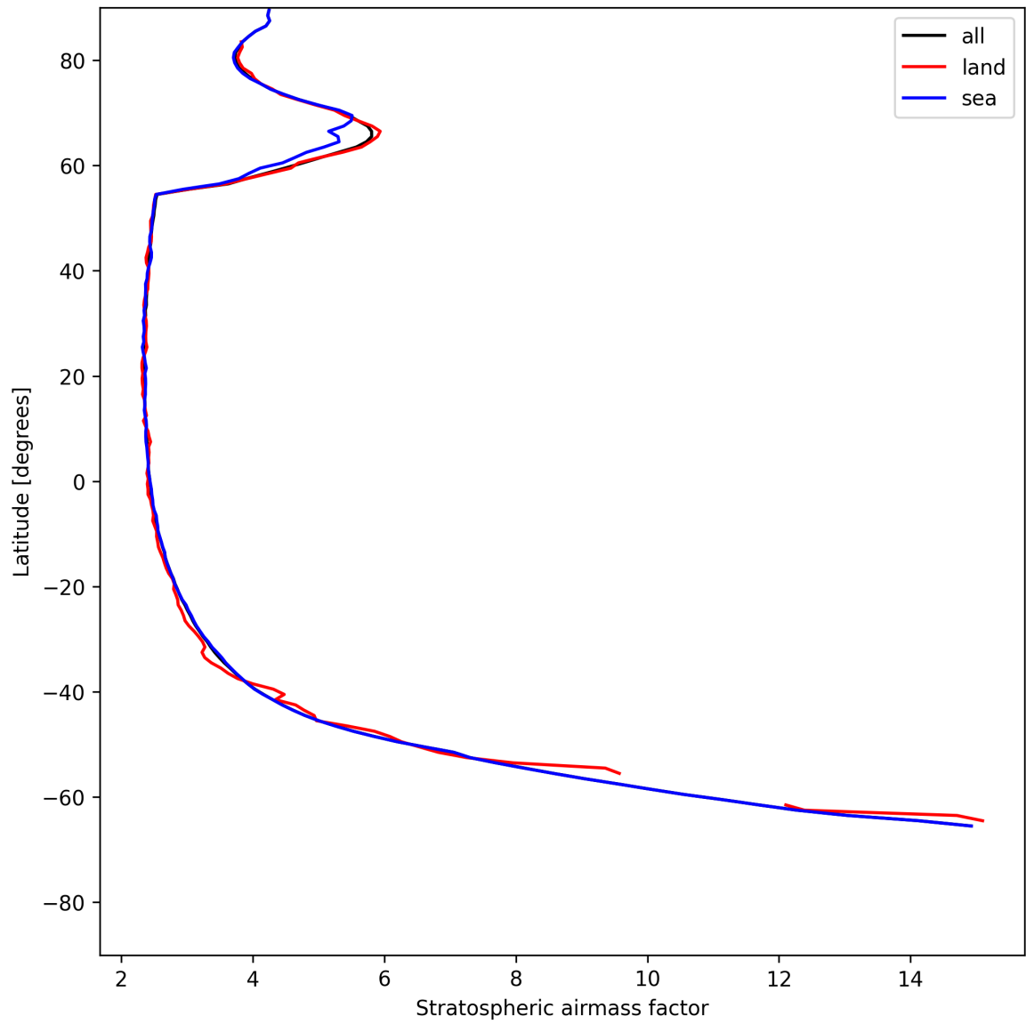
Figure 25: Zonal average of “Stratospheric air mass factor” for 2025-05-30 to 2025-05-31.
