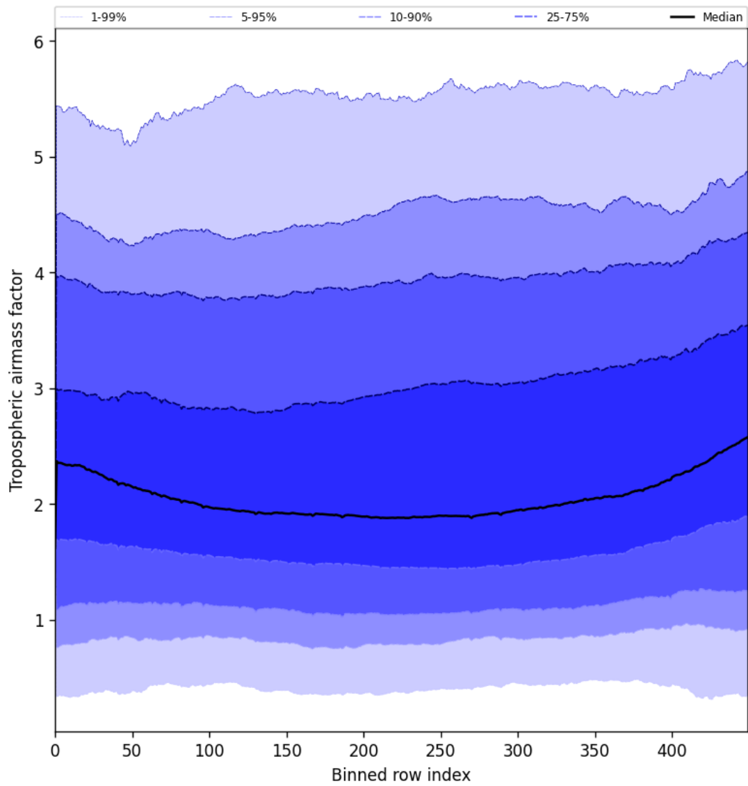
Figure 46: Along track statistics of “Tropospheric airmass factor” for 2025-05-30 to 2025-05-31
