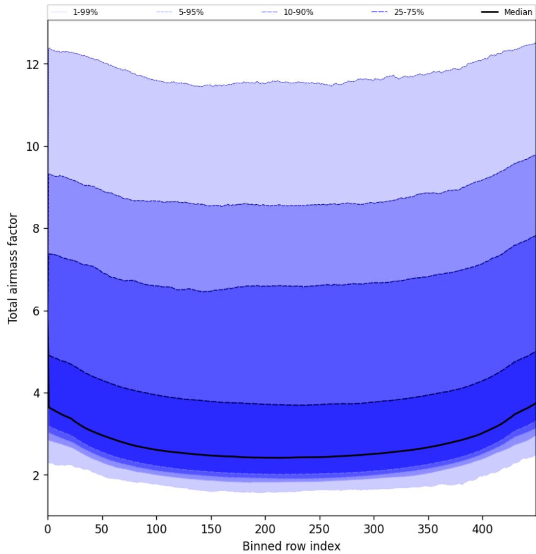
Figure 47: Along track statistics of “Total airmass factor” for 2025-05-30 to 2025-05-31
