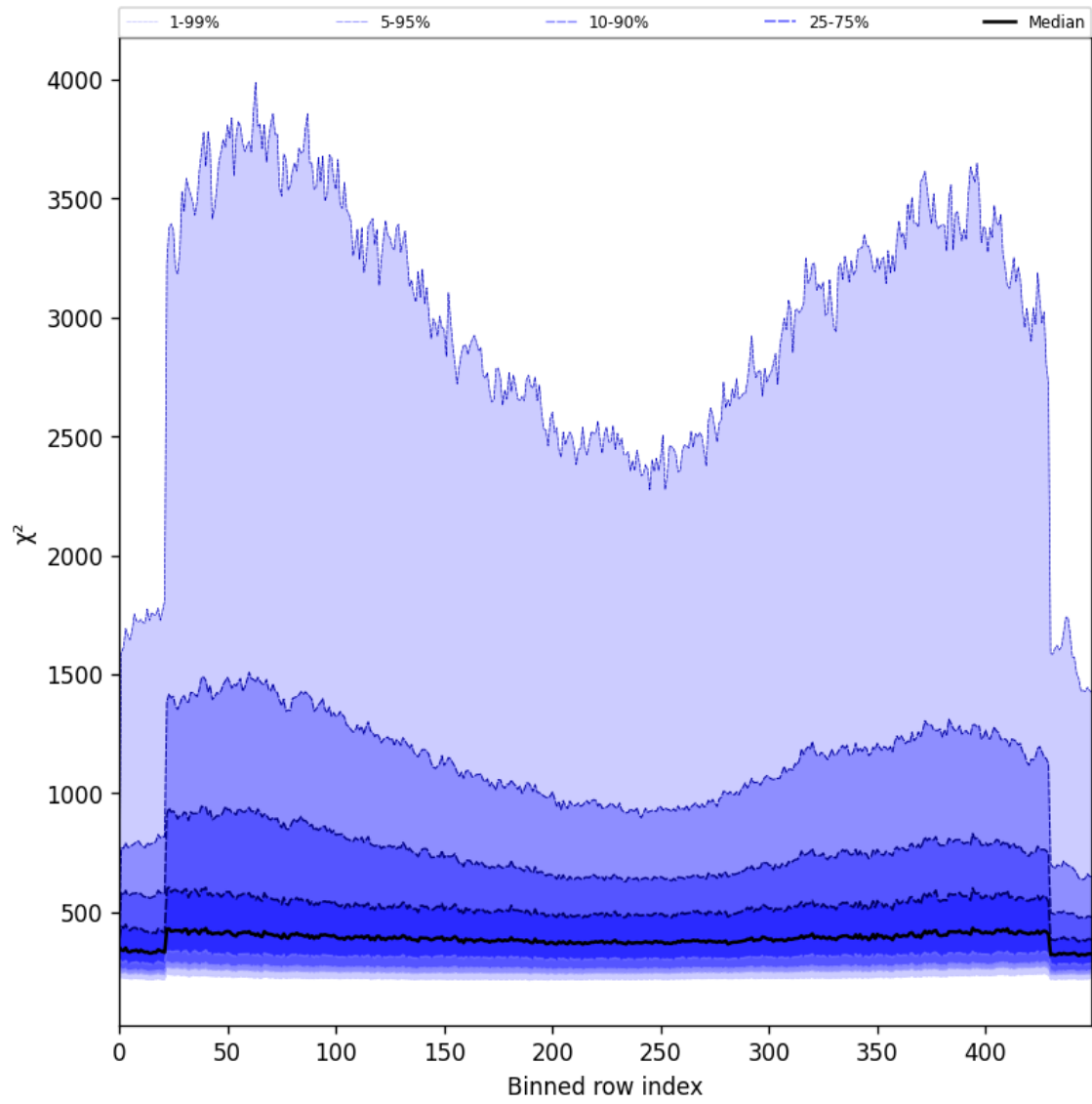
Figure 57: Along track statistics of “ \chi^2 ” for 2025-05-30 to 2025-05-31
