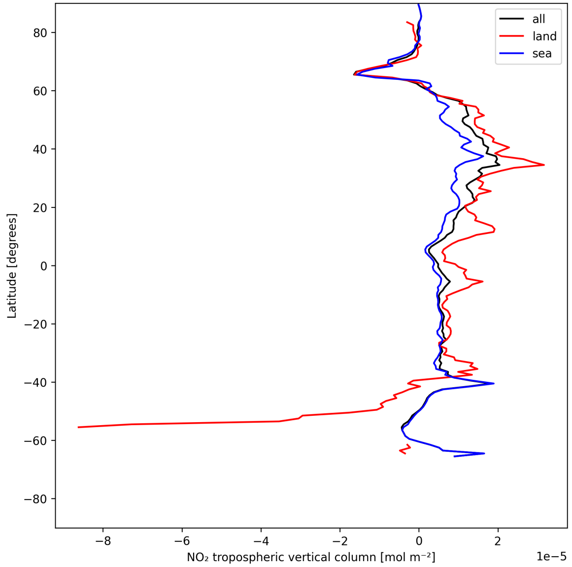
Figure 10: Zonal average of “NO 2 tropospheric vertical column” for 2025-05-30 to 2025-05-31.
