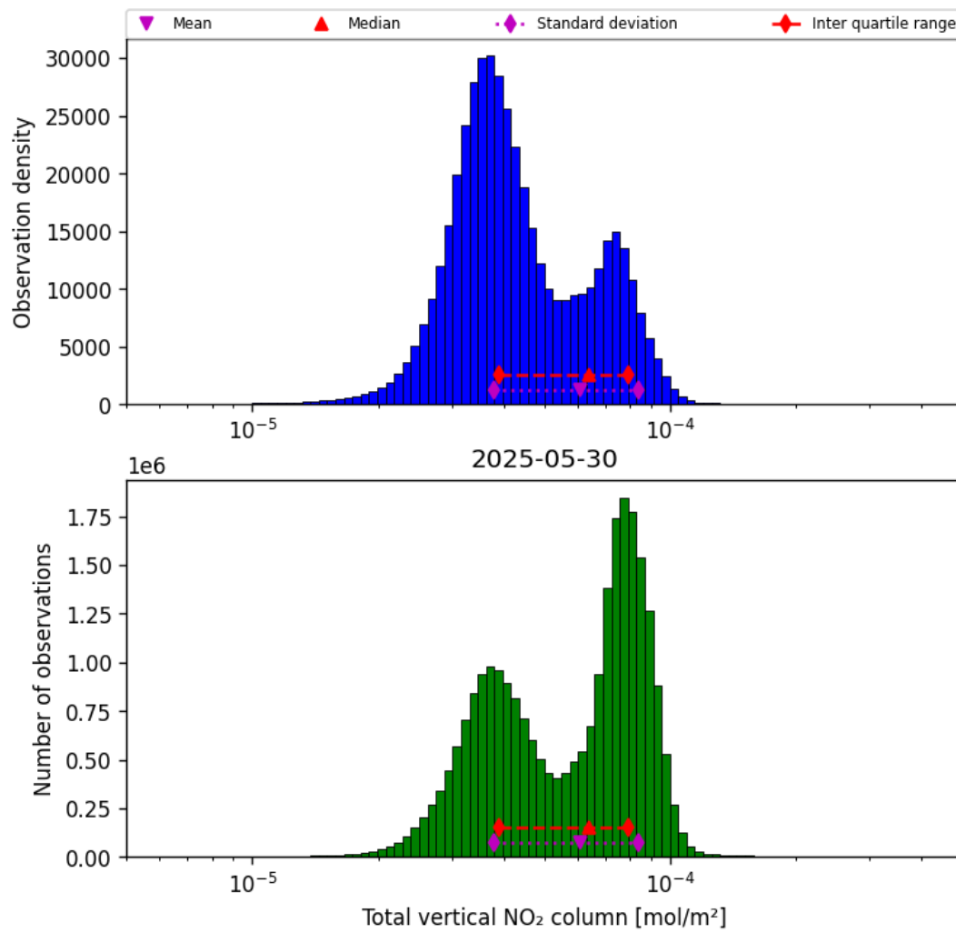
Figure 36: Histogram of “Total vertical NO 2 column” for 2025-05-30 to 2025-05-31
