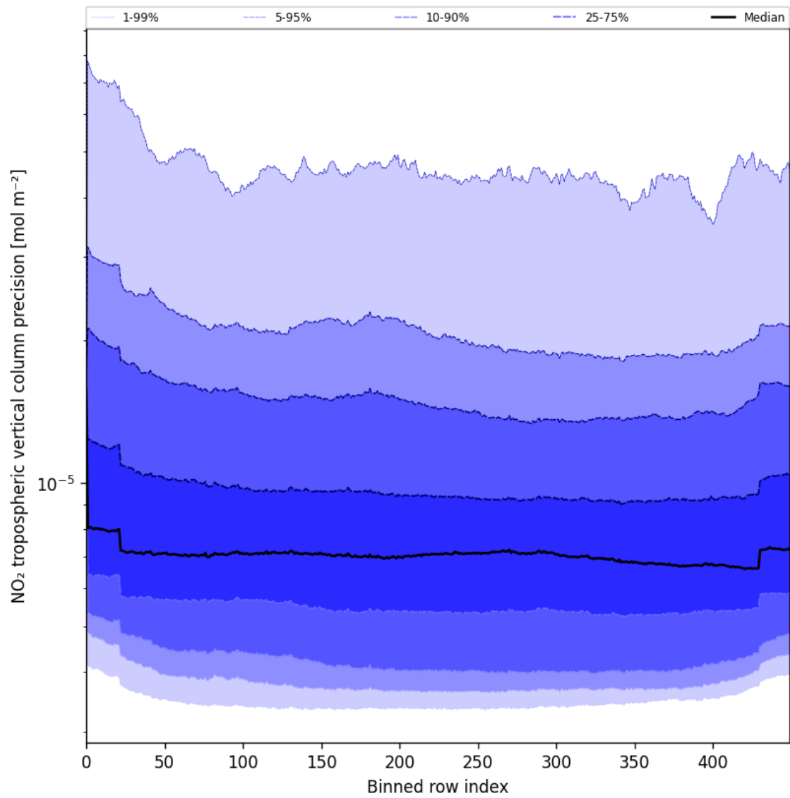
Figure 45: Along track statistics of “NO 2 tropospheric vertical column precision” for 2025-05-30 to 2025-05-31
