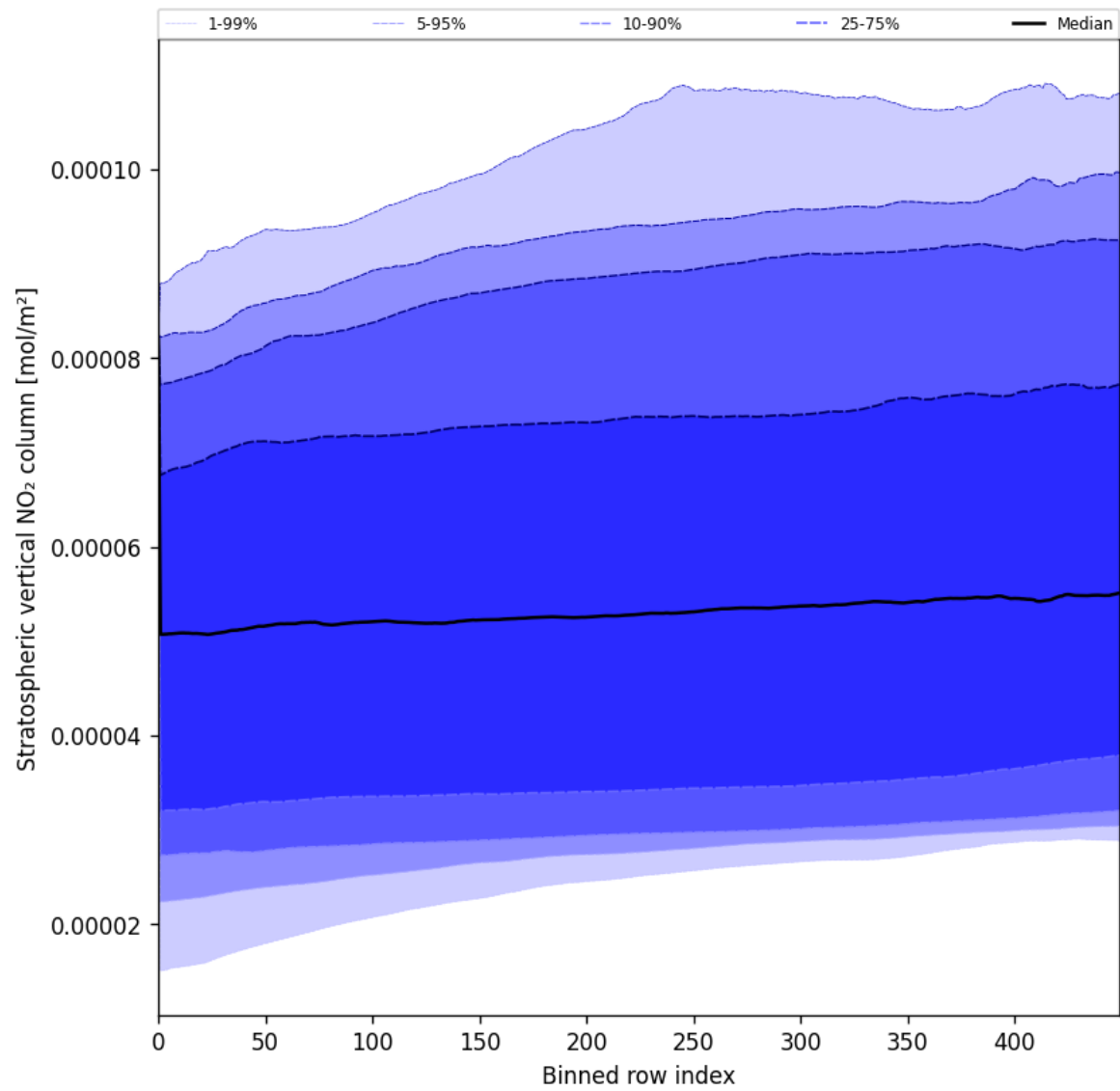
Figure 51: Along track statistics of “Stratospheric vertical NO 2 column” for 2025-05-30 to 2025-05-31
