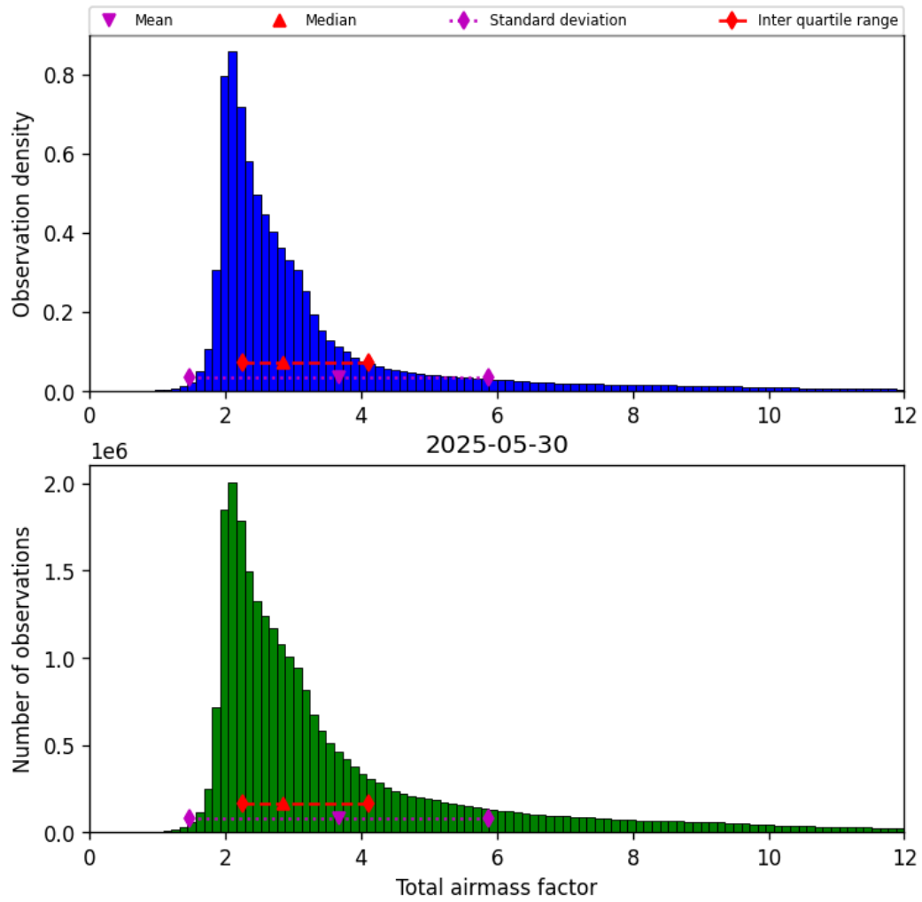
Figure 30: Histogram of “Total airmass factor” for 2025-05-30 to 2025-05-31
