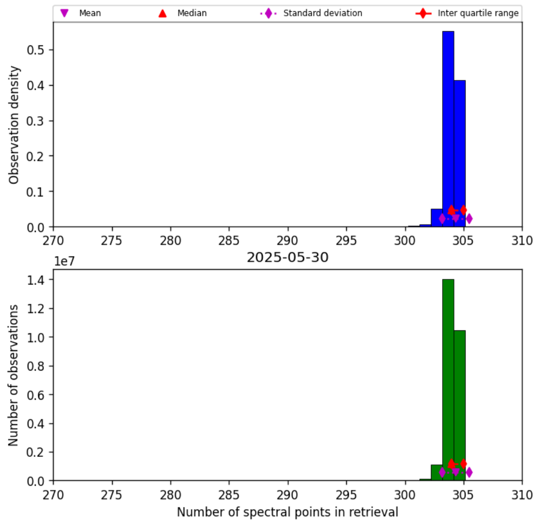
Figure 31: Histogram of “Number of spectral points in retrieval” for 2025-05-30 to 2025-05-31
