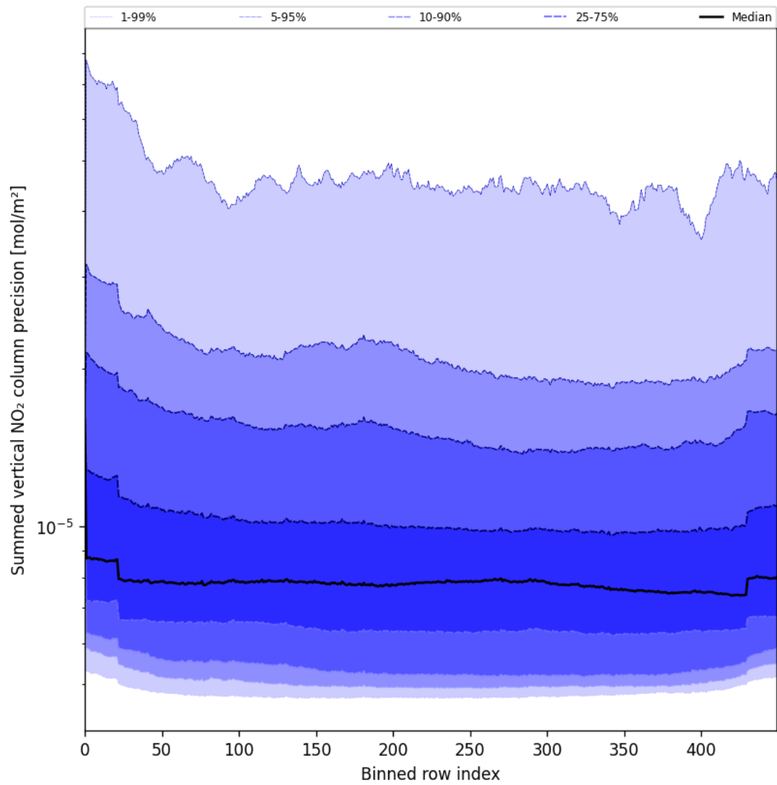
Figure 56: Along track statistics of “Summed vertical NO 2 column precision” for 2025-05-30 to 2025-05-31
