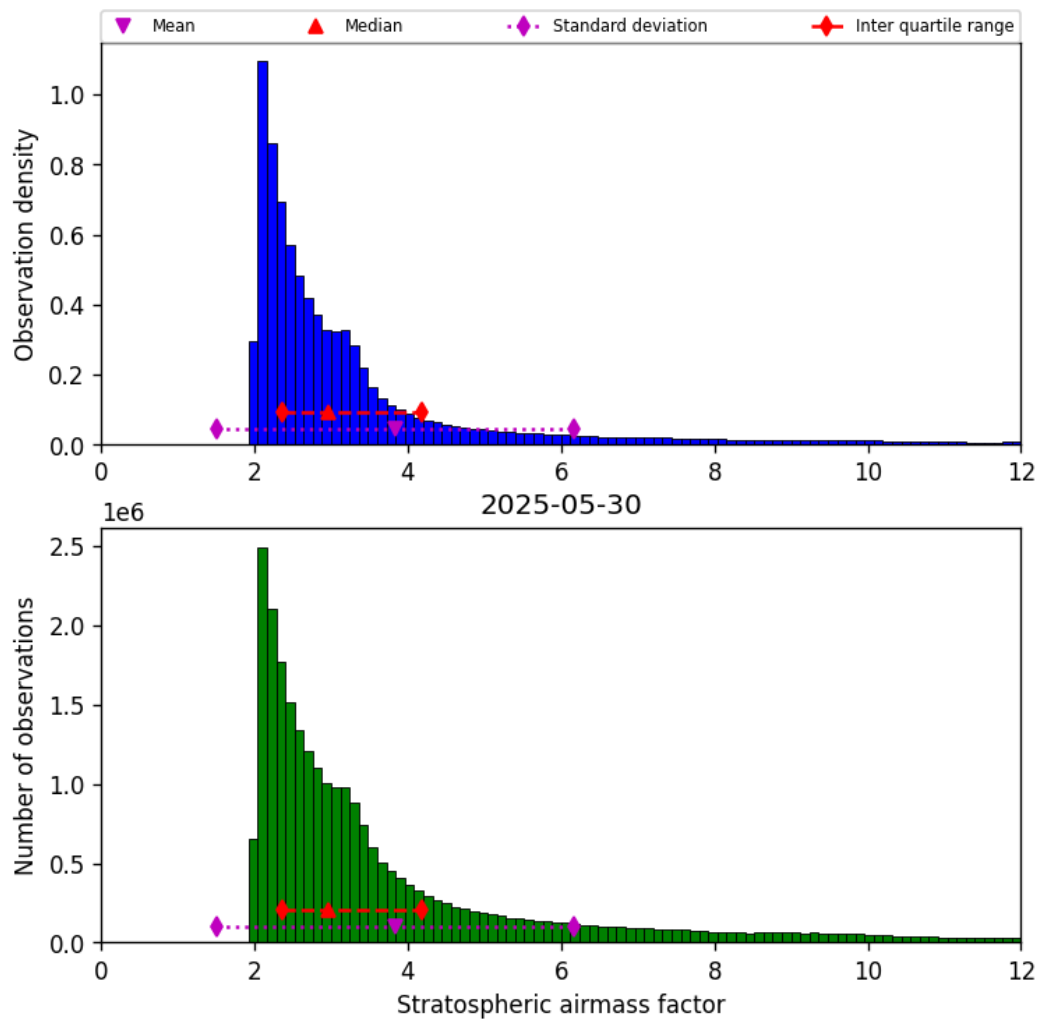
Figure 42: Histogram of “Stratospheric airmass factor” for 2025-05-30 to 2025-05-31
