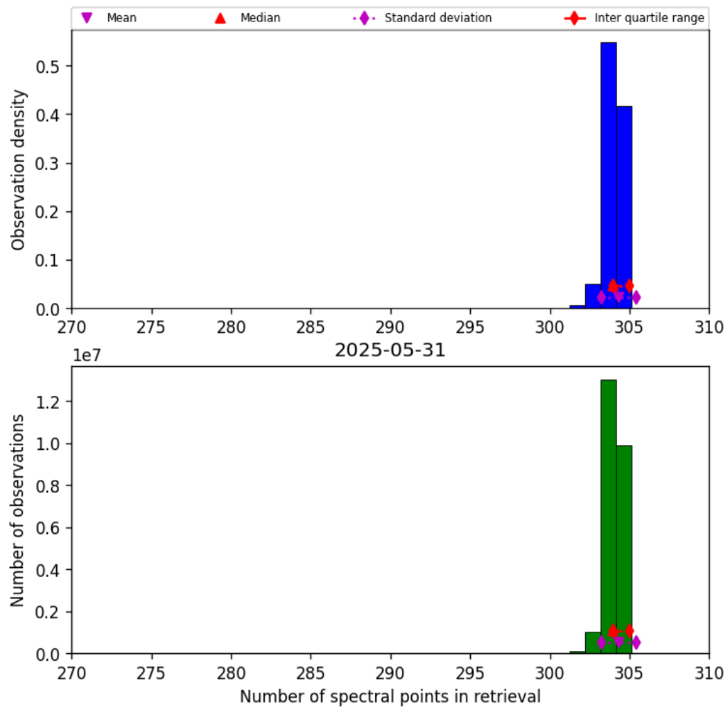
Figure 31: Histogram of “Number of spectral points in retrieval” for 2025-05-31 to 2025-06-01
