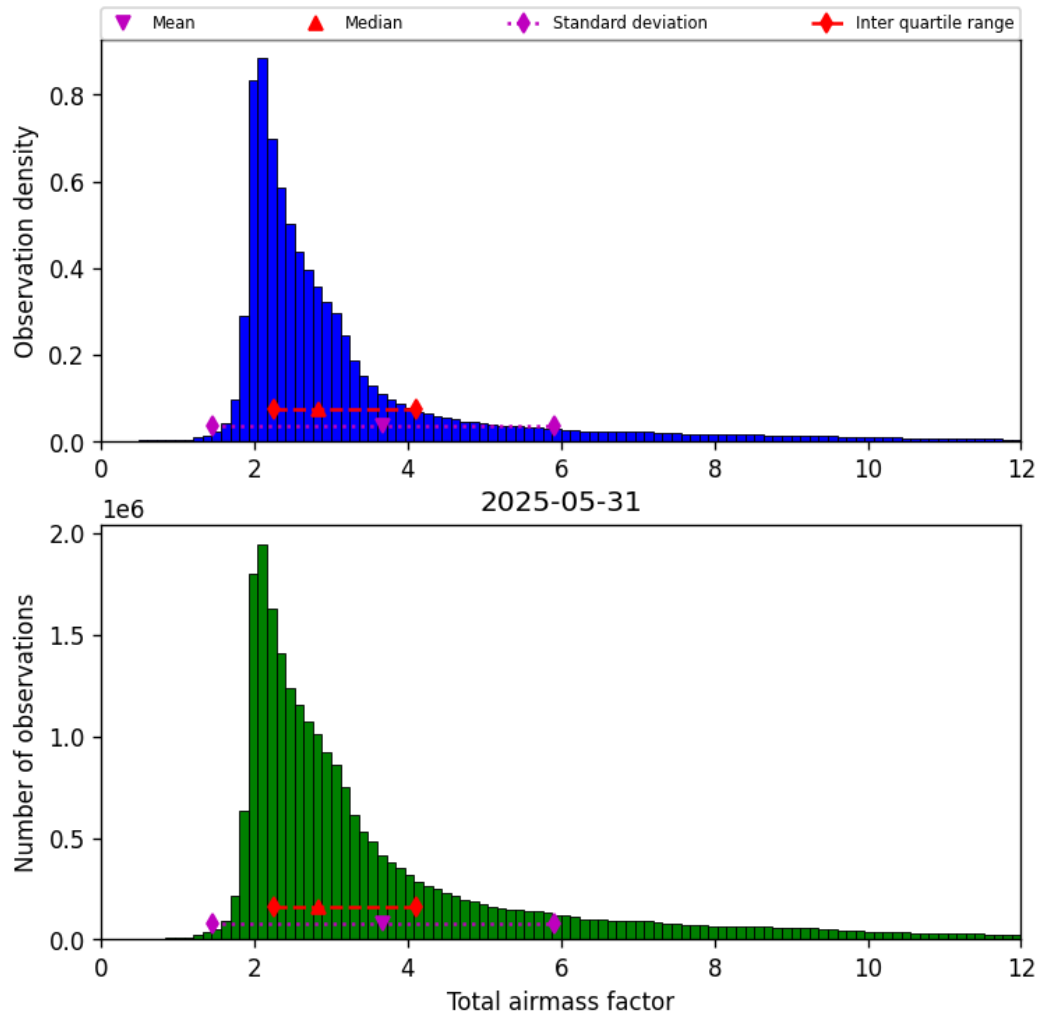
Figure 30: Histogram of “Total airmass factor” for 2025-05-31 to 2025-06-01
