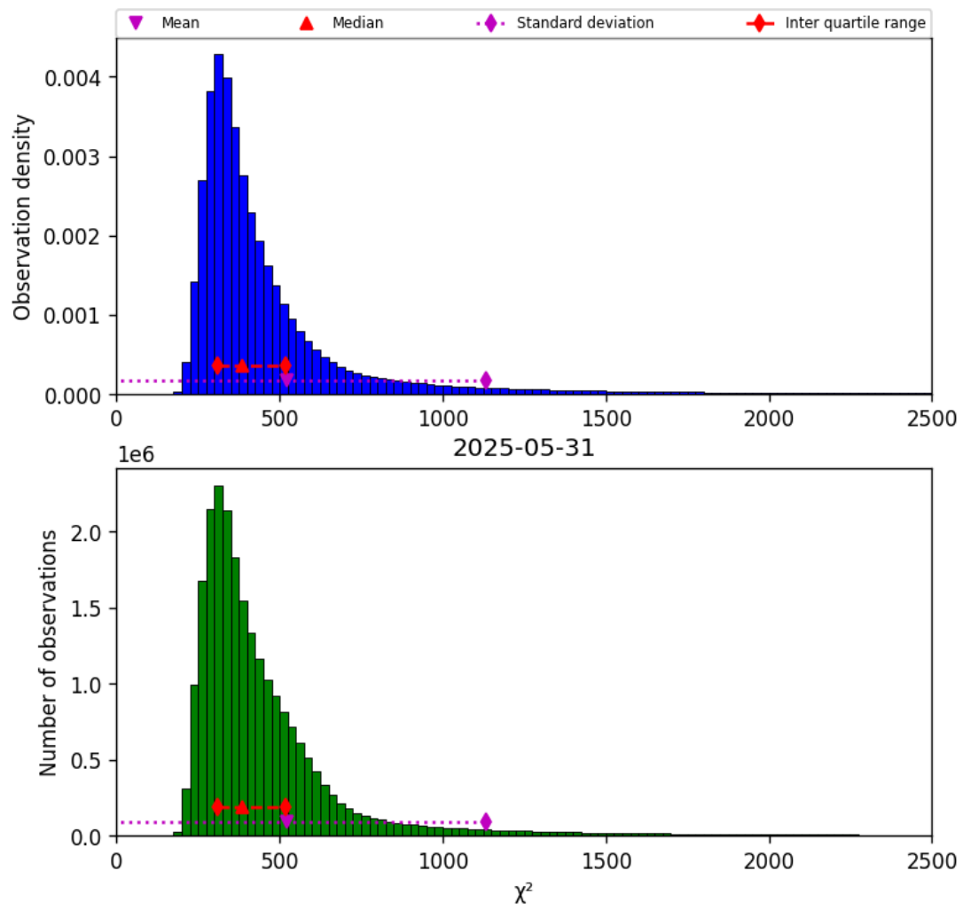
Figure 40: Histogram of “ \chi^2 ” for 2025-05-31 to 2025-06-01
