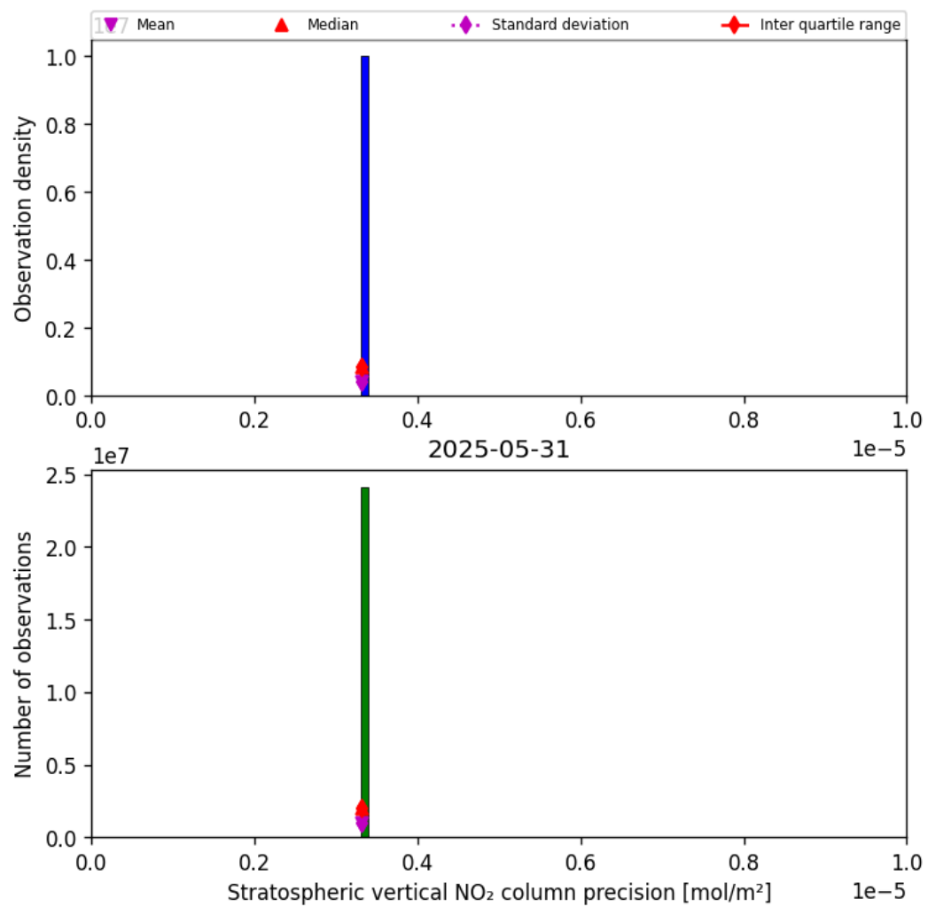
Figure 35: Histogram of “Stratospheric vertical NO 2 column precision” for 2025-05-31 to 2025-06-01
