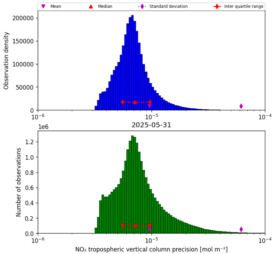
Figure 28: Histogram of “NO 2 tropospheric vertical column precision” for 2025-05-31 to 2025-06-01
