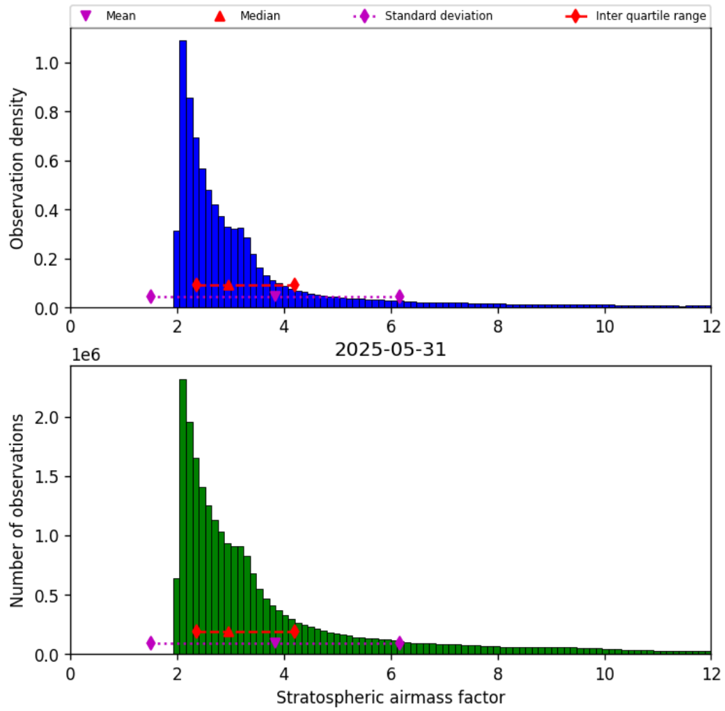
Figure 42: Histogram of “Stratospheric airmass factor” for 2025-05-31 to 2025-06-01
