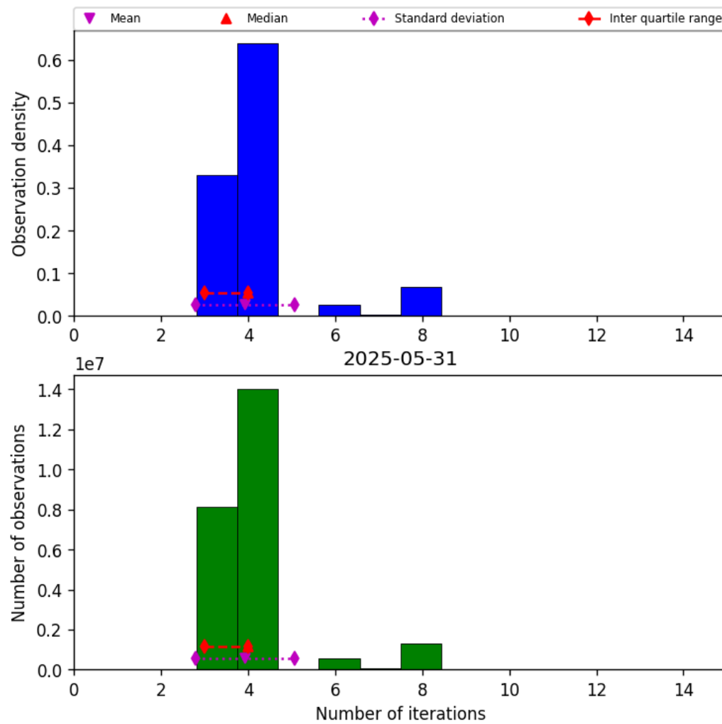
Figure 32: Histogram of “Number of iterations” for 2025-05-31 to 2025-06-01
