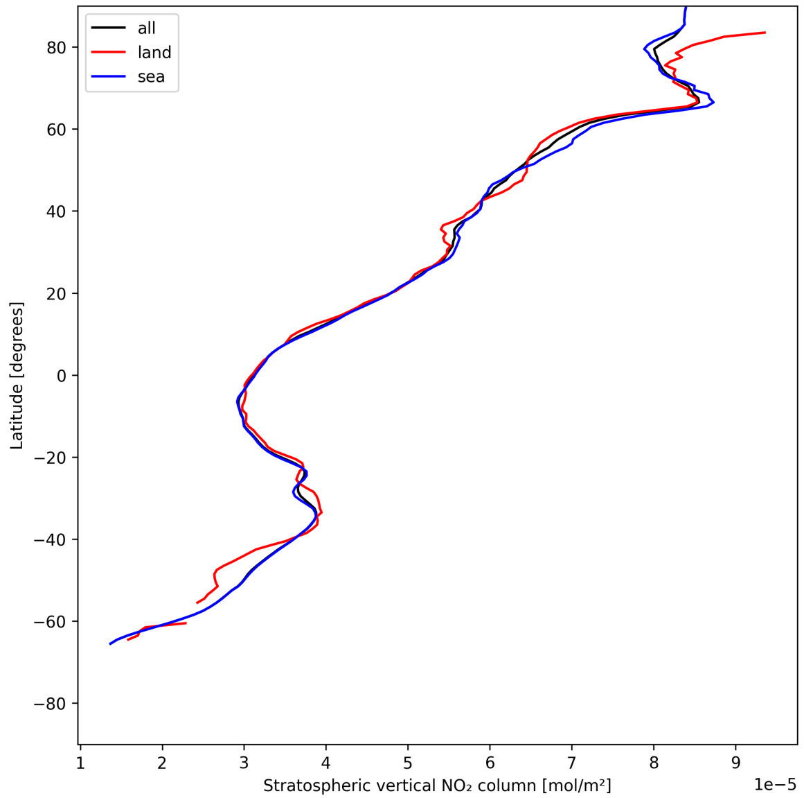
Figure 17: Zonal average of “Stratospheric vertical NO 2 column” for 2025-05-31 to 2025-06-01.
