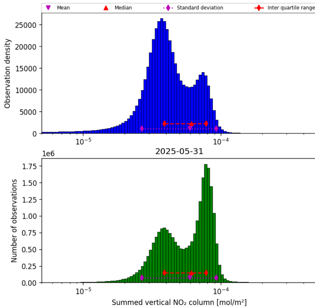
Figure 38: Histogram of “Summed vertical NO 2 column” for 2025-05-31 to 2025-06-01
