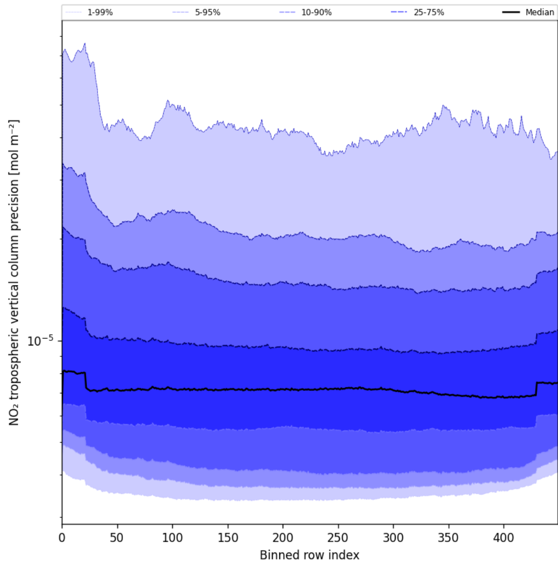
Figure 45: Along track statistics of “NO 2 tropospheric vertical column precision” for 2025-05-31 to 2025-06-01
