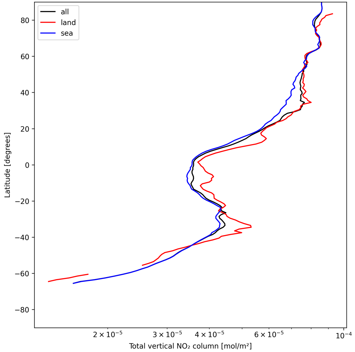
Figure 19: Zonal average of “Total vertical NO 2 column” for 2025-05-31 to 2025-06-01.
