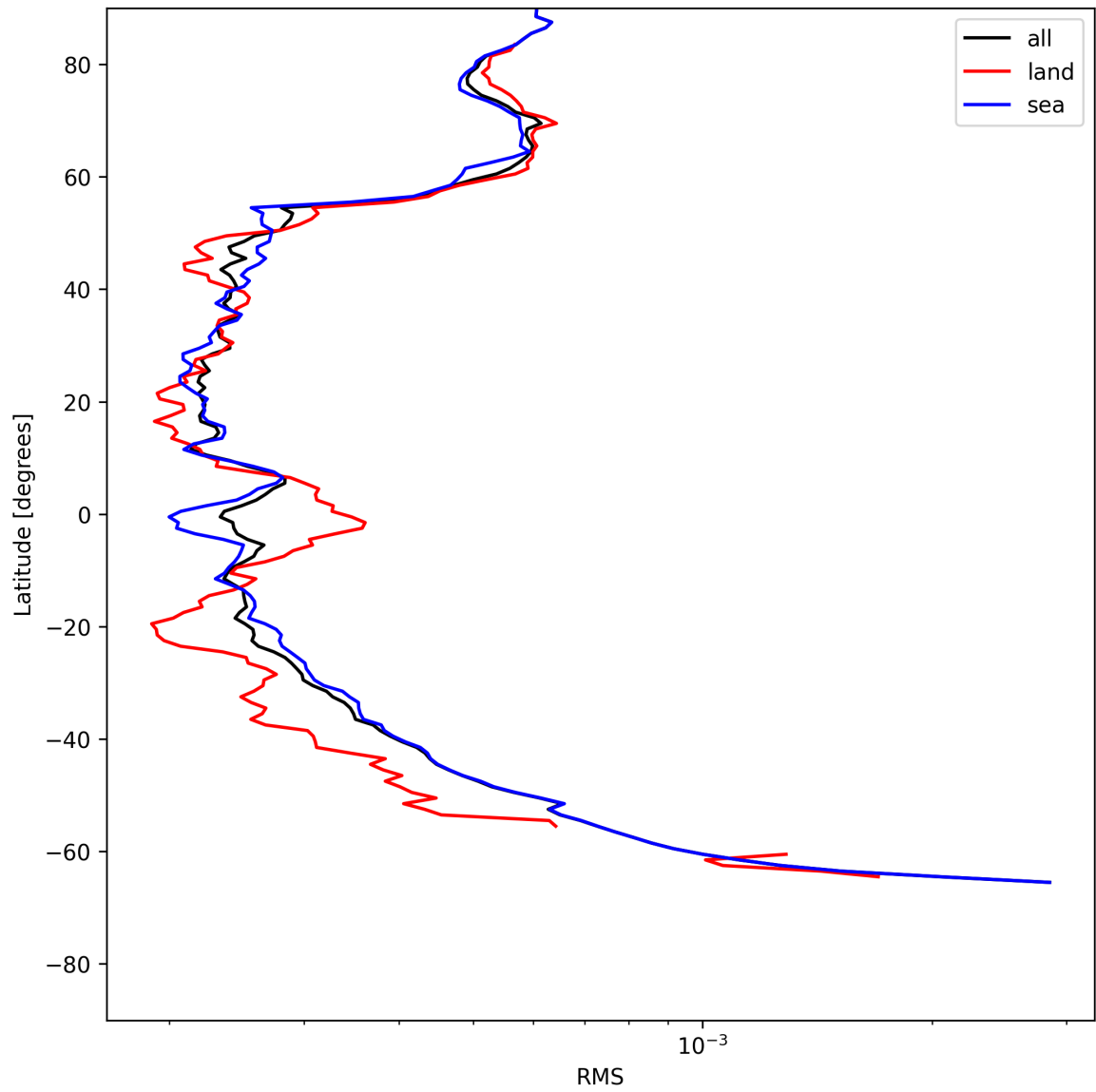
Figure 24: Zonal average of “RMS” for 2025-05-31 to 2025-06-01.
