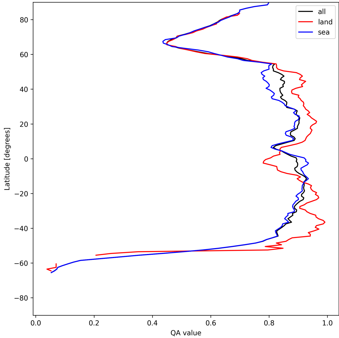
Figure 9: Zonal average of “QA value” for 2025-05-31 to 2025-06-01.
