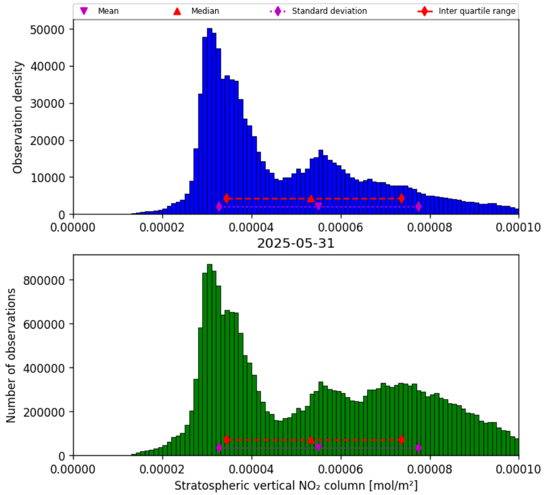
Figure 34: Histogram of “Stratospheric vertical NO 2 column” for 2025-05-31 to 2025-06-01
