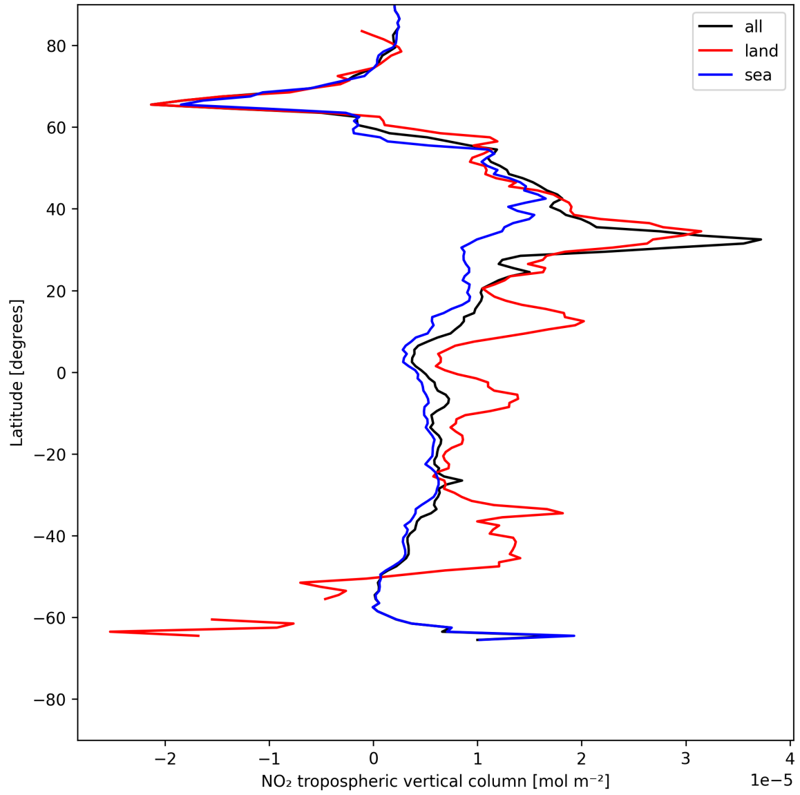
Figure 10: Zonal average of “NO 2 tropospheric vertical column” for 2025-05-31 to 2025-06-01.
