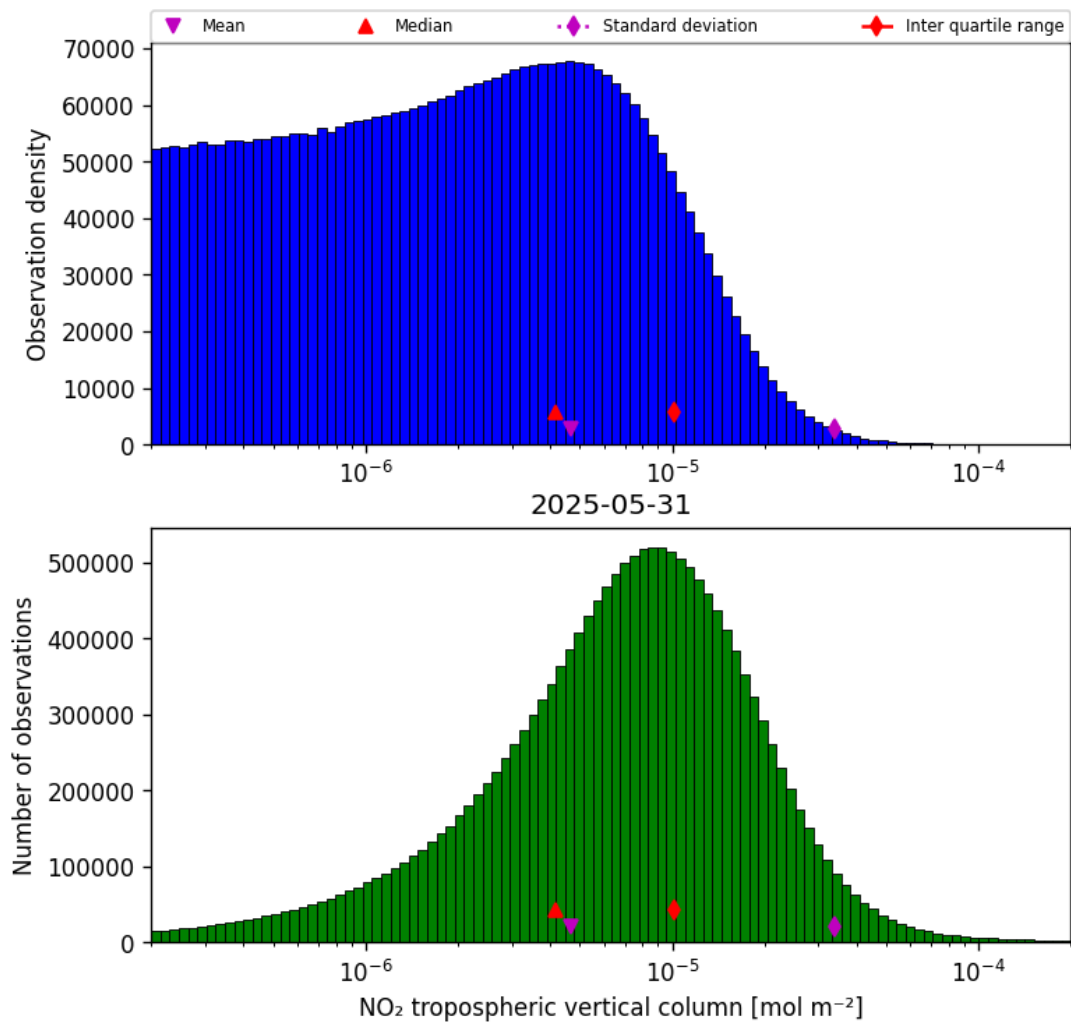
Figure 27: Histogram of “NO 2 tropospheric vertical column” for 2025-05-31 to 2025-06-01
