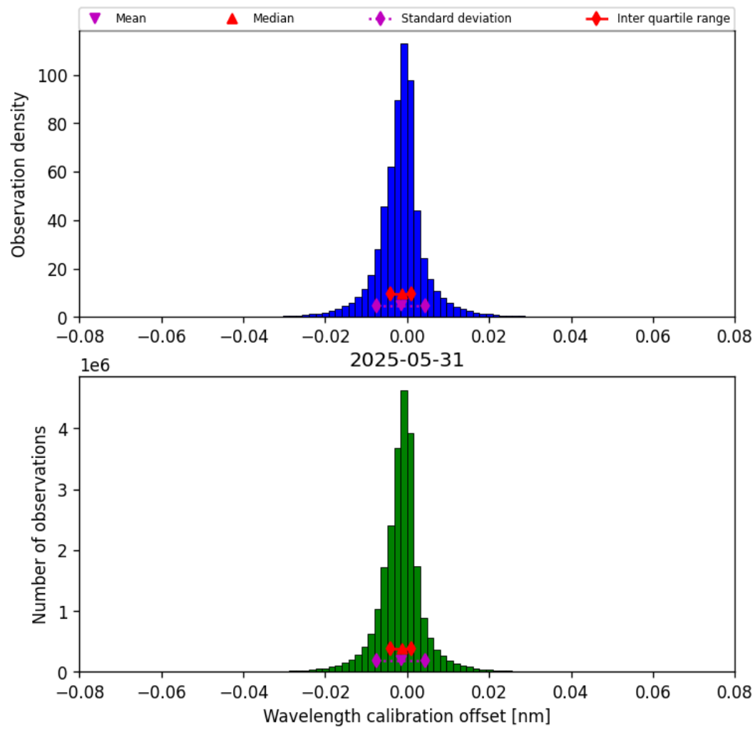
Figure 33: Histogram of “Wavelength calibration offset” for 2025-05-31 to 2025-06-01
