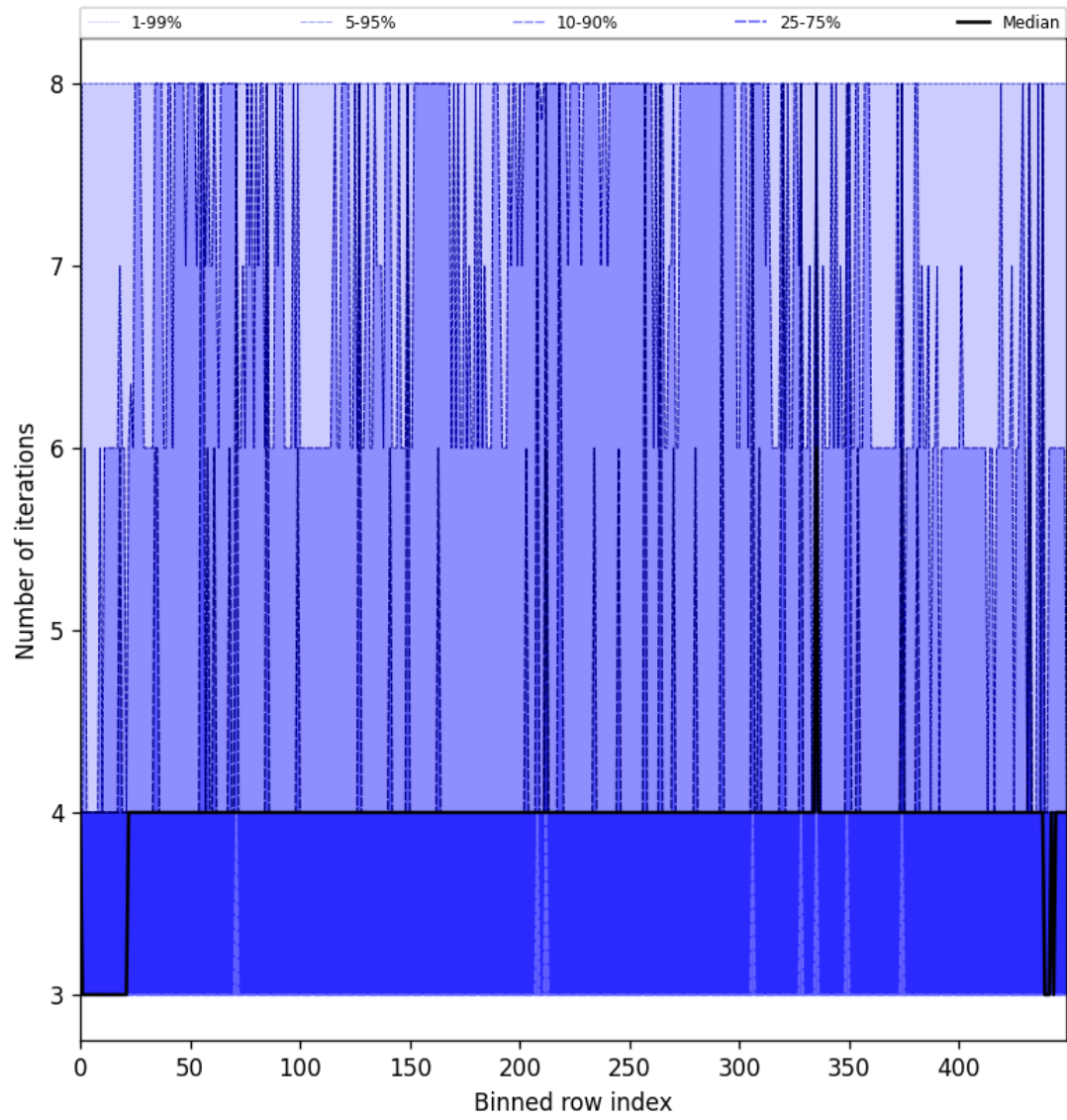
Figure 49: Along track statistics of “Number of iterations” for 2025-05-31 to 2025-06-01
