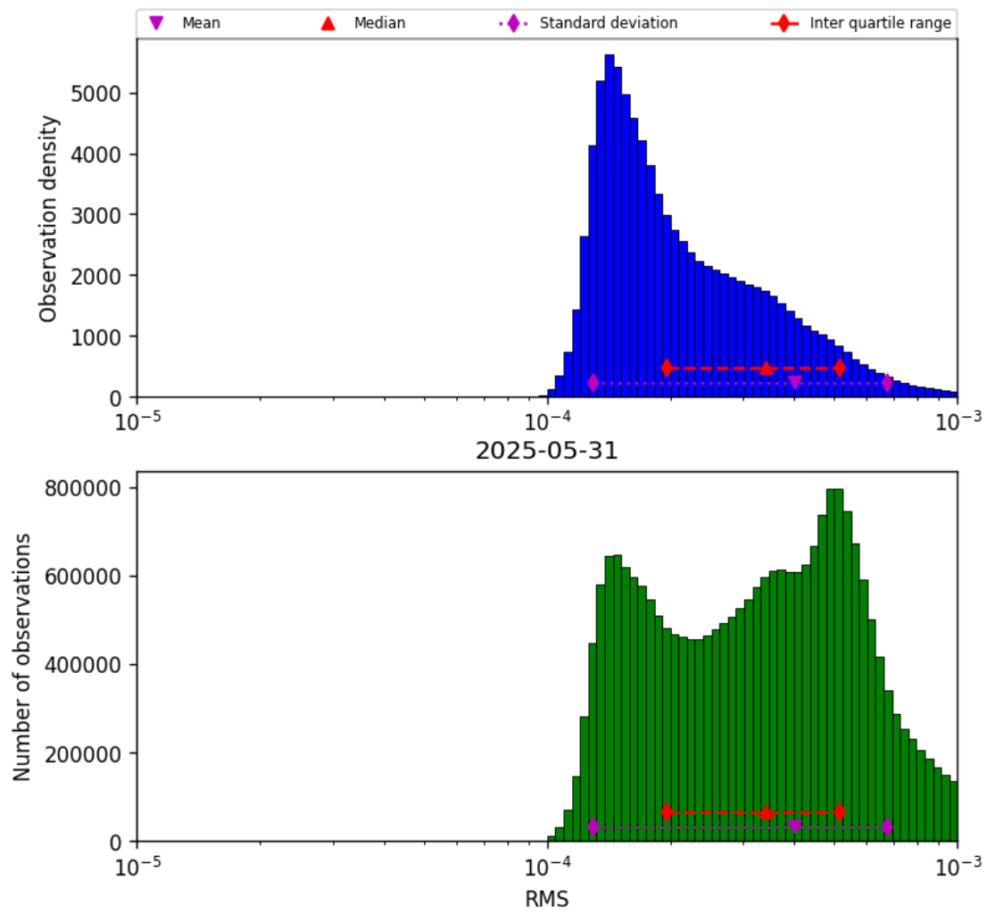
Figure 41: Histogram of “RMS” for 2025-05-31 to 2025-06-01
