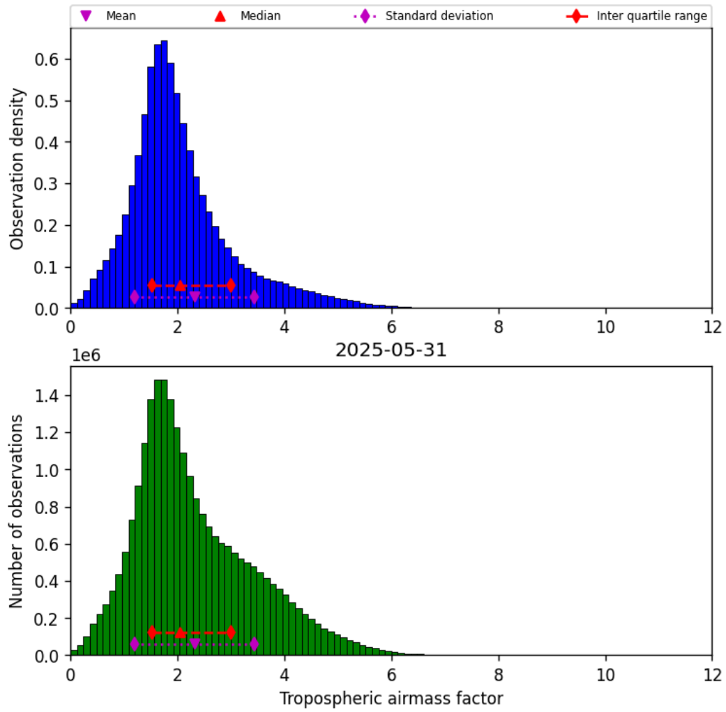
Figure 29: Histogram of “Tropospheric airmass factor” for 2025-05-31 to 2025-06-01
