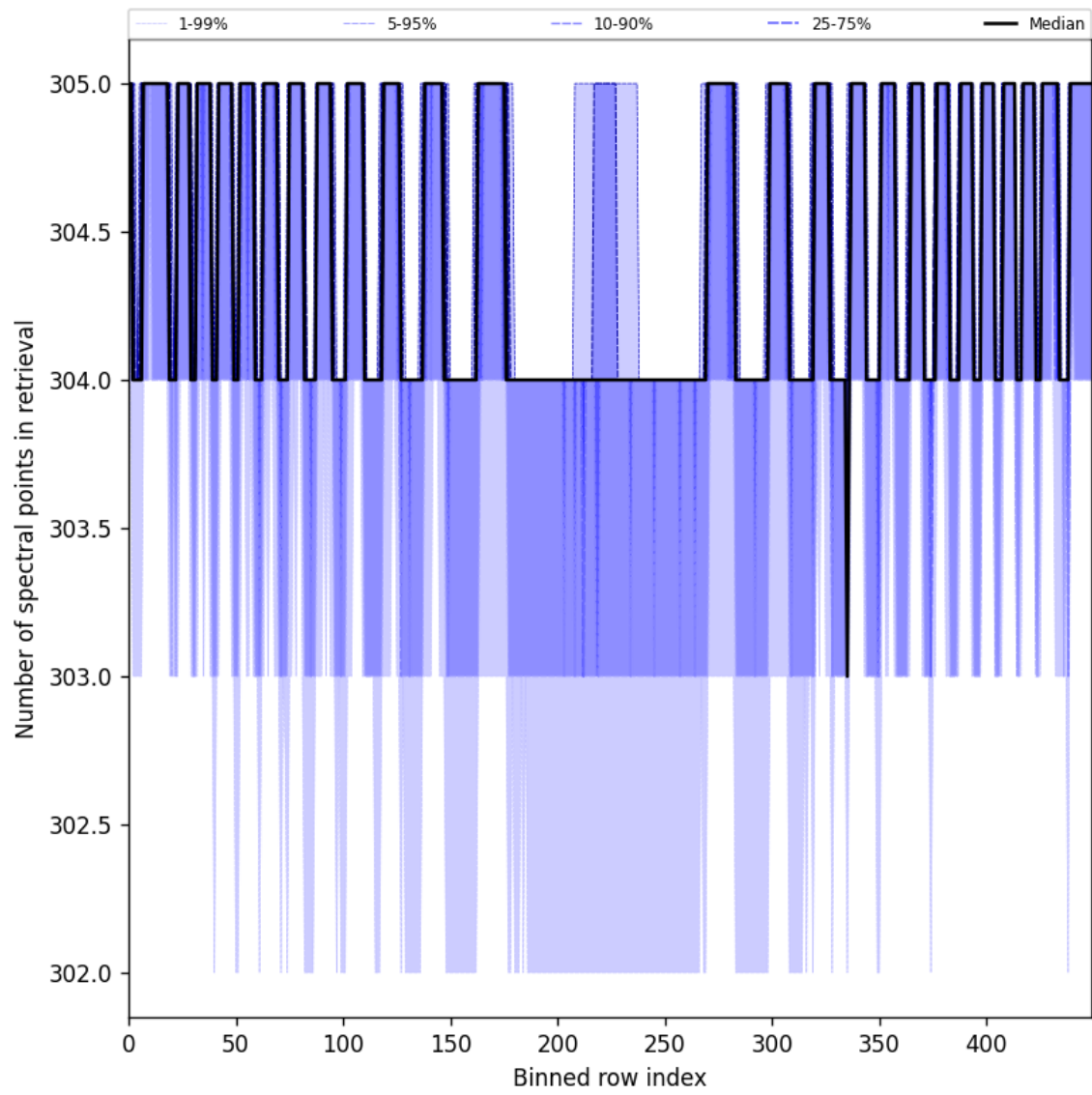
Figure 48: Along track statistics of “Number of spectral points in retrieval” for 2025-05-31 to 2025-06-01
