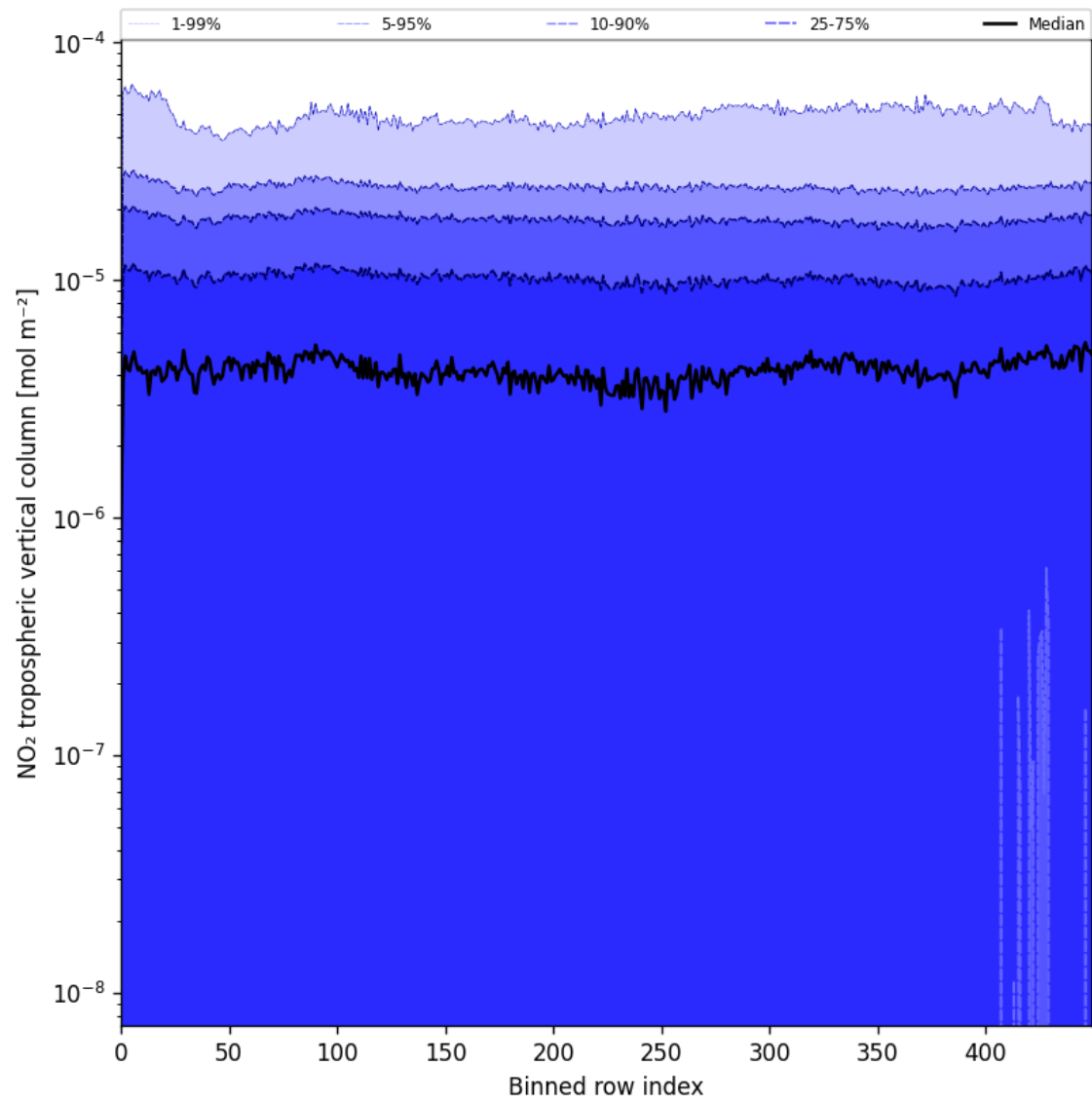
Figure 44: Along track statistics of “NO 2 tropospheric vertical column” for 2025-05-31 to 2025-06-01
