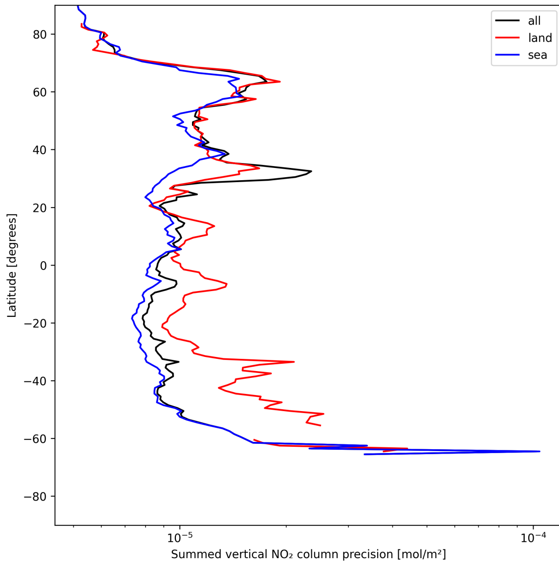
Figure 22: Zonal average of “Summed vertical NO 2 column precision” for 2025-05-31 to 2025-06-01.
