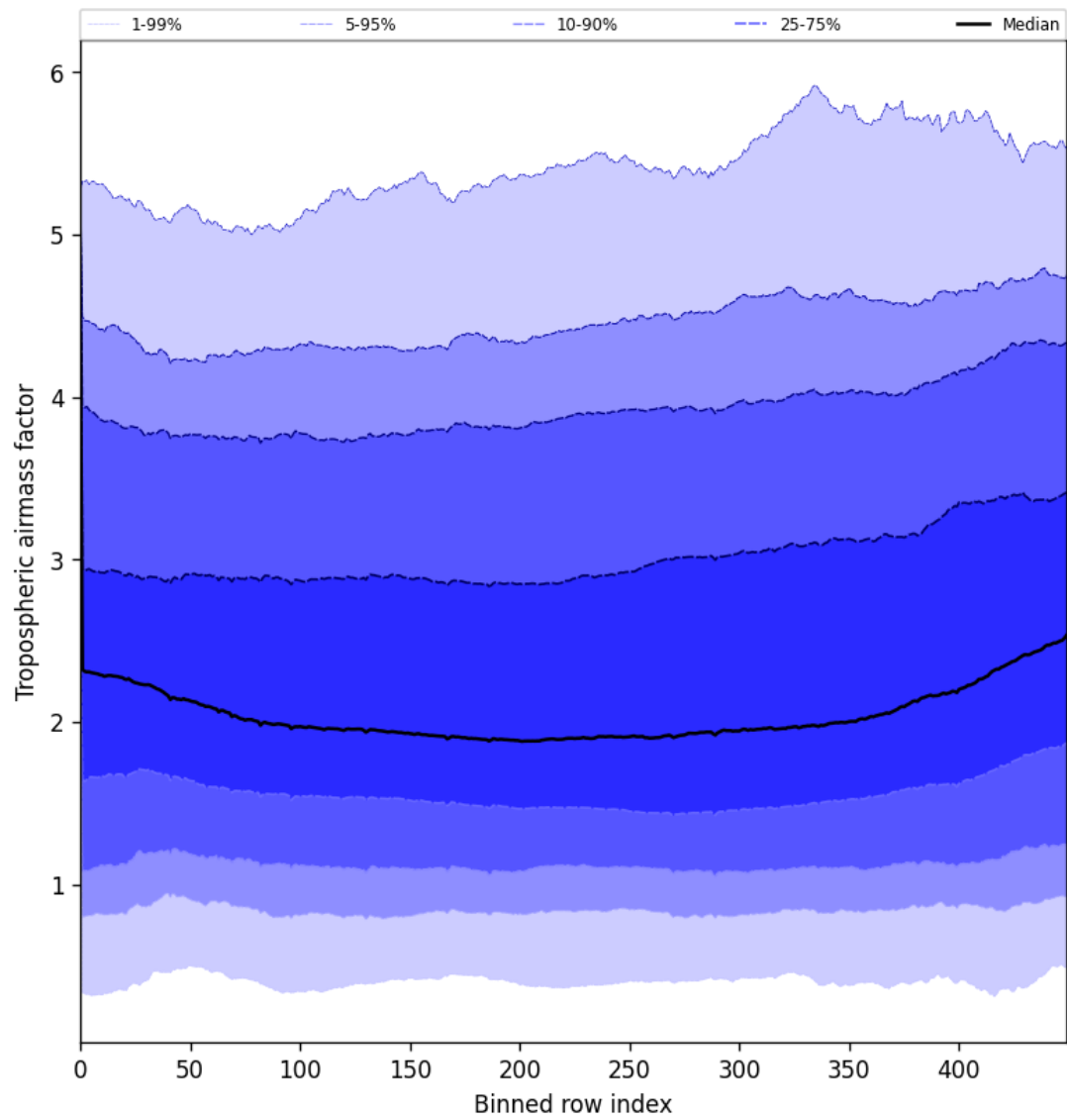
Figure 46: Along track statistics of “Tropospheric airmass factor” for 2025-05-31 to 2025-06-01
