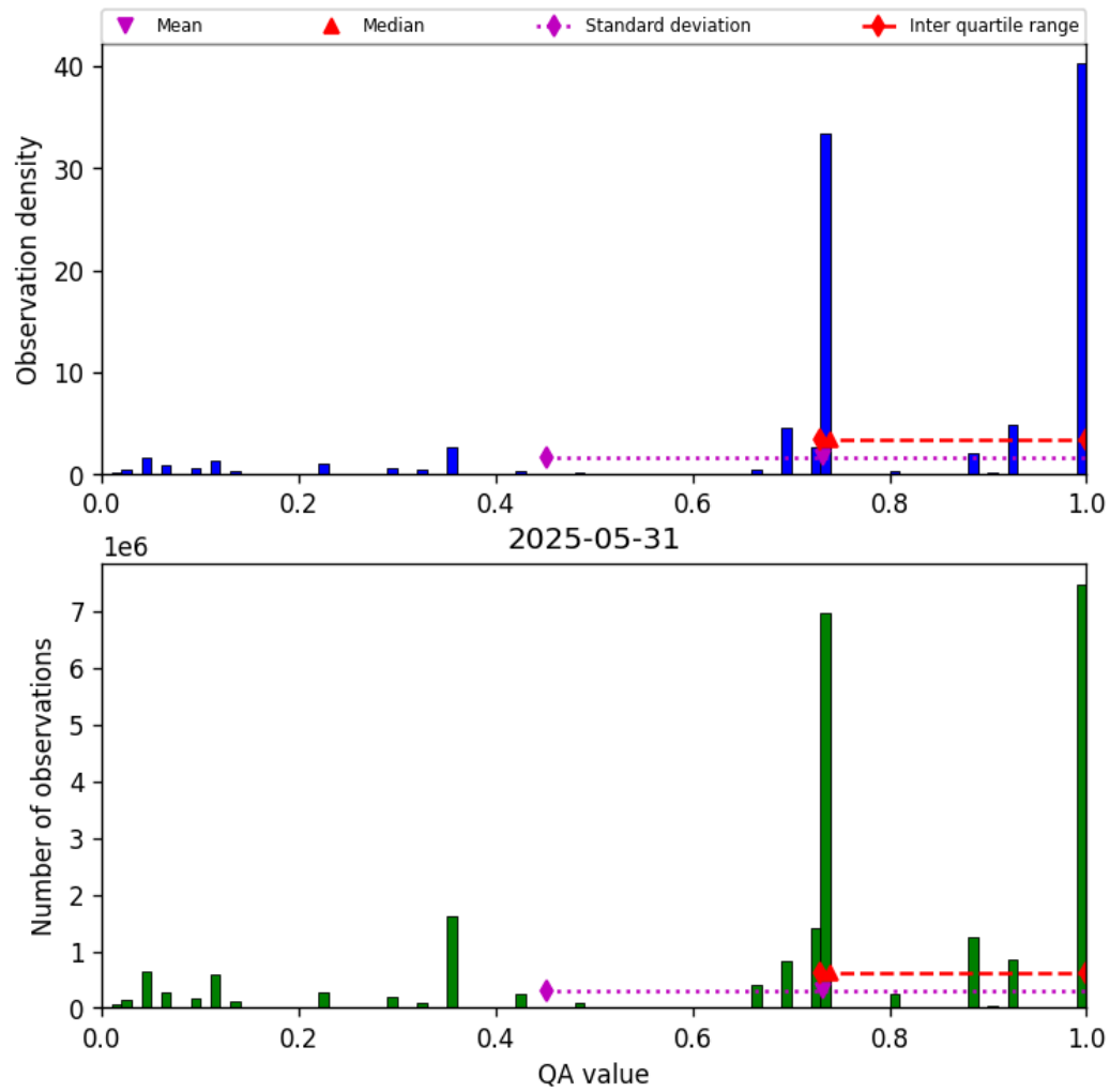
Figure 26: Histogram of “QA value” for 2025-05-31 to 2025-06-01
