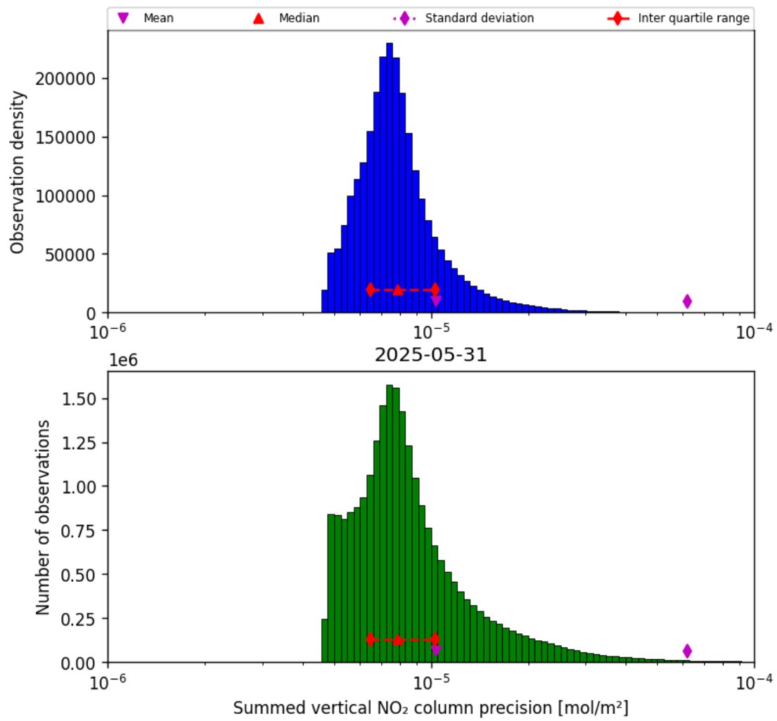
Figure 39: Histogram of “Summed vertical NO 2 column precision” for 2025-05-31 to 2025-06-01
