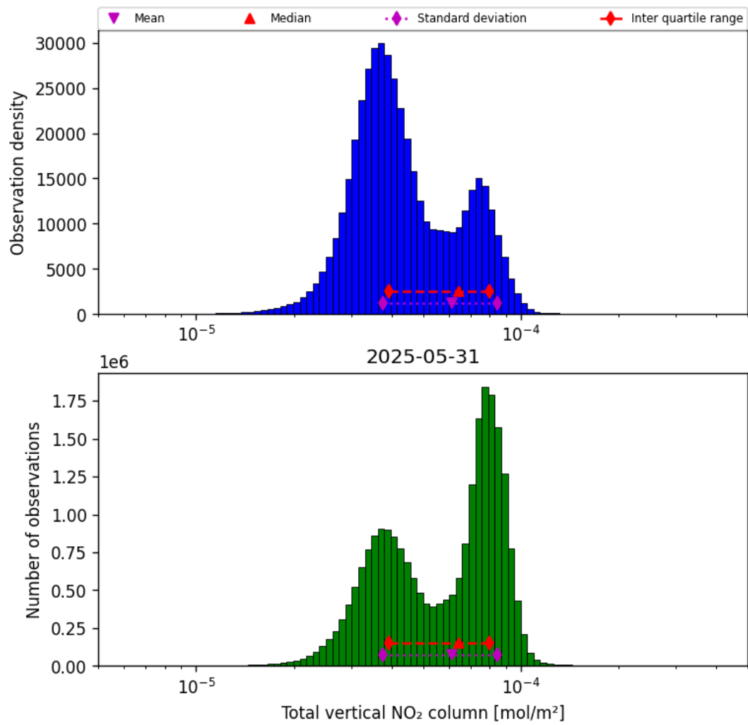
Figure 36: Histogram of “Total vertical NO 2 column” for 2025-05-31 to 2025-06-01
