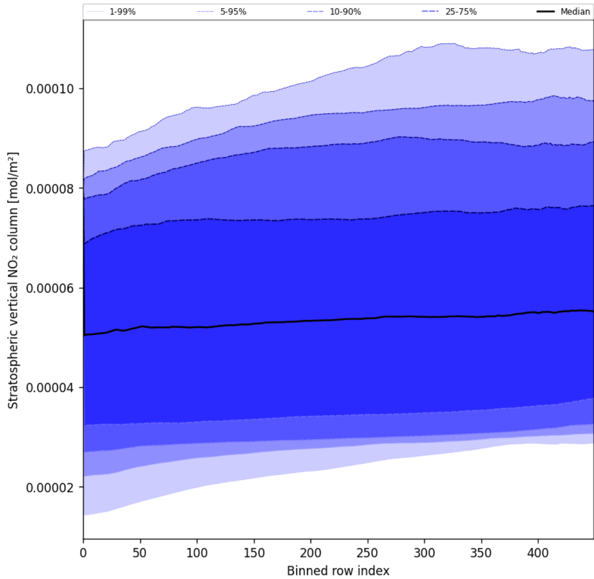
Figure 51: Along track statistics of “Stratospheric vertical NO 2 column” for 2025-05-31 to 2025-06-01
