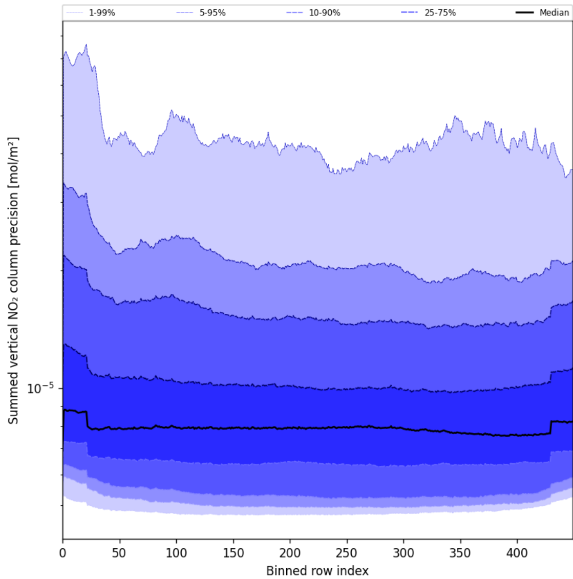
Figure 56: Along track statistics of “Summed vertical NO 2 column precision” for 2025-05-31 to 2025-06-01
