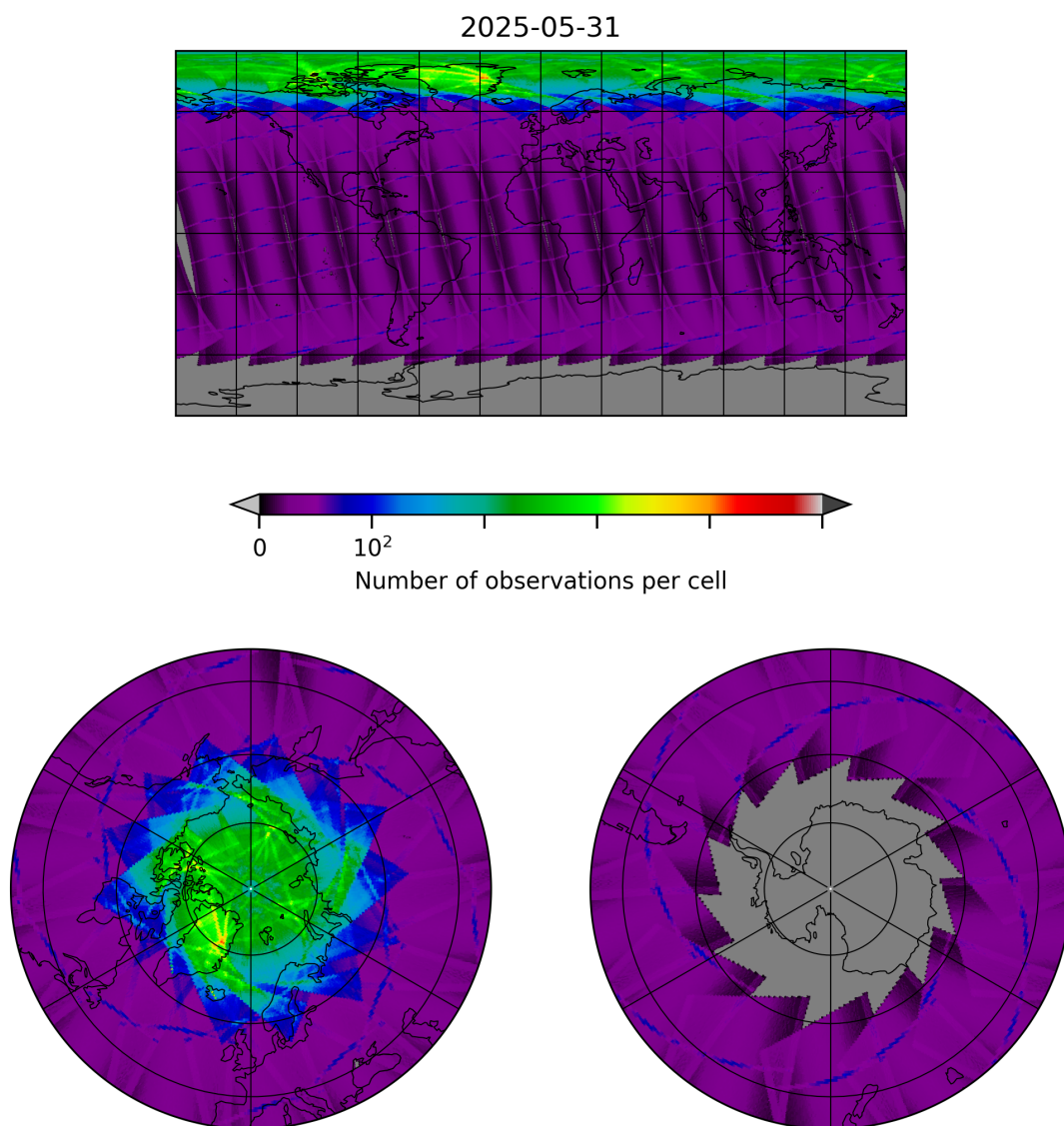
Figure 8: Map of the number of observations for 2025-05-31 to 2025-06-01
