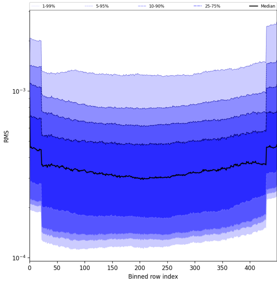
Figure 58: Along track statistics of “RMS” for 2025-05-31 to 2025-06-01
