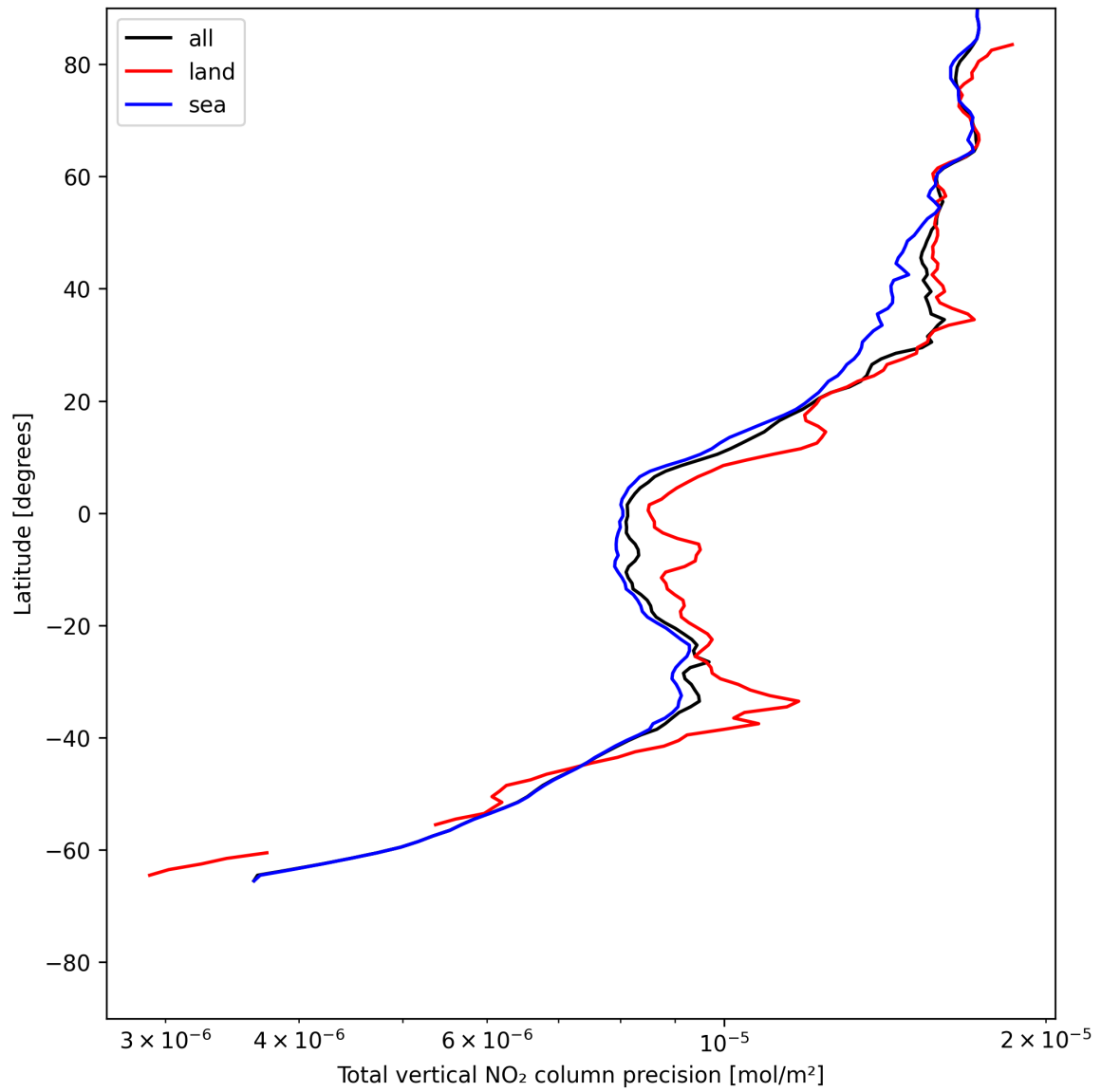
Figure 20: Zonal average of “Total vertical NO 2 column precision” for 2025-05-31 to 2025-06-01.
