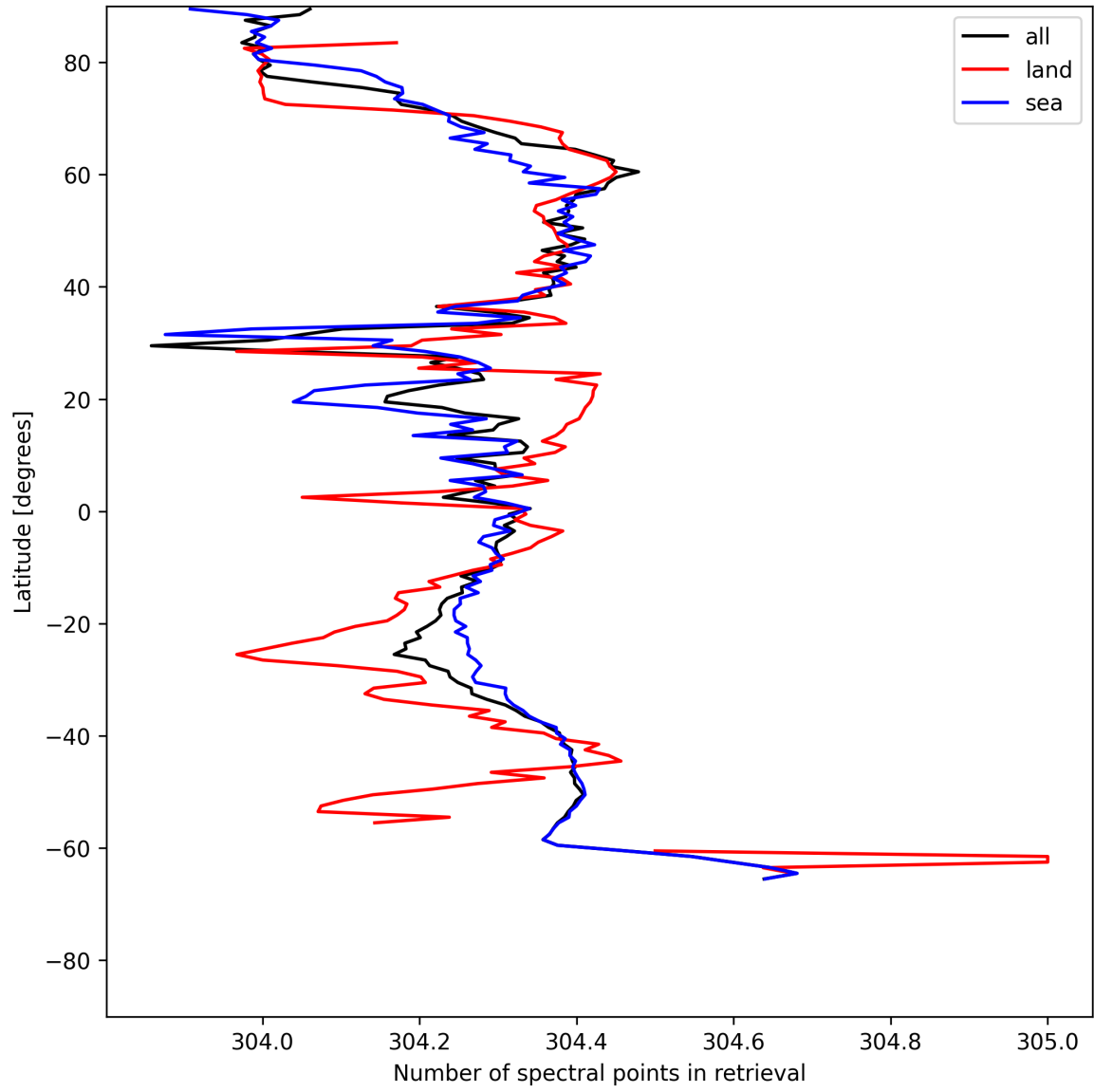
Figure 14: Zonal average of “Number of spectral points in retrieval” for 2025-05-31 to 2025-06-01.
