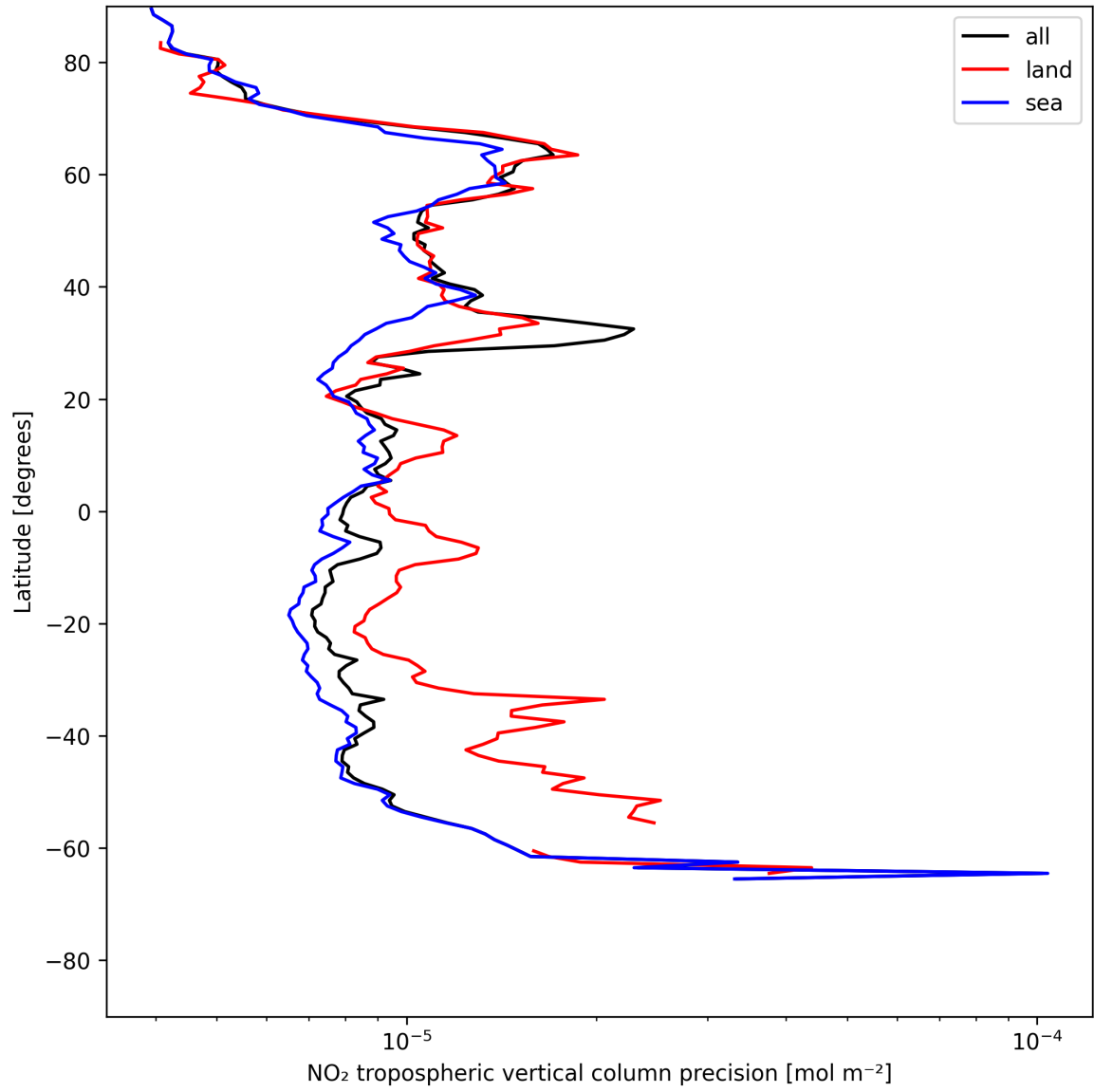
Figure 11: Zonal average of “NO 2 tropospheric vertical column precision” for 2025-05-31 to 2025-06-01.
