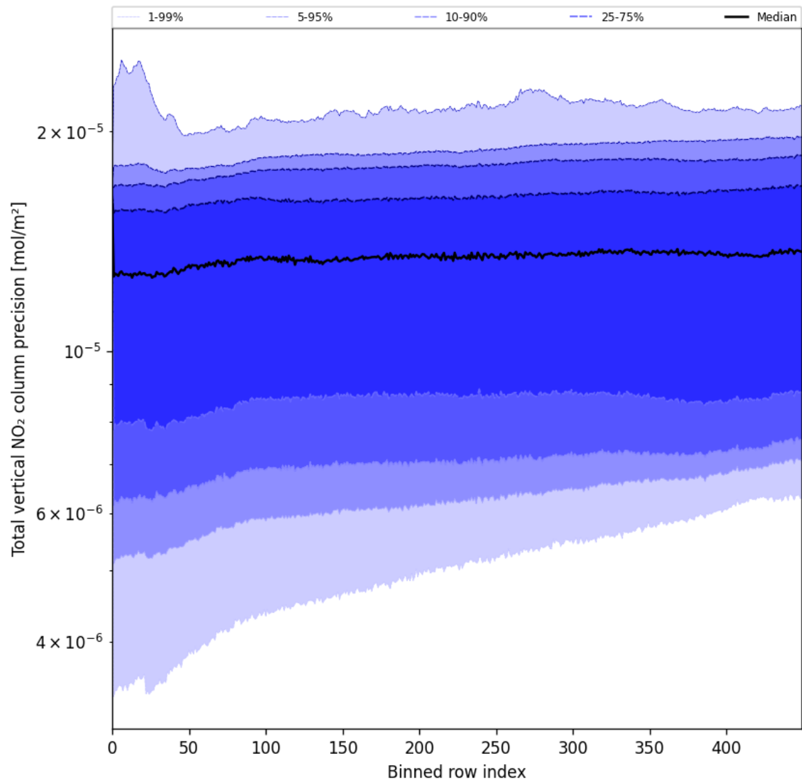
Figure 54: Along track statistics of “Total vertical NO 2 column precision” for 2025-05-31 to 2025-06-01
