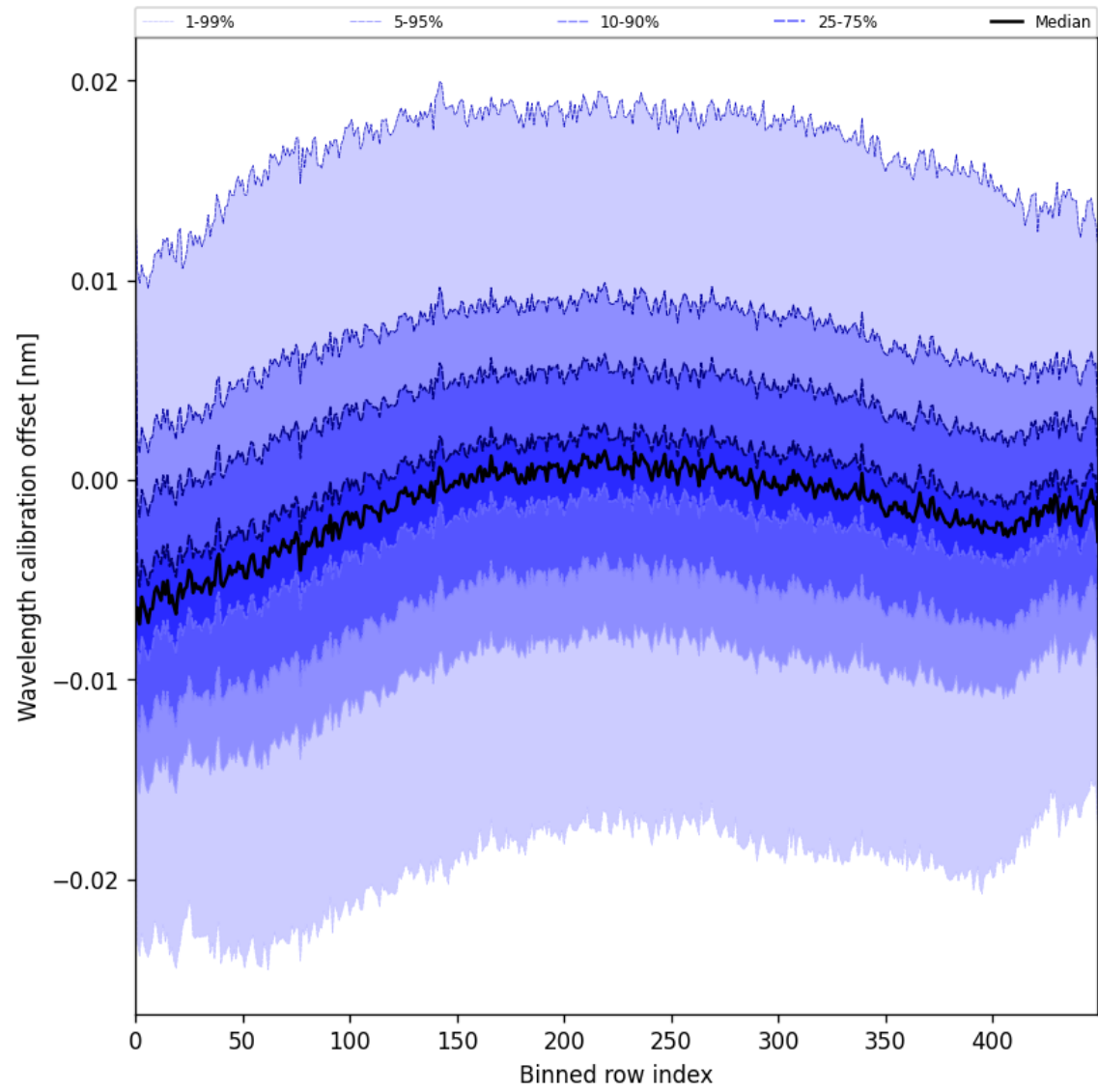
Figure 50: Along track statistics of “Wavelength calibration offset” for 2025-05-31 to 2025-06-01
