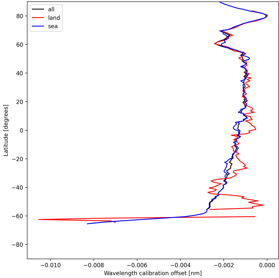
Figure 16: Zonal average of “Wavelength calibration offset” for 2025-05-31 to 2025-06-01.
