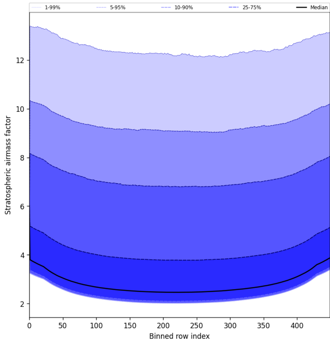
Figure 59: Along track statistics of “Stratospheric airmass factor” for 2025-05-31 to 2025-06-01
