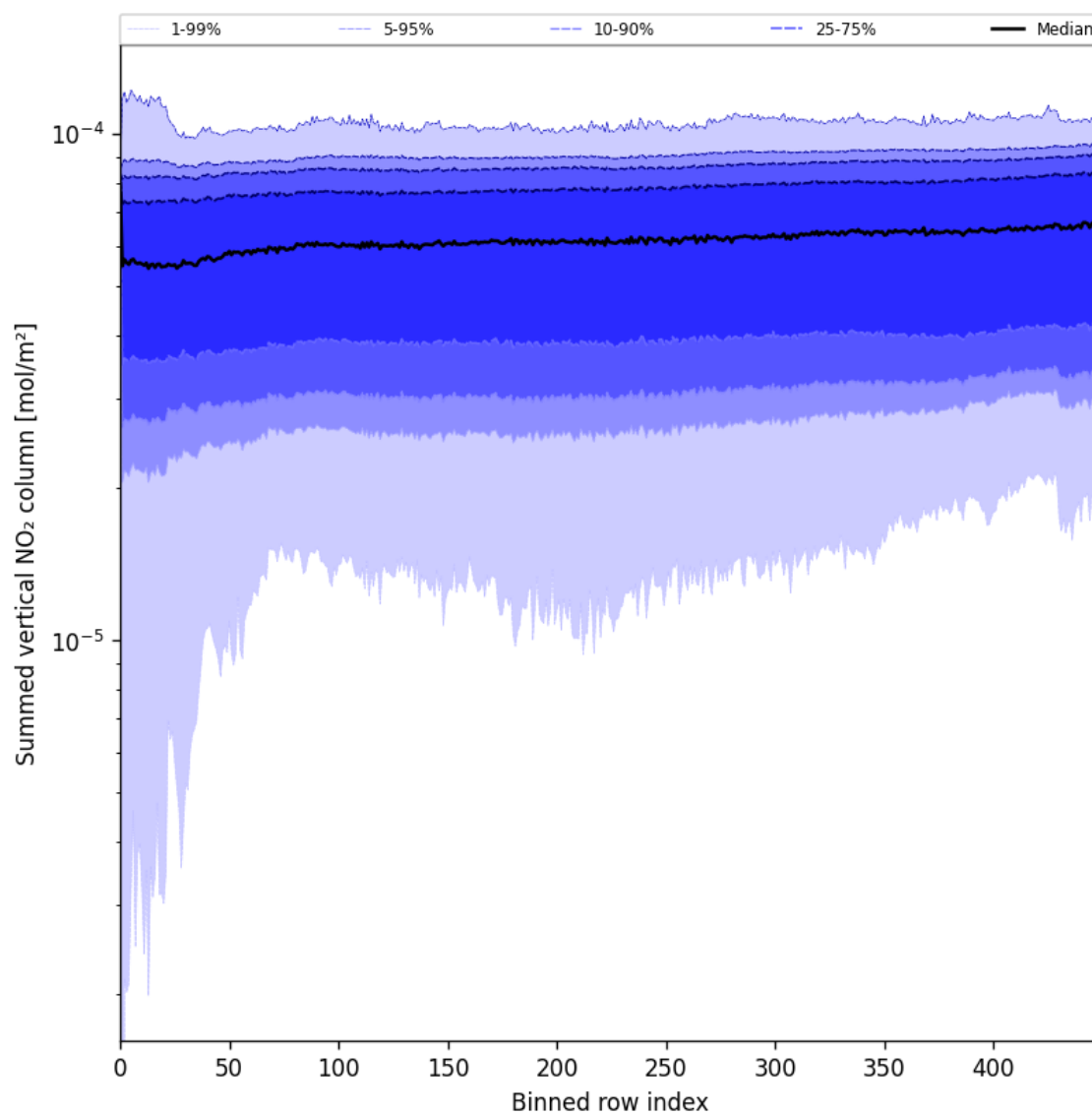
Figure 55: Along track statistics of “Summed vertical NO 2 column” for 2025-05-31 to 2025-06-01
