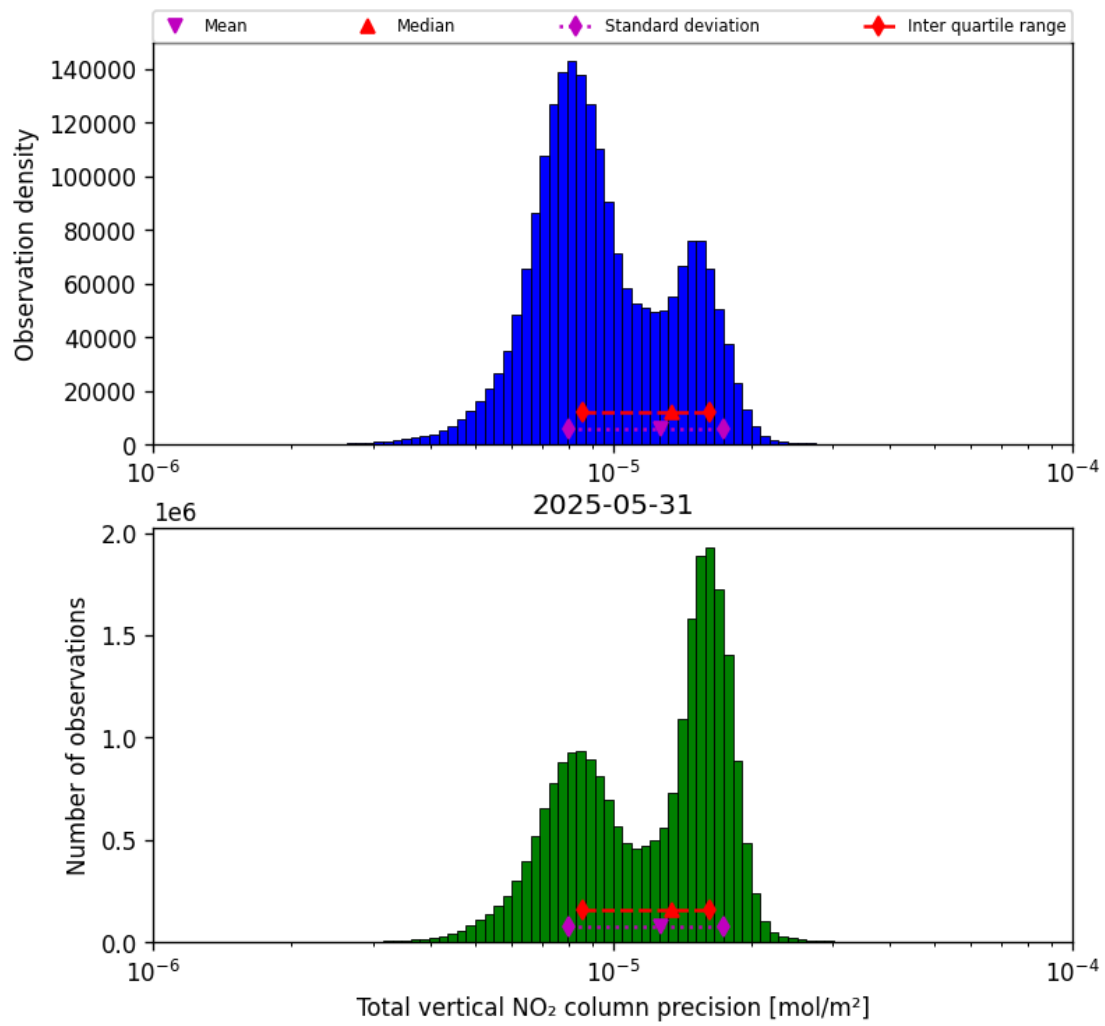
Figure 37: Histogram of “Total vertical NO 2 column precision” for 2025-05-31 to 2025-06-01
