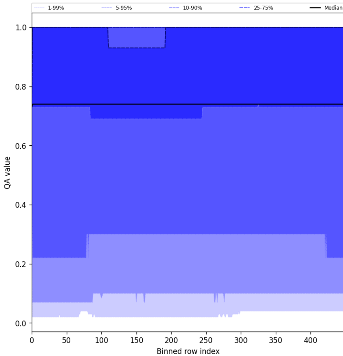
Figure 43: Along track statistics of “QA value” for 2025-05-31 to 2025-06-01
