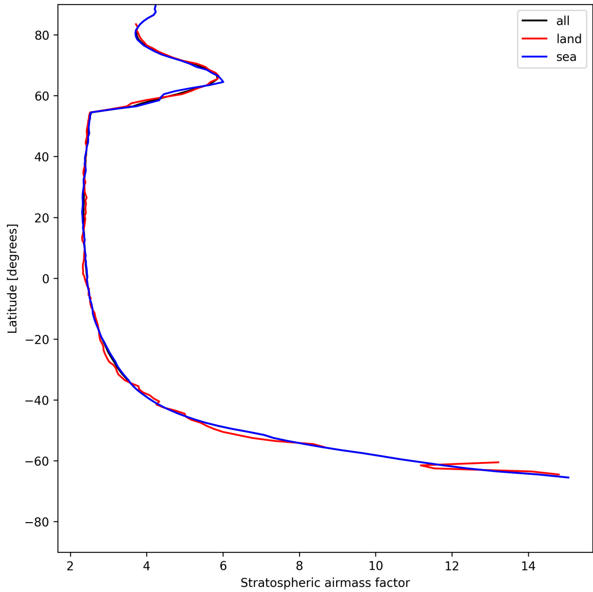
Figure 25: Zonal average of “Stratospheric air mass factor” for 2025-05-31 to 2025-06-01.
