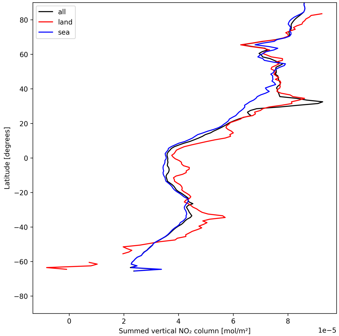
Figure 21: Zonal average of “Summed vertical NO 2 column” for 2025-05-31 to 2025-06-01.
