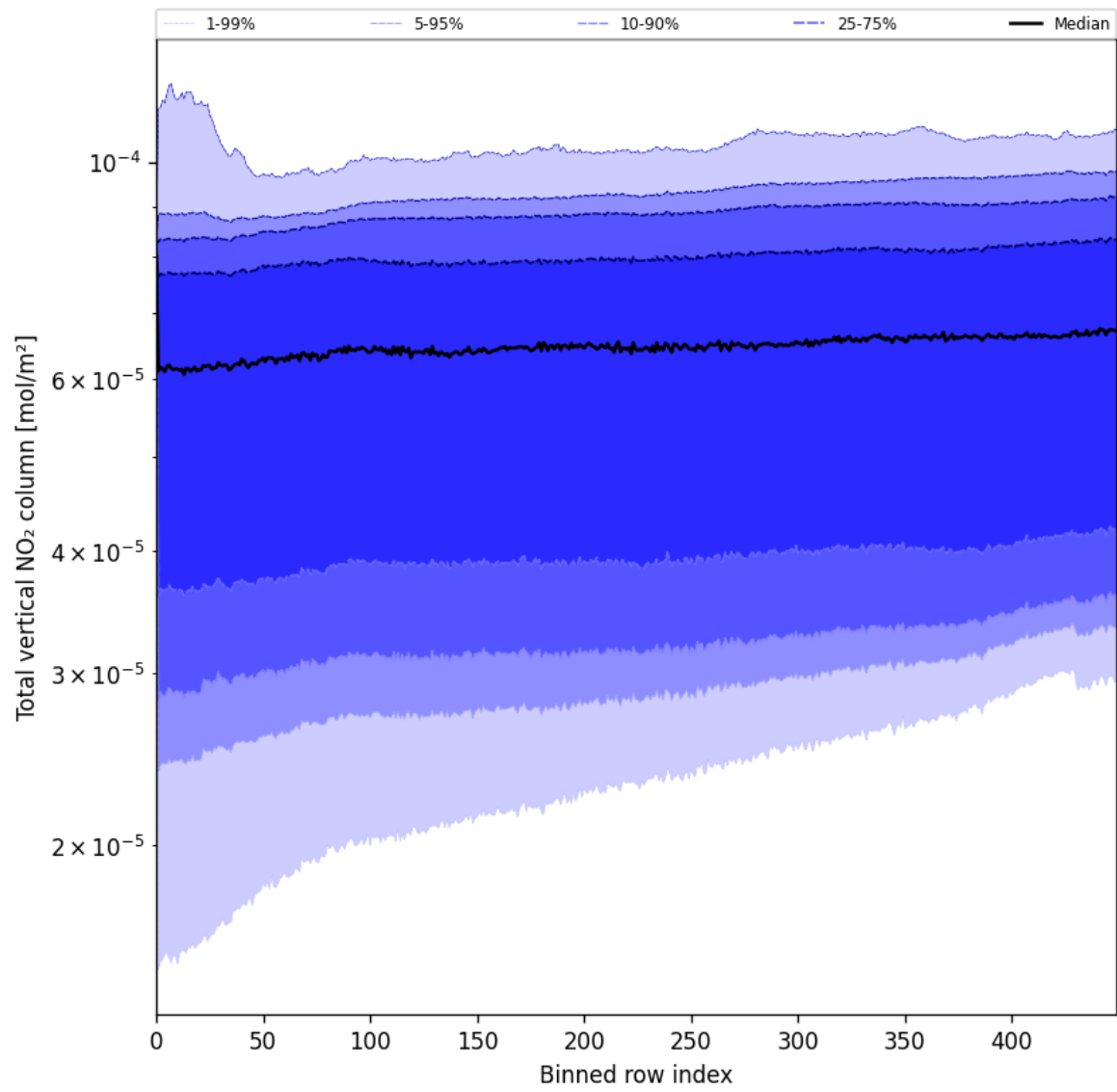
Figure 53: Along track statistics of “Total vertical NO 2 column” for 2025-05-31 to 2025-06-01
