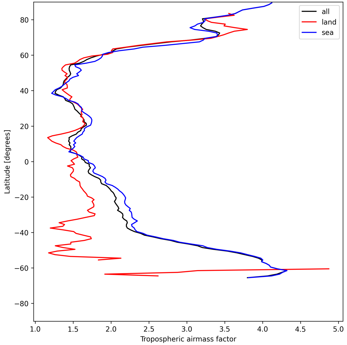
Figure 12: Zonal average of “Tropospheric airmass factor” for 2025-05-31 to 2025-06-01.
