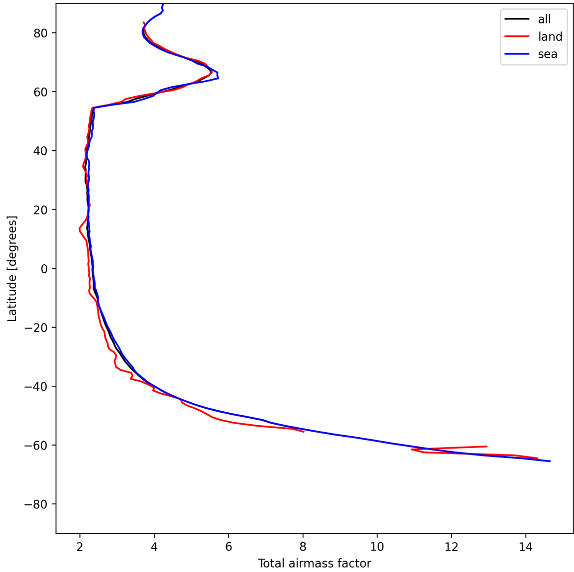
Figure 13: Zonal average of “Total airmass factor” for 2025-05-31 to 2025-06-01.
