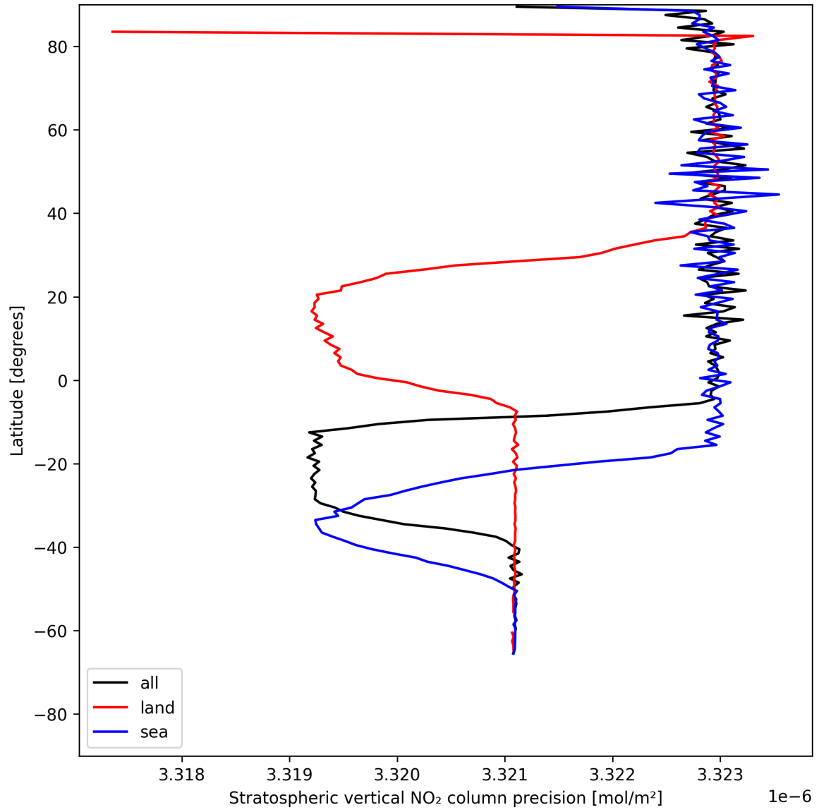
Figure 18: Zonal average of “Stratospheric vertical NO 2 column precision” for 2025-05-31 to 2025-06-01.
