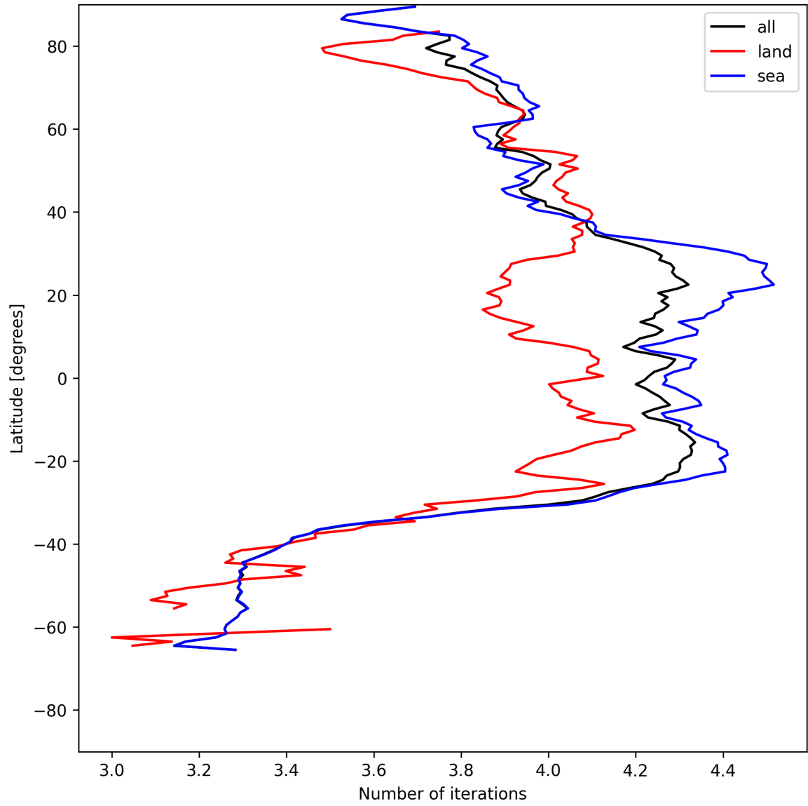
Figure 15: Zonal average of “Number of iterations” for 2025-05-31 to 2025-06-01.
