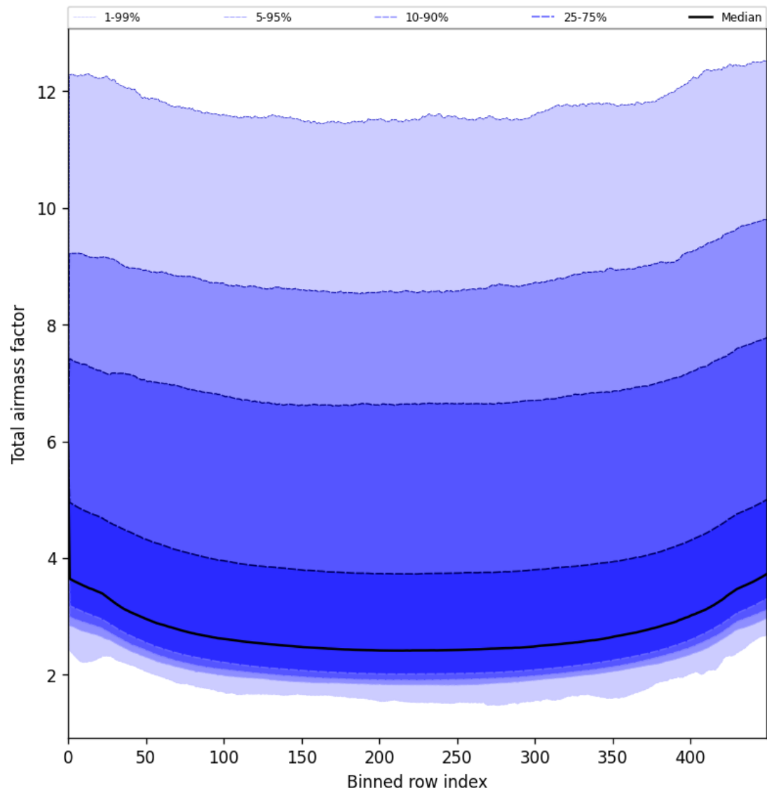
Figure 47: Along track statistics of “Total airmass factor” for 2025-05-31 to 2025-06-01
