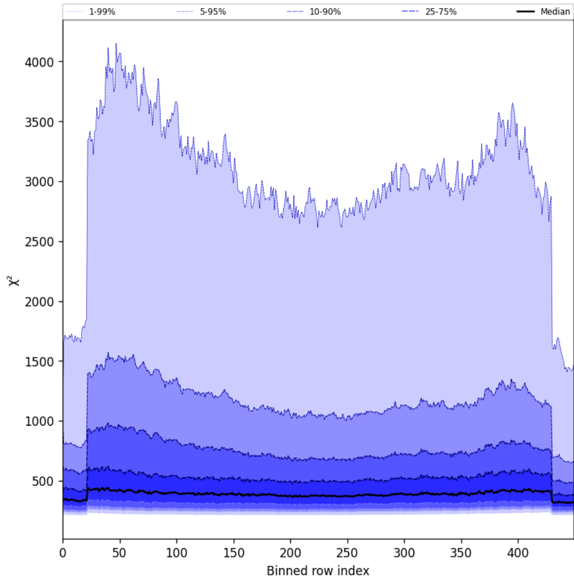
Figure 57: Along track statistics of “ \chi^2 ” for 2025-05-31 to 2025-06-01
